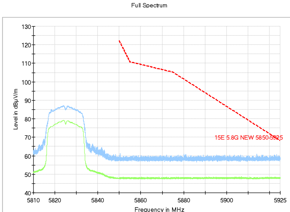
Fig. 48 Band Edges (802.11a, 5825MHz)
