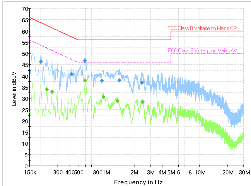
Fig. 55 AC Powerline Conducted Emission-Idle
