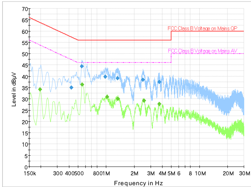
Fig. 54 AC Powerline Conducted Emission-802.11a
