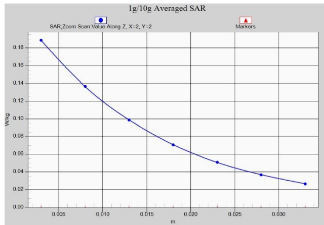
Fig.A.1- 1 Z-Scan at power reference point (GSM850 normal power)
