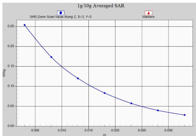
Fig.A.1- 17 Z-Scan at power reference point (LTE B12 normal power)
