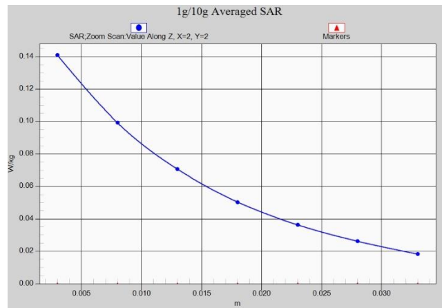
Fig.A.1- 13 Z-Scan at power reference point (LTE B5 normal power)
