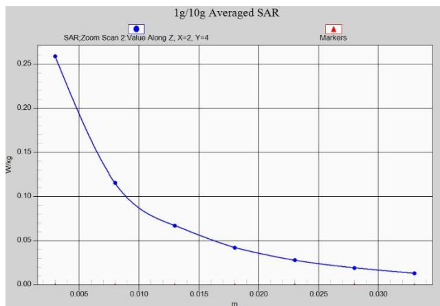
Fig.A.1- 18 Z-Scan at power reference point (LTE B12 low power)
