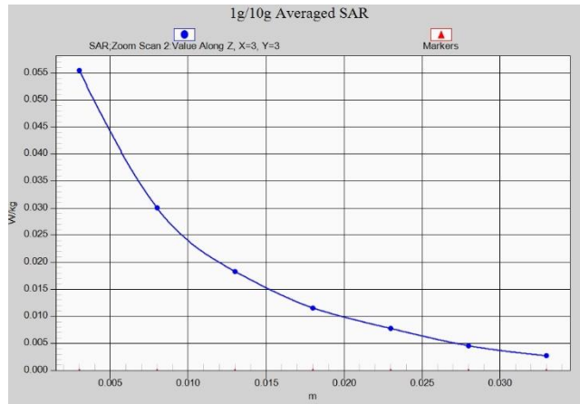
Fig.A.1- 10 Z-Scan at power reference point (W850 low power)
