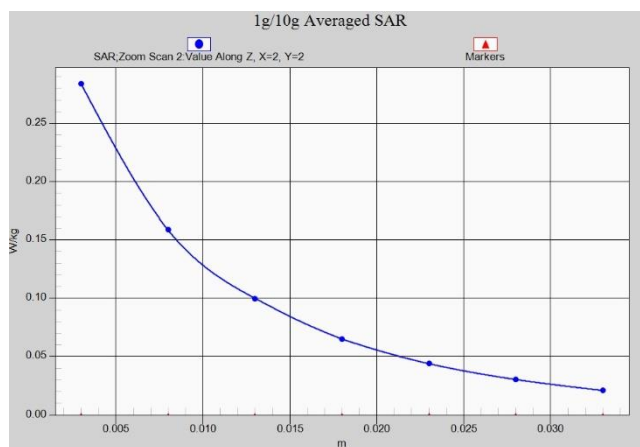
Fig.A.1- 2 Z-Scan at power reference point (GSM850 low power)
