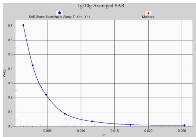
Fig.A.1- 26 Z-Scan at power reference point (Wifi 5G low power)
