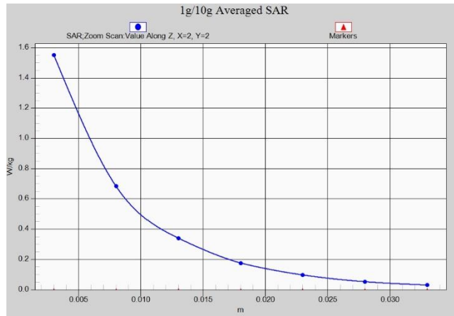
Fig.A.1- 4 Z-Scan at power reference point (PCS1900 low power)
