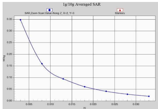
Fig.A.1- 21 Z-Scan at power reference point (LTE B71 normal power)
