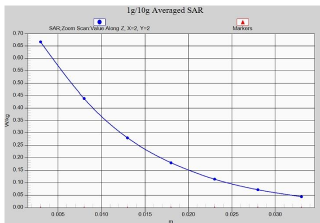
Fig.A.1- 3 Z-Scan at power reference point (PCS1900 normal power)
