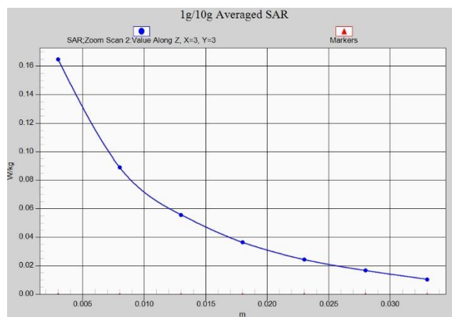
Fig.A.1- 14 Z-Scan at power reference point (LTE B5 low power)
