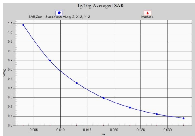
Fig.A.1- 5 Z-Scan at power reference point (W1900 normal power)
