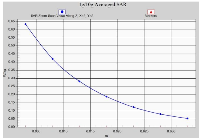
Fig.A.1- 19 Z-Scan at power reference point (LTE B66 normal power)
