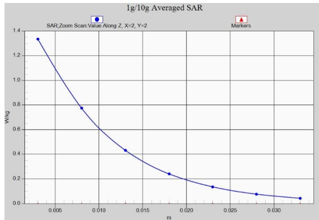
Fig.A.1- 12 Z-Scan at power reference point (LTE B2 low power)
