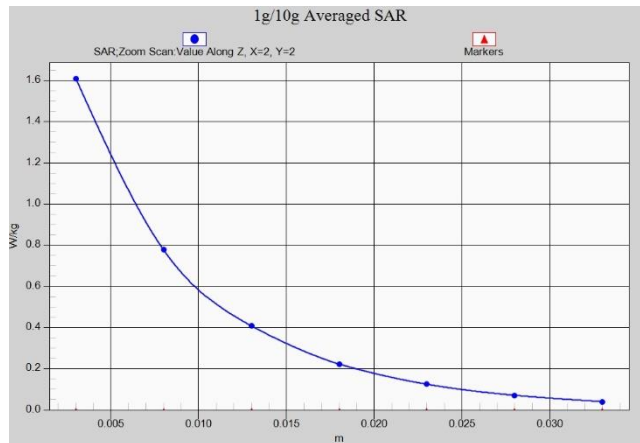
Fig.A.1- 6 Z-Scan at power reference point (W1900 low power)
