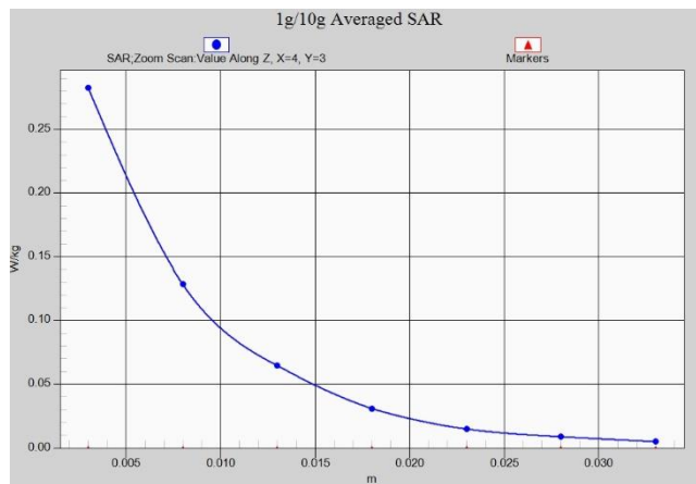
Fig.A.1- 24 Z-Scan at power reference point (Wifi 2.4G low power)
