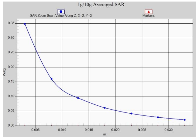
Fig.A.1- 22 Z-Scan at power reference point (LTE B71 low power)
