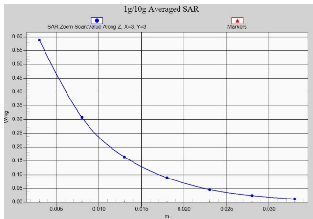
Fig.A.1- 23 Z-Scan at power reference point (Wifi 2.4G normal power)
