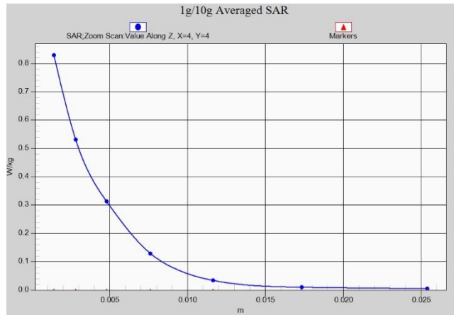
Fig.A.1- 25 Z-Scan at power reference point (Wifi 5G normal power)
