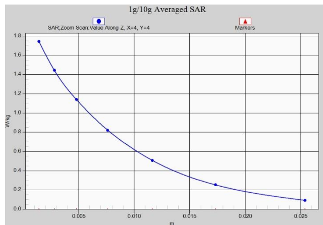
Fig.A.1- 15 Z-Scan at power reference point (LTE B7 normal power)
