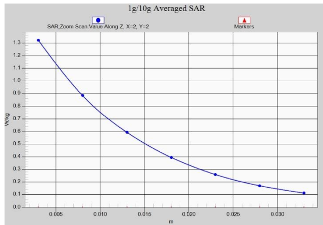
Fig.A.1- 7 Z-Scan at power reference point (W1700 normal power)
