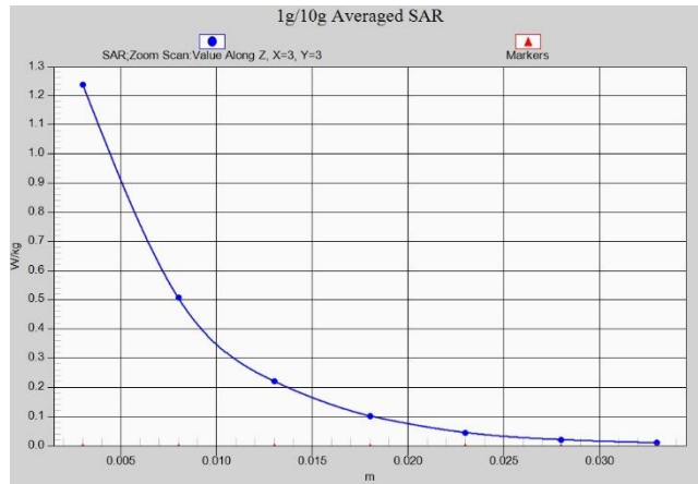
Fig.A.1- 16 Z-Scan at power reference point (LTE B7 low power)
