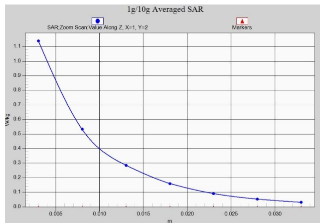
Fig.A.1- 20 Z-Scan at power reference point (LTE B66 low power)
