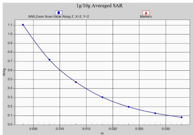
Fig.A.1- 11 Z-Scan at power reference point (LTE B2 normal power)
