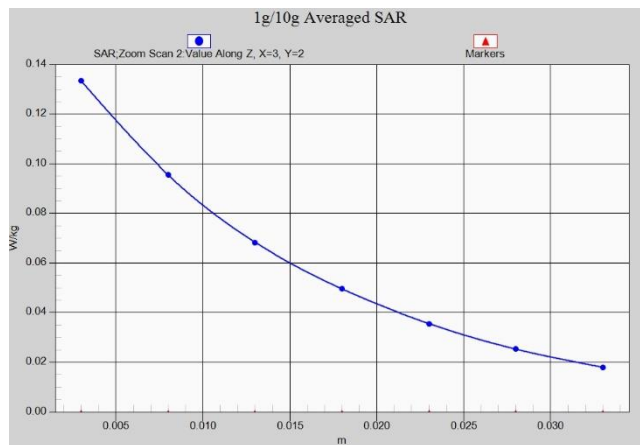
Fig.A.1- 9 Z-Scan at power reference point (W850 normal power)
