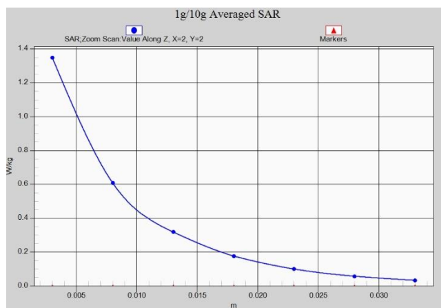
Fig.A.1- 8 Z-Scan at power reference point (W1700 low power)
