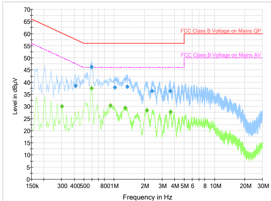
Fig. 25 Conducted Emission(802.11a, IDLE)
