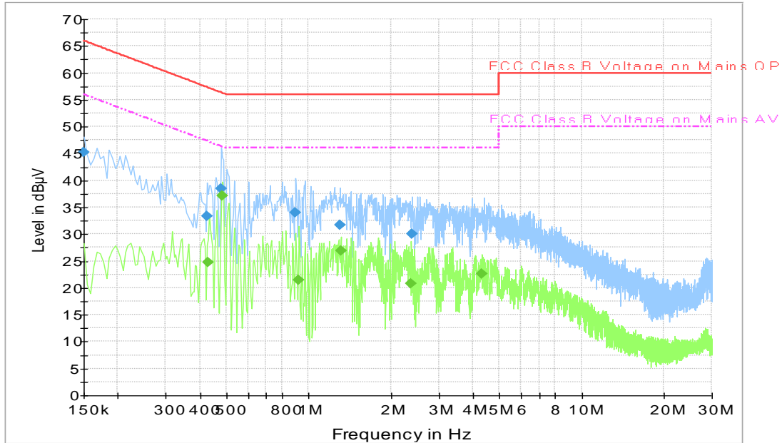
Fig.A.7.3 AC Power line Conducted Emission-802.11b
