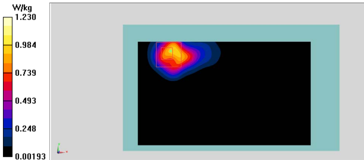
Fig.1 2450 MHz
