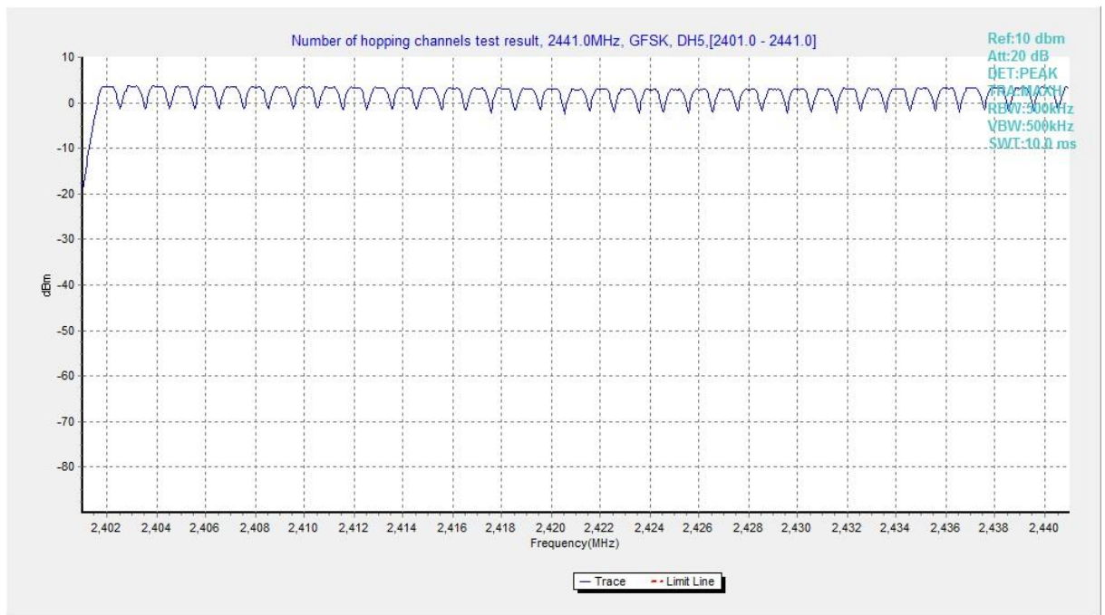
Fig.94. Number of hopping frequencies: GFSK, Channel 0 - 39
