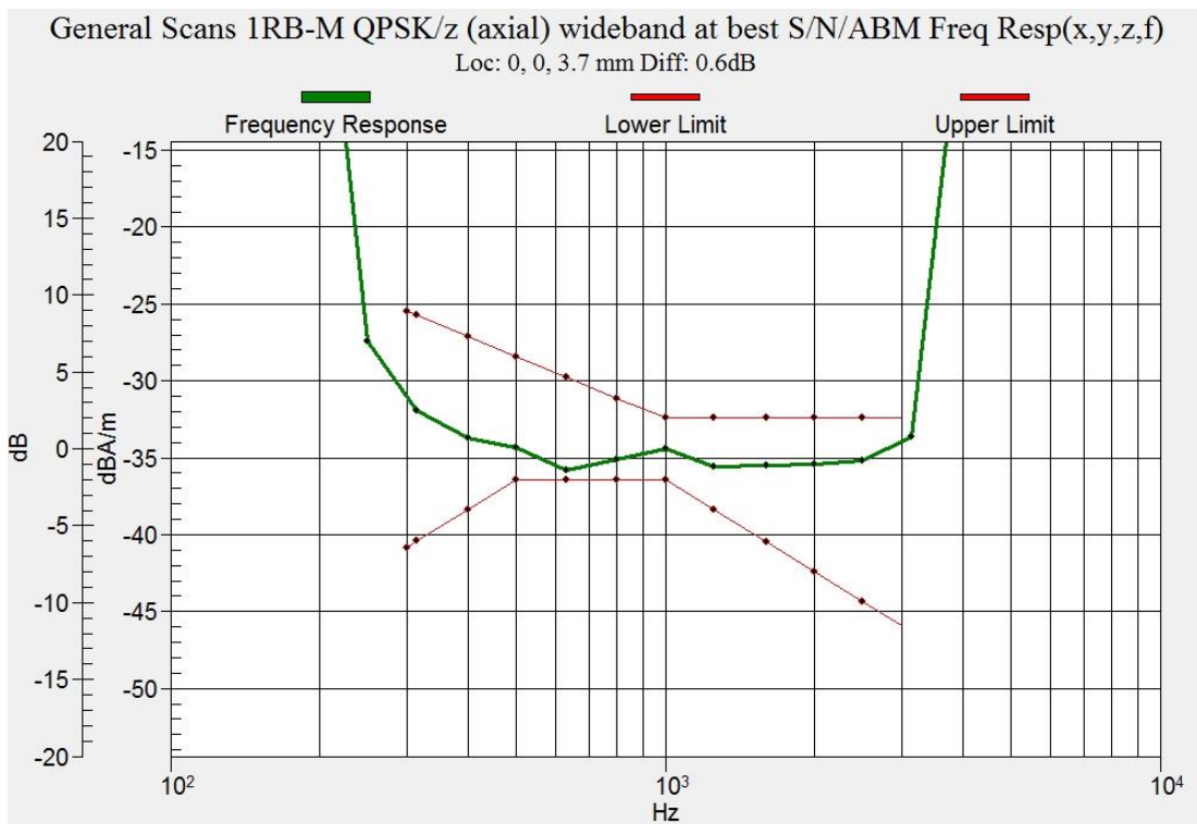
Figure C.12 Frequency Response of LTE B71
