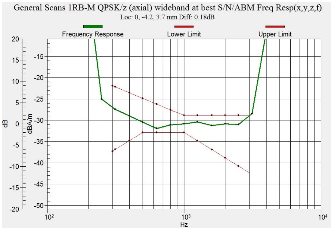
Figure C.11 Frequency Response of LTE B66
