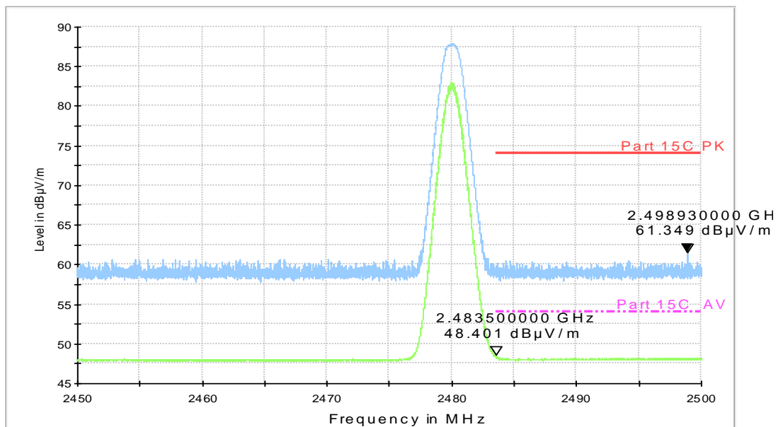
RE - Power-2.45GHz-2.5GHz
