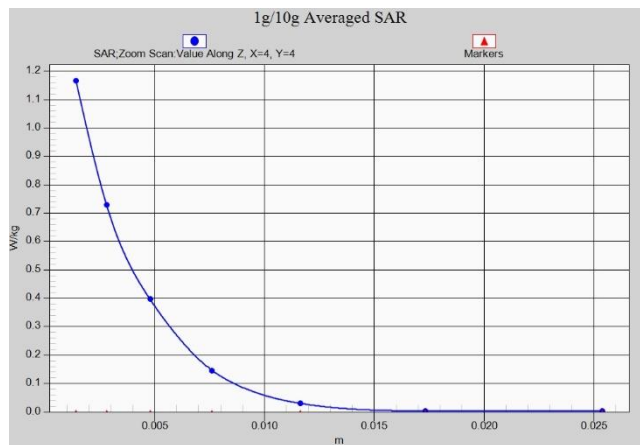
Fig.A.1- 27 Z-Scan at power reference point (Wifi5G)
