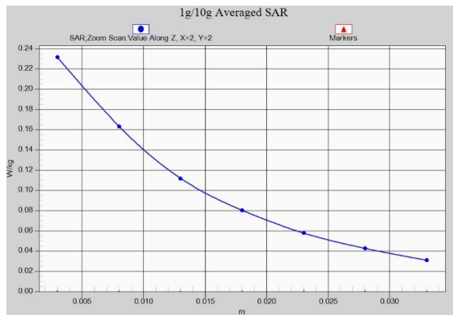
Fig.A.1- 15 Z-Scan at power reference point (LTE band4)
