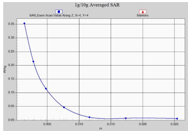
Fig.A.1- 28 Z-Scan at power reference point (Wifi5G)
