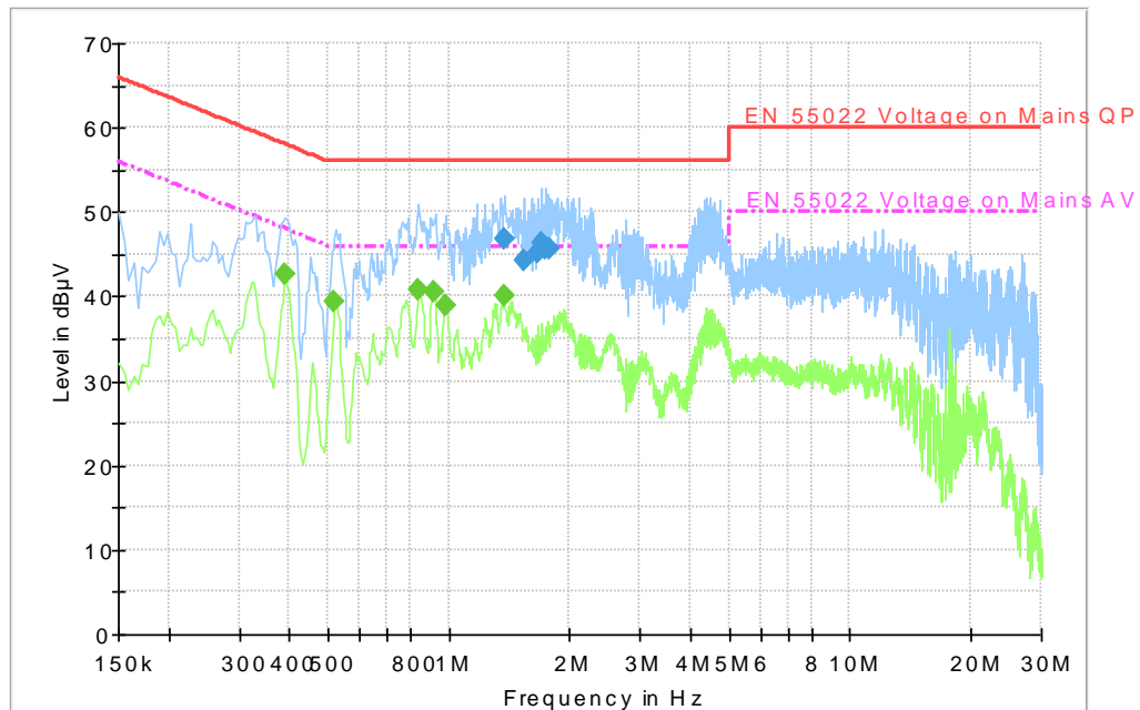
Fig A.10 Conducted Emission
