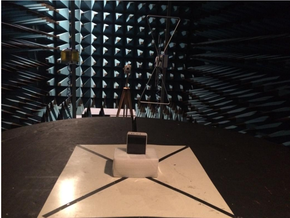
FCC Part15C Radiated Emission above 18-25GHz
