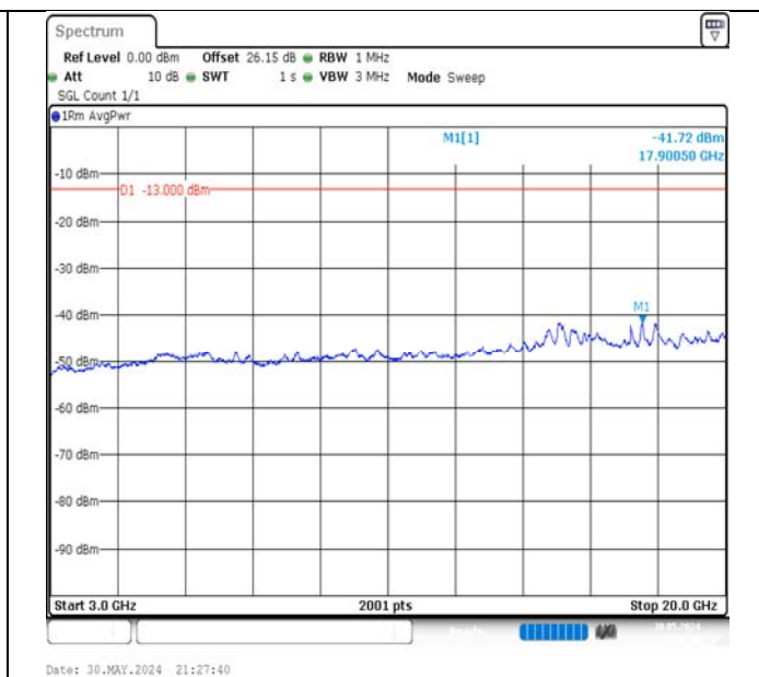
Band66-20MHz-16QAM-132072-1RB#99-3000~20000-PASS
