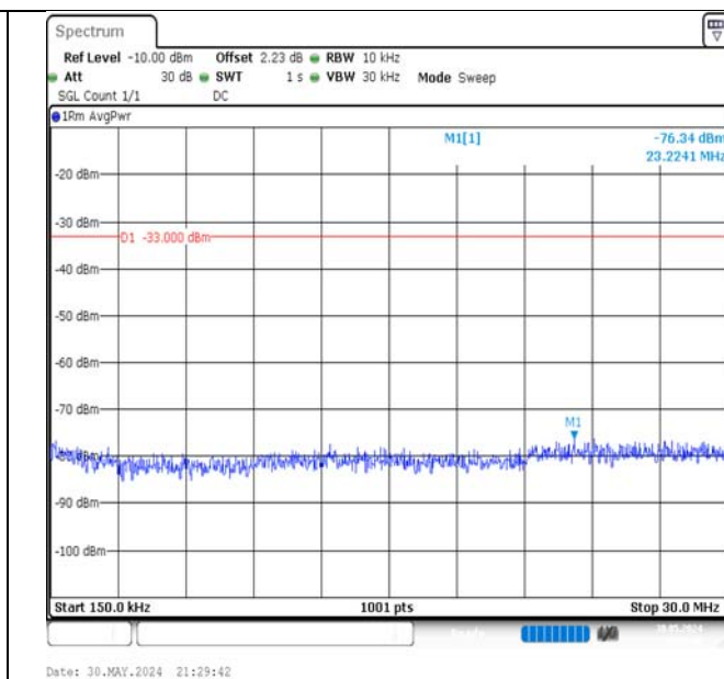
Band66-20MHz-16QAM-132322-1RB#99-0.15~30-PASS
