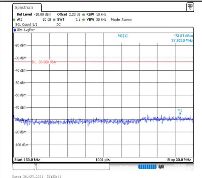
Band66-20MHz-16QAM-132572-100RB#0-0.15~30-PASS
