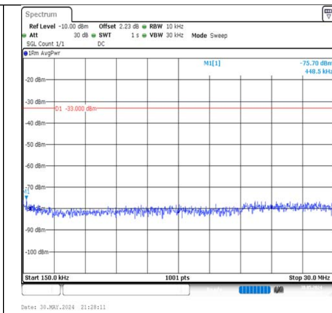
Band66-20MHz-16QAM-132072-100RB#0-0.15~30-PASS
