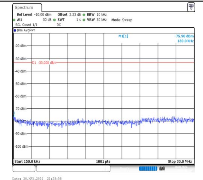
Band66-20MHz-16QAM-132322-1RB#0-0.15~30-PASS
