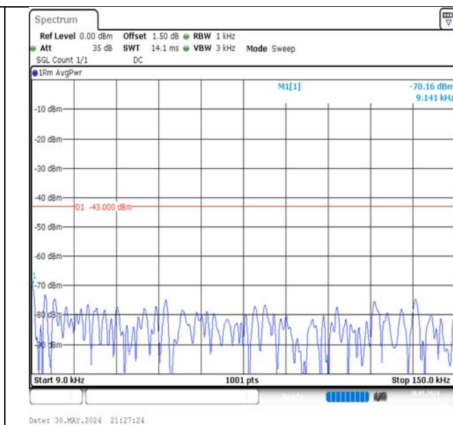
Band66-20MHz-16QAM-132072-1RB#99-0.009~0.15-PASS
