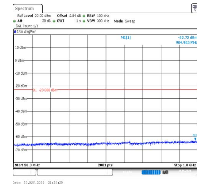
Band66-20MHz-16QAM-132322-100RB#0-30~1000-PASS
