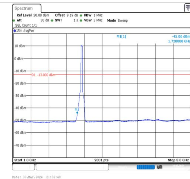
Band66-20MHz-16QAM-132572-100RB#0-1000~3000-PASS
