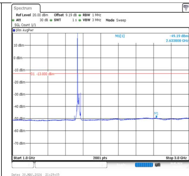
Band66-20MHz-16QAM-132322-1RB#0-1000~3000-PASS
