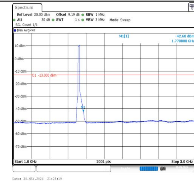
Band66-20MHz-16QAM-132072-100RB#0-1000~3000-PASS
