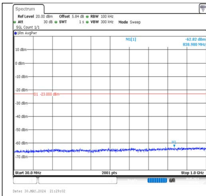
Band66-20MHz-16QAM-132322-1RB#0-30~1000-PASS
