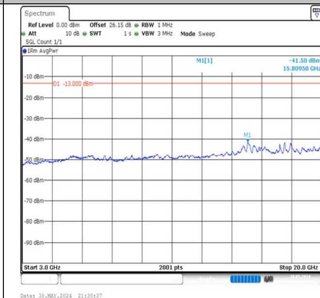
Band66-20MHz-16QAM-132322-100RB#0-3000~20000-PASS
