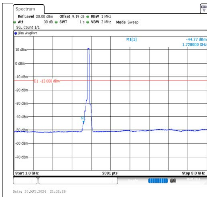
Band66-20MHz-QPSK-132572-100RB#0-1000~3000-PASS
