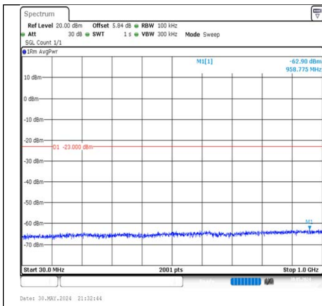
Band66-20MHz-16QAM-132572-100RB#0-30~1000-PASS
