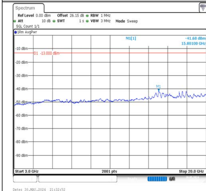
Band66-20MHz-16QAM-132572-100RB#0-3000~20000-PASS
