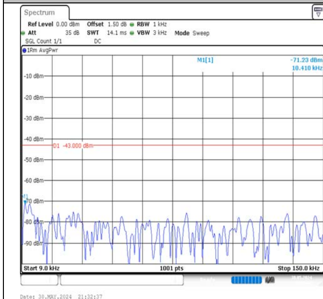
Band66-20MHz-16QAM-132572-100RB#0-0.009~0.15-PASS
