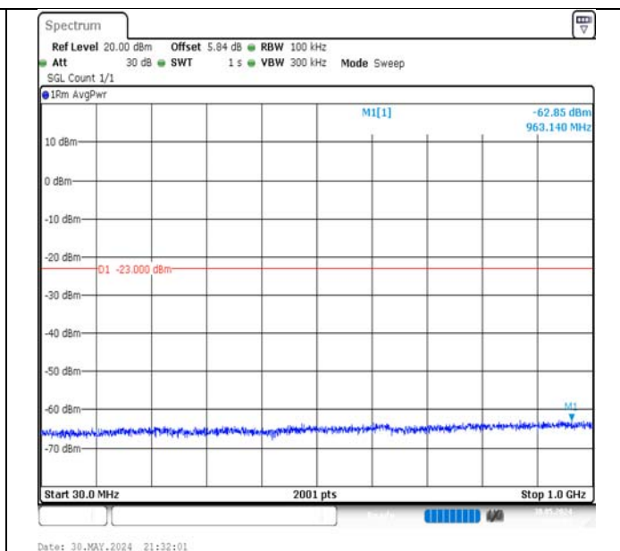
Band66-20MHz-16QAM-132572-1RB#99-30~1000-PASS
