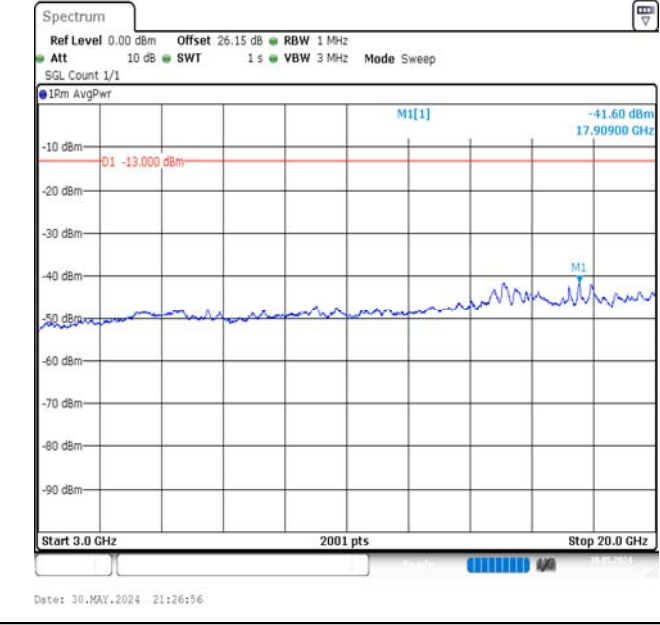
Band66-20MHz-16QAM-132072-1RB#0-3000~20000-PASS
