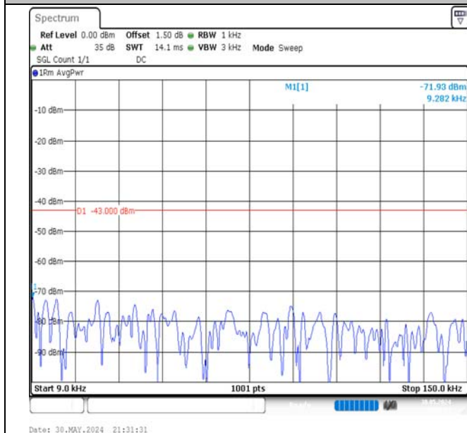
Band66-20MHz-QPSK-132572-1RB#99-0.009~0.15-PASS
