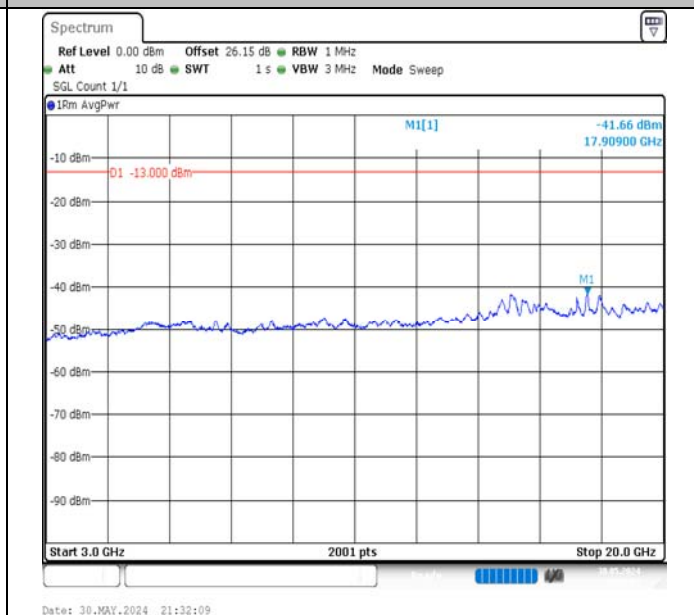
Band66-20MHz-16QAM-132572-1RB#99-3000~20000-PASS
