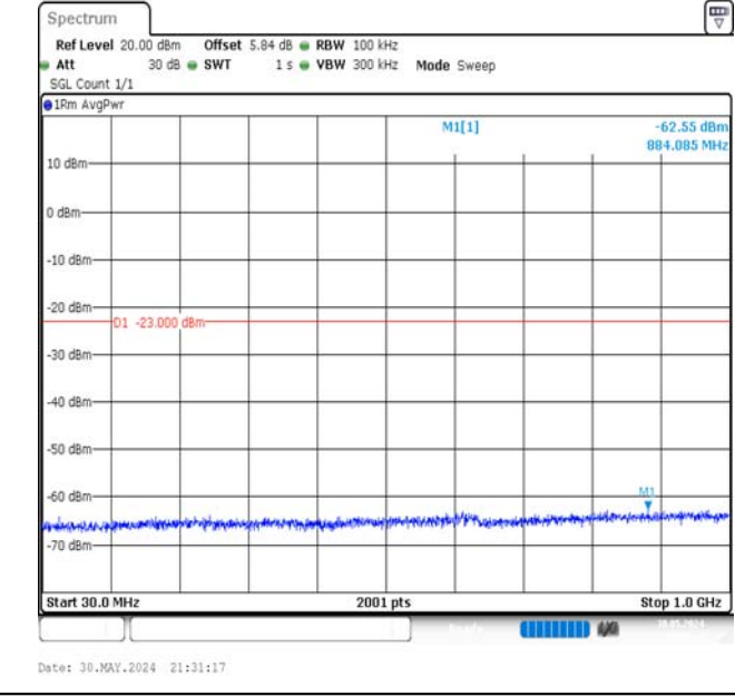
Band66-20MHz-16QAM-132572-1RB#0-30~1000-PASS
