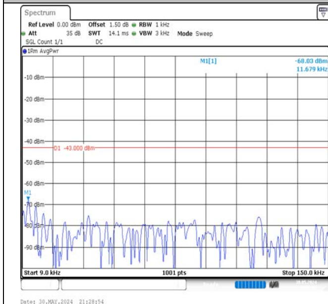
Band66-20MHz-16QAM-132322-1RB#0-0.009~0.15-PASS
