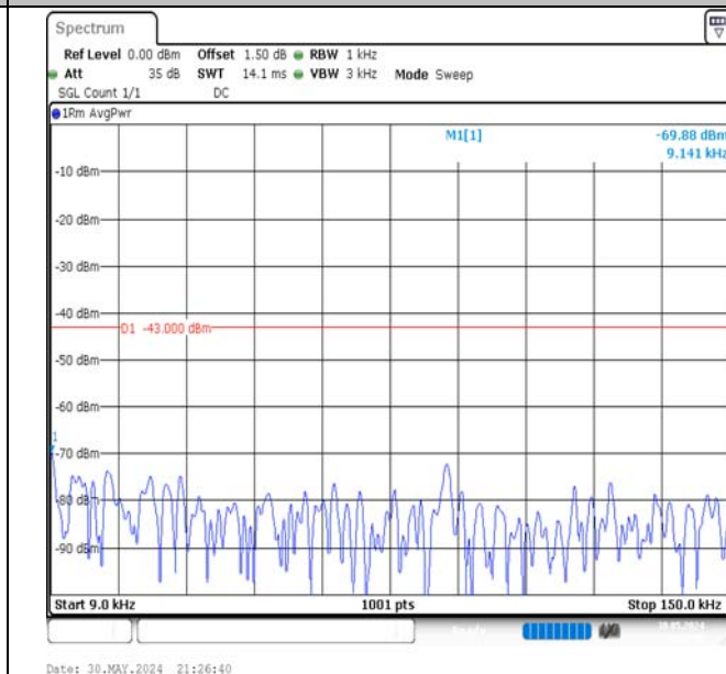
Band66-20MHz-16QAM-132072-1RB#0-0.009~0.15-PASS
