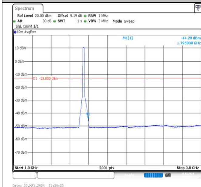
Band66-20MHz-16QAM-132322-100RB#0-1000~3000-PASS
