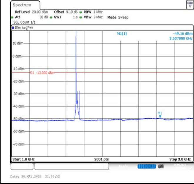
Band66-20MHz-16QAM-132072-1RB#0-1000~3000-PASS
