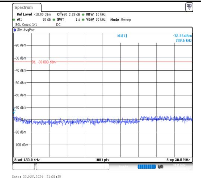
Band66-20MHz-QPSK-132572-1RB#99-0.15~30-PASS
