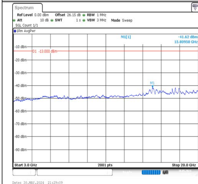
Band66-20MHz-16QAM-132322-1RB#0-3000~20000-PASS
