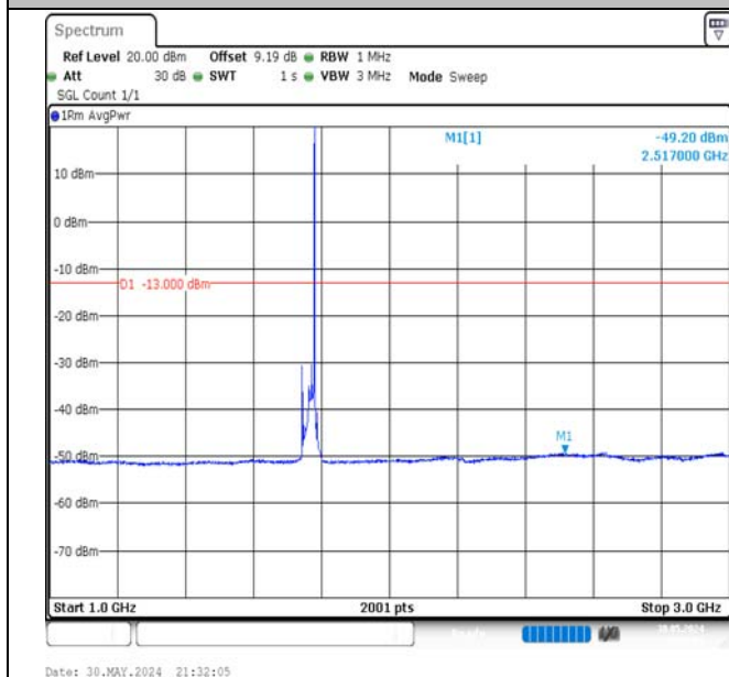
Band66-20MHz-16QAM-132572-1RB#99-1000~3000-PASS
