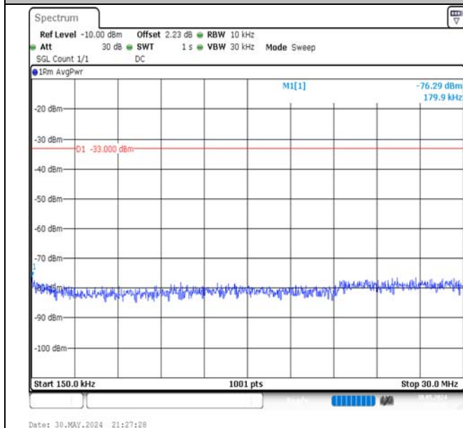
Band66-20MHz-16QAM-132072-1RB#99-0.15~30-PASS
