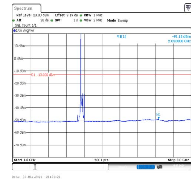
Band66-20MHz-16QAM-132572-1RB#0-1000~3000-PASS
