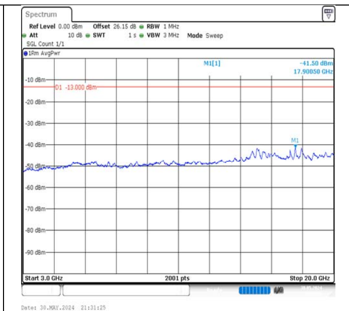
Band66-20MHz-16QAM-132572-1RB#0-3000~20000-PASS
