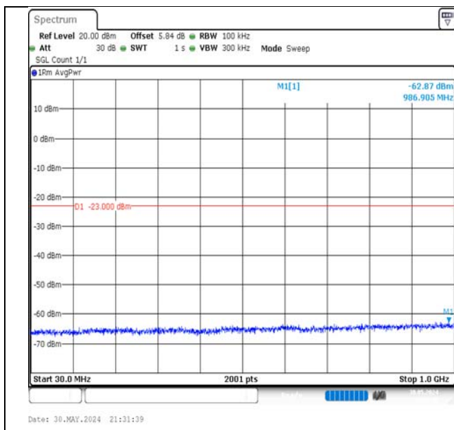
Band66-20MHz-QPSK-132572-1RB#99-30~1000-PASS
