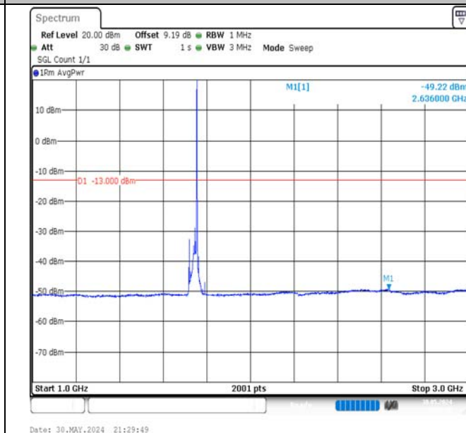
Band66-20MHz-16QAM-132322-1RB#99-1000~3000-PASS
