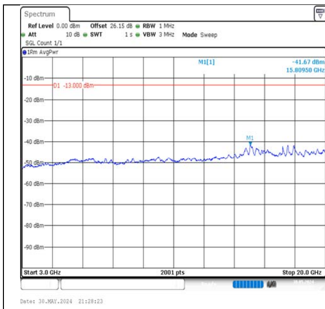
Band66-20MHz-16QAM-132072-100RB#0-3000~20000-PASS
