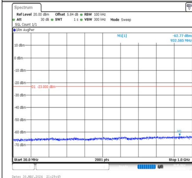
Band66-20MHz-16QAM-132322-1RB#99-30~1000-PASS
