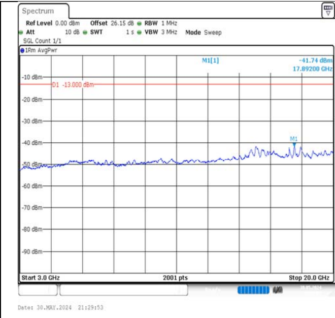
Band66-20MHz-16QAM-132322-1RB#99-3000~20000-PASS
