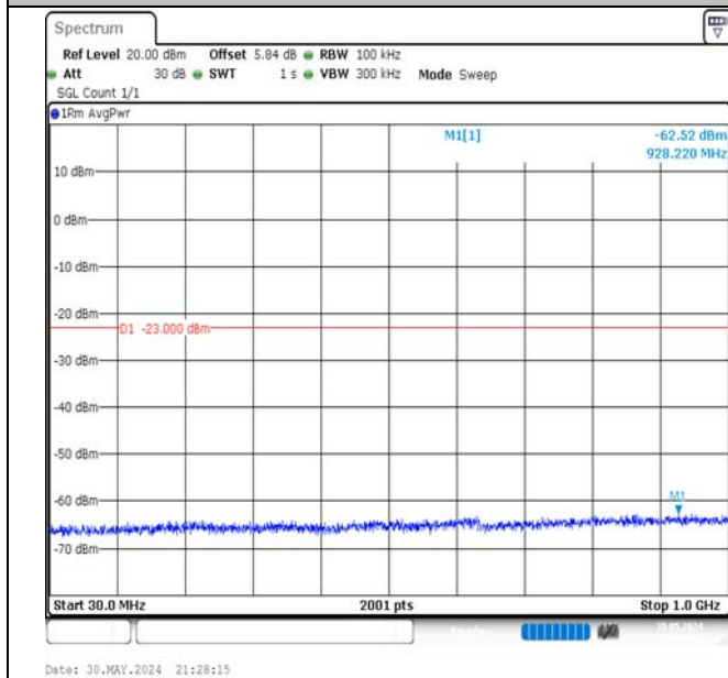
Band66-20MHz-16QAM-132072-100RB#0-30~1000-PASS
