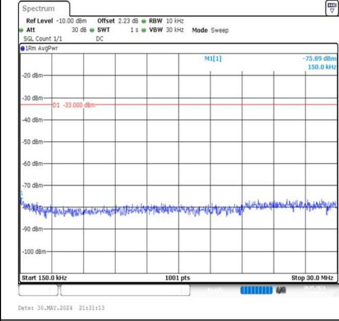
Band66-20MHz-16QAM-132572-1RB#0-0.15~30-PASS
