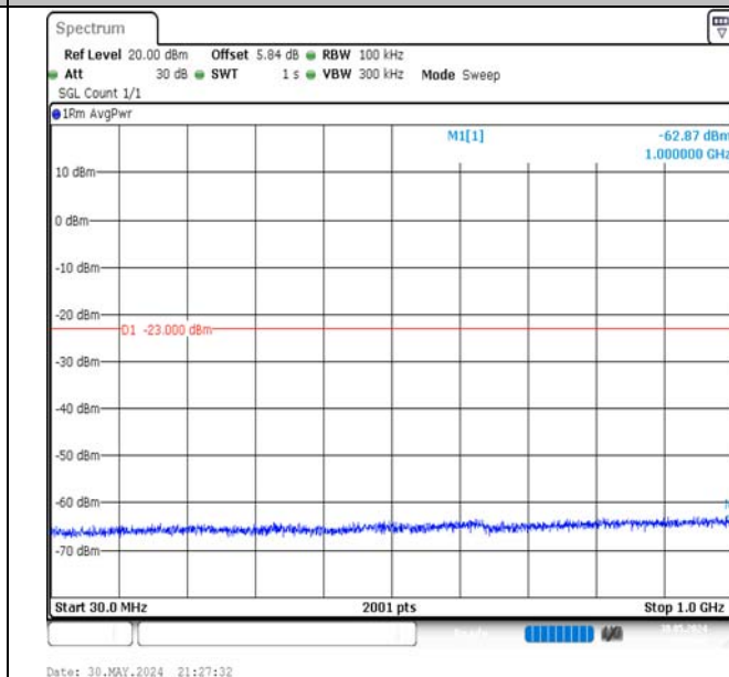
Band66-20MHz-16QAM-132072-1RB#99-30~1000-PASS
