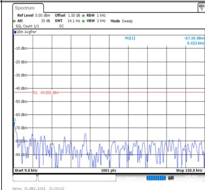
Band66-20MHz-16QAM-132322-100RB#0-0.009~0.15-PASS
