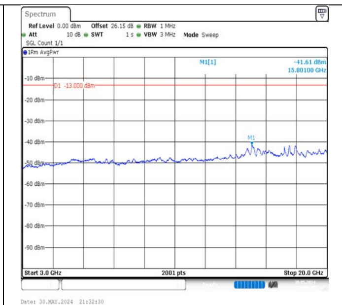
Band66-20MHz-QPSK-132572-100RB#0-3000~20000-PASS
