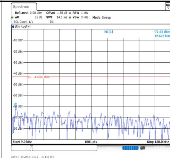
Band66-20MHz-16QAM-132572-1RB#99-0.009~0.15-PASS
