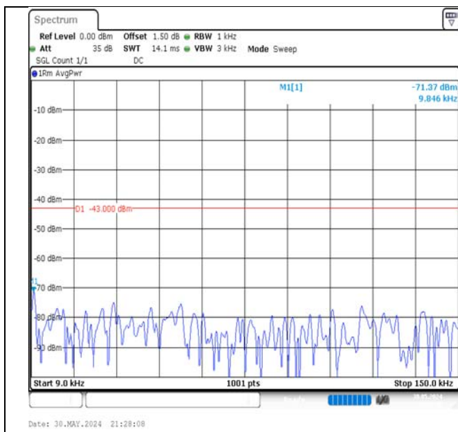
Band66-20MHz-16QAM-132072-100RB#0-0.009~0.15-PASS
