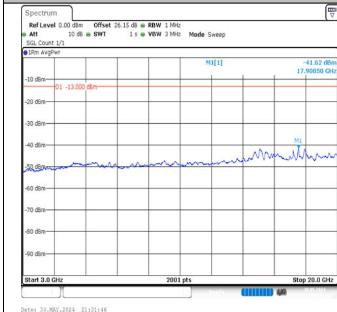
Band66-20MHz-QPSK-132572-1RB#99-3000~20000-PASS
