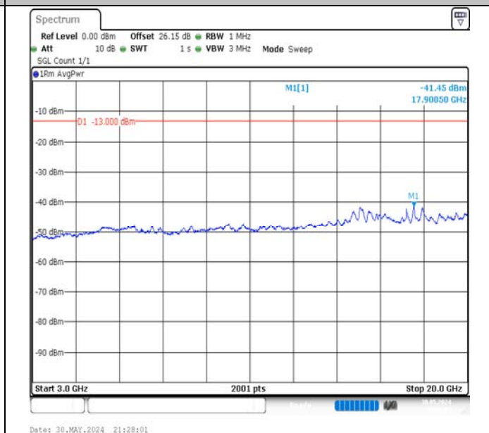
Band66-20MHz-QPSK-132072-100RB#0-3000~20000-PASS
