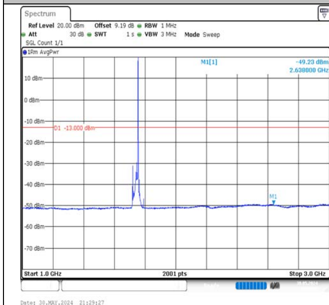
Band66-20MHz-QPSK-132322-1RB#99-1000~3000-PASS
