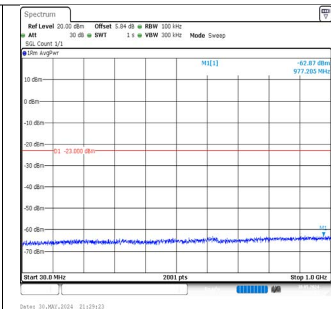
Band66-20MHz-QPSK-132322-1RB#99-30~1000-PASS
