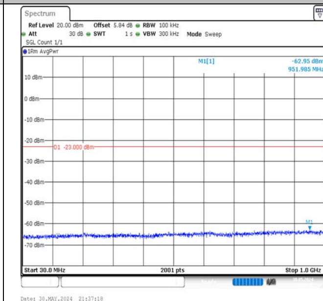
Band66-15MHz-16QAM-132322-75RB#0-30~1000-PASS
