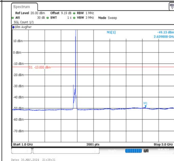
Band66-15MHz-QPSK-132597-1RB#74-1000~3000-PASS
