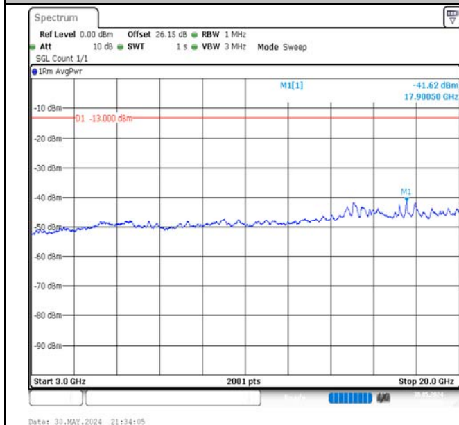
Band66-15MHz-QPSK-132047-1RB#74-3000~20000-PASS
