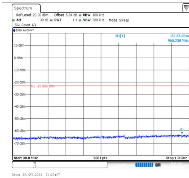
Band66-20MHz-QPSK-132322-100RB#0-30~1000-PASS
