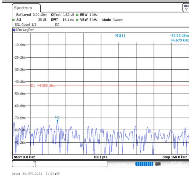
Band66-15MHz-16QAM-132047-75RB#0-0.009-0.15-PASS
