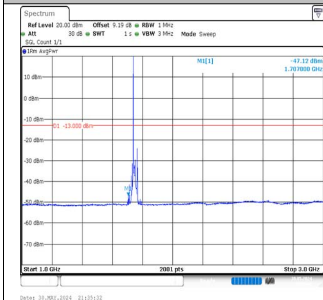
Band66-15MHz-QPSK-132322-1RB#0-1000~3000-PASS
