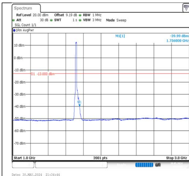
Band66-15MHz-QPSK-132047-75RB#0-1000~3000-PASS
