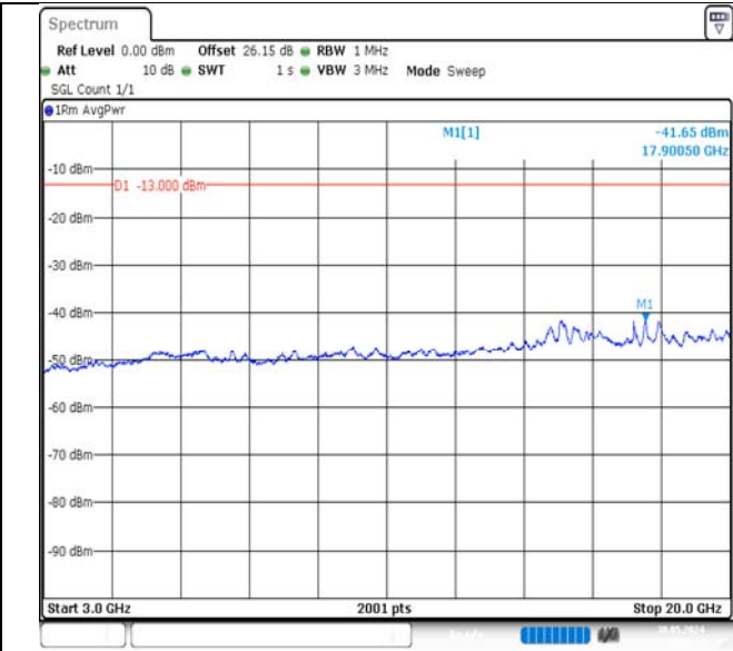
Band66-20MHz-QPSK-132072-1RB#99-3000~20000-PASS
