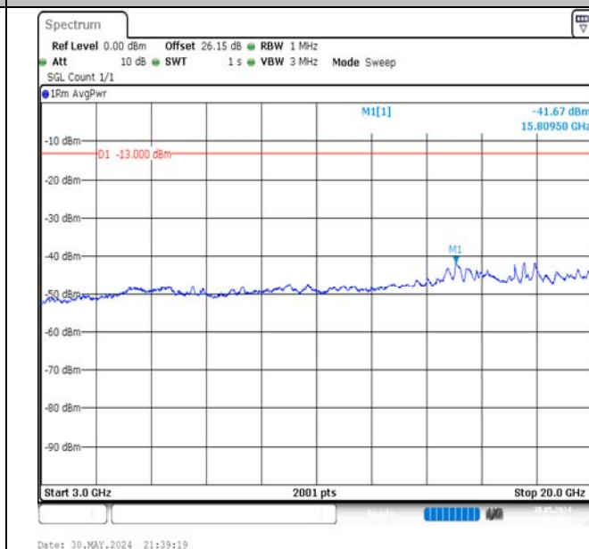
Band66-15MHz-QPSK-132597-75RB#0-3000~20000-PASS
