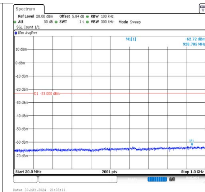
Band66-15MHz-QPSK-132597-75RB#0-30~1000-PASS
