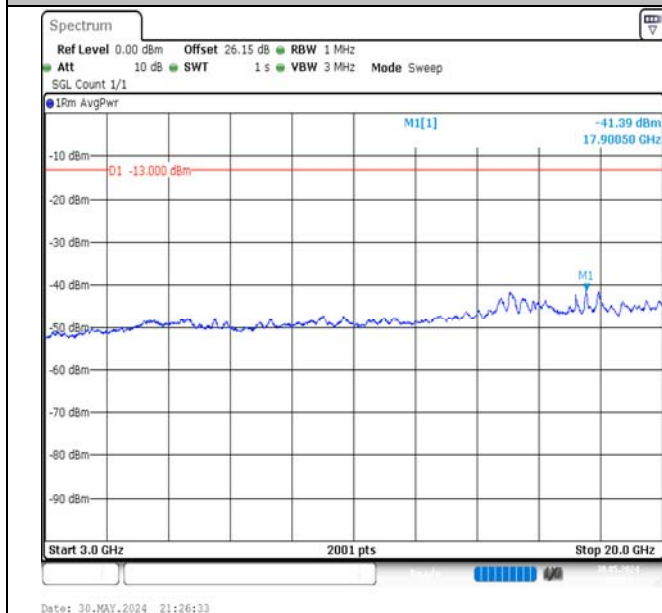
Band66-20MHz-QPSK-132072-1RB#0-3000~20000-PASS
