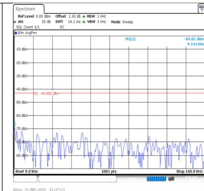
Band66-15MHz-16QAM-132322-75RB#0-0.009~0.15-PASS
