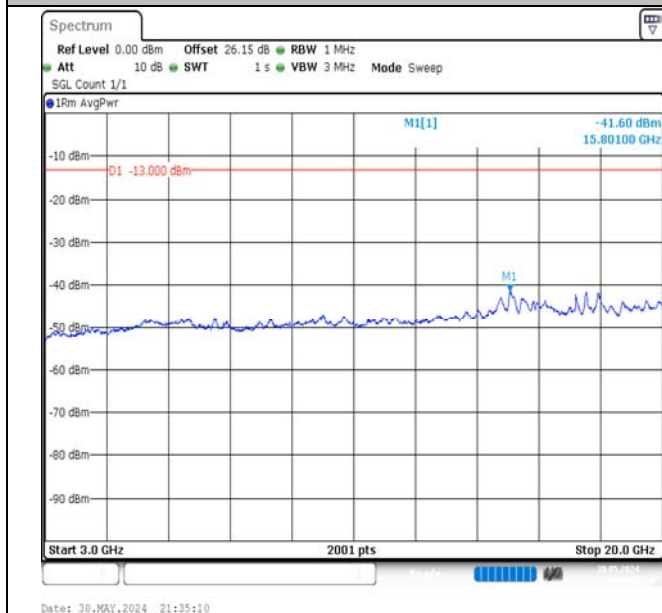
Band66-15MHz-16QAM-132047-75RB#0-3000~20000-PASS
