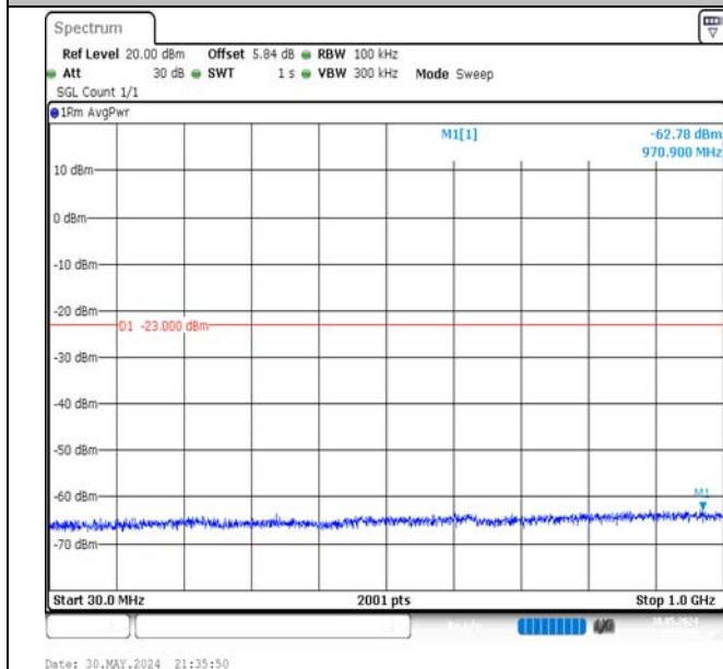
Band66-15MHz-16QAM-132322-1RB#0-30~1000-PASS
