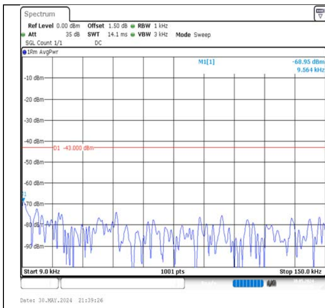
Band66-15MHz-16QAM-132597-75RB#0-0.009~0.15-PASS
