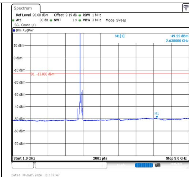
Band66-15MHz-QPSK-132597-1RB#0-1000~3000-PASS
