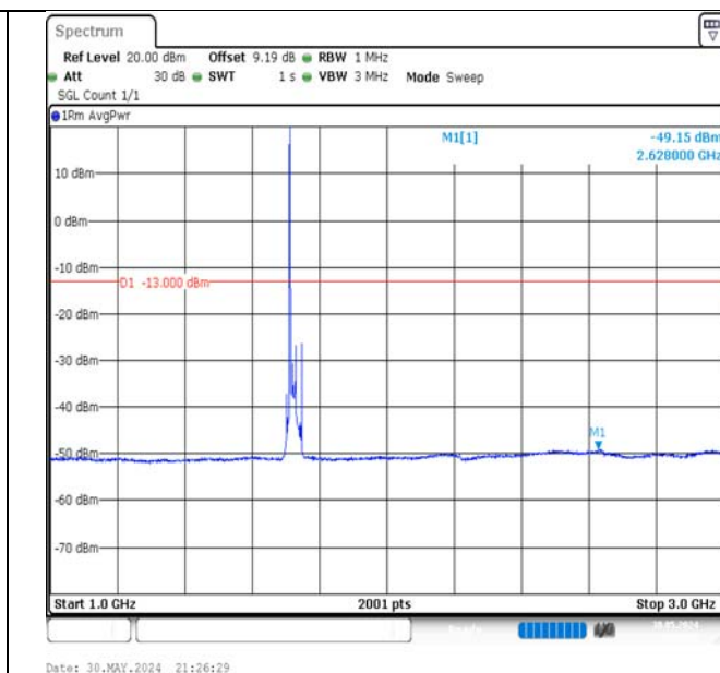
Band66-20MHz-QPSK-132072-1RB#0-1000~3000-PASS
