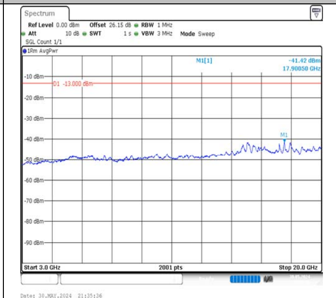
Band66-15MHz-QPSK-132322-1RB#0-3000~20000-PASS
