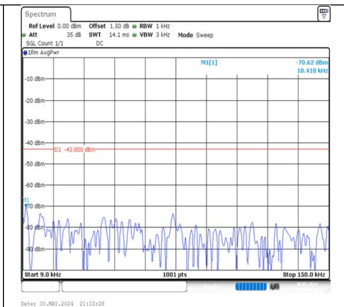
Band66-15MHz-16QAM-132047-1RB#0-0.009~0.15-PASS
