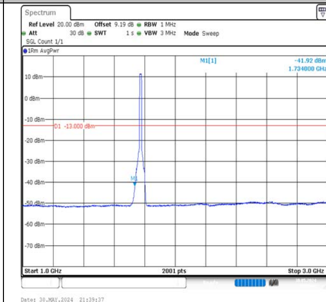
Band66-15MHz-16QAM-132597-75RB#0-1000~3000-PASS
