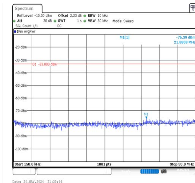
Band66-15MHz-16QAM-132322-1RB#0-0.15~30-PASS
