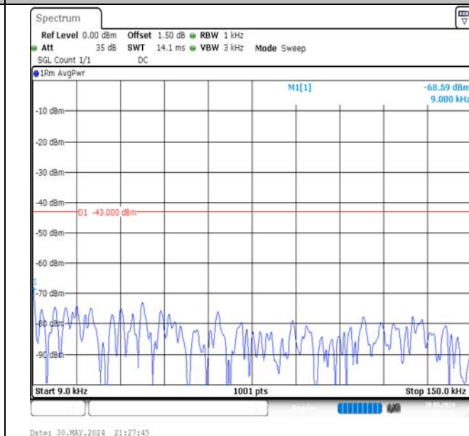
Band66-20MHz-QPSK-132072-100RB#0-0.009~0.15-PASS
