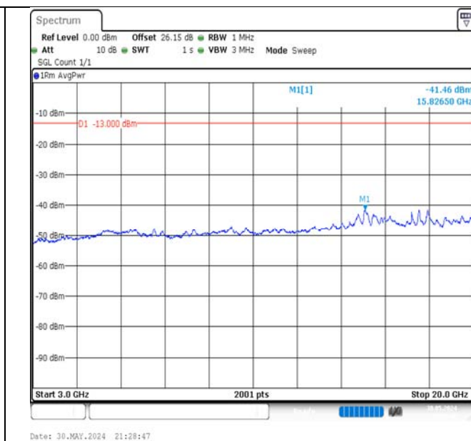
Band66-20MHz-QPSK-132322-1RB#0-3000~20000-PASS
