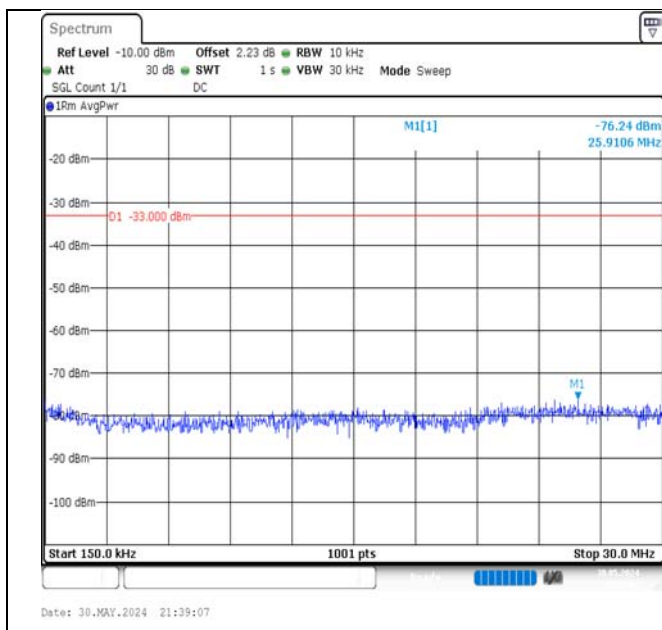
Band66-15MHz-QPSK-132597-75RB#0-0.15~30-PASS
