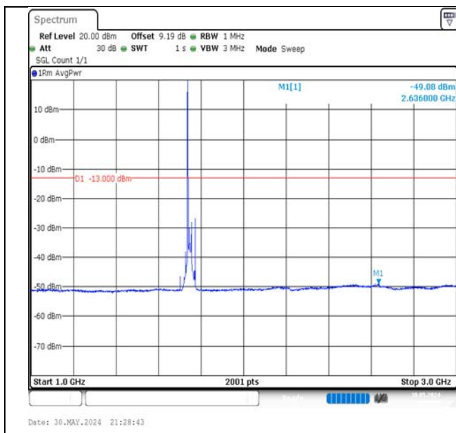
Band66-20MHz-QPSK-132322-1RB#0-1000~3000-PASS
