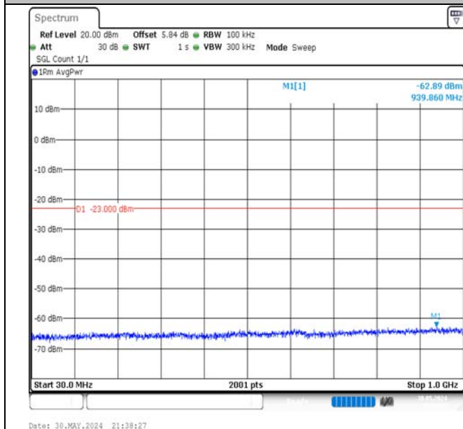
Band66-15MHz-QPSK-132597-1RB#74-30~1000-PASS
