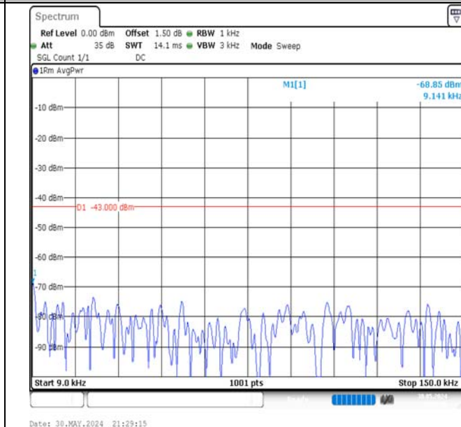
Band66-20MHz-QPSK-132322-1RB#99-0.009~0.15-PASS
