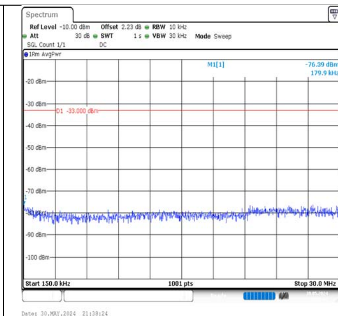
Band66-15MHz-QPSK-132597-1RB#74-0.15~30-PASS
