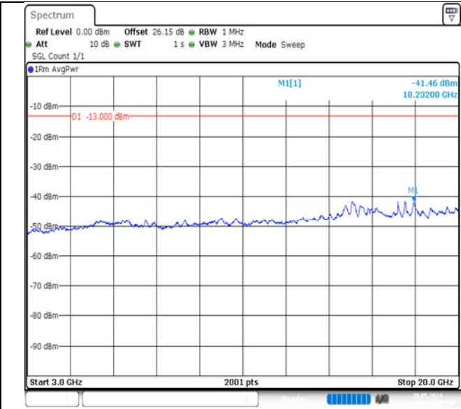
Band66-20MHz-QPSK-132572-1RB#0-3000~20000-PASS
