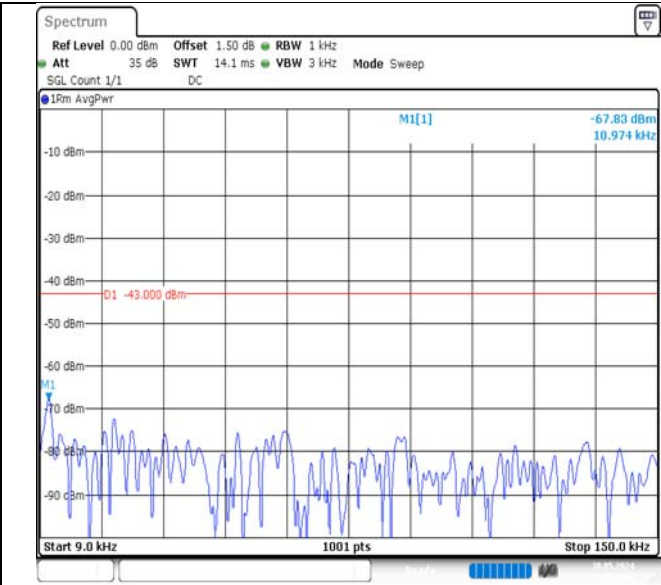
Band66-20MHz-QPSK-132322-1RB#0-0.009~0.15-PASS
