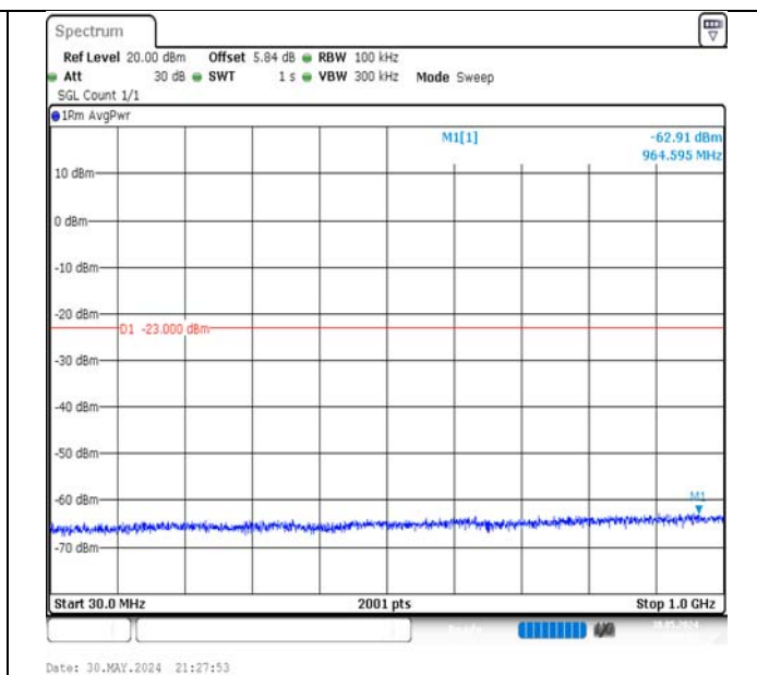
Band66-20MHz-QPSK-132072-100RB#0-30~1000-PASS
