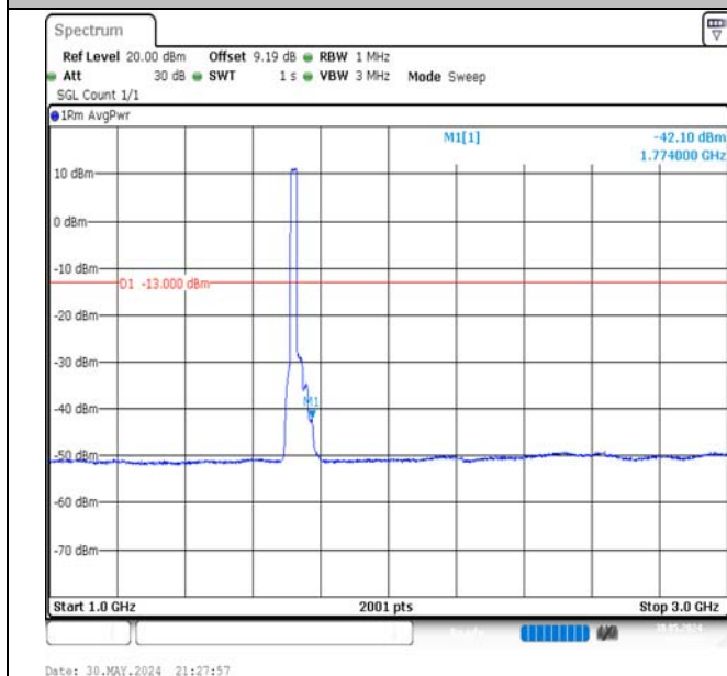
Band66-20MHz-QPSK-132072-100RB#0-1000~3000-PASS
