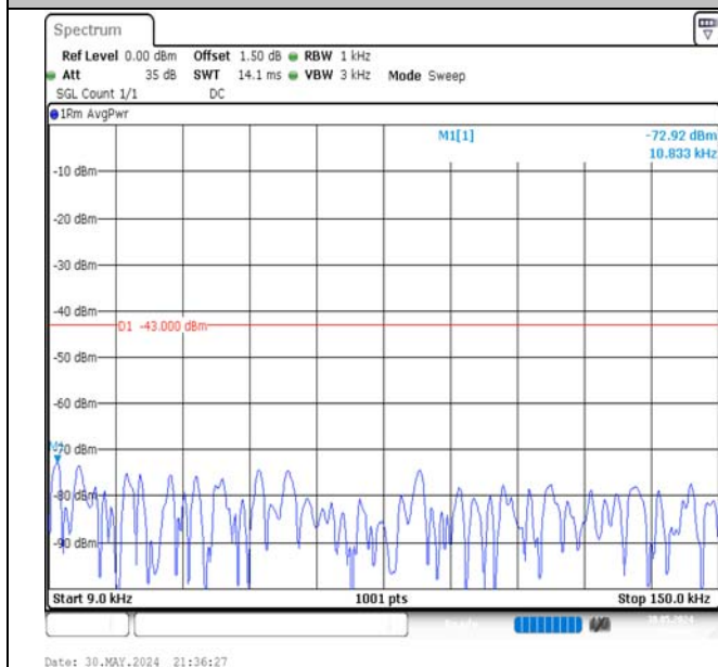
Band66-15MHz-16QAM-132322-1RB#74-0.009~0.15-PASS
