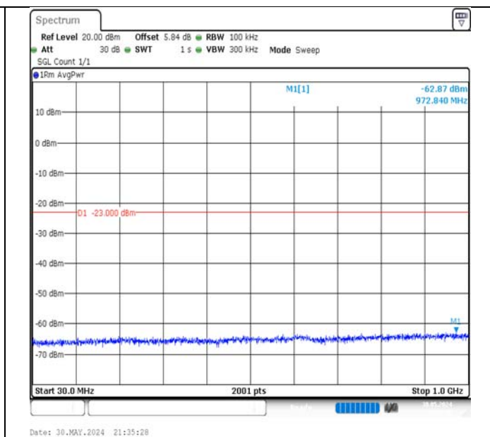
Band66-15MHz-QPSK-132322-1RB#0-30~1000-PASS
