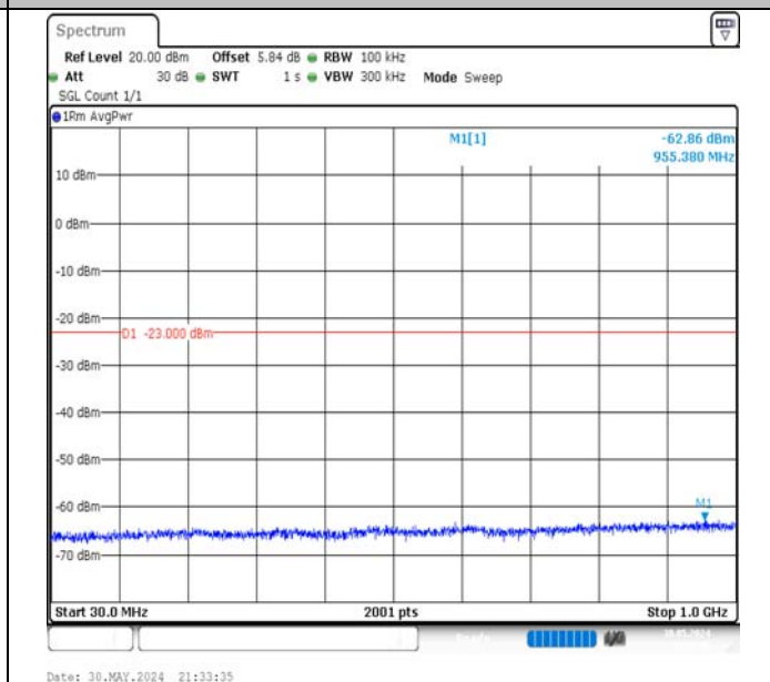
Band66-15MHz-16QAM-132047-1RB#0-30~1000-PASS
