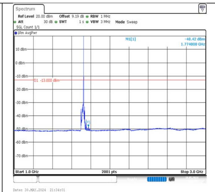
Band66-15MHz-QPSK-132047-1RB#74-1000~3000-PASS
