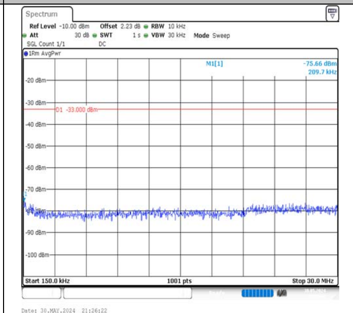
Band66-20MHz-QPSK-132072-1RB#0-0.15~30-PASS
