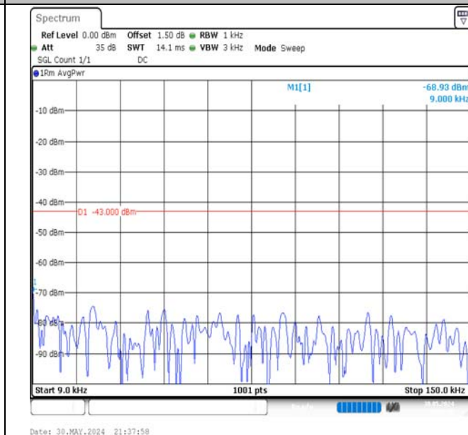
Band66-15MHz-16QAM-132597-1RB#0-0.009~0.15-PASS
