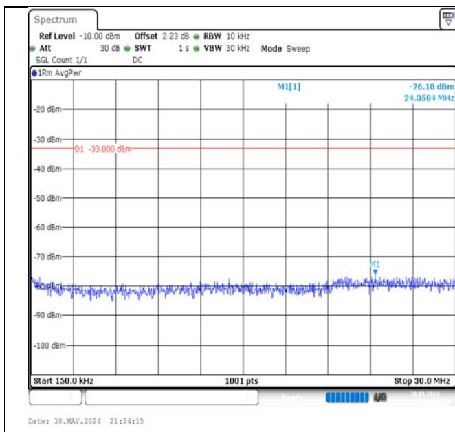
Band66-15MHz-16QAM-132047-1RB#74-0.15~30-PASS
