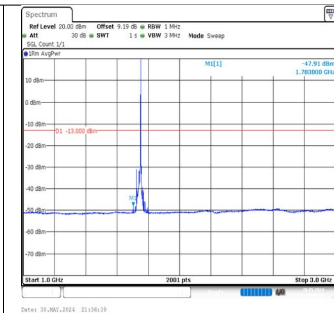
Band66-15MHz-16QAM-132322-1RB#74-1000~3000-PASS
