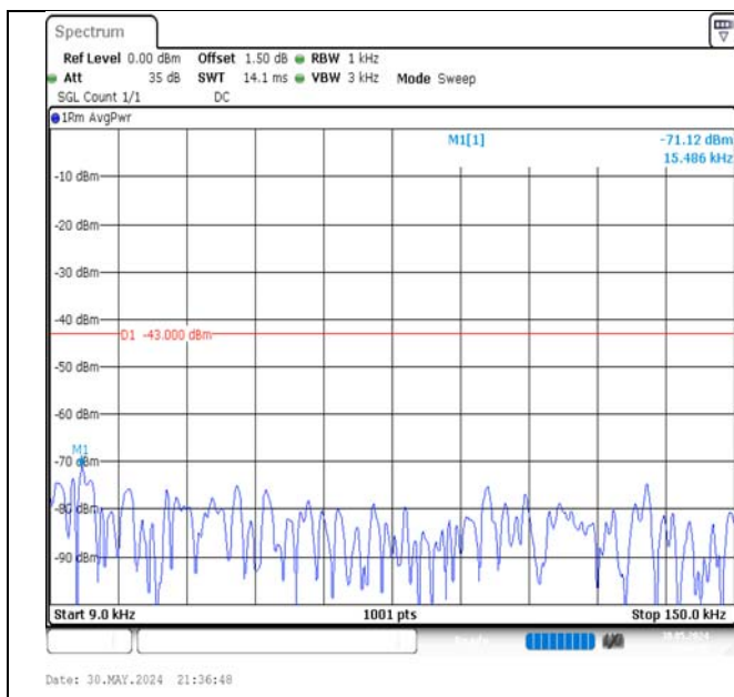
Band66-15MHz-QPSK-132322-75RB#0-0.009~0.15-PASS
