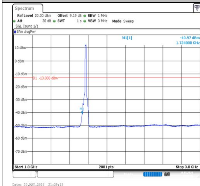
Band66-15MHz-QPSK-132597-75RB#0-1000~3000-PASS
