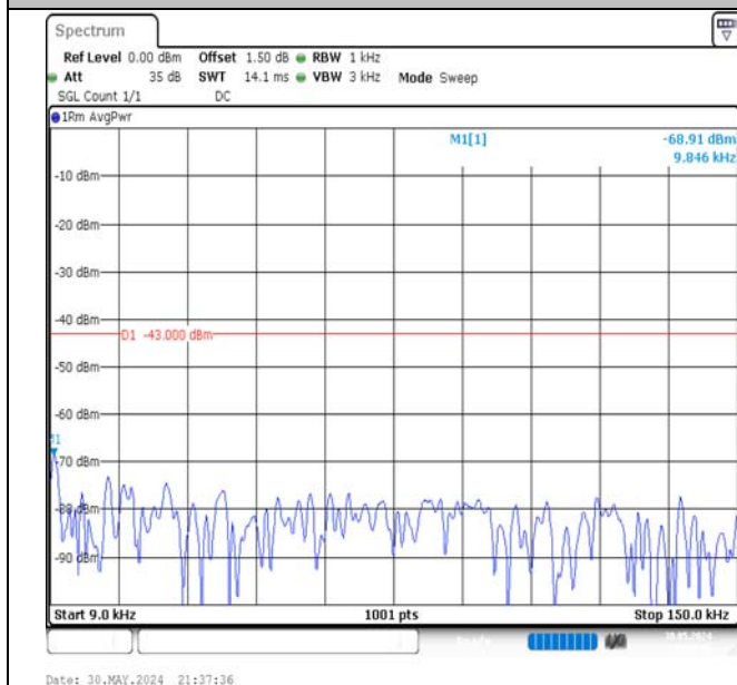
Band66-15MHz-QPSK-132597-1RB#0-0.009~0.15-PASS
