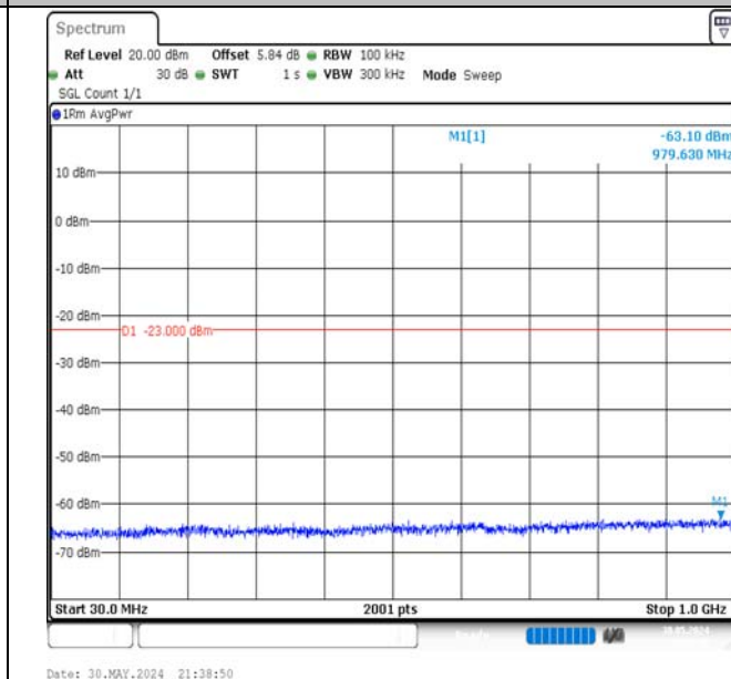
Band66-15MHz-16QAM-132597-1RB#74-30~1000-PASS
