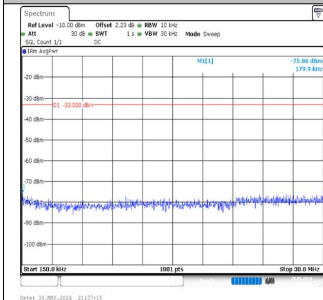
Band66-15MHz-16QAM-132322-75RB#0-0.15~30-PASS
