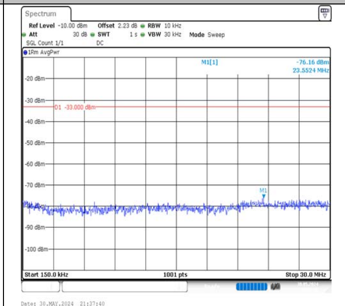
Band66-15MHz-QPSK-132597-1RB#0-0.15~30-PASS
