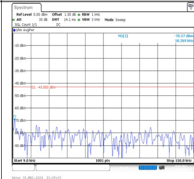
Band66-15MHz-QPSK-132597-75RB#0-0.009~0.15-PASS
