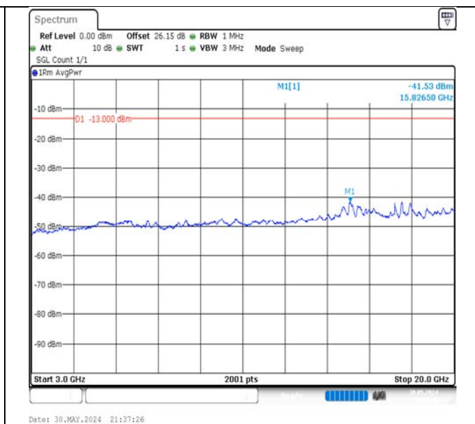
Band66-15MHz-16QAM-132322-75RB#0-3000~20000-PASS
