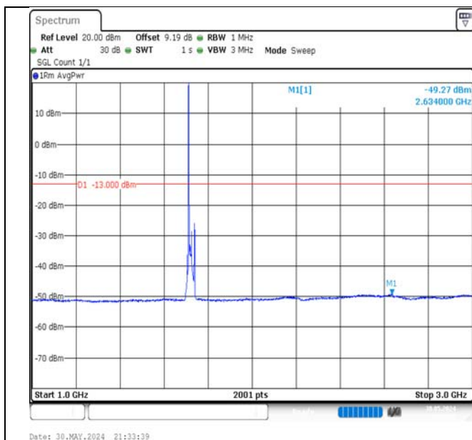
Band66-15MHz-16QAM-132047-1RB#0-1000-3000-PASS
