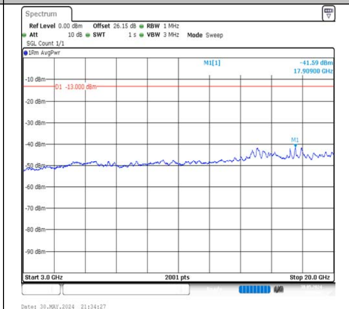
Band66-15MHz-16QAM-132047-1RB#74-3000~20000-PASS
