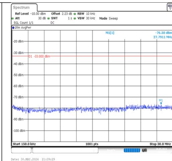
Band66-15MHz-16QAM-132597-75RB#0-0.15~30-PASS
