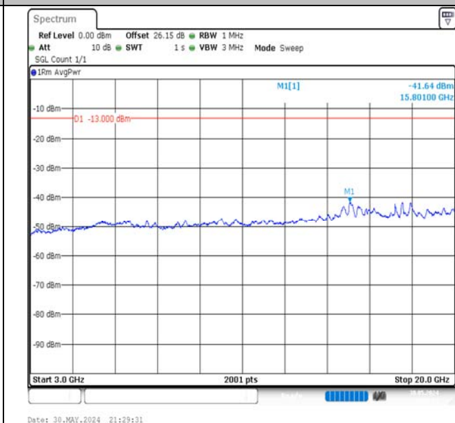
Band66-20MHz-QPSK-132322-1RB#99-3000~20000-PASS
