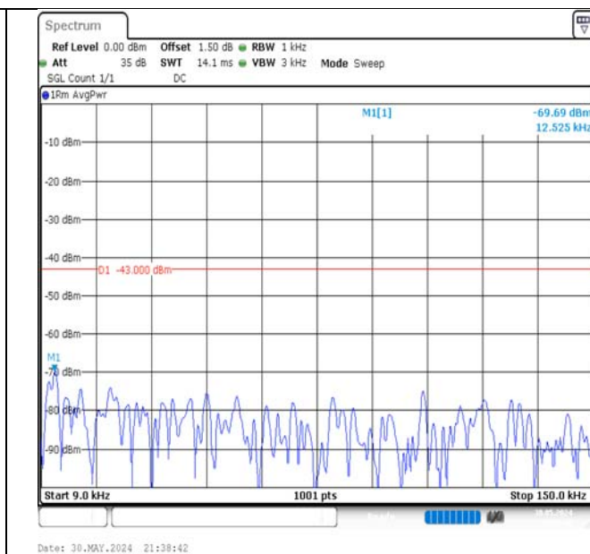
Band66-15MHz-16QAM-132597-1RB#74-0.009~0.15-PASS
