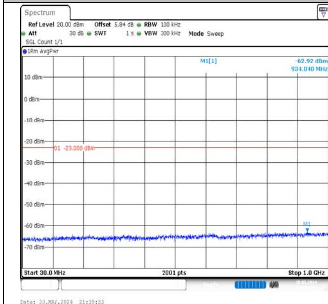
Band66-15MHz-16QAM-132597-75RB#0-30~1000-PASS
