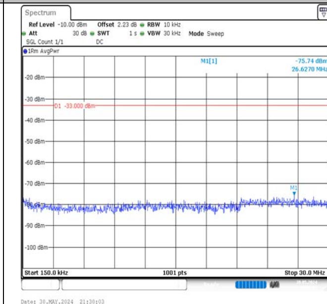
Band66-20MHz-QPSK-132322-100RB#0-0.15~30-PASS
