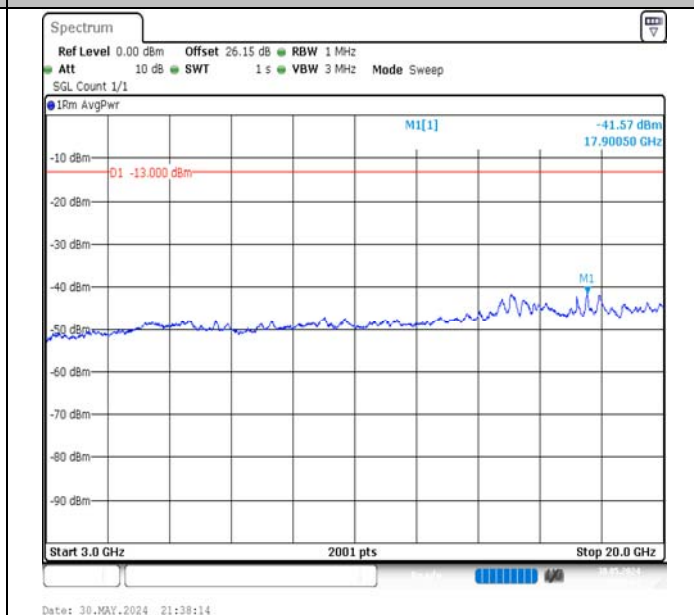
Band66-15MHz-16QAM-132597-1RB#0-3000~20000-PASS
