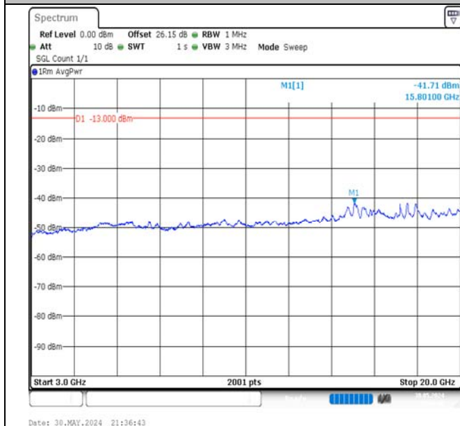
Band66-15MHz-16QAM-132322-1RB#74-3000~20000-PASS
