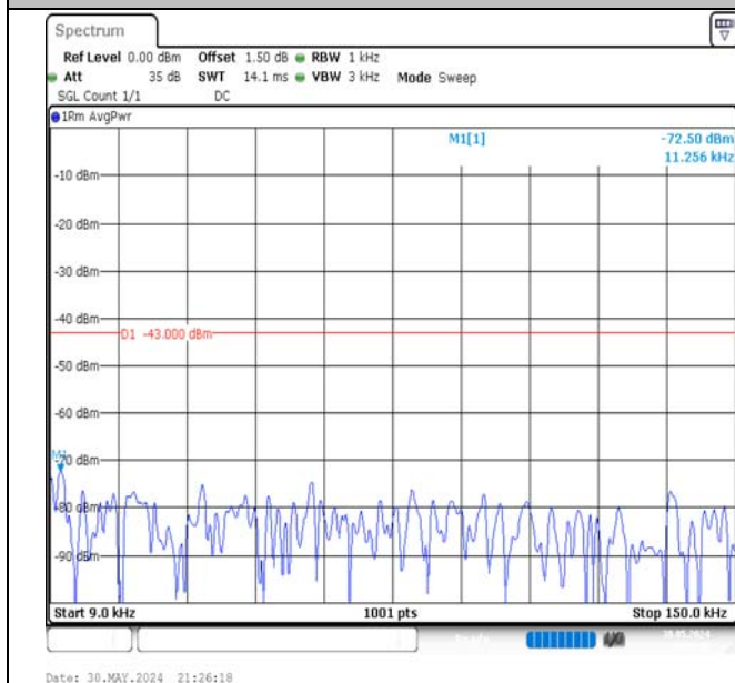
Band66-20MHz-QPSK-132072-1RB#0-0.009~0.15-PASS
