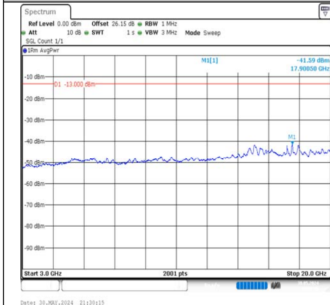
Band66-20MHz-QPSK-132322-100RB#0-3000~20000-PASS
