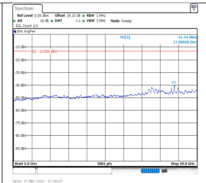
Band66-15MHz-QPSK-132322-1RB#74-3000~20000-PASS
