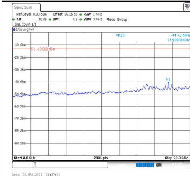
Band66-15MHz-QPSK-132597-1RB#0-3000~20000-PASS
