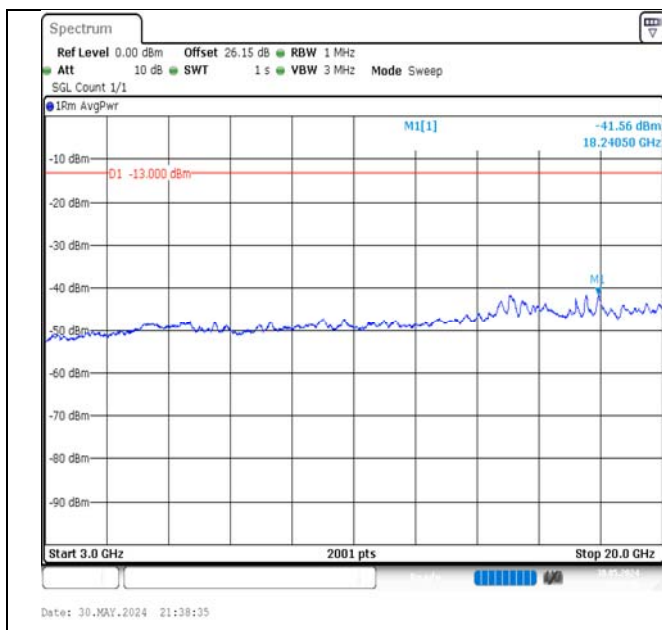
Band66-15MHz-QPSK-132597-1RB#74-3000~20000-PASS
