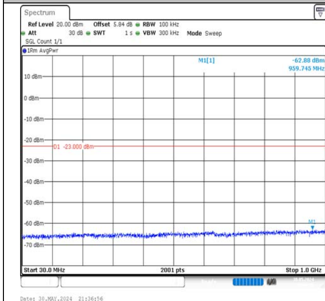
Band66-15MHz-QPSK-132322-75RB#0-30~1000-PASS
