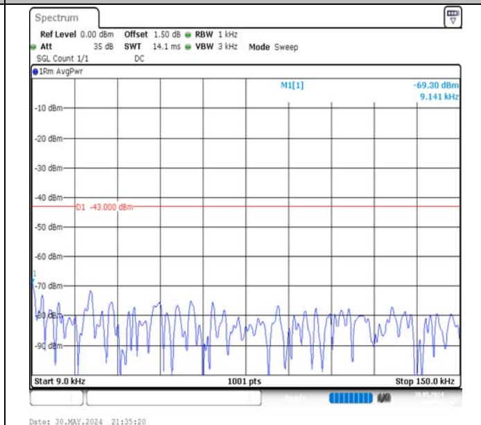
Band66-15MHz-QPSK-132322-1RB#0-0.009~0.15-PASS
