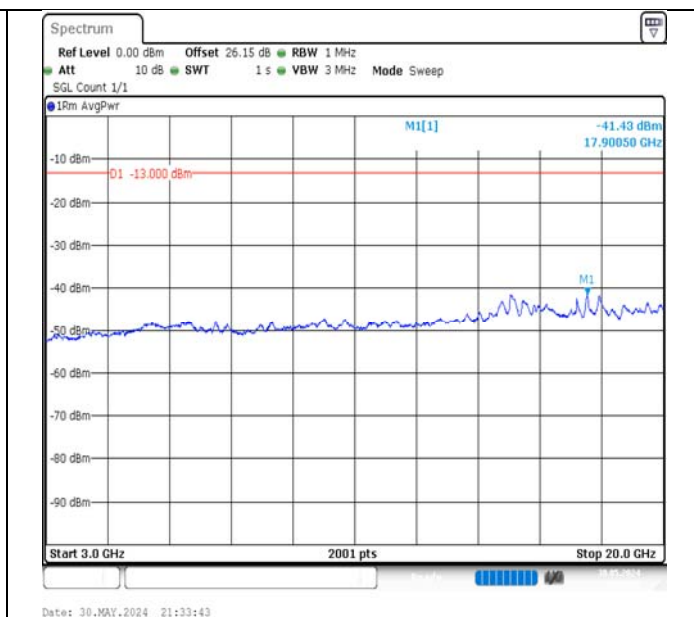
Band66-15MHz-16QAM-132047-1RB#0-3000-20000-PASS
