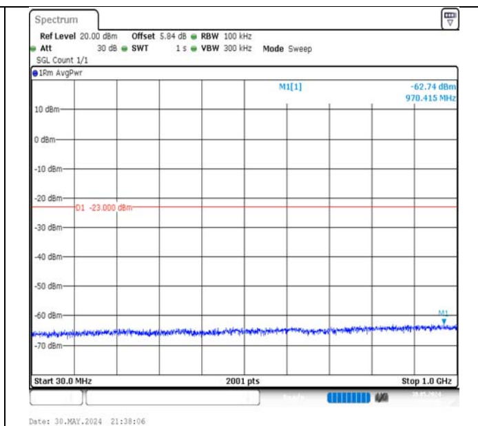
Band66-15MHz-16QAM-132597-1RB#0-30~1000-PASS
