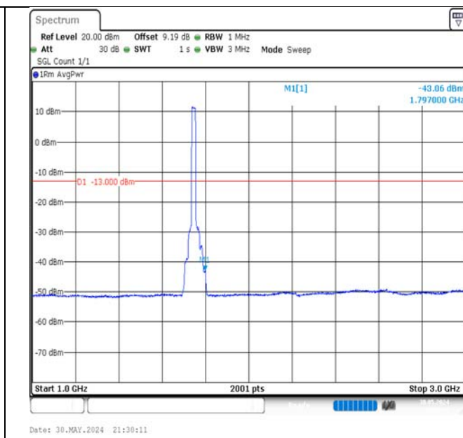
Band66-20MHz-QPSK-132322-100RB#0-1000~3000-PASS
