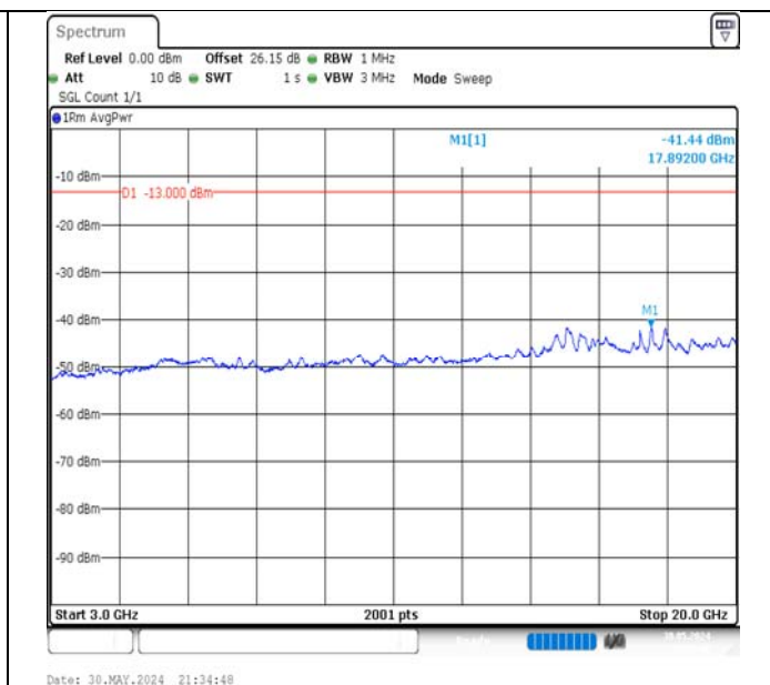
Band66-15MHz-QPSK-132047-75RB#0-3000~20000-PASS
