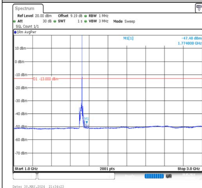
Band66-15MHz-16QAM-132047-1RB#74-1000~3000-PASS
