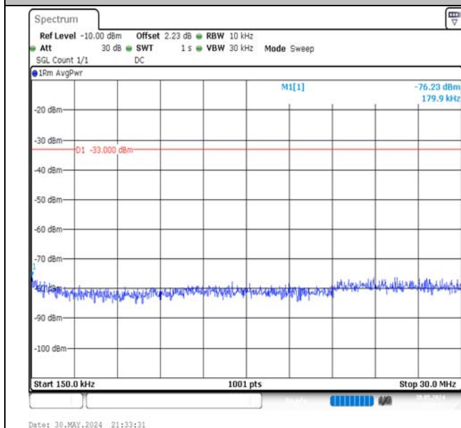
Band66-15MHz-16QAM-132047-1RB#0-0.15~30-PASS
