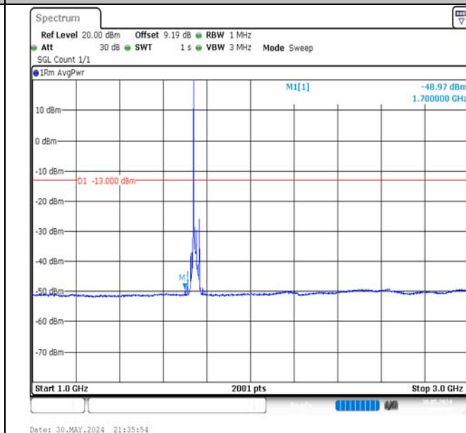
Band66-15MHz-16QAM-132322-1RB#0-1000~3000-PASS
