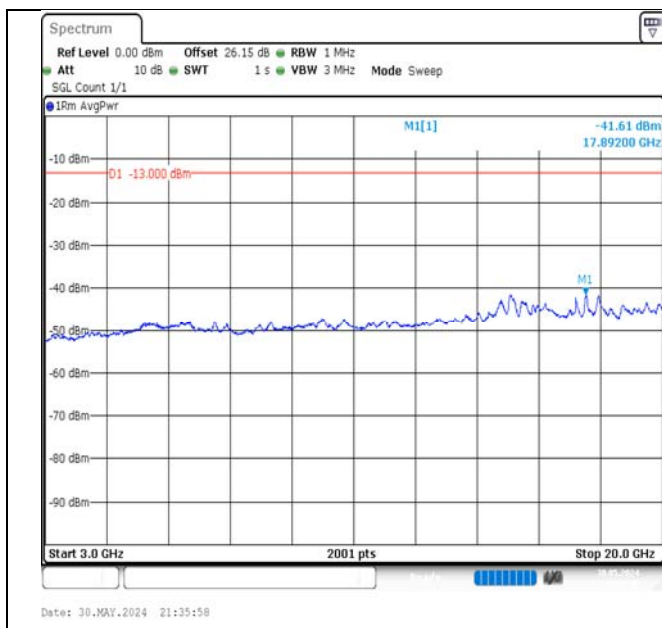
Band66-15MHz-16QAM-132322-1RB#0-3000~20000-PASS
