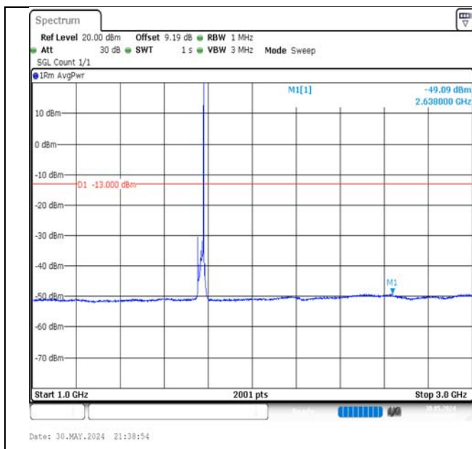
Band66-15MHz-16QAM-132597-1RB#74-1000~3000-PASS
