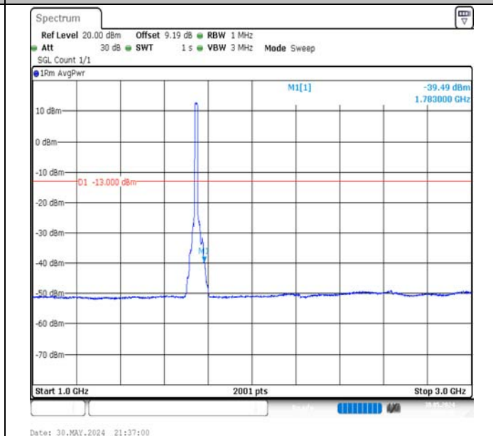
Band66-15MHz-QPSK-132322-75RB#0-1000~3000-PASS
