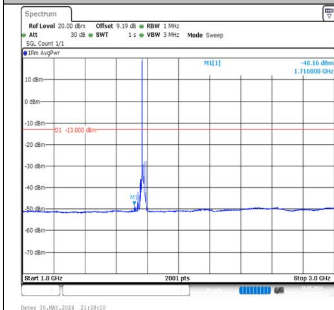
Band66-15MHz-16QAM-132597-1RB#0-1000~3000-PASS
