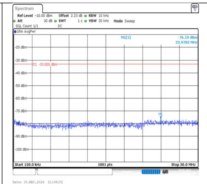
Band66-15MHz-QPSK-132322-75RB#0-0.15~30-PASS
