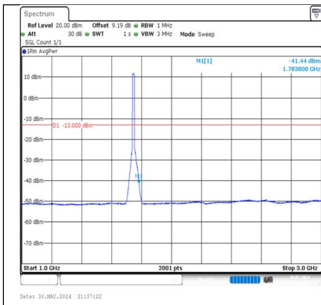
Band66-15MHz-16QAM-132322-75RB#0-1000~3000-PASS
