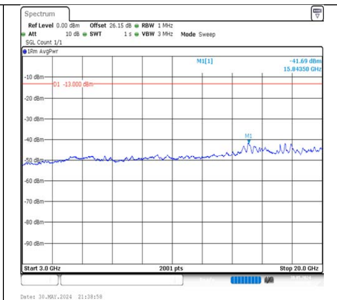
Band66-15MHz-16QAM-132597-1RB#74-3000~20000-PASS
