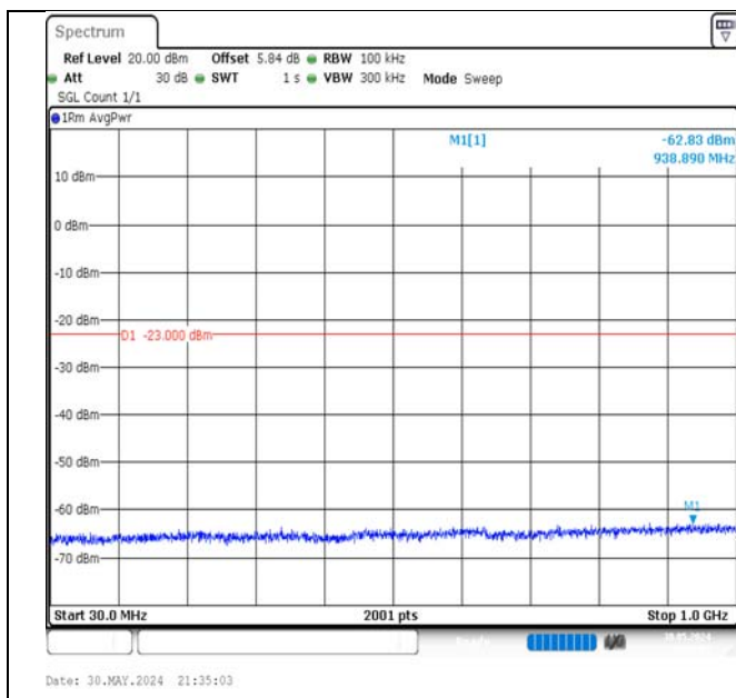
Band66-15MHz-16QAM-132047-75RB#0-30~1000-PASS
