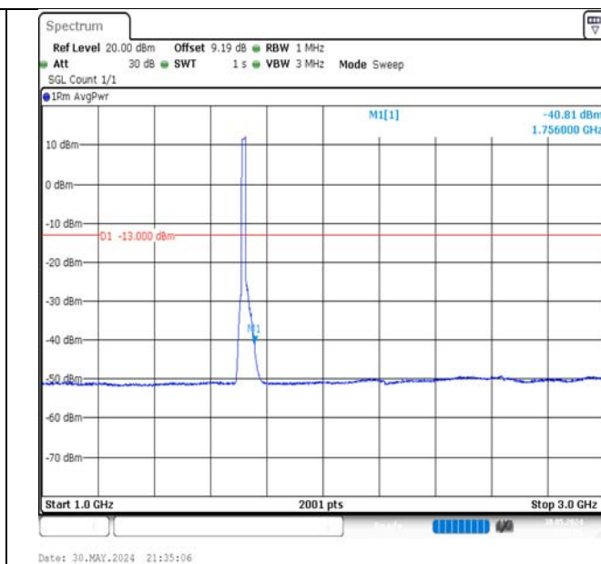
Band66-15MHz-16QAM-132047-75RB#0-1000~3000-PASS
