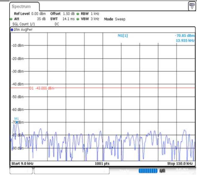
Band66-15MHz-QPSK-132322-1RB#74-0.009~0.15-PASS
