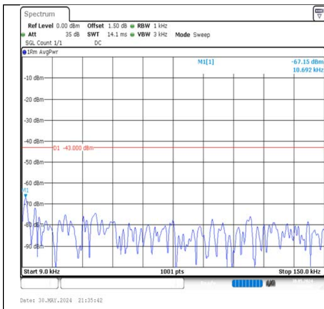
Band66-15MHz-16QAM-132322-1RB#0-0.009~0.15-PASS
