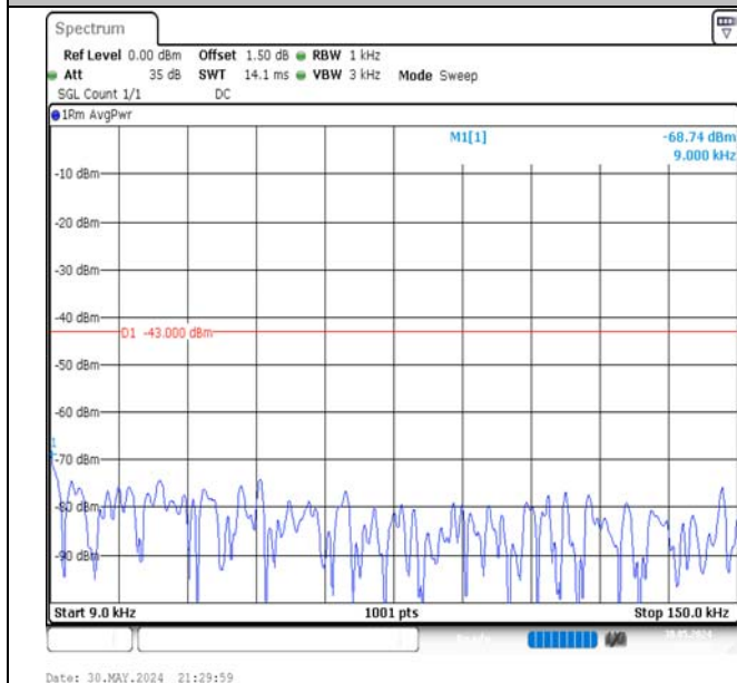
Band66-20MHz-QPSK-132322-100RB#0-0.009~0.15-PASS
