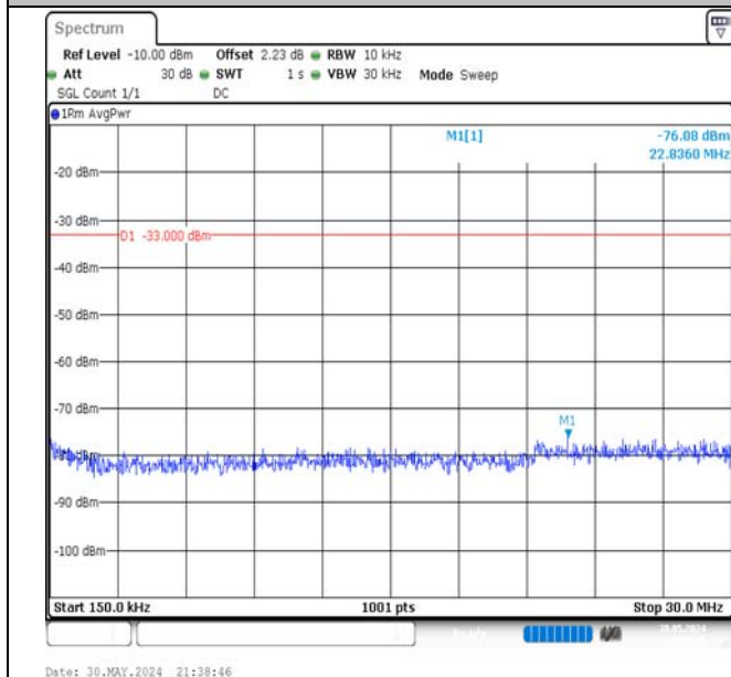
Band66-15MHz-16QAM-132597-1RB#74-0.15~30-PASS
