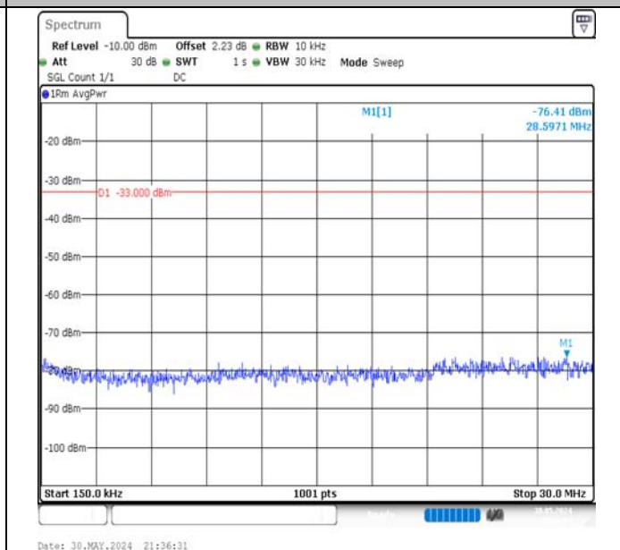
Band66-15MHz-16QAM-132322-1RB#74-0.15~30-PASS
