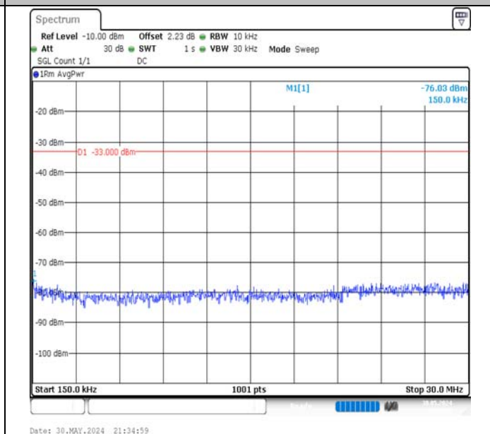
Band66-15MHz-16QAM-132047-75RB#0-0.15-30-PASS
