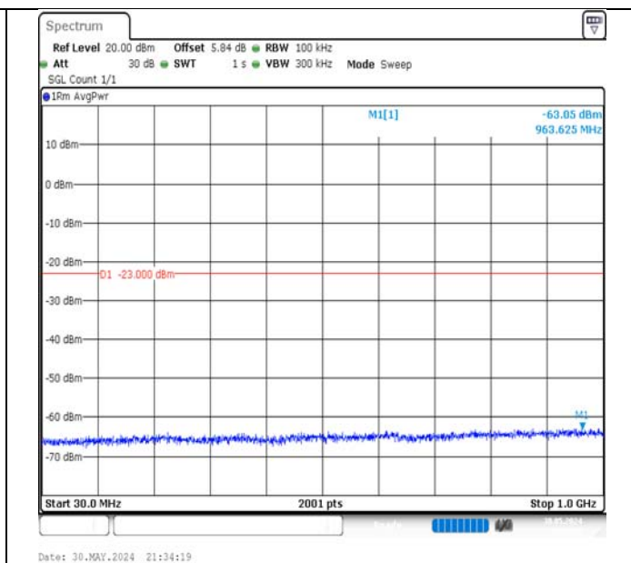
Band66-15MHz-16QAM-132047-1RB#74-30~1000-PASS
