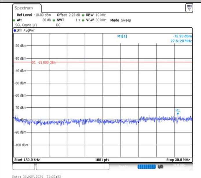
Band66-15MHz-QPSK-132047-1RB#74-0.15~30-PASS
