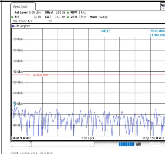
Band66-15MHz-16QAM-132047-1RB#74-0.009~0.15-PASS
