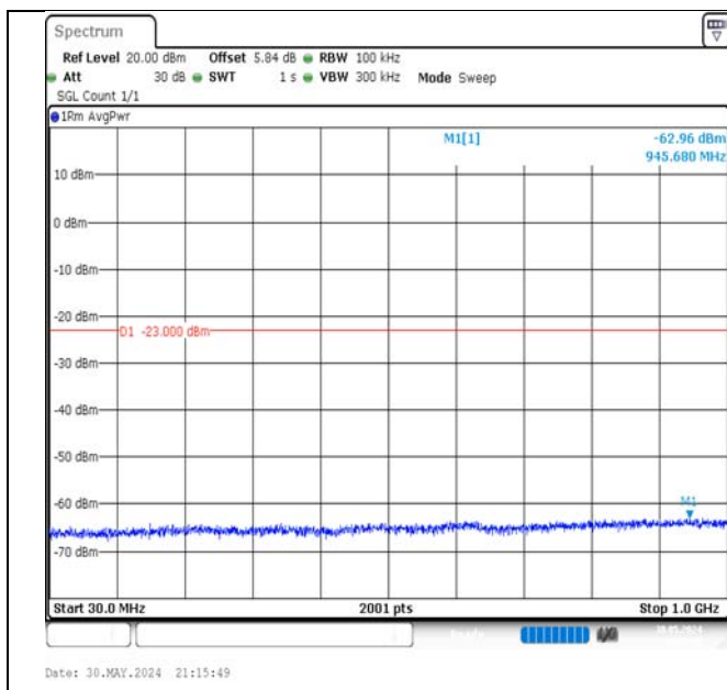
Band66-10MHz-16QAM-132322-1RB#0-30~1000-PASS
