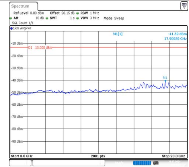
Band66-5MHz-16QAM-132322-25RB#0-3000~20000-PASS
