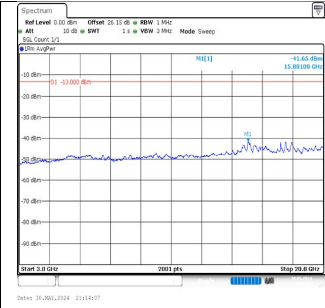
Band66-10MHz-QPSK-132022-1RB#49-3000~20000-PASS
