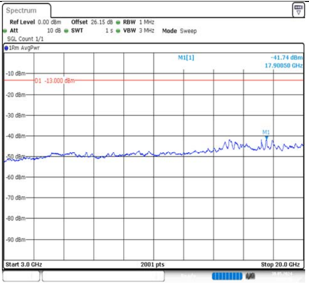
Band66-10MHz-QPSK-132322-1RB#0-3000~20000-PASS
