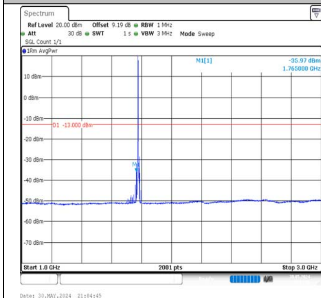
Band66-5MHz-16QAM-132647-1RB#0-1000~3000-PASS
