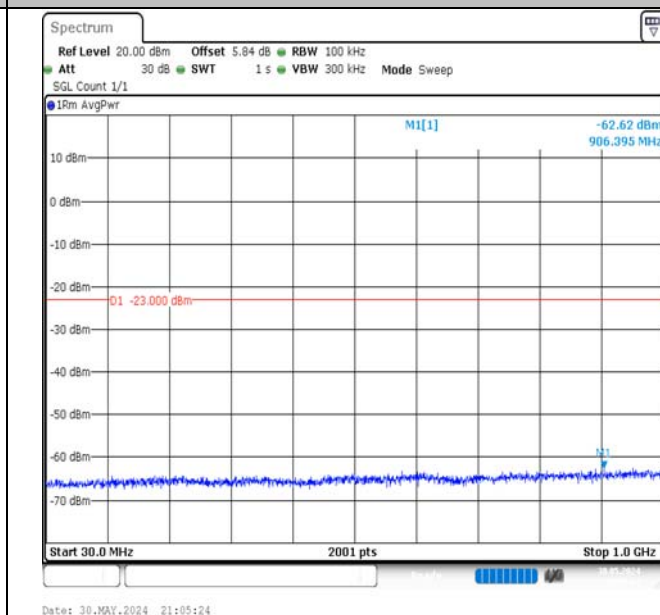
Band66-5MHz-16QAM-132647-1RB#24-30~1000-PASS
