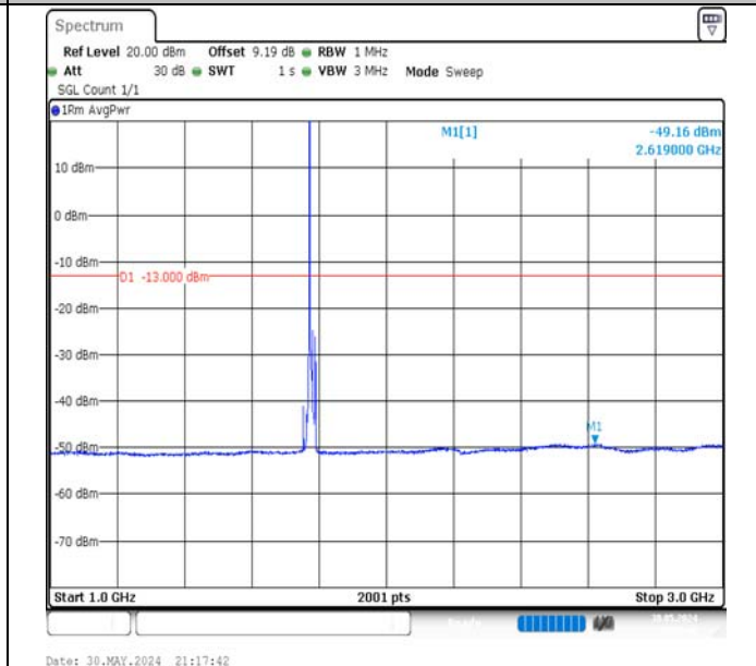
Band66-10MHz-QPSK-132622-1RB#0-1000~3000-PASS
