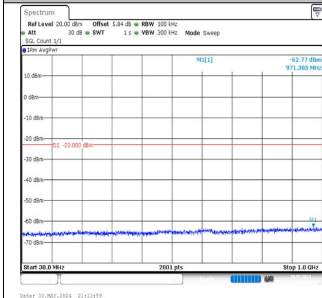
Band66-10MHz-QPSK-132022-1RB#49-30~1000-PASS
