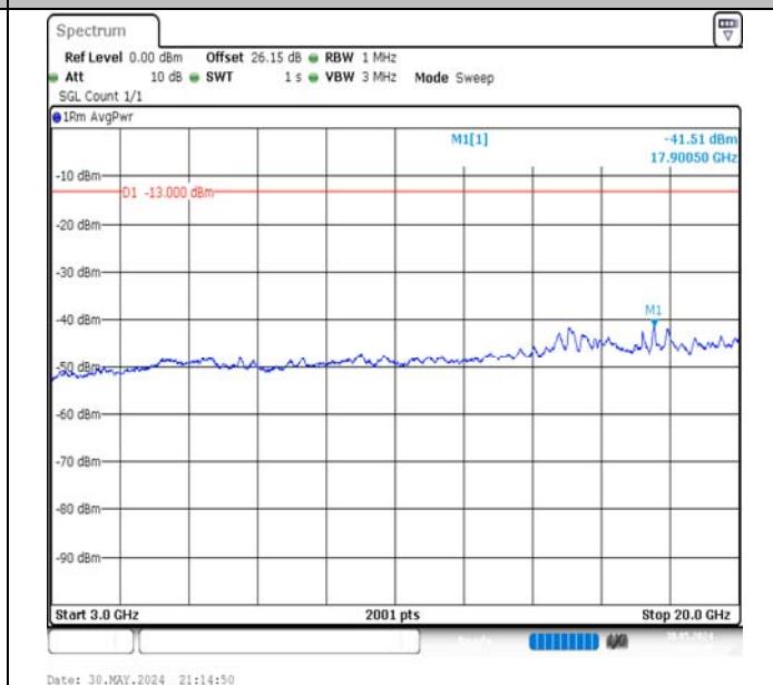
Band66-10MHz-QPSK-132022-50RB#0-3000~20000-PASS
