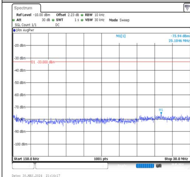
Band66-10MHz-16QAM-132022-1RB#49-0.15~30-PASS
