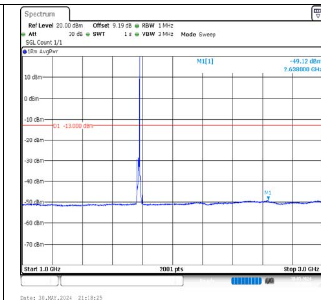
Band66-10MHz-QPSK-132622-1RB#49-1000~3000-PASS
