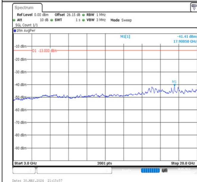
Band66-10MHz-16QAM-132322-1RB#0-3000~20000-PASS
