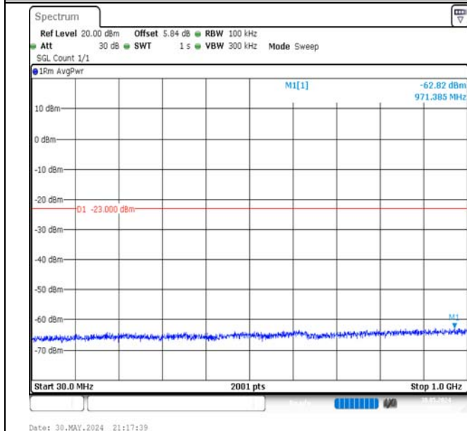
Band66-10MHz-QPSK-132622-1RB#0-30~1000-PASS
