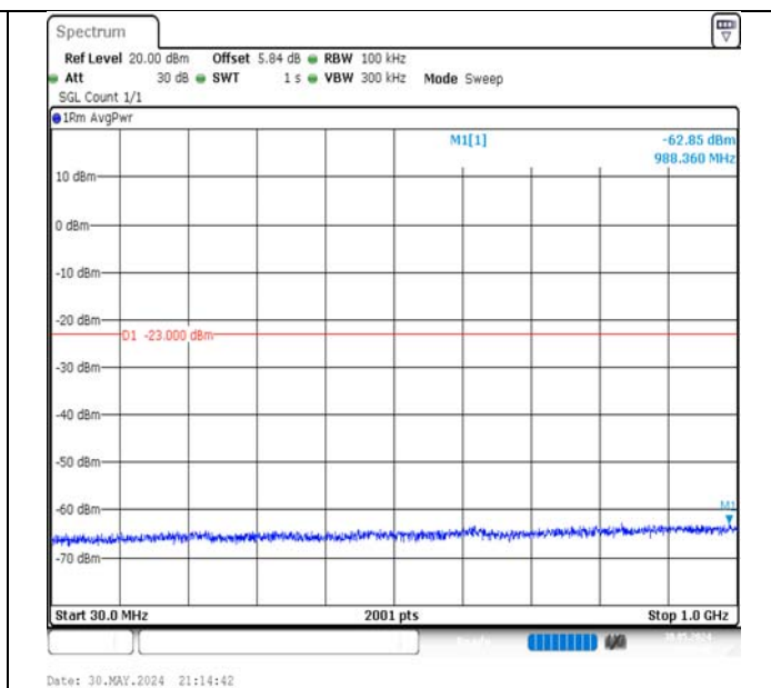
Band66-10MHz-QPSK-132022-50RB#0-30~1000-PASS
