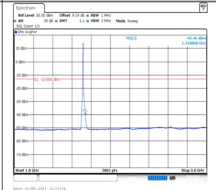
Band66-10MHz-16QAM-132022-50RB#0-1000~3000-PASS
