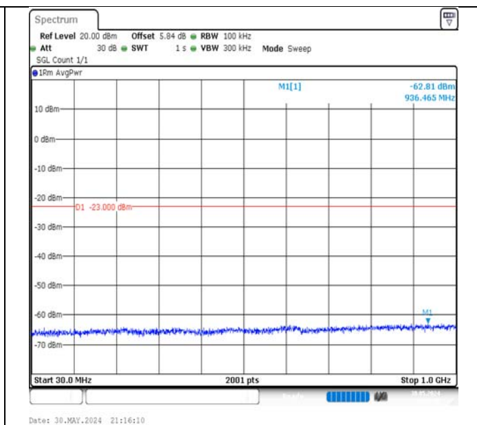
Band66-10MHz-QPSK-132322-1RB#49-30~1000-PASS
