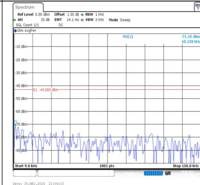
Band66-5MHz-16QAM-132647-1RB#0-0.009~0.15-PASS
