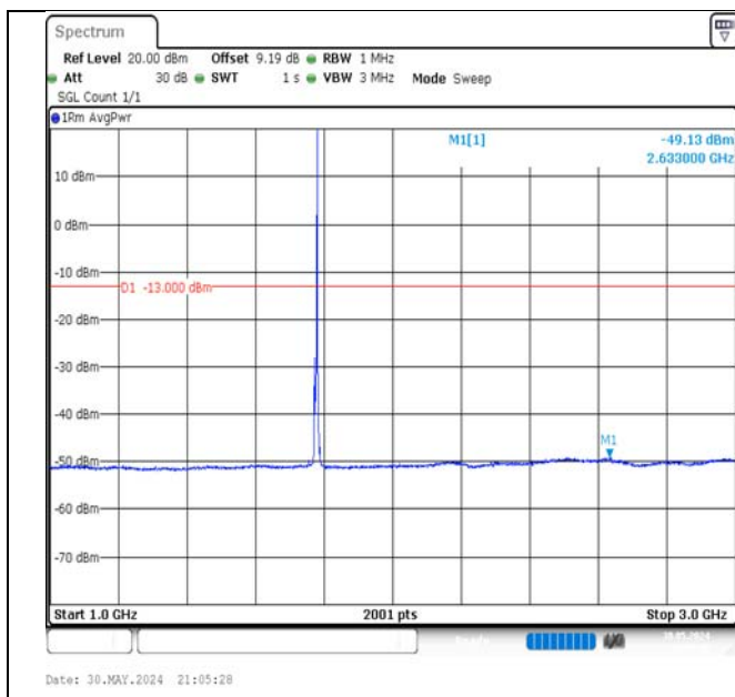
Band66-5MHz-16QAM-132647-1RB#24-1000~3000-PASS
