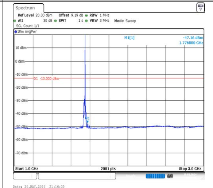
Band66-10MHz-16QAM-132322-1RB#49-1000~3000-PASS
