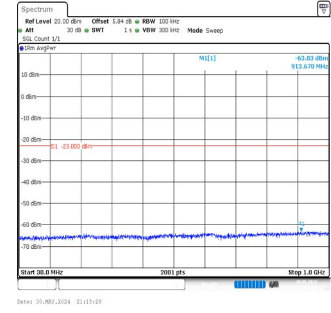
Band66-10MHz-QPSK-132322-1RB#0-30~1000-PASS
