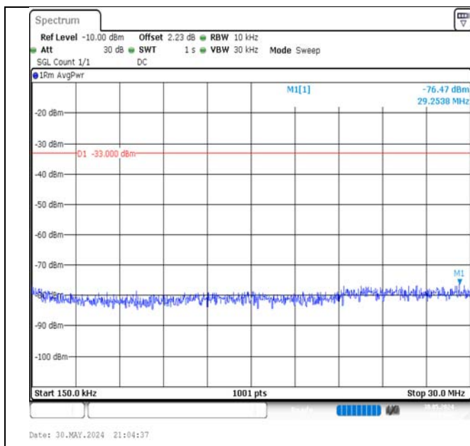
Band66-5MHz-16QAM-132647-1RB#0-0.15~30-PASS
