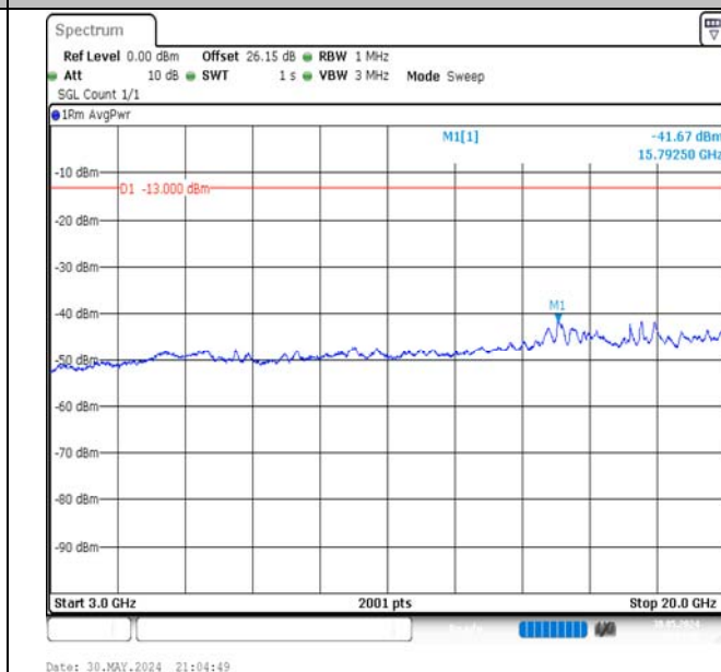
Band66-5MHz-16QAM-132647-1RB#0-3000~20000-PASS
