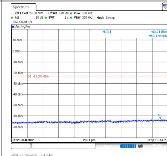
Band66-10MHz-16QAM-132022-1RB#49-30~1000-PASS
