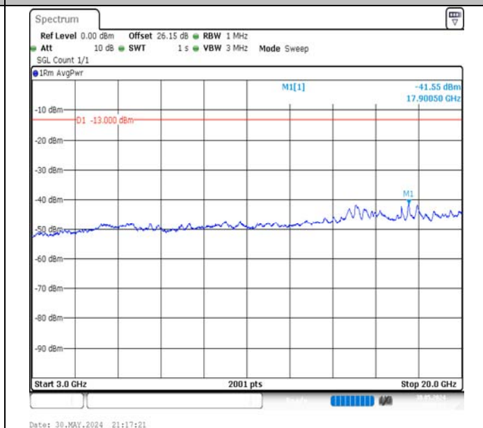
Band66-10MHz-16QAM-132322-50RB#0-3000~20000-PASS
