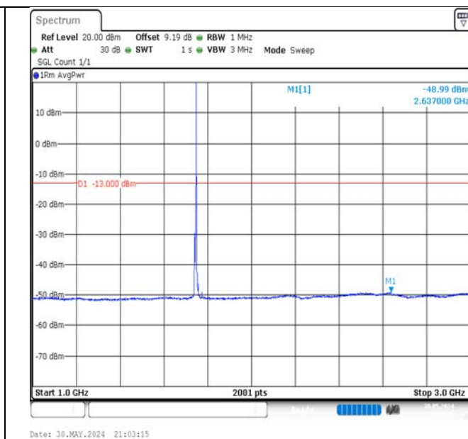
Band66-5MHz-16QAM-132322-1RB#24-1000~3000-PASS
