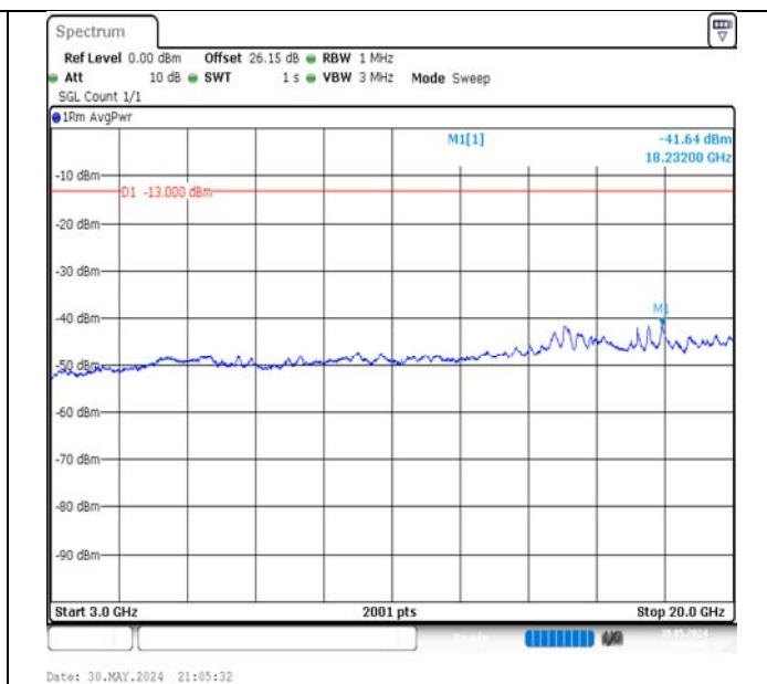
Band66-5MHz-16QAM-132647-1RB#24-3000~20000-PASS
