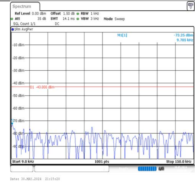
Band66-10MHz-QPSK-132322-1RB#0-0.009~0.15-PASS
