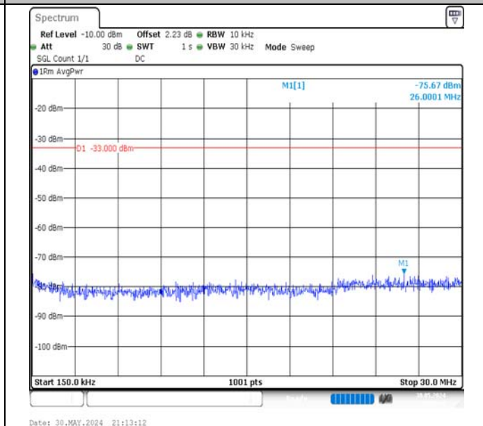
Band66-10MHz-QPSK-132022-1RB#0-0.15~30-PASS
