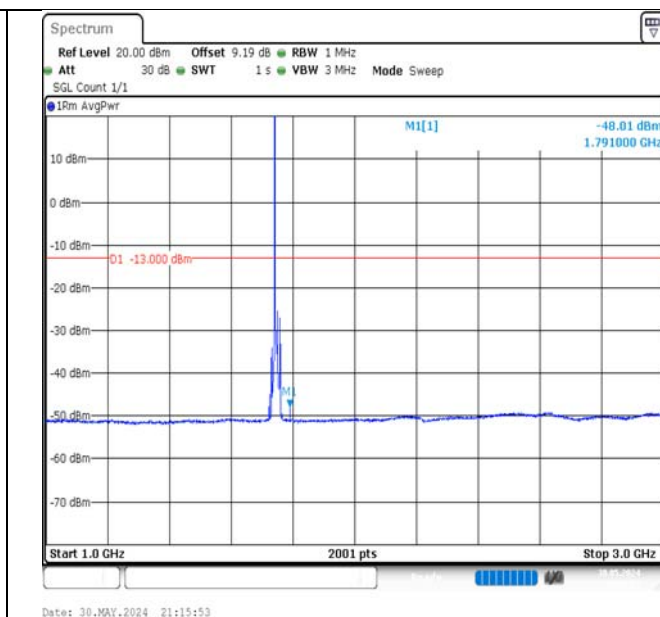
Band66-10MHz-16QAM-132322-1RB#0-1000~3000-PASS
