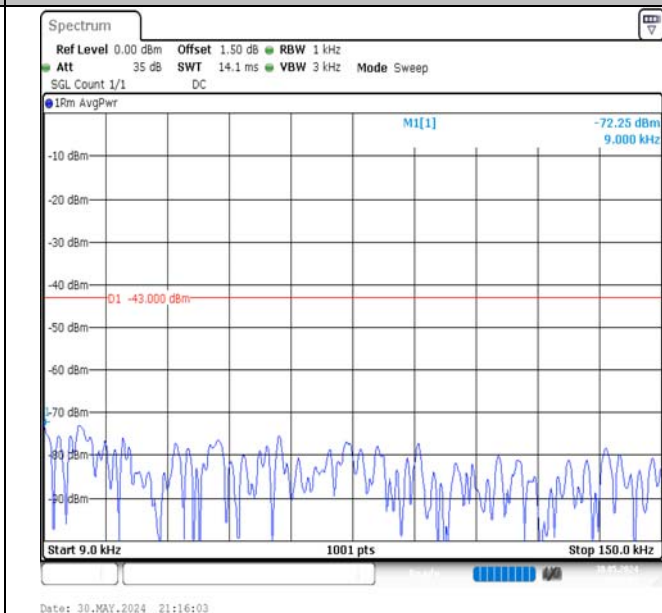
Band66-10MHz-QPSK-132322-1RB#49-0.009~0.15-PASS
