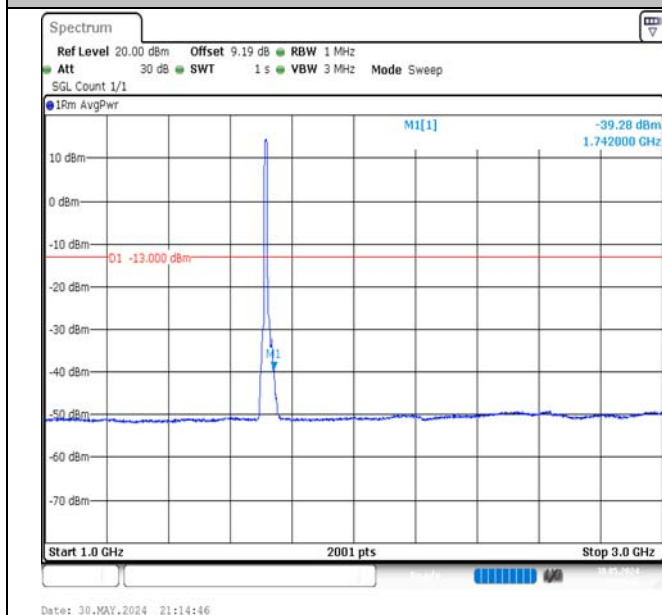
Band66-10MHz-QPSK-132022-50RB#0-1000~3000-PASS
