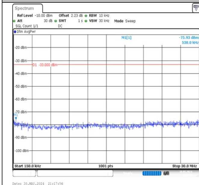
Band66-10MHz-16QAM-132622-1RB#0-0.15~30-PASS
