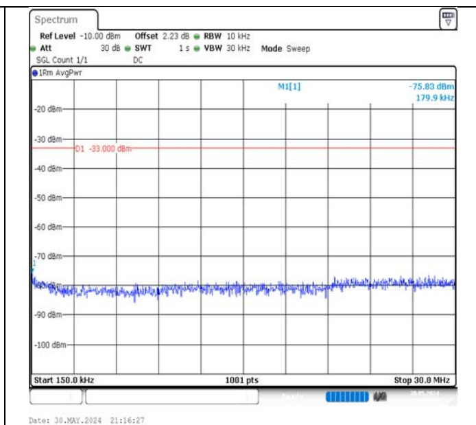
Band66-10MHz-16QAM-132322-1RB#49-0.15~30-PASS
