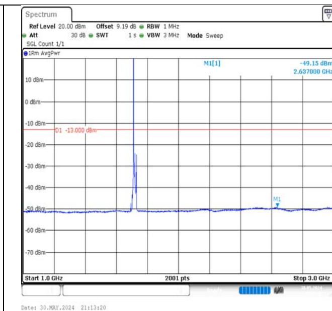
Band66-10MHz-QPSK-132022-1RB#0-1000~3000-PASS
