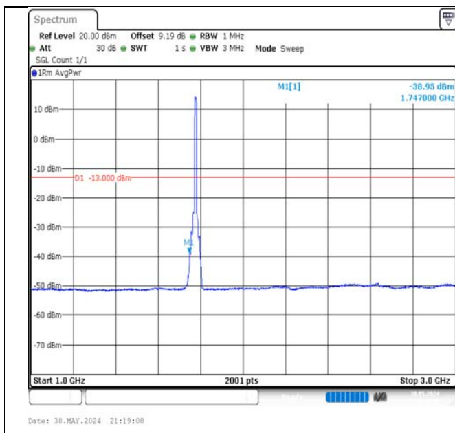
Band66-10MHz-QPSK-132622-50RB#0-1000~3000-PASS
