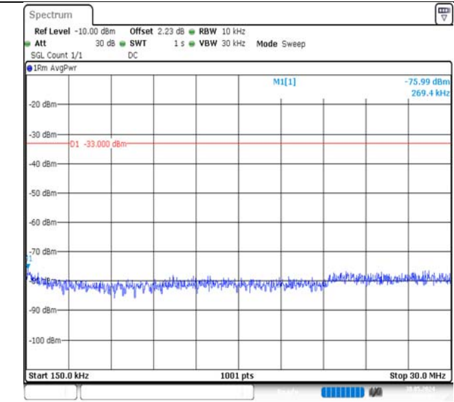
Band66-15MHz-QPSK-132047-1RB#0-0.15~30-PASS
