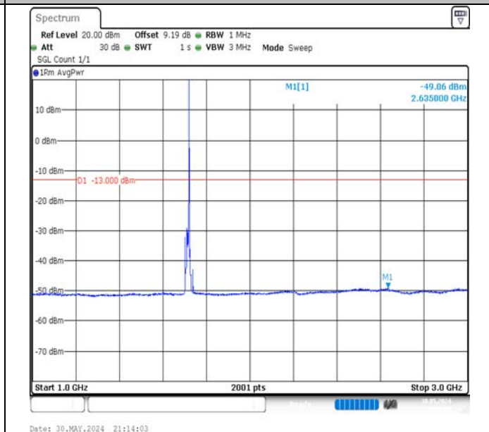
Band66-10MHz-QPSK-132022-1RB#49-1000~3000-PASS
