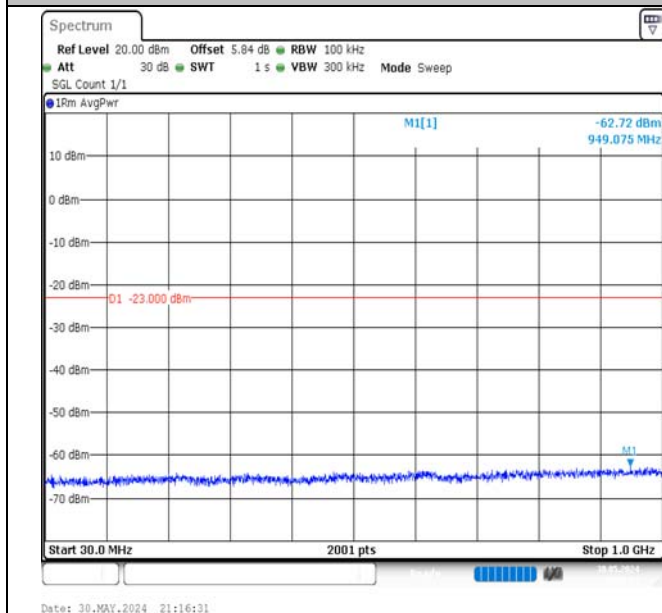
Band66-10MHz-16QAM-132322-1RB#49-30~1000-PASS
