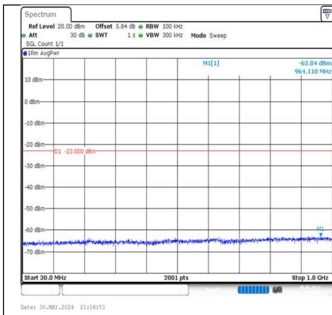
Band66-10MHz-QPSK-132322-50RB#0-30~1000-PASS
