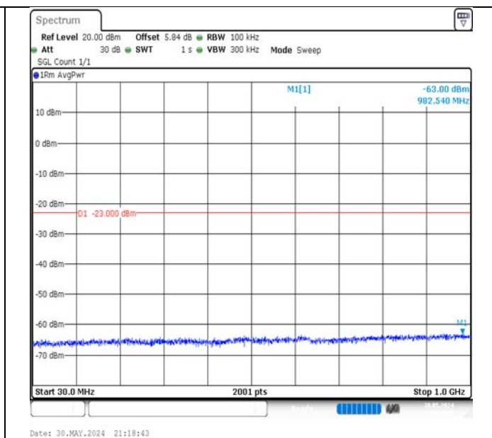
Band66-10MHz-16QAM-132622-1RB#49-30~1000-PASS
