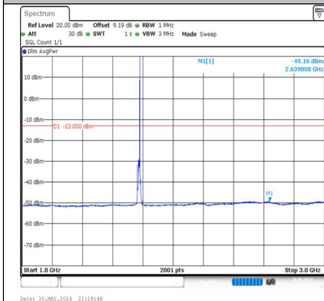
Band66-10MHz-16QAM-132622-1RB#49-1000~3000-PASS
