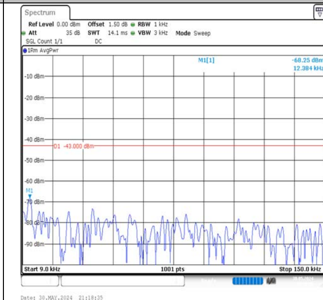
Band66-10MHz-16QAM-132622-1RB#49-0.009~0.15-PASS
