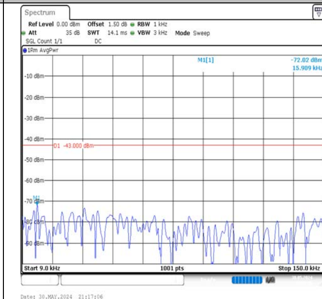
Band66-10MHz-16QAM-132322-50RB#0-0.009~0.15-PASS
