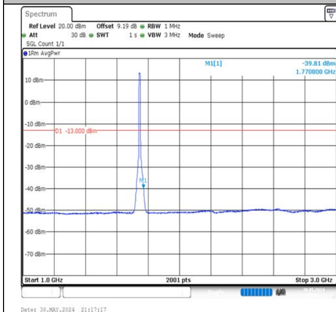
Band66-10MHz-16QAM-132322-50RB#0-1000~3000-PASS
