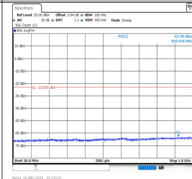
Band66-10MHz-16QAM-132622-1RB#0-30~1000-PASS
