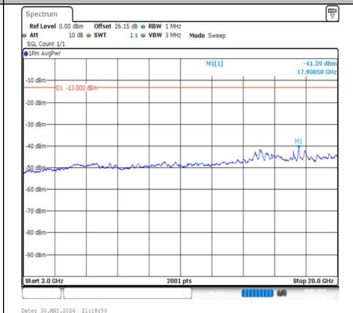
Band66-10MHz-16QAM-132622-1RB#49-3000~20000-PASS
