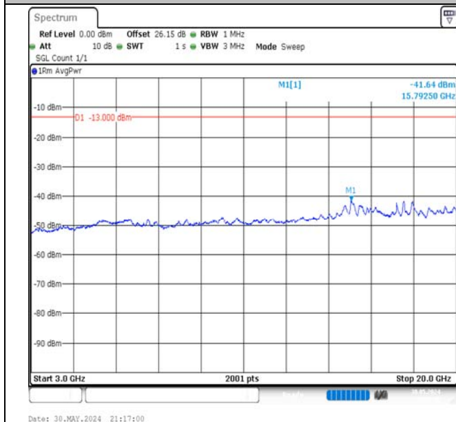
Band66-10MHz-QPSK-132322-50RB#0-3000~20000-PASS
