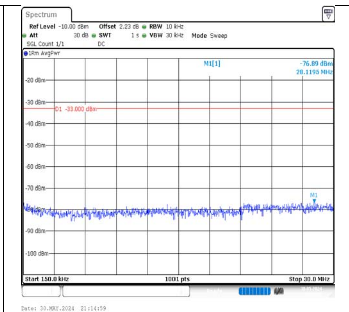
Band66-10MHz-16QAM-132022-50RB#0-0.15~30-PASS
