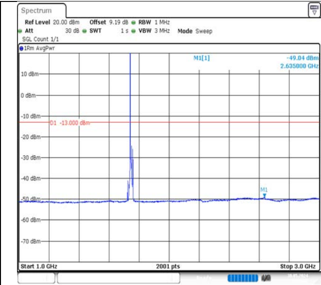
Band66-10MHz-QPSK-132322-1RB#0-1000~3000-PASS
