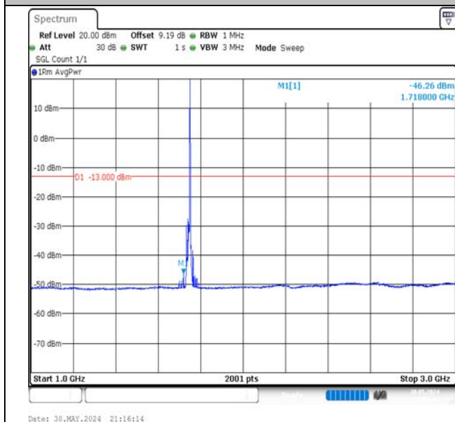
Band66-10MHz-QPSK-132322-1RB#49-1000~3000-PASS
