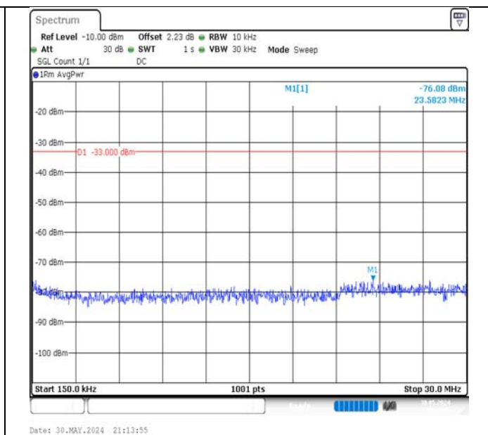
Band66-10MHz-QPSK-132022-1RB#49-0.15~30-PASS
