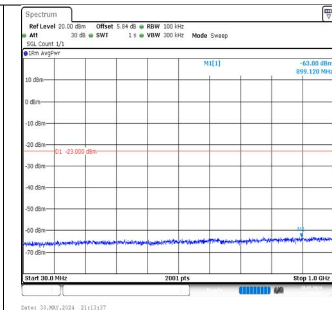
Band66-10MHz-16QAM-132022-1RB#0-30~1000-PASS
