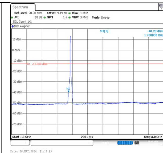
Band66-10MHz-16QAM-132622-50RB#0-1000~3000-PASS
