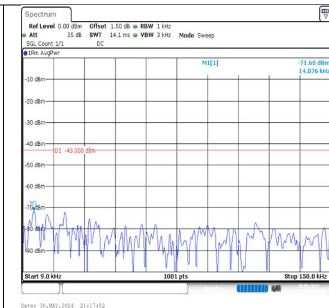
Band66-10MHz-16QAM-132622-1RB#0-0.009~0.15-PASS
