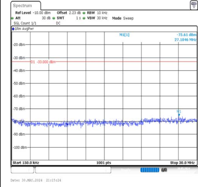
Band66-10MHz-QPSK-132322-1RB#0-0.15~30-PASS
