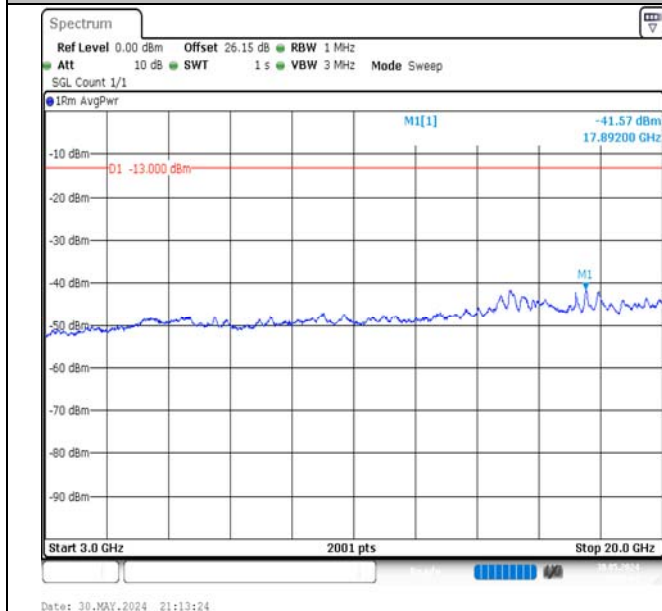
Band66-10MHz-QPSK-132022-1RB#0-3000~20000-PASS
