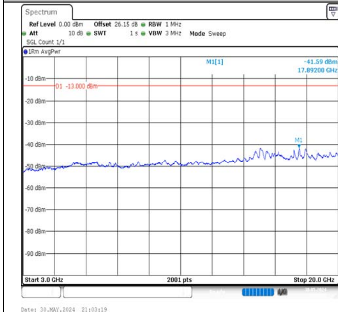
Band66-5MHz-16QAM-132322-1RB#24-3000~20000-PASS
