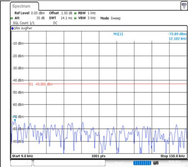
Band66-15MHz-QPSK-132047-1RB#0-0.009~0.15-PASS
