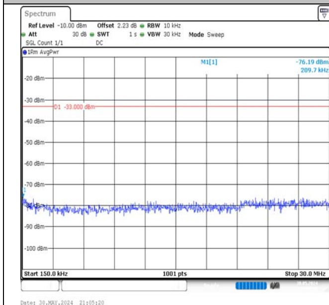
Band66-5MHz-16QAM-132647-1RB#24-0.15~30-PASS
