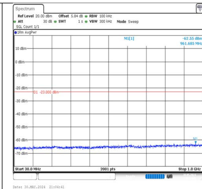
Band66-5MHz-16QAM-132647-1RB#0-30~1000-PASS
