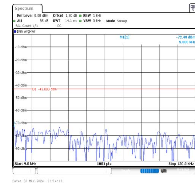
Band66-10MHz-16QAM-132022-1RB#49-0.009~0.15-PASS
