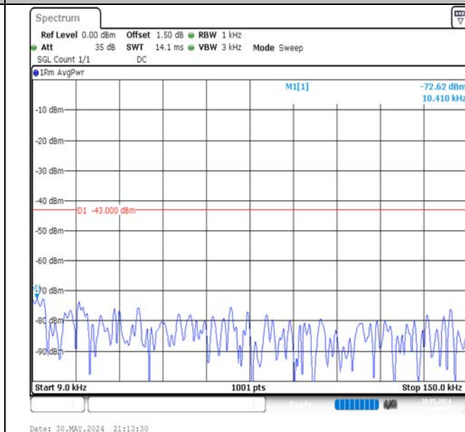
Band66-10MHz-16QAM-132022-1RB#0-0.009~0.15-PASS
