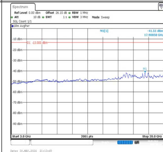
Band66-10MHz-16QAM-132022-1RB#0-3000~20000-PASS
