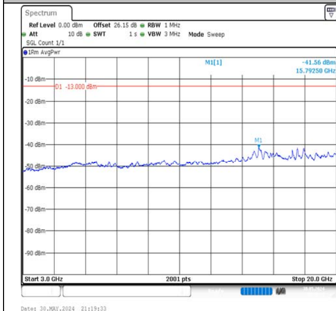
Band66-10MHz-16QAM-132622-50RB#0-3000~20000-PASS
