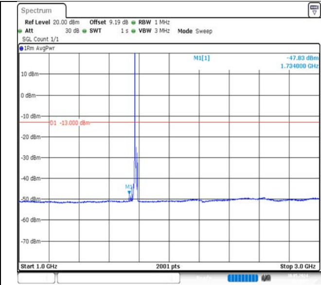
Band66-10MHz-16QAM-132622-1RB#0-1000~3000-PASS
