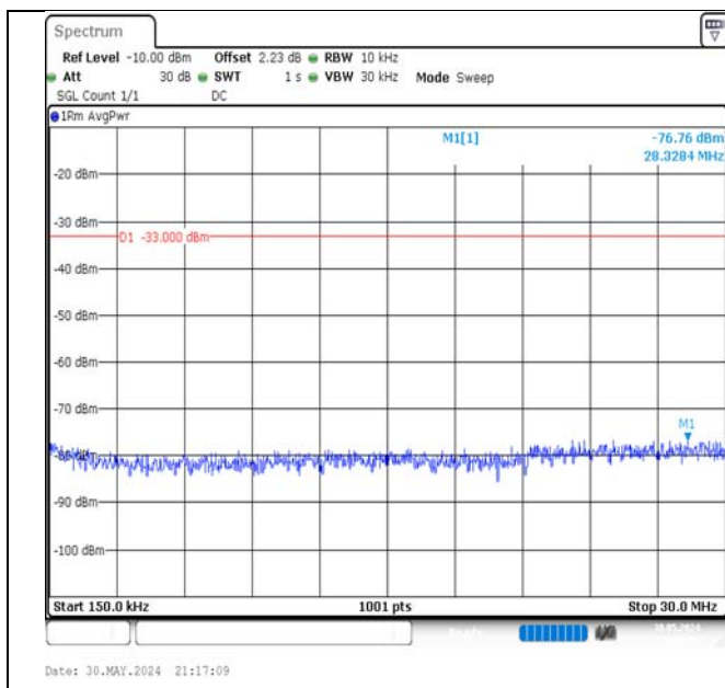
Band66-10MHz-16QAM-132322-50RB#0-0.15~30-PASS
