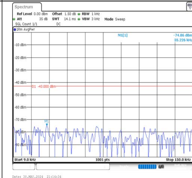
Band66-10MHz-QPSK-132022-50RB#0-0.009~0.15-PASS
