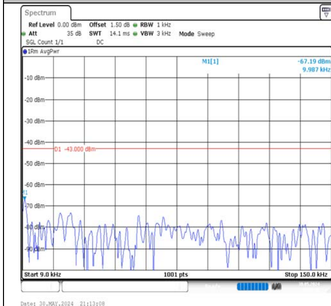
Band66-10MHz-QPSK-132022-1RB#0-0.009~0.15-PASS
