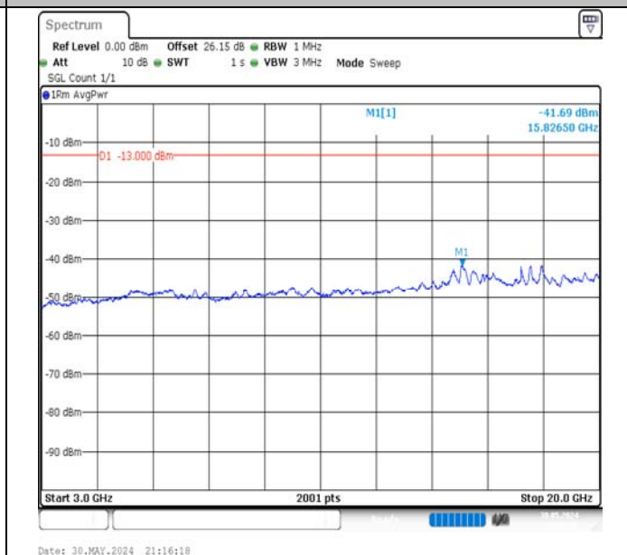
Band66-10MHz-QPSK-132322-1RB#49-3000~20000-PASS
