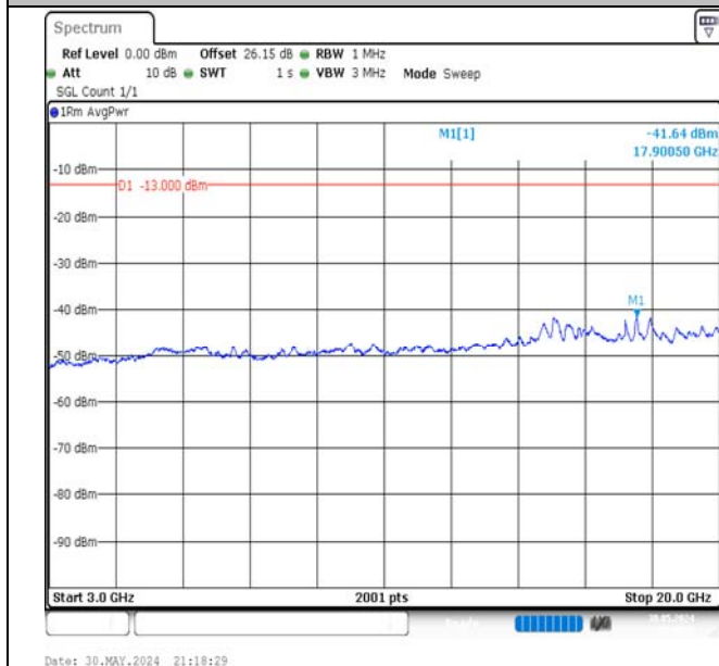
Band66-10MHz-QPSK-132622-1RB#49-3000~20000-PASS
