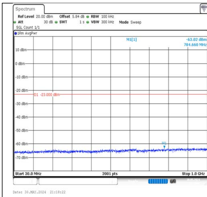
Band66-10MHz-QPSK-132622-1RB#49-30~1000-PASS
