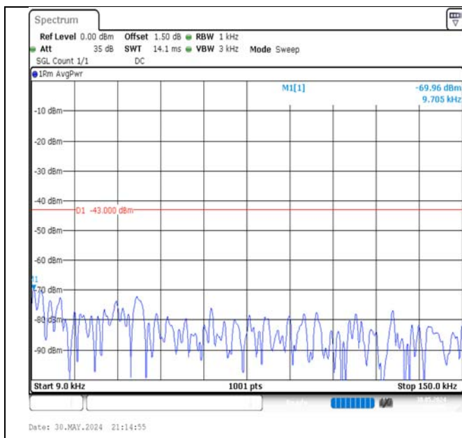
Band66-10MHz-16QAM-132022-50RB#0-0.009~0.15-PASS
