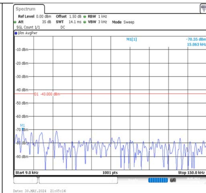
Band66-5MHz-16QAM-132647-1RB#24-0.009~0.15-PASS
