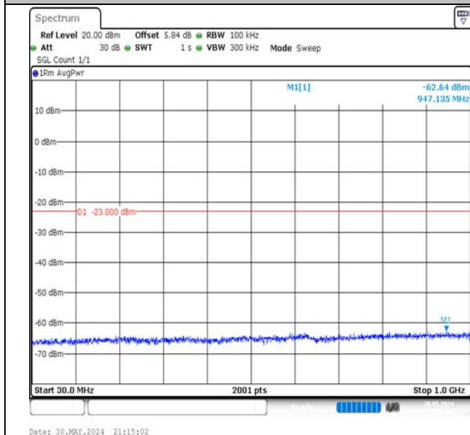
Band66-10MHz-16QAM-132022-50RB#0-30~1000-PASS
