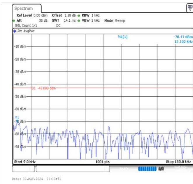
Band66-10MHz-QPSK-132022-1RB#49-0.009~0.15-PASS
