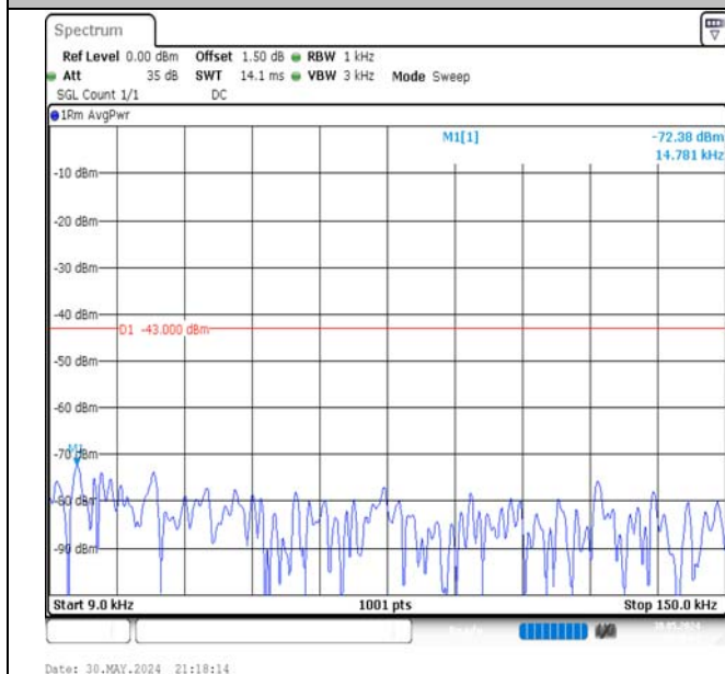
Band66-10MHz-QPSK-132622-1RB#49-0.009~0.15-PASS
