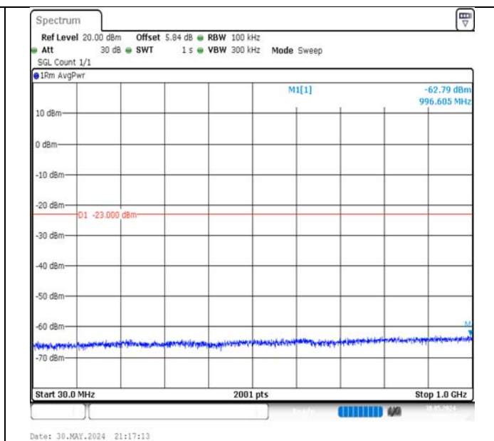
Band66-10MHz-16QAM-132322-50RB#0-30~1000-PASS
