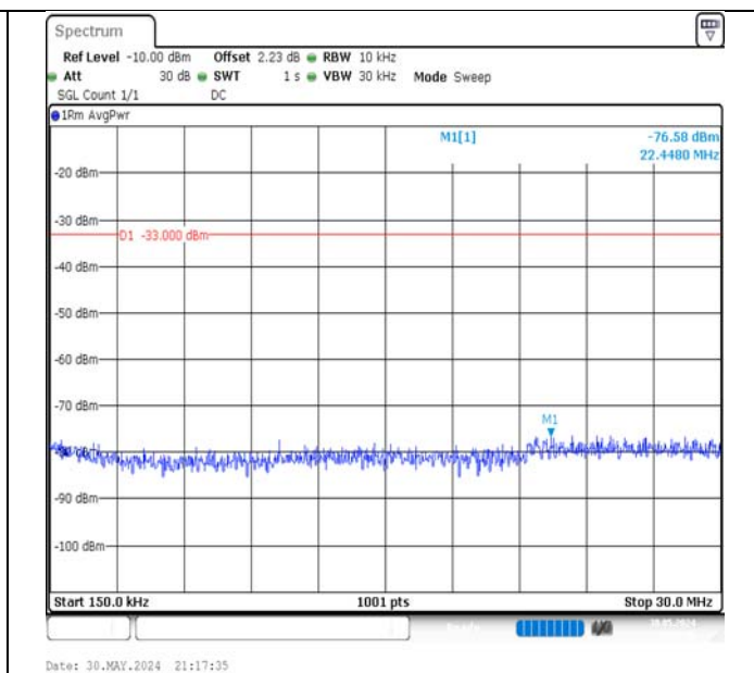
Band66-10MHz-QPSK-132622-1RB#0-0.15~30-PASS
