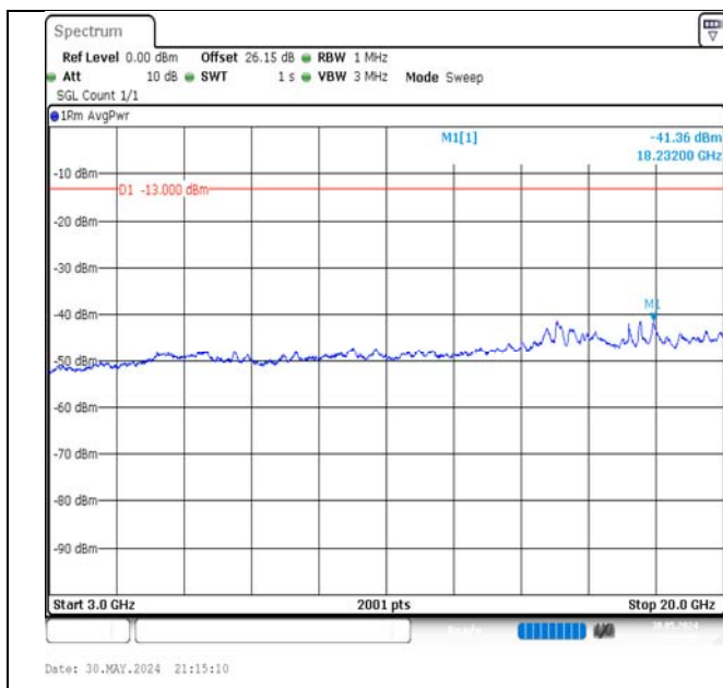
Band66-10MHz-16QAM-132022-50RB#0-3000~20000-PASS
