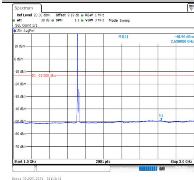
Band66-10MHz-16QAM-132022-1RB#0-1000~3000-PASS
