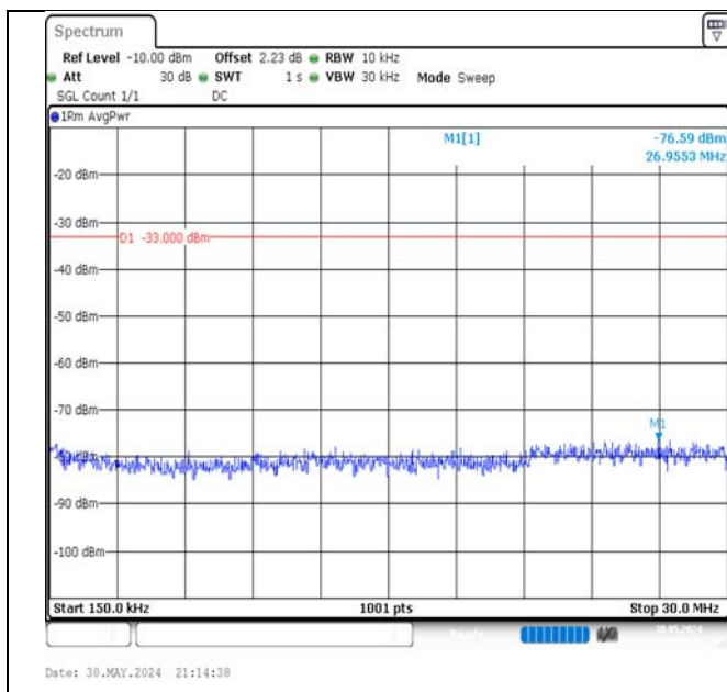
Band66-10MHz-QPSK-132022-50RB#0-0.15~30-PASS
