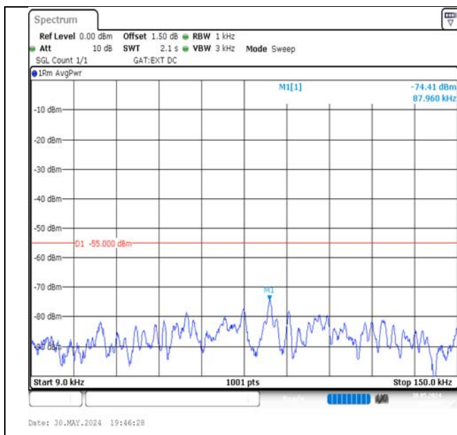
Band41-20MHz-QPSK-41490-1RB#0-0.009~0.15-PASS
