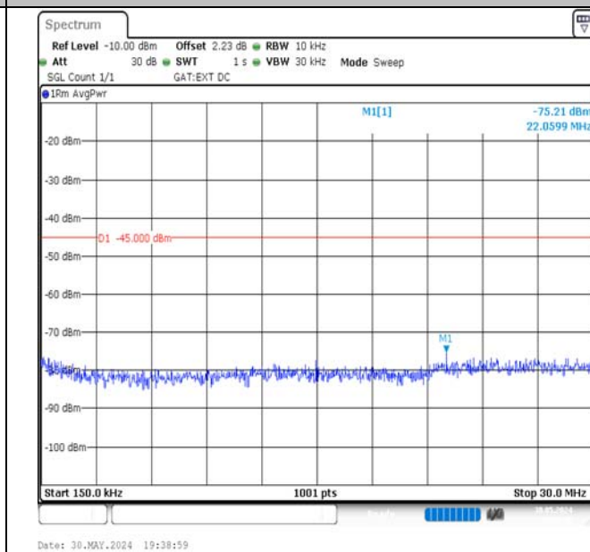
Band41-20MHz-QPSK-40620-1RB#99-0.15~30-PASS
