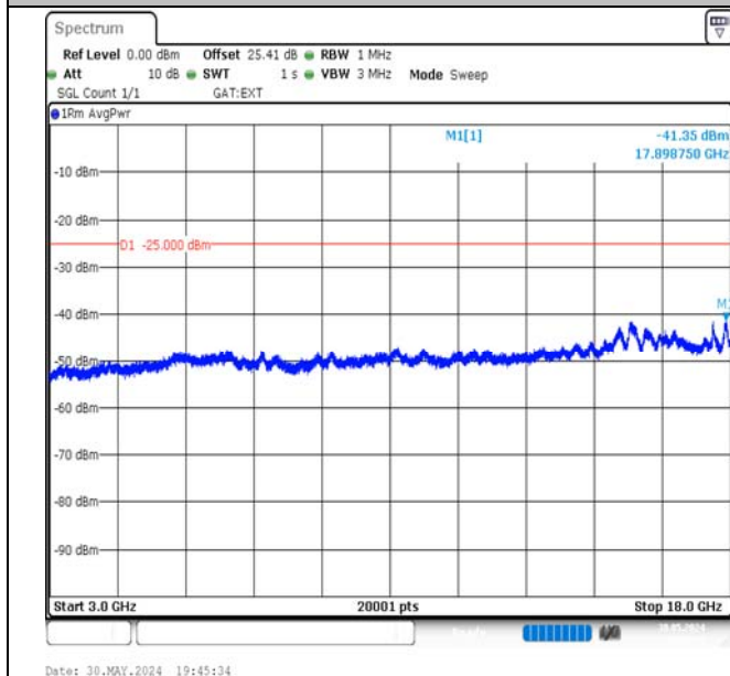
Band41-20MHz-16QAM-40620-100RB#0-3000~18000-PASS
