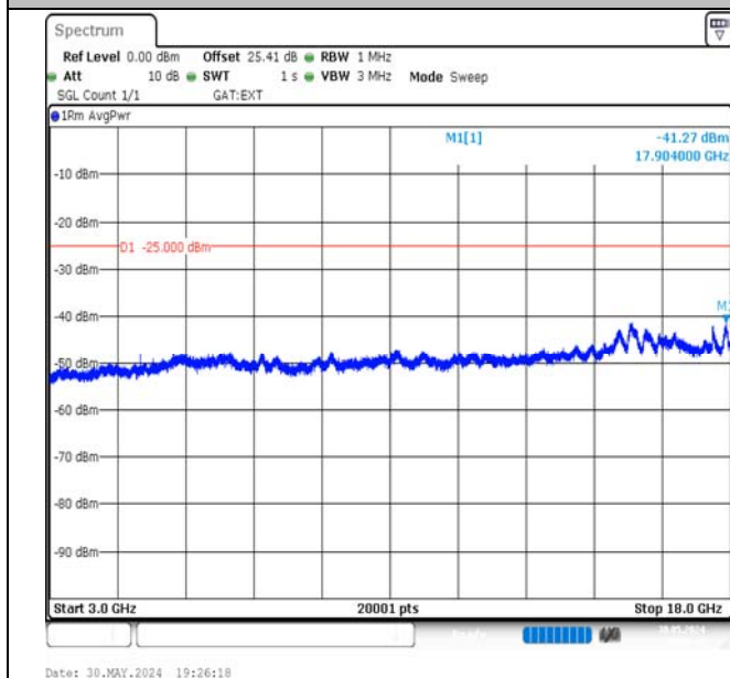
Band41-20MHz-16QAM-39750-1RB#0-3000~18000-PASS
