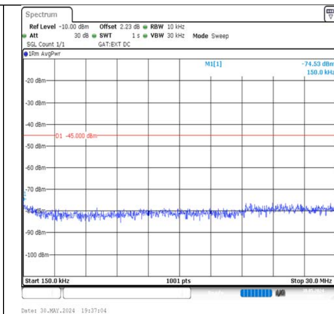
Band41-20MHz-16QAM-40620-1RB#0-0.15~30-PASS
