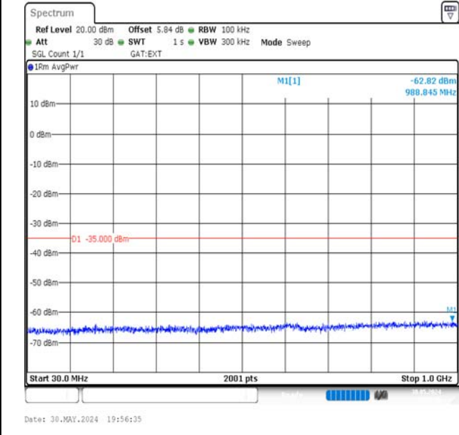
Band41-20MHz-16QAM-41490-100RB#0-30~1000-PASS
