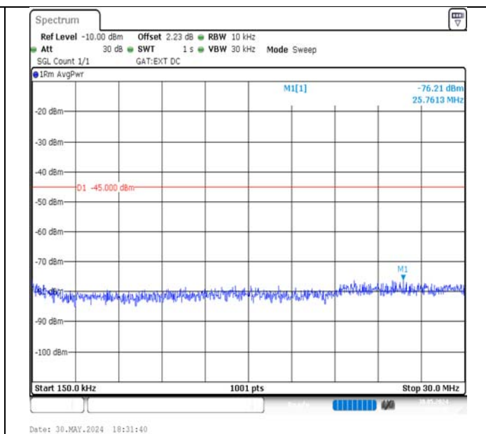
Band41-15MHz-16QAM-40620-1RB#74-0.15~30-PASS
