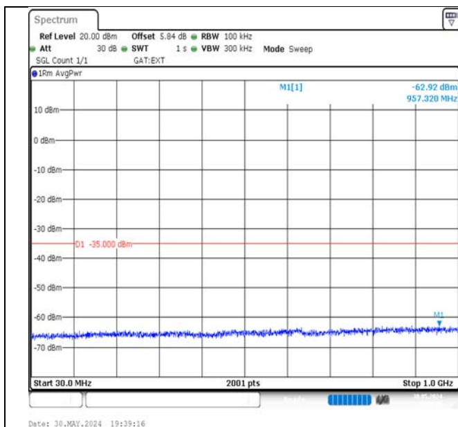
Band41-20MHz-QPSK-40620-1RB#99-30~1000-PASS
