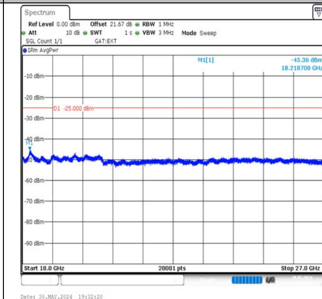
Band41-20MHz-QPSK-39750-100RB#0-18000~27000-PASS
