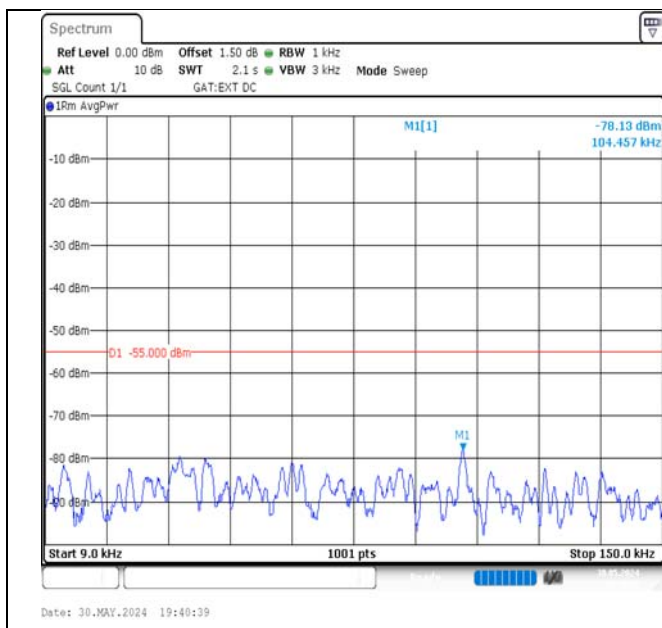
Band41-20MHz-16QAM-40620-1RB#99-0.009~0.15-PASS
