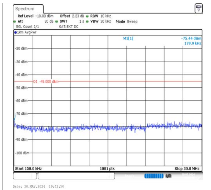
Band41-20MHz-QPSK-40620-100RB#0-0.15~30-PASS
