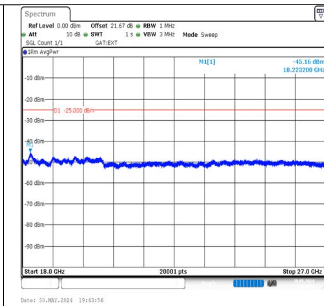
Band41-20MHz-QPSK-40620-100RB#0-18000~27000-PASS
