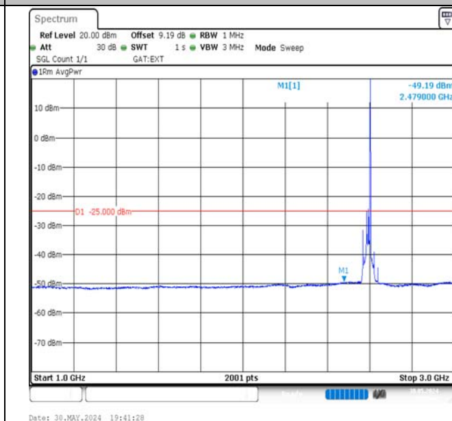
Band41-20MHz-16QAM-40620-1RB#99-1000~3000-PASS
