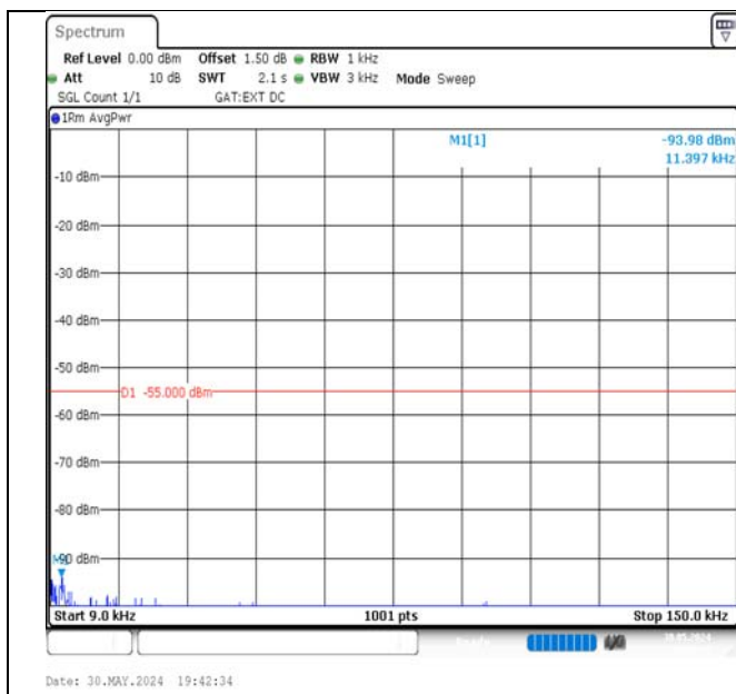
Band41-20MHz-QPSK-40620-100RB#0-0.009~0.15-PASS
