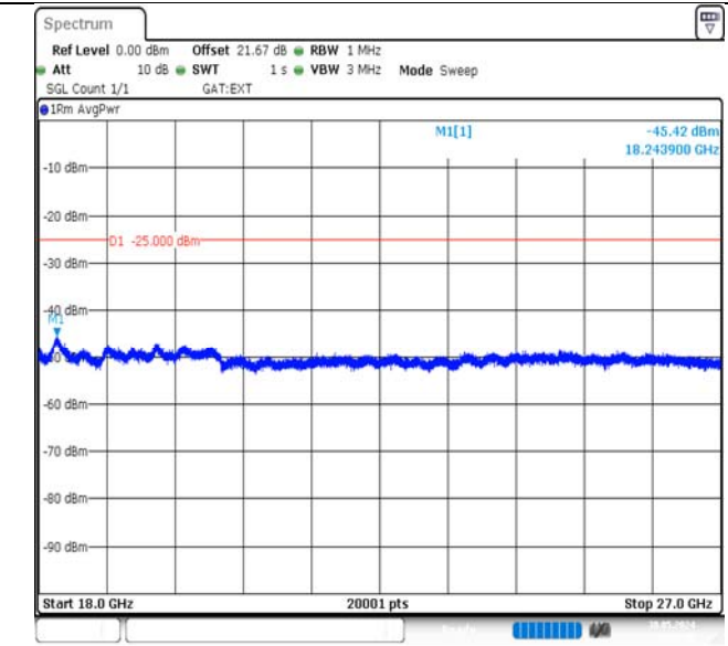
Band41-20MHz-QPSK-39750-1RB#99-18000~27000-PASS
