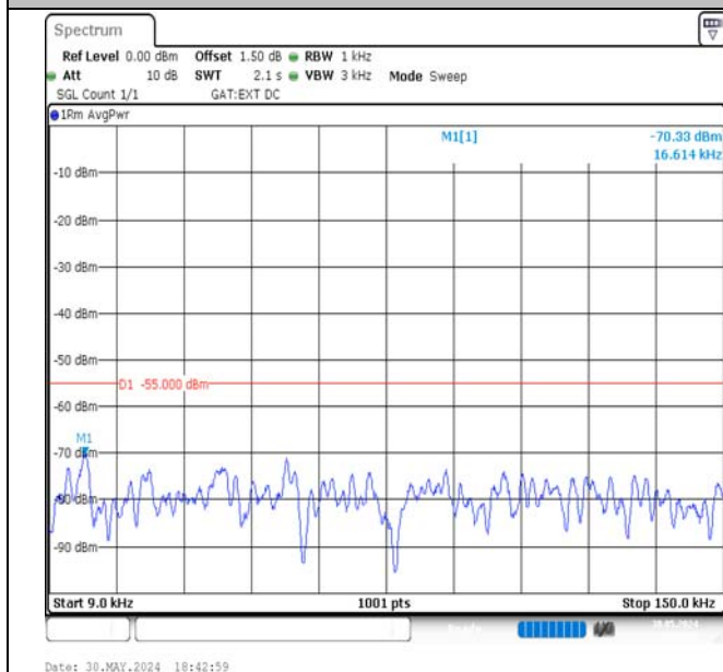
Band41-15MHz-16QAM-41515-1RB#74-0.009~0.15-PASS
