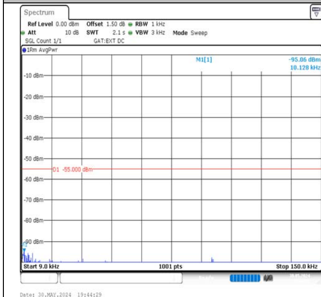
Band41-20MHz-16QAM-40620-100RB#0-0.009~0.15-PASS
