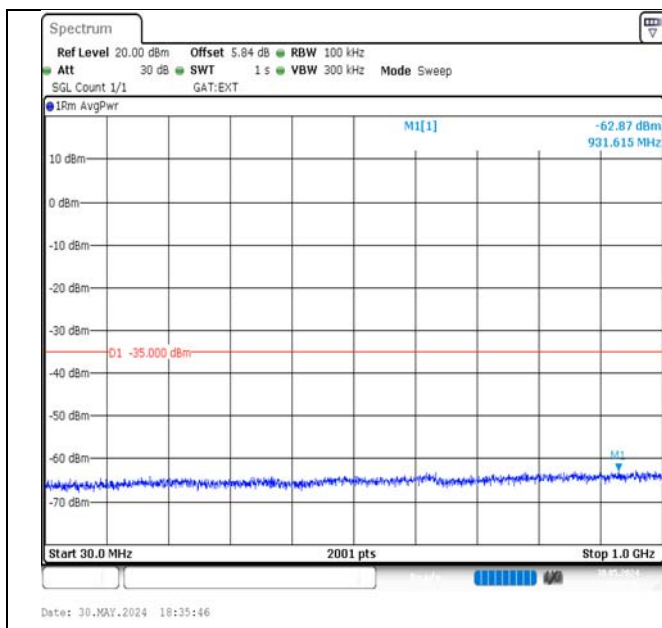
Band41-15MHz-16QAM-40620-75RB#0-30~1000-PASS
