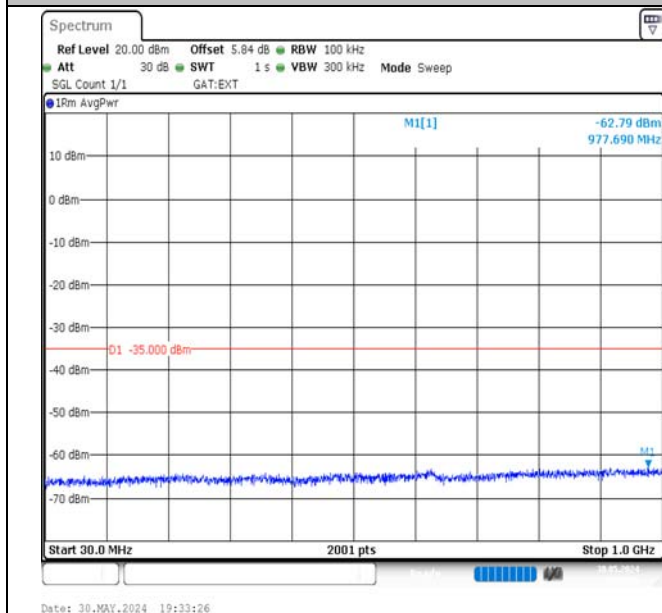
Band41-20MHz-16QAM-39750-100RB#0-30~1000-PASS
