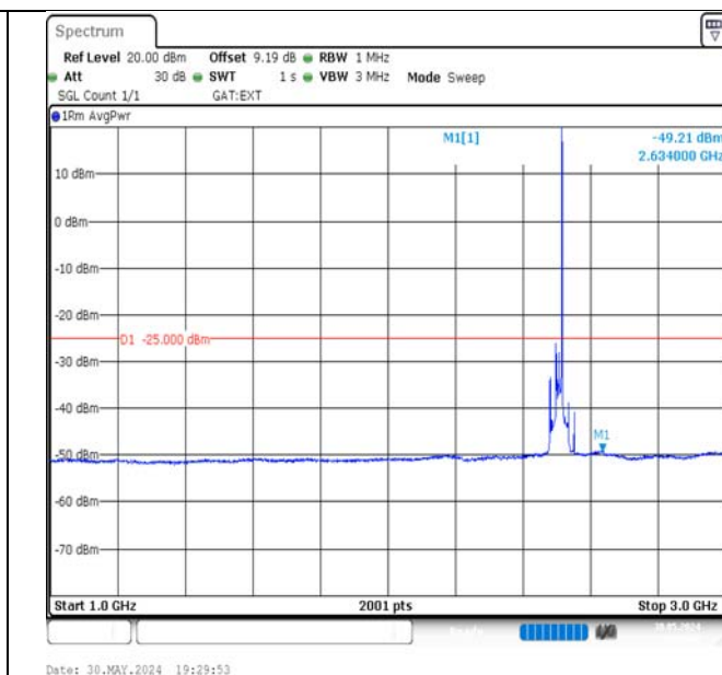
Band41-20MHz-16QAM-39750-1RB#99-1000~3000-PASS
