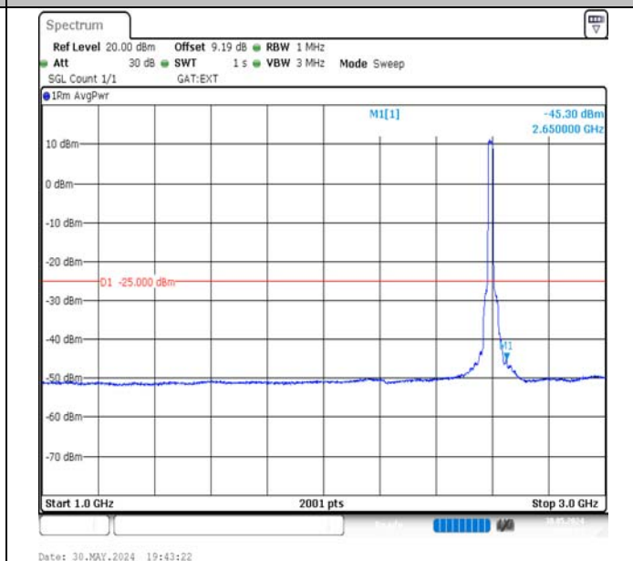
Band41-20MHz-QPSK-40620-100RB#0-1000~3000-PASS
