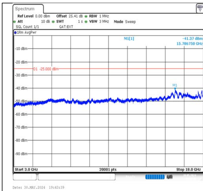
Band41-20MHz-QPSK-40620-100RB#0-3000~18000-PASS
