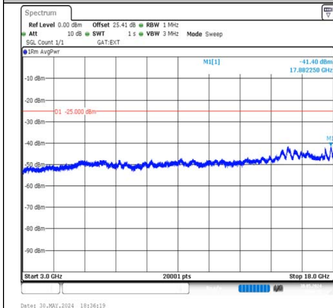
Band41-15MHz-16QAM-40620-75RB#0-3000~18000-PASS
