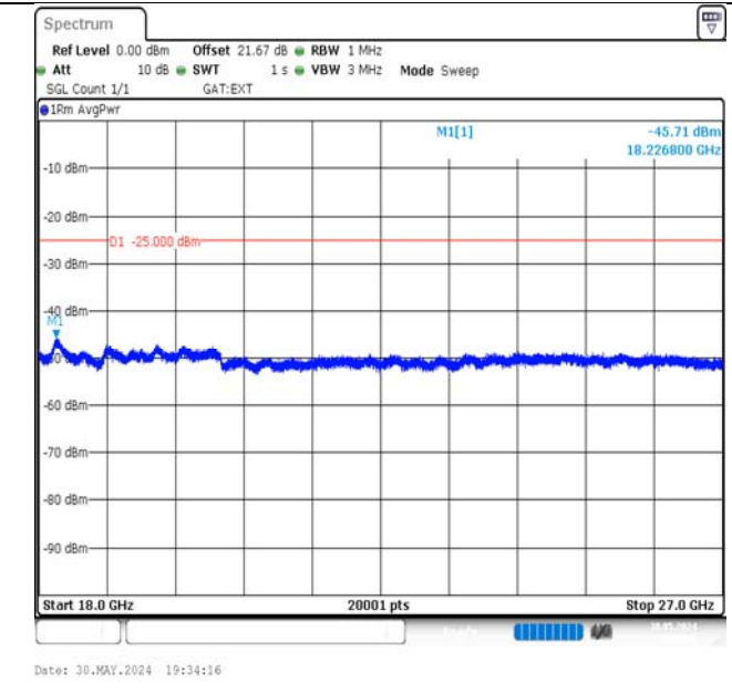
Band41-20MHz-16QAM-39750-100RB#0-18000~27000-PASS
