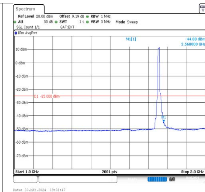
Band41-20MHz-QPSK-39750-100RB#0-1000~3000-PASS
