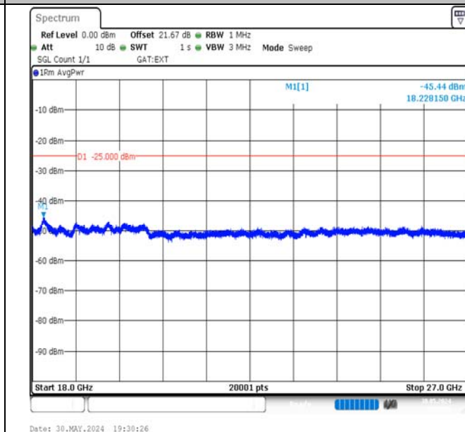
Band41-20MHz-16QAM-39750-1RB#99-18000~27000-PASS
