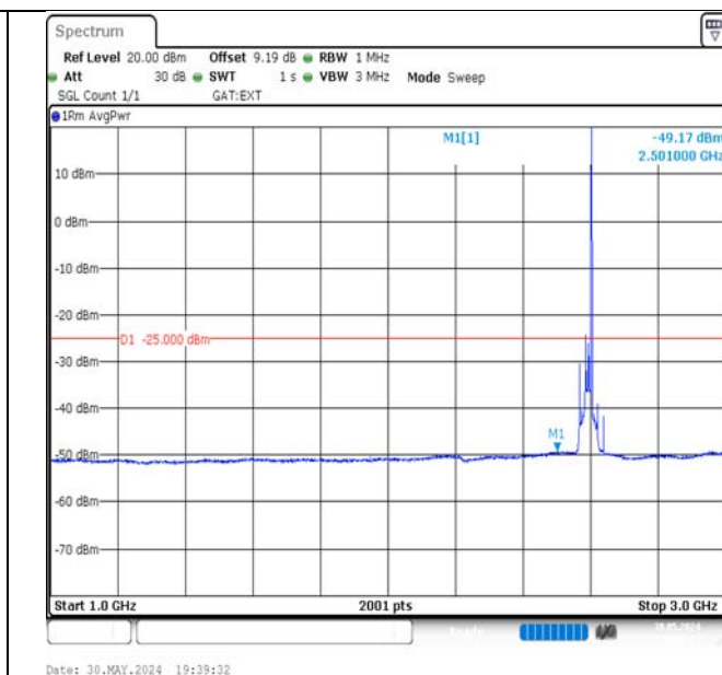
Band41-20MHz-QPSK-40620-1RB#99-1000~3000-PASS
