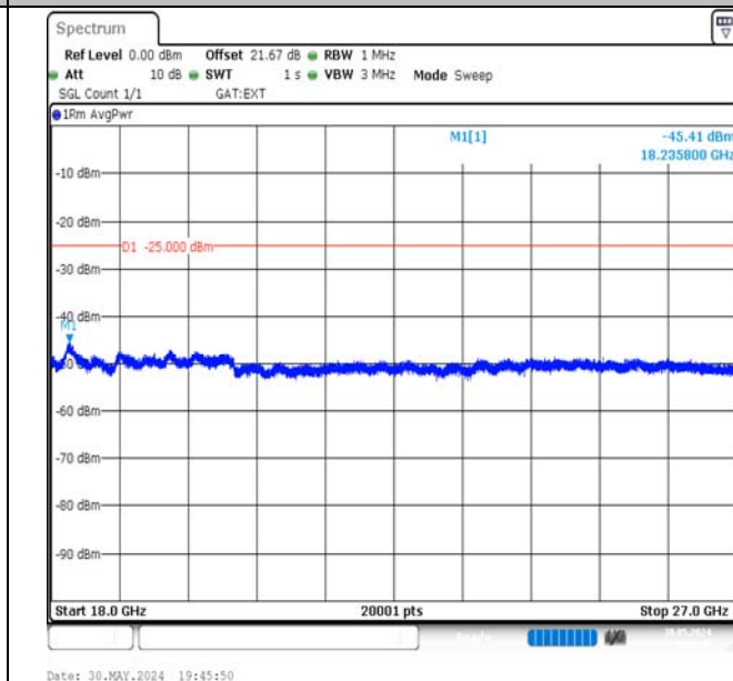
Band41-20MHz-16QAM-40620-100RB#0-18000~27000-PASS
