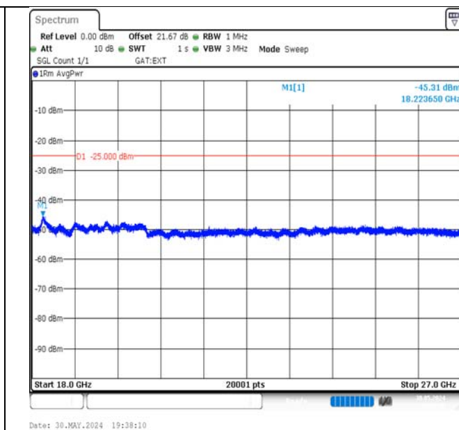
Band41-20MHz-16QAM-40620-1RB#0-18000~27000-PASS
