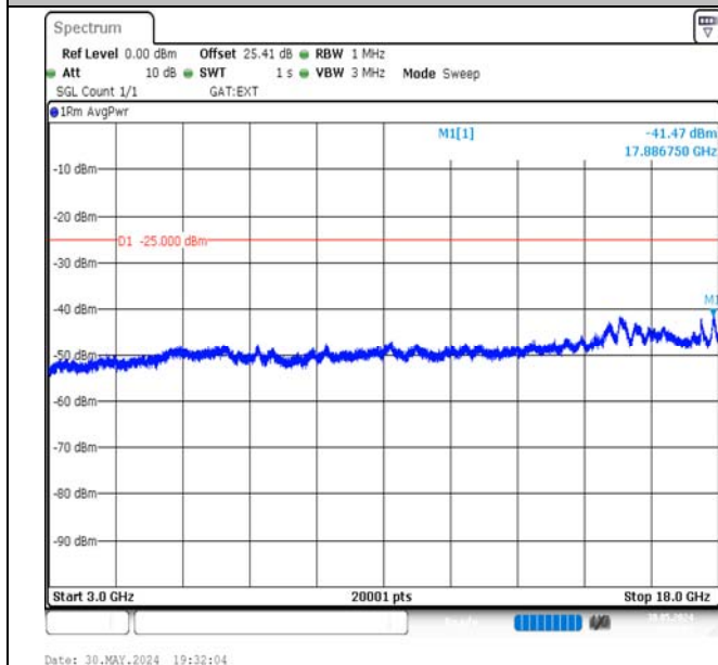
Band41-20MHz-QPSK-39750-100RB#0-3000~18000-PASS
