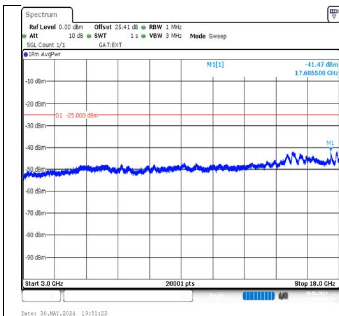
Band41-20MHz-QPSK-41490-1RB#99-3000~18000-PASS
