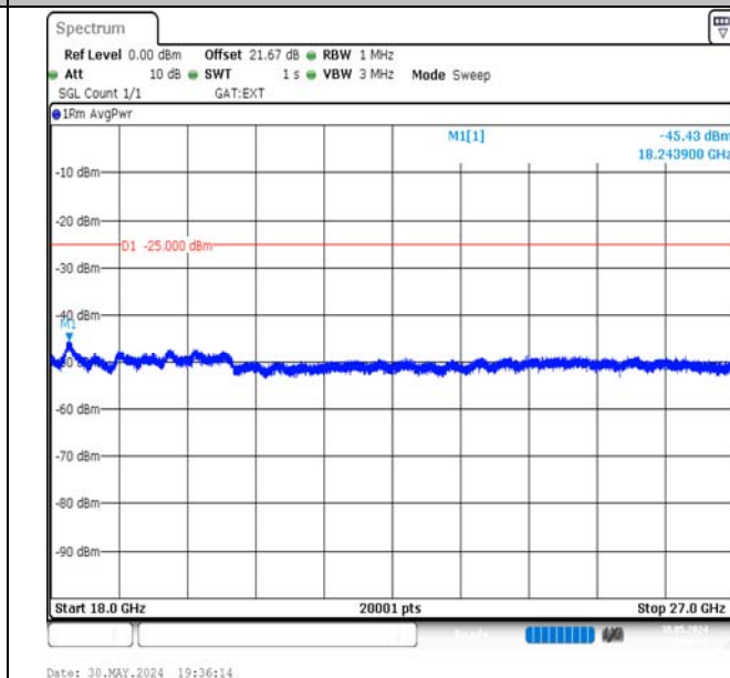
Band41-20MHz-QPSK-40620-1RB#0-18000~27000-PASS
