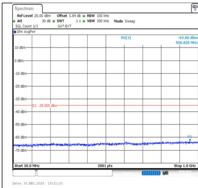
Band41-20MHz-QPSK-39750-100RB#0-30~1000-PASS
