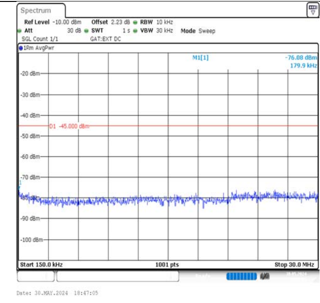
Band41-15MHz-16QAM-41515-75RB#0-0.15~30-PASS
