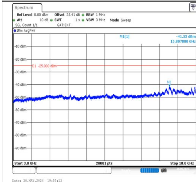
Band41-20MHz-QPSK-41490-100RB#0-3000~18000-PASS
