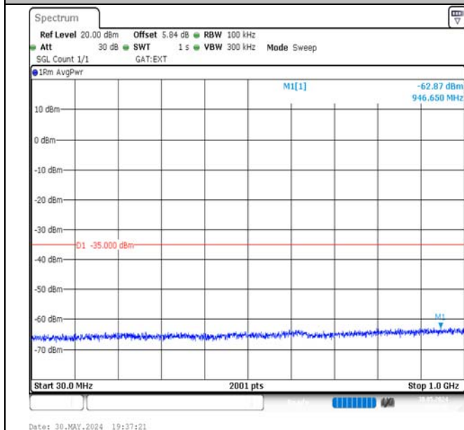
Band41-20MHz-16QAM-40620-1RB#0-30~1000-PASS
