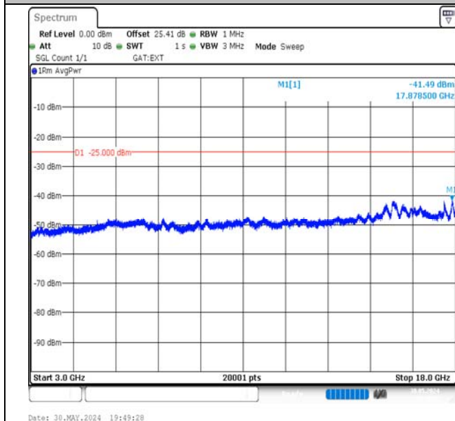
Band41-20MHz-16QAM-41490-1RB#0-3000~18000-PASS
