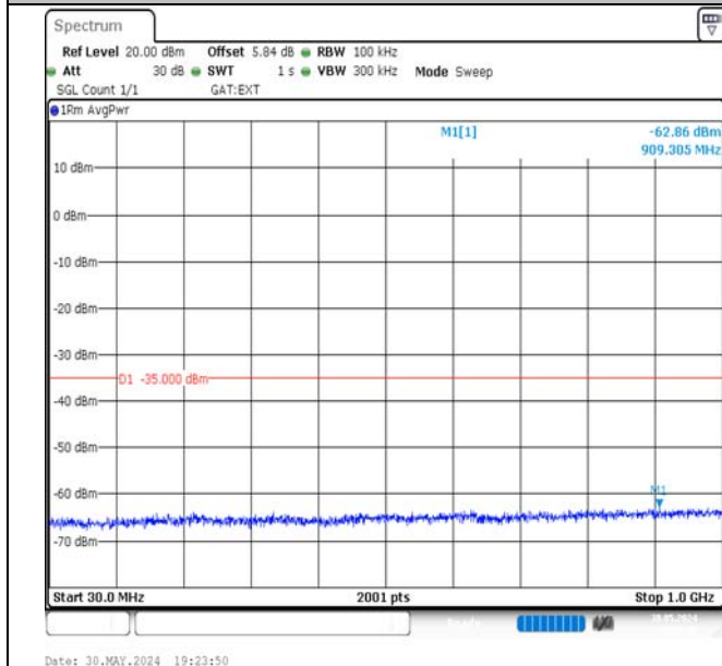
Band41-20MHz-QPSK-39750-1RB#0-30~1000-PASS
