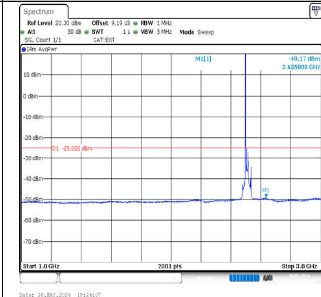
Band41-20MHz-QPSK-39750-1RB#0-1000~3000-PASS
