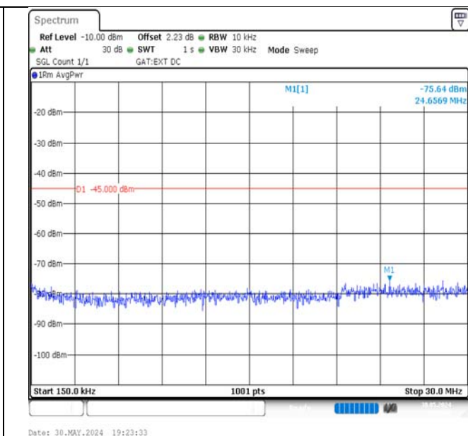
Band41-20MHz-QPSK-39750-1RB#0-0.15~30-PASS
