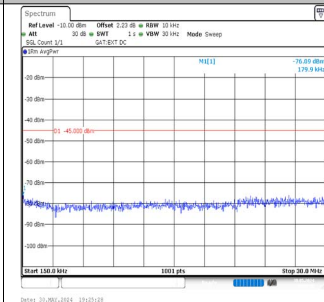
Band41-20MHz-16QAM-39750-1RB#0-0.15~30-PASS
