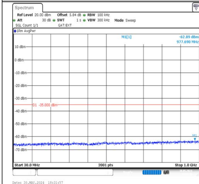
Band41-15MHz-16QAM-40620-1RB#74-30~1000-PASS
