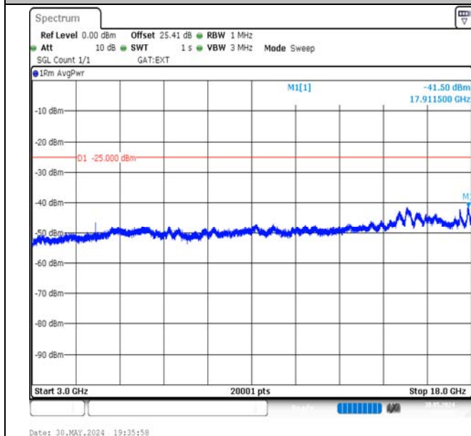
Band41-20MHz-QPSK-40620-1RB#0-3000~18000-PASS
