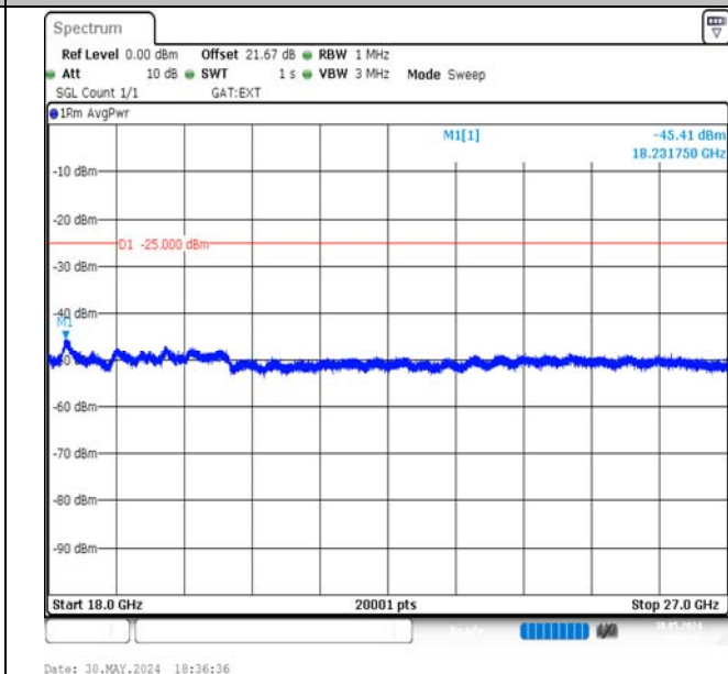
Band41-15MHz-16QAM-40620-75RB#0-18000~27000-PASS
