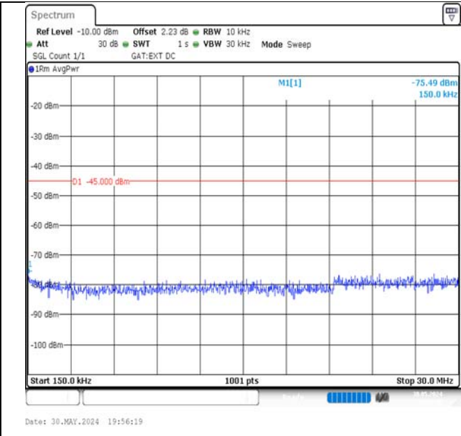
Band41-20MHz-16QAM-41490-100RB#0-0.15~30-PASS
