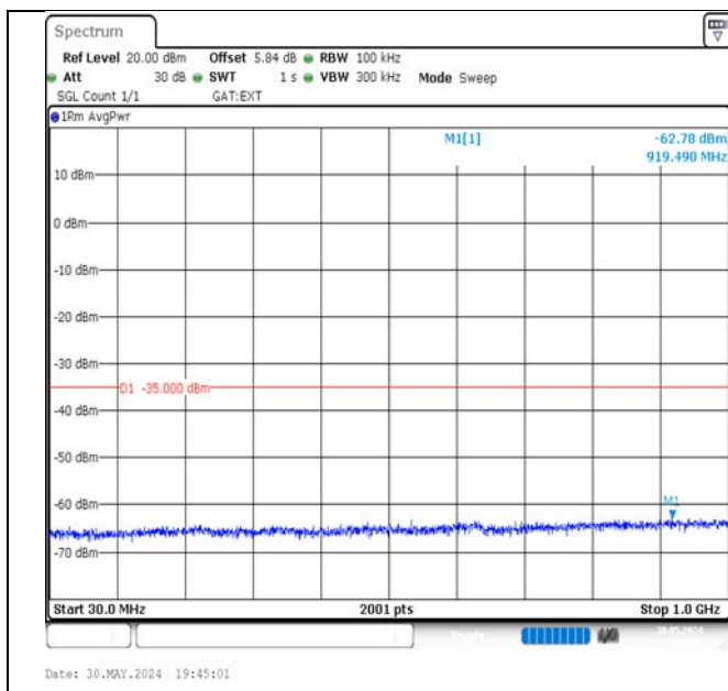
Band41-20MHz-16QAM-40620-100RB#0-30~1000-PASS
