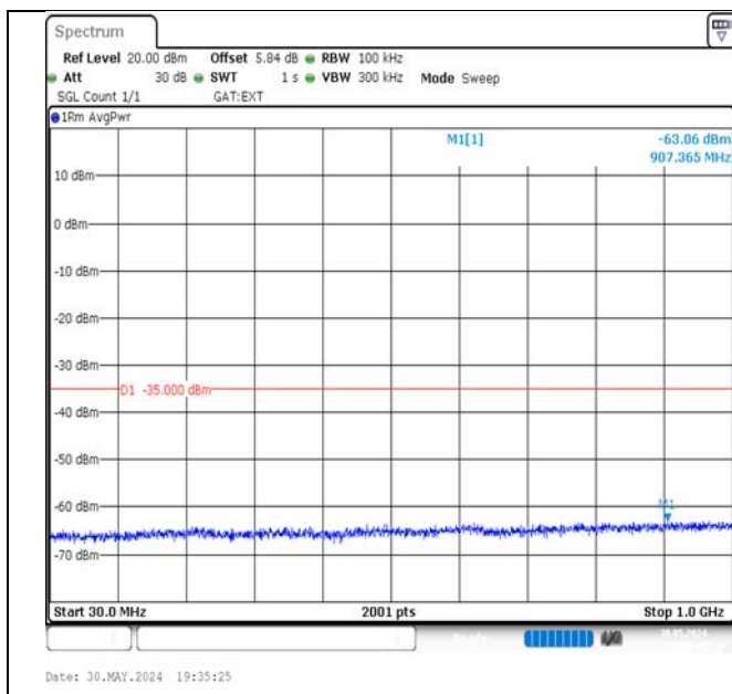
Band41-20MHz-QPSK-40620-1RB#0-30~1000-PASS
