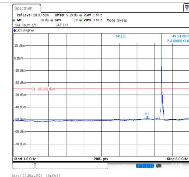
Band41-15MHz-16QAM-41515-1RB#0-1000~3000-PASS
