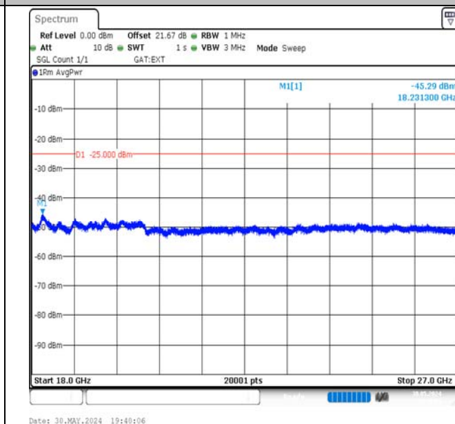
Band41-20MHz-QPSK-40620-1RB#99-18000~27000-PASS
