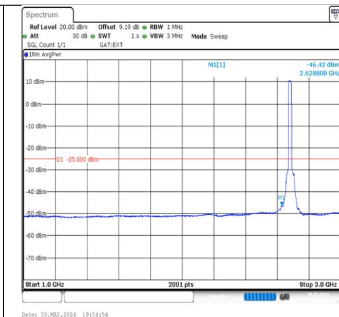
Band41-20MHz-QPSK-41490-100RB#0-1000~3000-PASS
