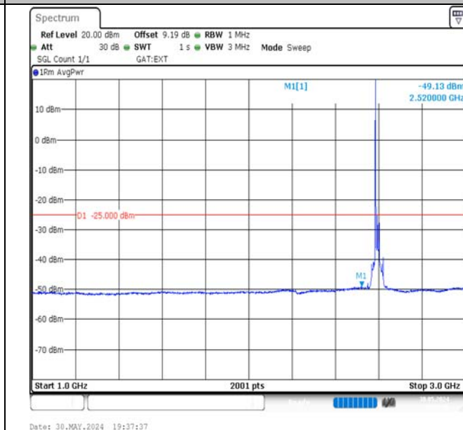
Band41-20MHz-16QAM-40620-1RB#0-1000~3000-PASS
