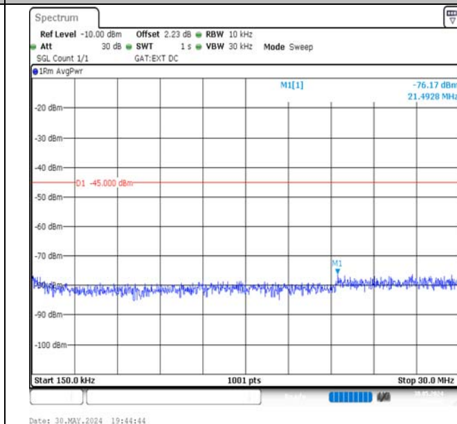
Band41-20MHz-16QAM-40620-100RB#0-0.15~30-PASS
