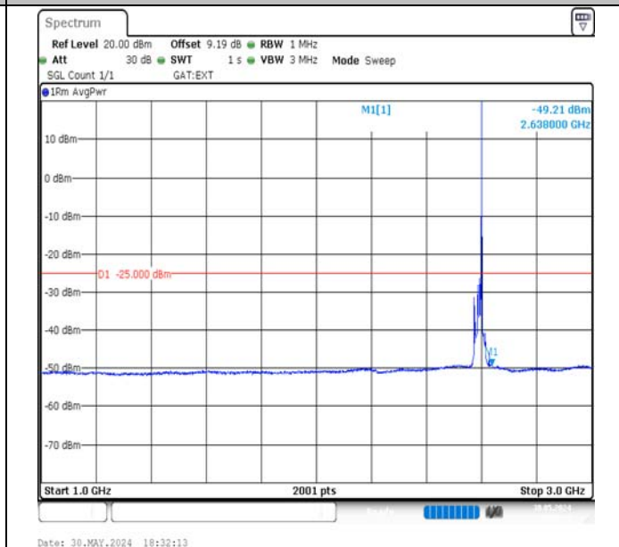
Band41-15MHz-16QAM-40620-1RB#74-1000~3000-PASS
