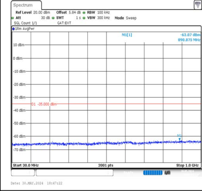
Band41-15MHz-16QAM-41515-75RB#0-30~1000-PASS
