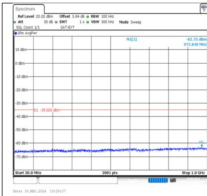
Band41-20MHz-16QAM-39750-1RB#99-30~1000-PASS
