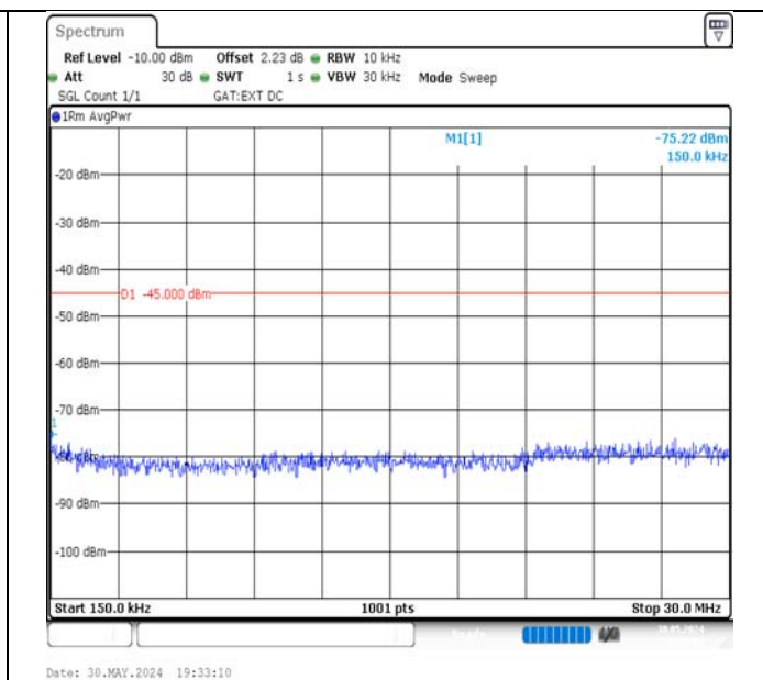
Band41-20MHz-16QAM-39750-100RB#0-0.15~30-PASS
