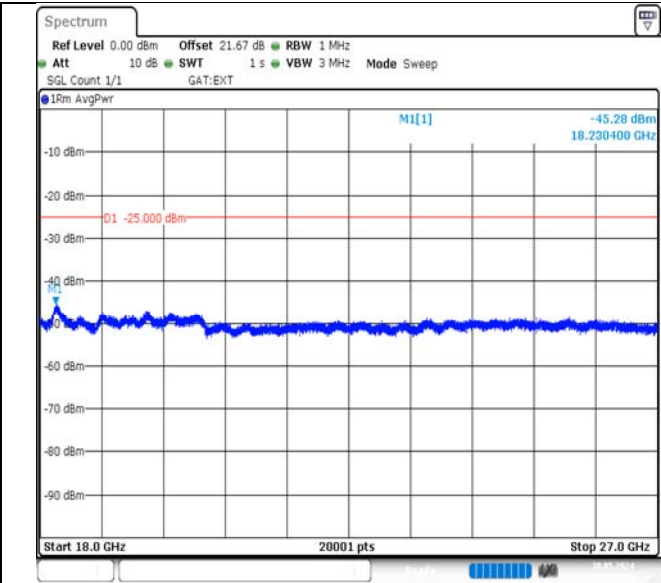
Band41-15MHz-16QAM-40620-1RB#74-18000~27000-PASS
