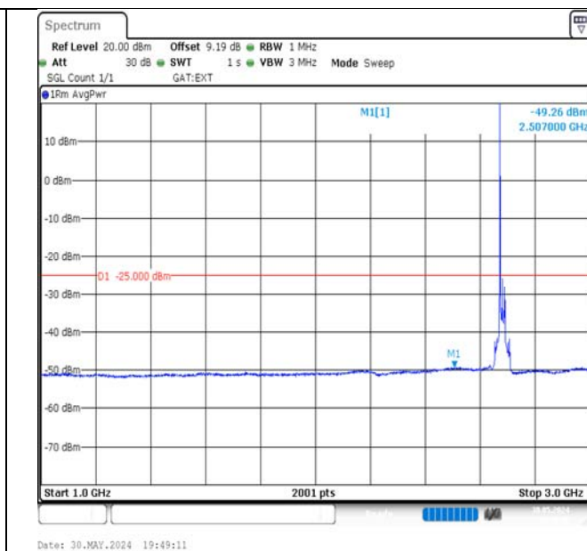
Band41-20MHz-16QAM-41490-1RB#0-1000~3000-PASS
