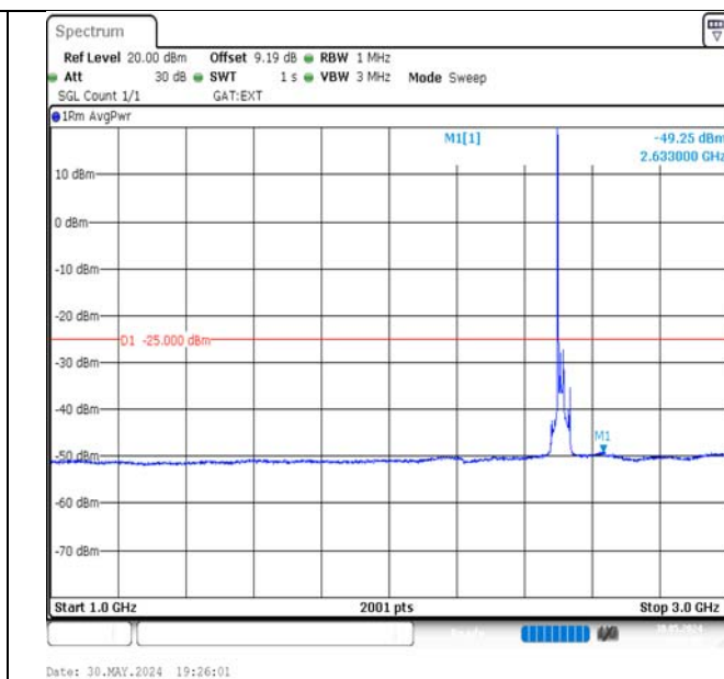
Band41-20MHz-16QAM-39750-1RB#0-1000~3000-PASS
