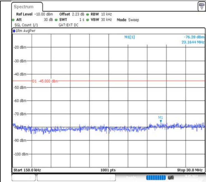
Band41-20MHz-QPSK-39750-1RB#99-0.15~30-PASS
