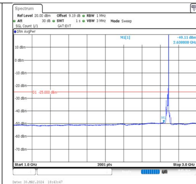
Band41-15MHz-16QAM-41515-1RB#74-1000~3000-PASS
