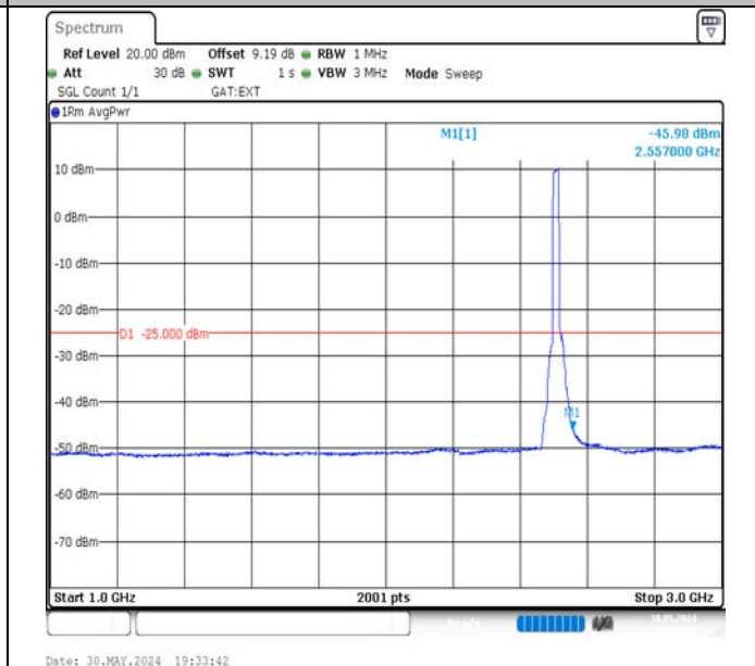
Band41-20MHz-16QAM-39750-100RB#0-1000~3000-PASS
