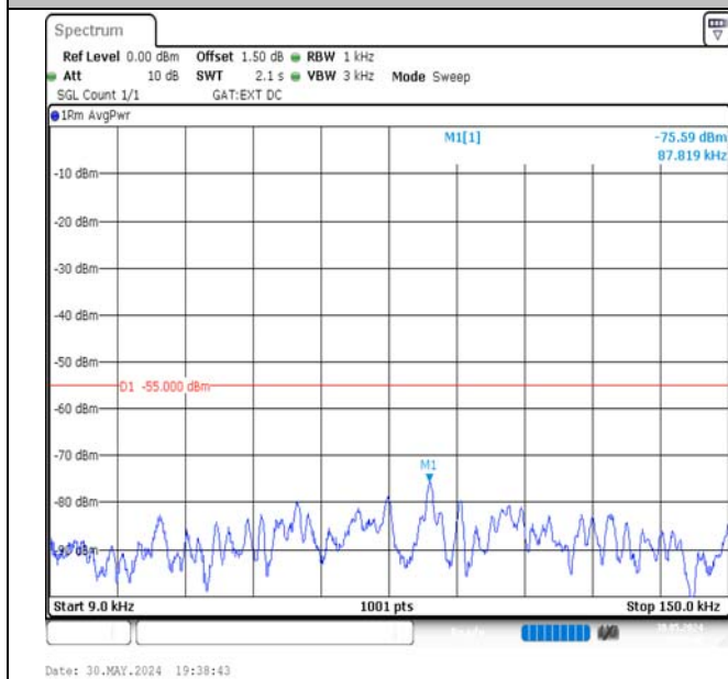
Band41-20MHz-QPSK-40620-1RB#99-0.009~0.15-PASS
