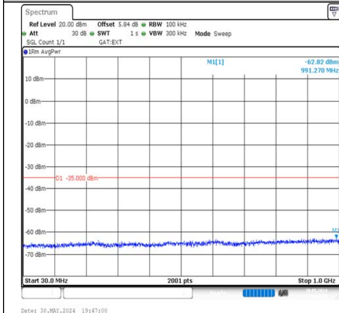
Band41-20MHz-QPSK-41490-1RB#0-30~1000-PASS
