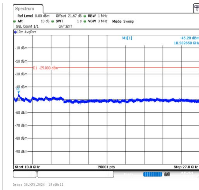
Band41-15MHz-16QAM-41515-75RB#0-18000~27000-PASS
