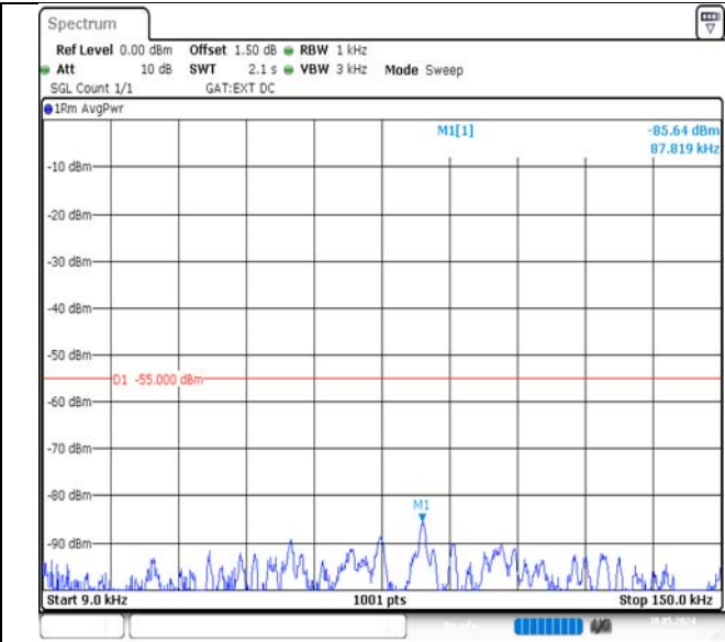
Band41-20MHz-QPSK-39750-1RB#99-0.009~0.15-PASS
