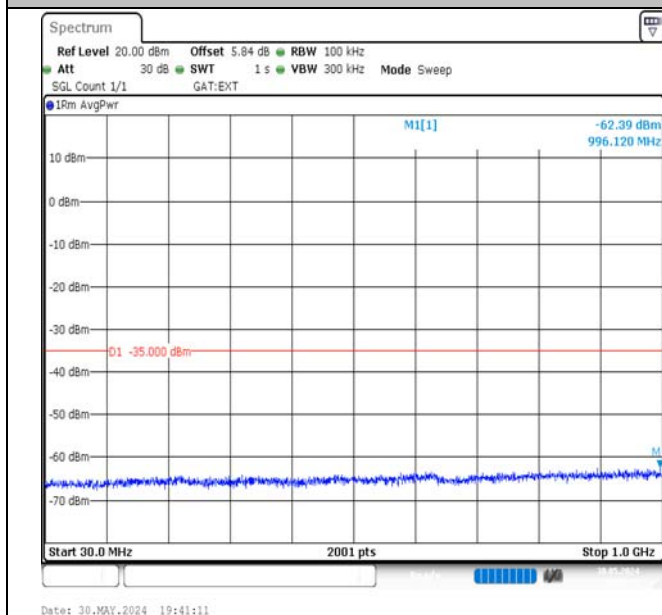
Band41-20MHz-16QAM-40620-1RB#99-30~1000-PASS
