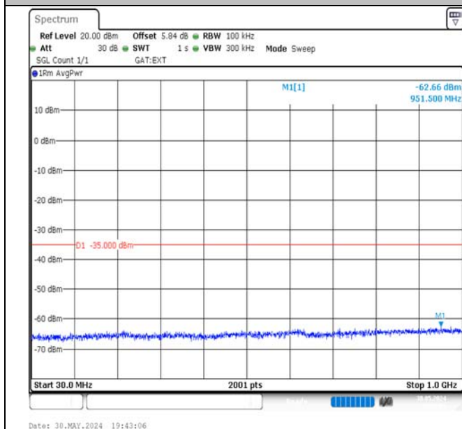
Band41-20MHz-QPSK-40620-100RB#0-30~1000-PASS
