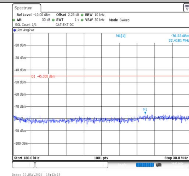
Band41-15MHz-16QAM-41515-1RB#74-0.15~30-PASS
