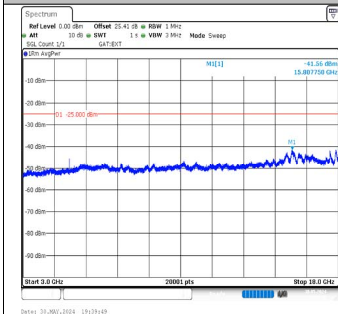
Band41-20MHz-QPSK-40620-1RB#99-3000~18000-PASS
