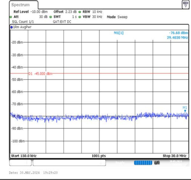
Band41-20MHz-16QAM-39750-1RB#99-0.15~30-PASS
