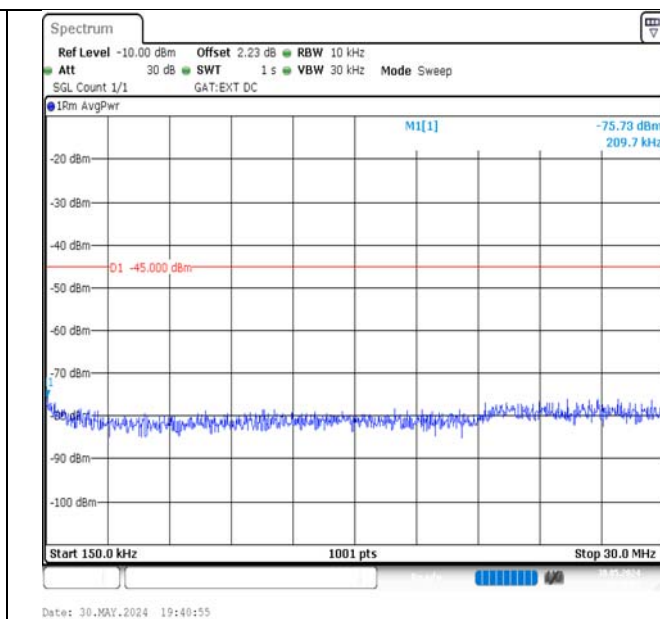
Band41-20MHz-16QAM-40620-1RB#99-0.15~30-PASS
