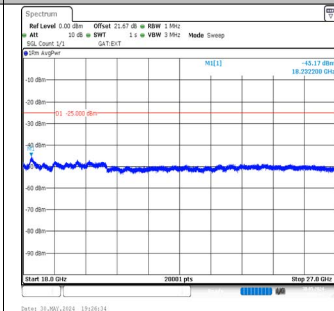
Band41-20MHz-16QAM-39750-1RB#0-18000~27000-PASS
