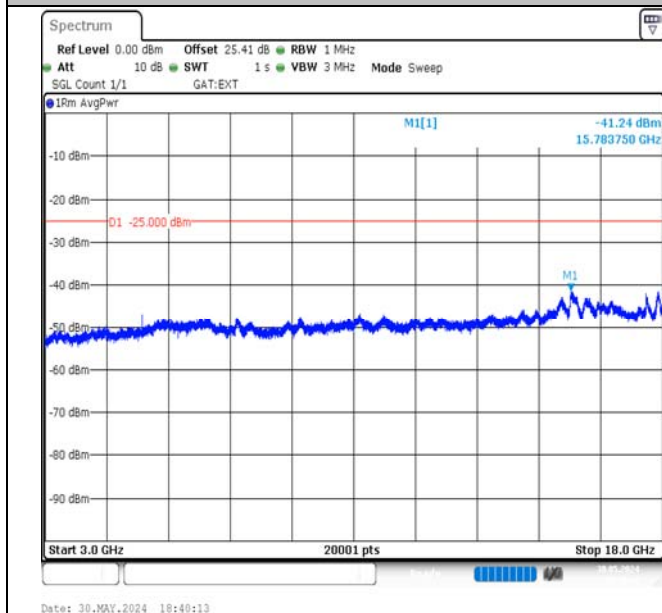
Band41-15MHz-16QAM-41515-1RB#0-3000~18000-PASS
