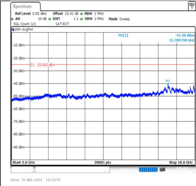
Band41-20MHz-16QAM-39750-100RB#0-3000~18000-PASS
