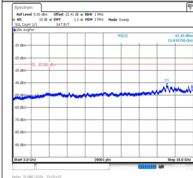
Band41-20MHz-16QAM-39750-1RB#99-3000~18000-PASS
