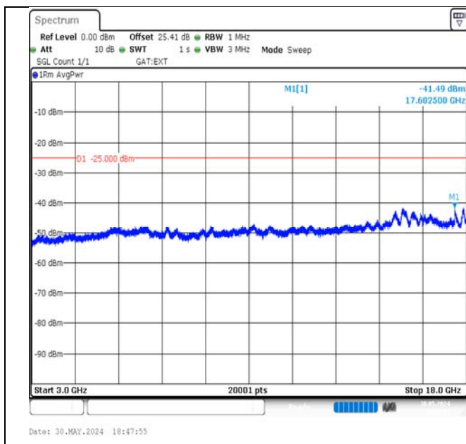
Band41-15MHz-16QAM-41515-75RB#0-3000~18000-PASS
