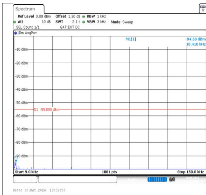
Band41-20MHz-16QAM-39750-100RB#0-0.009~0.15-PASS
