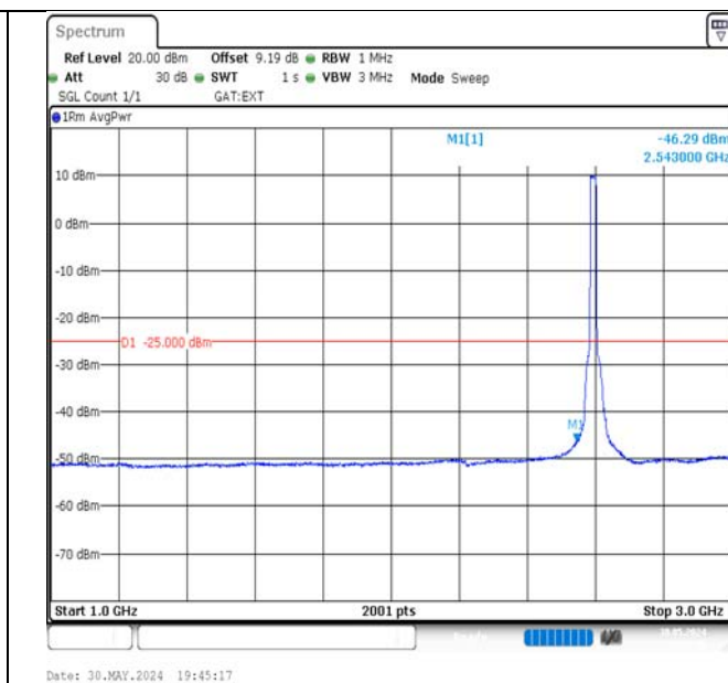
Band41-20MHz-16QAM-40620-100RB#0-1000~3000-PASS
