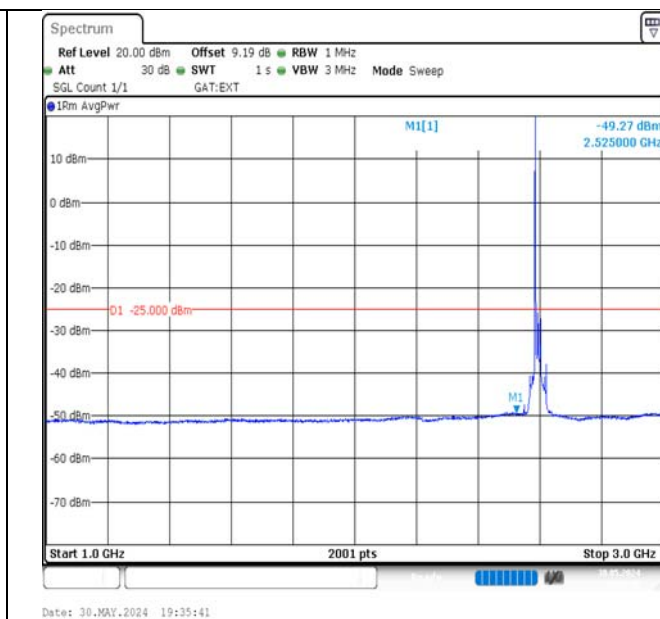
Band41-20MHz-QPSK-40620-1RB#0-1000~3000-PASS
