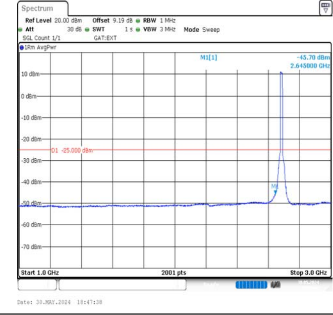
Band41-15MHz-16QAM-41515-75RB#0-1000~3000-PASS
