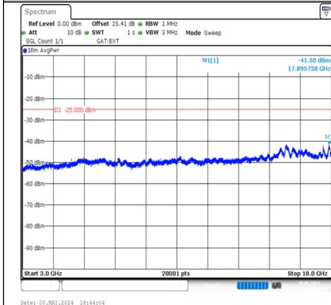
Band41-15MHz-16QAM-41515-1RB#74-3000~18000-PASS
