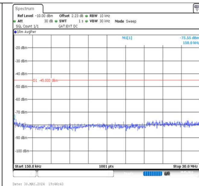
Band41-20MHz-QPSK-41490-1RB#0-0.15~30-PASS
