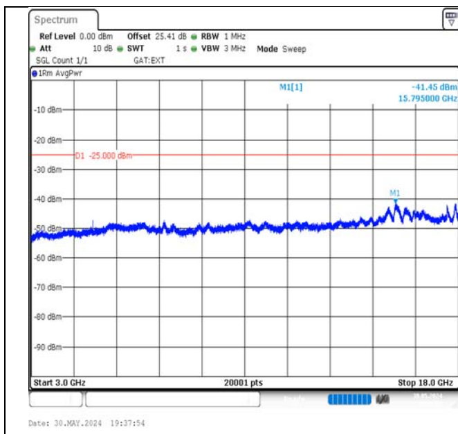
Band41-20MHz-16QAM-40620-1RB#0-3000~18000-PASS
