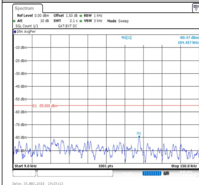
Band41-20MHz-16QAM-39750-1RB#0-0.009~0.15-PASS
