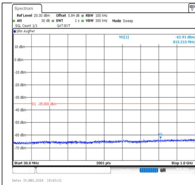
Band41-15MHz-16QAM-41515-1RB#74-30~1000-PASS
