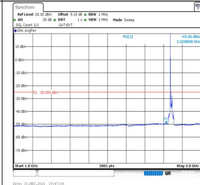
Band41-20MHz-QPSK-41490-1RB#0-1000~3000-PASS
