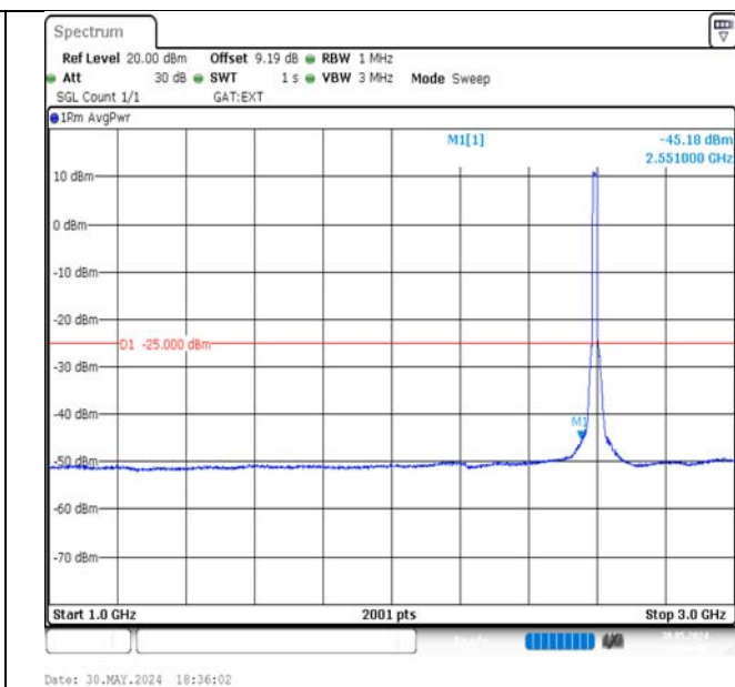
Band41-15MHz-16QAM-40620-75RB#0-1000~3000-PASS
