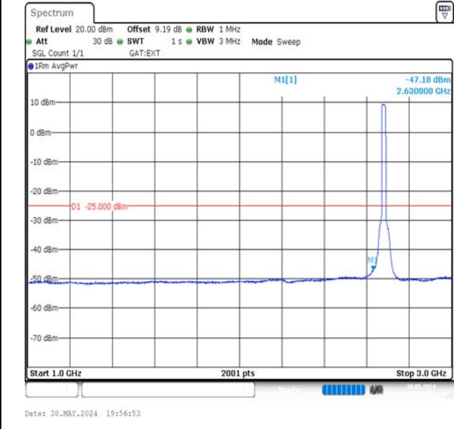
Band41-20MHz-16QAM-41490-100RB#0-1000~3000-PASS
