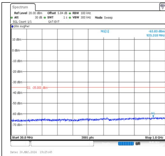
Band41-20MHz-16QAM-39750-1RB#0-30~1000-PASS
