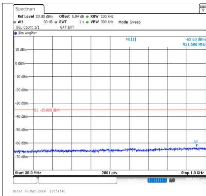
Band41-20MHz-QPSK-41490-100RB#0-30~1000-PASS
