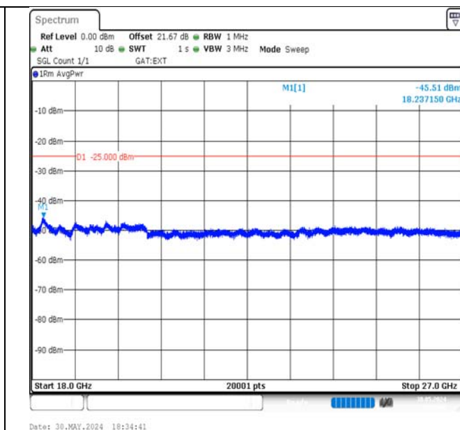
Band41-15MHz-QPSK-40620-75RB#0-18000~27000-PASS
