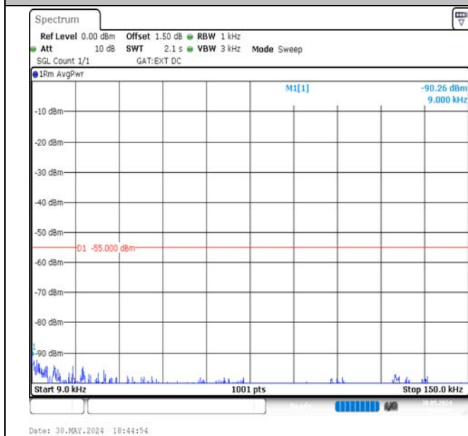
Band41-15MHz-QPSK-41515-75RB#0-0.009~0.15-PASS
