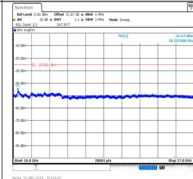
Band41-10MHz-16QAM-41540-1RB#0-18000~27000-PASS
