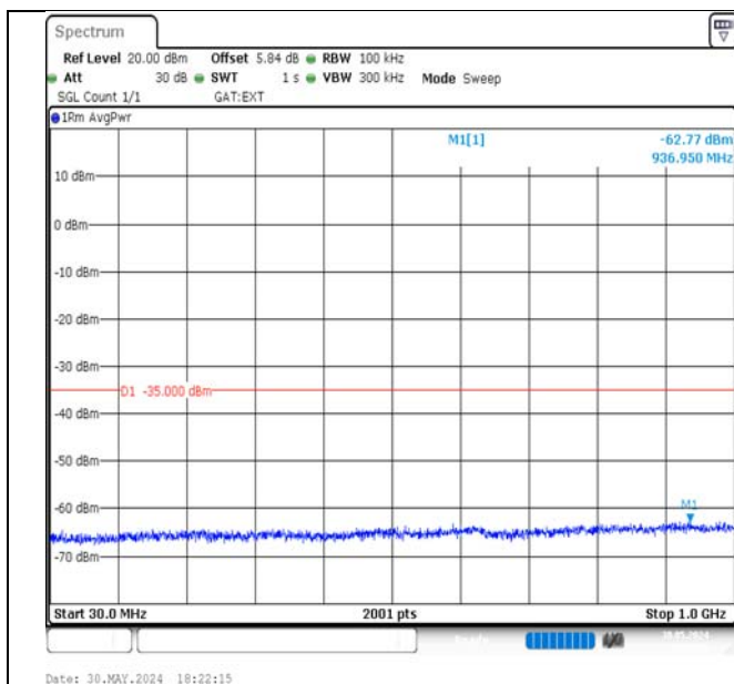
Band41-15MHz-QPSK-39725-75RB#0-30~1000-PASS
