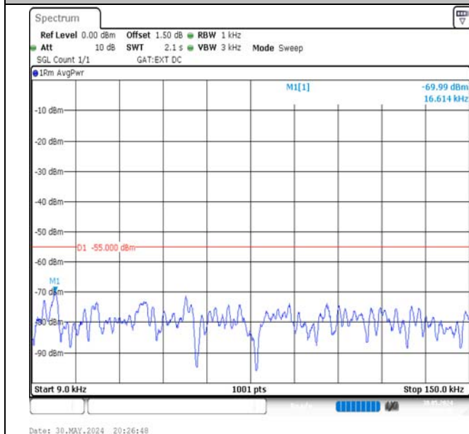
Band41-10MHz-16QAM-41540-1RB#49-0.009~0.15-PASS
