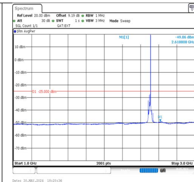
Band41-15MHz-16QAM-39725-1RB#74-1000~3000-PASS
