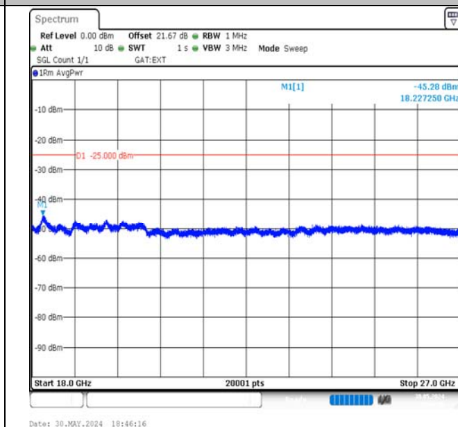
Band41-15MHz-QPSK-41515-75RB#0-18000~27000-PASS
