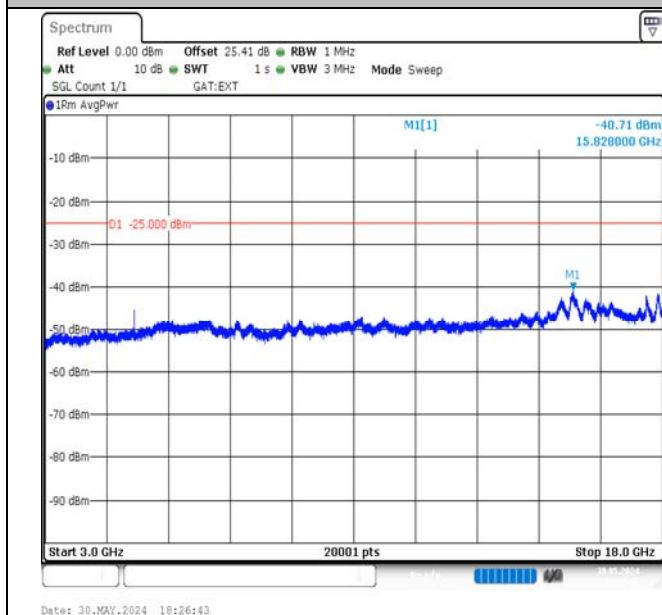
Band41-15MHz-QPSK-40620-1RB#0-3000~18000-PASS
