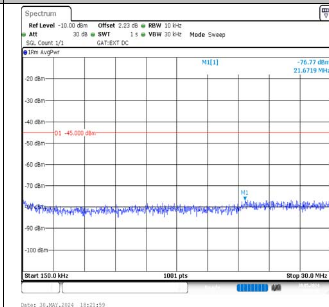
Band41-15MHz-QPSK-39725-75RB#0-0.15~30-PASS
