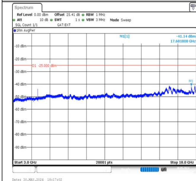
Band41-15MHz-16QAM-39725-1RB#0-3000~18000-PASS
