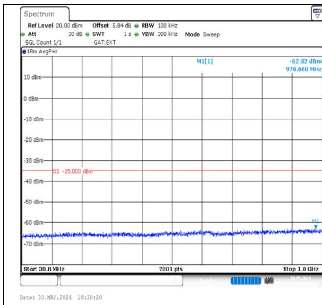
Band41-15MHz-16QAM-39725-1RB#74-30~1000-PASS
