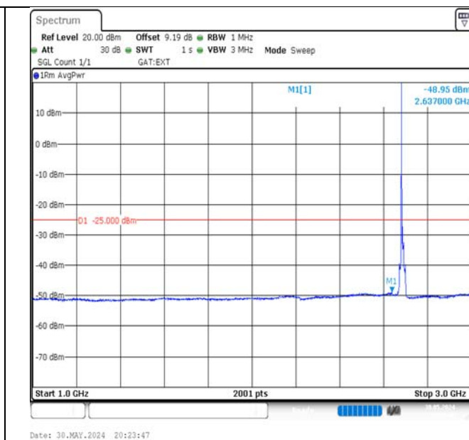
Band41-10MHz-16QAM-41540-1RB#0-1000~3000-PASS
