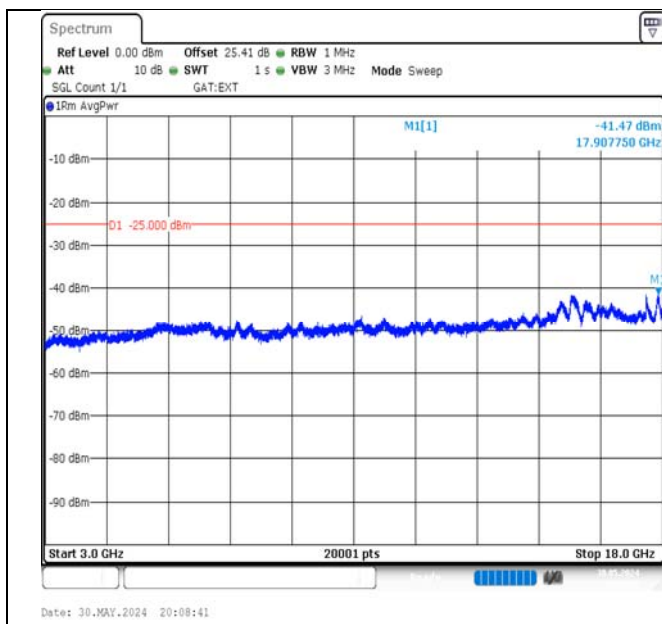
Band41-10MHz-16QAM-39700-50RB#0-3000~18000-PASS
