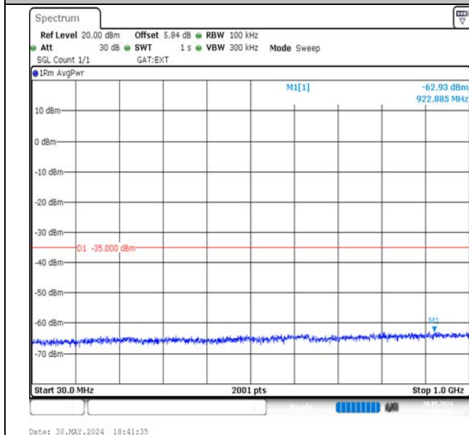
Band41-15MHz-QPSK-41515-1RB#74-30~1000-PASS
