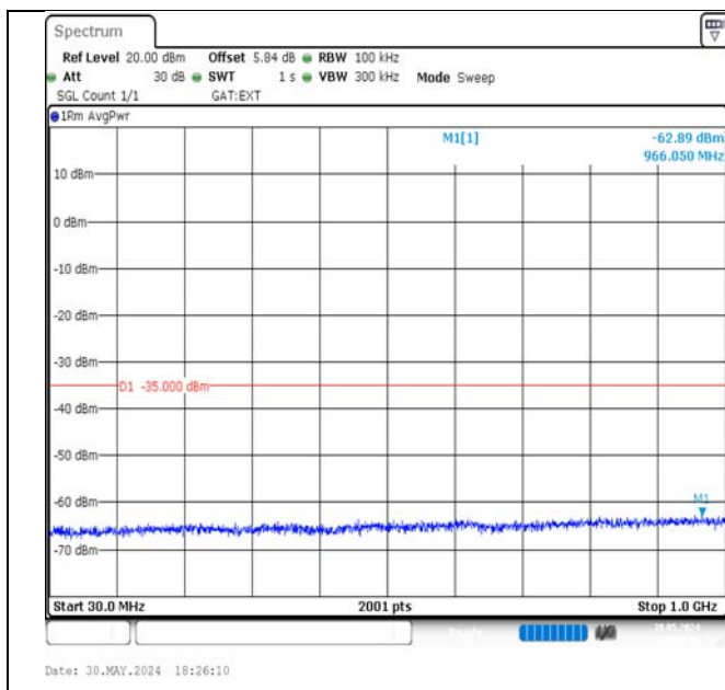
Band41-15MHz-QPSK-40620-1RB#0-30~1000-PASS
