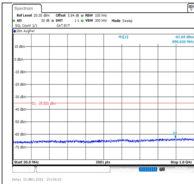
Band41-10MHz-16QAM-39700-1RB#49-30~1000-PASS
