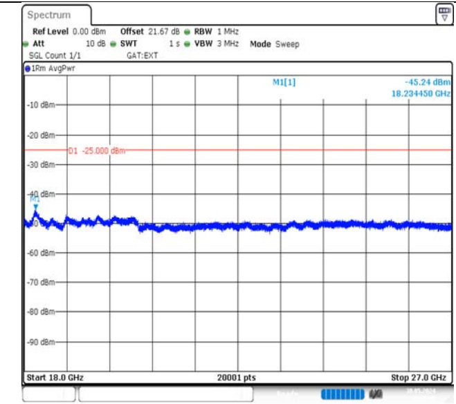
Band41-10MHz-16QAM-40620-1RB#0-18000~27000-PASS
