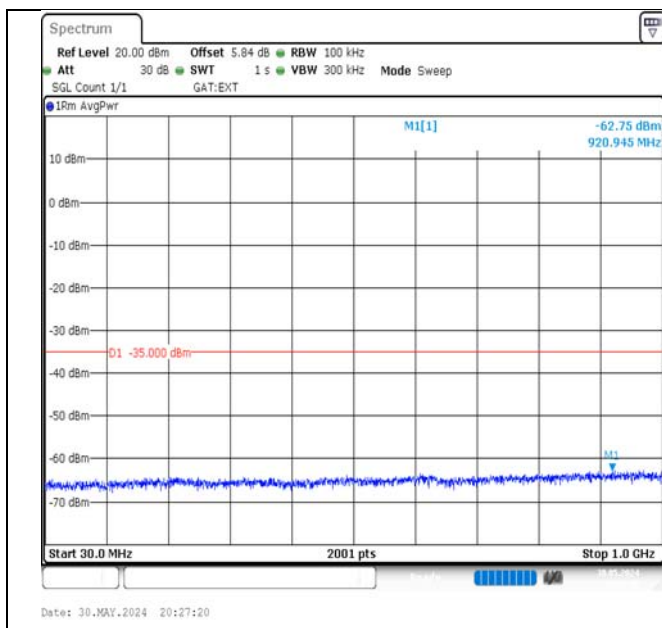
Band41-10MHz-16QAM-41540-1RB#49-30~1000-PASS
