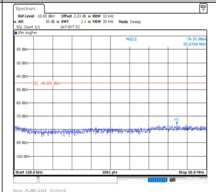
Band41-10MHz-16QAM-39700-1RB#49-0.15~30-PASS
