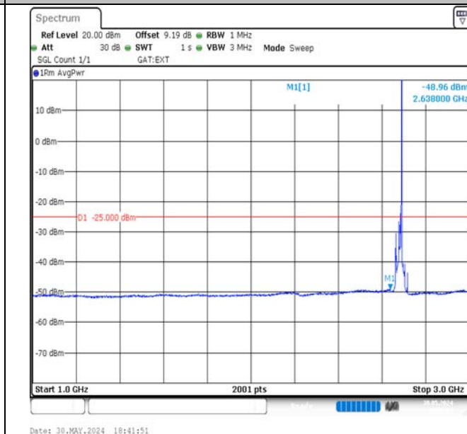
Band41-15MHz-QPSK-41515-1RB#74-1000~3000-PASS
