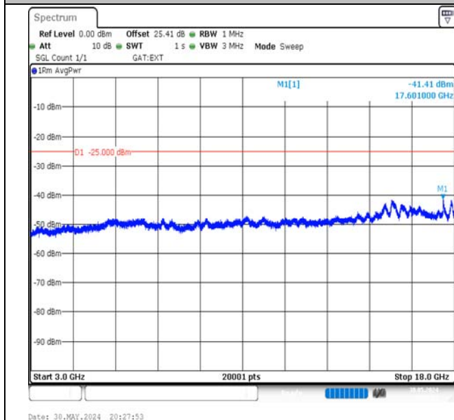
Band41-10MHz-16QAM-41540-1RB#49-3000~18000-PASS
