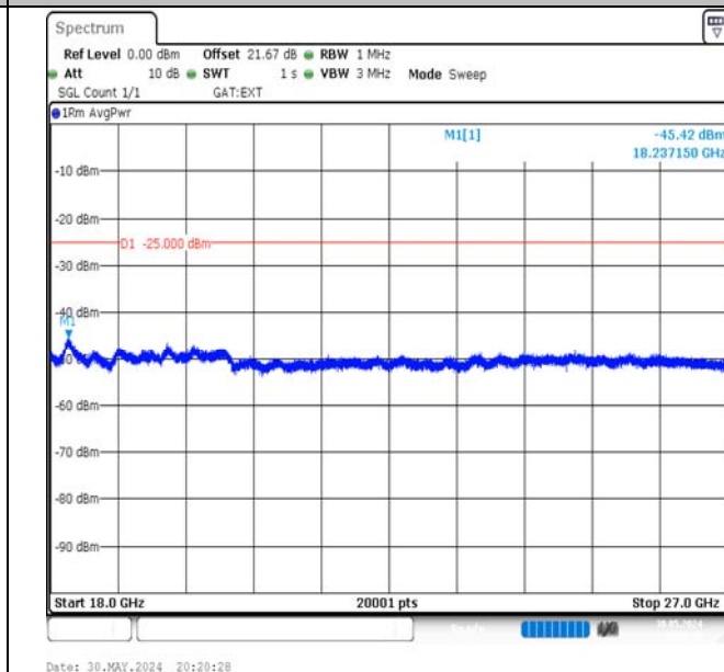
Band41-10MHz-16QAM-40620-50RB#0-18000~27000-PASS
