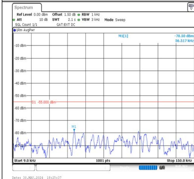
Band41-15MHz-QPSK-40620-1RB#0-0.009~0.15-PASS
