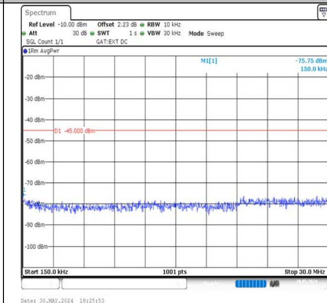
Band41-15MHz-QPSK-40620-1RB#0-0.15~30-PASS
