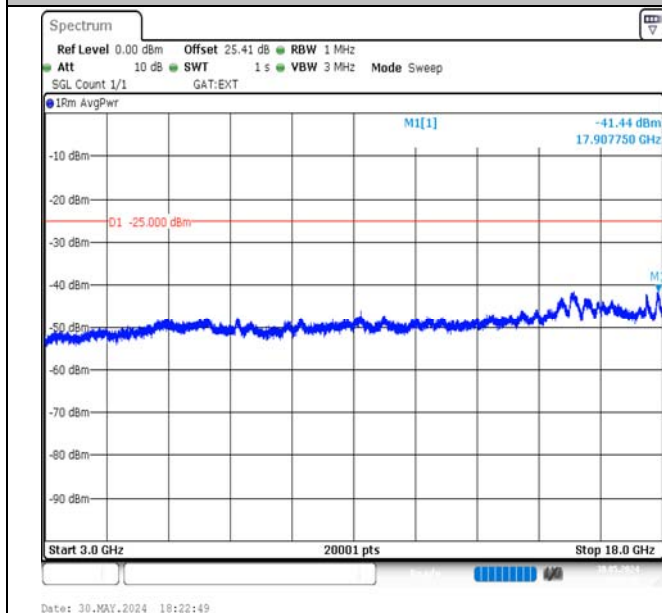
Band41-15MHz-QPSK-39725-75RB#0-3000~18000-PASS
