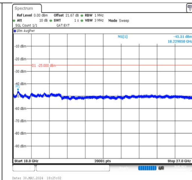
Band41-15MHz-16QAM-39725-75RB#0-18000~27000-PASS
