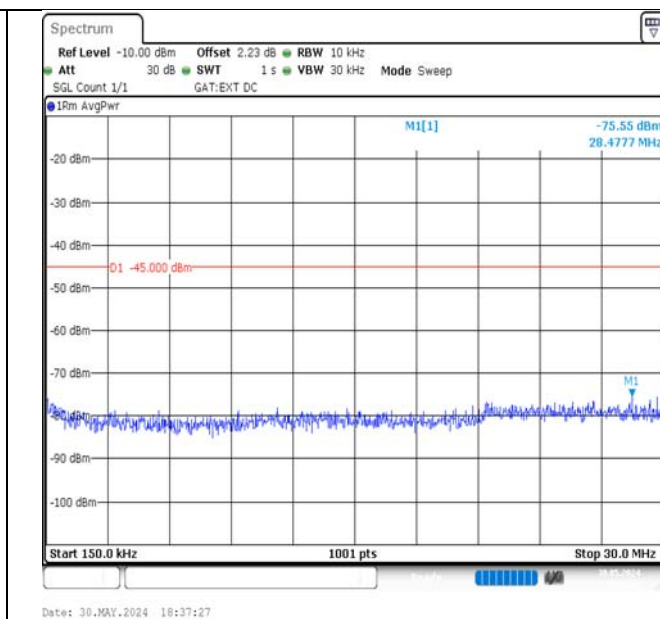
Band41-15MHz-QPSK-41515-1RB#0-0.15~30-PASS
