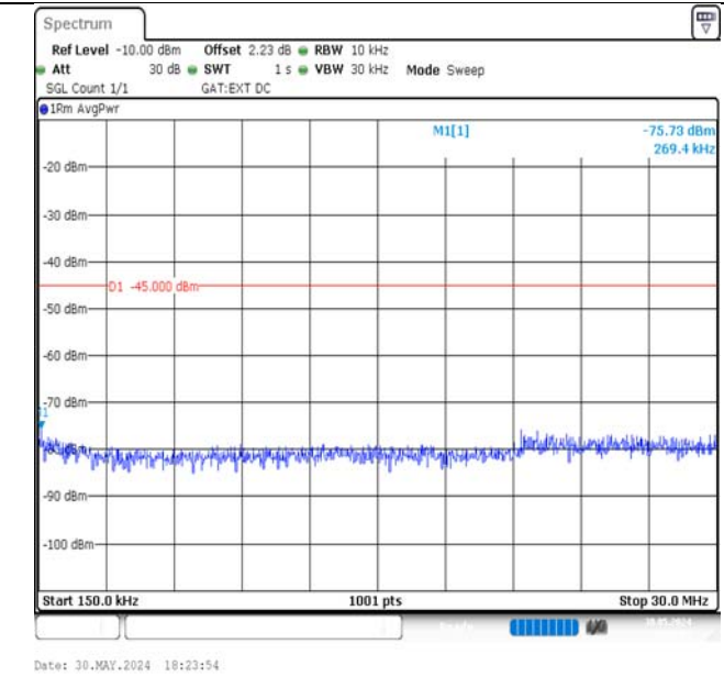
Band41-15MHz-16QAM-39725-75RB#0-0.15~30-PASS
