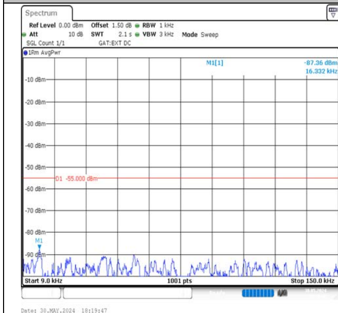
Band41-15MHz-16QAM-39725-1RB#74-0.009~0.15-PASS
