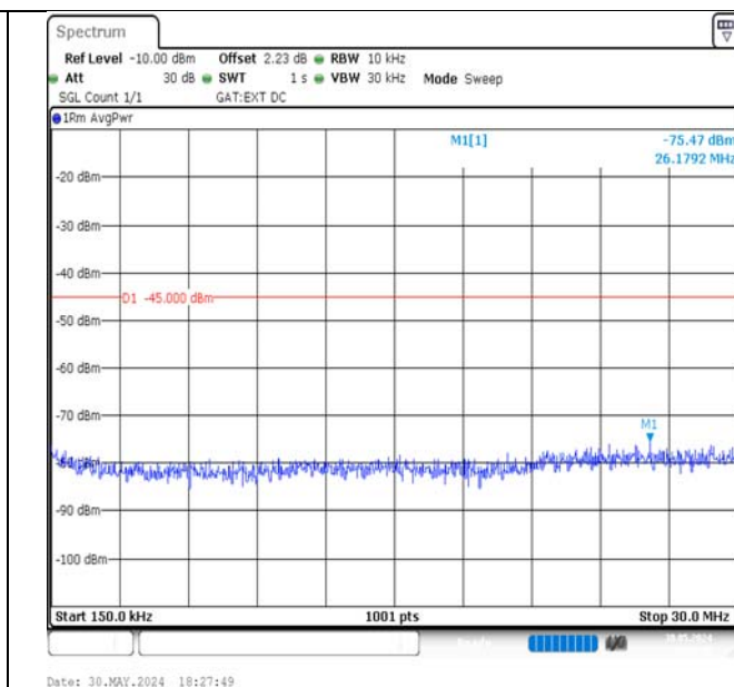
Band41-15MHz-16QAM-40620-1RB#0-0.15~30-PASS
