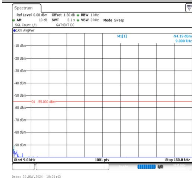
Band41-15MHz-QPSK-39725-75RB#0-0.009~0.15-PASS
