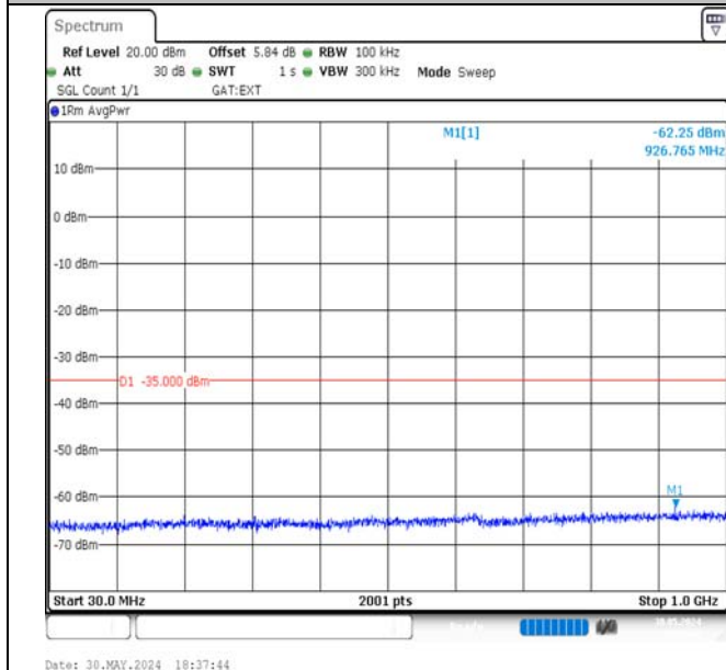
Band41-15MHz-QPSK-41515-1RB#0-30~1000-PASS
