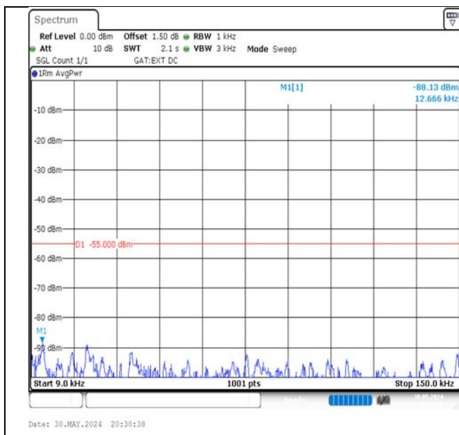
Band41-10MHz-16QAM-41540-50RB#0-0.009~0.15-PASS
