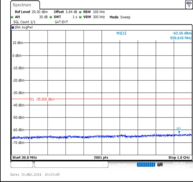
Band41-10MHz-16QAM-40620-1RB#49-30~1000-PASS
