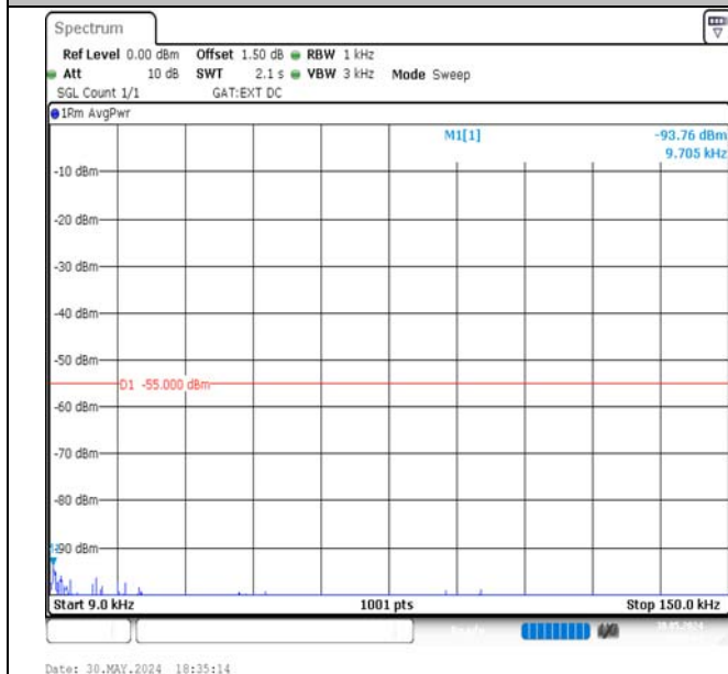
Band41-15MHz-16QAM-40620-75RB#0-0.009~0.15-PASS
