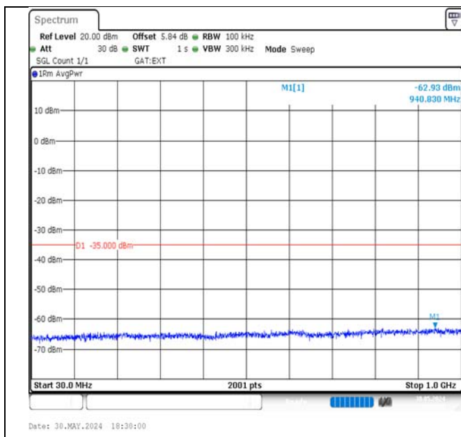
Band41-15MHz-QPSK-40620-1RB#74-30~1000-PASS
