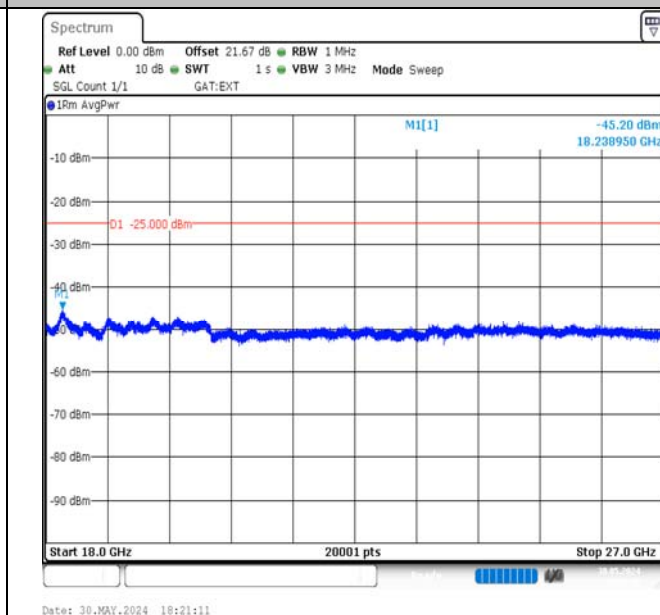
Band41-15MHz-16QAM-39725-1RB#74-18000~27000-PASS
