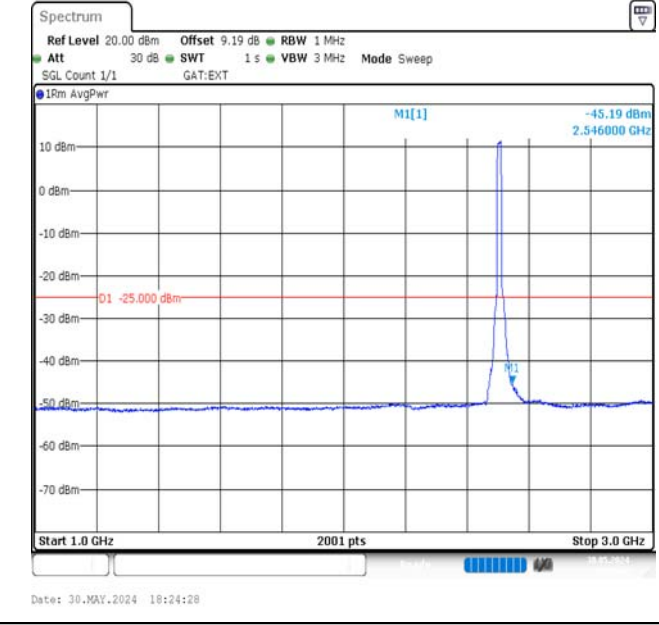
Band41-15MHz-16QAM-39725-75RB#0-1000~3000-PASS
