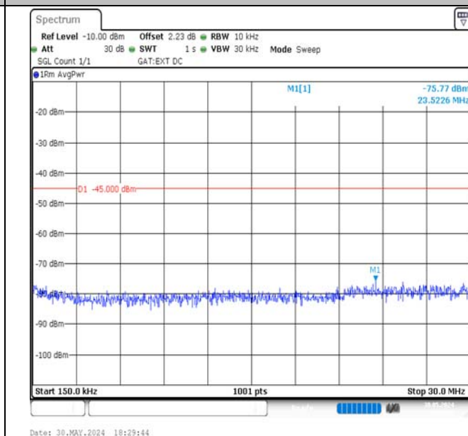
Band41-15MHz-QPSK-40620-1RB#74-0.15~30-PASS
