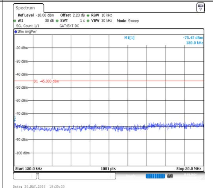
Band41-15MHz-16QAM-40620-75RB#0-0.15~30-PASS
