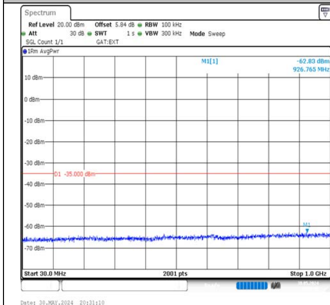
Band41-10MHz-16QAM-41540-50RB#0-30~1000-PASS
