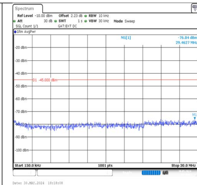
Band41-15MHz-QPSK-39725-1RB#74-0.15~30-PASS
