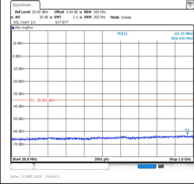
Band41-15MHz-16QAM-39725-75RB#0-30~1000-PASS
