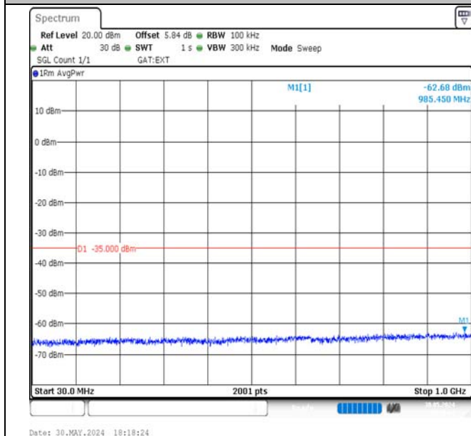
Band41-15MHz-QPSK-39725-1RB#74-30~1000-PASS
