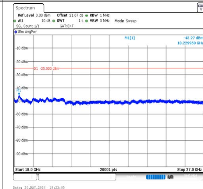
Band41-15MHz-QPSK-39725-75RB#0-18000~27000-PASS
