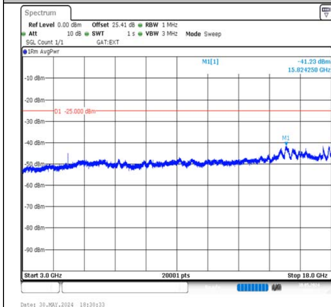
Band41-15MHz-QPSK-40620-1RB#74-3000~18000-PASS
