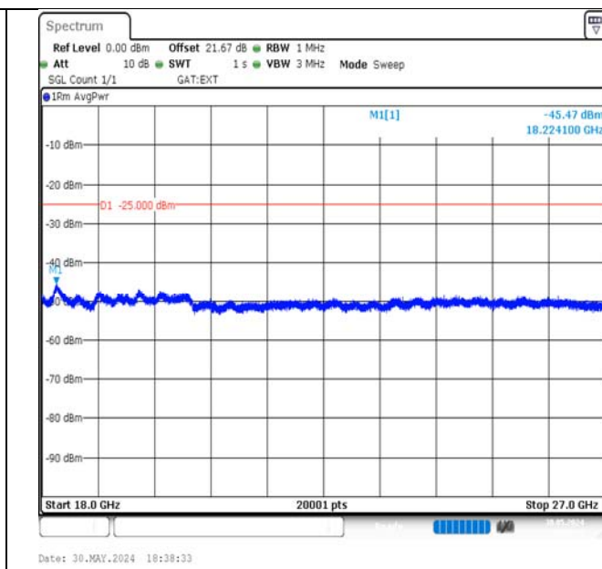
Band41-15MHz-QPSK-41515-1RB#0-18000~27000-PASS
