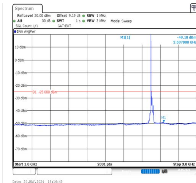
Band41-15MHz-16QAM-39725-1RB#0-1000~3000-PASS
