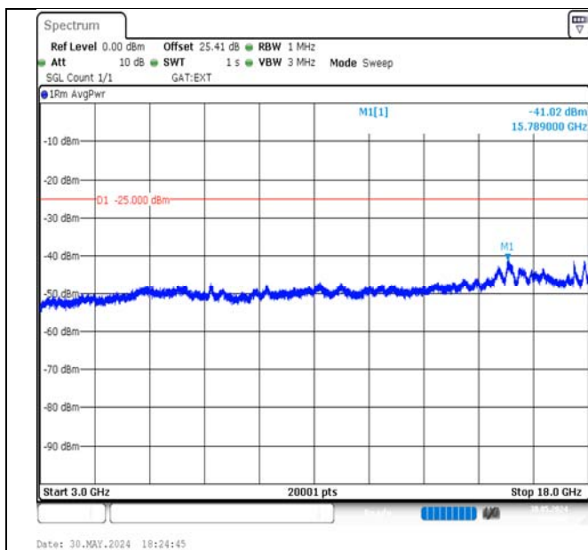
Band41-15MHz-16QAM-39725-75RB#0-3000~18000-PASS
