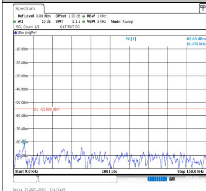
Band41-10MHz-16QAM-39700-1RB#49-0.009~0.15-PASS
