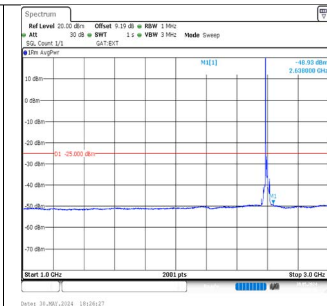
Band41-15MHz-QPSK-40620-1RB#0-1000~3000-PASS
