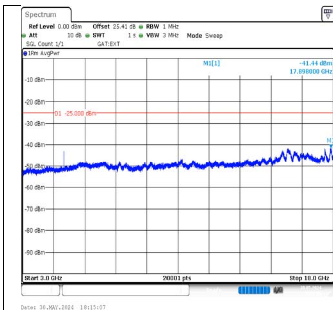
Band41-15MHz-QPSK-39725-1RB#0-3000~18000-PASS
