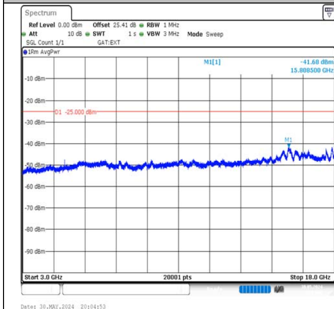
Band41-10MHz-16QAM-39700-1RB#49-3000~18000-PASS
