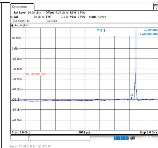
Band41-10MHz-16QAM-41540-1RB#49-1000~3000-PASS
