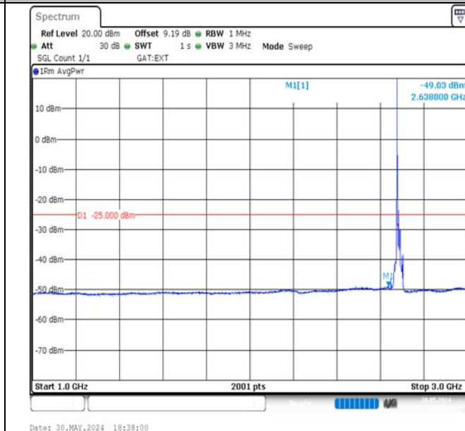
Band41-15MHz-QPSK-41515-1RB#0-1000~3000-PASS
