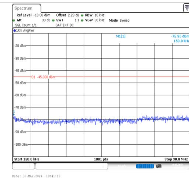
Band41-15MHz-QPSK-41515-1RB#74-0.15~30-PASS
