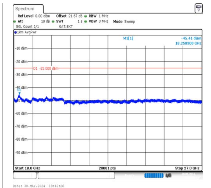
Band41-15MHz-QPSK-41515-1RB#74-18000~27000-PASS
