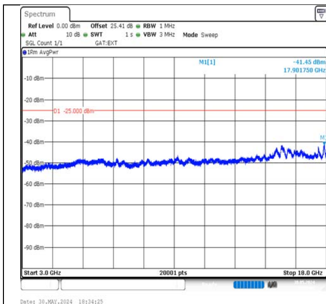
Band41-15MHz-QPSK-40620-75RB#0-3000~18000-PASS
