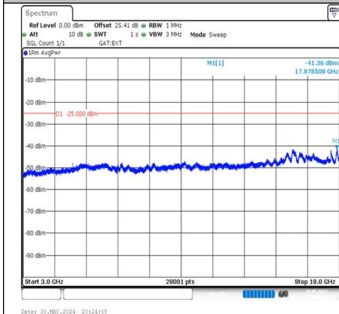
Band41-10MHz-16QAM-41540-1RB#0-3000~18000-PASS
