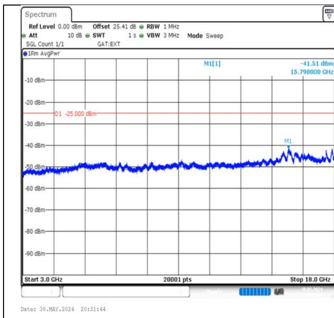
Band41-10MHz-16QAM-41540-50RB#0-3000~18000-PASS
