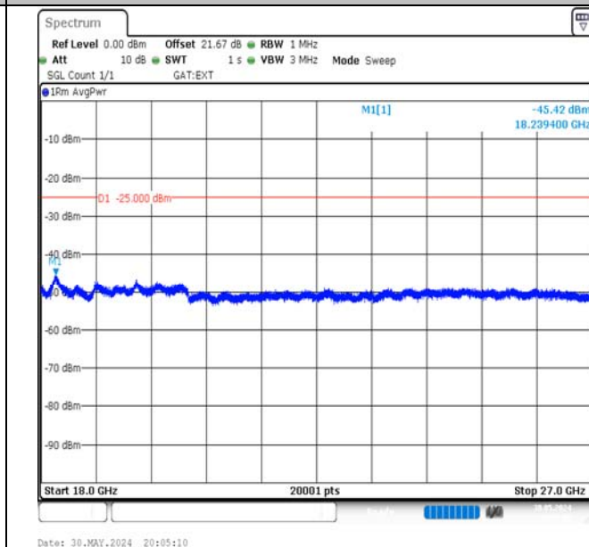
Band41-10MHz-16QAM-39700-1RB#49-18000~27000-PASS
