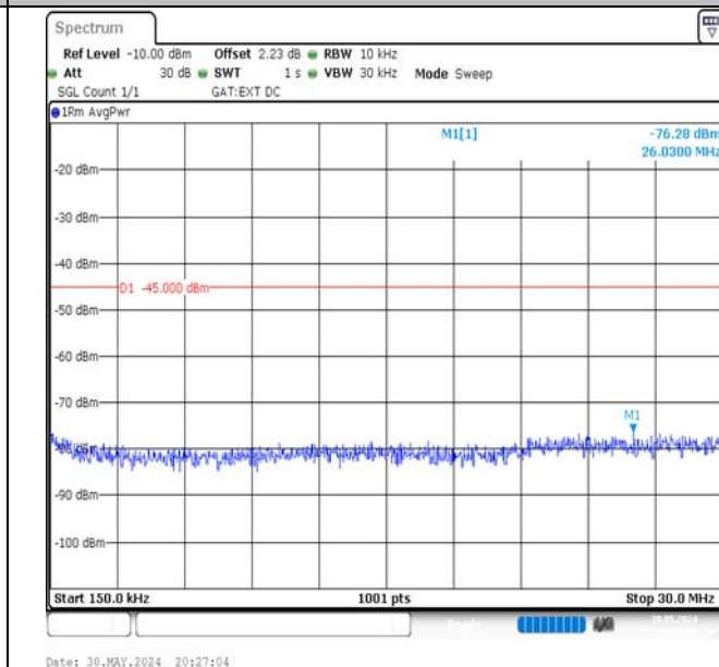
Band41-10MHz-16QAM-41540-1RB#49-0.15~30-PASS
