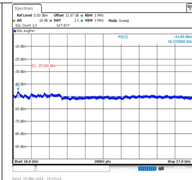
Band41-15MHz-QPSK-39725-1RB#74-18000~27000-PASS
