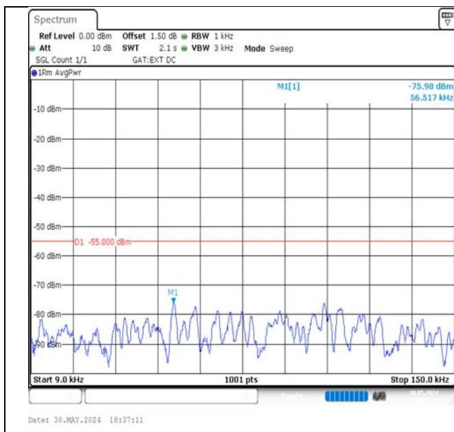
Band41-15MHz-QPSK-41515-1RB#0-0.009~0.15-PASS
