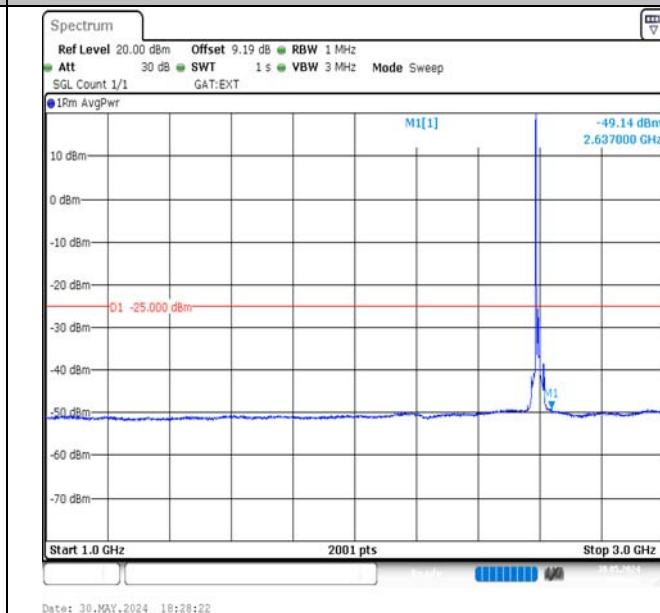
Band41-15MHz-16QAM-40620-1RB#0-1000~3000-PASS
