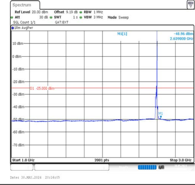
Band41-10MHz-16QAM-40620-1RB#49-1000~3000-PASS
