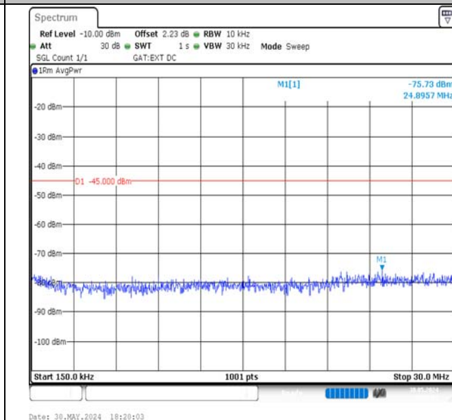
Band41-15MHz-16QAM-39725-1RB#74-0.15~30-PASS
