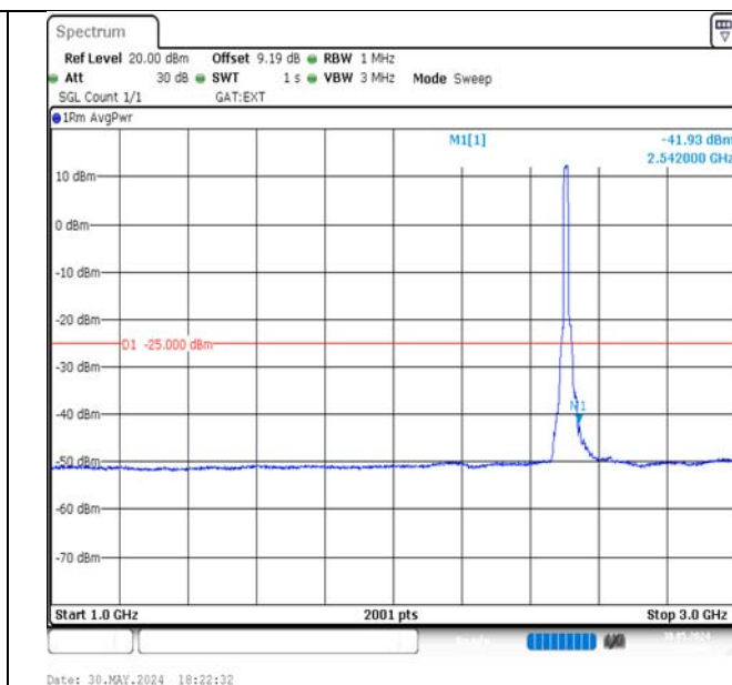
Band41-15MHz-QPSK-39725-75RB#0-1000~3000-PASS
