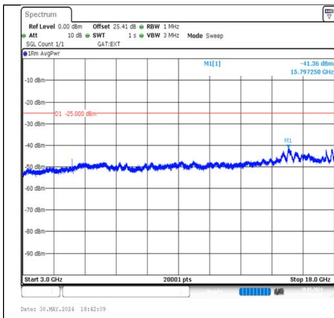
Band41-15MHz-QPSK-41515-1RB#74-3000~18000-PASS
