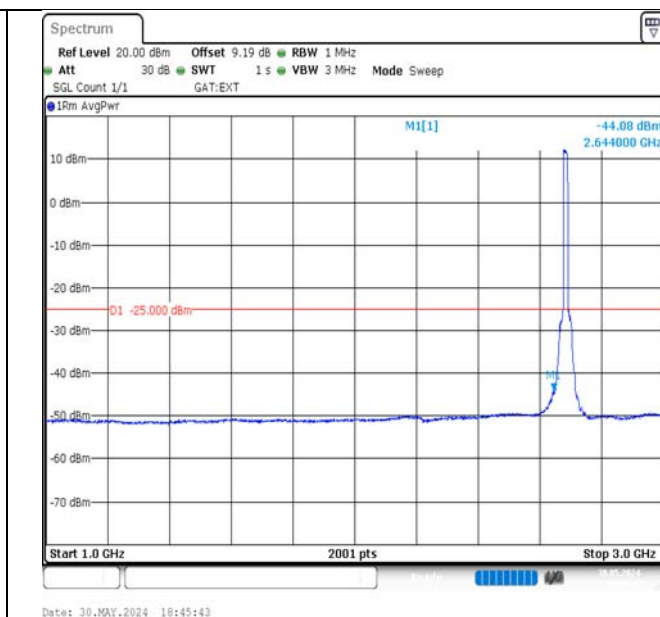
Band41-15MHz-QPSK-41515-75RB#0-1000~3000-PASS
