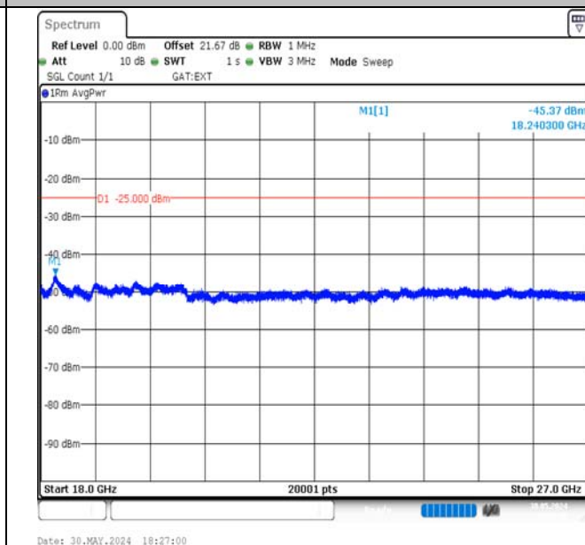
Band41-15MHz-QPSK-40620-1RB#0-18000~27000-PASS
