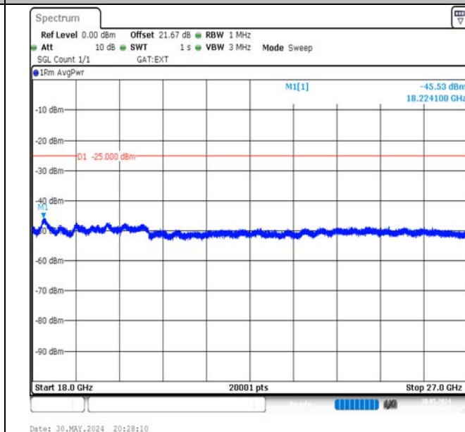
Band41-10MHz-16QAM-41540-1RB#49-18000~27000-PASS
