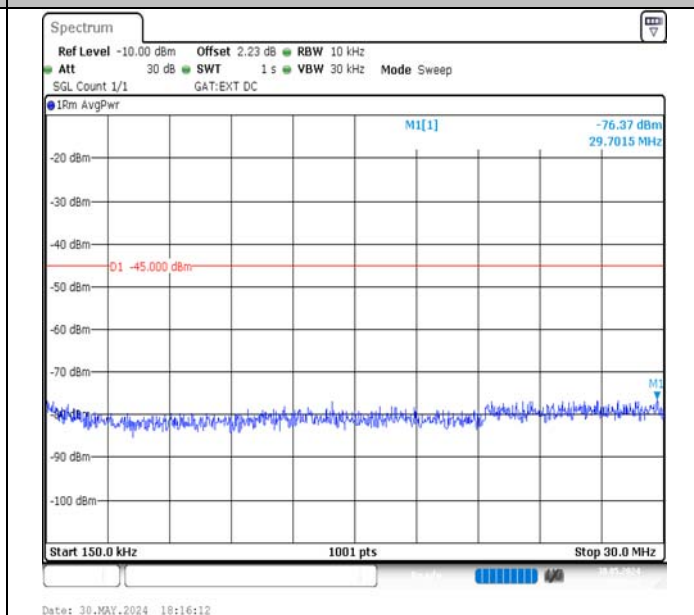
Band41-15MHz-16QAM-39725-1RB#0-0.15~30-PASS
