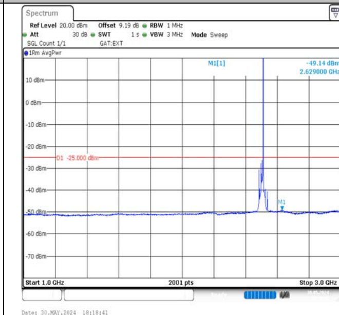
Band41-15MHz-QPSK-39725-1RB#74-1000~3000-PASS
