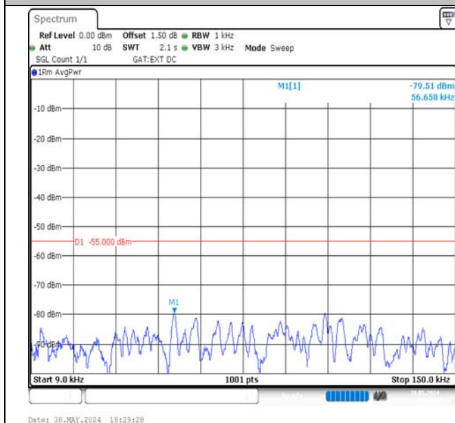
Band41-15MHz-QPSK-40620-1RB#74-0.009~0.15-PASS
