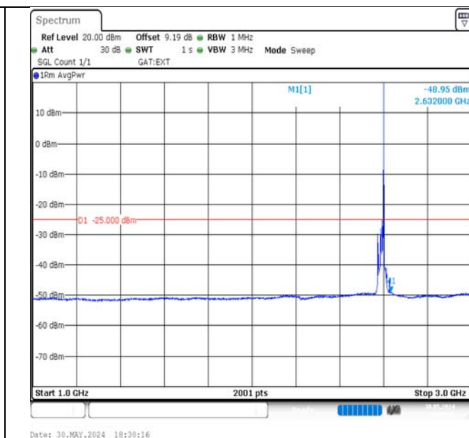
Band41-15MHz-QPSK-40620-1RB#74-1000~3000-PASS
