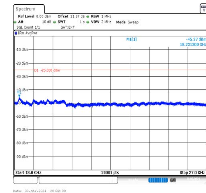
Band41-10MHz-16QAM-41540-50RB#0-18000~27000-PASS
