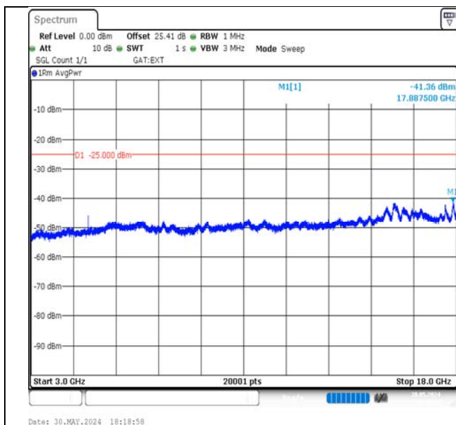
Band41-15MHz-QPSK-39725-1RB#74-3000~18000-PASS
