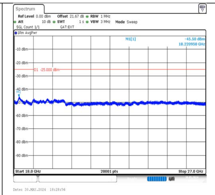
Band41-15MHz-16QAM-40620-1RB#0-18000~27000-PASS
