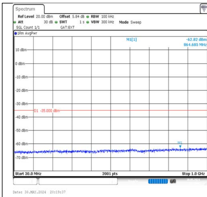
Band41-10MHz-16QAM-40620-50RB#0-30~1000-PASS
