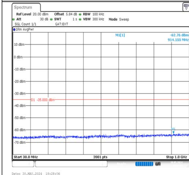
Band41-15MHz-16QAM-40620-1RB#0-30~1000-PASS
