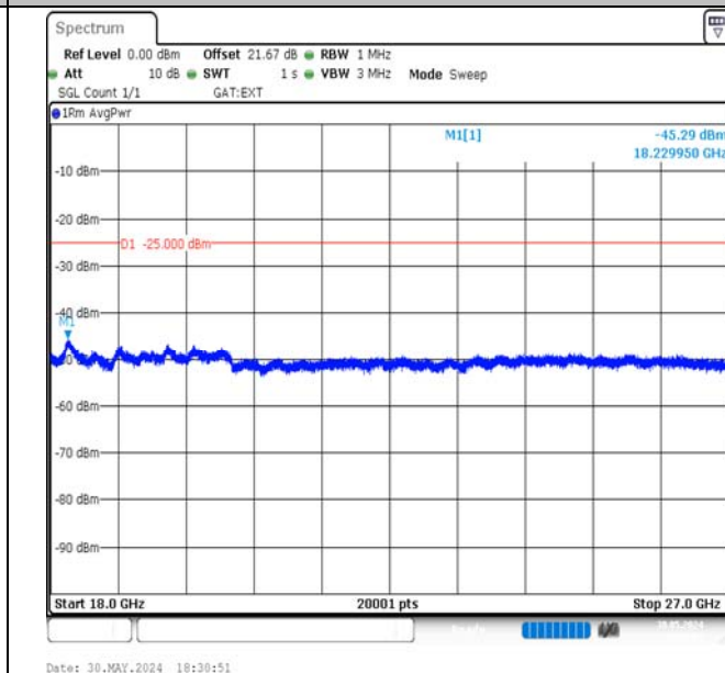
Band41-15MHz-QPSK-40620-1RB#74-18000~27000-PASS
