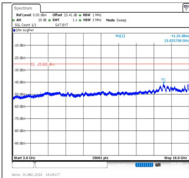
Band41-15MHz-QPSK-41515-1RB#0-3000~18000-PASS
