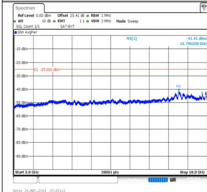
Band41-10MHz-16QAM-40620-50RB#0-3000~18000-PASS
