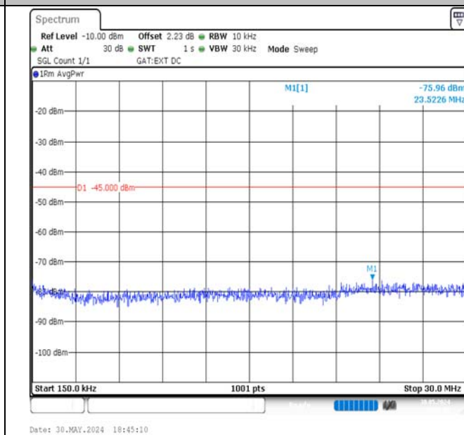
Band41-15MHz-QPSK-41515-75RB#0-0.15~30-PASS
