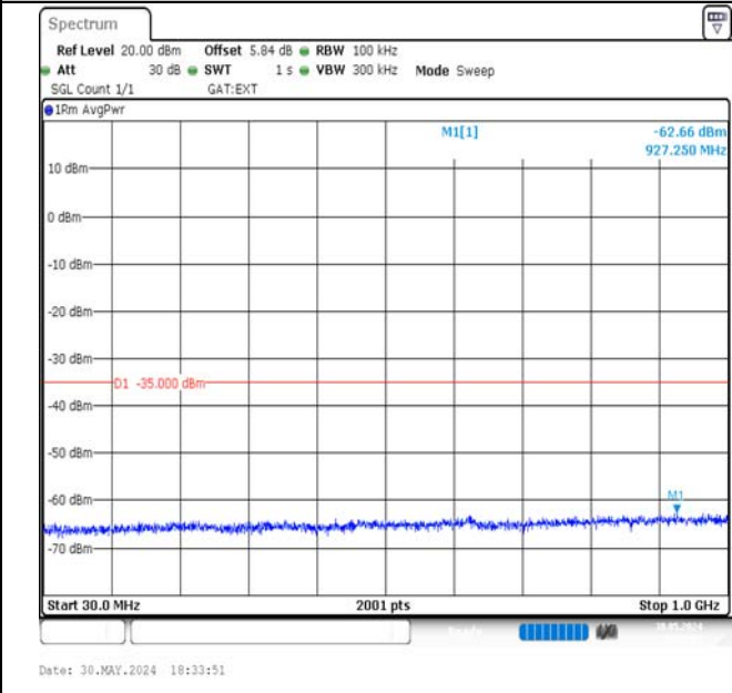
Band41-15MHz-QPSK-40620-75RB#0-30~1000-PASS
