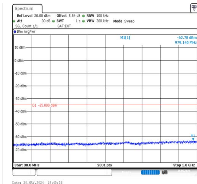
Band41-15MHz-QPSK-41515-75RB#0-30~1000-PASS
