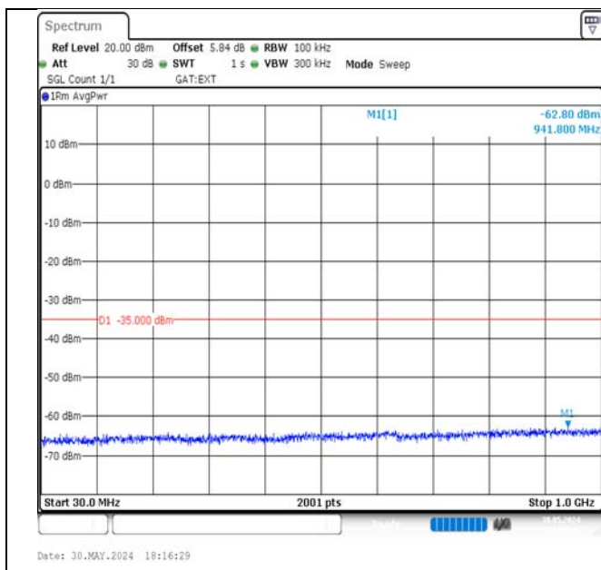
Band41-15MHz-16QAM-39725-1RB#0-30~1000-PASS
