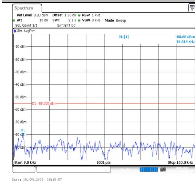
Band41-15MHz-16QAM-39725-1RB#0-0.009~0.15-PASS
