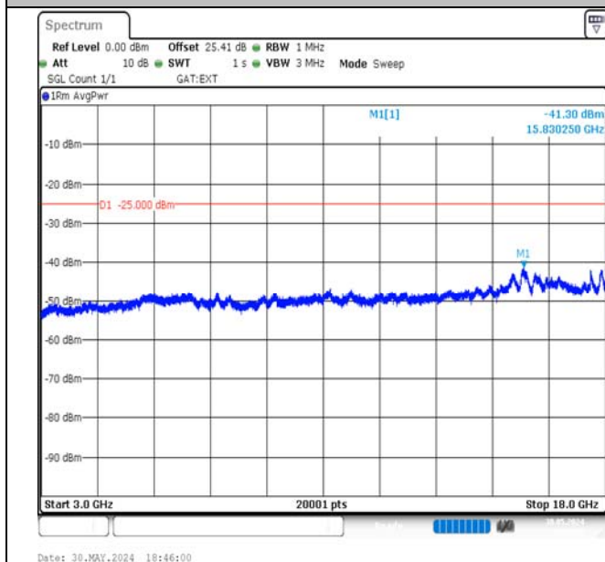
Band41-15MHz-QPSK-41515-75RB#0-3000~18000-PASS
