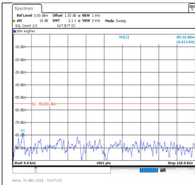
Band41-15MHz-16QAM-40620-1RB#0-0.009~0.15-PASS
