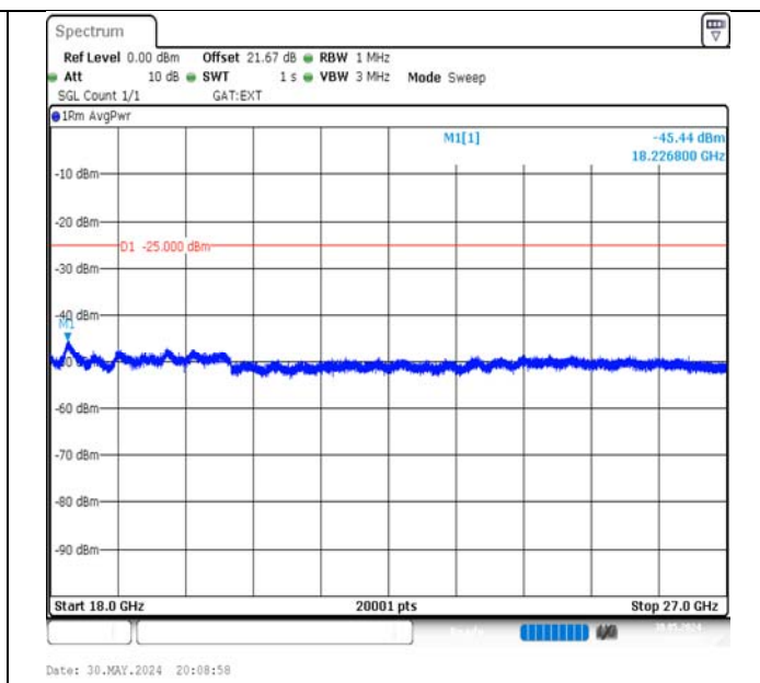
Band41-10MHz-16QAM-39700-50RB#0-18000~27000-PASS
