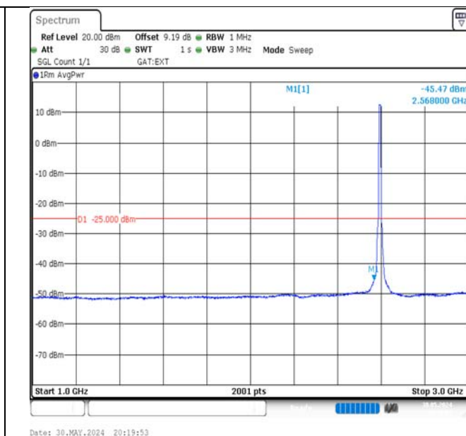
Band41-10MHz-16QAM-40620-50RB#0-1000~3000-PASS
