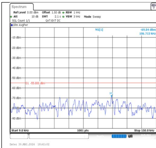
Band41-15MHz-QPSK-41515-1RB#74-0.009~0.15-PASS
