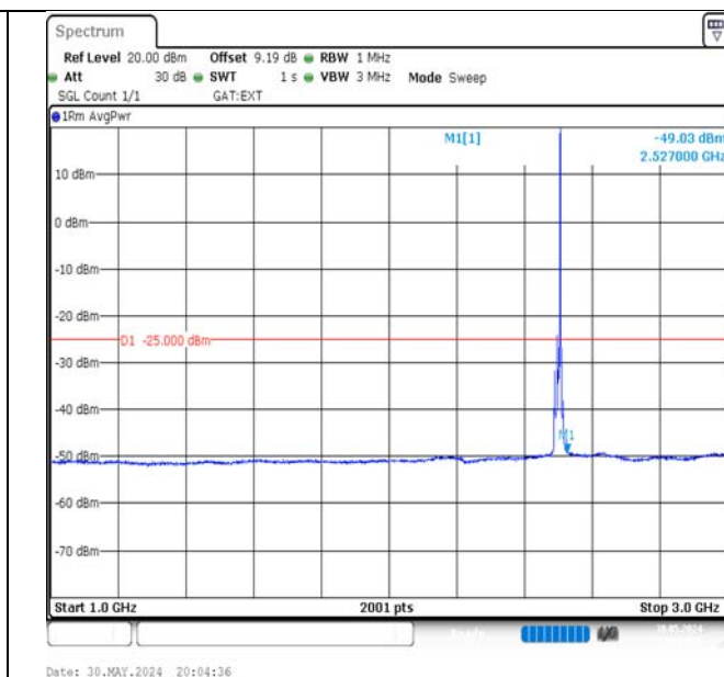
Band41-10MHz-16QAM-39700-1RB#49-1000~3000-PASS
