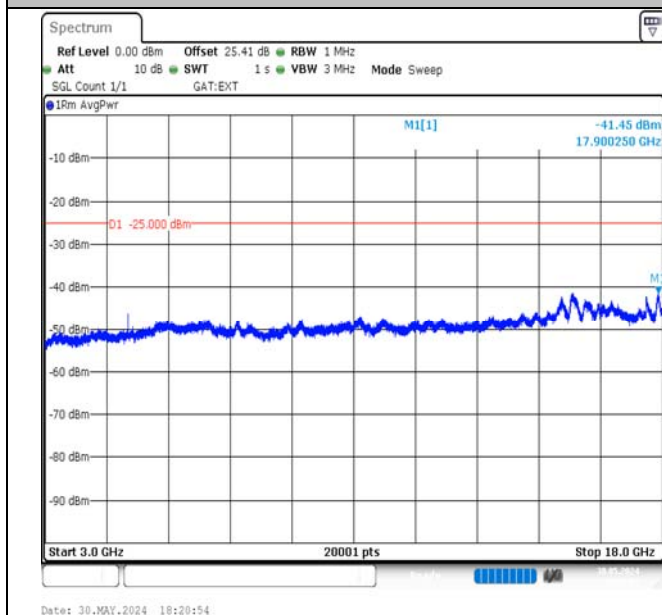
Band41-15MHz-16QAM-39725-1RB#74-3000~18000-PASS
