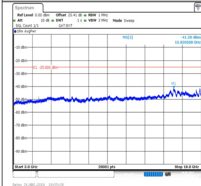
Band41-5MHz-16QAM-39675-1RB#24-3000~18000-PASS
