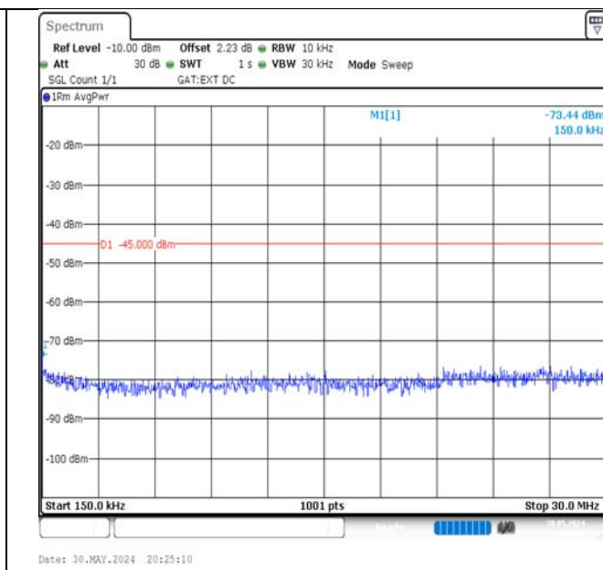
Band41-10MHz-QPSK-41540-1RB#49-0.15~30-PASS
