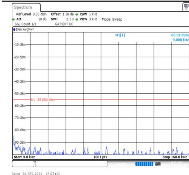
Band41-5MHz-QPSK-41565-25RB#0-0.009~0.15-PASS
