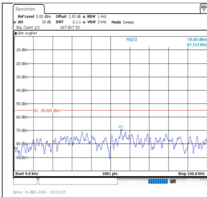
Band41-5MHz-QPSK-41565-1RB#24-0.009~0.15-PASS
