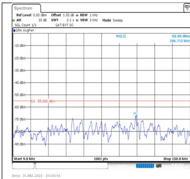
Band41-10MHz-QPSK-41540-1RB#49-0.009~0.15-PASS
