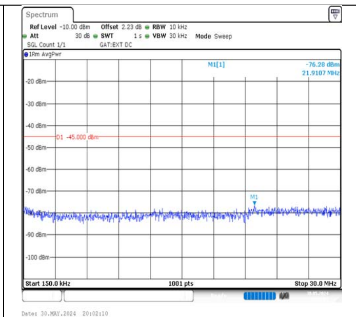
Band41-10MHz-QPSK-39700-1RB#49-0.15~30-PASS
