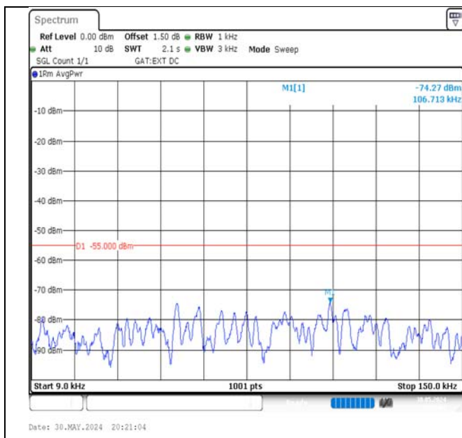
Band41-10MHz-QPSK-41540-1RB#0-0.009~0.15-PASS
