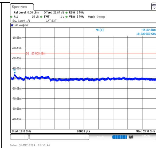
Band41-5MHz-16QAM-39675-25RB#0-18000~27000-PASS
