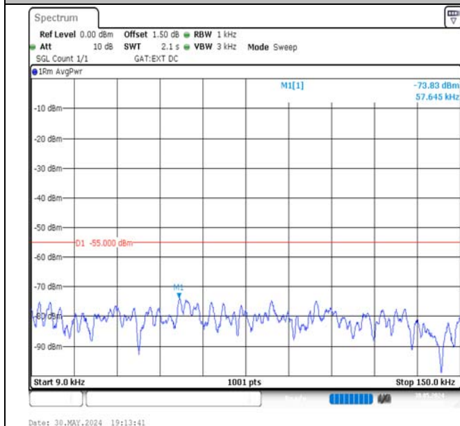
Band41-5MHz-16QAM-41565-1RB#0-0.009~0.15-PASS
