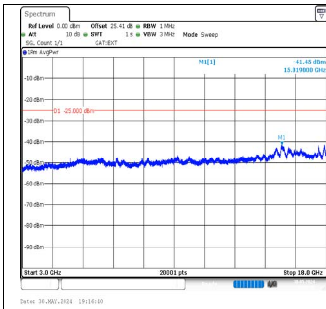
Band41-5MHz-QPSK-41565-1RB#24-3000~18000-PASS
