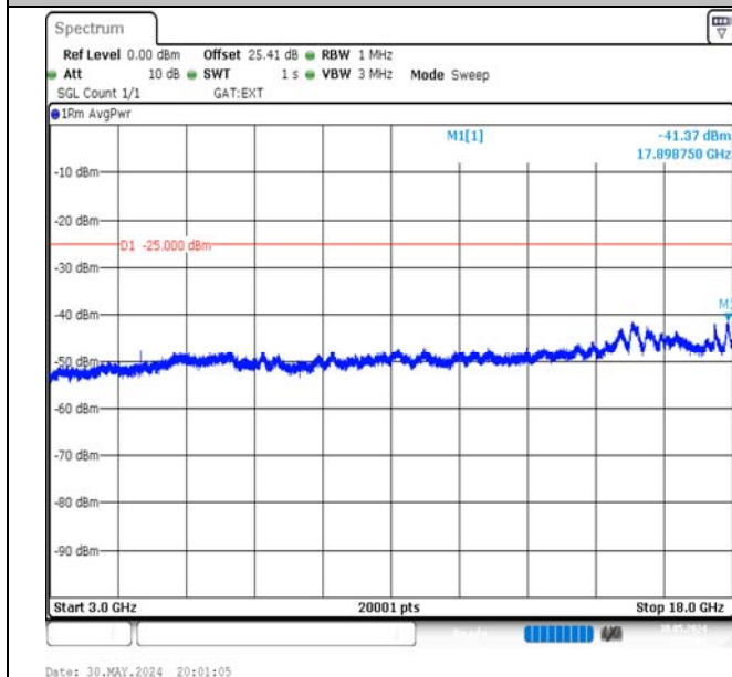
Band41-10MHz-16QAM-39700-1RB#0-3000~18000-PASS
