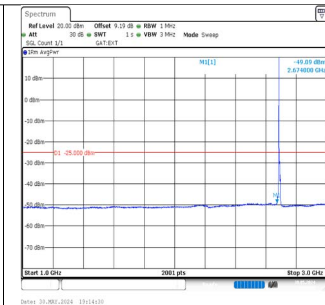
Band41-5MHz-16QAM-41565-1RB#0-1000~3000-PASS
