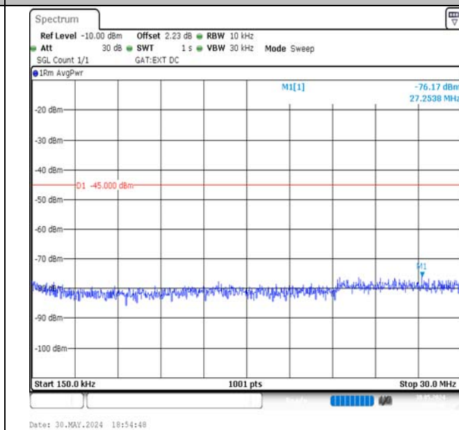
Band41-5MHz-16QAM-39675-1RB#24-0.15~30-PASS
