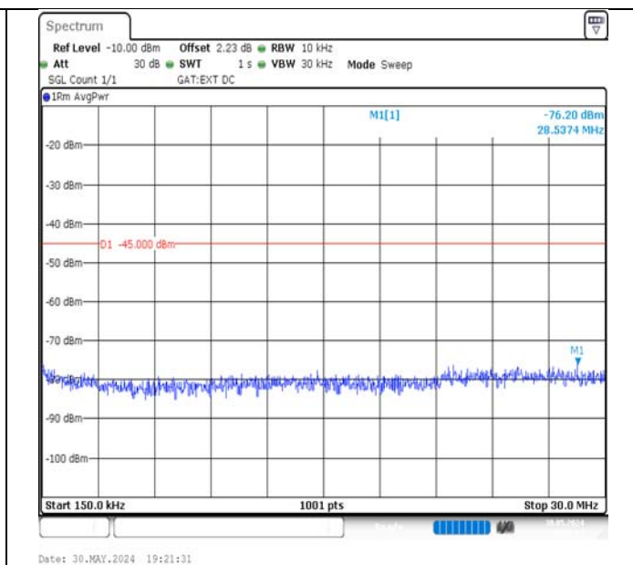
Band41-5MHz-16QAM-41565-25RB#0-0.15~30-PASS
