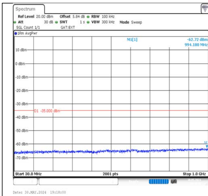
Band41-5MHz-16QAM-41565-1RB#24-30~1000-PASS
