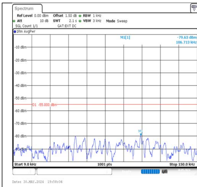
Band41-10MHz-QPSK-39700-1RB#0-0.009~0.15-PASS
