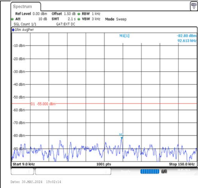
Band41-5MHz-16QAM-40620-1RB#0-0.009~0.15-PASS
