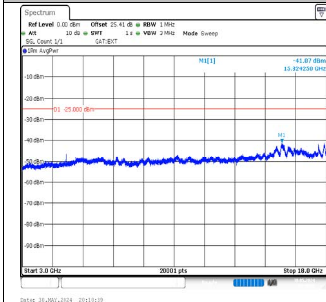
Band41-10MHz-QPSK-40620-1RB#0-3000~18000-PASS
