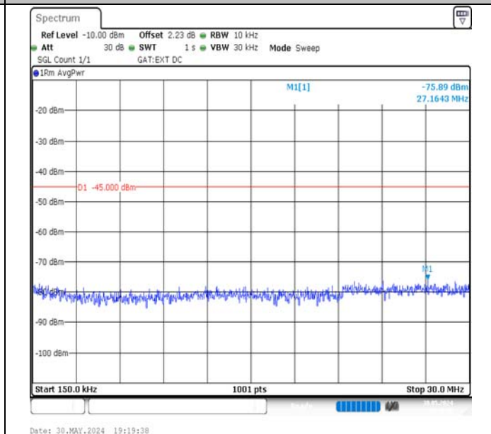
Band41-5MHz-QPSK-41565-25RB#0-0.15~30-PASS
