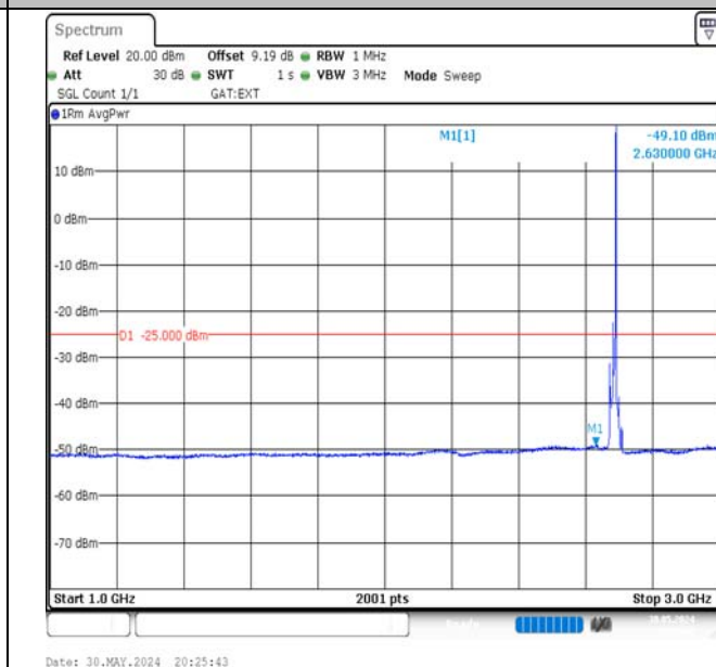
Band41-10MHz-QPSK-41540-1RB#49-1000~3000-PASS
