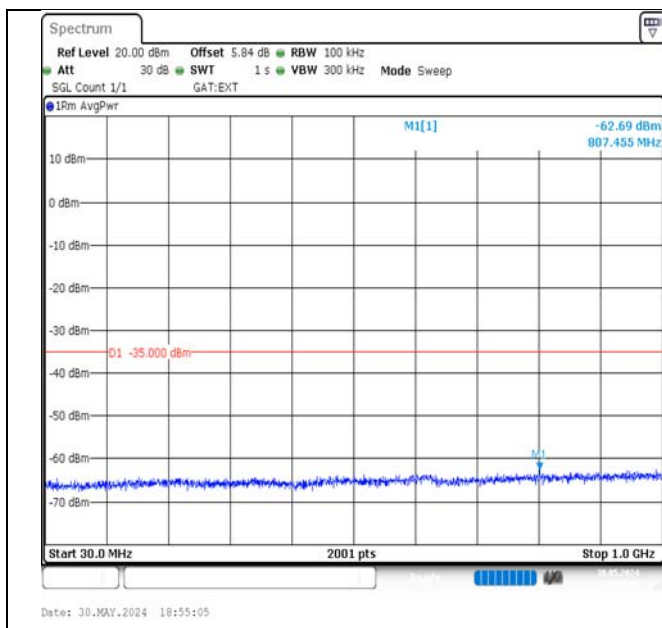
Band41-5MHz-16QAM-39675-1RB#24-30~1000-PASS
