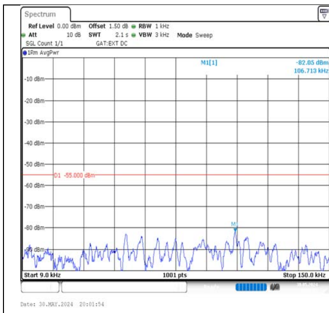
Band41-10MHz-QPSK-39700-1RB#49-0.009~0.15-PASS
