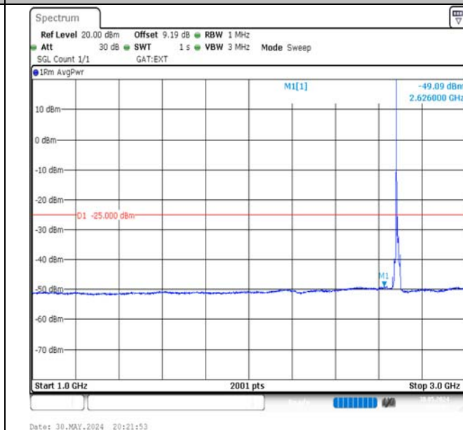
Band41-10MHz-QPSK-41540-1RB#0-1000~3000-PASS
