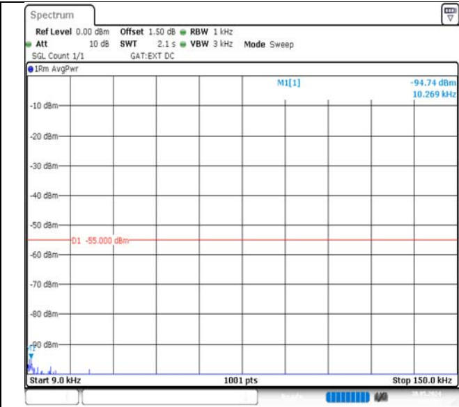
Band41-10MHz-QPSK-40620-50RB#0-0.009~0.15-PASS
