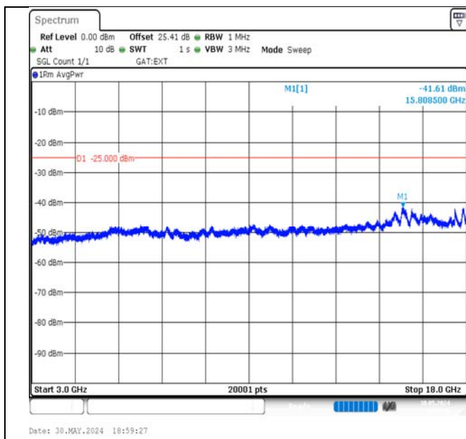
Band41-5MHz-16QAM-39675-25RB#0-3000~18000-PASS
