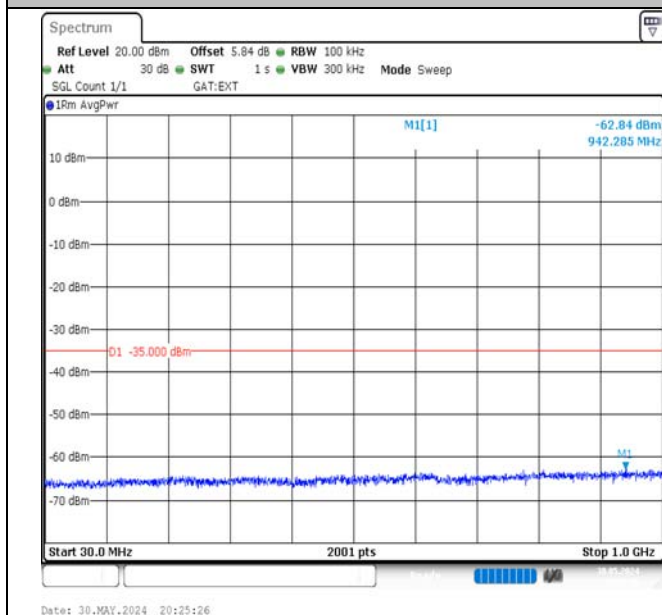
Band41-10MHz-QPSK-41540-1RB#49-30~1000-PASS
