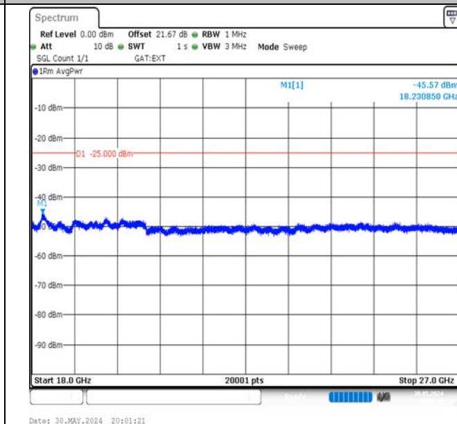
Band41-10MHz-16QAM-39700-1RB#0-18000~27000-PASS
