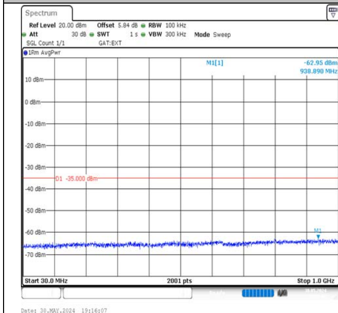
Band41-5MHz-QPSK-41565-1RB#24-30~1000-PASS
