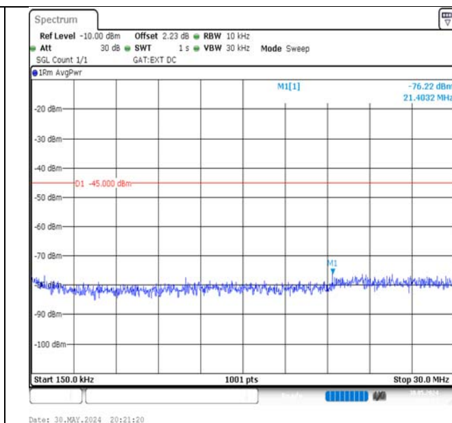
Band41-10MHz-QPSK-41540-1RB#0-0.15~30-PASS
