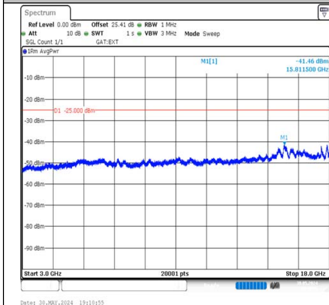
Band41-5MHz-16QAM-40620-25RB#0-3000~18000-PASS
