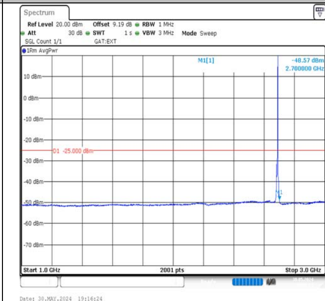
Band41-5MHz-QPSK-41565-1RB#24-1000~3000-PASS
