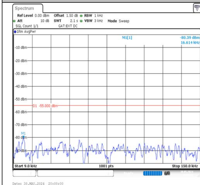
Band41-10MHz-16QAM-39700-1RB#0-0.009~0.15-PASS
