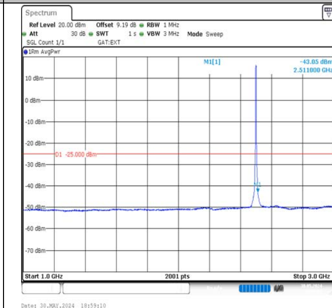
Band41-5MHz-16QAM-39675-25RB#0-1000~3000-PASS
