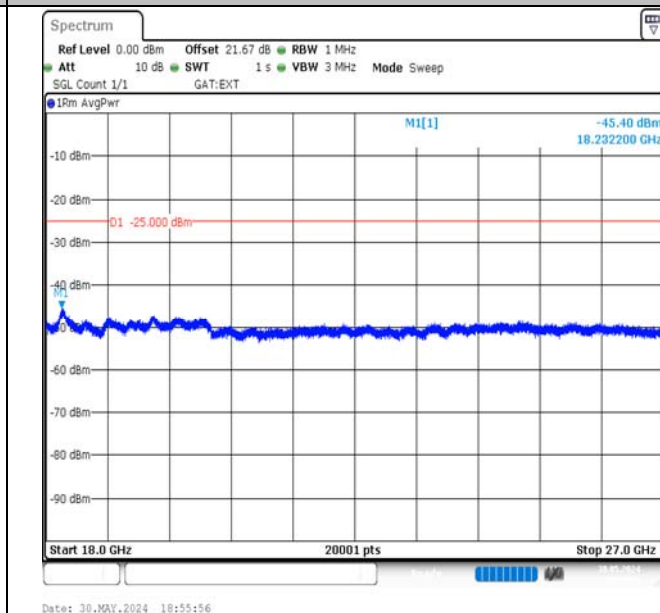
Band41-5MHz-16QAM-39675-1RB#24-18000~27000-PASS
