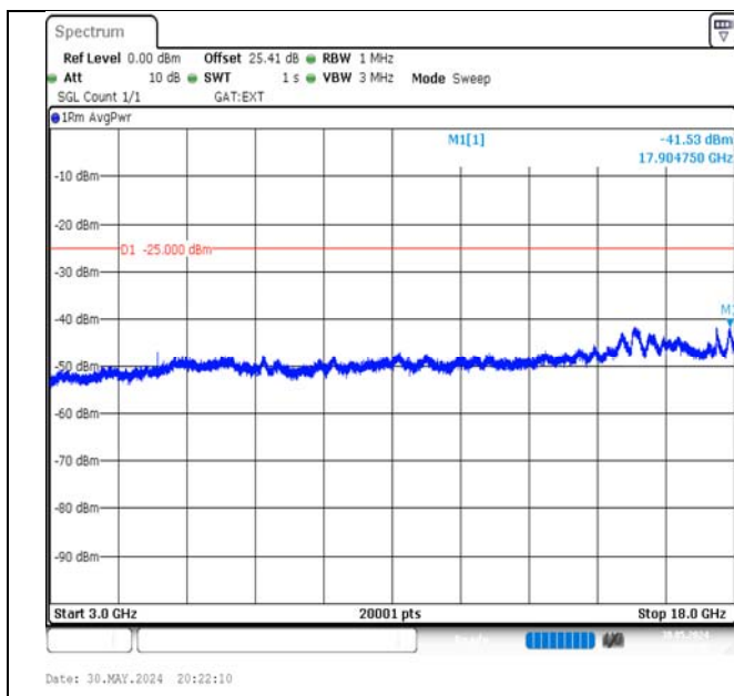
Band41-10MHz-QPSK-41540-1RB#0-3000~18000-PASS
