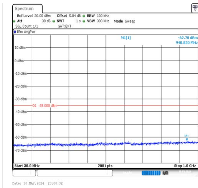
Band41-10MHz-16QAM-39700-1RB#0-30~1000-PASS
