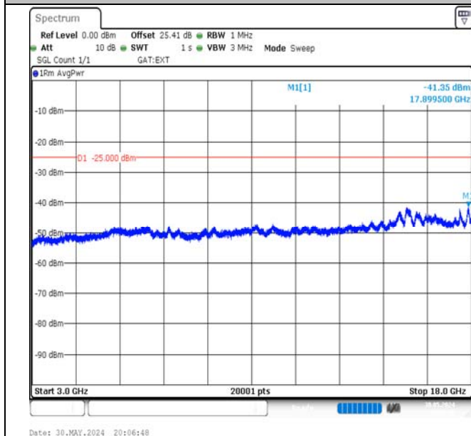
Band41-10MHz-QPSK-39700-50RB#0-3000~18000-PASS
