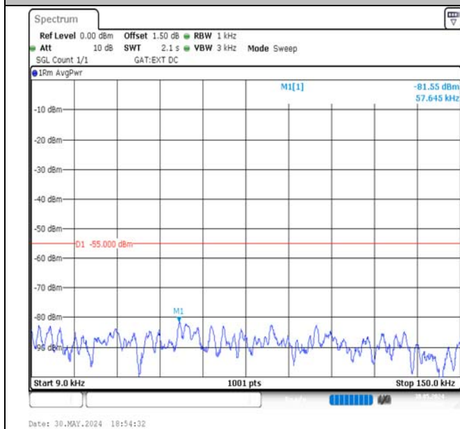
Band41-5MHz-16QAM-39675-1RB#24-0.009~0.15-PASS
