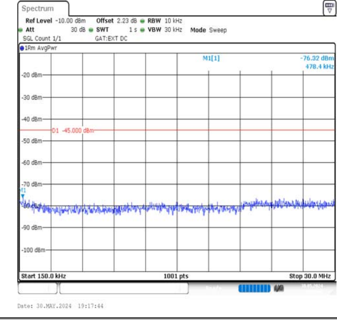
Band41-5MHz-16QAM-41565-1RB#24-0.15~30-PASS
