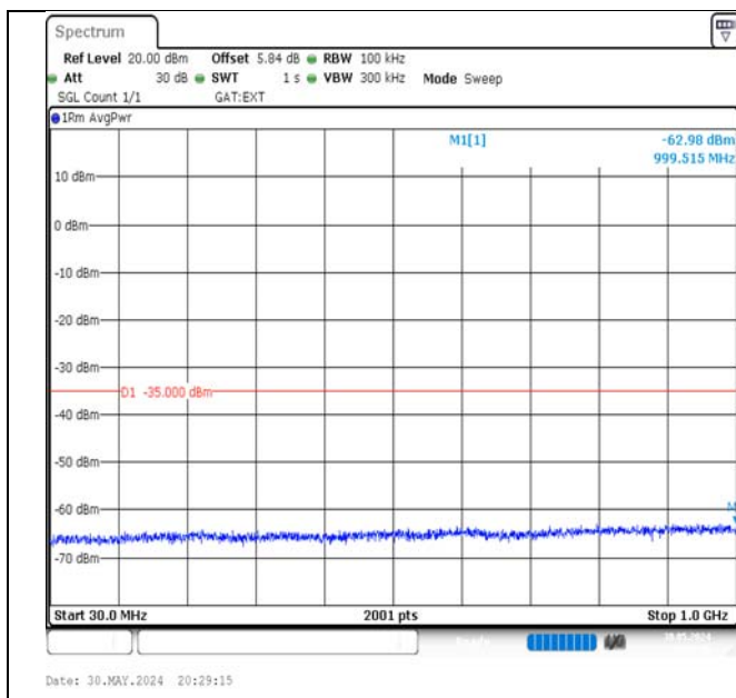
Band41-10MHz-QPSK-41540-50RB#0-30~1000-PASS
