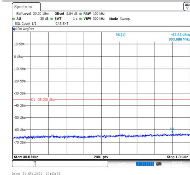
Band41-10MHz-QPSK-39700-1RB#49-30~1000-PASS
