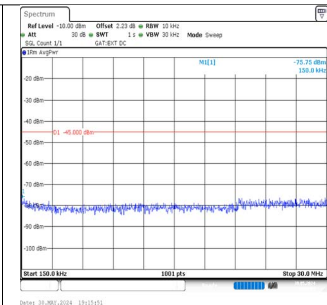
Band41-5MHz-QPSK-41565-1RB#24-0.15~30-PASS
