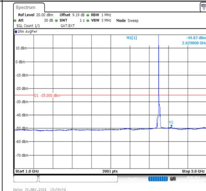
Band41-10MHz-QPSK-39700-1RB#0-1000~3000-PASS
