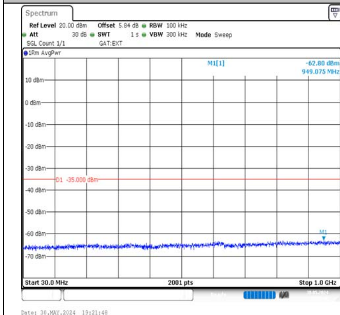
Band41-5MHz-16QAM-41565-25RB#0-30~1000-PASS
