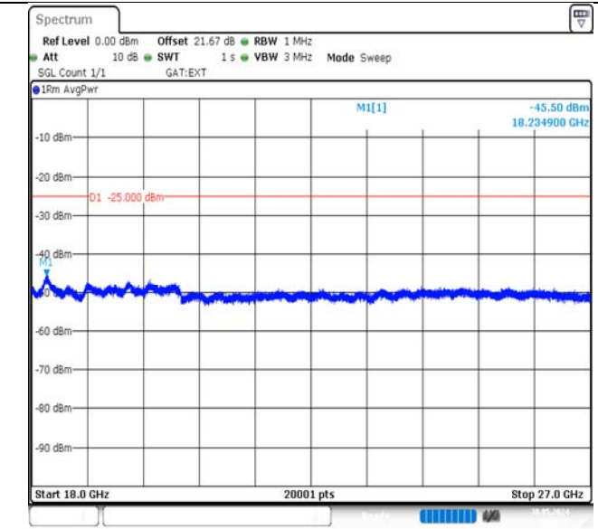
Band41-5MHz-16QAM-40620-1RB#0-18000~27000-PASS
