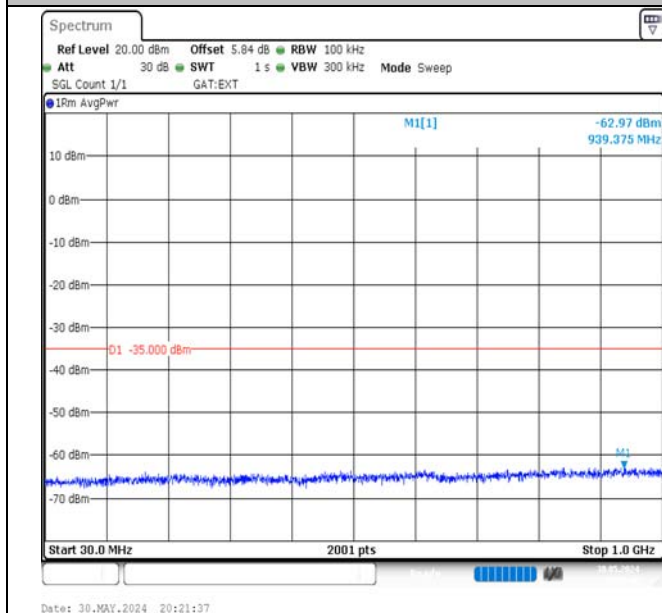
Band41-10MHz-QPSK-41540-1RB#0-30~1000-PASS
