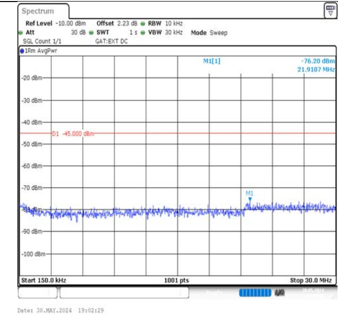
Band41-5MHz-16QAM-40620-1RB#0-0.15~30-PASS
