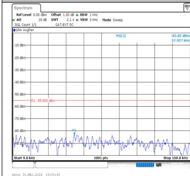
Band41-5MHz-16QAM-39675-1RB#0-0.009~0.15-PASS
