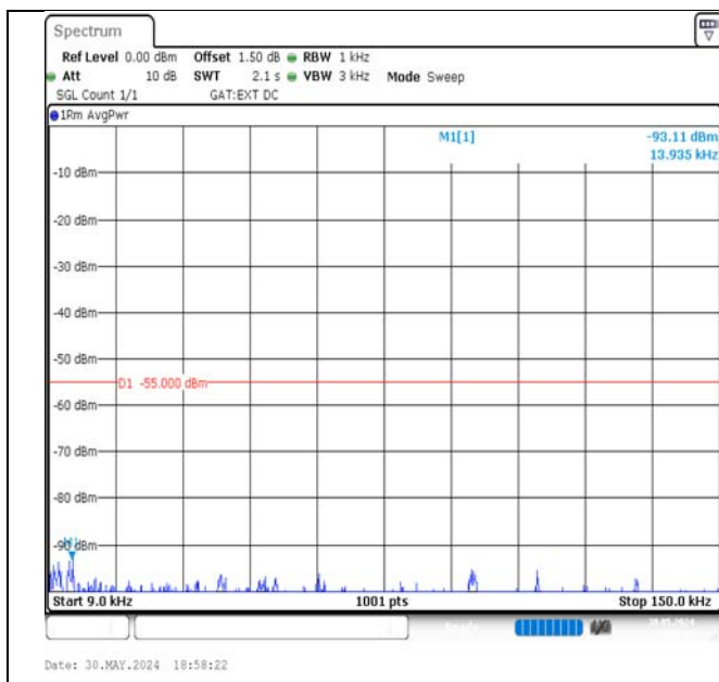
Band41-5MHz-16QAM-39675-25RB#0-0.009~0.15-PASS
