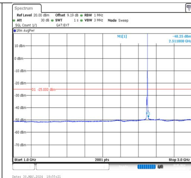
Band41-5MHz-16QAM-39675-1RB#24-1000~3000-PASS
