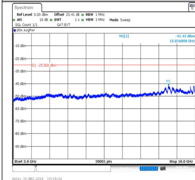
Band41-5MHz-16QAM-41565-1RB#24-3000~18000-PASS
