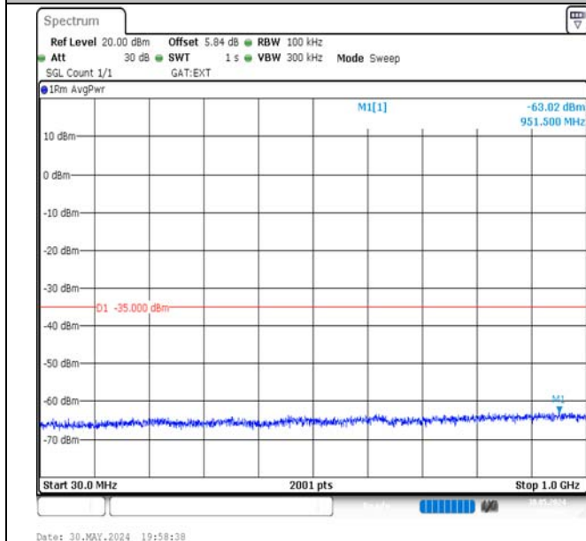
Band41-10MHz-QPSK-39700-1RB#0-30~1000-PASS
