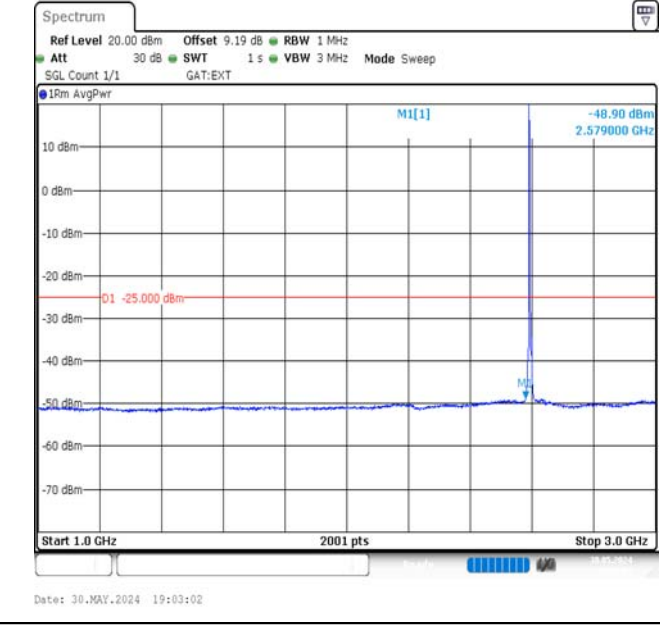
Band41-5MHz-16QAM-40620-1RB#0-1000~3000-PASS
