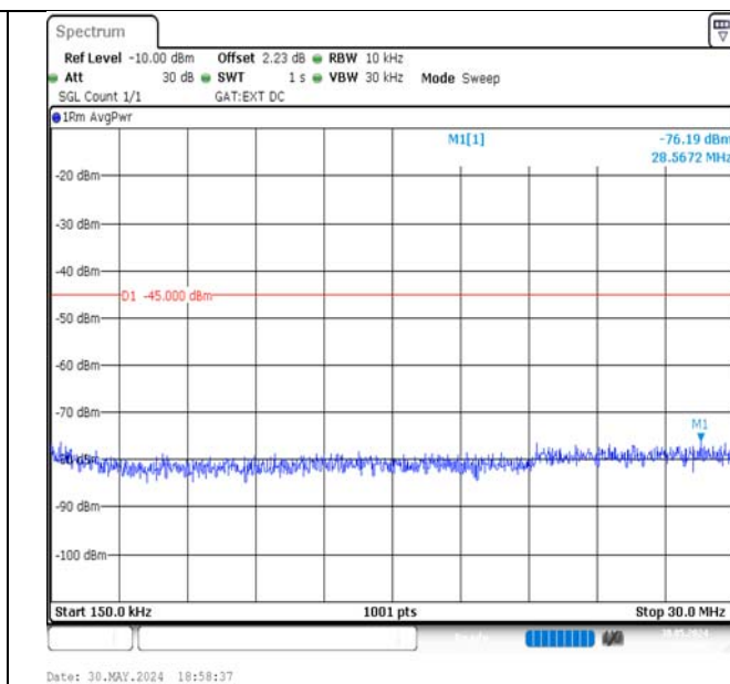
Band41-5MHz-16QAM-39675-25RB#0-0.15~30-PASS
