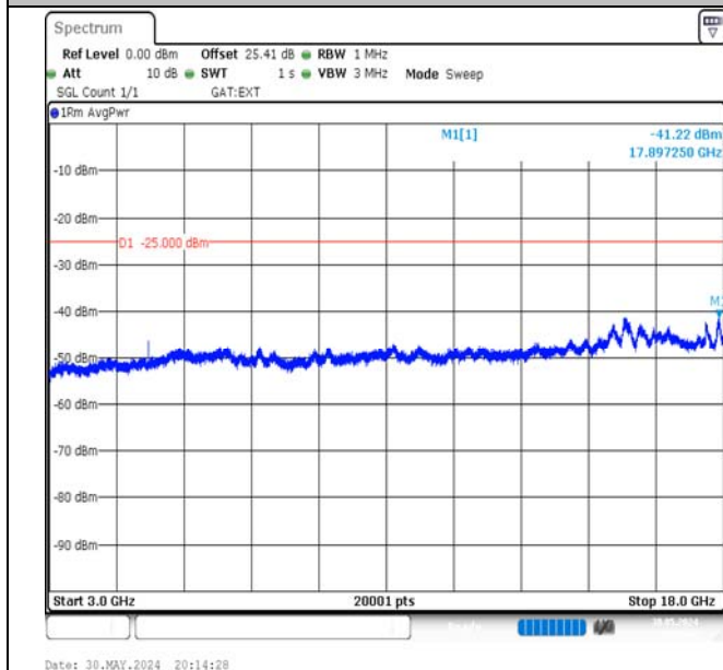
Band41-10MHz-QPSK-40620-1RB#49-3000~18000-PASS
