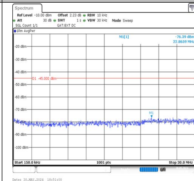
Band41-5MHz-16QAM-39675-1RB#0-0.15~30-PASS
