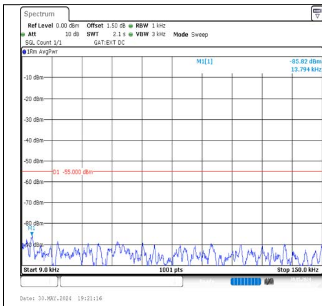
Band41-5MHz-16QAM-41565-25RB#0-0.009~0.15-PASS
