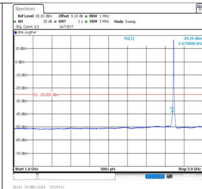
Band41-5MHz-QPSK-41565-25RB#0-1000~3000-PASS
