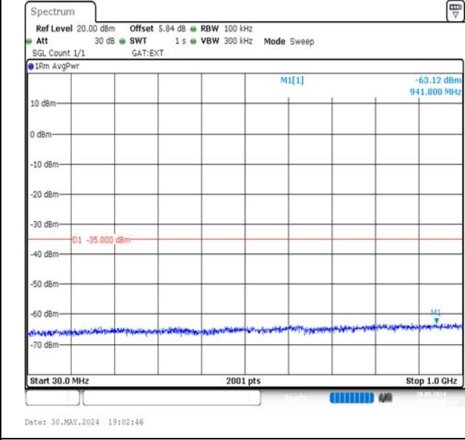
Band41-5MHz-16QAM-40620-1RB#0-30~1000-PASS
