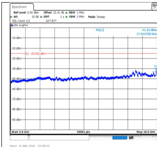
Band41-10MHz-QPSK-41540-1RB#49-3000~18000-PASS
