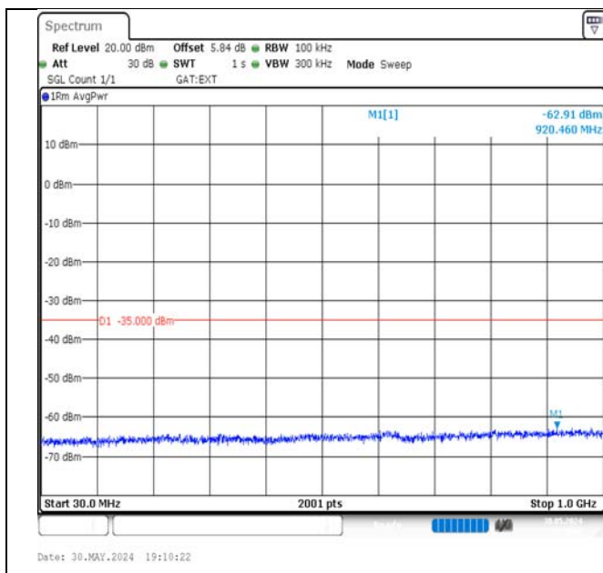
Band41-5MHz-16QAM-40620-25RB#0-30~1000-PASS
