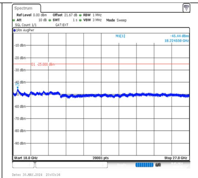
Band41-10MHz-QPSK-39700-1RB#49-18000~27000-PASS
