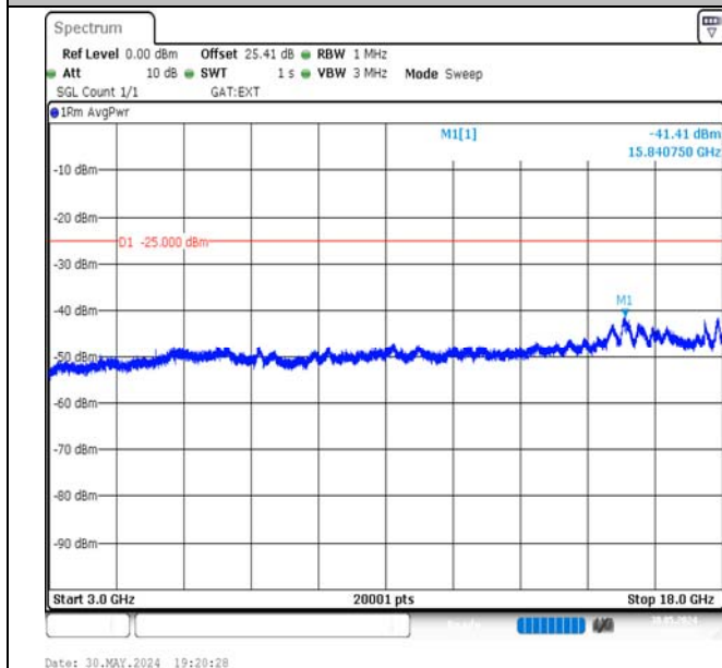
Band41-5MHz-QPSK-41565-25RB#0-3000~18000-PASS
