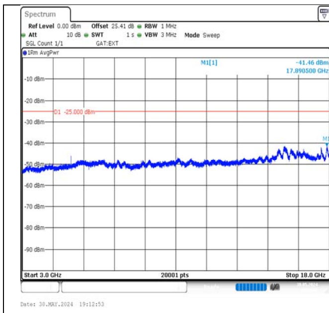
Band41-5MHz-QPSK-41565-1RB#0-3000~18000-PASS
