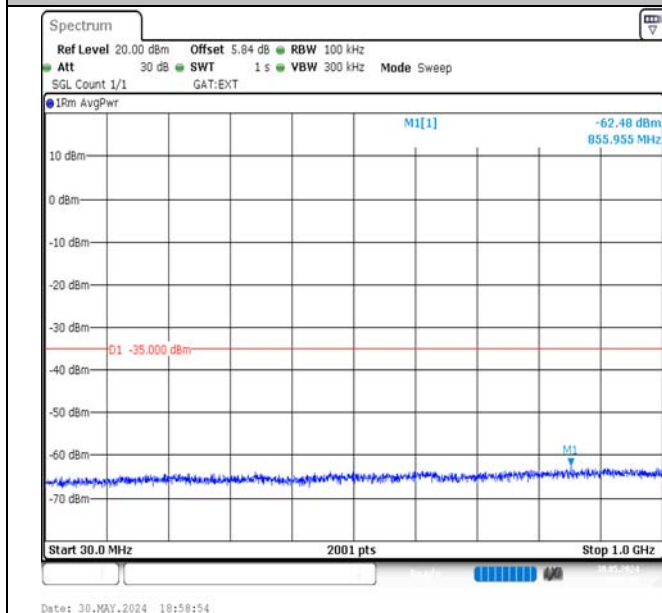
Band41-5MHz-16QAM-39675-25RB#0-30~1000-PASS
