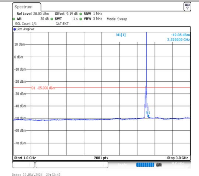
Band41-10MHz-QPSK-39700-1RB#49-1000~3000-PASS
