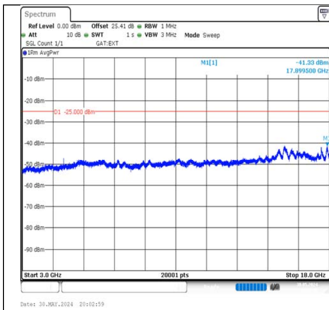
Band41-10MHz-QPSK-39700-1RB#49-3000~18000-PASS
