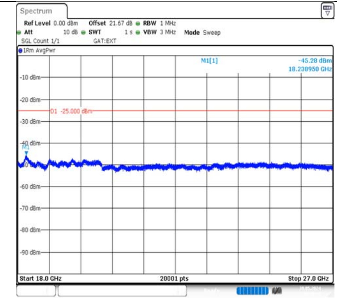
Band41-10MHz-QPSK-40620-50RB#0-18000~27000-PASS
