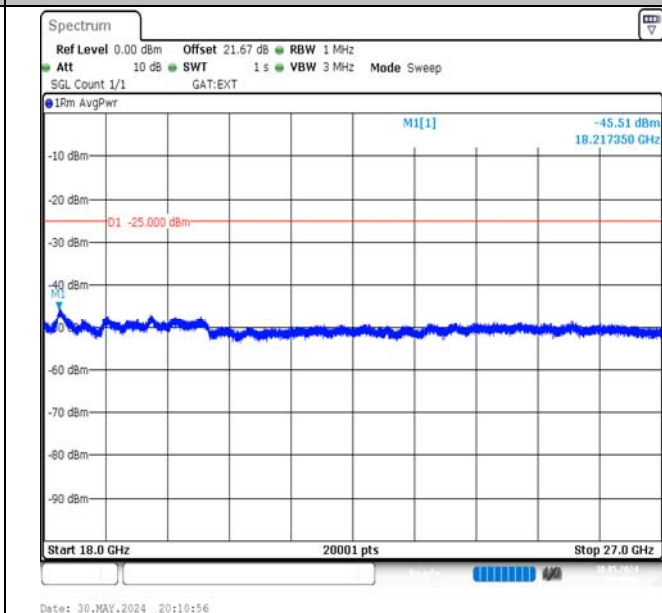
Band41-10MHz-QPSK-40620-1RB#0-18000~27000-PASS
