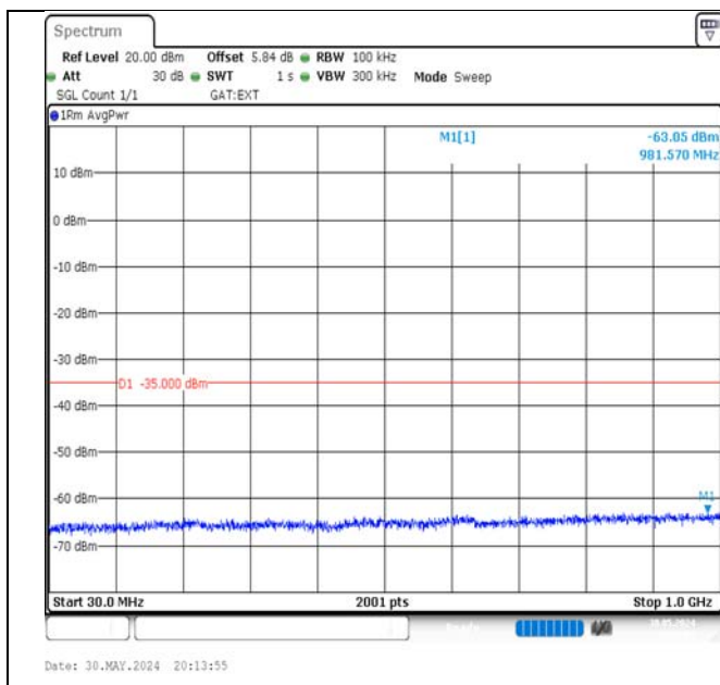
Band41-10MHz-QPSK-40620-1RB#49-30~1000-PASS
