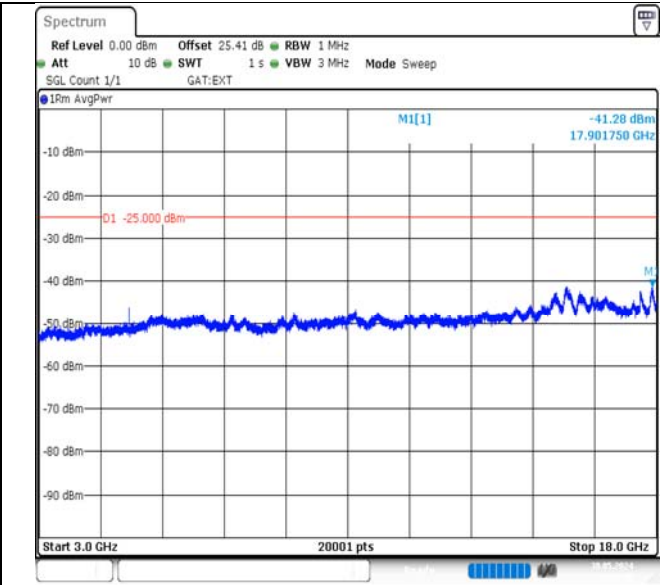
Band41-5MHz-16QAM-40620-1RB#0-3000~18000-PASS
