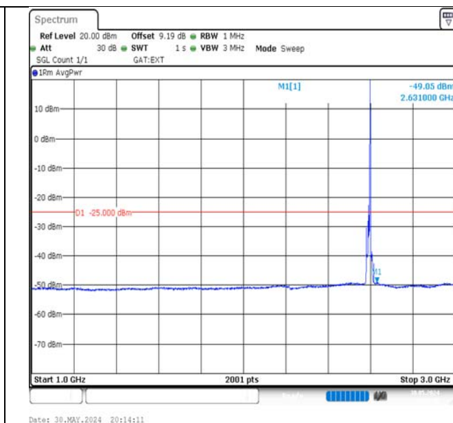
Band41-10MHz-QPSK-40620-1RB#49-1000~3000-PASS
