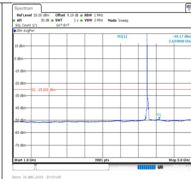
Band41-10MHz-16QAM-39700-1RB#0-1000~3000-PASS
