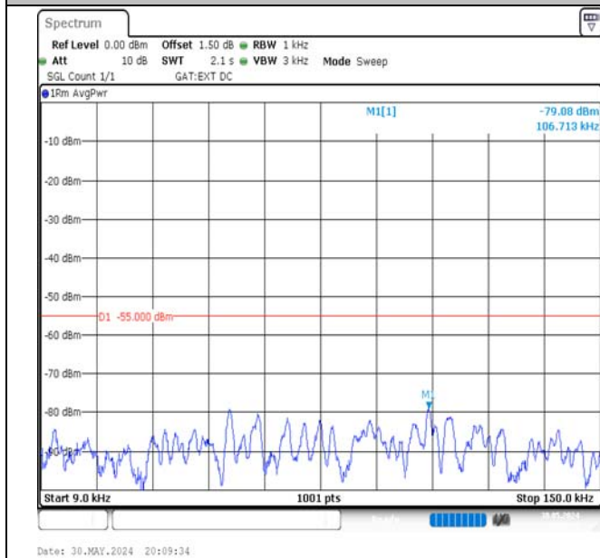
Band41-10MHz-QPSK-40620-1RB#0-0.009~0.15-PASS
