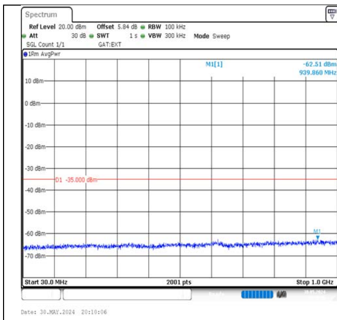
Band41-10MHz-QPSK-40620-1RB#0-30~1000-PASS
