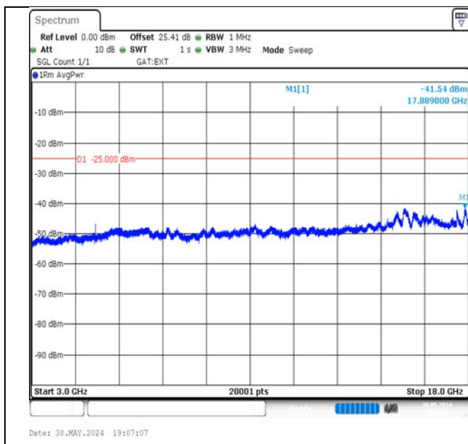
Band41-5MHz-16QAM-40620-1RB#24-3000~18000-PASS
