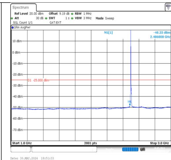
Band41-5MHz-16QAM-39675-1RB#0-1000~3000-PASS
