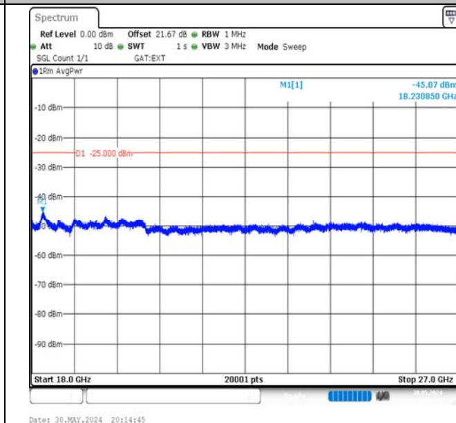
Band41-10MHz-QPSK-40620-1RB#49-18000~27000-PASS
