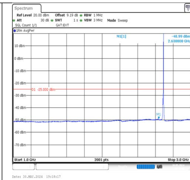
Band41-5MHz-16QAM-41565-1RB#24-1000~3000-PASS
