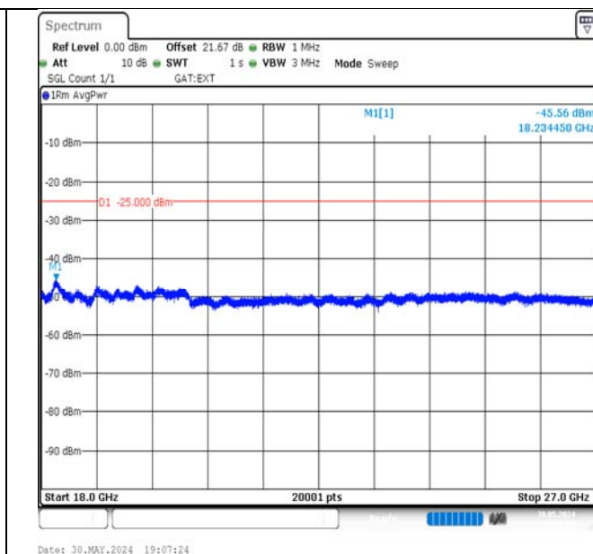
Band41-5MHz-16QAM-40620-1RB#24-18000~27000-PASS
