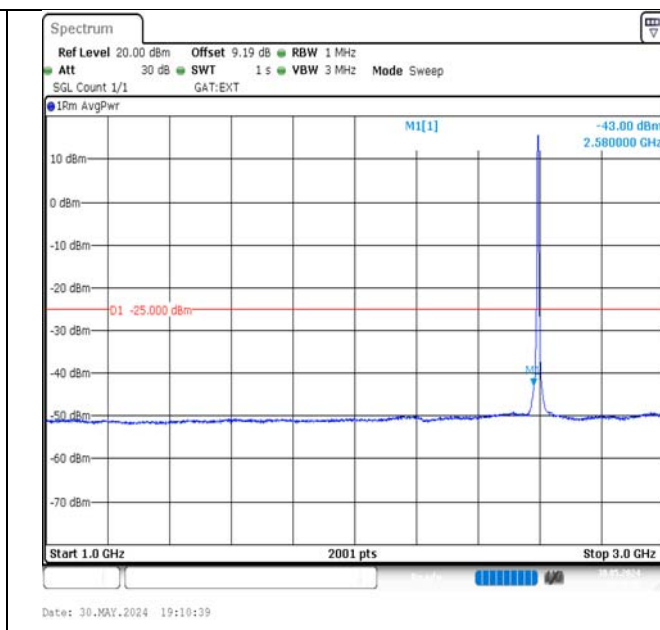
Band41-5MHz-16QAM-40620-25RB#0-1000~3000-PASS
