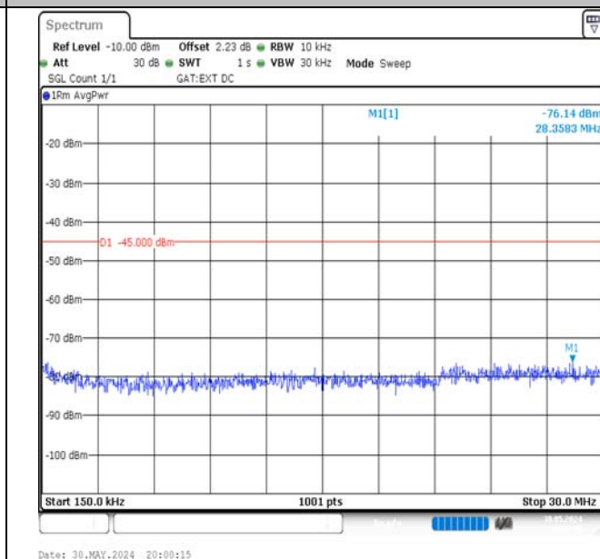
Band41-10MHz-16QAM-39700-1RB#0-0.15~30-PASS
