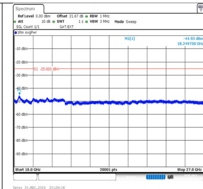
Band41-10MHz-QPSK-41540-1RB#49-18000~27000-PASS
