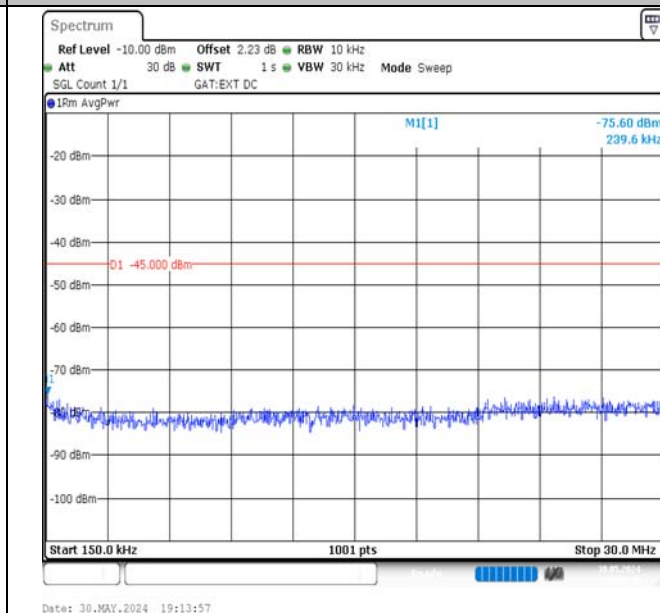
Band41-5MHz-16QAM-41565-1RB#0-0.15~30-PASS
