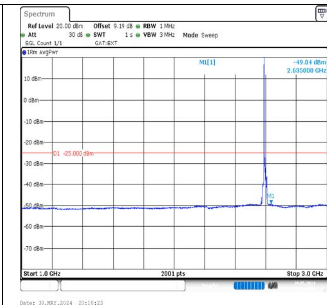
Band41-10MHz-QPSK-40620-1RB#0-1000~3000-PASS
