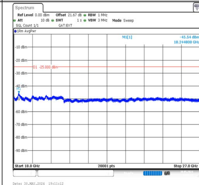
Band41-5MHz-16QAM-40620-25RB#0-18000~27000-PASS
