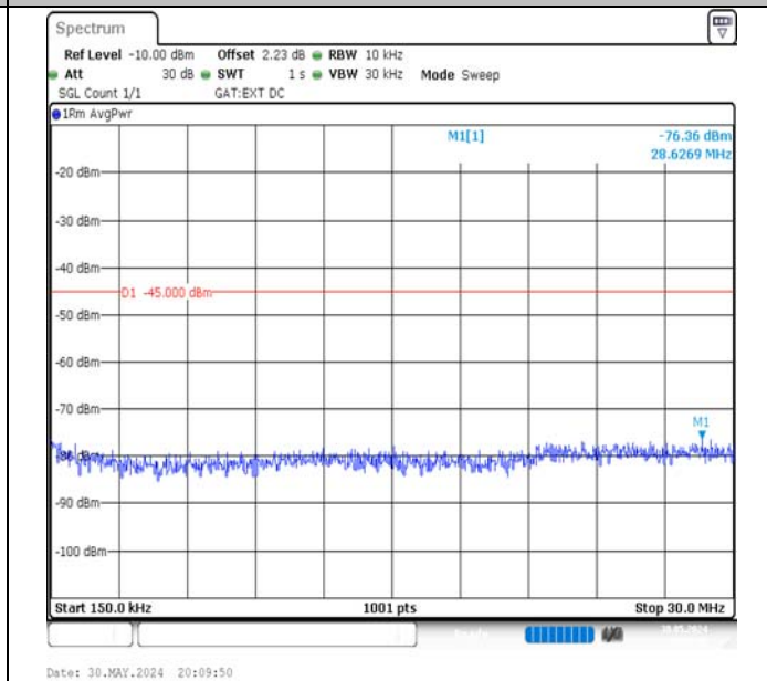
Band41-10MHz-QPSK-40620-1RB#0-0.15~30-PASS
