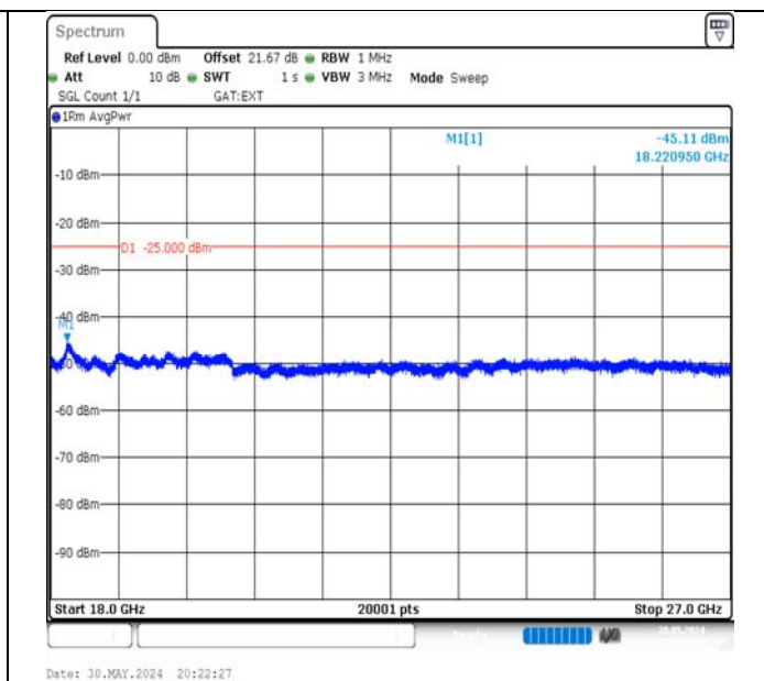
Band41-10MHz-QPSK-41540-1RB#0-18000~27000-PASS
