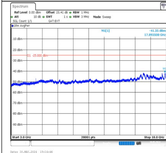
Band41-5MHz-16QAM-41565-1RB#0-3000~18000-PASS
