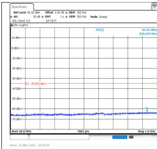
Band41-5MHz-QPSK-41565-25RB#0-30~1000-PASS
