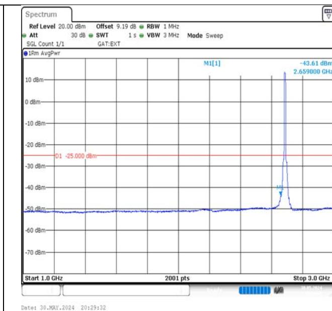
Band41-10MHz-QPSK-41540-50RB#0-1000~3000-PASS
