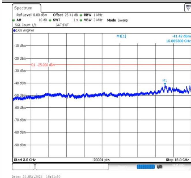
Band41-5MHz-16QAM-39675-1RB#0-3000~18000-PASS
