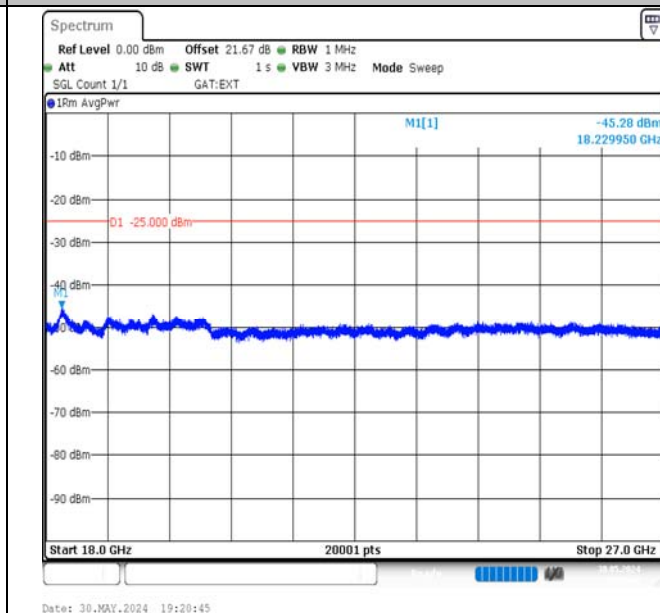
Band41-5MHz-QPSK-41565-25RB#0-18000~27000-PASS
