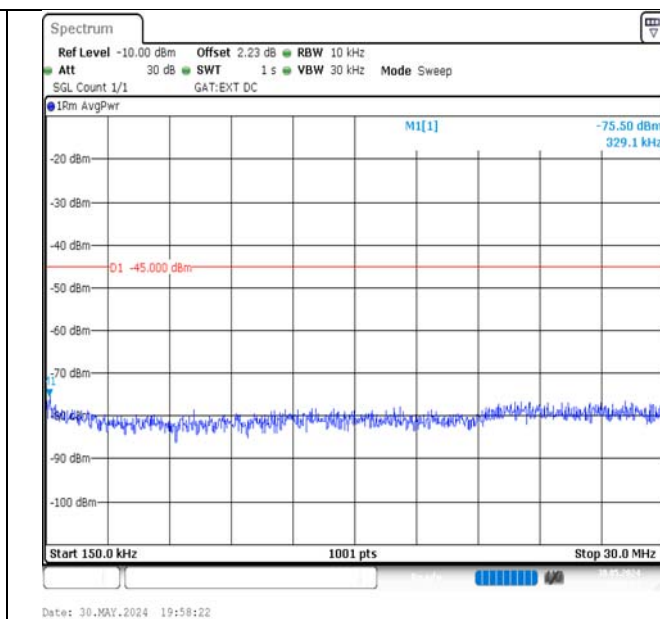
Band41-10MHz-QPSK-39700-1RB#0-0.15~30-PASS
