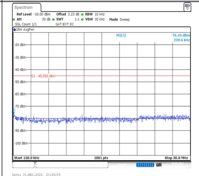
Band41-10MHz-QPSK-41540-50RB#0-0.15~30-PASS
