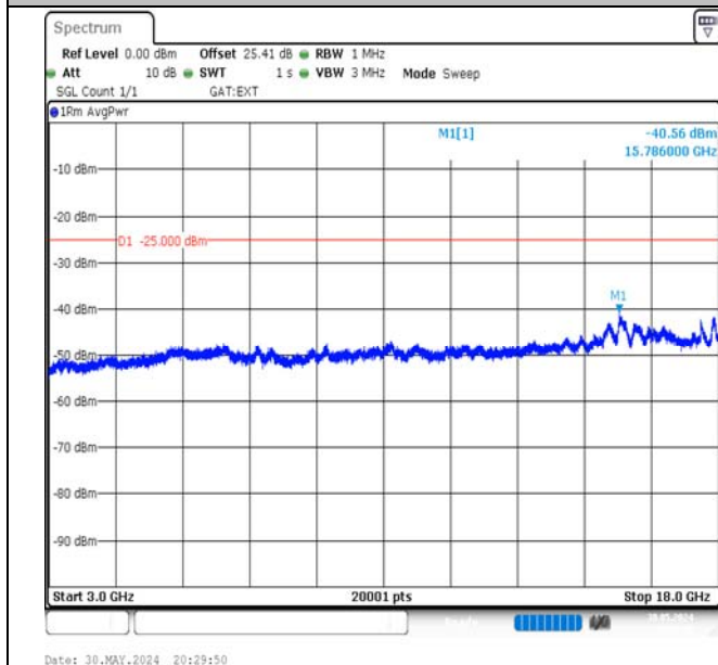
Band41-10MHz-QPSK-41540-50RB#0-3000~18000-PASS
