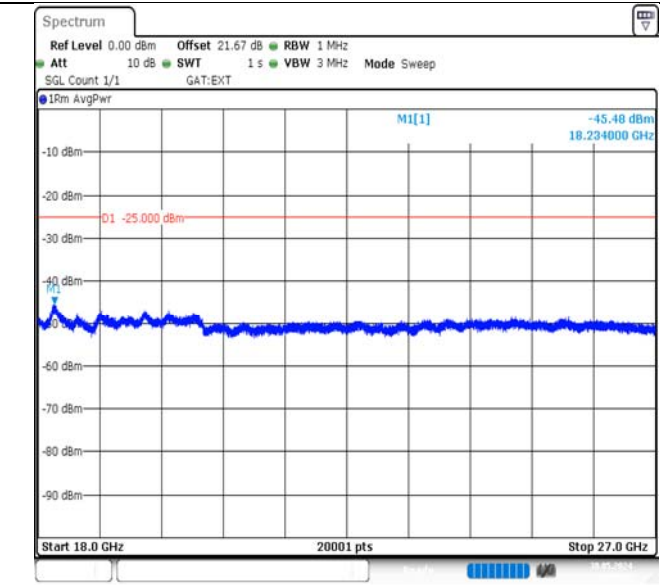
Band41-10MHz-QPSK-39700-1RB#0-18000~27000-PASS
