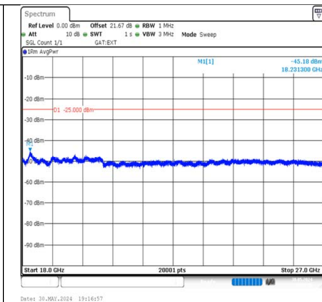
Band41-5MHz-QPSK-41565-1RB#24-18000~27000-PASS
