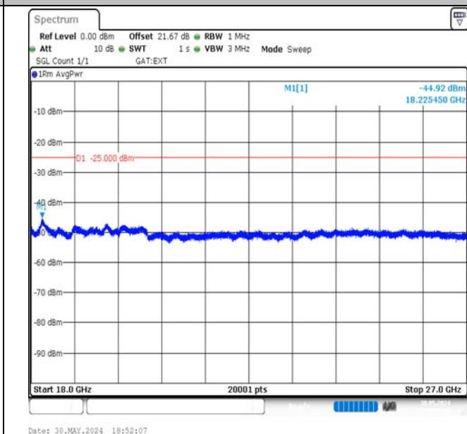
Band41-5MHz-16QAM-39675-1RB#0-18000~27000-PASS
