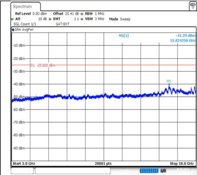
Band41-10MHz-QPSK-39700-1RB#0-3000~18000-PASS
