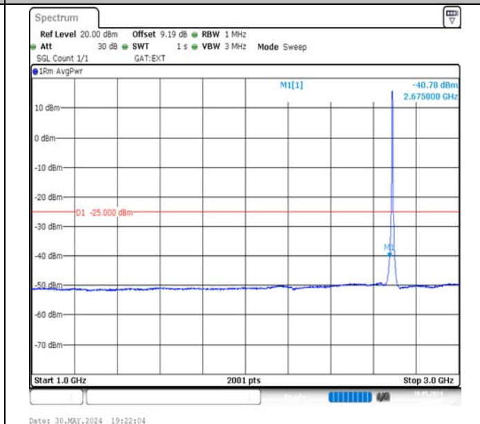
Band41-5MHz-16QAM-41565-25RB#0-1000~3000-PASS
