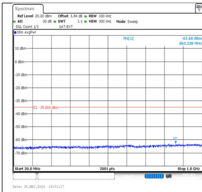
Band41-5MHz-16QAM-39675-1RB#0-30~1000-PASS
