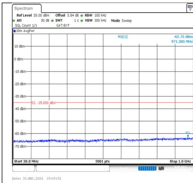
Band41-5MHz-QPSK-40620-1RB#0-30~1000-PASS
