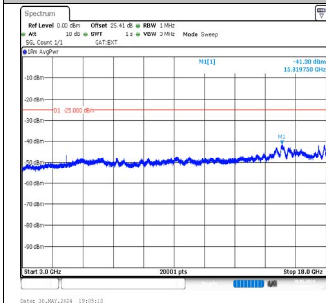
Band41-5MHz-QPSK-40620-1RB#24-3000~18000-PASS
