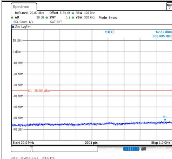
Band38-20MHz-QPSK-38000-100RB#0-30~1000-PASS
