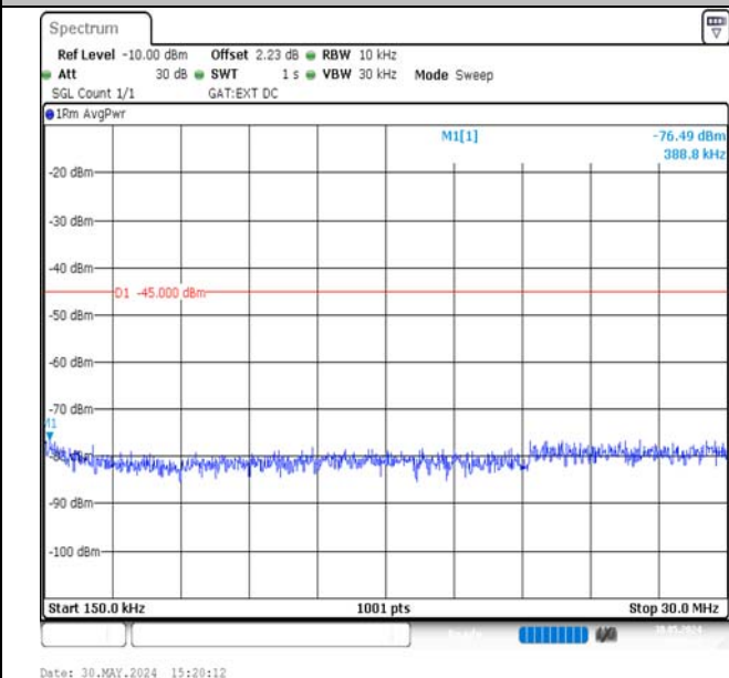
Band38-20MHz-16QAM-37850-1RB#99-0.15~30-PASS
