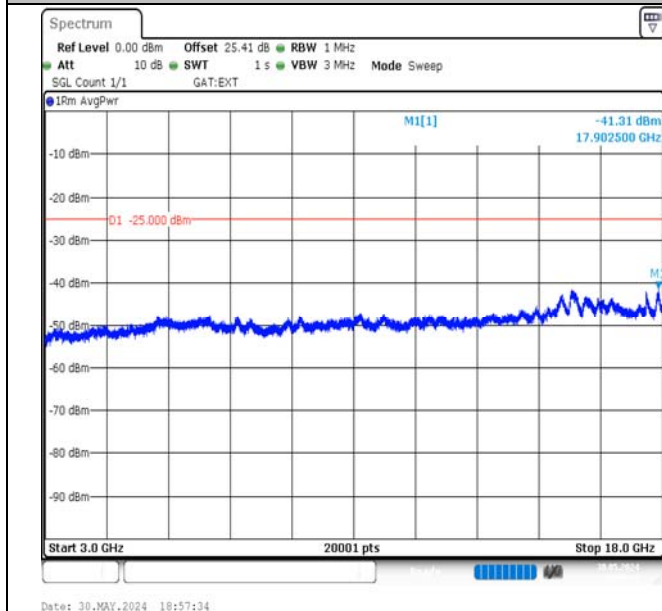
Band41-5MHz-QPSK-39675-25RB#0-3000~18000-PASS
