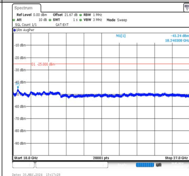
Band38-20MHz-16QAM-37850-1RB#0-18000~27000-PASS
