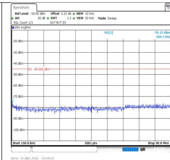
Band41-5MHz-QPSK-40620-25RB#0-0.15~30-PASS
