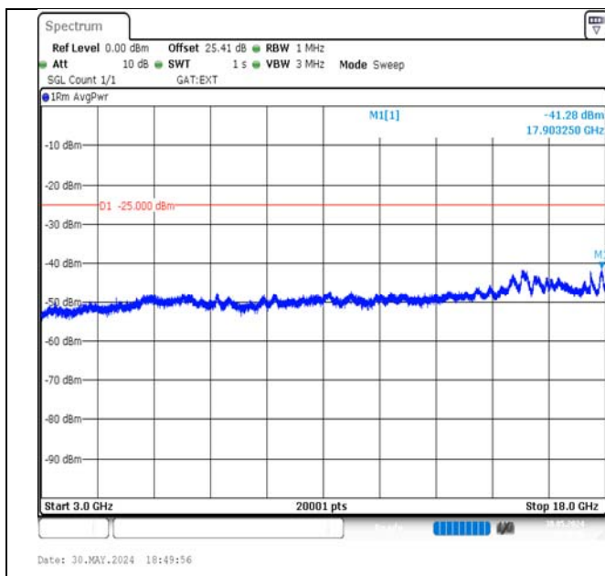
Band41-5MHz-QPSK-39675-1RB#0-3000~18000-PASS
