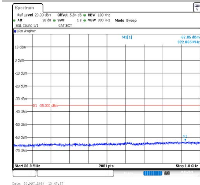
Band38-20MHz-16QAM-38150-100RB#0-30~1000-PASS
