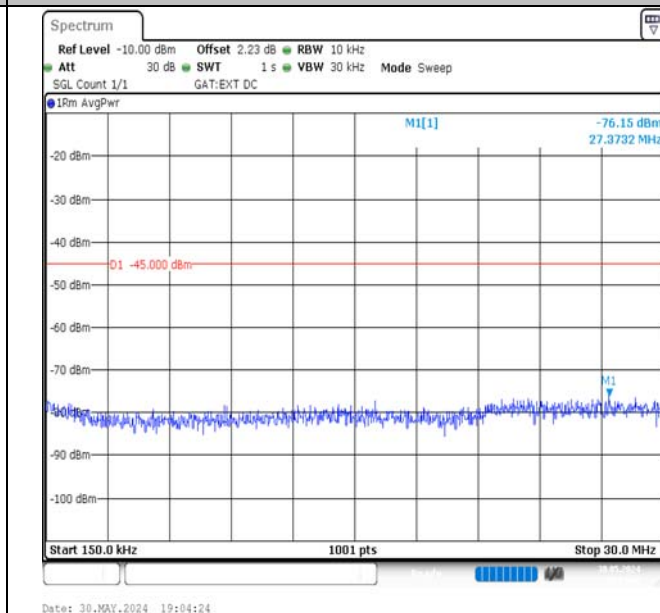
Band41-5MHz-QPSK-40620-1RB#24-0.15~30-PASS
