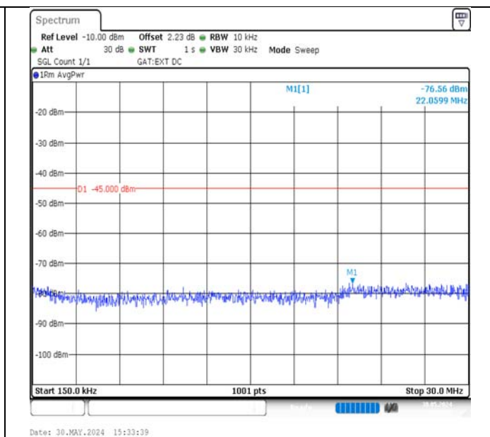
Band38-20MHz-QPSK-38000-100RB#0-0.15~30-PASS
