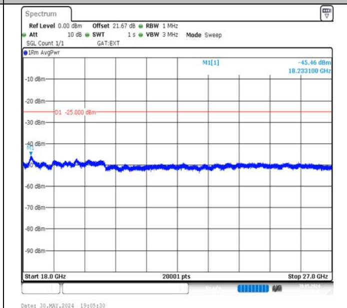
Band41-5MHz-QPSK-40620-1RB#24-18000~27000-PASS
