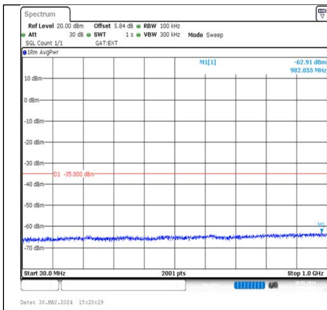
Band38-20MHz-16QAM-37850-1RB#99-30~1000-PASS
