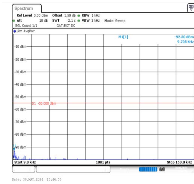
Band38-20MHz-16QAM-38150-100RB#0-0.009~0.15-PASS
