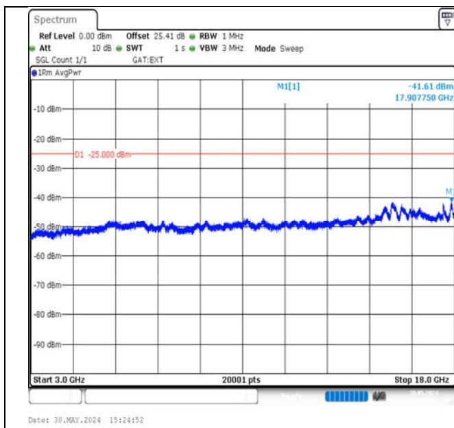
Band38-20MHz-16QAM-37850-100RB#0-3000~18000-PASS
