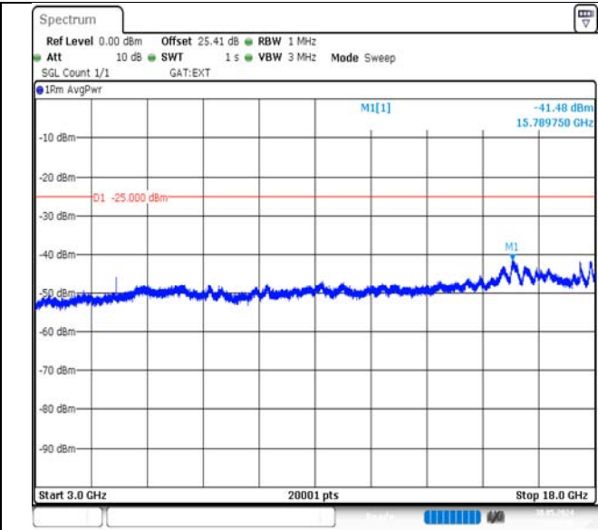
Band38-20MHz-16QAM-38000-1RB#0-3000~18000-PASS
