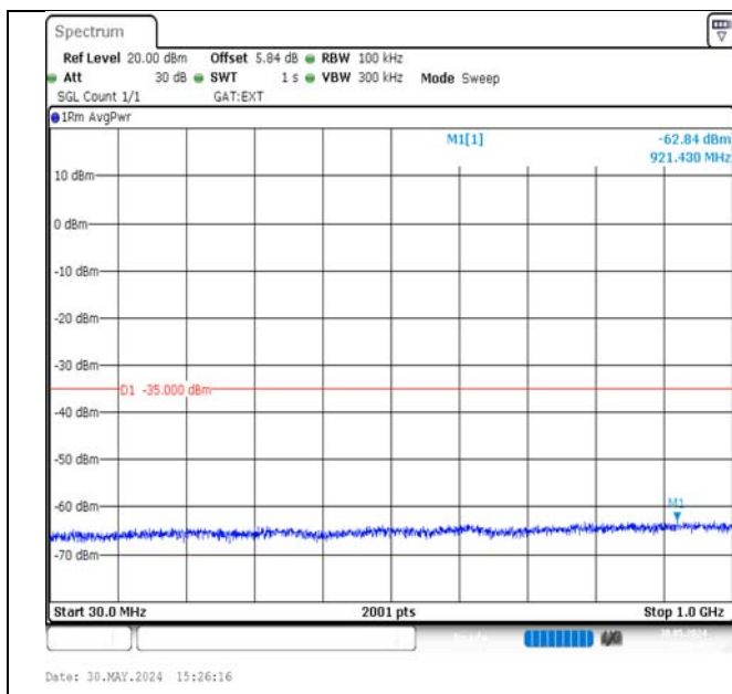
Band38-20MHz-QPSK-38000-1RB#0-30~1000-PASS
