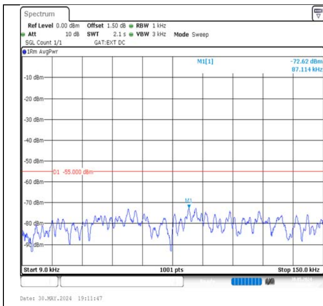
Band41-5MHz-QPSK-41565-1RB#0-0.009~0.15-PASS
