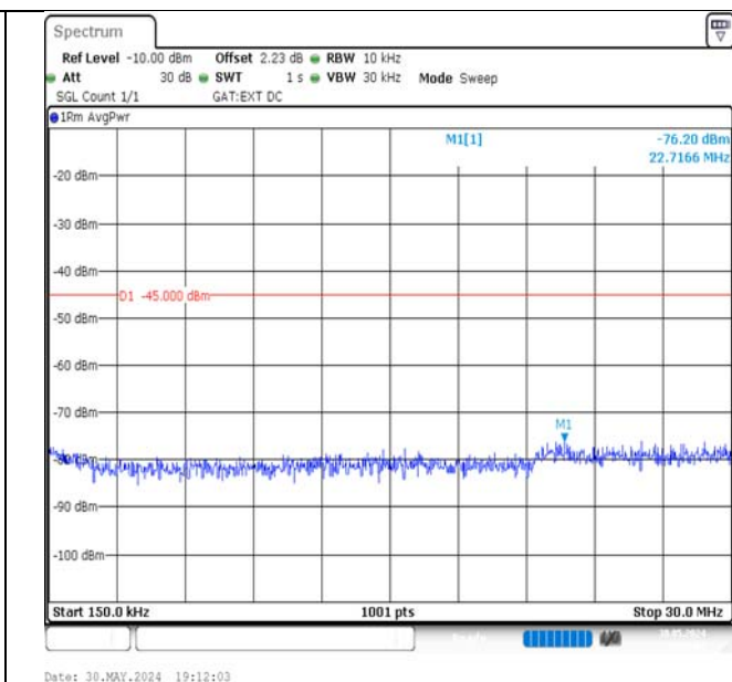
Band41-5MHz-QPSK-41565-1RB#0-0.15~30-PASS
