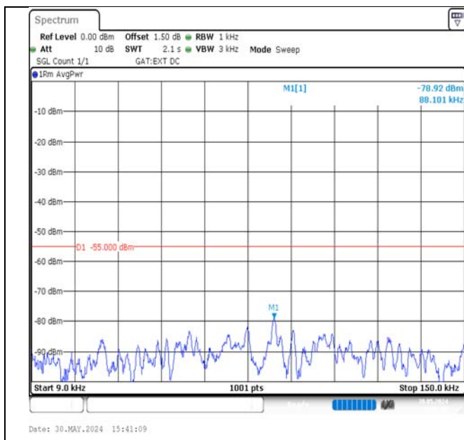
Band38-20MHz-QPSK-38150-1RB#99-0.009~0.15-PASS
