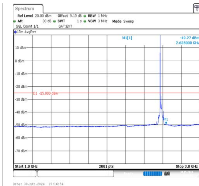
Band38-20MHz-16QAM-37850-1RB#0-1000~3000-PASS
