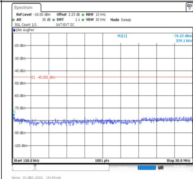
Band41-5MHz-QPSK-39675-25RB#0-0.15~30-PASS
