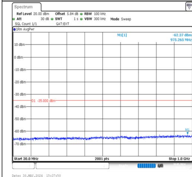
Band38-20MHz-QPSK-38150-1RB#0-30~1000-PASS
