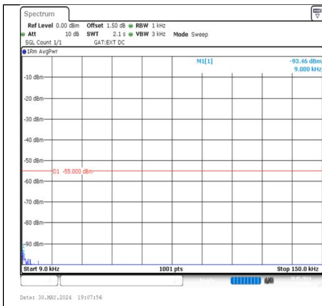
Band41-5MHz-QPSK-40620-25RB#0-0.009~0.15-PASS
