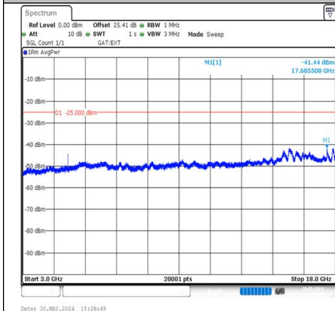
Band38-20MHz-QPSK-38000-1RB#0-3000~18000-PASS
