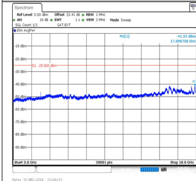
Band38-20MHz-16QAM-38150-1RB#99-3000~18000-PASS
