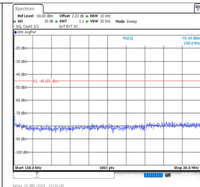
Band38-20MHz-16QAM-38000-1RB#99-0.15~30-PASS
