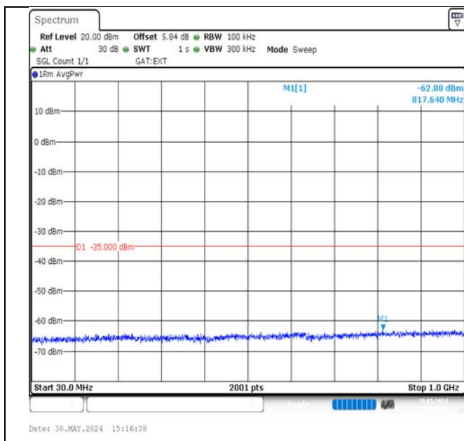
Band38-20MHz-16QAM-37850-1RB#0-30~1000-PASS
