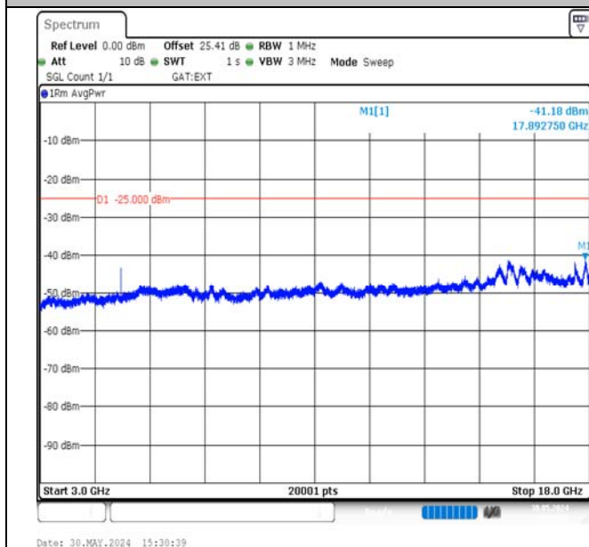
Band38-20MHz-QPSK-38000-1RB#99-3000~18000-PASS
