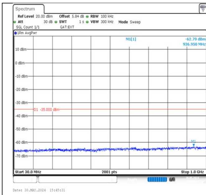
Band38-20MHz-QPSK-38150-100RB#0-30~1000-PASS
