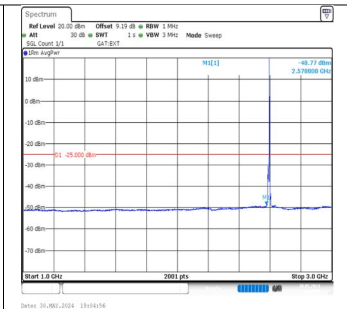
Band41-5MHz-QPSK-40620-1RB#24-1000~3000-PASS
