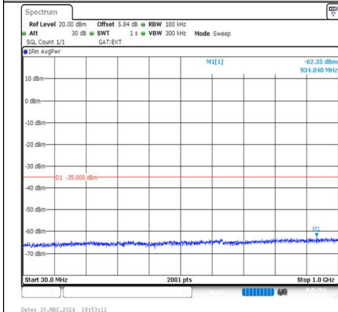
Band41-5MHz-QPSK-39675-1RB#24-30~1000-PASS
