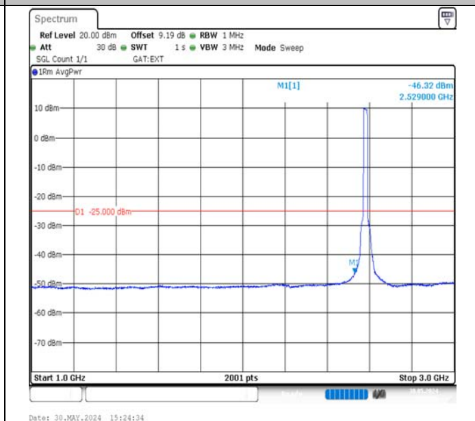
Band38-20MHz-16QAM-37850-100RB#0-1000~3000-PASS
