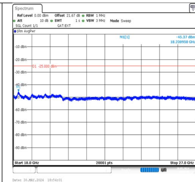
Band41-5MHz-QPSK-39675-1RB#24-18000~27000-PASS
