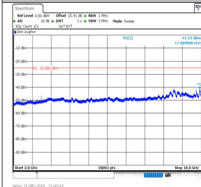
Band38-20MHz-16QAM-38150-1RB#0-3000~18000-PASS
