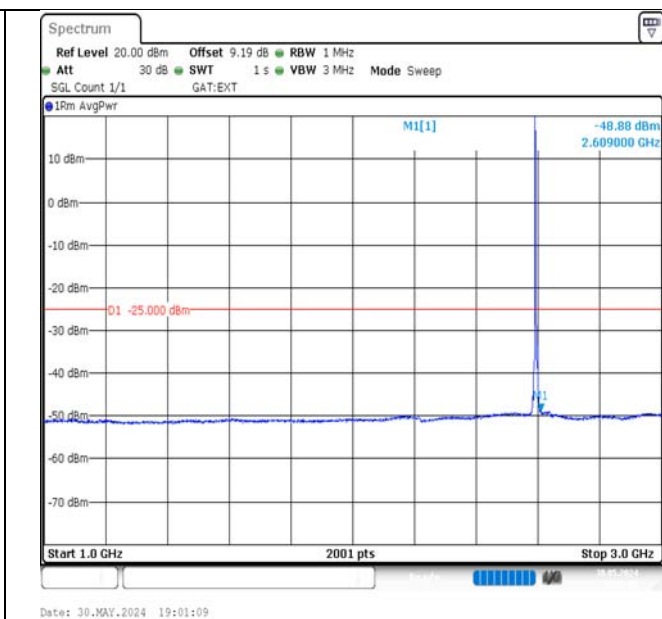
Band41-5MHz-QPSK-40620-1RB#0-1000~3000-PASS
