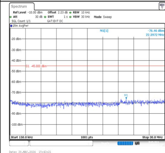
Band38-20MHz-16QAM-38150-1RB#99-0.15~30-PASS
