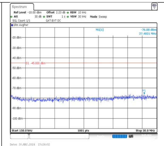
Band38-20MHz-16QAM-37850-100RB#0-0.15~30-PASS
