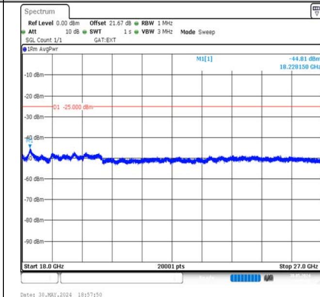
Band41-5MHz-QPSK-39675-25RB#0-18000~27000-PASS
