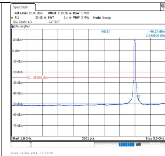
Band38-20MHz-16QAM-38000-100RB#0-1000~3000-PASS
