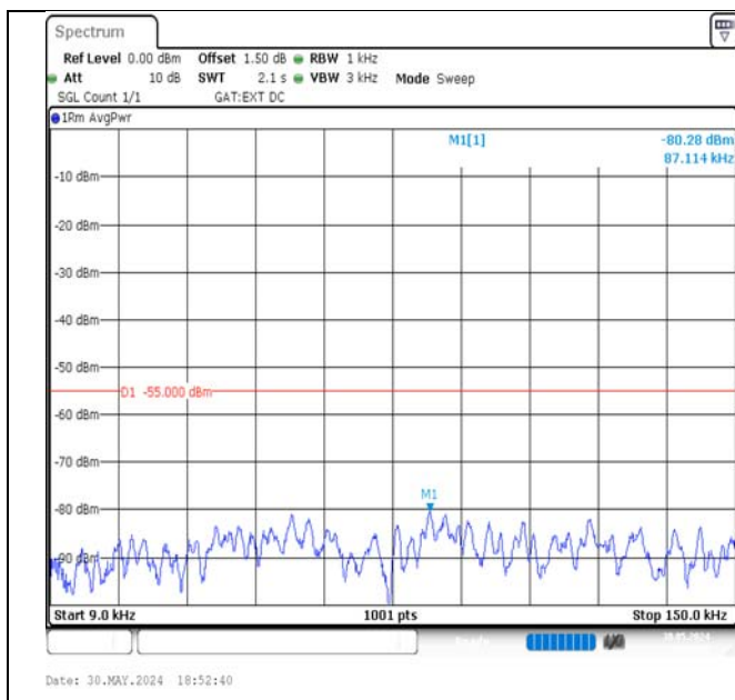
Band41-5MHz-QPSK-39675-1RB#24-0.009~0.15-PASS
