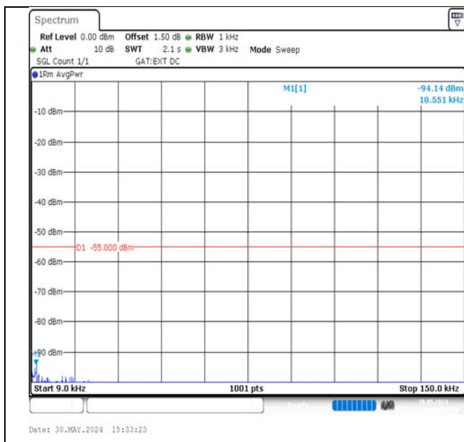
Band38-20MHz-QPSK-38000-100RB#0-0.009~0.15-PASS
