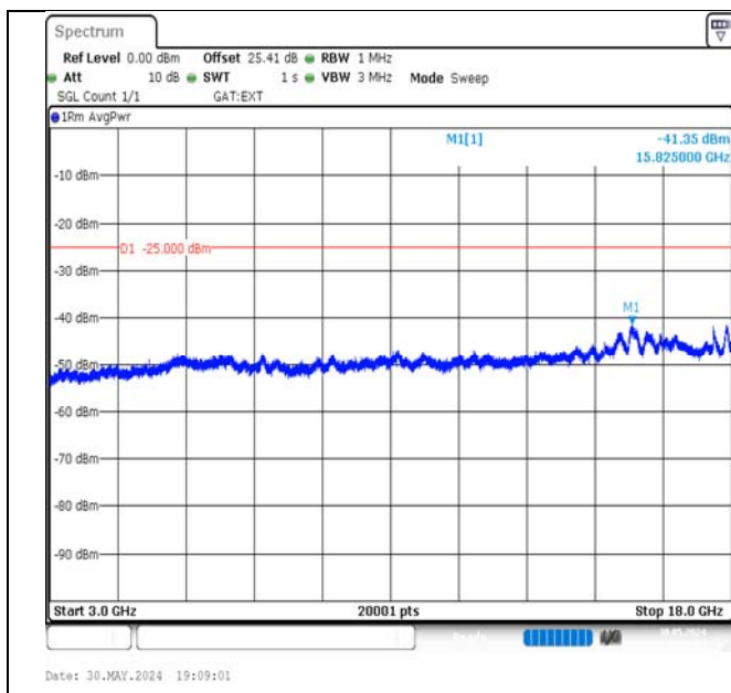
Band41-5MHz-QPSK-40620-25RB#0-3000~18000-PASS
