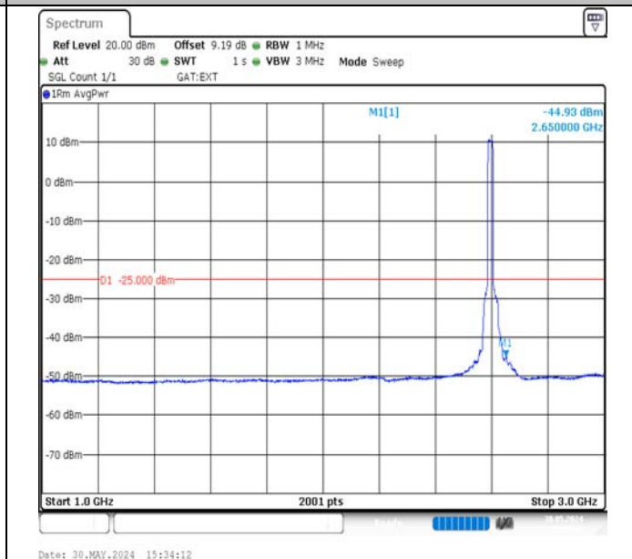
Band38-20MHz-QPSK-38000-100RB#0-1000~3000-PASS
