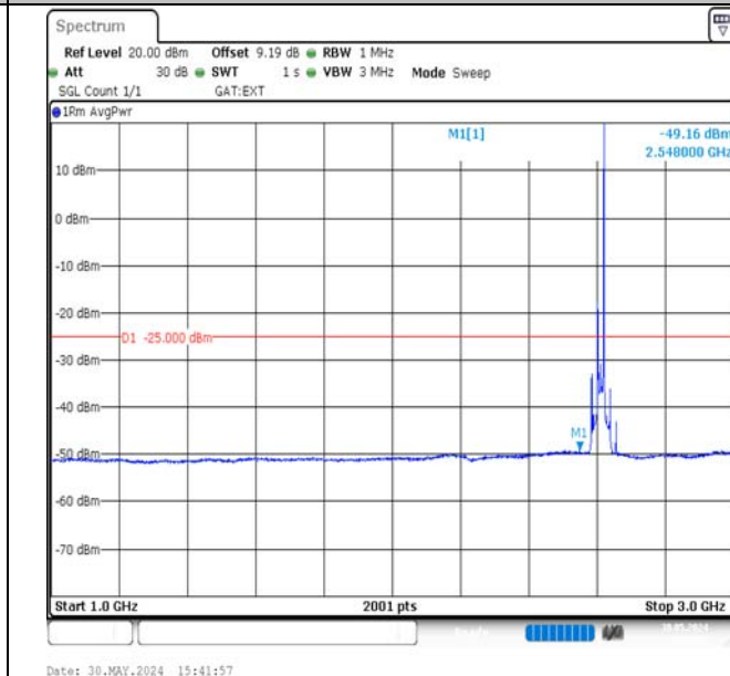
Band38-20MHz-QPSK-38150-1RB#99-1000~3000-PASS
