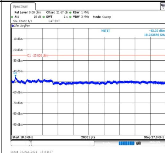
Band38-20MHz-16QAM-38150-1RB#99-18000~27000-PASS
