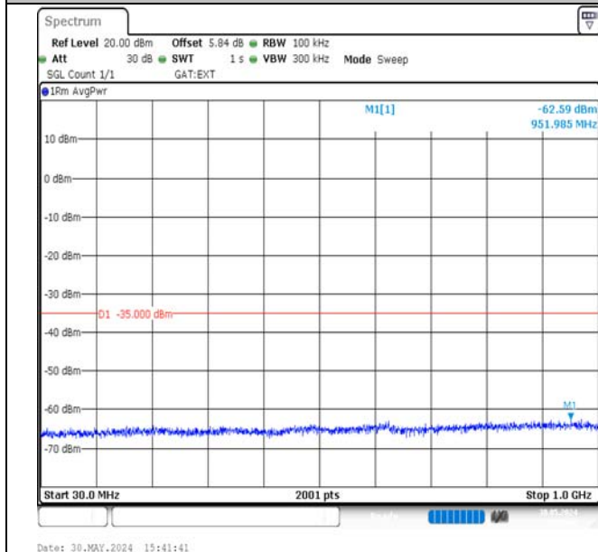
Band38-20MHz-QPSK-38150-1RB#99-30~1000-PASS
