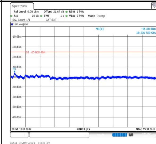
Band38-20MHz-16QAM-37850-1RB#99-18000~27000-PASS
