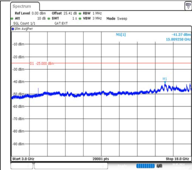
Band38-20MHz-QPSK-38150-1RB#99-3000~18000-PASS
