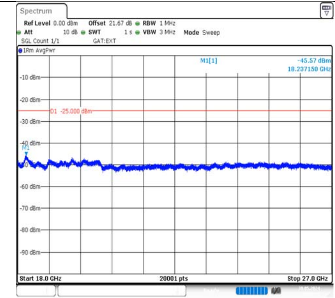
Band38-20MHz-QPSK-38150-1RB#99-18000~27000-PASS
