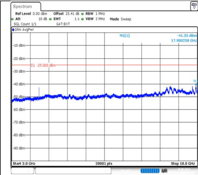
Band38-20MHz-16QAM-38000-1RB#99-3000~18000-PASS
