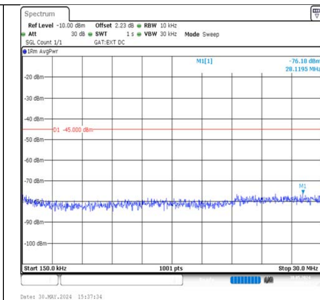
Band38-20MHz-QPSK-38150-1RB#0-0.15~30-PASS
