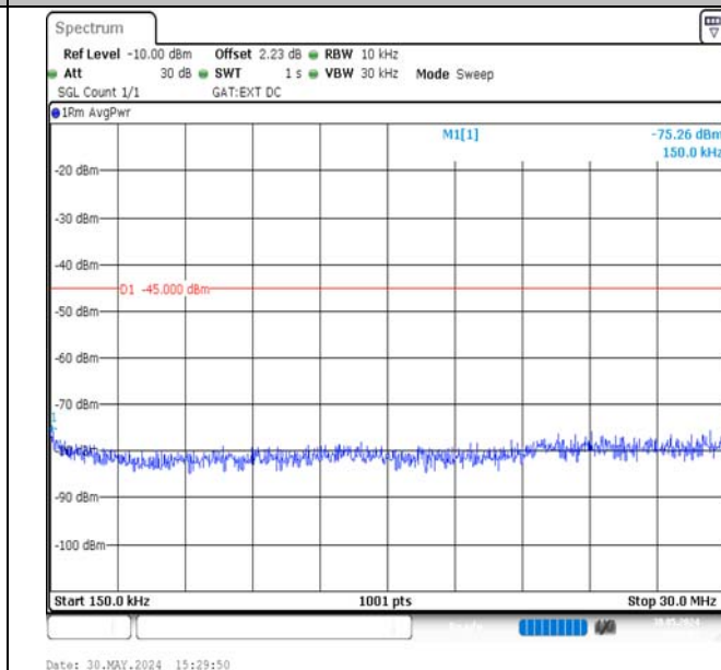
Band38-20MHz-QPSK-38000-1RB#99-0.15~30-PASS
