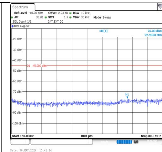
Band38-20MHz-QPSK-38150-1RB#99-0.15~30-PASS
