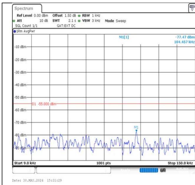
Band38-20MHz-16QAM-38000-1RB#99-0.009~0.15-PASS
