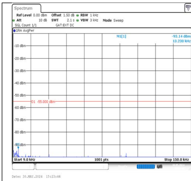
Band38-20MHz-16QAM-37850-100RB#0-0.009~0.15-PASS
