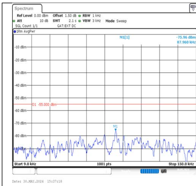
Band38-20MHz-QPSK-38150-1RB#0-0.009~0.15-PASS
