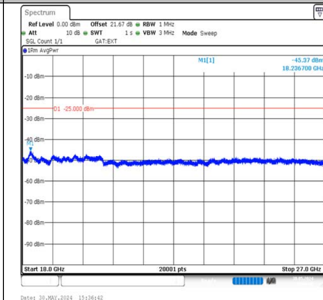
Band38-20MHz-16QAM-38000-100RB#0-18000~27000-PASS
