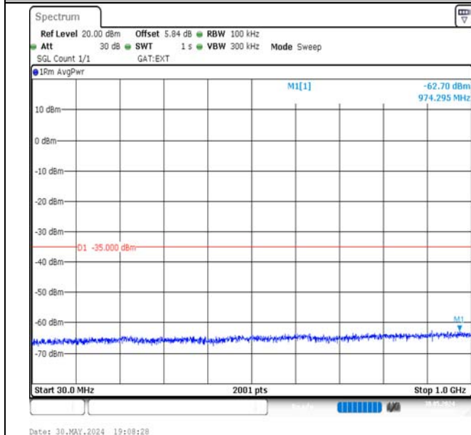
Band41-5MHz-QPSK-40620-25RB#0-30~1000-PASS
