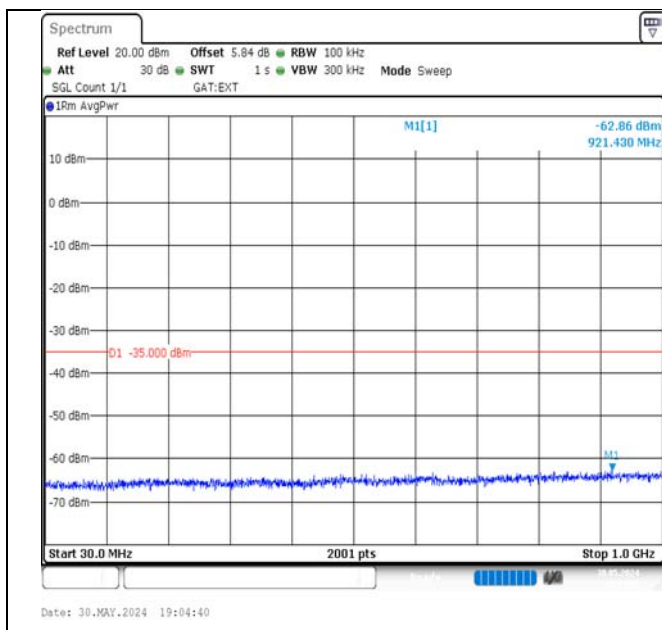
Band41-5MHz-QPSK-40620-1RB#24-30~1000-PASS
