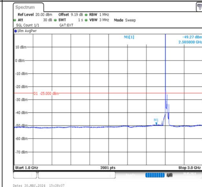
Band38-20MHz-QPSK-38150-1RB#0-1000~3000-PASS
