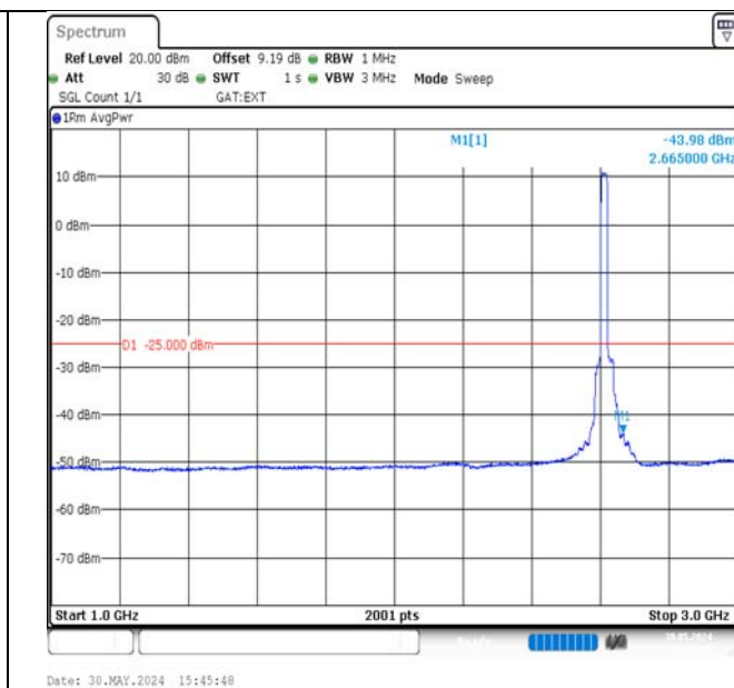
Band38-20MHz-QPSK-38150-100RB#0-1000~3000-PASS
