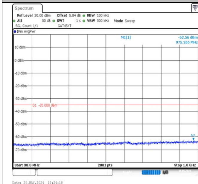
Band38-20MHz-16QAM-37850-100RB#0-30~1000-PASS
