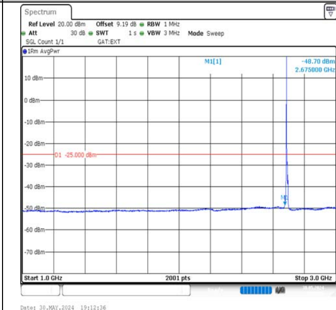
Band41-5MHz-QPSK-41565-1RB#0-1000~3000-PASS
