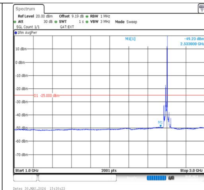
Band38-20MHz-QPSK-38000-1RB#99-1000~3000-PASS
