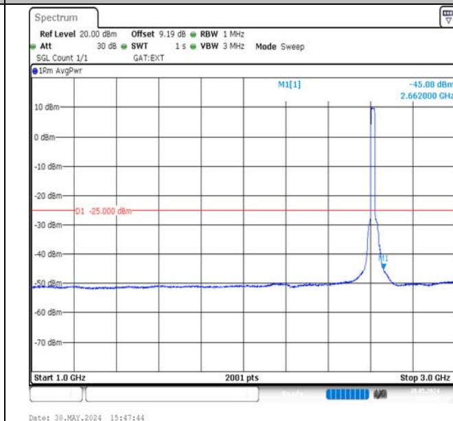
Band38-20MHz-16QAM-38150-100RB#0-1000~3000-PASS
