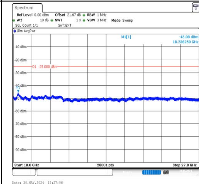
Band38-20MHz-QPSK-38000-1RB#0-18000~27000-PASS
