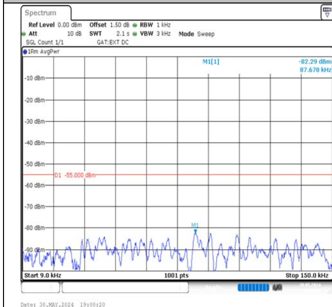
Band41-5MHz-QPSK-40620-1RB#0-0.009~0.15-PASS
