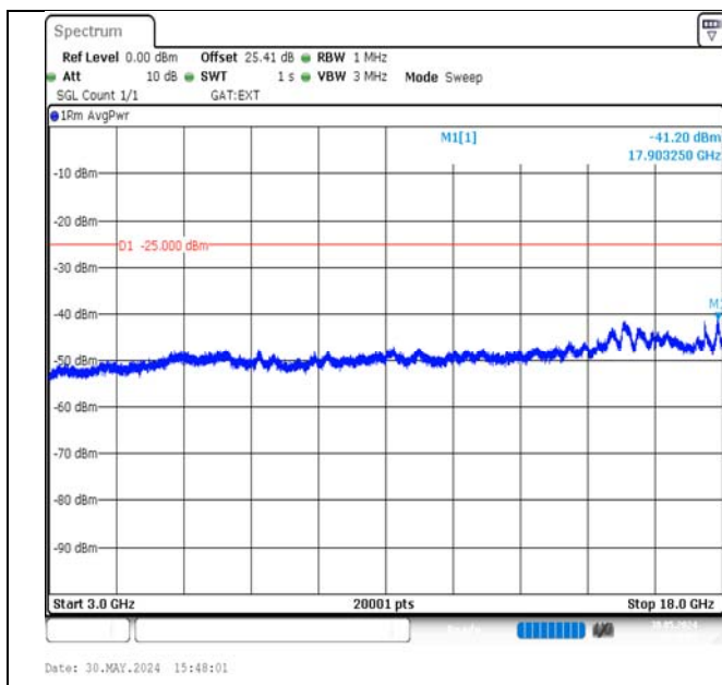
Band38-20MHz-16QAM-38150-100RB#0-3000~18000-PASS
