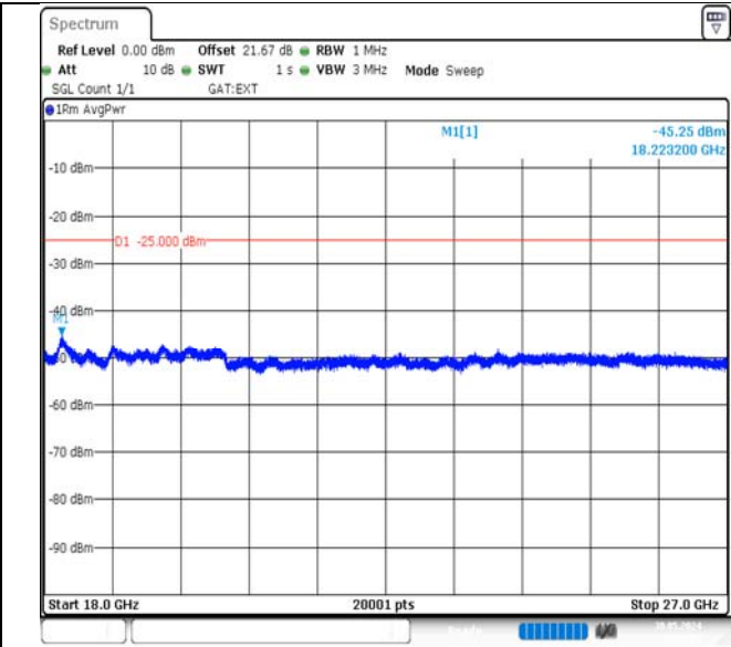
Band38-20MHz-16QAM-38000-1RB#99-18000~27000-PASS
