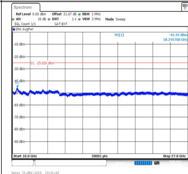
Band41-5MHz-QPSK-40620-1RB#0-18000~27000-PASS
