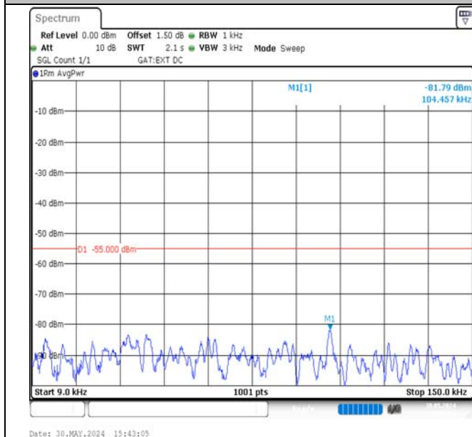
Band38-20MHz-16QAM-38150-1RB#99-0.009~0.15-PASS
