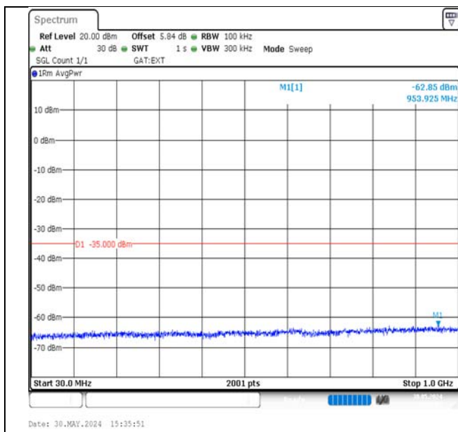
Band38-20MHz-16QAM-38000-100RB#0-30~1000-PASS
