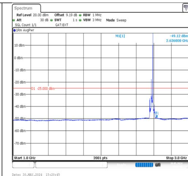
Band38-20MHz-16QAM-37850-1RB#99-1000~3000-PASS
