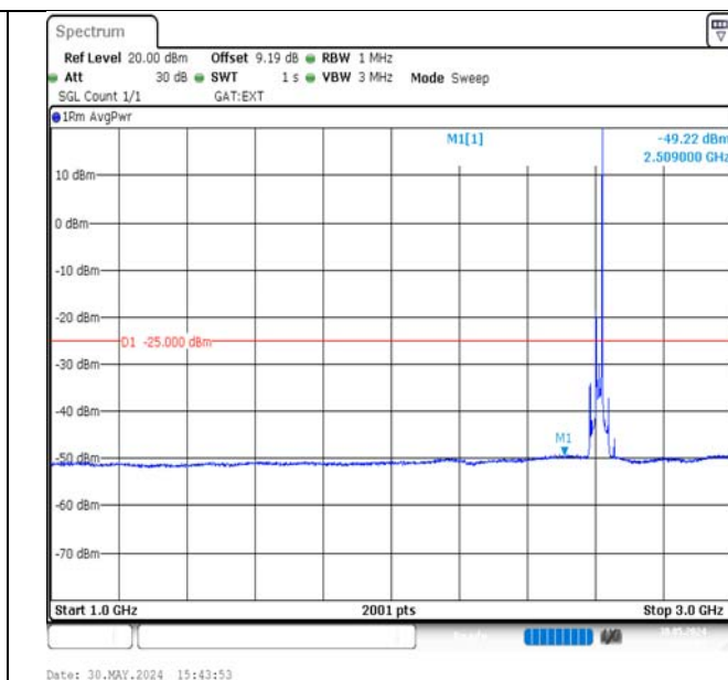
Band38-20MHz-16QAM-38150-1RB#99-1000~3000-PASS
