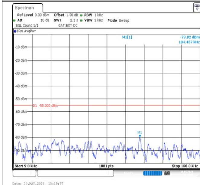
Band38-20MHz-16QAM-37850-1RB#99-0.009~0.15-PASS
