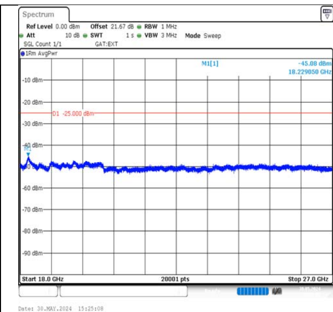
Band38-20MHz-16QAM-37850-100RB#0-18000~27000-PASS
