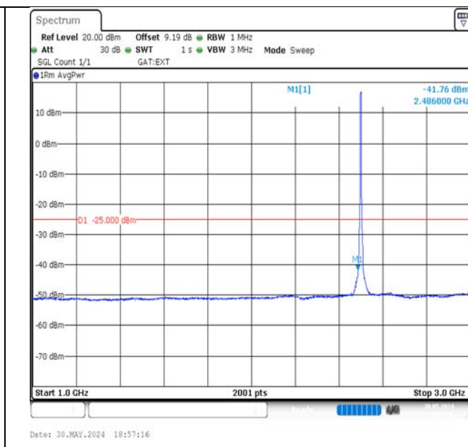
Band41-5MHz-QPSK-39675-25RB#0-1000~3000-PASS
