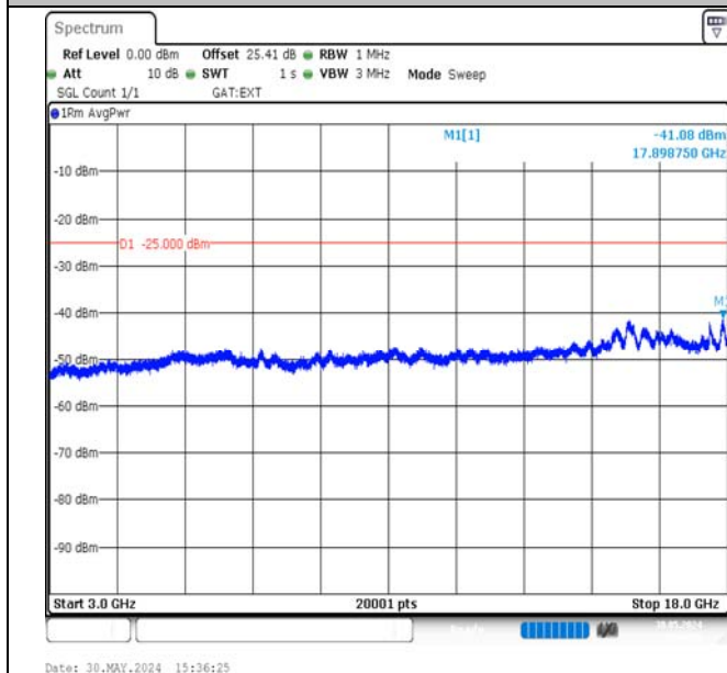
Band38-20MHz-16QAM-38000-100RB#0-3000~18000-PASS
