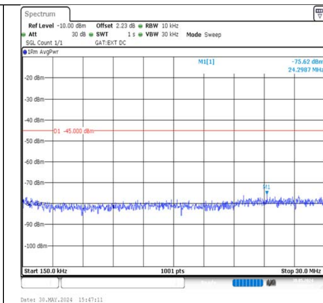
Band38-20MHz-16QAM-38150-100RB#0-0.15~30-PASS
