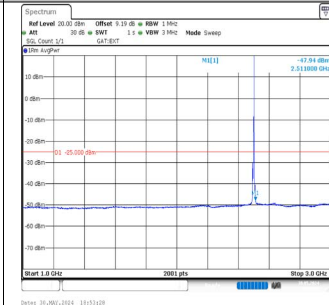
Band41-5MHz-QPSK-39675-1RB#24-1000~3000-PASS
