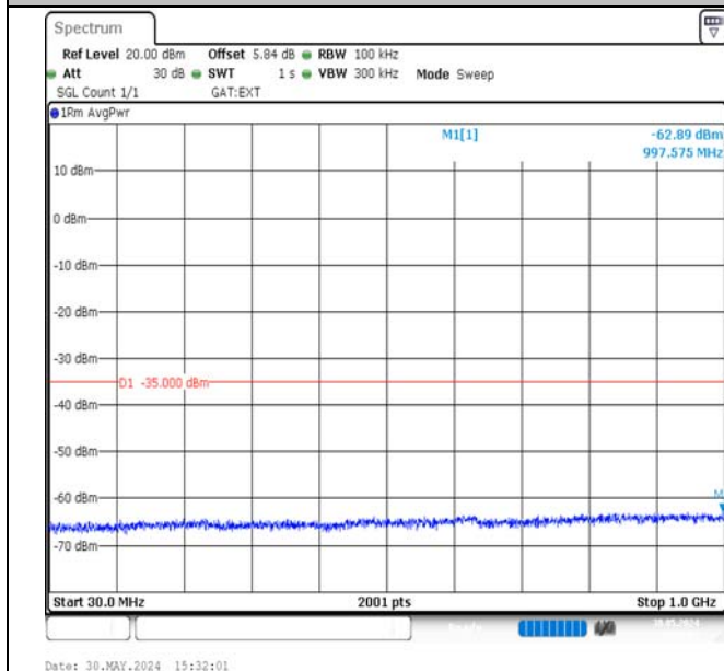
Band38-20MHz-16QAM-38000-1RB#99-30~1000-PASS
