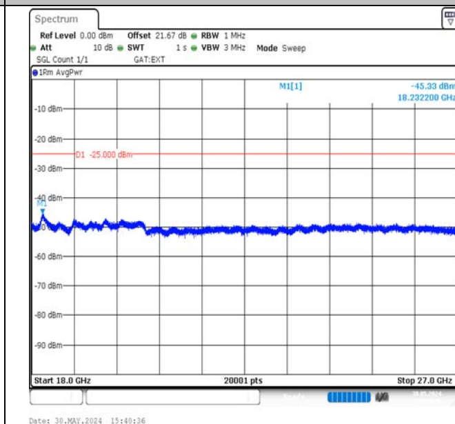
Band38-20MHz-16QAM-38150-1RB#0-18000~27000-PASS
