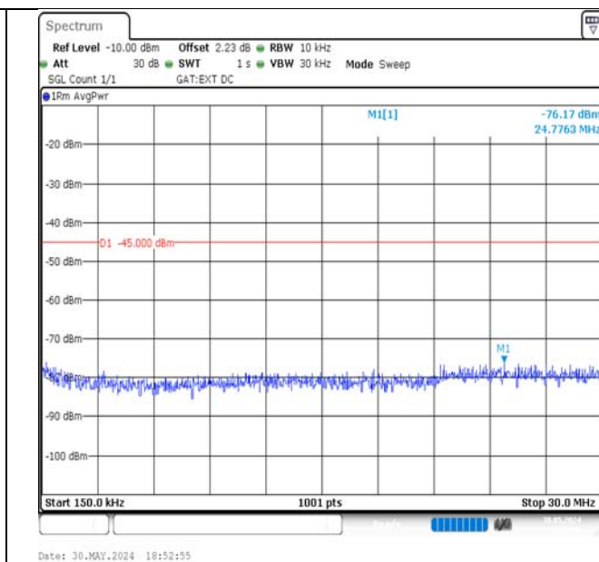
Band41-5MHz-QPSK-39675-1RB#24-0.15~30-PASS
