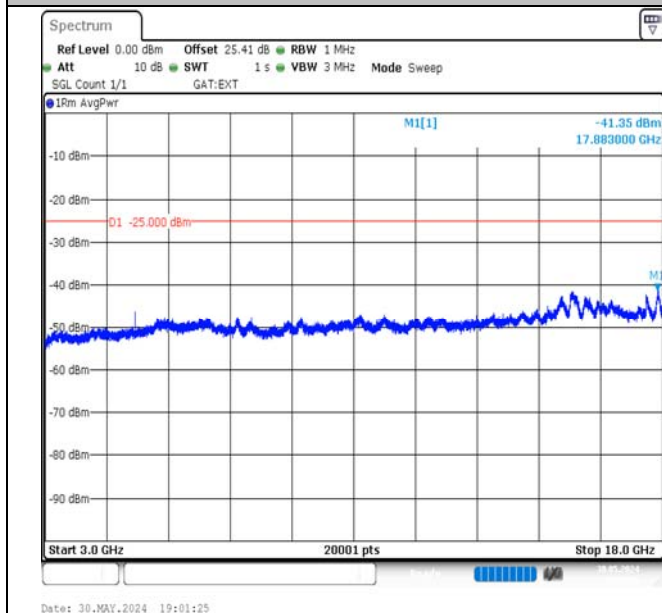
Band41-5MHz-QPSK-40620-1RB#0-3000~18000-PASS
