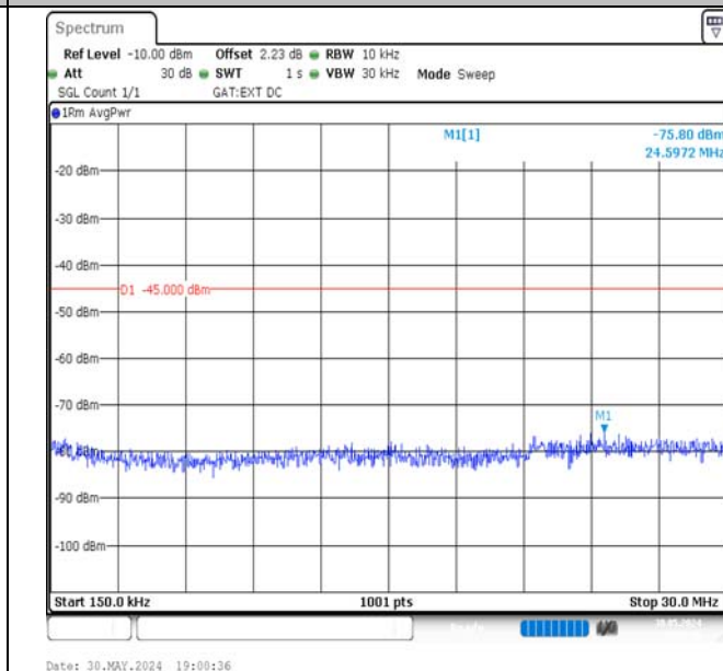
Band41-5MHz-QPSK-40620-1RB#0-0.15~30-PASS
