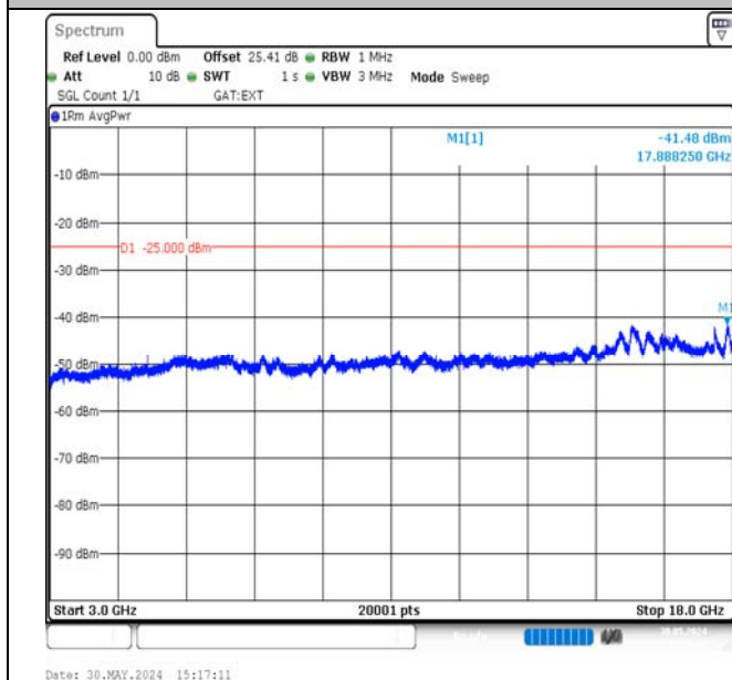
Band38-20MHz-16QAM-37850-1RB#0-3000~18000-PASS
