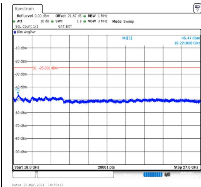
Band41-5MHz-QPSK-39675-1RB#0-18000~27000-PASS
