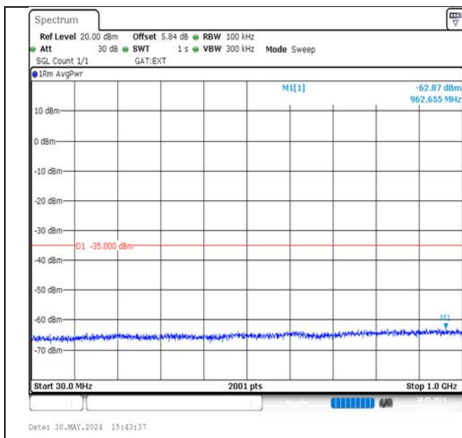
Band38-20MHz-16QAM-38150-1RB#99-30~1000-PASS
