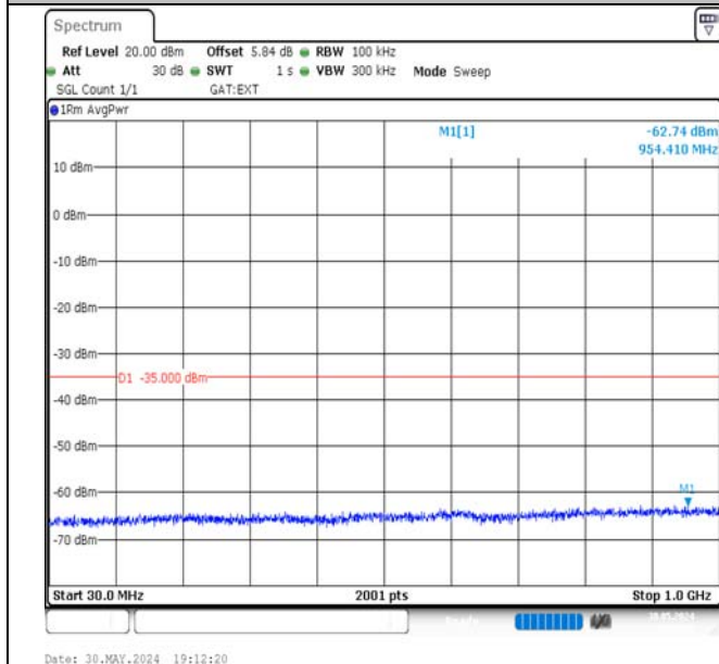
Band41-5MHz-QPSK-41565-1RB#0-30~1000-PASS
