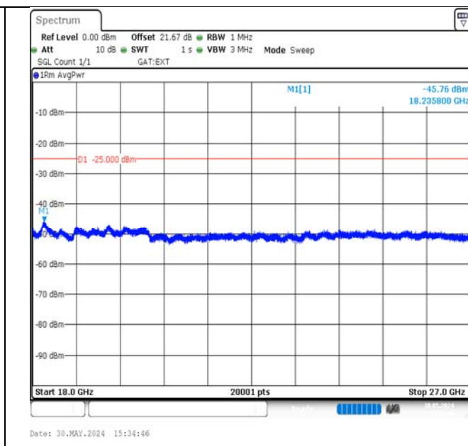
Band38-20MHz-QPSK-38000-100RB#0-18000~27000-PASS
