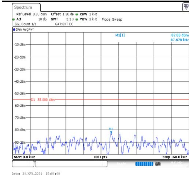
Band41-5MHz-QPSK-40620-1RB#24-0.009~0.15-PASS
