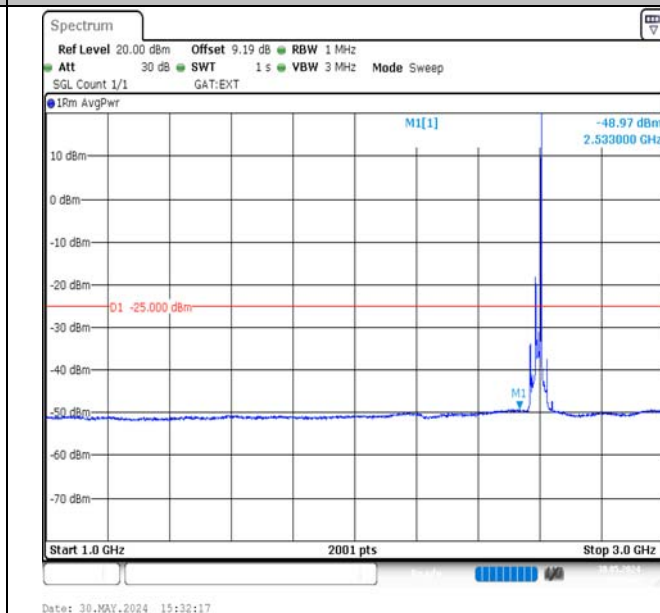
Band38-20MHz-16QAM-38000-1RB#99-1000~3000-PASS
