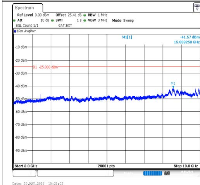
Band38-20MHz-16QAM-37850-1RB#99-3000~18000-PASS
