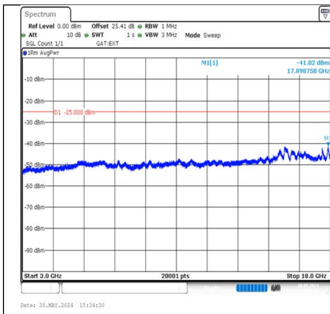
Band38-20MHz-QPSK-38000-100RB#0-3000~18000-PASS
