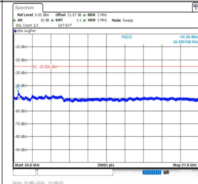
Band38-20MHz-QPSK-38150-100RB#0-18000~27000-PASS
