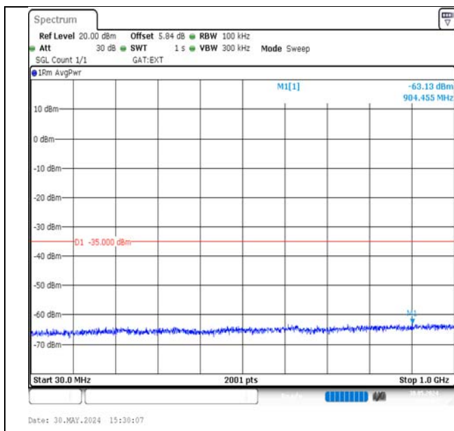
Band38-20MHz-QPSK-38000-1RB#99-30~1000-PASS
