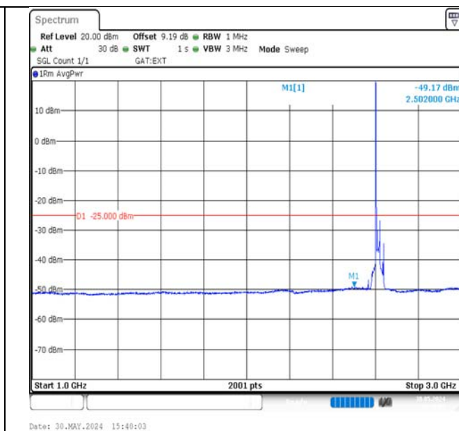
Band38-20MHz-16QAM-38150-1RB#0-1000~3000-PASS
