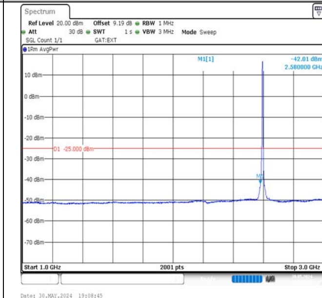
Band41-5MHz-QPSK-40620-25RB#0-1000~3000-PASS
