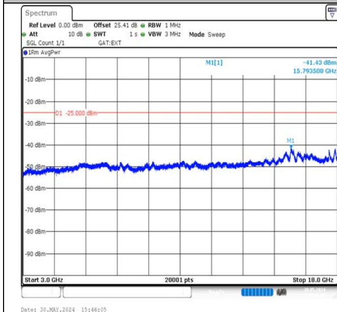
Band38-20MHz-QPSK-38150-100RB#0-3000~18000-PASS
