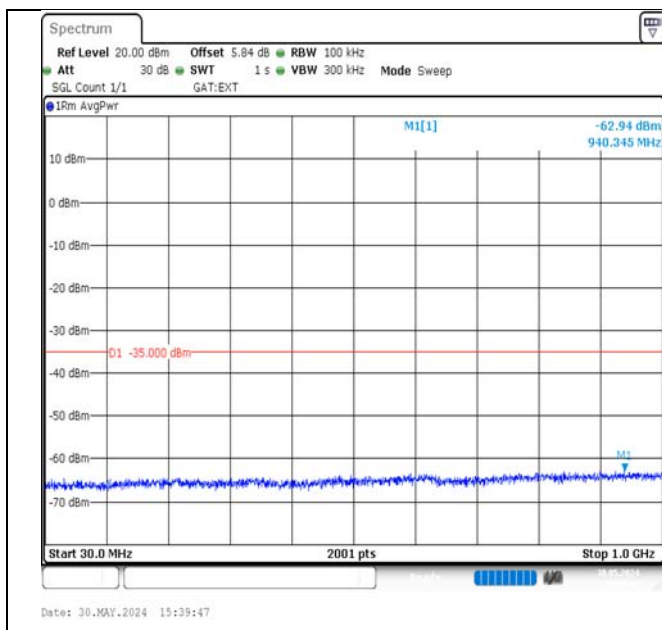
Band38-20MHz-16QAM-38150-1RB#0-30~1000-PASS
