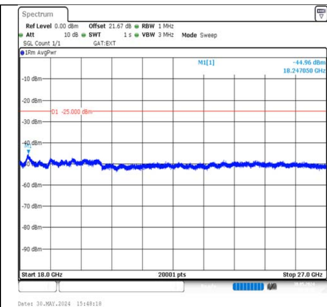
Band38-20MHz-16QAM-38150-100RB#0-18000~27000-PASS
