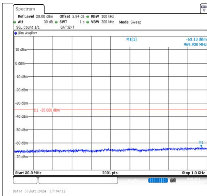
Band38-15MHz-16QAM-37825-1RB#74-30~1000-PASS
