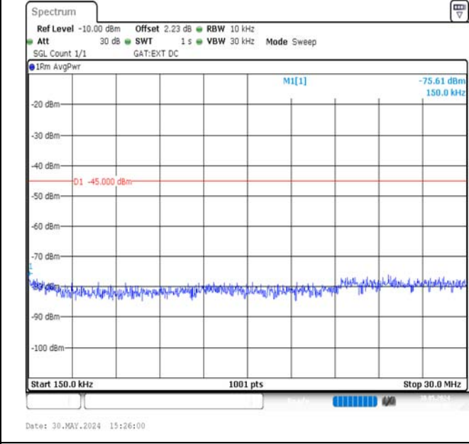
Band38-20MHz-QPSK-38000-1RB#0-0.15~30-PASS
