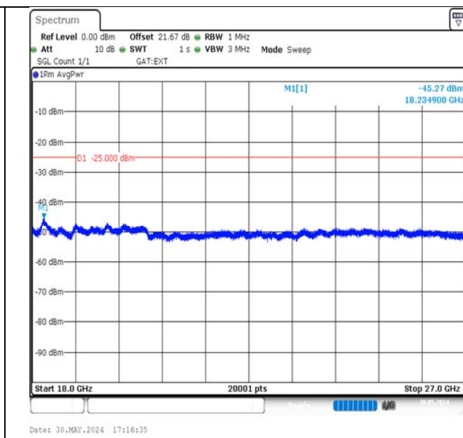
Band38-15MHz-16QAM-38000-1RB#74-18000~27000-PASS
