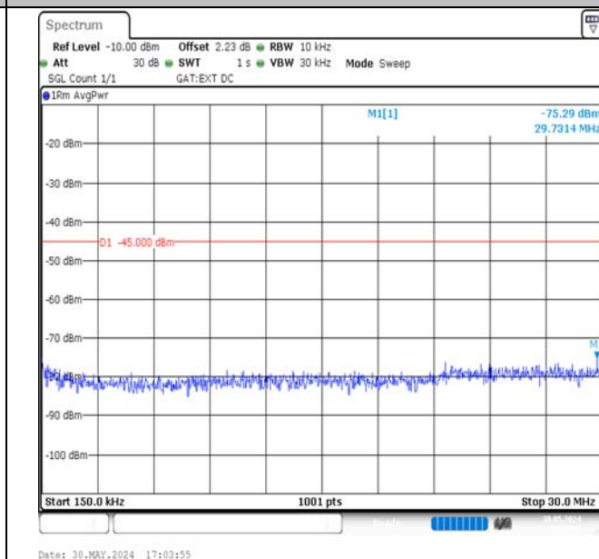
Band38-15MHz-16QAM-37825-1RB#74-0.15~30-PASS
