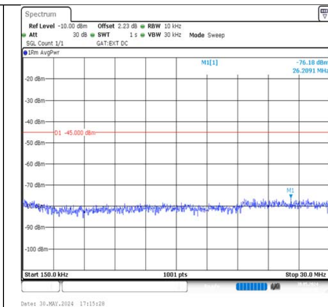
Band38-15MHz-16QAM-38000-1RB#74-0.15~30-PASS
