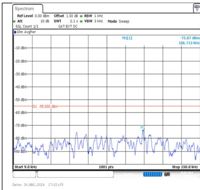
Band38-15MHz-QPSK-38175-1RB#0-0.009~0.15-PASS
