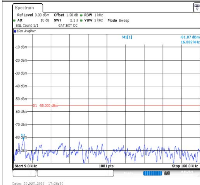
Band38-15MHz-16QAM-38175-1RB#74-0.009~0.15-PASS
