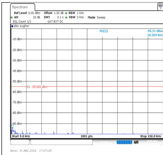
Band38-15MHz-16QAM-37825-75RB#0-0.009~0.15-PASS
