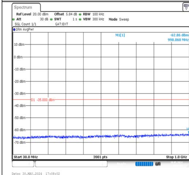
Band38-15MHz-16QAM-37825-75RB#0-30~1000-PASS
