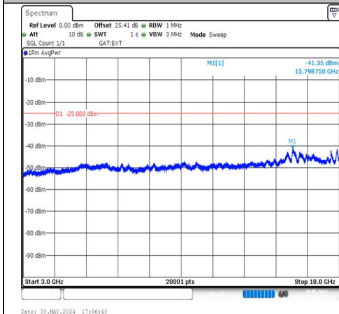
Band38-15MHz-QPSK-37825-75RB#0-3000~18000-PASS
