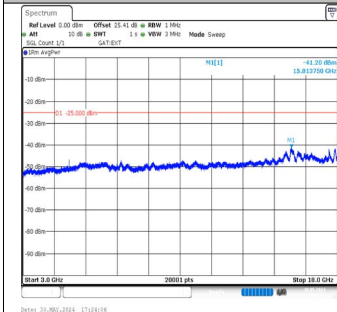
Band38-15MHz-16QAM-38175-1RB#0-3000~18000-PASS
