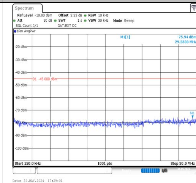
Band38-15MHz-QPSK-38175-75RB#0-0.15~30-PASS
