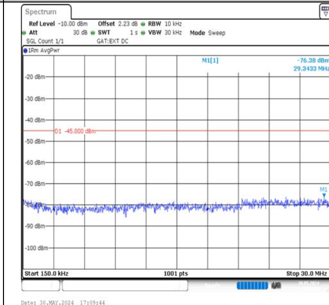
Band38-15MHz-QPSK-38000-1RB#0-0.15~30-PASS
