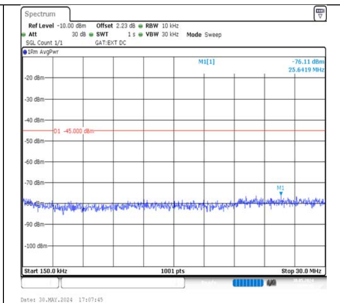
Band38-15MHz-16QAM-37825-75RB#0-0.15~30-PASS
