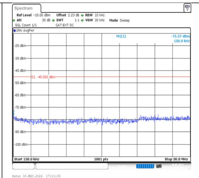
Band38-15MHz-16QAM-38000-1RB#0-0.15~30-PASS
