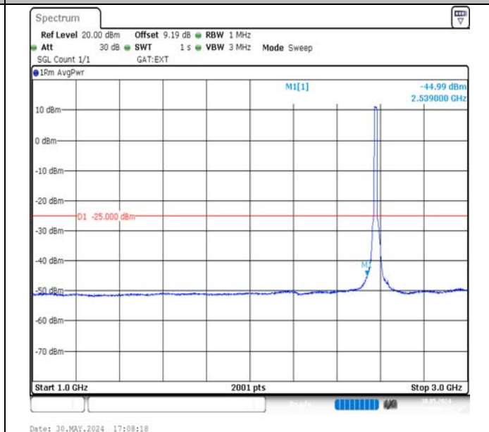
Band38-15MHz-16QAM-37825-75RB#0-1000~3000-PASS
