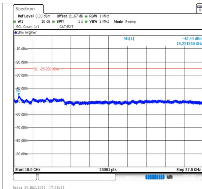
Band38-15MHz-QPSK-38000-75RB#0-18000~27000-PASS
