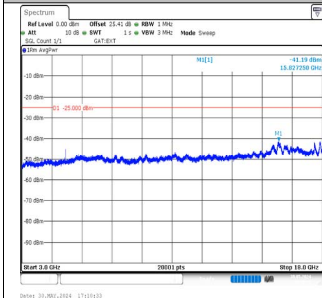
Band38-15MHz-QPSK-38000-1RB#0-3000~18000-PASS
