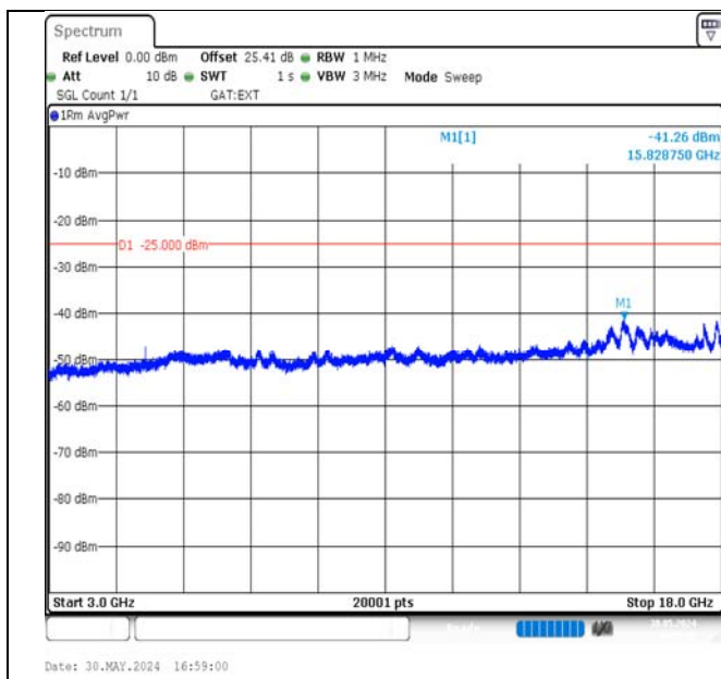
Band38-15MHz-QPSK-37825-1RB#0-3000~18000-PASS
