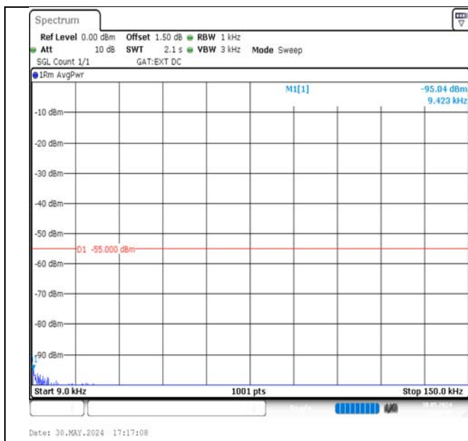
Band38-15MHz-QPSK-38000-75RB#0-0.009~0.15-PASS
