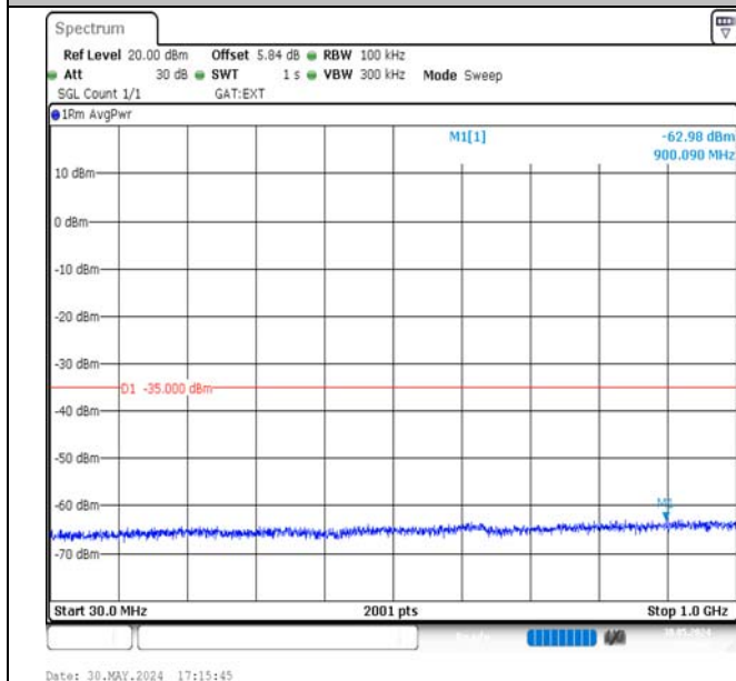
Band38-15MHz-16QAM-38000-1RB#74-30~1000-PASS
