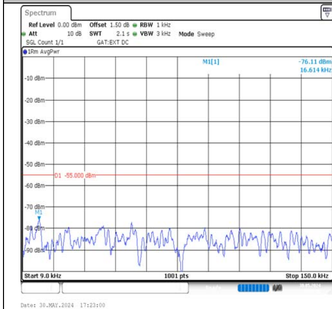
Band38-15MHz-16QAM-38175-1RB#0-0.009~0.15-PASS
