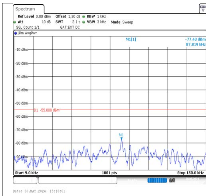
Band38-20MHz-QPSK-37850-1RB#99-0.009~0.15-PASS
