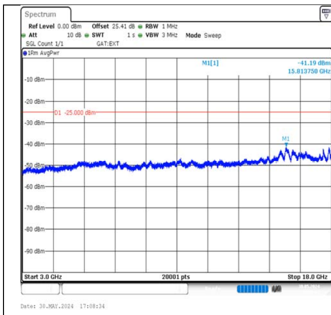
Band38-15MHz-16QAM-37825-75RB#0-3000~18000-PASS
