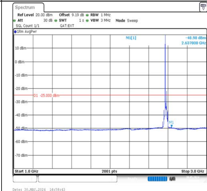
Band38-15MHz-QPSK-37825-1RB#0-1000~3000-PASS
