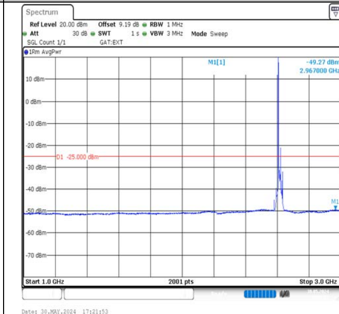
Band38-15MHz-QPSK-38175-1RB#0-1000~3000-PASS
