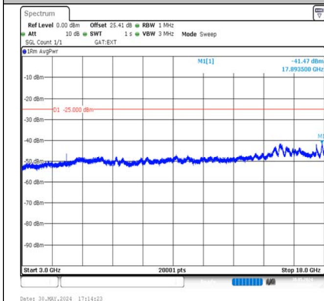
Band38-15MHz-QPSK-38000-1RB#74-3000~18000-PASS
