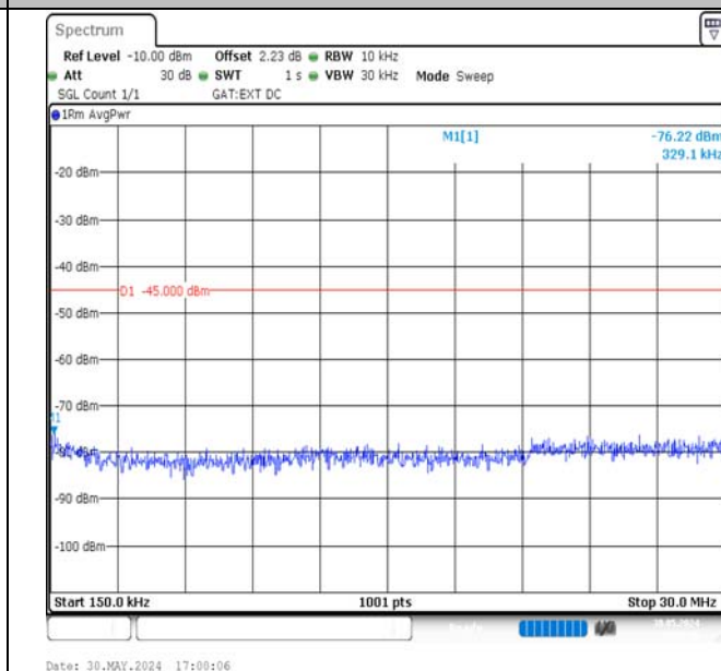
Band38-15MHz-16QAM-37825-1RB#0-0.15~30-PASS
