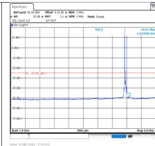
Band38-15MHz-16QAM-37825-1RB#0-1000~3000-PASS
