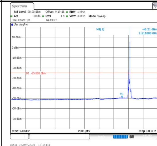
Band38-15MHz-QPSK-38175-1RB#74-1000~3000-PASS
