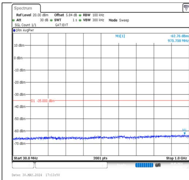
Band38-15MHz-QPSK-38000-1RB#74-30~1000-PASS
