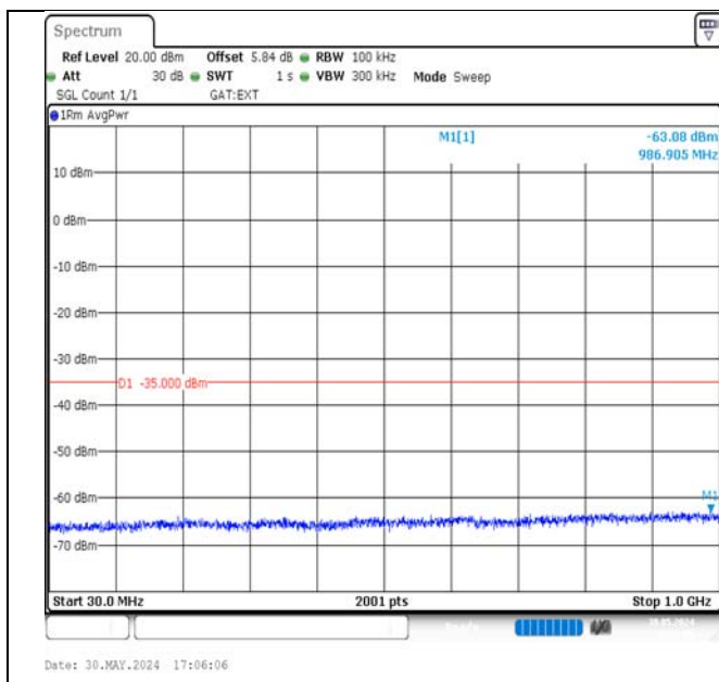
Band38-15MHz-QPSK-37825-75RB#0-30~1000-PASS
