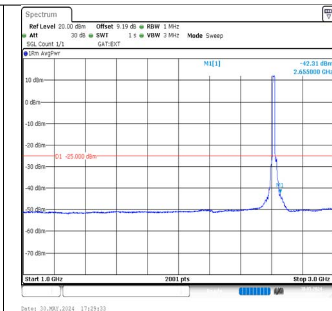
Band38-15MHz-QPSK-38175-75RB#0-1000~3000-PASS
