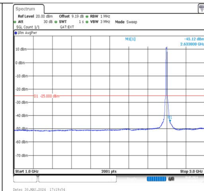
Band38-15MHz-16QAM-38000-75RB#0-1000~3000-PASS
