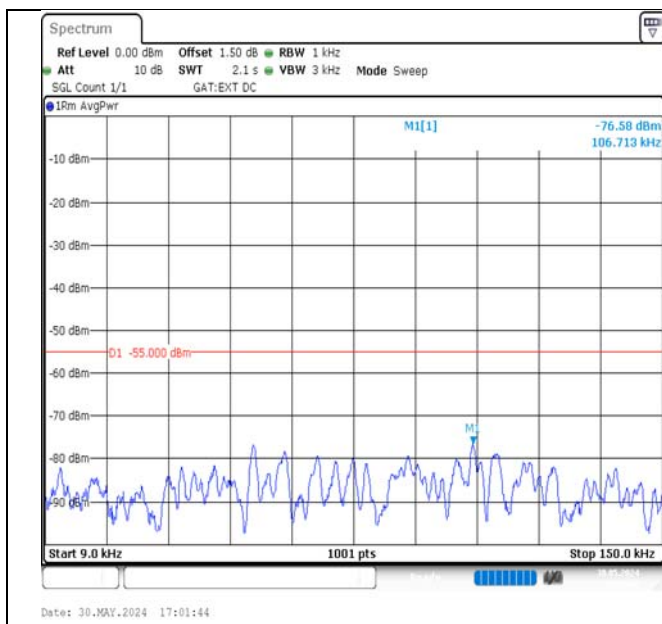
Band38-15MHz-QPSK-37825-1RB#74-0.009~0.15-PASS
