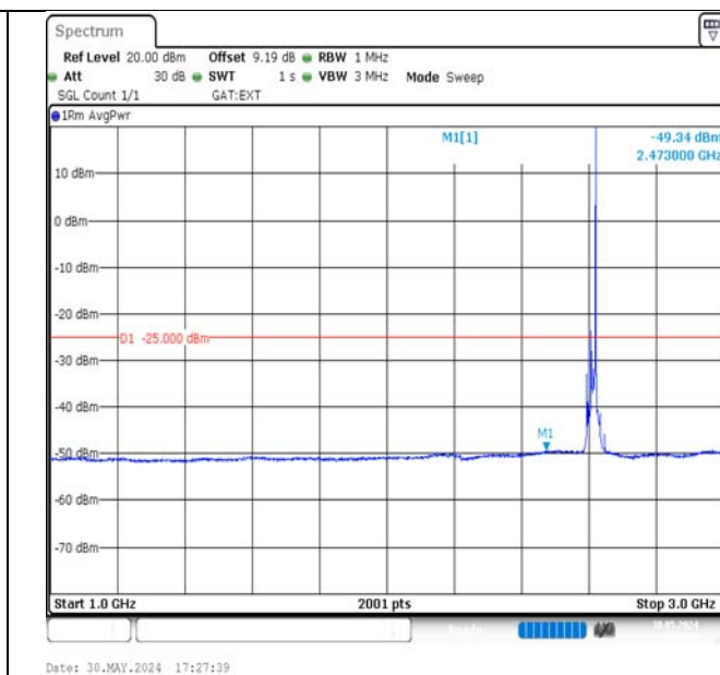
Band38-15MHz-16QAM-38175-1RB#74-1000~3000-PASS
