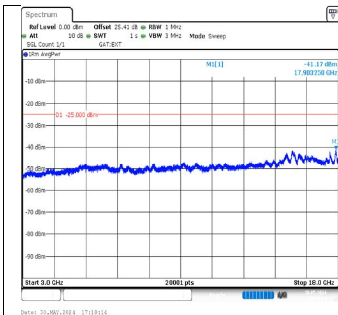
Band38-15MHz-QPSK-38000-75RB#0-3000~18000-PASS
