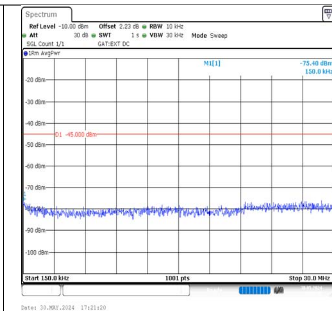
Band38-15MHz-QPSK-38175-1RB#0-0.15~30-PASS
