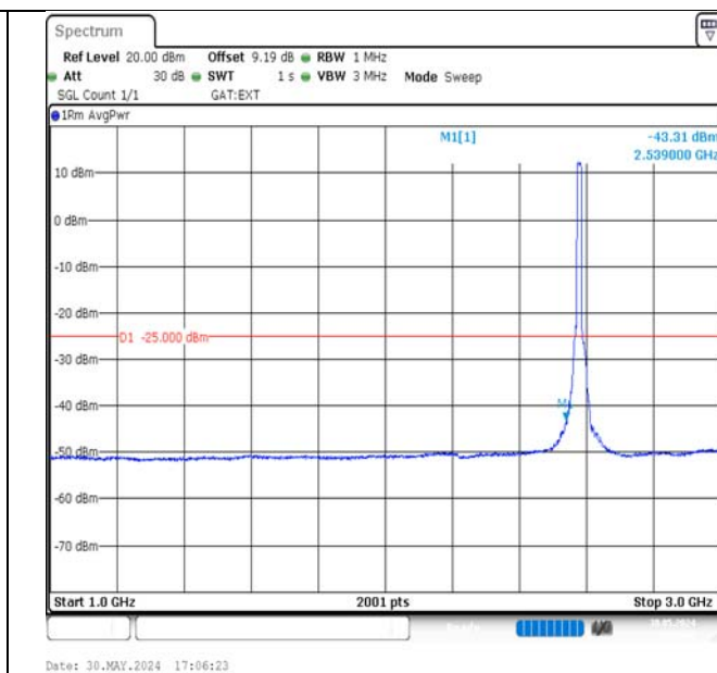
Band38-15MHz-QPSK-37825-75RB#0-1000~3000-PASS
