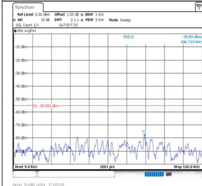
Band38-15MHz-QPSK-38000-1RB#0-0.009~0.15-PASS
