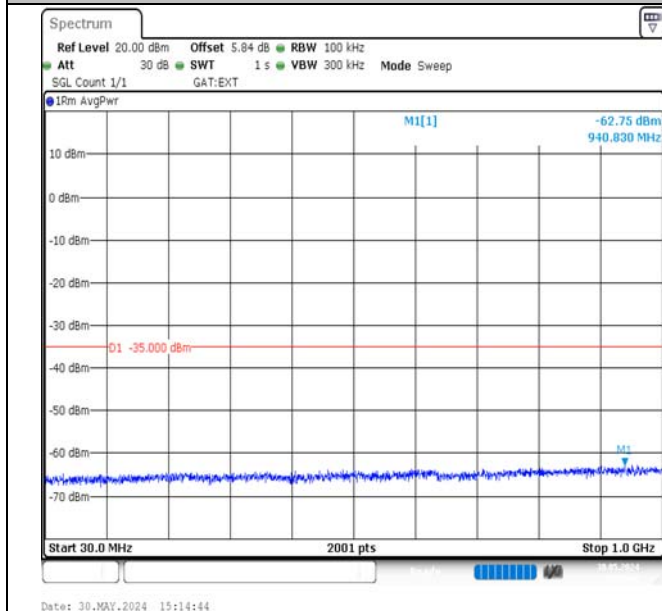
Band38-20MHz-QPSK-37850-1RB#0-30~1000-PASS
