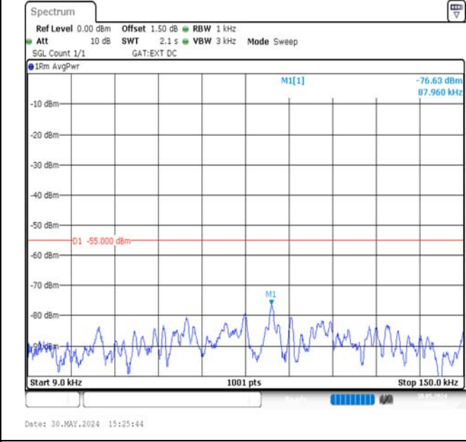
Band38-20MHz-QPSK-38000-1RB#0-0.009~0.15-PASS
