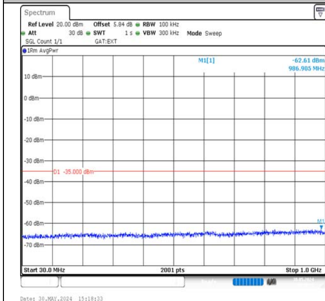
Band38-20MHz-QPSK-37850-1RB#99-30~1000-PASS
