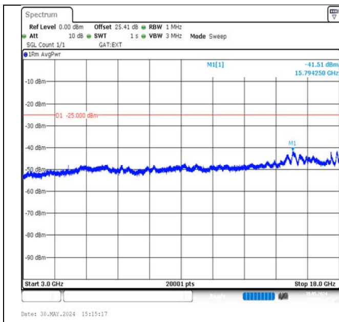
Band38-20MHz-QPSK-37850-1RB#0-3000~18000-PASS
