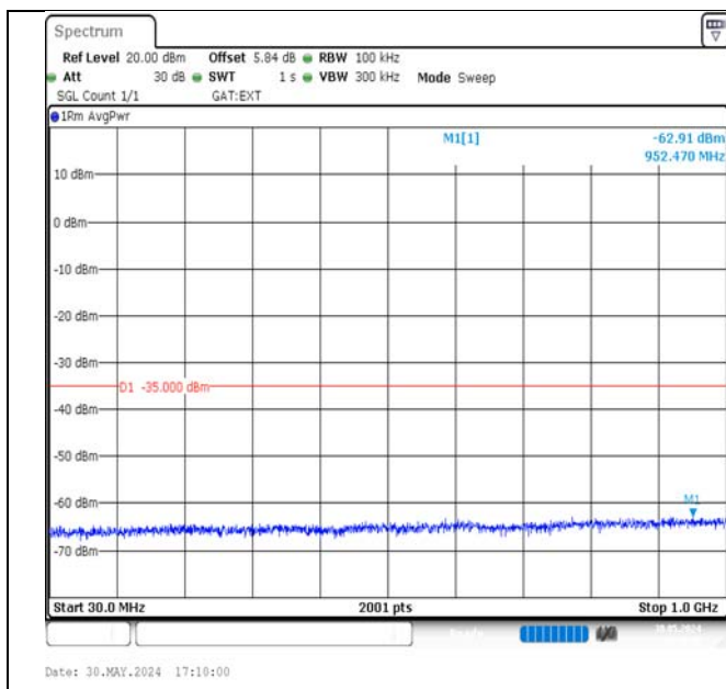
Band38-15MHz-QPSK-38000-1RB#0-30~1000-PASS
