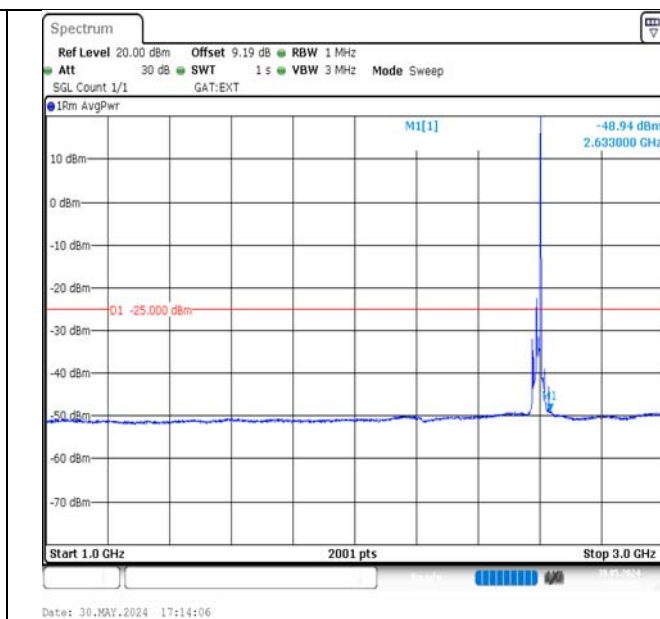
Band38-15MHz-QPSK-38000-1RB#74-1000~3000-PASS
