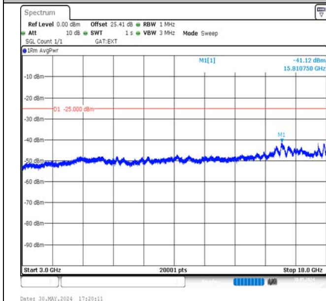
Band38-15MHz-16QAM-38000-75RB#0-3000~18000-PASS
