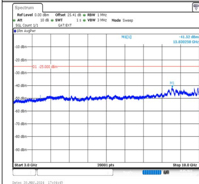
Band38-15MHz-16QAM-37825-1RB#74-3000~18000-PASS
