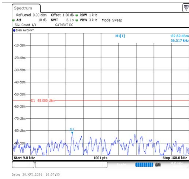
Band38-15MHz-QPSK-37825-1RB#0-0.009~0.15-PASS
