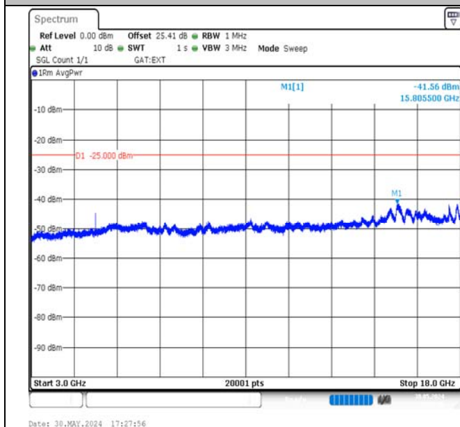
Band38-15MHz-16QAM-38175-1RB#74-3000~18000-PASS
