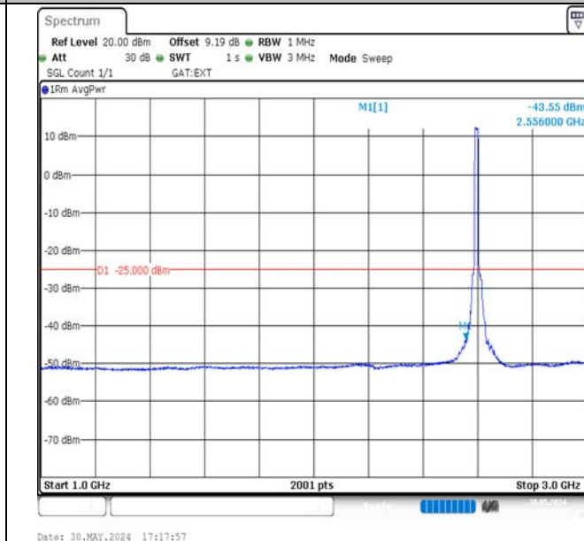
Band38-15MHz-QPSK-38000-75RB#0-1000~3000-PASS
