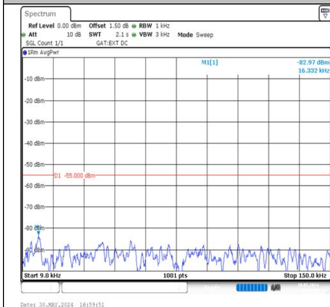
Band38-15MHz-16QAM-37825-1RB#0-0.009~0.15-PASS
