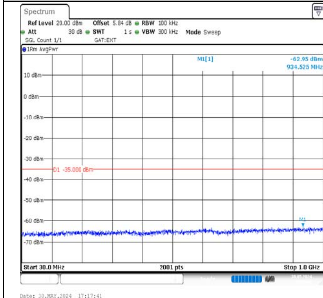
Band38-15MHz-QPSK-38000-75RB#0-30~1000-PASS
