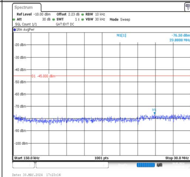
Band38-15MHz-16QAM-38175-1RB#0-0.15~30-PASS
