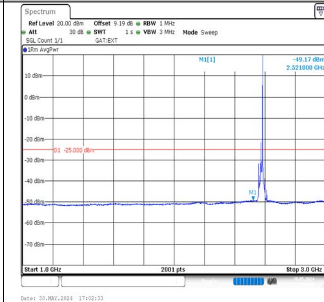
Band38-15MHz-QPSK-37825-1RB#74-1000~3000-PASS
