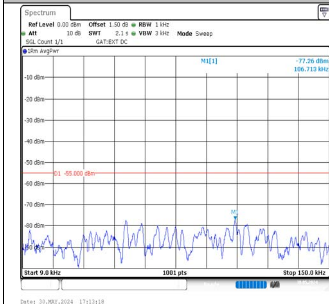
Band38-15MHz-QPSK-38000-1RB#74-0.009~0.15-PASS
