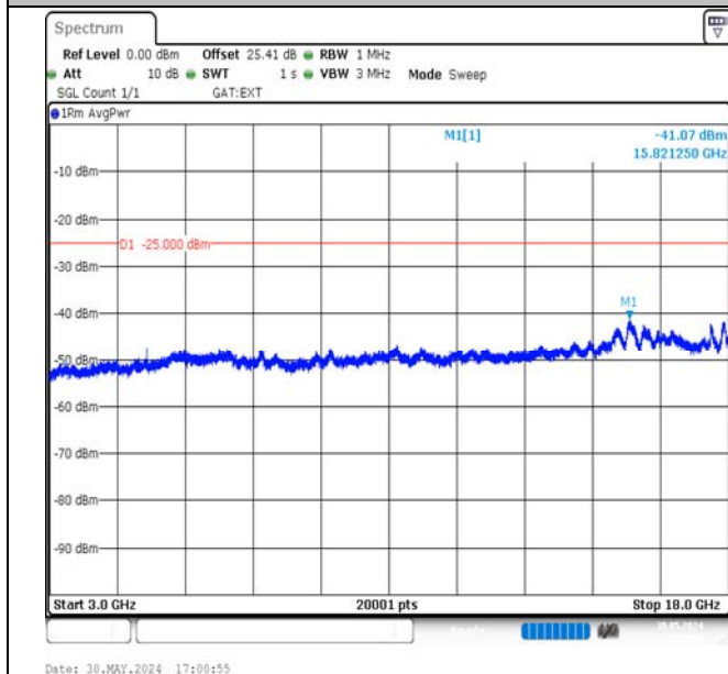
Band38-15MHz-16QAM-37825-1RB#0-3000~18000-PASS
