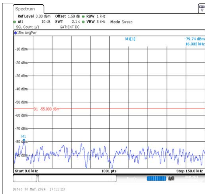
Band38-15MHz-16QAM-38000-1RB#0-0.009~0.15-PASS
