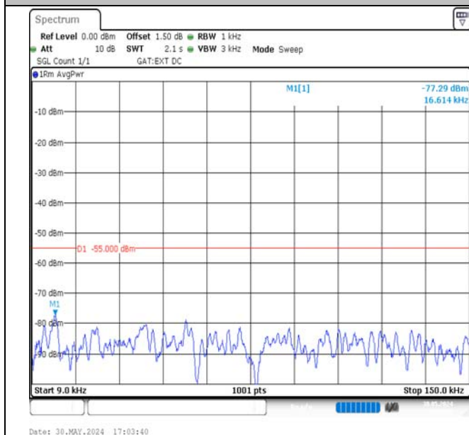
Band38-15MHz-16QAM-37825-1RB#74-0.009~0.15-PASS
