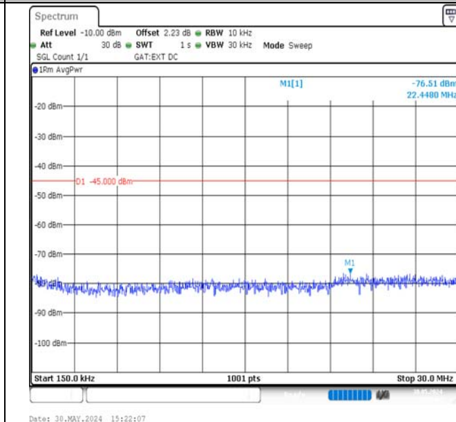
Band38-20MHz-QPSK-37850-100RB#0-0.15~30-PASS
