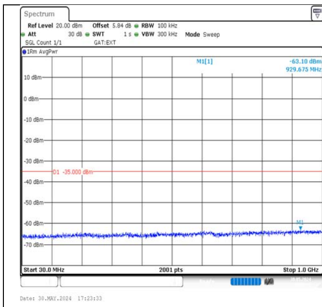
Band38-15MHz-16QAM-38175-1RB#0-30~1000-PASS
