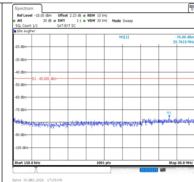
Band38-15MHz-16QAM-38175-75RB#0-0.15~30-PASS
