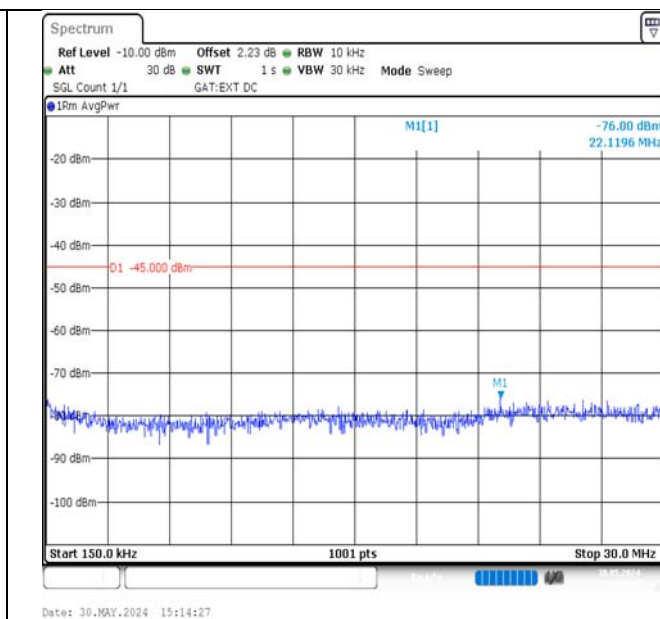
Band38-20MHz-QPSK-37850-1RB#0-0.15~30-PASS
