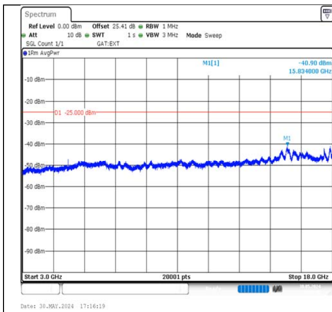
Band38-15MHz-16QAM-38000-1RB#74-3000~18000-PASS
