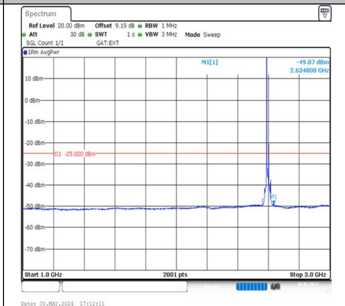
Band38-15MHz-16QAM-38000-1RB#0-1000~3000-PASS
