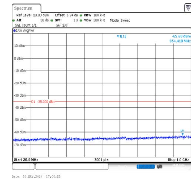
Band38-15MHz-16QAM-37825-1RB#0-30~1000-PASS
