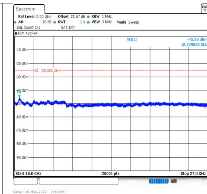
Band38-15MHz-16QAM-37825-75RB#0-18000~27000-PASS
