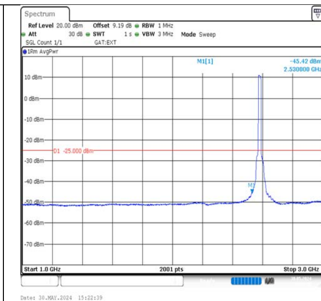
Band38-20MHz-QPSK-37850-100RB#0-1000~3000-PASS
