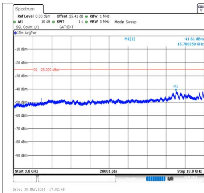
Band38-15MHz-QPSK-37825-1RB#74-3000~18000-PASS
