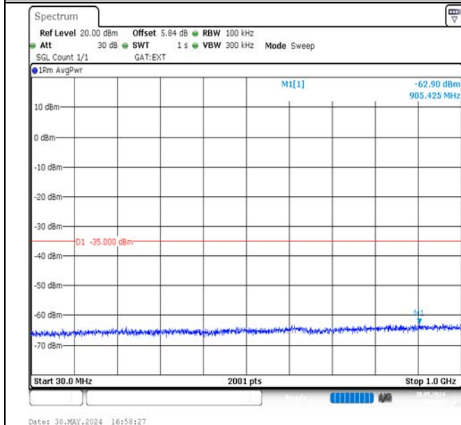
Band38-15MHz-QPSK-37825-1RB#0-30~1000-PASS
