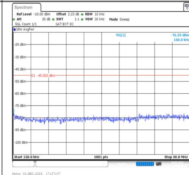
Band38-15MHz-16QAM-38175-1RB#74-0.15~30-PASS
