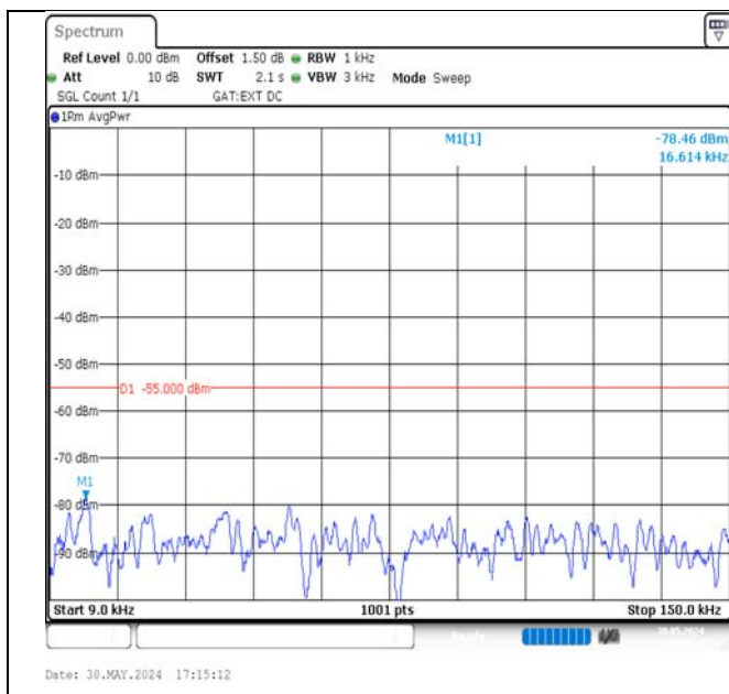
Band38-15MHz-16QAM-38000-1RB#74-0.009~0.15-PASS
