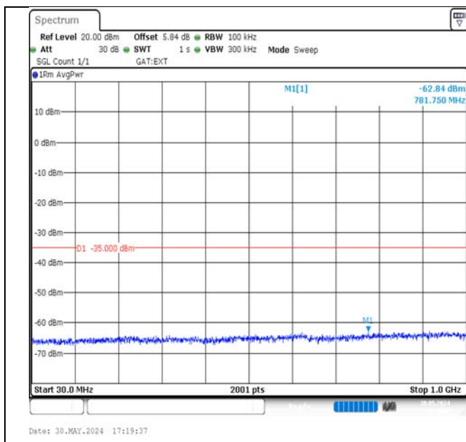
Band38-15MHz-16QAM-38000-75RB#0-30~1000-PASS
