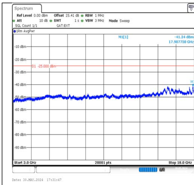
Band38-15MHz-16QAM-38175-75RB#0-3000~18000-PASS
