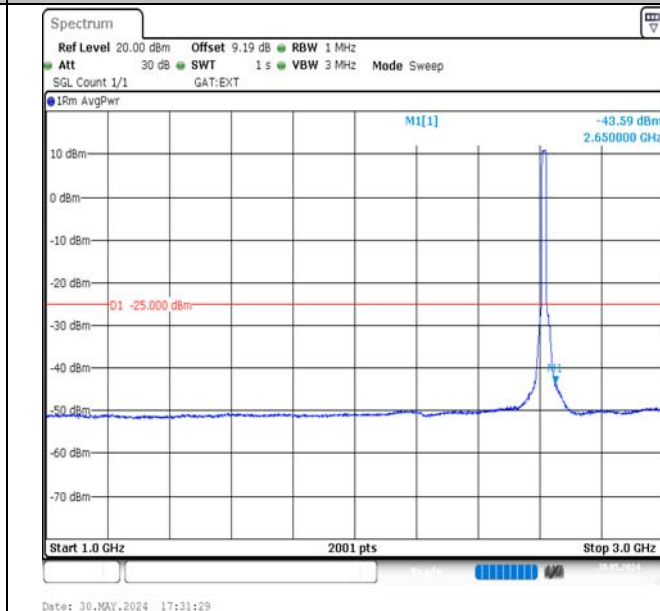
Band38-15MHz-16QAM-38175-75RB#0-1000~3000-PASS
