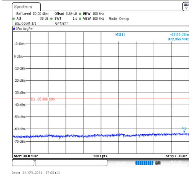
Band38-15MHz-16QAM-38175-75RB#0-30~1000-PASS
