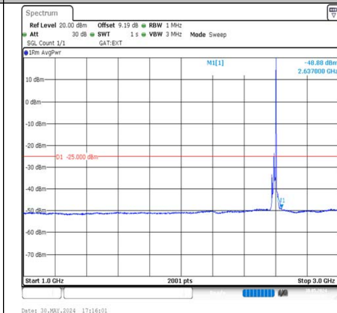
Band38-15MHz-16QAM-38000-1RB#74-1000~3000-PASS
