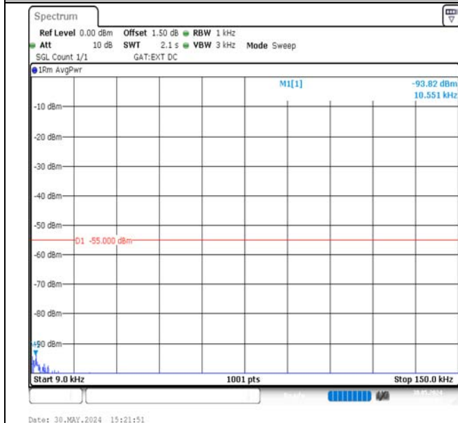
Band38-20MHz-QPSK-37850-100RB#0-0.009~0.15-PASS
