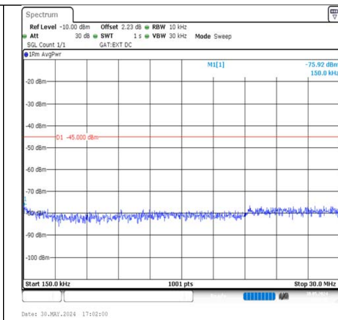
Band38-15MHz-QPSK-37825-1RB#74-0.15~30-PASS
