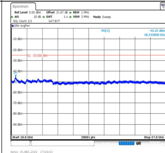
Band38-15MHz-16QAM-38175-1RB#0-18000~27000-PASS
