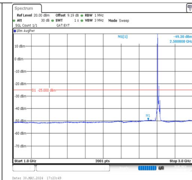
Band38-15MHz-16QAM-38175-1RB#0-1000~3000-PASS
