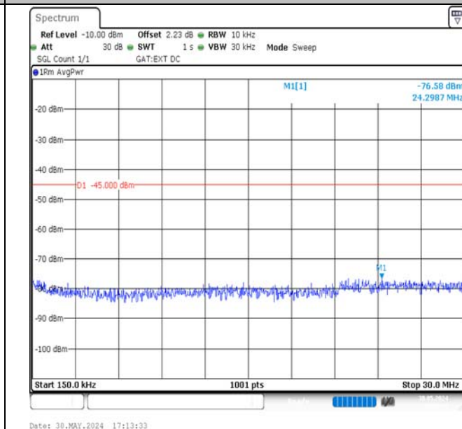
Band38-15MHz-QPSK-38000-1RB#74-0.15~30-PASS
