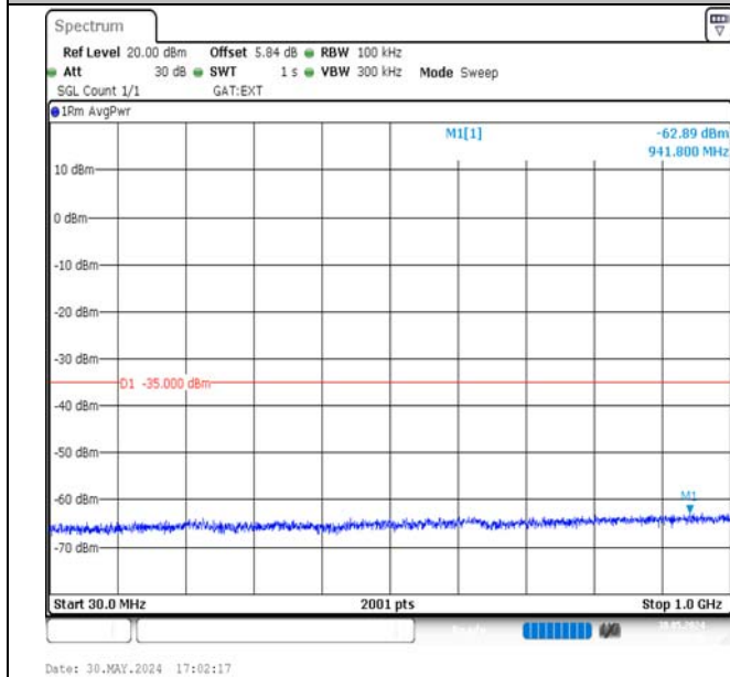
Band38-15MHz-QPSK-37825-1RB#74-30~1000-PASS
