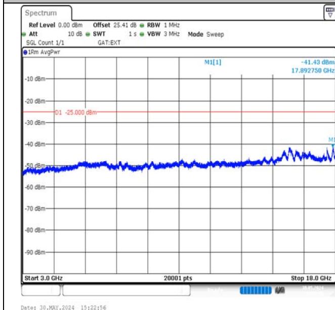
Band38-20MHz-QPSK-37850-100RB#0-3000~18000-PASS
