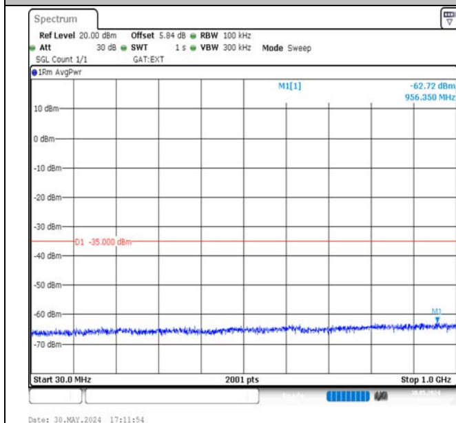
Band38-15MHz-16QAM-38000-1RB#0-30~1000-PASS
