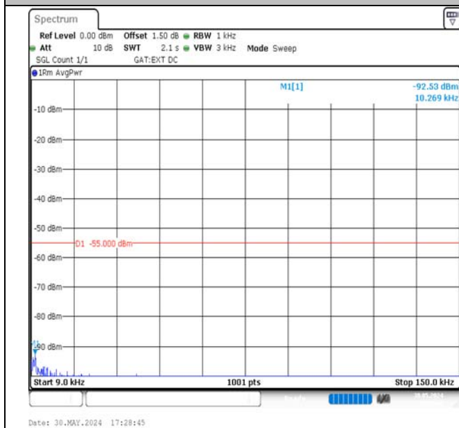
Band38-15MHz-QPSK-38175-75RB#0-0.009~0.15-PASS
