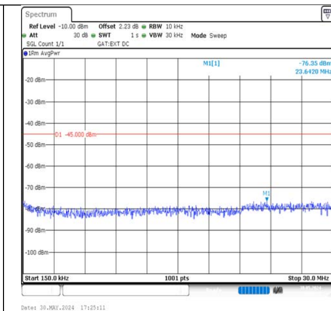
Band38-15MHz-QPSK-38175-1RB#74-0.15~30-PASS
