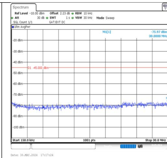
Band38-15MHz-QPSK-38000-75RB#0-0.15~30-PASS
