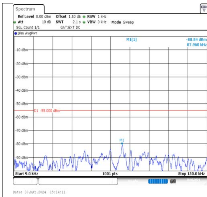
Band38-20MHz-QPSK-37850-1RB#0-0.009~0.15-PASS
