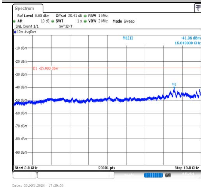
Band38-15MHz-QPSK-38175-75RB#0-3000~18000-PASS
