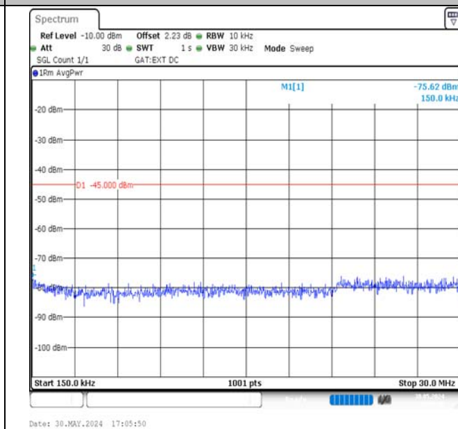
Band38-15MHz-QPSK-37825-75RB#0-0.15~30-PASS
