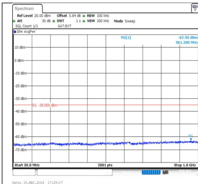
Band38-15MHz-QPSK-38175-75RB#0-30~1000-PASS
