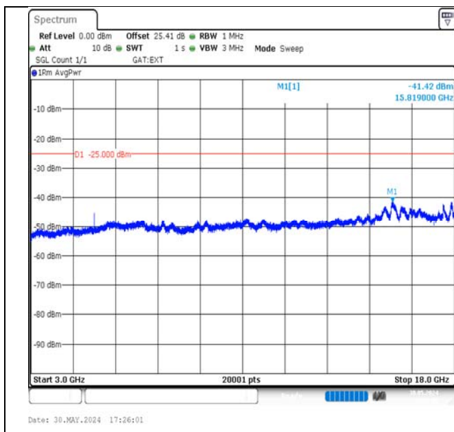
Band38-15MHz-QPSK-38175-1RB#74-3000~18000-PASS
