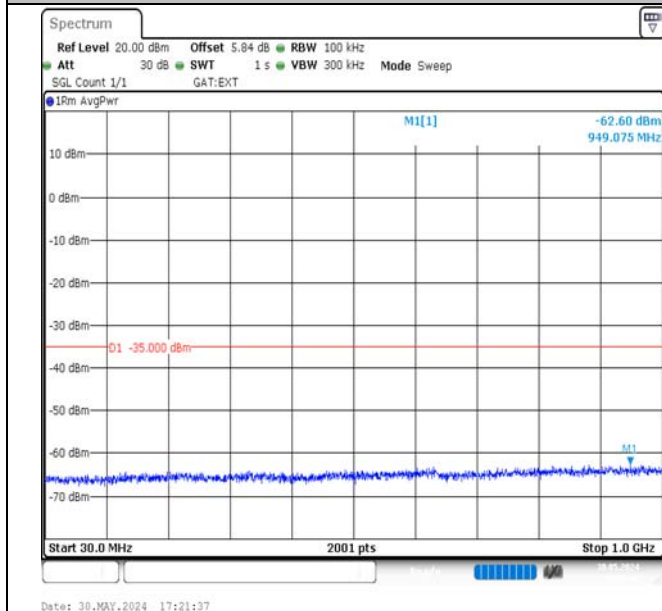
Band38-15MHz-QPSK-38175-1RB#0-30~1000-PASS
