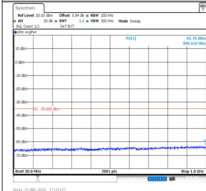
Band38-15MHz-QPSK-38175-1RB#74-30~1000-PASS
