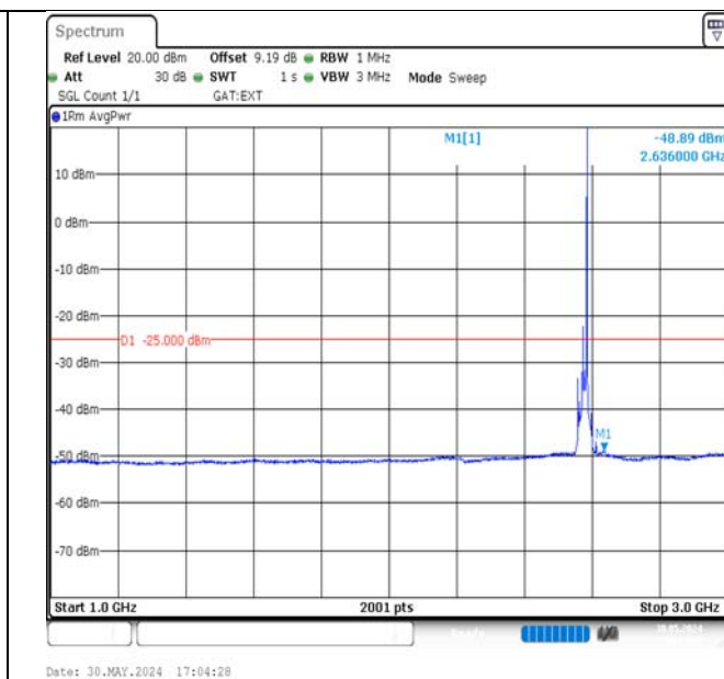
Band38-15MHz-16QAM-37825-1RB#74-1000~3000-PASS
