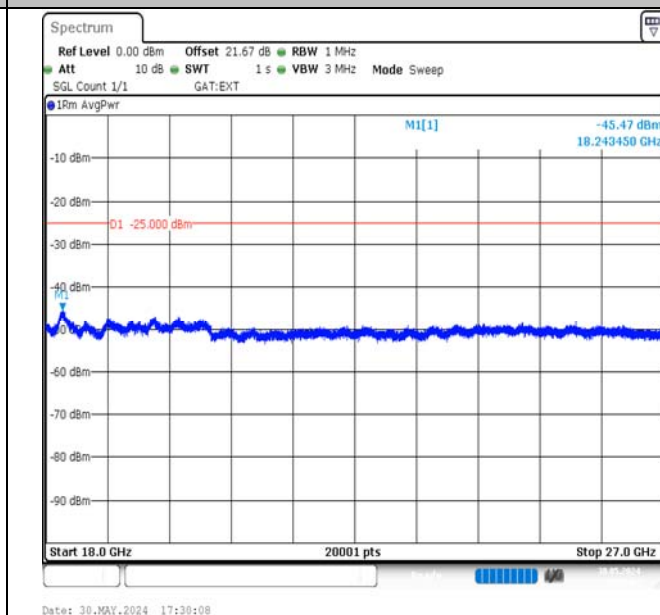
Band38-15MHz-QPSK-38175-75RB#0-18000~27000-PASS
