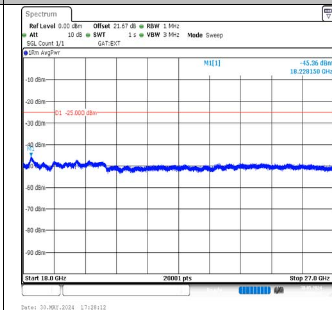
Band38-15MHz-16QAM-38175-1RB#74-18000~27000-PASS
