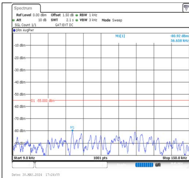
Band38-15MHz-QPSK-38175-1RB#74-0.009~0.15-PASS
