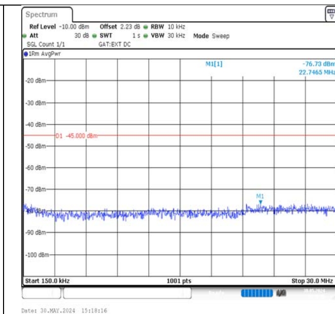
Band38-20MHz-QPSK-37850-1RB#99-0.15~30-PASS
