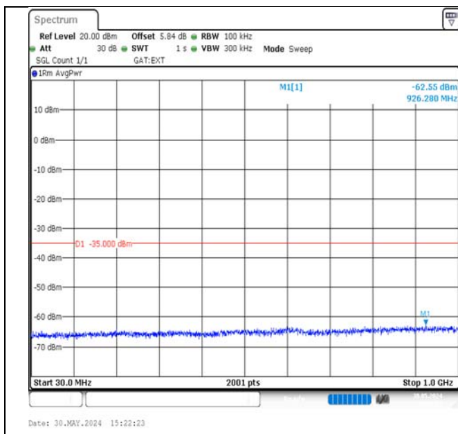
Band38-20MHz-QPSK-37850-100RB#0-30~1000-PASS
