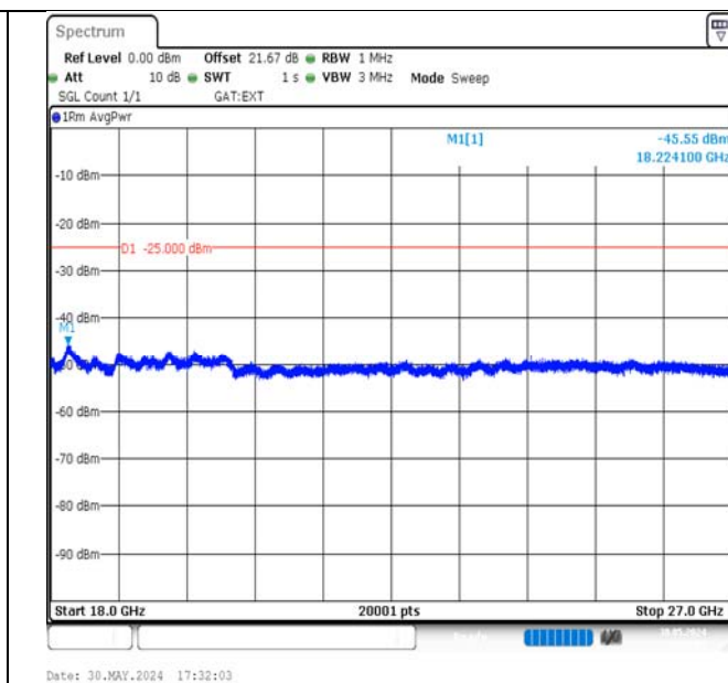
Band38-15MHz-16QAM-38175-75RB#0-18000~27000-PASS
