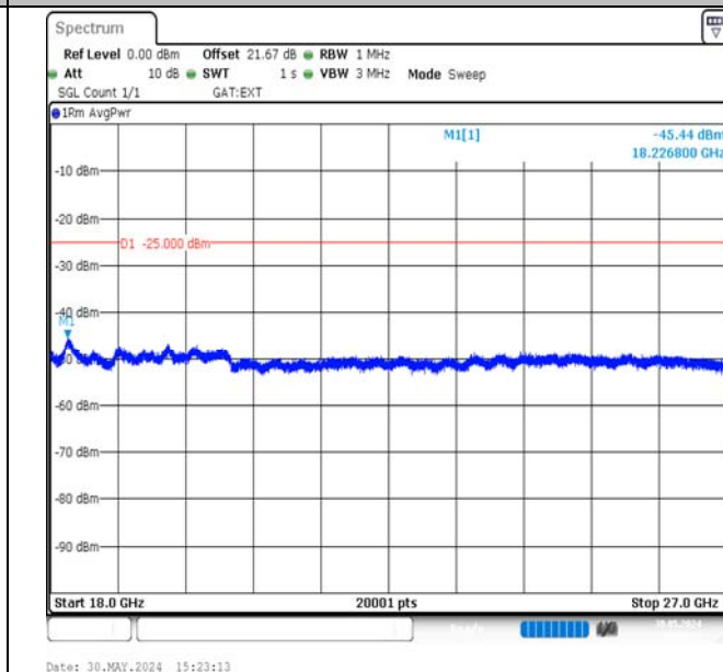
Band38-20MHz-QPSK-37850-100RB#0-18000~27000-PASS
