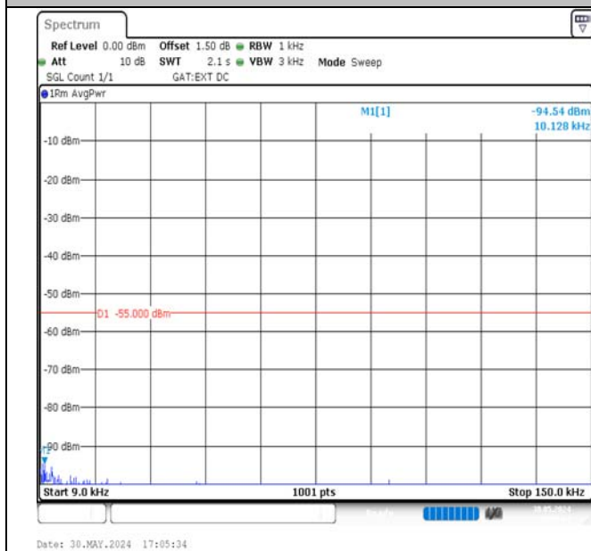
Band38-15MHz-QPSK-37825-75RB#0-0.009~0.15-PASS
