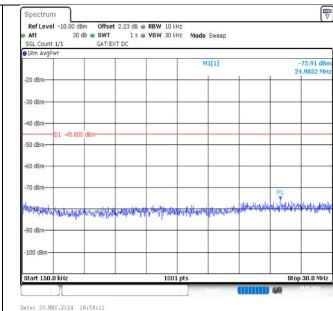
Band38-15MHz-QPSK-37825-1RB#0-0.15~30-PASS
