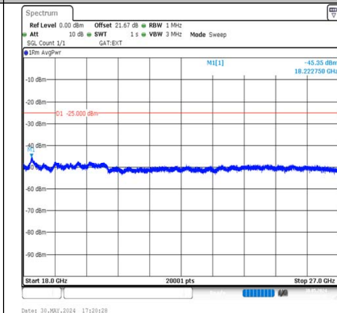
Band38-15MHz-16QAM-38000-75RB#0-18000~27000-PASS
