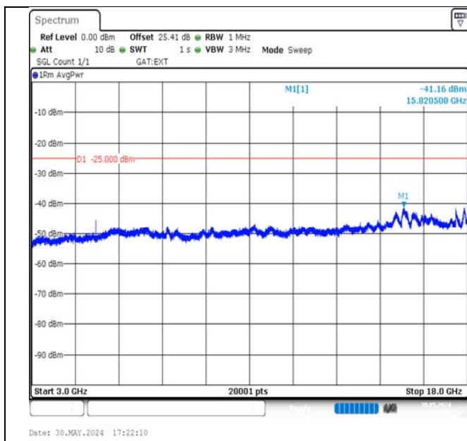
Band38-15MHz-QPSK-38175-1RB#0-3000~18000-PASS
