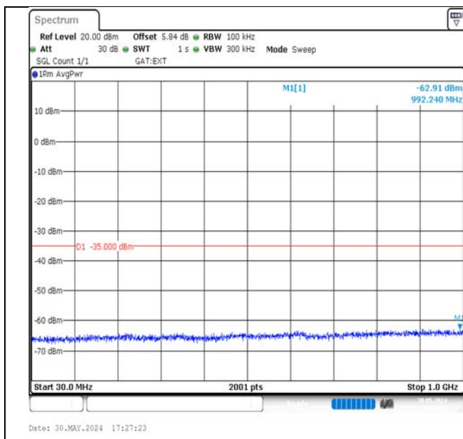
Band38-15MHz-16QAM-38175-1RB#74-30~1000-PASS
