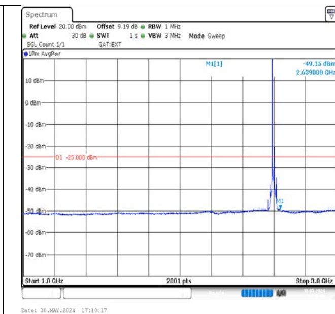
Band38-15MHz-QPSK-38000-1RB#0-1000~3000-PASS
