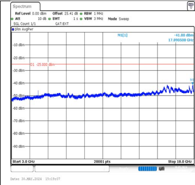
Band38-20MHz-QPSK-37850-1RB#99-3000~18000-PASS
