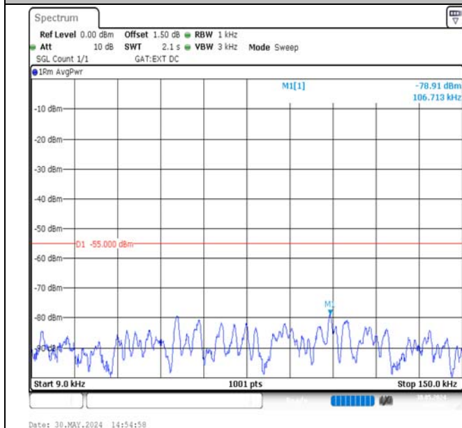
Band38-10MHz-QPSK-38000-1RB#49-0.009~0.15-PASS
