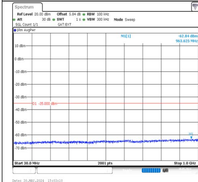
Band38-10MHz-QPSK-38200-1RB#0-30~1000-PASS
