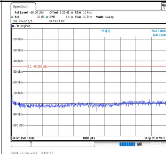
Band38-10MHz-16QAM-38200-1RB#0-0.15~30-PASS
