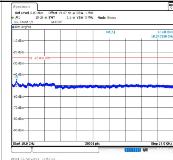
Band38-10MHz-QPSK-38000-1RB#0-18000~27000-PASS
