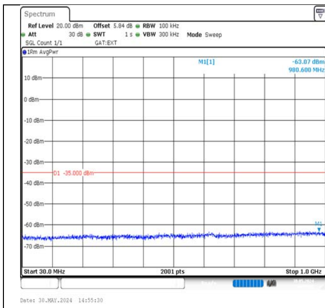
Band38-10MHz-QPSK-38000-1RB#49-30~1000-PASS
