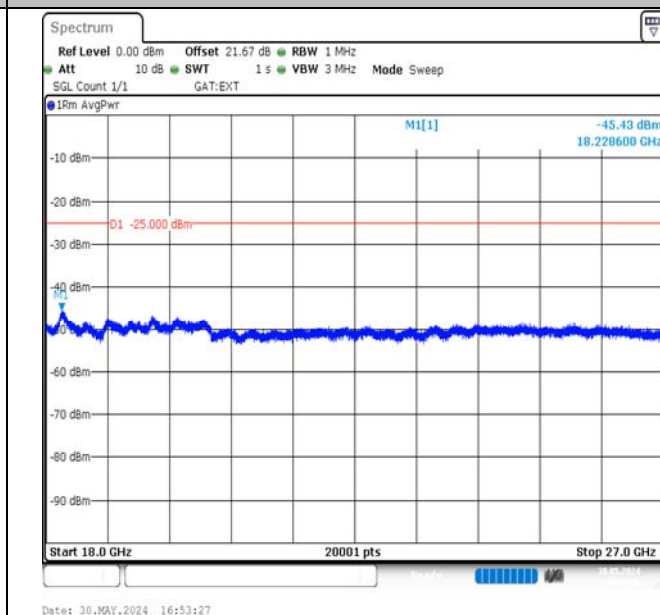
Band38-5MHz-16QAM-38225-1RB#24-18000~27000-PASS
