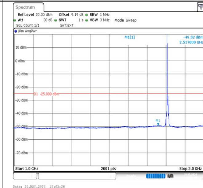
Band38-10MHz-QPSK-38200-1RB#0-1000~3000-PASS
