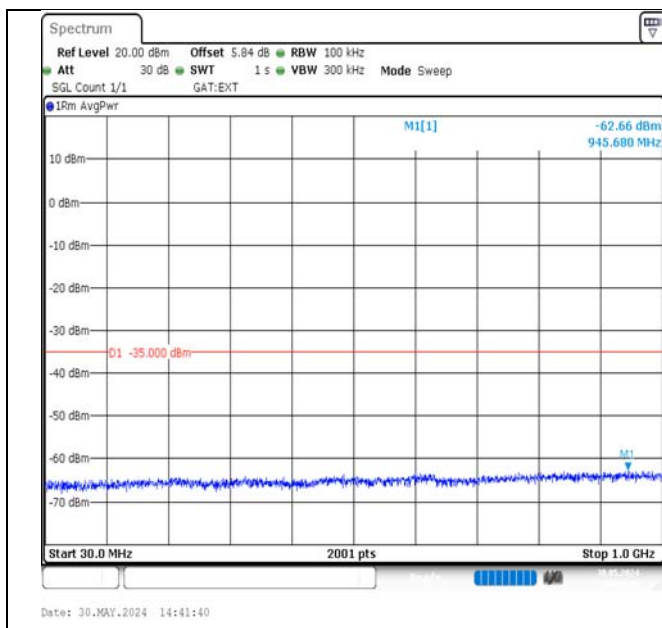
Band38-10MHz-16QAM-37800-1RB#0-30~1000-PASS
