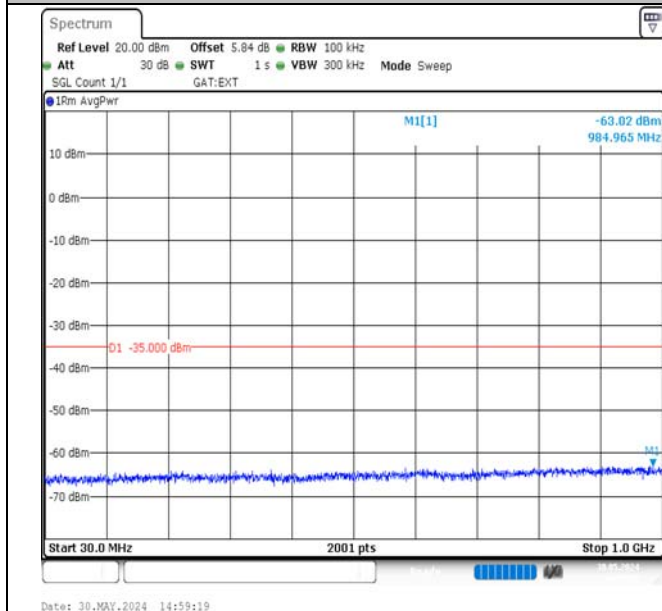
Band38-10MHz-QPSK-38000-50RB#0-30~1000-PASS
