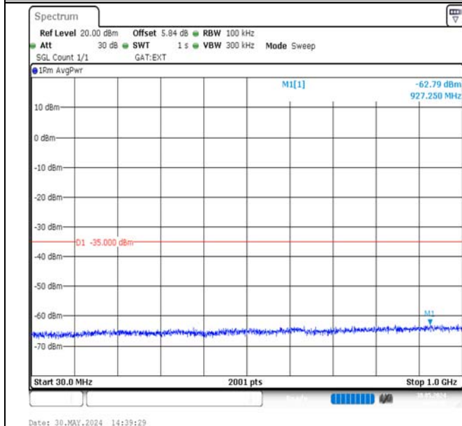
Band38-10MHz-QPSK-37800-1RB#0-30~1000-PASS
