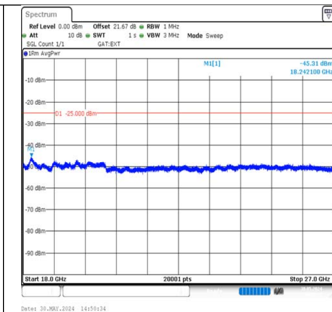
Band38-10MHz-16QAM-37800-50RB#0-18000~27000-PASS
