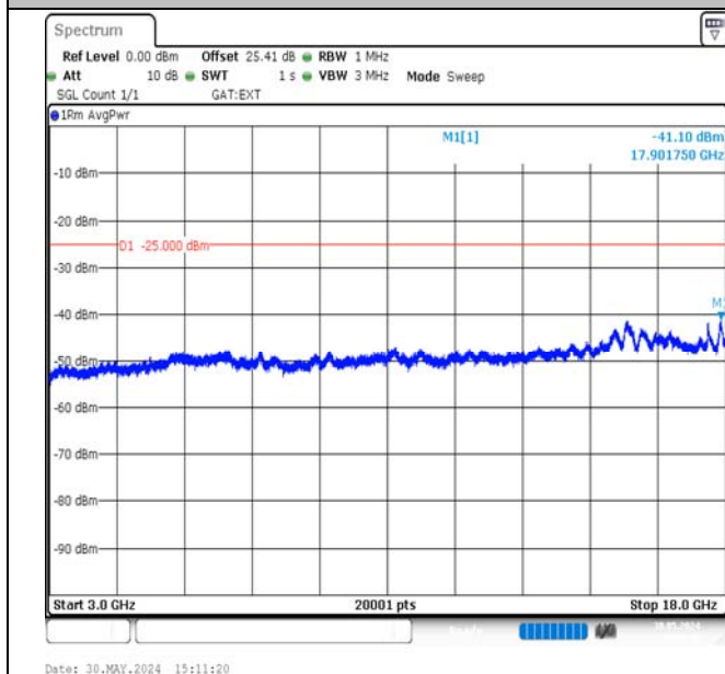
Band38-10MHz-QPSK-38200-50RB#0-3000~18000-PASS
