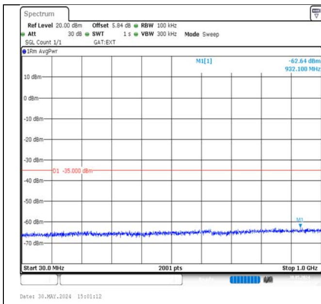
Band38-10MHz-16QAM-38000-50RB#0-30~1000-PASS
