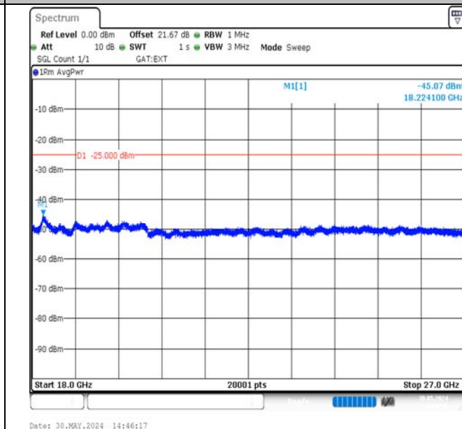
Band38-10MHz-16QAM-37800-1RB#49-18000~27000-PASS
