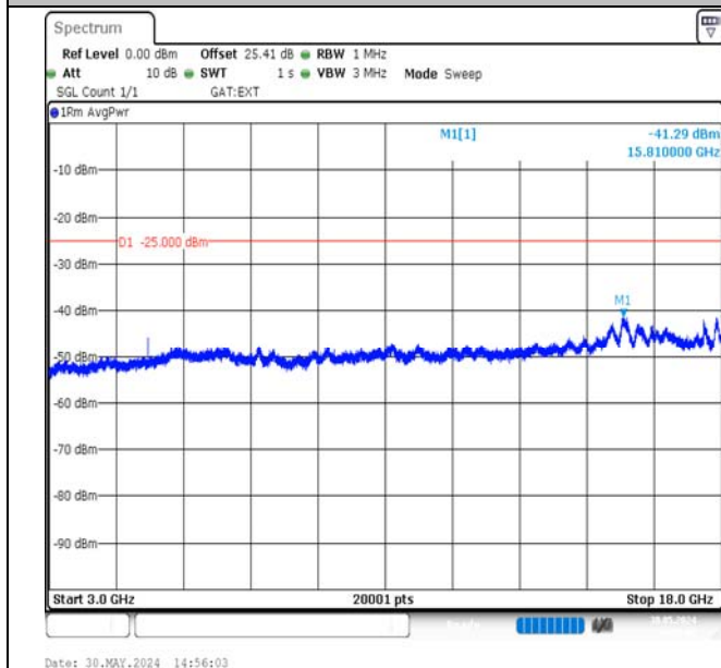
Band38-10MHz-QPSK-38000-1RB#49-3000~18000-PASS
