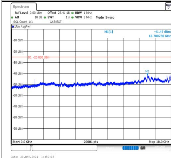
Band38-10MHz-QPSK-38000-1RB#0-3000~18000-PASS
