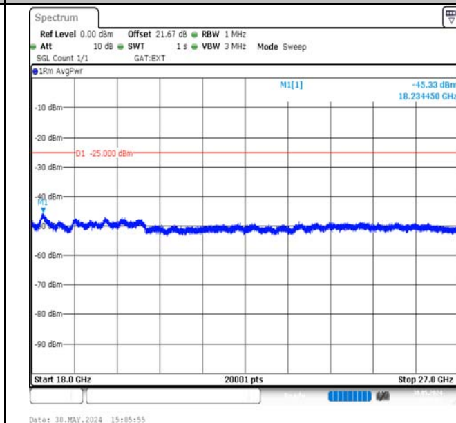
Band38-10MHz-16QAM-38200-1RB#0-18000~27000-PASS
