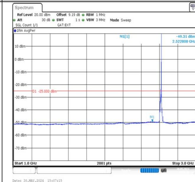
Band38-10MHz-QPSK-38200-1RB#49-1000~3000-PASS
