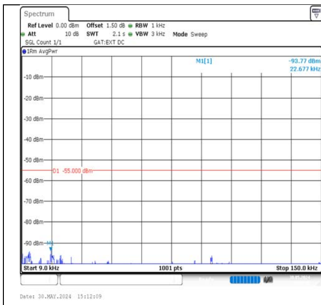
Band38-10MHz-16QAM-38200-50RB#0-0.009~0.15-PASS
