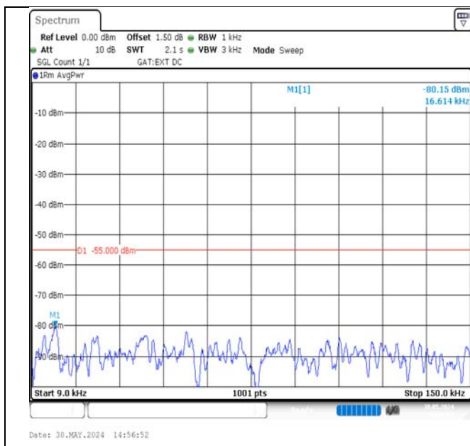
Band38-10MHz-16QAM-38000-1RB#49-0.009~0.15-PASS
