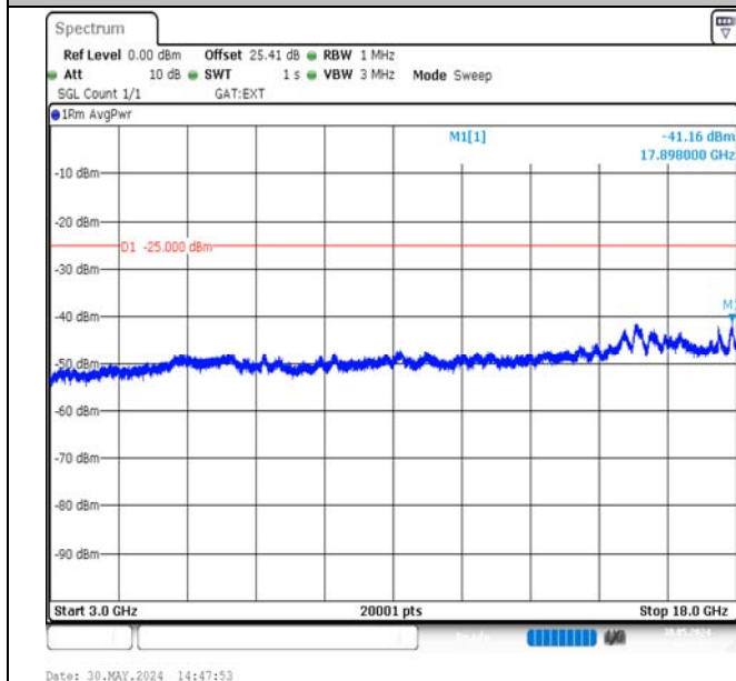
Band38-10MHz-QPSK-37800-50RB#0-3000~18000-PASS
