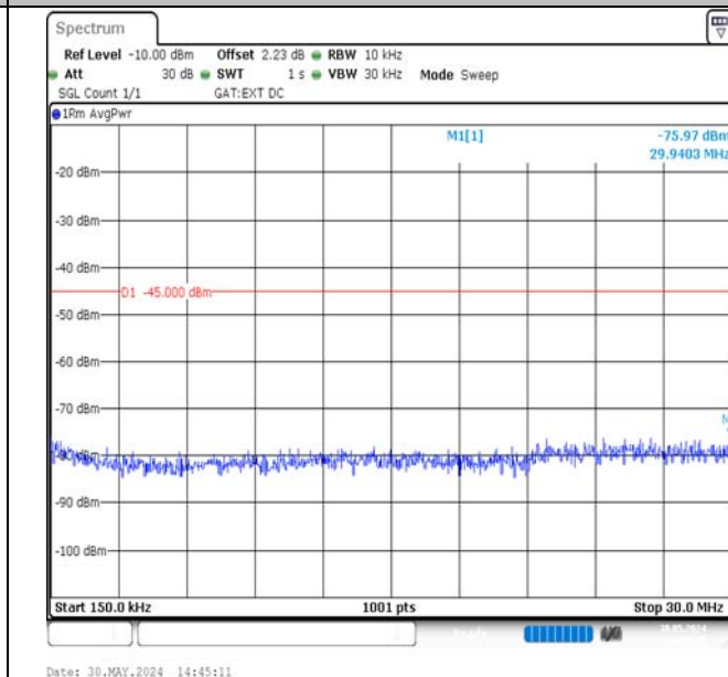
Band38-10MHz-16QAM-37800-1RB#49-0.15~30-PASS
