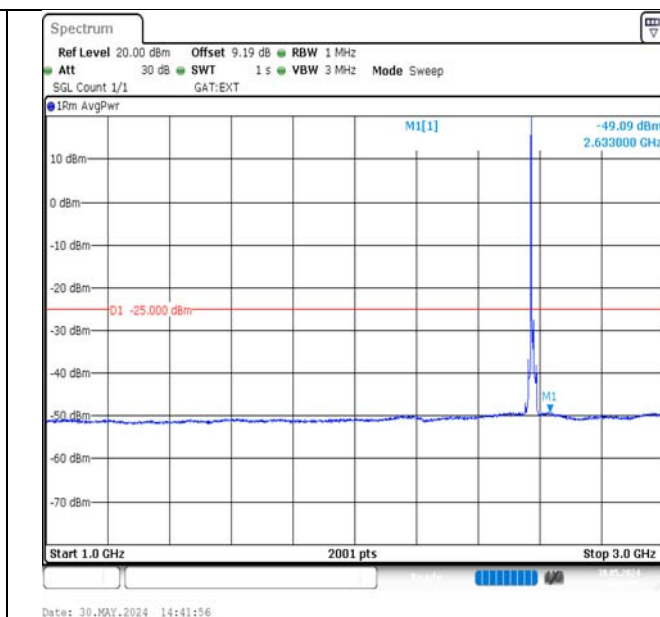
Band38-10MHz-16QAM-37800-1RB#0-1000~3000-PASS
