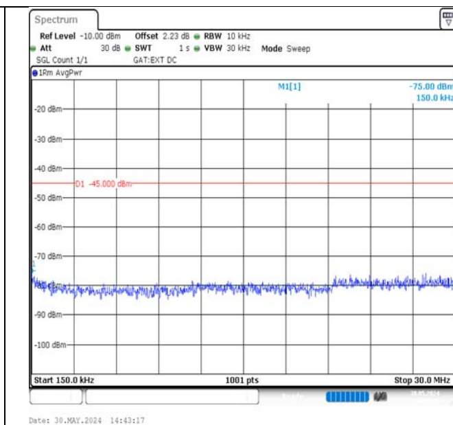
Band38-10MHz-QPSK-37800-1RB#49-0.15~30-PASS
