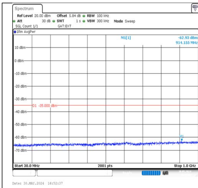
Band38-5MHz-16QAM-38225-1RB#24-30~1000-PASS
