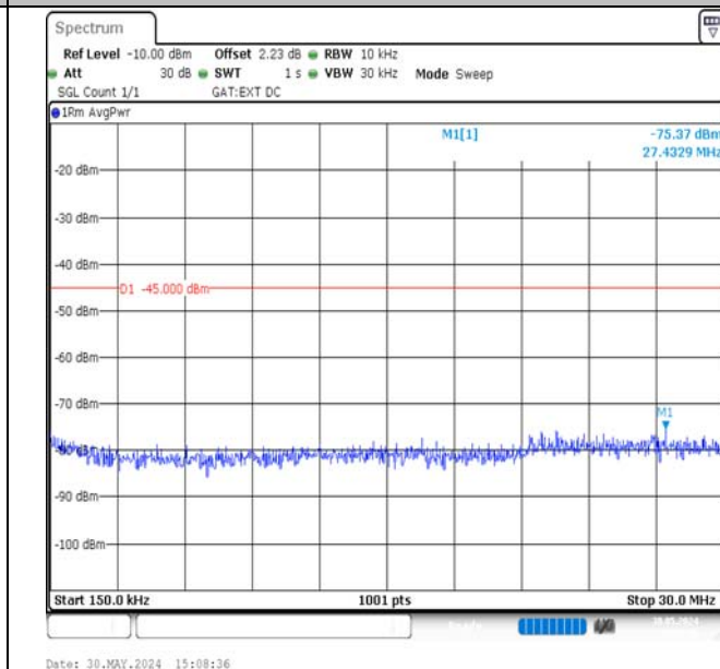
Band38-10MHz-16QAM-38200-1RB#49-0.15~30-PASS
