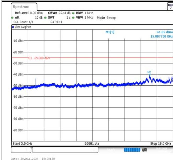
Band38-10MHz-16QAM-38200-1RB#0-3000~18000-PASS
