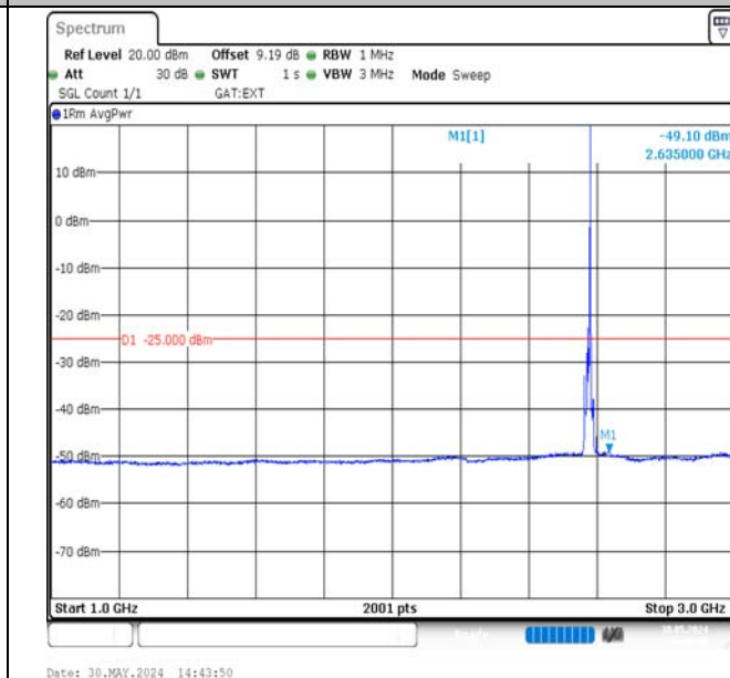
Band38-10MHz-QPSK-37800-1RB#49-1000~3000-PASS
