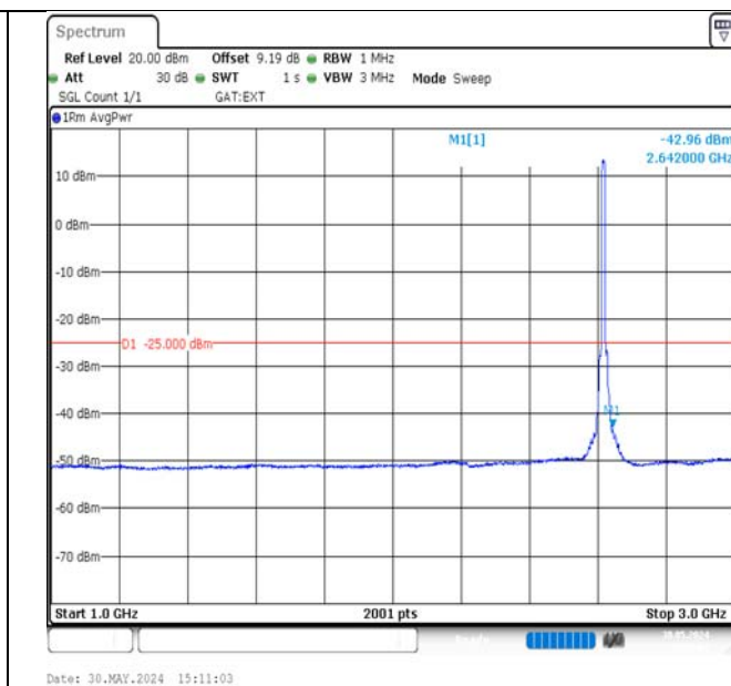
Band38-10MHz-QPSK-38200-50RB#0-1000~3000-PASS
