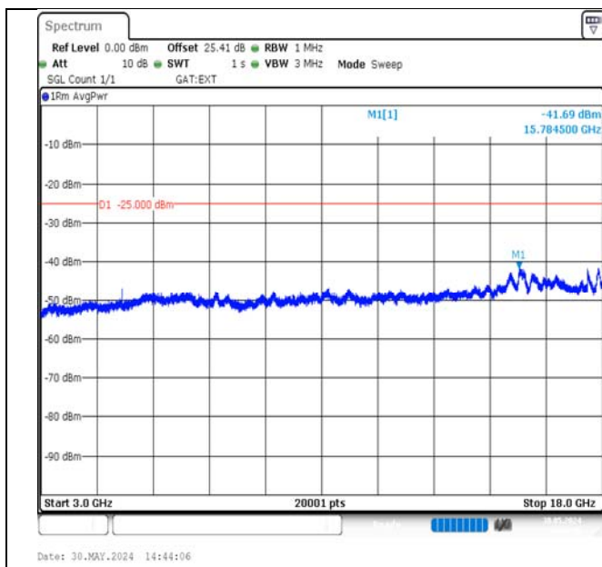
Band38-10MHz-QPSK-37800-1RB#49-3000~18000-PASS
