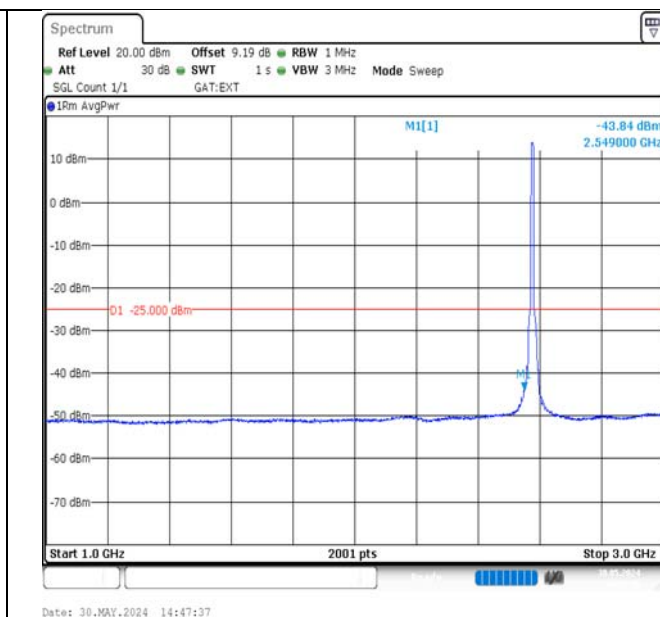
Band38-10MHz-QPSK-37800-50RB#0-1000~3000-PASS
