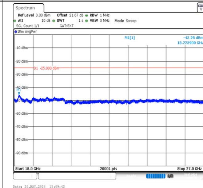
Band38-10MHz-16QAM-38200-1RB#49-18000~27000-PASS
