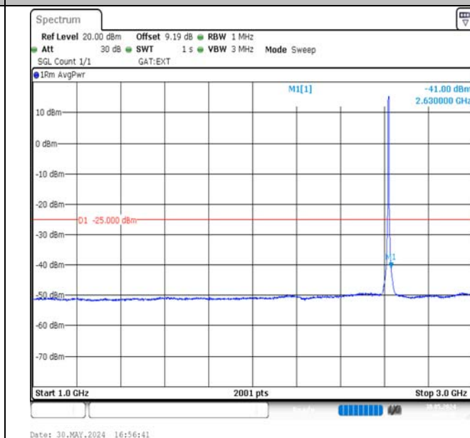
Band38-5MHz-16QAM-38225-25RB#0-1000~3000-PASS
