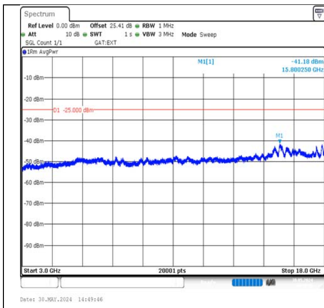
Band38-10MHz-16QAM-37800-50RB#0-3000~18000-PASS
