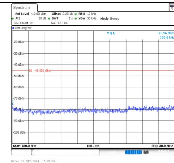
Band38-10MHz-QPSK-38200-1RB#0-0.15~30-PASS
