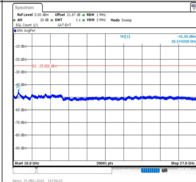
Band38-10MHz-QPSK-38000-1RB#49-18000~27000-PASS
