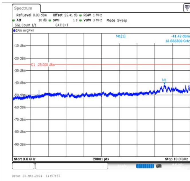
Band38-10MHz-16QAM-38000-1RB#49-3000~18000-PASS
