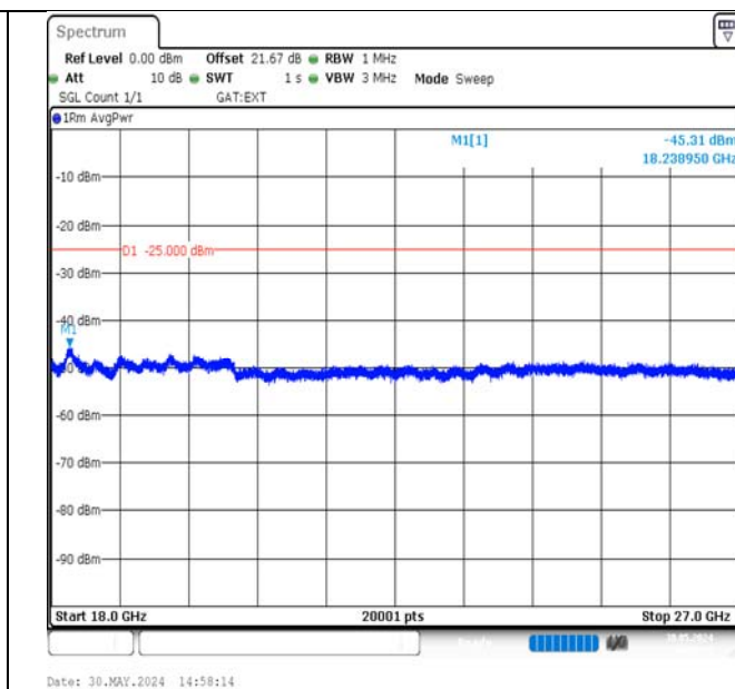
Band38-10MHz-16QAM-38000-1RB#49-18000~27000-PASS
