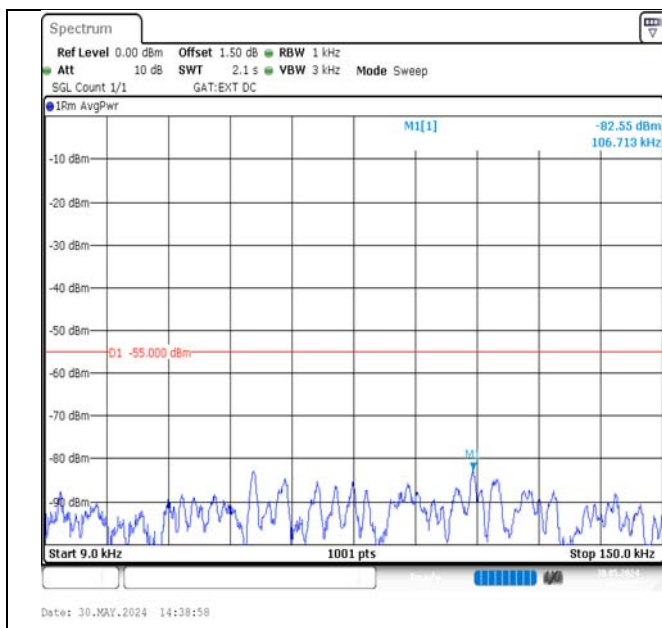
Band38-10MHz-QPSK-37800-1RB#0-0.009~0.15-PASS
