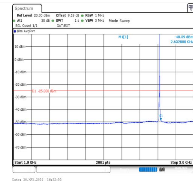
Band38-5MHz-16QAM-38225-1RB#24-1000~3000-PASS
