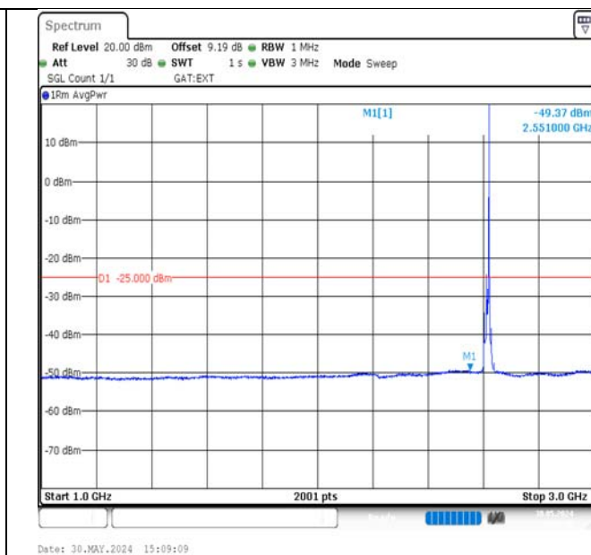
Band38-10MHz-16QAM-38200-1RB#49-1000~3000-PASS
