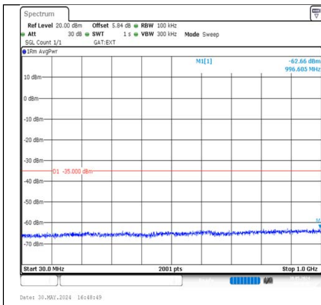
Band38-5MHz-16QAM-38225-1RB#0-30~1000-PASS
