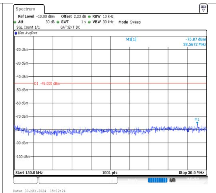
Band38-10MHz-16QAM-38200-50RB#0-0.15~30-PASS
