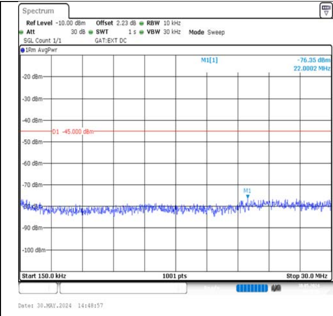
Band38-10MHz-16QAM-37800-50RB#0-0.15~30-PASS
