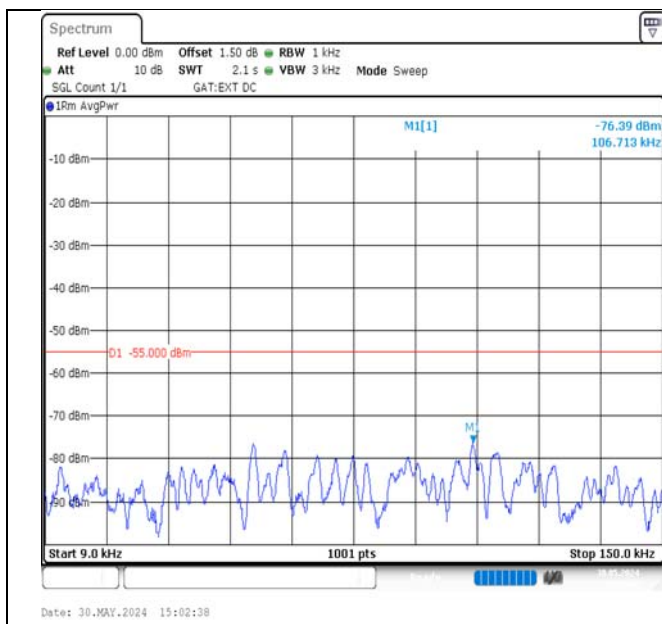
Band38-10MHz-QPSK-38200-1RB#0-0.009~0.15-PASS
