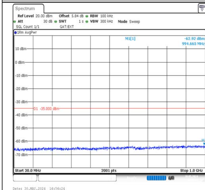
Band38-5MHz-16QAM-38225-25RB#0-30~1000-PASS
