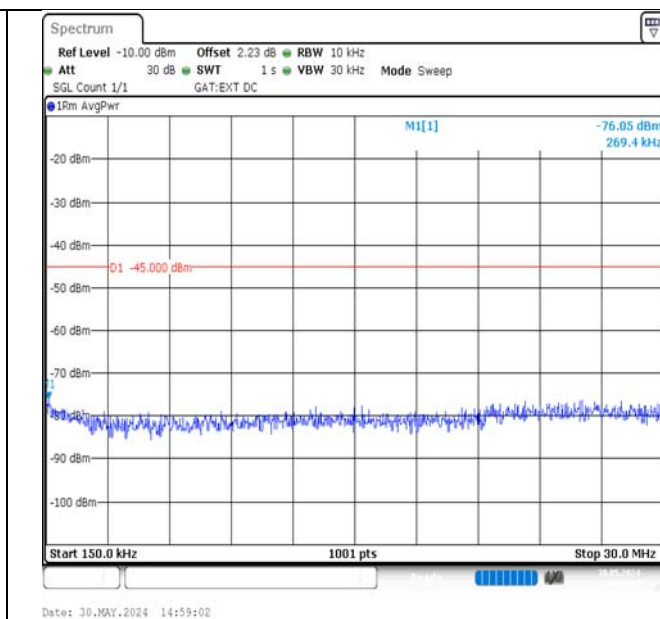
Band38-10MHz-QPSK-38000-50RB#0-0.15~30-PASS
