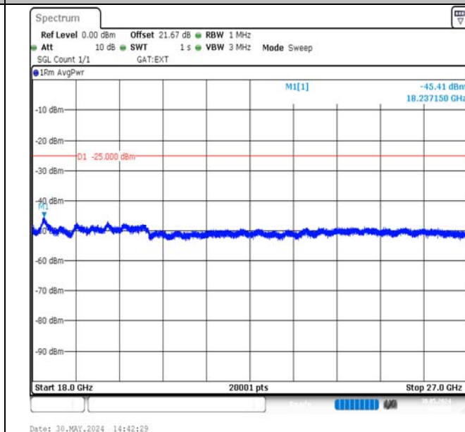
Band38-10MHz-16QAM-37800-1RB#0-18000~27000-PASS
