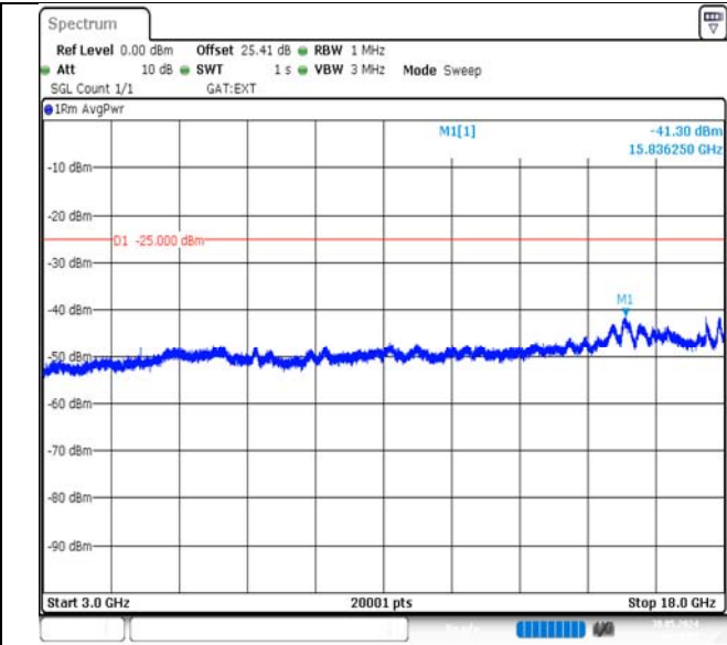
Band38-10MHz-QPSK-37800-1RB#0-3000~18000-PASS
