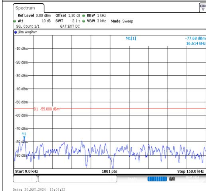
Band38-10MHz-16QAM-38200-1RB#0-0.009~0.15-PASS
