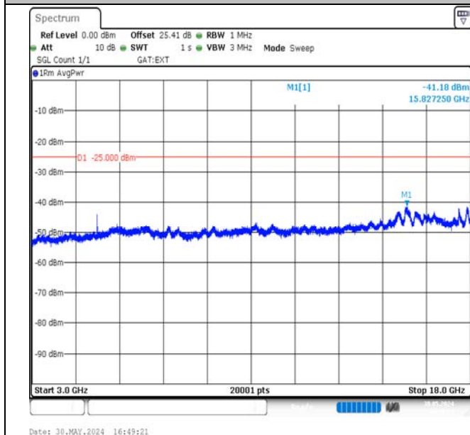
Band38-5MHz-16QAM-38225-1RB#0-3000~18000-PASS
