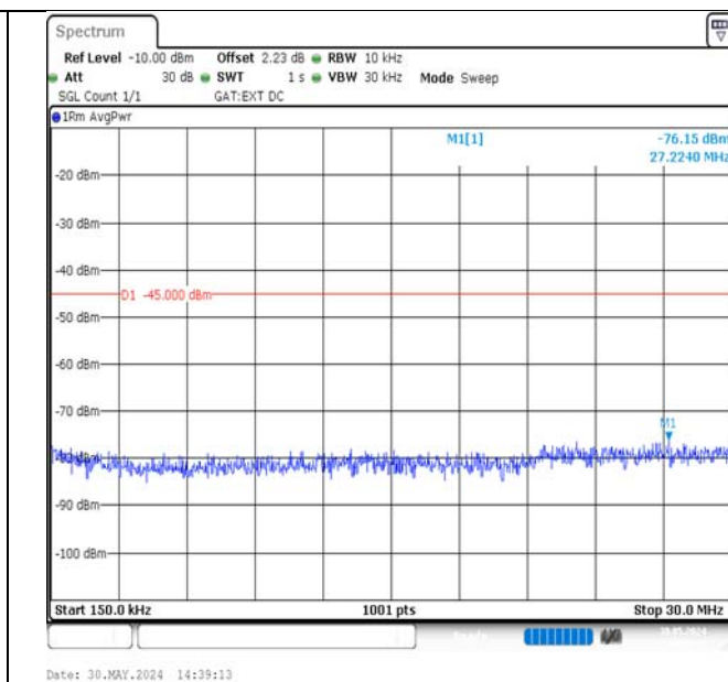
Band38-10MHz-QPSK-37800-1RB#0-0.15~30-PASS
