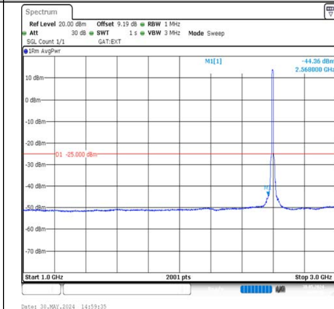
Band38-10MHz-QPSK-38000-50RB#0-1000~3000-PASS
