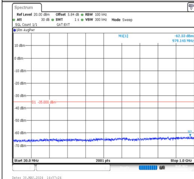
Band38-10MHz-16QAM-38000-1RB#49-30~1000-PASS
