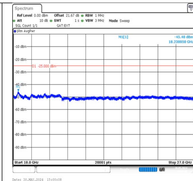
Band38-10MHz-QPSK-38000-50RB#0-18000~27000-PASS
