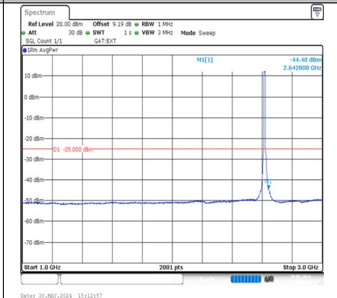
Band38-10MHz-16QAM-38200-50RB#0-1000~3000-PASS
