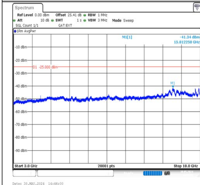
Band38-10MHz-16QAM-37800-1RB#49-3000~18000-PASS
