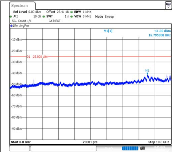
Band38-5MHz-16QAM-38000-1RB#24-3000~18000-PASS
