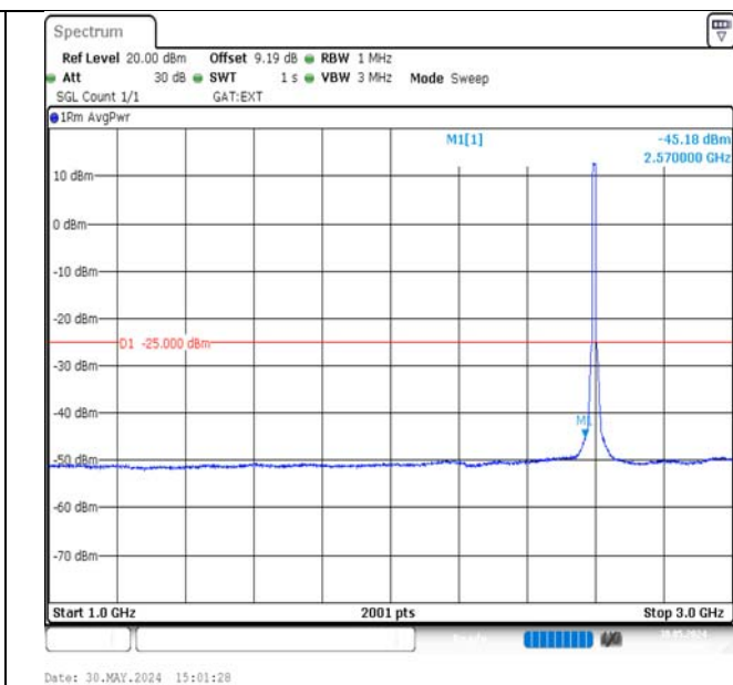
Band38-10MHz-16QAM-38000-50RB#0-1000~3000-PASS
