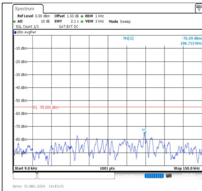
Band38-10MHz-QPSK-37800-1RB#49-0.009~0.15-PASS
