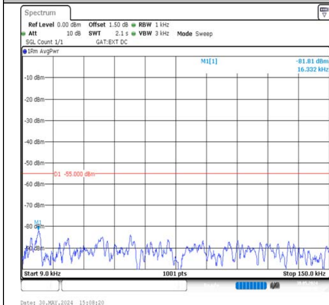
Band38-10MHz-16QAM-38200-1RB#49-0.009~0.15-PASS
