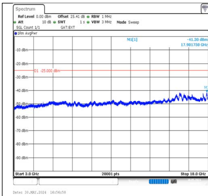
Band38-5MHz-16QAM-38225-25RB#0-3000~18000-PASS
