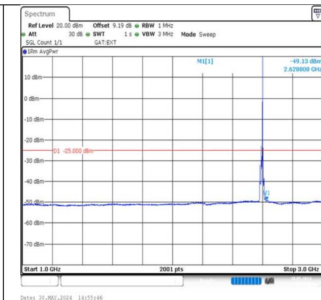
Band38-10MHz-QPSK-38000-1RB#49-1000~3000-PASS
