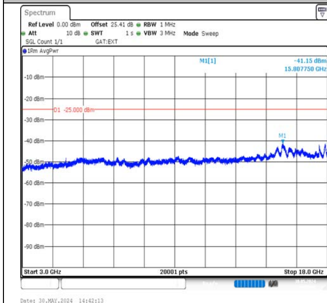
Band38-10MHz-16QAM-37800-1RB#0-3000~18000-PASS
