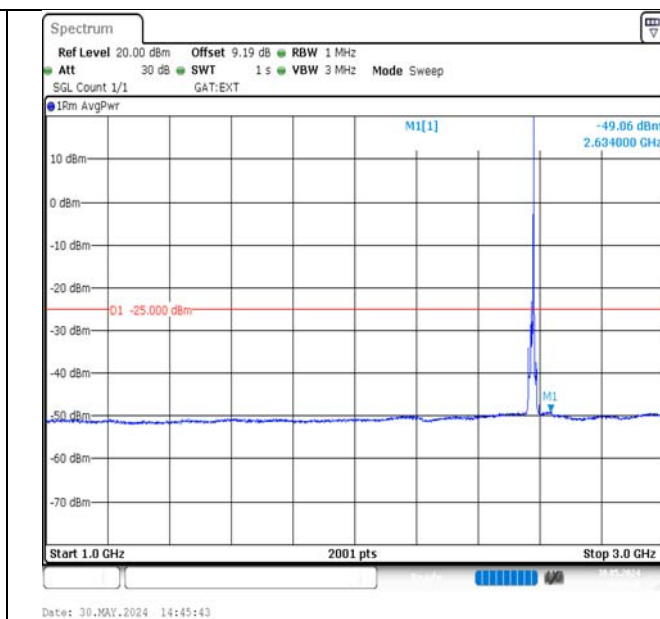
Band38-10MHz-16QAM-37800-1RB#49-1000~3000-PASS
