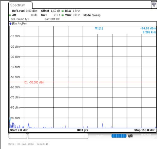
Band38-10MHz-16QAM-37800-50RB#0-0.009~0.15-PASS
