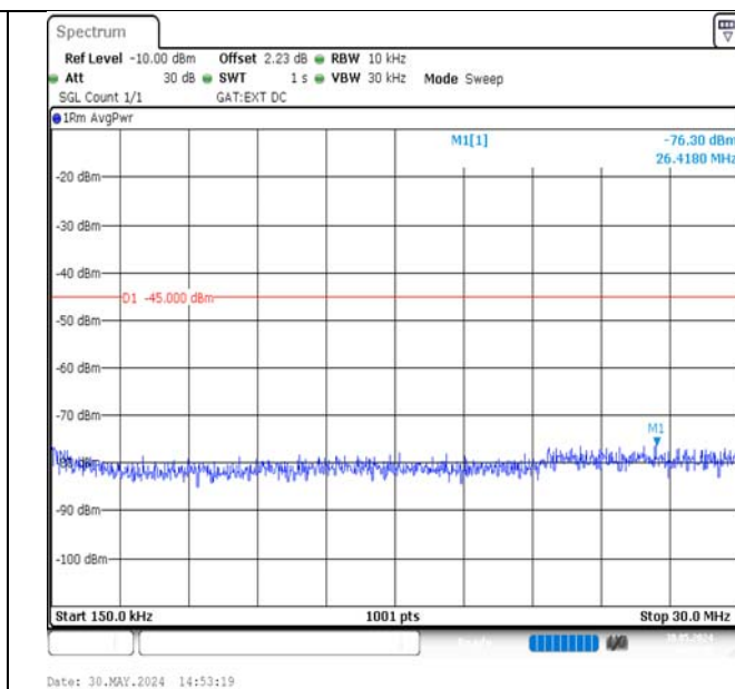
Band38-10MHz-16QAM-38000-1RB#0-0.15~30-PASS
