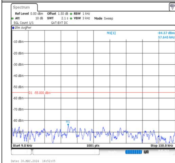
Band38-5MHz-16QAM-38225-1RB#24-0.009~0.15-PASS
