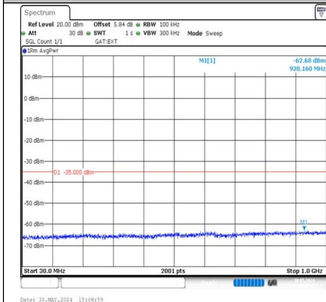
Band38-10MHz-QPSK-38200-1RB#49-30~1000-PASS
