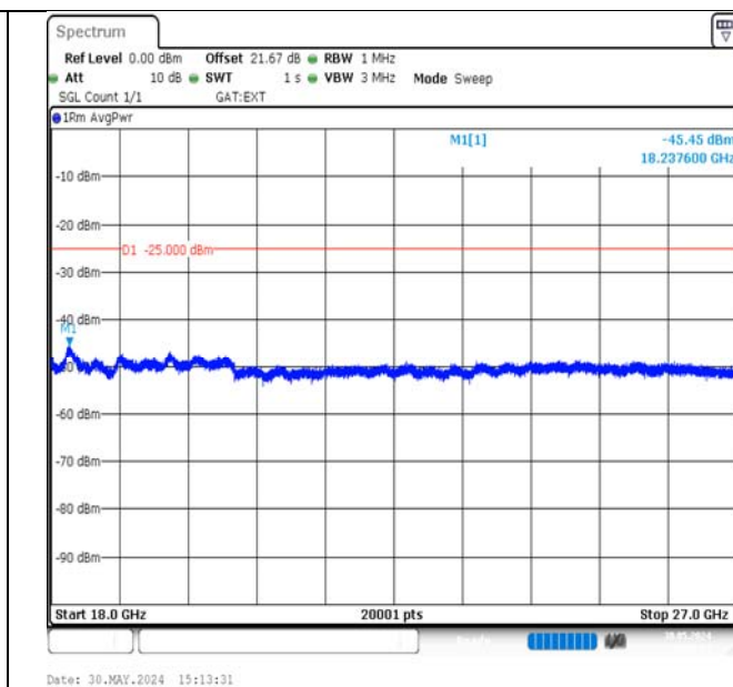
Band38-10MHz-16QAM-38200-50RB#0-18000~27000-PASS
