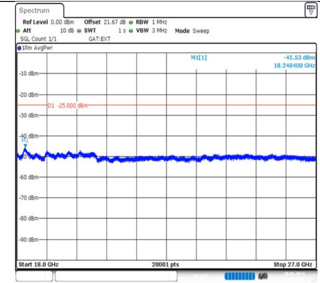
Band38-5MHz-16QAM-38000-1RB#24-18000~27000-PASS
