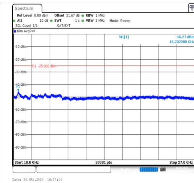
Band38-5MHz-16QAM-38225-25RB#0-18000~27000-PASS
