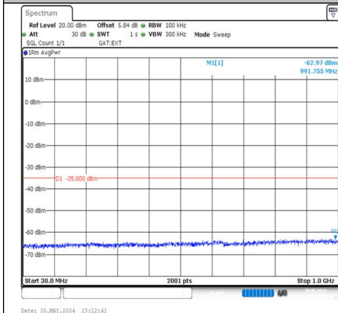
Band38-10MHz-16QAM-38200-50RB#0-30~1000-PASS
