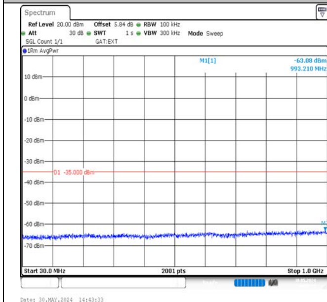
Band38-10MHz-QPSK-37800-1RB#49-30~1000-PASS
