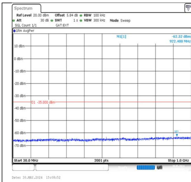
Band38-10MHz-16QAM-38200-1RB#49-30~1000-PASS
