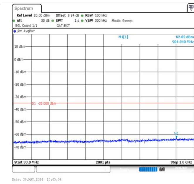
Band38-10MHz-16QAM-38200-1RB#0-30~1000-PASS
