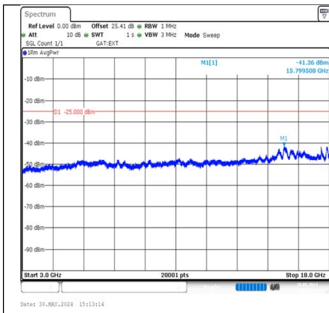
Band38-10MHz-16QAM-38200-50RB#0-3000~18000-PASS
