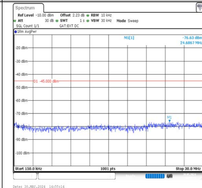
Band38-10MHz-QPSK-38000-1RB#49-0.15~30-PASS
