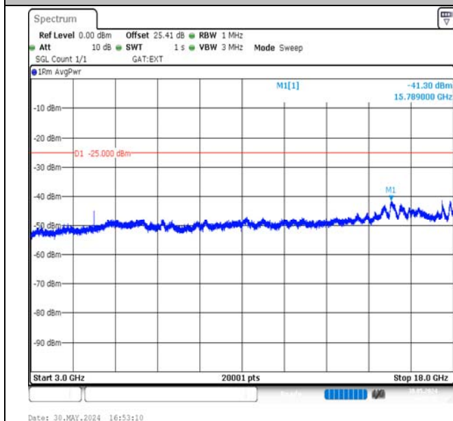
Band38-5MHz-16QAM-38225-1RB#24-3000~18000-PASS
