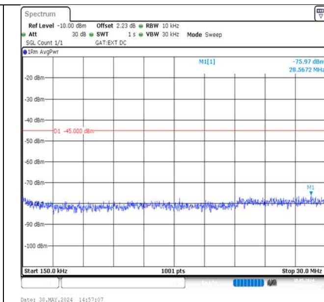
Band38-10MHz-16QAM-38000-1RB#49-0.15~30-PASS
