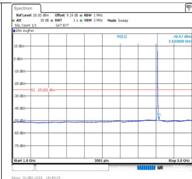
Band38-5MHz-16QAM-38225-1RB#0-1000~3000-PASS
