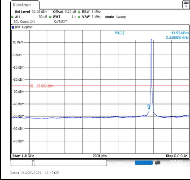
Band38-10MHz-16QAM-37800-50RB#0-1000~3000-PASS
