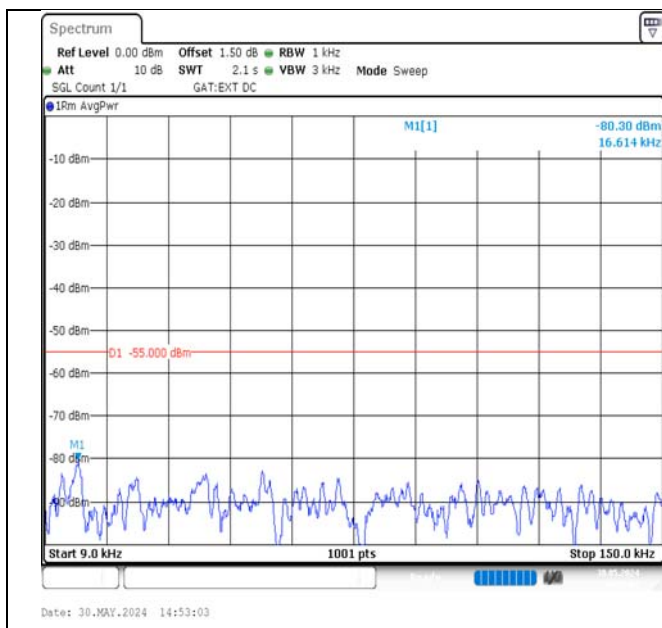
Band38-10MHz-16QAM-38000-1RB#0-0.009~0.15-PASS
