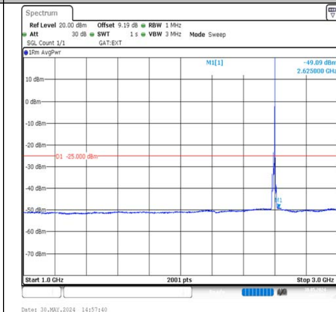
Band38-10MHz-16QAM-38000-1RB#49-1000~3000-PASS
