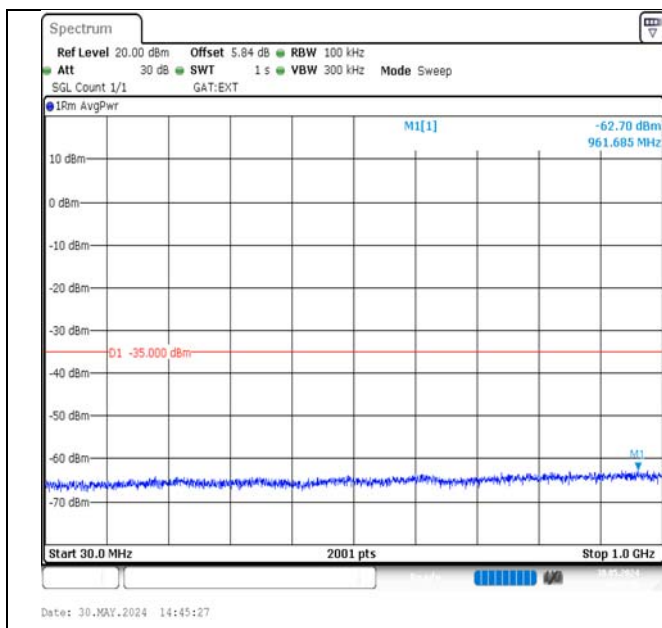
Band38-10MHz-16QAM-37800-1RB#49-30~1000-PASS
