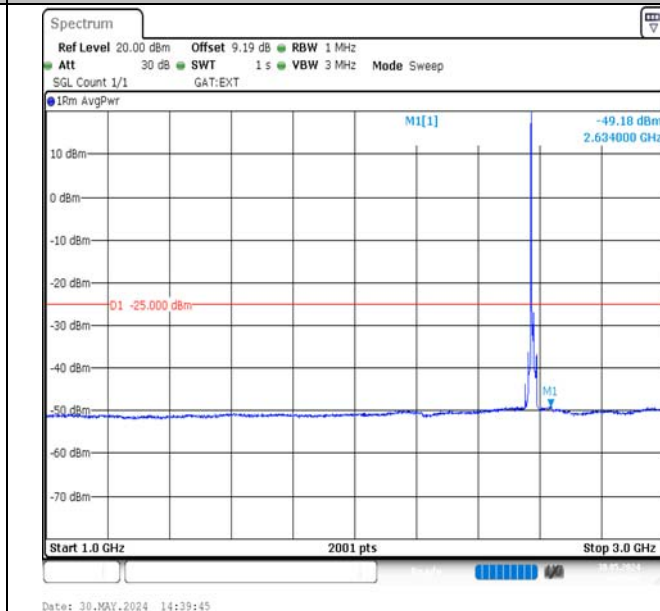
Band38-10MHz-QPSK-37800-1RB#0-1000~3000-PASS
