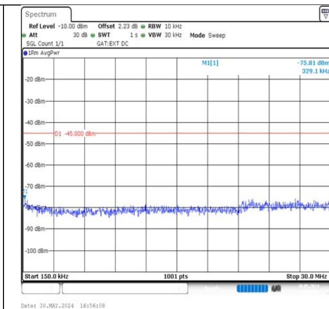
Band38-5MHz-16QAM-38225-25RB#0-0.15~30-PASS
