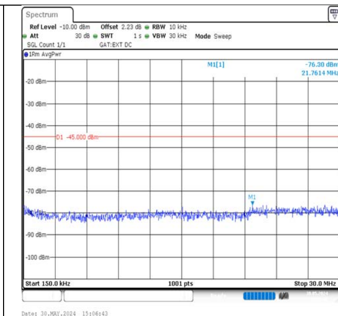
Band38-10MHz-QPSK-38200-1RB#49-0.15~30-PASS
