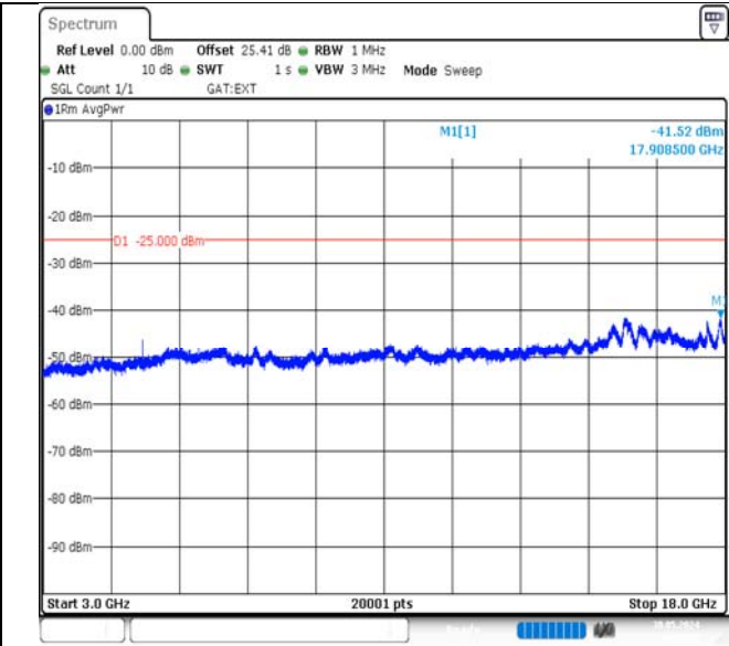
Band38-10MHz-16QAM-38000-1RB#0-3000~18000-PASS
