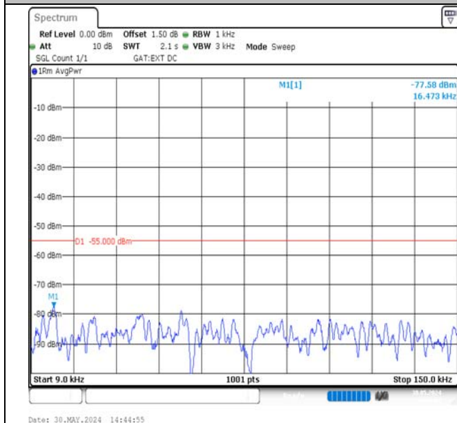
Band38-10MHz-16QAM-37800-1RB#49-0.009~0.15-PASS
