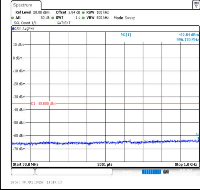
Band38-10MHz-16QAM-37800-50RB#0-30~1000-PASS
