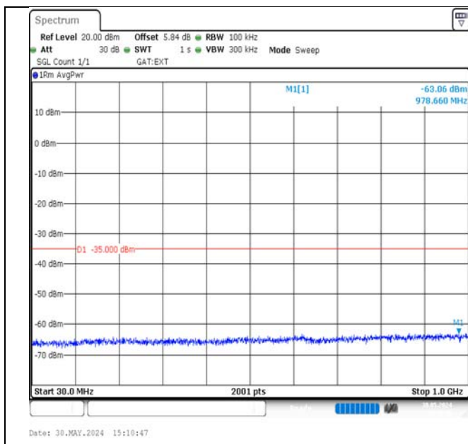
Band38-10MHz-QPSK-38200-50RB#0-30~1000-PASS
