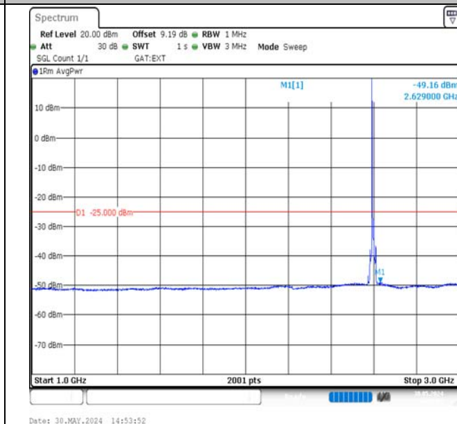
Band38-10MHz-16QAM-38000-1RB#0-1000~3000-PASS
