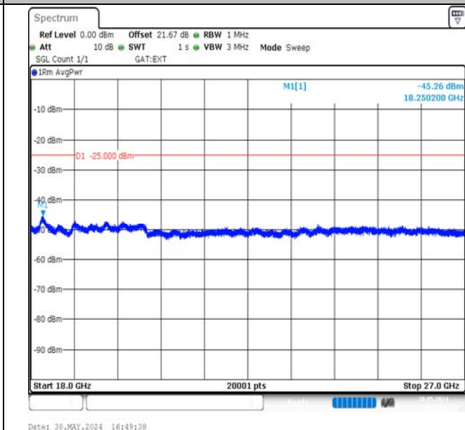
Band38-5MHz-16QAM-38225-1RB#0-18000~27000-PASS
