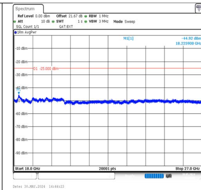
Band38-10MHz-QPSK-37800-1RB#49-18000~27000-PASS
