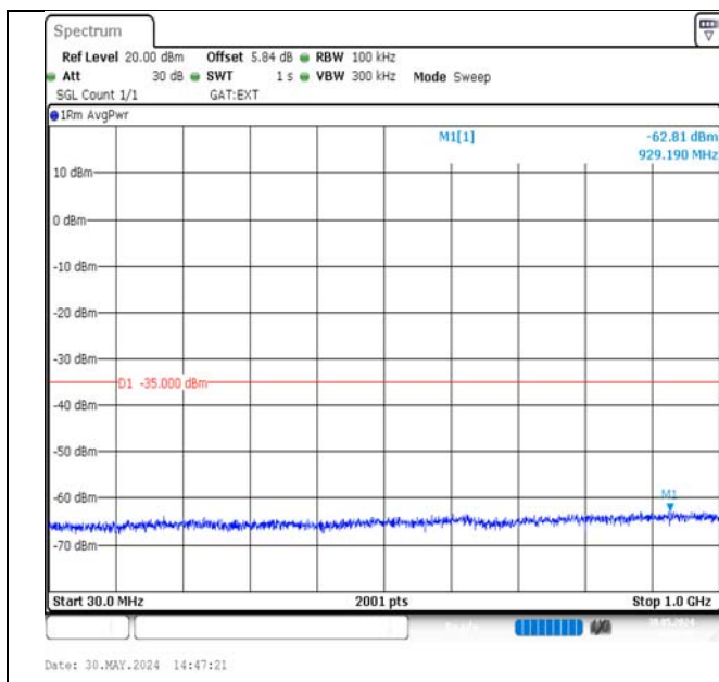
Band38-10MHz-QPSK-37800-50RB#0-30~1000-PASS
