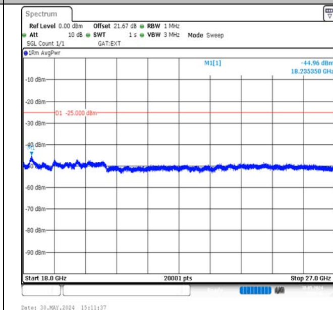
Band38-10MHz-QPSK-38200-50RB#0-18000~27000-PASS
