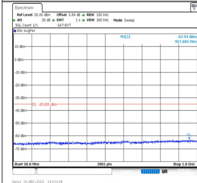
Band38-10MHz-16QAM-38000-1RB#0-30~1000-PASS
