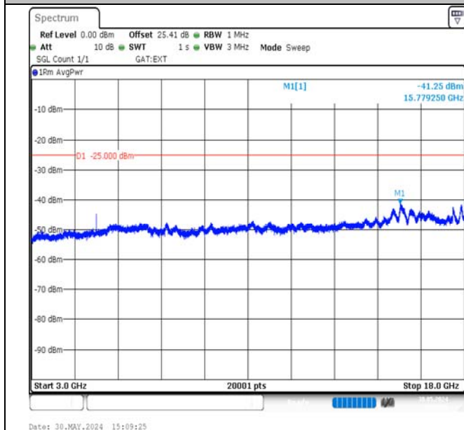
Band38-10MHz-16QAM-38200-1RB#49-3000~18000-PASS
