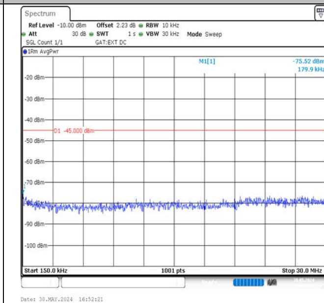
Band38-5MHz-16QAM-38225-1RB#24-0.15~30-PASS
