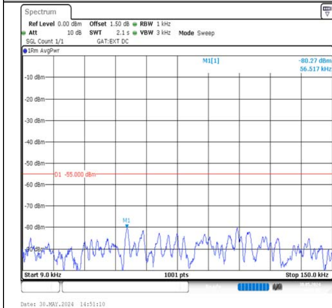
Band38-10MHz-QPSK-38000-1RB#0-0.009~0.15-PASS
