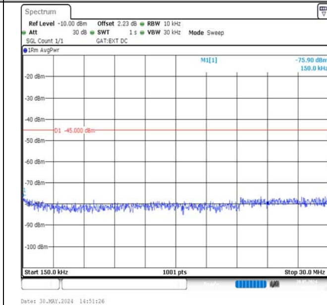
Band38-10MHz-QPSK-38000-1RB#0-0.15~30-PASS
