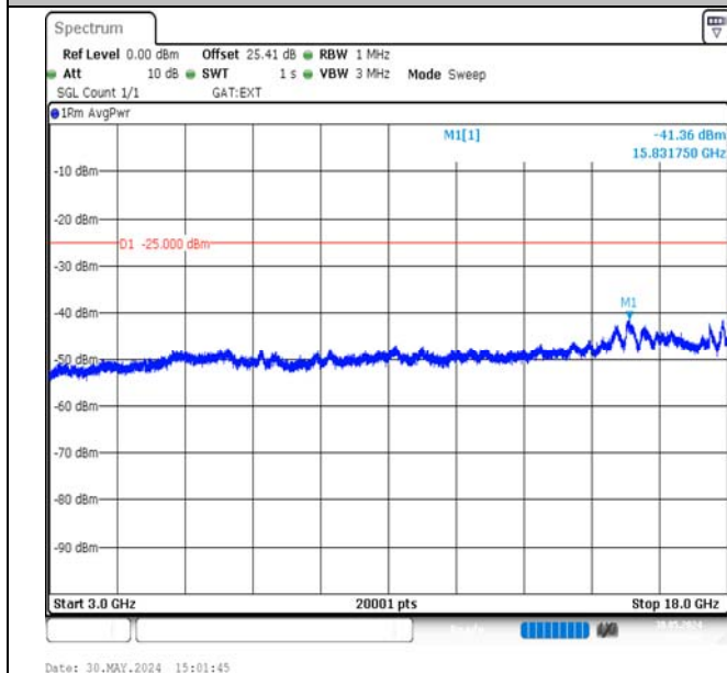
Band38-10MHz-16QAM-38000-50RB#0-3000~18000-PASS
