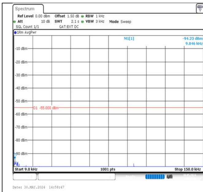
Band38-10MHz-QPSK-38000-50RB#0-0.009~0.15-PASS
