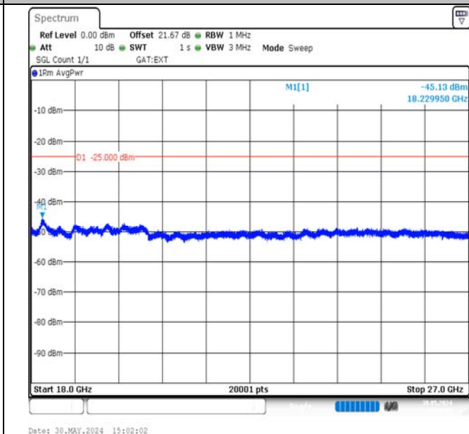
Band38-10MHz-16QAM-38000-50RB#0-18000~27000-PASS
