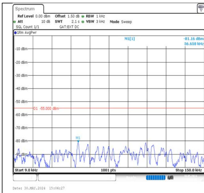
Band38-10MHz-QPSK-38200-1RB#49-0.009~0.15-PASS
