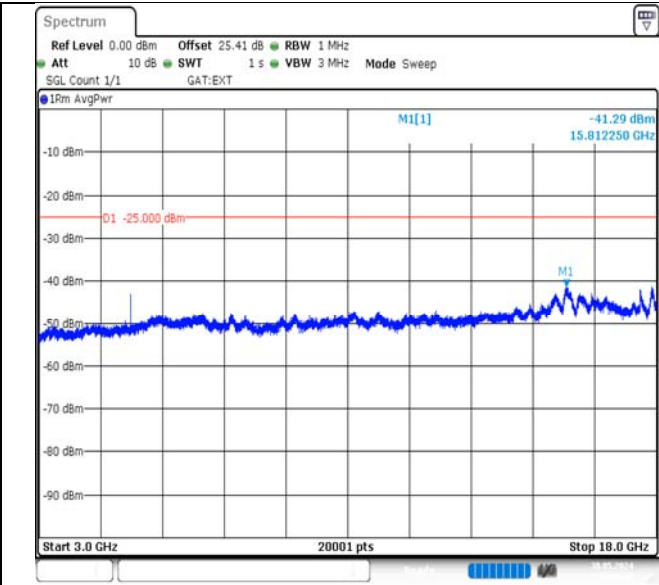
Band38-10MHz-QPSK-38200-1RB#0-3000~18000-PASS
