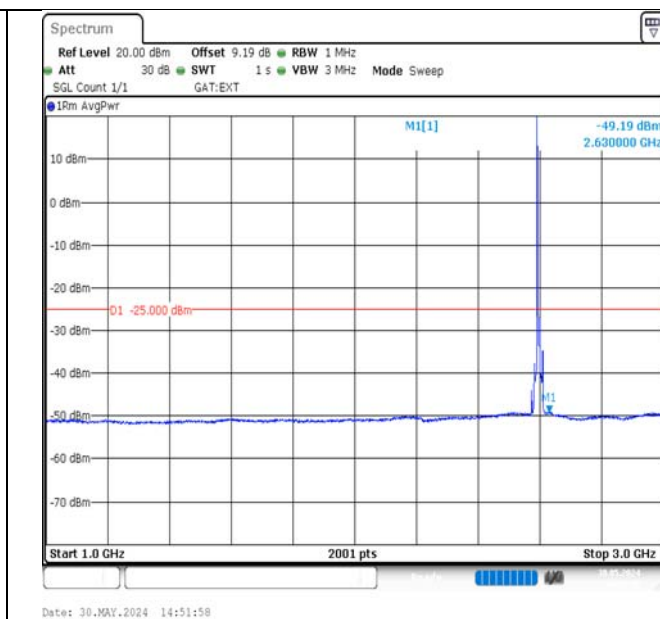
Band38-10MHz-QPSK-38000-1RB#0-1000~3000-PASS
