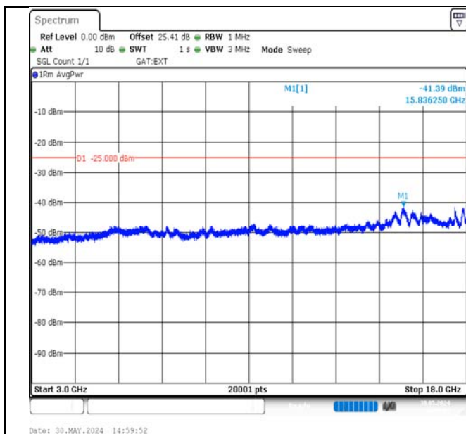
Band38-10MHz-QPSK-38000-50RB#0-3000~18000-PASS
