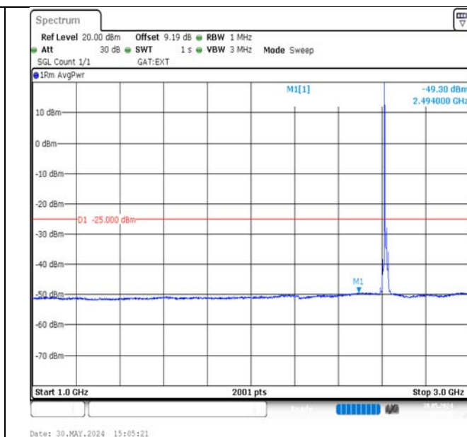
Band38-10MHz-16QAM-38200-1RB#0-1000~3000-PASS
