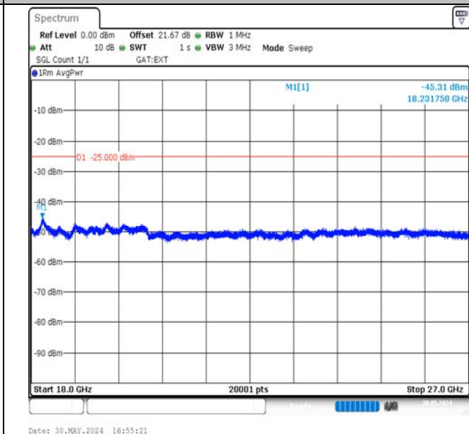
Band38-5MHz-QPSK-38225-25RB#0-18000~27000-PASS
