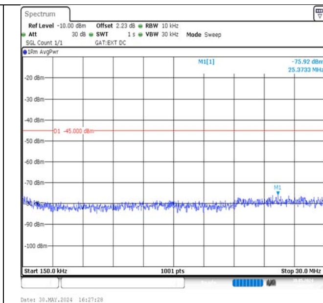
Band38-5MHz-QPSK-37775-1RB#24-0.15~30-PASS
