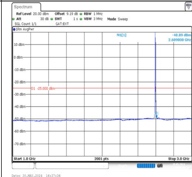
Band38-5MHz-16QAM-38000-1RB#0-1000~3000-PASS
