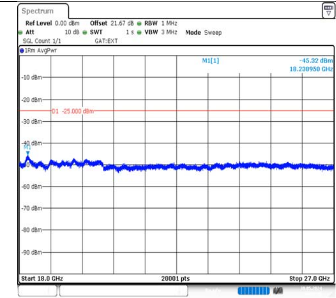
Band38-5MHz-QPSK-38225-1RB#0-18000~27000-PASS
