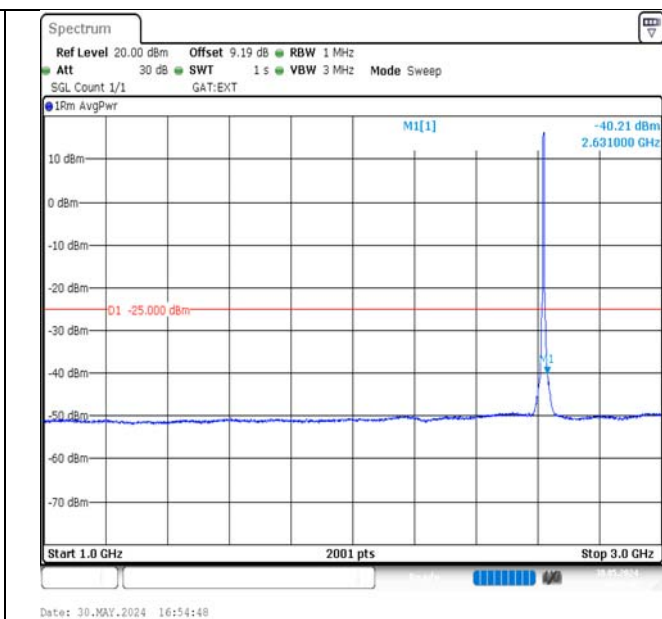
Band38-5MHz-QPSK-38225-25RB#0-1000~3000-PASS
