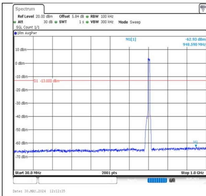
Band17-10MHz-16QAM-23800-50RB#0-30~1000-PASS
