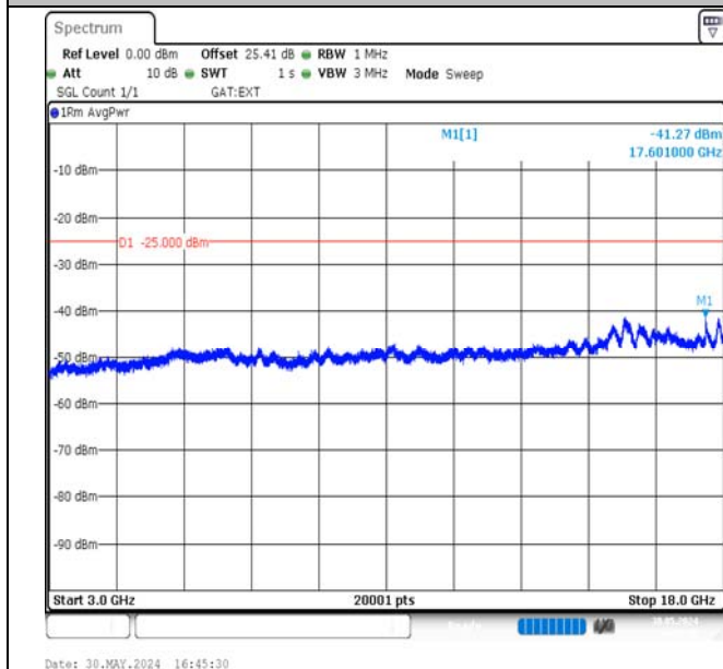
Band38-5MHz-16QAM-38000-25RB#0-3000~18000-PASS
