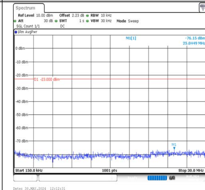
Band17-10MHz-16QAM-23800-50RB#0-0.15~30-PASS
