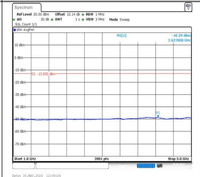
Band17-10MHz-16QAM-23780-50RB#0-1000~3000-PASS
