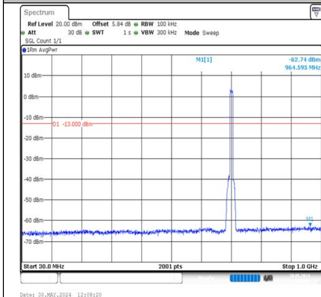
Band17-10MHz-16QAM-23780-50RB#0-30~1000-PASS
