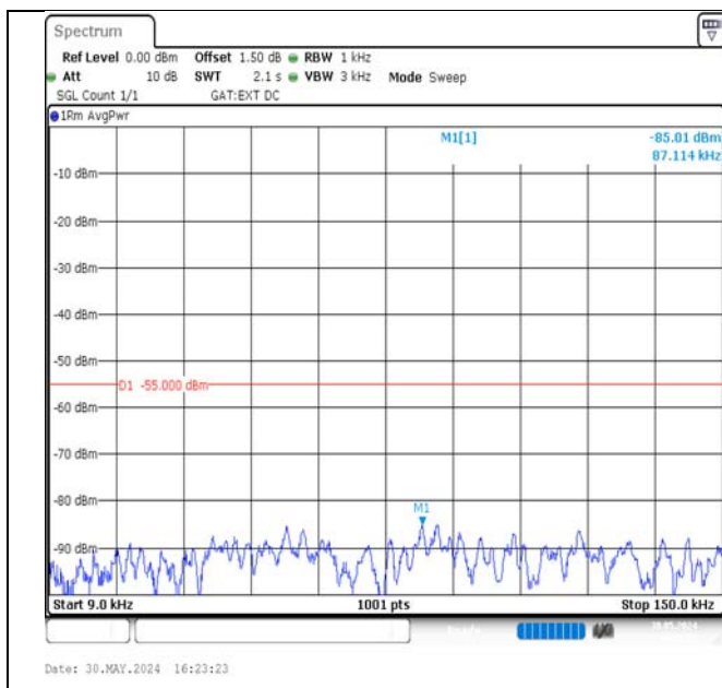
Band38-5MHz-QPSK-37775-1RB#0-0.009~0.15-PASS
