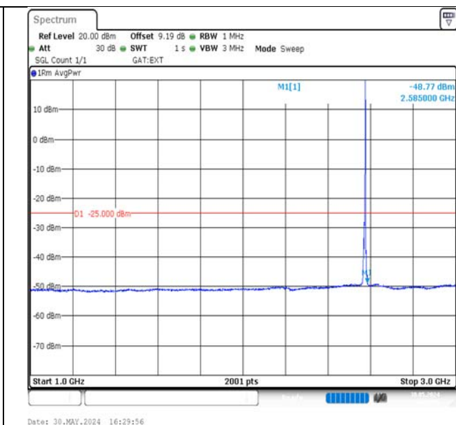
Band38-5MHz-16QAM-37775-1RB#24-1000~3000-PASS
