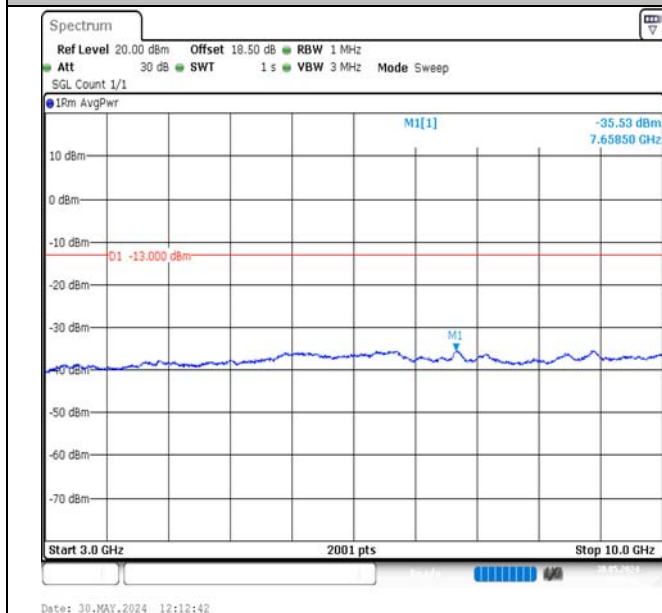
Band17-10MHz-16QAM-23800-50RB#0-3000~10000-PASS
