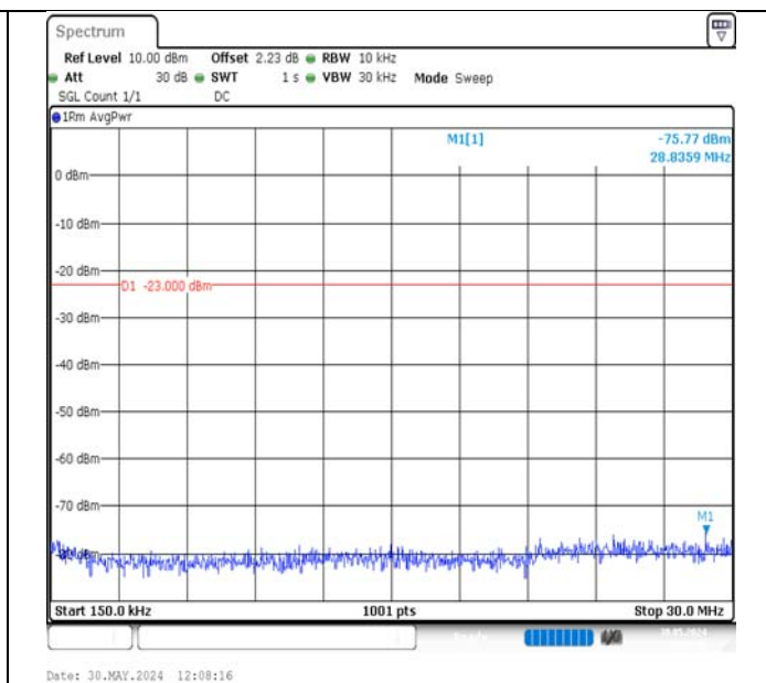
Band17-10MHz-16QAM-23780-50RB#0-0.15~30-PASS
