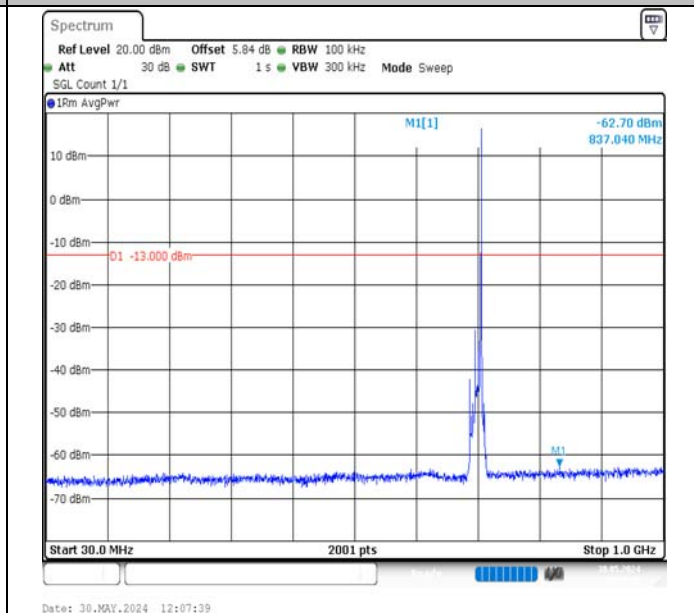
Band17-10MHz-16QAM-23780-1RB#49-30~1000-PASS
