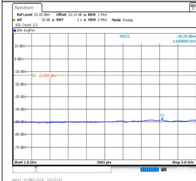
Band17-10MHz-16QAM-23790-50RB#0-1000~3000-PASS
