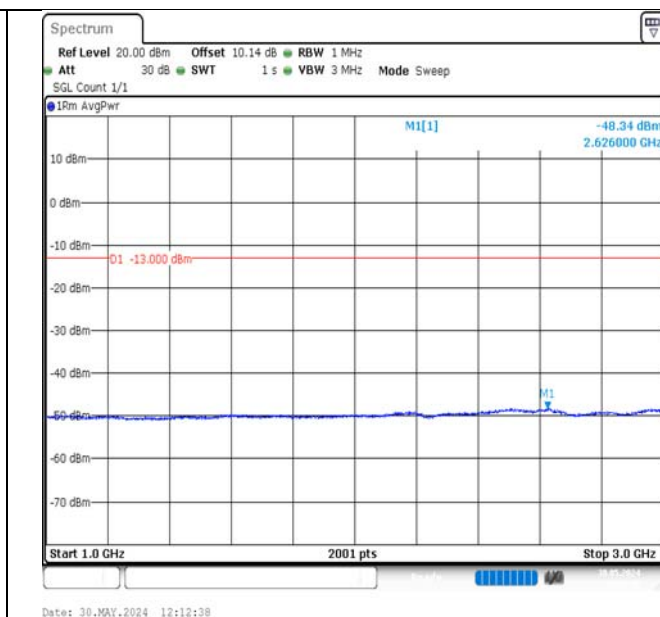
Band17-10MHz-16QAM-23800-50RB#0-1000~3000-PASS
