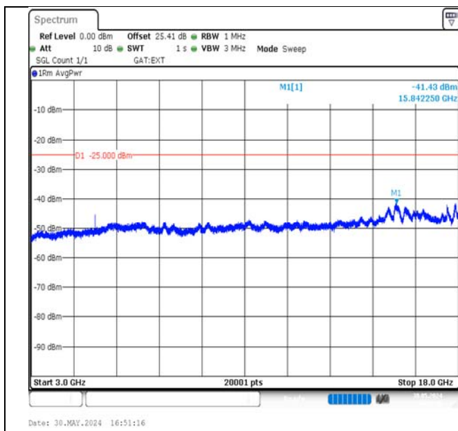
Band38-5MHz-QPSK-38225-1RB#24-3000~18000-PASS
