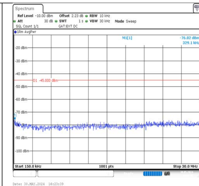
Band38-5MHz-QPSK-37775-1RB#0-0.15~30-PASS
