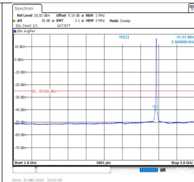
Band38-5MHz-QPSK-37775-25RB#0-1000~3000-PASS
