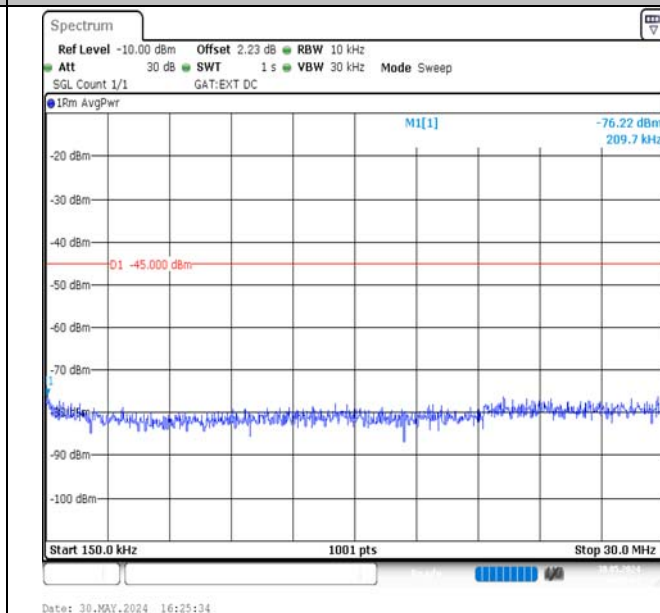
Band38-5MHz-16QAM-37775-1RB#0-0.15~30-PASS
