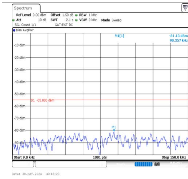
Band38-5MHz-QPSK-38225-1RB#0-0.009~0.15-PASS
