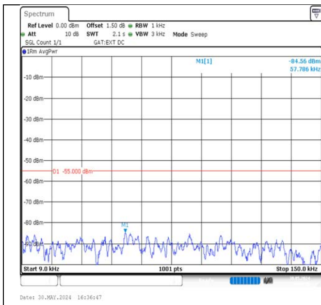
Band38-5MHz-16QAM-38000-1RB#0-0.009~0.15-PASS
