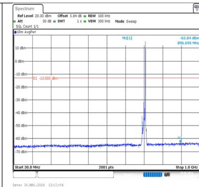
Band17-10MHz-16QAM-23800-1RB#49-30~1000-PASS
