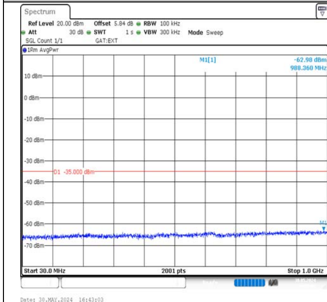
Band38-5MHz-QPSK-38000-25RB#0-30~1000-PASS
