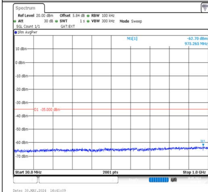
Band38-5MHz-16QAM-38000-1RB#24-30~1000-PASS
