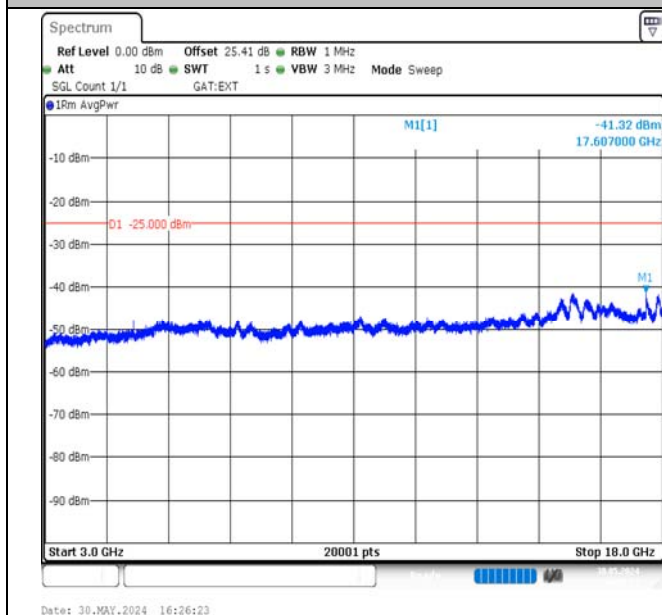
Band38-5MHz-16QAM-37775-1RB#0-3000~18000-PASS
