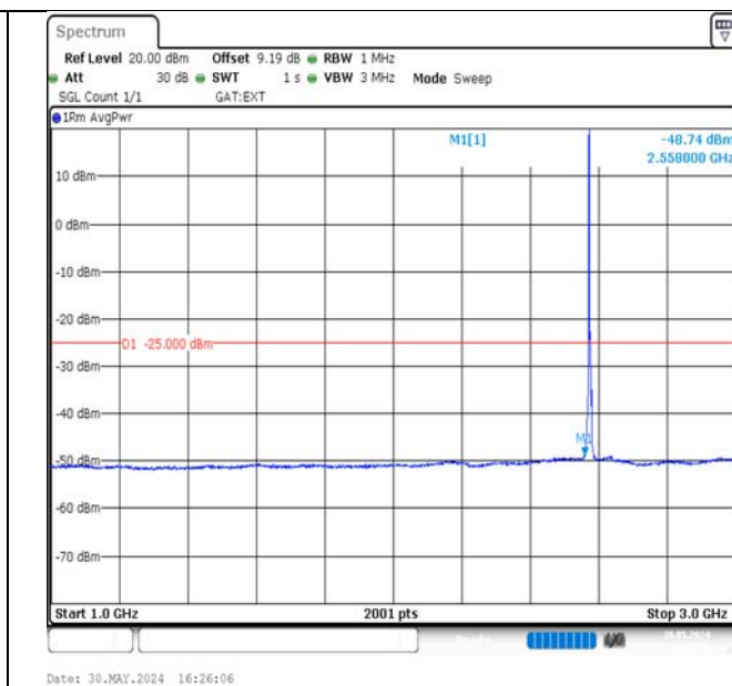
Band38-5MHz-16QAM-37775-1RB#0-1000~3000-PASS
