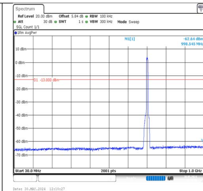
Band17-10MHz-16QAM-23790-50RB#0-30~1000-PASS
