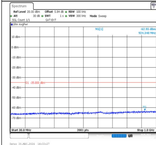
Band38-5MHz-16QAM-37775-25RB#0-30~1000-PASS
