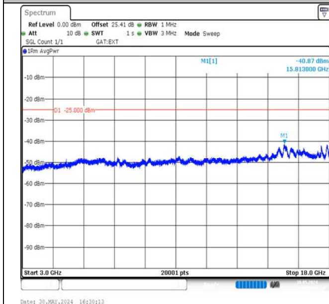
Band38-5MHz-16QAM-37775-1RB#24-3000~18000-PASS
