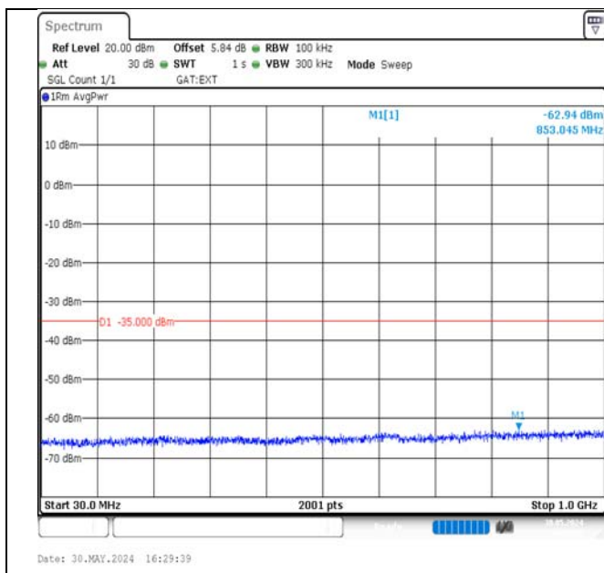
Band38-5MHz-16QAM-37775-1RB#24-30~1000-PASS
