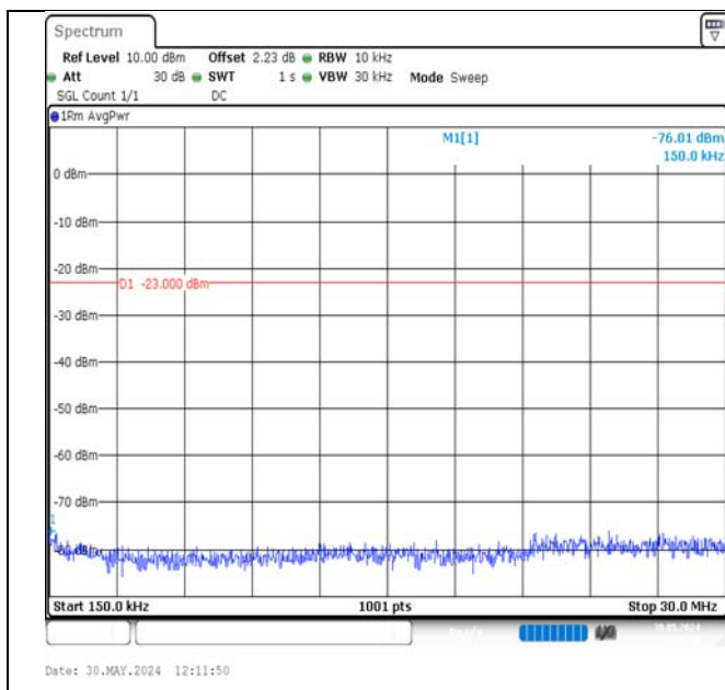
Band17-10MHz-16QAM-23800-1RB#49-0.15~30-PASS
