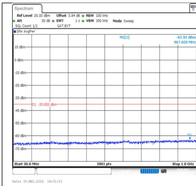
Band38-5MHz-QPSK-37775-25RB#0-30~1000-PASS
