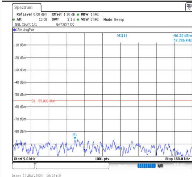
Band38-5MHz-16QAM-37775-1RB#0-0.009~0.15-PASS
