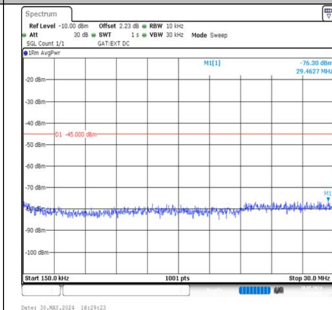
Band38-5MHz-16QAM-37775-1RB#24-0.15~30-PASS
