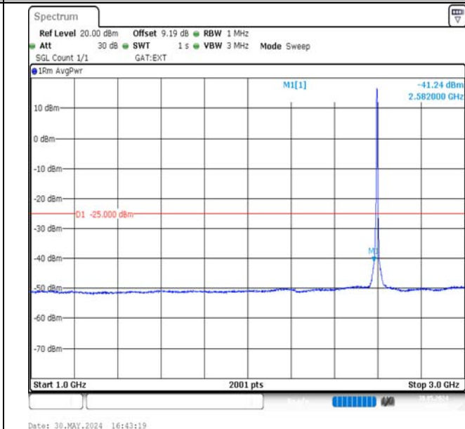
Band38-5MHz-QPSK-38000-25RB#0-1000~3000-PASS
