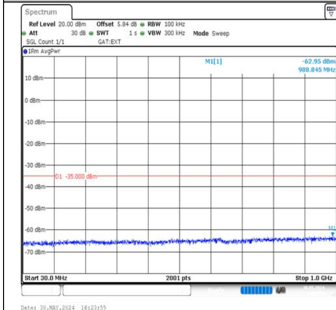
Band38-5MHz-QPSK-37775-1RB#0-30~1000-PASS
