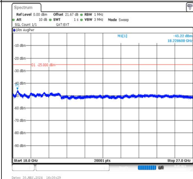
Band38-5MHz-16QAM-37775-1RB#24-18000~27000-PASS
