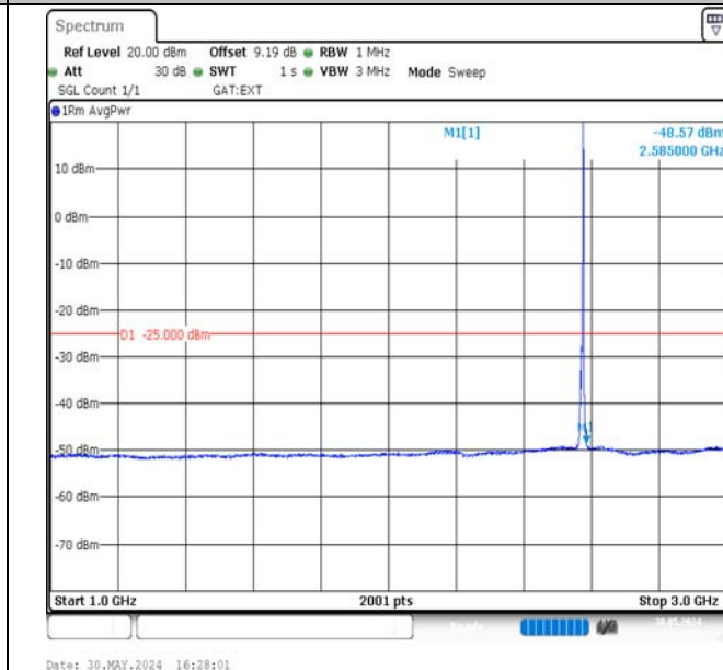
Band38-5MHz-QPSK-37775-1RB#24-1000~3000-PASS
