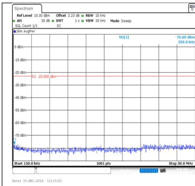
Band17-10MHz-16QAM-23790-50RB#0-0.15~30-PASS
