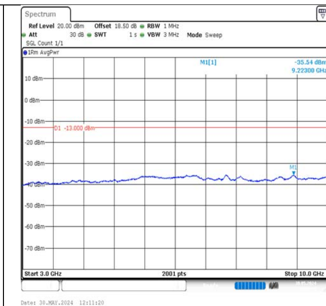
Band17-10MHz-16QAM-23800-1RB#0-3000~10000-PASS
