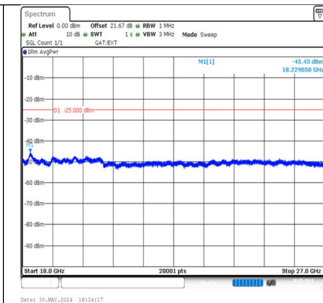
Band38-5MHz-16QAM-37775-25RB#0-18000~27000-PASS
