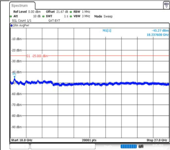
Band38-5MHz-QPSK-37775-1RB#0-18000~27000-PASS
