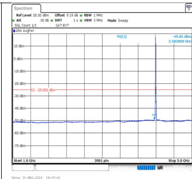
Band38-5MHz-QPSK-38000-1RB#0-1000~3000-PASS
