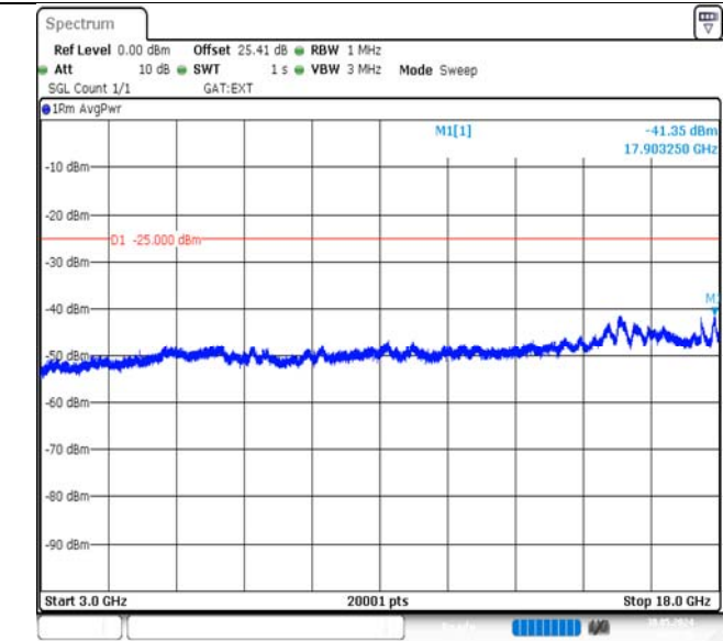
Band38-5MHz-QPSK-38000-25RB#0-3000~18000-PASS
