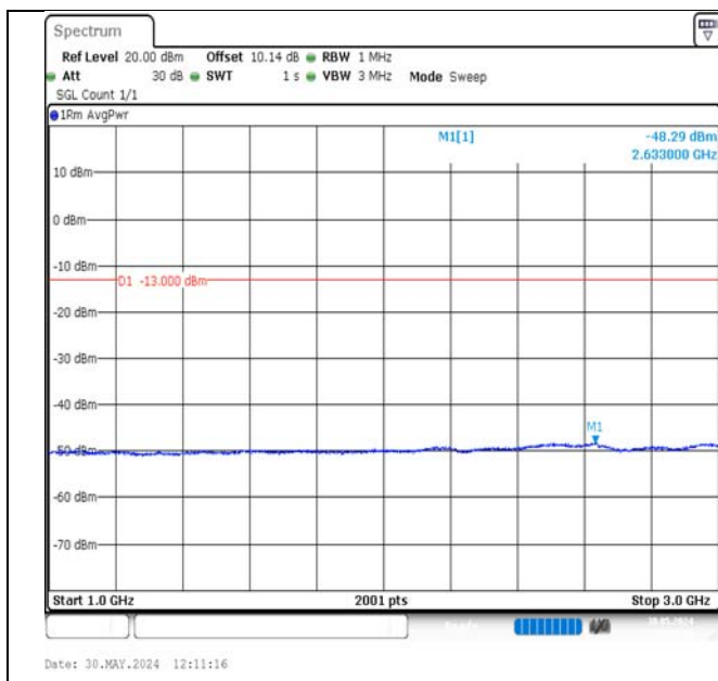
Band17-10MHz-16QAM-23800-1RB#0-1000~3000-PASS
