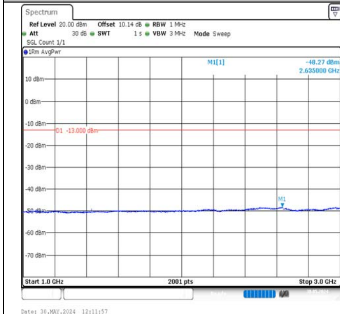
Band17-10MHz-16QAM-23800-1RB#49-1000~3000-PASS
