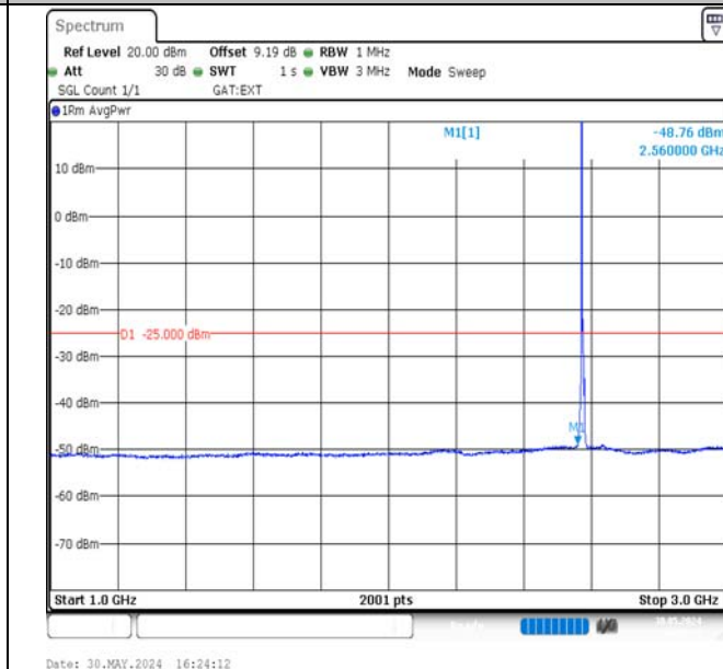
Band38-5MHz-QPSK-37775-1RB#0-1000~3000-PASS
