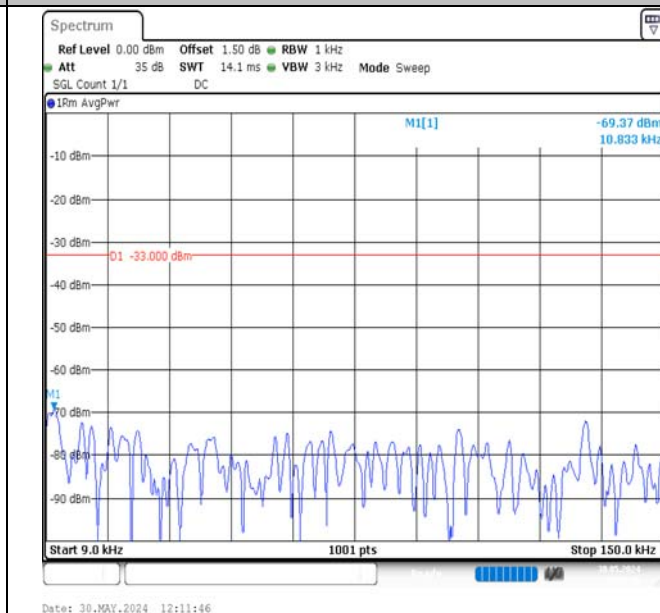
Band17-10MHz-16QAM-23800-1RB#49-0.009~0.15-PASS
