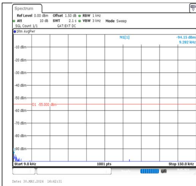
Band38-5MHz-QPSK-38000-25RB#0-0.009~0.15-PASS
