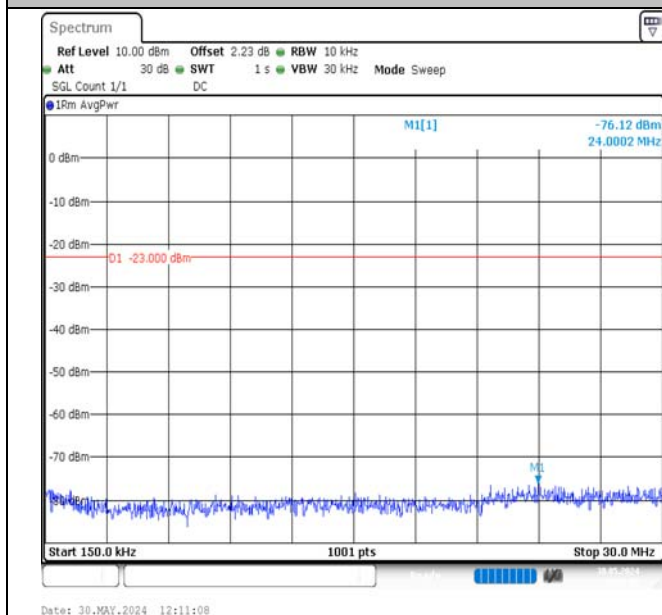
Band17-10MHz-16QAM-23800-1RB#0-0.15~30-PASS
