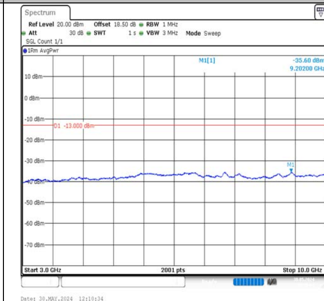
Band17-10MHz-16QAM-23790-50RB#0-3000~10000-PASS
