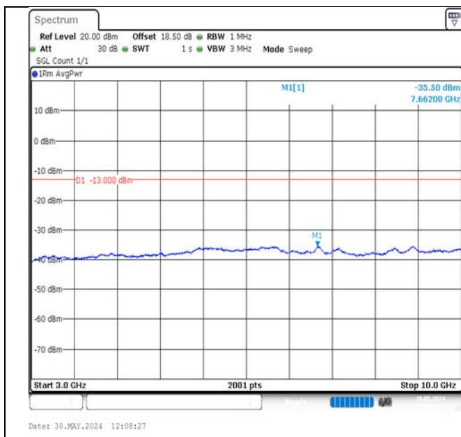
Band17-10MHz-16QAM-23780-50RB#0-3000~10000-PASS
