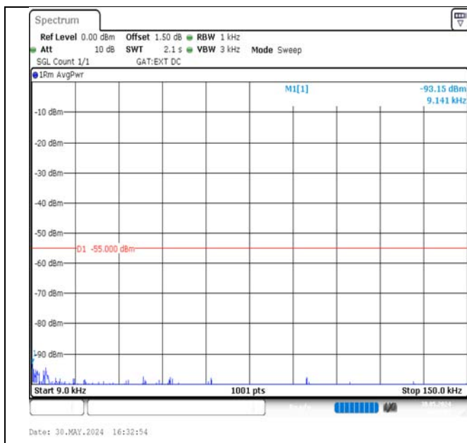
Band38-5MHz-16QAM-37775-25RB#0-0.009~0.15-PASS
