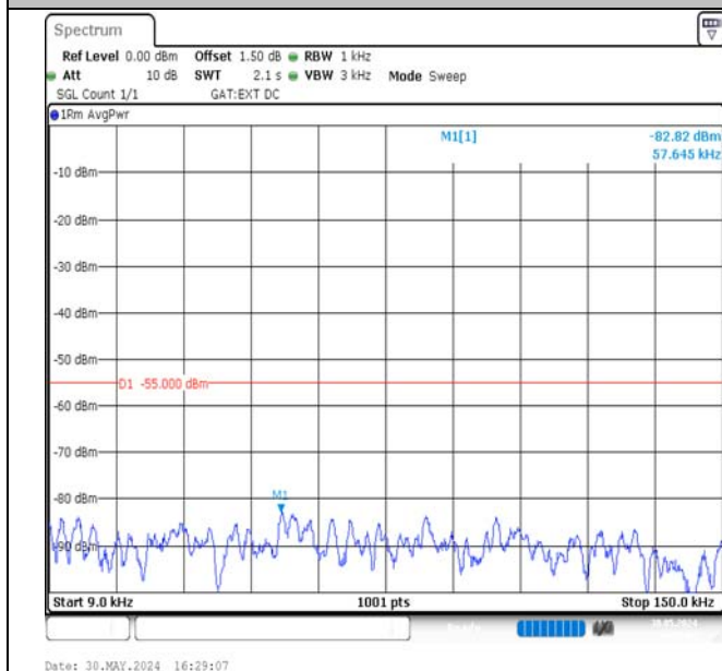
Band38-5MHz-16QAM-37775-1RB#24-0.009~0.15-PASS
