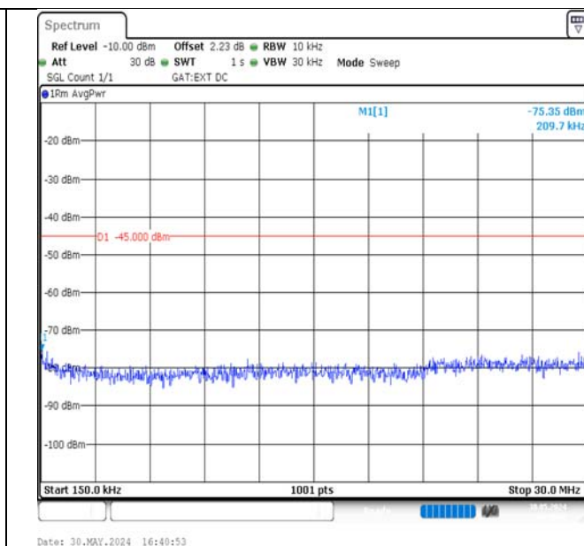
Band38-5MHz-16QAM-38000-1RB#24-0.15~30-PASS
