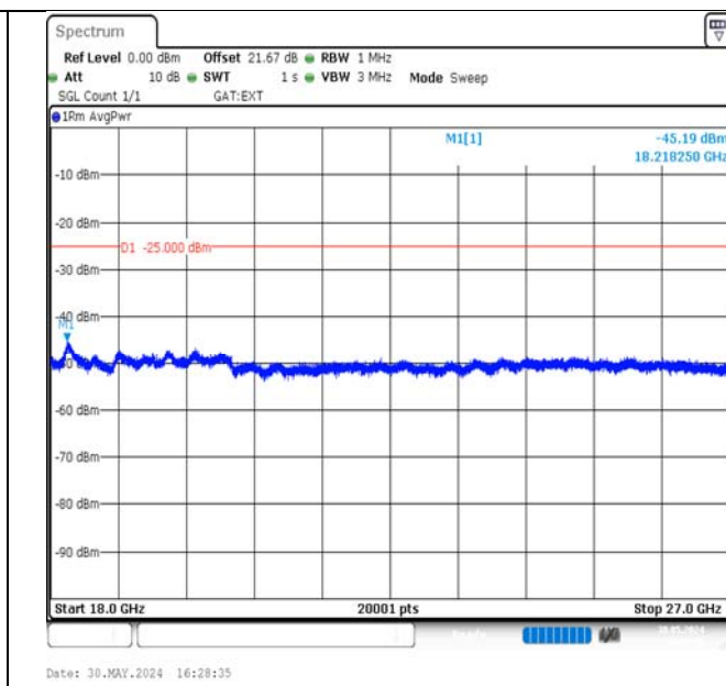
Band38-5MHz-QPSK-37775-1RB#24-18000~27000-PASS
