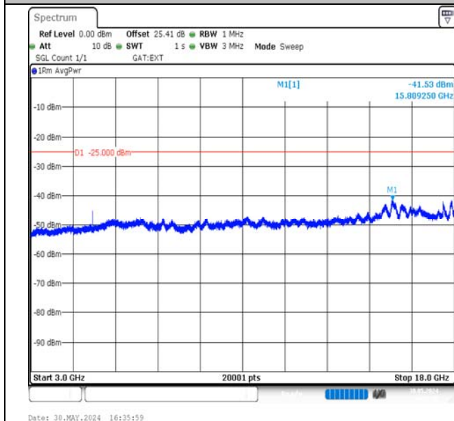
Band38-5MHz-QPSK-38000-1RB#0-3000~18000-PASS
