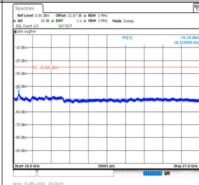
Band38-5MHz-16QAM-37775-1RB#0-18000~27000-PASS
