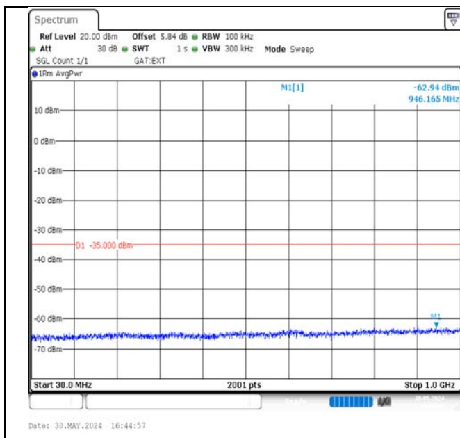
Band38-5MHz-16QAM-38000-25RB#0-30~1000-PASS
