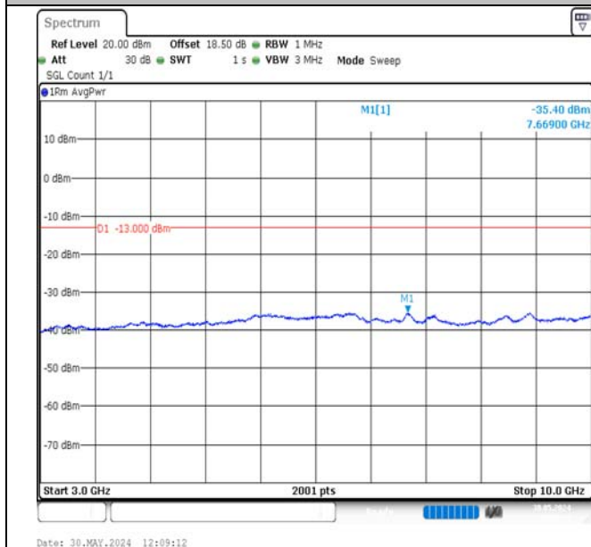
Band17-10MHz-16QAM-23790-1RB#0-3000~10000-PASS
