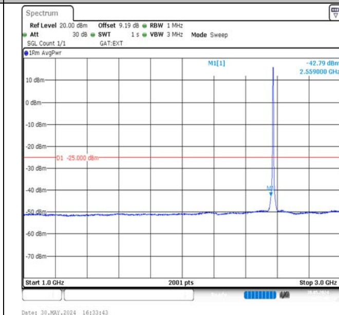
Band38-5MHz-16QAM-37775-25RB#0-1000~3000-PASS
