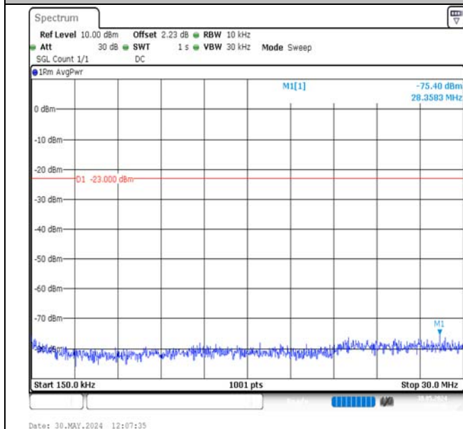
Band17-10MHz-16QAM-23780-1RB#49-0.15~30-PASS
