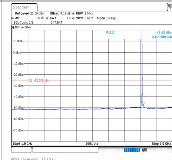
Band38-5MHz-QPSK-38225-1RB#0-1000~3000-PASS
