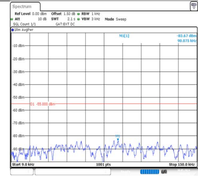
Band38-5MHz-QPSK-38225-1RB#24-0.009~0.15-PASS
