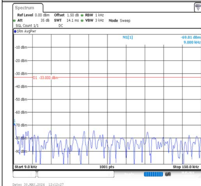
Band17-10MHz-16QAM-23800-50RB#0-0.009~0.15-PASS
