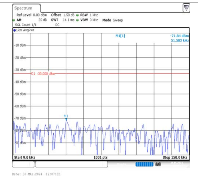
Band17-10MHz-16QAM-23780-1RB#49-0.009~0.15-PASS
