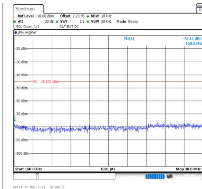
Band38-5MHz-QPSK-38225-1RB#0-0.15~30-PASS
