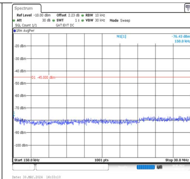
Band38-5MHz-16QAM-37775-25RB#0-0.15~30-PASS
