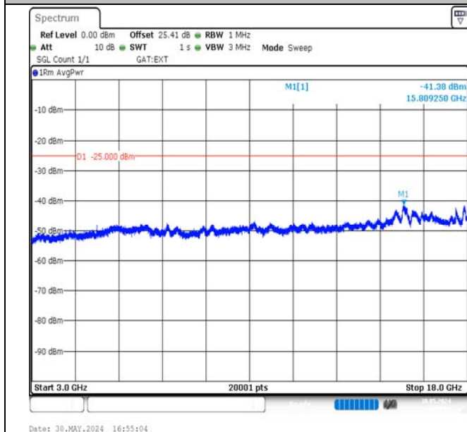
Band38-5MHz-QPSK-38225-25RB#0-3000~18000-PASS
