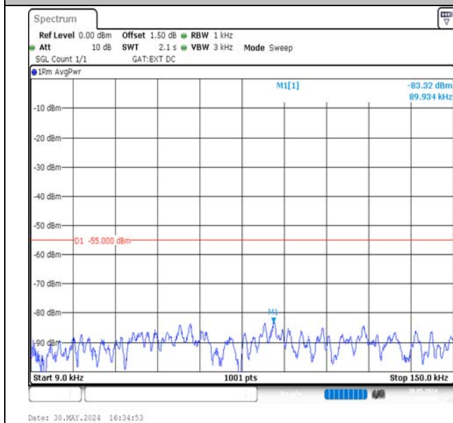
Band38-5MHz-QPSK-38000-1RB#0-0.009~0.15-PASS
