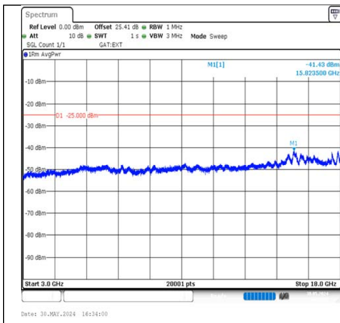
Band38-5MHz-16QAM-37775-25RB#0-3000~18000-PASS
