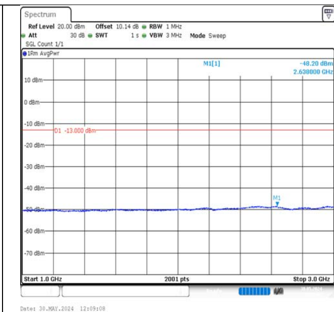
Band17-10MHz-16QAM-23790-1RB#0-1000~3000-PASS
