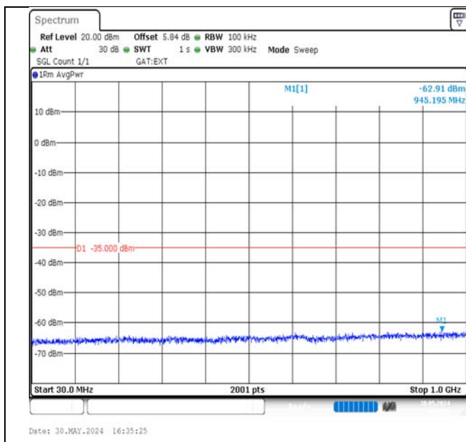
Band38-5MHz-QPSK-38000-1RB#0-30~1000-PASS
