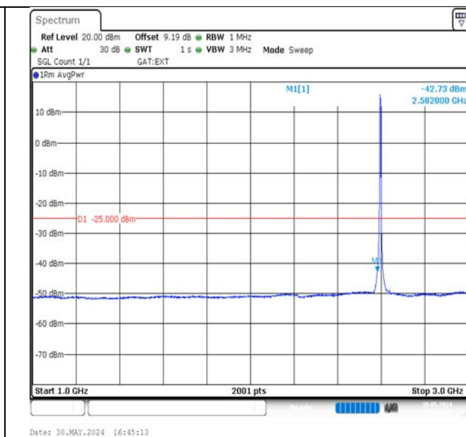
Band38-5MHz-16QAM-38000-25RB#0-1000~3000-PASS
