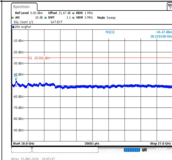
Band38-5MHz-16QAM-38000-25RB#0-18000~27000-PASS
