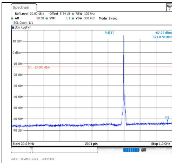
Band17-10MHz-16QAM-23790-1RB#0-30~1000-PASS
