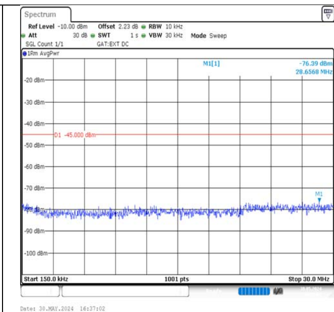
Band38-5MHz-16QAM-38000-1RB#0-0.15~30-PASS
