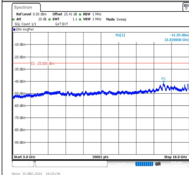
Band38-5MHz-QPSK-37775-25RB#0-3000~18000-PASS
