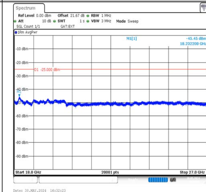
Band38-5MHz-QPSK-37775-25RB#0-18000~27000-PASS
