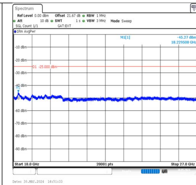
Band38-5MHz-QPSK-38225-1RB#24-18000~27000-PASS
