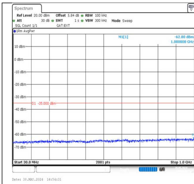
Band38-5MHz-QPSK-38225-25RB#0-30~1000-PASS
