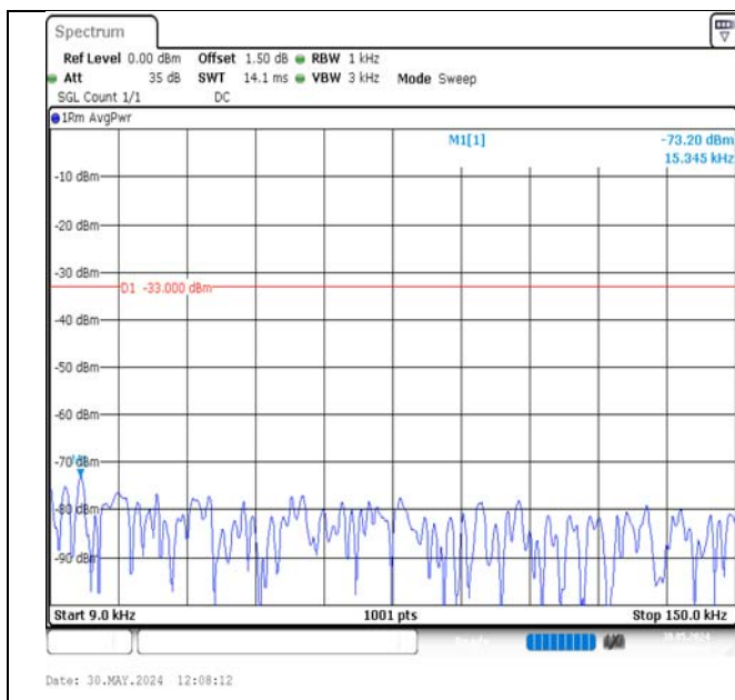
Band17-10MHz-16QAM-23780-50RB#0-0.009~0.15-PASS
