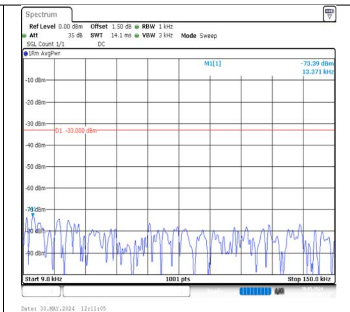
Band17-10MHz-16QAM-23800-1RB#0-0.009~0.15-PASS
