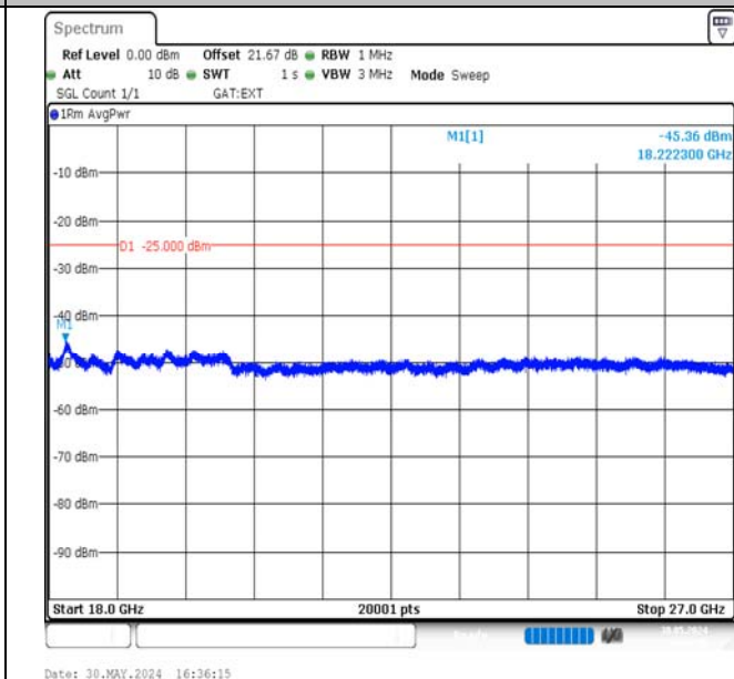
Band38-5MHz-QPSK-38000-1RB#0-18000~27000-PASS
