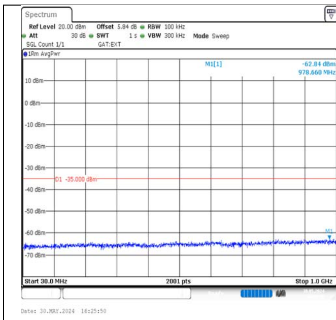
Band38-5MHz-16QAM-37775-1RB#0-30~1000-PASS
