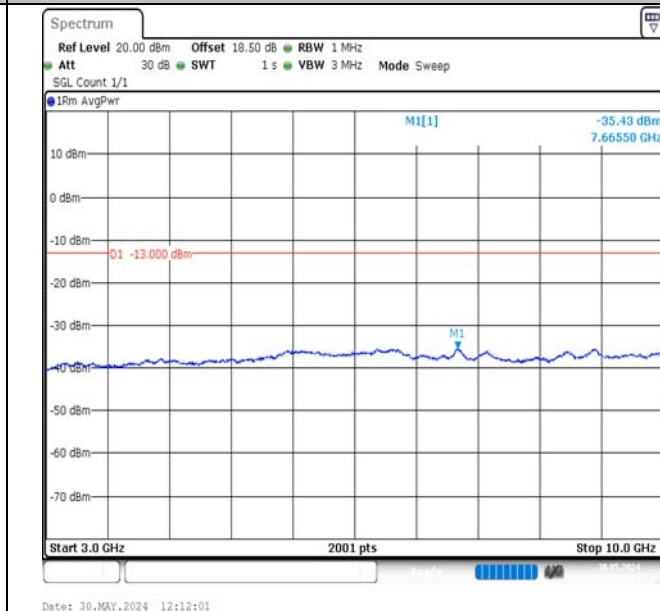
Band17-10MHz-16QAM-23800-1RB#49-3000~10000-PASS
