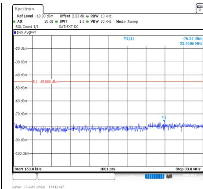
Band38-5MHz-QPSK-38000-25RB#0-0.15~30-PASS
