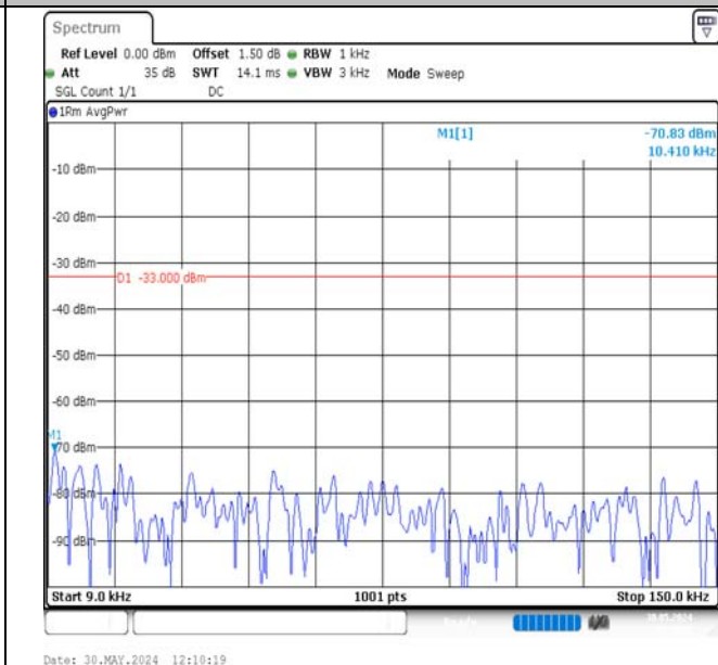
Band17-10MHz-16QAM-23790-50RB#0-0.009~0.15-PASS
