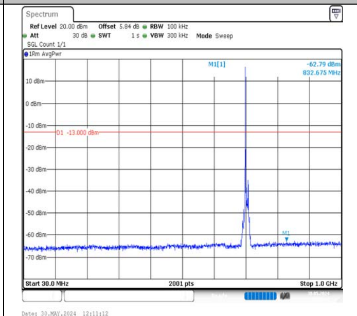
Band17-10MHz-16QAM-23800-1RB#0-30~1000-PASS
