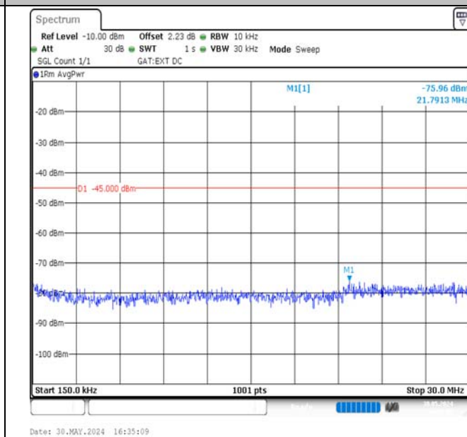
Band38-5MHz-QPSK-38000-1RB#0-0.15~30-PASS
