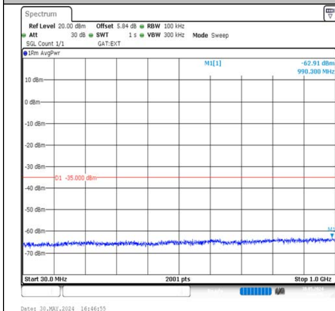
Band38-5MHz-QPSK-38225-1RB#0-30~1000-PASS
