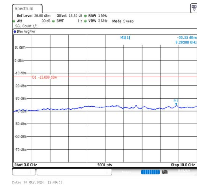
Band17-10MHz-16QAM-23790-1RB#49-3000~10000-PASS
