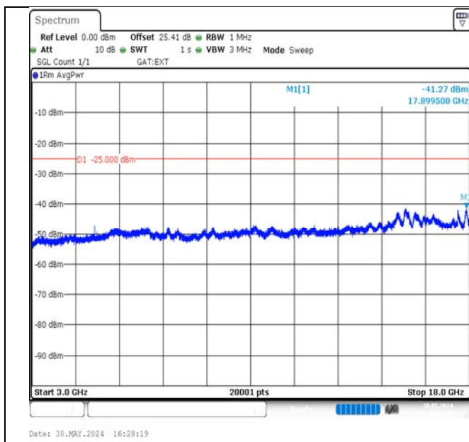
Band38-5MHz-QPSK-37775-1RB#24-3000~18000-PASS
