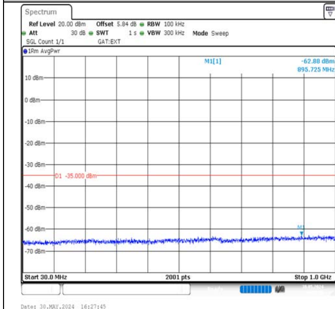
Band38-5MHz-QPSK-37775-1RB#24-30~1000-PASS
