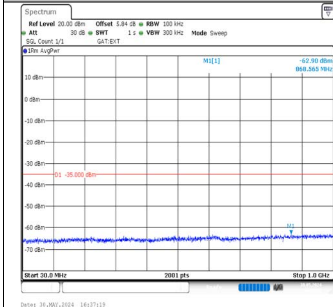
Band38-5MHz-16QAM-38000-1RB#0-30~1000-PASS
