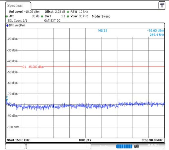
Band38-5MHz-QPSK-38225-1RB#24-0.15~30-PASS
