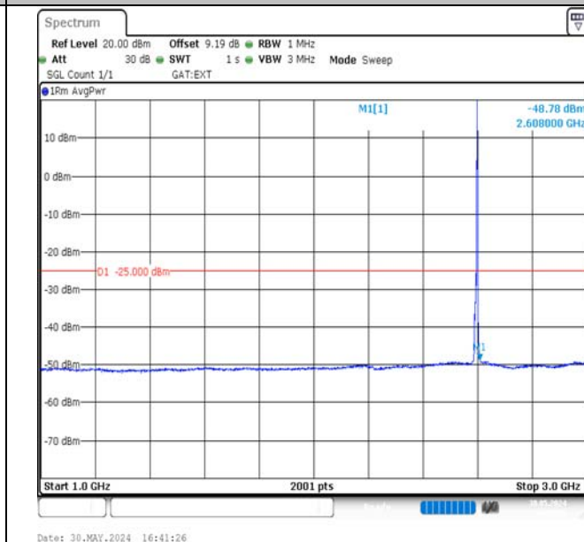
Band38-5MHz-16QAM-38000-1RB#24-1000~3000-PASS
