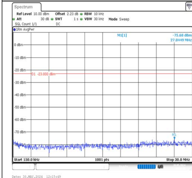
Band17-5MHz-QPSK-23790-1RB#24-0.15~30-PASS
