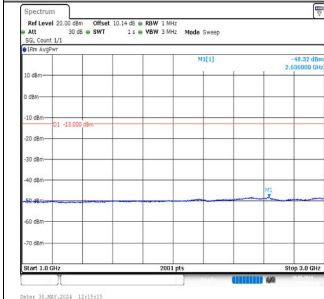
Band17-5MHz-QPSK-23790-1RB#0-1000~3000-PASS
