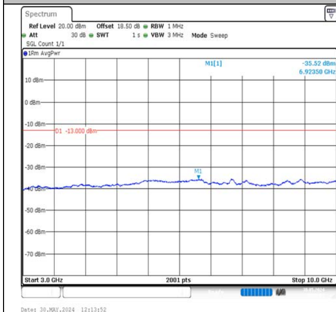
Band17-5MHz-QPSK-23755-1RB#24-3000~10000-PASS
