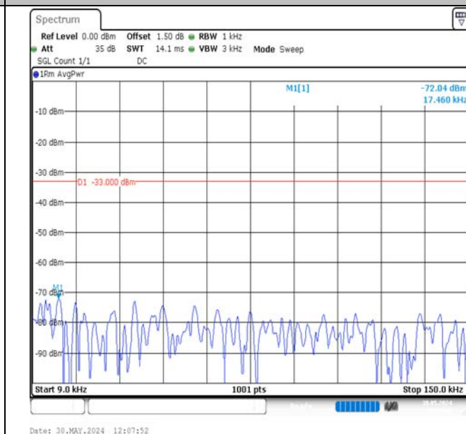
Band17-10MHz-QPSK-23780-50RB#0-0.009~0.15-PASS
