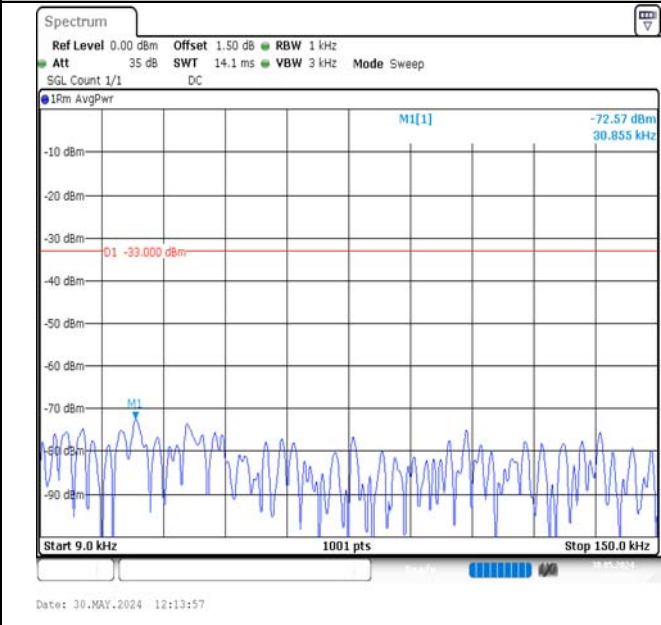
Band17-5MHz-16QAM-23755-1RB#24-0.009~0.15-PASS
