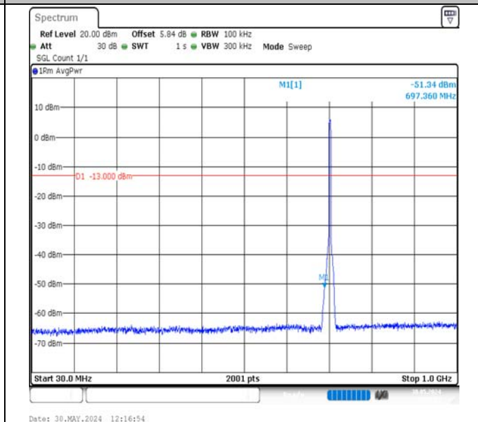
Band17-5MHz-16QAM-23790-25RB#0-30~1000-PASS
