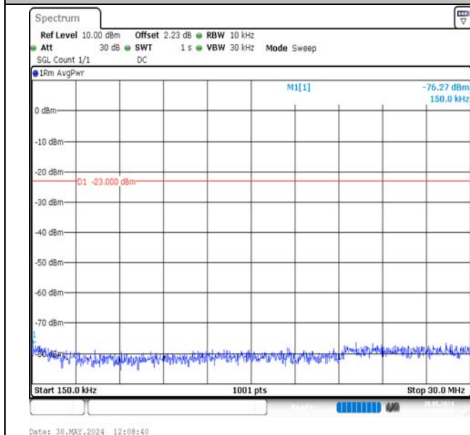
Band17-10MHz-QPSK-23790-1RB#0-0.15~30-PASS
