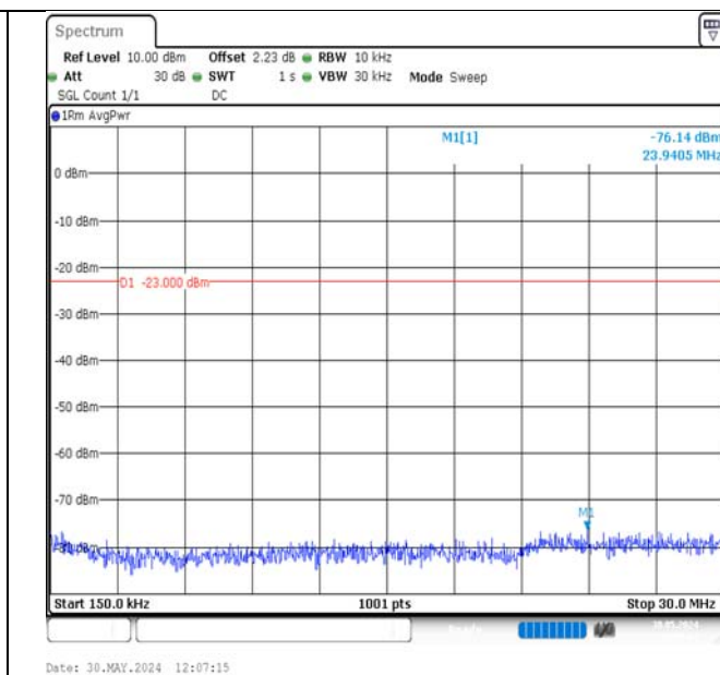
Band17-10MHz-QPSK-23780-1RB#49-0.15~30-PASS
