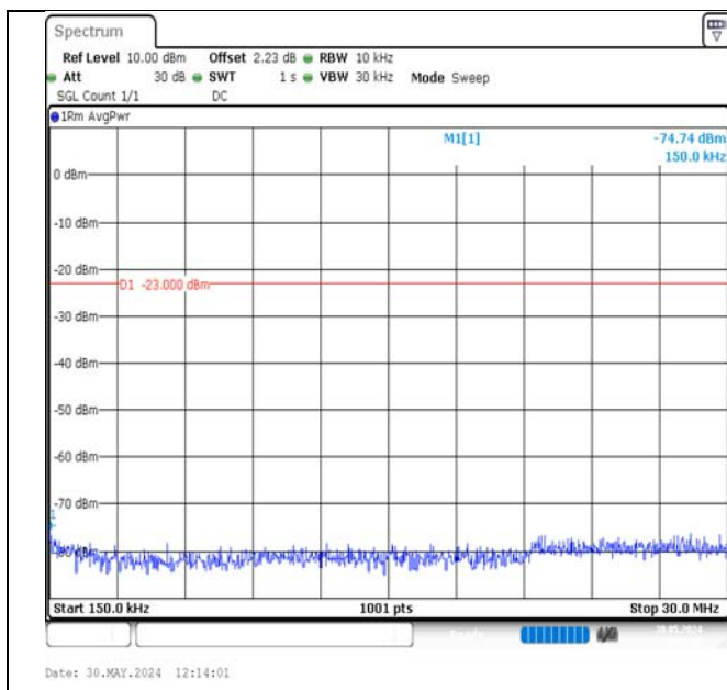
Band17-5MHz-16QAM-23755-1RB#24-0.15~30-PASS
