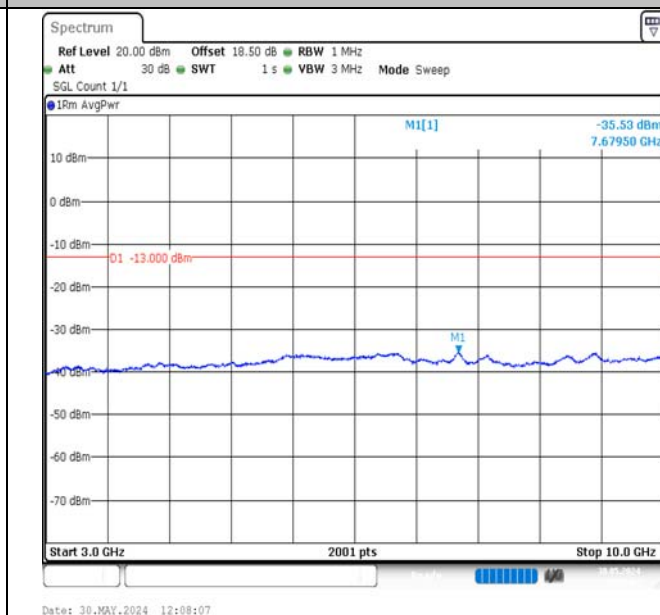
Band17-10MHz-QPSK-23780-50RB#0-3000~10000-PASS
