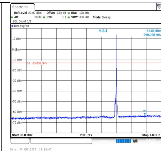
Band17-5MHz-16QAM-23755-1RB#24-30~1000-PASS
