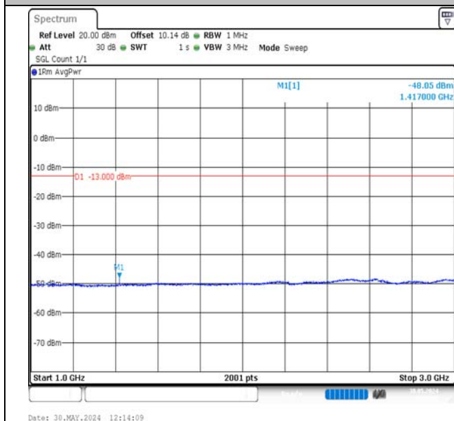
Band17-5MHz-16QAM-23755-1RB#24-1000~3000-PASS
