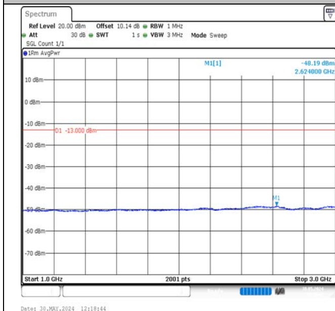
Band17-5MHz-QPSK-23825-25RB#0-1000~3000-PASS
