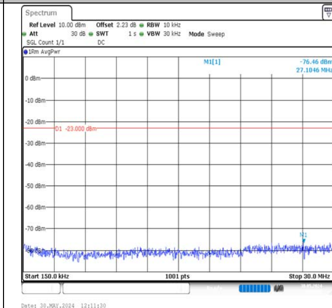
Band17-10MHz-QPSK-23800-1RB#49-0.15~30-PASS
