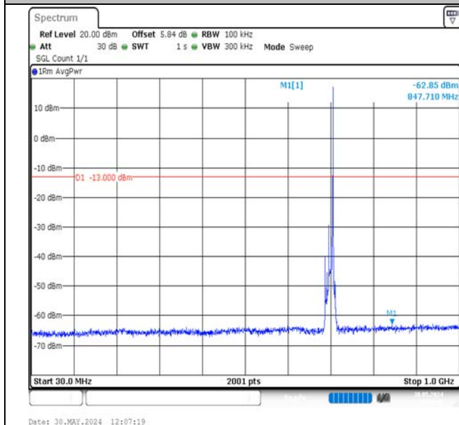
Band17-10MHz-QPSK-23780-1RB#49-30~1000-PASS
