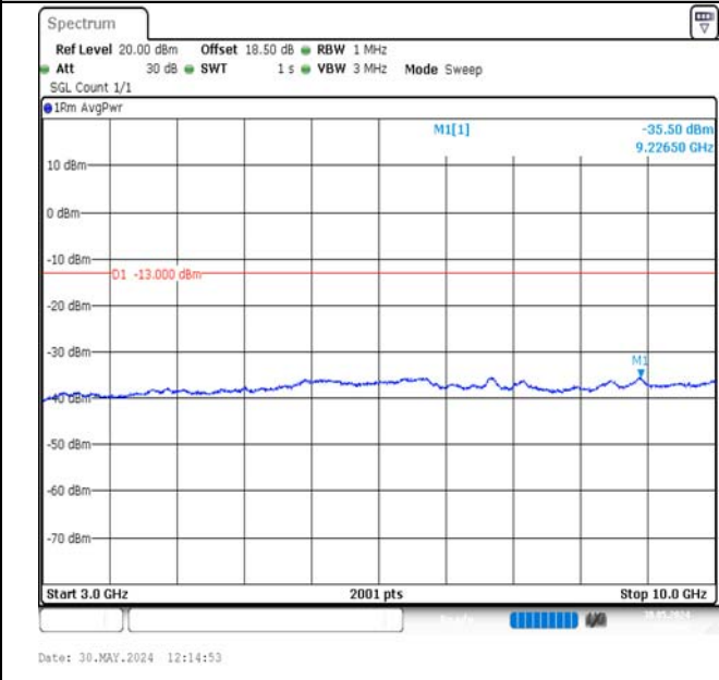
Band17-5MHz-16QAM-23755-25RB#0-3000~10000-PASS
