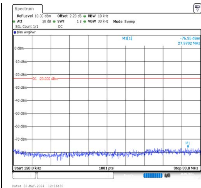
Band17-5MHz-QPSK-23790-25RB#0-0.15~30-PASS
