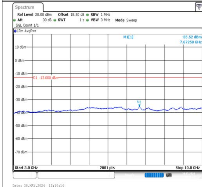
Band17-10MHz-QPSK-23790-50RB#0-3000~10000-PASS
