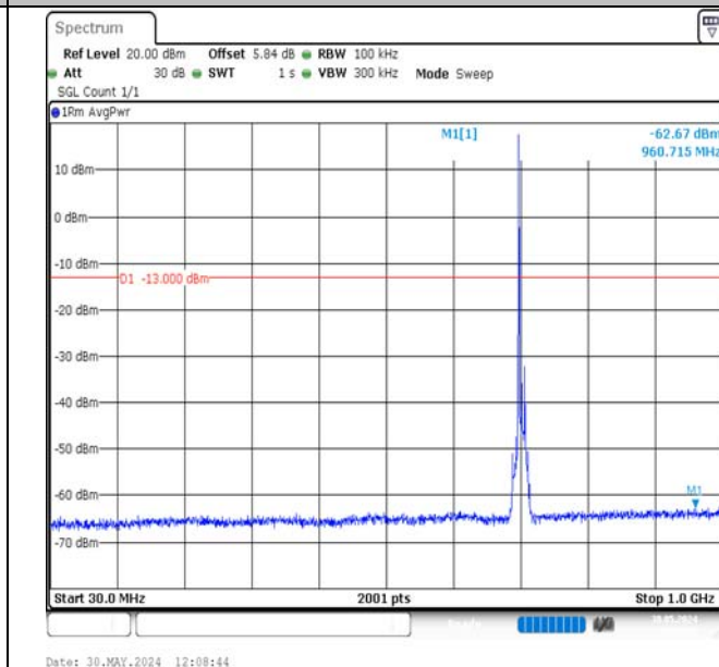
Band17-10MHz-QPSK-23790-1RB#0-30~1000-PASS
