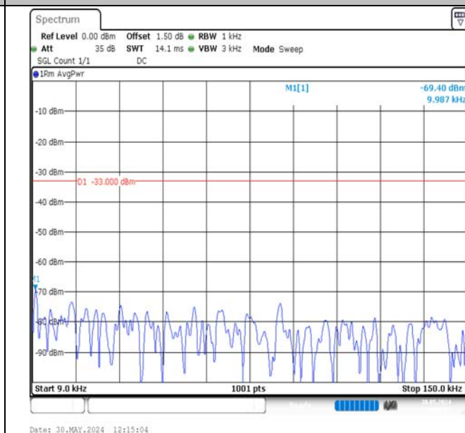
Band17-5MHz-QPSK-23790-1RB#0-0.009~0.15-PASS
