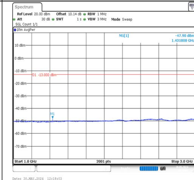
Band17-5MHz-QPSK-23825-1RB#24-1000~3000-PASS
