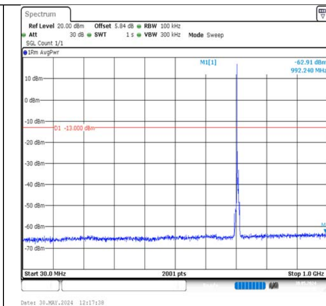
Band17-5MHz-16QAM-23825-1RB#0-30~1000-PASS
