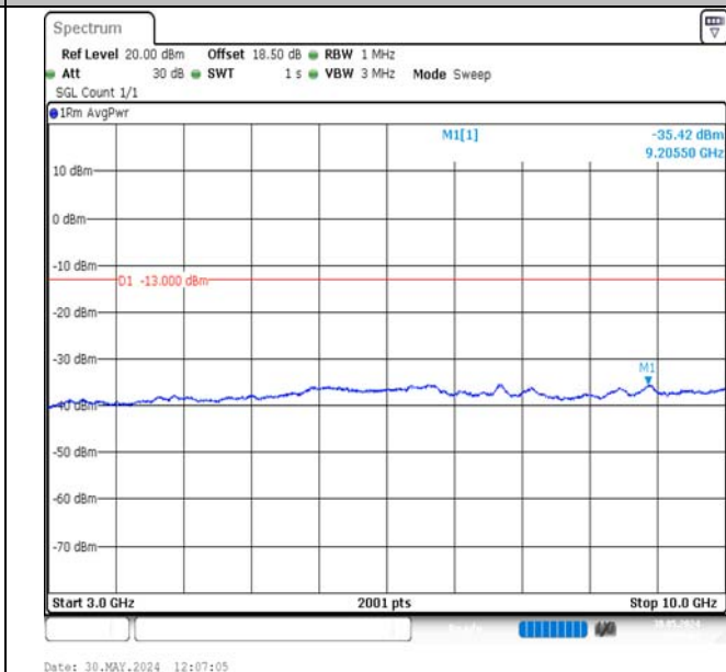
Band17-10MHz-16QAM-23780-1RB#0-3000~10000-PASS
