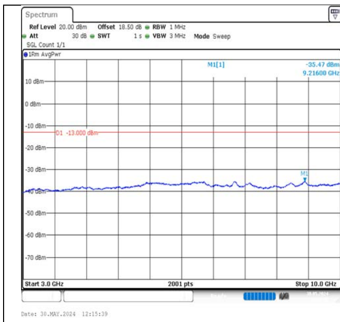
Band17-5MHz-16QAM-23790-1RB#0-3000~10000-PASS
