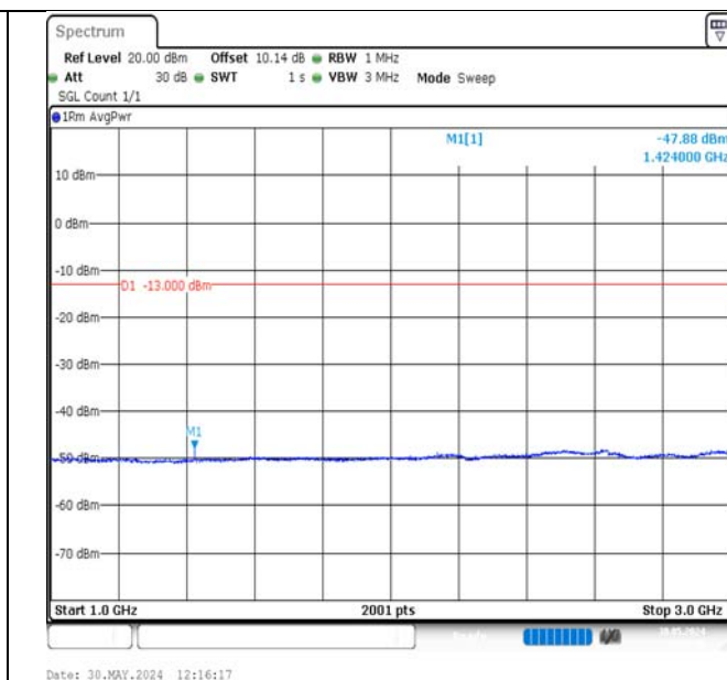
Band17-5MHz-16QAM-23790-1RB#24-1000~3000-PASS
