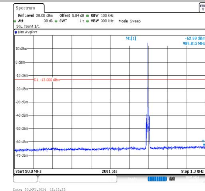
Band17-5MHz-16QAM-23755-1RB#0-30~1000-PASS
