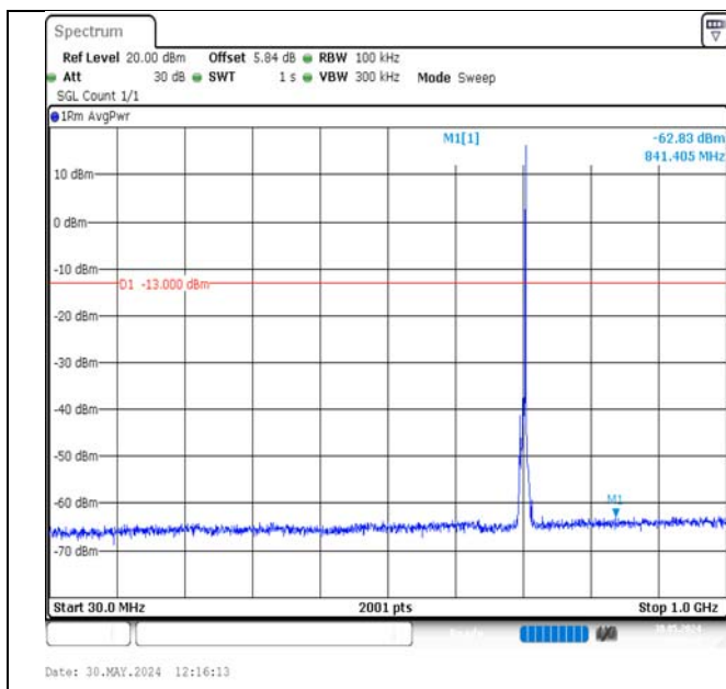
Band17-5MHz-16QAM-23790-1RB#24-30~1000-PASS
