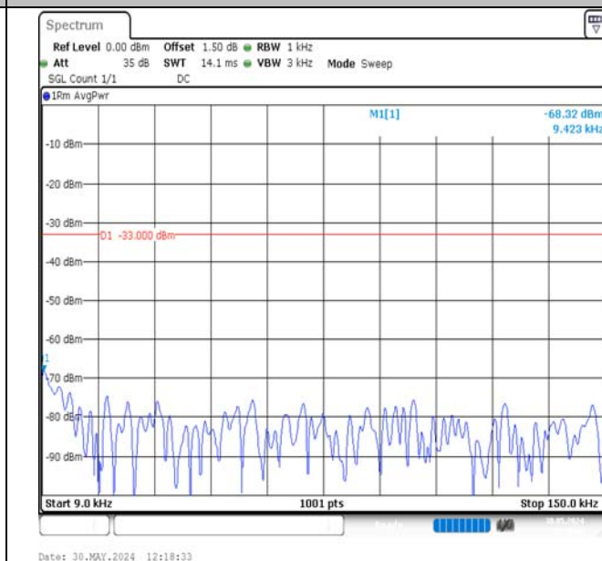
Band17-5MHz-QPSK-23825-25RB#0-0.009~0.15-PASS
