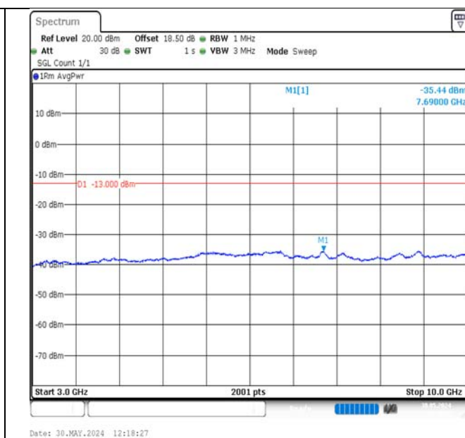
Band17-5MHz-16QAM-23825-1RB#24-3000~10000-PASS
