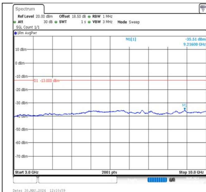
Band17-10MHz-QPSK-23800-1RB#0-3000~10000-PASS
