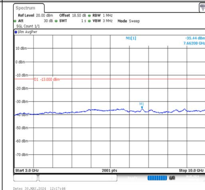
Band17-5MHz-16QAM-23825-1RB#0-3000~10000-PASS
