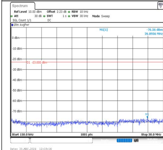
Band17-5MHz-16QAM-23825-1RB#24-0.15~30-PASS
