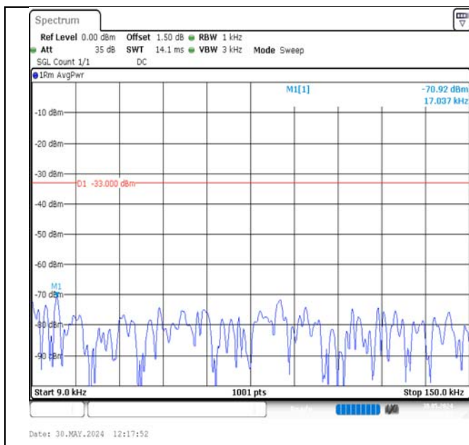
Band17-5MHz-QPSK-23825-1RB#24-0.009~0.15-PASS
