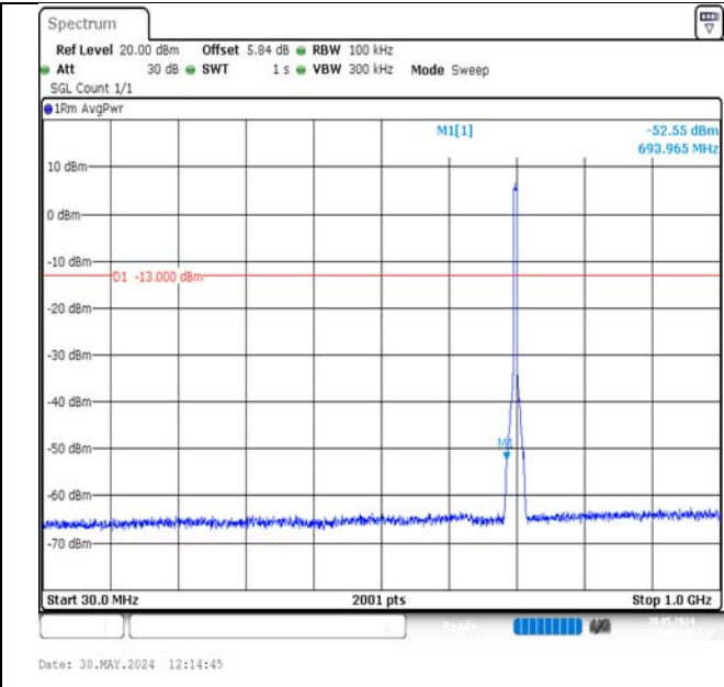
Band17-5MHz-16QAM-23755-25RB#0-30~1000-PASS
