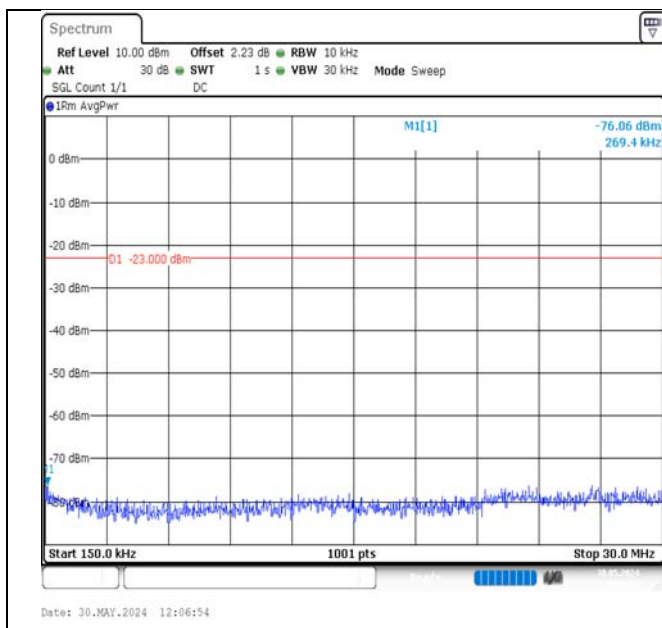
Band17-10MHz-16QAM-23780-1RB#0-0.15~30-PASS
