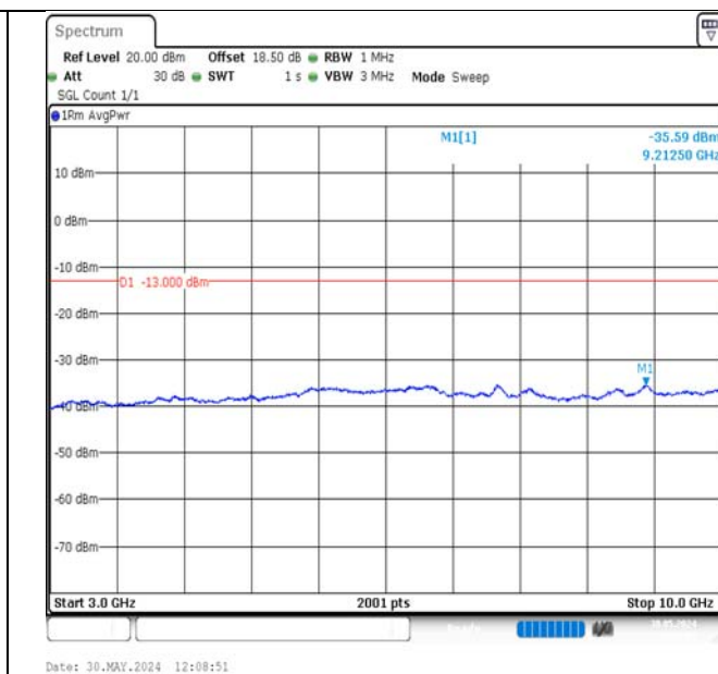
Band17-10MHz-QPSK-23790-1RB#0-3000~10000-PASS
