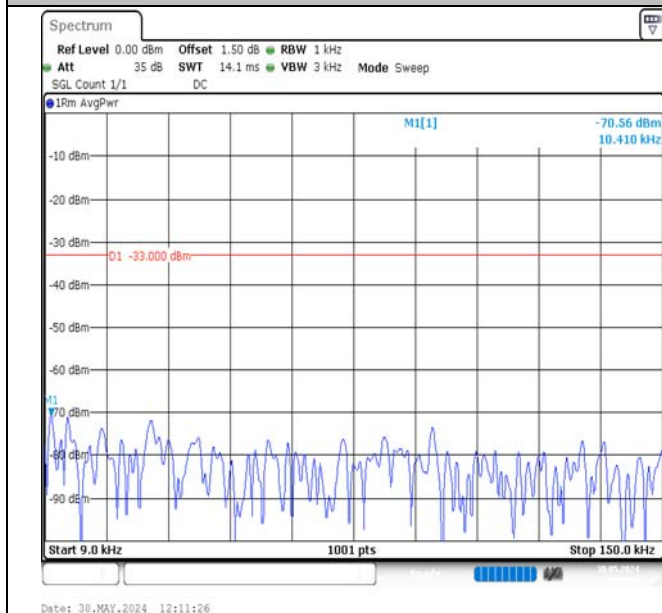
Band17-10MHz-QPSK-23800-1RB#49-0.009~0.15-PASS
