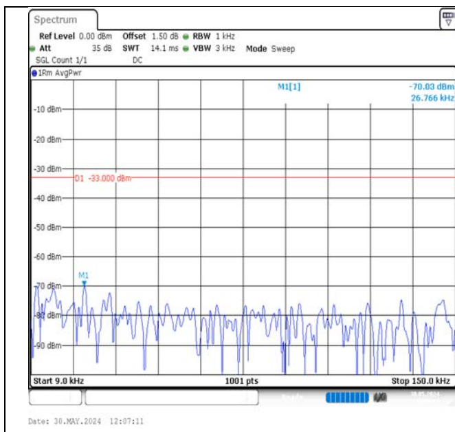
Band17-10MHz-QPSK-23780-1RB#49-0.009~0.15-PASS
