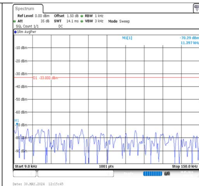
Band17-5MHz-QPSK-23790-1RB#24-0.009~0.15-PASS
