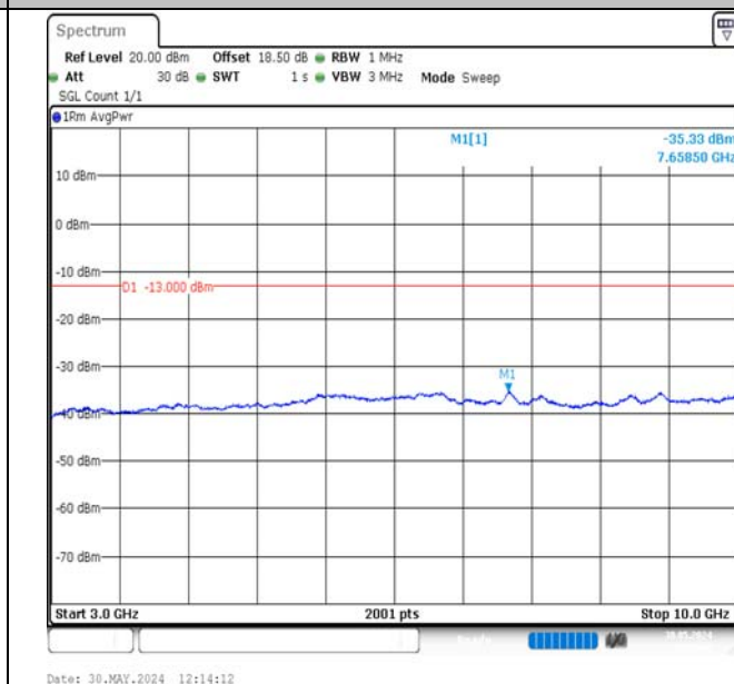
Band17-5MHz-16QAM-23755-1RB#24-3000~10000-PASS
