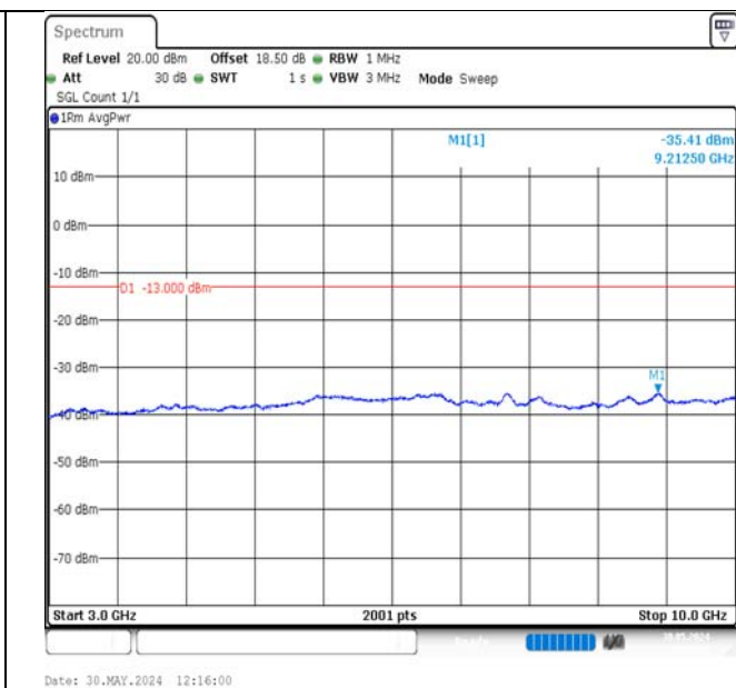
Band17-5MHz-QPSK-23790-1RB#24-3000~10000-PASS
