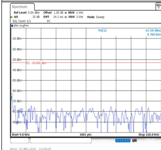
Band17-10MHz-QPSK-23780-1RB#0-0.009~0.15-PASS
