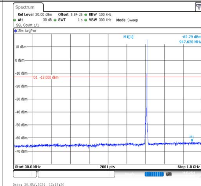
Band17-5MHz-16QAM-23825-1RB#24-30~1000-PASS
