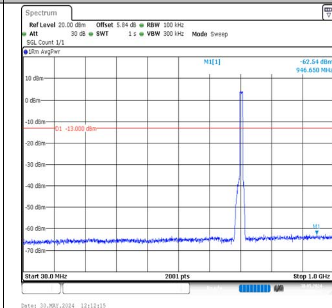
Band17-10MHz-QPSK-23800-50RB#0-30~1000-PASS
