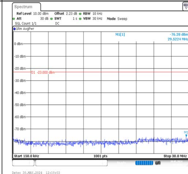
Band17-10MHz-QPSK-23790-50RB#0-0.15~30-PASS
