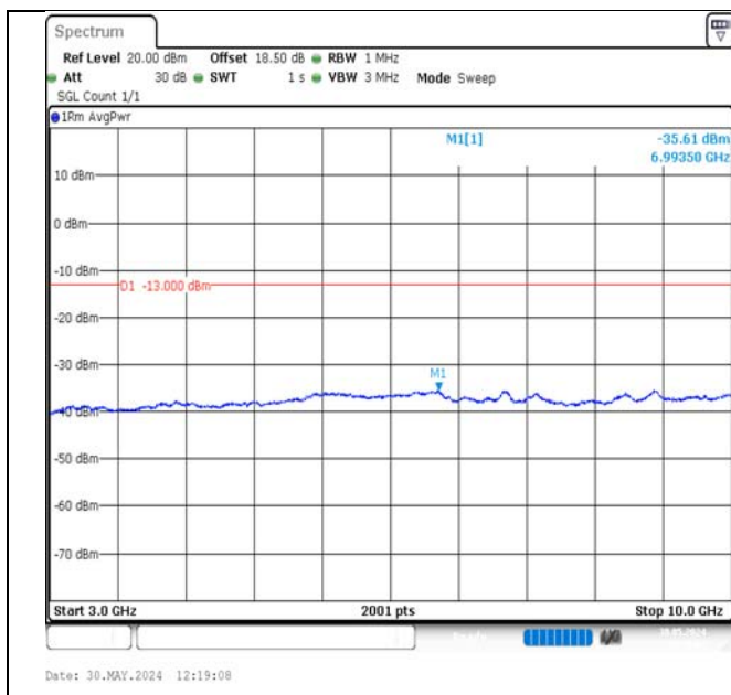
Band17-5MHz-16QAM-23825-25RB#0-3000~10000-PASS
