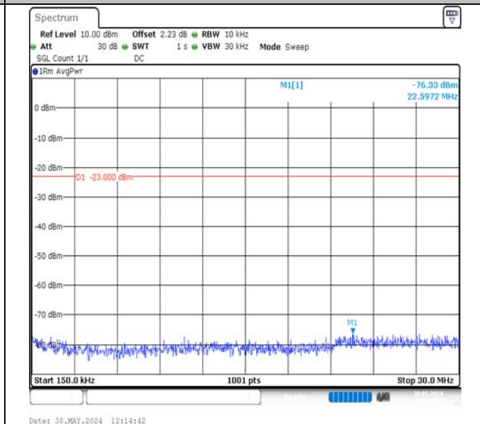
Band17-5MHz-16QAM-23755-25RB#0-0.15~30-PASS
