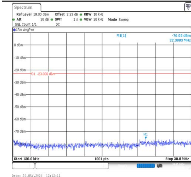
Band17-10MHz-QPSK-23800-50RB#0-0.15~30-PASS
