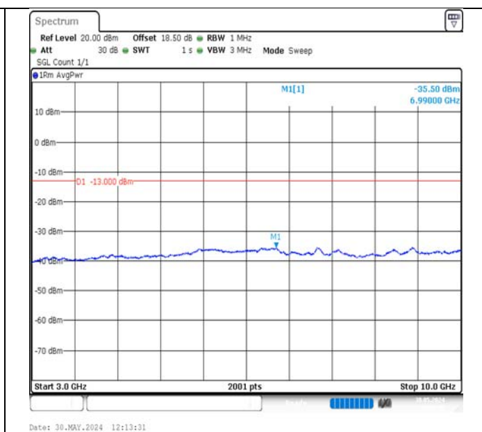
Band17-5MHz-16QAM-23755-1RB#0-3000~10000-PASS
