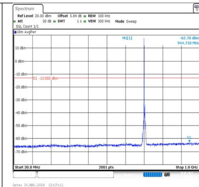
Band17-5MHz-QPSK-23790-1RB#0-30~1000-PASS
