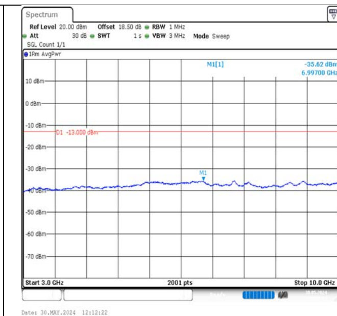
Band17-10MHz-QPSK-23800-50RB#0-3000~10000-PASS
