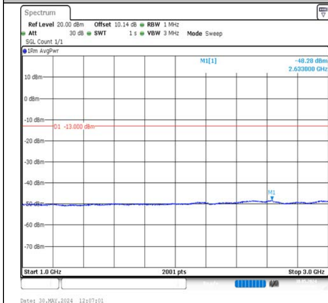
Band17-10MHz-16QAM-23780-1RB#0-1000~3000-PASS
