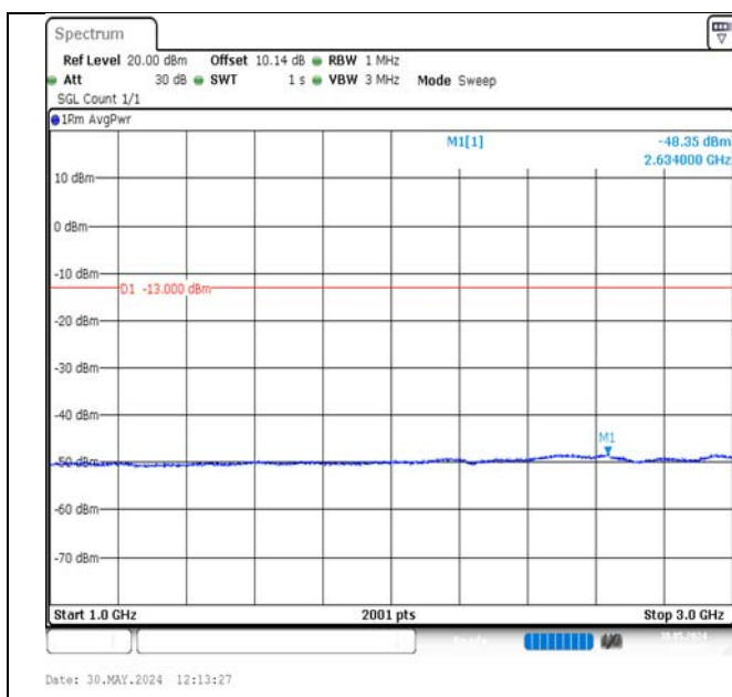
Band17-5MHz-16QAM-23755-1RB#0-1000~3000-PASS
