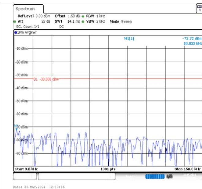
Band17-5MHz-16QAM-23755-1RB#0-0.009~0.15-PASS
