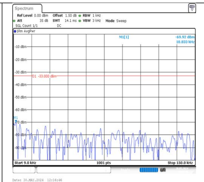
Band17-5MHz-16QAM-23790-25RB#0-0.009~0.15-PASS
