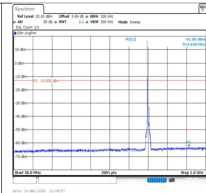
Band17-10MHz-16QAM-23780-1RB#0-30~1000-PASS
