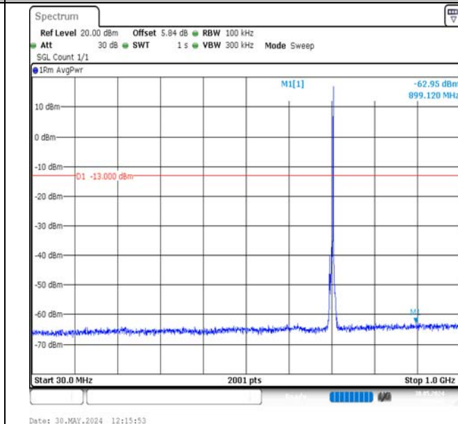
Band17-5MHz-QPSK-23790-1RB#24-30~1000-PASS
