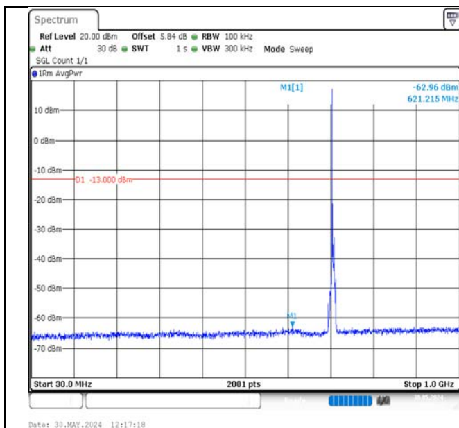
Band17-5MHz-QPSK-23825-1RB#0-30~1000-PASS
