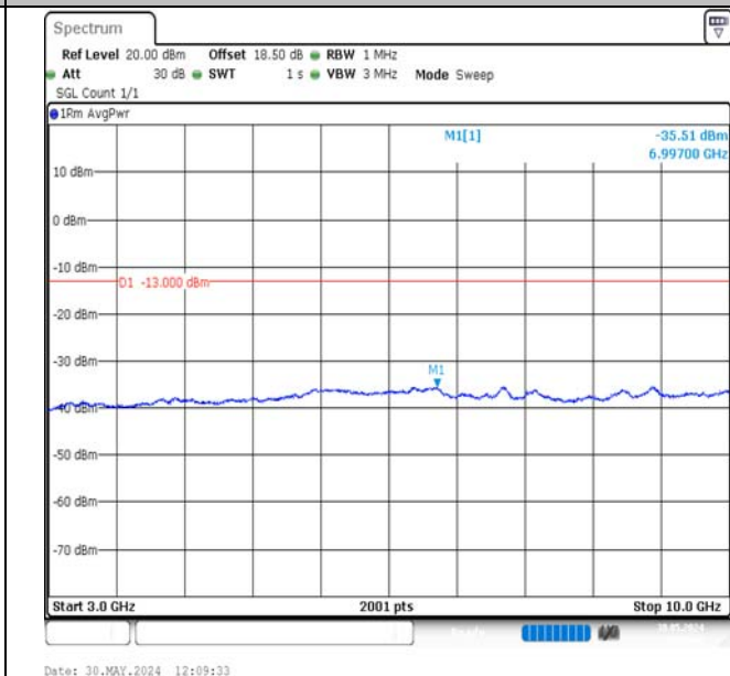
Band17-10MHz-QPSK-23790-1RB#49-3000~10000-PASS
