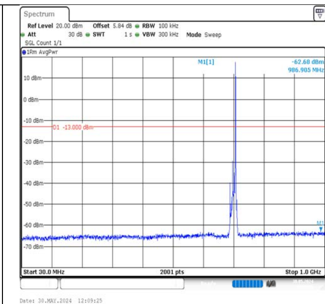
Band17-10MHz-QPSK-23790-1RB#49-30~1000-PASS
