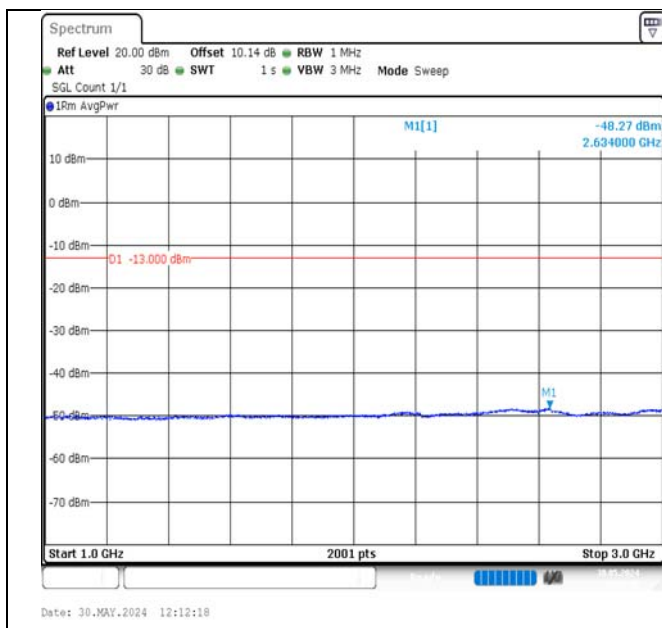
Band17-10MHz-QPSK-23800-50RB#0-1000~3000-PASS
