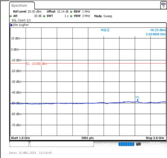
Band17-5MHz-16QAM-23755-25RB#0-1000~3000-PASS
