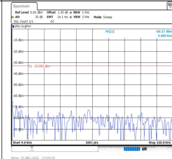
Band17-10MHz-QPSK-23790-1RB#49-0.009~0.15-PASS
