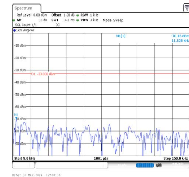
Band17-10MHz-QPSK-23790-1RB#0-0.009~0.15-PASS
