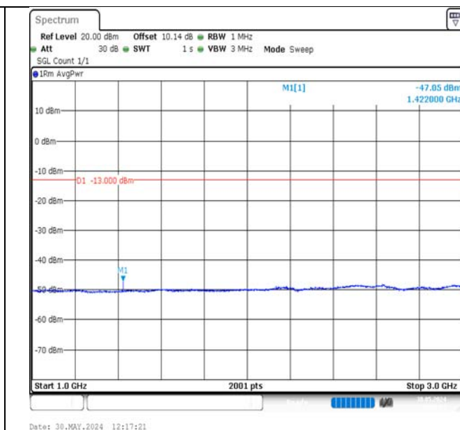
Band17-5MHz-QPSK-23825-1RB#0-1000~3000-PASS
