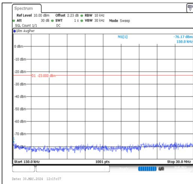
Band17-5MHz-QPSK-23790-1RB#0-0.15~30-PASS
