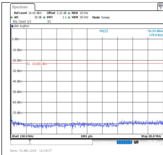
Band17-5MHz-QPSK-23825-25RB#0-0.15~30-PASS
