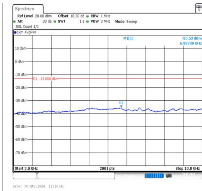
Band17-5MHz-QPSK-23790-25RB#0-3000~10000-PASS
