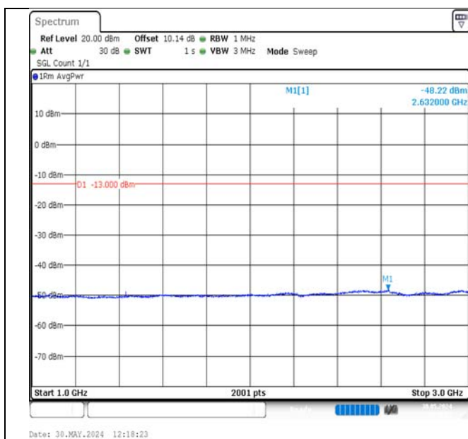
Band17-5MHz-16QAM-23825-1RB#24-1000~3000-PASS
