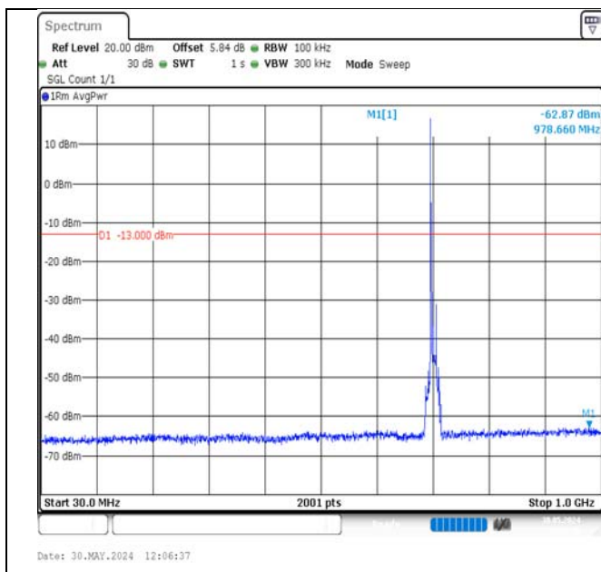
Band17-10MHz-QPSK-23780-1RB#0-30~1000-PASS
