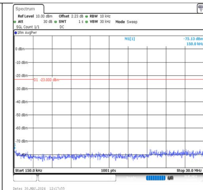
Band17-5MHz-QPSK-23825-1RB#24-0.15~30-PASS
