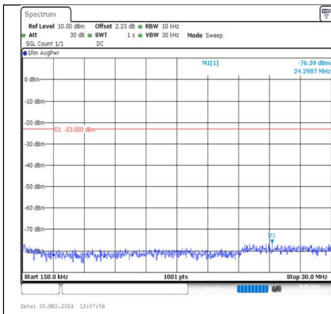
Band17-10MHz-QPSK-23780-50RB#0-0.15~30-PASS
