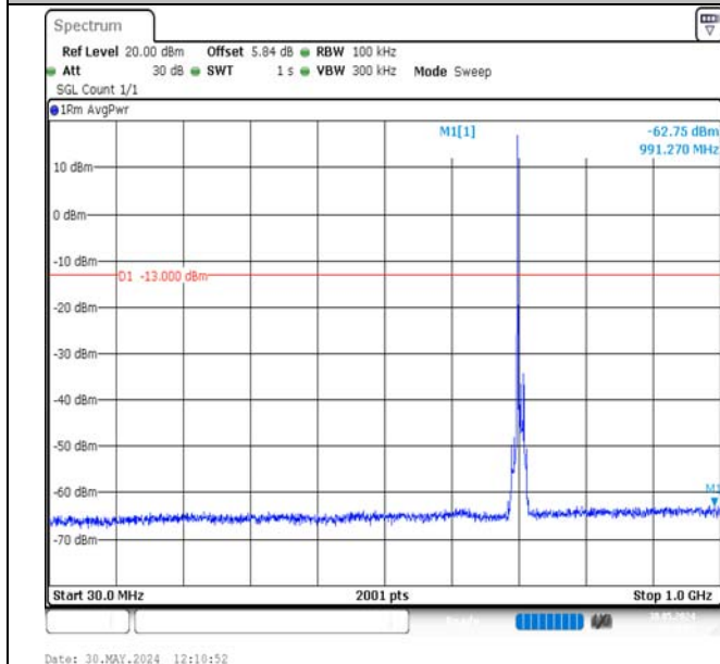
Band17-10MHz-QPSK-23800-1RB#0-30~1000-PASS
