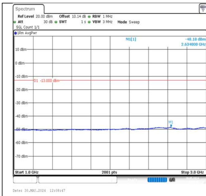
Band17-10MHz-QPSK-23790-1RB#0-1000~3000-PASS
