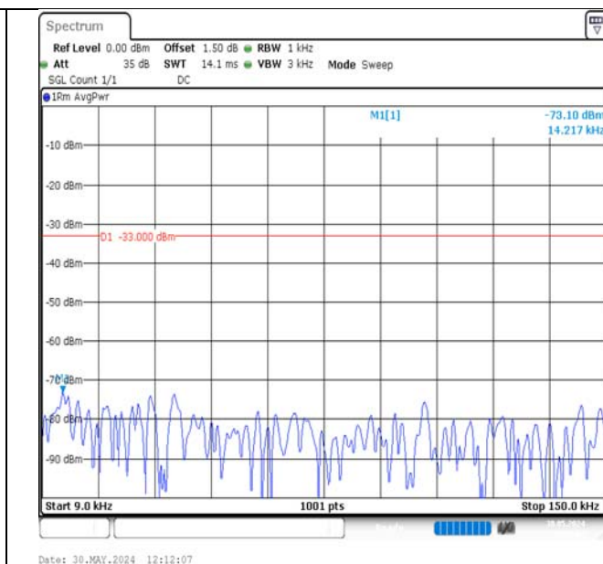
Band17-10MHz-QPSK-23800-50RB#0-0.009~0.15-PASS
