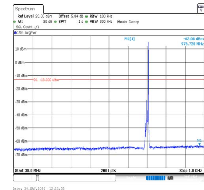
Band17-10MHz-QPSK-23800-1RB#49-30~1000-PASS
