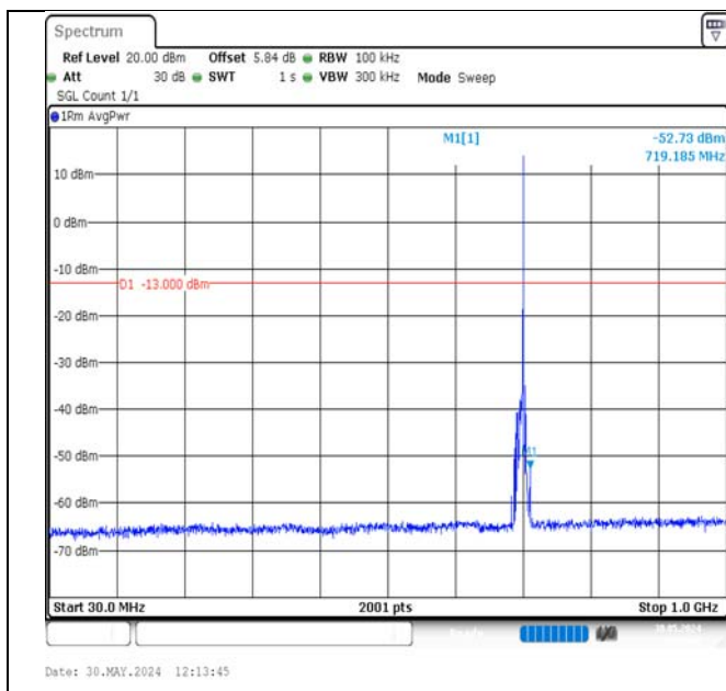
Band17-5MHz-QPSK-23755-1RB#24-30~1000-PASS
