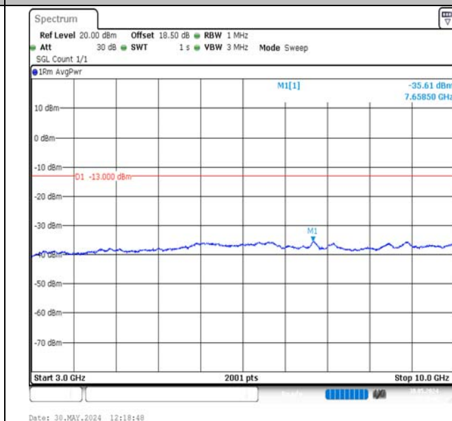
Band17-5MHz-QPSK-23825-25RB#0-3000~10000-PASS
