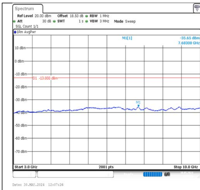
Band17-10MHz-QPSK-23780-1RB#49-3000~10000-PASS
