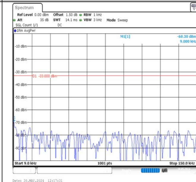
Band17-5MHz-16QAM-23825-1RB#0-0.009~0.15-PASS
