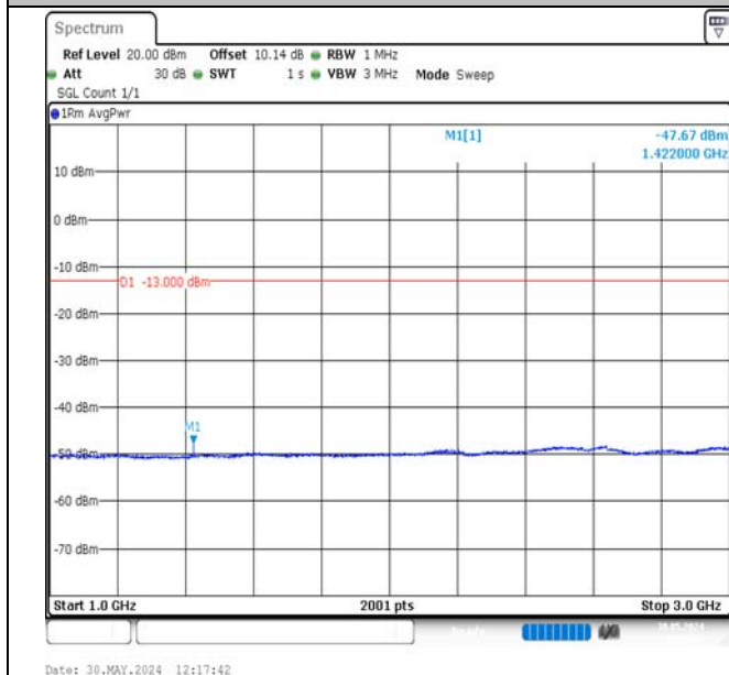
Band17-5MHz-16QAM-23825-1RB#0-1000~3000-PASS
