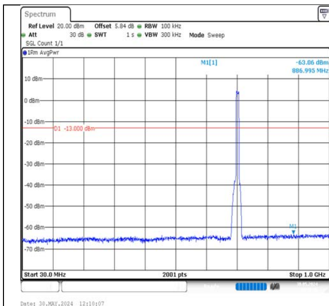
Band17-10MHz-QPSK-23790-50RB#0-30~1000-PASS
