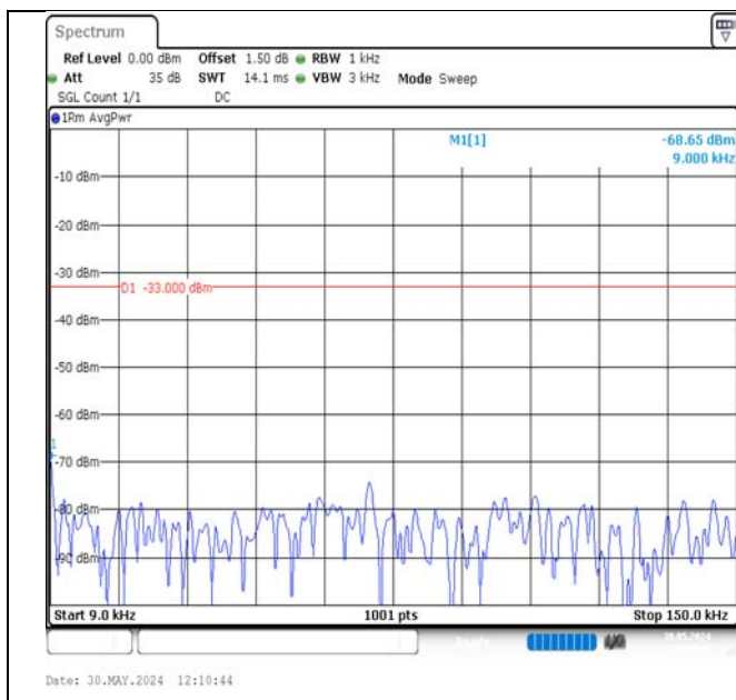
Band17-10MHz-QPSK-23800-1RB#0-0.009~0.15-PASS
