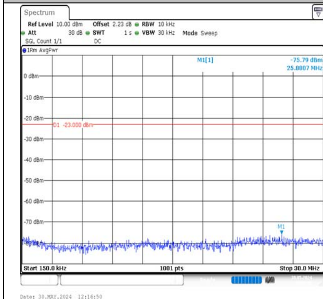
Band17-5MHz-16QAM-23790-25RB#0-0.15~30-PASS
