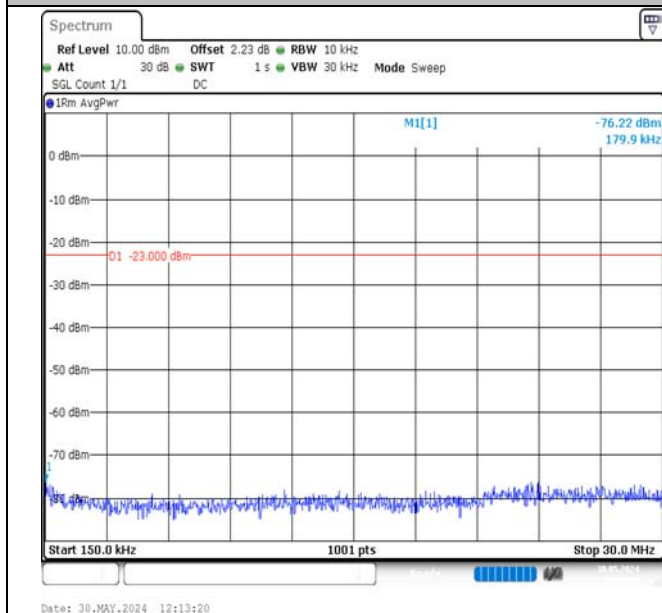
Band17-5MHz-16QAM-23755-1RB#0-0.15~30-PASS
