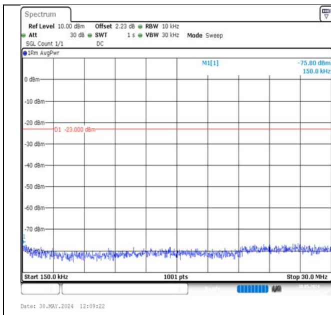
Band17-10MHz-QPSK-23790-1RB#49-0.15~30-PASS
