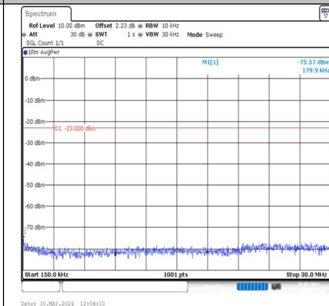
Band17-10MHz-QPSK-23780-1RB#0-0.15~30-PASS
