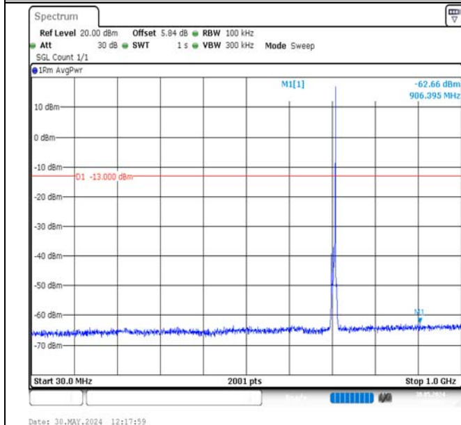
Band17-5MHz-QPSK-23825-1RB#24-30~1000-PASS
