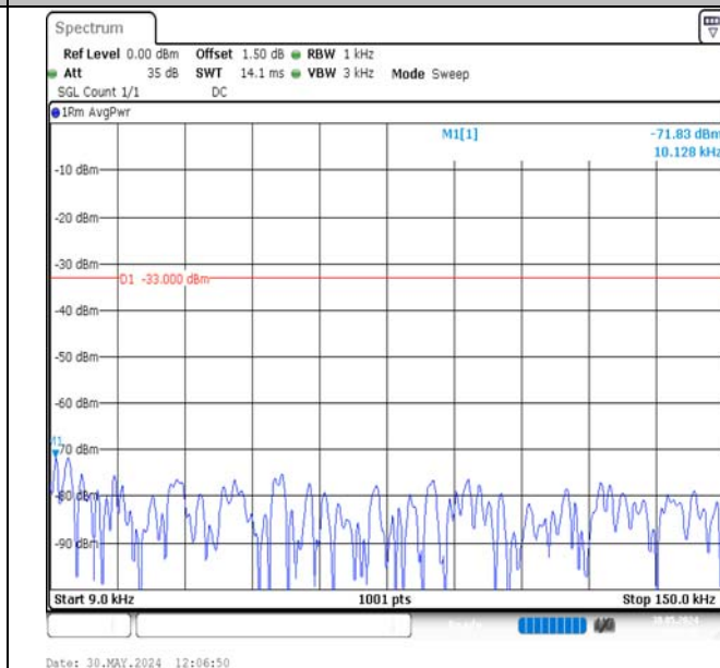
Band17-10MHz-16QAM-23780-1RB#0-0.009~0.15-PASS
