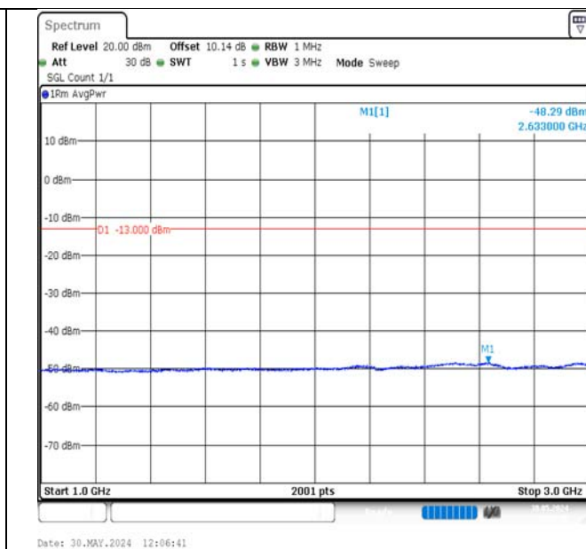
Band17-10MHz-QPSK-23780-1RB#0-1000~3000-PASS
