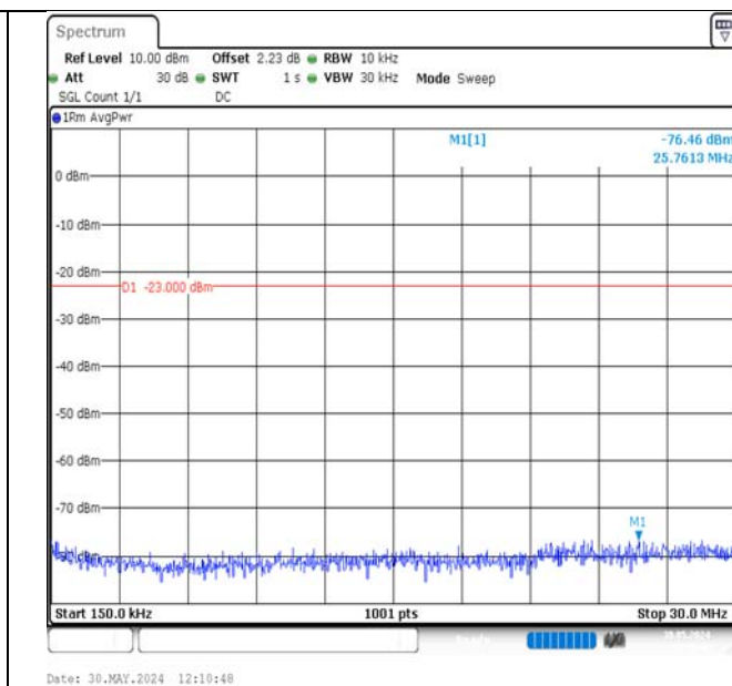
Band17-10MHz-QPSK-23800-1RB#0-0.15~30-PASS
