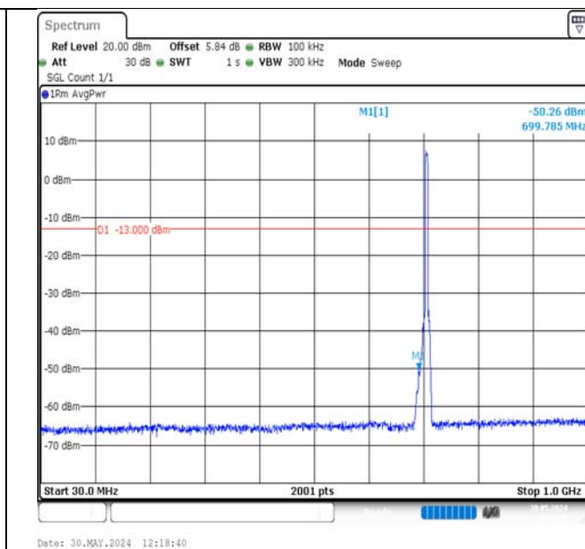
Band17-5MHz-QPSK-23825-25RB#0-30~1000-PASS
