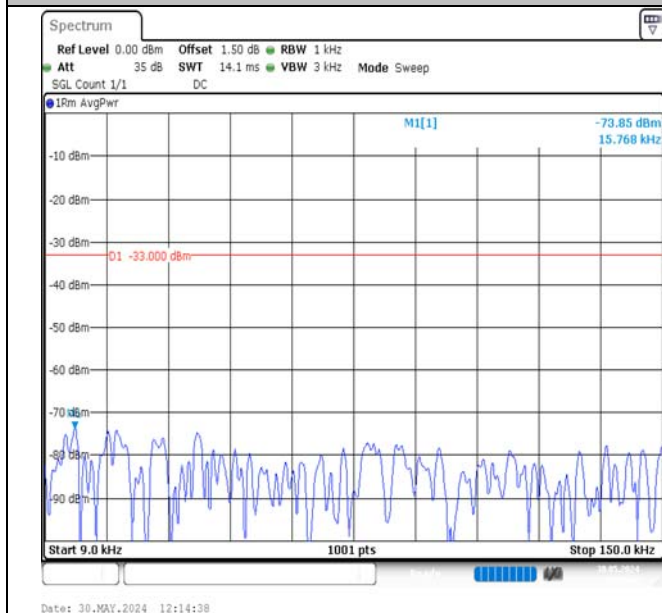
Band17-5MHz-16QAM-23755-25RB#0-0.009~0.15-PASS
