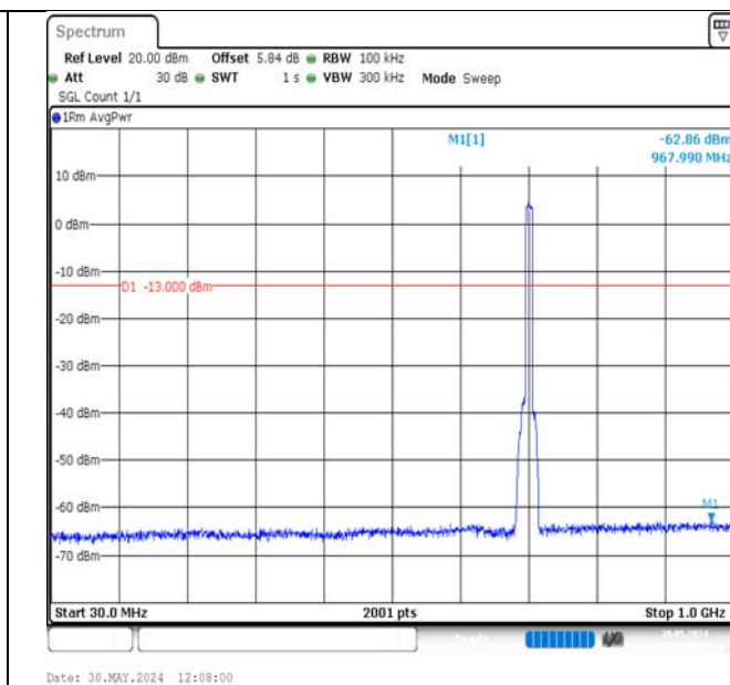
Band17-10MHz-QPSK-23780-50RB#0-30~1000-PASS
