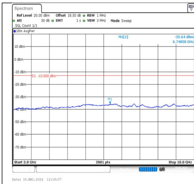
Band17-5MHz-QPSK-23825-1RB#24-3000~10000-PASS
