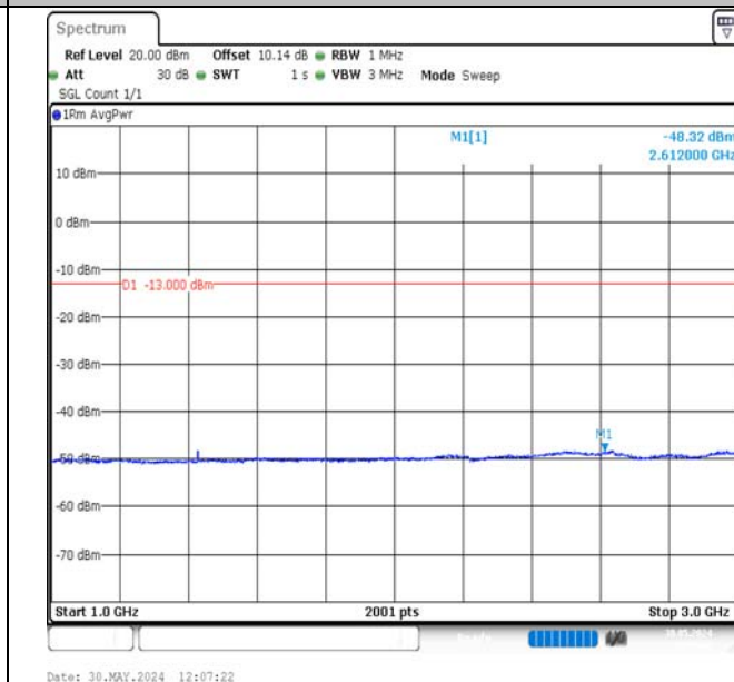
Band17-10MHz-QPSK-23780-1RB#49-1000~3000-PASS
