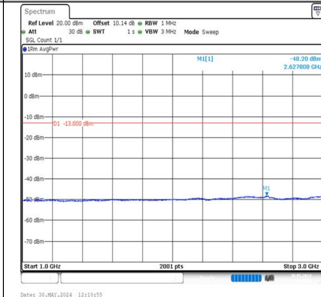
Band17-10MHz-QPSK-23800-1RB#0-1000~3000-PASS
