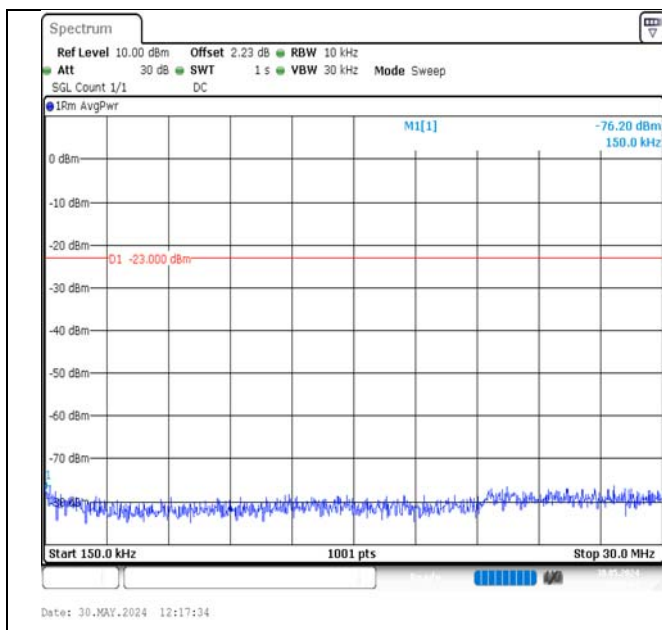
Band17-5MHz-16QAM-23825-1RB#0-0.15~30-PASS
