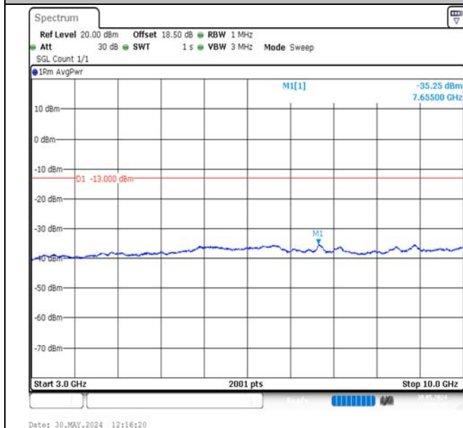
Band17-5MHz-16QAM-23790-1RB#24-3000~10000-PASS
