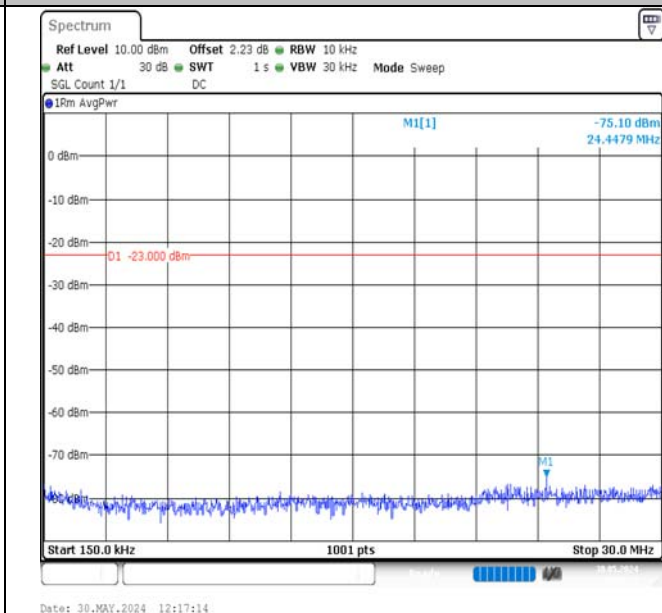
Band17-5MHz-QPSK-23825-1RB#0-0.15~30-PASS
