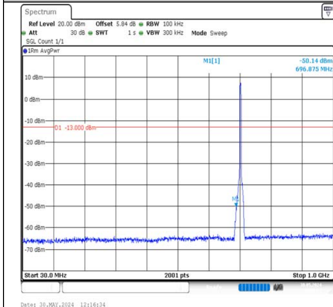
Band17-5MHz-QPSK-23790-25RB#0-30~1000-PASS
