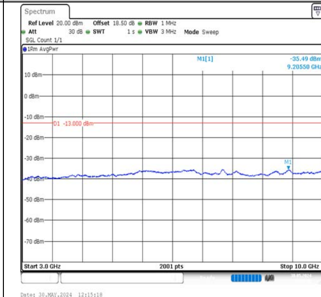
Band17-5MHz-QPSK-23790-1RB#0-3000~10000-PASS
