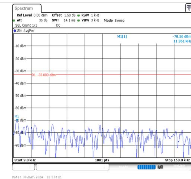
Band17-5MHz-16QAM-23825-1RB#24-0.009~0.15-PASS
