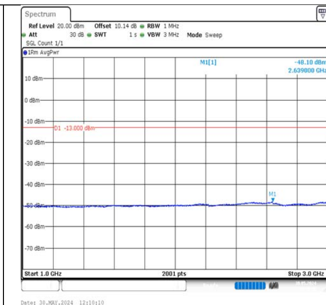
Band17-10MHz-QPSK-23790-50RB#0-1000~3000-PASS
