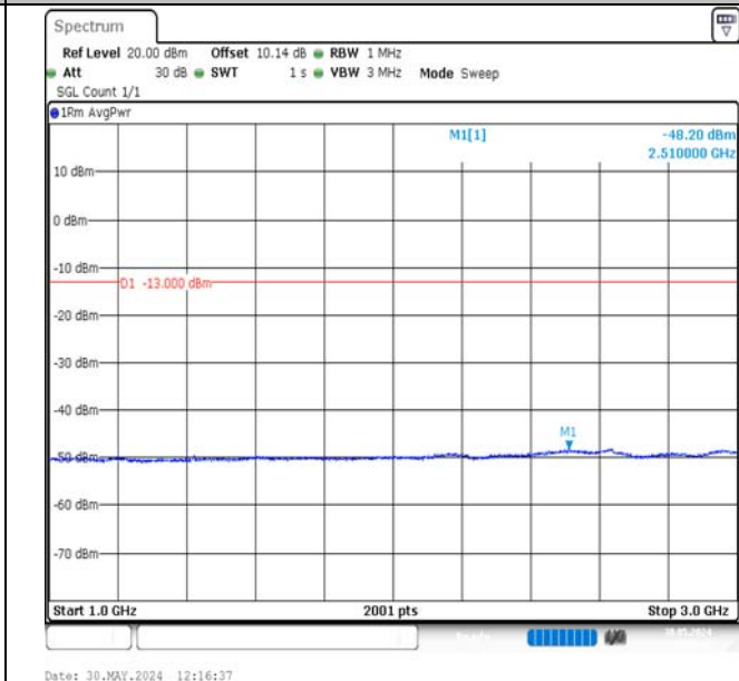
Band17-5MHz-QPSK-23790-25RB#0-1000~3000-PASS
