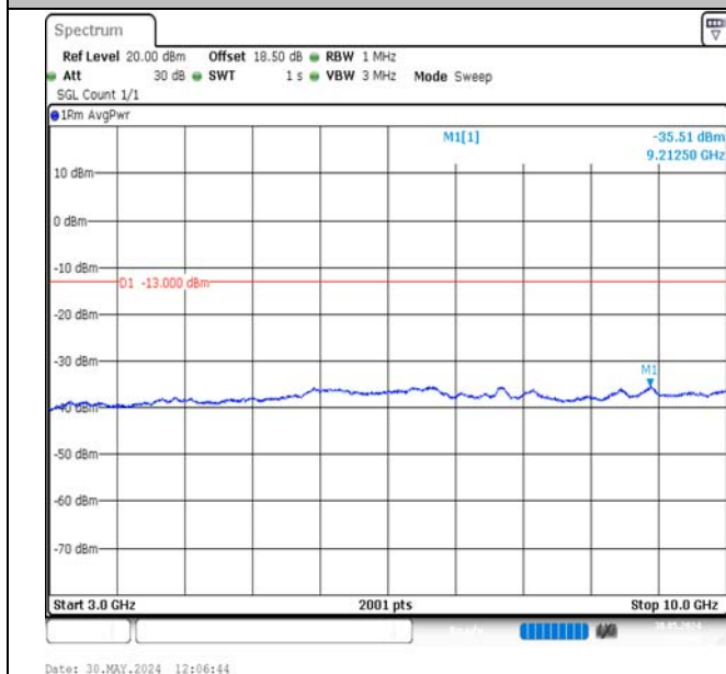
Band17-10MHz-QPSK-23780-1RB#0-3000~10000-PASS
