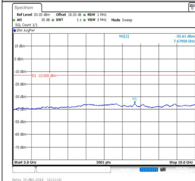
Band17-10MHz-QPSK-23800-1RB#49-3000~10000-PASS
