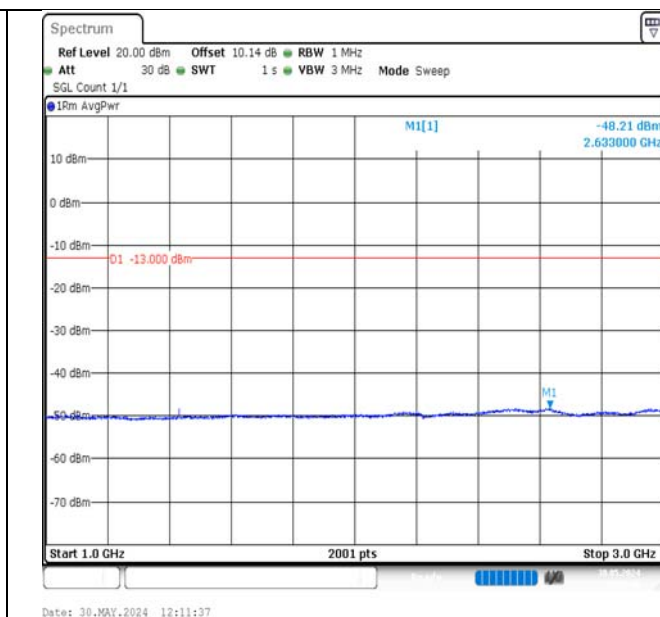
Band17-10MHz-QPSK-23800-1RB#49-1000~3000-PASS
