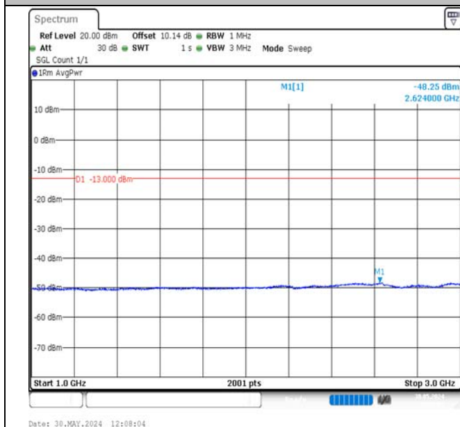
Band17-10MHz-QPSK-23780-50RB#0-1000~3000-PASS
