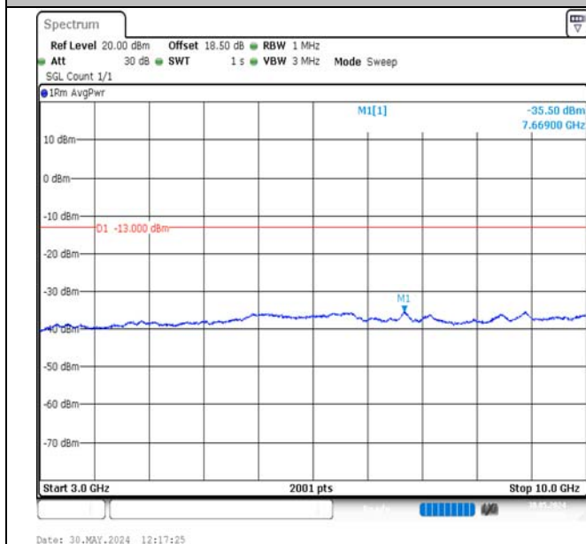
Band17-5MHz-QPSK-23825-1RB#0-3000~10000-PASS
