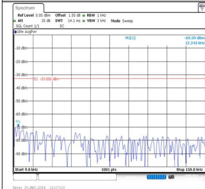
Band17-5MHz-QPSK-23825-1RB#0-0.009~0.15-PASS
