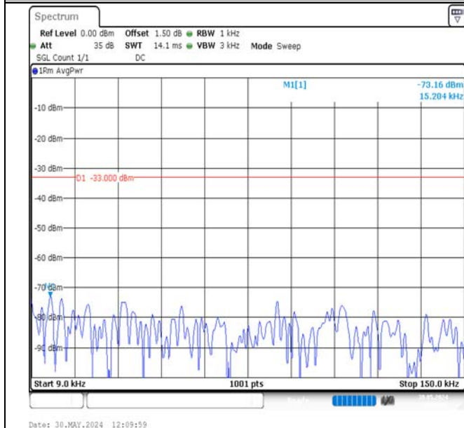
Band17-10MHz-QPSK-23790-50RB#0-0.009~0.15-PASS
