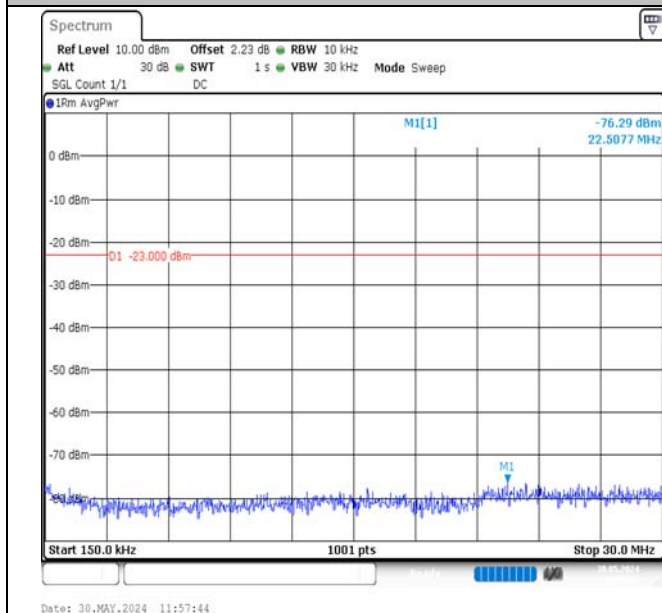
Band13-10MHz-16QAM-23230-1RB#0-0.15~30-PASS
