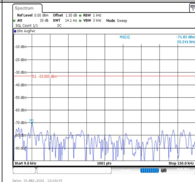
Band13-5MHz-16QAM-23255-1RB#0-0.009~0.15-PASS
