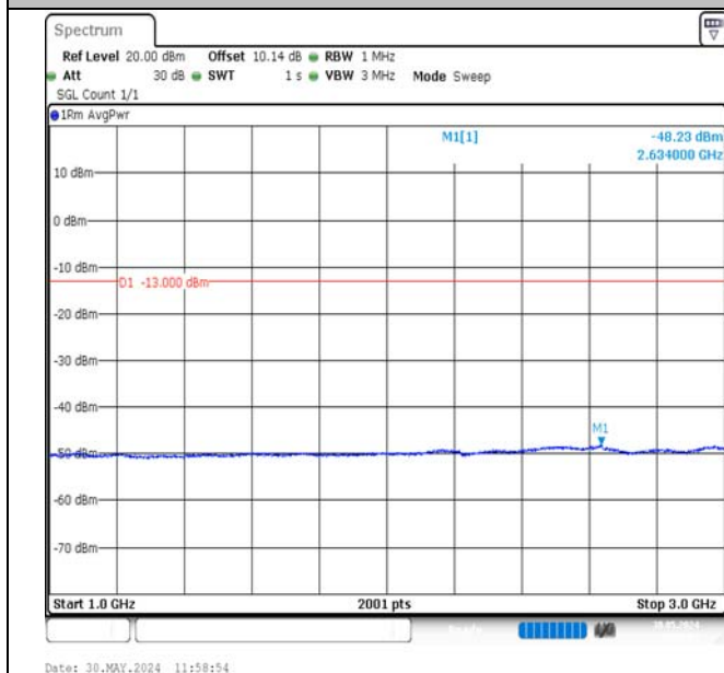
Band13-10MHz-QPSK-23230-50RB#0-1000~3000-PASS
