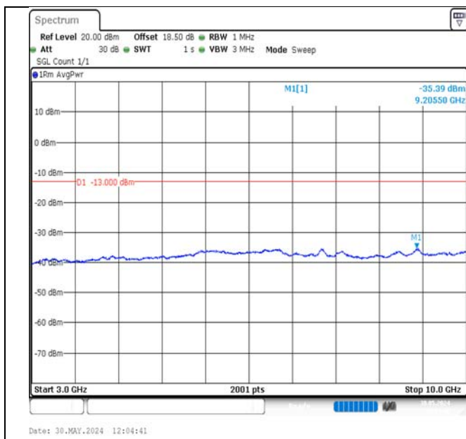
Band13-5MHz-QPSK-23255-1RB#24-3000~10000-PASS
