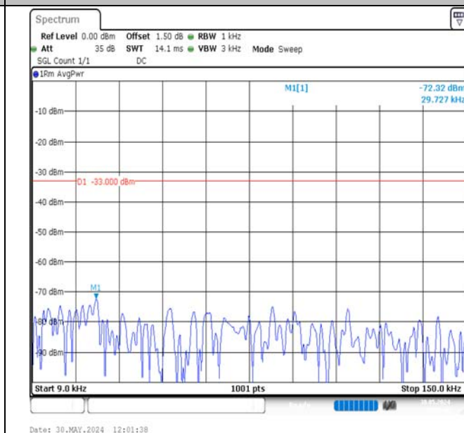
Band13-5MHz-QPSK-23230-1RB#0-0.009~0.15-PASS
