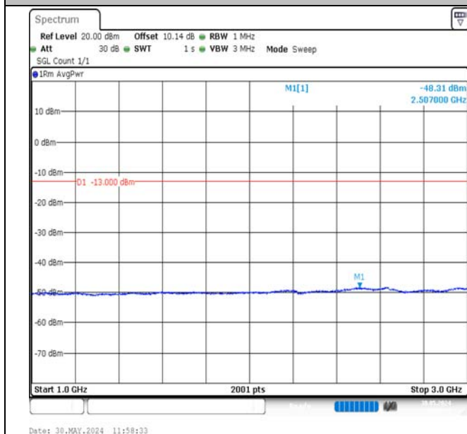
Band13-10MHz-16QAM-23230-1RB#49-1000~3000-PASS
