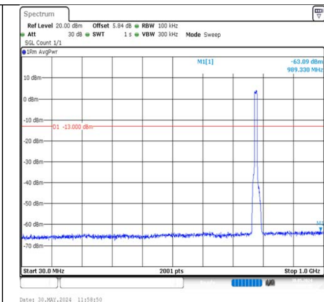
Band13-10MHz-QPSK-23230-50RB#0-30~1000-PASS
