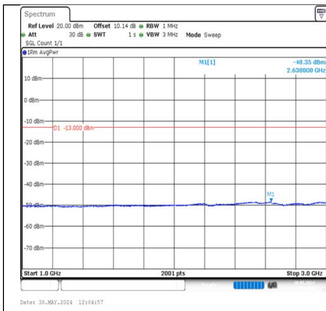
Band13-5MHz-16QAM-23255-1RB#24-1000~3000-PASS
