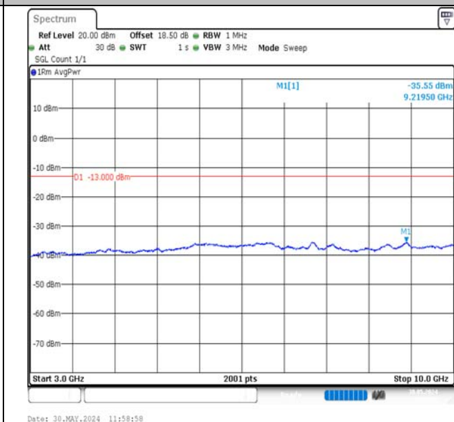
Band13-10MHz-QPSK-23230-50RB#0-3000~10000-PASS
