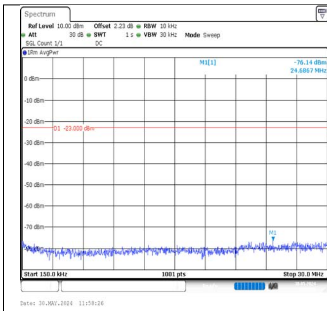
Band13-10MHz-16QAM-23230-1RB#49-0.15~30-PASS
