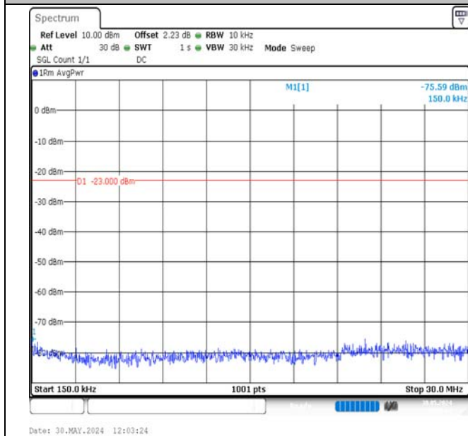
Band13-5MHz-16QAM-23230-25RB#0-0.15~30-PASS
