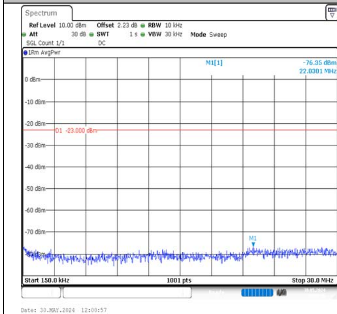
Band13-5MHz-QPSK-23205-25RB#0-0.15~30-PASS
