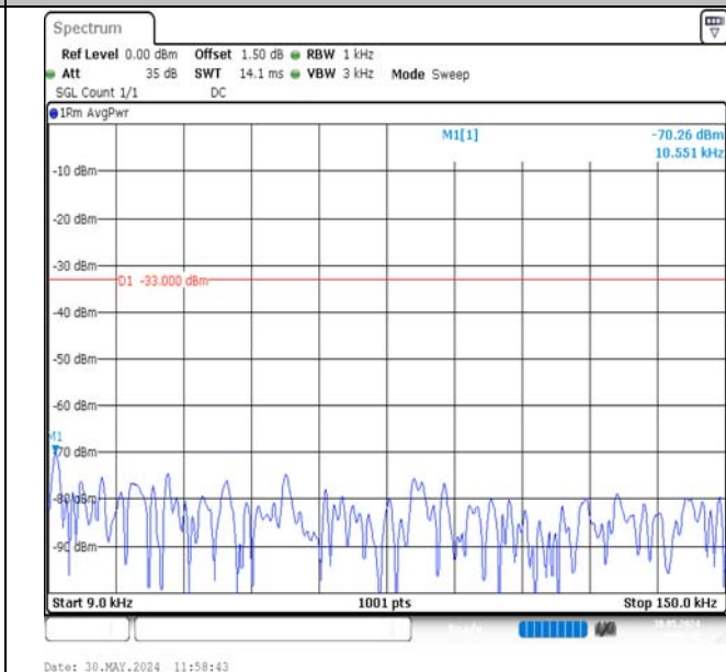
Band13-10MHz-QPSK-23230-50RB#0-0.009~0.15-PASS
