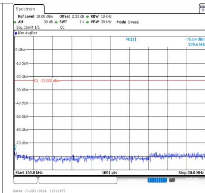
Band17-5MHz-QPSK-23755-1RB#0-0.15~30-PASS
