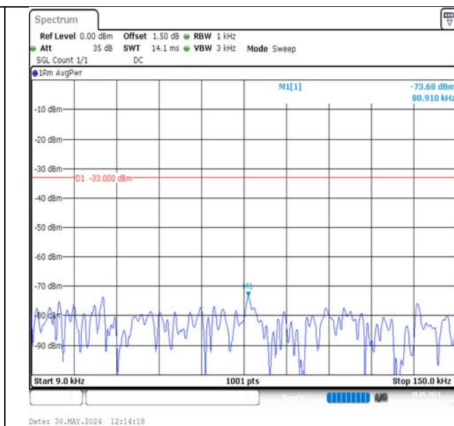
Band17-5MHz-QPSK-23755-25RB#0-0.009~0.15-PASS
