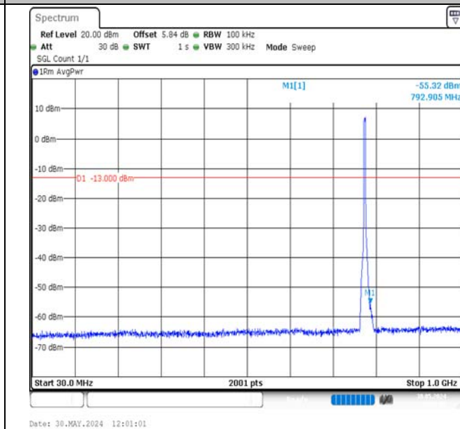
Band13-5MHz-QPSK-23205-25RB#0-30~1000-PASS
