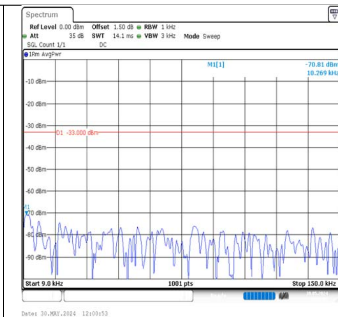
Band13-5MHz-QPSK-23205-25RB#0-0.009~0.15-PASS
