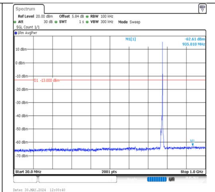
Band13-5MHz-16QAM-23205-1RB#24-30~1000-PASS
