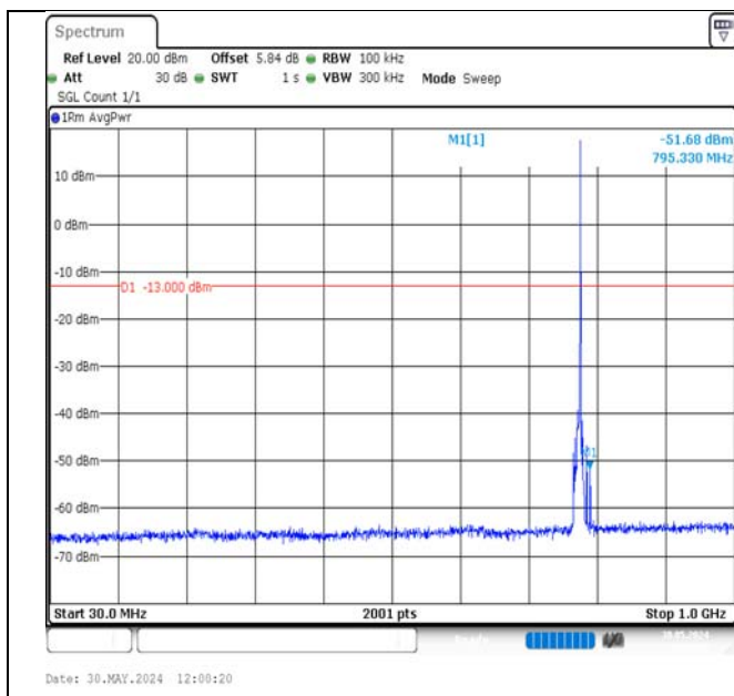
Band13-5MHz-QPSK-23205-1RB#24-30~1000-PASS
