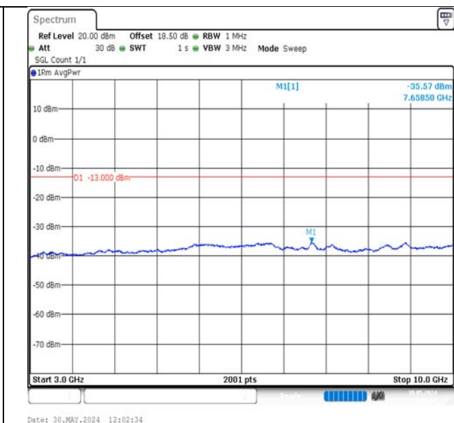
Band13-5MHz-QPSK-23230-1RB#24-3000~10000-PASS
