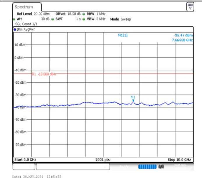
Band13-5MHz-QPSK-23230-1RB#0-3000~10000-PASS
