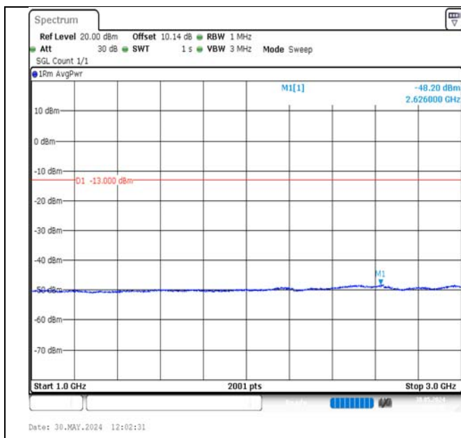
Band13-5MHz-QPSK-23230-1RB#24-1000~3000-PASS
