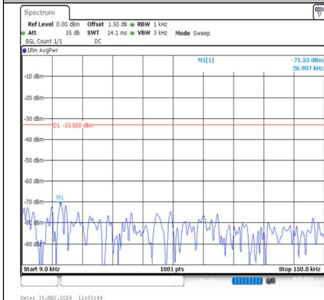
Band13-5MHz-QPSK-23255-1RB#0-0.009~0.15-PASS
