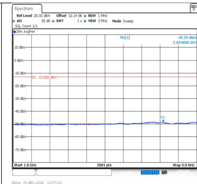
Band13-10MHz-QPSK-23230-1RB#0-1000~3000-PASS
