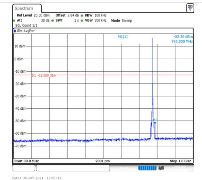
Band13-5MHz-QPSK-23230-1RB#0-30~1000-PASS
