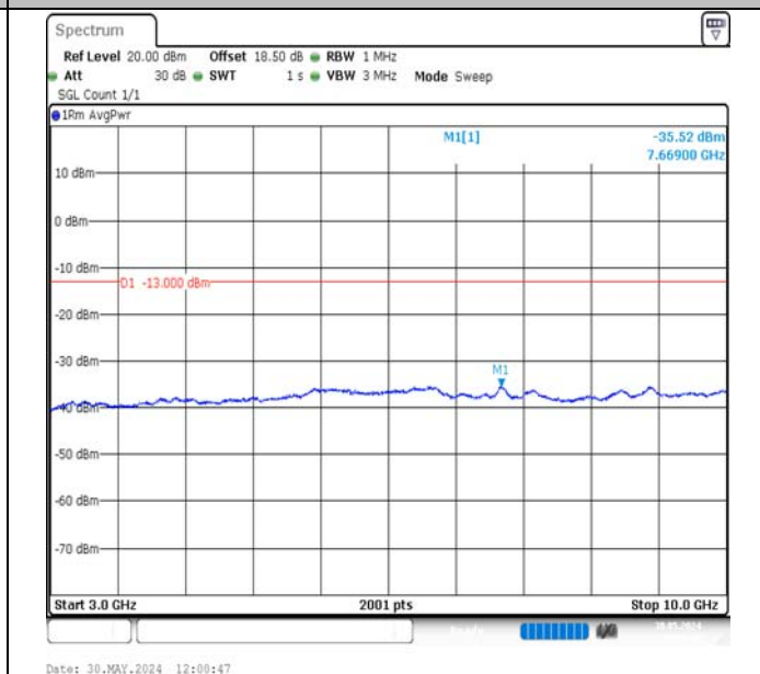
Band13-5MHz-16QAM-23205-1RB#24-3000~10000-PASS
