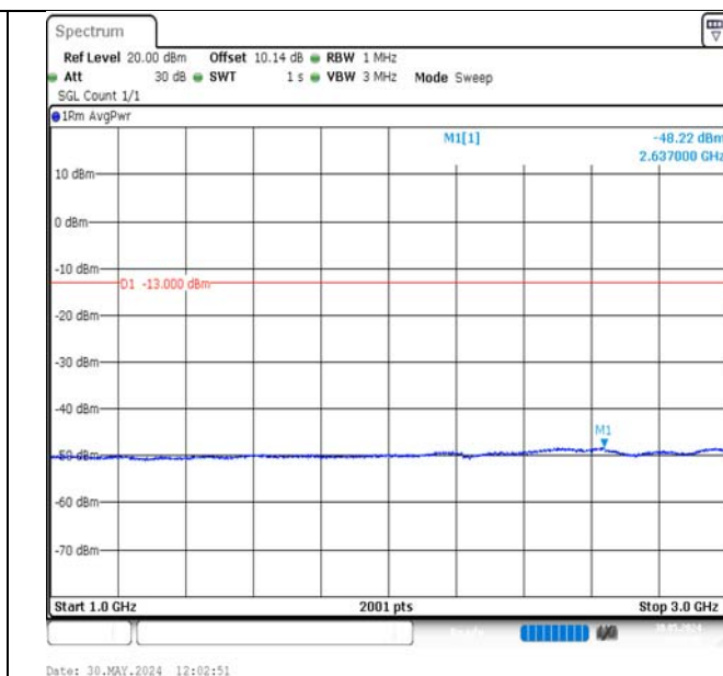
Band13-5MHz-16QAM-23230-1RB#24-1000~3000-PASS
