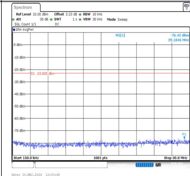
Band13-5MHz-QPSK-23255-1RB#0-0.15~30-PASS
