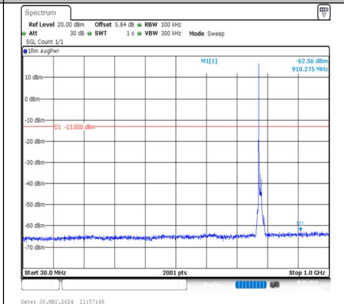
Band13-10MHz-16QAM-23230-1RB#0-30~1000-PASS
