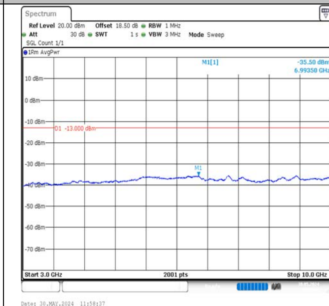
Band13-10MHz-16QAM-23230-1RB#49-3000~10000-PASS
