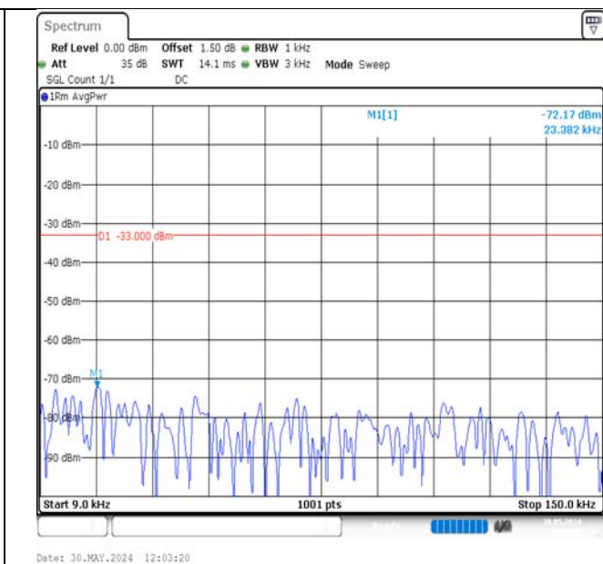
Band13-5MHz-16QAM-23230-25RB#0-0.009~0.15-PASS
