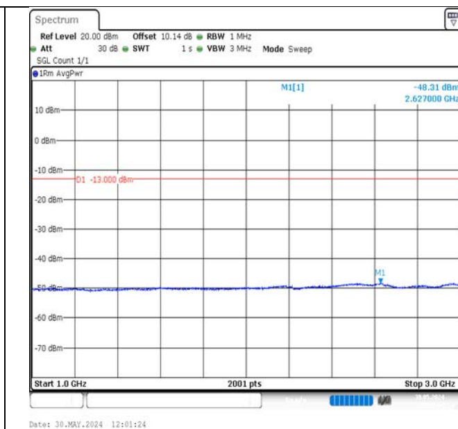
Band13-5MHz-16QAM-23205-25RB#0-1000~3000-PASS
