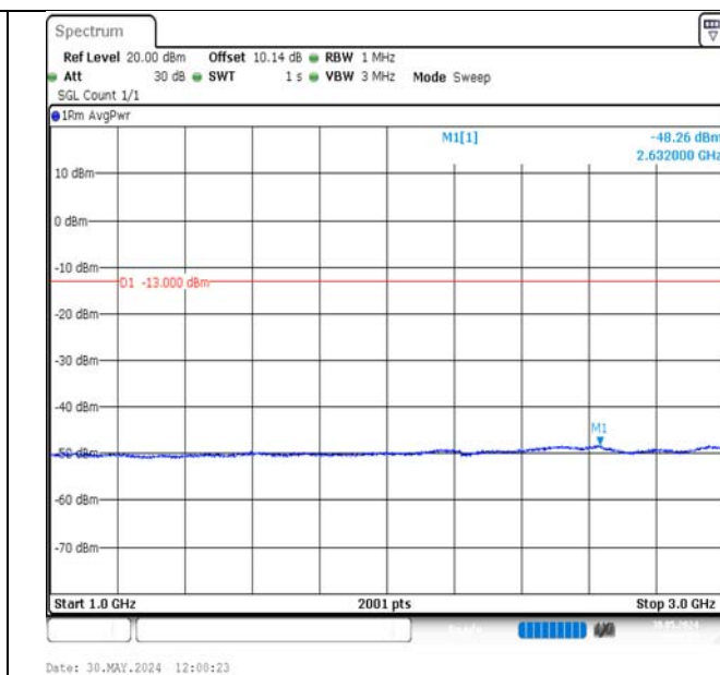
Band13-5MHz-QPSK-23205-1RB#24-1000~3000-PASS
