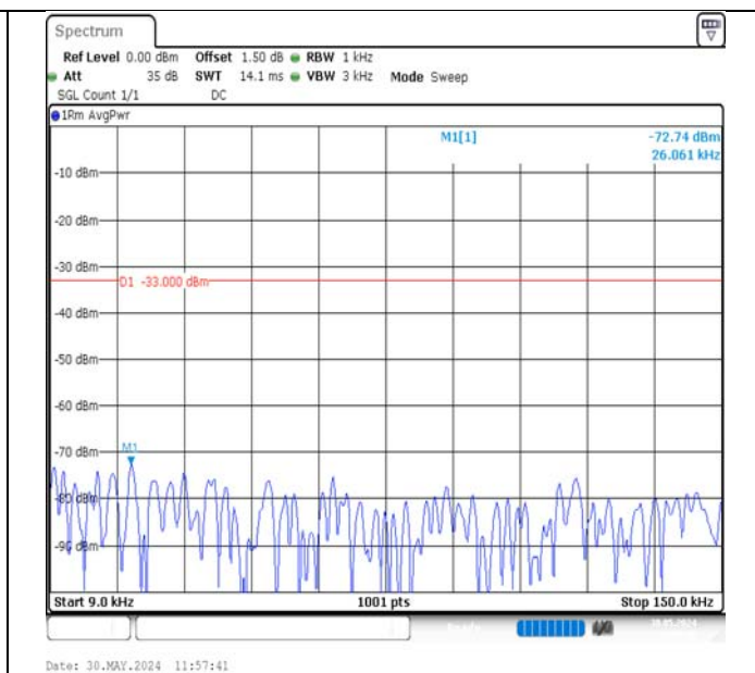
Band13-10MHz-16QAM-23230-1RB#0-0.009~0.15-PASS
