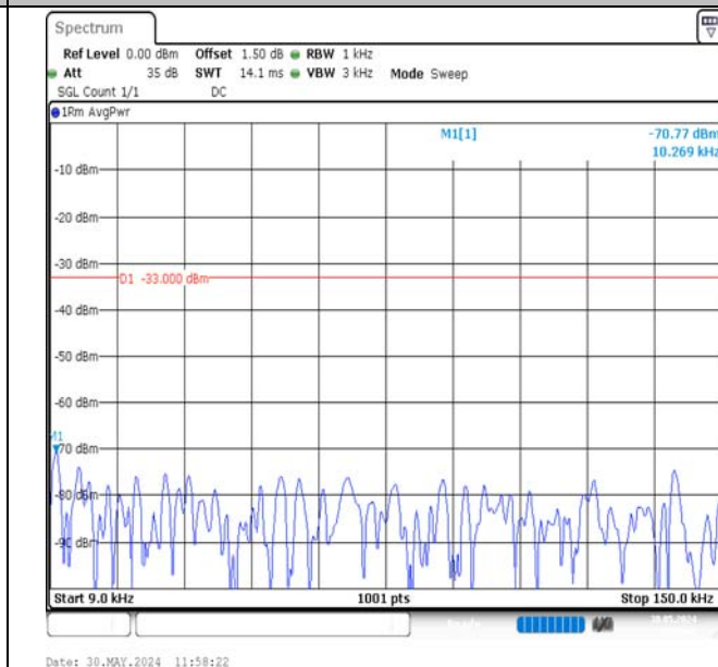
Band13-10MHz-16QAM-23230-1RB#49-0.009~0.15-PASS
