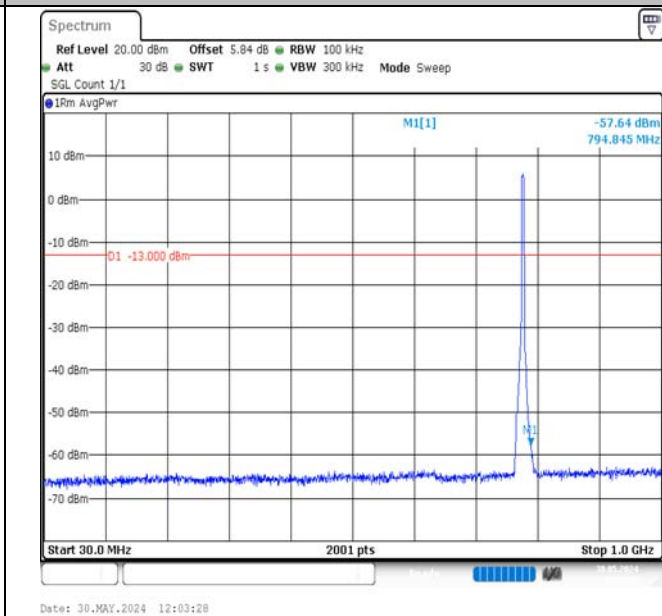
Band13-5MHz-16QAM-23230-25RB#0-30~1000-PASS
