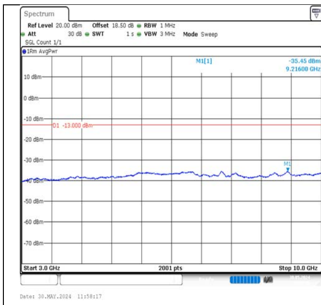
Band13-10MHz-QPSK-23230-1RB#49-3000~10000-PASS
