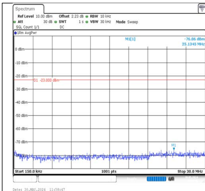
Band13-10MHz-QPSK-23230-50RB#0-0.15~30-PASS
