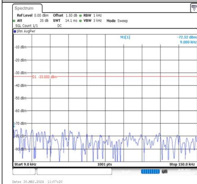
Band13-10MHz-QPSK-23230-1RB#0-0.009~0.15-PASS
