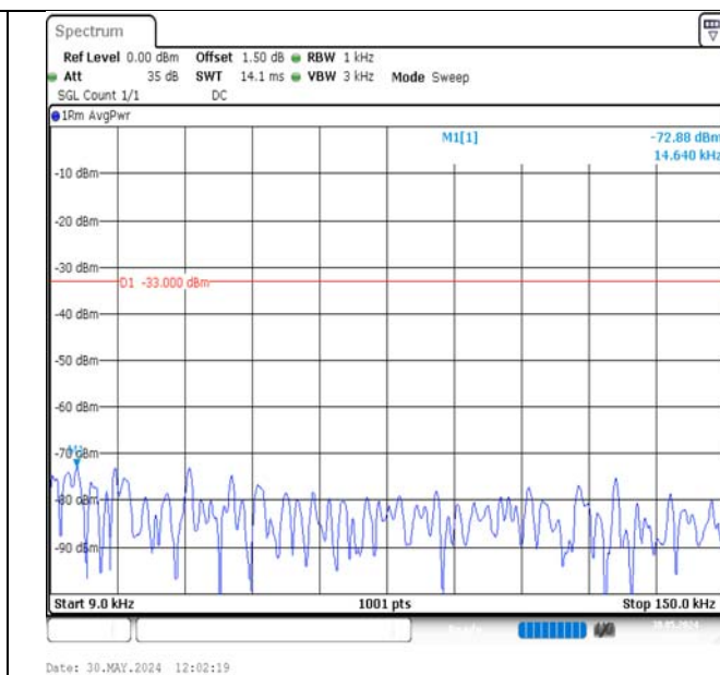
Band13-5MHz-QPSK-23230-1RB#24-0.009~0.15-PASS
