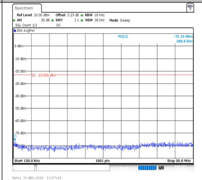
Band13-10MHz-QPSK-23230-1RB#0-0.15~30-PASS
