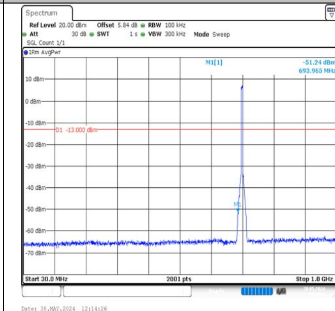
Band17-5MHz-QPSK-23755-25RB#0-30~1000-PASS
