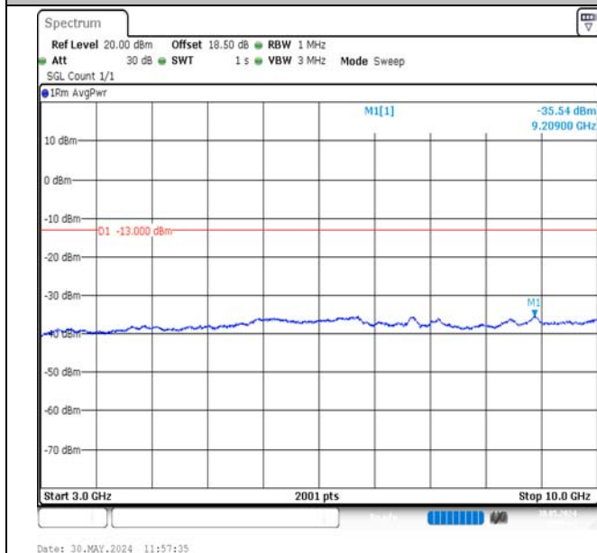
Band13-10MHz-QPSK-23230-1RB#0-3000~10000-PASS
