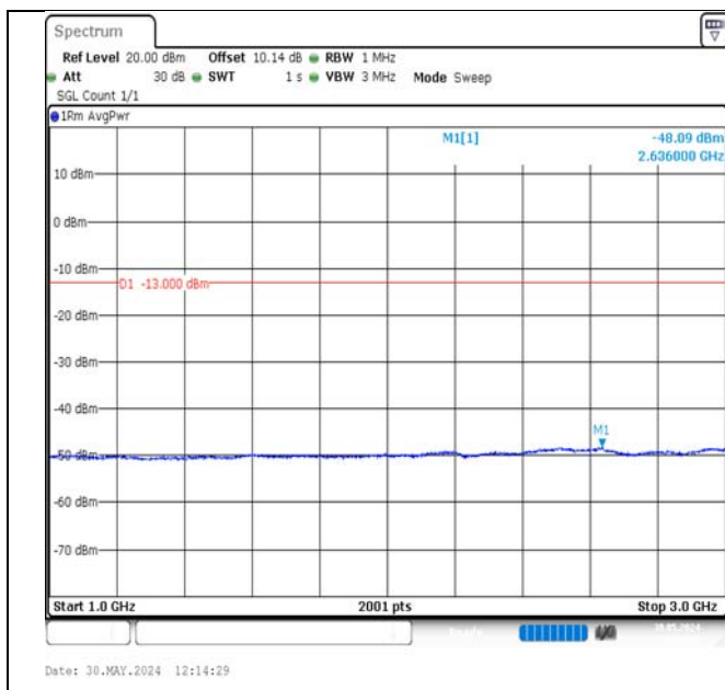
Band17-5MHz-QPSK-23755-25RB#0-1000~3000-PASS
