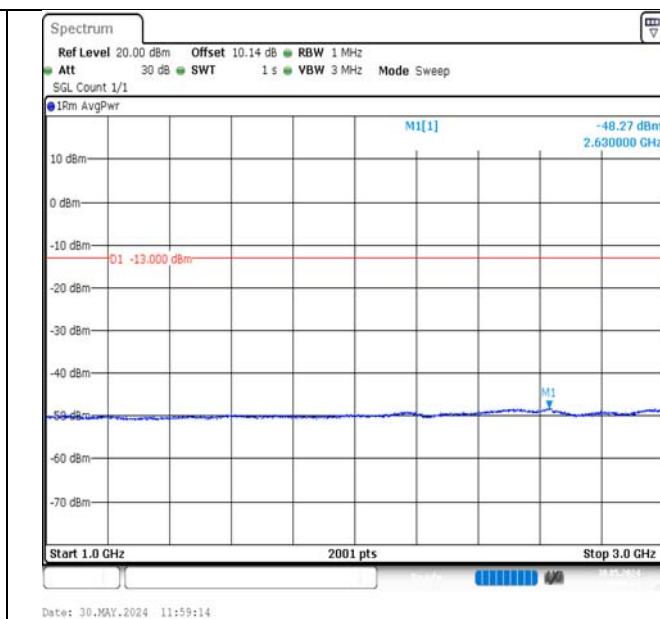
Band13-10MHz-16QAM-23230-50RB#0-1000~3000-PASS
