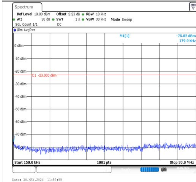
Band13-5MHz-16QAM-23205-1RB#0-0.15~30-PASS
