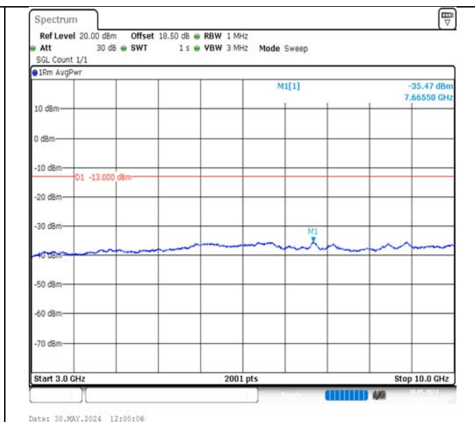
Band13-5MHz-16QAM-23205-1RB#0-3000~10000-PASS
