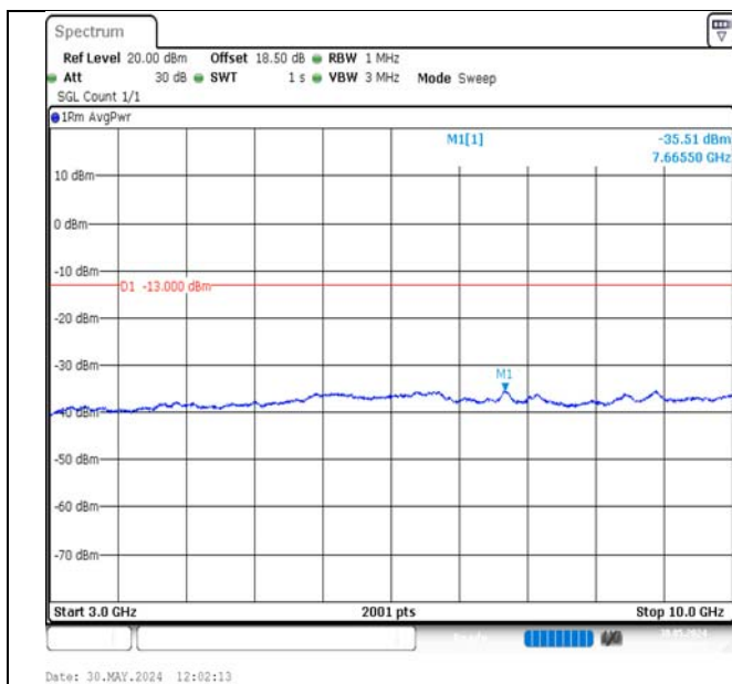
Band13-5MHz-16QAM-23230-1RB#0-3000~10000-PASS
