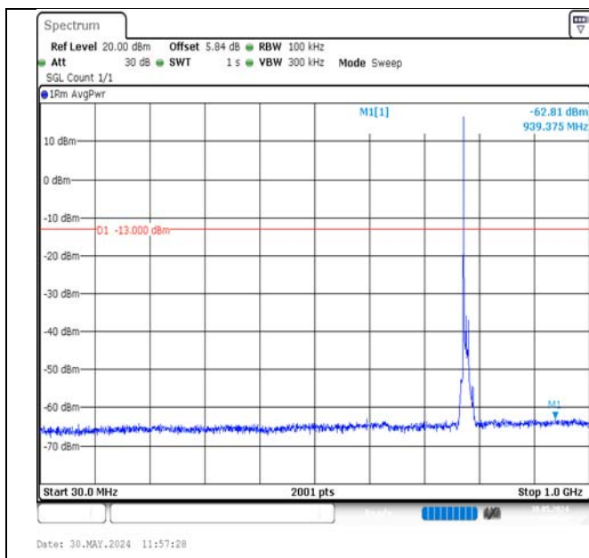
Band13-10MHz-QPSK-23230-1RB#0-30~1000-PASS
