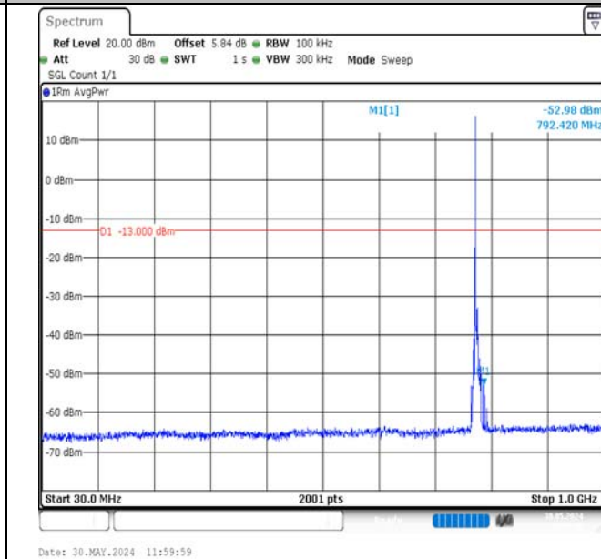
Band13-5MHz-16QAM-23205-1RB#0-30~1000-PASS
