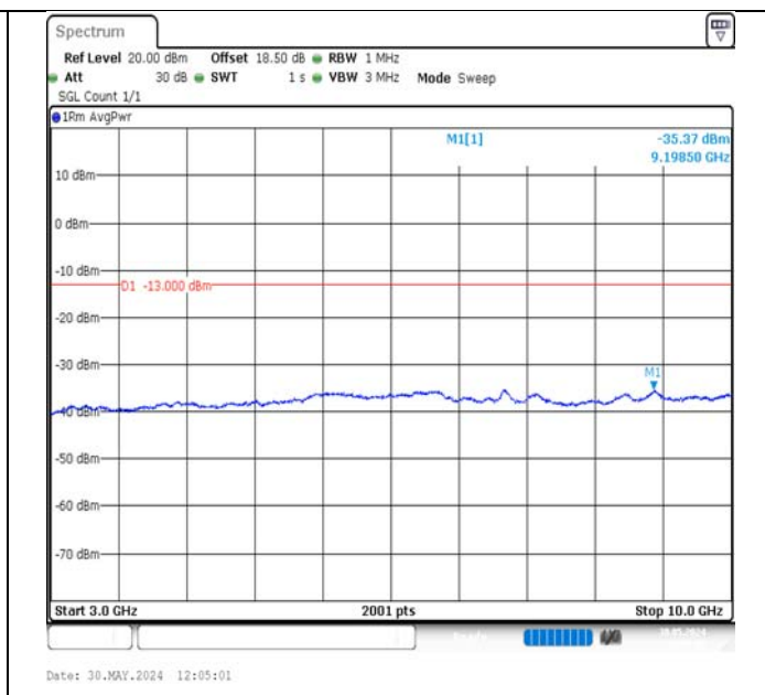
Band13-5MHz-16QAM-23255-1RB#24-3000~10000-PASS
