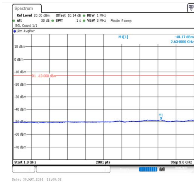
Band13-5MHz-16QAM-23205-1RB#0-1000~3000-PASS
