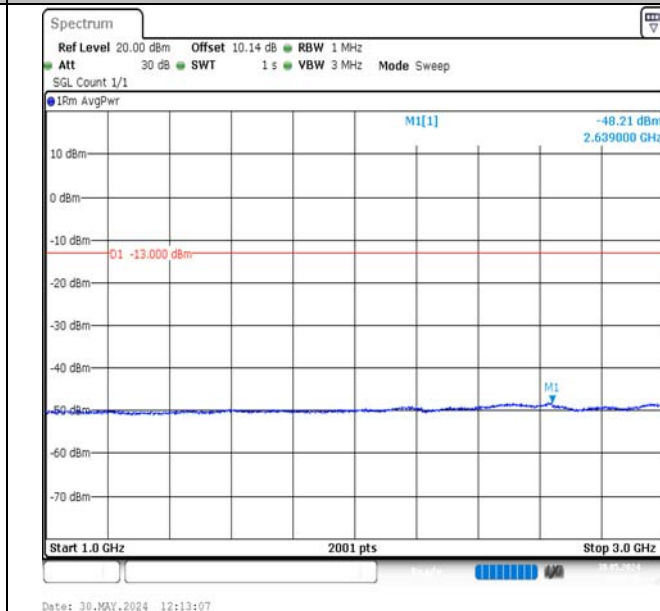
Band17-5MHz-QPSK-23755-1RB#0-1000~3000-PASS
