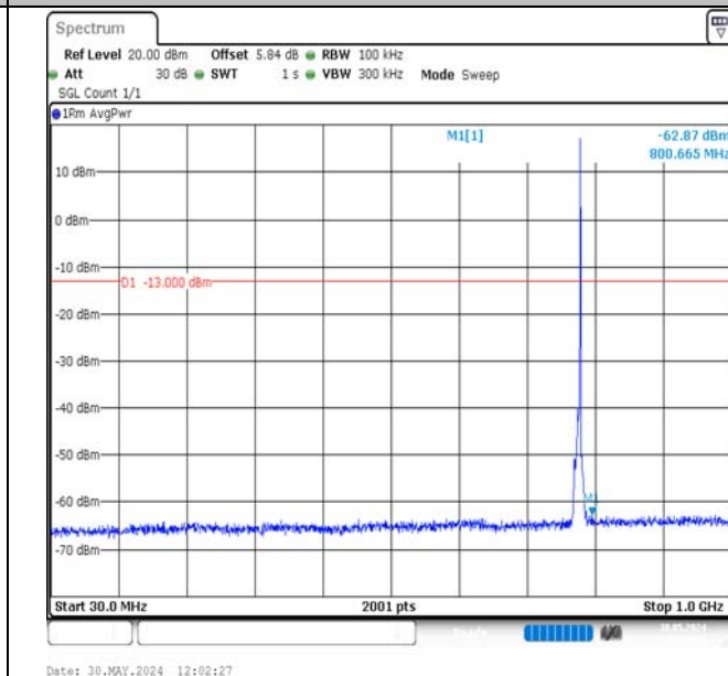
Band13-5MHz-QPSK-23230-1RB#24-30~1000-PASS
