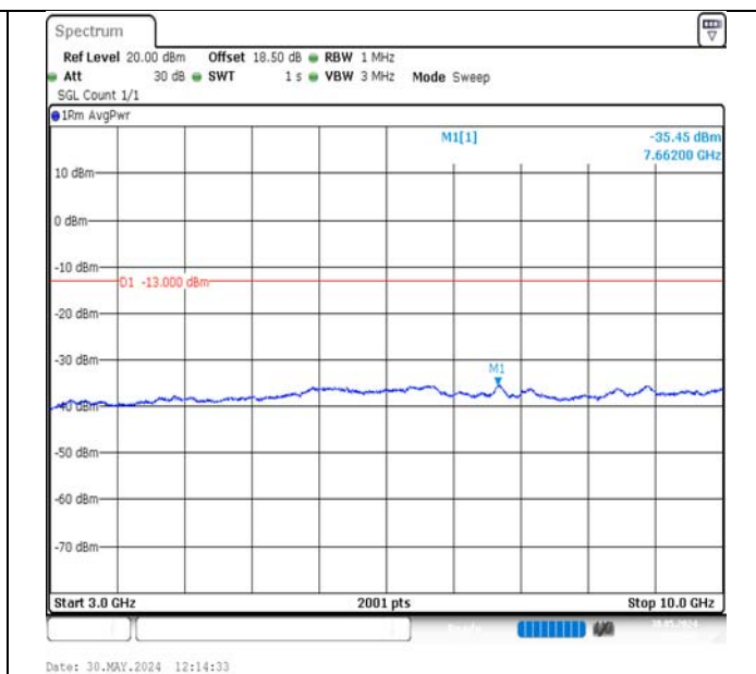
Band17-5MHz-QPSK-23755-25RB#0-3000~10000-PASS
