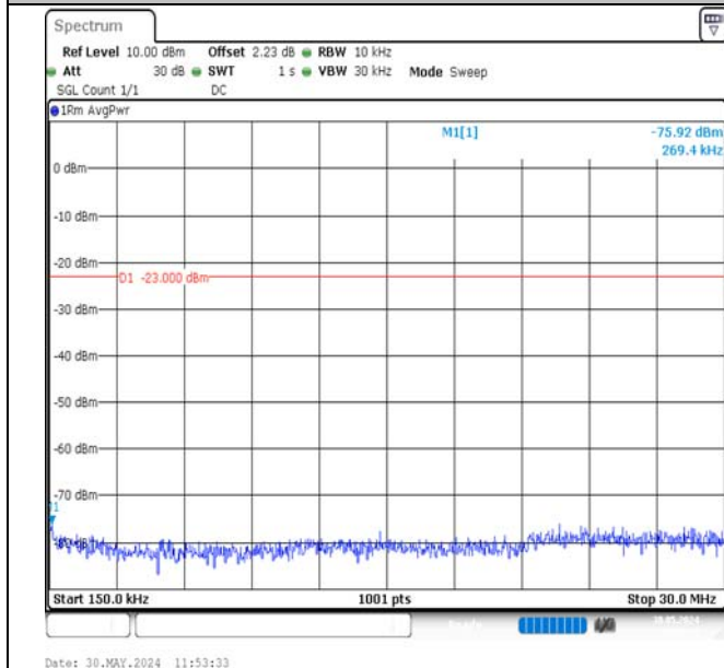
Band12-5MHz-QPSK-23095-1RB#24-0.15~30-PASS
