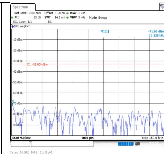
Band12-5MHz-QPSK-23035-25RB#0-0.009~0.15-PASS
