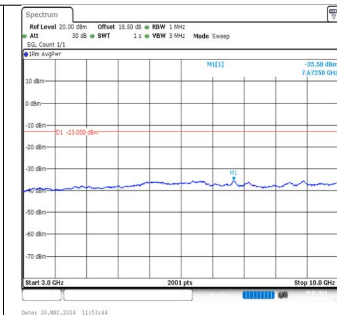
Band12-5MHz-QPSK-23095-1RB#24-3000~10000-PASS
