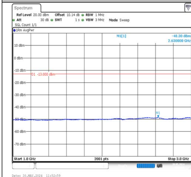
Band12-5MHz-QPSK-23095-1RB#0-1000~3000-PASS
