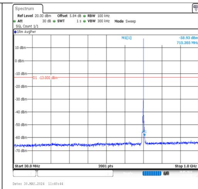
Band12-3MHz-QPSK-23095-1RB#14-30~1000-PASS
