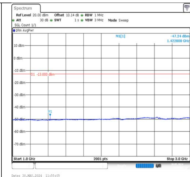
Band12-5MHz-QPSK-23155-1RB#0-1000~3000-PASS
