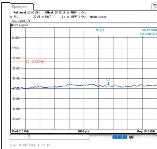
Band12-5MHz-QPSK-23155-1RB#24-3000~10000-PASS
