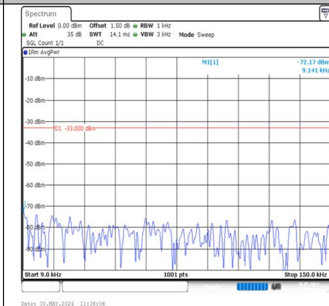
Band12-3MHz-16QAM-23025-1RB#0-0.009~0.15-PASS
