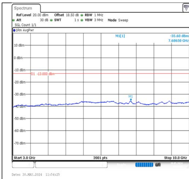
Band12-5MHz-QPSK-23095-25RB#0-3000~10000-PASS
