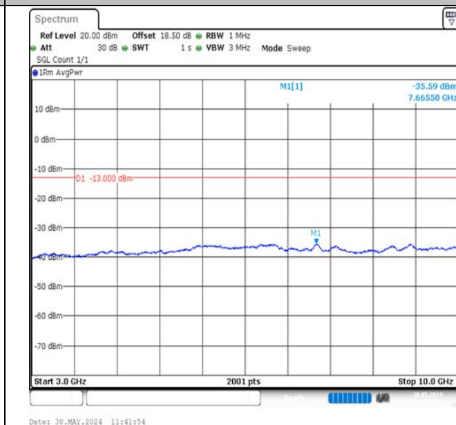
Band12-3MHz-16QAM-23095-15RB#0-3000~10000-PASS
