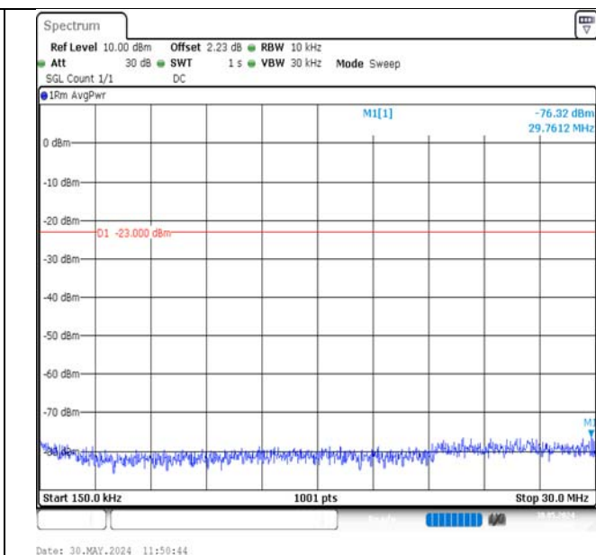
Band12-5MHz-QPSK-23035-1RB#0-0.15~30-PASS
