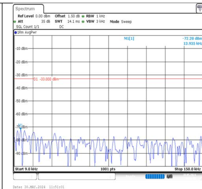
Band12-5MHz-16QAM-23035-1RB#0-0.009~0.15-PASS
