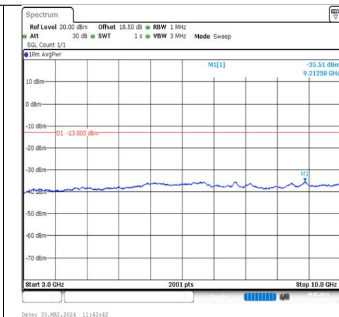
Band12-3MHz-QPSK-23165-15RB#0-3000~10000-PASS
