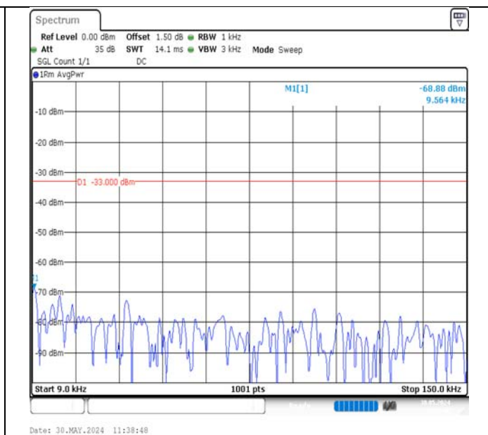
Band12-3MHz-16QAM-23025-1RB#14-0.009~0.15-PASS
