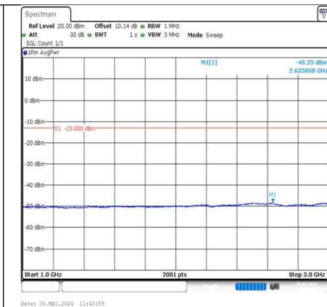
Band12-3MHz-16QAM-23165-15RB#0-1000~3000-PASS
