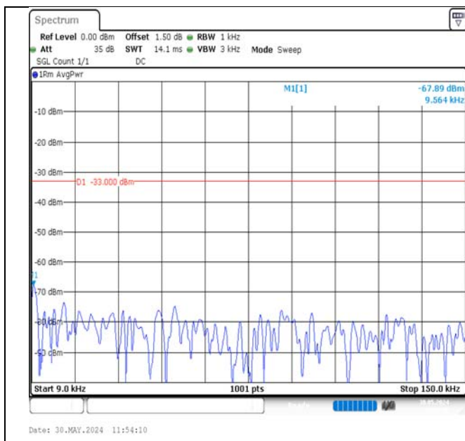
Band12-5MHz-QPSK-23095-25RB#0-0.009~0.15-PASS
