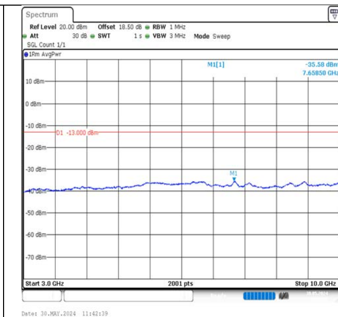
Band12-3MHz-16QAM-23165-1RB#0-3000~10000-PASS
