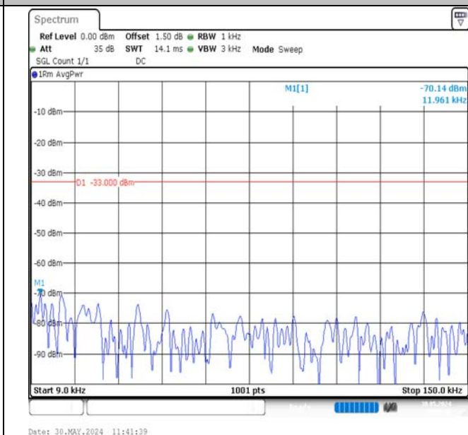
Band12-3MHz-16QAM-23095-15RB#0-0.009~0.15-PASS
