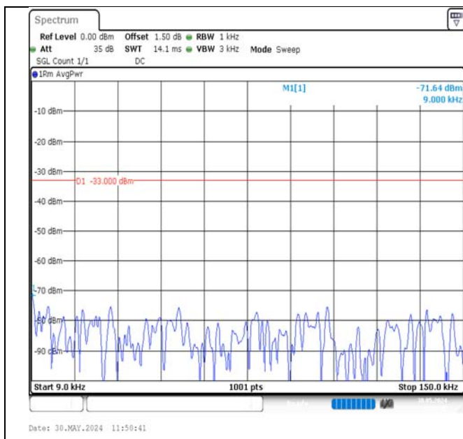
Band12-5MHz-QPSK-23035-1RB#0-0.009~0.15-PASS
