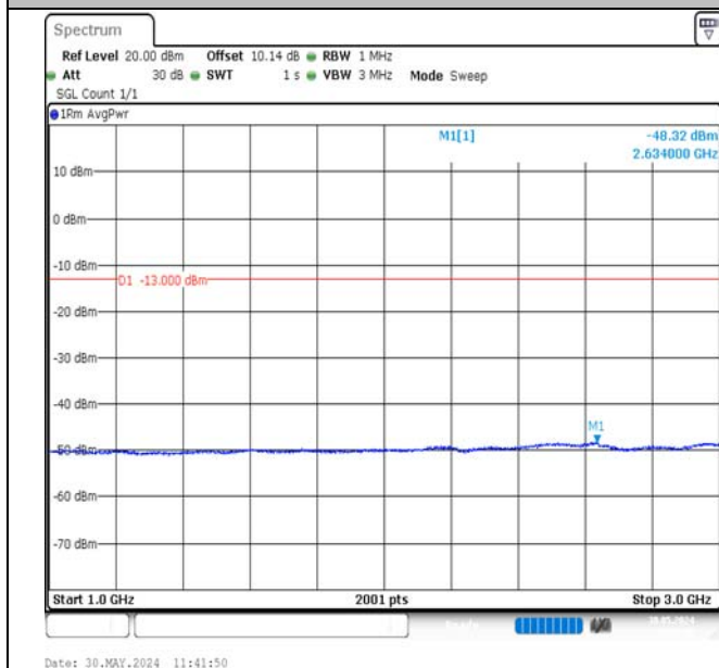
Band12-3MHz-16QAM-23095-15RB#0-1000~3000-PASS
