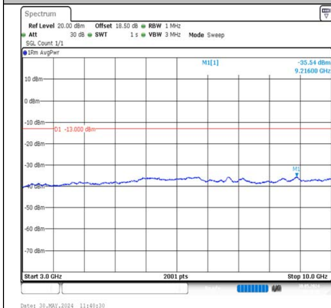
Band12-3MHz-16QAM-23095-1RB#0-3000~10000-PASS
