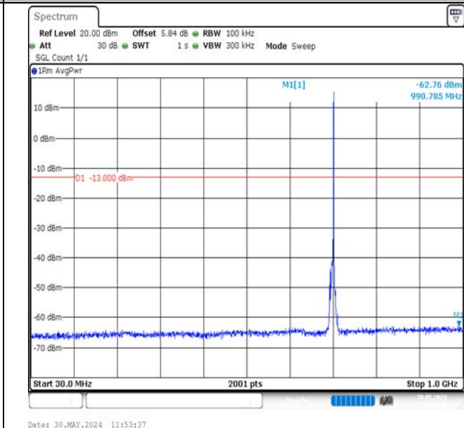
Band12-5MHz-QPSK-23095-1RB#24-30~1000-PASS
