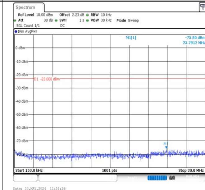
Band12-5MHz-QPSK-23035-1RB#24-0.15~30-PASS
