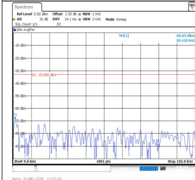
Band12-5MHz-QPSK-23035-1RB#24-0.009~0.15-PASS
