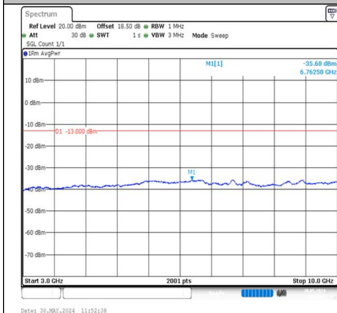
Band12-5MHz-16QAM-23035-25RB#0-3000~10000-PASS
