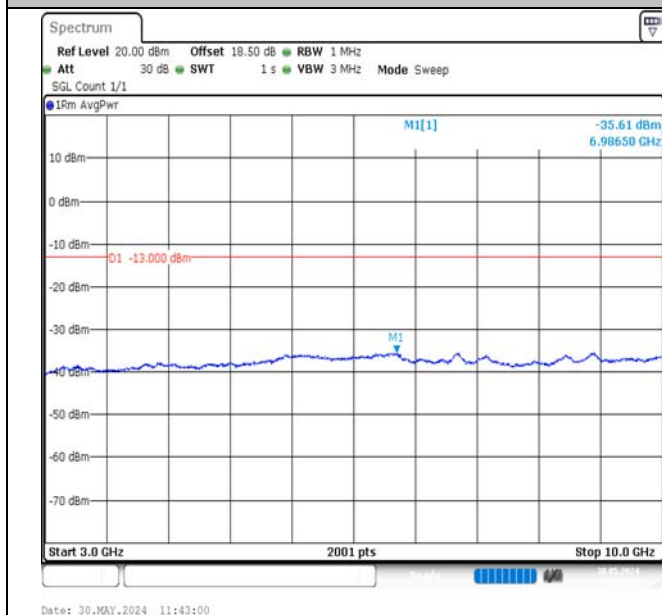
Band12-3MHz-QPSK-23165-1RB#14-3000~10000-PASS
