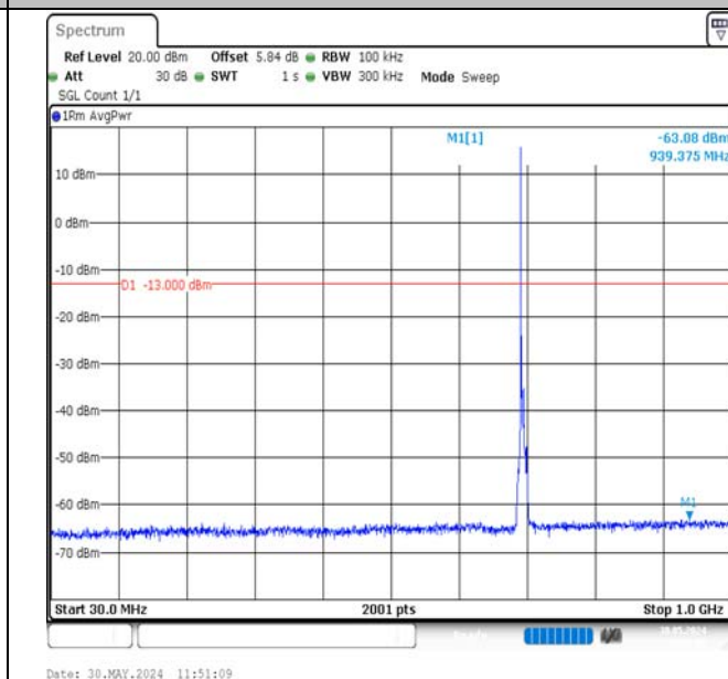
Band12-5MHz-16QAM-23035-1RB#0-30~1000-PASS
