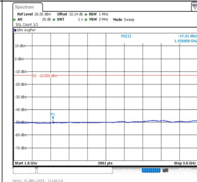
Band12-3MHz-QPSK-23165-1RB#0-1000~3000-PASS
