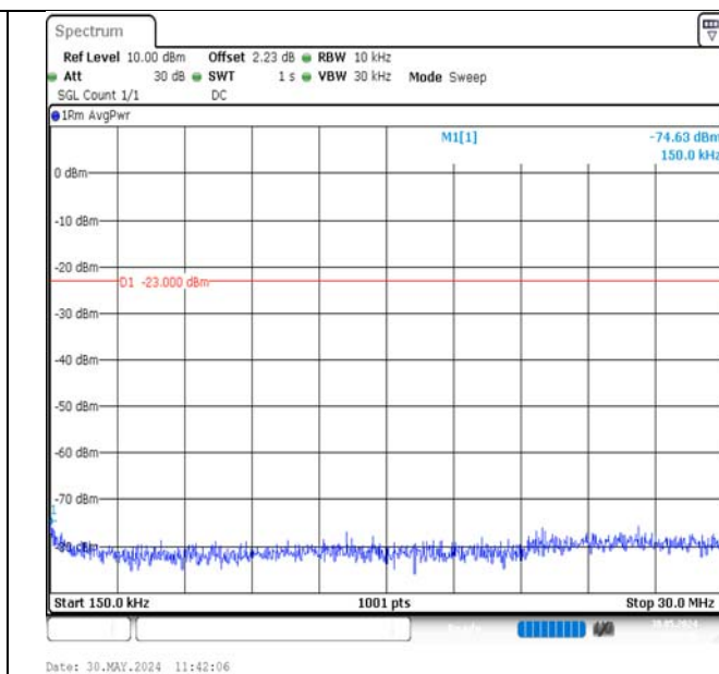
Band12-3MHz-QPSK-23165-1RB#0-0.15~30-PASS
