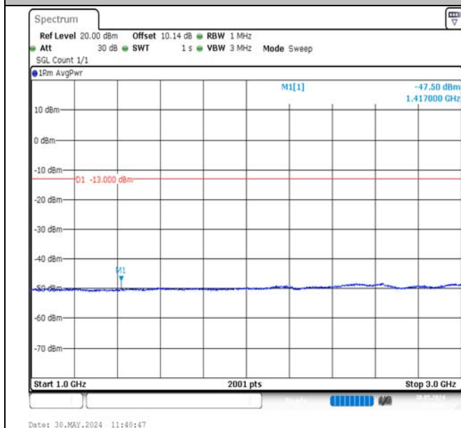
Band12-3MHz-QPSK-23095-1RB#14-1000~3000-PASS
