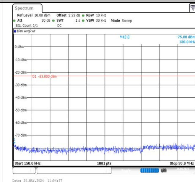
Band12-5MHz-QPSK-23155-1RB#0-0.15~30-PASS
