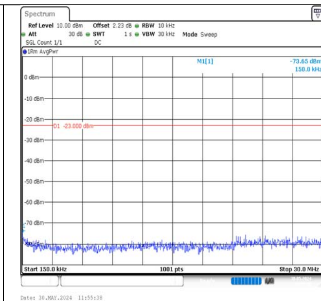
Band12-5MHz-QPSK-23155-1RB#24-0.15~30-PASS
