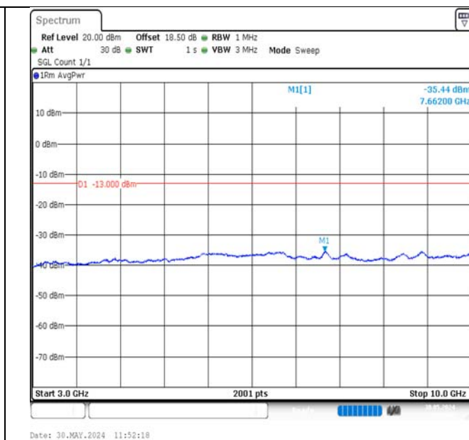
Band12-5MHz-QPSK-23035-25RB#0-3000~10000-PASS
