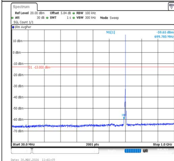
Band12-3MHz-16QAM-23095-1RB#14-30~1000-PASS
