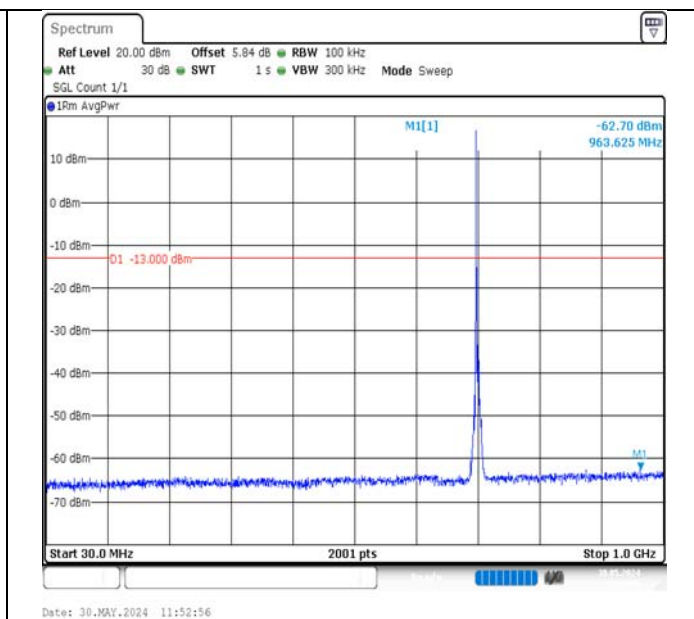
Band12-5MHz-QPSK-23095-1RB#0-30~1000-PASS
