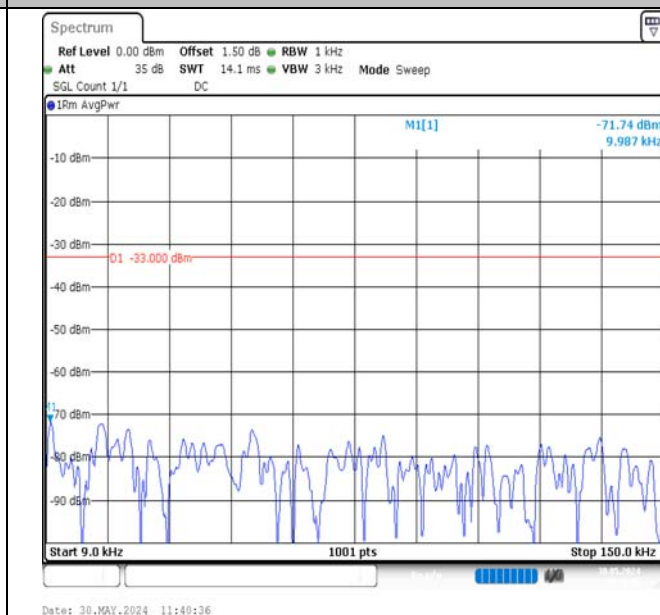
Band12-3MHz-QPSK-23095-1RB#14-0.009~0.15-PASS
