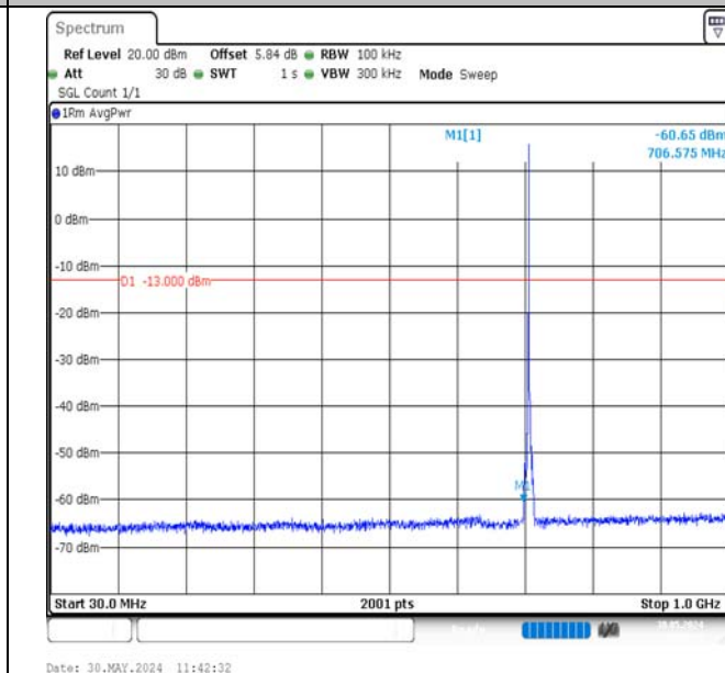
Band12-3MHz-16QAM-23165-1RB#0-30~1000-PASS
