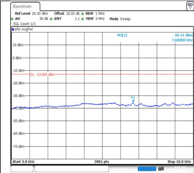
Band12-3MHz-QPSK-23165-1RB#0-3000~10000-PASS
