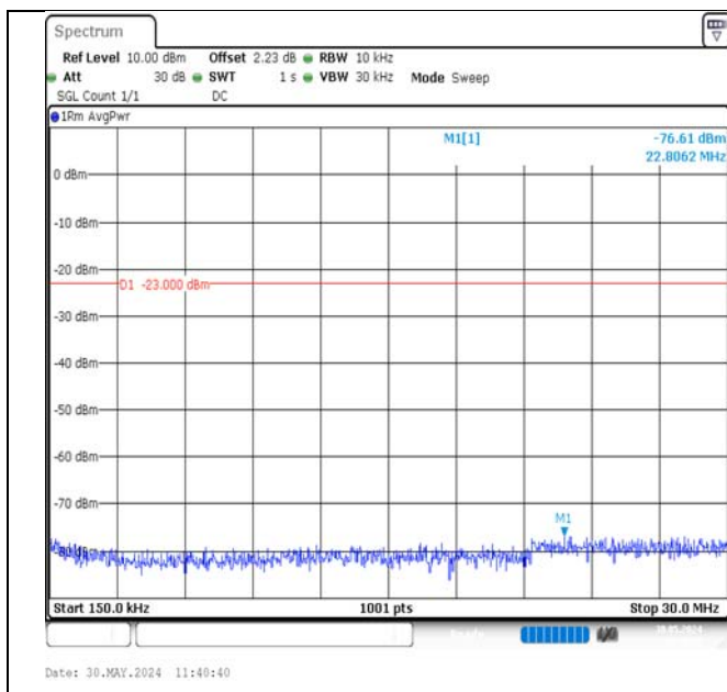
Band12-3MHz-QPSK-23095-1RB#14-0.15~30-PASS
