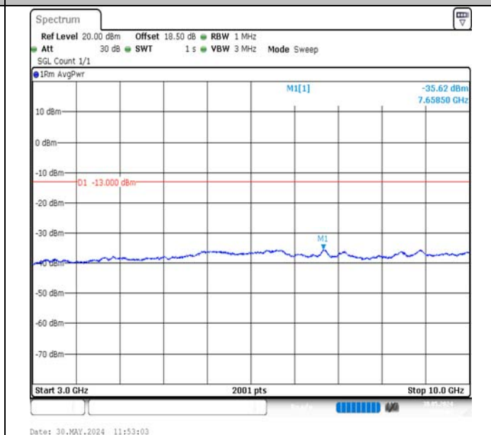
Band12-5MHz-QPSK-23095-1RB#0-3000~10000-PASS
