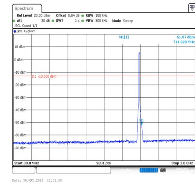
Band12-5MHz-16QAM-23035-25RB#0-30~1000-PASS
