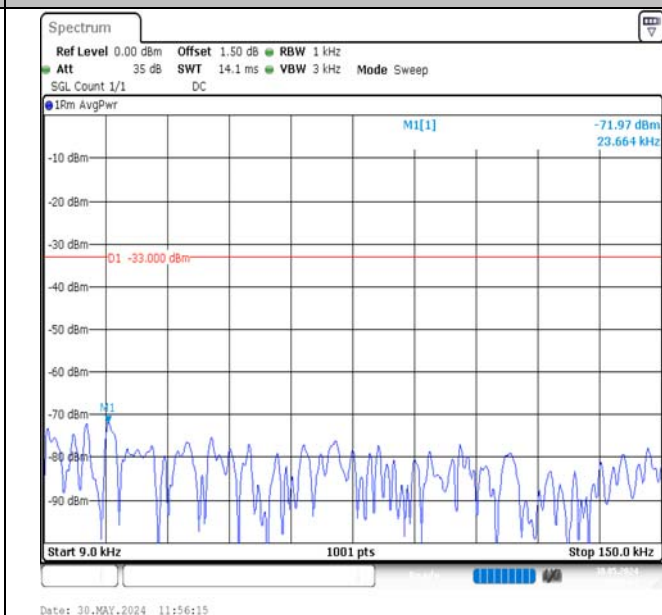
Band12-5MHz-QPSK-23155-25RB#0-0.009~0.15-PASS
