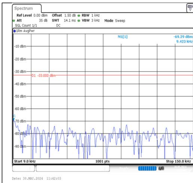
Band12-3MHz-QPSK-23165-1RB#0-0.009~0.15-PASS
