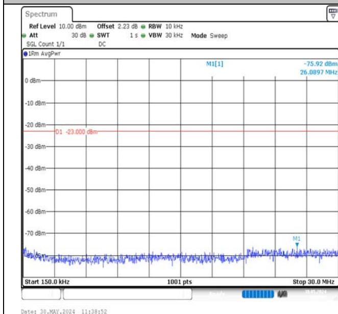
Band12-3MHz-16QAM-23025-1RB#14-0.15~30-PASS
