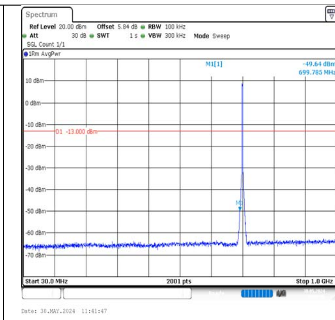
Band12-3MHz-16QAM-23095-15RB#0-30~1000-PASS
