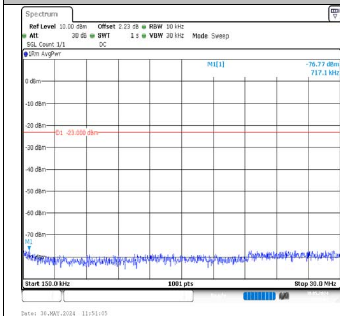
Band12-5MHz-16QAM-23035-1RB#0-0.15~30-PASS
