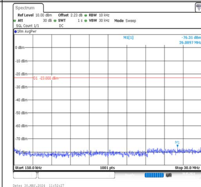
Band12-5MHz-16QAM-23035-25RB#0-0.15~30-PASS
