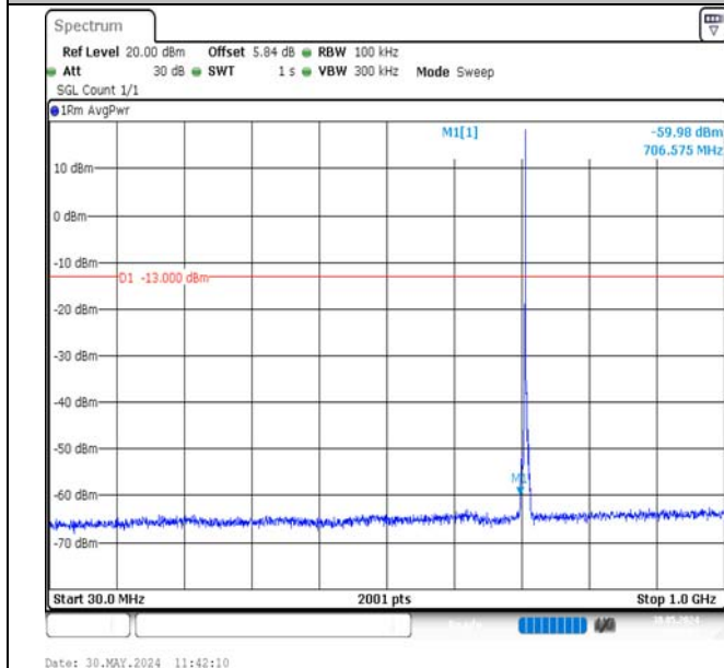
Band12-3MHz-QPSK-23165-1RB#0-30~1000-PASS
