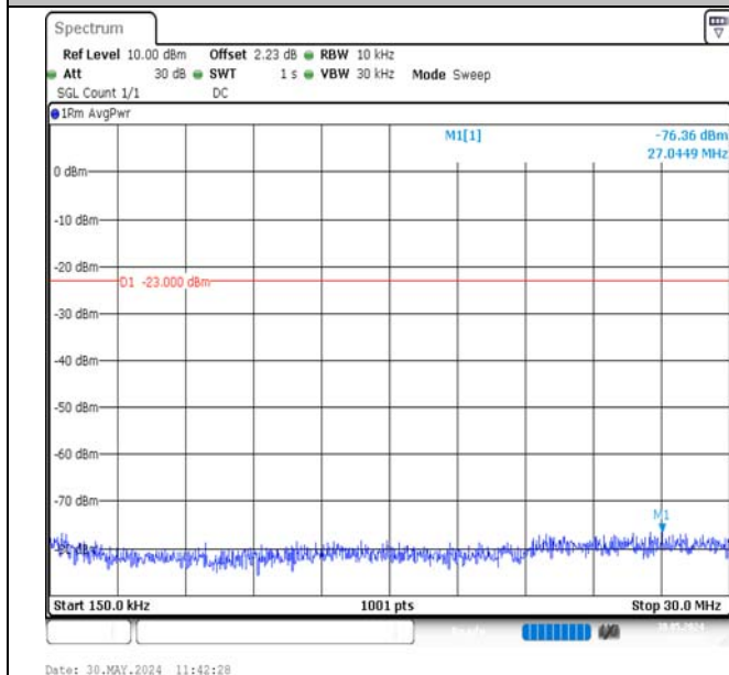
Band12-3MHz-16QAM-23165-1RB#0-0.15~30-PASS
