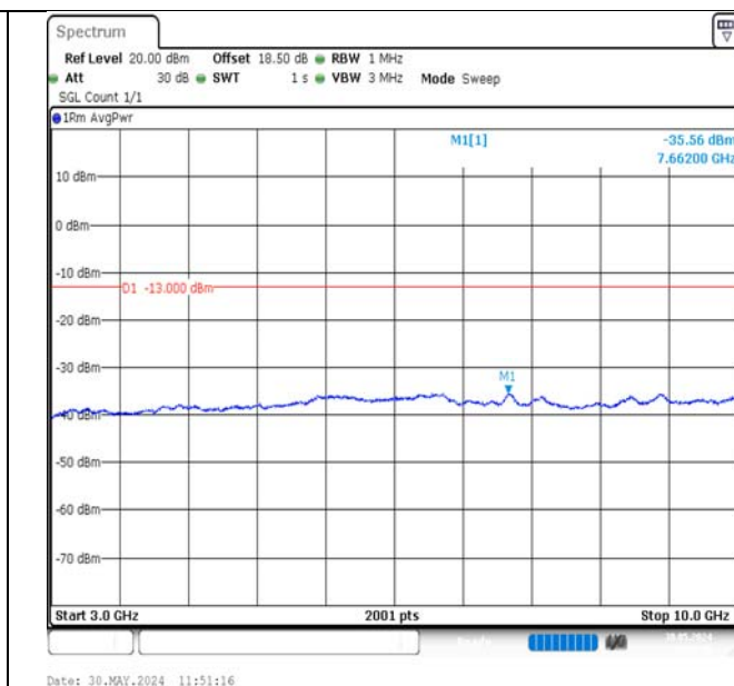
Band12-5MHz-16QAM-23035-1RB#0-3000~10000-PASS
