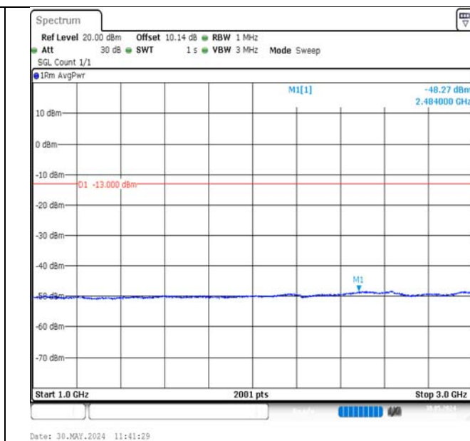
Band12-3MHz-QPSK-23095-15RB#0-1000~3000-PASS
