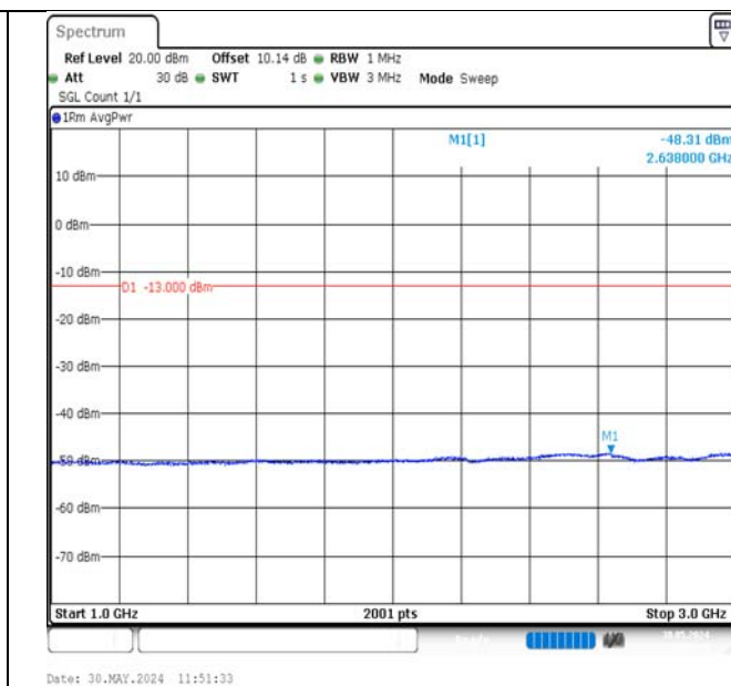
Band12-5MHz-QPSK-23035-1RB#24-1000~3000-PASS
