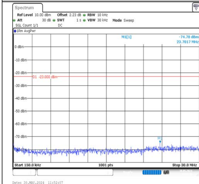
Band12-5MHz-QPSK-23035-25RB#0-0.15~30-PASS
