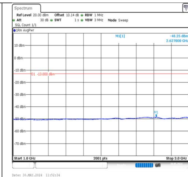
Band12-5MHz-16QAM-23035-25RB#0-1000~3000-PASS
