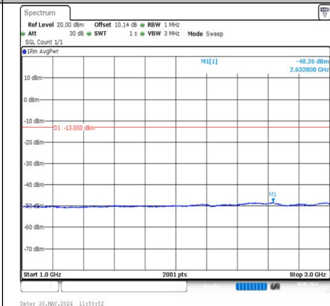
Band12-5MHz-QPSK-23035-1RB#0-1000~3000-PASS
