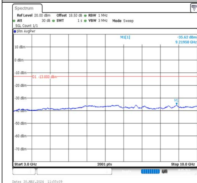
Band12-5MHz-QPSK-23155-1RB#0-3000~10000-PASS
