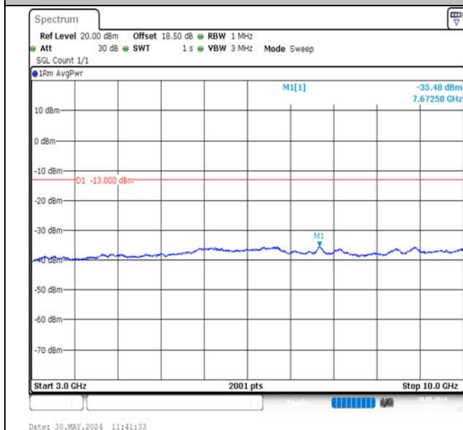
Band12-3MHz-QPSK-23095-15RB#0-3000~10000-PASS
