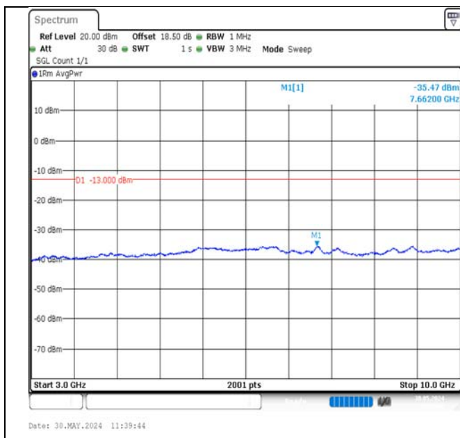
Band12-3MHz-16QAM-23025-15RB#0-3000~10000-PASS
