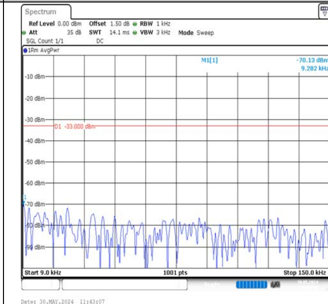
Band12-3MHz-16QAM-23165-1RB#14-0.009~0.15-PASS
