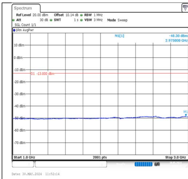
Band12-5MHz-QPSK-23035-25RB#0-1000~3000-PASS
