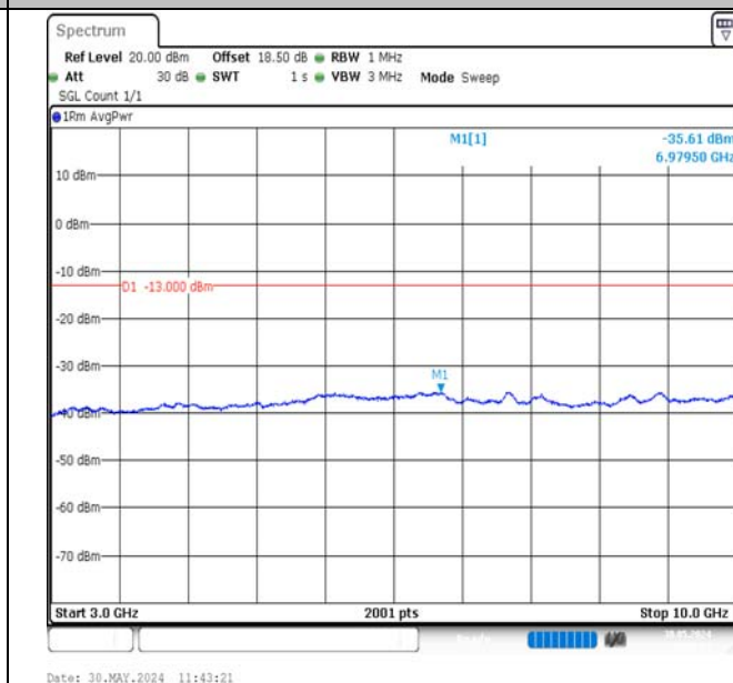
Band12-3MHz-16QAM-23165-1RB#14-3000~10000-PASS
