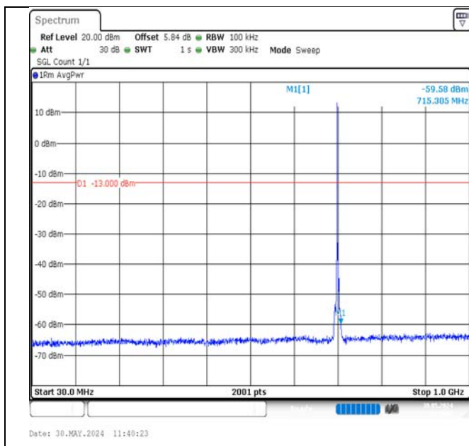
Band12-3MHz-16QAM-23095-1RB#0-30~1000-PASS
