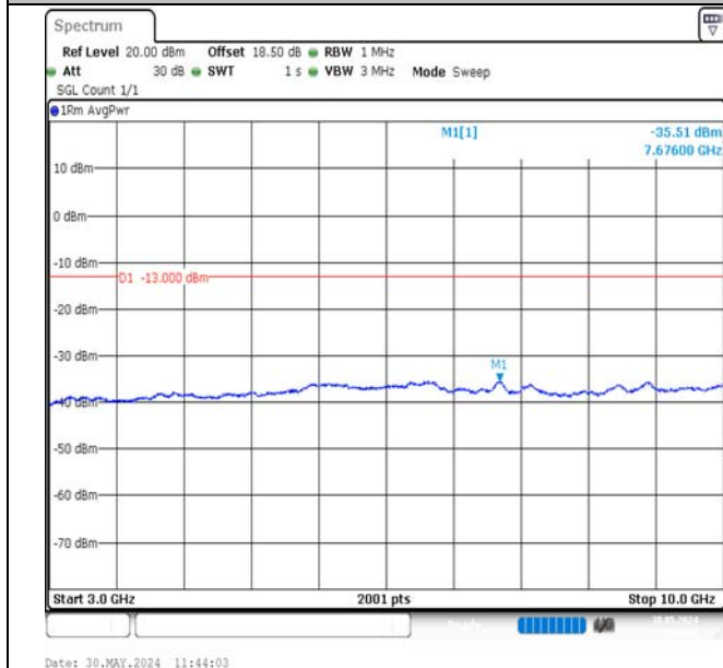
Band12-3MHz-16QAM-23165-15RB#0-3000~10000-PASS
