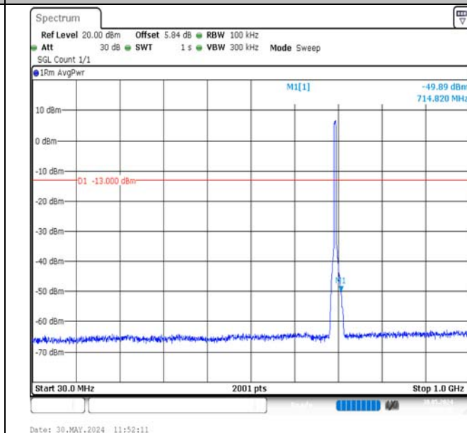
Band12-5MHz-QPSK-23035-25RB#0-30~1000-PASS
