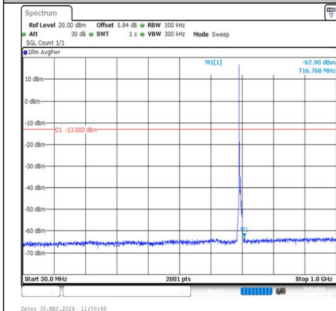
Band12-5MHz-QPSK-23035-1RB#0-30~1000-PASS
