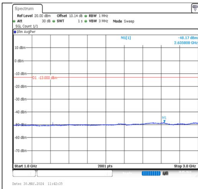
Band12-3MHz-16QAM-23165-1RB#0-1000~3000-PASS
