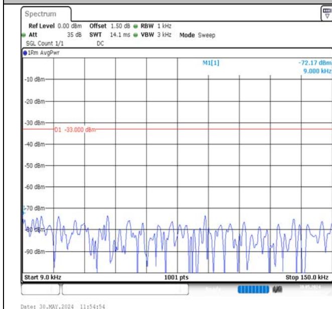
Band12-5MHz-QPSK-23155-1RB#0-0.009~0.15-PASS
