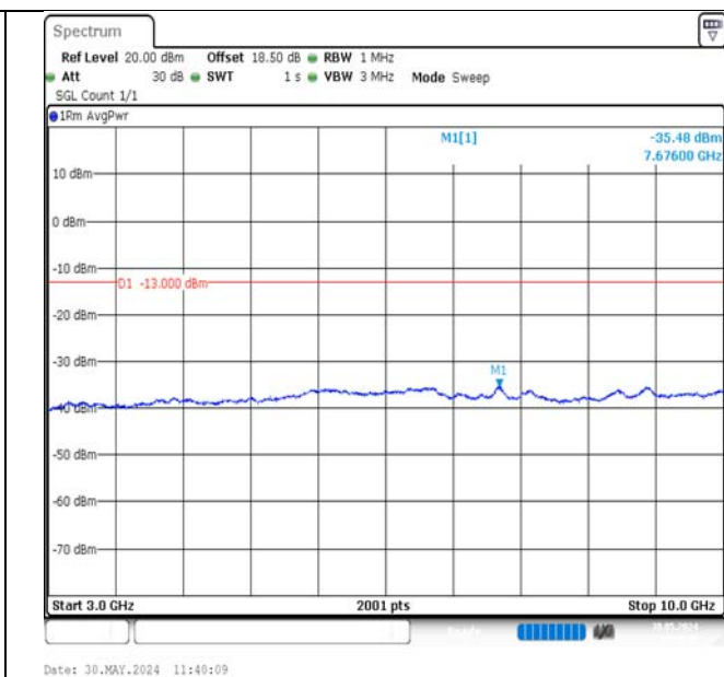
Band12-3MHz-QPSK-23095-1RB#0-3000~10000-PASS
