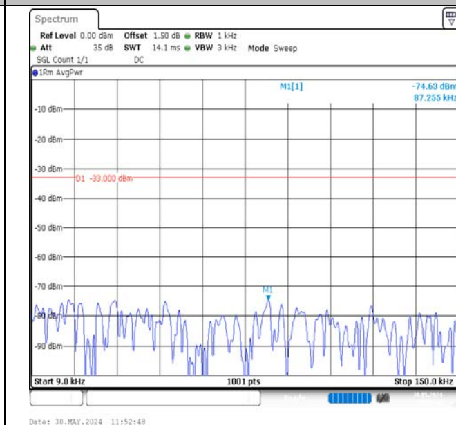
Band12-5MHz-QPSK-23095-1RB#0-0.009~0.15-PASS
