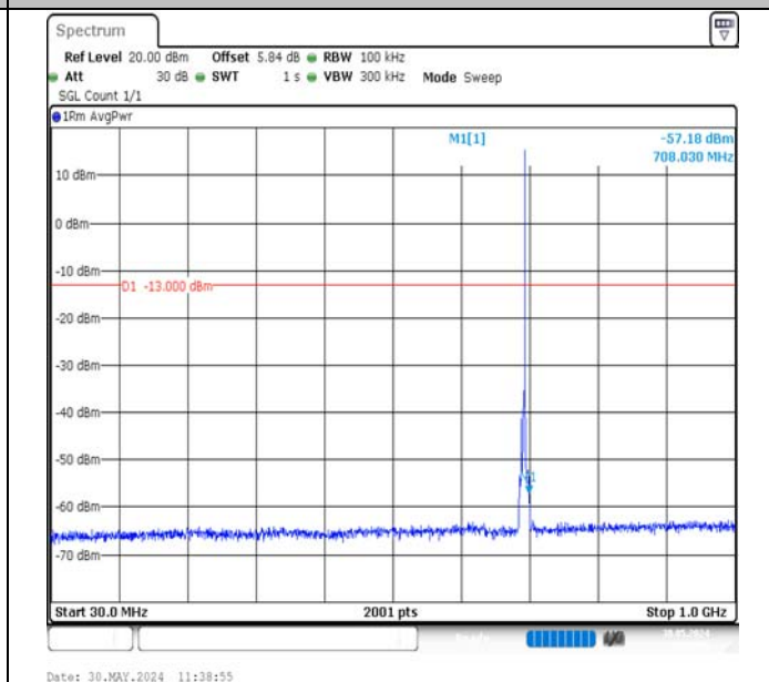
Band12-3MHz-16QAM-23025-1RB#14-30~1000-PASS
