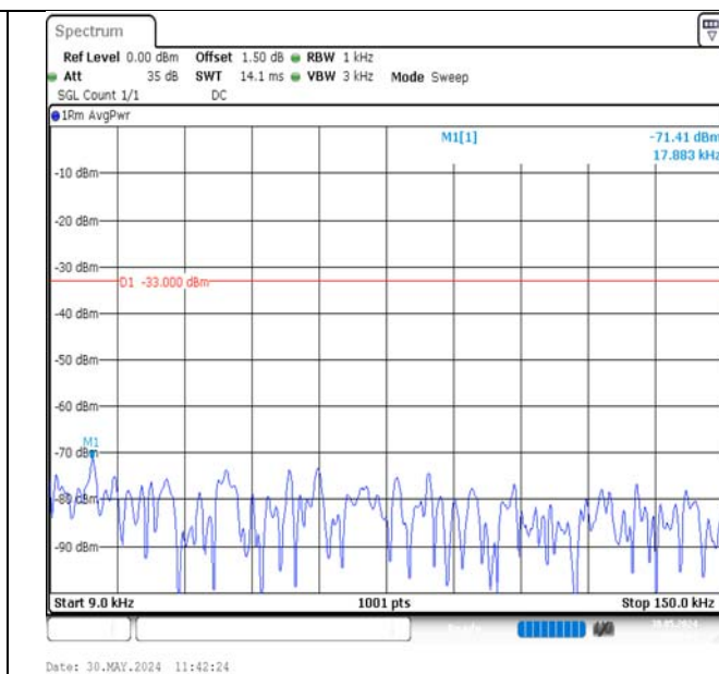
Band12-3MHz-16QAM-23165-1RB#0-0.009~0.15-PASS
