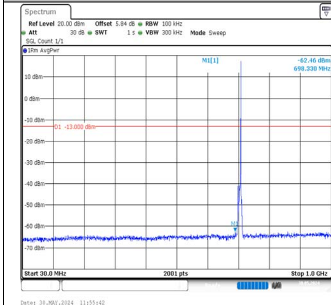
Band12-5MHz-QPSK-23155-1RB#24-30~1000-PASS
