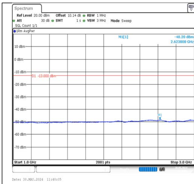
Band12-3MHz-QPSK-23095-1RB#0-1000~3000-PASS
