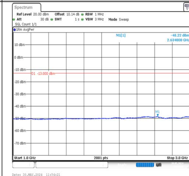
Band12-5MHz-QPSK-23095-25RB#0-1000~3000-PASS
