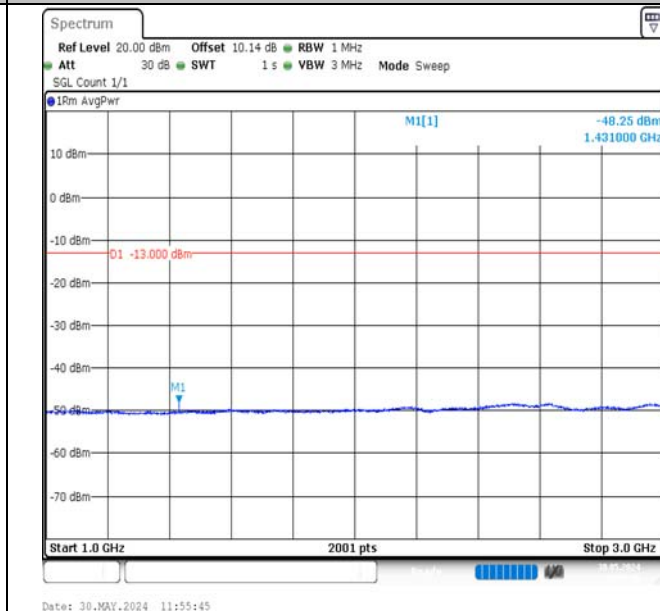
Band12-5MHz-QPSK-23155-1RB#24-1000~3000-PASS
