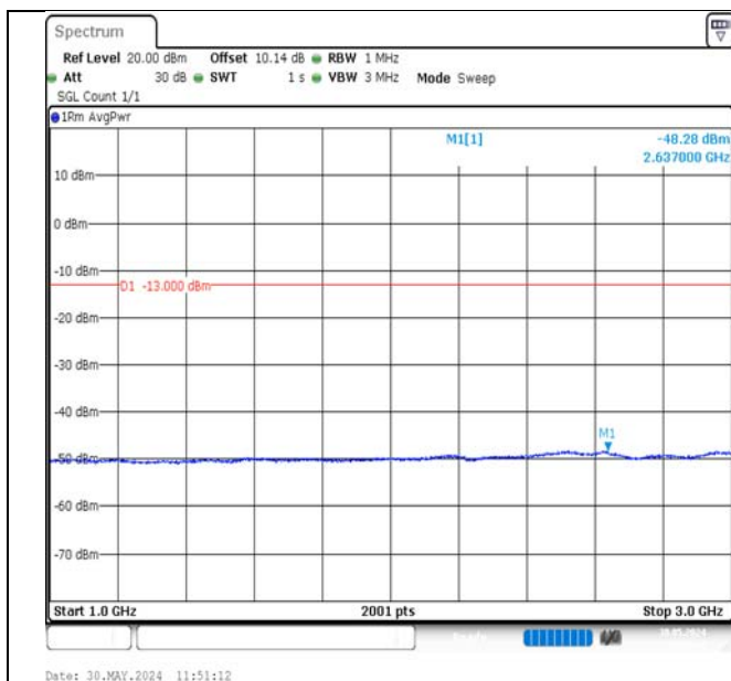
Band12-5MHz-16QAM-23035-1RB#0-1000~3000-PASS
