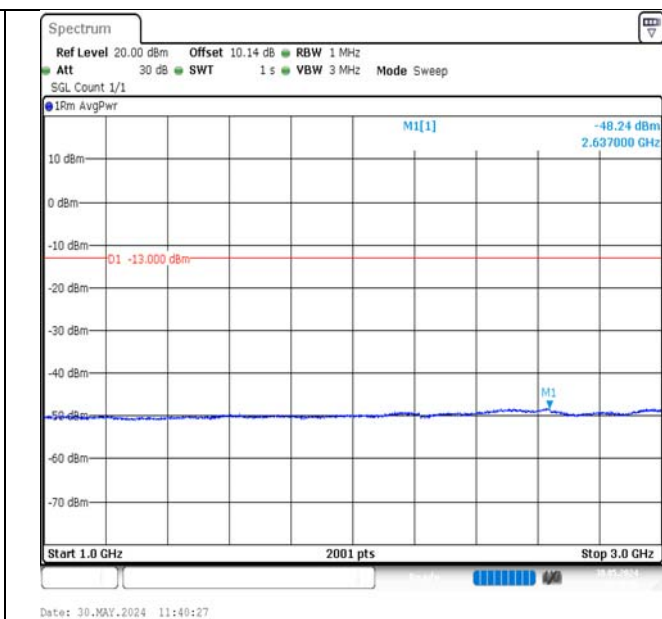
Band12-3MHz-16QAM-23095-1RB#0-1000~3000-PASS
