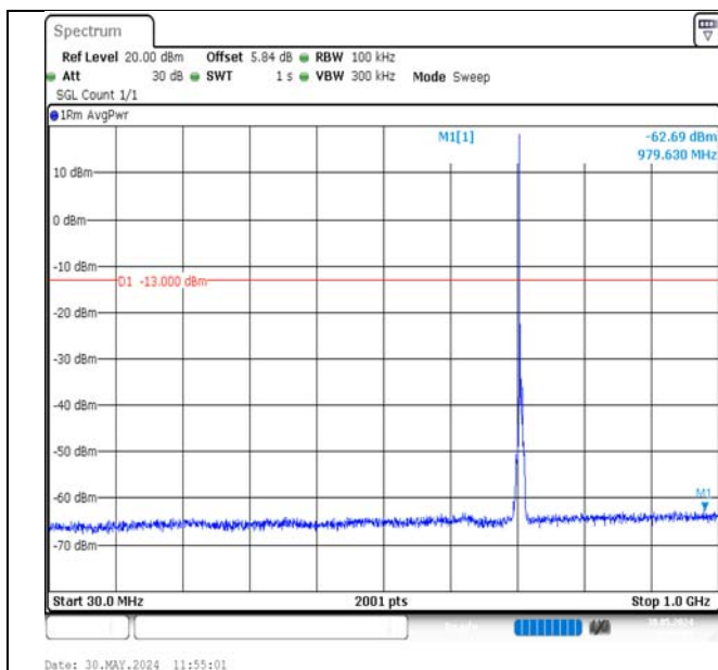
Band12-5MHz-QPSK-23155-1RB#0-30~1000-PASS
