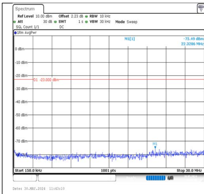
Band12-3MHz-16QAM-23165-1RB#14-0.15~30-PASS
