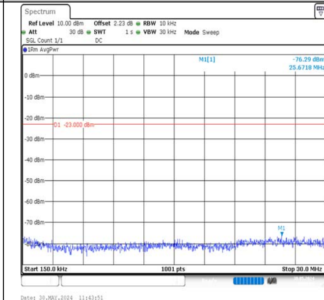
Band12-3MHz-16QAM-23165-15RB#0-0.15~30-PASS
