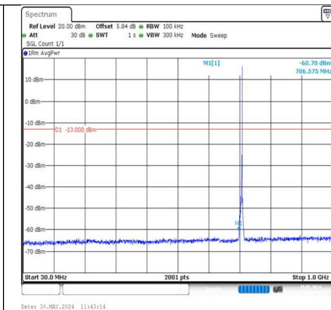
Band12-3MHz-16QAM-23165-1RB#14-30~1000-PASS
