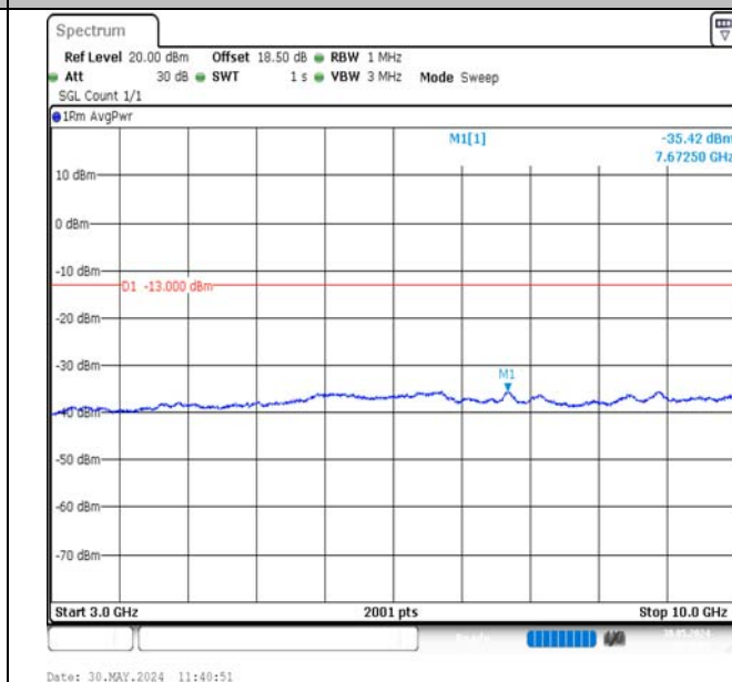
Band12-3MHz-QPSK-23095-1RB#14-3000~10000-PASS
