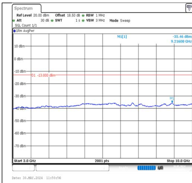
Band12-5MHz-QPSK-23035-1RB#0-3000~10000-PASS
