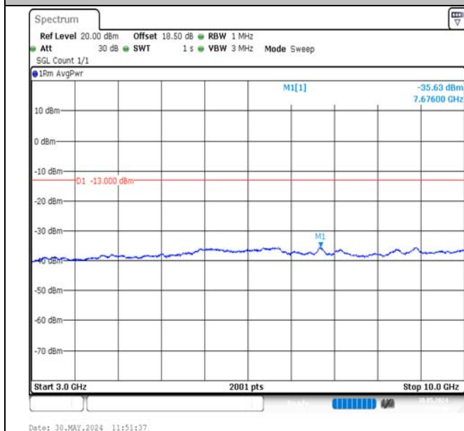
Band12-5MHz-QPSK-23035-1RB#24-3000~10000-PASS
