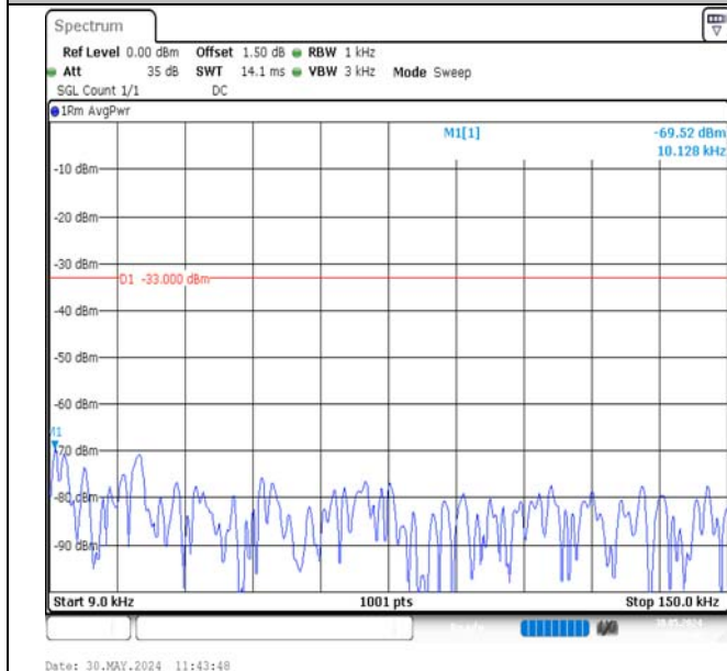
Band12-3MHz-16QAM-23165-15RB#0-0.009~0.15-PASS
