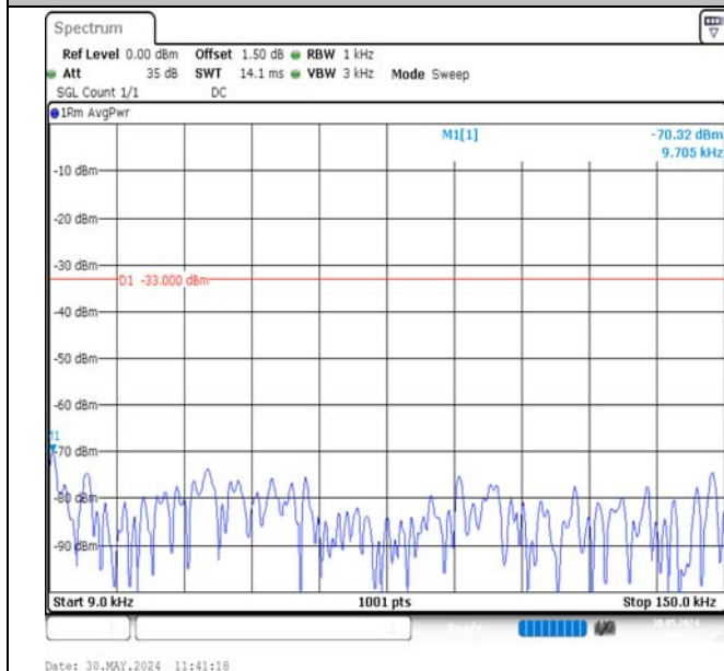
Band12-3MHz-QPSK-23095-15RB#0-0.009~0.15-PASS
