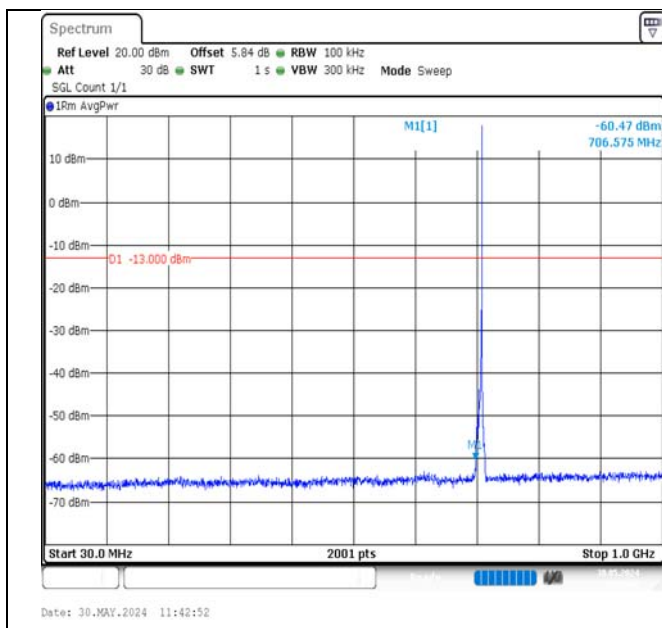
Band12-3MHz-QPSK-23165-1RB#14-30~1000-PASS
