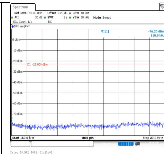
Band12-3MHz-16QAM-23095-1RB#14-0.15~30-PASS
