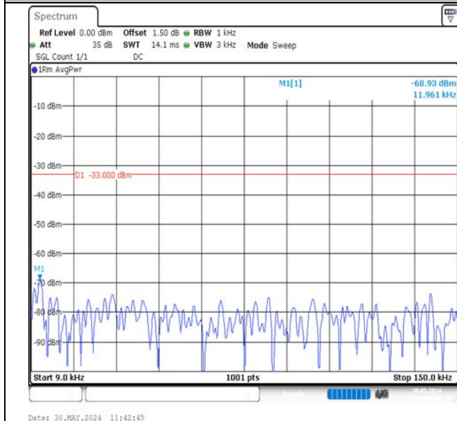
Band12-3MHz-QPSK-23165-1RB#14-0.009~0.15-PASS
