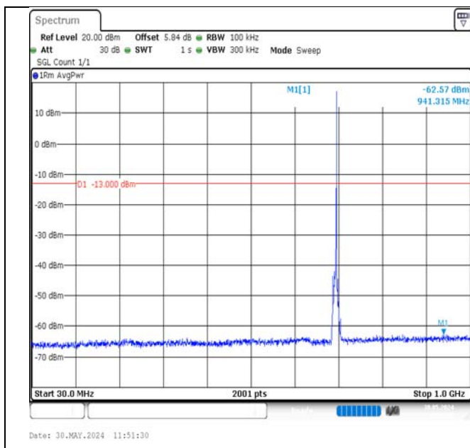
Band12-5MHz-QPSK-23035-1RB#24-30~1000-PASS
