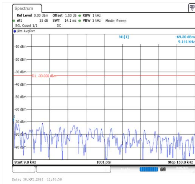
Band12-3MHz-16QAM-23095-1RB#14-0.009~0.15-PASS
