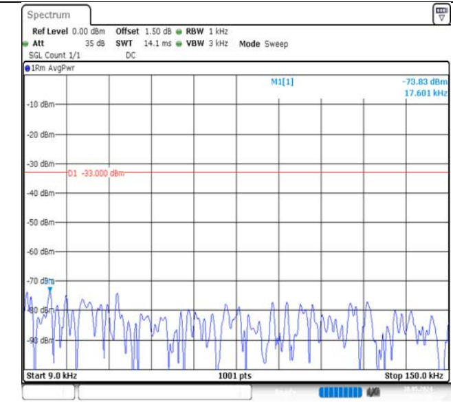
Band12-3MHz-QPSK-23165-15RB#0-0.009~0.15-PASS
