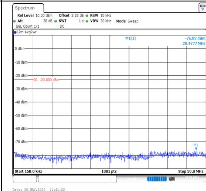
Band12-3MHz-QPSK-23095-15RB#0-0.15~30-PASS
