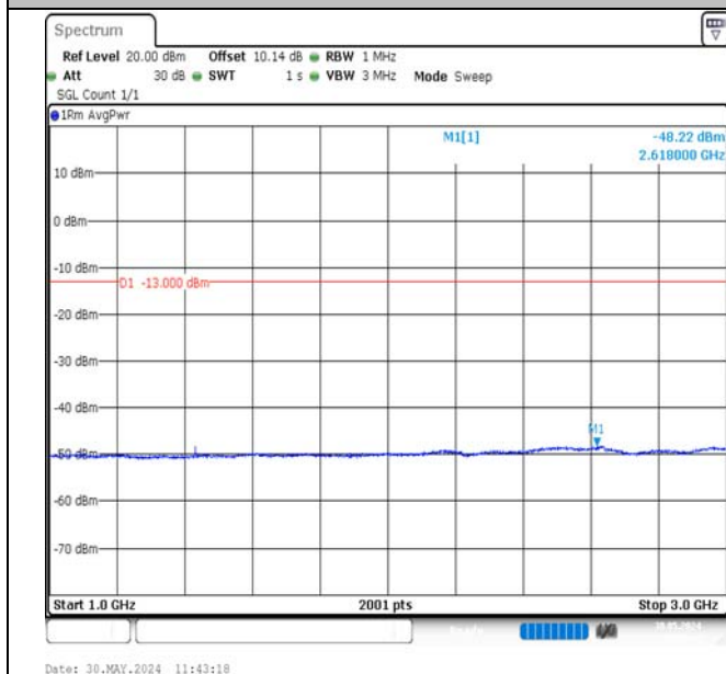
Band12-3MHz-16QAM-23165-1RB#14-1000~3000-PASS
