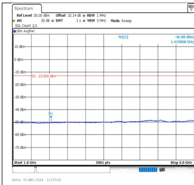
Band12-5MHz-QPSK-23095-1RB#24-1000~3000-PASS
