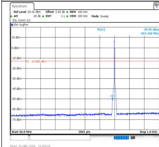
Band12-5MHz-QPSK-23095-25RB#0-30~1000-PASS
