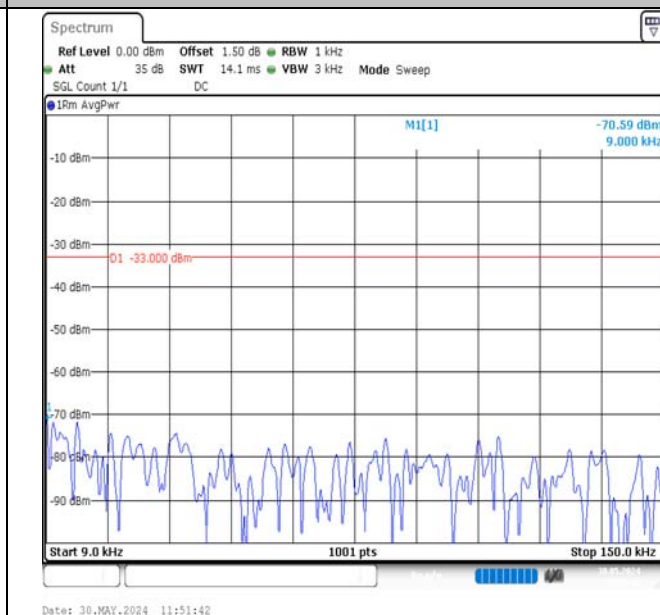
Band12-5MHz-16QAM-23035-1RB#24-0.009~0.15-PASS
