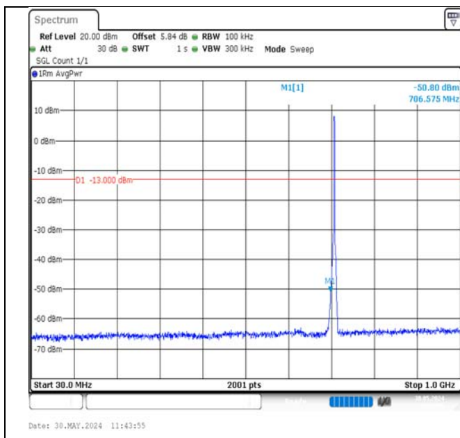
Band12-3MHz-16QAM-23165-15RB#0-30~1000-PASS
