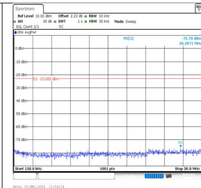
Band12-5MHz-QPSK-23095-25RB#0-0.15~30-PASS
