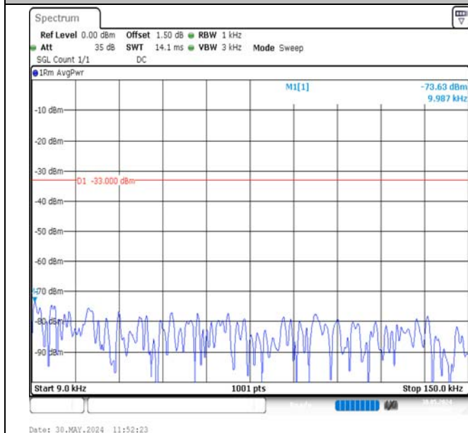
Band12-5MHz-16QAM-23035-25RB#0-0.009~0.15-PASS
