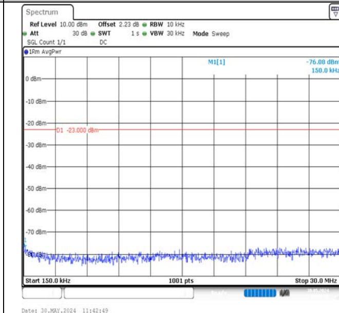
Band12-3MHz-QPSK-23165-1RB#14-0.15~30-PASS
