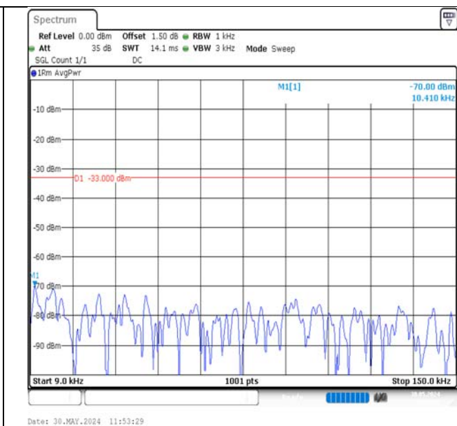
Band12-5MHz-QPSK-23095-1RB#24-0.009~0.15-PASS
