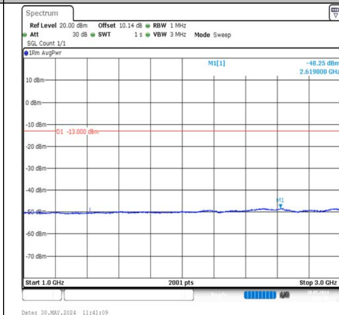
Band12-3MHz-16QAM-23095-1RB#14-1000~3000-PASS
