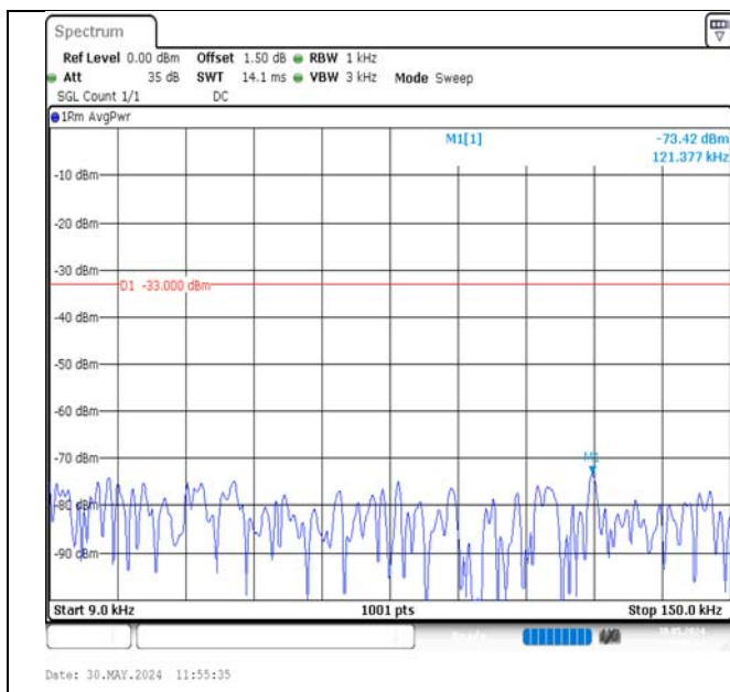
Band12-5MHz-QPSK-23155-1RB#24-0.009~0.15-PASS
