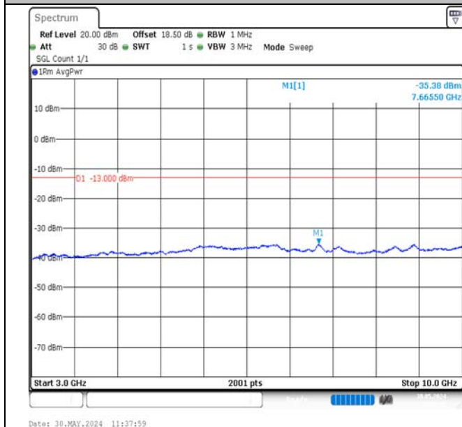
Band12-3MHz-QPSK-23025-1RB#0-3000~10000-PASS
