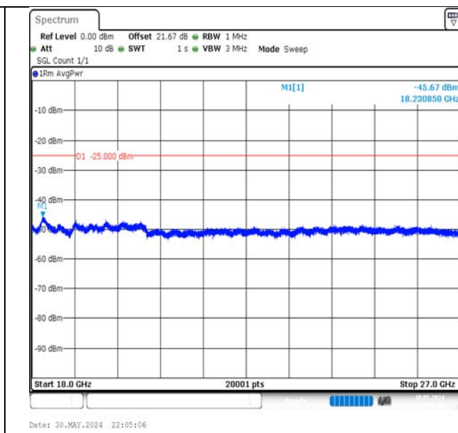
Band7-20MHz-16QAM-21350-100RB#0-18000~27000-PASS
