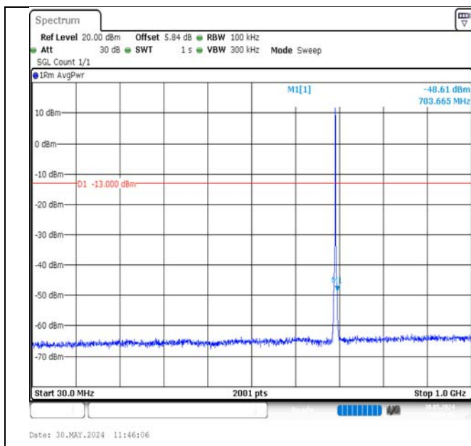
Band12-1.4MHz-16QAM-23017-6RB#0-30~1000-PASS
