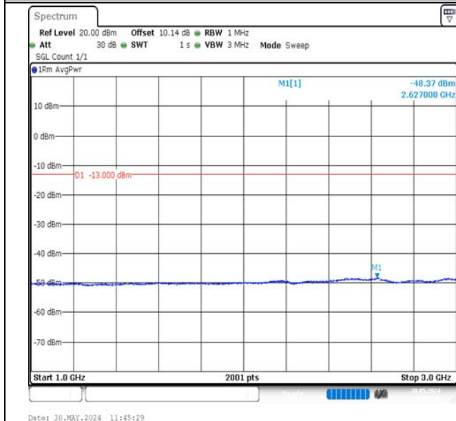
Band12-1.4MHz-16QAM-23017-1RB#5-1000~3000-PASS
