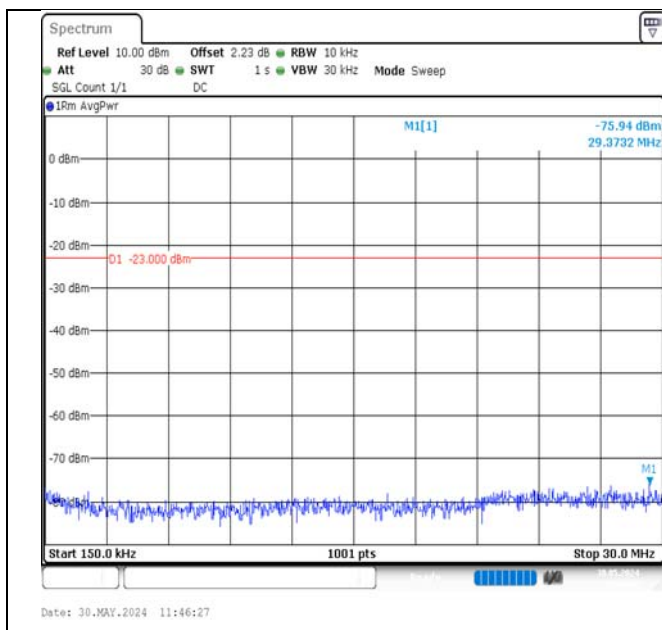
Band12-1.4MHz-QPSK-23095-1RB#0-0.15~30-PASS
