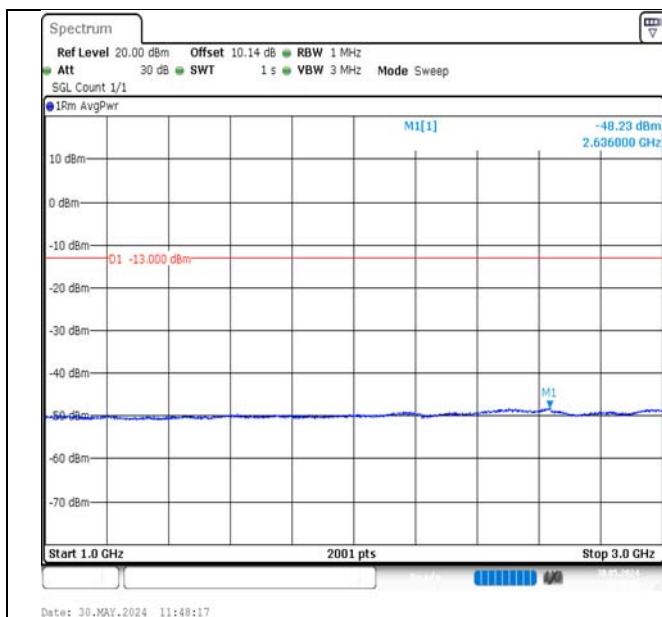
Band12-1.4MHz-16QAM-23095-6RB#0-1000~3000-PASS
