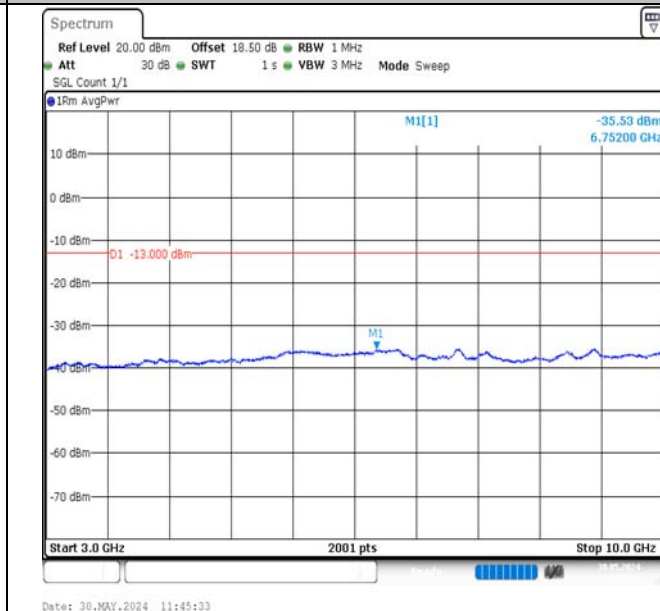
Band12-1.4MHz-16QAM-23017-1RB#5-3000~10000-PASS
