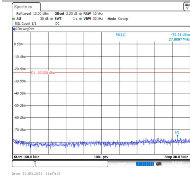
Band12-1.4MHz-QPSK-23095-1RB#5-0.15~30-PASS
