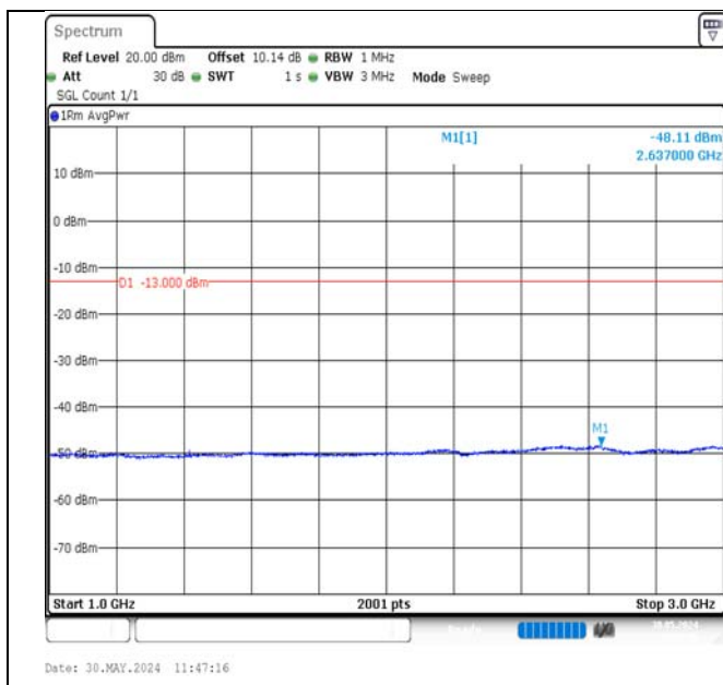
Band12-1.4MHz-QPSK-23095-1RB#5-1000~3000-PASS
