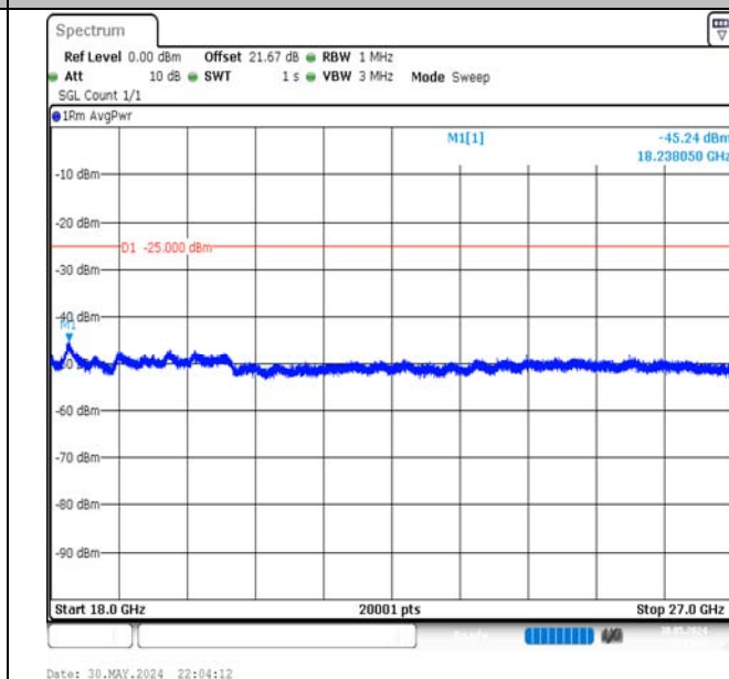
Band7-20MHz-16QAM-21350-1RB#99-18000~27000-PASS
