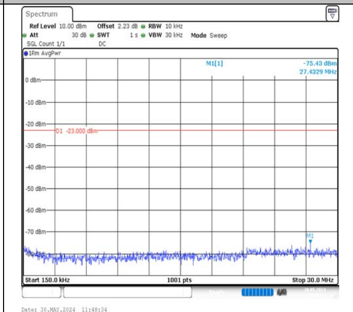
Band12-1.4MHz-QPSK-23173-1RB#0-0.15~30-PASS
