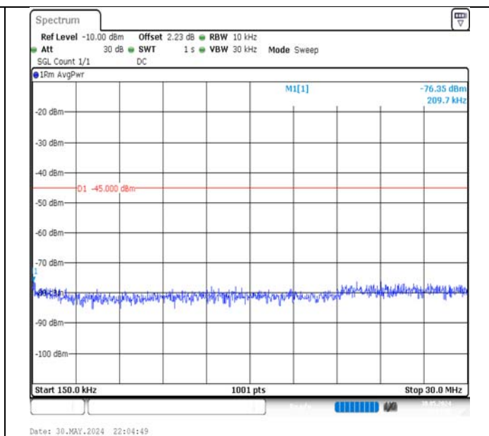
Band7-20MHz-16QAM-21350-100RB#0-0.15~30-PASS
