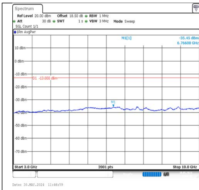
Band12-1.4MHz-16QAM-23095-1RB#0-3000~10000-PASS
