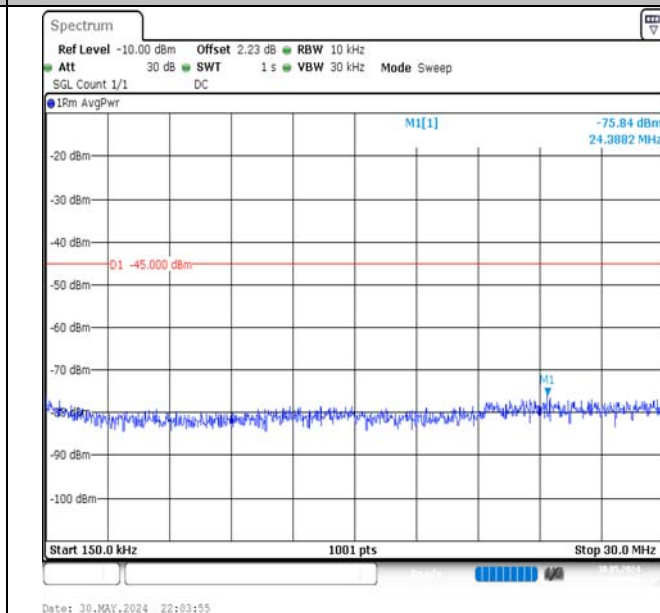
Band7-20MHz-16QAM-21350-1RB#99-0.15~30-PASS
