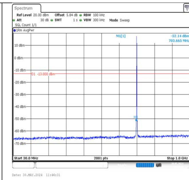
Band12-1.4MHz-QPSK-23095-1RB#0-30~1000-PASS
