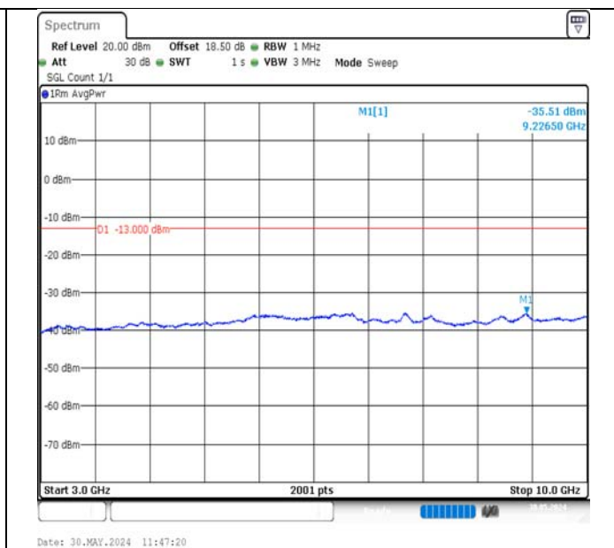
Band12-1.4MHz-QPSK-23095-1RB#5-3000~10000-PASS
