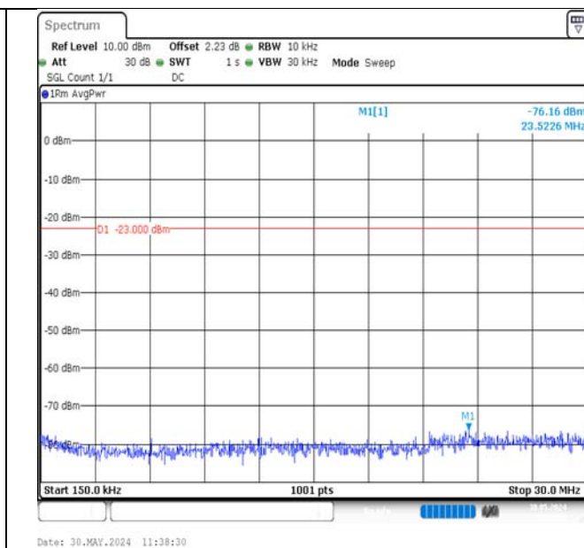
Band12-3MHz-QPSK-23025-1RB#14-0.15~30-PASS
