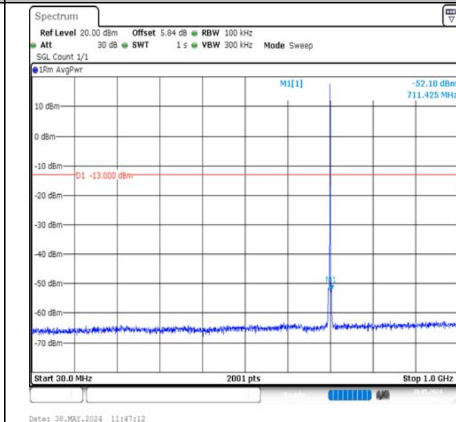
Band12-1.4MHz-QPSK-23095-1RB#5-30~1000-PASS
