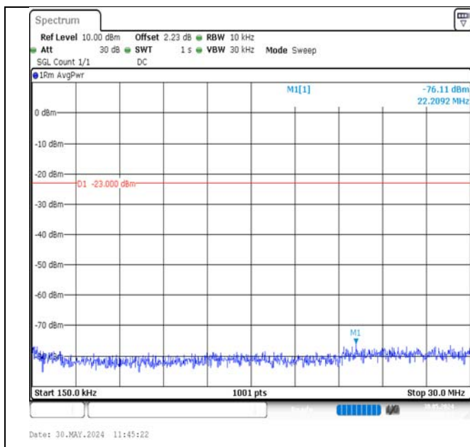
Band12-1.4MHz-16QAM-23017-1RB#5-0.15~30-PASS
