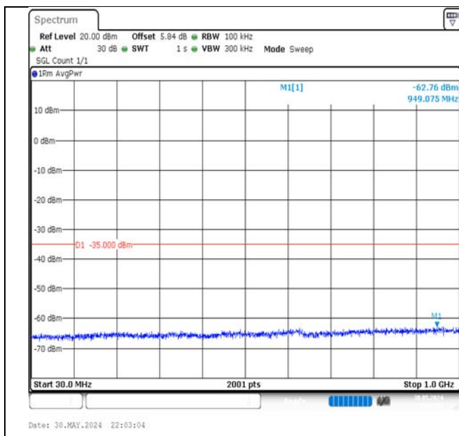
Band7-20MHz-16QAM-21350-1RB#0-30~1000-PASS
