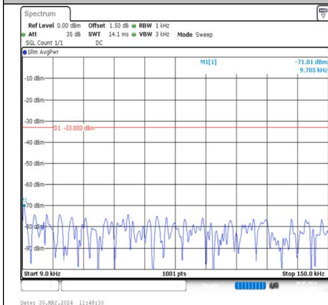
Band12-1.4MHz-QPSK-23173-1RB#0-0.009~0.15-PASS
