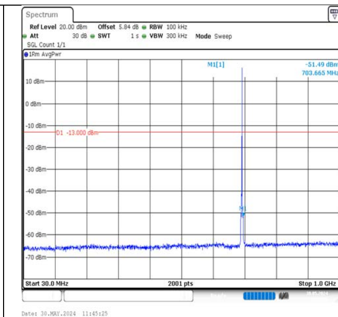
Band12-1.4MHz-16QAM-23017-1RB#5-30~1000-PASS
