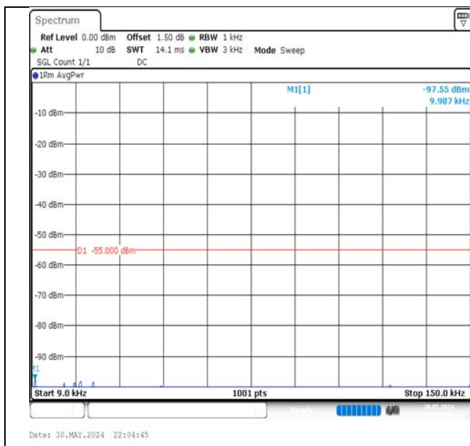
Band7-20MHz-16QAM-21350-100RB#0-0.009~0.15-PASS
