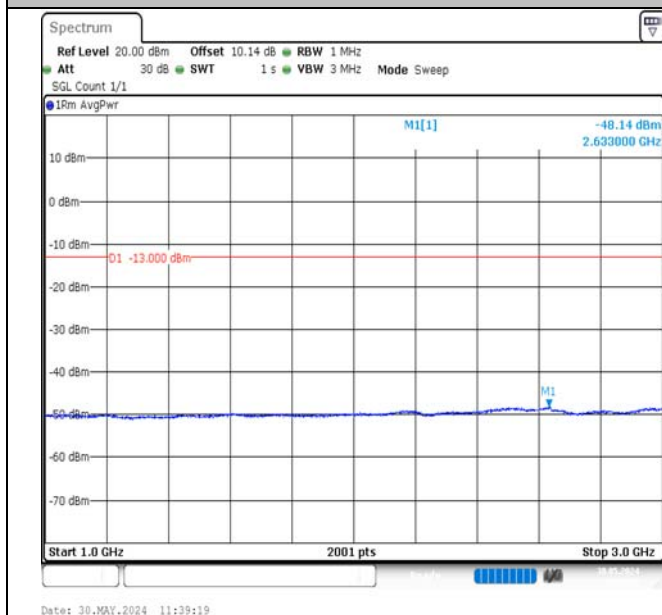
Band12-3MHz-QPSK-23025-15RB#0-1000~3000-PASS
