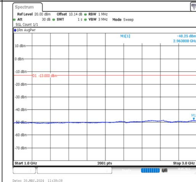
Band12-3MHz-QPSK-23025-1RB#14-1000~3000-PASS
