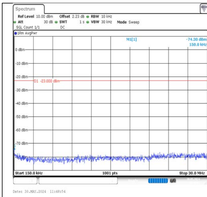
Band12-1.4MHz-16QAM-23173-1RB#0-0.15~30-PASS
