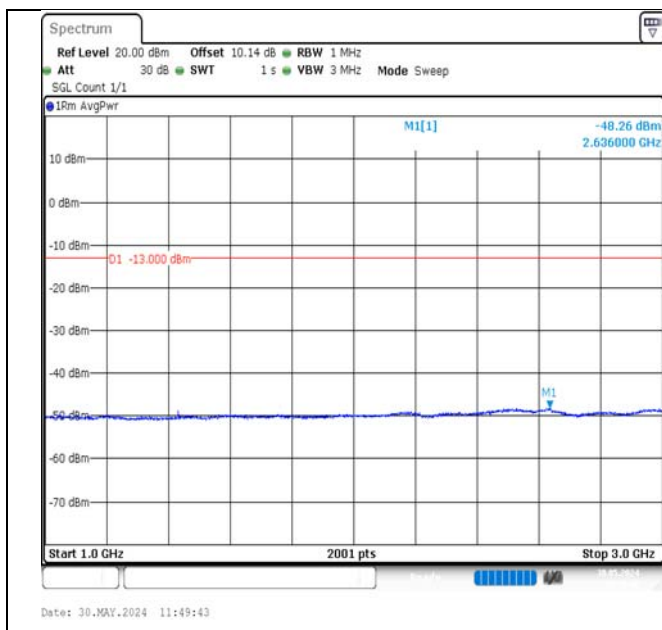
Band12-1.4MHz-16QAM-23173-1RB#5-1000~3000-PASS
