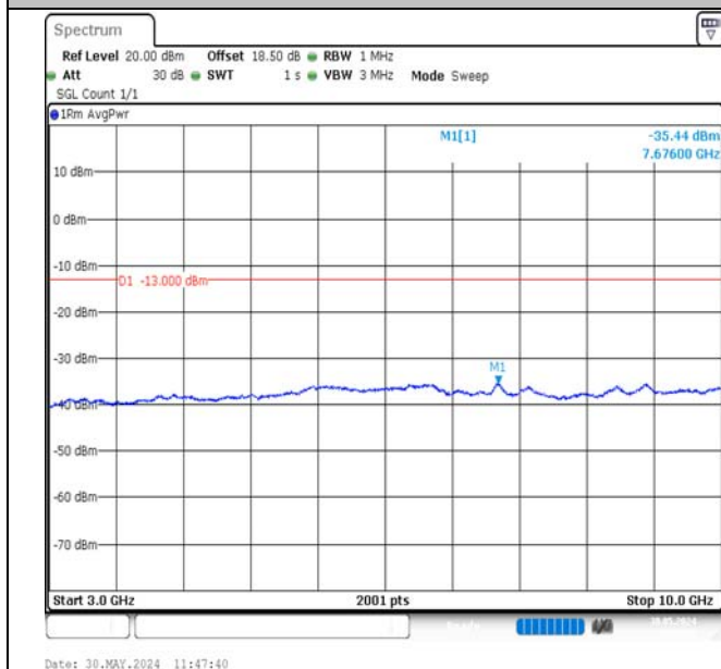
Band12-1.4MHz-16QAM-23095-1RB#5-3000~10000-PASS
