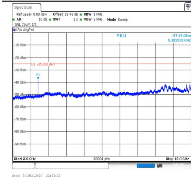
Band7-20MHz-16QAM-21350-1RB#0-3000~18000-PASS
