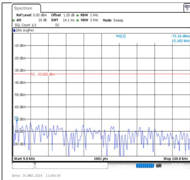
Band12-1.4MHz-QPSK-23017-1RB#0-0.009~0.15-PASS
