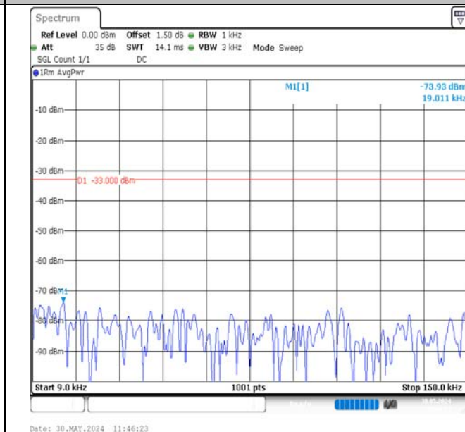
Band12-1.4MHz-QPSK-23095-1RB#0-0.009~0.15-PASS
