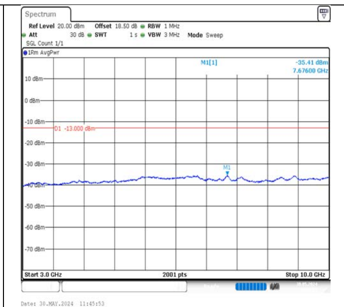
Band12-1.4MHz-QPSK-23017-6RB#0-3000~10000-PASS
