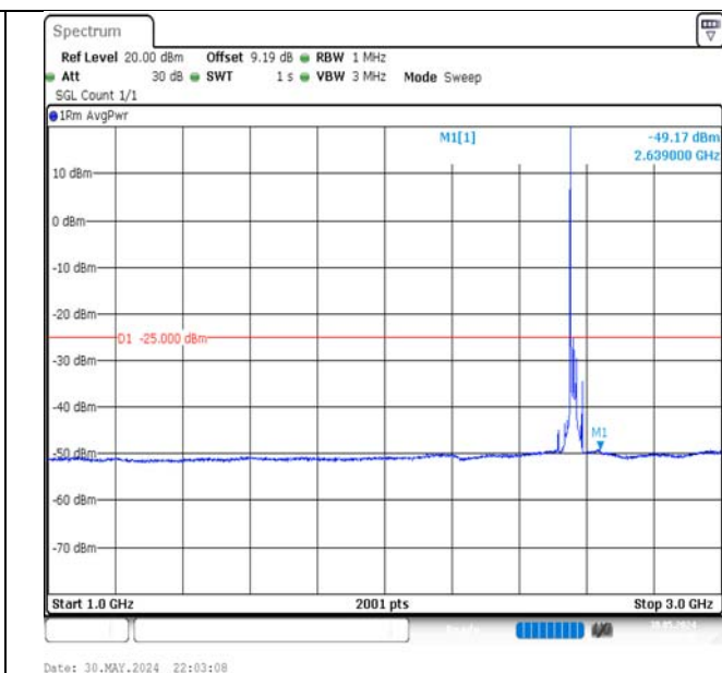
Band7-20MHz-16QAM-21350-1RB#0-1000~3000-PASS
