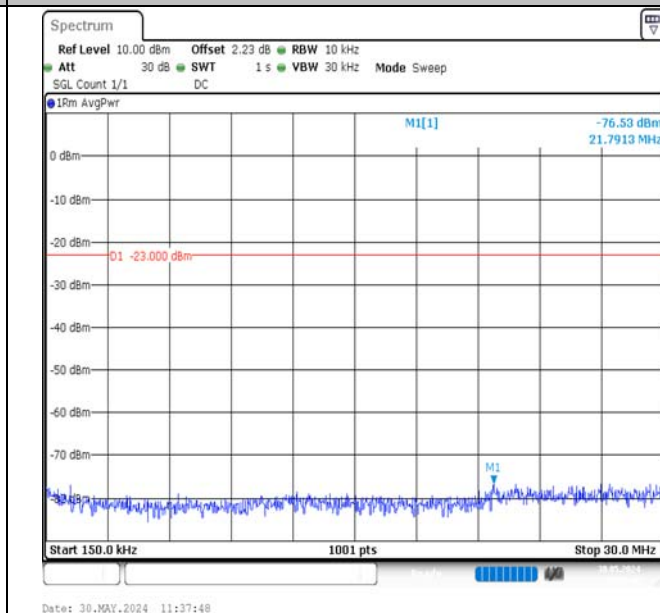
Band12-3MHz-QPSK-23025-1RB#0-0.15~30-PASS
