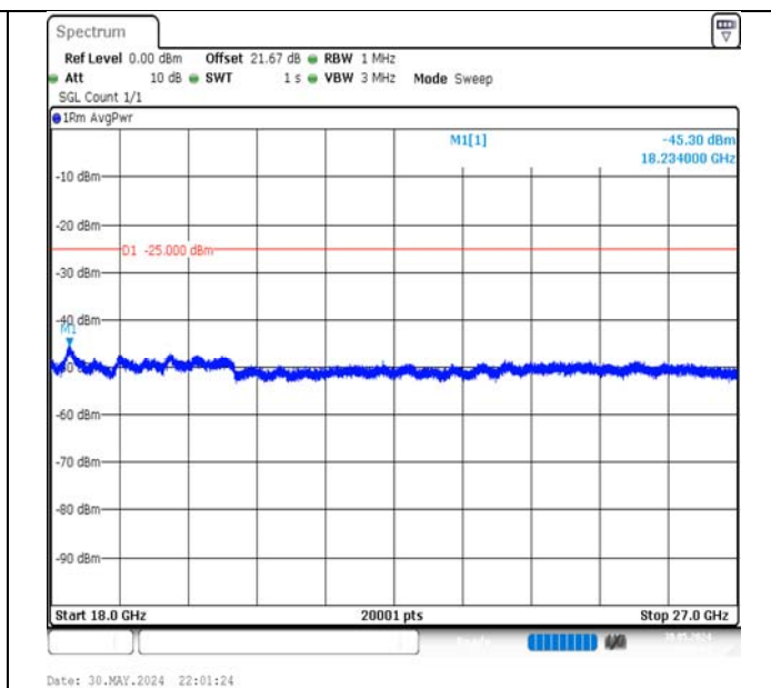
Band7-20MHz-16QAM-21100-1RB#99-18000~27000-PASS
