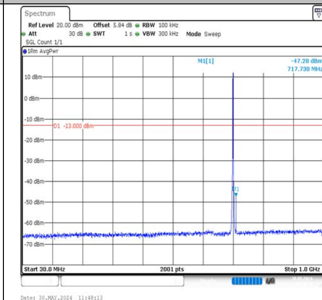
Band12-1.4MHz-16QAM-23095-6RB#0-30~1000-PASS
