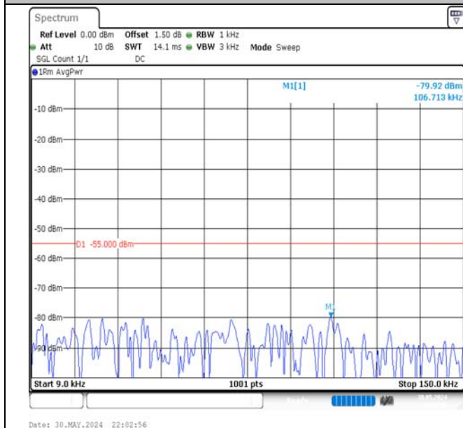
Band7-20MHz-16QAM-21350-1RB#0-0.009~0.15-PASS
