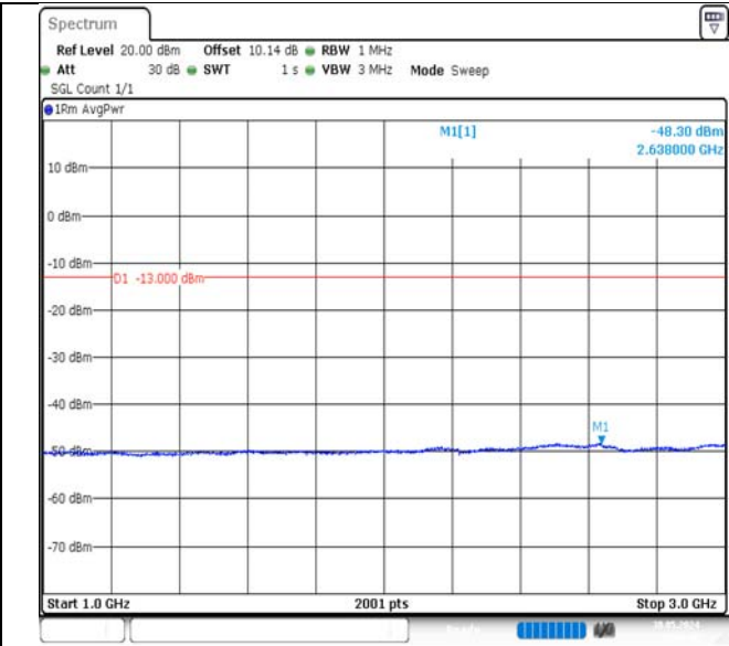
Band12-1.4MHz-16QAM-23017-1RB#0-1000~3000-PASS
