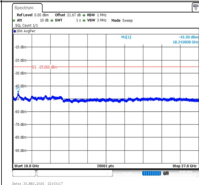
Band7-20MHz-16QAM-21350-1RB#0-18000~27000-PASS
