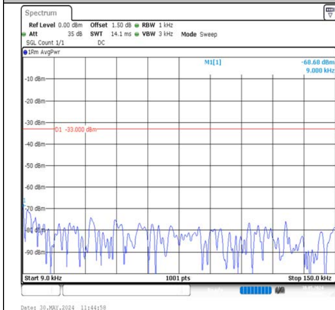
Band12-1.4MHz-QPSK-23017-1RB#5-0.009~0.15-PASS
