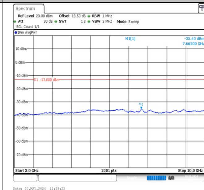
Band12-3MHz-QPSK-23025-15RB#0-3000~10000-PASS
