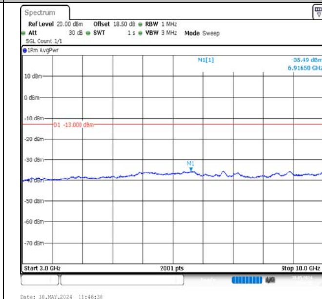
Band12-1.4MHz-QPSK-23095-1RB#0-3000~10000-PASS
