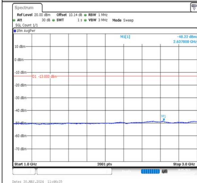
Band12-1.4MHz-QPSK-23095-1RB#0-1000~3000-PASS
