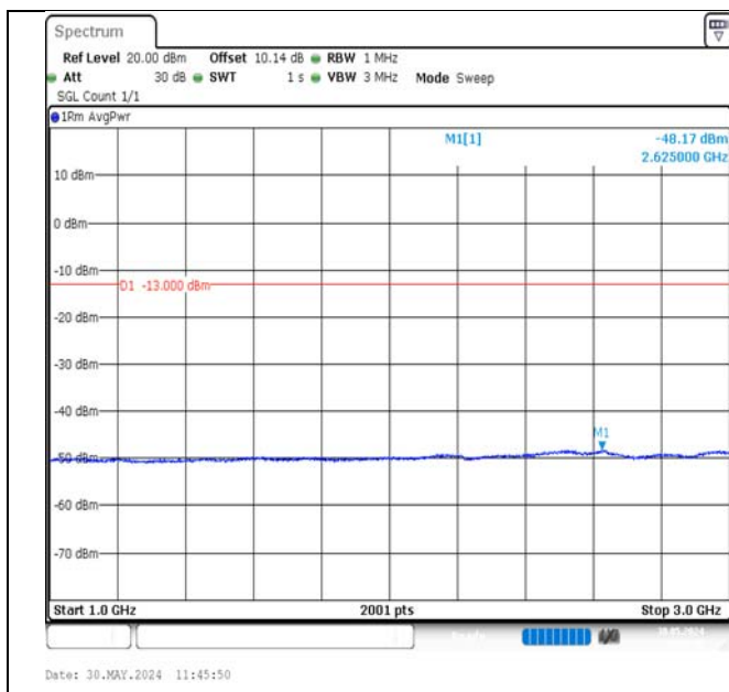
Band12-1.4MHz-QPSK-23017-6RB#0-1000~3000-PASS
