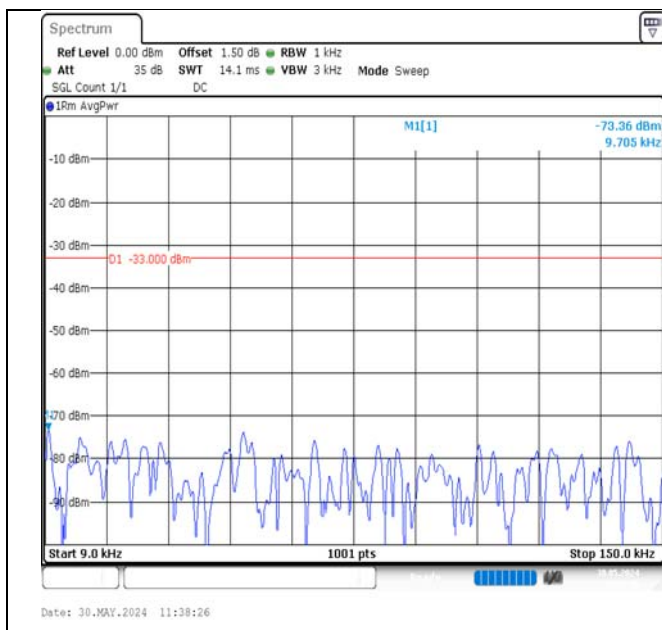
Band12-3MHz-QPSK-23025-1RB#14-0.009~0.15-PASS
