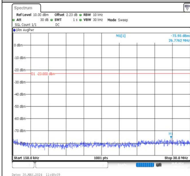
Band12-1.4MHz-16QAM-23095-6RB#0-0.15~30-PASS
