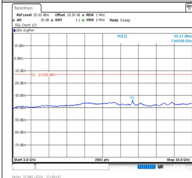
Band12-1.4MHz-QPSK-23173-1RB#0-3000~10000-PASS
