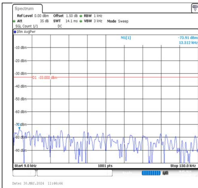
Band12-1.4MHz-16QAM-23095-1RB#0-0.009~0.15-PASS
