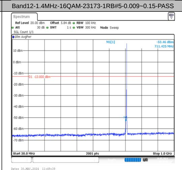
Band12-1.4MHz-16QAM-23173-1RB#5-30~1000-PASS
