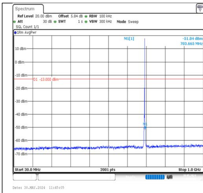
Band12-1.4MHz-QPSK-23017-1RB#5-30~1000-PASS
