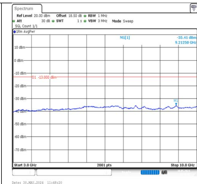
Band12-1.4MHz-16QAM-23095-6RB#0-3000~10000-PASS
