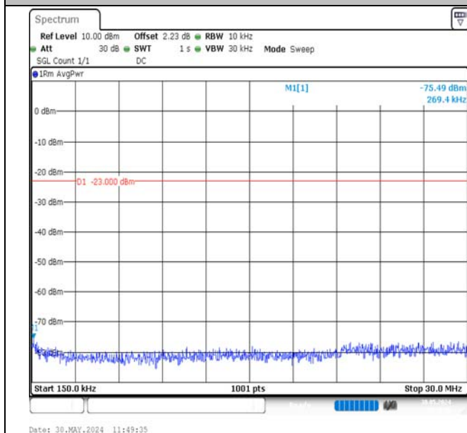
Band12-1.4MHz-16QAM-23173-1RB#5-0.15~30-PASS
