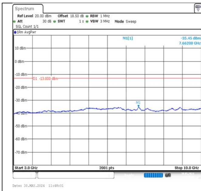
Band12-1.4MHz-QPSK-23095-6RB#0-3000~10000-PASS
