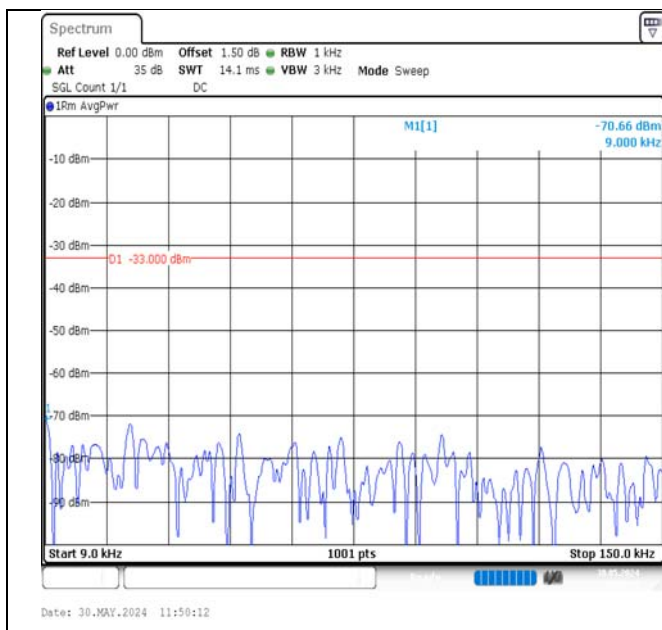
Band12-1.4MHz-16QAM-23173-6RB#0-0.009~0.15-PASS
