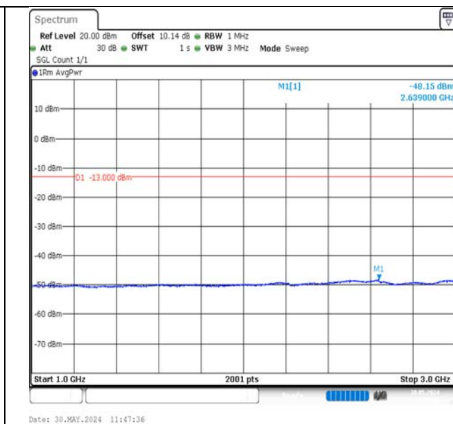
Band12-1.4MHz-16QAM-23095-1RB#5-1000~3000-PASS
