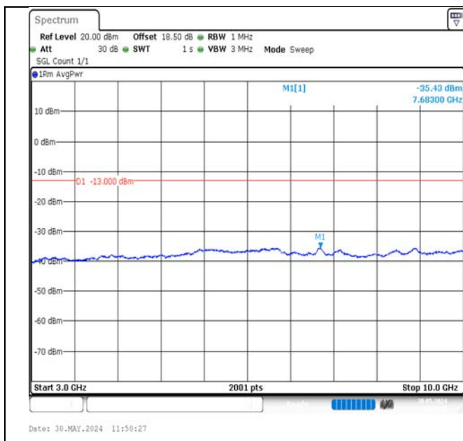
Band12-1.4MHz-16QAM-23173-6RB#0-3000~10000-PASS
