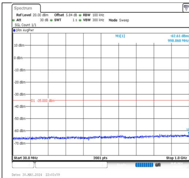
Band7-20MHz-16QAM-21350-1RB#99-30~1000-PASS
