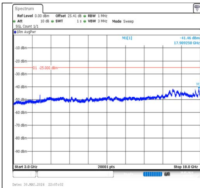
Band7-20MHz-16QAM-21350-100RB#0-3000~18000-PASS
