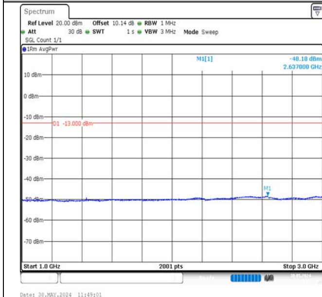
Band12-1.4MHz-16QAM-23173-1RB#0-1000~3000-PASS
