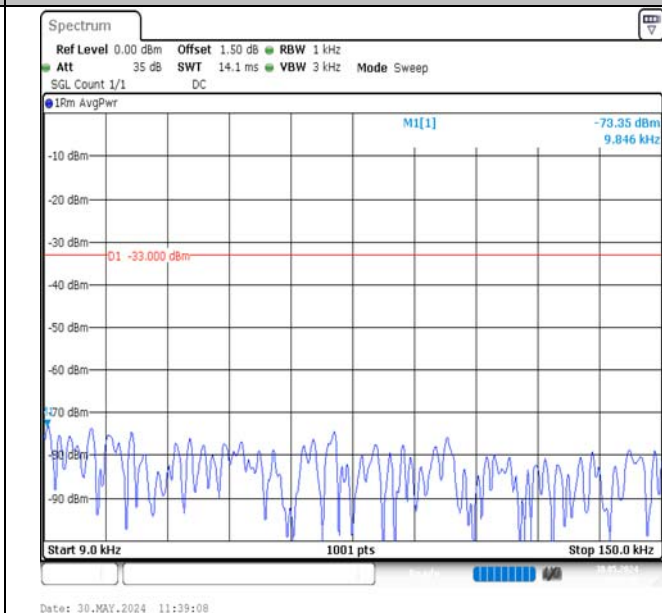
Band12-3MHz-QPSK-23025-15RB#0-0.009~0.15-PASS
