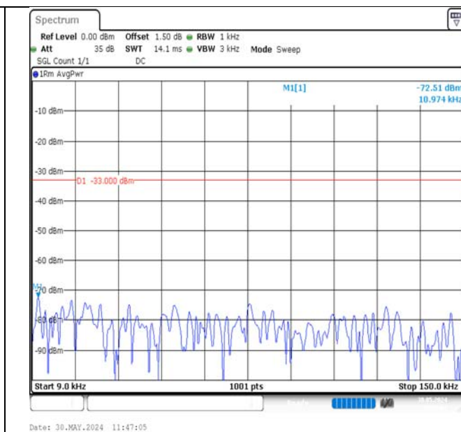
Band12-1.4MHz-QPSK-23095-1RB#5-0.009~0.15-PASS
