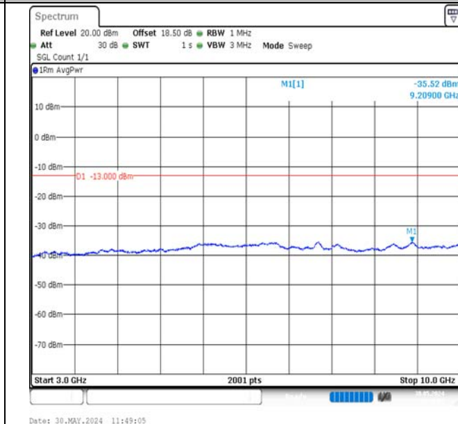
Band12-1.4MHz-16QAM-23173-1RB#0-3000~10000-PASS
