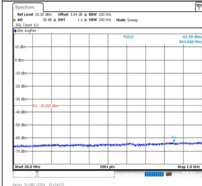
Band7-20MHz-16QAM-21350-100RB#0-30~1000-PASS
