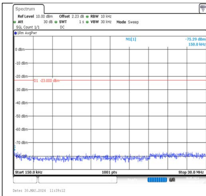
Band12-3MHz-QPSK-23025-15RB#0-0.15~30-PASS
