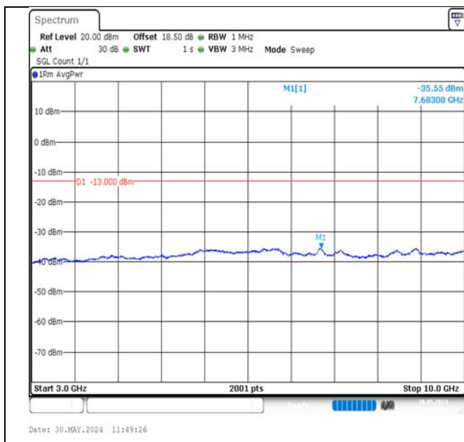
Band12-1.4MHz-QPSK-23173-1RB#5-3000~10000-PASS
