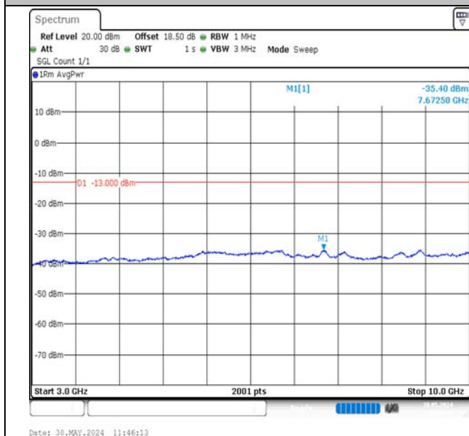
Band12-1.4MHz-16QAM-23017-6RB#0-3000~10000-PASS
