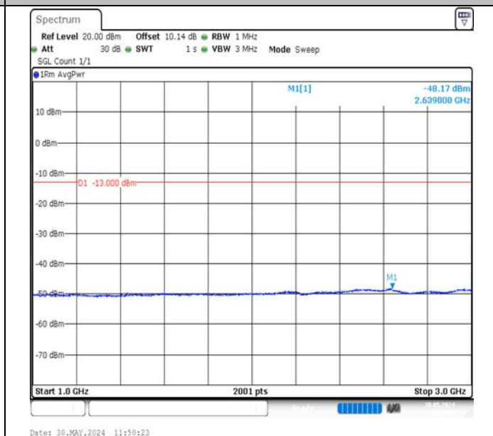
Band12-1.4MHz-16QAM-23173-6RB#0-1000~3000-PASS
