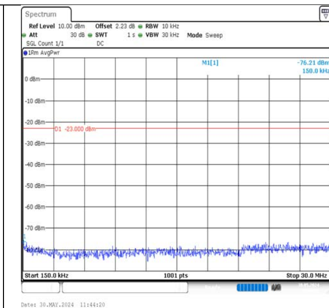
Band12-1.4MHz-QPSK-23017-1RB#0-0.15~30-PASS
