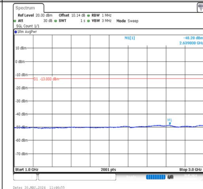
Band12-1.4MHz-16QAM-23095-1RB#0-1000~3000-PASS
