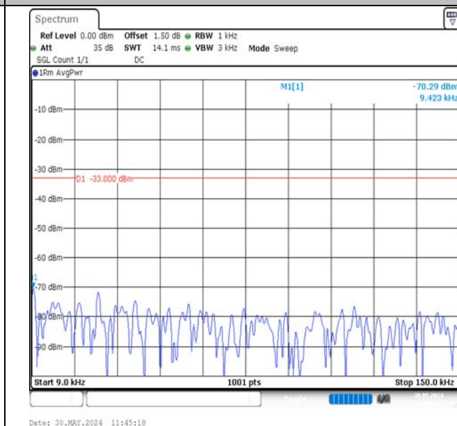
Band12-1.4MHz-16QAM-23017-1RB#5-0.009~0.15-PASS
