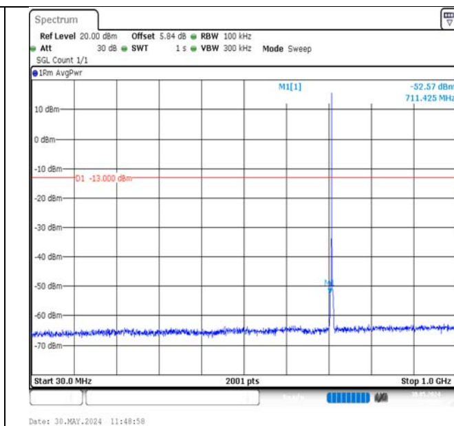
Band12-1.4MHz-16QAM-23173-1RB#0-30~1000-PASS
