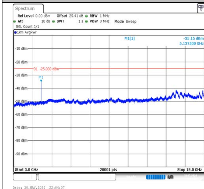
Band7-20MHz-16QAM-21350-1RB#99-3000~18000-PASS
