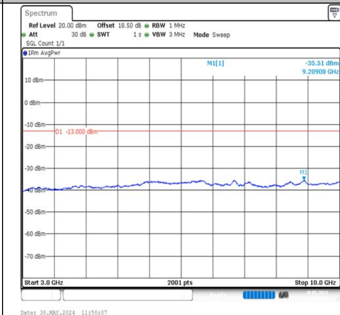
Band12-1.4MHz-QPSK-23173-6RB#0-3000~10000-PASS
