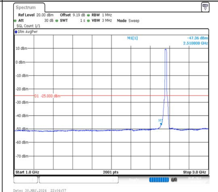
Band7-20MHz-16QAM-21350-100RB#0-1000~3000-PASS
