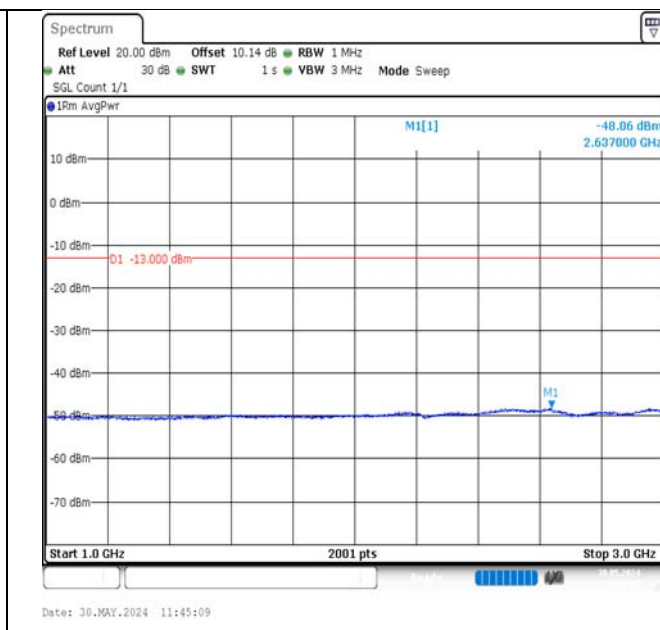
Band12-1.4MHz-QPSK-23017-1RB#5-1000~3000-PASS
