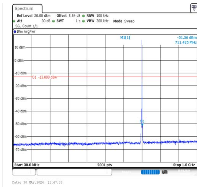
Band12-1.4MHz-16QAM-23095-1RB#5-30~1000-PASS
