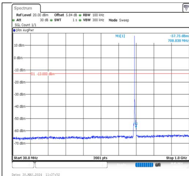
Band12-3MHz-QPSK-23025-1RB#0-30~1000-PASS
