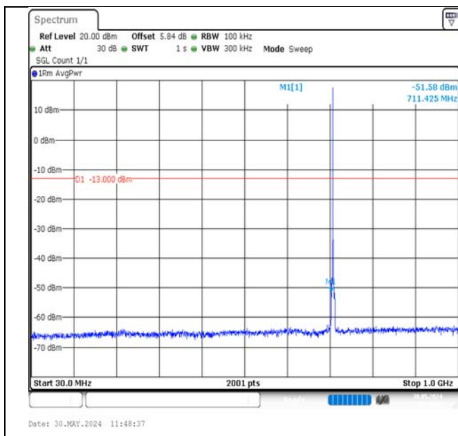
Band12-1.4MHz-QPSK-23173-1RB#0-30~1000-PASS
