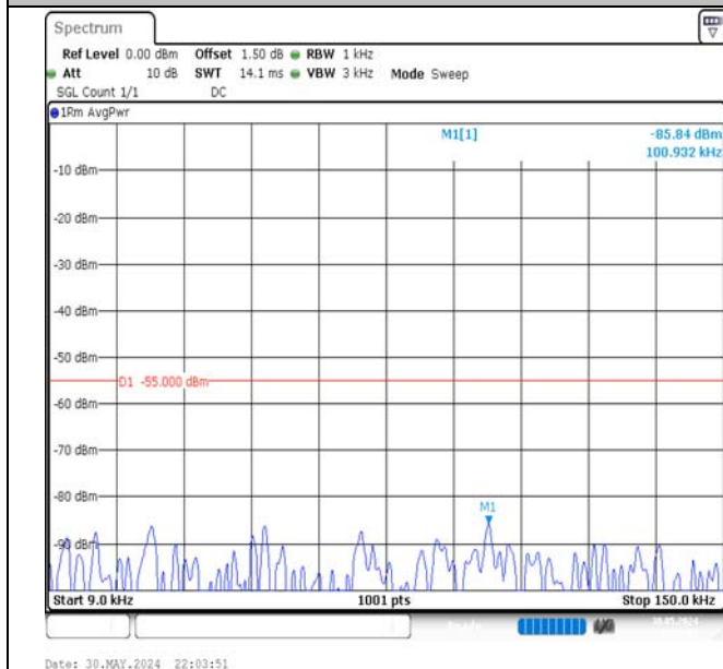
Band7-20MHz-16QAM-21350-1RB#99-0.009~0.15-PASS
