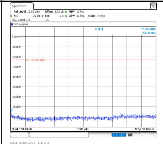
Band12-1.4MHz-QPSK-23017-1RB#5-0.15~30-PASS
