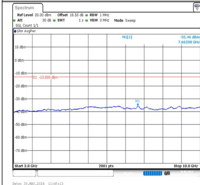
Band12-1.4MHz-QPSK-23017-1RB#5-3000~10000-PASS
