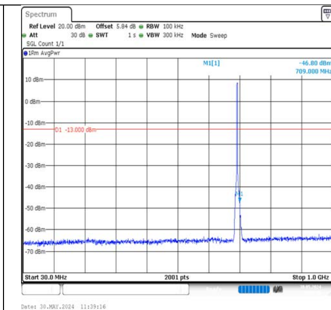
Band12-3MHz-QPSK-23025-15RB#0-30~1000-PASS
