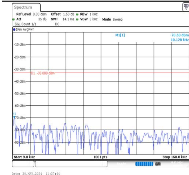
Band12-3MHz-QPSK-23025-1RB#0-0.009~0.15-PASS
