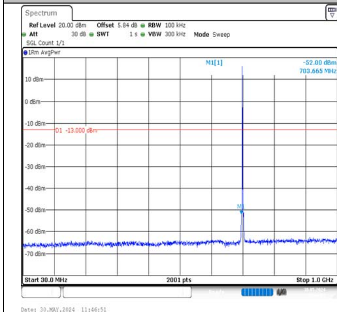
Band12-1.4MHz-16QAM-23095-1RB#0-30~1000-PASS
