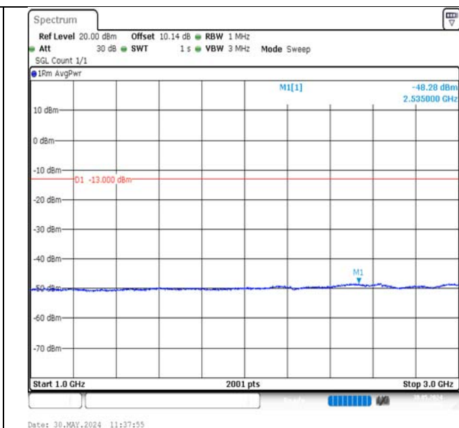
Band12-3MHz-QPSK-23025-1RB#0-1000~3000-PASS
