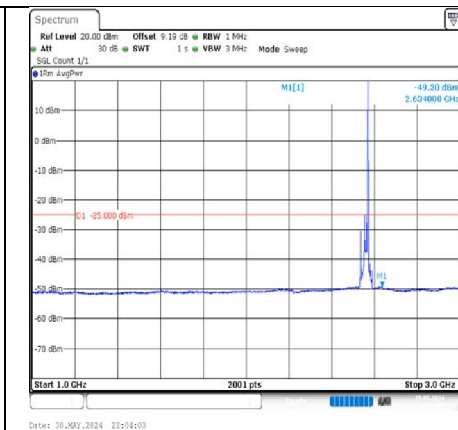
Band7-20MHz-16QAM-21350-1RB#99-1000~3000-PASS
