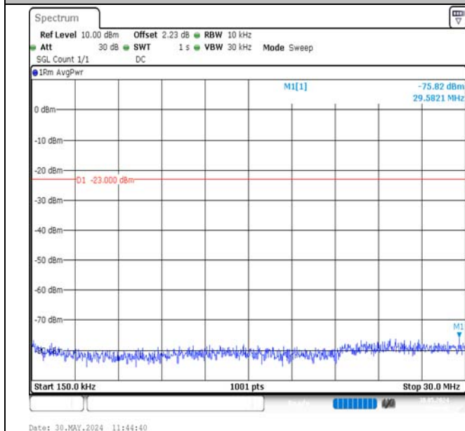
Band12-1.4MHz-16QAM-23017-1RB#0-0.15~30-PASS
