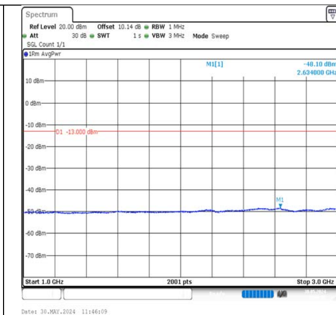
Band12-1.4MHz-16QAM-23017-6RB#0-1000~3000-PASS
