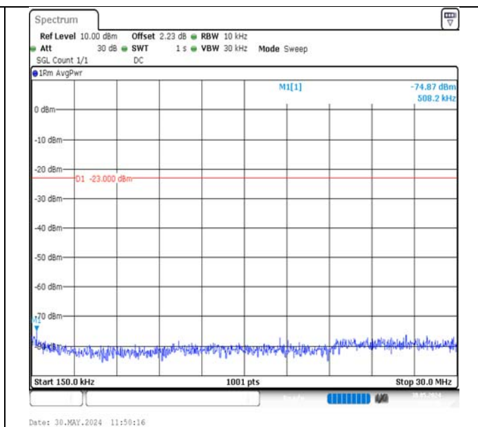
Band12-1.4MHz-16QAM-23173-6RB#0-0.15~30-PASS
