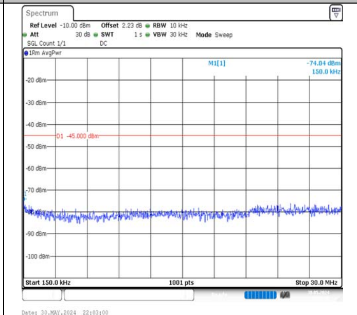
Band7-20MHz-16QAM-21350-1RB#0-0.15~30-PASS
