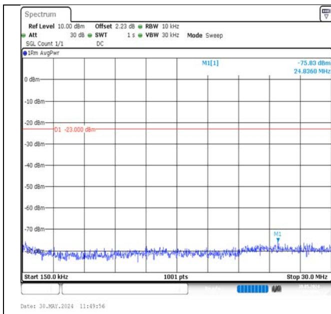
Band12-1.4MHz-QPSK-23173-6RB#0-0.15~30-PASS
