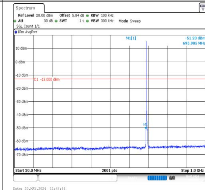
Band12-1.4MHz-16QAM-23017-1RB#0-30~1000-PASS
