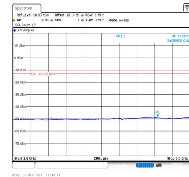
Band12-1.4MHz-QPSK-23173-1RB#0-1000~3000-PASS
