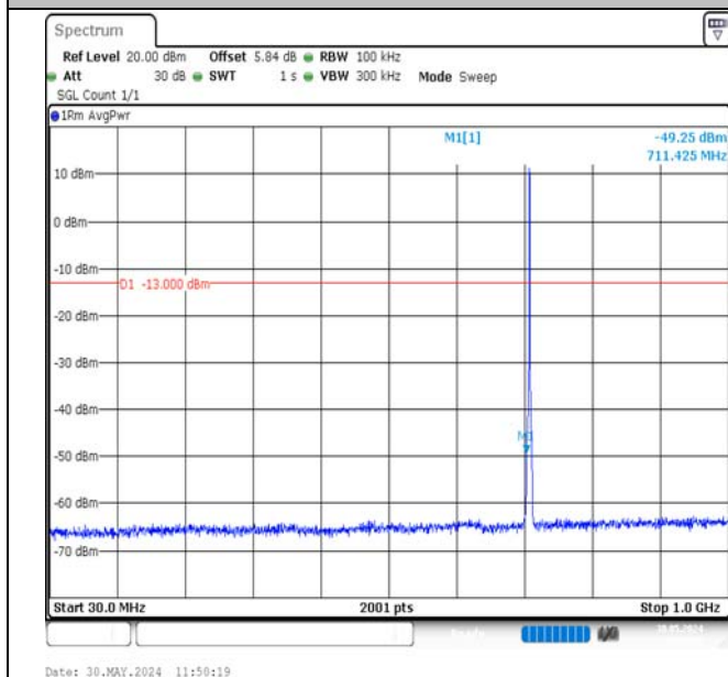
Band12-1.4MHz-16QAM-23173-6RB#0-30~1000-PASS
