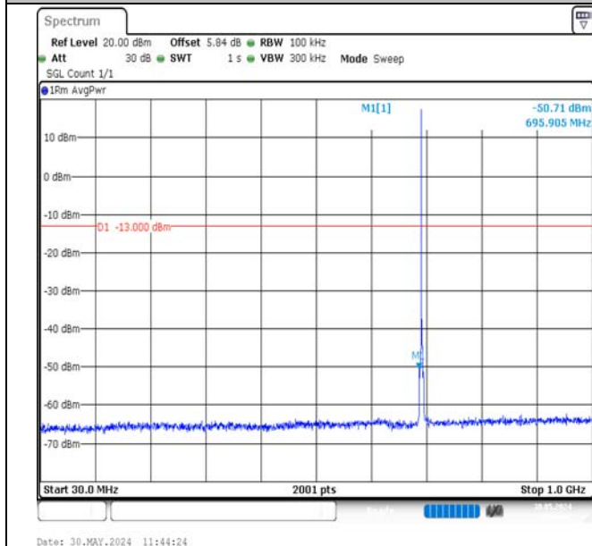
Band12-1.4MHz-QPSK-23017-1RB#0-30~1000-PASS
