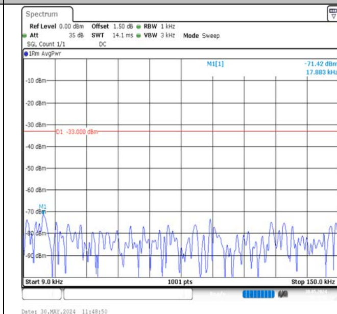
Band12-1.4MHz-16QAM-23173-1RB#0-0.009~0.15-PASS
