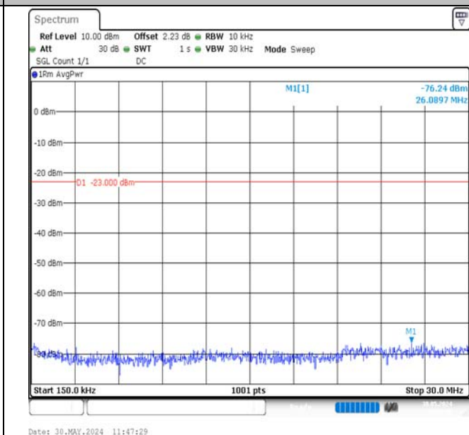
Band12-1.4MHz-16QAM-23095-1RB#5-0.15~30-PASS
