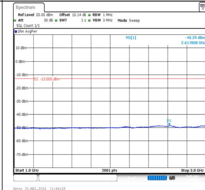
Band12-1.4MHz-QPSK-23017-1RB#0-1000~3000-PASS
