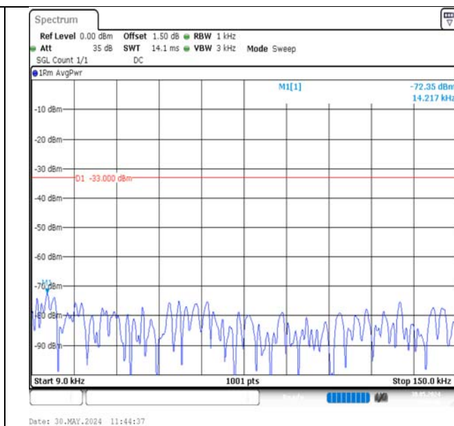
Band12-1.4MHz-16QAM-23017-1RB#0-0.009~0.15-PASS
