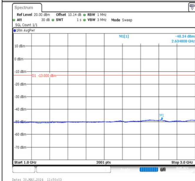
Band12-1.4MHz-QPSK-23173-6RB#0-1000~3000-PASS
