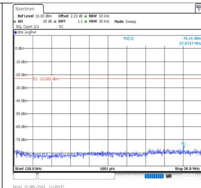
Band12-1.4MHz-16QAM-23095-1RB#0-0.15~30-PASS
