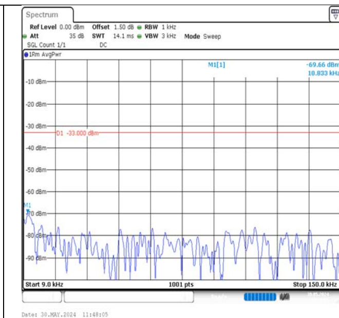
Band12-1.4MHz-16QAM-23095-6RB#0-0.009~0.15-PASS
