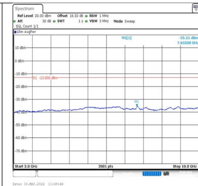
Band12-1.4MHz-16QAM-23173-1RB#5-3000~10000-PASS
