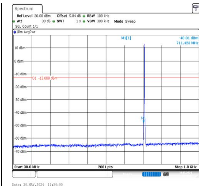
Band12-1.4MHz-QPSK-23173-6RB#0-30~1000-PASS
