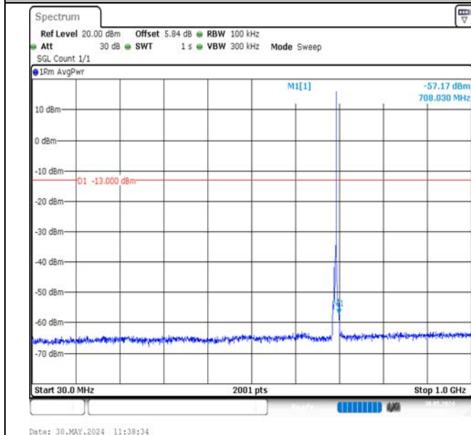
Band12-3MHz-QPSK-23025-1RB#14-30~1000-PASS
