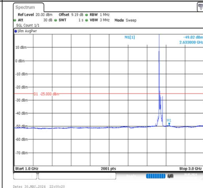
Band7-20MHz-16QAM-21100-1RB#0-1000~3000-PASS
