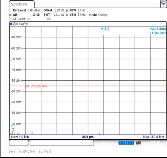
Band7-20MHz-QPSK-20850-100RB#0-0.009~0.15-PASS
