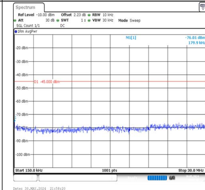
Band7-20MHz-16QAM-20850-1RB#99-0.15~30-PASS
