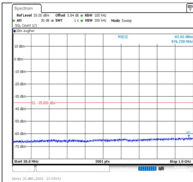
Band7-20MHz-QPSK-20850-100RB#0-30~1000-PASS
