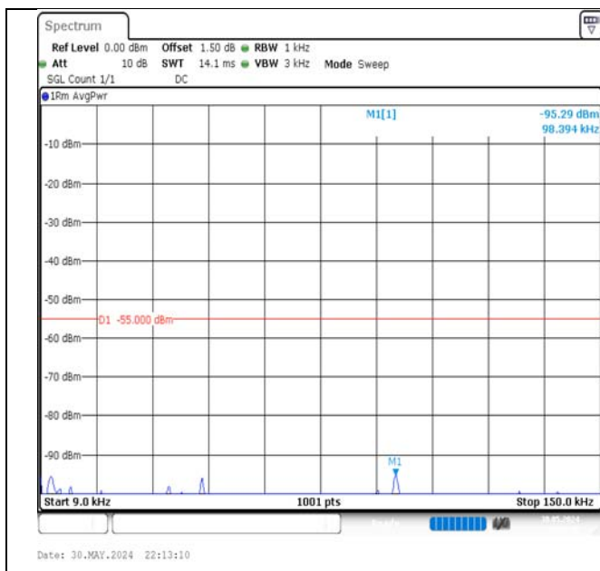
Band7-15MHz-16QAM-21375-75RB#0-0.009~0.15-PASS
