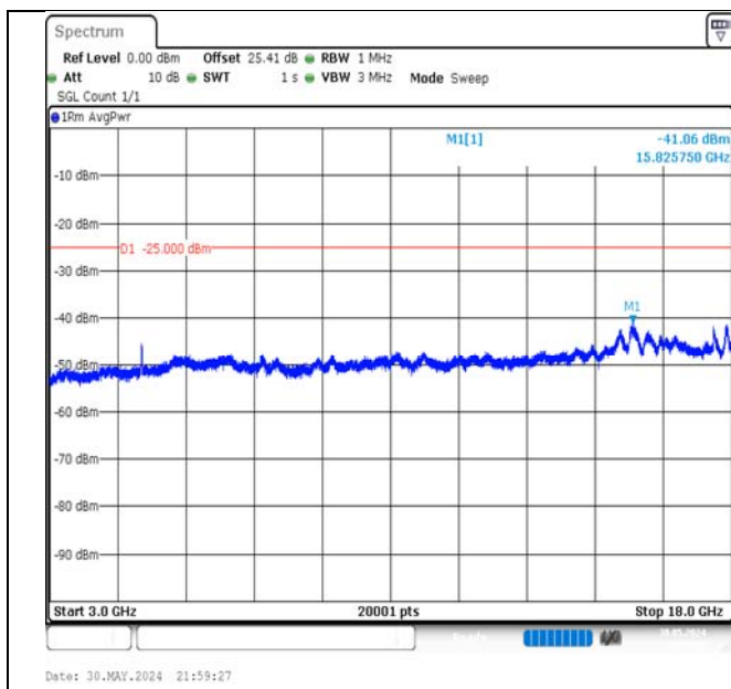
Band7-20MHz-16QAM-20850-100RB#0-3000~18000-PASS
