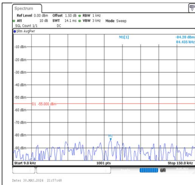
Band7-20MHz-QPSK-20850-1RB#99-0.009~0.15-PASS
