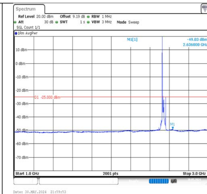
Band7-20MHz-QPSK-21100-1RB#0-1000~3000-PASS
