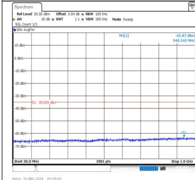
Band7-15MHz-16QAM-21100-1RB#0-30~1000-PASS
