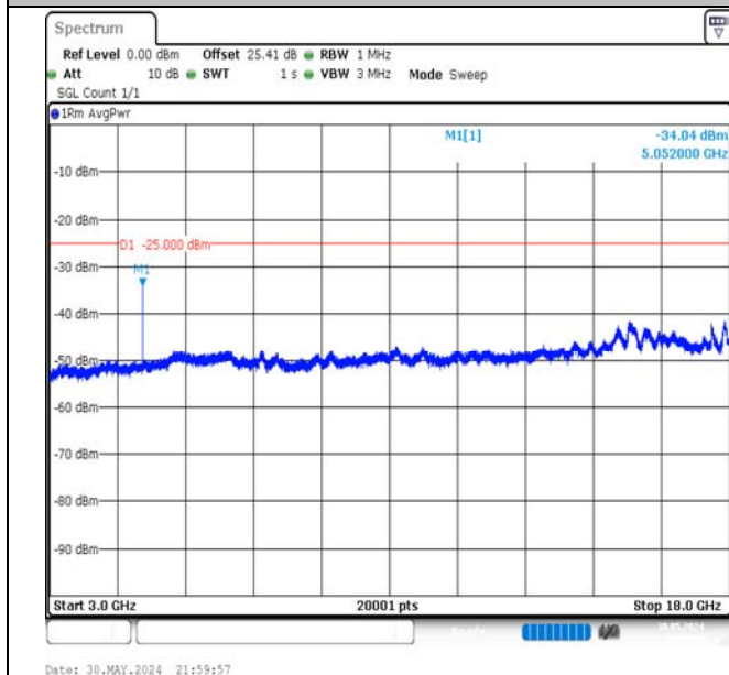
Band7-20MHz-QPSK-21100-1RB#0-3000~18000-PASS
