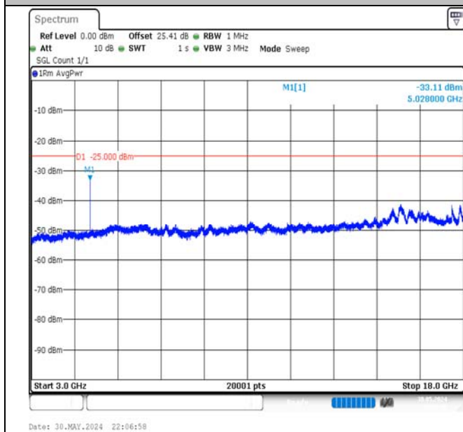
Band7-15MHz-16QAM-20825-1RB#74-3000~18000-PASS
