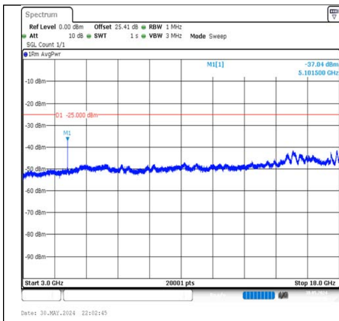
Band7-20MHz-QPSK-21350-1RB#0-3000~18000-PASS
