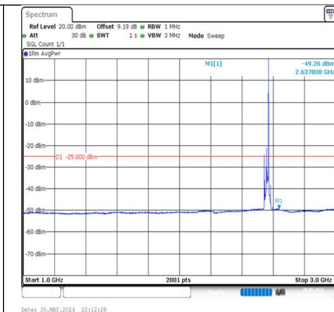
Band7-15MHz-16QAM-21375-1RB#74-1000~3000-PASS
