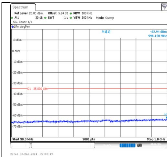
Band7-15MHz-16QAM-20825-1RB#74-30~1000-PASS
