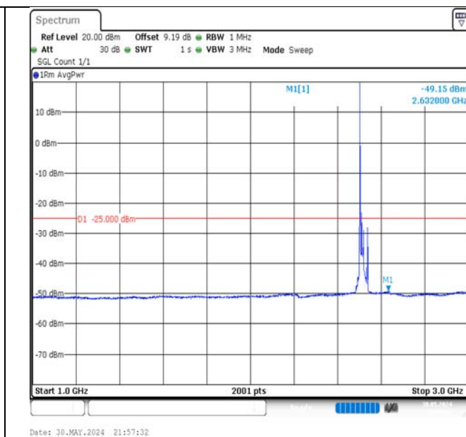
Band7-20MHz-16QAM-20850-1RB#0-1000~3000-PASS
