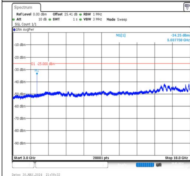
Band7-20MHz-16QAM-20850-1RB#99-3000~18000-PASS
