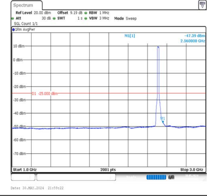
Band7-20MHz-16QAM-20850-100RB#0-1000~3000-PASS
