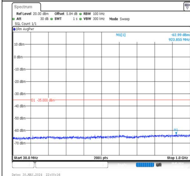
Band7-20MHz-16QAM-21100-1RB#0-30~1000-PASS
