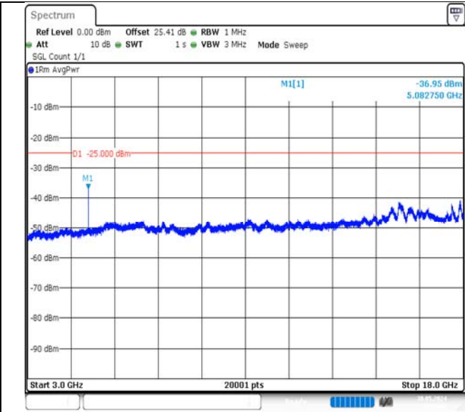
Band7-15MHz-16QAM-21100-1RB#74-3000~18000-PASS
