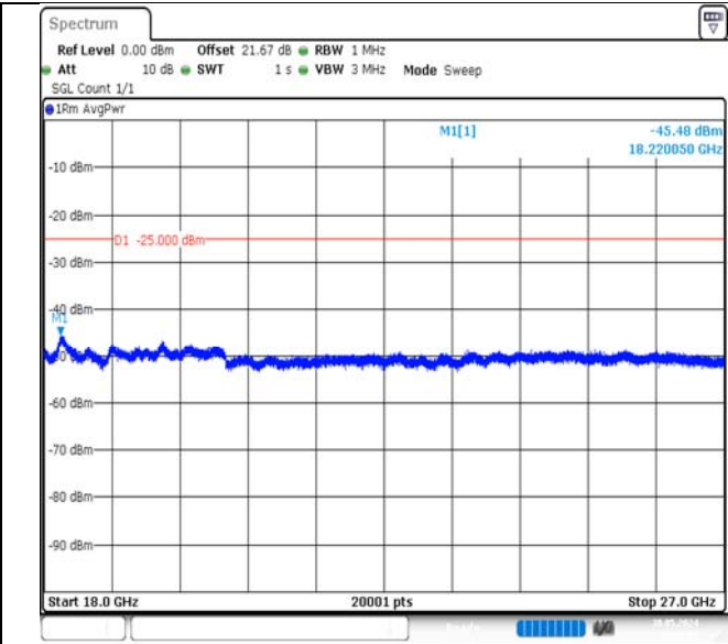
Band7-20MHz-QPSK-21100-100RB#0-18000~27000-PASS
