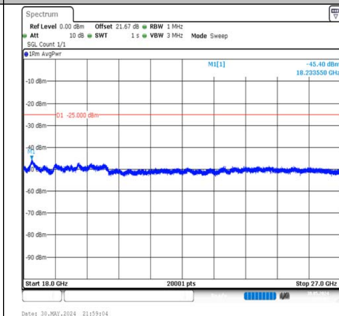
Band7-20MHz-QPSK-20850-100RB#0-18000~27000-PASS
