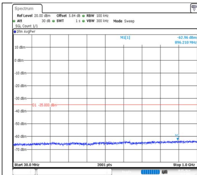
Band7-20MHz-QPSK-21350-100RB#0-30~1000-PASS
