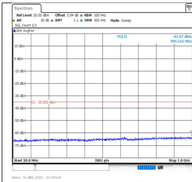
Band7-20MHz-16QAM-20850-1RB#99-30~1000-PASS
