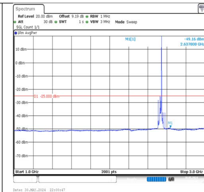
Band7-20MHz-QPSK-21100-1RB#99-1000~3000-PASS
