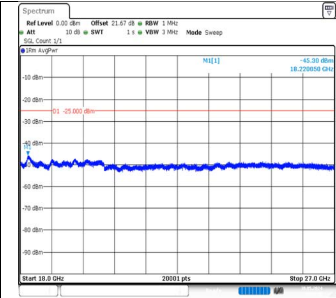
Band7-15MHz-16QAM-21100-1RB#74-18000~27000-PASS
