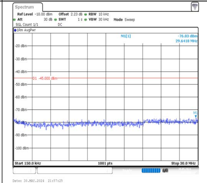
Band7-20MHz-16QAM-20850-1RB#0-0.15~30-PASS
