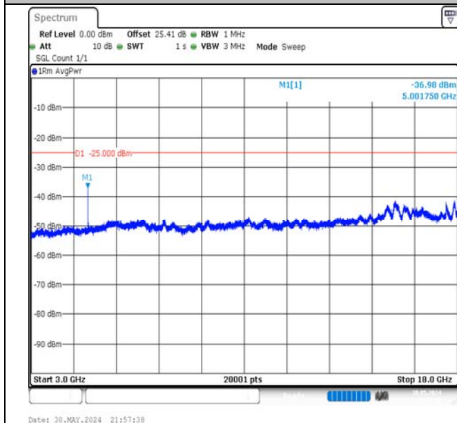
Band7-20MHz-16QAM-20850-1RB#0-3000~18000-PASS
