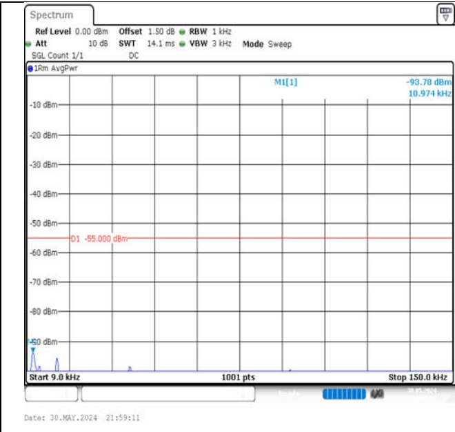
Band7-20MHz-16QAM-20850-100RB#0-0.009~0.15-PASS
