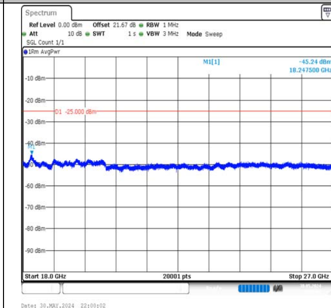
Band7-20MHz-QPSK-21100-1RB#0-18000~27000-PASS
