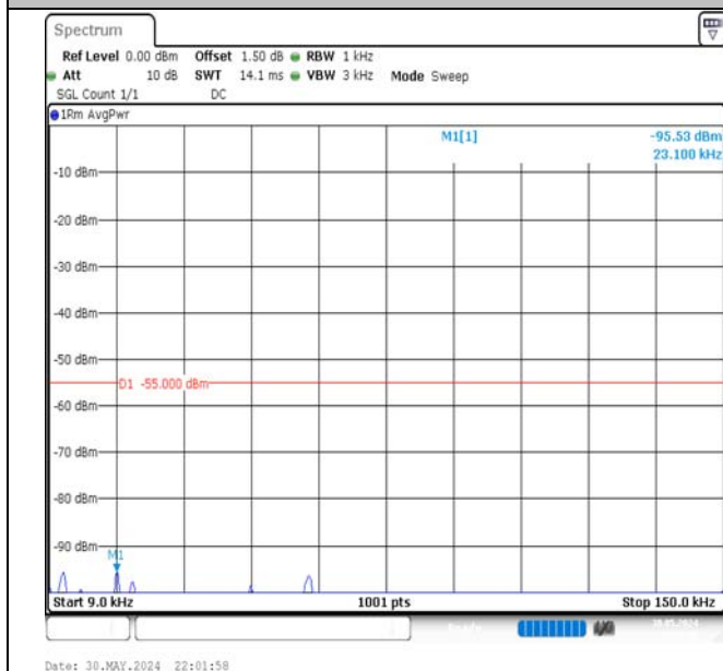
Band7-20MHz-16QAM-21100-100RB#0-0.009~0.15-PASS
