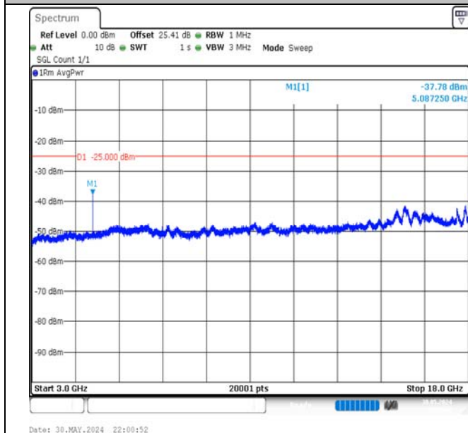
Band7-20MHz-QPSK-21100-1RB#99-3000~18000-PASS
