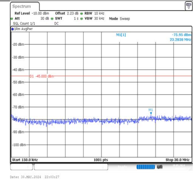
Band7-20MHz-QPSK-21350-1RB#99-0.15~30-PASS
