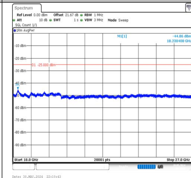
Band7-15MHz-16QAM-21100-75RB#0-18000~27000-PASS
