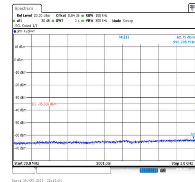
Band7-15MHz-16QAM-21375-1RB#74-30~1000-PASS
