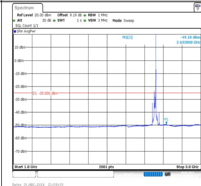
Band7-20MHz-QPSK-20850-1RB#99-1000~3000-PASS
