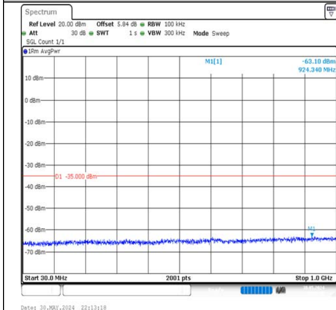
Band7-15MHz-16QAM-21375-75RB#0-30~1000-PASS
