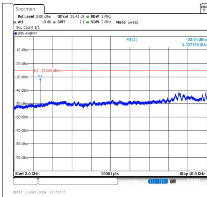
Band7-20MHz-QPSK-20850-1RB#99-3000~18000-PASS
