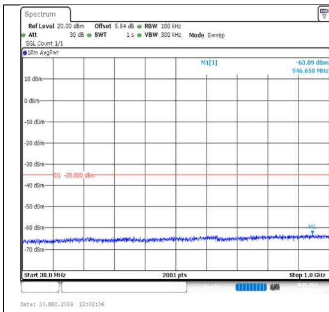
Band7-20MHz-16QAM-21100-100RB#0-30~1000-PASS
