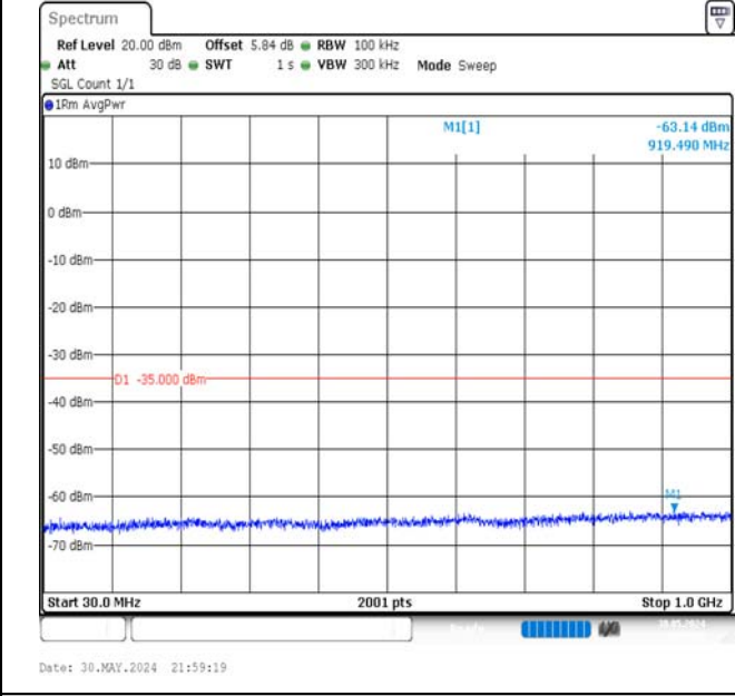
Band7-20MHz-16QAM-20850-100RB#0-30~1000-PASS
