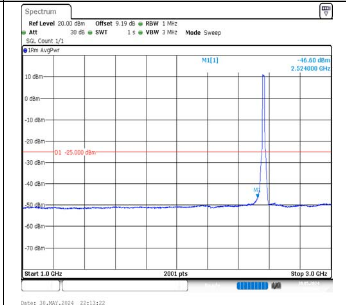
Band7-15MHz-16QAM-21375-75RB#0-1000~3000-PASS
