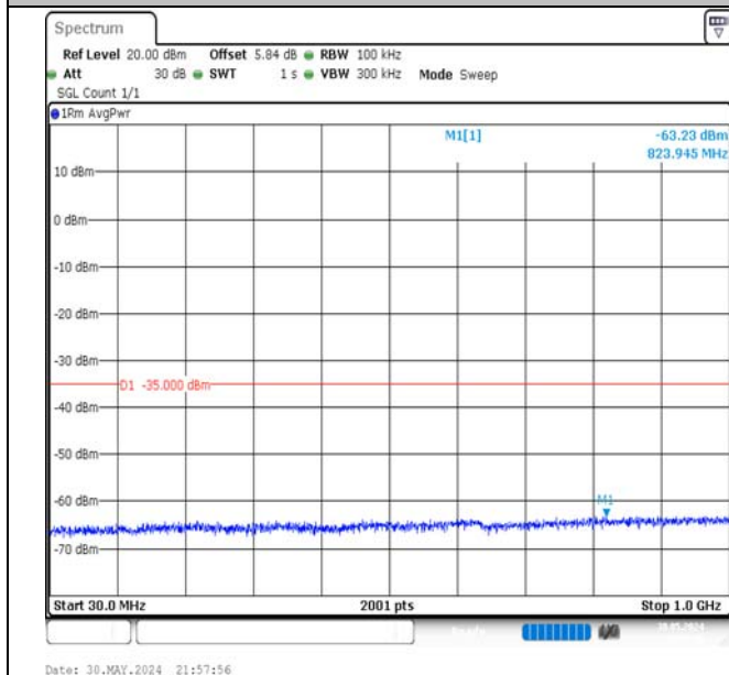
Band7-20MHz-QPSK-20850-1RB#99-30~1000-PASS
