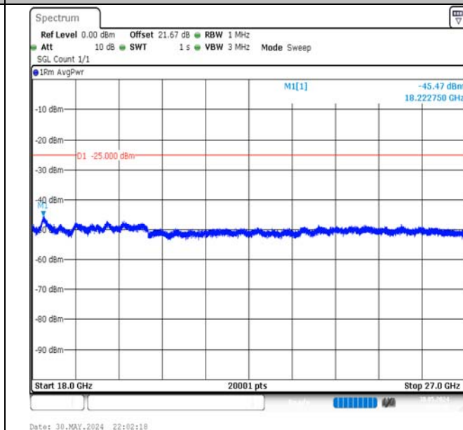
Band7-20MHz-16QAM-21100-100RB#0-18000~27000-PASS
