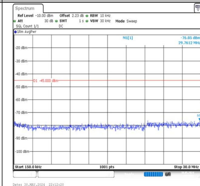
Band7-15MHz-16QAM-21375-1RB#74-0.15~30-PASS
