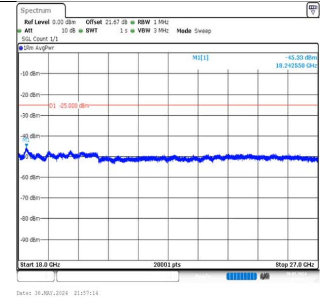
Band7-20MHz-QPSK-20850-1RB#0-18000~27000-PASS
