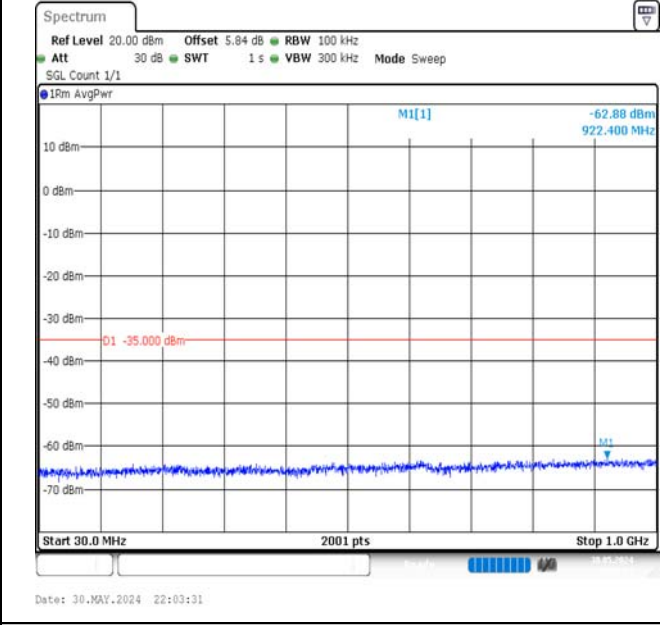
Band7-20MHz-QPSK-21350-1RB#99-30~1000-PASS
