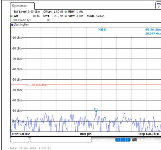
Band7-20MHz-16QAM-20850-1RB#0-0.009~0.15-PASS
