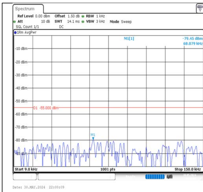
Band7-20MHz-16QAM-21100-1RB#0-0.009~0.15-PASS
