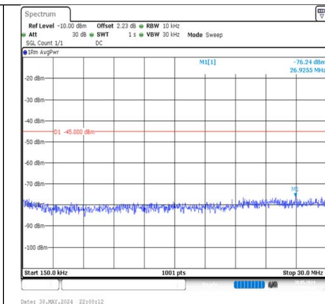
Band7-20MHz-16QAM-21100-1RB#0-0.15~30-PASS
