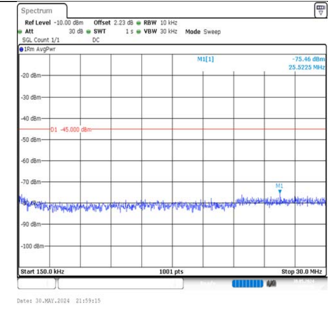
Band7-20MHz-16QAM-20850-100RB#0-0.15~30-PASS
