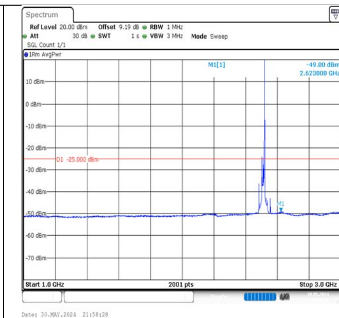
Band7-20MHz-16QAM-20850-1RB#99-1000~3000-PASS
