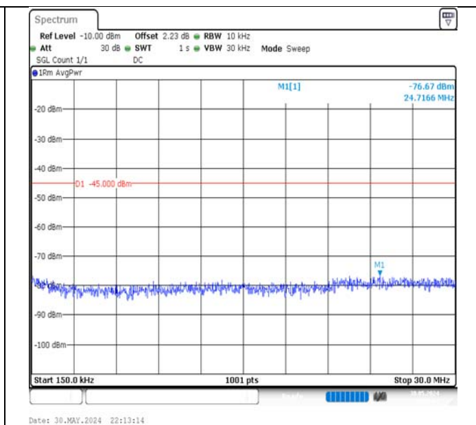
Band7-15MHz-16QAM-21375-75RB#0-0.15~30-PASS
