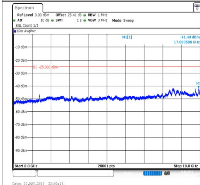
Band7-20MHz-16QAM-21100-100RB#0-3000~18000-PASS
