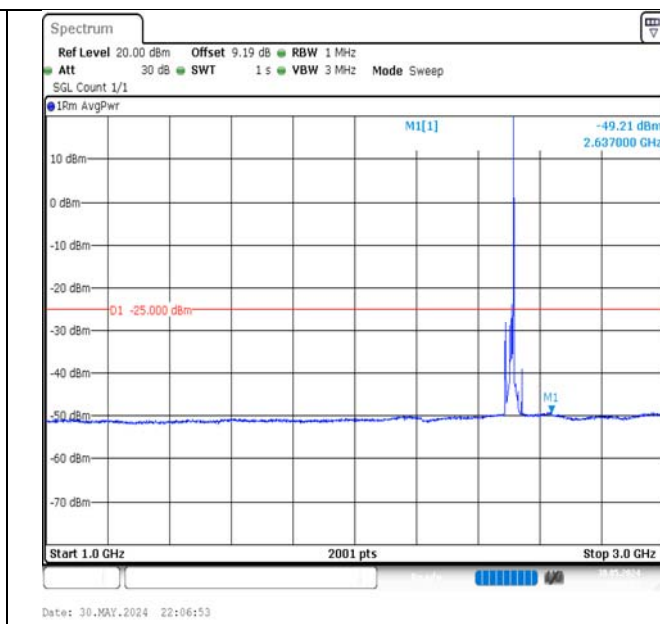
Band7-15MHz-16QAM-20825-1RB#74-1000~3000-PASS
