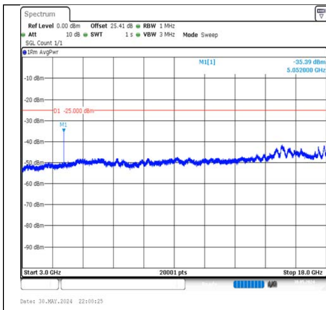
Band7-20MHz-16QAM-21100-1RB#0-3000~18000-PASS
