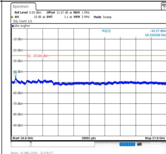
Band7-20MHz-16QAM-20850-1RB#99-18000~27000-PASS
