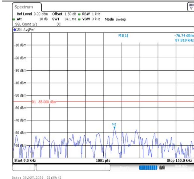
Band7-20MHz-QPSK-21100-1RB#0-0.009~0.15-PASS
