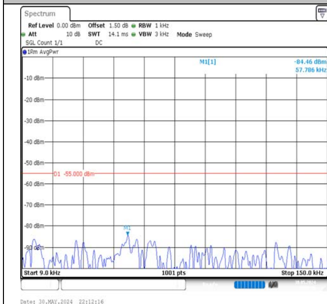
Band7-15MHz-16QAM-21375-1RB#74-0.009~0.15-PASS
