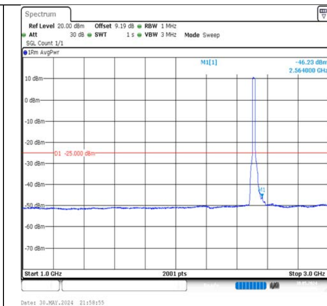
Band7-20MHz-QPSK-20850-100RB#0-1000~3000-PASS
