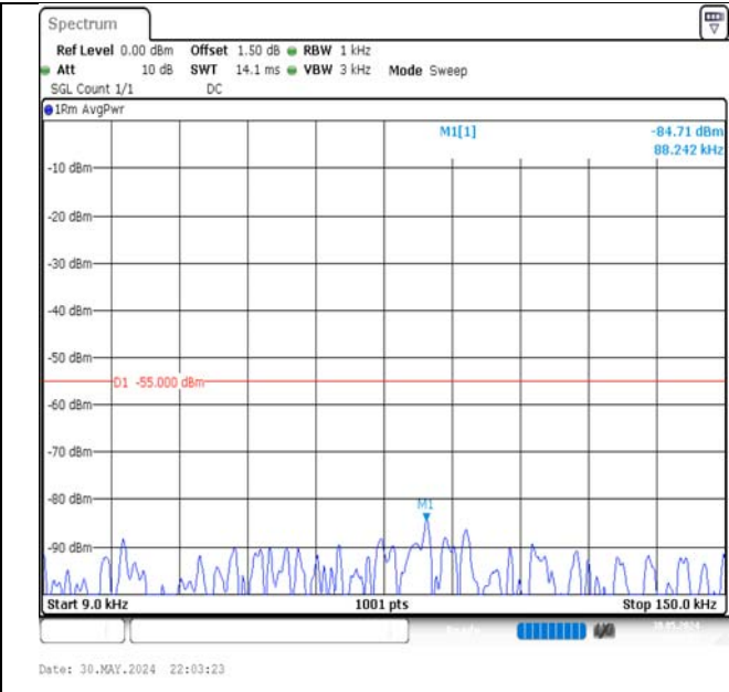
Band7-20MHz-QPSK-21350-1RB#99-0.009~0.15-PASS
