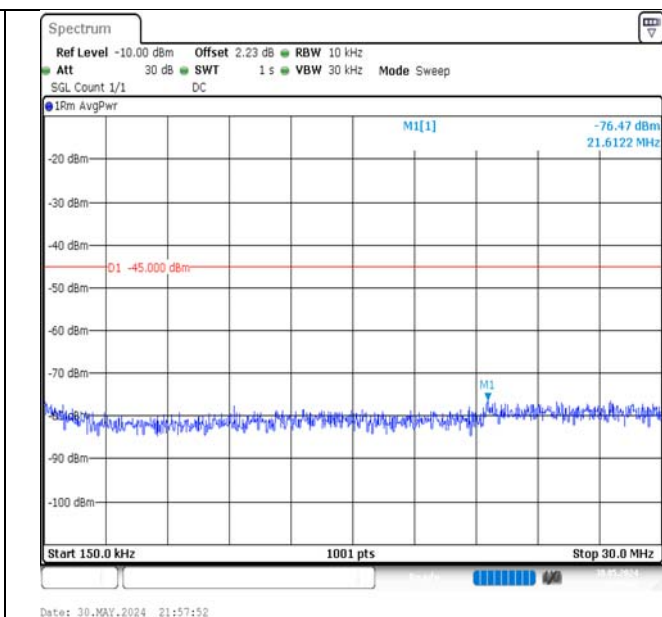
Band7-20MHz-QPSK-20850-1RB#99-0.15~30-PASS
