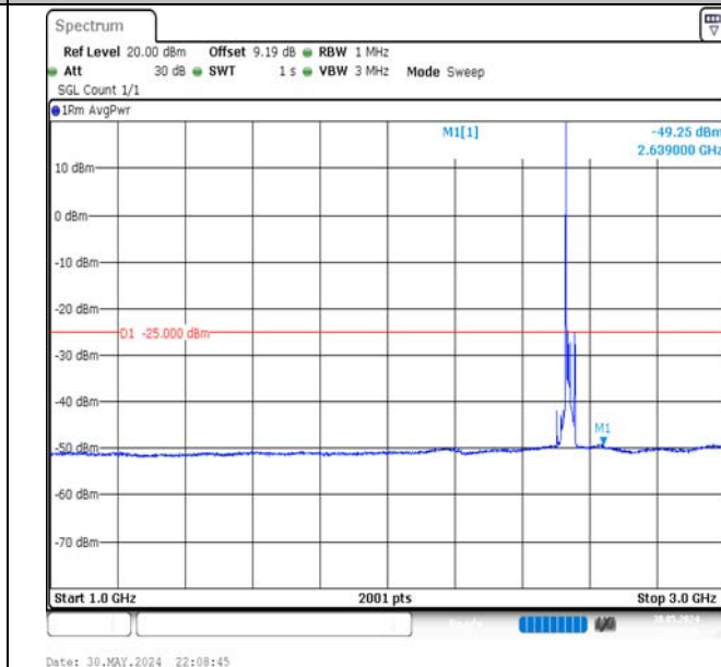
Band7-15MHz-16QAM-21100-1RB#0-1000~3000-PASS
