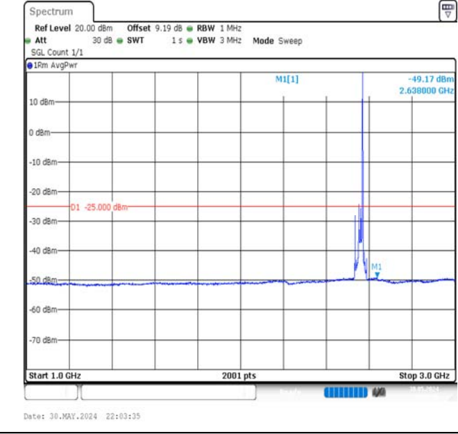
Band7-20MHz-QPSK-21350-1RB#99-1000~3000-PASS
