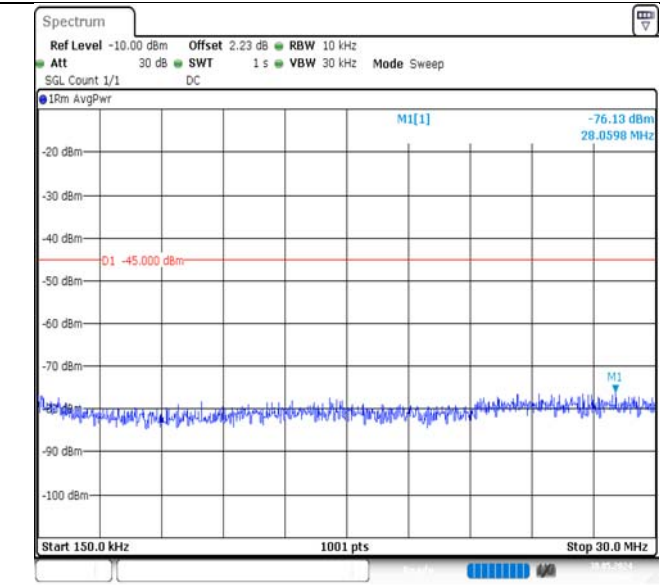
Band7-20MHz-QPSK-21350-1RB#0-0.15~30-PASS
