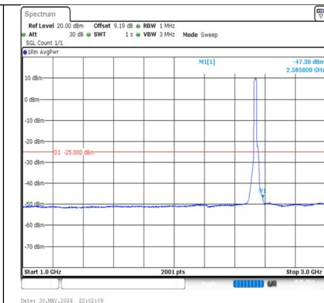
Band7-20MHz-16QAM-21100-100RB#0-1000~3000-PASS
