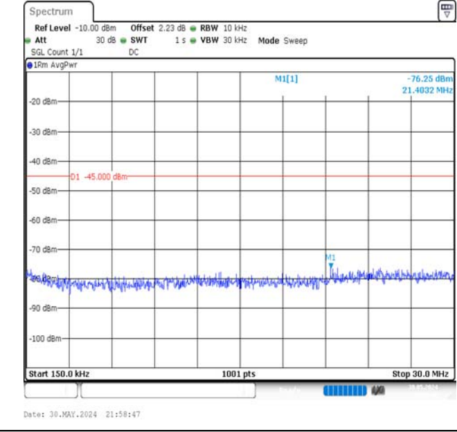
Band7-20MHz-QPSK-20850-100RB#0-0.15~30-PASS
