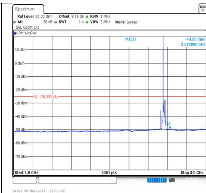
Band7-15MHz-16QAM-21375-1RB#0-1000~3000-PASS
