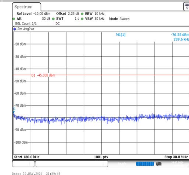
Band7-20MHz-QPSK-21100-1RB#0-0.15~30-PASS
