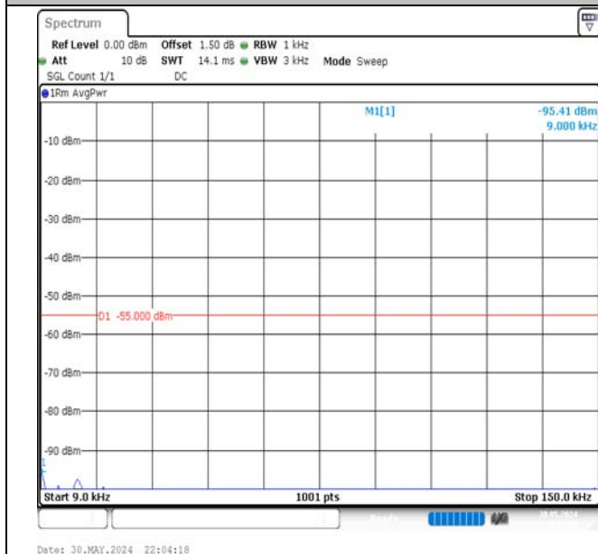
Band7-20MHz-QPSK-21350-100RB#0-0.009~0.15-PASS
