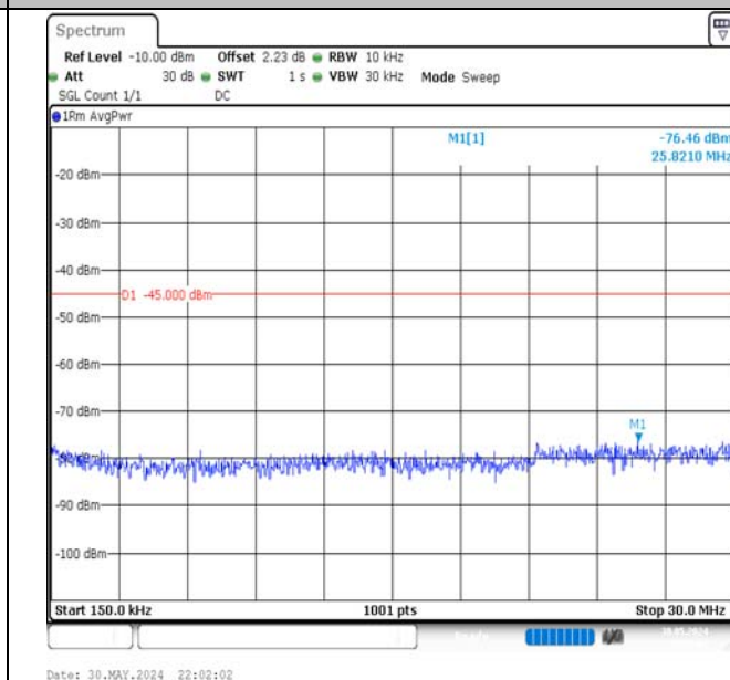
Band7-20MHz-16QAM-21100-100RB#0-0.15~30-PASS
