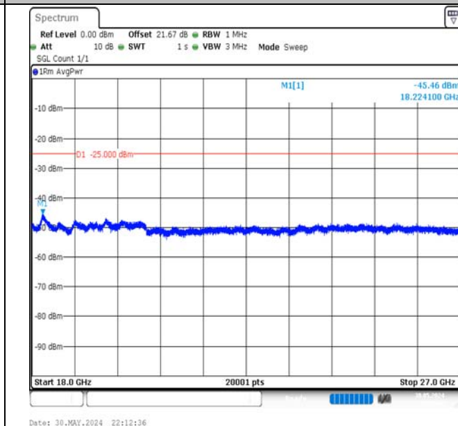
Band7-15MHz-16QAM-21375-1RB#74-18000~27000-PASS
