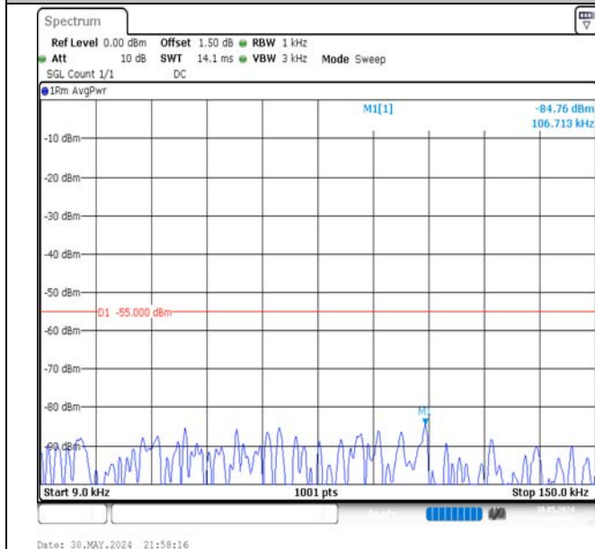
Band7-20MHz-16QAM-20850-1RB#99-0.009~0.15-PASS
