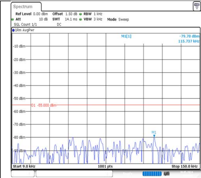
Band7-20MHz-QPSK-21350-1RB#0-0.009~0.15-PASS
