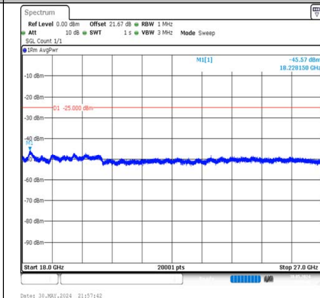
Band7-20MHz-16QAM-20850-1RB#0-18000~27000-PASS
