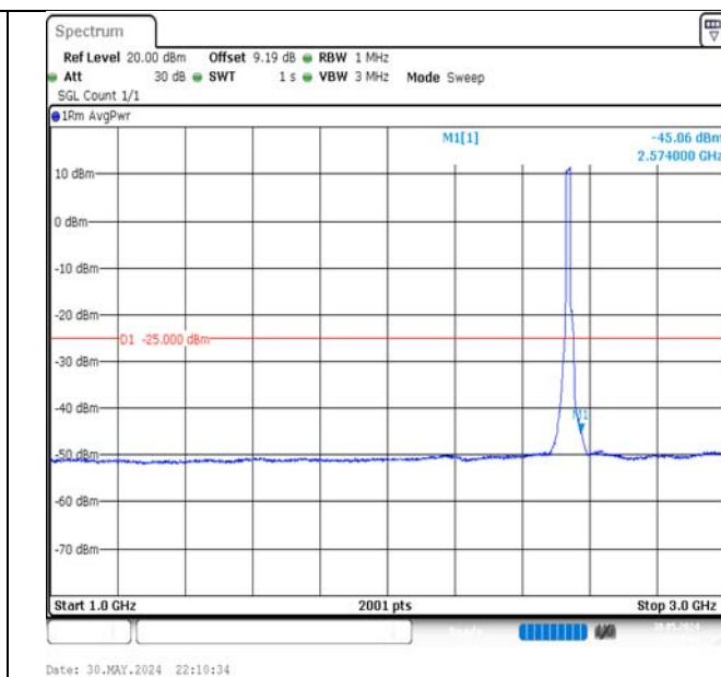
Band7-15MHz-16QAM-21100-75RB#0-1000~3000-PASS
