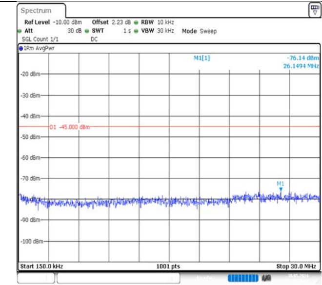
Band7-20MHz-16QAM-21100-1RB#99-0.15~30-PASS
