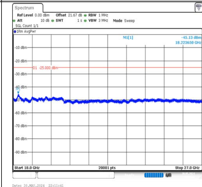
Band7-15MHz-16QAM-21375-1RB#0-18000~27000-PASS
