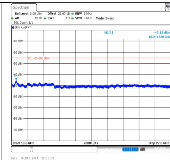
Band7-15MHz-16QAM-21375-75RB#0-18000~27000-PASS
