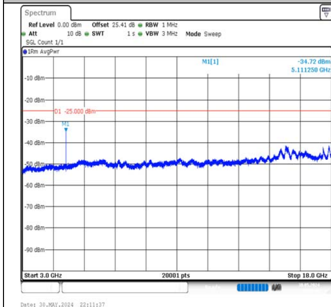
Band7-15MHz-16QAM-21375-1RB#0-3000~18000-PASS
