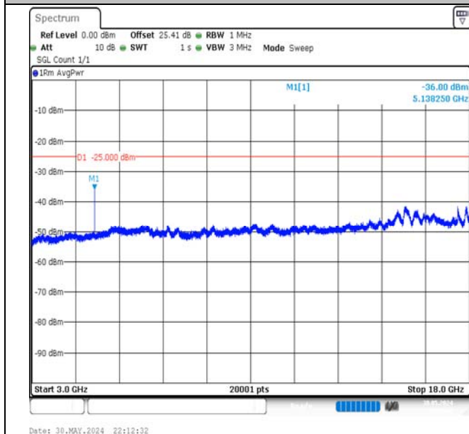
Band7-15MHz-16QAM-21375-1RB#74-3000~18000-PASS
