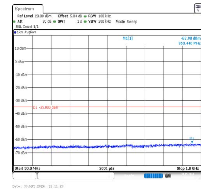
Band7-15MHz-16QAM-21375-1RB#0-30~1000-PASS
