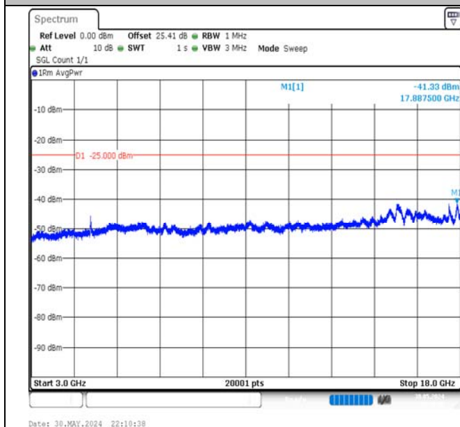
Band7-15MHz-16QAM-21100-75RB#0-3000~18000-PASS
