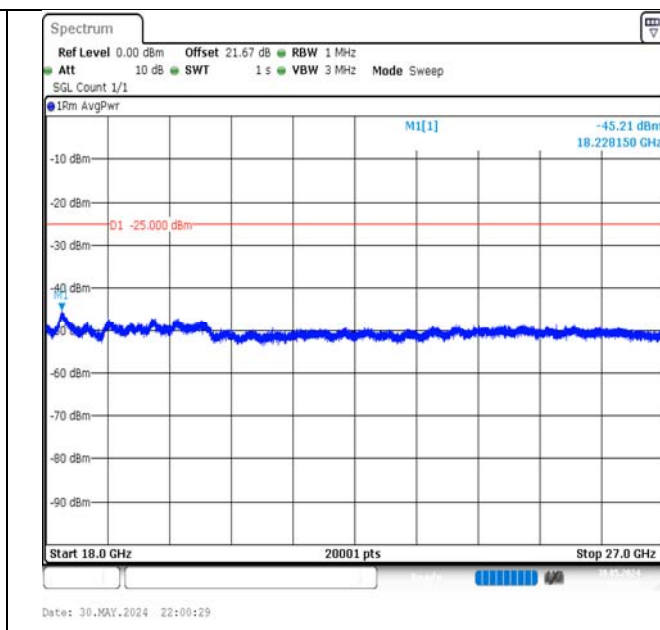
Band7-20MHz-16QAM-21100-1RB#0-18000~27000-PASS
