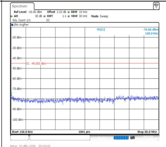
Band7-20MHz-QPSK-21350-100RB#0-0.15~30-PASS
