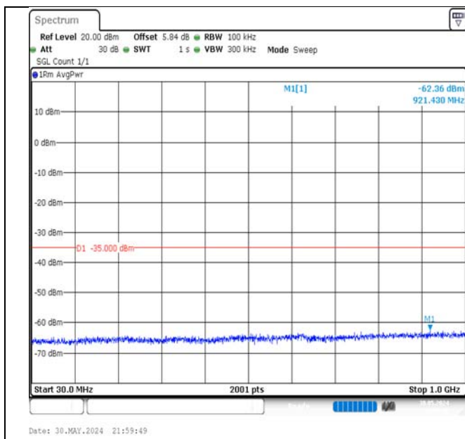
Band7-20MHz-QPSK-21100-1RB#0-30~1000-PASS
