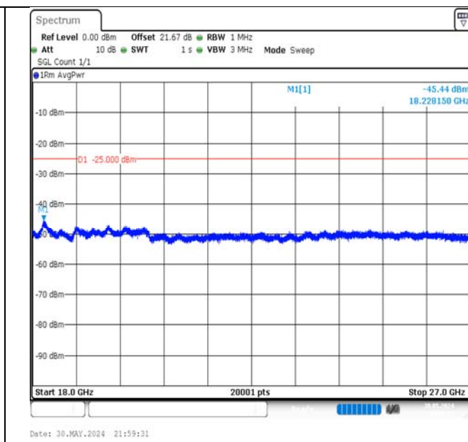
Band7-20MHz-16QAM-20850-100RB#0-18000~27000-PASS
