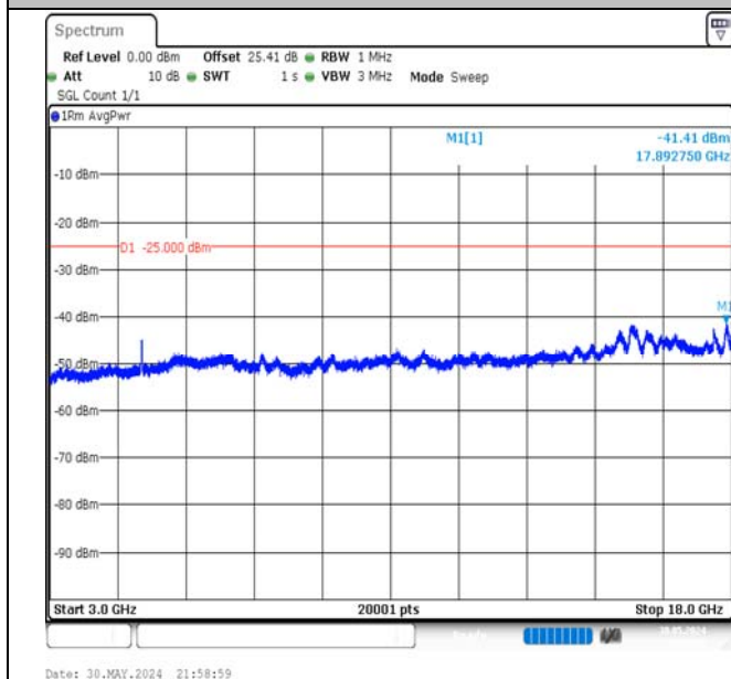
Band7-20MHz-QPSK-20850-100RB#0-3000~18000-PASS
