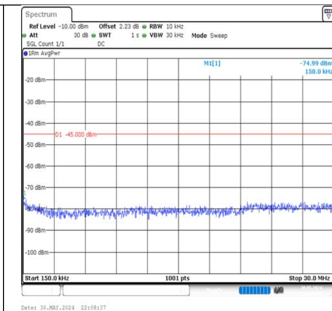
Band7-15MHz-16QAM-21100-1RB#0-0.15~30-PASS
