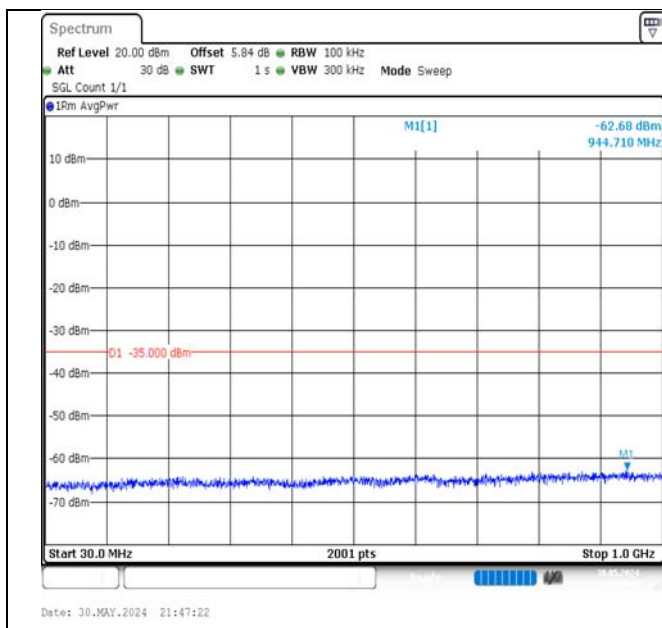
Band7-10MHz-16QAM-21400-1RB#49-30~1000-PASS
