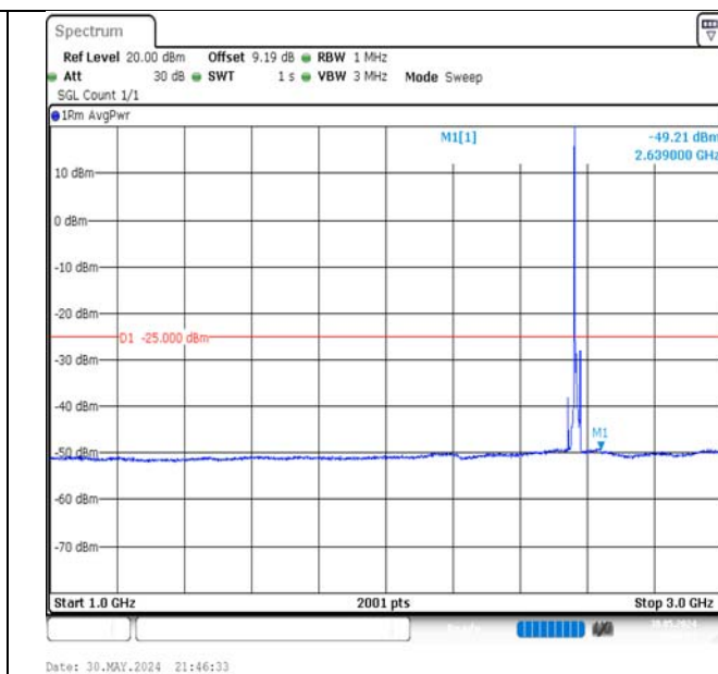
Band7-10MHz-16QAM-21400-1RB#0-1000~3000-PASS
