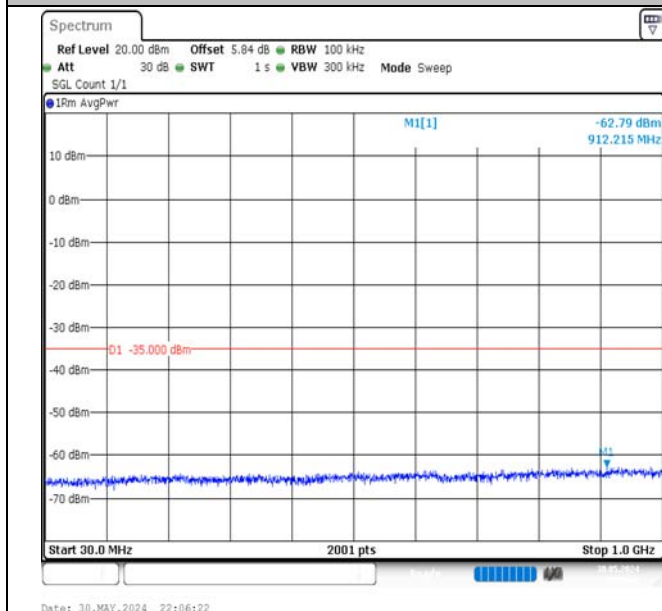
Band7-15MHz-QPSK-20825-1RB#74-30~1000-PASS
