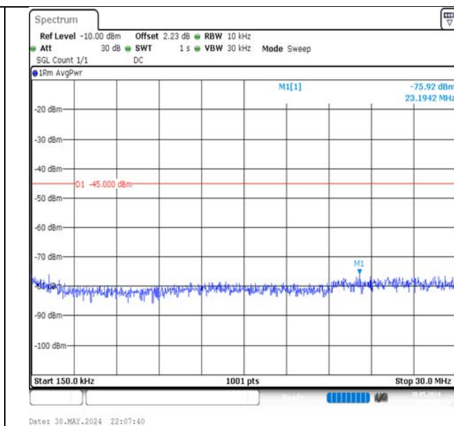
Band7-15MHz-16QAM-20825-75RB#0-0.15~30-PASS
