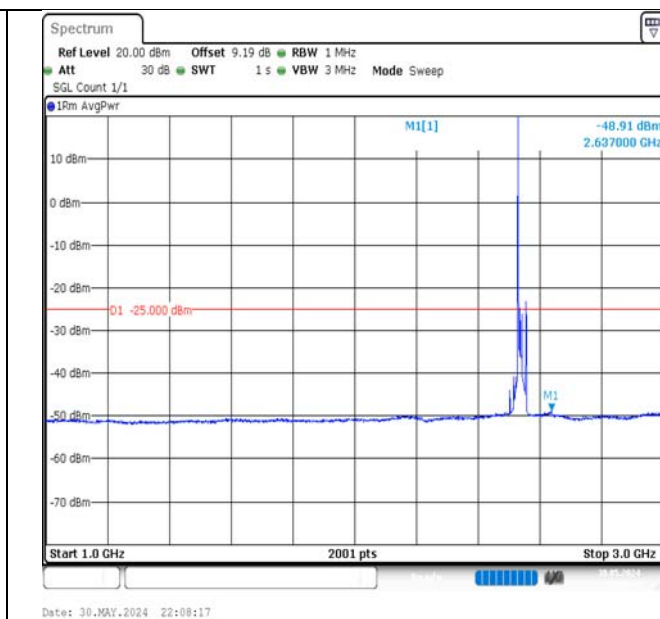
Band7-15MHz-QPSK-21100-1RB#0-1000~3000-PASS
