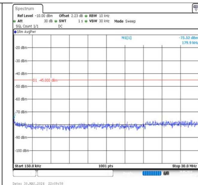
Band7-15MHz-QPSK-21100-75RB#0-0.15~30-PASS
