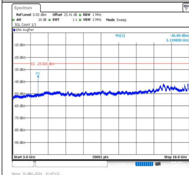
Band7-10MHz-16QAM-21400-1RB#49-3000~18000-PASS
