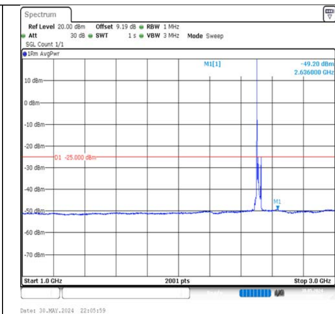
Band7-15MHz-16QAM-20825-1RB#0-1000~3000-PASS
