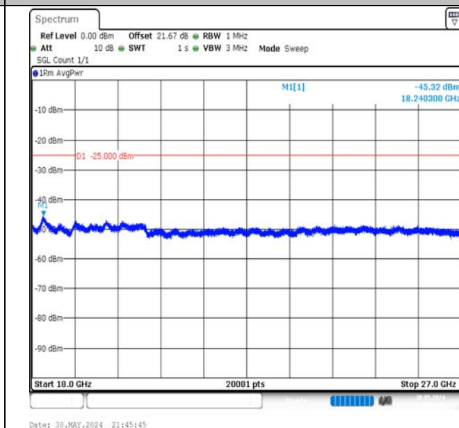
Band7-10MHz-16QAM-21100-50RB#0-18000~27000-PASS
