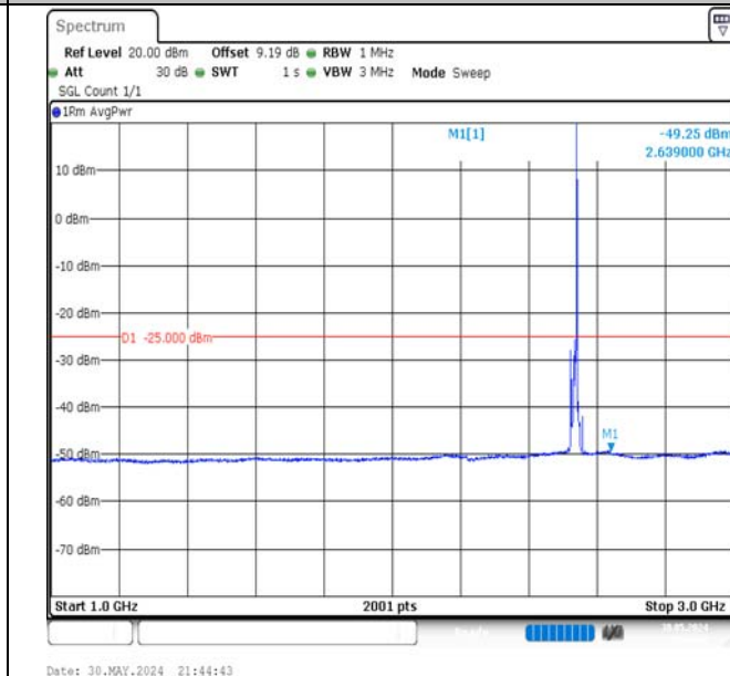
Band7-10MHz-16QAM-21100-1RB#49-1000~3000-PASS
