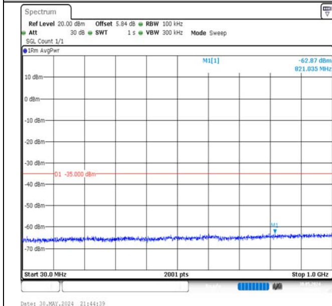
Band7-10MHz-16QAM-21100-1RB#49-30~1000-PASS
