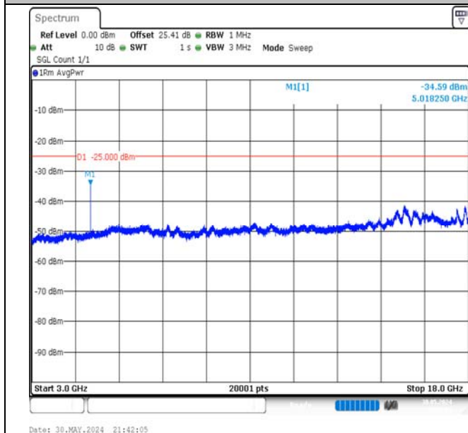
Band7-10MHz-16QAM-20800-1RB#49-3000~18000-PASS
