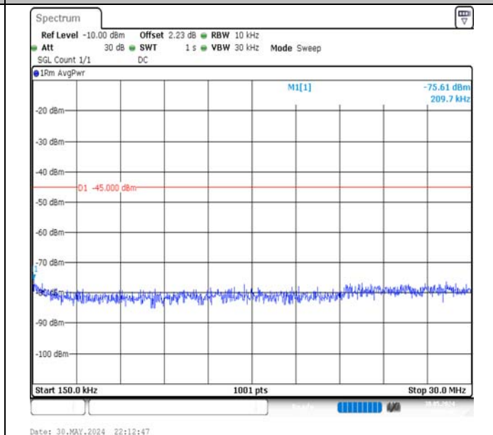
Band7-15MHz-QPSK-21375-75RB#0-0.15~30-PASS
