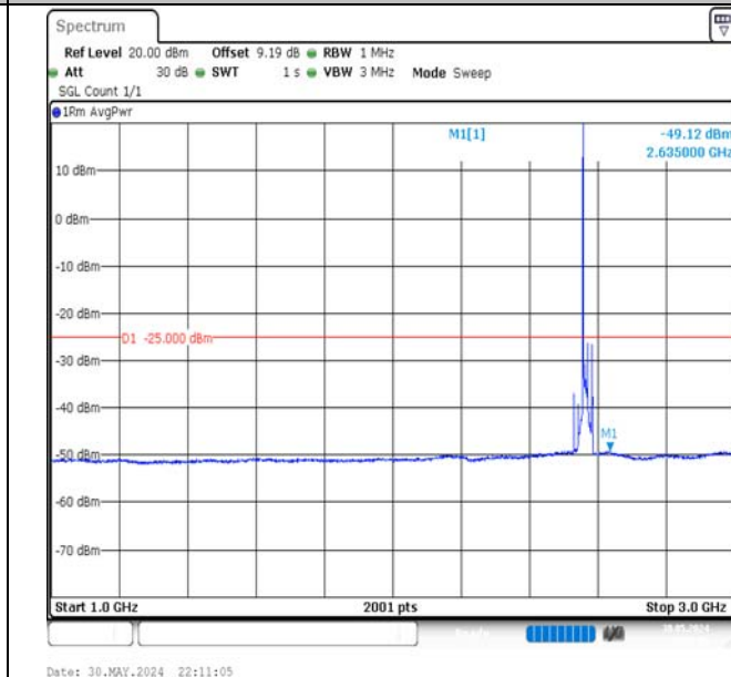
Band7-15MHz-QPSK-21375-1RB#0-1000~3000-PASS
