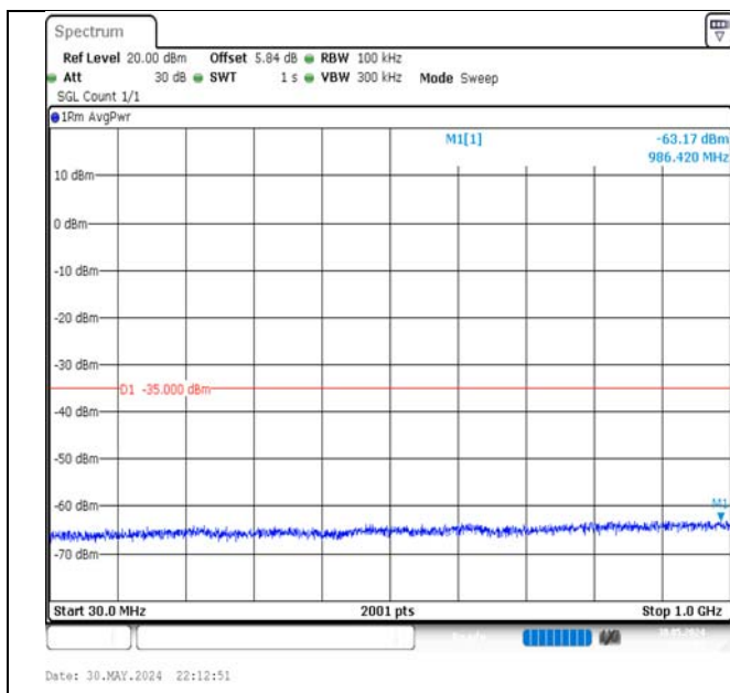
Band7-15MHz-QPSK-21375-75RB#0-30~1000-PASS
