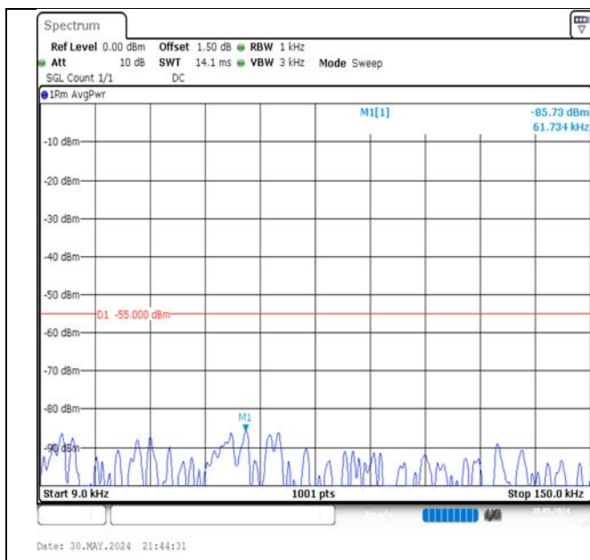
Band7-10MHz-16QAM-21100-1RB#49-0.009~0.15-PASS
