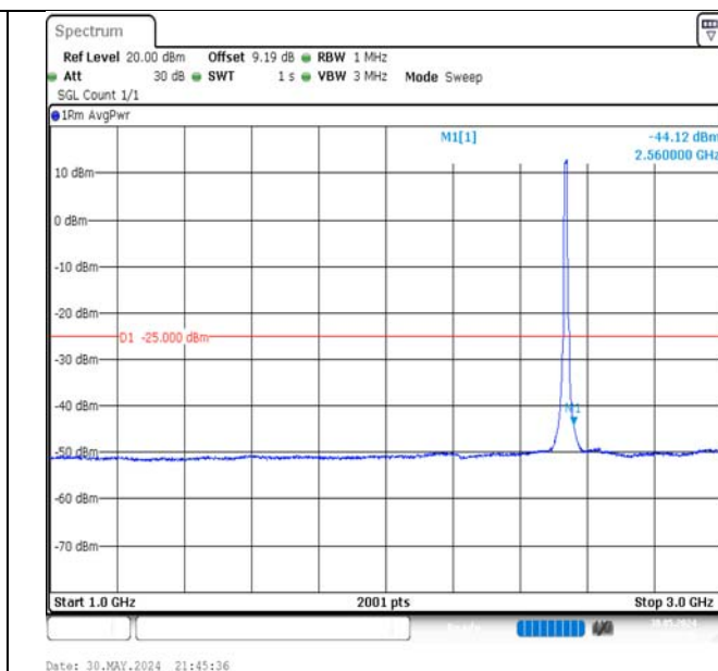
Band7-10MHz-16QAM-21100-50RB#0-1000~3000-PASS
