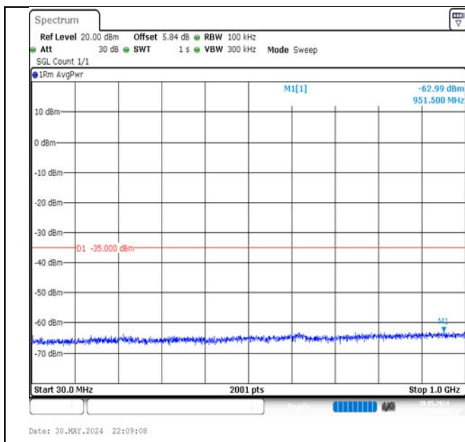
Band7-15MHz-QPSK-21100-1RB#74-30~1000-PASS
