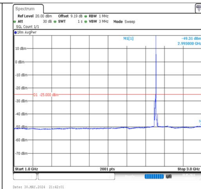
Band7-10MHz-16QAM-20800-1RB#49-1000~3000-PASS
