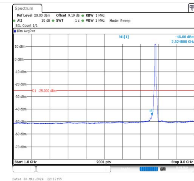
Band7-15MHz-QPSK-21375-75RB#0-1000~3000-PASS
