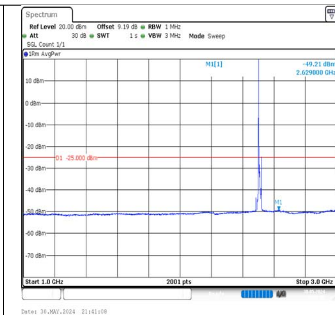
Band7-10MHz-16QAM-20800-1RB#0-1000~3000-PASS
