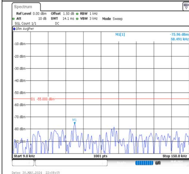
Band7-15MHz-QPSK-21100-1RB#0-0.009~0.15-PASS
