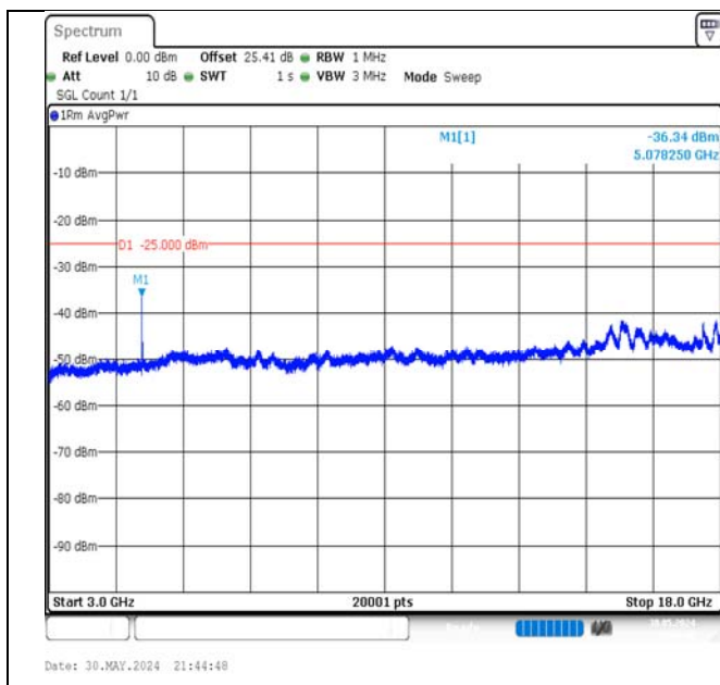
Band7-10MHz-16QAM-21100-1RB#49-3000~18000-PASS
