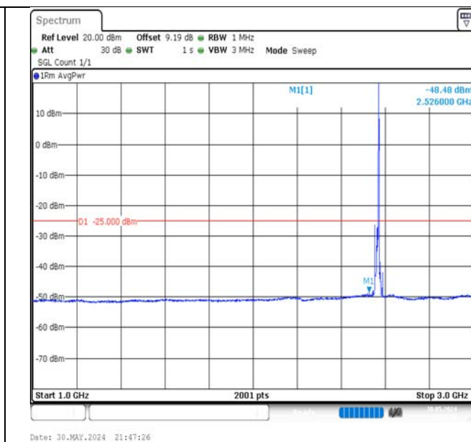
Band7-10MHz-16QAM-21400-1RB#49-1000~3000-PASS
