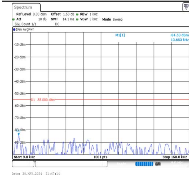
Band7-10MHz-16QAM-21400-1RB#49-0.009~0.15-PASS
