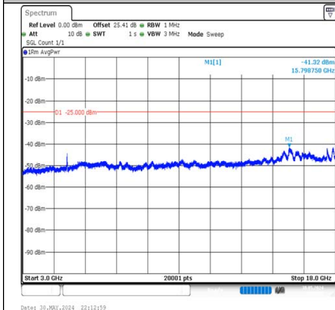
Band7-15MHz-QPSK-21375-75RB#0-3000~18000-PASS
