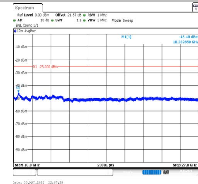
Band7-15MHz-QPSK-20825-75RB#0-18000~27000-PASS
