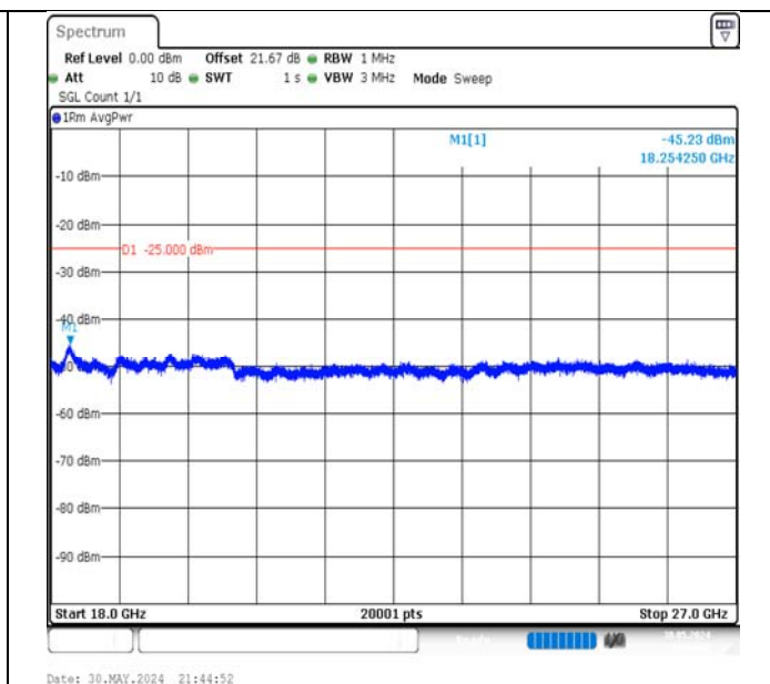
Band7-10MHz-16QAM-21100-1RB#49-18000~27000-PASS
