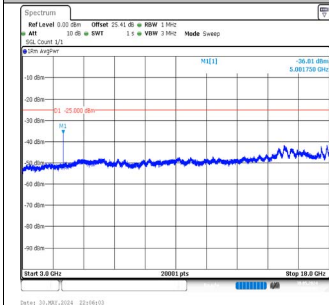
Band7-15MHz-16QAM-20825-1RB#0-3000~18000-PASS
