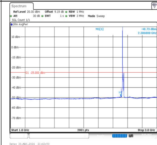
Band7-10MHz-16QAM-21100-1RB#0-1000~3000-PASS
