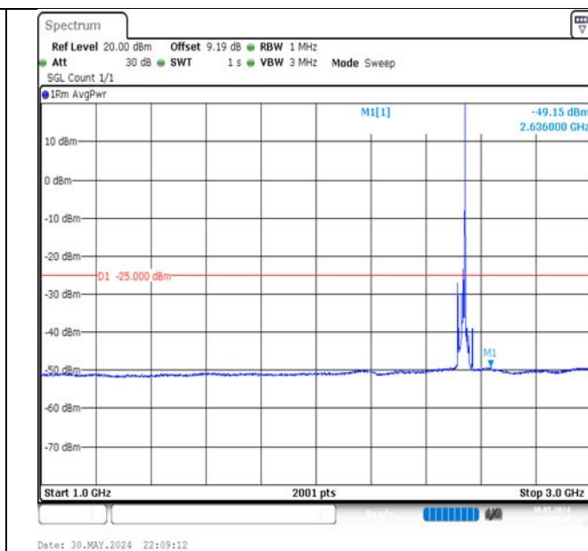
Band7-15MHz-QPSK-21100-1RB#74-1000~3000-PASS
