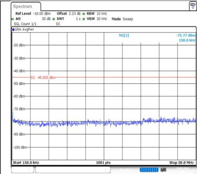
Band7-15MHz-QPSK-20825-1RB#0-0.15~30-PASS
