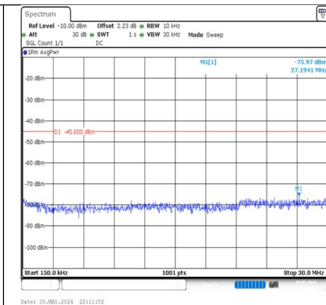
Band7-15MHz-QPSK-21375-1RB#74-0.15~30-PASS
