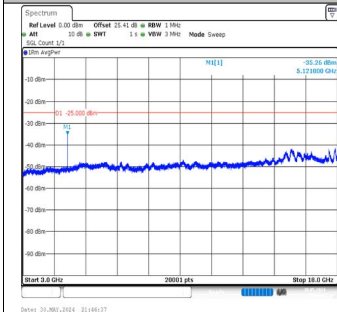
Band7-10MHz-16QAM-21400-1RB#0-3000~18000-PASS
