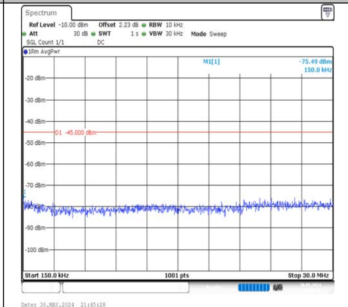
Band7-10MHz-16QAM-21100-50RB#0-0.15~30-PASS
