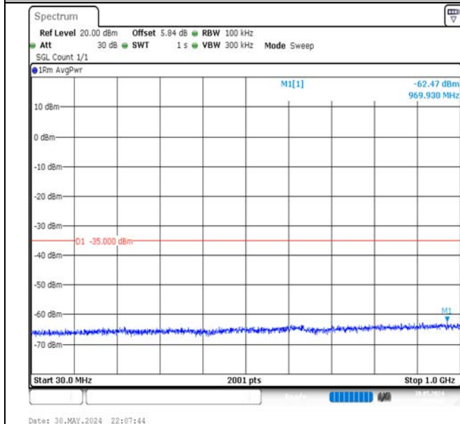
Band7-15MHz-16QAM-20825-75RB#0-30~1000-PASS
