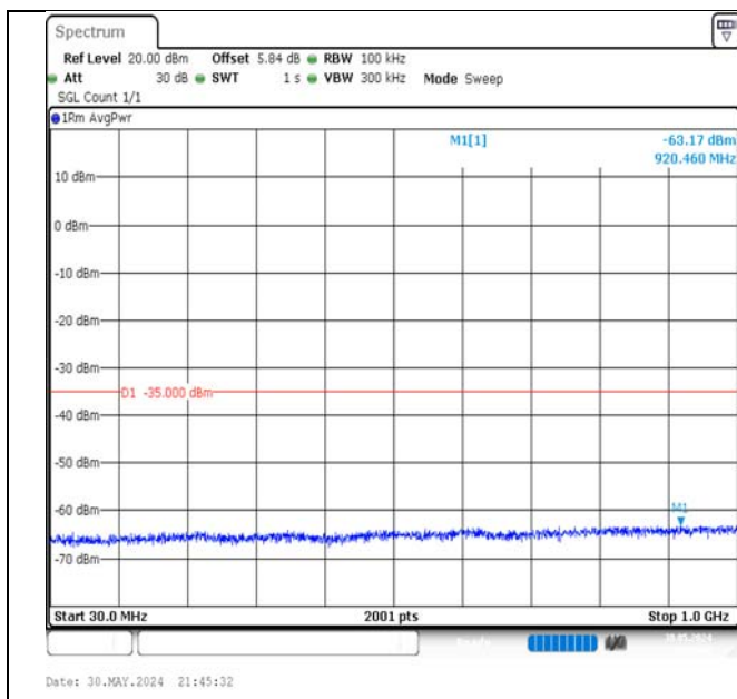
Band7-10MHz-16QAM-21100-50RB#0-30~1000-PASS
