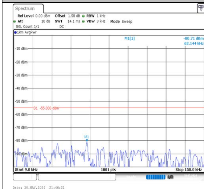
Band7-10MHz-16QAM-21400-1RB#0-0.009~0.15-PASS
