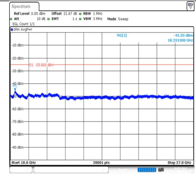
Band7-15MHz-QPSK-21375-1RB#74-18000~27000-PASS
