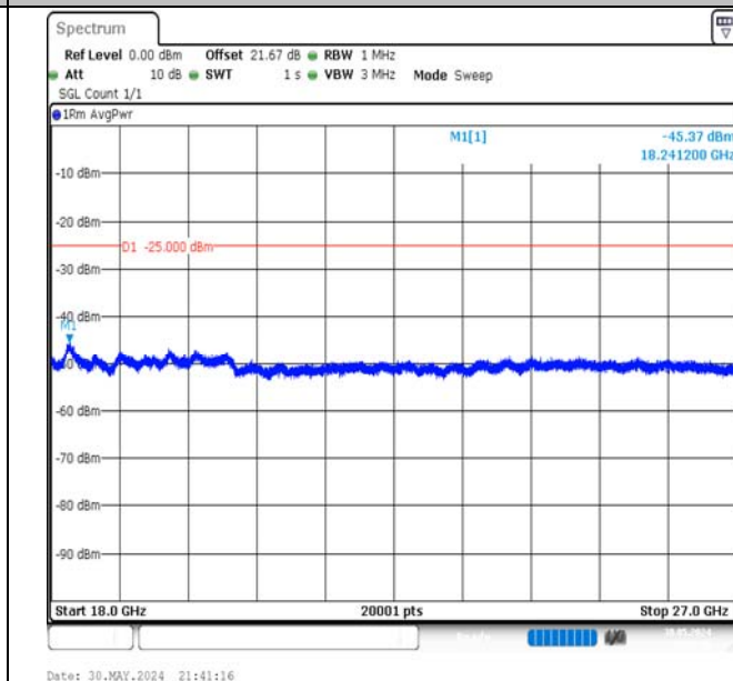
Band7-10MHz-16QAM-20800-1RB#0-18000~27000-PASS
