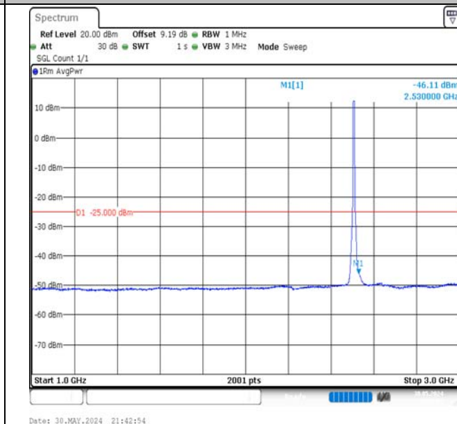
Band7-10MHz-16QAM-20800-50RB#0-1000~3000-PASS
