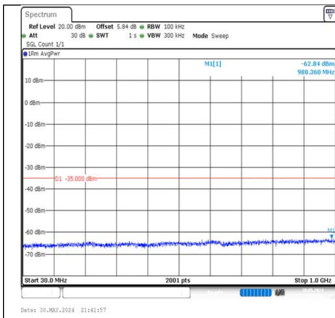
Band7-10MHz-16QAM-20800-1RB#49-30~1000-PASS
