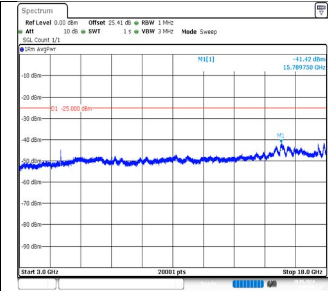
Band7-15MHz-16QAM-20825-75RB#0-3000~18000-PASS
