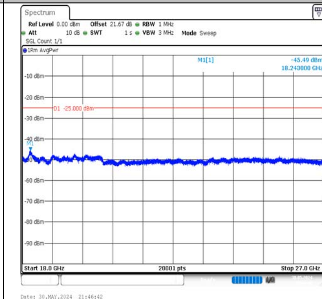
Band7-10MHz-16QAM-21400-1RB#0-18000~27000-PASS
