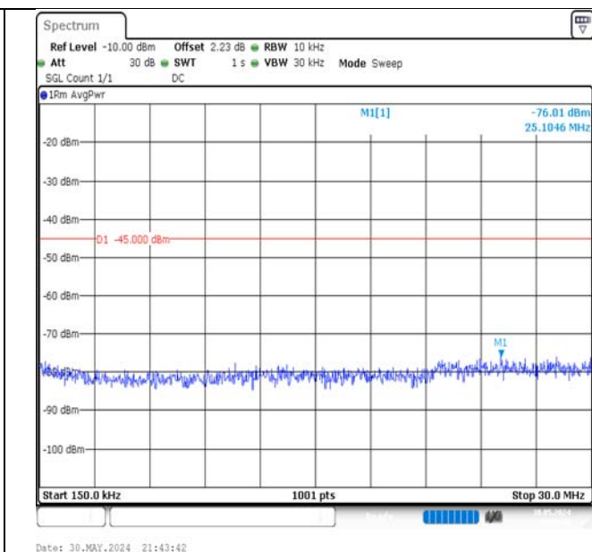
Band7-10MHz-16QAM-21100-1RB#0-0.15~30-PASS
