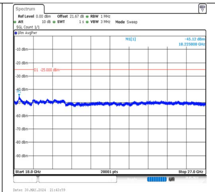
Band7-10MHz-16QAM-21100-1RB#0-18000~27000-PASS
