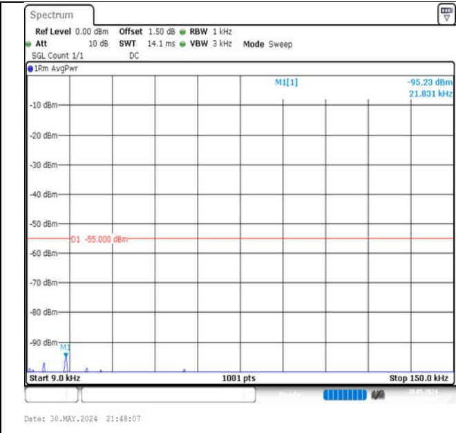
Band7-10MHz-16QAM-21400-50RB#0-0.009~0.15-PASS
