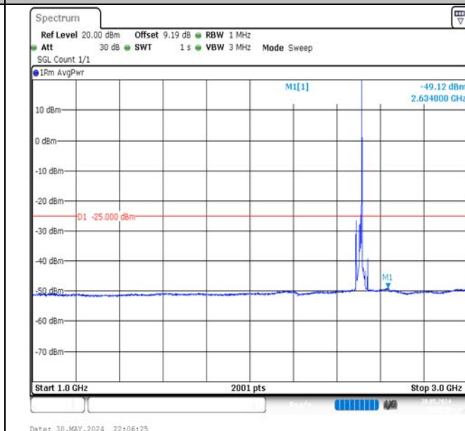
Band7-15MHz-QPSK-20825-1RB#74-1000~3000-PASS
