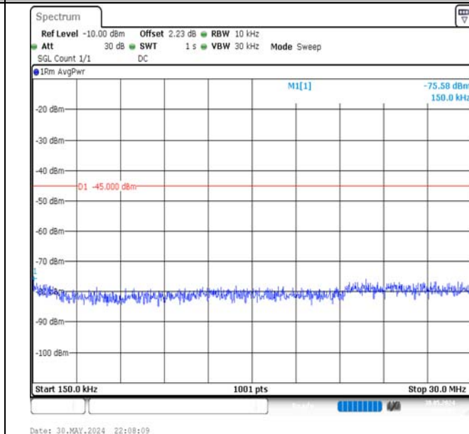
Band7-15MHz-QPSK-21100-1RB#0-0.15~30-PASS
