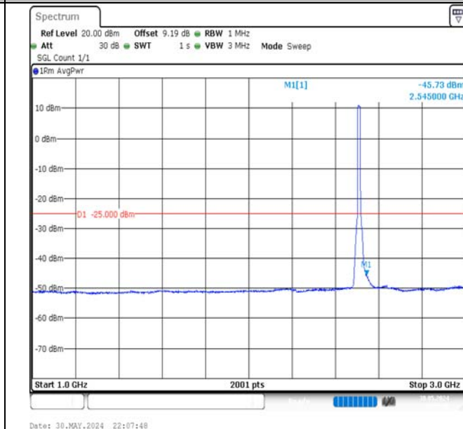
Band7-15MHz-16QAM-20825-75RB#0-1000~3000-PASS
