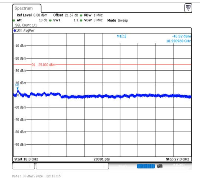
Band7-15MHz-QPSK-21100-75RB#0-18000~27000-PASS
