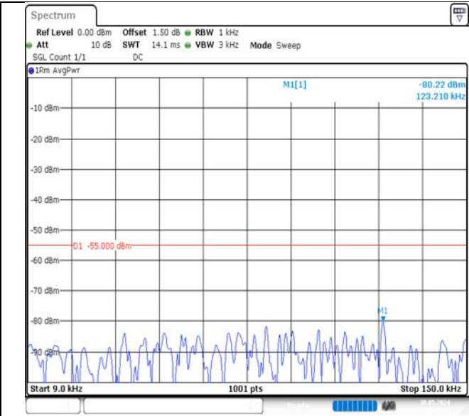
Band7-15MHz-QPSK-20825-1RB#0-0.009~0.15-PASS
