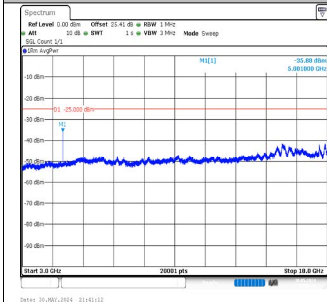
Band7-10MHz-16QAM-20800-1RB#0-3000~18000-PASS
