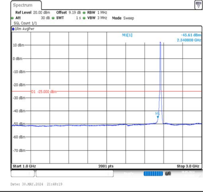
Band7-10MHz-16QAM-21400-50RB#0-1000~3000-PASS
