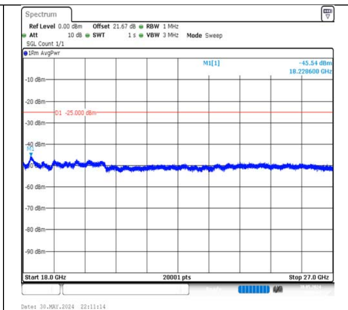
Band7-15MHz-QPSK-21375-1RB#0-18000~27000-PASS
