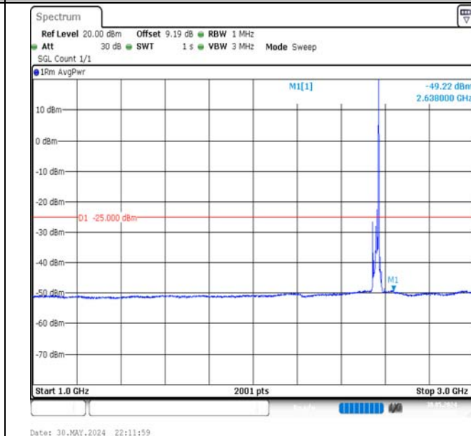
Band7-15MHz-QPSK-21375-1RB#74-1000~3000-PASS
