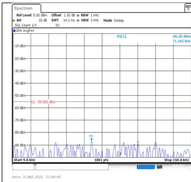
Band7-10MHz-QPSK-21400-1RB#49-0.009~0.15-PASS
