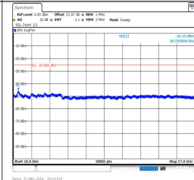
Band7-15MHz-QPSK-21375-75RB#0-18000~27000-PASS
