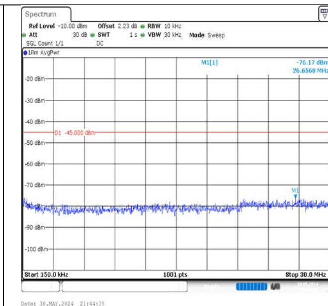
Band7-10MHz-16QAM-21100-1RB#49-0.15~30-PASS
