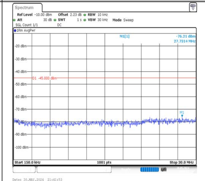
Band7-10MHz-16QAM-20800-1RB#49-0.15~30-PASS
