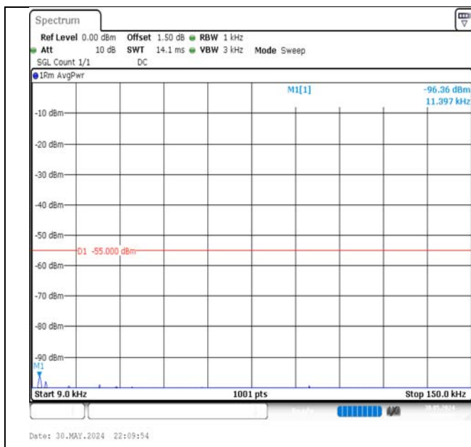
Band7-15MHz-QPSK-21100-75RB#0-0.009~0.15-PASS
