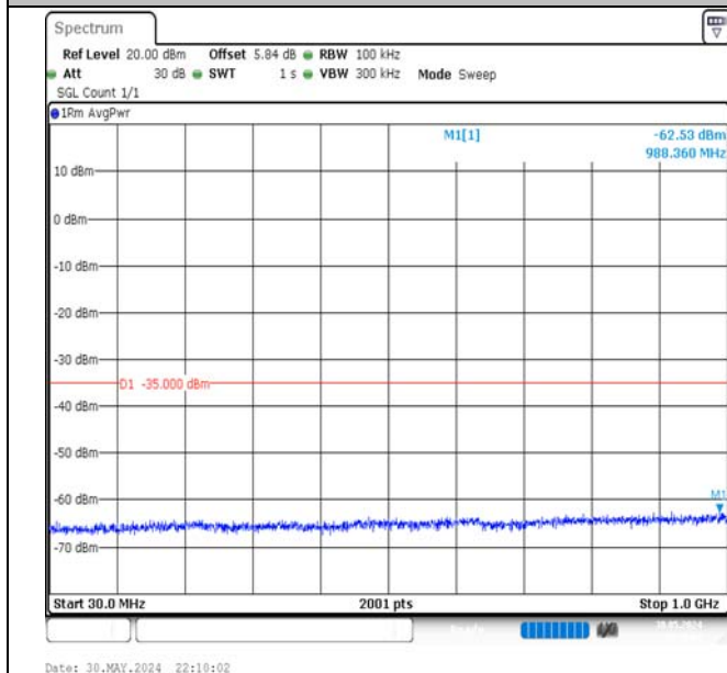
Band7-15MHz-QPSK-21100-75RB#0-30~1000-PASS
