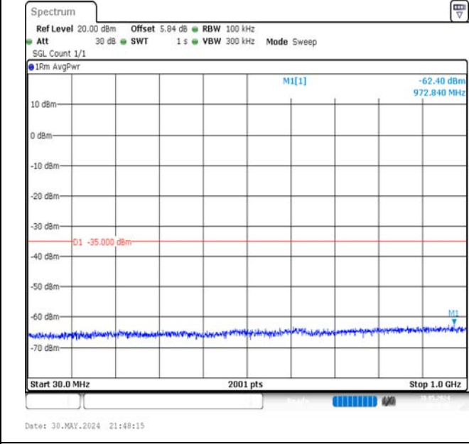
Band7-10MHz-16QAM-21400-50RB#0-30~1000-PASS
