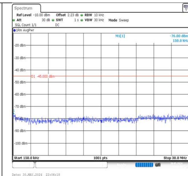
Band7-15MHz-QPSK-20825-1RB#74-0.15~30-PASS
