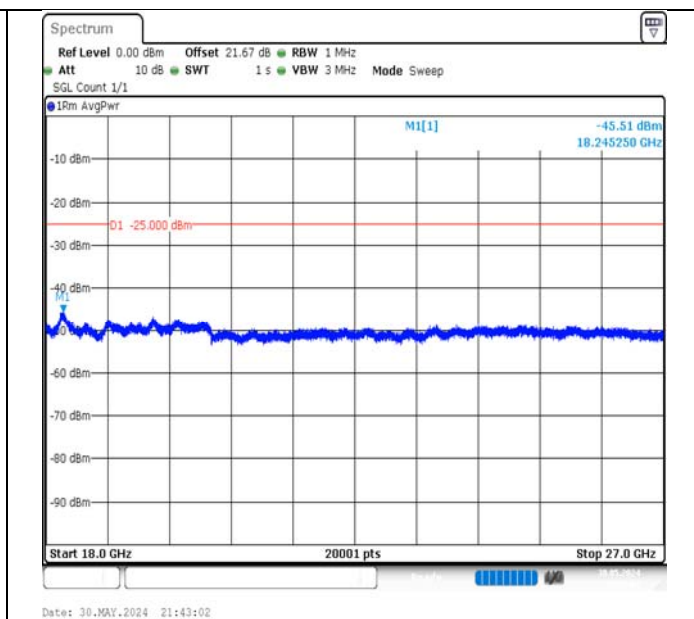
Band7-10MHz-16QAM-20800-50RB#0-18000~27000-PASS
