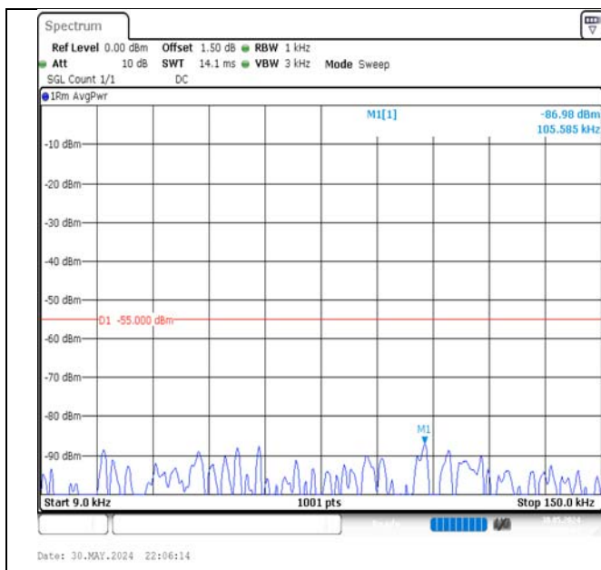
Band7-15MHz-QPSK-20825-1RB#74-0.009~0.15-PASS
