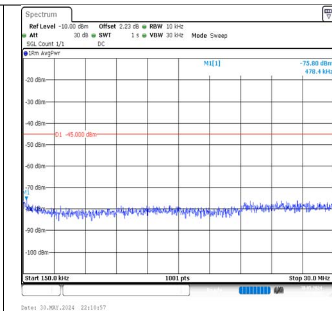
Band7-15MHz-QPSK-21375-1RB#0-0.15~30-PASS
