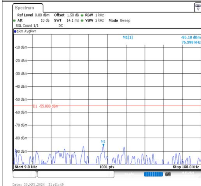
Band7-10MHz-16QAM-20800-1RB#49-0.009~0.15-PASS
