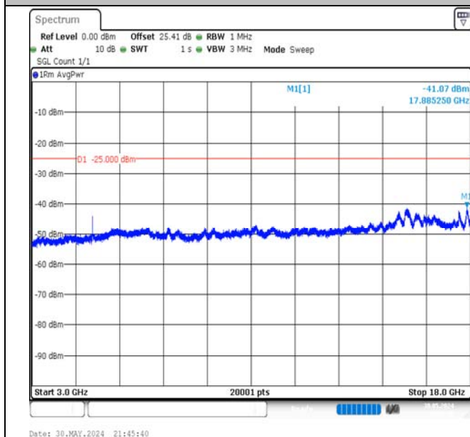
Band7-10MHz-16QAM-21100-50RB#0-3000~18000-PASS
