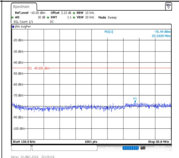
Band7-15MHz-QPSK-21100-1RB#74-0.15~30-PASS
