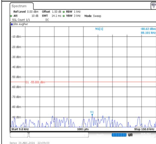
Band7-15MHz-QPSK-21100-1RB#74-0.009~0.15-PASS
