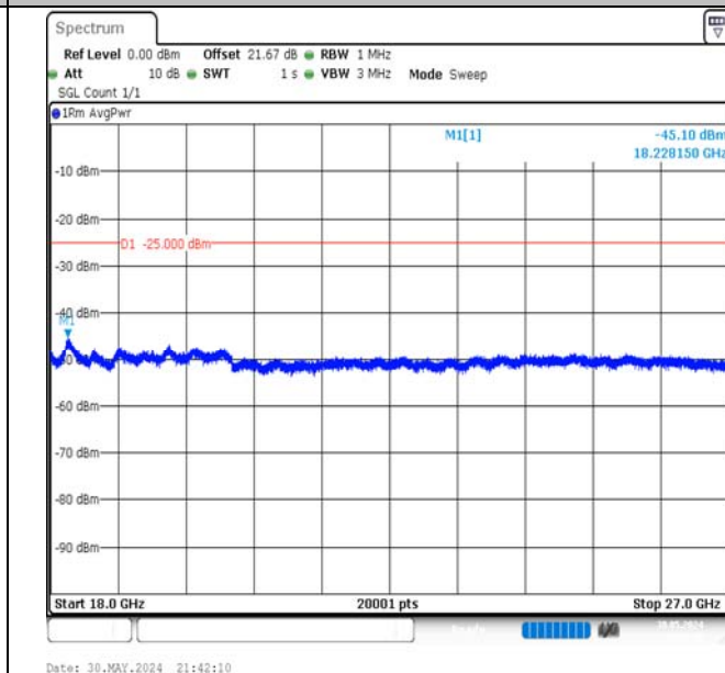
Band7-10MHz-16QAM-20800-1RB#49-18000~27000-PASS
