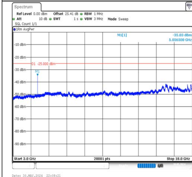
Band7-15MHz-QPSK-21100-1RB#0-3000~18000-PASS
