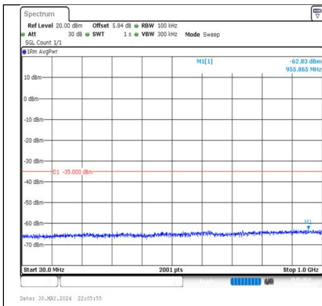
Band7-15MHz-16QAM-20825-1RB#0-30~1000-PASS
