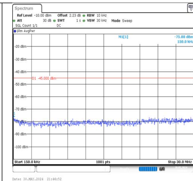
Band7-10MHz-QPSK-21400-1RB#49-0.15~30-PASS
