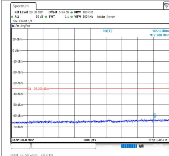
Band7-15MHz-QPSK-21375-1RB#0-30~1000-PASS
