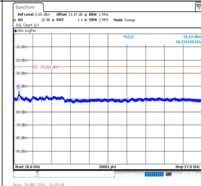
Band7-15MHz-QPSK-21100-1RB#0-18000~27000-PASS
