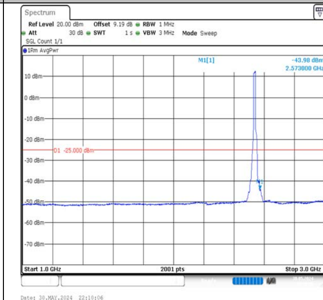
Band7-15MHz-QPSK-21100-75RB#0-1000~3000-PASS
