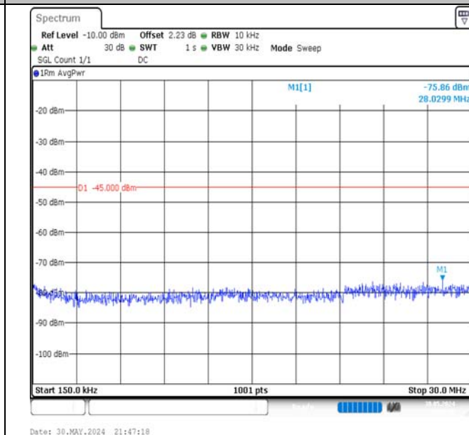
Band7-10MHz-16QAM-21400-1RB#49-0.15~30-PASS
