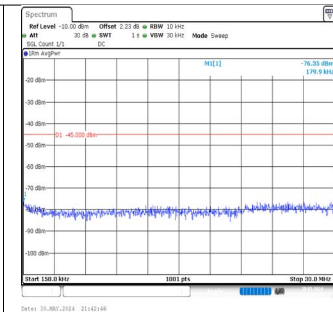
Band7-10MHz-16QAM-20800-50RB#0-0.15~30-PASS
