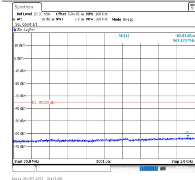
Band7-10MHz-QPSK-21400-1RB#49-30~1000-PASS
