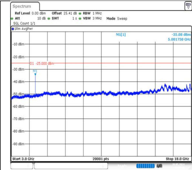
Band7-15MHz-QPSK-20825-1RB#0-3000~18000-PASS
