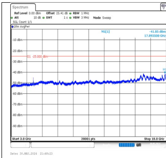
Band7-10MHz-16QAM-21400-50RB#0-3000~18000-PASS
