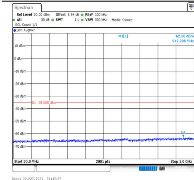
Band7-10MHz-16QAM-20800-50RB#0-30~1000-PASS
