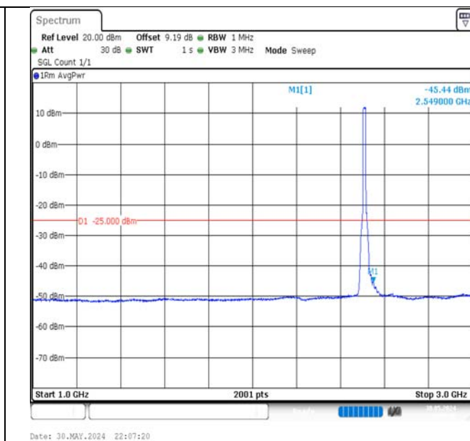
Band7-15MHz-QPSK-20825-75RB#0-1000~3000-PASS
