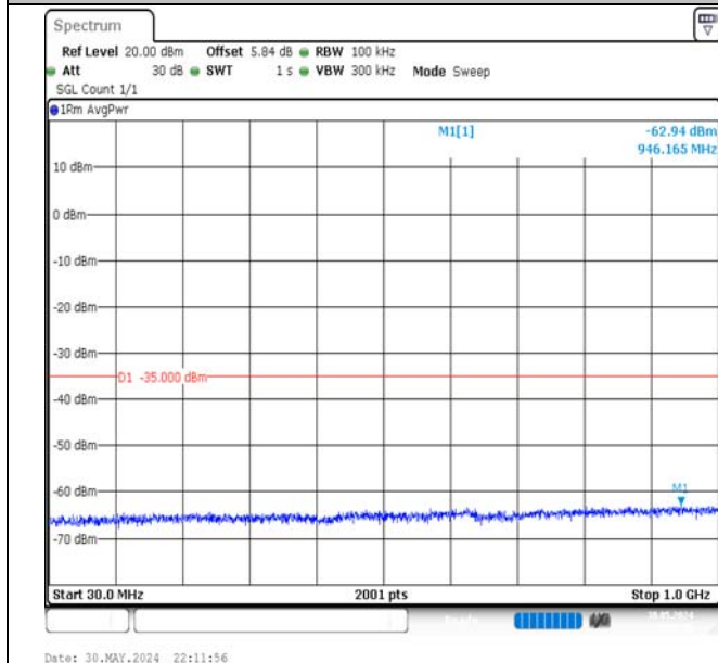
Band7-15MHz-QPSK-21375-1RB#74-30~1000-PASS
