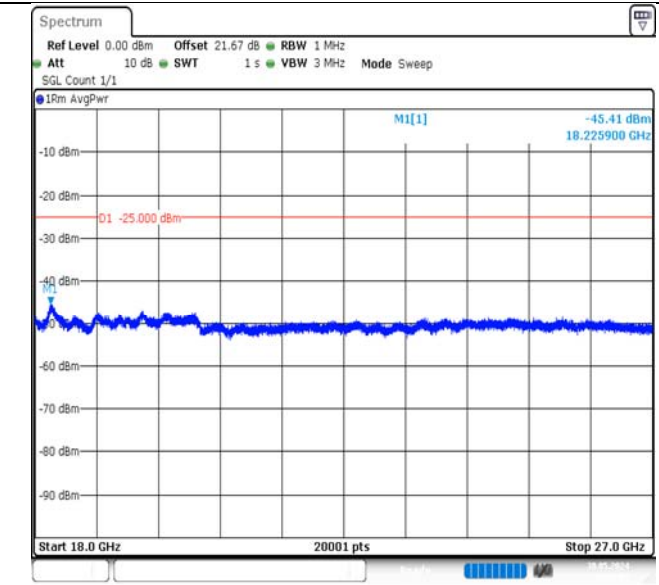
Band7-10MHz-QPSK-21400-1RB#49-18000~27000-PASS
