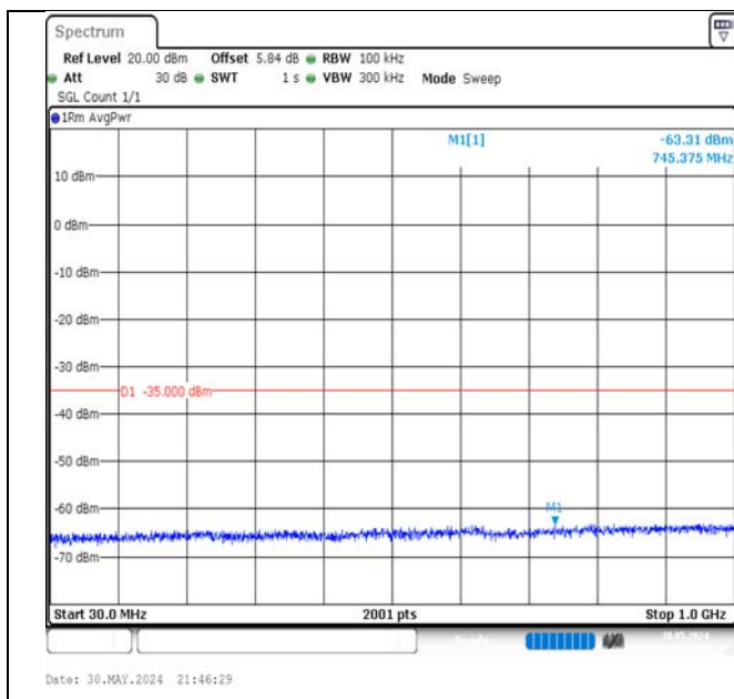
Band7-10MHz-16QAM-21400-1RB#0-30~1000-PASS
