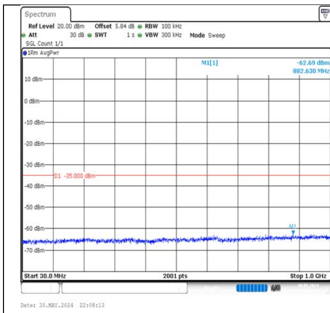
Band7-15MHz-QPSK-21100-1RB#0-30~1000-PASS
