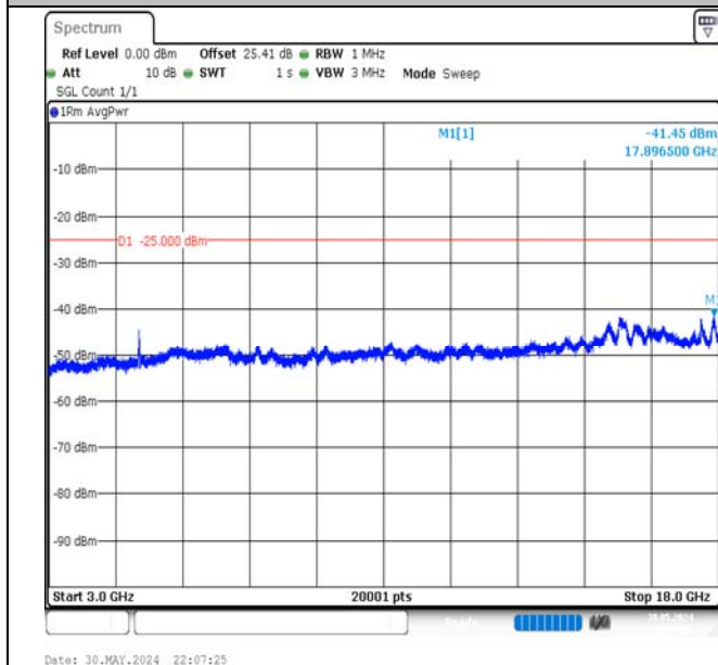
Band7-15MHz-QPSK-20825-75RB#0-3000~18000-PASS
