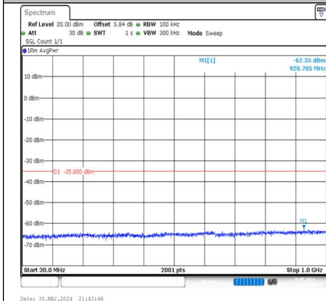
Band7-10MHz-16QAM-21100-1RB#0-30~1000-PASS
