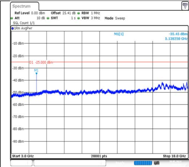
Band7-15MHz-QPSK-21375-1RB#74-3000~18000-PASS
