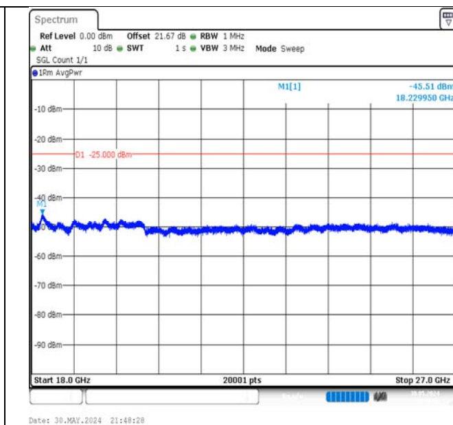
Band7-10MHz-16QAM-21400-50RB#0-18000~27000-PASS
