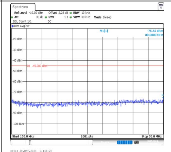
Band7-10MHz-16QAM-21400-1RB#0-0.15~30-PASS
