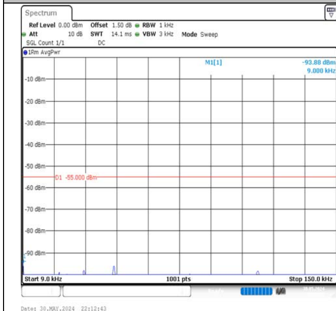
Band7-15MHz-QPSK-21375-75RB#0-0.009~0.15-PASS
