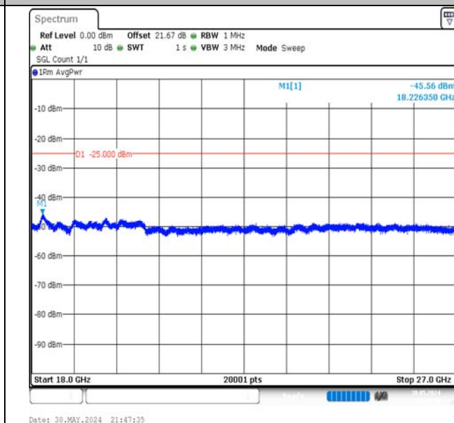
Band7-10MHz-16QAM-21400-1RB#49-18000~27000-PASS
