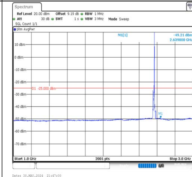
Band7-10MHz-QPSK-21400-1RB#49-1000~3000-PASS
