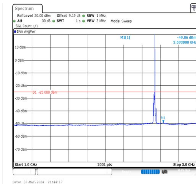
Band7-10MHz-QPSK-21100-1RB#49-1000~3000-PASS
