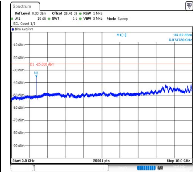
Band7-5MHz-16QAM-21100-1RB#24-3000~18000-PASS
