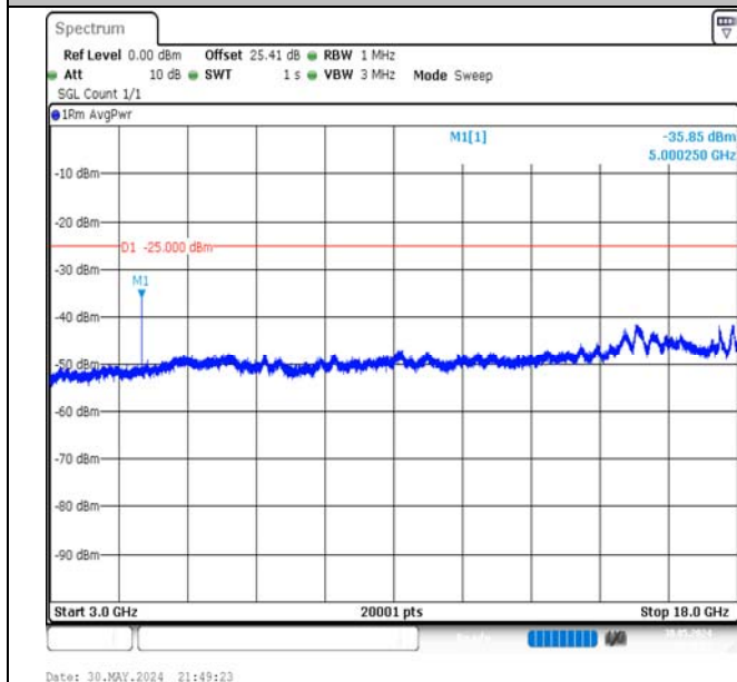
Band7-5MHz-16QAM-20775-1RB#0-3000~18000-PASS
