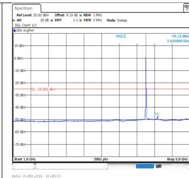
Band7-5MHz-16QAM-20775-1RB#0-1000~3000-PASS
