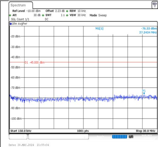
Band7-5MHz-QPSK-21425-1RB#24-0.15~30-PASS
