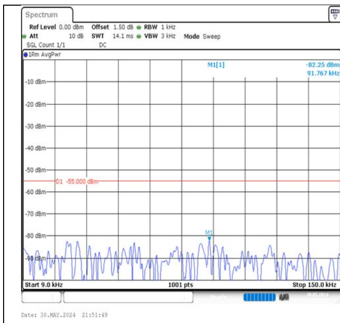
Band7-5MHz-16QAM-21100-1RB#0-0.009~0.15-PASS
