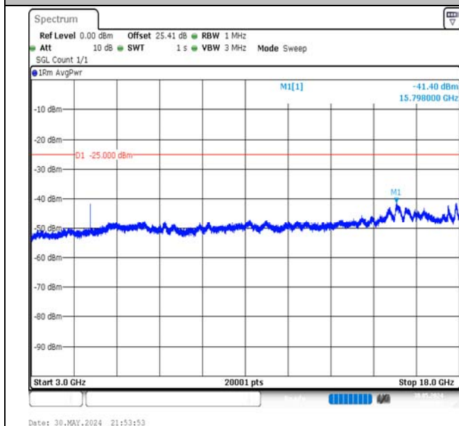
Band7-5MHz-16QAM-21100-25RB#0-3000~18000-PASS
