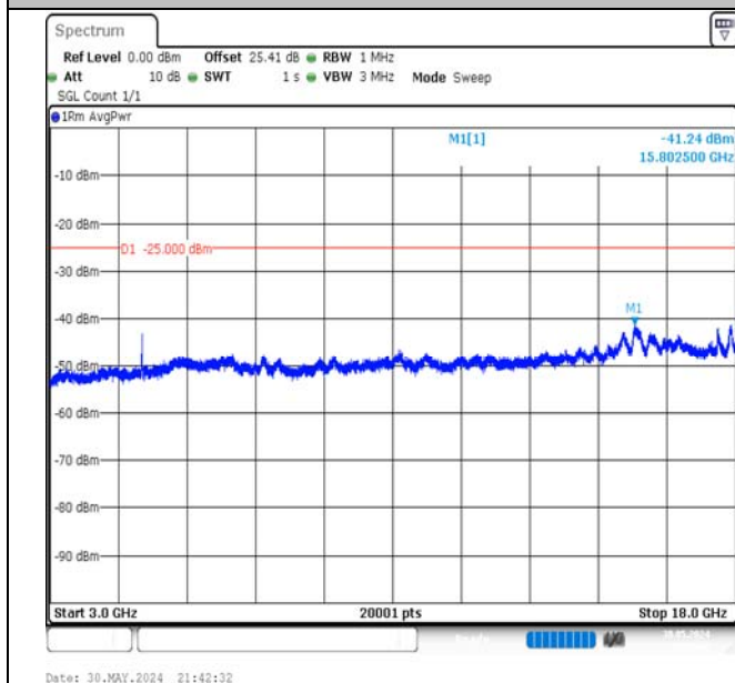
Band7-10MHz-QPSK-20800-50RB#0-3000~18000-PASS
