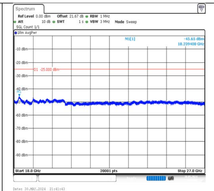
Band7-10MHz-QPSK-20800-1RB#49-18000~27000-PASS
