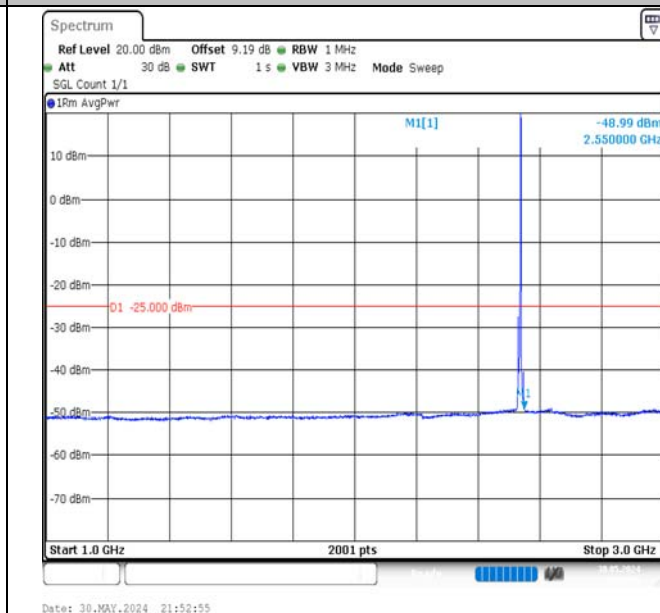
Band7-5MHz-16QAM-21100-1RB#24-1000~3000-PASS
