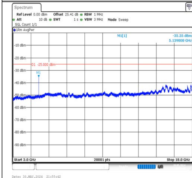
Band7-5MHz-16QAM-21425-1RB#24-3000~18000-PASS
