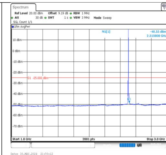
Band7-5MHz-16QAM-20775-1RB#24-1000~3000-PASS
