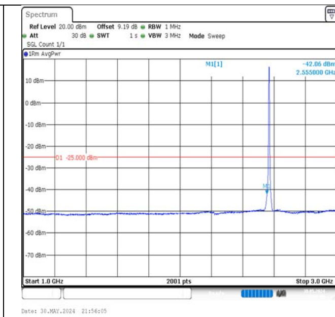
Band7-5MHz-QPSK-21425-25RB#0-1000~3000-PASS
