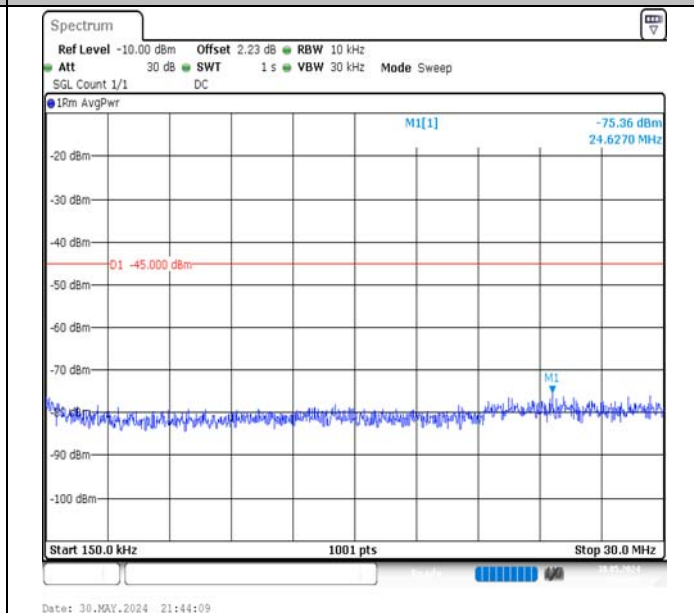
Band7-10MHz-QPSK-21100-1RB#49-0.15~30-PASS
