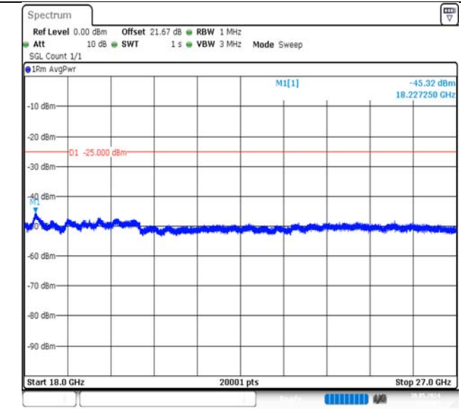
Band7-5MHz-16QAM-21100-1RB#24-18000~27000-PASS
