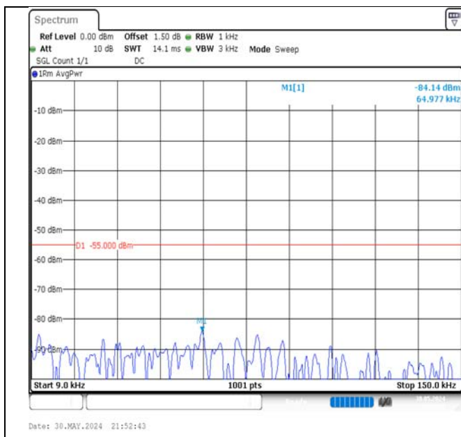
Band7-5MHz-16QAM-21100-1RB#24-0.009~0.15-PASS
