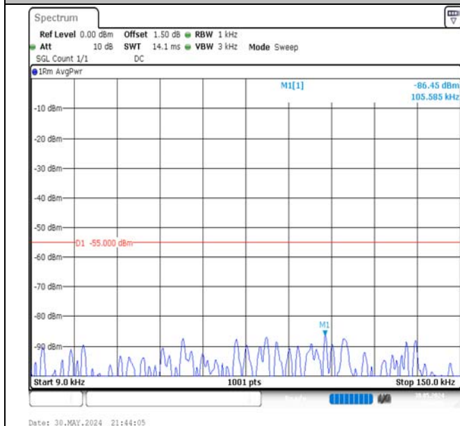
Band7-10MHz-QPSK-21100-1RB#49-0.009~0.15-PASS
