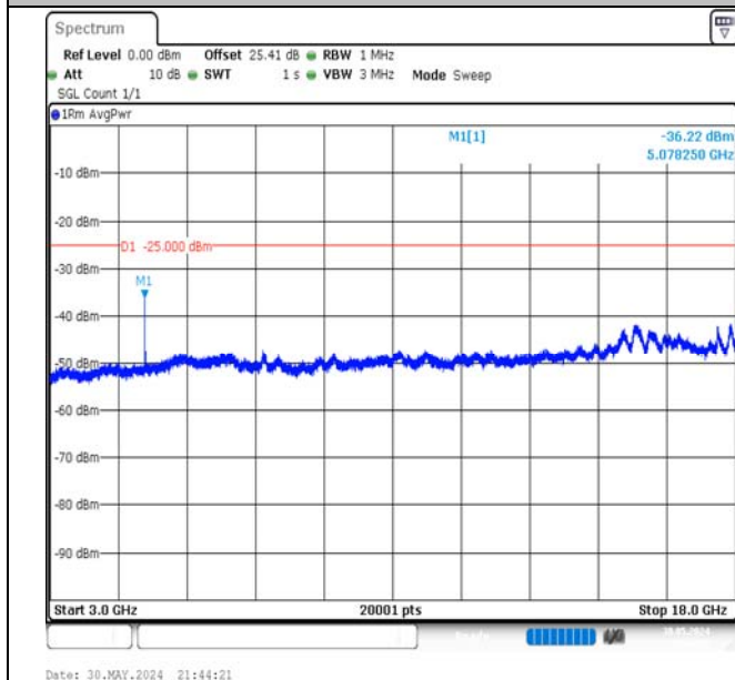
Band7-10MHz-QPSK-21100-1RB#49-3000~18000-PASS
