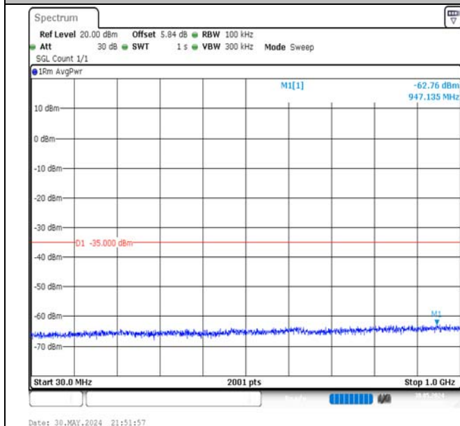
Band7-5MHz-16QAM-21100-1RB#0-30~1000-PASS
