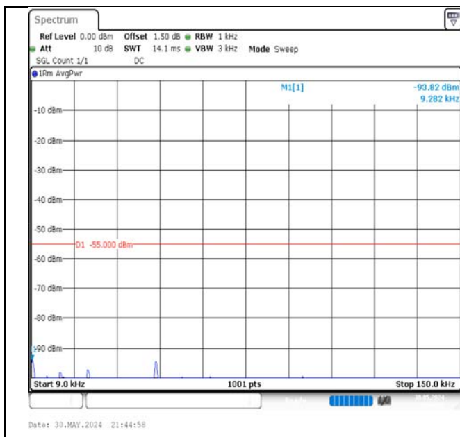
Band7-10MHz-QPSK-21100-50RB#0-0.009~0.15-PASS
