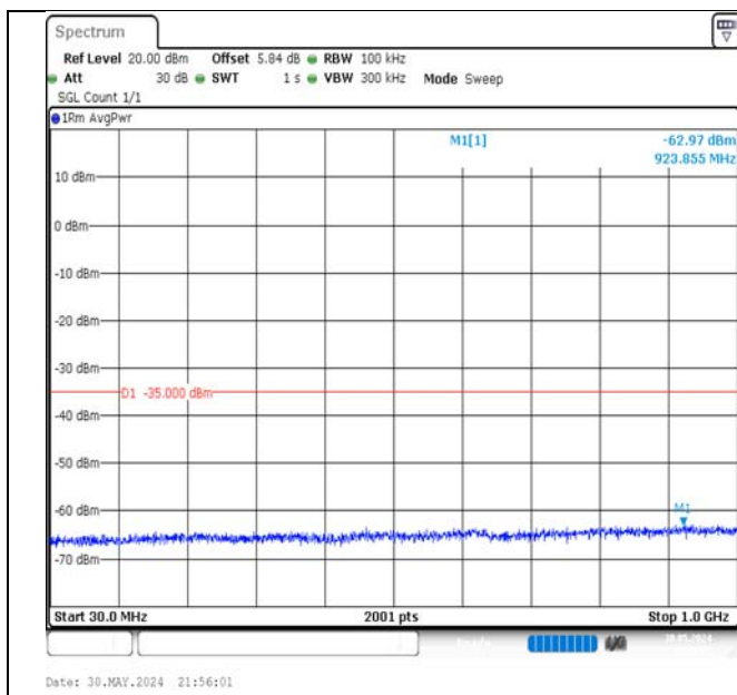
Band7-5MHz-QPSK-21425-25RB#0-30~1000-PASS
