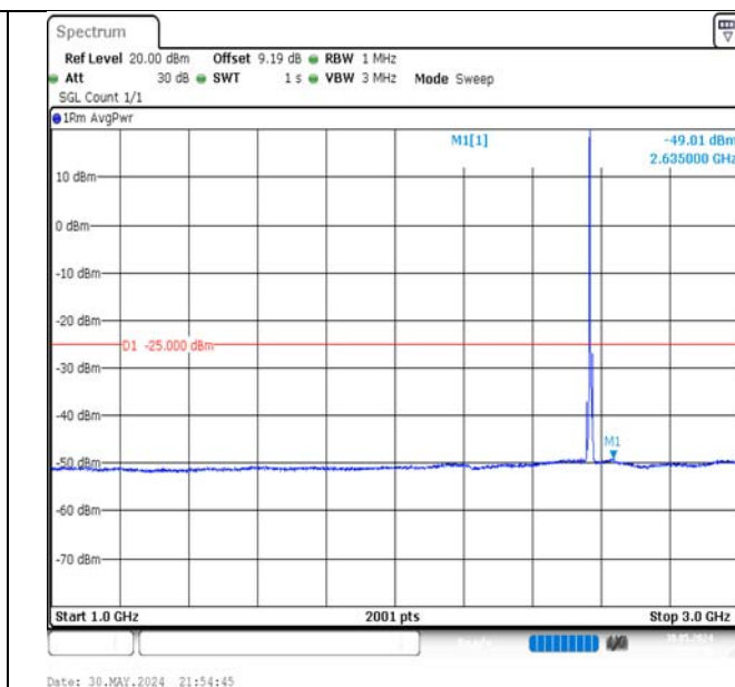
Band7-5MHz-16QAM-21425-1RB#0-1000~3000-PASS
