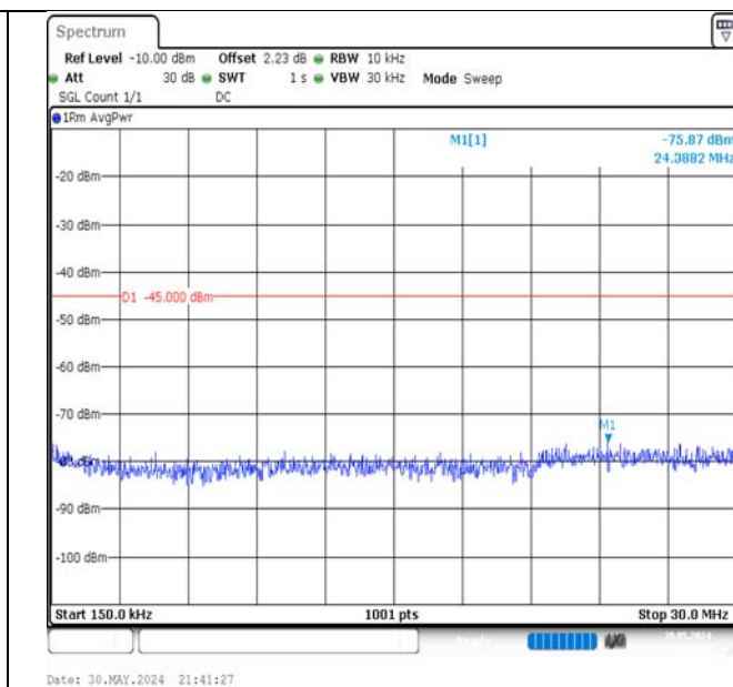
Band7-10MHz-QPSK-20800-1RB#49-0.15~30-PASS
