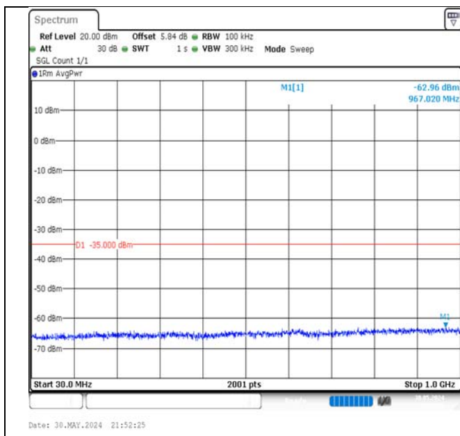
Band7-5MHz-QPSK-21100-1RB#24-30~1000-PASS
