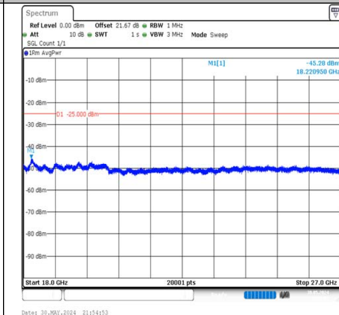
Band7-5MHz-16QAM-21425-1RB#0-18000~27000-PASS
