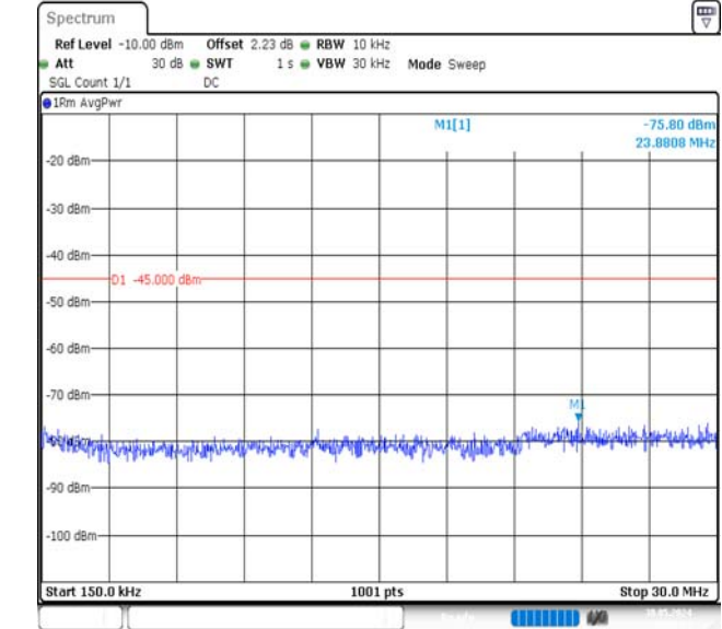
Band7-5MHz-QPSK-21100-25RB#0-18000~27000-PASS
