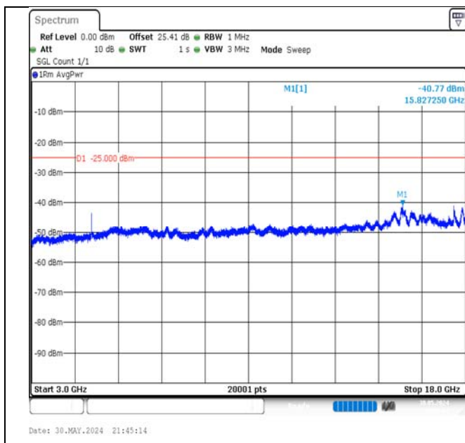
Band7-10MHz-QPSK-21100-50RB#0-3000~18000-PASS
