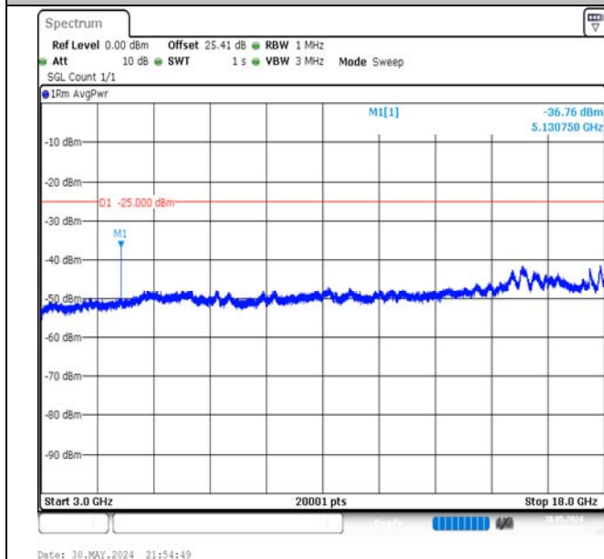
Band7-5MHz-16QAM-21425-1RB#0-3000~18000-PASS
