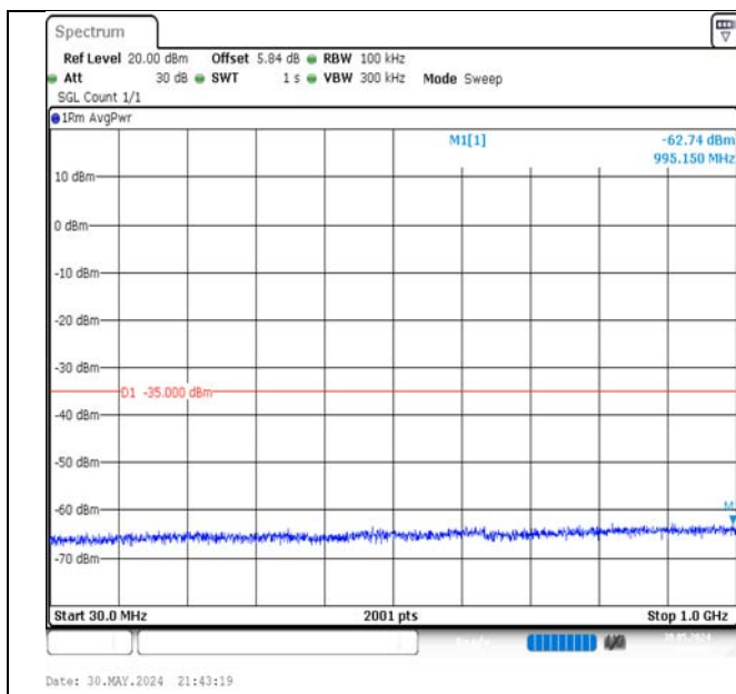
Band7-10MHz-QPSK-21100-1RB#0-30~1000-PASS
