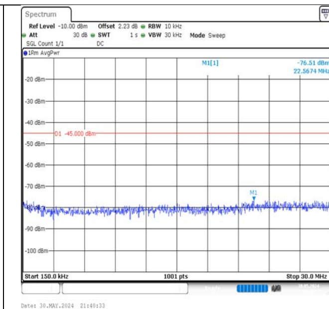
Band7-10MHz-QPSK-20800-1RB#0-0.15~30-PASS
