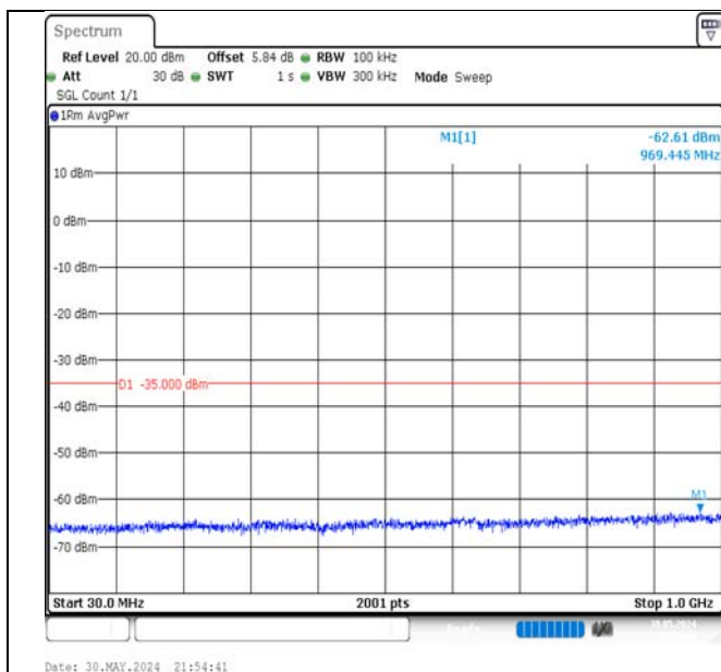
Band7-5MHz-16QAM-21425-1RB#0-30~1000-PASS
