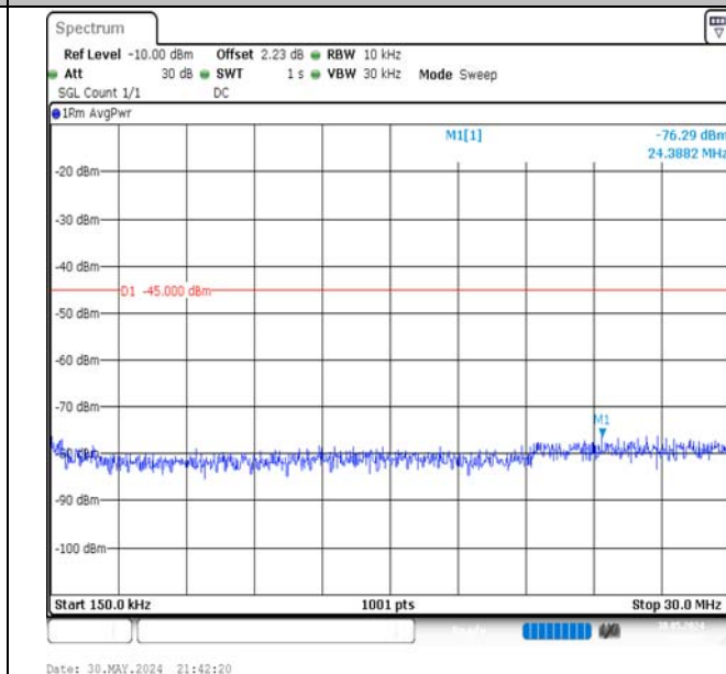
Band7-10MHz-QPSK-20800-50RB#0-0.15~30-PASS
