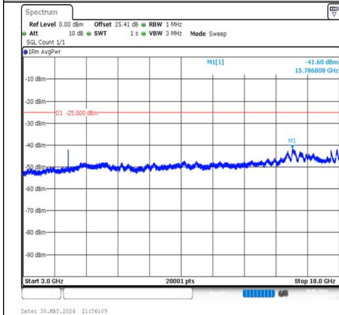
Band7-5MHz-QPSK-21425-25RB#0-3000~18000-PASS
