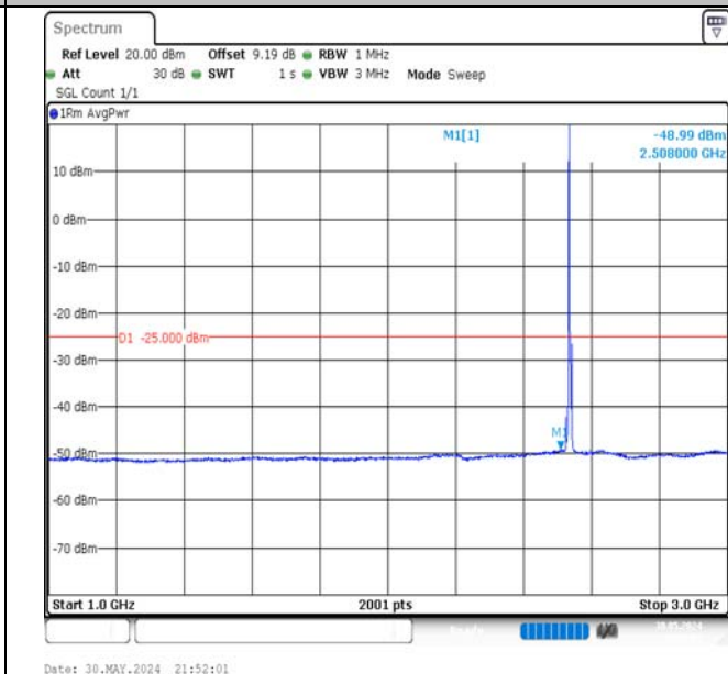
Band7-5MHz-16QAM-21100-1RB#0-1000~3000-PASS
