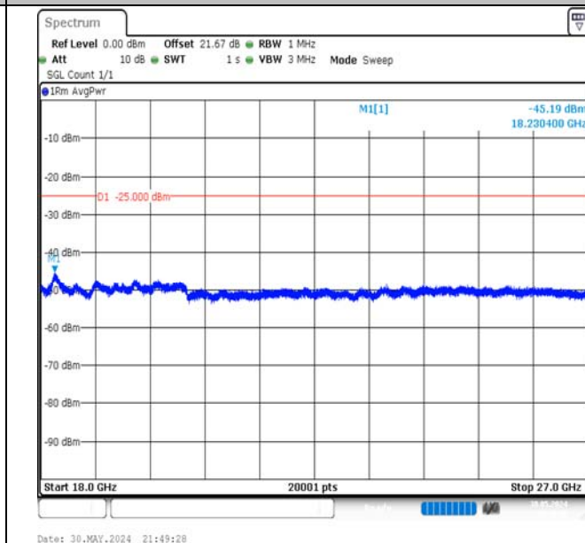
Band7-5MHz-16QAM-20775-1RB#0-18000~27000-PASS
