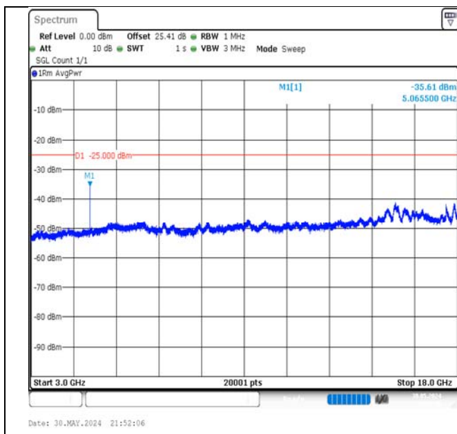
Band7-5MHz-16QAM-21100-1RB#0-3000~18000-PASS
