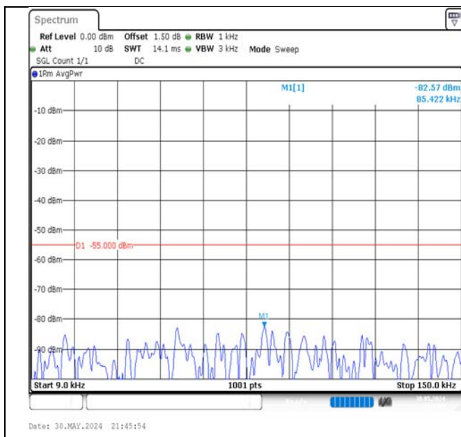
Band7-10MHz-QPSK-21400-1RB#0-0.009~0.15-PASS
