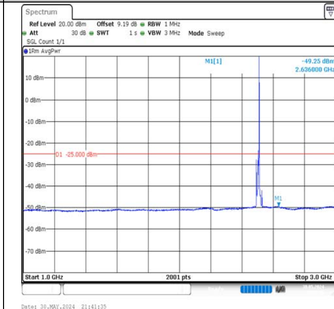
Band7-10MHz-QPSK-20800-1RB#49-1000~3000-PASS
