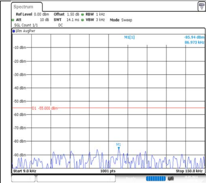
Band7-5MHz-QPSK-21425-1RB#0-0.009~0.15-PASS
