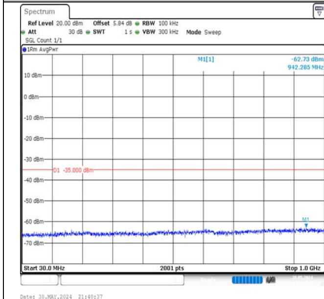
Band7-10MHz-QPSK-20800-1RB#0-30~1000-PASS
