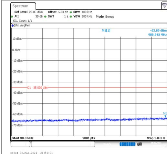
Band7-5MHz-16QAM-20775-25RB#0-30~1000-PASS
