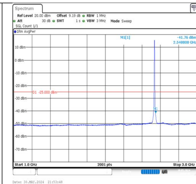
Band7-5MHz-16QAM-21100-25RB#0-1000~3000-PASS
