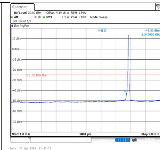
Band7-10MHz-QPSK-21400-50RB#0-1000~3000-PASS
