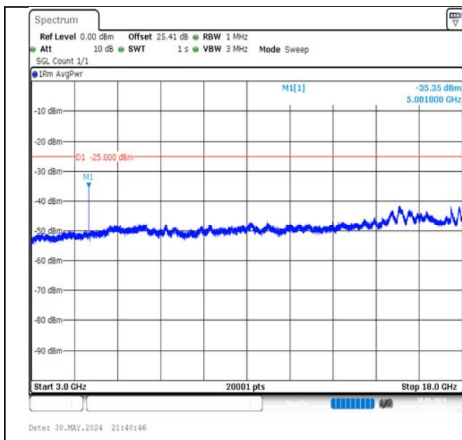
Band7-10MHz-QPSK-20800-1RB#0-3000~18000-PASS
