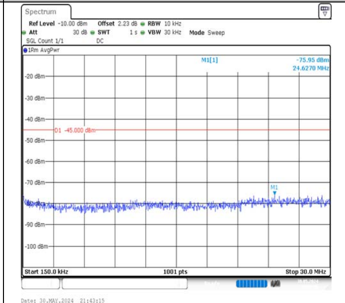
Band7-10MHz-QPSK-21100-1RB#0-0.15~30-PASS
