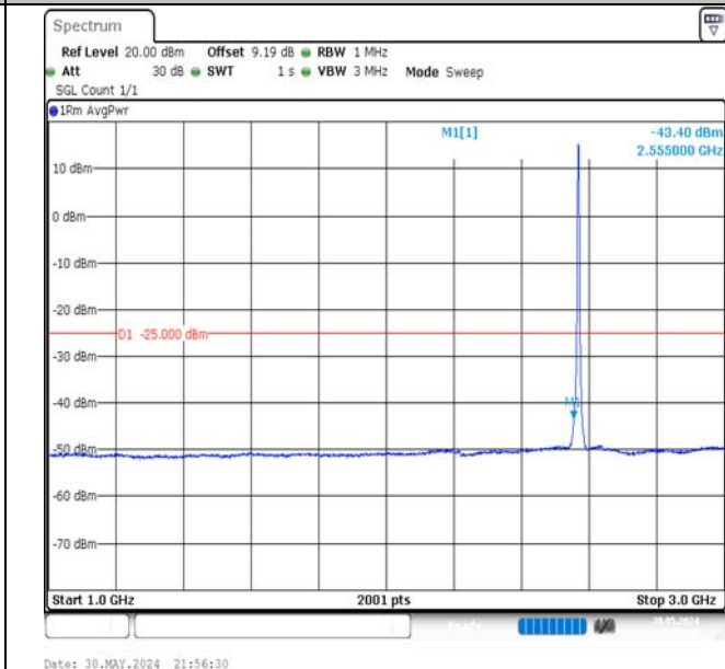
Band7-5MHz-16QAM-21425-25RB#0-1000~3000-PASS
