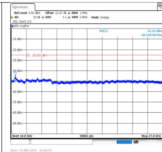
Band7-10MHz-QPSK-20800-1RB#0-18000~27000-PASS
