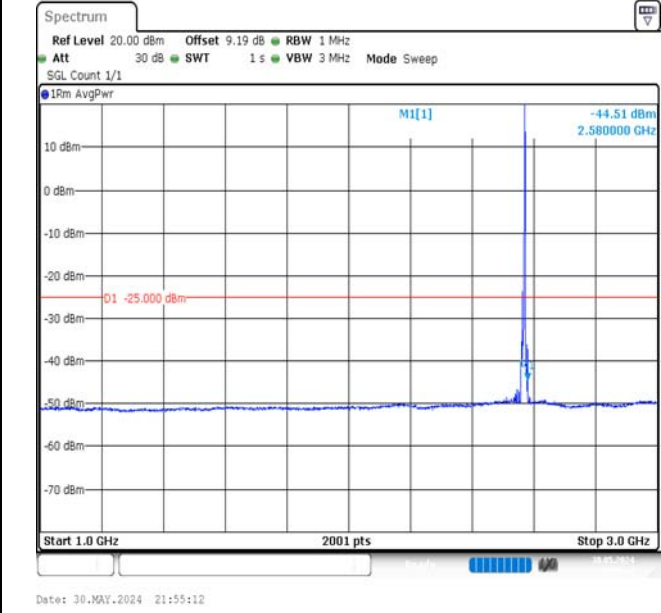
Band7-5MHz-QPSK-21425-1RB#24-1000~3000-PASS
