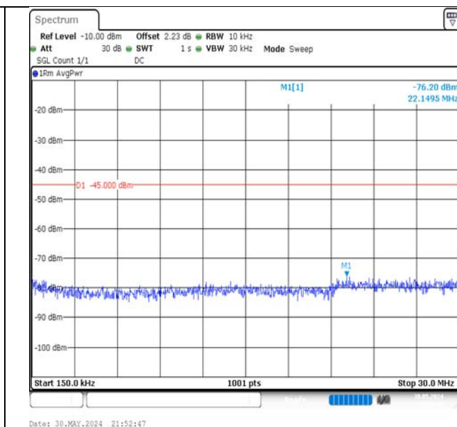
Band7-5MHz-16QAM-21100-1RB#24-0.15~30-PASS
