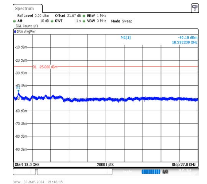
Band7-10MHz-QPSK-21400-1RB#0-18000~27000-PASS
