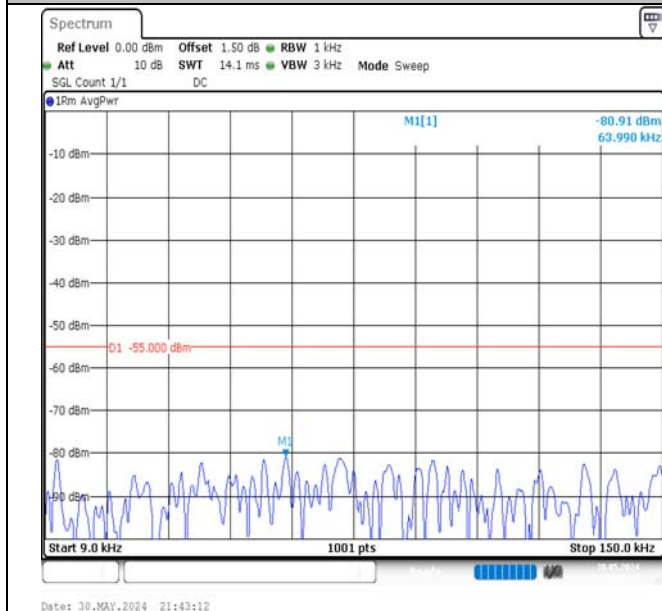
Band7-10MHz-QPSK-21100-1RB#0-0.009~0.15-PASS
