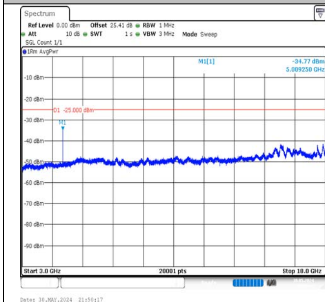
Band7-5MHz-16QAM-20775-1RB#24-3000~18000-PASS
