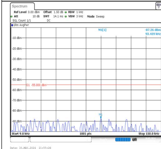
Band7-5MHz-16QAM-21425-1RB#24-0.009~0.15-PASS
