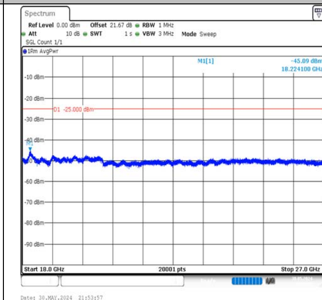
Band7-5MHz-16QAM-21100-25RB#0-18000~27000-PASS
