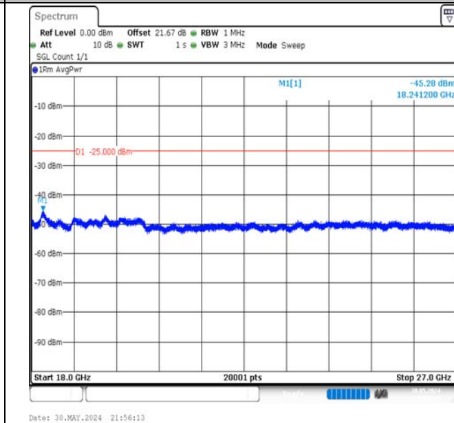
Band7-5MHz-QPSK-21425-25RB#0-18000~27000-PASS
