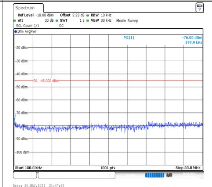
Band7-10MHz-QPSK-21400-50RB#0-0.15~30-PASS
