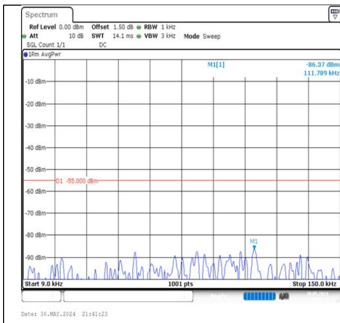
Band7-10MHz-QPSK-20800-1RB#49-0.009~0.15-PASS
