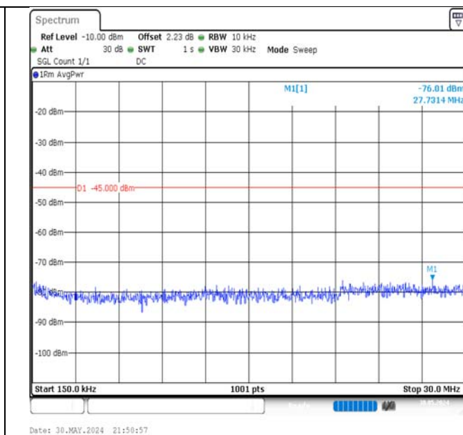
Band7-5MHz-16QAM-20775-25RB#0-0.15~30-PASS
