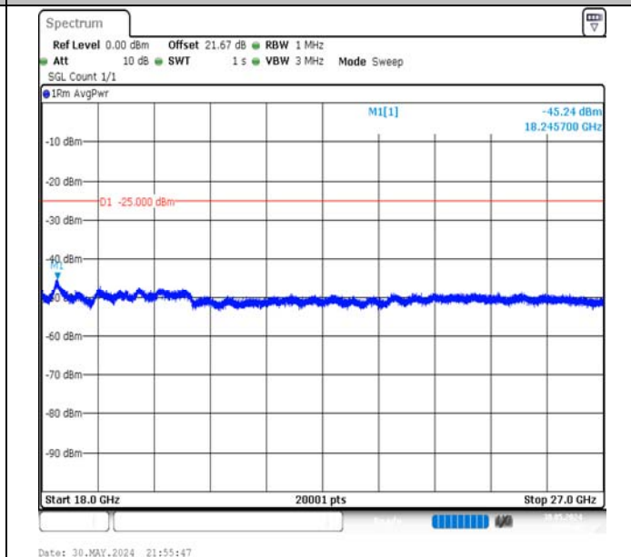
Band7-5MHz-16QAM-21425-1RB#24-18000~27000-PASS
