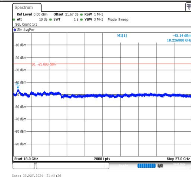
Band7-10MHz-QPSK-21100-1RB#49-18000~27000-PASS
