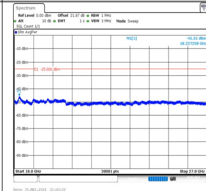
Band7-10MHz-QPSK-21100-1RB#0-18000~27000-PASS
