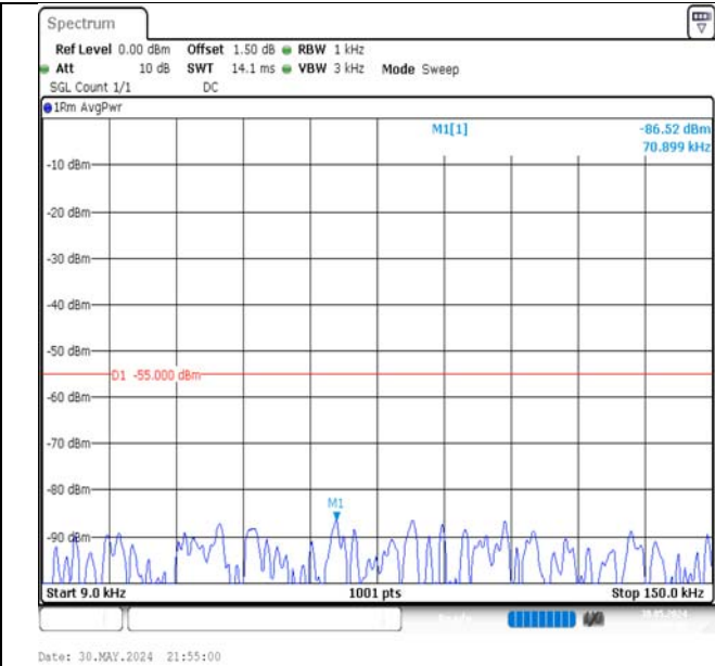
Band7-5MHz-QPSK-21425-1RB#24-0.009~0.15-PASS
