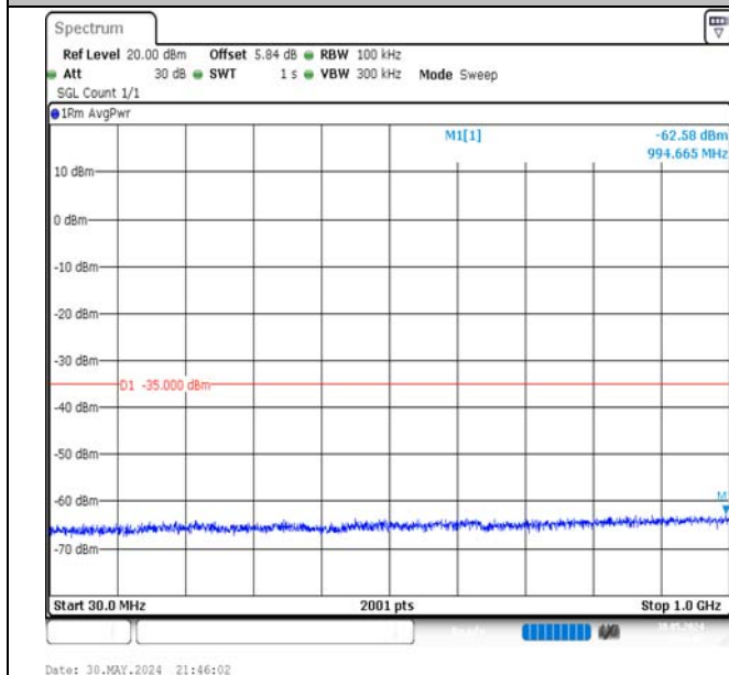
Band7-10MHz-QPSK-21400-1RB#0-30~1000-PASS
