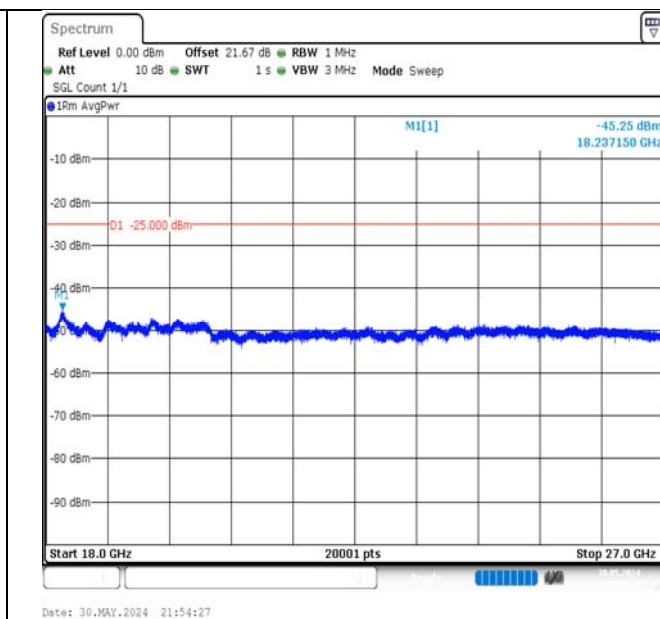
Band7-5MHz-QPSK-21425-1RB#0-18000~27000-PASS
