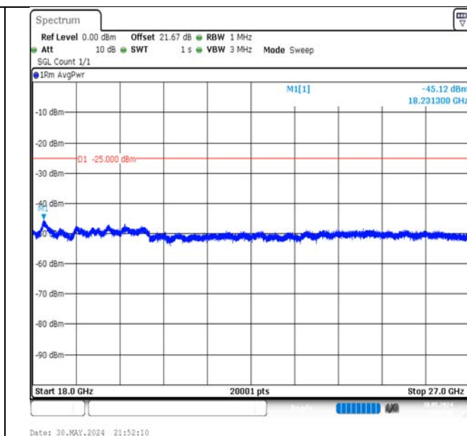
Band7-5MHz-16QAM-21100-1RB#0-18000~27000-PASS
