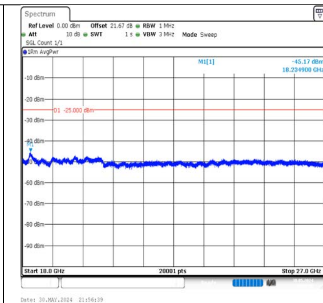
Band7-5MHz-16QAM-21425-25RB#0-18000~27000-PASS
