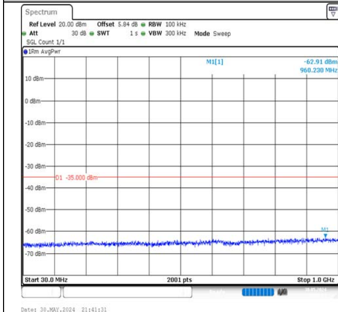
Band7-10MHz-QPSK-20800-1RB#49-30~1000-PASS
