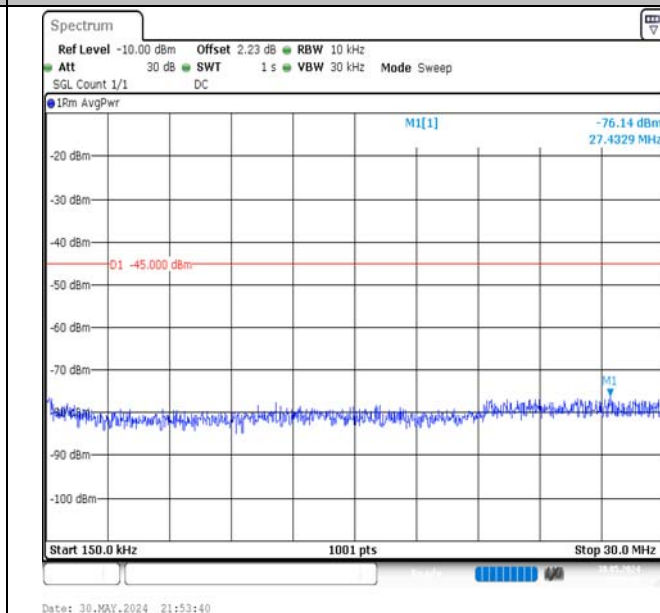
Band7-5MHz-16QAM-21100-25RB#0-0.15~30-PASS
