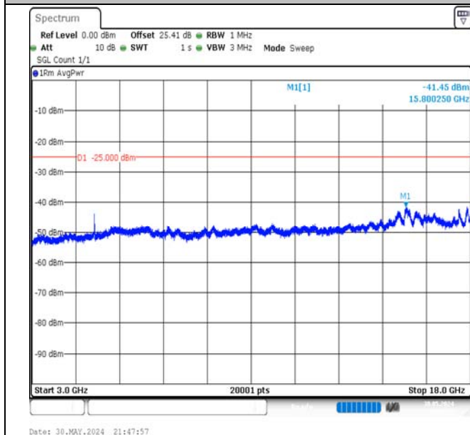
Band7-10MHz-QPSK-21400-50RB#0-3000~18000-PASS
