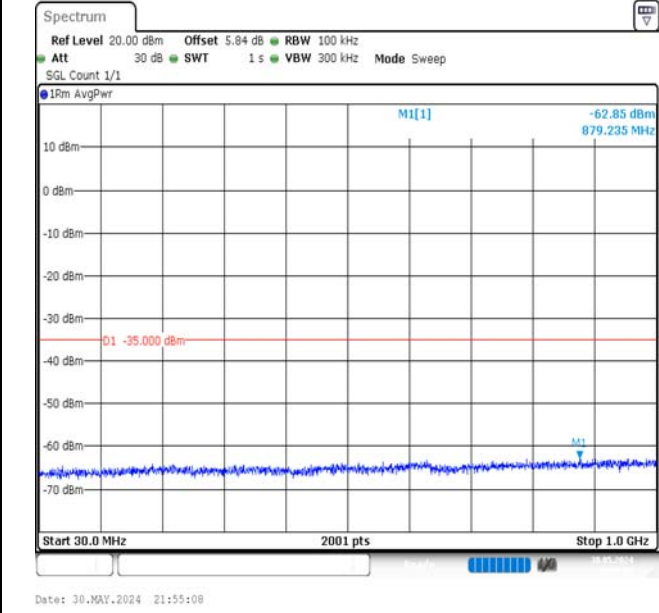
Band7-5MHz-QPSK-21425-1RB#24-30~1000-PASS
