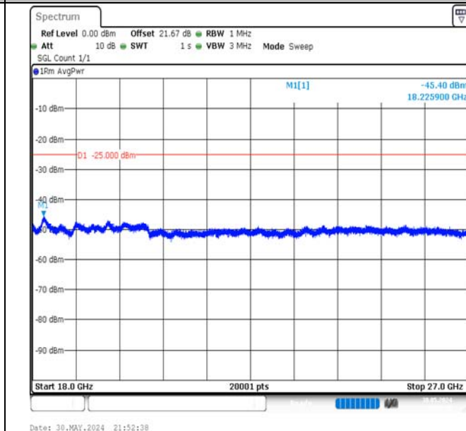
Band7-5MHz-QPSK-21100-1RB#24-18000~27000-PASS
