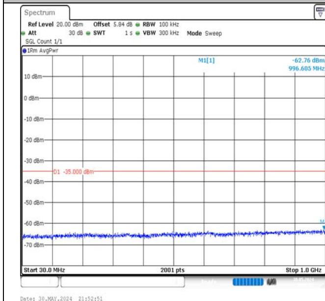
Band7-5MHz-16QAM-21100-1RB#24-30~1000-PASS
