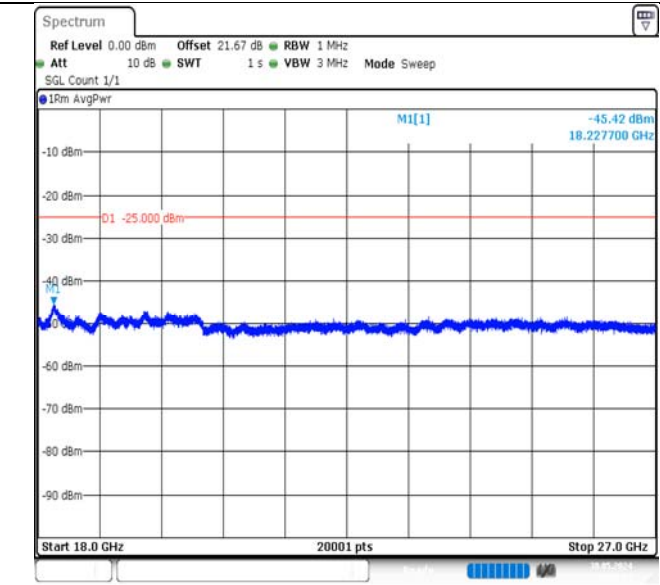
Band7-5MHz-QPSK-21100-25RB#0-18000~27000-PASS
