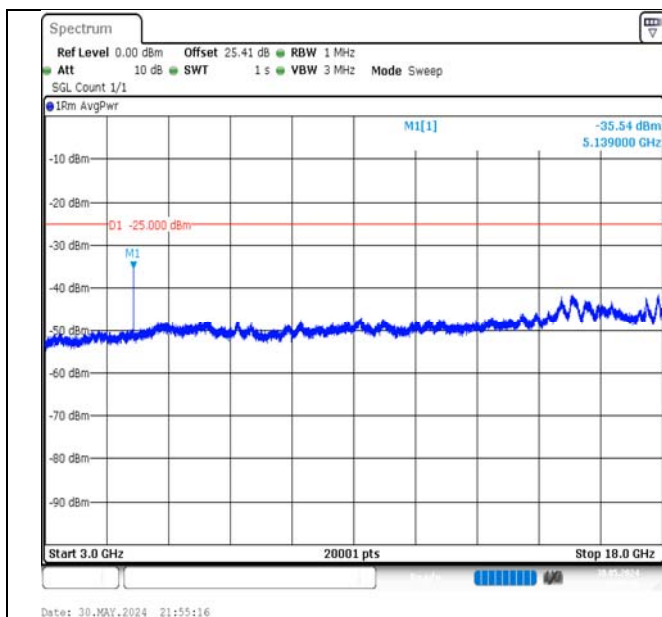
Band7-5MHz-QPSK-21425-1RB#24-3000~18000-PASS
