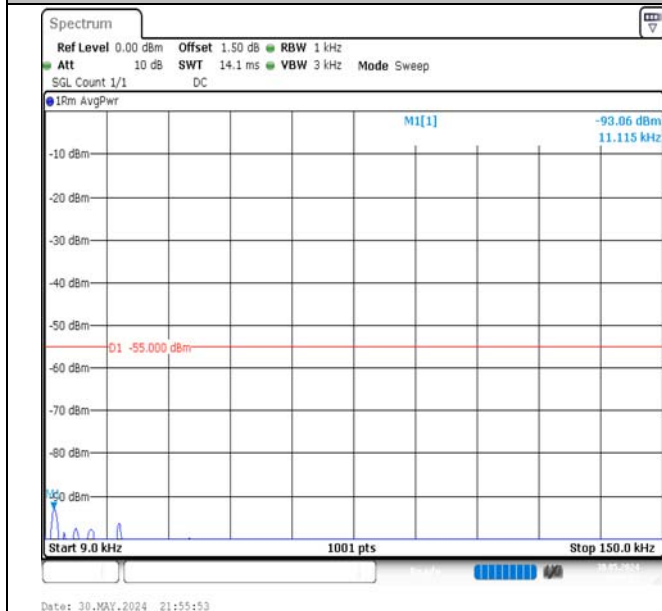
Band7-5MHz-QPSK-21425-25RB#0-0.009~0.15-PASS
