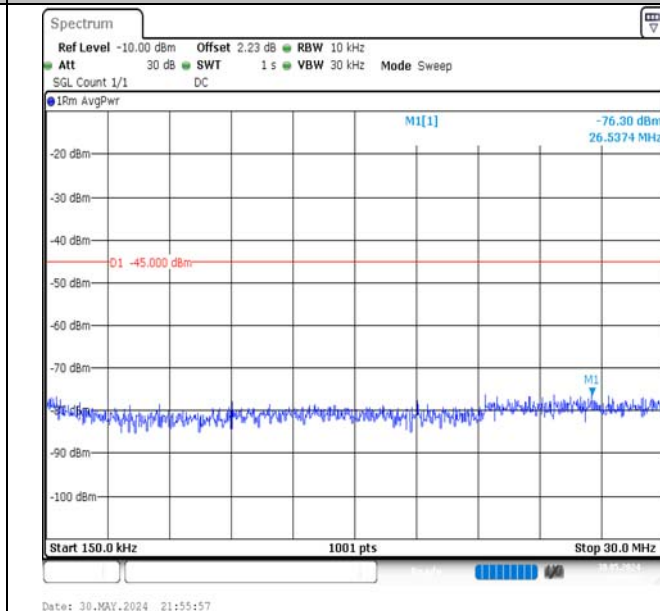
Band7-5MHz-QPSK-21425-25RB#0-0.15~30-PASS
