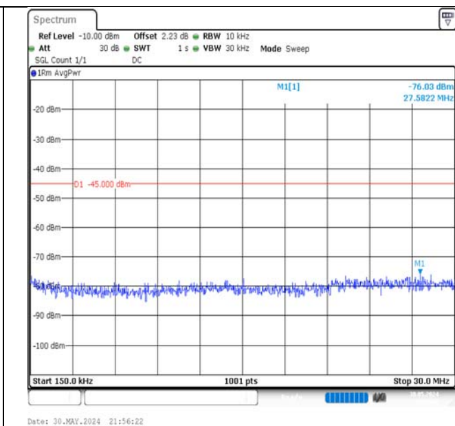
Band7-5MHz-16QAM-21425-25RB#0-0.15~30-PASS
