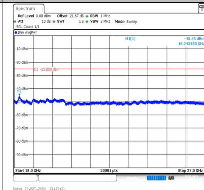
Band7-5MHz-16QAM-20775-1RB#24-18000~27000-PASS
