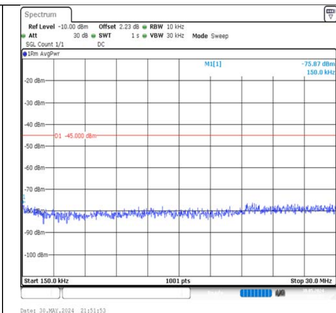
Band7-5MHz-16QAM-21100-1RB#0-0.15~30-PASS
