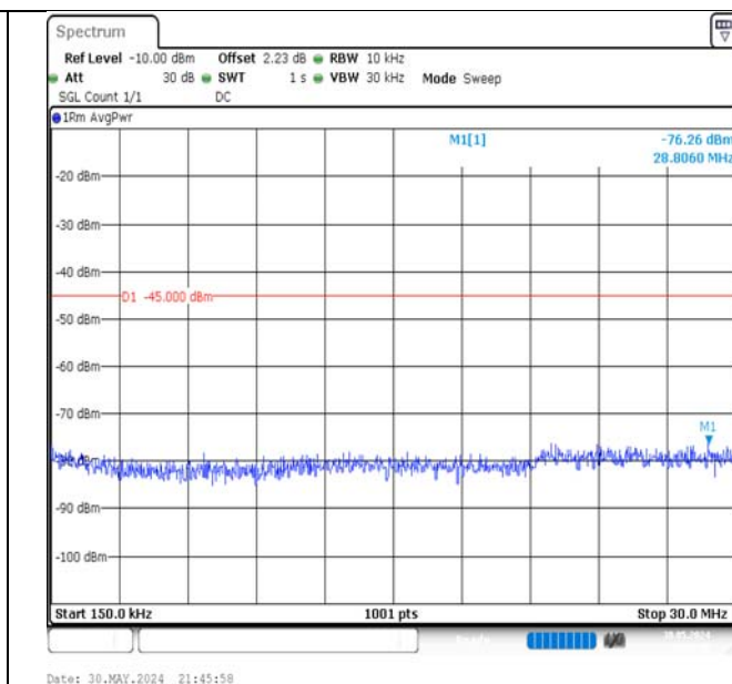
Band7-10MHz-QPSK-21400-1RB#0-0.15~30-PASS
