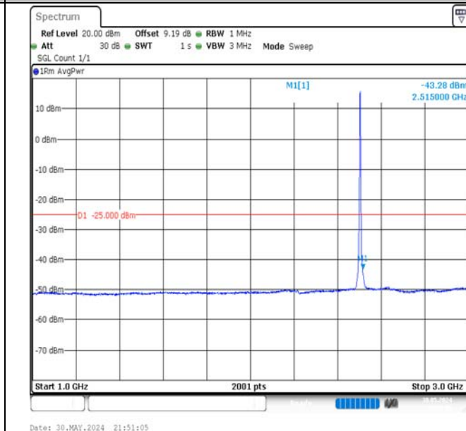
Band7-5MHz-16QAM-20775-25RB#0-1000~3000-PASS
