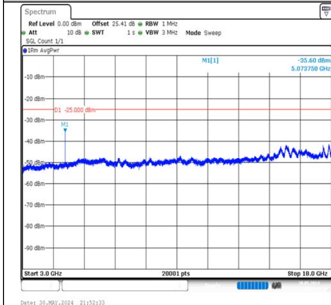
Band7-5MHz-QPSK-21100-1RB#24-3000~18000-PASS
