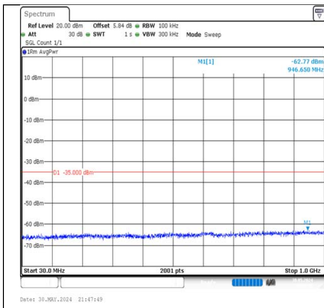
Band7-10MHz-QPSK-21400-50RB#0-30~1000-PASS
