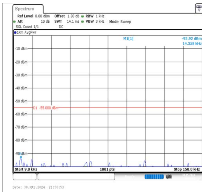
Band7-5MHz-16QAM-20775-25RB#0-0.009~0.15-PASS
