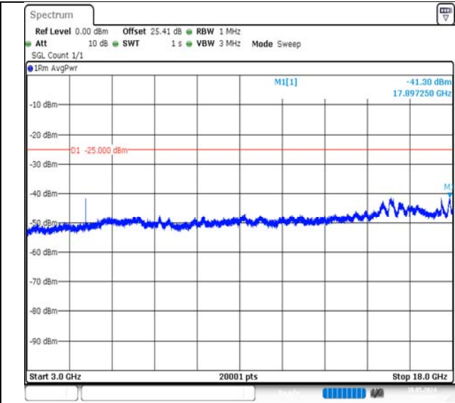
Band7-5MHz-QPSK-21100-25RB#0-3000~18000-PASS
