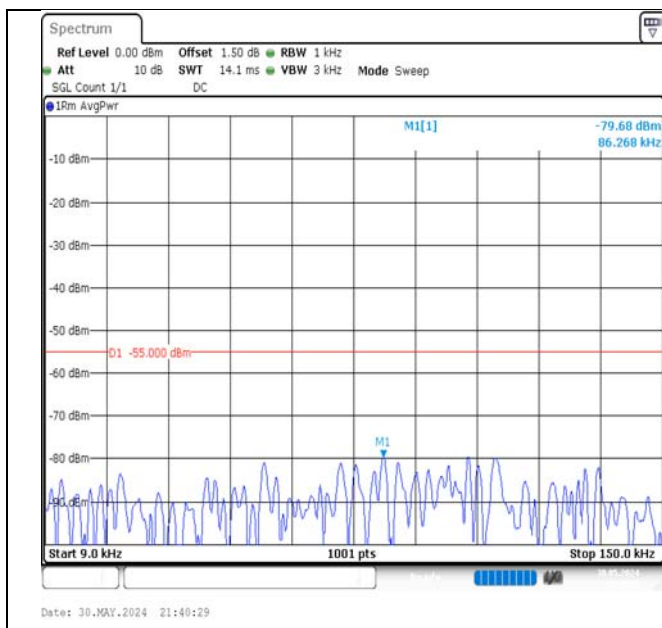
Band7-10MHz-QPSK-20800-1RB#0-0.009~0.15-PASS
