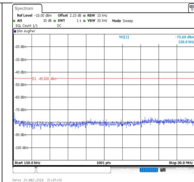
Band7-10MHz-QPSK-21100-50RB#0-0.15~30-PASS
