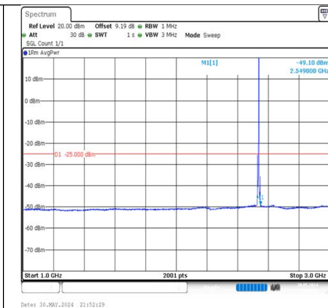
Band7-5MHz-QPSK-21100-1RB#24-1000~3000-PASS
