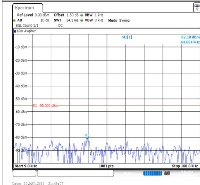
Band7-5MHz-16QAM-20775-1RB#0-0.009~0.15-PASS
