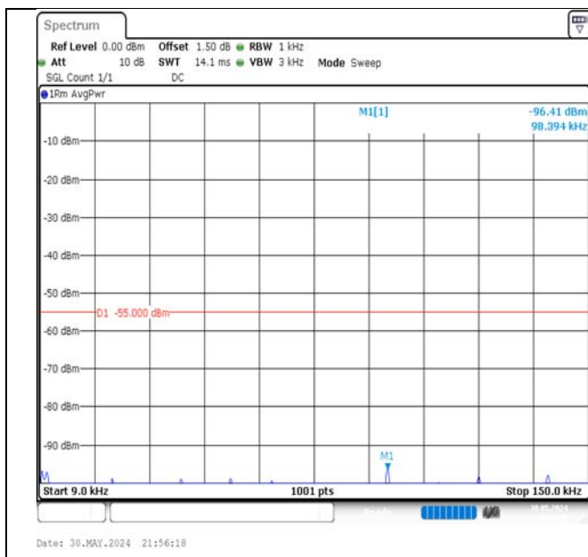
Band7-5MHz-16QAM-21425-25RB#0-0.009~0.15-PASS
