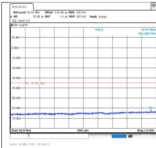
Band7-5MHz-16QAM-20775-1RB#0-30~1000-PASS
