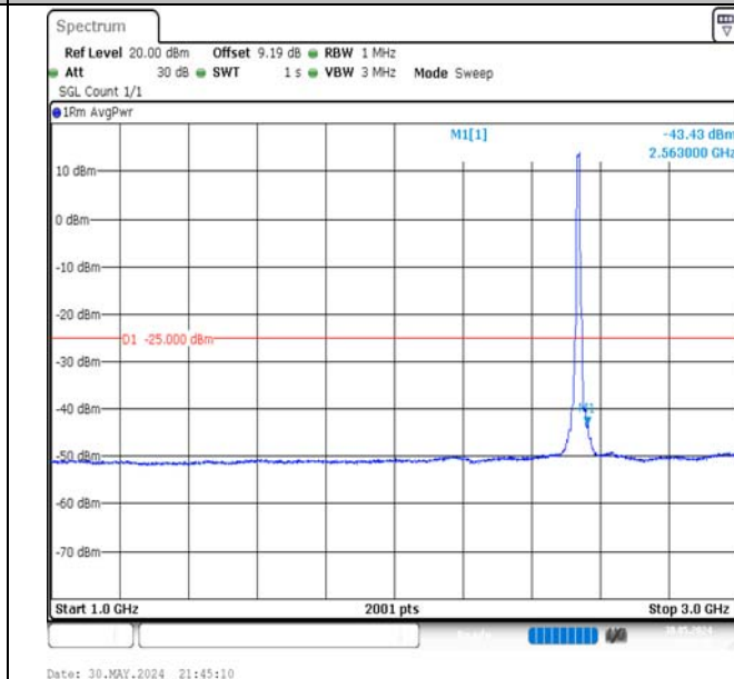
Band7-10MHz-QPSK-21100-50RB#0-1000~3000-PASS
