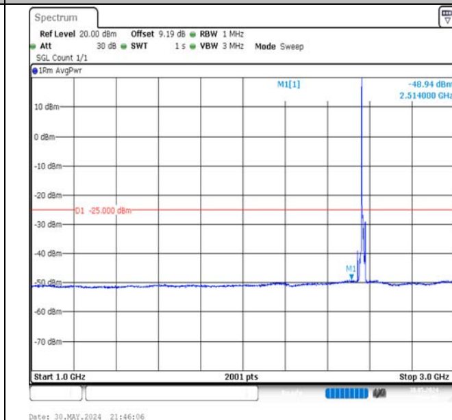
Band7-10MHz-QPSK-21400-1RB#0-1000~3000-PASS
