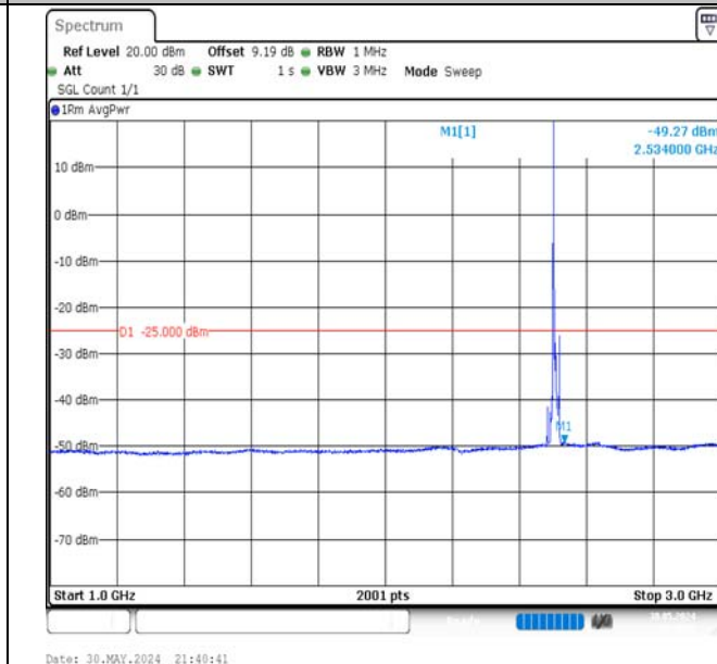
Band7-10MHz-QPSK-20800-1RB#0-1000~3000-PASS
