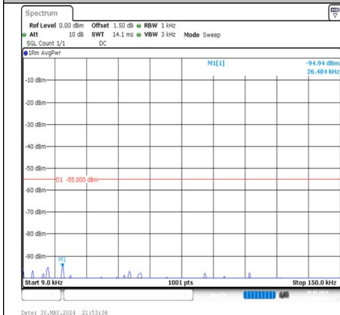
Band7-5MHz-16QAM-21100-25RB#0-0.009~0.15-PASS
