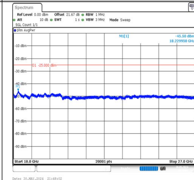
Band7-10MHz-QPSK-21400-50RB#0-18000~27000-PASS
