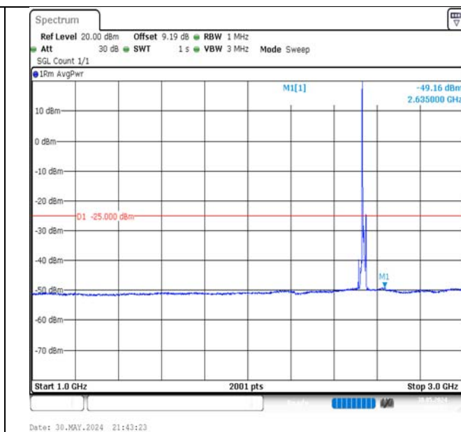
Band7-10MHz-QPSK-21100-1RB#0-1000~3000-PASS
