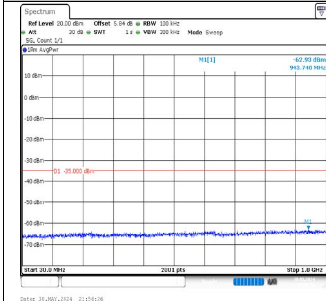
Band7-5MHz-16QAM-21425-25RB#0-30~1000-PASS
