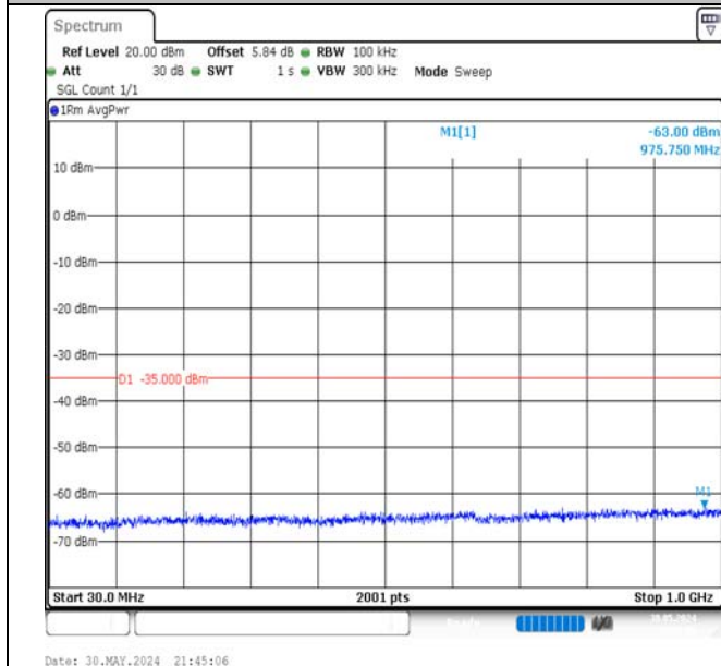
Band7-10MHz-QPSK-21100-50RB#0-30~1000-PASS
