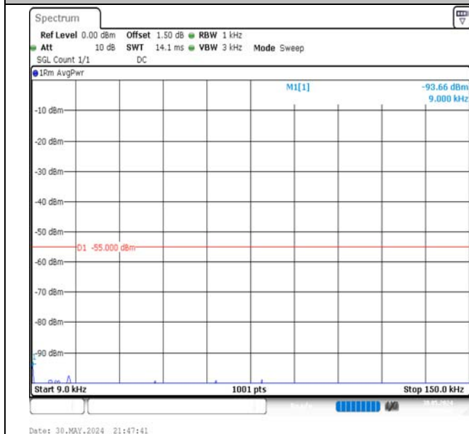
Band7-10MHz-QPSK-21400-50RB#0-0.009~0.15-PASS
