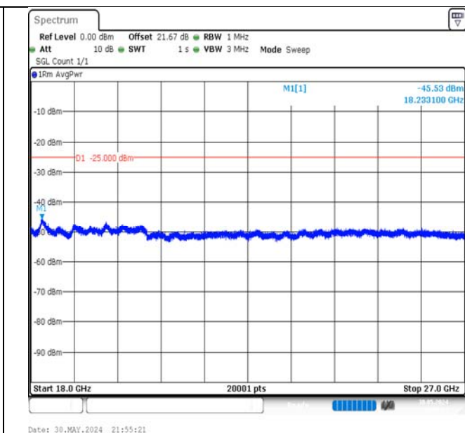
Band7-5MHz-QPSK-21425-1RB#24-18000~27000-PASS
