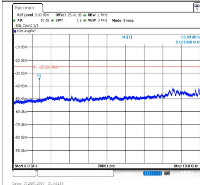
Band7-10MHz-QPSK-21100-1RB#0-3000~18000-PASS
