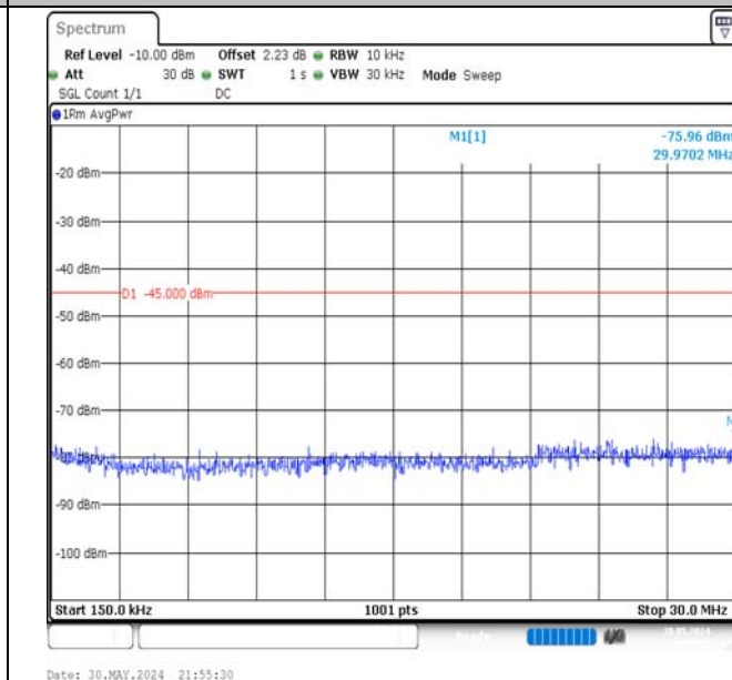
Band7-5MHz-16QAM-21425-1RB#24-0.15~30-PASS
