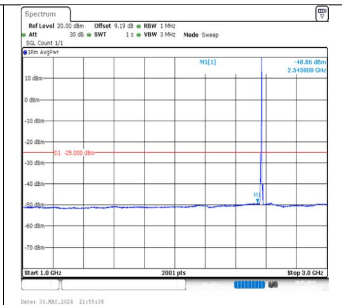
Band7-5MHz-16QAM-21425-1RB#24-1000~3000-PASS
