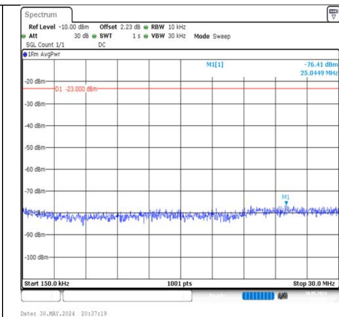
Band5-10MHz-QPSK-20600-1RB#0-0.15~30-PASS
