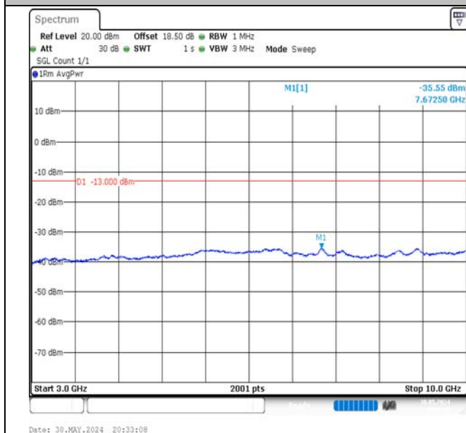
Band5-10MHz-QPSK-20450-1RB#0-3000~10000-PASS
