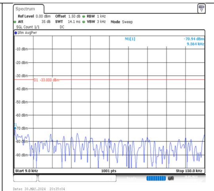
Band5-10MHz-QPSK-20525-1RB#0-0.009~0.15-PASS
