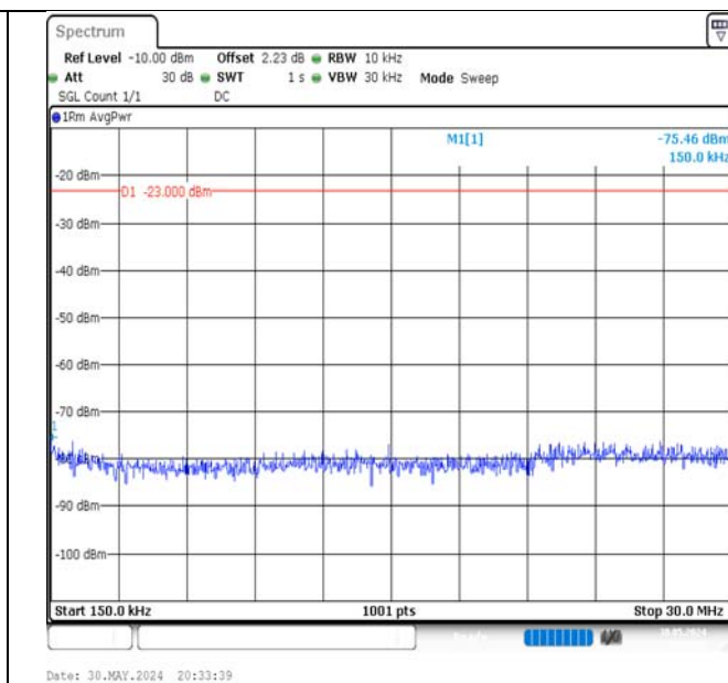
Band5-10MHz-QPSK-20450-1RB#49-0.15~30-PASS
