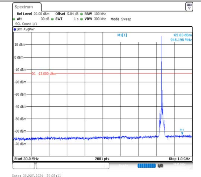
Band5-10MHz-QPSK-20525-1RB#0-30~1000-PASS
