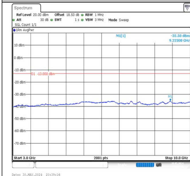
Band5-10MHz-16QAM-20600-50RB#0-3000~10000-PASS
