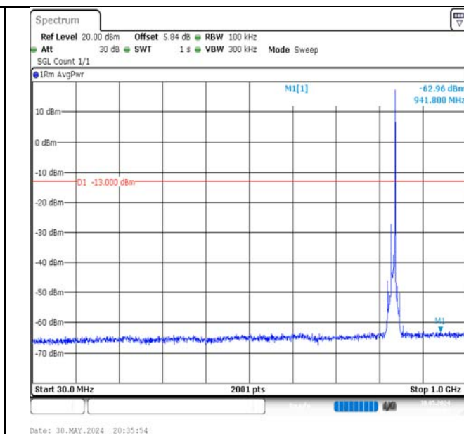
Band5-10MHz-QPSK-20525-1RB#49-30~1000-PASS
