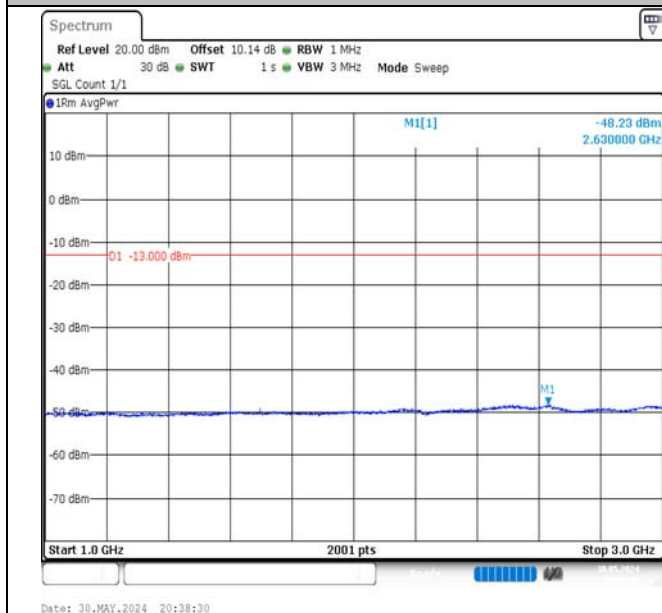
Band5-10MHz-16QAM-20600-1RB#49-1000~3000-PASS
