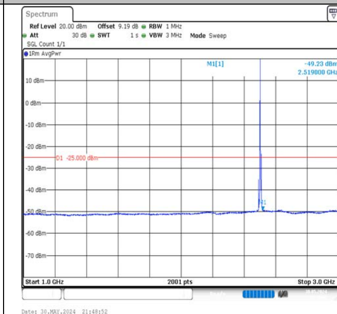
Band7-5MHz-QPSK-20775-1RB#0-1000~3000-PASS
