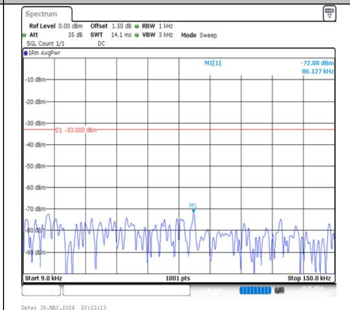
Band5-10MHz-16QAM-20450-1RB#0-0.009~0.15-PASS
