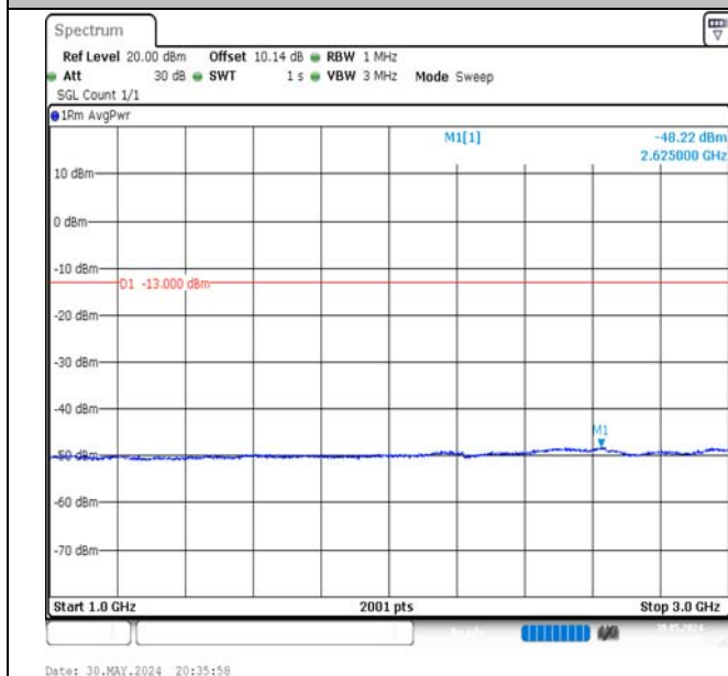
Band5-10MHz-QPSK-20525-1RB#49-1000~3000-PASS
