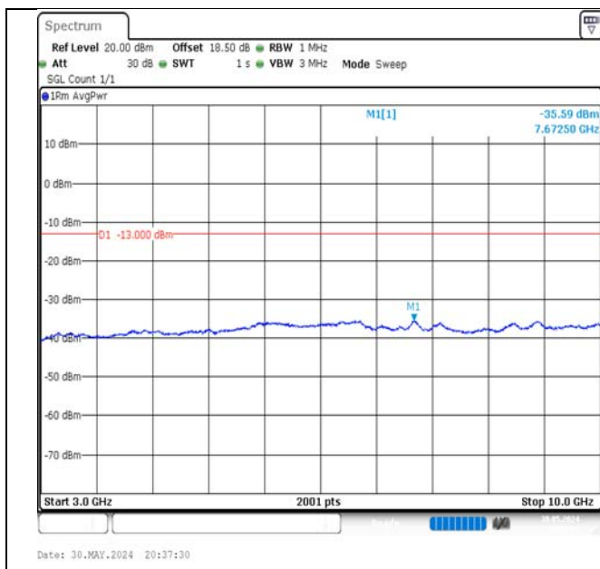
Band5-10MHz-QPSK-20600-1RB#0-3000~10000-PASS
