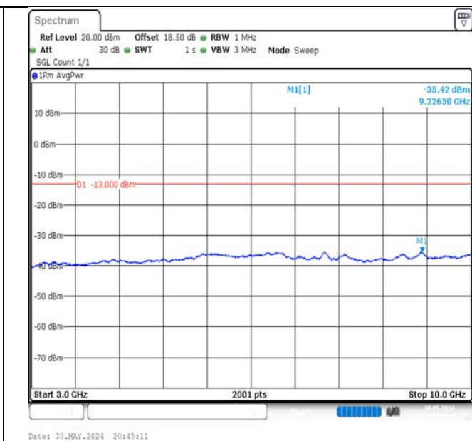
Band5-5MHz-16QAM-20625-1RB#24-3000~10000-PASS
