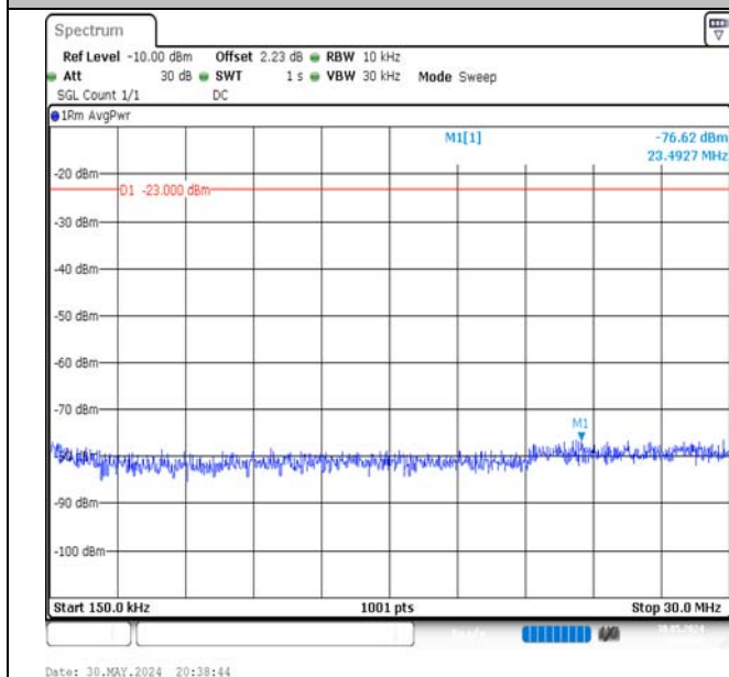
Band5-10MHz-QPSK-20600-50RB#0-0.15~30-PASS
