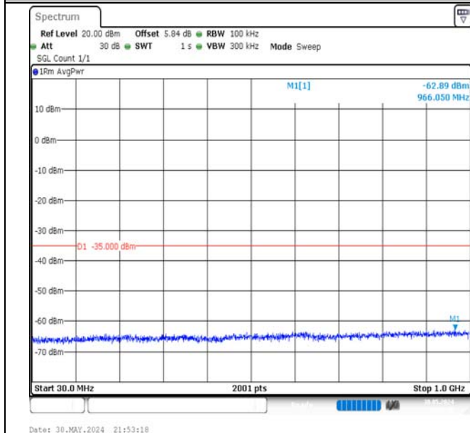
Band7-5MHz-QPSK-21100-25RB#0-30~1000-PASS
