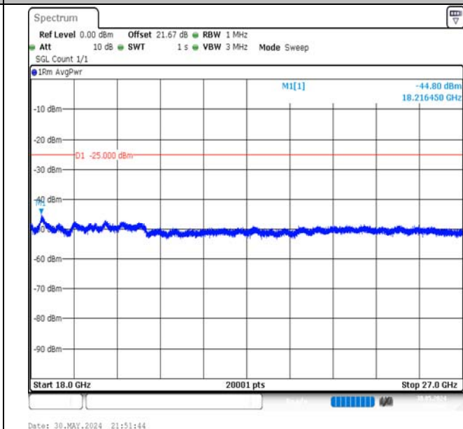
Band7-5MHz-QPSK-21100-1RB#0-18000~27000-PASS
