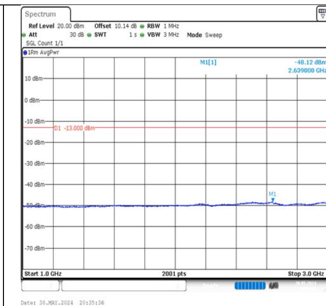
Band5-10MHz-16QAM-20525-1RB#0-1000~3000-PASS
