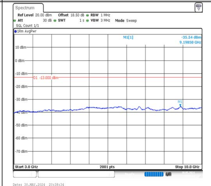
Band5-10MHz-16QAM-20600-1RB#49-3000~10000-PASS
