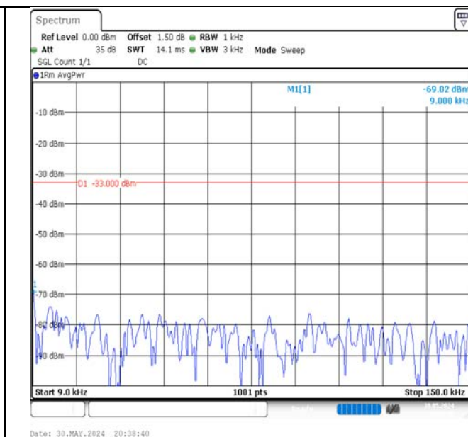
Band5-10MHz-QPSK-20600-50RB#0-0.009~0.15-PASS
