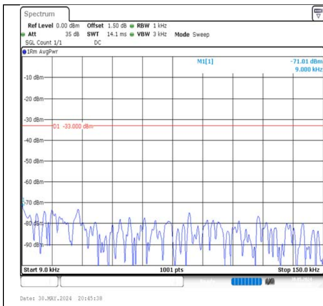
Band5-5MHz-16QAM-20625-25RB#0-0.009~0.15-PASS
