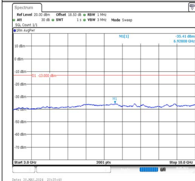
Band5-10MHz-16QAM-20525-1RB#0-3000~10000-PASS
