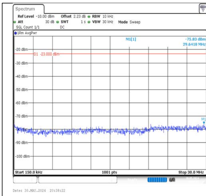
Band5-10MHz-16QAM-20600-1RB#49-0.15~30-PASS
