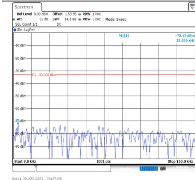
Band5-10MHz-QPSK-20600-1RB#49-0.009~0.15-PASS
