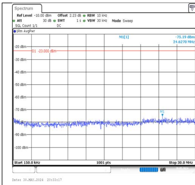
Band5-10MHz-16QAM-20450-1RB#0-0.15~30-PASS
