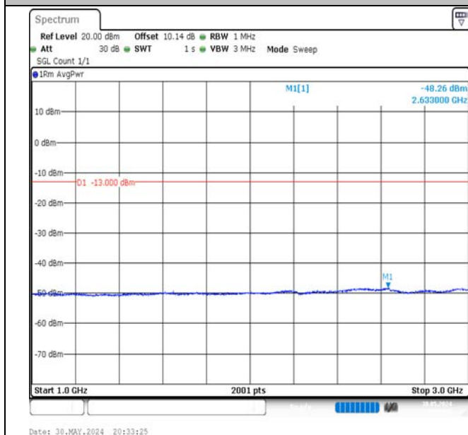
Band5-10MHz-16QAM-20450-1RB#0-1000~3000-PASS
