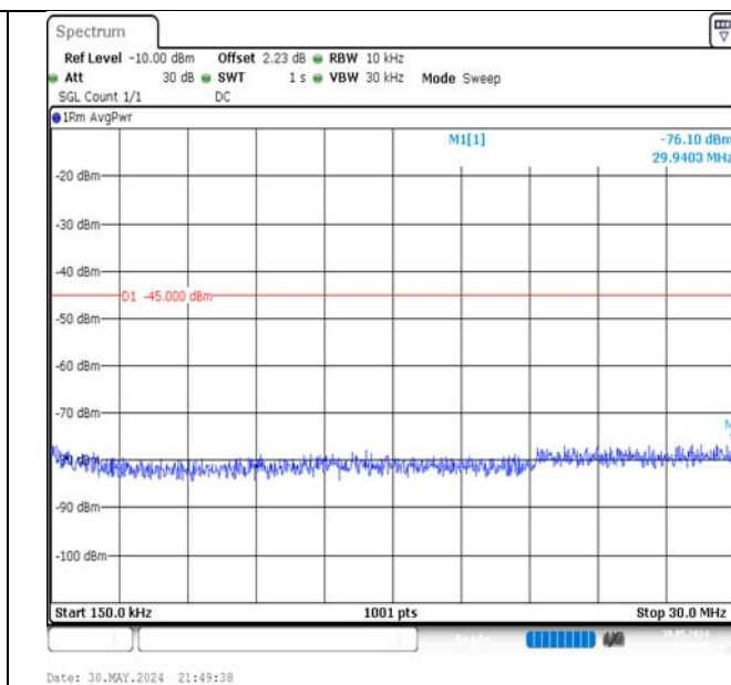
Band7-5MHz-QPSK-20775-1RB#24-0.15~30-PASS
