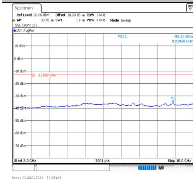
Band5-10MHz-QPSK-20600-1RB#49-3000~10000-PASS
