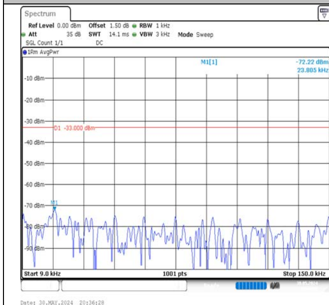
Band5-10MHz-QPSK-20525-50RB#0-0.009~0.15-PASS
