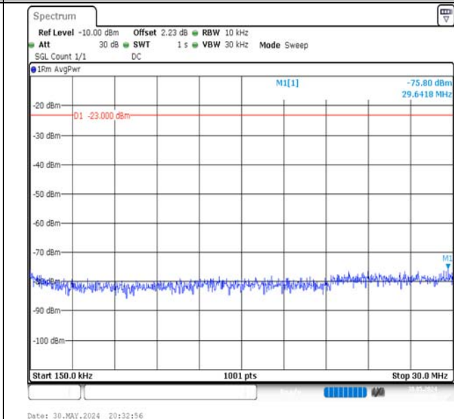
Band5-10MHz-QPSK-20450-1RB#0-0.15~30-PASS
