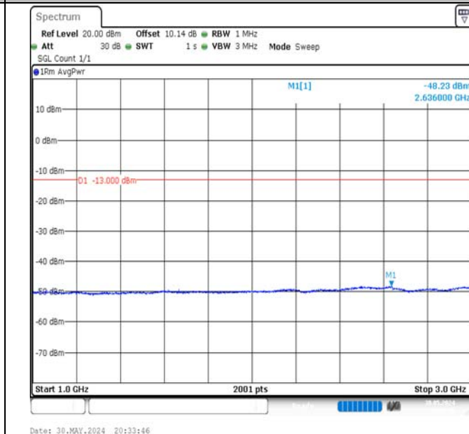
Band5-10MHz-QPSK-20450-1RB#49-1000~3000-PASS
