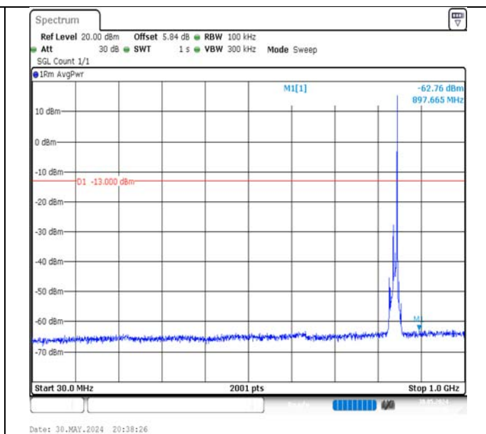
Band5-10MHz-16QAM-20600-1RB#49-30~1000-PASS
