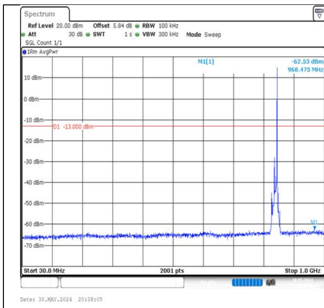
Band5-10MHz-QPSK-20600-1RB#49-30~1000-PASS
