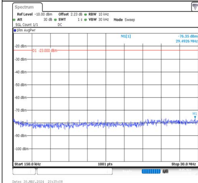
Band5-10MHz-QPSK-20525-1RB#0-0.15~30-PASS
