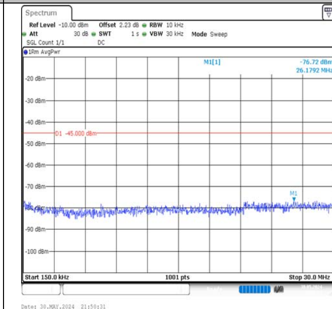
Band7-5MHz-QPSK-20775-25RB#0-0.15~30-PASS
