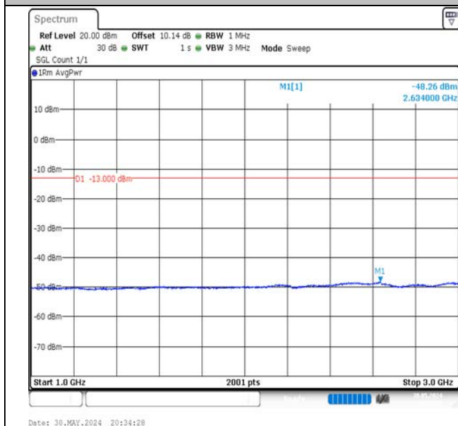
Band5-10MHz-QPSK-20450-50RB#0-1000~3000-PASS
