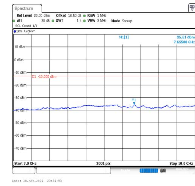
Band5-10MHz-16QAM-20450-50RB#0-3000~10000-PASS
