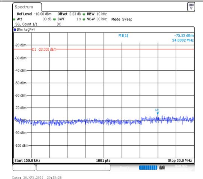
Band5-10MHz-16QAM-20525-1RB#0-0.15~30-PASS
