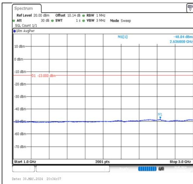
Band5-10MHz-16QAM-20450-1RB#49-1000~3000-PASS
