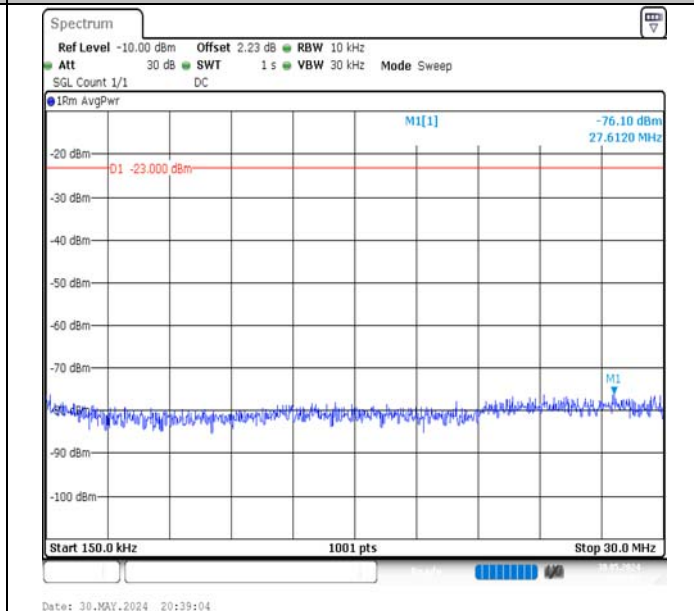
Band5-10MHz-16QAM-20600-50RB#0-0.15~30-PASS
