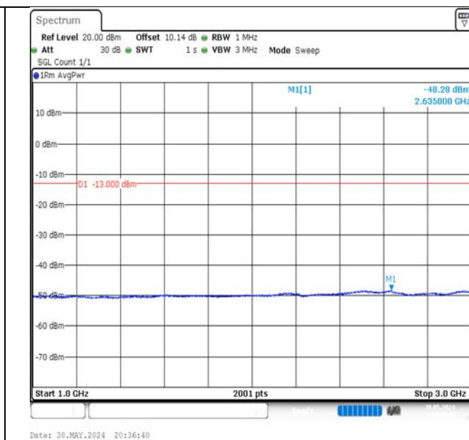
Band5-10MHz-QPSK-20525-50RB#0-1000~3000-PASS
