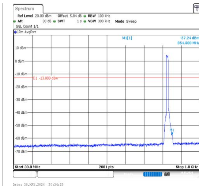
Band5-10MHz-QPSK-20450-50RB#0-30~1000-PASS
