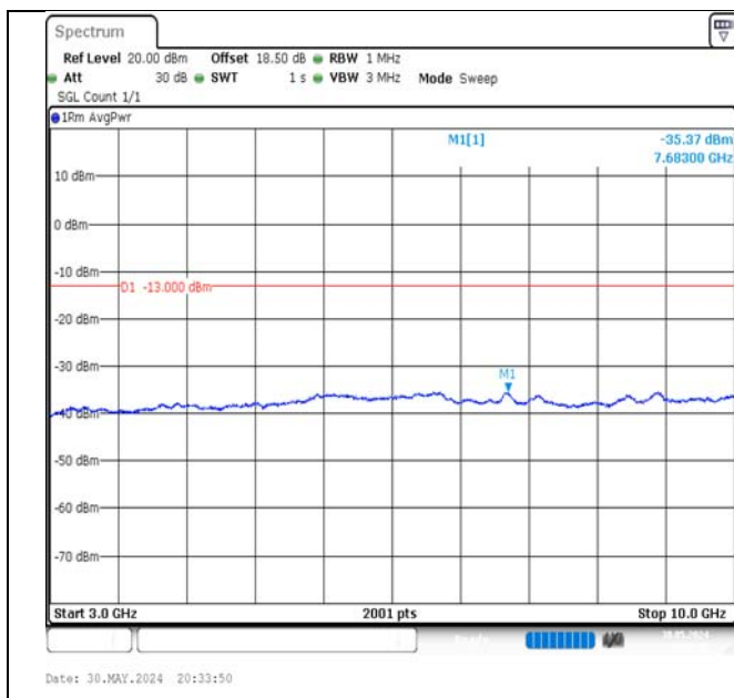
Band5-10MHz-QPSK-20450-1RB#49-3000~10000-PASS
