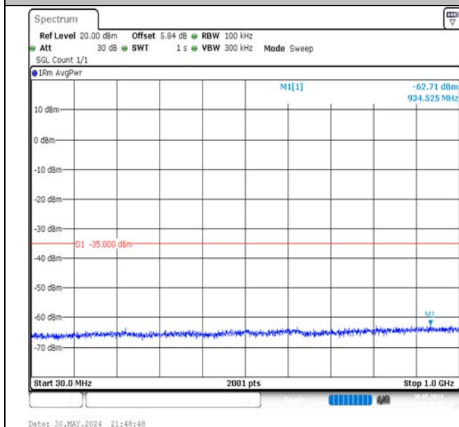
Band7-5MHz-QPSK-20775-1RB#0-30~1000-PASS
