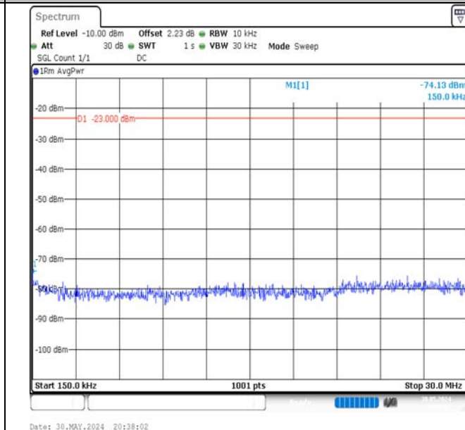
Band5-10MHz-QPSK-20600-1RB#49-0.15~30-PASS
