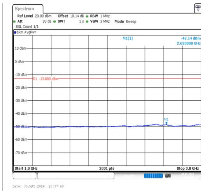
Band5-10MHz-16QAM-20600-1RB#0-1000~3000-PASS
