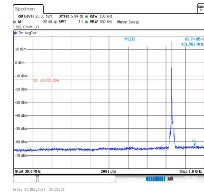
Band5-10MHz-16QAM-20525-1RB#0-30~1000-PASS
