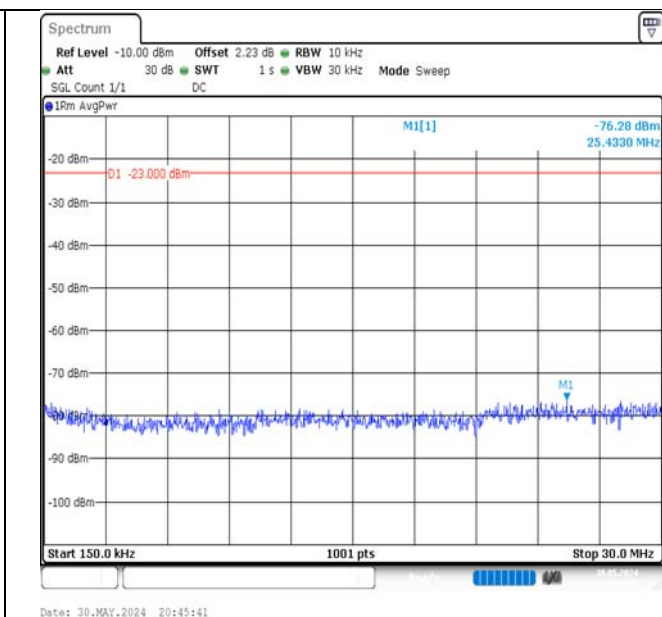
Band5-5MHz-16QAM-20625-25RB#0-0.15~30-PASS
