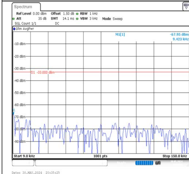
Band5-10MHz-16QAM-20525-1RB#0-0.009~0.15-PASS
