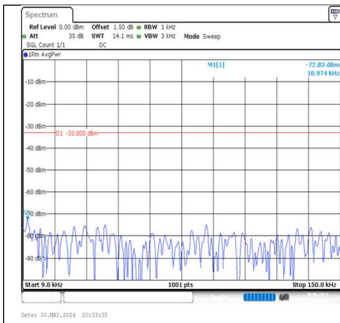
Band5-10MHz-QPSK-20450-1RB#49-0.009~0.15-PASS
