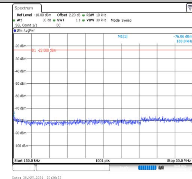
Band5-10MHz-QPSK-20525-50RB#0-0.15~30-PASS
