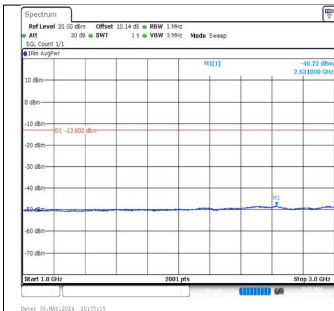
Band5-10MHz-QPSK-20525-1RB#0-1000~3000-PASS
