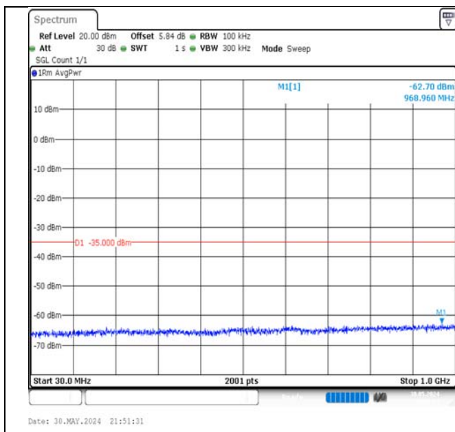
Band7-5MHz-QPSK-21100-1RB#0-30~1000-PASS
