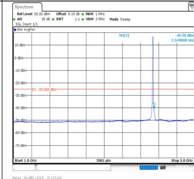
Band7-5MHz-QPSK-21100-25RB#0-1000~3000-PASS
