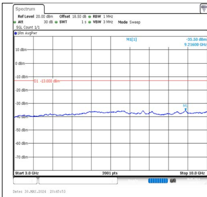
Band5-5MHz-16QAM-20625-25RB#0-3000~10000-PASS
