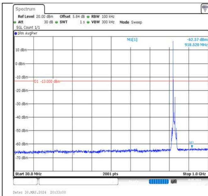
Band5-10MHz-QPSK-20450-1RB#0-30~1000-PASS
