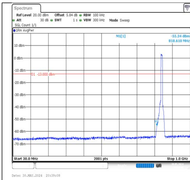
Band5-10MHz-16QAM-20600-50RB#0-30~1000-PASS
