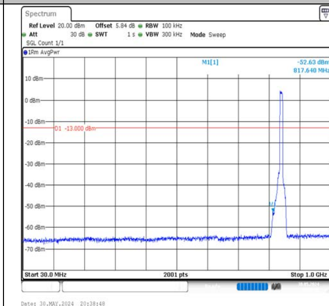
Band5-10MHz-QPSK-20600-50RB#0-30~1000-PASS
