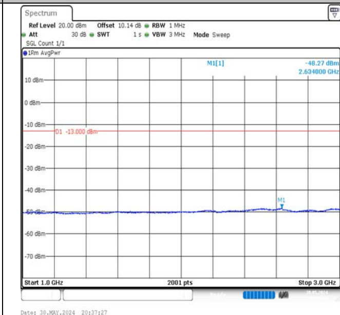
Band5-10MHz-QPSK-20600-1RB#0-1000~3000-PASS
