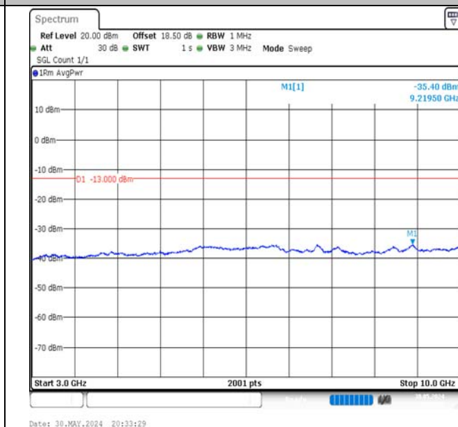
Band5-10MHz-16QAM-20450-1RB#0-3000~10000-PASS
