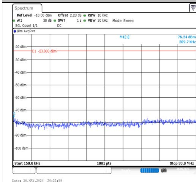
Band5-10MHz-16QAM-20450-1RB#49-0.15~30-PASS
