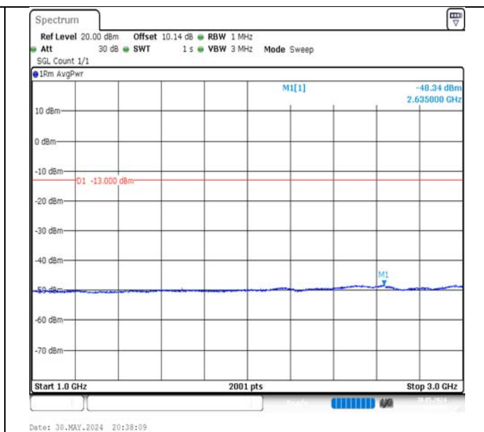
Band5-10MHz-QPSK-20600-1RB#49-1000~3000-PASS
