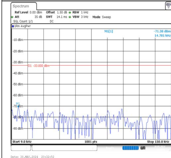
Band5-10MHz-QPSK-20450-1RB#0-0.009~0.15-PASS
