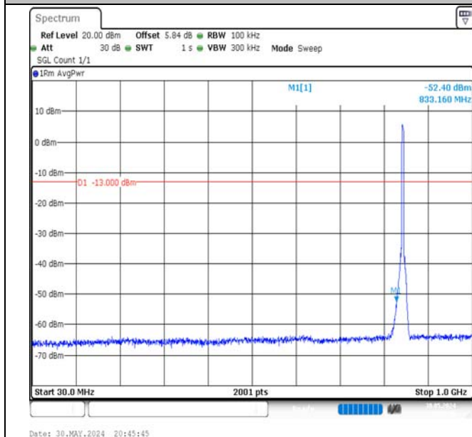
Band5-5MHz-16QAM-20625-25RB#0-30~1000-PASS
