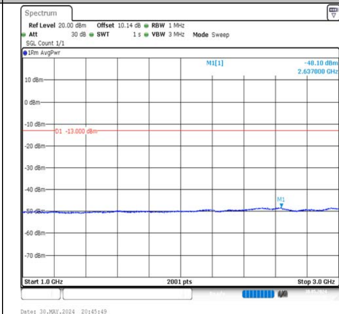
Band5-5MHz-16QAM-20625-25RB#0-1000~3000-PASS
