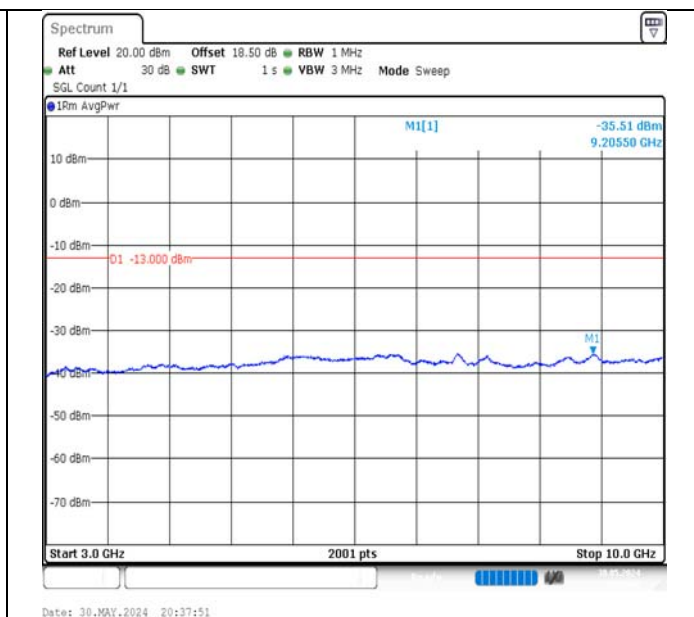
Band5-10MHz-16QAM-20600-1RB#0-3000~10000-PASS
