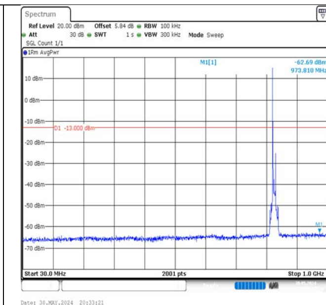
Band5-10MHz-16QAM-20450-1RB#0-30~1000-PASS
