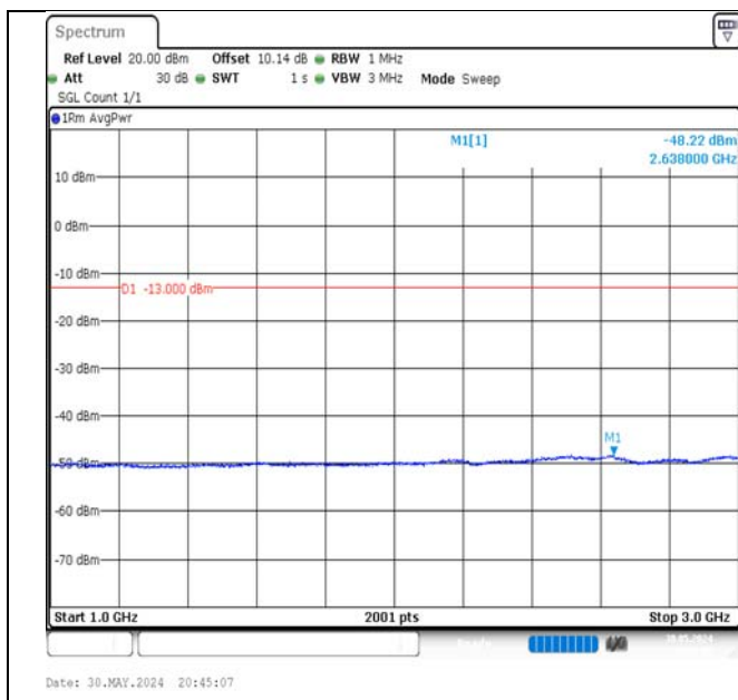
Band5-5MHz-16QAM-20625-1RB#24-1000~3000-PASS
