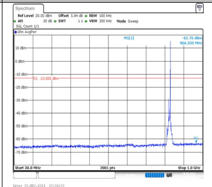
Band5-10MHz-16QAM-20450-1RB#49-30~1000-PASS
