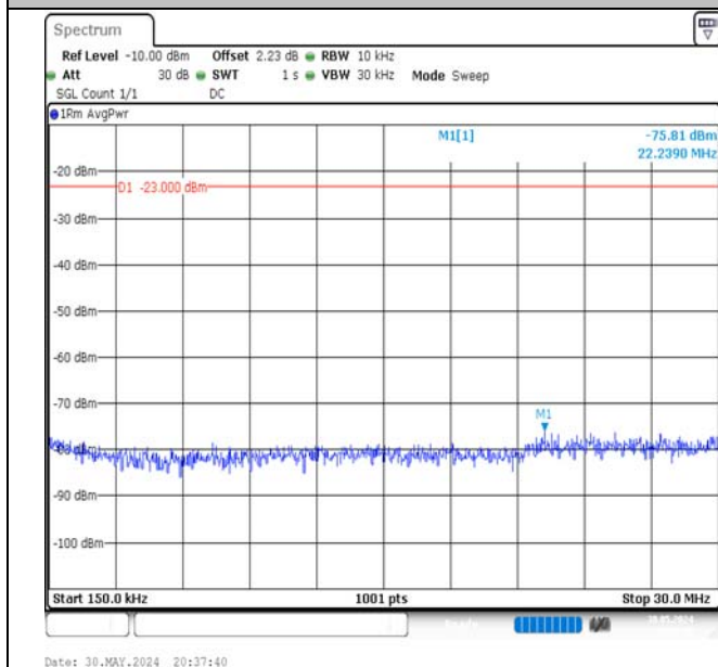
Band5-10MHz-16QAM-20600-1RB#0-0.15~30-PASS
