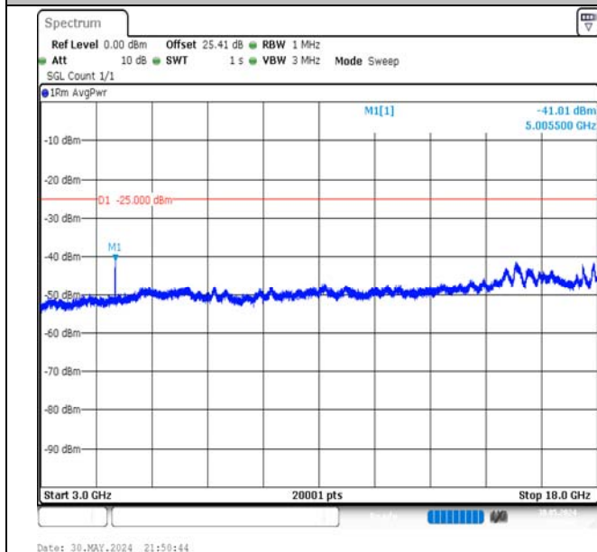
Band7-5MHz-QPSK-20775-25RB#0-3000~18000-PASS
