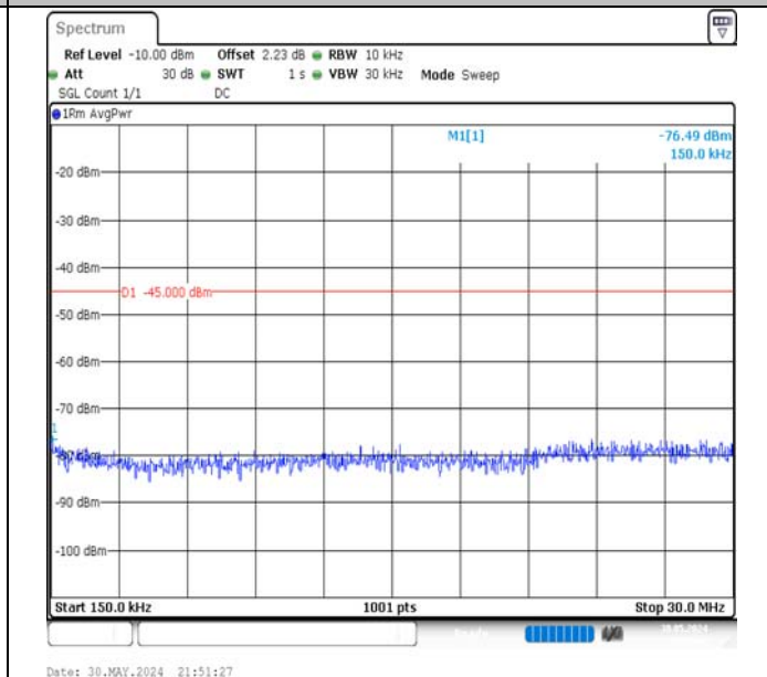
Band7-5MHz-QPSK-21100-1RB#0-0.15~30-PASS
