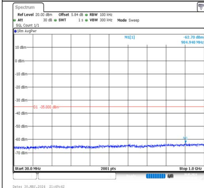
Band7-5MHz-QPSK-20775-1RB#24-30~1000-PASS
