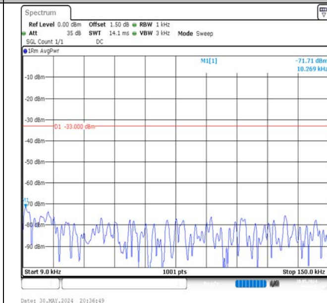
Band5-10MHz-16QAM-20525-50RB#0-0.009~0.15-PASS
