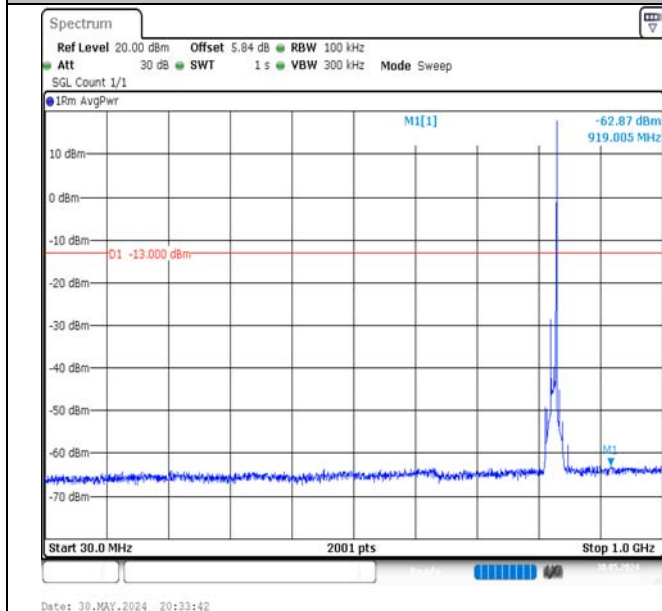
Band5-10MHz-QPSK-20450-1RB#49-30~1000-PASS
