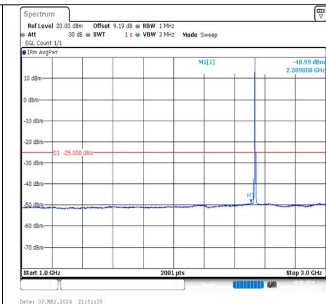
Band7-5MHz-QPSK-21100-1RB#0-1000~3000-PASS
