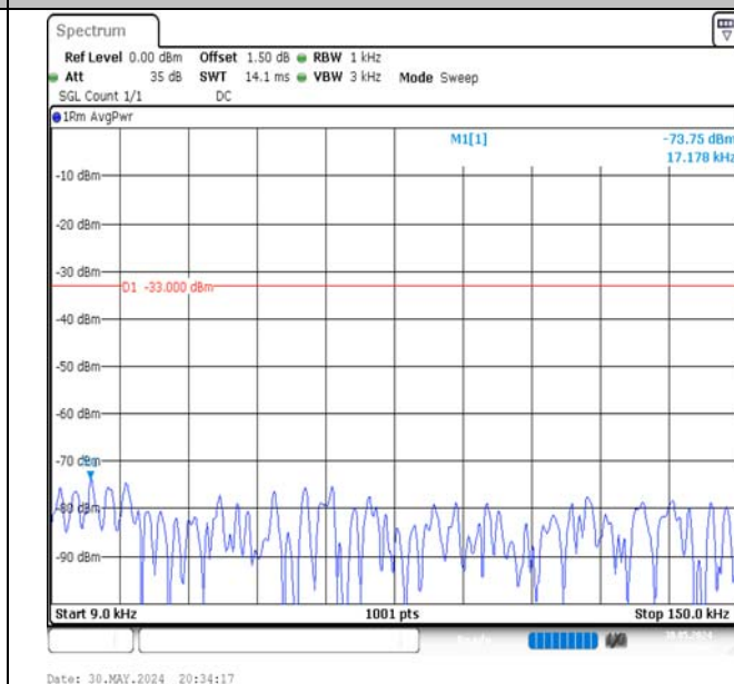
Band5-10MHz-QPSK-20450-50RB#0-0.009~0.15-PASS
