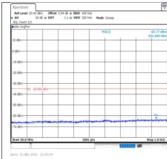
Band7-5MHz-QPSK-20775-25RB#0-30~1000-PASS
