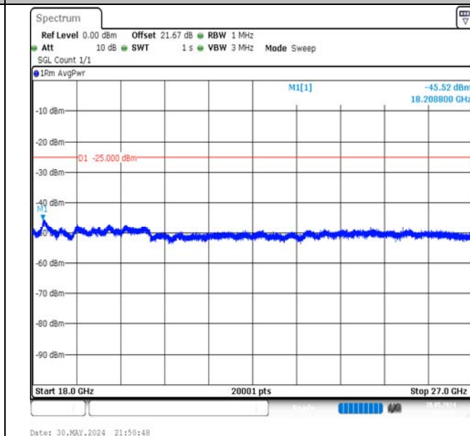
Band7-5MHz-QPSK-20775-25RB#0-18000~27000-PASS
