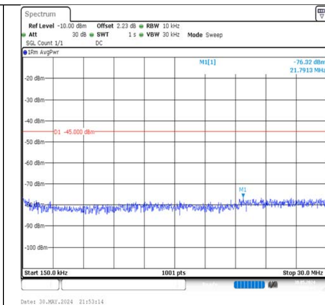
Band7-5MHz-QPSK-21100-25RB#0-0.15~30-PASS
