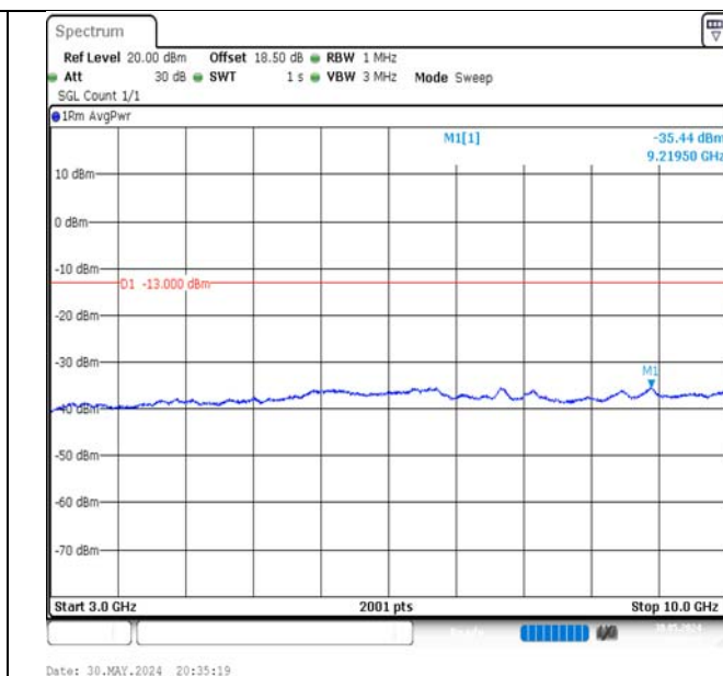
Band5-10MHz-QPSK-20525-1RB#0-3000~10000-PASS
