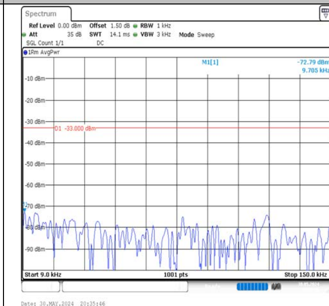
Band5-10MHz-QPSK-20525-1RB#49-0.009~0.15-PASS
