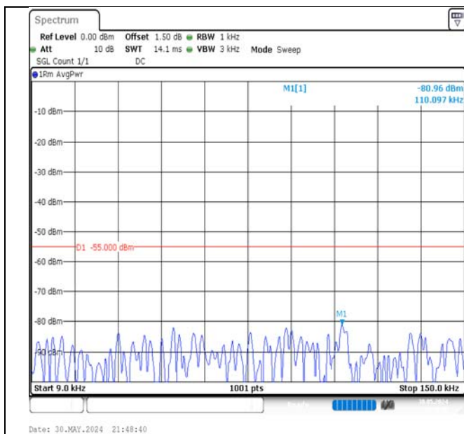
Band7-5MHz-QPSK-20775-1RB#0-0.009~0.15-PASS
