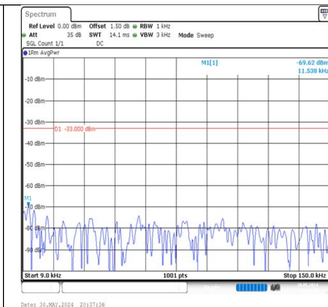
Band5-10MHz-16QAM-20600-1RB#0-0.009~0.15-PASS
