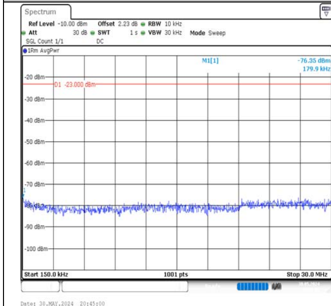
Band5-5MHz-16QAM-20625-1RB#24-0.15~30-PASS
