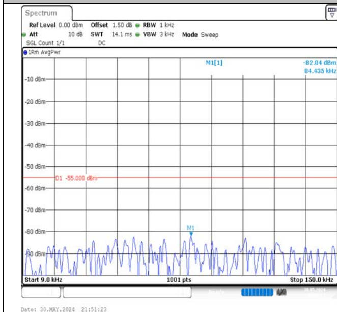
Band7-5MHz-QPSK-21100-1RB#0-0.009~0.15-PASS
