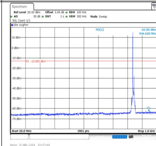
Band5-10MHz-16QAM-20600-1RB#0-30~1000-PASS
