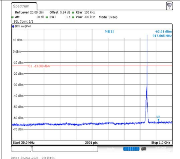
Band5-5MHz-16QAM-20625-1RB#24-30~1000-PASS
