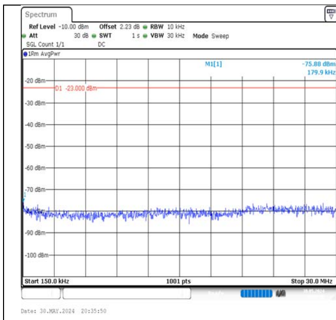
Band5-10MHz-QPSK-20525-1RB#49-0.15~30-PASS
