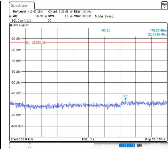
Band5-10MHz-16QAM-20525-50RB#0-0.15~30-PASS
