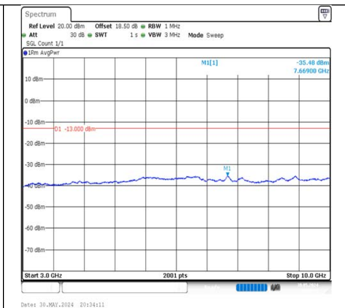
Band5-10MHz-16QAM-20450-1RB#49-3000~10000-PASS
