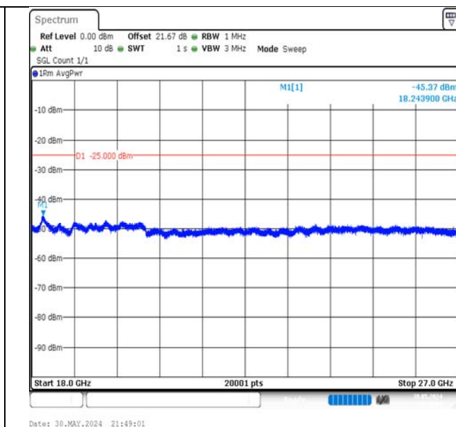
Band7-5MHz-QPSK-20775-1RB#0-18000~27000-PASS
