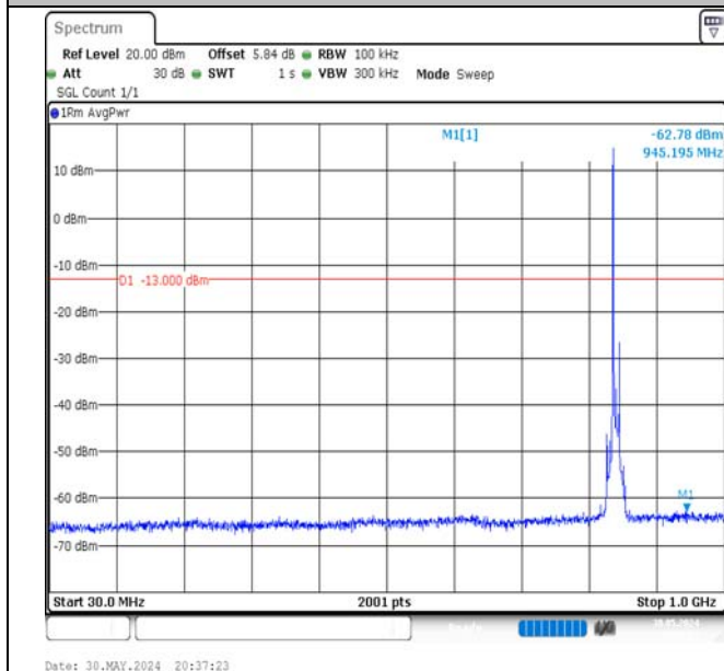
Band5-10MHz-QPSK-20600-1RB#0-30~1000-PASS
