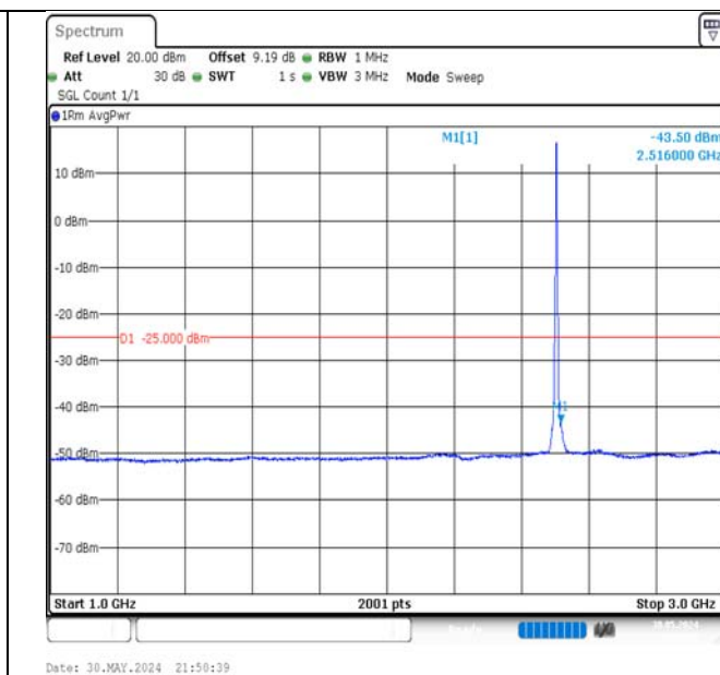
Band7-5MHz-QPSK-20775-25RB#0-1000~3000-PASS
