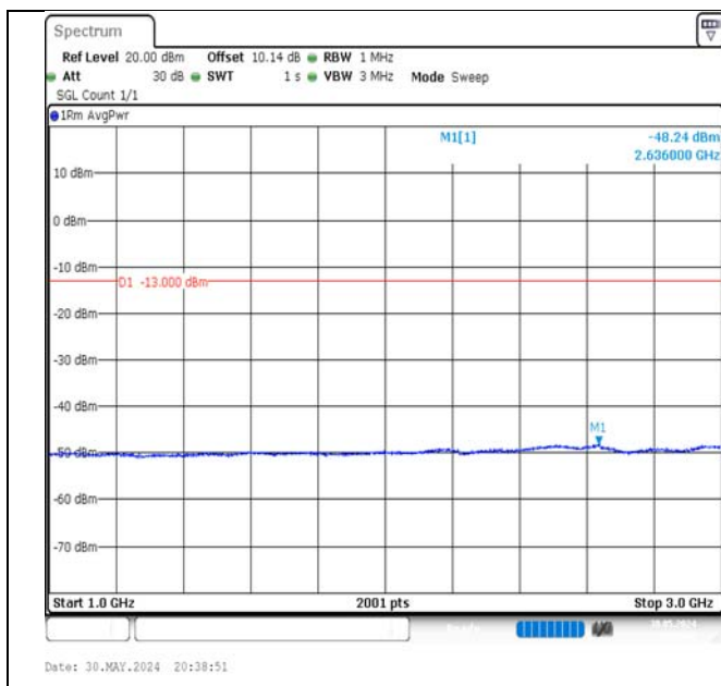
Band5-10MHz-QPSK-20600-50RB#0-1000~3000-PASS
