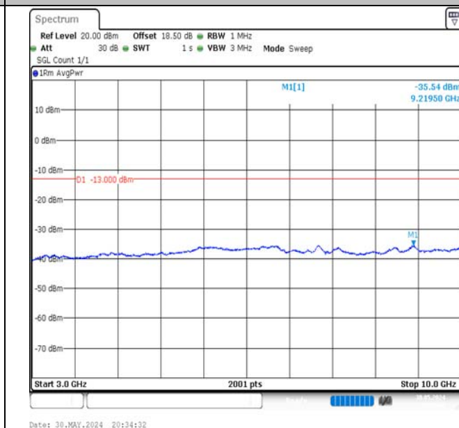
Band5-10MHz-QPSK-20450-50RB#0-3000~10000-PASS
