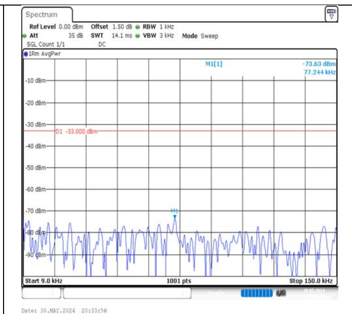
Band5-10MHz-16QAM-20450-1RB#49-0.009~0.15-PASS
