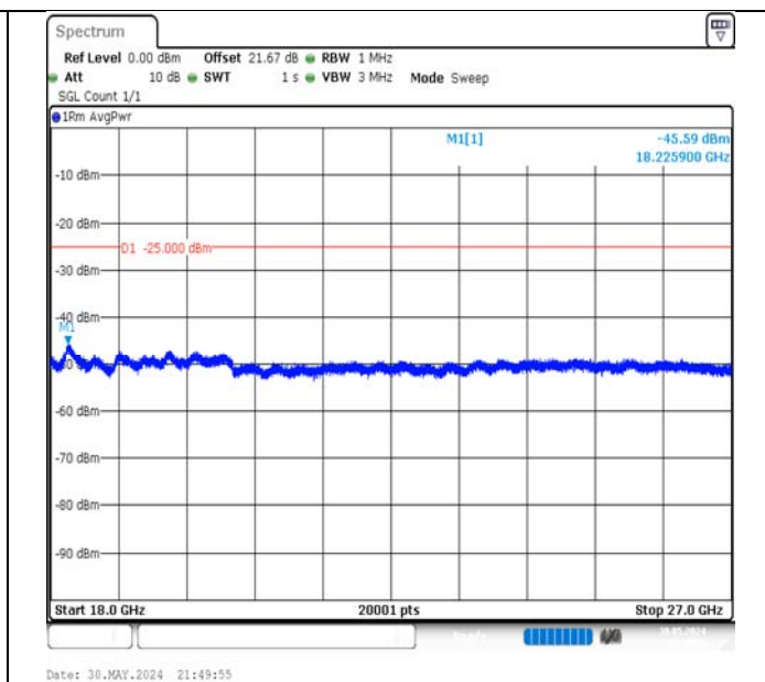
Band7-5MHz-QPSK-20775-1RB#24-18000~27000-PASS
