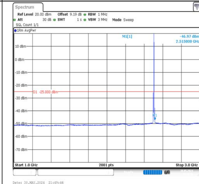
Band7-5MHz-QPSK-20775-1RB#24-1000~3000-PASS
