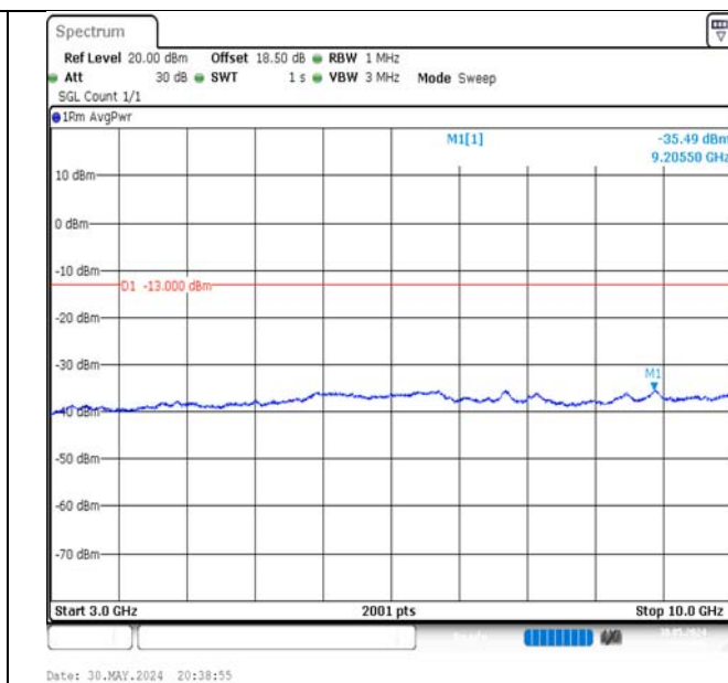
Band5-10MHz-QPSK-20600-50RB#0-3000~10000-PASS
