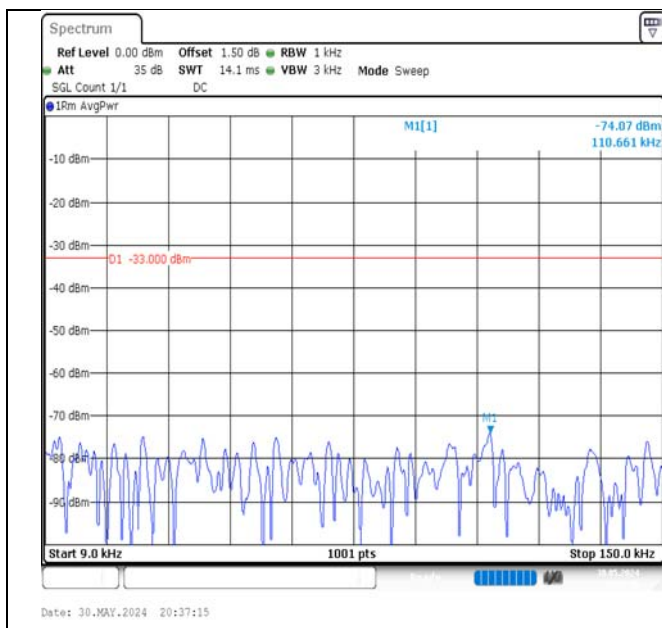
Band5-10MHz-QPSK-20600-1RB#0-0.009~0.15-PASS
