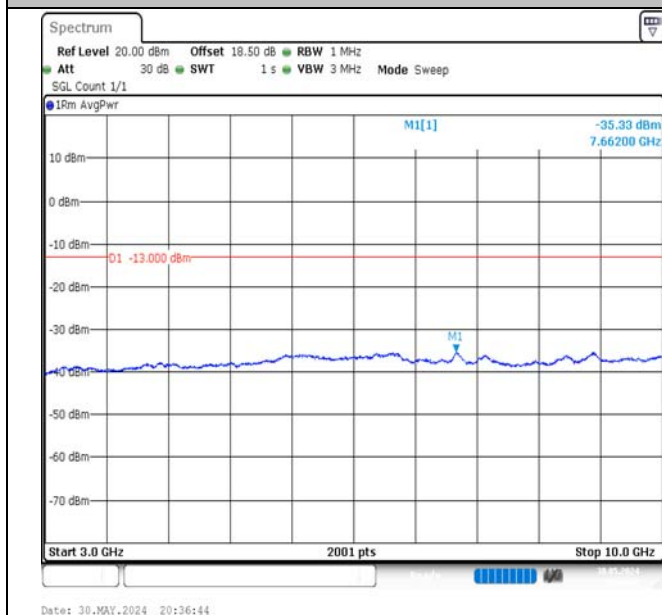
Band5-10MHz-QPSK-20525-50RB#0-3000~10000-PASS
