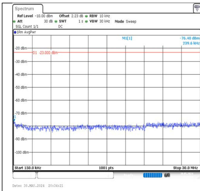
Band5-10MHz-QPSK-20450-50RB#0-0.15~30-PASS
