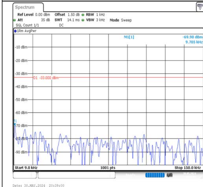
Band5-10MHz-16QAM-20600-50RB#0-0.009~0.15-PASS
