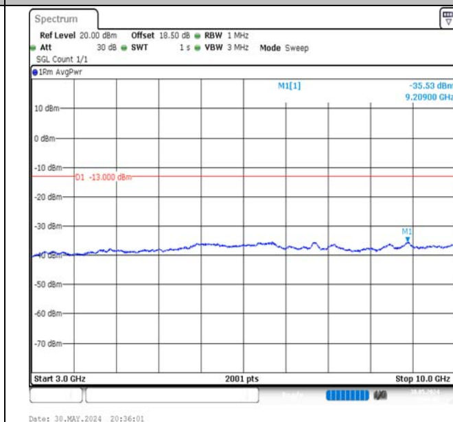
Band5-10MHz-QPSK-20525-1RB#49-3000~10000-PASS
