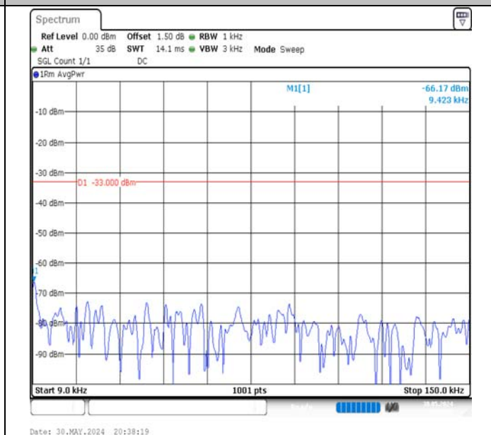
Band5-10MHz-16QAM-20600-1RB#49-0.009~0.15-PASS
