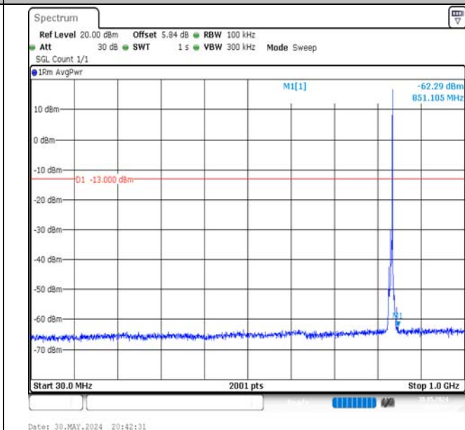
Band5-5MHz-QPSK-20525-1RB#24-30~1000-PASS
