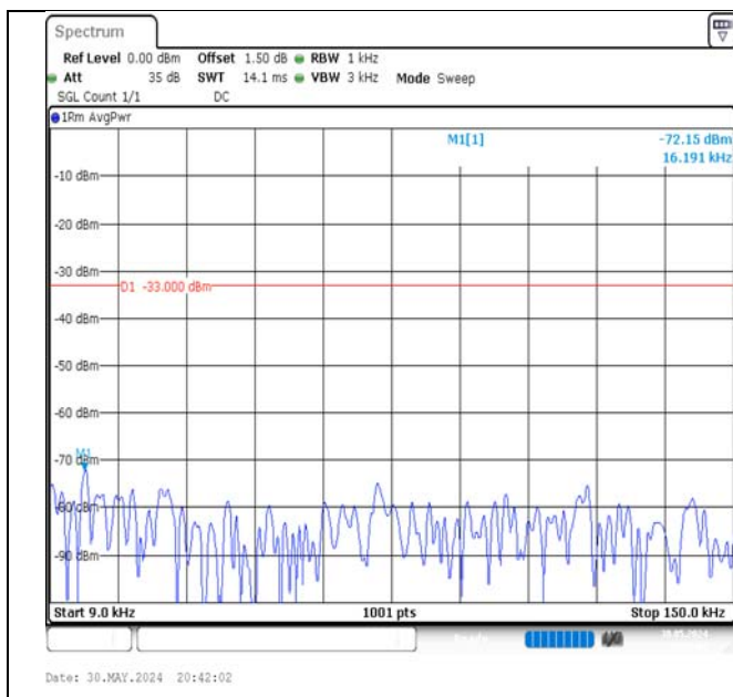
Band5-5MHz-16QAM-20525-1RB#0-0.009~0.15-PASS
