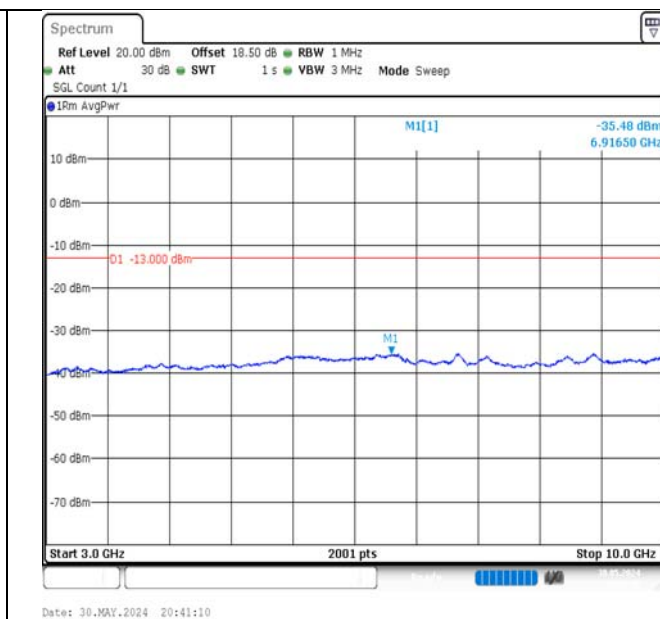
Band5-5MHz-QPSK-20425-25RB#0-3000~10000-PASS
