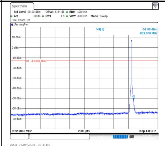
Band5-5MHz-QPSK-20425-25RB#0-30~1000-PASS
