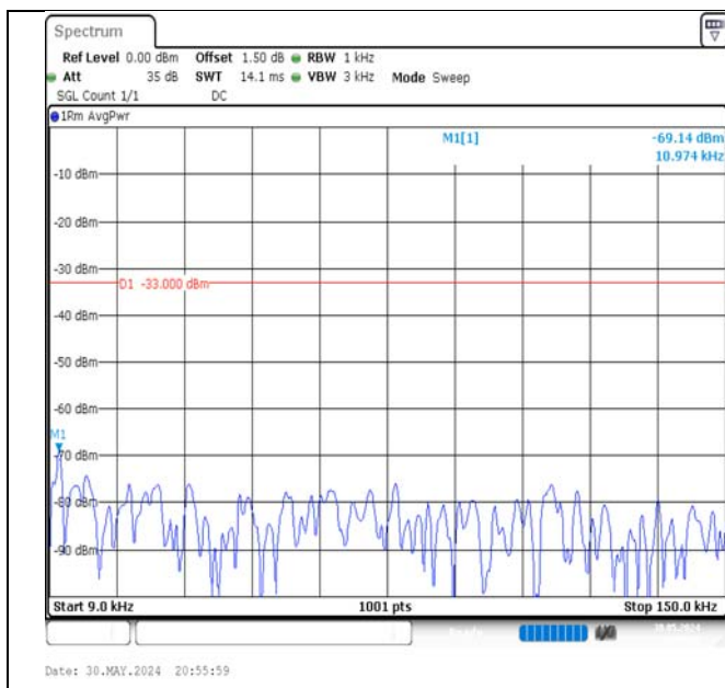
Band5-3MHz-16QAM-20525-1RB#14-0.009~0.15-PASS
