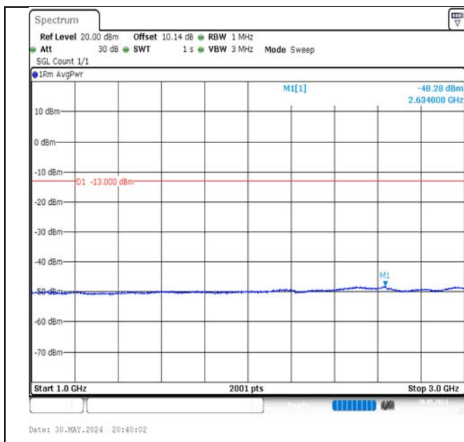
Band5-5MHz-16QAM-20425-1RB#0-1000~3000-PASS
