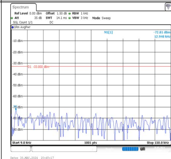
Band5-5MHz-QPSK-20625-25RB#0-0.009~0.15-PASS
