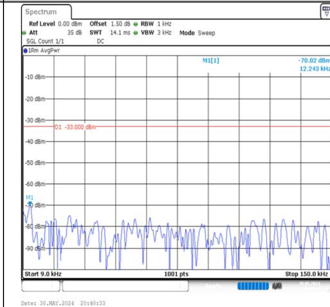
Band5-5MHz-16QAM-20425-1RB#24-0.009~0.15-PASS
