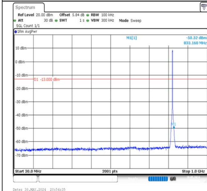
Band5-3MHz-16QAM-20415-15RB#0-30~1000-PASS
