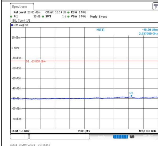
Band5-3MHz-16QAM-20525-15RB#0-1000~3000-PASS
