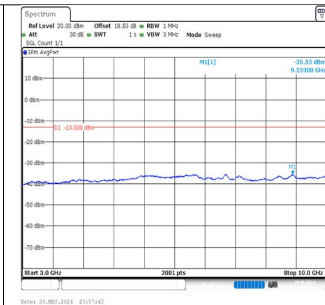
Band5-3MHz-16QAM-20635-1RB#0-3000~10000-PASS
