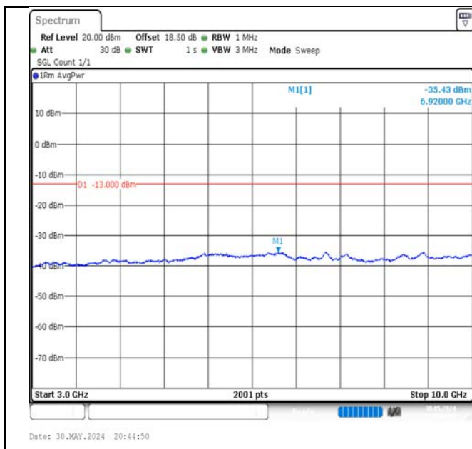
Band5-5MHz-QPSK-20625-1RB#24-3000~10000-PASS
