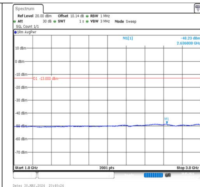
Band5-5MHz-QPSK-20425-1RB#24-1000~3000-PASS
