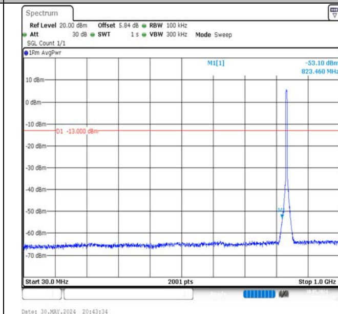
Band5-5MHz-16QAM-20525-25RB#0-30~1000-PASS
