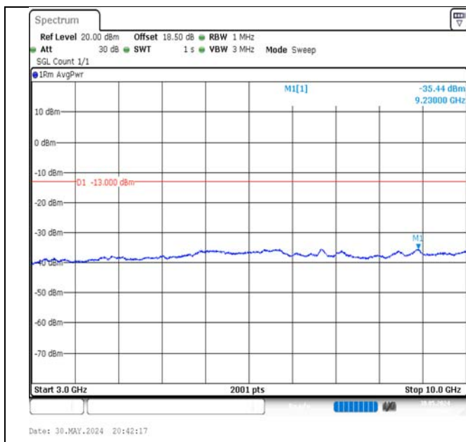
Band5-5MHz-16QAM-20525-1RB#0-3000~10000-PASS
