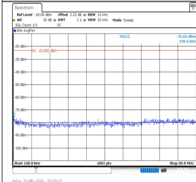
Band5-5MHz-16QAM-20525-25RB#0-0.15~30-PASS
