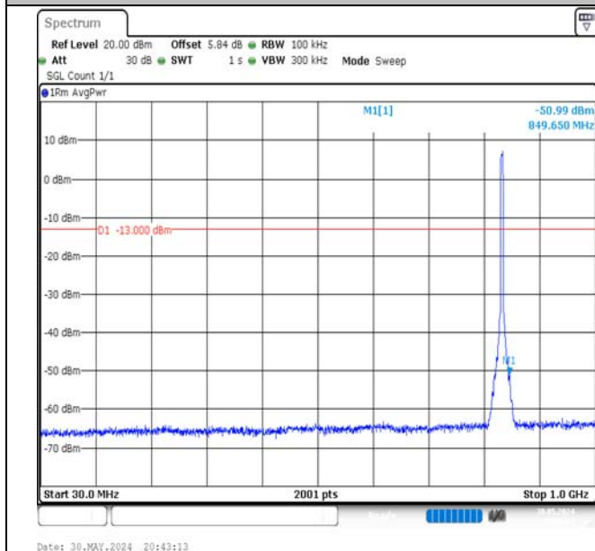
Band5-5MHz-QPSK-20525-25RB#0-30~1000-PASS
