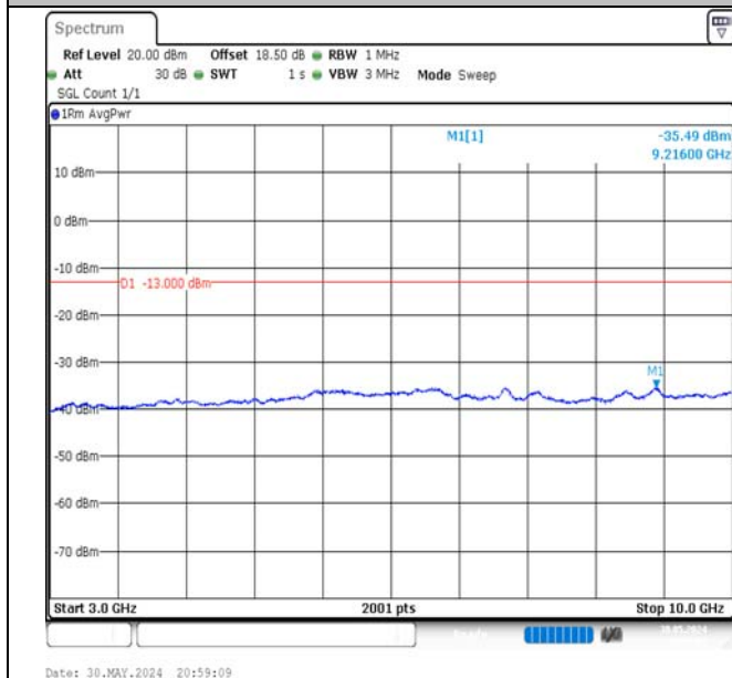
Band5-3MHz-16QAM-20635-15RB#0-3000~10000-PASS
