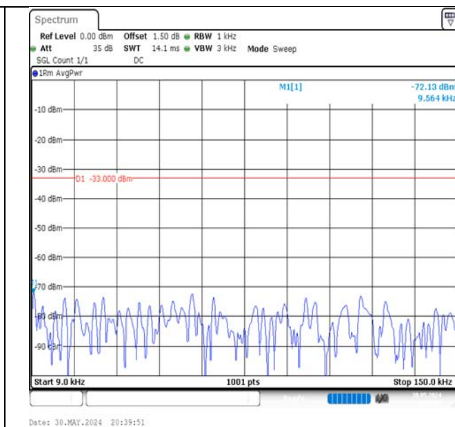
Band5-5MHz-16QAM-20425-1RB#0-0.009~0.15-PASS
