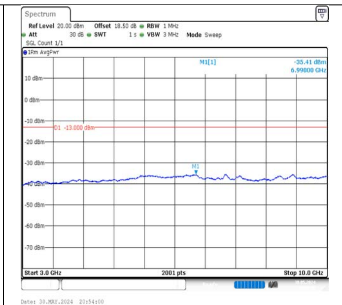
Band5-3MHz-16QAM-20415-1RB#14-3000~10000-PASS
