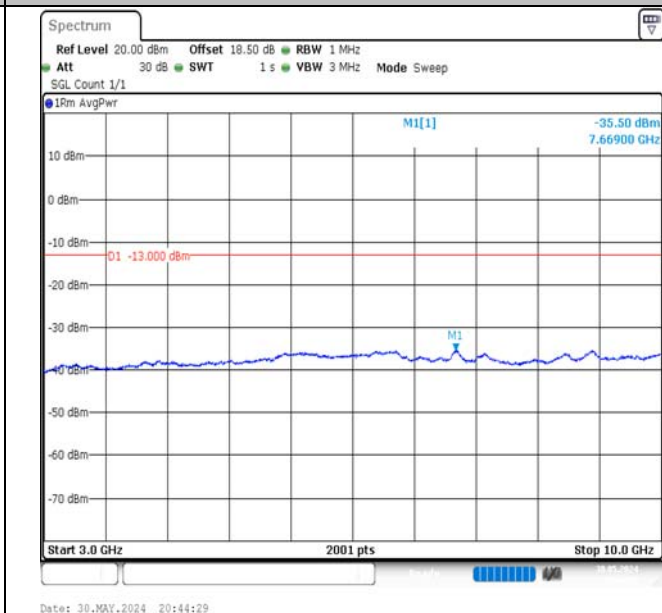
Band5-5MHz-16QAM-20625-1RB#0-3000~10000-PASS
