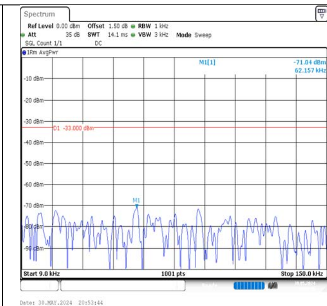
Band5-3MHz-16QAM-20415-1RB#14-0.009~0.15-PASS
