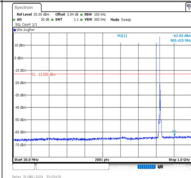
Band5-5MHz-16QAM-20425-1RB#0-30~1000-PASS
