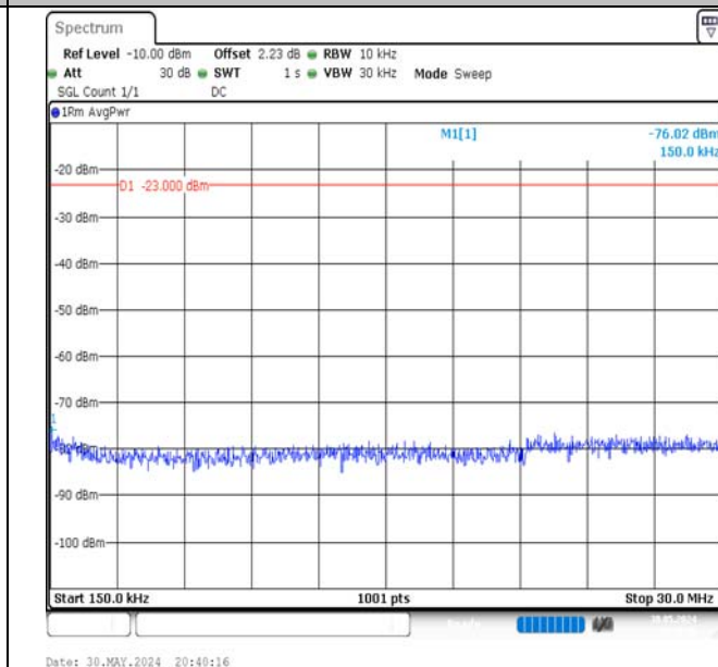
Band5-5MHz-QPSK-20425-1RB#24-0.15~30-PASS
