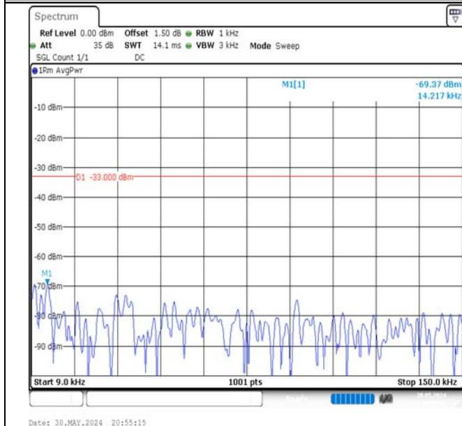
Band5-3MHz-16QAM-20525-1RB#0-0.009~0.15-PASS
