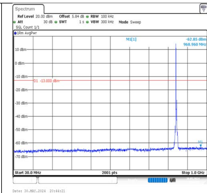
Band5-5MHz-16QAM-20625-1RB#0-30~1000-PASS
