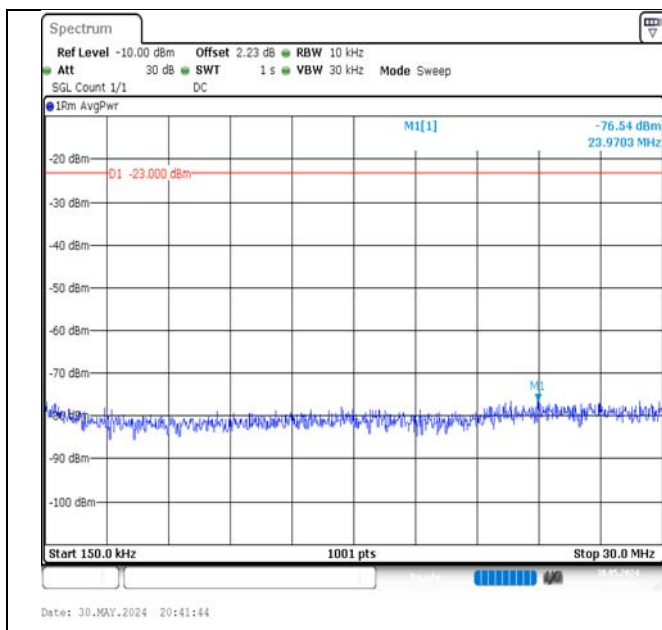
Band5-5MHz-QPSK-20525-1RB#0-0.15~30-PASS
