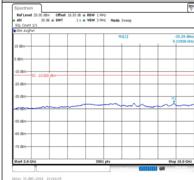
Band5-5MHz-QPSK-20625-1RB#0-3000~10000-PASS
