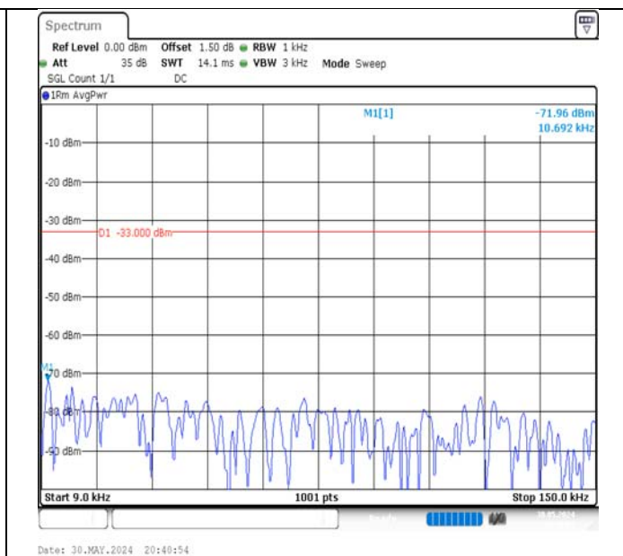
Band5-5MHz-QPSK-20425-25RB#0-0.009~0.15-PASS
