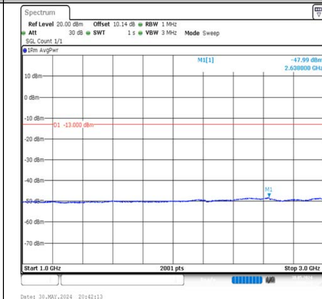
Band5-5MHz-16QAM-20525-1RB#0-1000~3000-PASS
