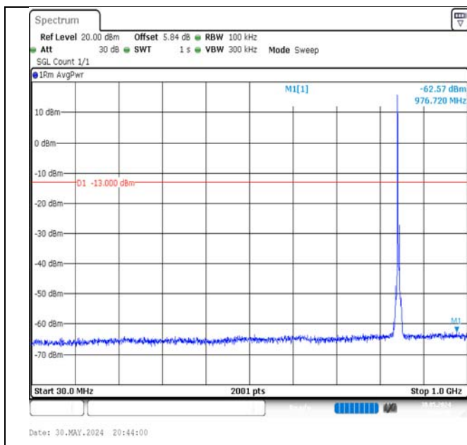
Band5-5MHz-QPSK-20625-1RB#0-30~1000-PASS
