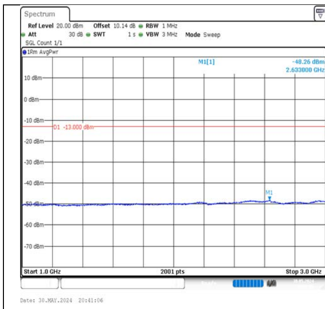
Band5-5MHz-QPSK-20425-25RB#0-1000~3000-PASS
