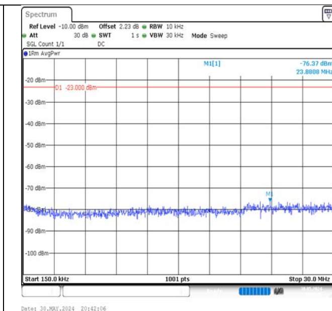
Band5-5MHz-16QAM-20525-1RB#0-0.15~30-PASS
