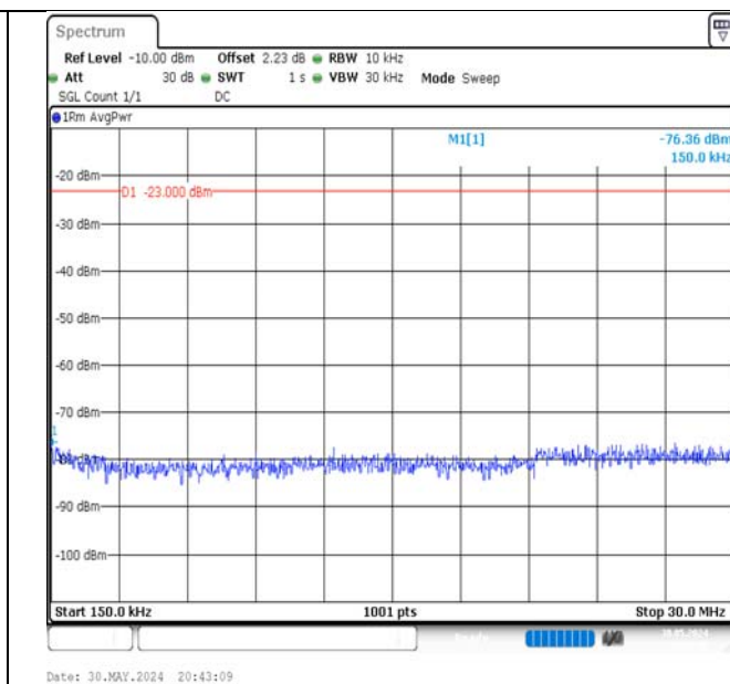
Band5-5MHz-QPSK-20525-25RB#0-0.15~30-PASS
