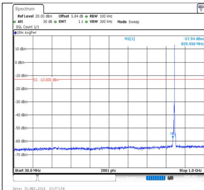
Band5-3MHz-QPSK-20635-1RB#14-30~1000-PASS
