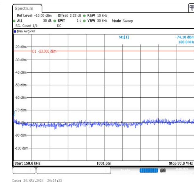
Band5-5MHz-QPSK-20425-1RB#0-0.15~30-PASS
