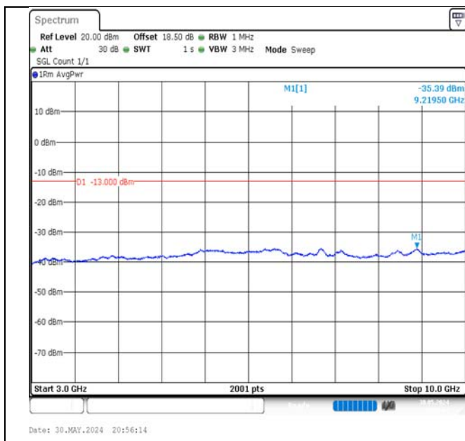
Band5-3MHz-16QAM-20525-1RB#14-3000~10000-PASS
