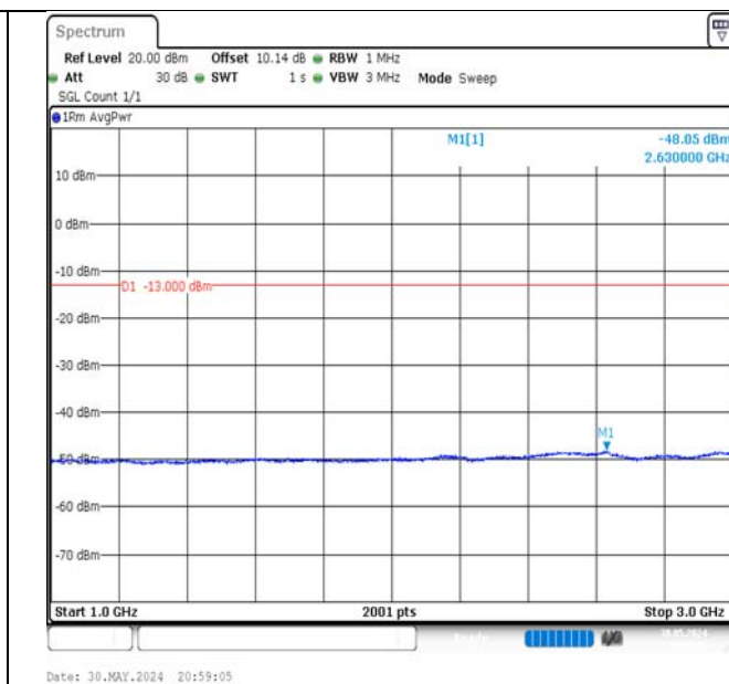
Band5-3MHz-16QAM-20635-15RB#0-1000~3000-PASS
