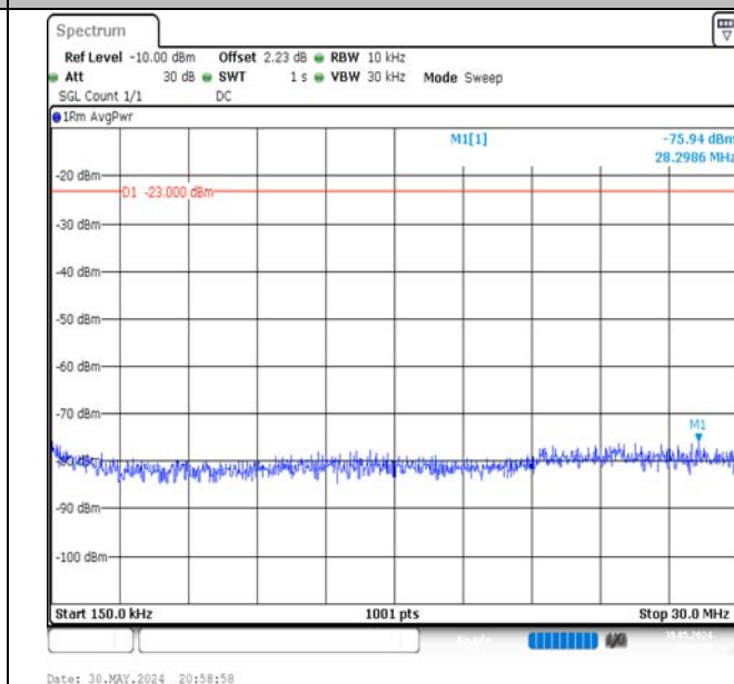
Band5-3MHz-16QAM-20635-15RB#0-0.15~30-PASS
