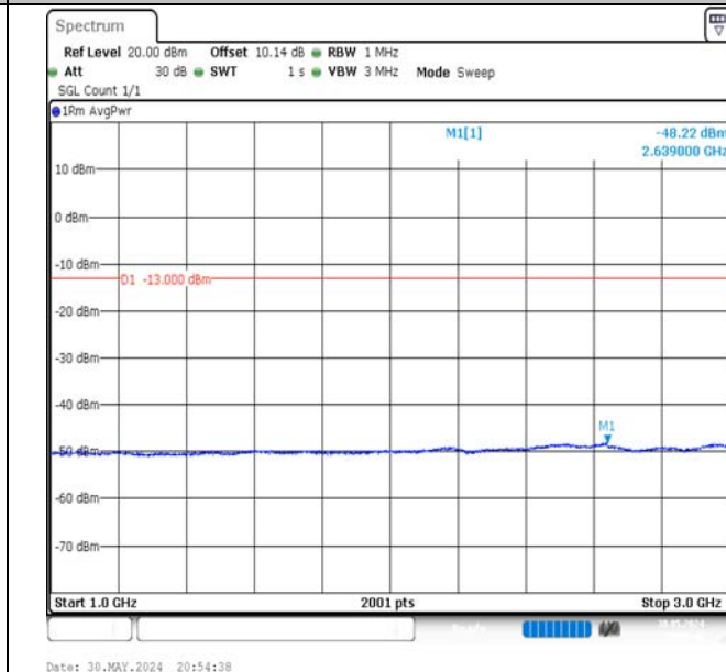
Band5-3MHz-16QAM-20415-15RB#0-1000~3000-PASS
