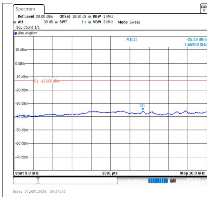
Band5-3MHz-16QAM-20415-15RB#0-3000~10000-PASS
