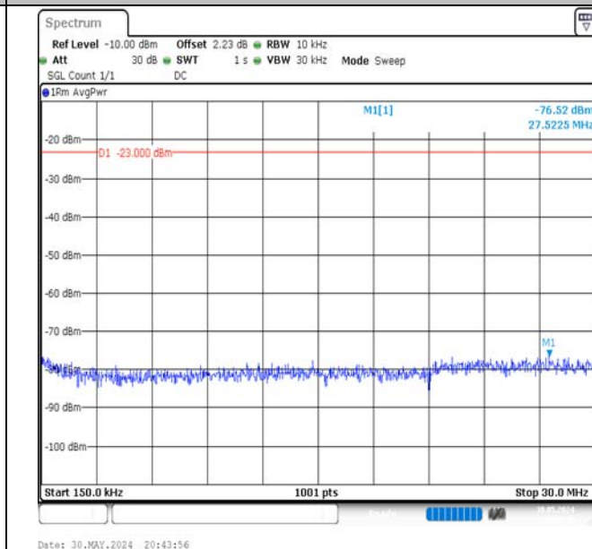
Band5-5MHz-QPSK-20625-1RB#0-0.15~30-PASS
