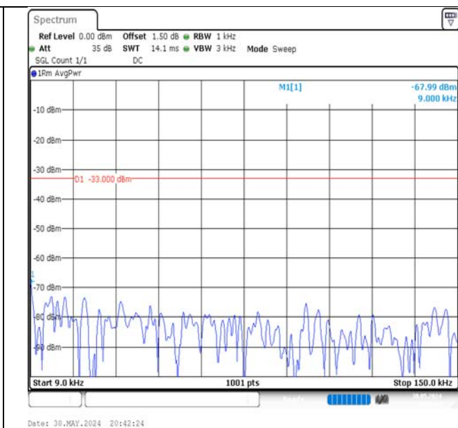
Band5-5MHz-QPSK-20525-1RB#24-0.009~0.15-PASS
