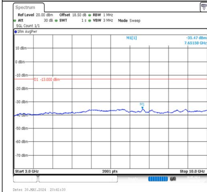
Band5-5MHz-16QAM-20425-25RB#0-3000~10000-PASS
