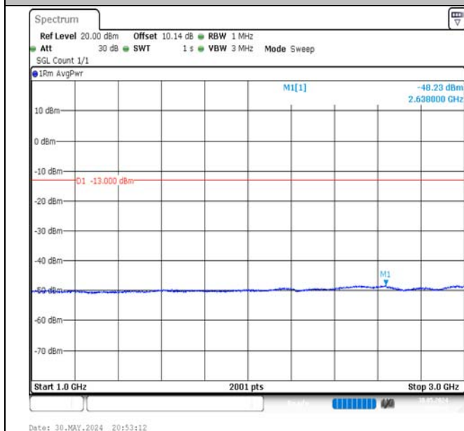
Band5-3MHz-16QAM-20415-1RB#0-1000~3000-PASS
