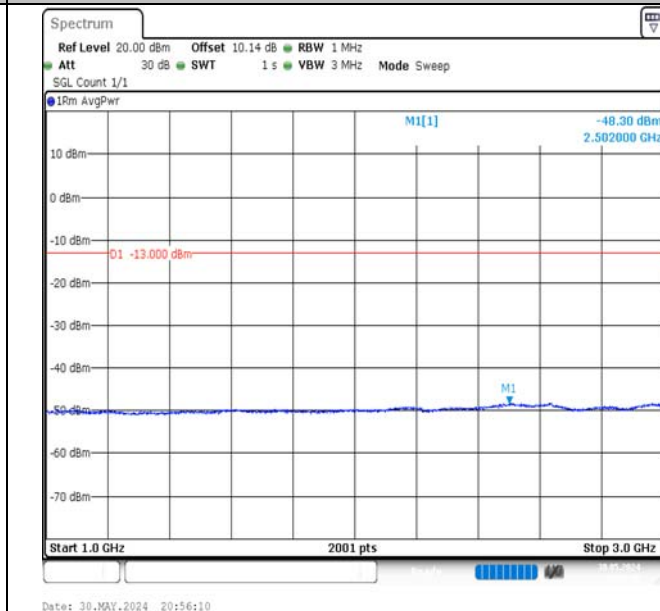
Band5-3MHz-16QAM-20525-1RB#14-1000~3000-PASS
