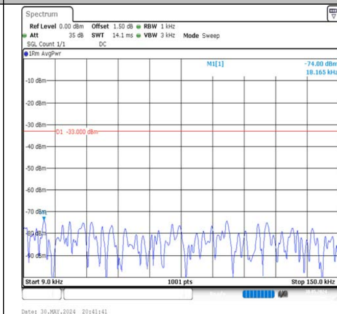
Band5-5MHz-QPSK-20525-1RB#0-0.009~0.15-PASS
