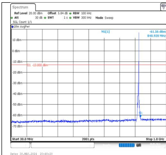
Band5-5MHz-QPSK-20425-1RB#24-30~1000-PASS
