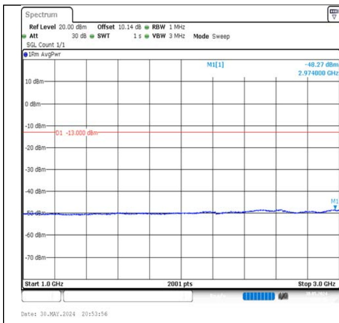
Band5-3MHz-16QAM-20415-1RB#14-1000~3000-PASS
