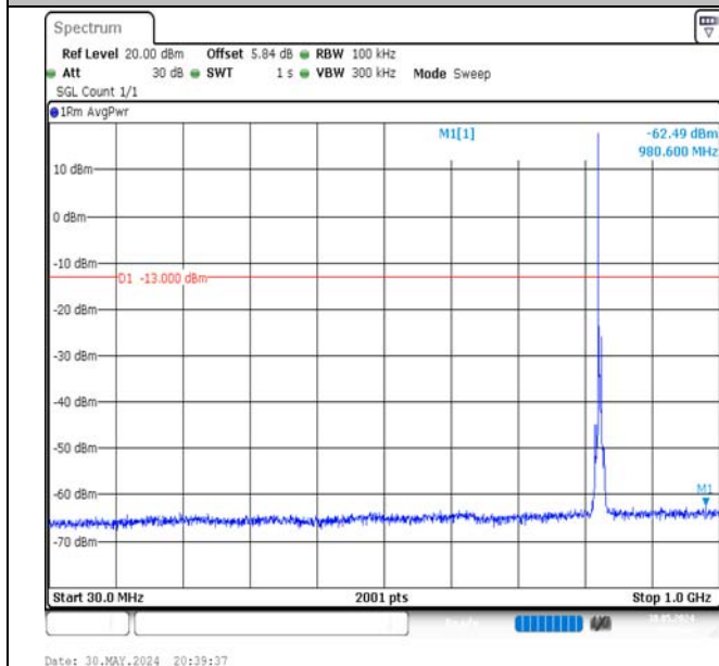
Band5-5MHz-QPSK-20425-1RB#0-30~1000-PASS
