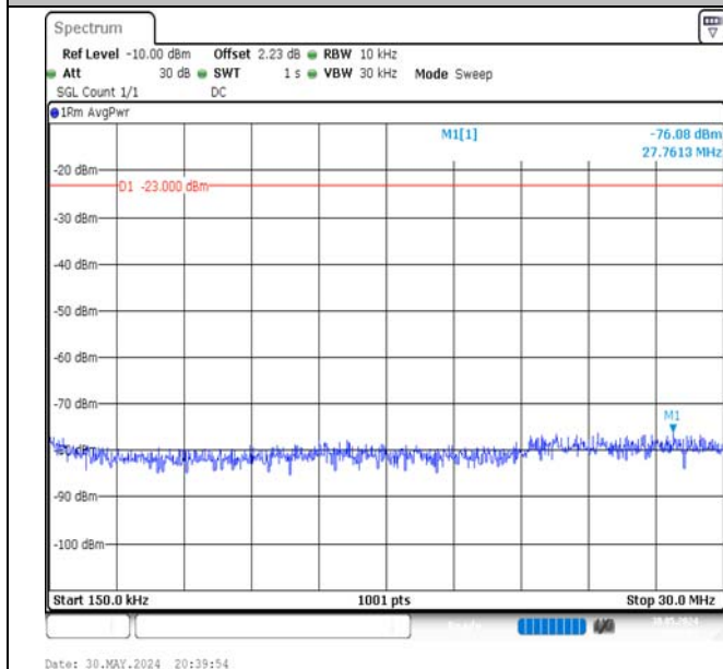
Band5-5MHz-16QAM-20425-1RB#0-0.15~30-PASS
