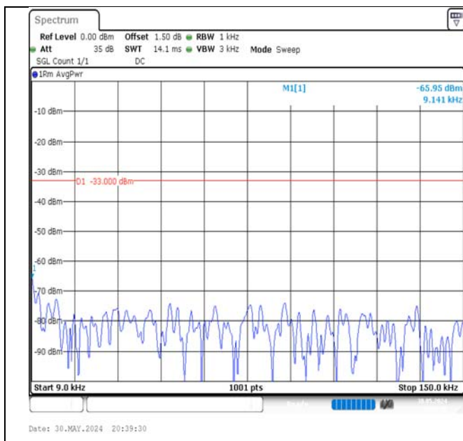
Band5-5MHz-QPSK-20425-1RB#0-0.009~0.15-PASS
