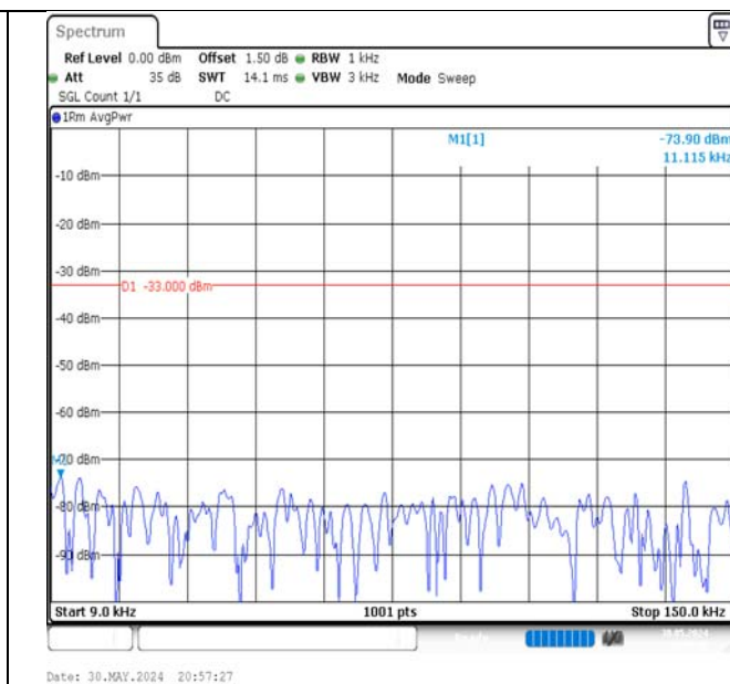
Band5-3MHz-16QAM-20635-1RB#0-0.009~0.15-PASS
