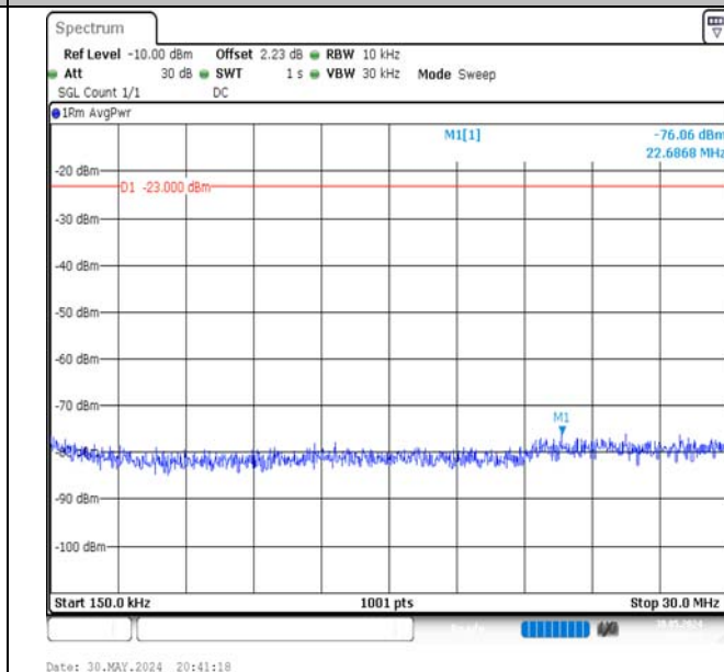
Band5-5MHz-16QAM-20425-25RB#0-0.15~30-PASS
