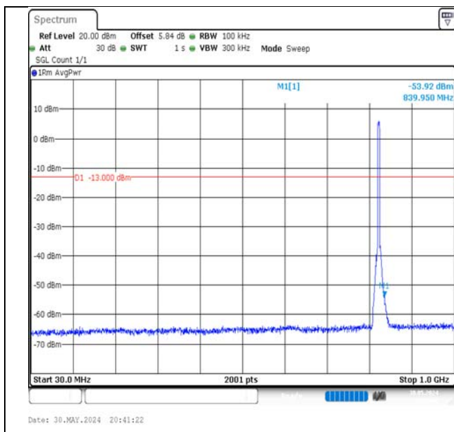
Band5-5MHz-16QAM-20425-25RB#0-30~1000-PASS
