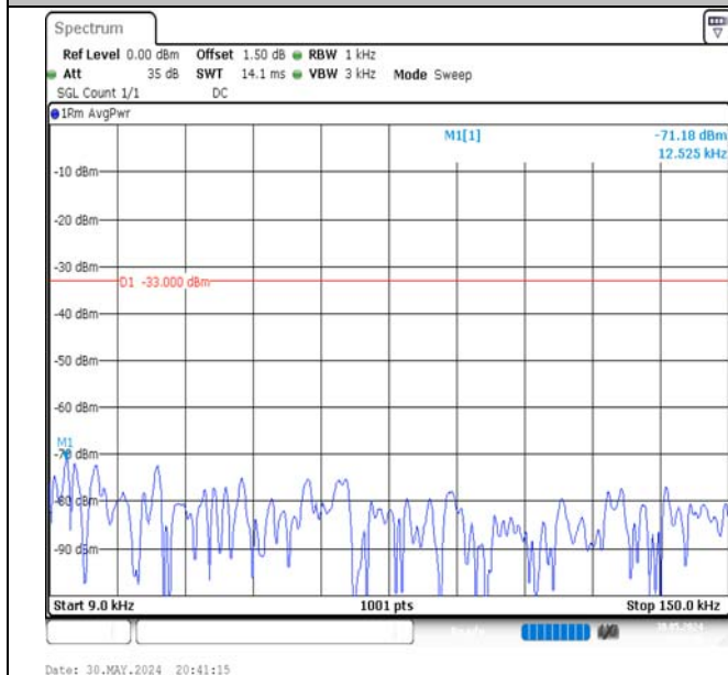
Band5-5MHz-16QAM-20425-25RB#0-0.009~0.15-PASS
