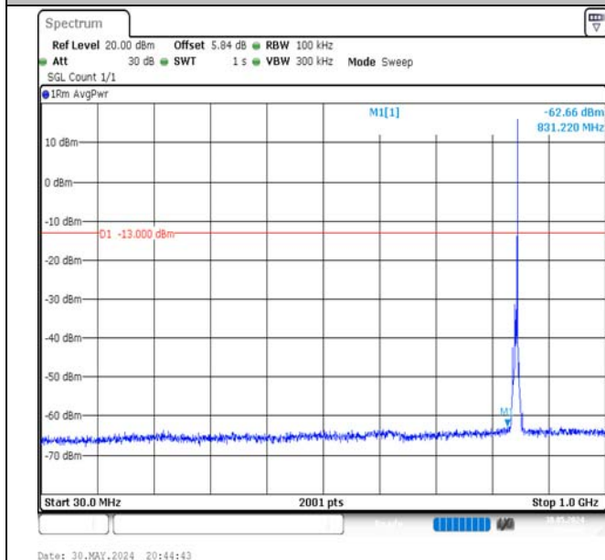
Band5-5MHz-QPSK-20625-1RB#24-30~1000-PASS
