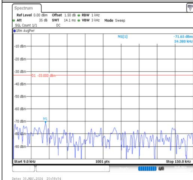
Band5-3MHz-16QAM-20635-15RB#0-0.009~0.15-PASS
