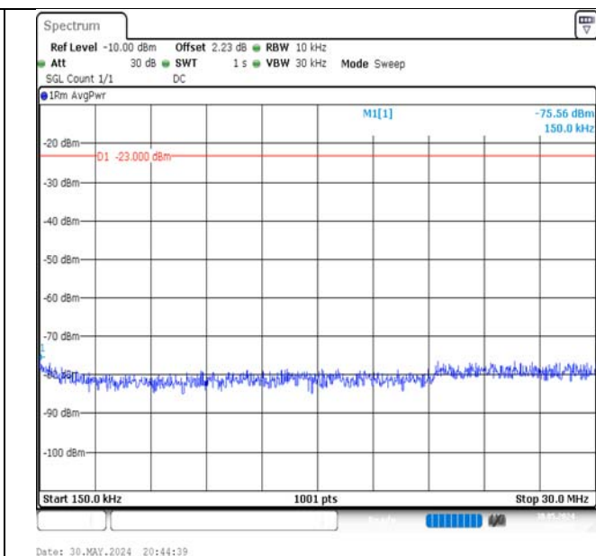
Band5-5MHz-QPSK-20625-1RB#24-0.15~30-PASS
