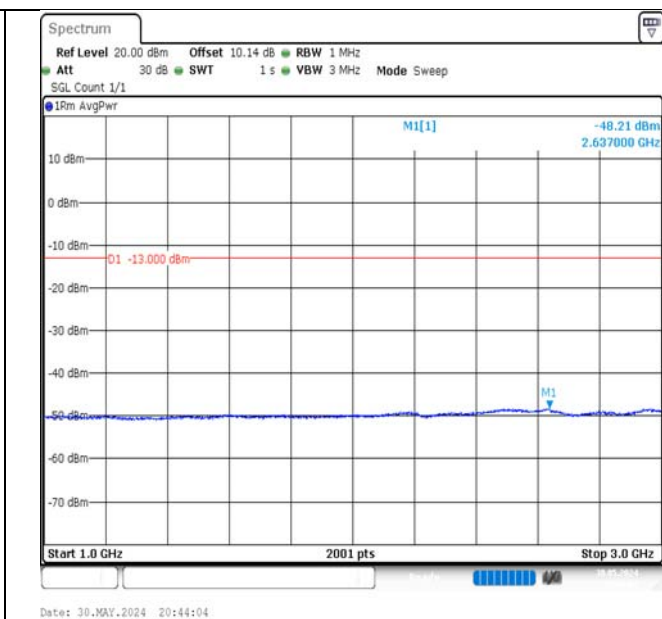
Band5-5MHz-QPSK-20625-1RB#0-1000~3000-PASS
