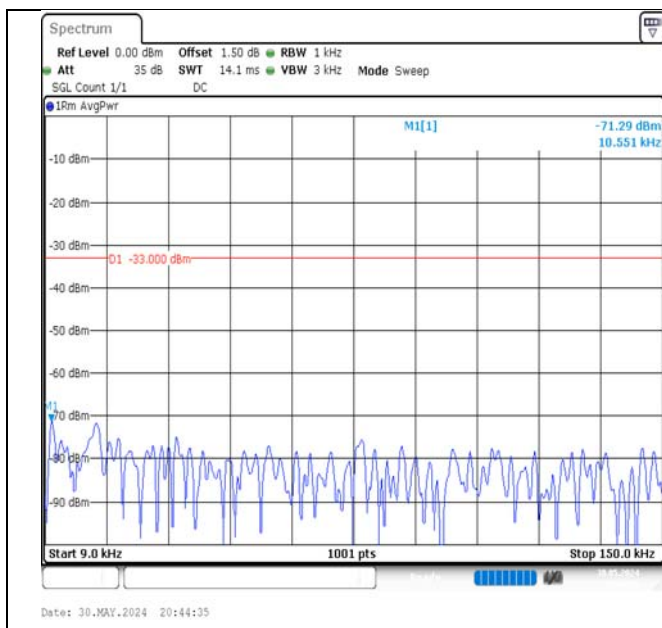
Band5-5MHz-QPSK-20625-1RB#24-0.009~0.15-PASS
