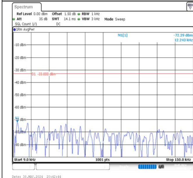
Band5-5MHz-16QAM-20525-1RB#24-0.009~0.15-PASS
