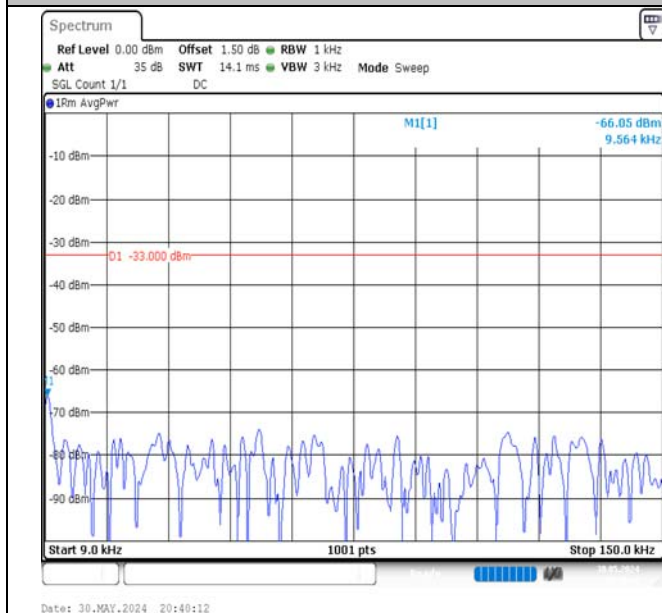
Band5-5MHz-QPSK-20425-1RB#24-0.009~0.15-PASS
