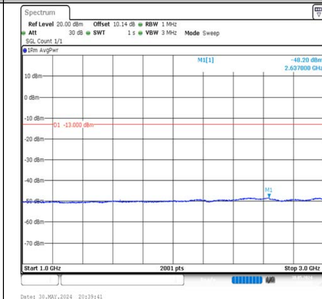
Band5-5MHz-QPSK-20425-1RB#0-1000~3000-PASS
