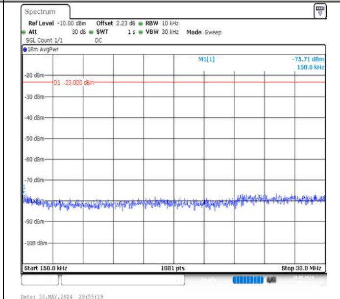
Band5-3MHz-16QAM-20525-1RB#0-0.15~30-PASS
