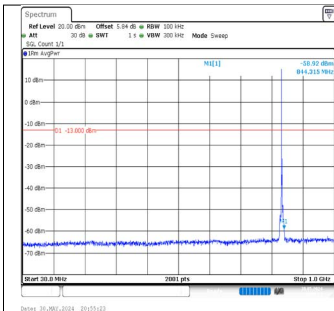
Band5-3MHz-16QAM-20525-1RB#0-30~1000-PASS
