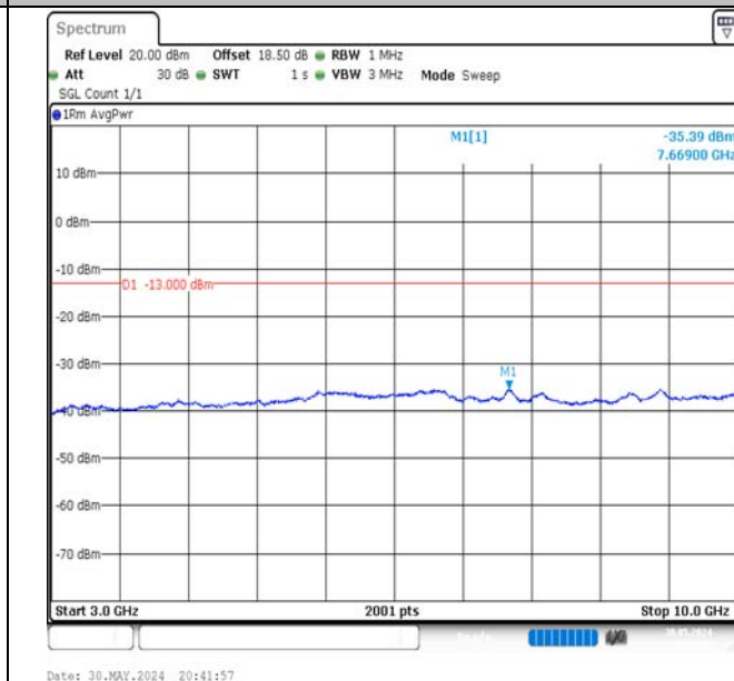
Band5-5MHz-QPSK-20525-1RB#0-3000~10000-PASS
