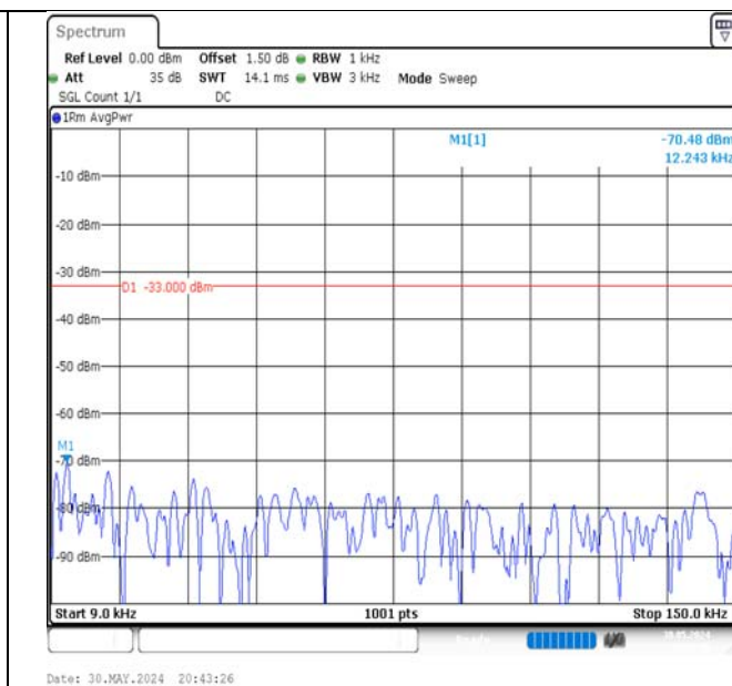
Band5-5MHz-16QAM-20525-25RB#0-0.009~0.15-PASS
