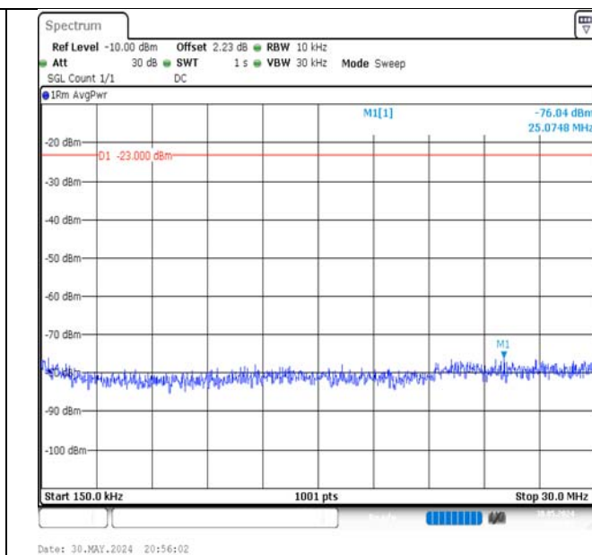
Band5-3MHz-16QAM-20525-1RB#14-0.15~30-PASS
