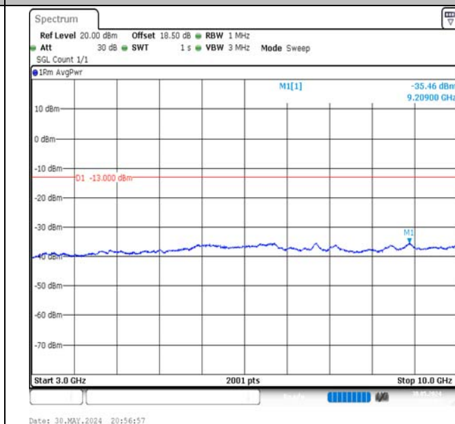
Band5-3MHz-16QAM-20525-15RB#0-3000~10000-PASS
