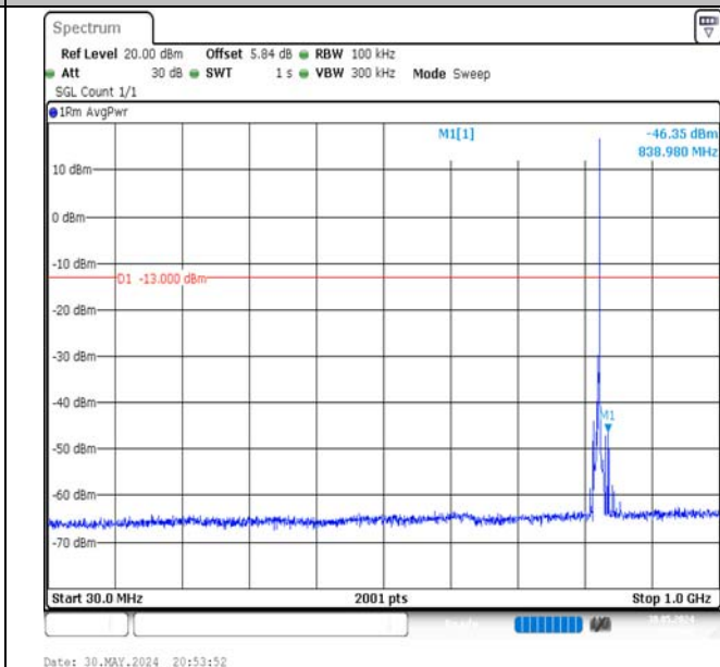
Band5-3MHz-16QAM-20415-1RB#14-30~1000-PASS
