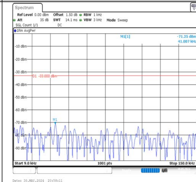
Band5-3MHz-16QAM-20635-1RB#14-0.009~0.15-PASS
