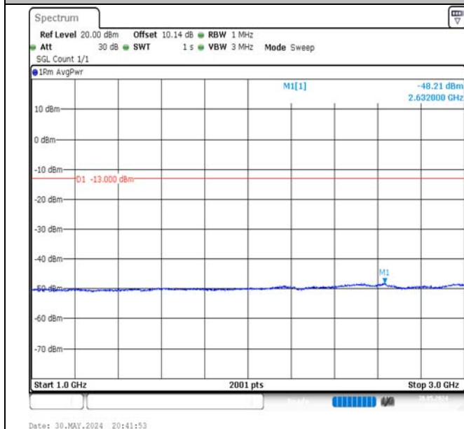
Band5-5MHz-QPSK-20525-1RB#0-1000~3000-PASS
