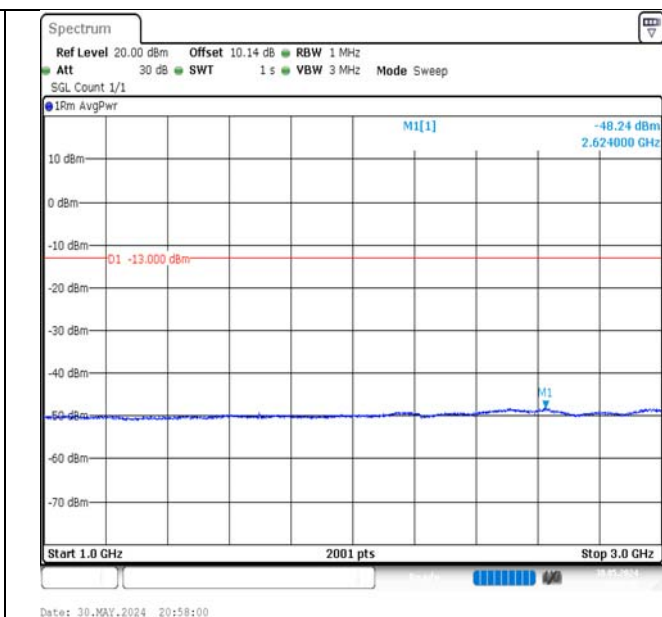
Band5-3MHz-QPSK-20635-1RB#14-1000~3000-PASS
