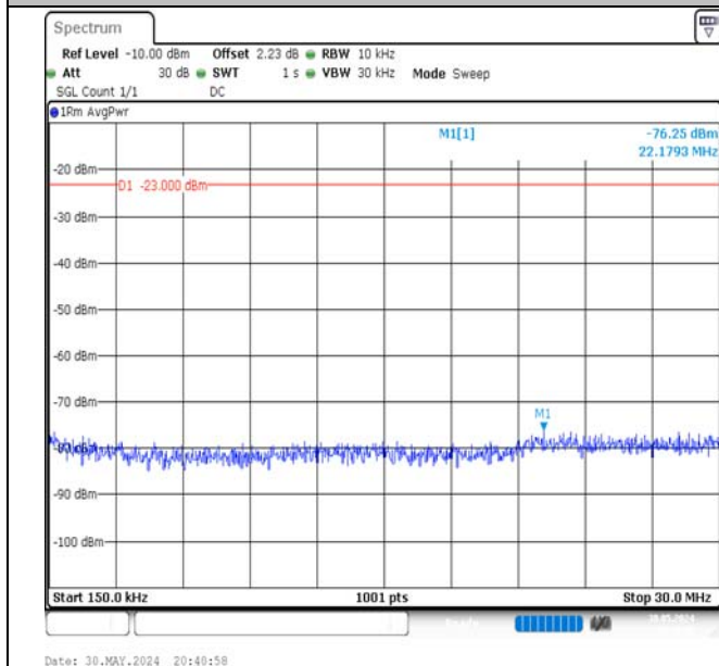
Band5-5MHz-QPSK-20425-25RB#0-0.15~30-PASS
