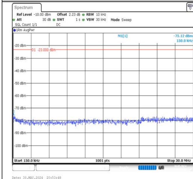
Band5-3MHz-16QAM-20415-1RB#14-0.15~30-PASS
