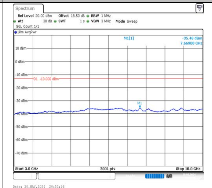
Band5-3MHz-16QAM-20415-1RB#0-3000~10000-PASS
