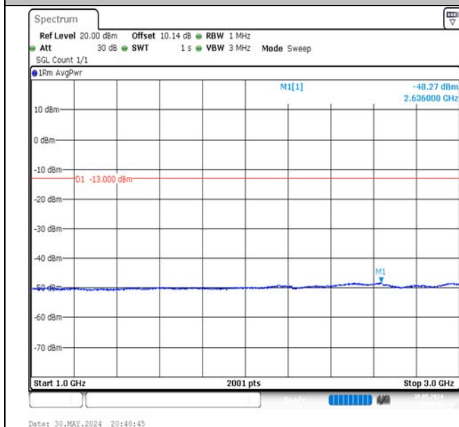
Band5-5MHz-16QAM-20425-1RB#24-1000~3000-PASS
