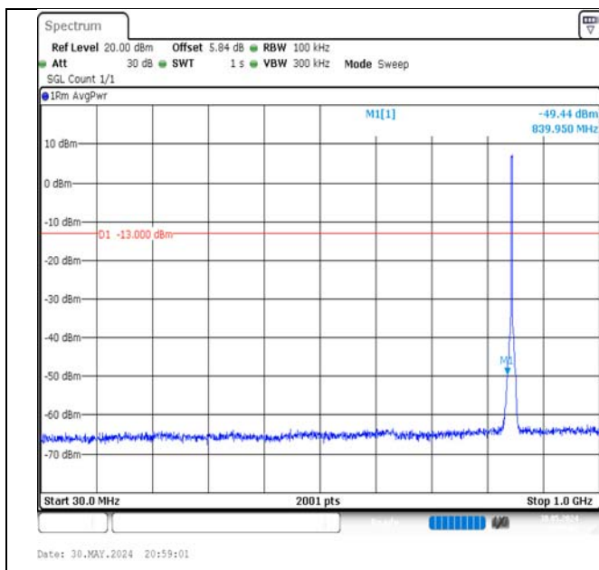
Band5-3MHz-16QAM-20635-15RB#0-30~1000-PASS
