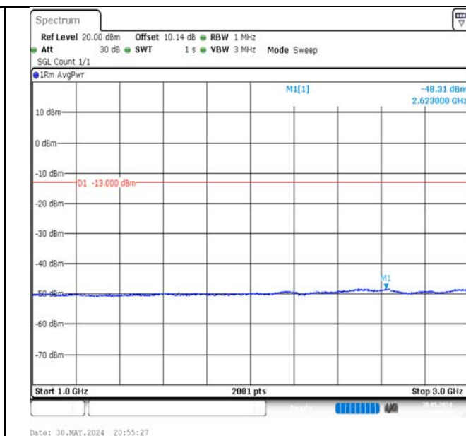
Band5-3MHz-16QAM-20525-1RB#0-1000~3000-PASS
