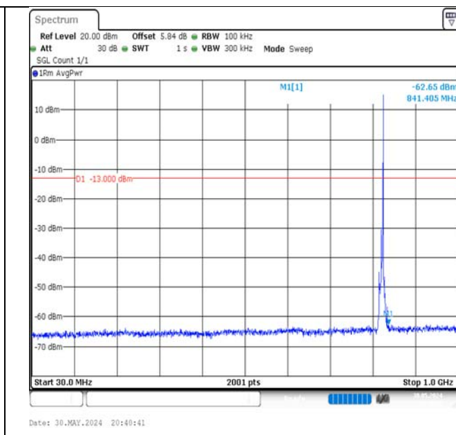
Band5-5MHz-16QAM-20425-1RB#24-30~1000-PASS
