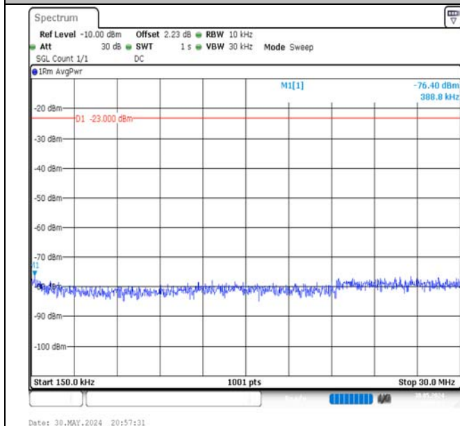
Band5-3MHz-16QAM-20635-1RB#0-0.15~30-PASS
