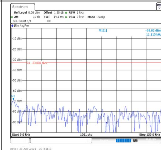
Band5-5MHz-16QAM-20625-1RB#0-0.009~0.15-PASS
