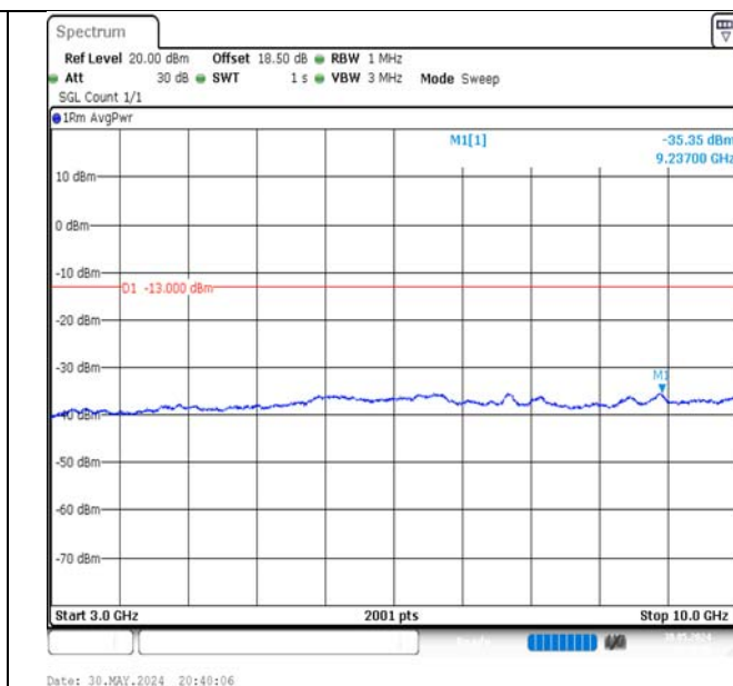
Band5-5MHz-16QAM-20425-1RB#0-3000~10000-PASS
