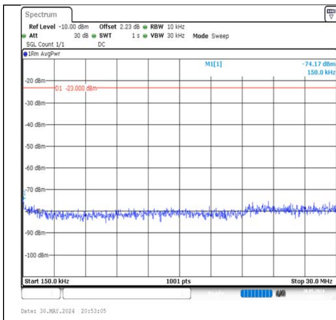
Band5-3MHz-16QAM-20415-1RB#0-0.15~30-PASS
