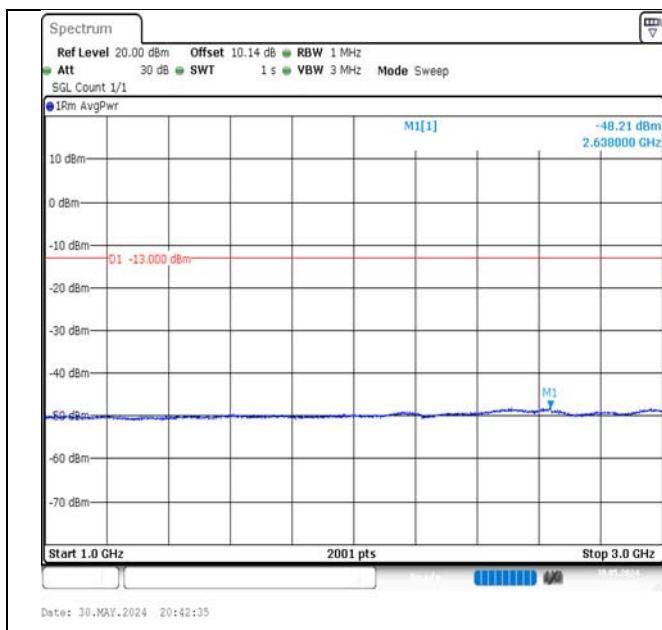
Band5-5MHz-QPSK-20525-1RB#24-1000~3000-PASS
