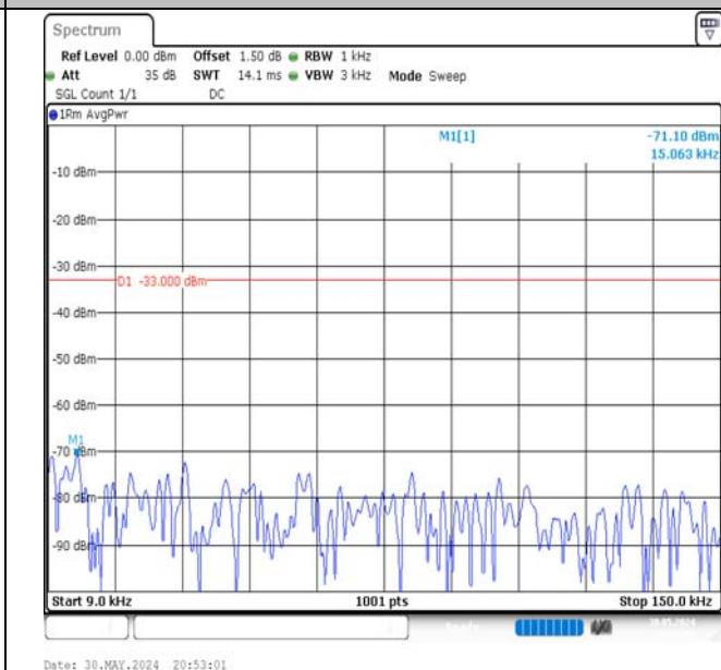
Band5-3MHz-16QAM-20415-1RB#0-0.009~0.15-PASS
