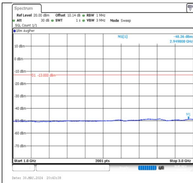
Band5-5MHz-16QAM-20525-25RB#0-1000~3000-PASS
