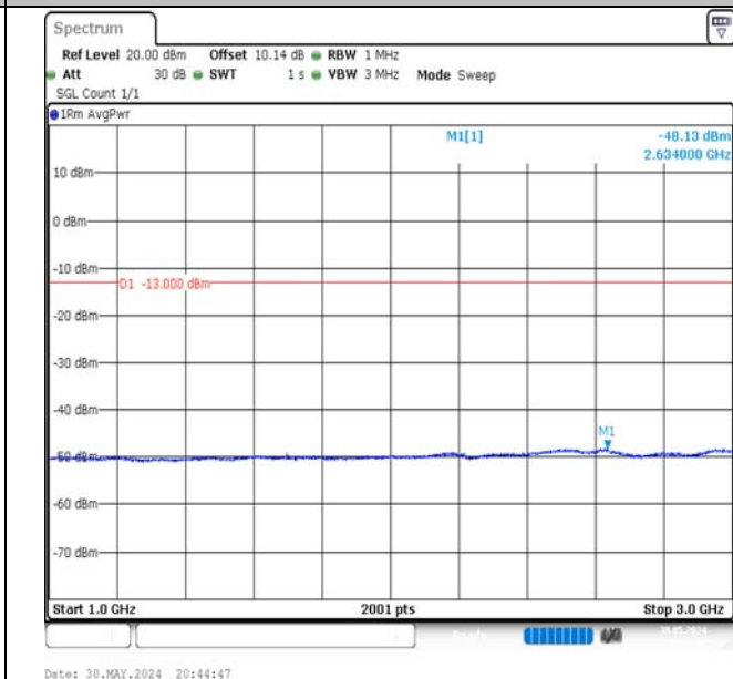
Band5-5MHz-QPSK-20625-1RB#24-1000~3000-PASS
