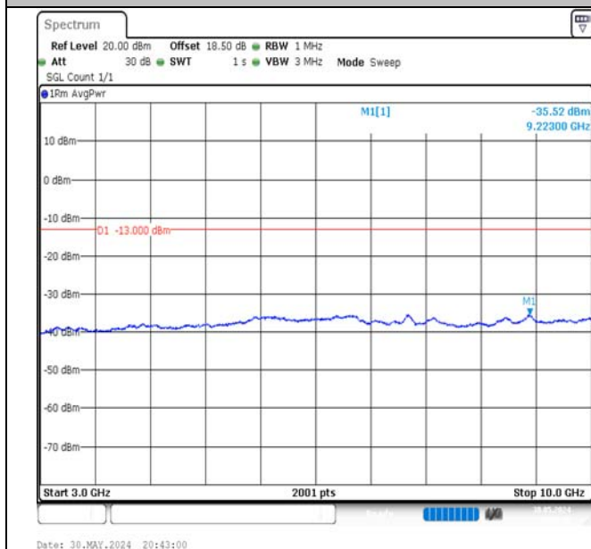
Band5-5MHz-16QAM-20525-1RB#24-3000~10000-PASS
