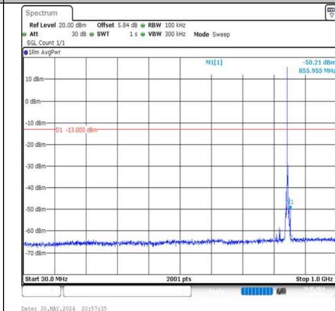
Band5-3MHz-16QAM-20635-1RB#0-30~1000-PASS
