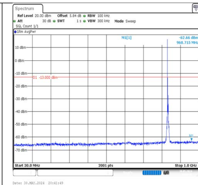
Band5-5MHz-QPSK-20525-1RB#0-30~1000-PASS
