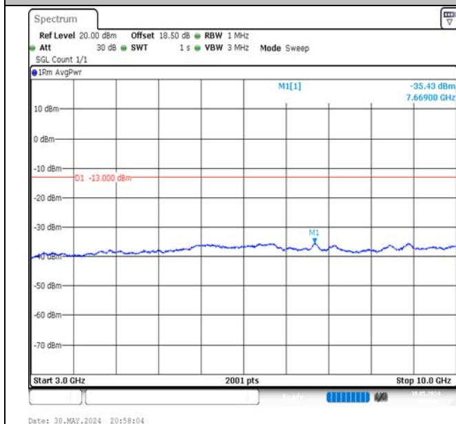
Band5-3MHz-QPSK-20635-1RB#14-3000~10000-PASS
