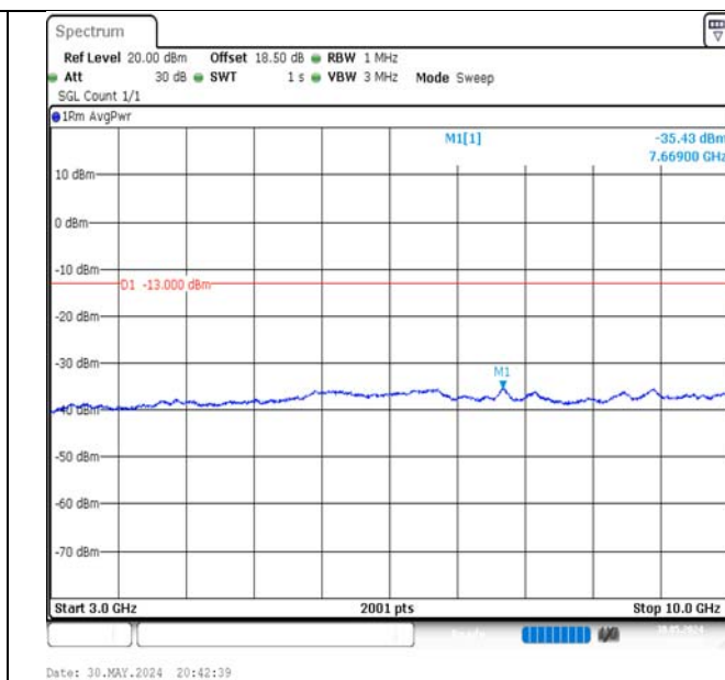
Band5-5MHz-QPSK-20525-1RB#24-3000~10000-PASS
