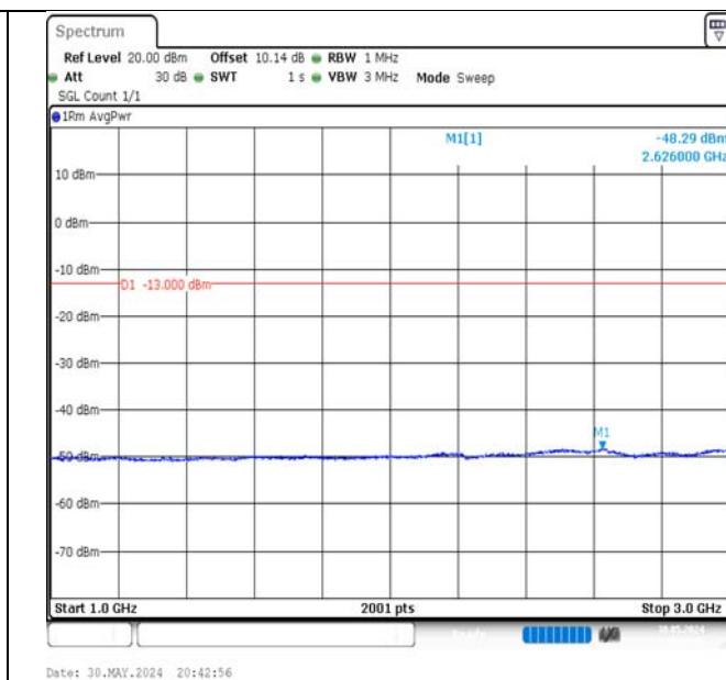
Band5-5MHz-16QAM-20525-1RB#24-1000~3000-PASS
