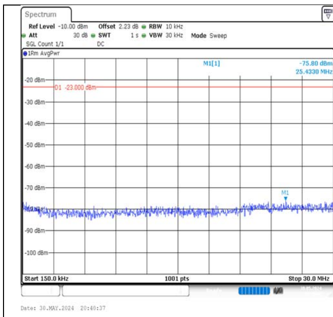
Band5-5MHz-16QAM-20425-1RB#24-0.15~30-PASS
