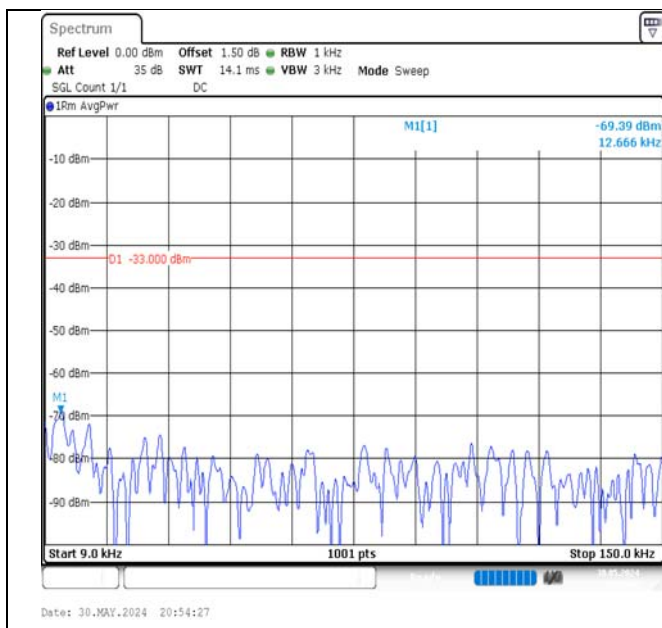
Band5-3MHz-16QAM-20415-15RB#0-0.009~0.15-PASS
