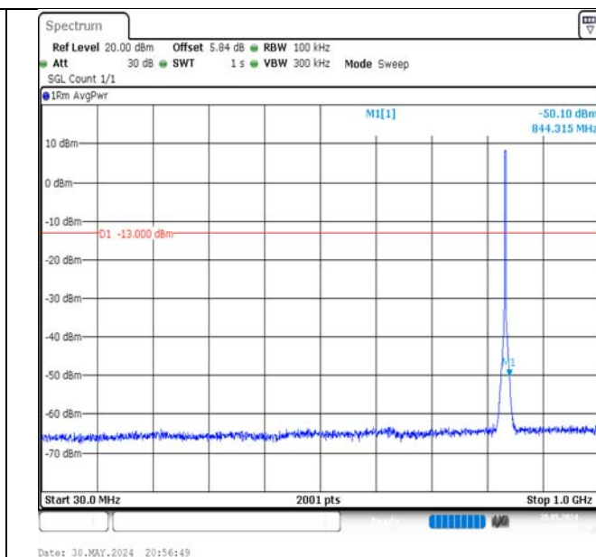
Band5-3MHz-16QAM-20525-15RB#0-30~1000-PASS
