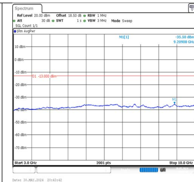
Band5-5MHz-16QAM-20525-25RB#0-3000~10000-PASS
