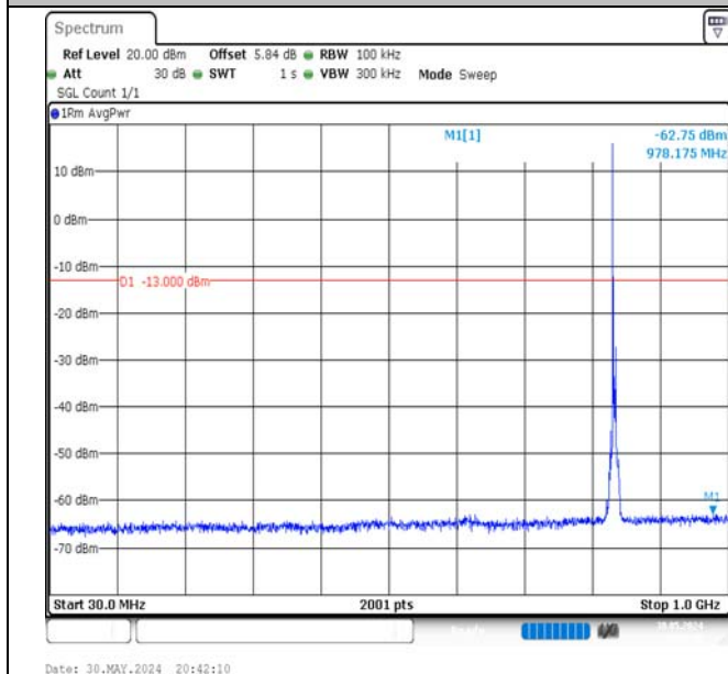
Band5-5MHz-16QAM-20525-1RB#0-30~1000-PASS
