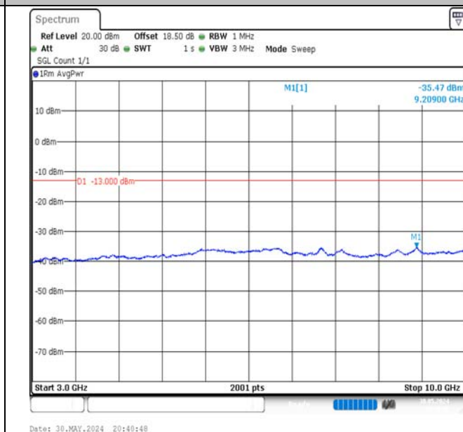
Band5-5MHz-16QAM-20425-1RB#24-3000~10000-PASS
