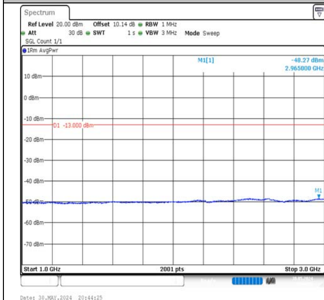
Band5-5MHz-16QAM-20625-1RB#0-1000~3000-PASS
