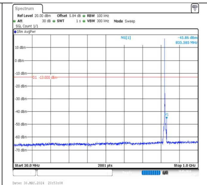
Band5-3MHz-16QAM-20415-1RB#0-30~1000-PASS
