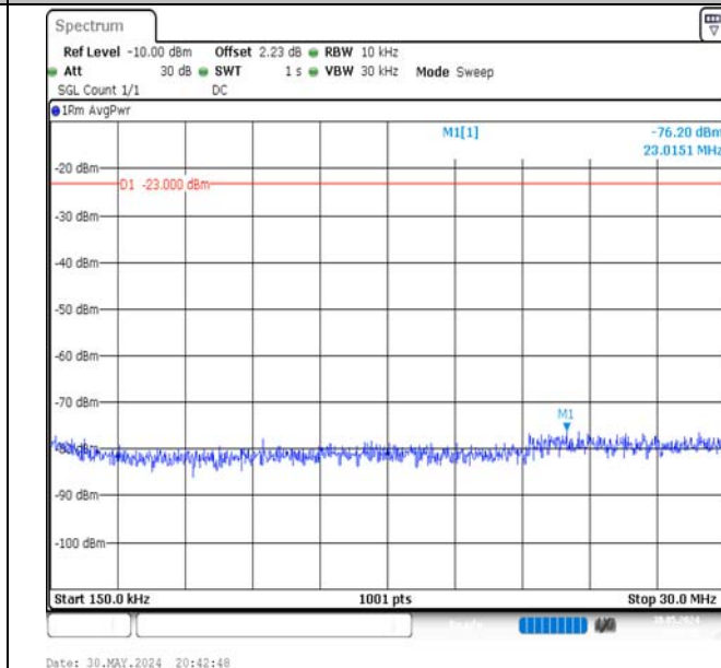
Band5-5MHz-16QAM-20525-1RB#24-0.15~30-PASS
