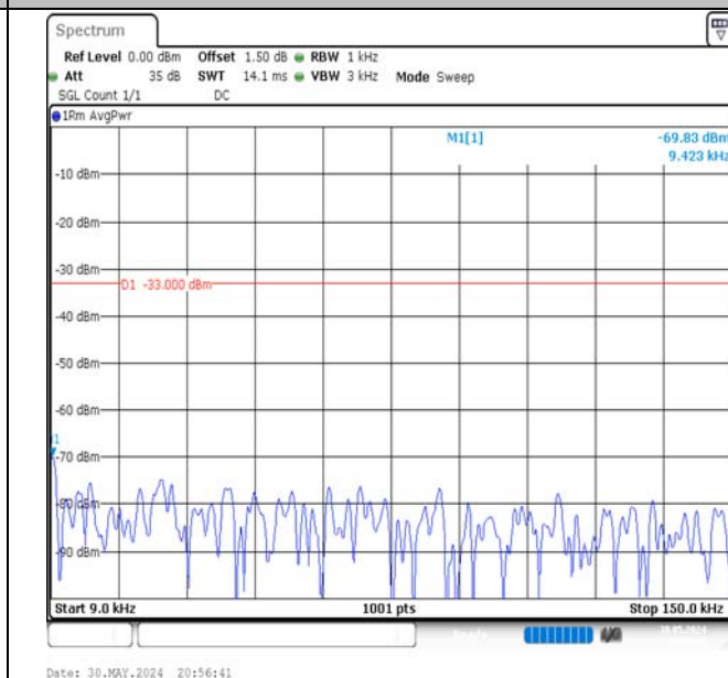
Band5-3MHz-16QAM-20525-15RB#0-0.009~0.15-PASS
