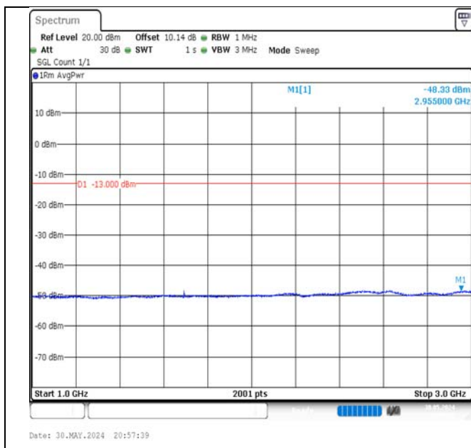
Band5-3MHz-16QAM-20635-1RB#0-1000~3000-PASS
