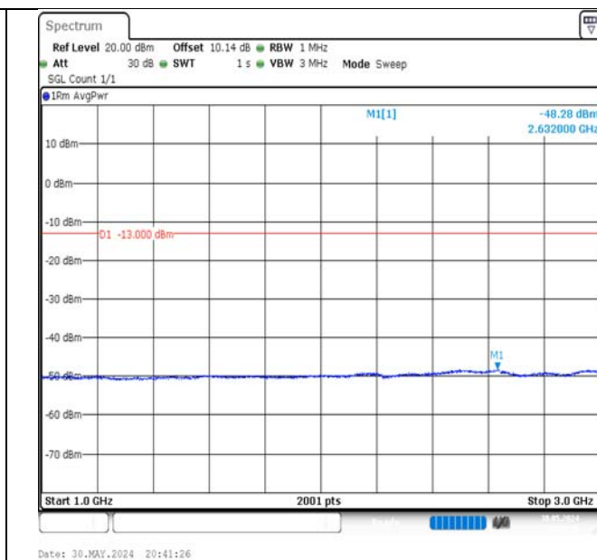
Band5-5MHz-16QAM-20425-25RB#0-1000~3000-PASS
