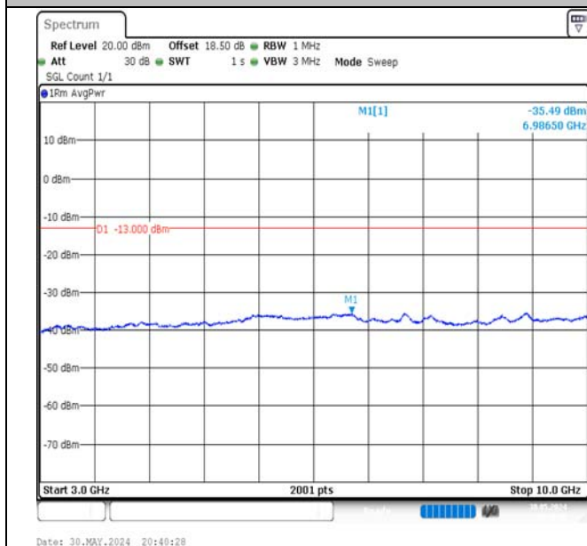
Band5-5MHz-QPSK-20425-1RB#24-3000~10000-PASS
