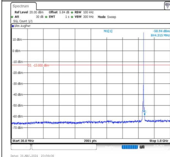
Band5-3MHz-16QAM-20525-1RB#14-30~1000-PASS
