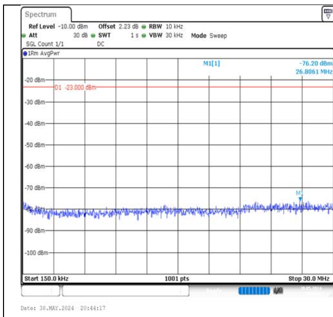
Band5-5MHz-16QAM-20625-1RB#0-0.15~30-PASS
