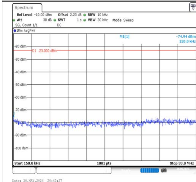
Band5-5MHz-QPSK-20525-1RB#24-0.15~30-PASS
