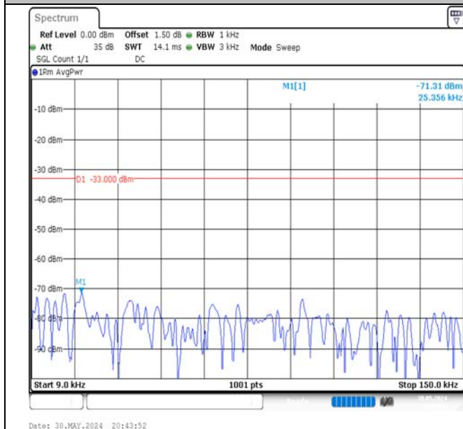
Band5-5MHz-QPSK-20625-1RB#0-0.009~0.15-PASS
