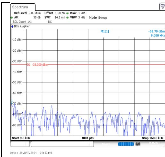
Band5-5MHz-QPSK-20525-25RB#0-0.009~0.15-PASS
