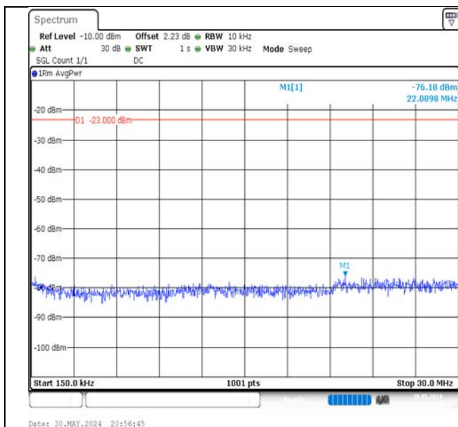
Band5-3MHz-16QAM-20525-15RB#0-0.15~30-PASS
