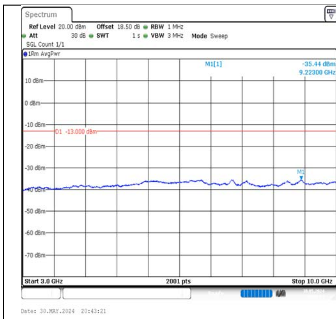
Band5-5MHz-QPSK-20525-25RB#0-3000~10000-PASS
