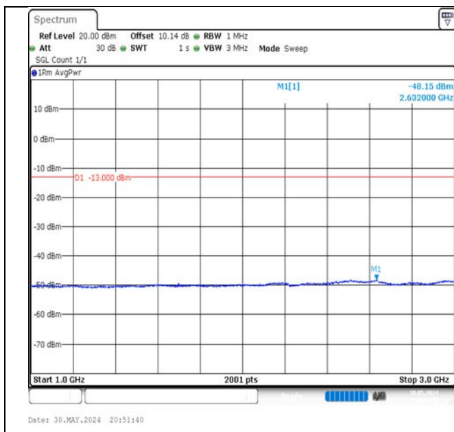
Band5-1.4MHz-16QAM-20643-1RB#5-1000~3000-PASS
