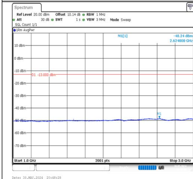
Band5-1.4MHz-QPSK-20525-1RB#0-1000~3000-PASS
