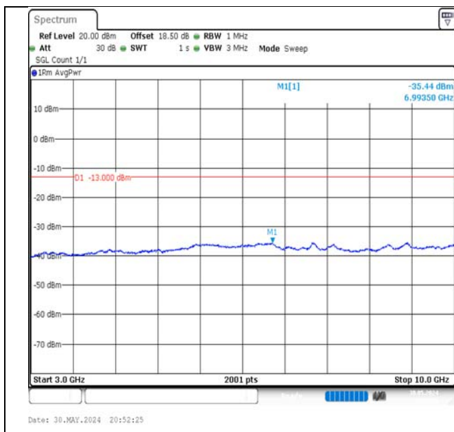
Band5-1.4MHz-16QAM-20643-6RB#0-3000~10000-PASS
