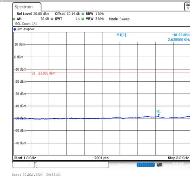
Band5-3MHz-QPSK-20415-1RB#14-1000~3000-PASS
