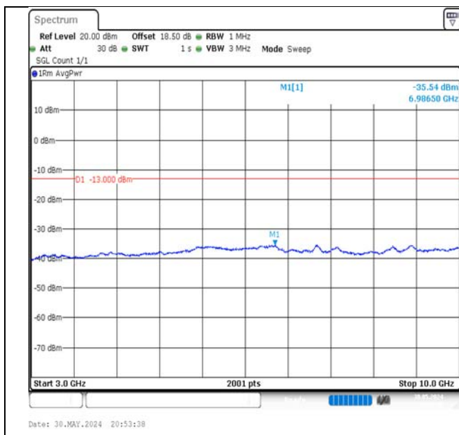
Band5-3MHz-QPSK-20415-1RB#14-3000~10000-PASS
