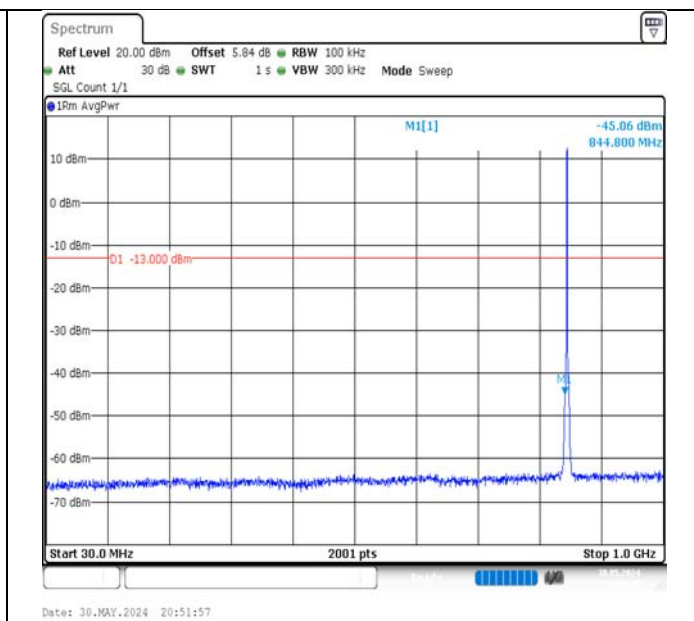
Band5-1.4MHz-QPSK-20643-6RB#0-30~1000-PASS
