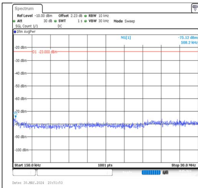
Band5-1.4MHz-QPSK-20643-6RB#0-0.15~30-PASS
