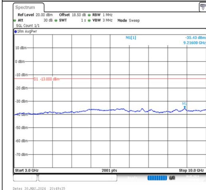
Band5-1.4MHz-16QAM-20525-1RB#5-3000~10000-PASS
