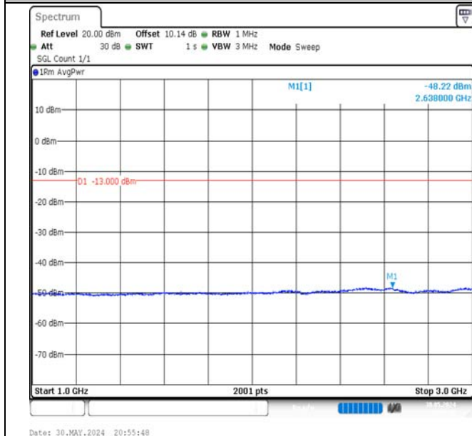
Band5-3MHz-QPSK-20525-1RB#14-1000~3000-PASS
