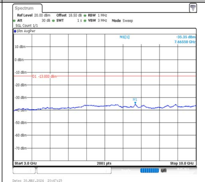
Band5-1.4MHz-16QAM-20407-1RB#5-3000~10000-PASS
