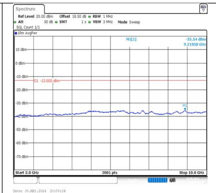
Band5-1.4MHz-16QAM-20525-6RB#0-3000~10000-PASS
