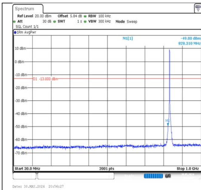
Band5-3MHz-QPSK-20525-15RB#0-30~1000-PASS
