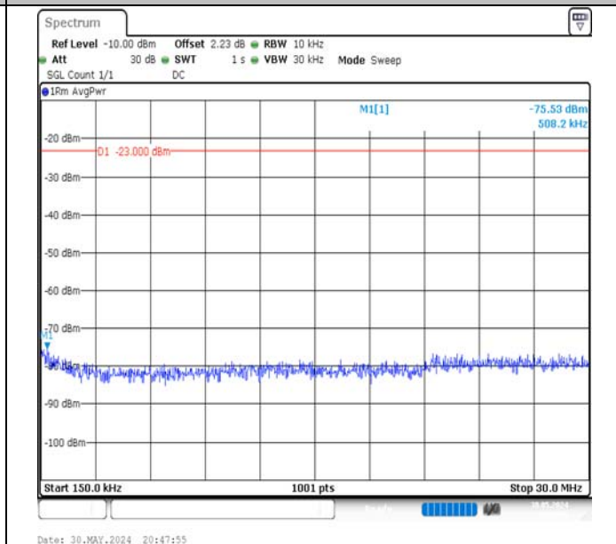
Band5-1.4MHz-16QAM-20407-6RB#0-0.15~30-PASS
