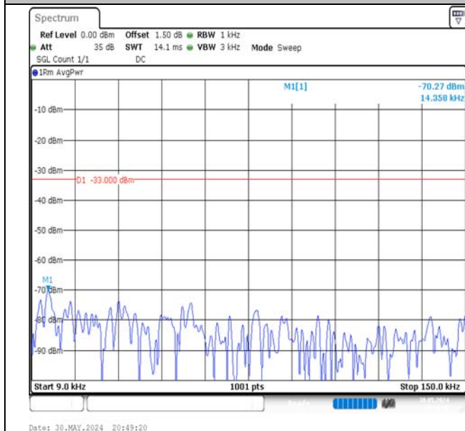
Band5-1.4MHz-16QAM-20525-1RB#5-0.009~0.15-PASS
