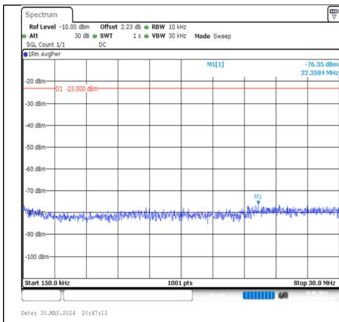
Band5-1.4MHz-16QAM-20407-1RB#5-0.15~30-PASS
