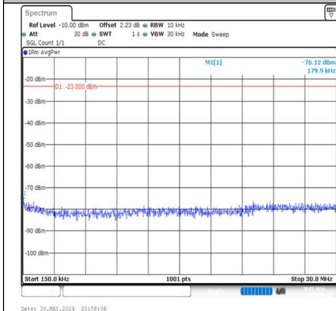
Band5-3MHz-QPSK-20635-15RB#0-0.15~30-PASS
