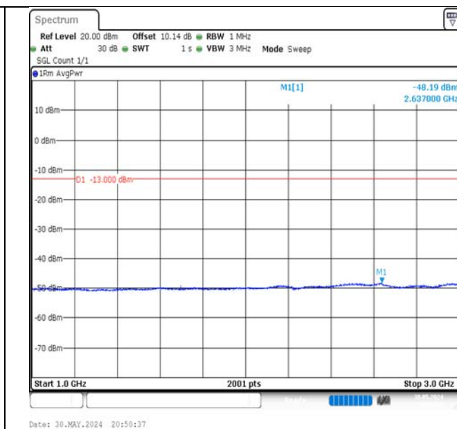
Band5-1.4MHz-QPSK-20643-1RB#0-1000~3000-PASS
