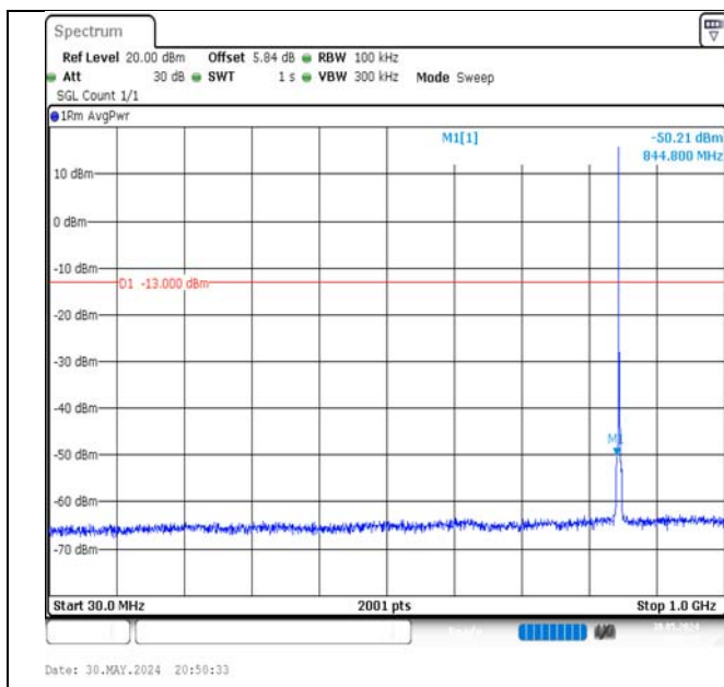
Band5-1.4MHz-QPSK-20643-1RB#0-30~1000-PASS
