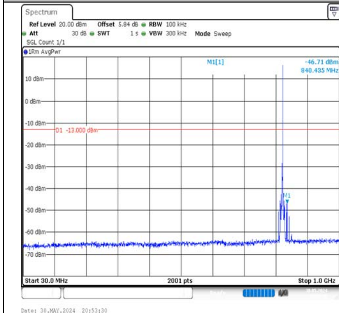
Band5-3MHz-QPSK-20415-1RB#14-30~1000-PASS
