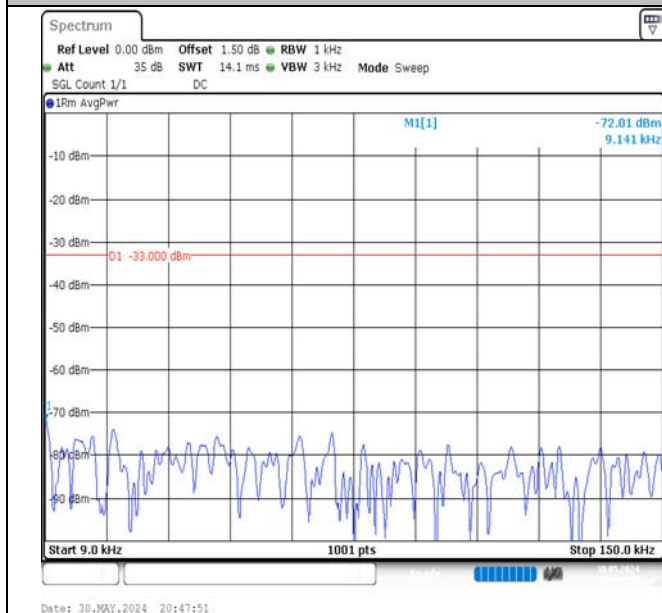
Band5-1.4MHz-16QAM-20407-6RB#0-0.009~0.15-PASS
