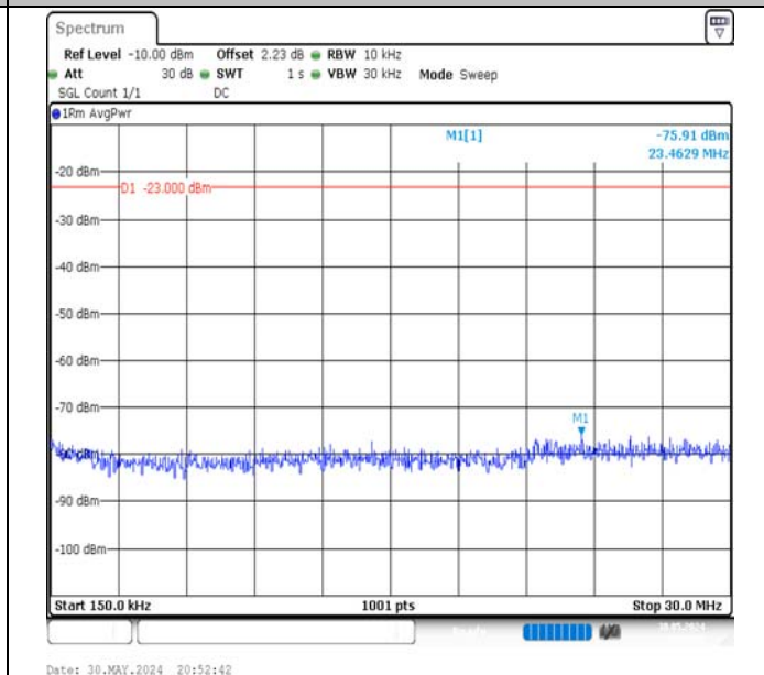
Band5-3MHz-QPSK-20415-1RB#0-0.15~30-PASS
