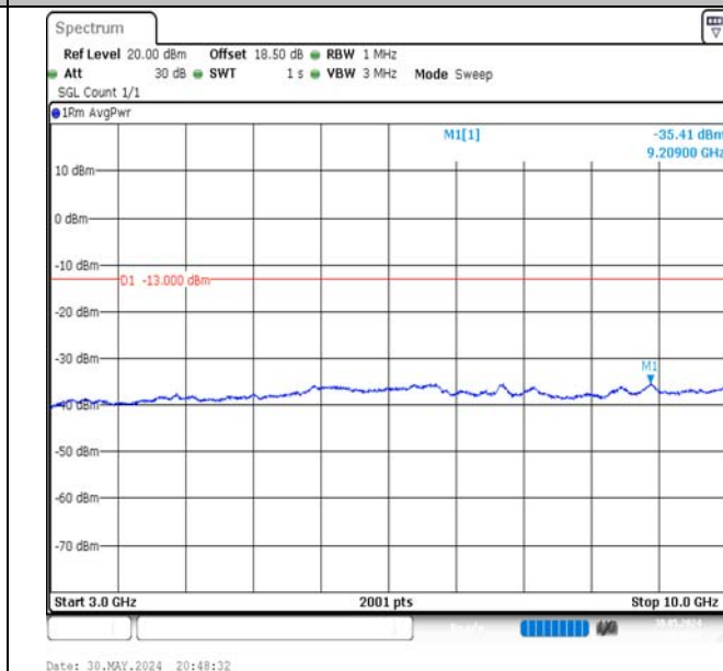
Band5-1.4MHz-QPSK-20525-1RB#0-3000~10000-PASS
