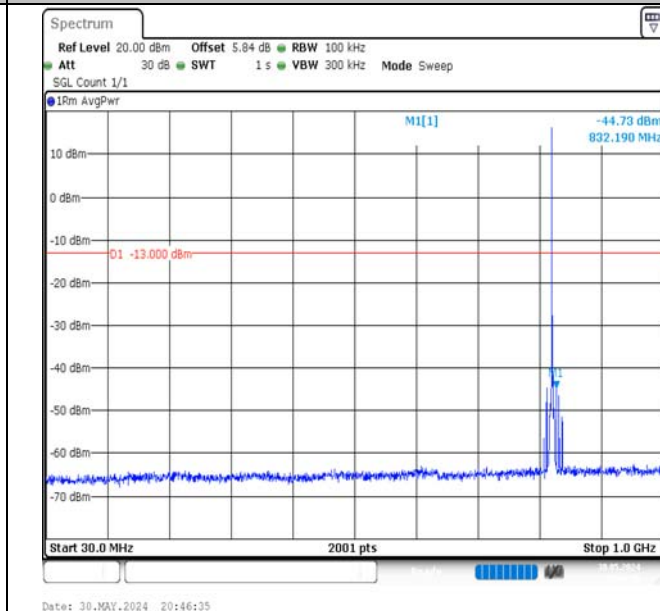
Band5-1.4MHz-16QAM-20407-1RB#0-30~1000-PASS
