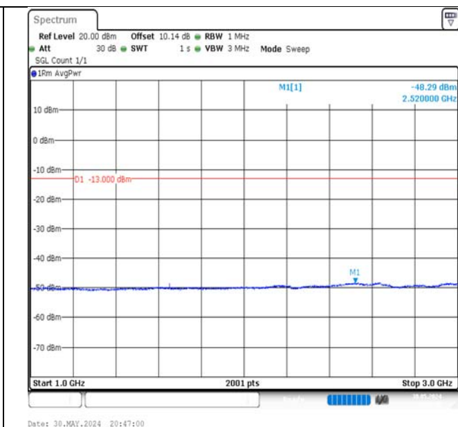
Band5-1.4MHz-QPSK-20407-1RB#5-1000~3000-PASS
