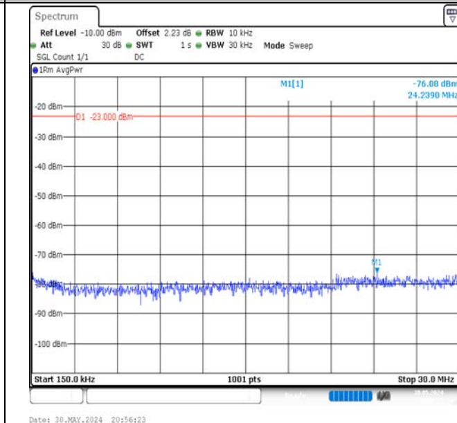
Band5-3MHz-QPSK-20525-15RB#0-0.15~30-PASS
