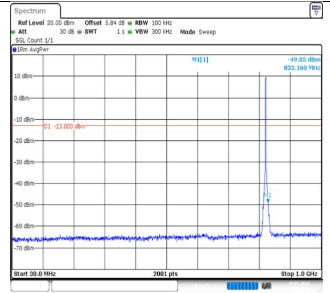
Band5-3MHz-QPSK-20415-15RB#0-30~1000-PASS
