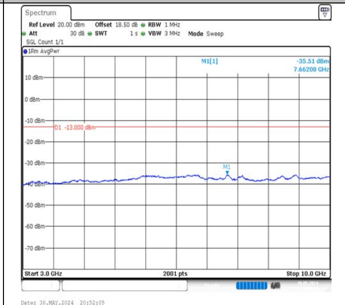
Band5-1.4MHz-QPSK-20643-6RB#0-3000~10000-PASS
