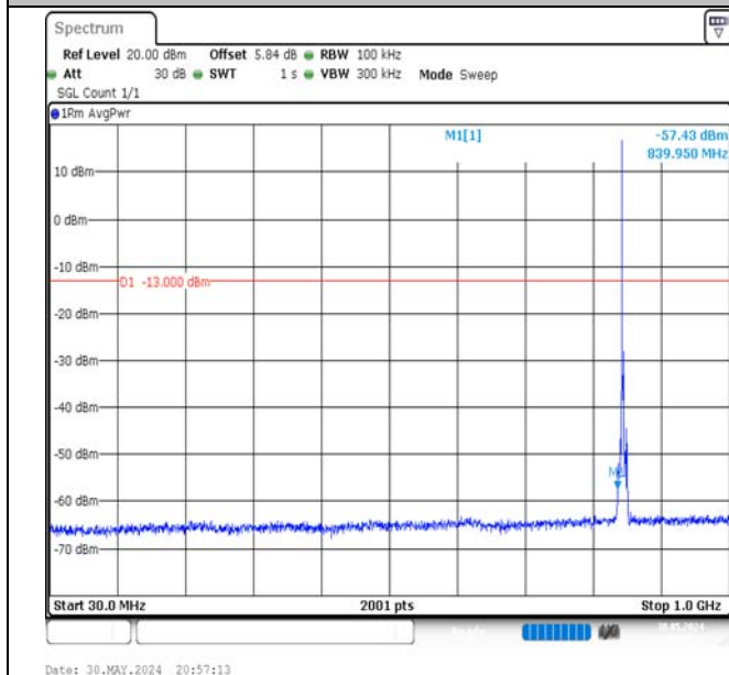
Band5-3MHz-QPSK-20635-1RB#0-30~1000-PASS
