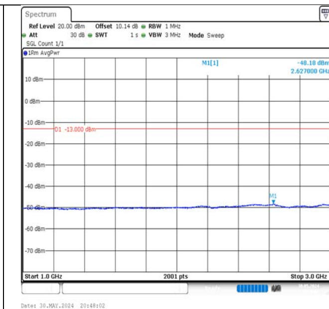
Band5-1.4MHz-16QAM-20407-6RB#0-1000~3000-PASS
