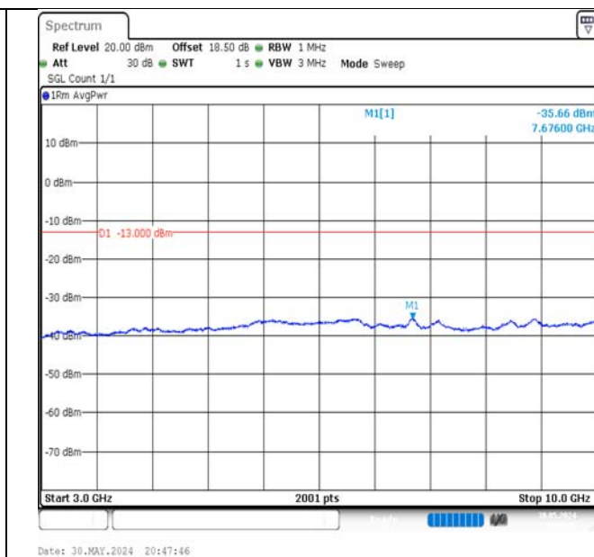
Band5-1.4MHz-QPSK-20407-6RB#0-3000~10000-PASS
