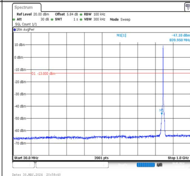
Band5-3MHz-QPSK-20635-15RB#0-30~1000-PASS
