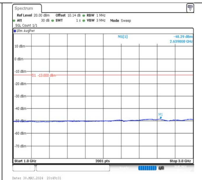
Band5-1.4MHz-16QAM-20525-1RB#5-1000~3000-PASS
