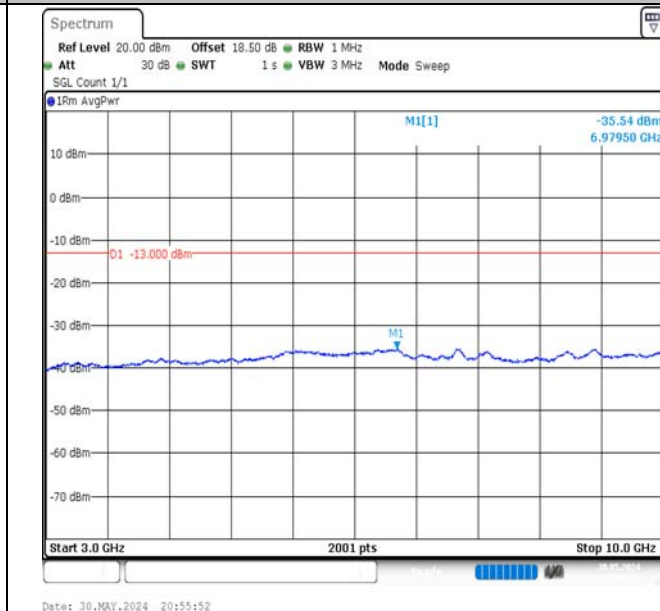
Band5-3MHz-QPSK-20525-1RB#14-3000~10000-PASS
