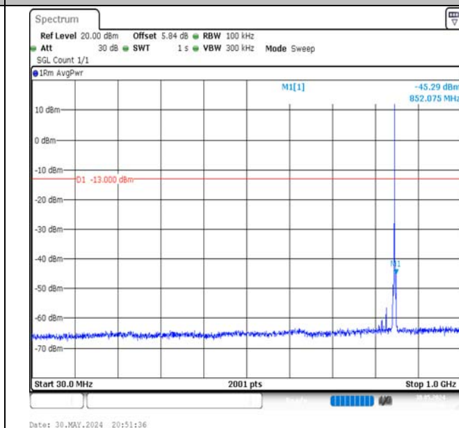
Band5-1.4MHz-16QAM-20643-1RB#5-30~1000-PASS
