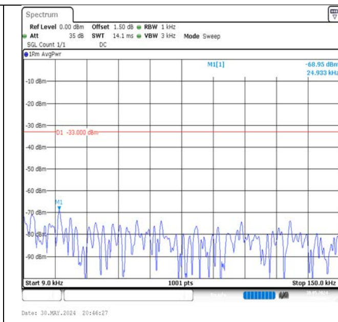
Band5-1.4MHz-16QAM-20407-1RB#0-0.009~0.15-PASS
