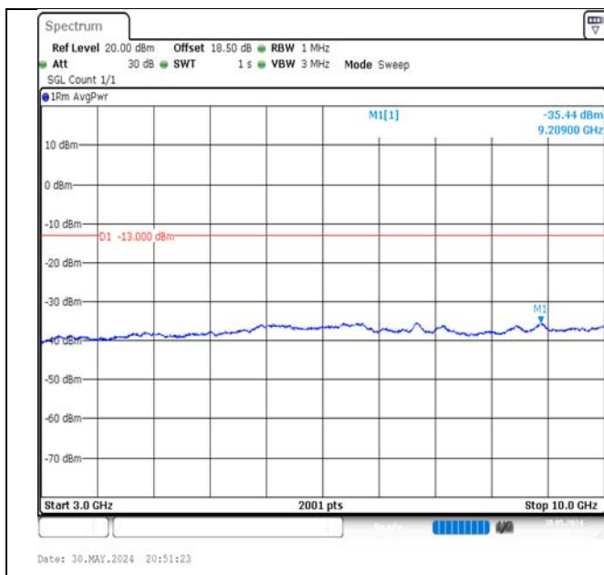
Band5-1.4MHz-QPSK-20643-1RB#5-3000~10000-PASS
