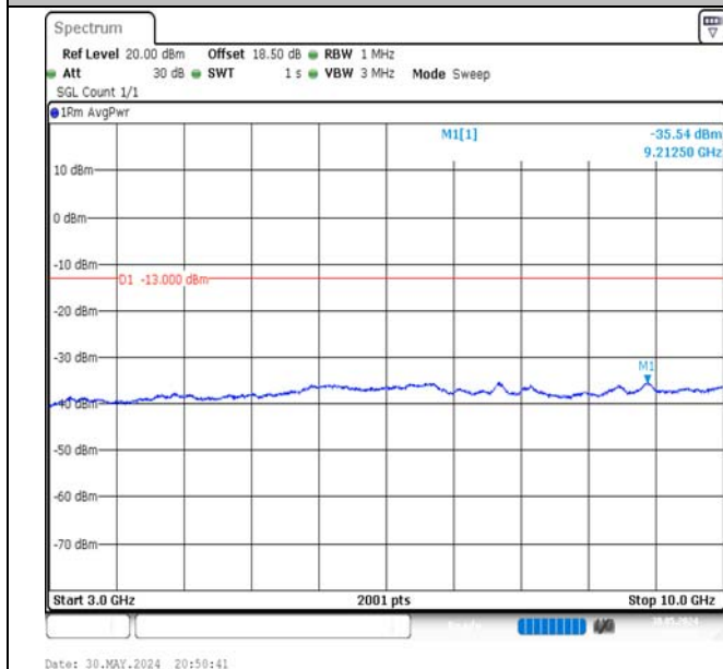
Band5-1.4MHz-QPSK-20643-1RB#0-3000~10000-PASS
