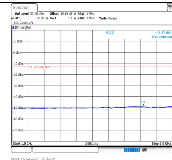
Band5-3MHz-QPSK-20415-1RB#0-1000~3000-PASS
