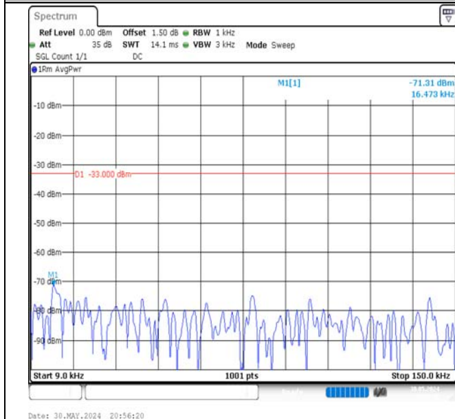
Band5-3MHz-QPSK-20525-15RB#0-0.009~0.15-PASS
