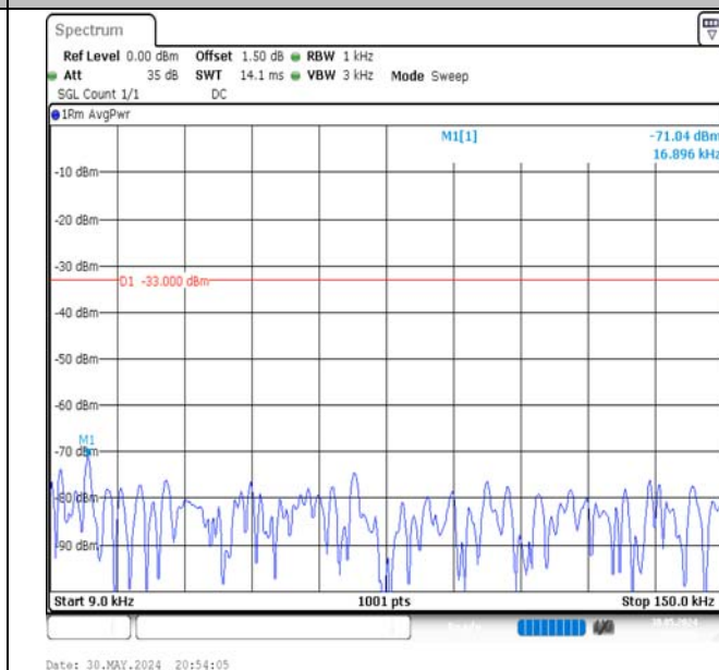
Band5-3MHz-QPSK-20415-15RB#0-0.009~0.15-PASS
