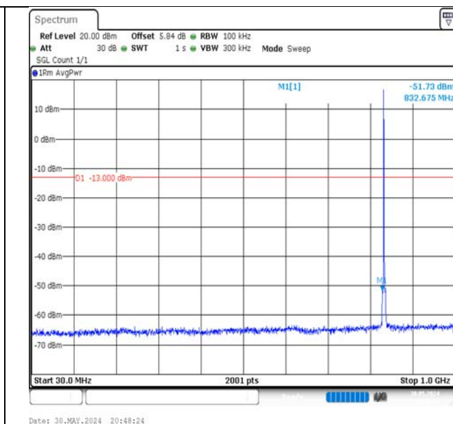
Band5-1.4MHz-QPSK-20525-1RB#0-30~1000-PASS
