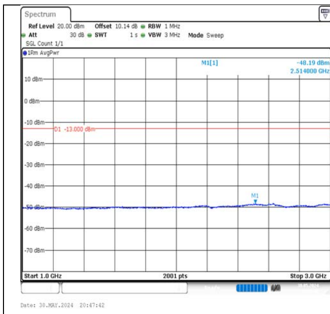
Band5-1.4MHz-QPSK-20407-6RB#0-1000~3000-PASS
