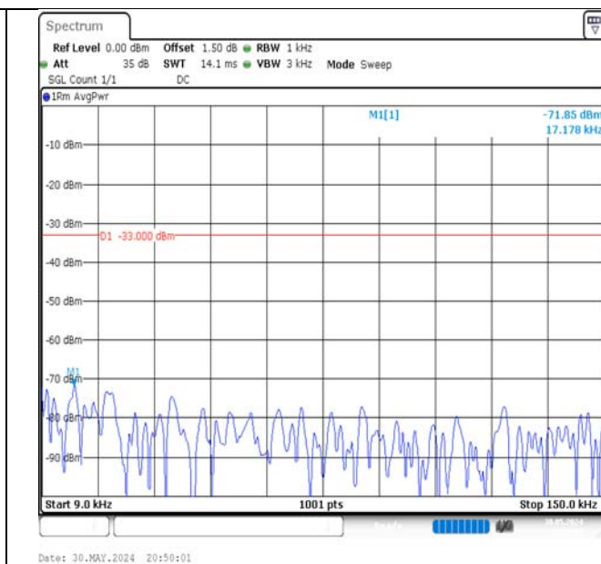
Band5-1.4MHz-16QAM-20525-6RB#0-0.009~0.15-PASS
