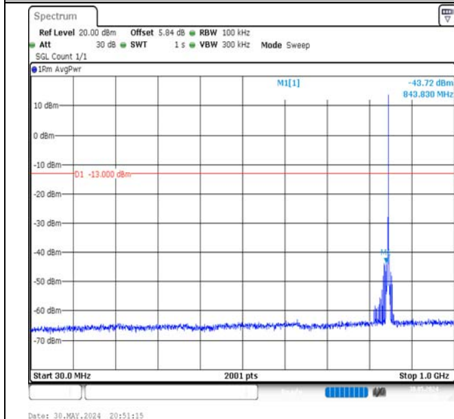
Band5-1.4MHz-QPSK-20643-1RB#5-30~1000-PASS
