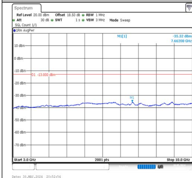
Band5-3MHz-QPSK-20415-1RB#0-3000~10000-PASS
