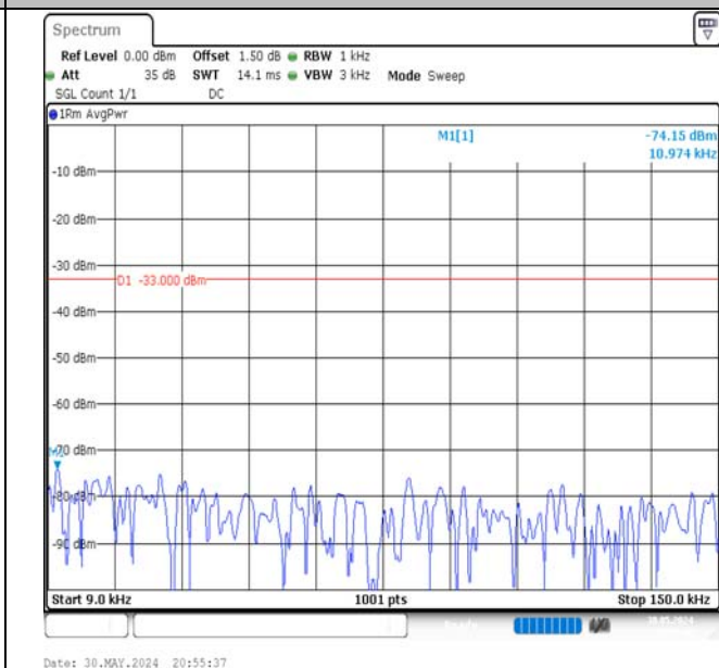
Band5-3MHz-QPSK-20525-1RB#14-0.009~0.15-PASS
