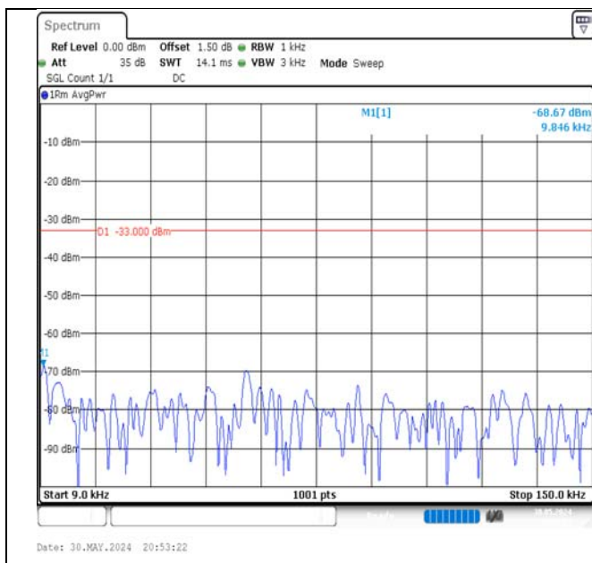
Band5-3MHz-QPSK-20415-1RB#14-0.009~0.15-PASS
