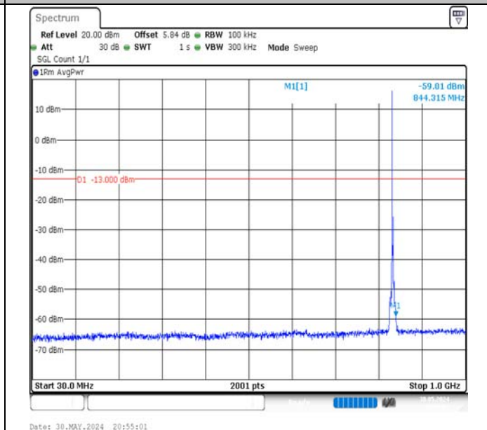
Band5-3MHz-QPSK-20525-1RB#0-30~1000-PASS
