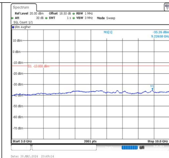
Band5-1.4MHz-QPSK-20525-1RB#5-3000~10000-PASS
