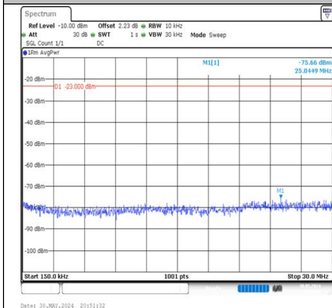
Band5-1.4MHz-16QAM-20643-1RB#5-0.15~30-PASS
