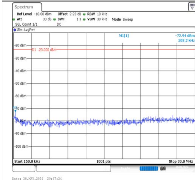
Band5-1.4MHz-QPSK-20407-6RB#0-0.15~30-PASS
