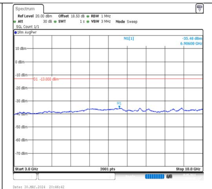
Band5-1.4MHz-16QAM-20407-1RB#0-3000~10000-PASS
