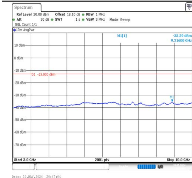
Band5-1.4MHz-QPSK-20407-1RB#5-3000~10000-PASS
