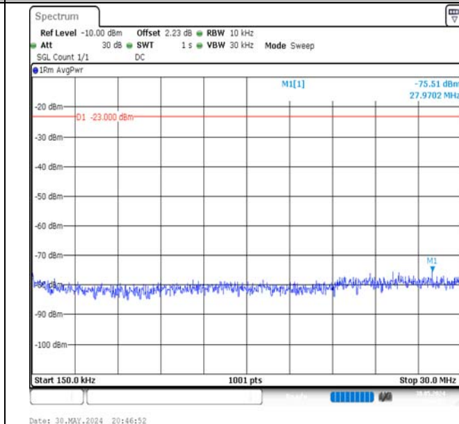
Band5-1.4MHz-QPSK-20407-1RB#5-0.15~30-PASS
