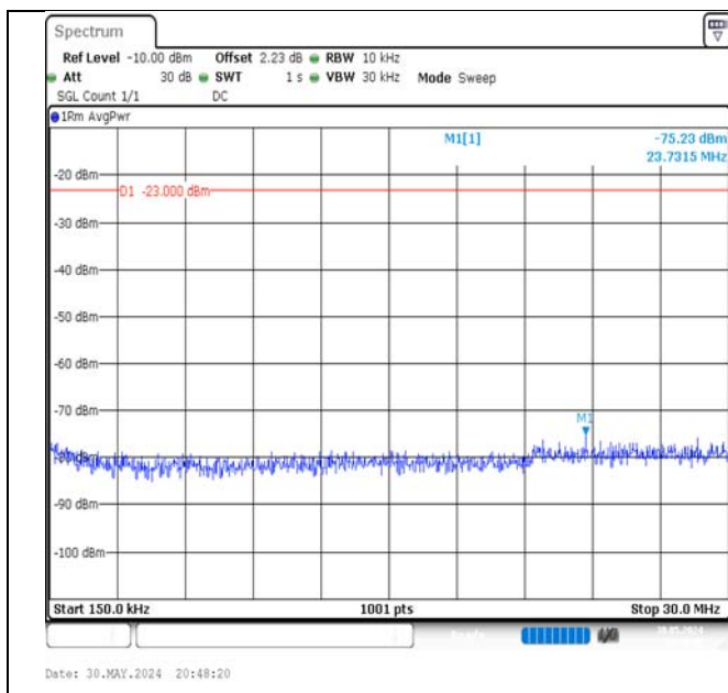
Band5-1.4MHz-QPSK-20525-1RB#0-0.15~30-PASS
