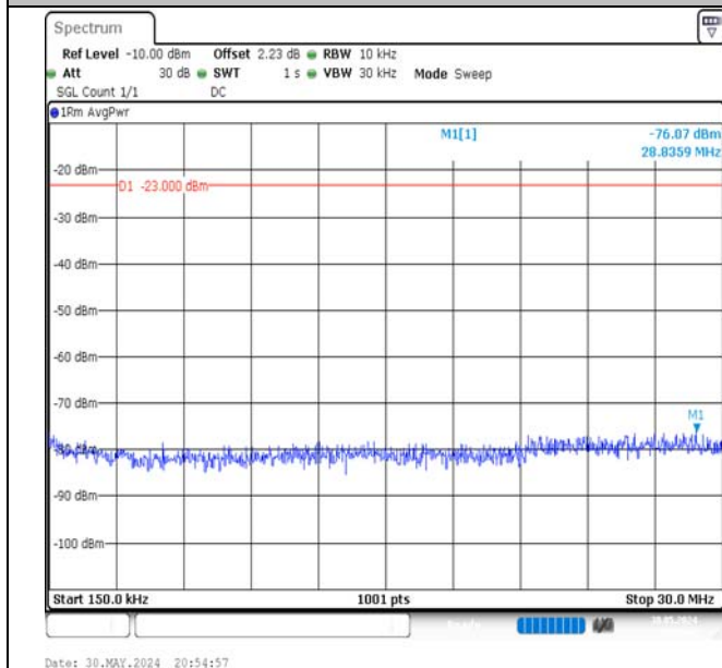
Band5-3MHz-QPSK-20525-1RB#0-0.15~30-PASS
