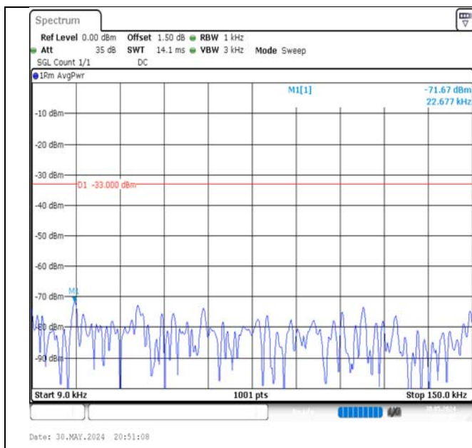
Band5-1.4MHz-QPSK-20643-1RB#5-0.009~0.15-PASS
