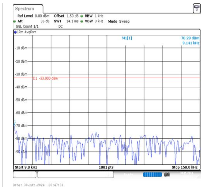
Band5-1.4MHz-QPSK-20407-6RB#0-0.009~0.15-PASS
