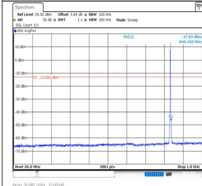
Band5-1.4MHz-QPSK-20525-6RB#0-30~1000-PASS
