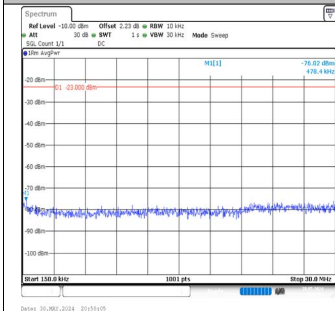
Band5-1.4MHz-16QAM-20525-6RB#0-0.15~30-PASS
