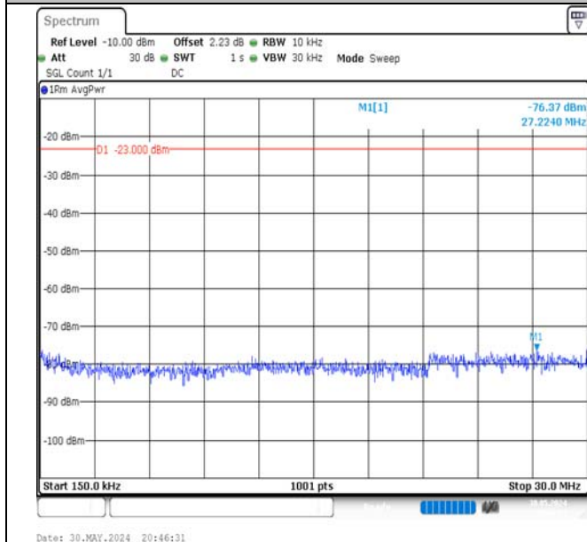
Band5-1.4MHz-16QAM-20407-1RB#0-0.15~30-PASS
