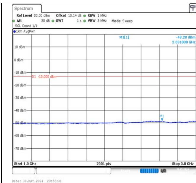
Band5-3MHz-QPSK-20525-15RB#0-1000~3000-PASS
