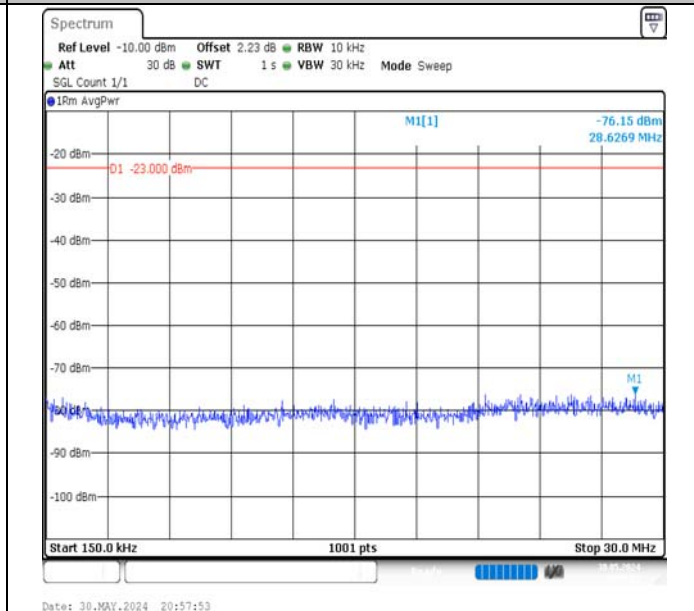
Band5-3MHz-QPSK-20635-1RB#14-0.15~30-PASS
