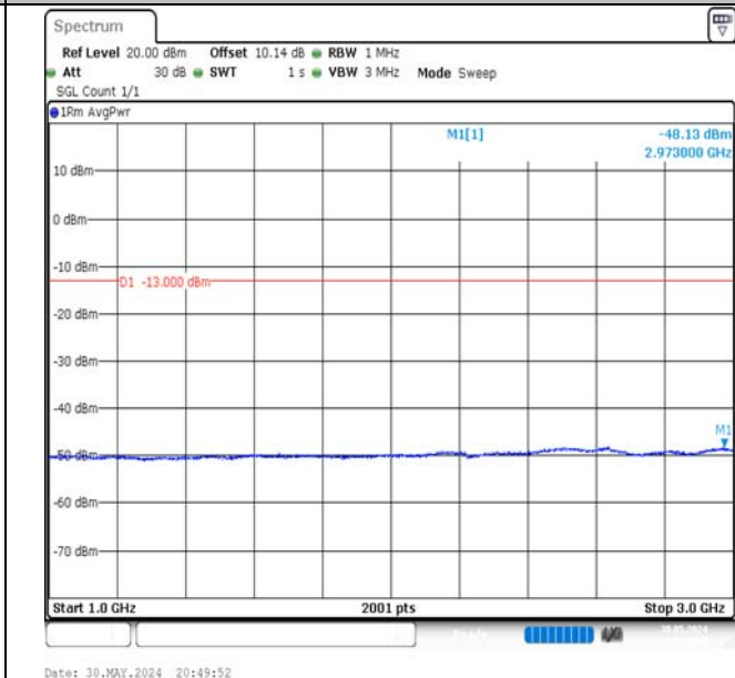
Band5-1.4MHz-QPSK-20525-6RB#0-1000~3000-PASS
