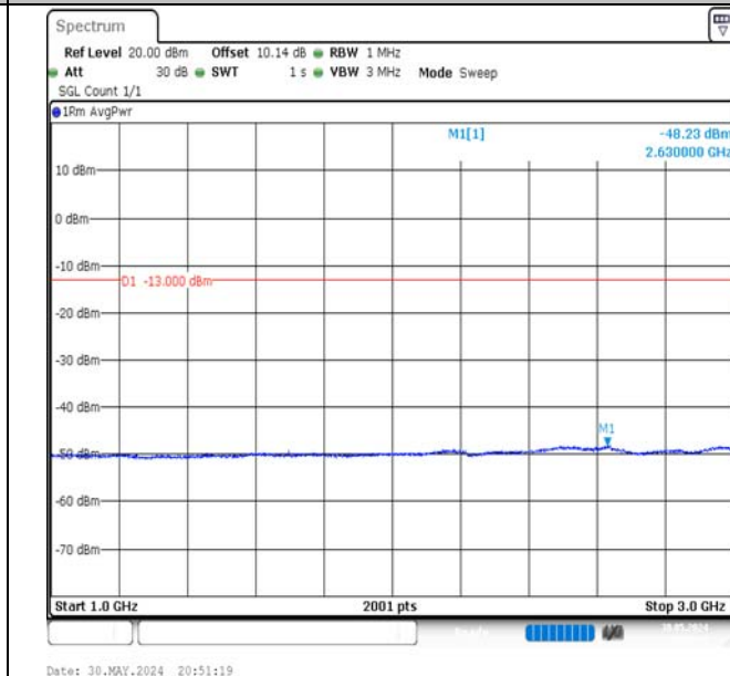
Band5-1.4MHz-QPSK-20643-1RB#5-1000~3000-PASS
