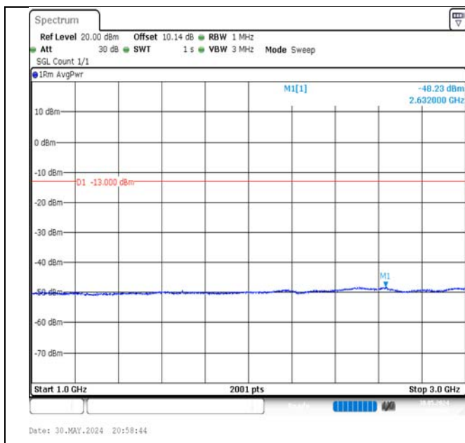
Band5-3MHz-QPSK-20635-15RB#0-1000~3000-PASS
