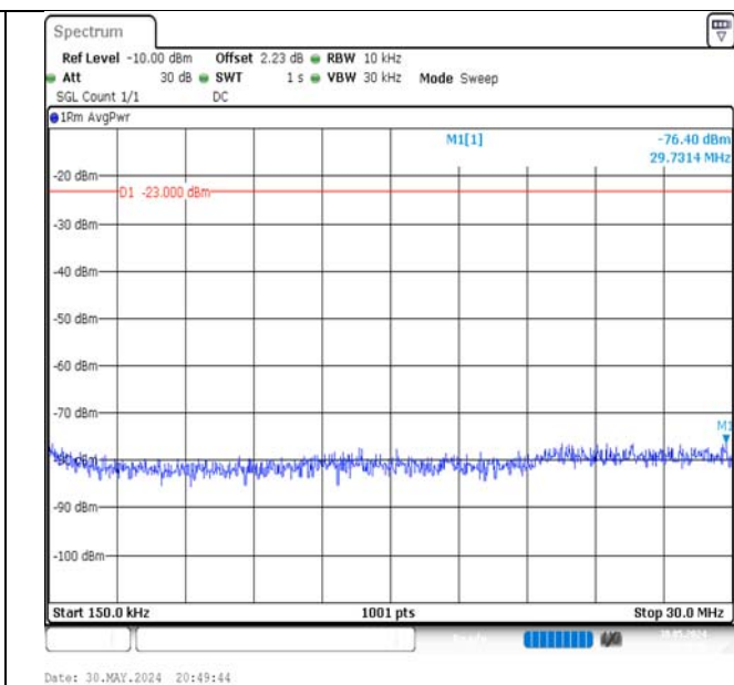
Band5-1.4MHz-QPSK-20525-6RB#0-0.15~30-PASS
