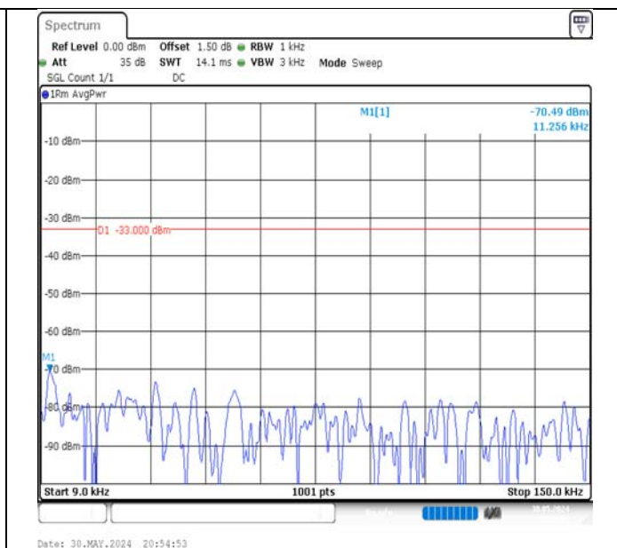
Band5-3MHz-QPSK-20525-1RB#0-0.009~0.15-PASS
