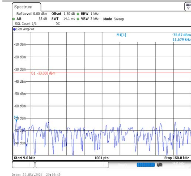
Band5-1.4MHz-QPSK-20407-1RB#5-0.009~0.15-PASS
