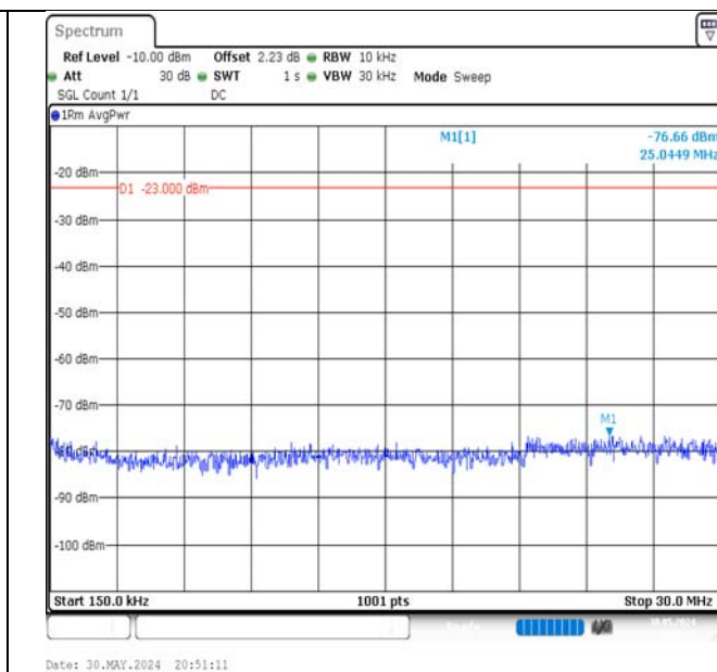
Band5-1.4MHz-QPSK-20643-1RB#5-0.15~30-PASS
