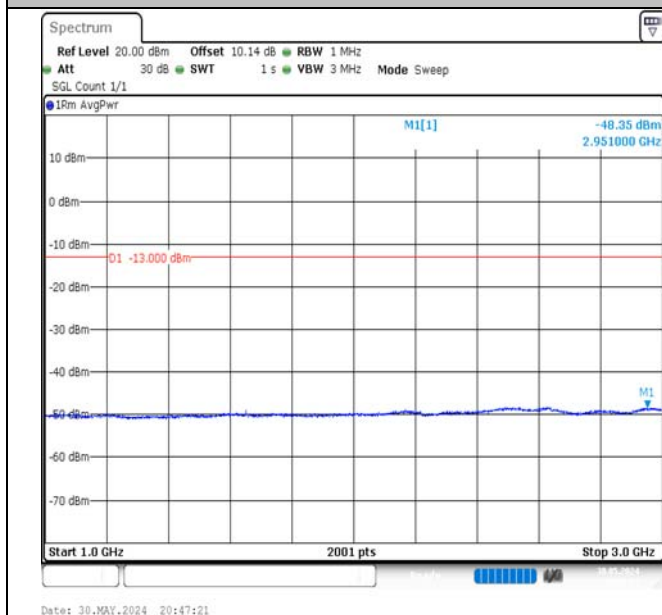
Band5-1.4MHz-16QAM-20407-1RB#5-1000~3000-PASS
