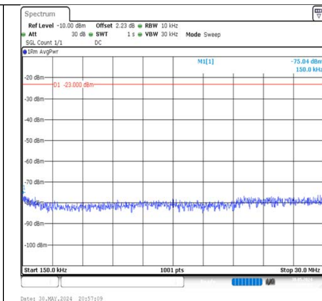
Band5-3MHz-QPSK-20635-1RB#0-0.15~30-PASS
