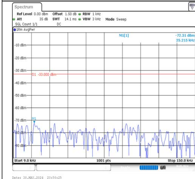
Band5-1.4MHz-QPSK-20643-1RB#0-0.009~0.15-PASS
