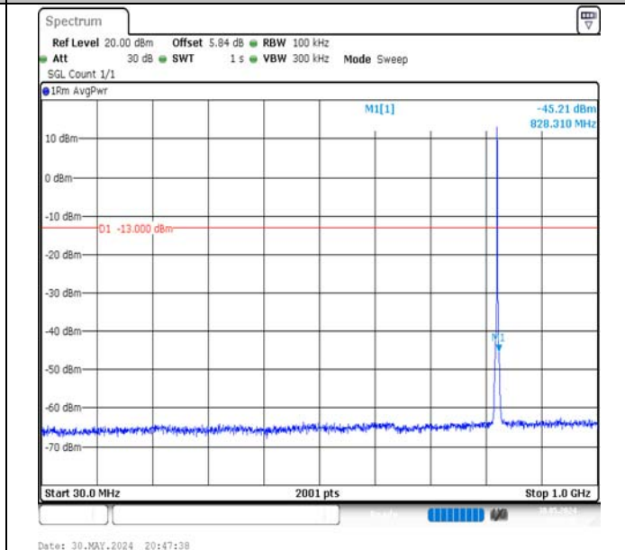
Band5-1.4MHz-QPSK-20407-6RB#0-30~1000-PASS
