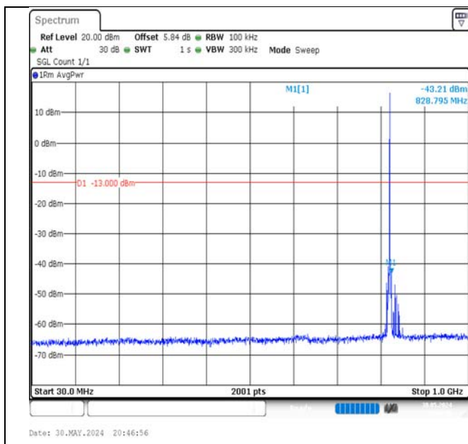
Band5-1.4MHz-QPSK-20407-1RB#5-30~1000-PASS
