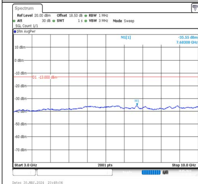
Band5-1.4MHz-16QAM-20407-6RB#0-3000~10000-PASS
