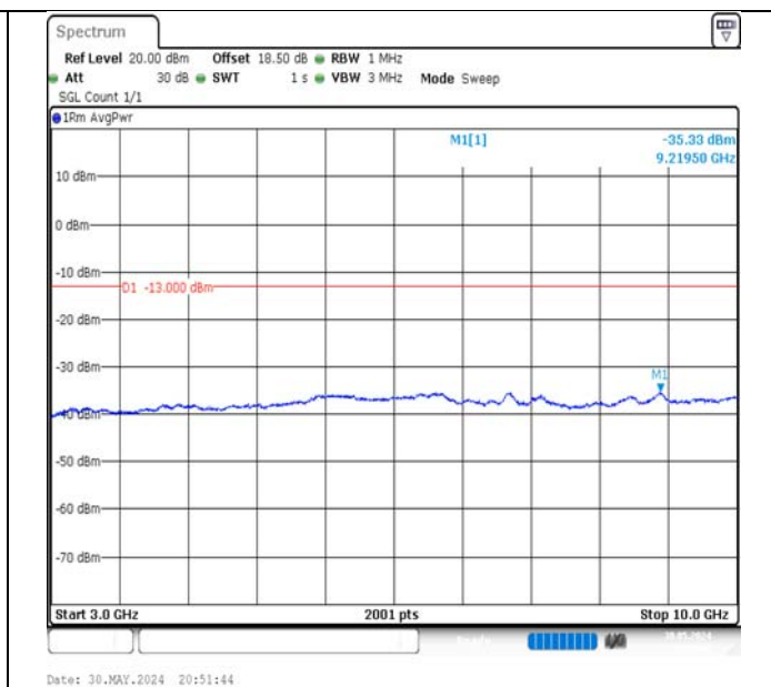
Band5-1.4MHz-16QAM-20643-1RB#5-3000~10000-PASS
