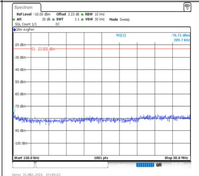
Band5-1.4MHz-16QAM-20525-1RB#5-0.15~30-PASS
