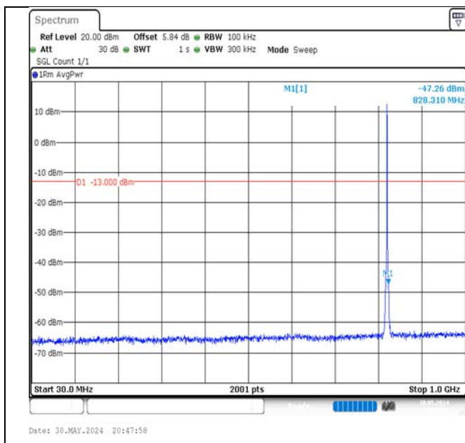
Band5-1.4MHz-16QAM-20407-6RB#0-30~1000-PASS
