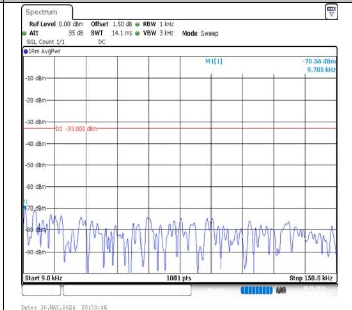
Band5-1.4MHz-16QAM-20643-1RB#0-0.009~0.15-PASS
