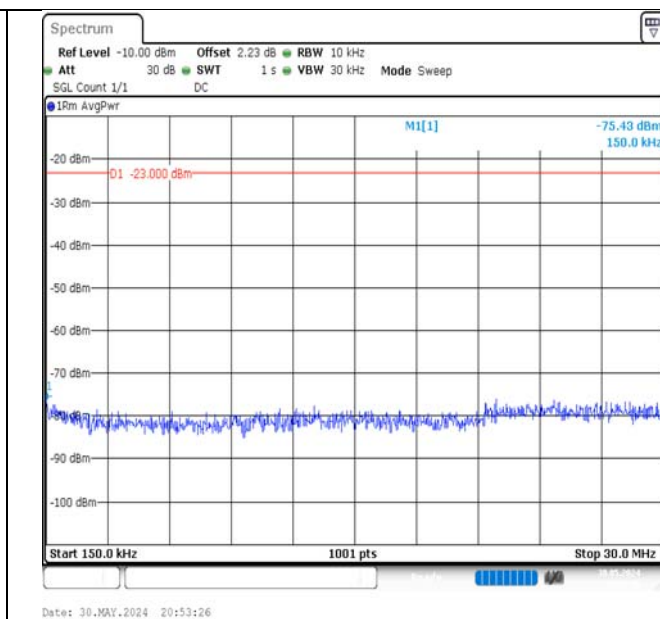
Band5-3MHz-QPSK-20415-1RB#14-0.15~30-PASS
