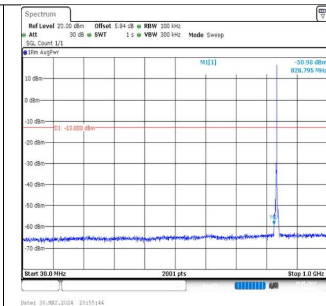
Band5-3MHz-QPSK-20525-1RB#14-30~1000-PASS
