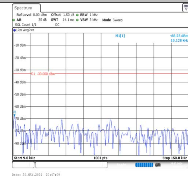
Band5-1.4MHz-16QAM-20407-1RB#5-0.009~0.15-PASS
