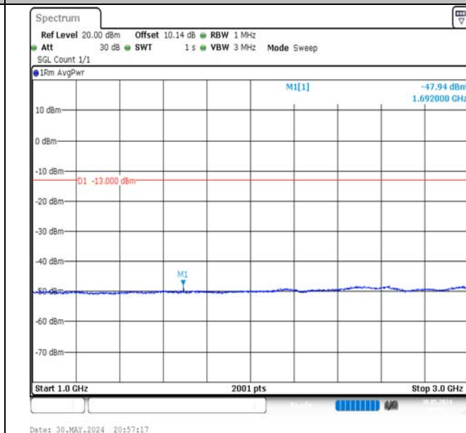
Band5-3MHz-QPSK-20635-1RB#0-1000~3000-PASS
