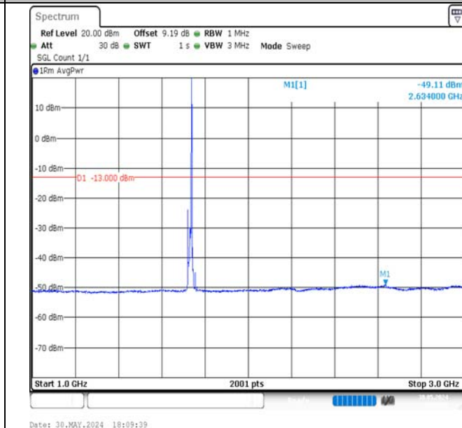
Band4-10MHz-16QAM-20175-1RB#49-1000~3000-PASS
