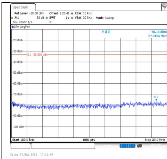
Band4-15MHz-QPSK-20175-1RB#0-0.15~30-PASS
