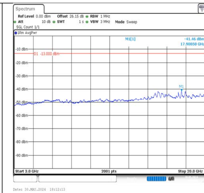
Band4-10MHz-QPSK-20350-50RB#0-3000~20000-PASS
