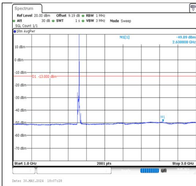
Band4-10MHz-16QAM-20000-1RB#49-1000~3000-PASS
