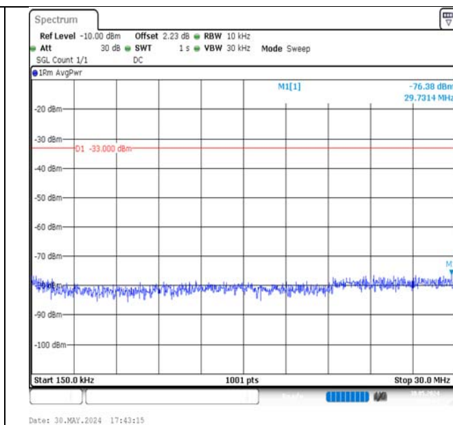
Band4-15MHz-QPSK-20175-75RB#0-0.15~30-PASS
