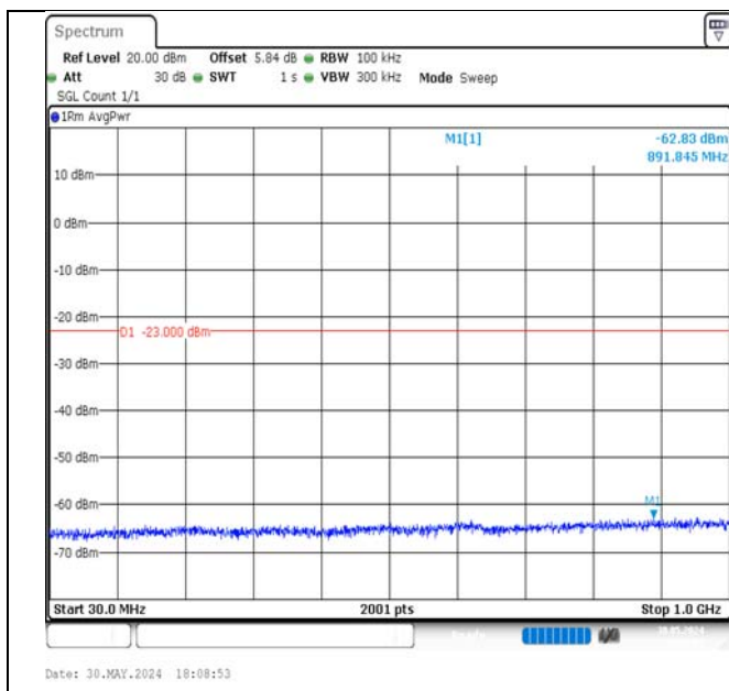
Band4-10MHz-16QAM-20175-1RB#0-30~1000-PASS
