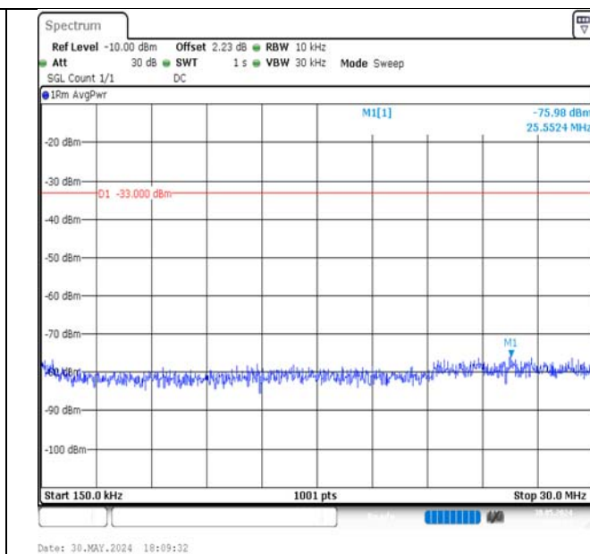
Band4-10MHz-16QAM-20175-1RB#49-0.15~30-PASS
