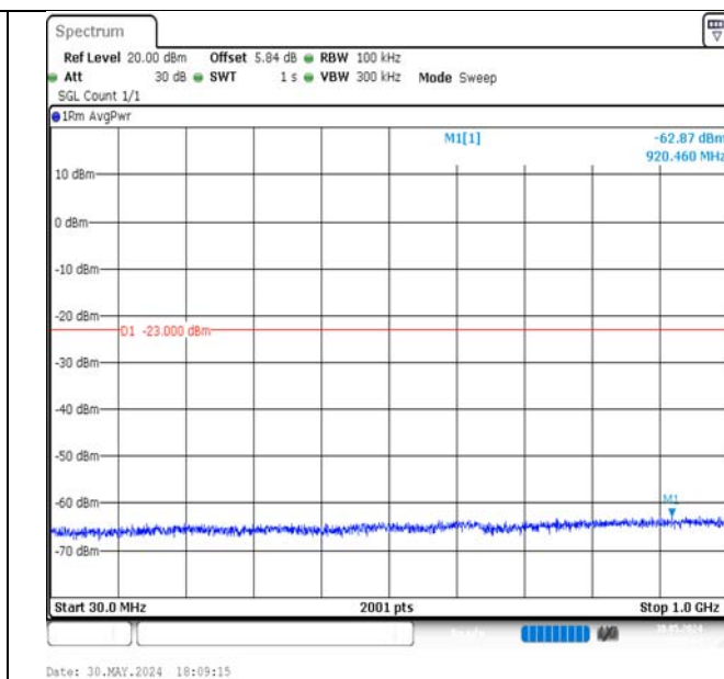
Band4-10MHz-QPSK-20175-1RB#49-30~1000-PASS
