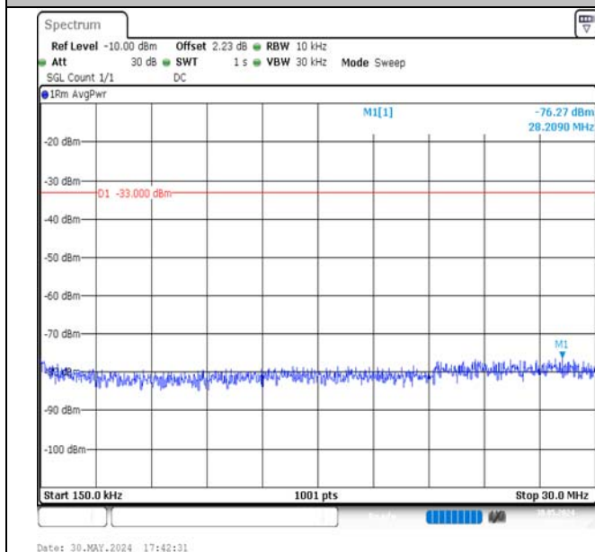
Band4-15MHz-QPSK-20175-1RB#74-0.15~30-PASS
