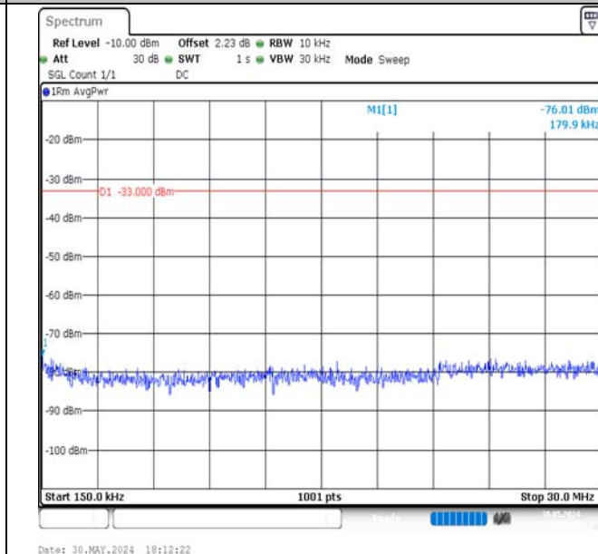
Band4-10MHz-16QAM-20350-50RB#0-0.15~30-PASS
