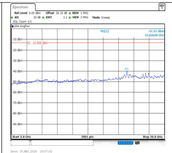
Band4-10MHz-16QAM-20000-1RB#49-3000~20000-PASS
