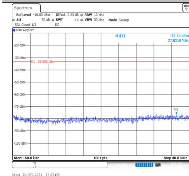
Band4-15MHz-16QAM-20025-1RB#0-0.15~30-PASS
