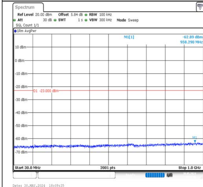
Band4-10MHz-16QAM-20175-1RB#49-30~1000-PASS
