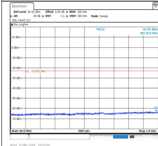
Band4-10MHz-QPSK-20350-1RB#0-30~1000-PASS
