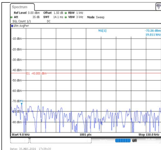
Band4-15MHz-QPSK-20025-1RB#0-0.009~0.15-PASS
