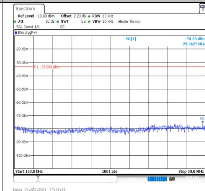
Band4-15MHz-16QAM-20025-75RB#0-0.15~30-PASS
