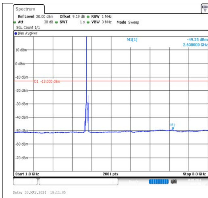
Band4-10MHz-16QAM-20350-1RB#0-1000~3000-PASS
