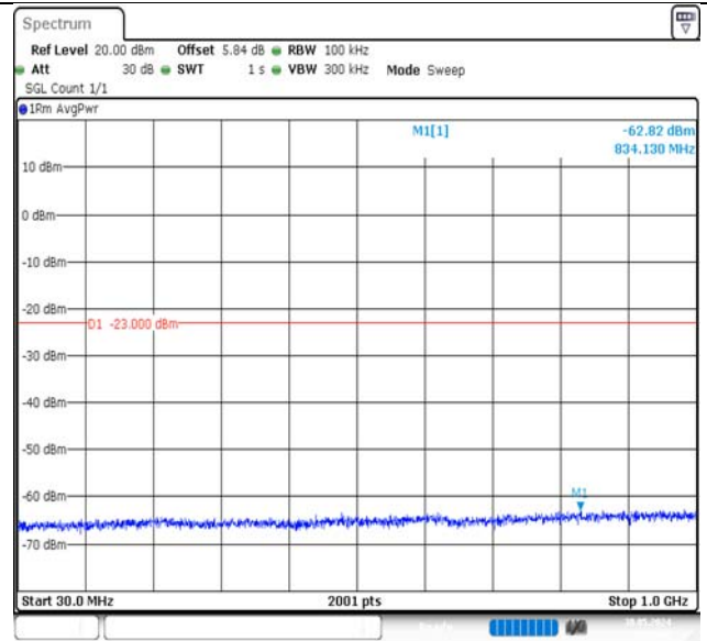
Band4-10MHz-16QAM-20350-1RB#49-30~1000-PASS
