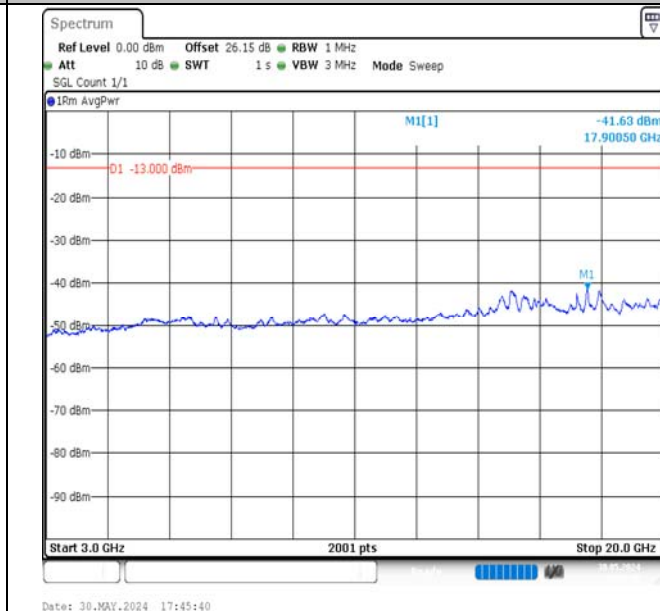
Band4-15MHz-QPSK-20325-75RB#0-3000~20000-PASS
