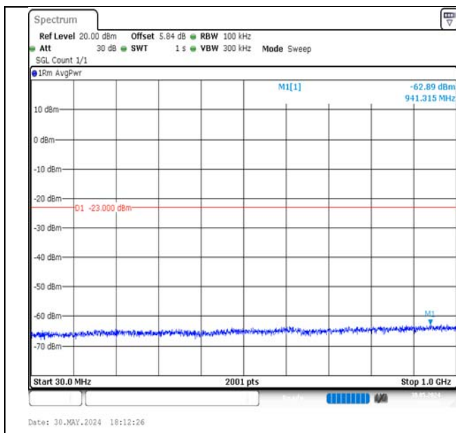
Band4-10MHz-16QAM-20350-50RB#0-30~1000-PASS
