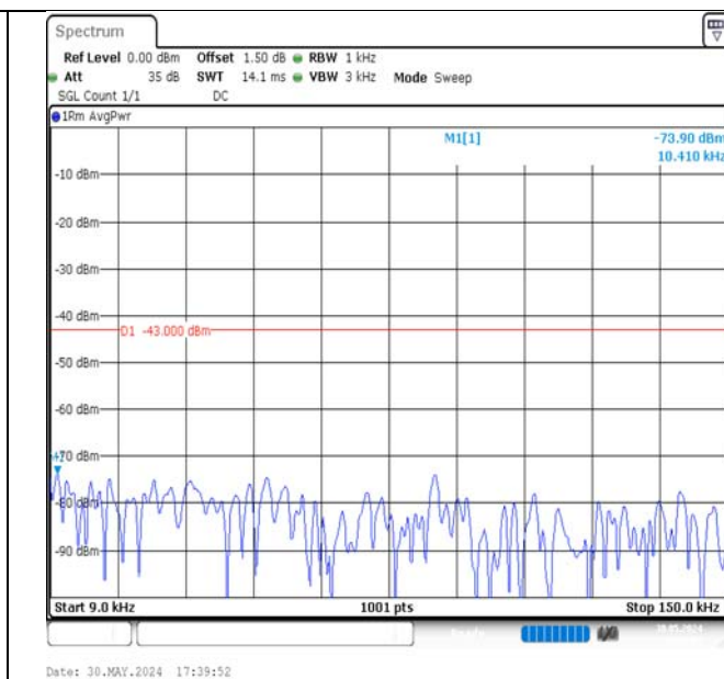
Band4-15MHz-16QAM-20025-1RB#0-0.009~0.15-PASS
