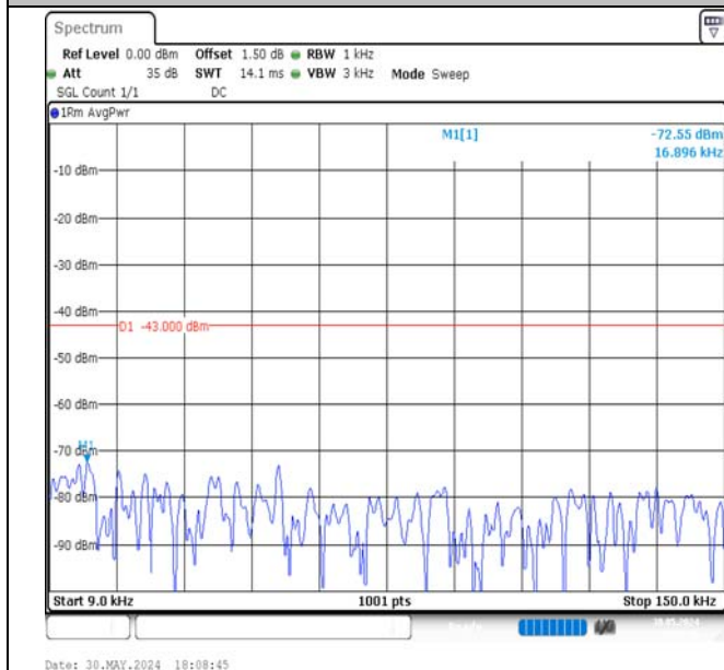
Band4-10MHz-16QAM-20175-1RB#0-0.009~0.15-PASS
