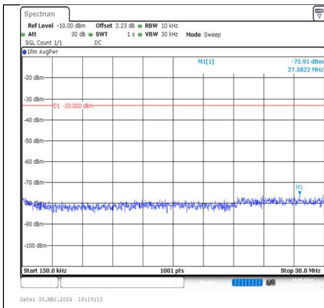
Band4-10MHz-16QAM-20175-50RB#0-0.15~30-PASS
