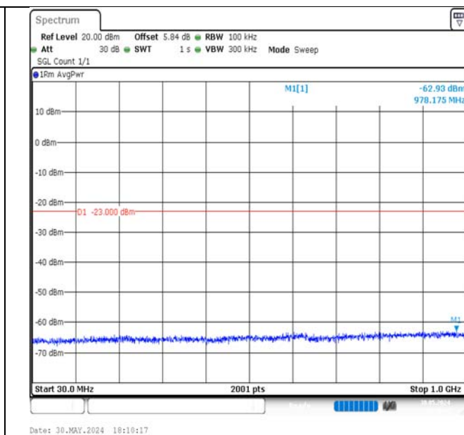
Band4-10MHz-16QAM-20175-50RB#0-30~1000-PASS
