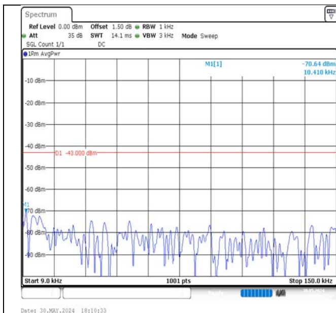
Band4-10MHz-QPSK-20350-1RB#0-0.009~0.15-PASS
