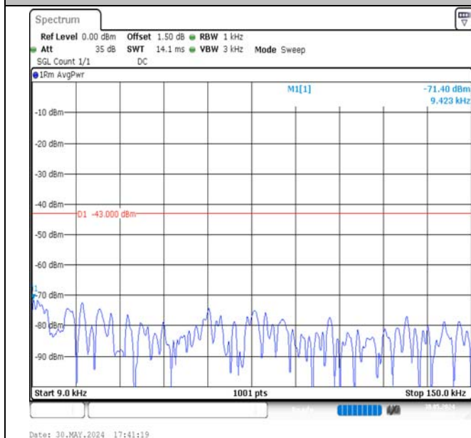
Band4-15MHz-16QAM-20025-75RB#0-0.009~0.15-PASS
