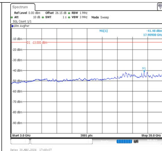
Band4-15MHz-16QAM-20025-1RB#0-3000~20000-PASS
