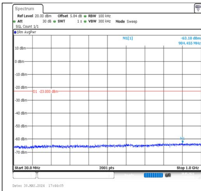
Band4-15MHz-QPSK-20325-1RB#0-30~1000-PASS
