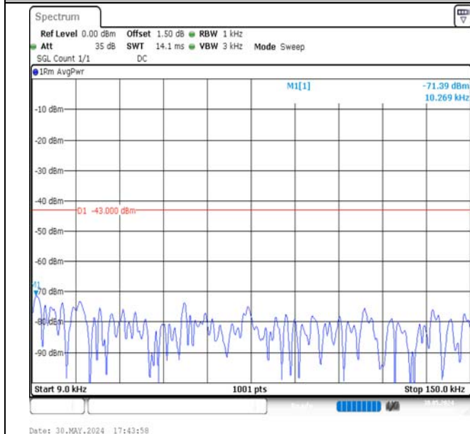
Band4-15MHz-QPSK-20325-1RB#0-0.009~0.15-PASS
