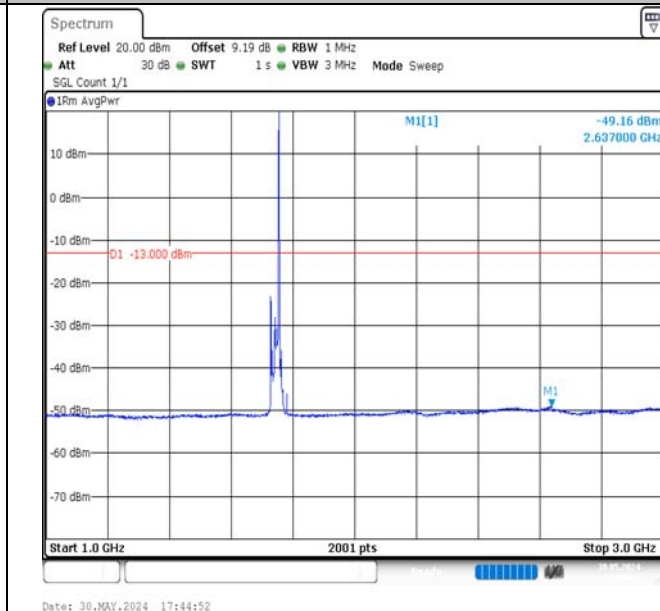
Band4-15MHz-QPSK-20325-1RB#74-1000~3000-PASS
