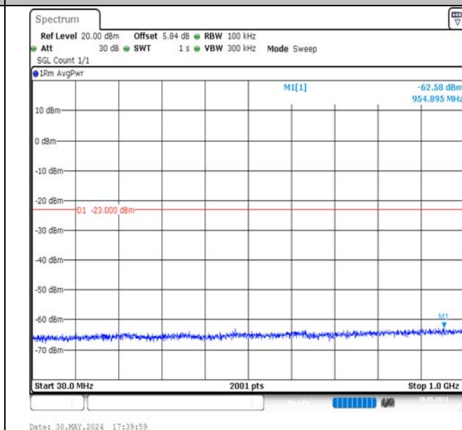
Band4-15MHz-16QAM-20025-1RB#0-30~1000-PASS
