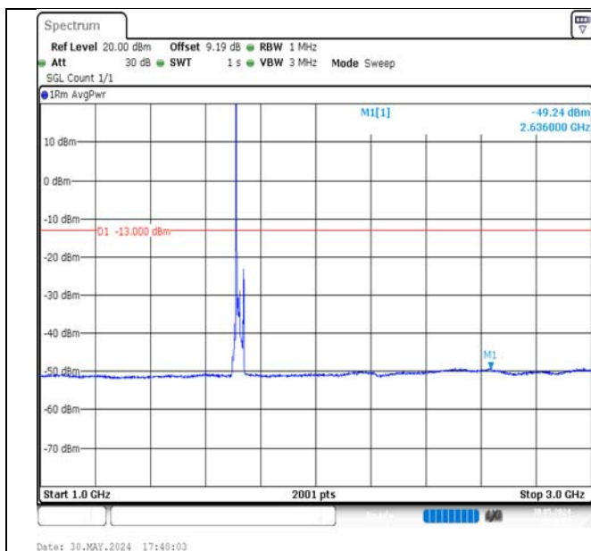
Band4-15MHz-16QAM-20025-1RB#0-1000~3000-PASS
