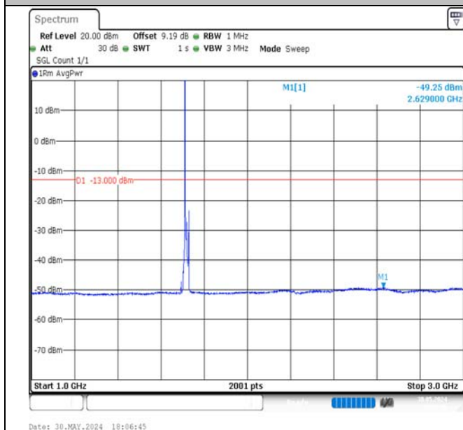
Band4-10MHz-16QAM-20000-1RB#0-1000~3000-PASS
