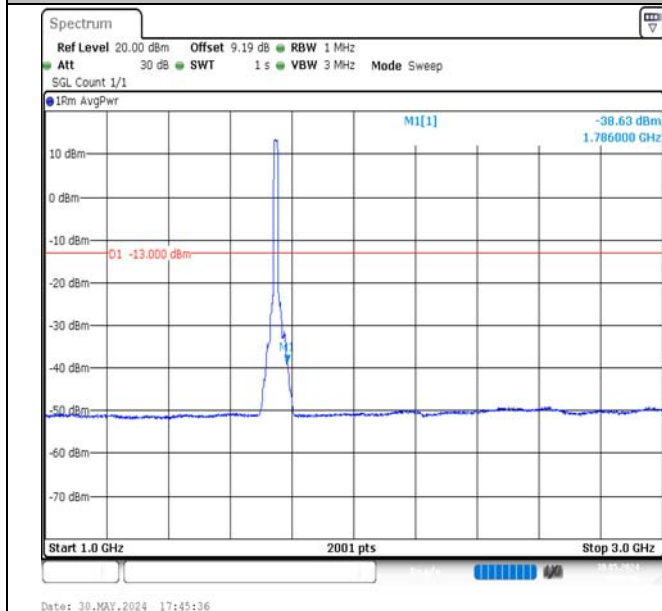
Band4-15MHz-QPSK-20325-75RB#0-1000~3000-PASS
