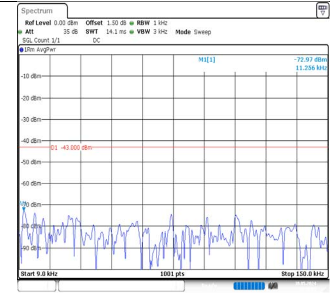
Band4-10MHz-16QAM-20350-1RB#0-0.009~0.15-PASS
