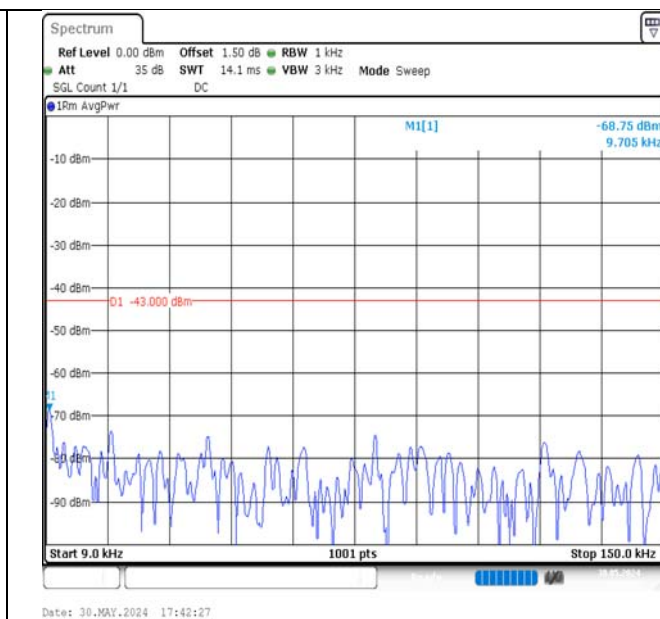
Band4-15MHz-QPSK-20175-1RB#74-0.009~0.15-PASS
