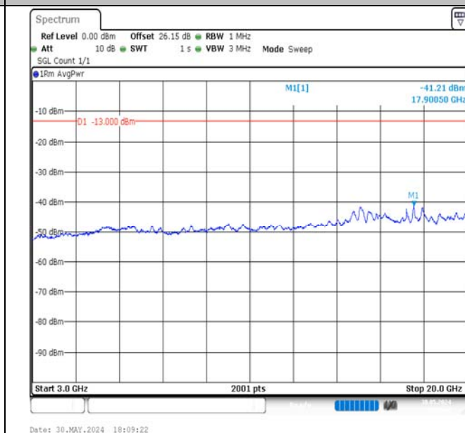
Band4-10MHz-QPSK-20175-1RB#49-3000~20000-PASS
