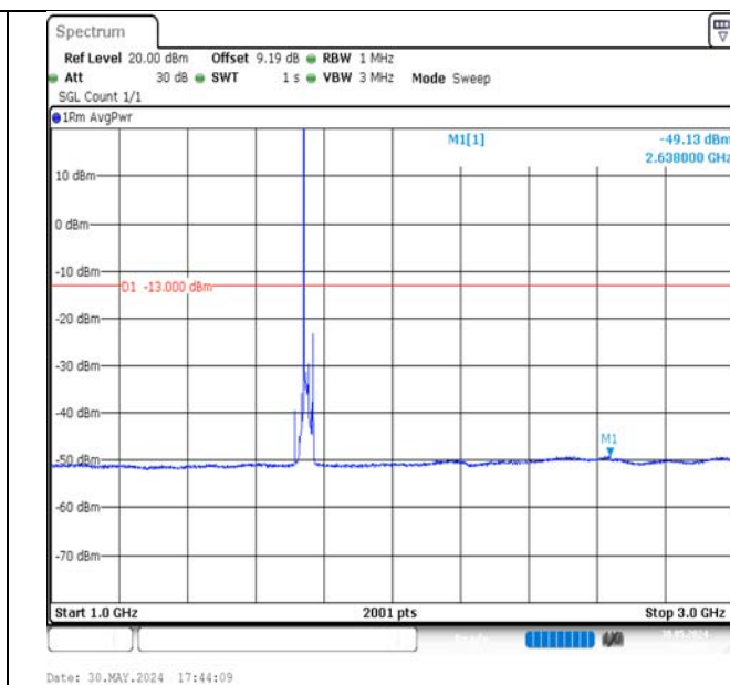
Band4-15MHz-QPSK-20325-1RB#0-1000~3000-PASS
