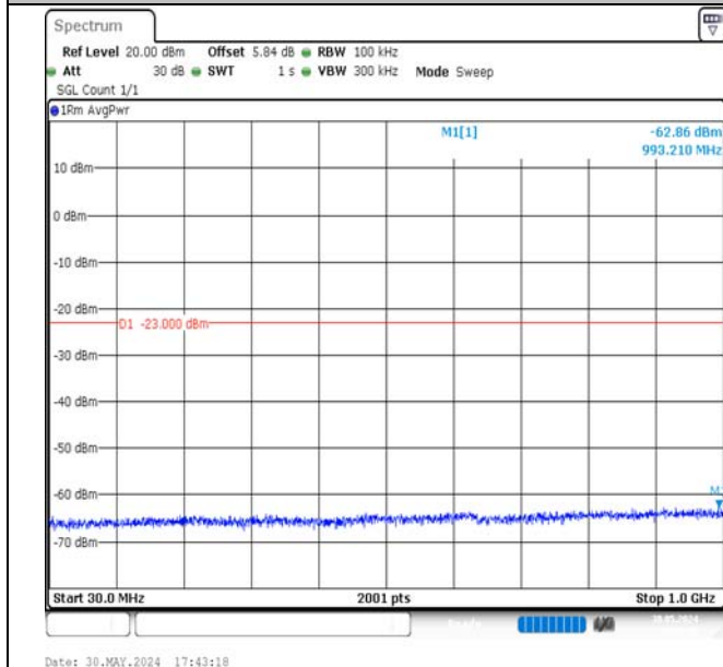
Band4-15MHz-QPSK-20175-75RB#0-30~1000-PASS
