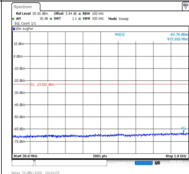
Band4-10MHz-QPSK-20350-50RB#0-30~1000-PASS
