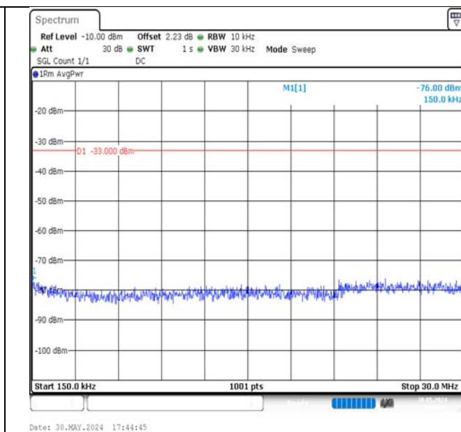
Band4-15MHz-QPSK-20325-1RB#74-0.15~30-PASS
