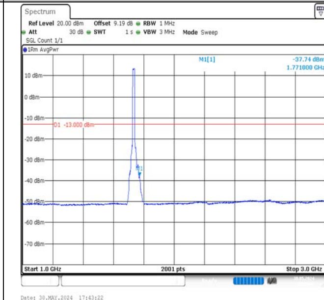
Band4-15MHz-QPSK-20175-75RB#0-1000~3000-PASS
