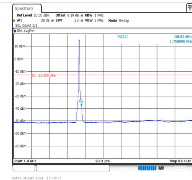
Band4-10MHz-QPSK-20175-50RB#0-1000~3000-PASS
