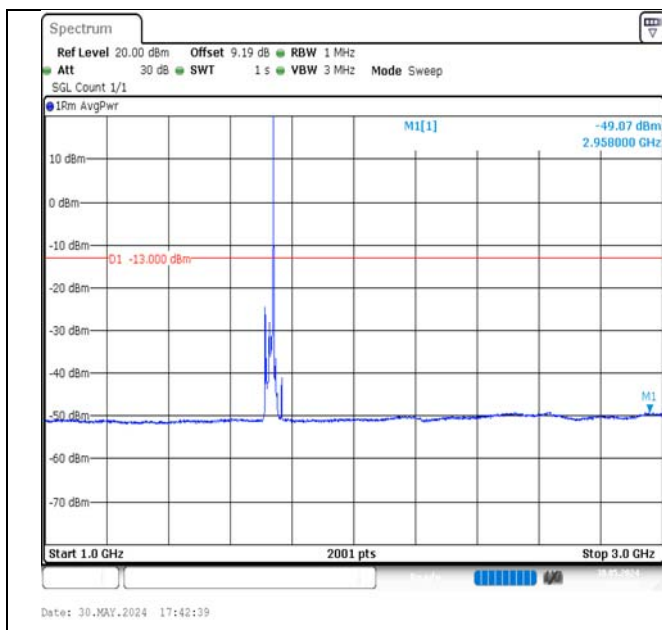
Band4-15MHz-QPSK-20175-1RB#74-1000~3000-PASS
