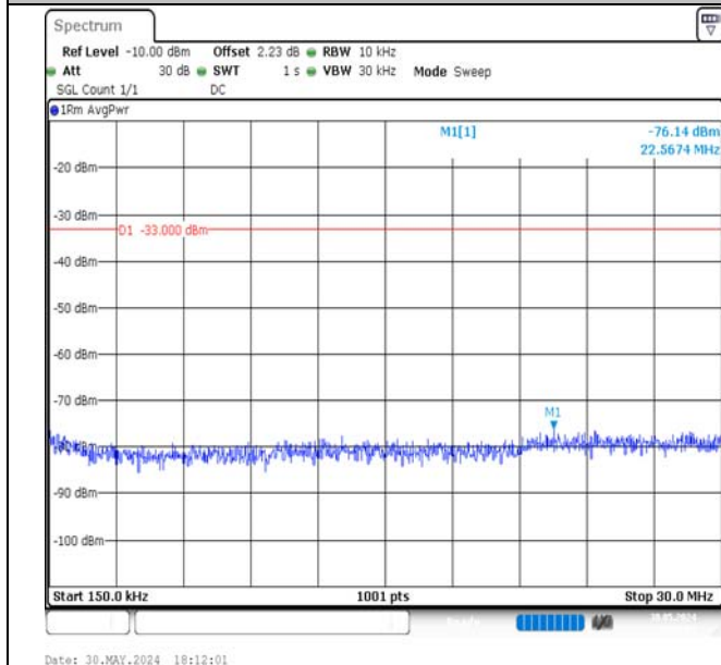
Band4-10MHz-QPSK-20350-50RB#0-0.15~30-PASS
