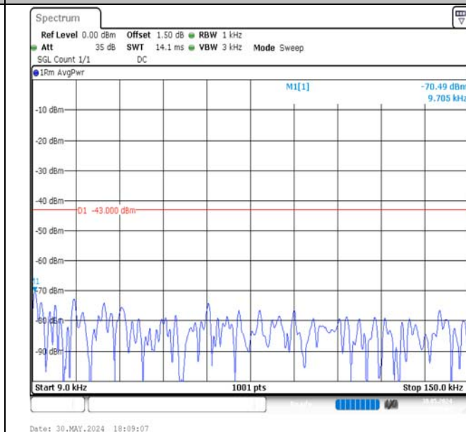
Band4-10MHz-QPSK-20175-1RB#49-0.009~0.15-PASS
