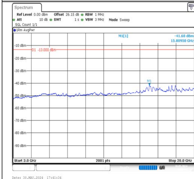
Band4-15MHz-16QAM-20025-75RB#0-3000~20000-PASS
