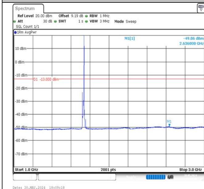
Band4-10MHz-QPSK-20175-1RB#49-1000~3000-PASS
