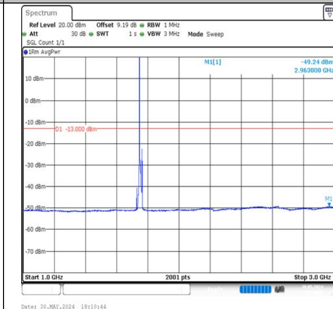
Band4-10MHz-QPSK-20350-1RB#0-1000~3000-PASS
