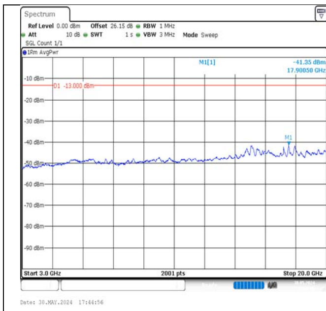
Band4-15MHz-QPSK-20325-1RB#74-3000~20000-PASS
