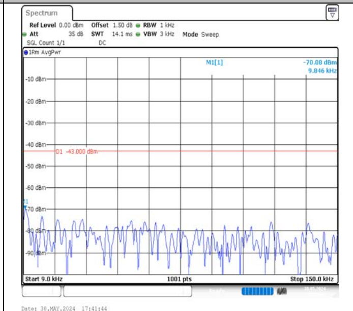
Band4-15MHz-QPSK-20175-1RB#0-0.009~0.15-PASS
