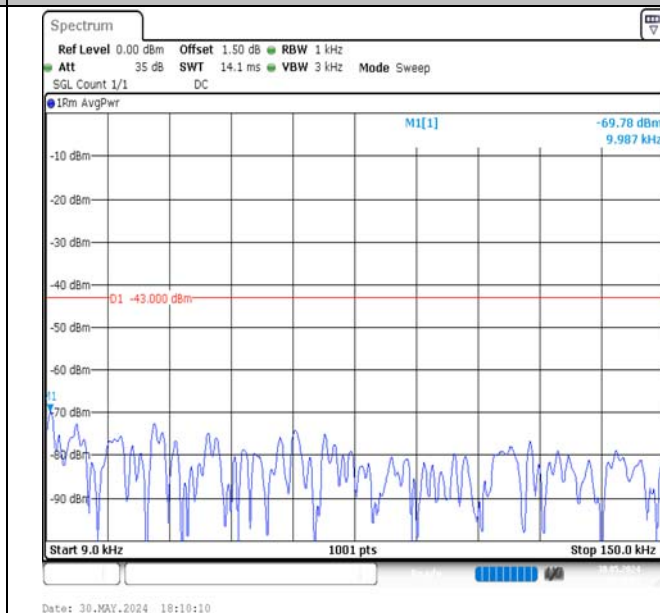
Band4-10MHz-16QAM-20175-50RB#0-0.009~0.15-PASS
