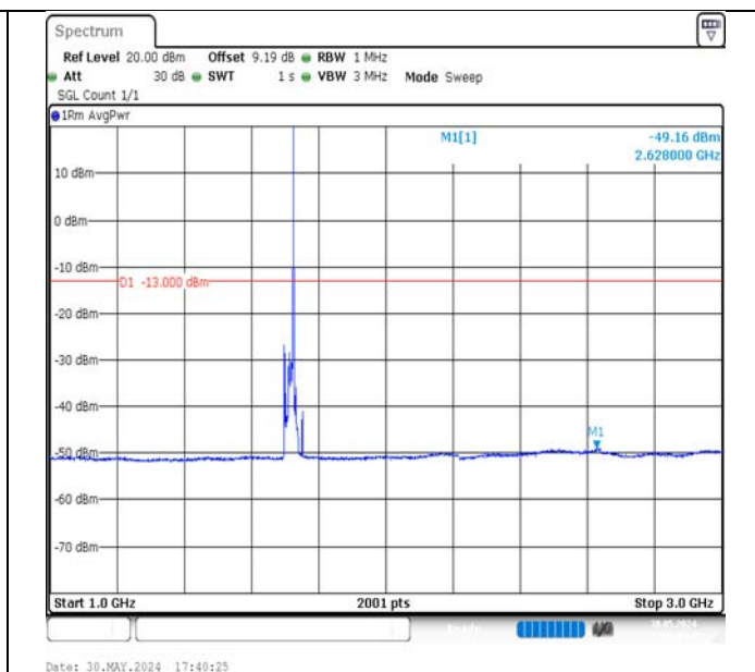
Band4-15MHz-QPSK-20025-1RB#74-1000~3000-PASS
