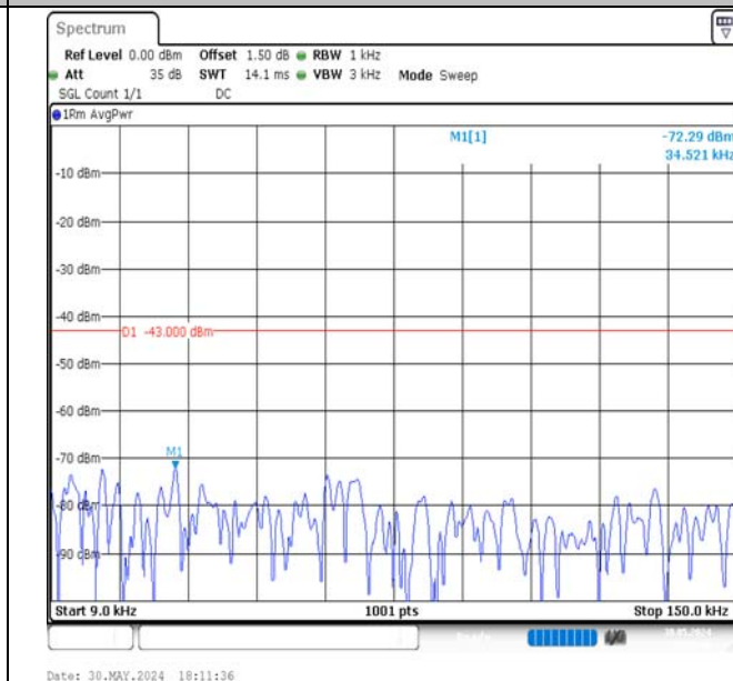
Band4-10MHz-16QAM-20350-1RB#49-0.009~0.15-PASS
