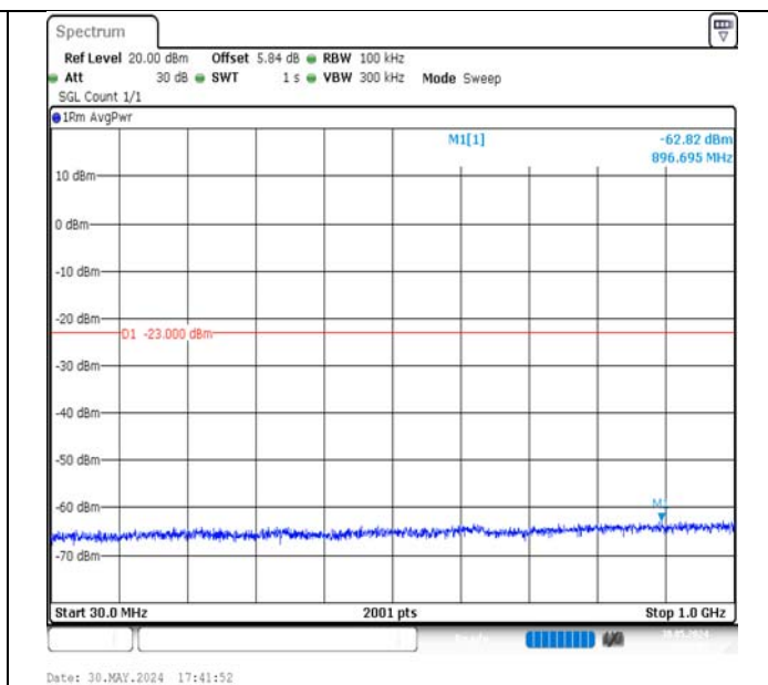
Band4-15MHz-QPSK-20175-1RB#0-30~1000-PASS
