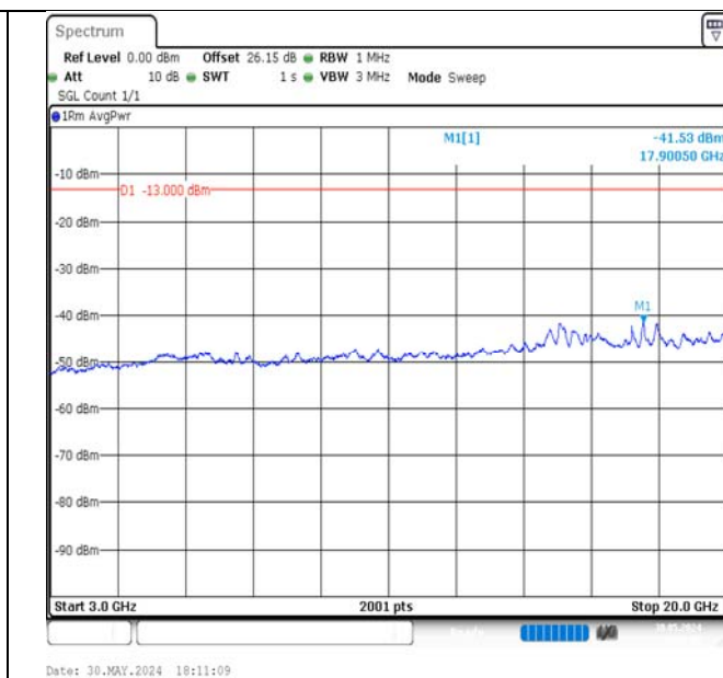
Band4-10MHz-16QAM-20350-1RB#0-3000~20000-PASS
