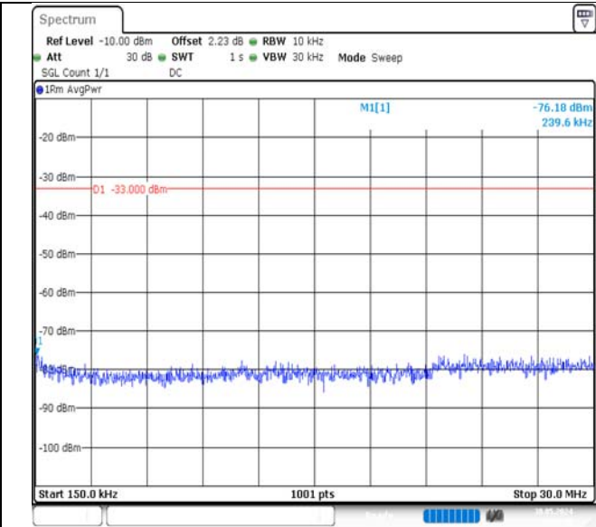
Band4-10MHz-16QAM-20350-1RB#49-0.15~30-PASS
