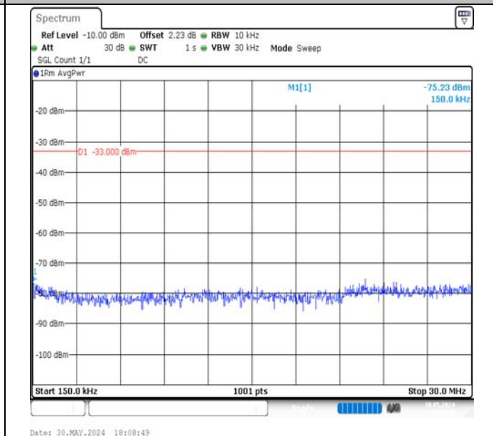
Band4-10MHz-16QAM-20175-1RB#0-0.15~30-PASS
