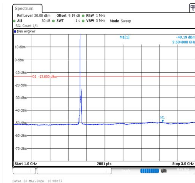
Band4-10MHz-16QAM-20175-1RB#0-1000~3000-PASS
