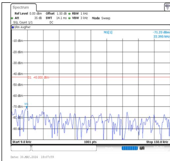
Band4-10MHz-16QAM-20000-50RB#0-0.009~0.15-PASS
