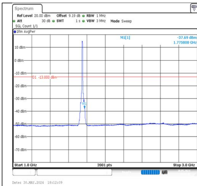
Band4-10MHz-QPSK-20350-50RB#0-1000~3000-PASS
