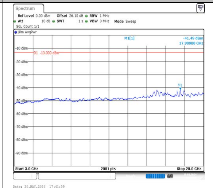
Band4-15MHz-QPSK-20175-1RB#0-3000~20000-PASS
