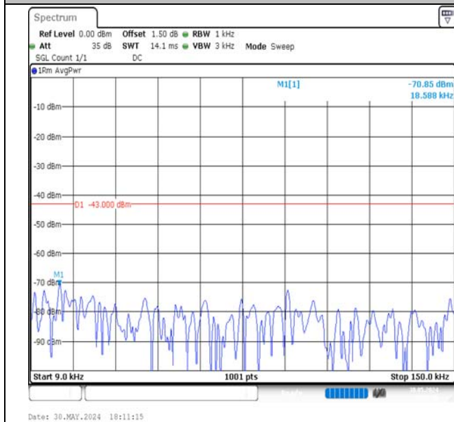
Band4-10MHz-QPSK-20350-1RB#49-0.009~0.15-PASS
