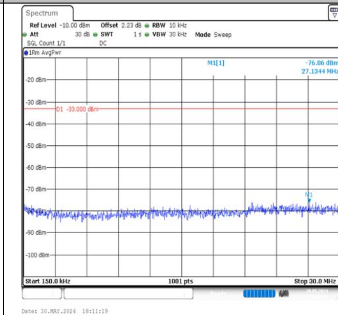
Band4-10MHz-QPSK-20350-1RB#49-0.15~30-PASS
