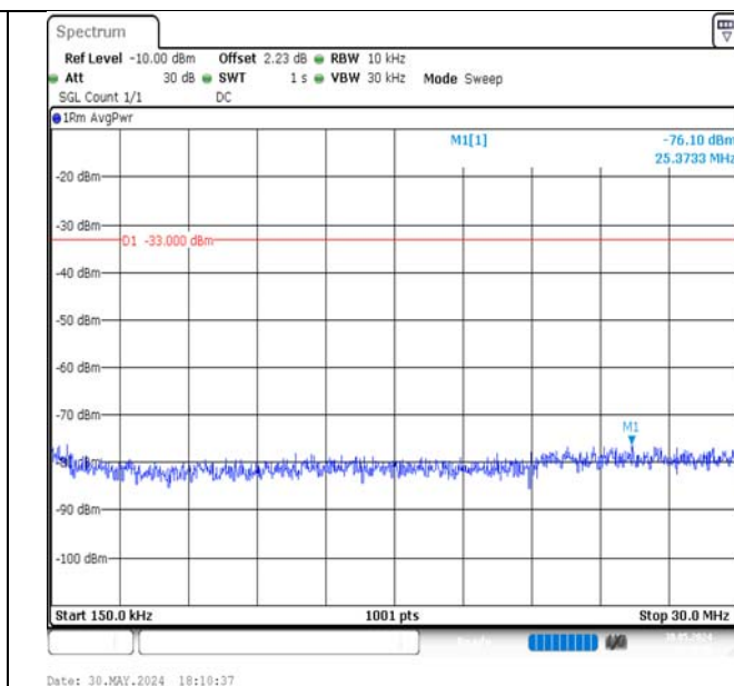
Band4-10MHz-QPSK-20350-1RB#0-0.15~30-PASS
