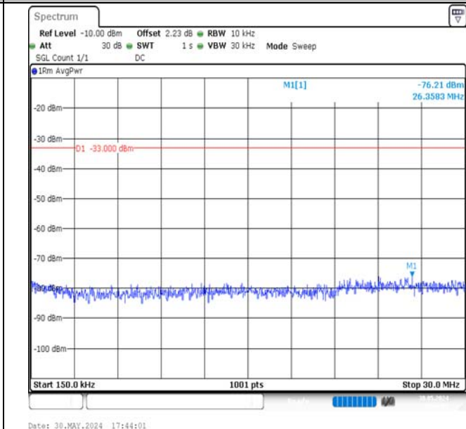
Band4-15MHz-QPSK-20325-1RB#0-0.15~30-PASS
