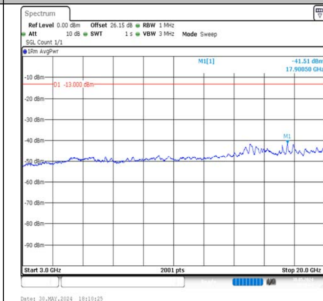
Band4-10MHz-16QAM-20175-50RB#0-3000~20000-PASS
