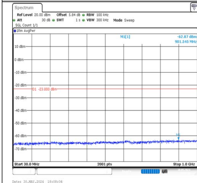
Band4-10MHz-16QAM-20000-50RB#0-30~1000-PASS
