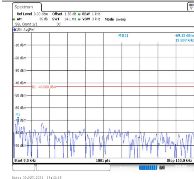
Band4-10MHz-16QAM-20350-50RB#0-0.009~0.15-PASS
