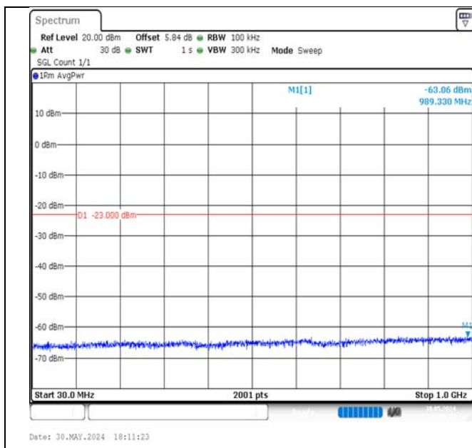
Band4-10MHz-QPSK-20350-1RB#49-30~1000-PASS
