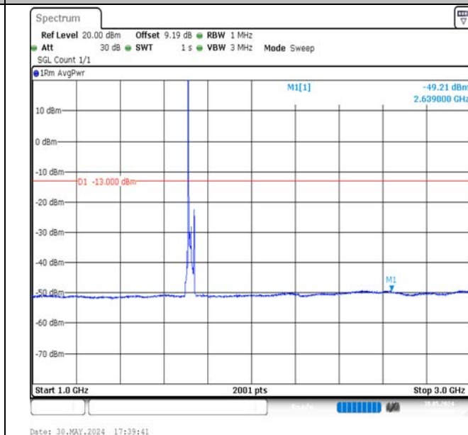
Band4-15MHz-QPSK-20025-1RB#0-1000~3000-PASS
