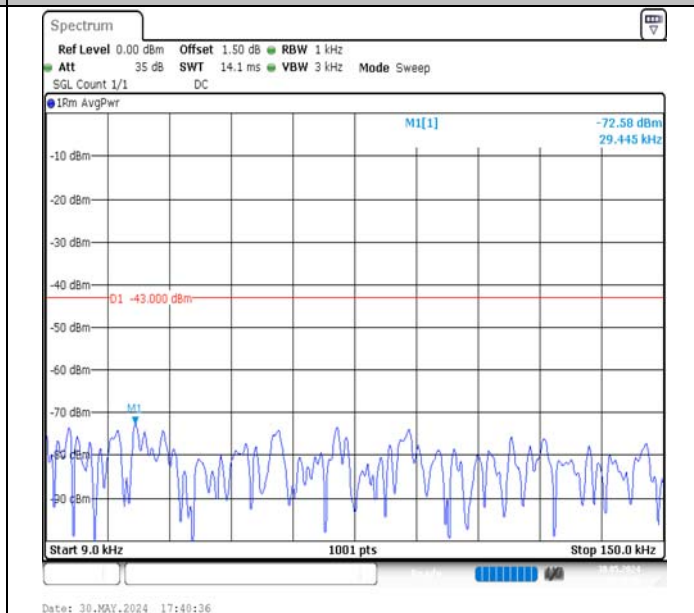
Band4-15MHz-16QAM-20025-1RB#74-0.009~0.15-PASS
