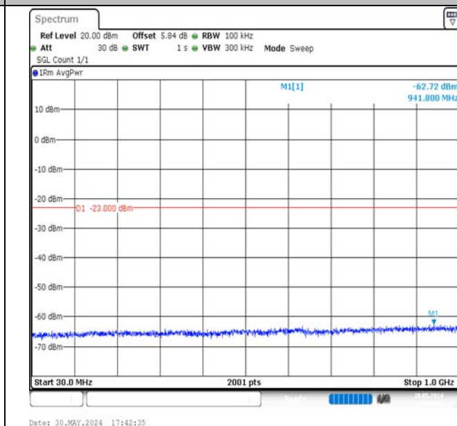
Band4-15MHz-QPSK-20175-1RB#74-30~1000-PASS
