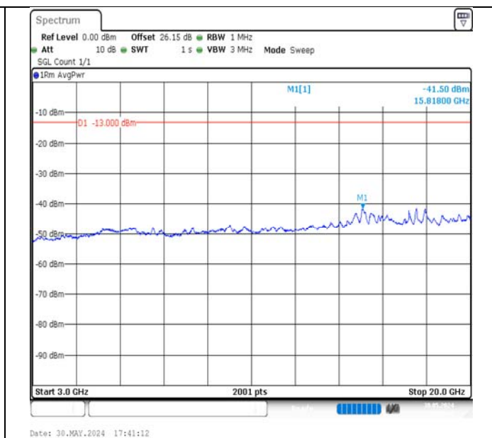
Band4-15MHz-QPSK-20025-75RB#0-3000~20000-PASS
