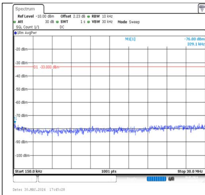
Band4-15MHz-QPSK-20325-75RB#0-0.15~30-PASS
