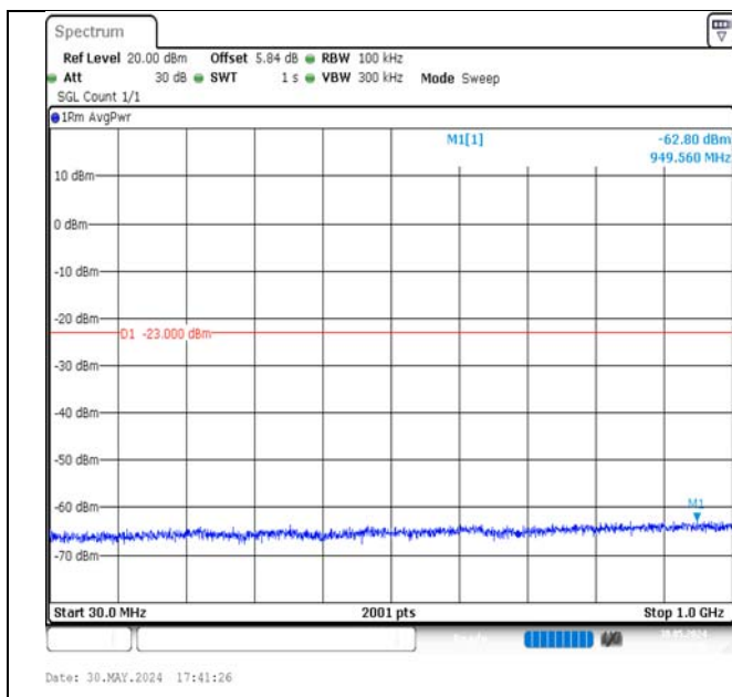
Band4-15MHz-16QAM-20025-75RB#0-30~1000-PASS
