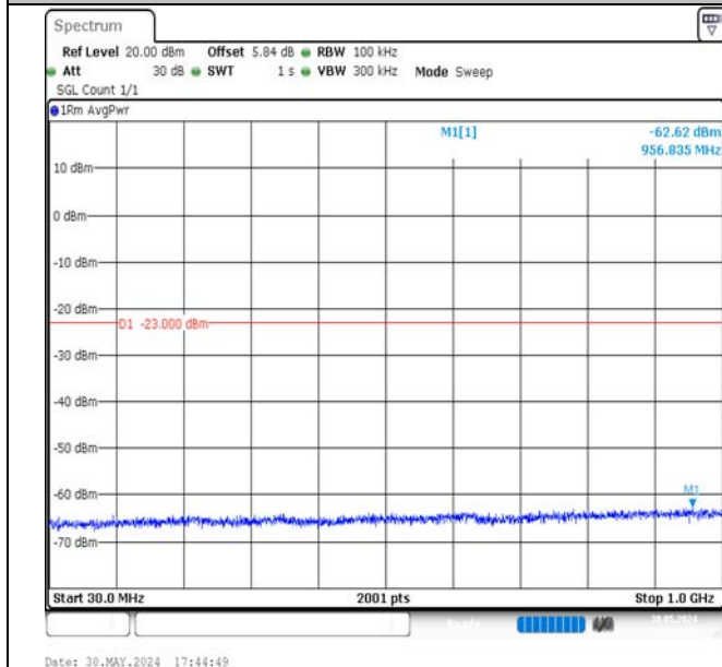
Band4-15MHz-QPSK-20325-1RB#74-30~1000-PASS
