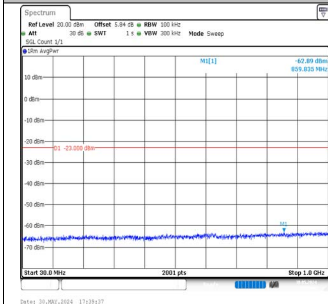
Band4-15MHz-QPSK-20025-1RB#0-30~1000-PASS
