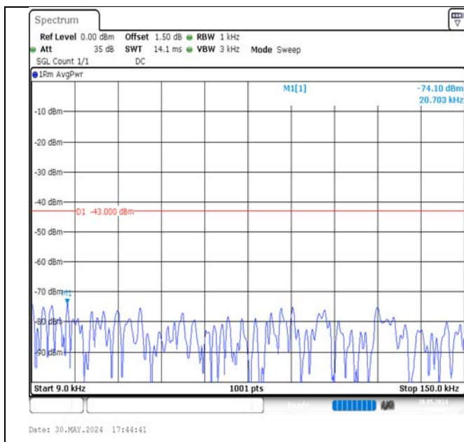
Band4-15MHz-QPSK-20325-1RB#74-0.009~0.15-PASS
