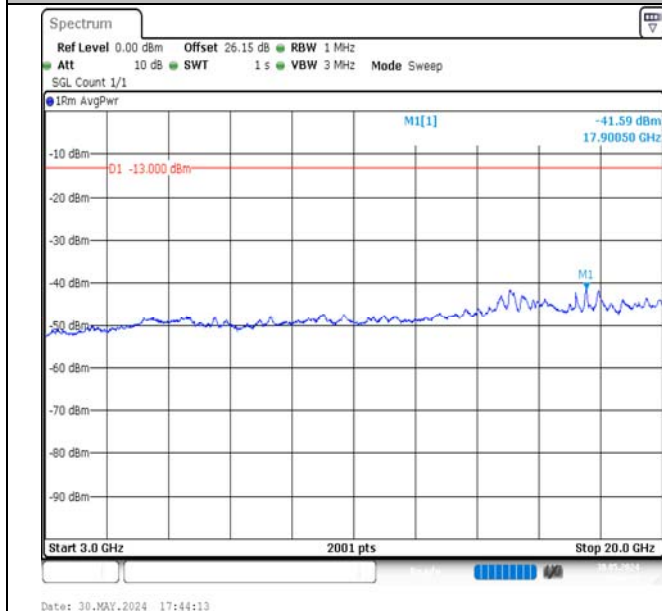
Band4-15MHz-QPSK-20325-1RB#0-3000~20000-PASS
