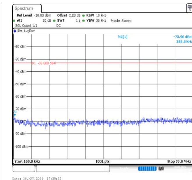
Band4-15MHz-QPSK-20025-1RB#0-0.15~30-PASS
