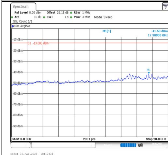
Band4-10MHz-16QAM-20350-50RB#0-3000~20000-PASS
