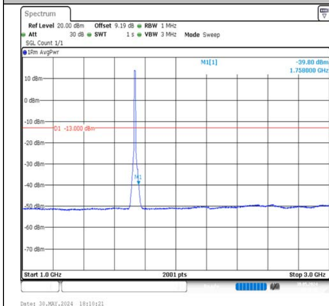
Band4-10MHz-16QAM-20175-50RB#0-1000~3000-PASS
