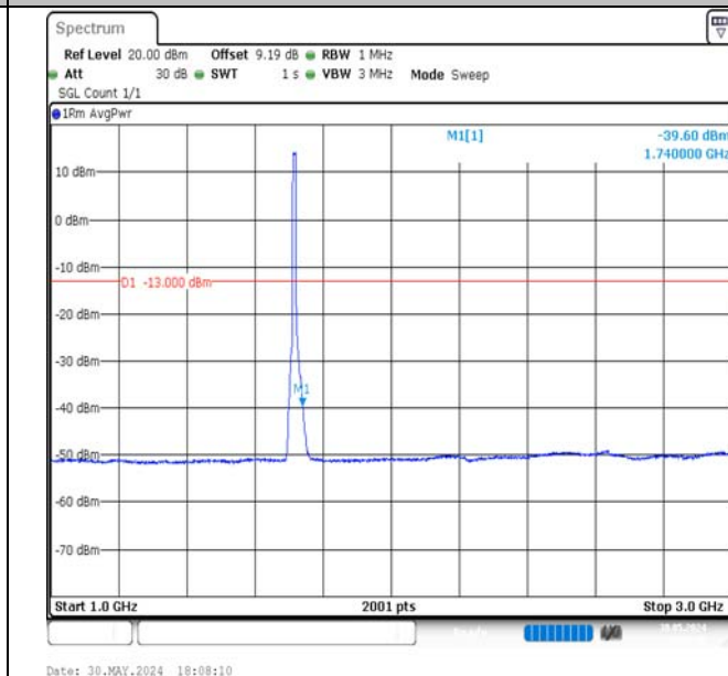
Band4-10MHz-16QAM-20000-50RB#0-1000~3000-PASS
