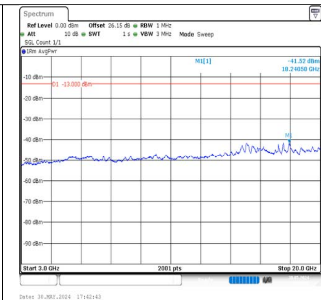
Band4-15MHz-QPSK-20175-1RB#74-3000~20000-PASS
