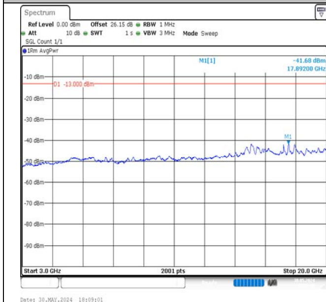
Band4-10MHz-16QAM-20175-1RB#0-3000~20000-PASS
