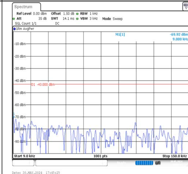
Band4-15MHz-QPSK-20325-75RB#0-0.009~0.15-PASS
