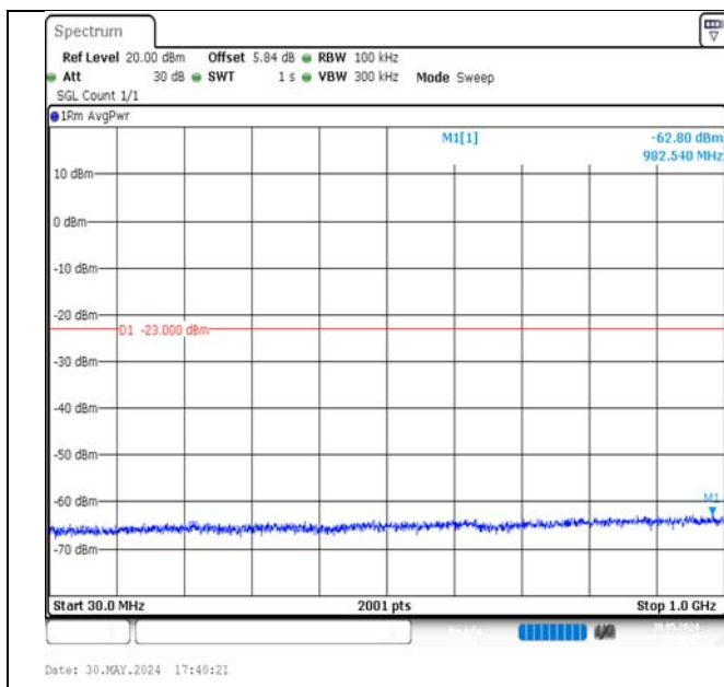
Band4-15MHz-QPSK-20025-1RB#74-30~1000-PASS
