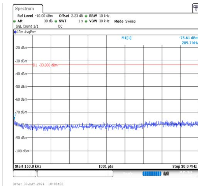
Band4-10MHz-16QAM-20000-50RB#0-0.15~30-PASS
