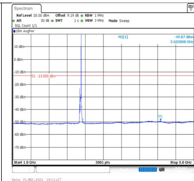
Band4-10MHz-QPSK-20350-1RB#49-1000~3000-PASS
