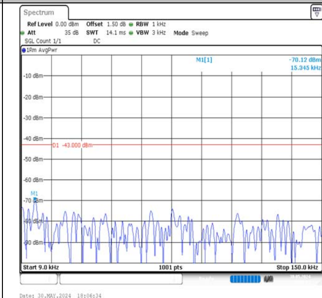
Band4-10MHz-16QAM-20000-1RB#0-0.009~0.15-PASS
