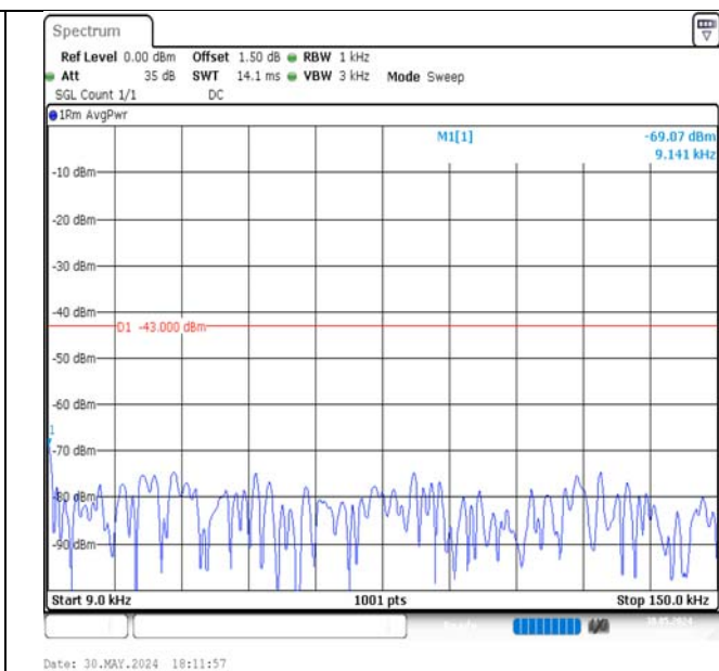
Band4-10MHz-QPSK-20350-50RB#0-0.009~0.15-PASS
