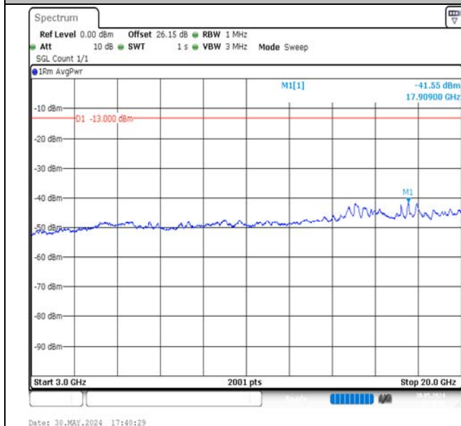
Band4-15MHz-QPSK-20025-1RB#74-3000~20000-PASS
