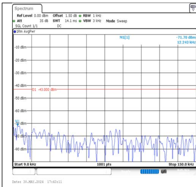
Band4-15MHz-QPSK-20175-75RB#0-0.009~0.15-PASS
