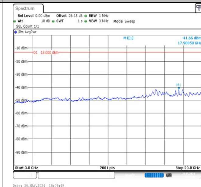
Band4-10MHz-16QAM-20000-1RB#0-3000~20000-PASS
