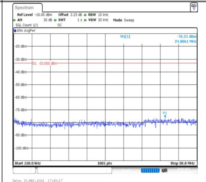
Band4-15MHz-QPSK-20025-1RB#74-0.15~30-PASS
