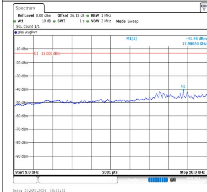
Band4-10MHz-QPSK-20350-1RB#49-3000~20000-PASS
