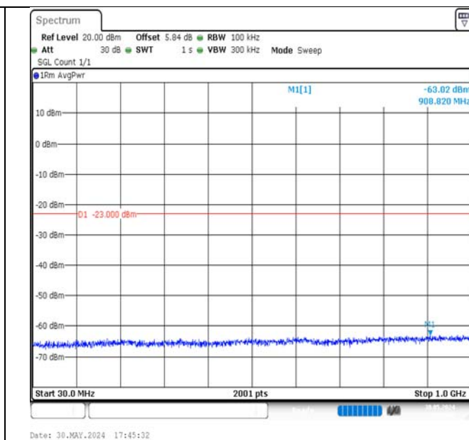
Band4-15MHz-QPSK-20325-75RB#0-30~1000-PASS
