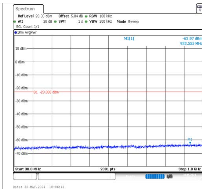
Band4-10MHz-16QAM-20000-1RB#0-30~1000-PASS
