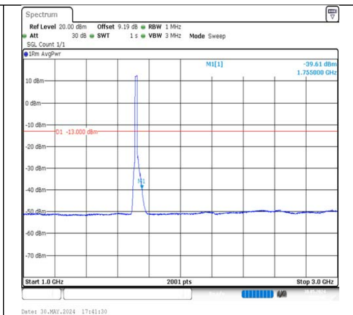
Band4-15MHz-16QAM-20025-75RB#0-1000~3000-PASS
