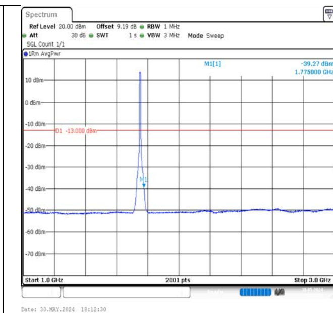
Band4-10MHz-16QAM-20350-50RB#0-1000~3000-PASS
