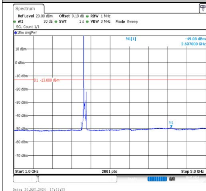
Band4-15MHz-QPSK-20175-1RB#0-1000~3000-PASS
