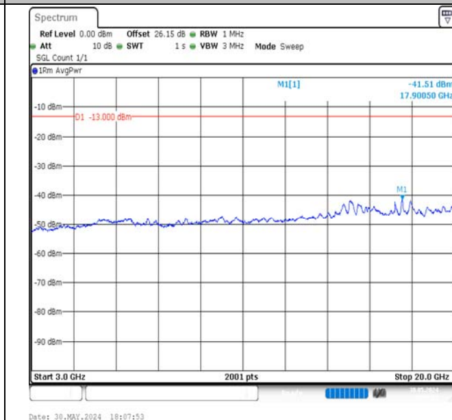
Band4-10MHz-QPSK-20000-50RB#0-3000~20000-PASS
