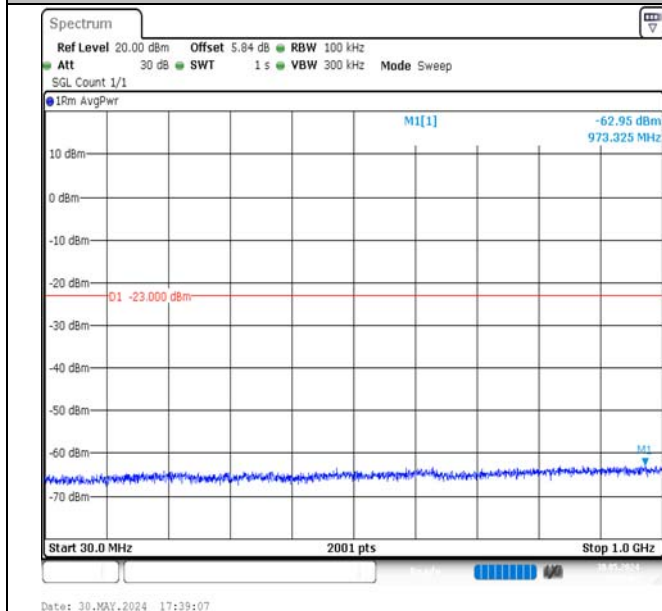
Band4-5MHz-16QAM-20375-25RB#0-30~1000-PASS
