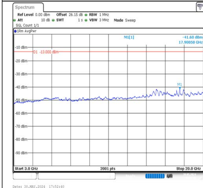
Band4-3MHz-16QAM-20385-15RB#0-3000~20000-PASS
