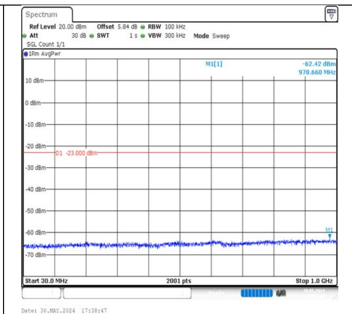
Band4-5MHz-QPSK-20375-25RB#0-30~1000-PASS
