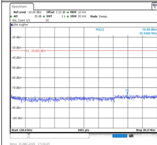
Band4-5MHz-QPSK-19975-25RB#0-0.15~30-PASS
