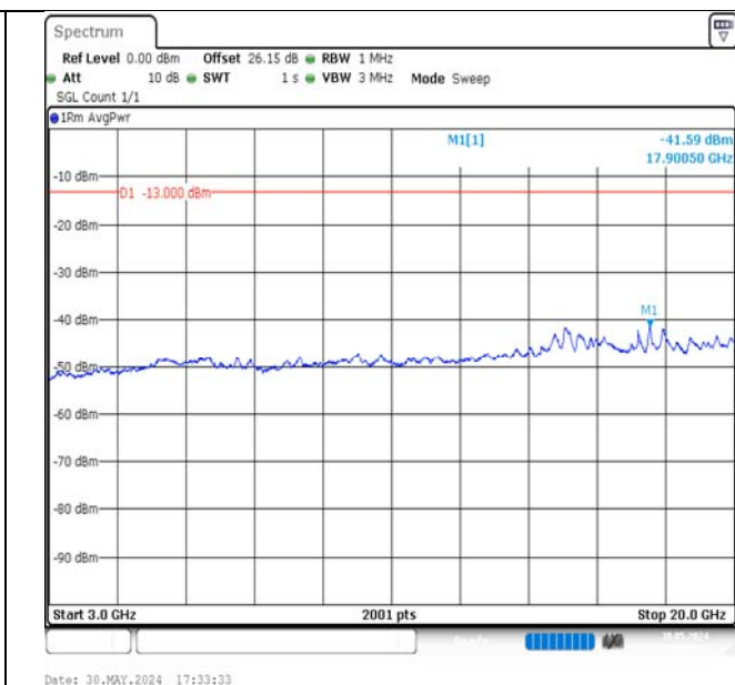
Band4-5MHz-16QAM-19975-1RB#0-3000~20000-PASS
