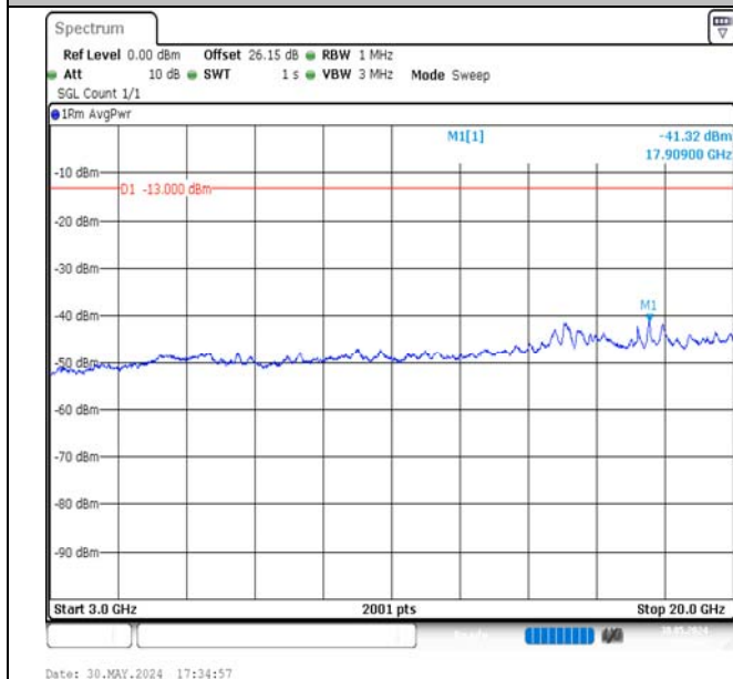
Band4-5MHz-16QAM-19975-25RB#0-3000~20000-PASS
