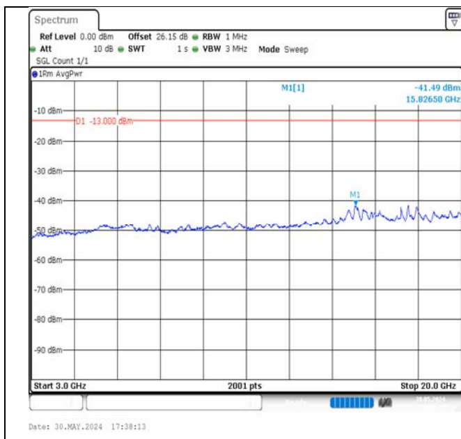
Band4-5MHz-QPSK-20375-1RB#24-3000~20000-PASS
