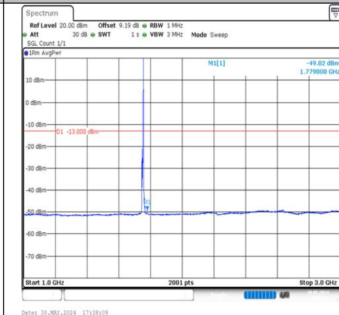
Band4-5MHz-QPSK-20375-1RB#24-1000~3000-PASS
