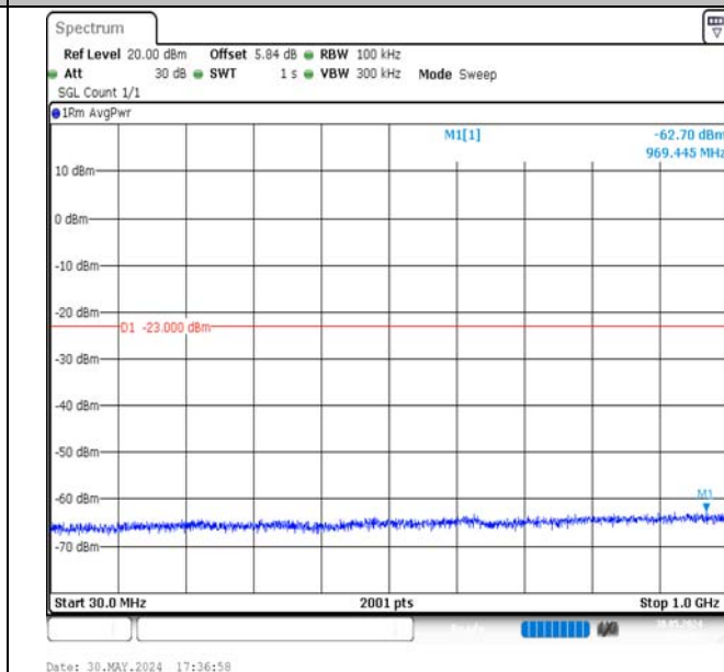
Band4-5MHz-16QAM-20175-25RB#0-30~1000-PASS
