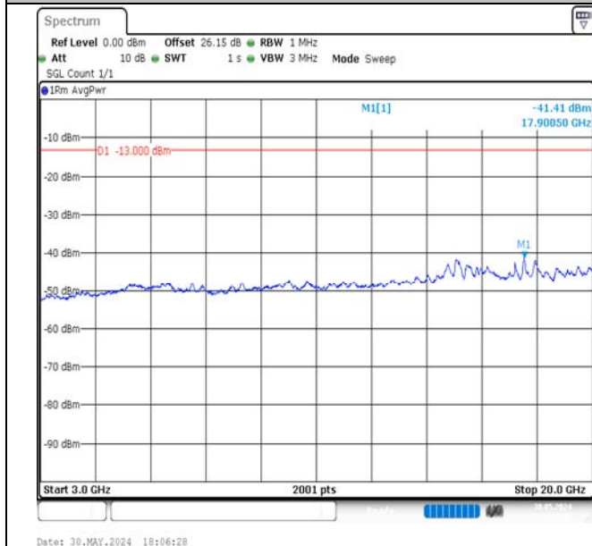
Band4-10MHz-QPSK-20000-1RB#0-3000~20000-PASS
