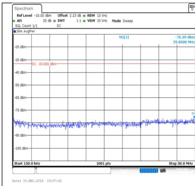
Band4-10MHz-QPSK-20000-50RB#0-0.15~30-PASS
