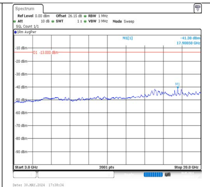
Band4-5MHz-16QAM-20375-1RB#24-3000~20000-PASS
