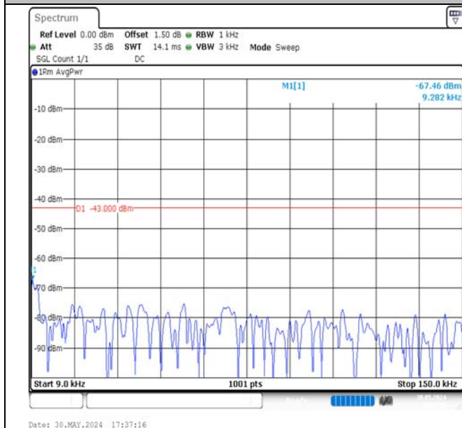
Band4-5MHz-QPSK-20375-1RB#0-0.009~0.15-PASS
