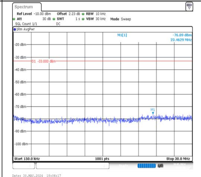
Band4-10MHz-QPSK-20000-1RB#0-0.15~30-PASS
