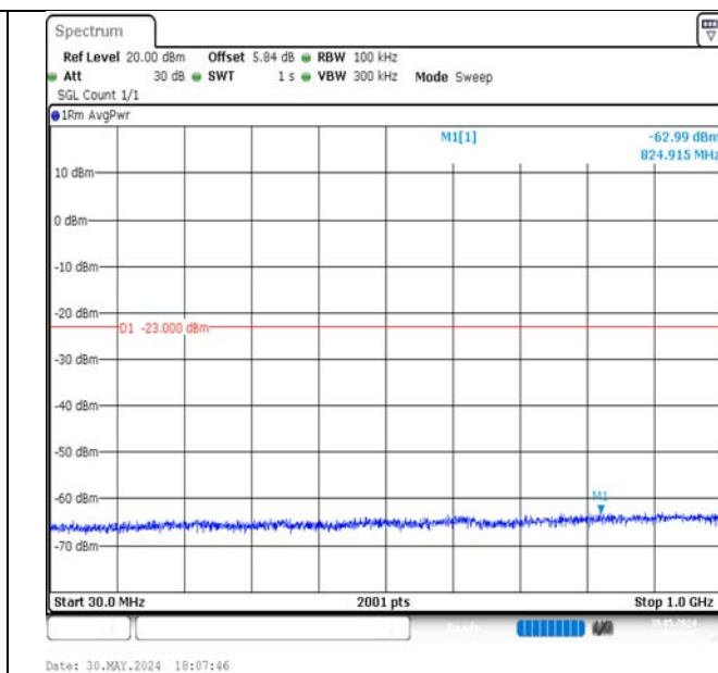
Band4-10MHz-QPSK-20000-50RB#0-30~1000-PASS
