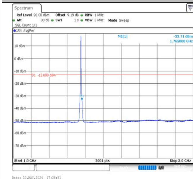
Band4-5MHz-QPSK-20375-25RB#0-1000~3000-PASS
