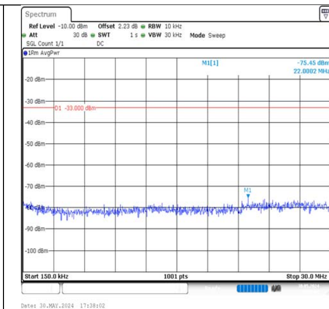
Band4-5MHz-QPSK-20375-1RB#24-0.15~30-PASS
