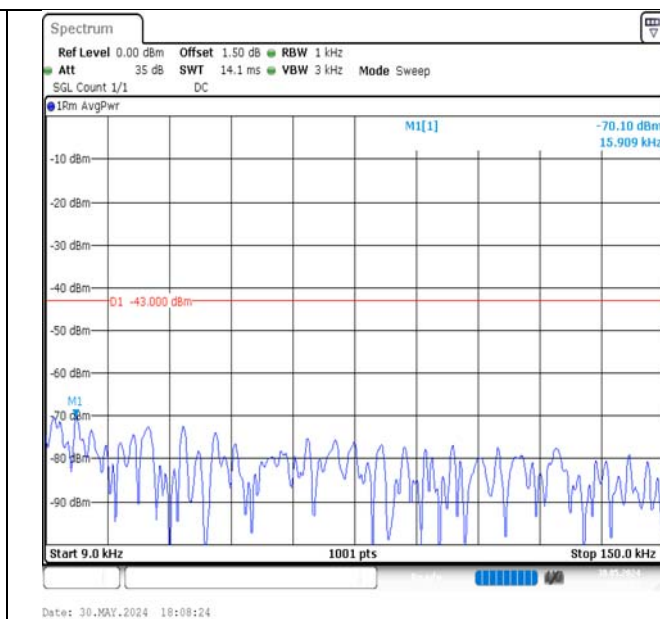
Band4-10MHz-QPSK-20175-1RB#0-0.009~0.15-PASS
