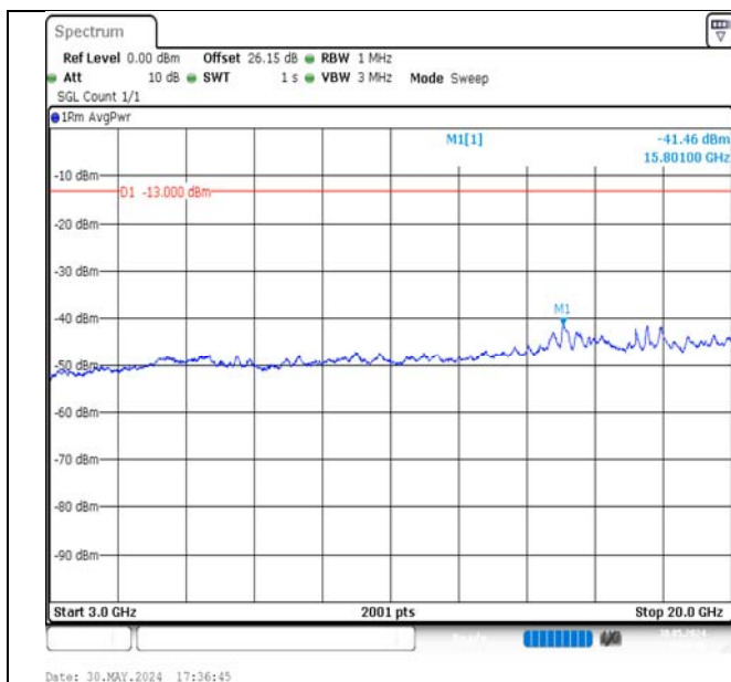
Band4-5MHz-QPSK-20175-25RB#0-3000~20000-PASS
