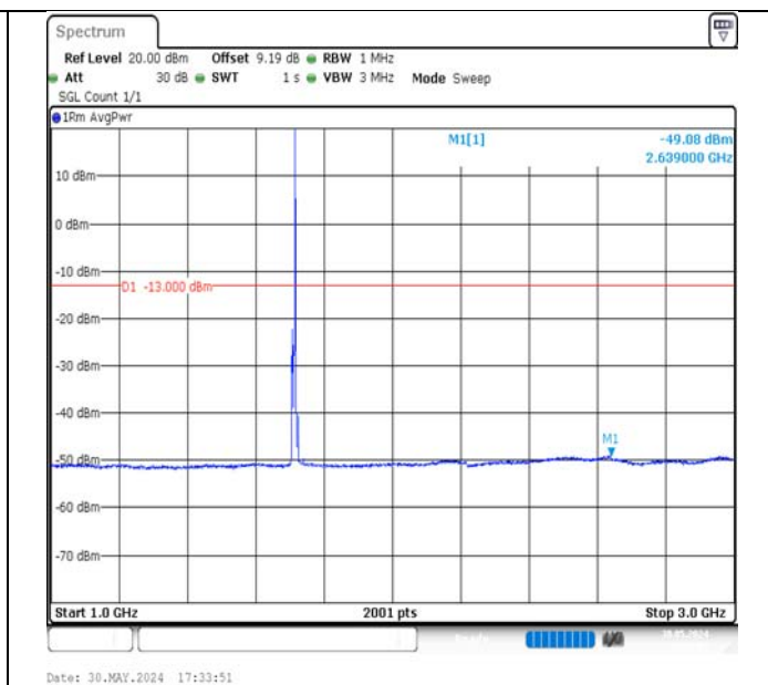
Band4-5MHz-QPSK-19975-1RB#24-1000~3000-PASS
