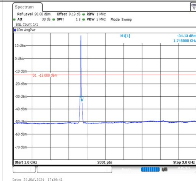
Band4-5MHz-QPSK-20175-25RB#0-1000~3000-PASS
