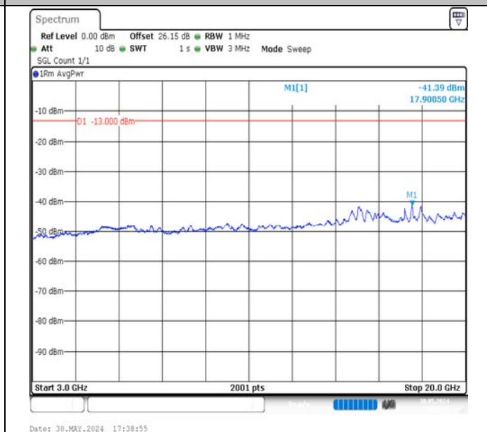
Band4-5MHz-QPSK-20375-25RB#0-3000~20000-PASS
