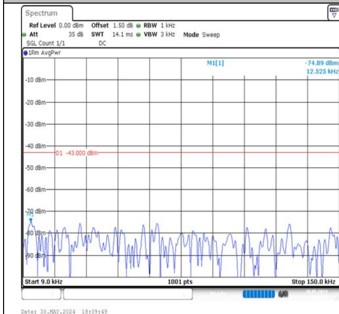
Band4-10MHz-QPSK-20175-50RB#0-0.009~0.15-PASS
