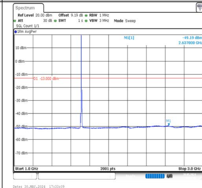
Band4-5MHz-QPSK-19975-1RB#0-1000~3000-PASS
