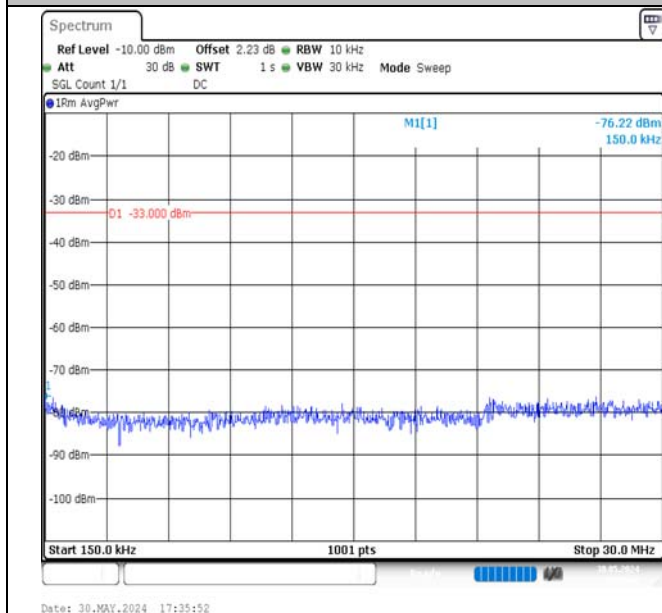
Band4-5MHz-QPSK-20175-1RB#24-0.15~30-PASS
