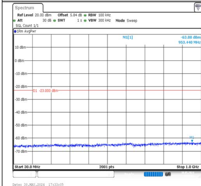
Band4-5MHz-QPSK-19975-1RB#0-30~1000-PASS
