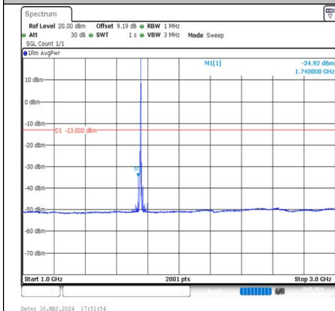
Band4-3MHz-16QAM-20385-1RB#14-1000~3000-PASS
