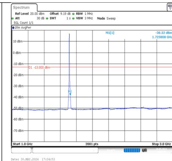
Band4-5MHz-16QAM-19975-25RB#0-1000~3000-PASS
