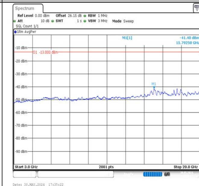
Band4-5MHz-QPSK-20175-1RB#0-3000~20000-PASS
