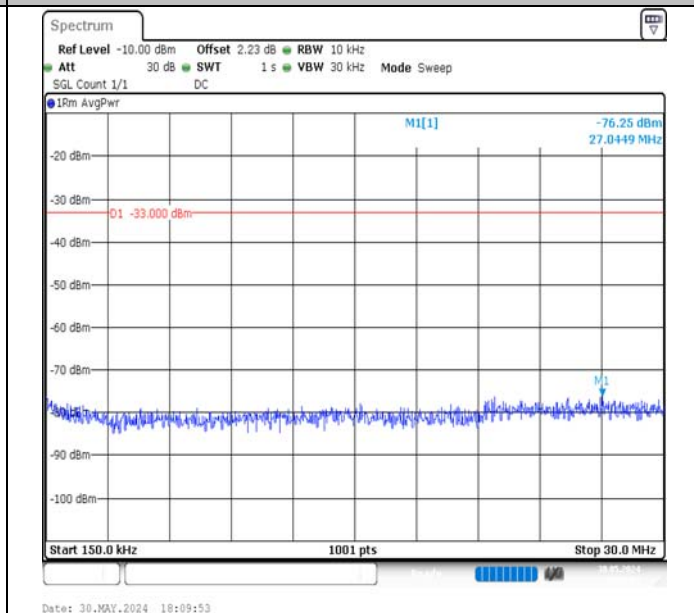
Band4-10MHz-QPSK-20175-50RB#0-0.15~30-PASS
