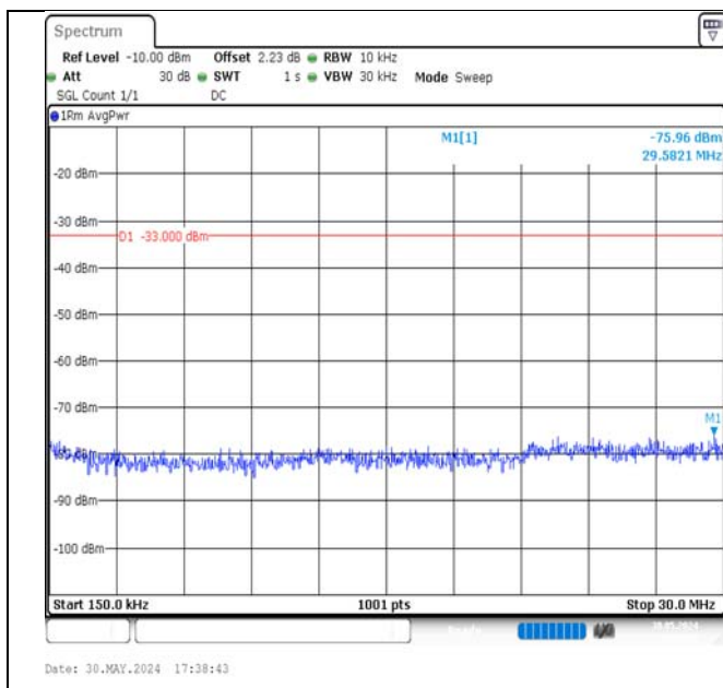
Band4-5MHz-QPSK-20375-25RB#0-0.15~30-PASS
