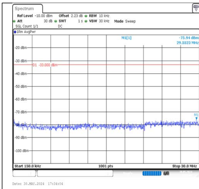
Band4-5MHz-16QAM-19975-1RB#24-0.15~30-PASS
