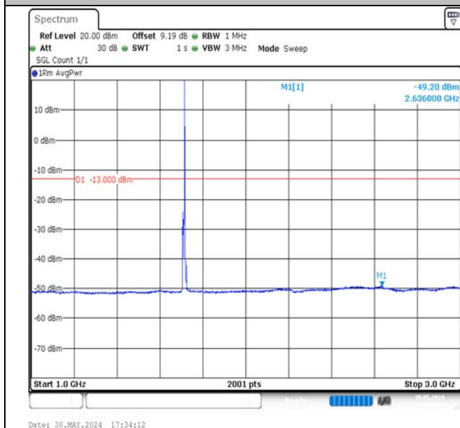
Band4-5MHz-16QAM-19975-1RB#24-1000~3000-PASS
