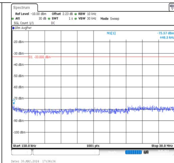
Band4-5MHz-QPSK-20175-25RB#0-0.15~30-PASS
