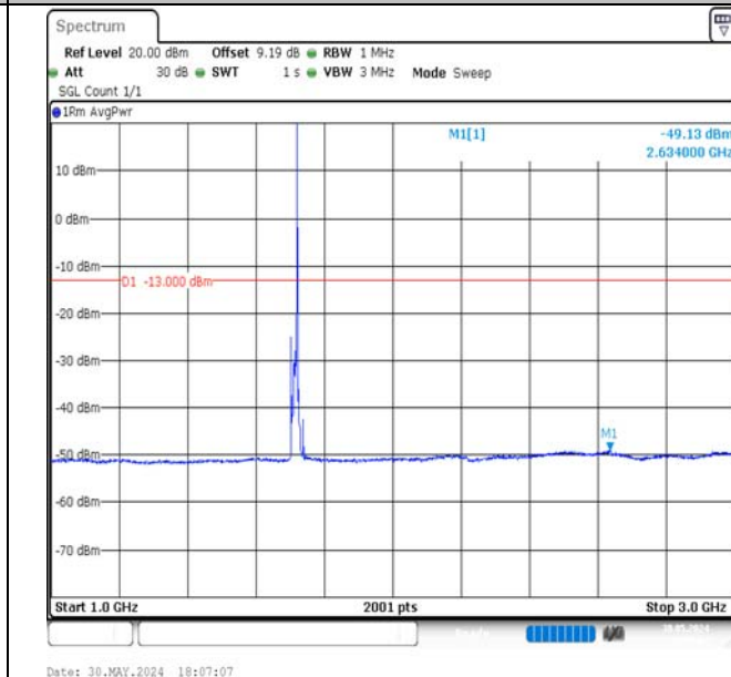
Band4-10MHz-QPSK-20000-1RB#49-1000~3000-PASS
