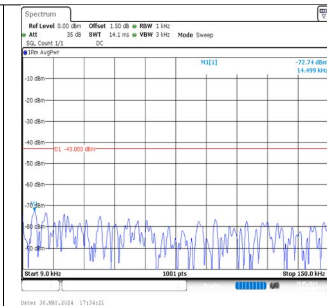
Band4-5MHz-QPSK-19975-25RB#0-0.009~0.15-PASS
