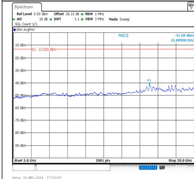
Band4-5MHz-QPSK-19975-1RB#24-3000~20000-PASS
