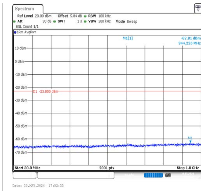
Band4-3MHz-16QAM-20385-15RB#0-30~1000-PASS
