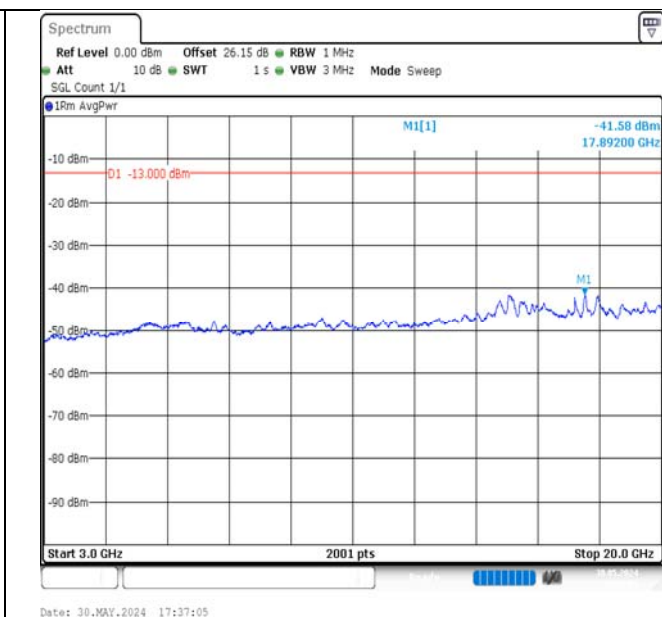
Band4-5MHz-16QAM-20175-25RB#0-3000~20000-PASS
