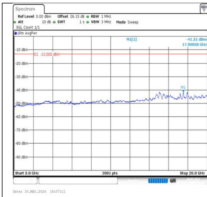
Band4-10MHz-QPSK-20000-1RB#49-3000~20000-PASS
