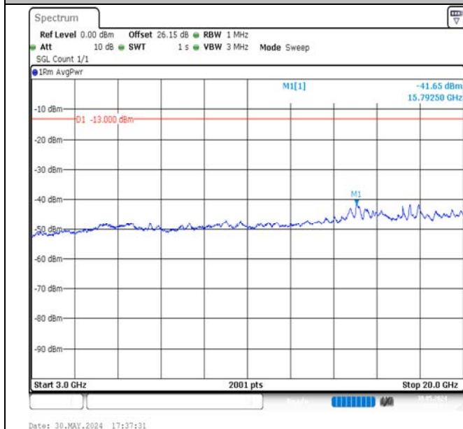
Band4-5MHz-QPSK-20375-1RB#0-3000~20000-PASS
