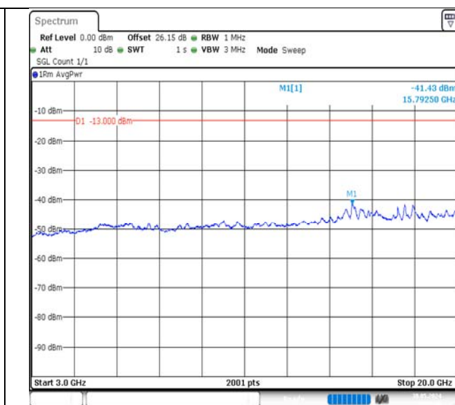
Band4-5MHz-QPSK-19975-25RB#0-3000~20000-PASS
