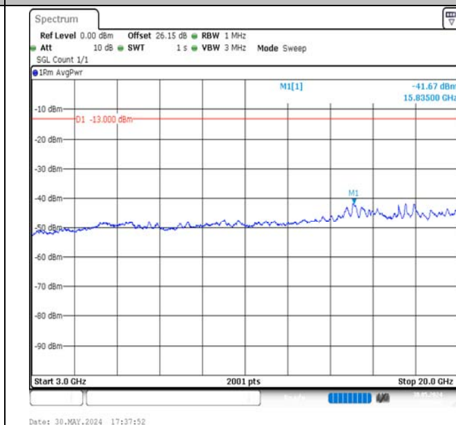
Band4-5MHz-16QAM-20375-1RB#0-3000~20000-PASS
