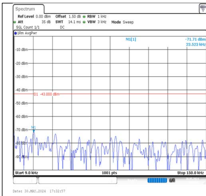
Band4-5MHz-QPSK-19975-1RB#0-0.009~0.15-PASS
