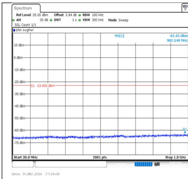
Band4-5MHz-16QAM-19975-25RB#0-30~1000-PASS
