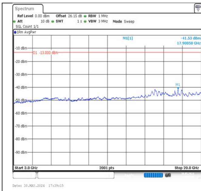
Band4-5MHz-16QAM-20375-25RB#0-3000~20000-PASS
