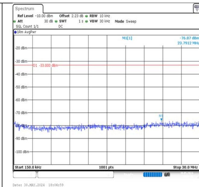
Band4-10MHz-QPSK-20000-1RB#49-0.15~30-PASS
