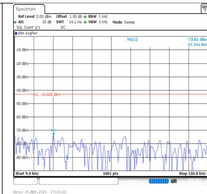
Band4-5MHz-16QAM-19975-1RB#0-0.009~0.15-PASS
