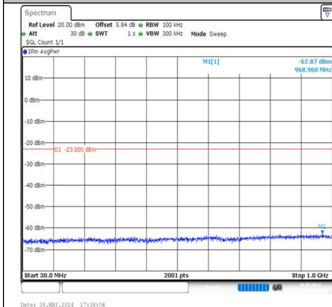
Band4-5MHz-QPSK-20375-1RB#24-30~1000-PASS
