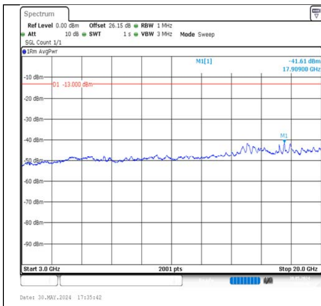
Band4-5MHz-16QAM-20175-1RB#0-3000~20000-PASS
