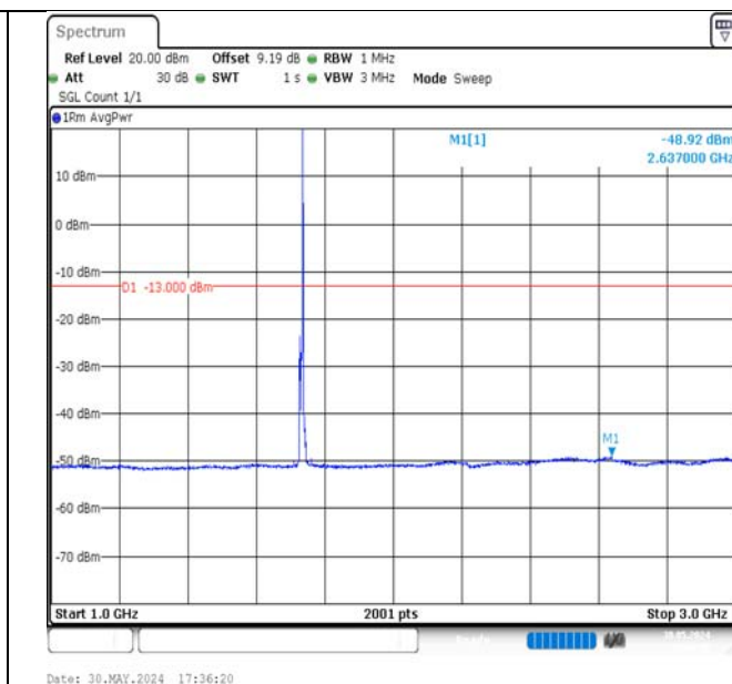
Band4-5MHz-16QAM-20175-1RB#24-1000~3000-PASS
