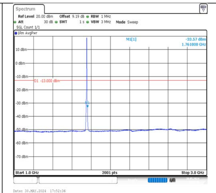
Band4-3MHz-16QAM-20385-15RB#0-1000~3000-PASS
