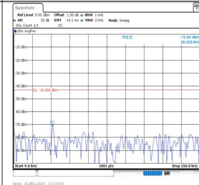
Band4-5MHz-16QAM-19975-1RB#24-0.009~0.15-PASS
