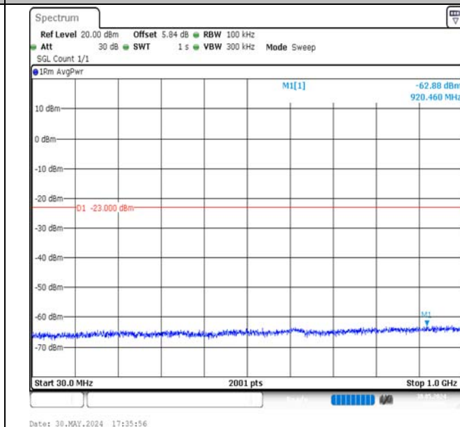
Band4-5MHz-QPSK-20175-1RB#24-30~1000-PASS
