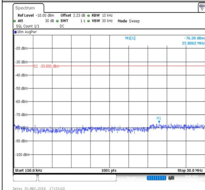
Band4-5MHz-16QAM-19975-1RB#0-0.15~30-PASS
