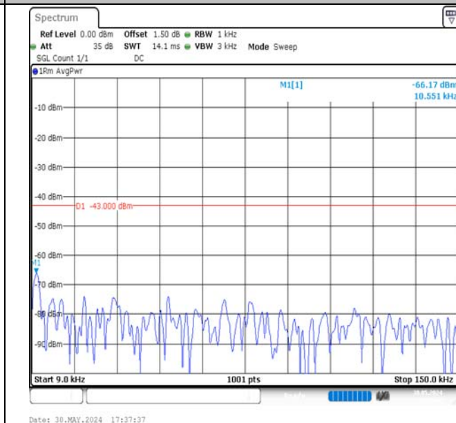
Band4-5MHz-16QAM-20375-1RB#0-0.009~0.15-PASS
