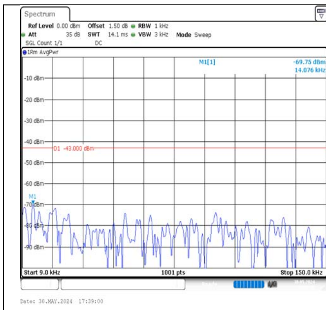
Band4-5MHz-16QAM-20375-25RB#0-0.009~0.15-PASS
