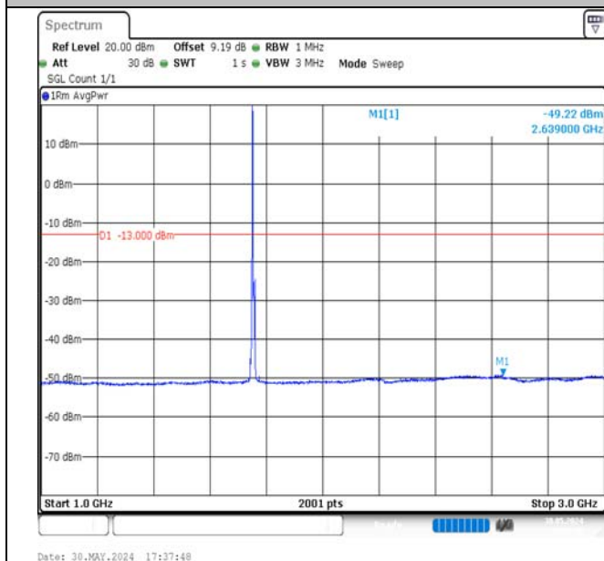
Band4-5MHz-16QAM-20375-1RB#0-1000~3000-PASS
