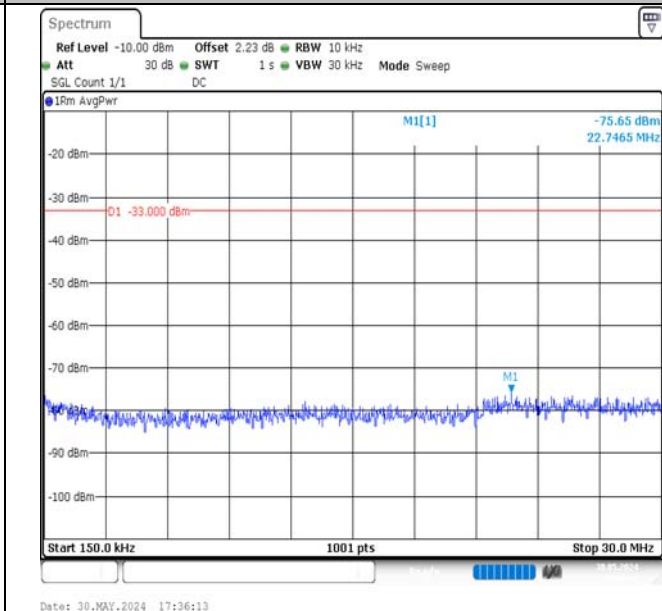
Band4-5MHz-16QAM-20175-1RB#24-0.15~30-PASS
