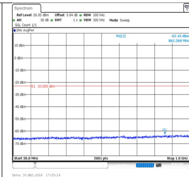
Band4-5MHz-QPSK-20175-1RB#0-30~1000-PASS
