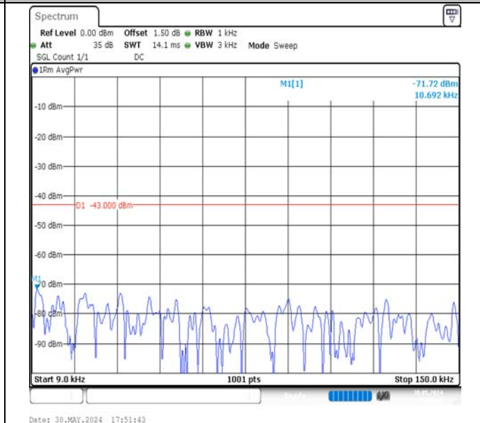
Band4-3MHz-16QAM-20385-1RB#14-0.009~0.15-PASS
