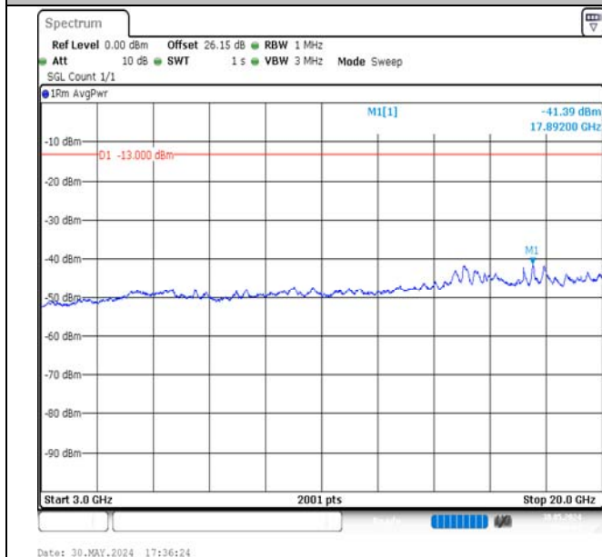
Band4-5MHz-16QAM-20175-1RB#24-3000~20000-PASS
