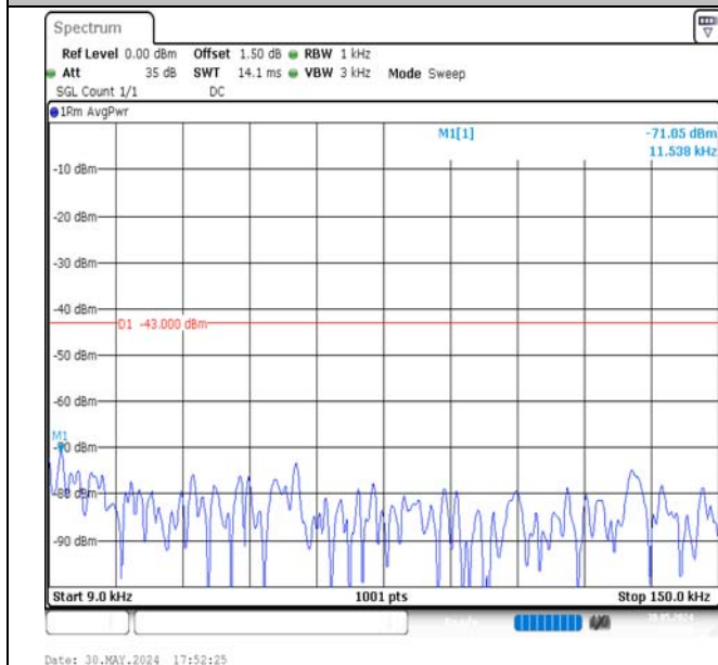
Band4-3MHz-16QAM-20385-15RB#0-0.009~0.15-PASS
