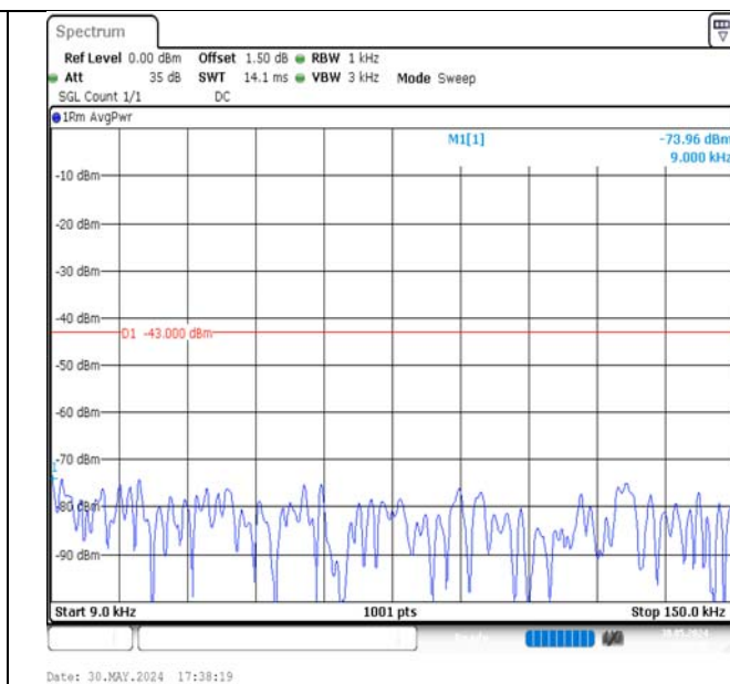
Band4-5MHz-16QAM-20375-1RB#24-0.009~0.15-PASS
