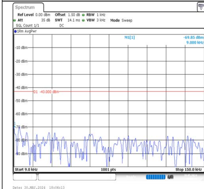
Band4-10MHz-QPSK-20000-1RB#0-0.009~0.15-PASS
