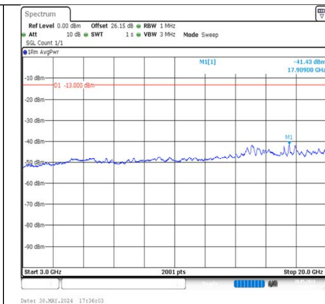
Band4-5MHz-QPSK-20175-1RB#24-3000~20000-PASS
