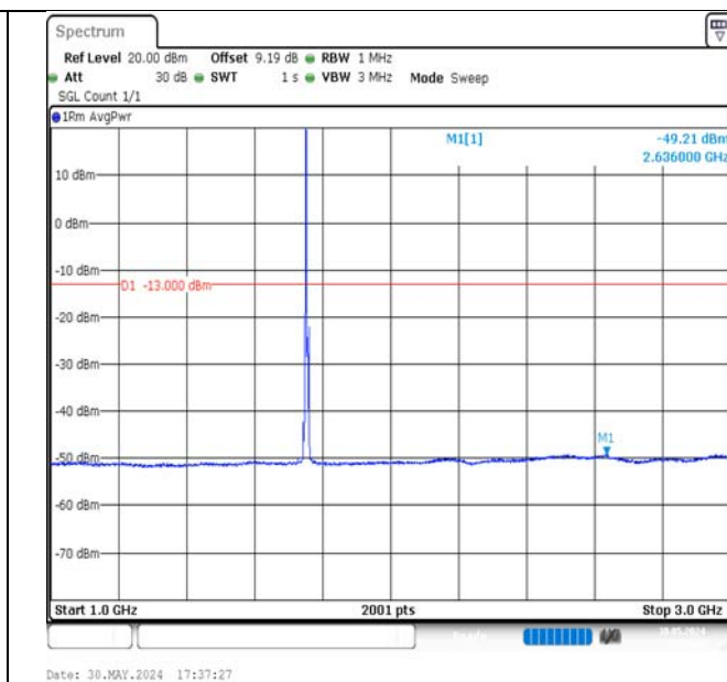
Band4-5MHz-QPSK-20375-1RB#0-1000~3000-PASS
