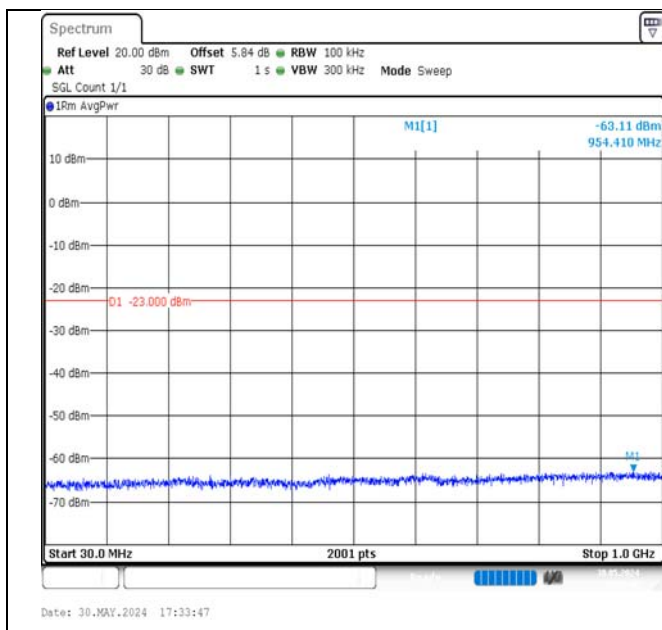
Band4-5MHz-QPSK-19975-1RB#24-30~1000-PASS
