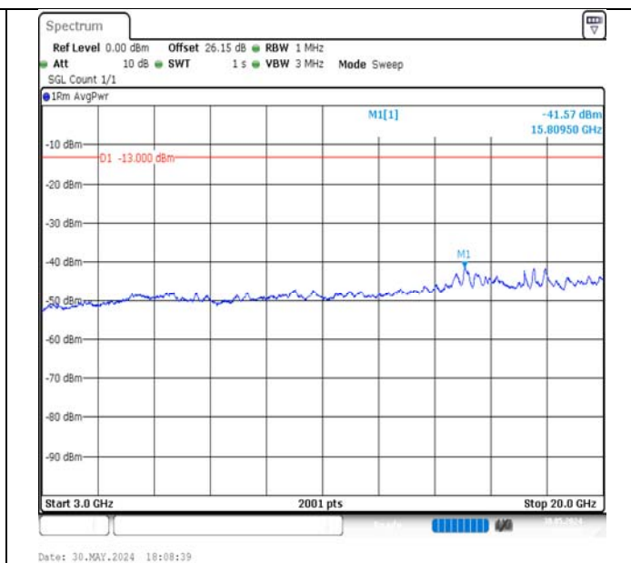
Band4-10MHz-QPSK-20175-1RB#0-3000~20000-PASS
