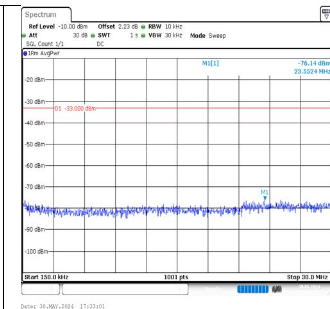
Band4-5MHz-QPSK-19975-1RB#0-0.15~30-PASS
