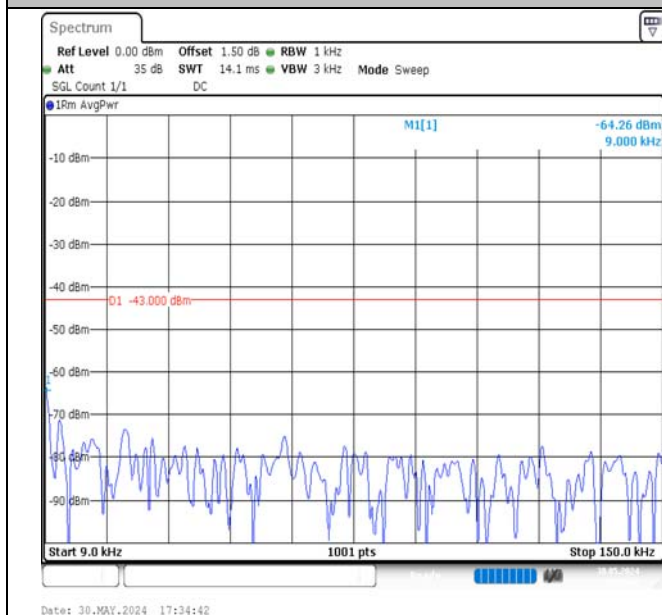
Band4-5MHz-16QAM-19975-25RB#0-0.009~0.15-PASS
