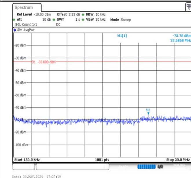
Band4-5MHz-QPSK-20375-1RB#0-0.15~30-PASS
