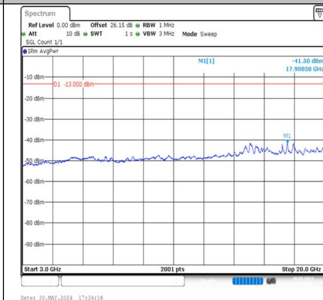
Band4-5MHz-16QAM-19975-1RB#24-3000~20000-PASS
