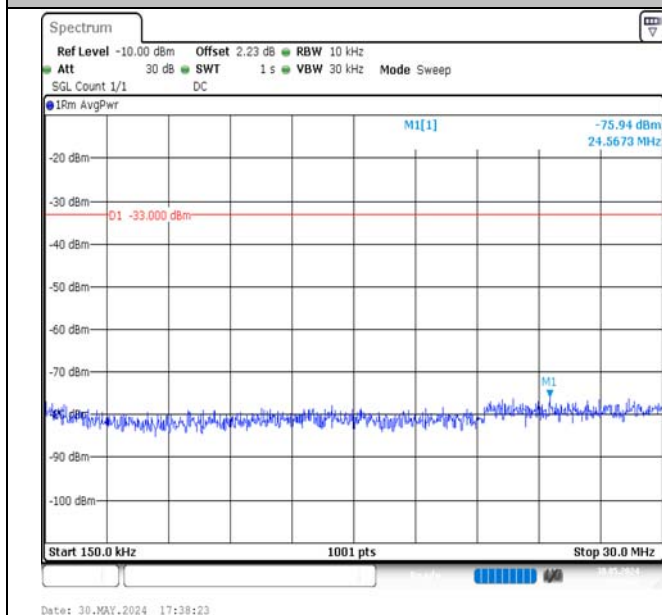
Band4-5MHz-16QAM-20375-1RB#24-0.15~30-PASS
