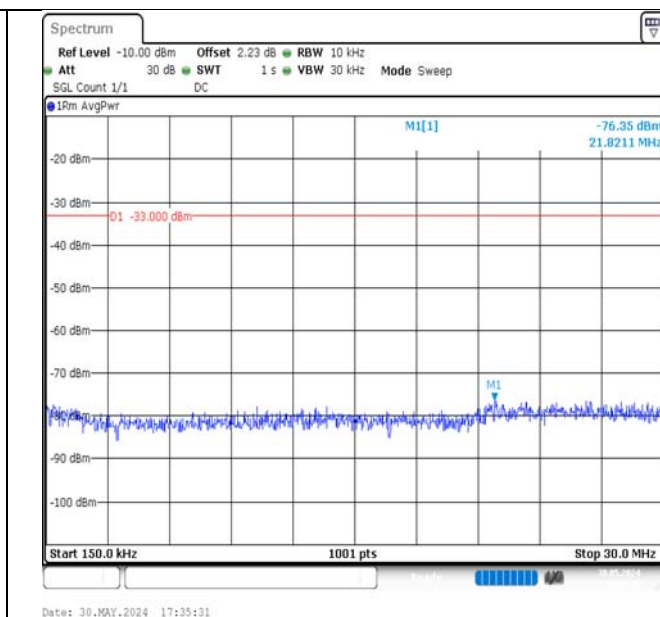
Band4-5MHz-16QAM-20175-1RB#0-0.15~30-PASS
