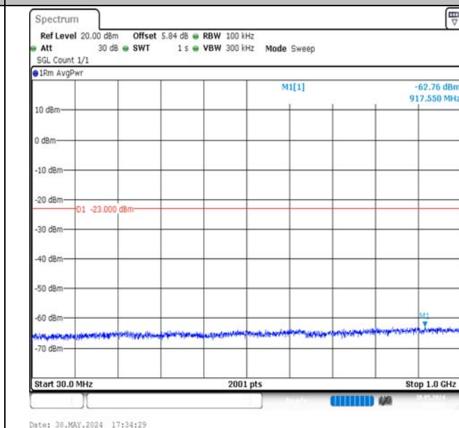
Band4-5MHz-QPSK-19975-25RB#0-30~1000-PASS
