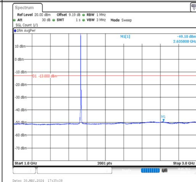
Band4-5MHz-16QAM-20175-1RB#0-1000~3000-PASS
