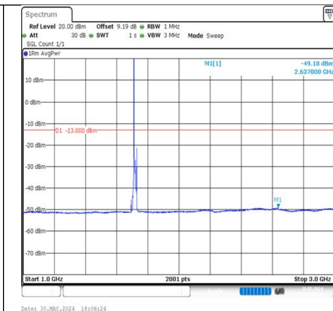
Band4-10MHz-QPSK-20000-1RB#0-1000~3000-PASS
