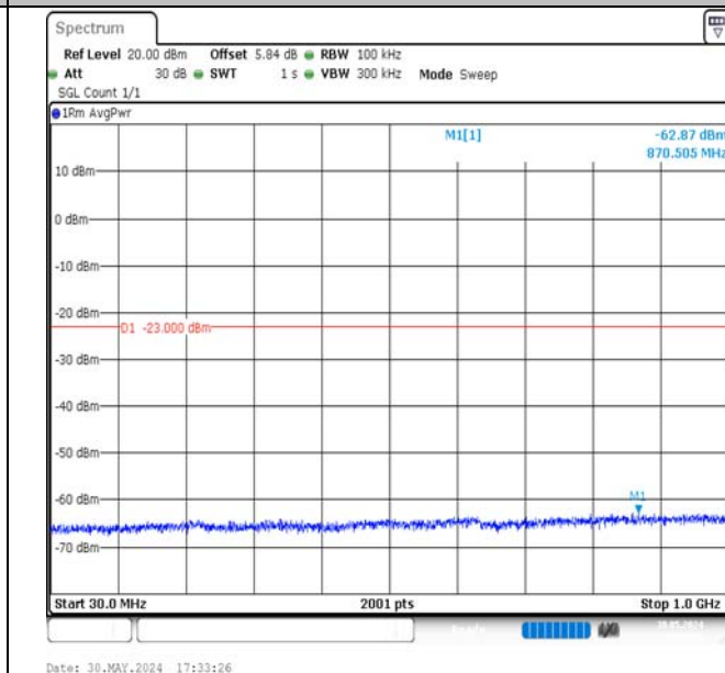
Band4-5MHz-16QAM-19975-1RB#0-30~1000-PASS
