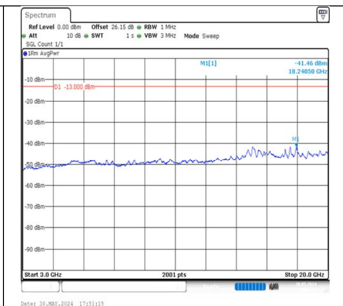
Band4-3MHz-16QAM-20385-1RB#0-3000~20000-PASS
