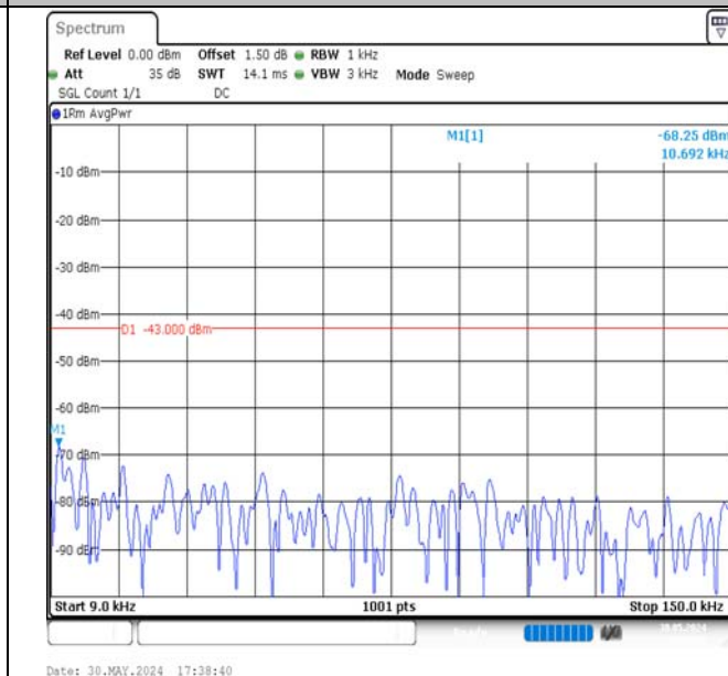
Band4-5MHz-QPSK-20375-25RB#0-0.009~0.15-PASS
