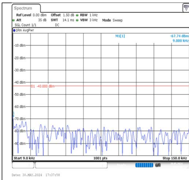
Band4-5MHz-QPSK-20375-1RB#24-0.009~0.15-PASS
