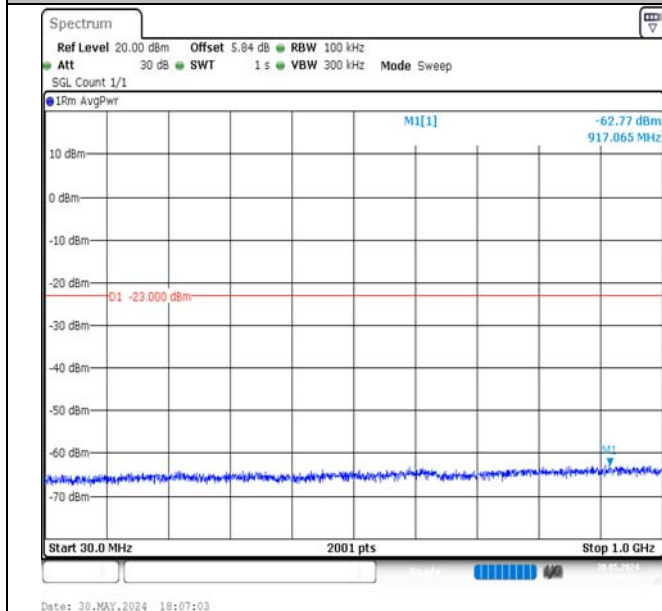
Band4-10MHz-QPSK-20000-1RB#49-30~1000-PASS
