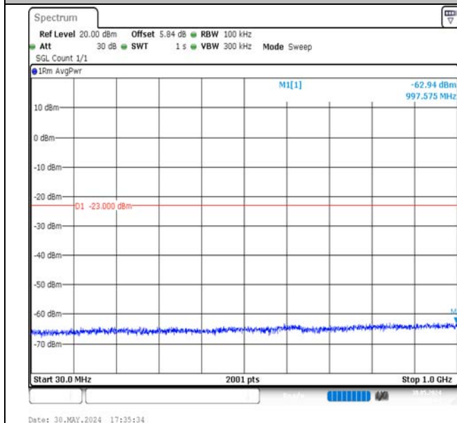
Band4-5MHz-16QAM-20175-1RB#0-30~1000-PASS
