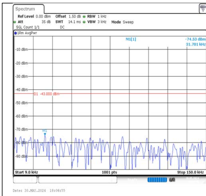
Band4-10MHz-QPSK-20000-1RB#49-0.009~0.15-PASS
