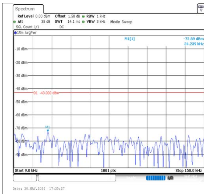
Band4-5MHz-16QAM-20175-1RB#0-0.009~0.15-PASS
