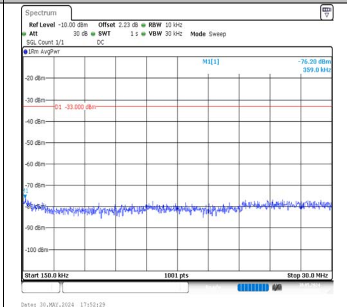
Band4-3MHz-16QAM-20385-15RB#0-0.15~30-PASS
