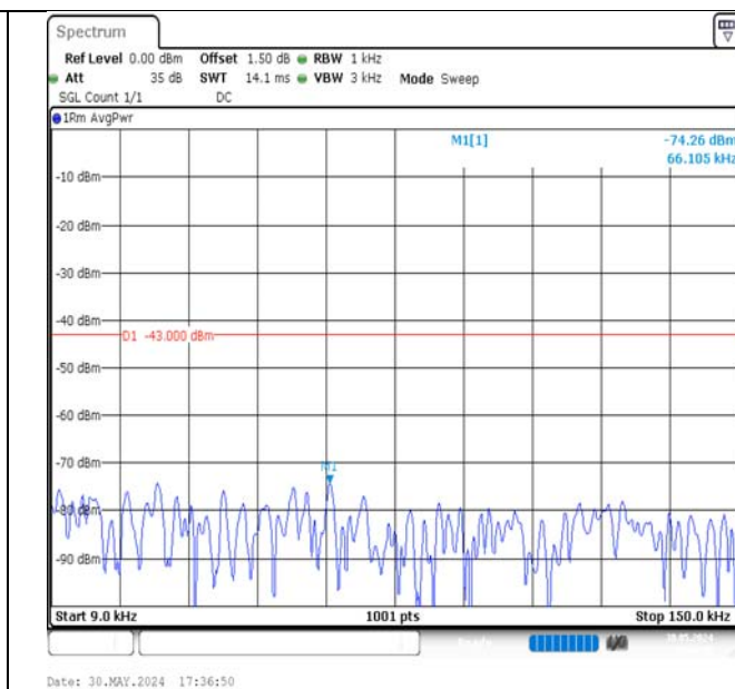
Band4-5MHz-16QAM-20175-25RB#0-0.009~0.15-PASS
