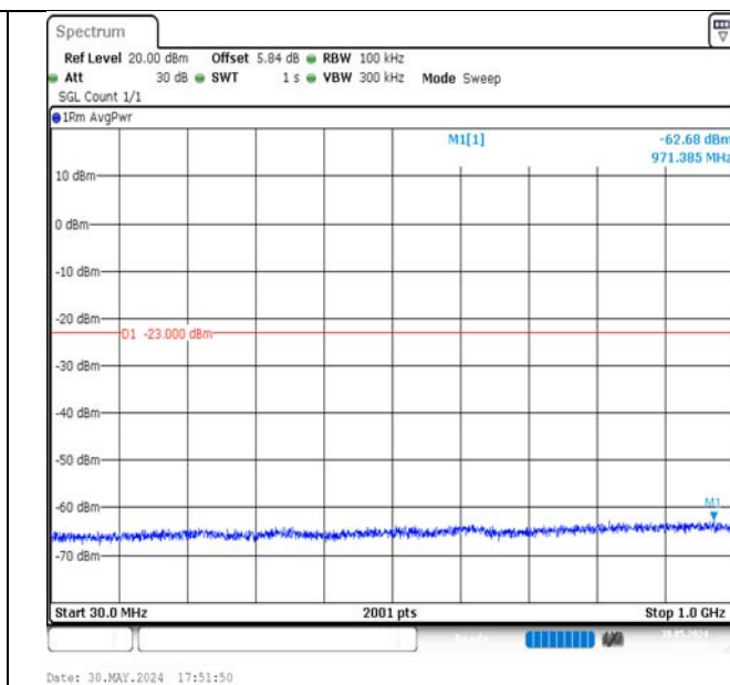
Band4-3MHz-16QAM-20385-1RB#14-30~1000-PASS
