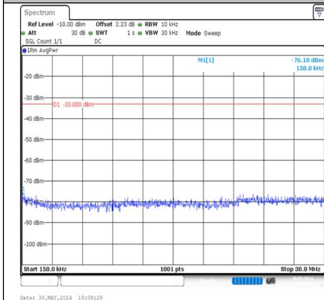
Band4-10MHz-QPSK-20175-1RB#0-0.15~30-PASS
