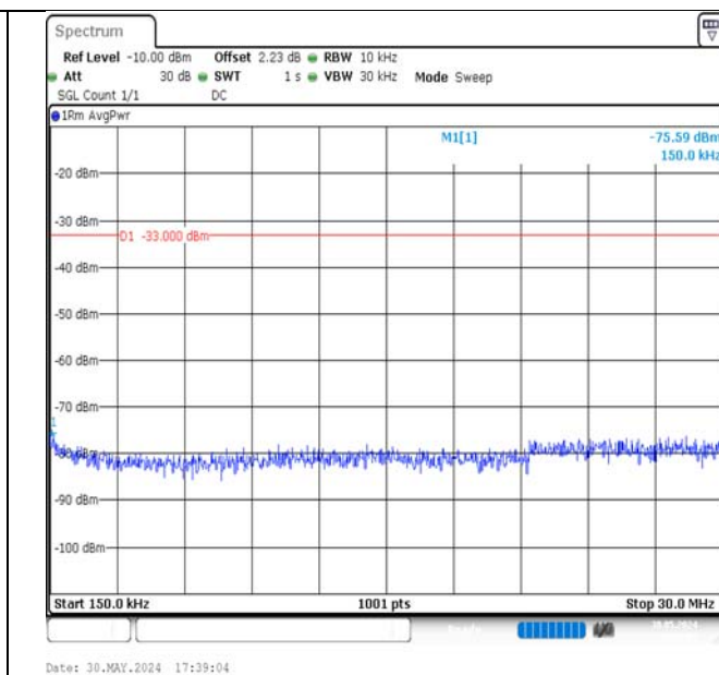
Band4-5MHz-16QAM-20375-25RB#0-0.15~30-PASS
