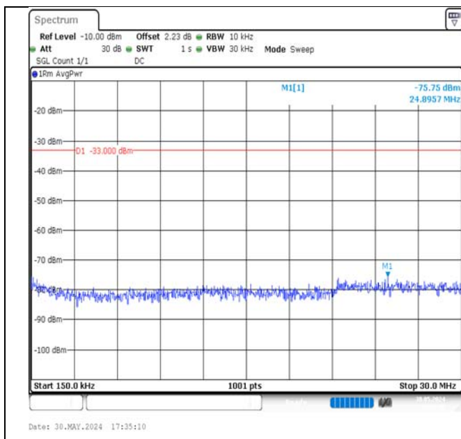
Band4-5MHz-QPSK-20175-1RB#0-0.15~30-PASS
