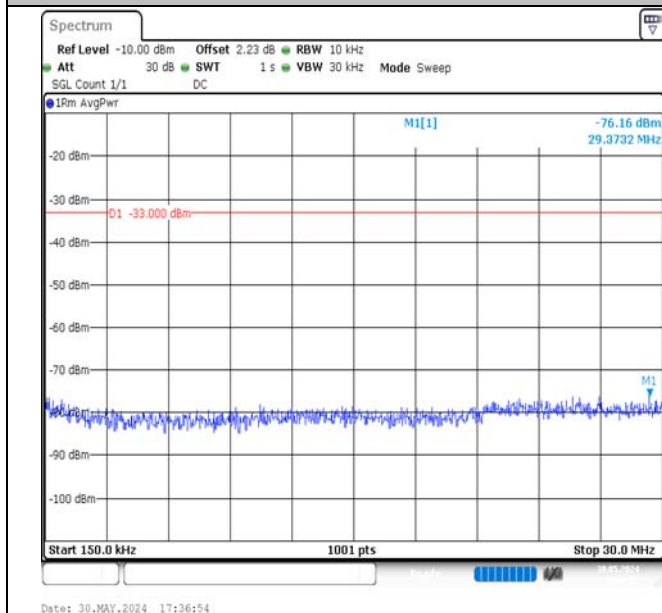
Band4-5MHz-16QAM-20175-25RB#0-0.15~30-PASS
