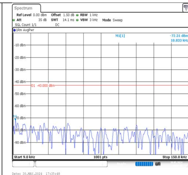
Band4-5MHz-QPSK-20175-1RB#24-0.009~0.15-PASS
