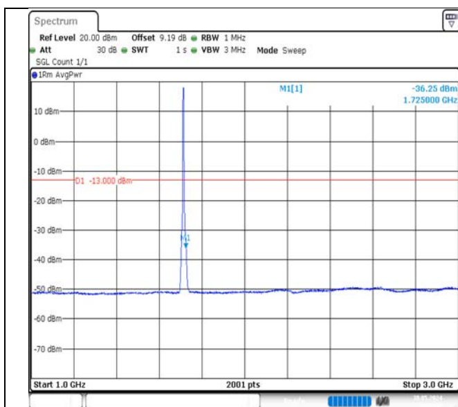
Band4-5MHz-QPSK-19975-25RB#0-1000~3000-PASS
