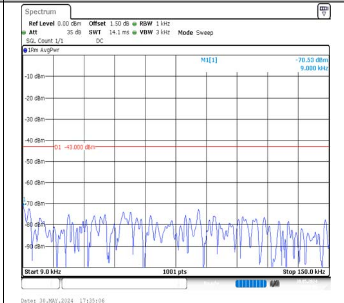
Band4-5MHz-QPSK-20175-1RB#0-0.009~0.15-PASS
