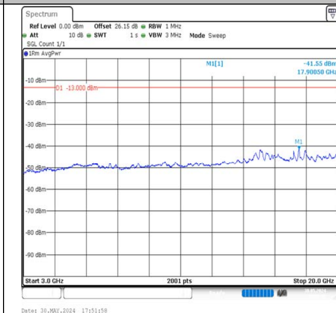
Band4-3MHz-16QAM-20385-1RB#14-3000~20000-PASS
