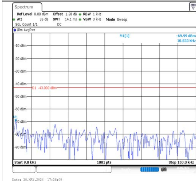
Band4-5MHz-16QAM-20175-1RB#24-0.009~0.15-PASS
