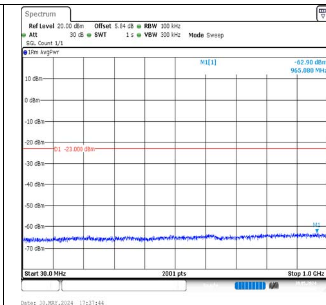
Band4-5MHz-16QAM-20375-1RB#0-30~1000-PASS
