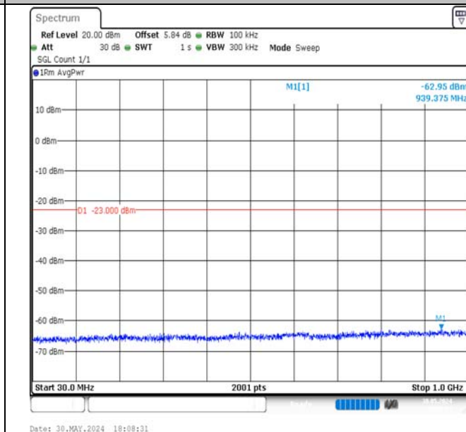
Band4-10MHz-QPSK-20175-1RB#0-30~1000-PASS
