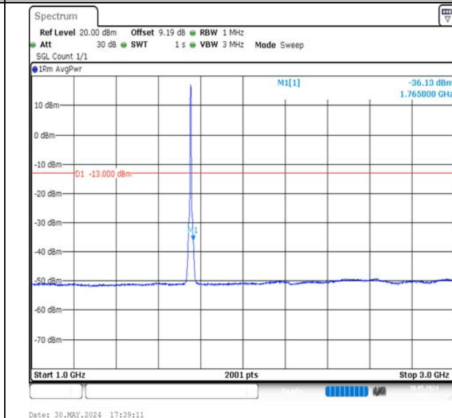
Band4-5MHz-16QAM-20375-25RB#0-1000~3000-PASS
