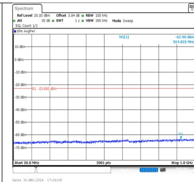
Band4-5MHz-16QAM-19975-1RB#24-30~1000-PASS
