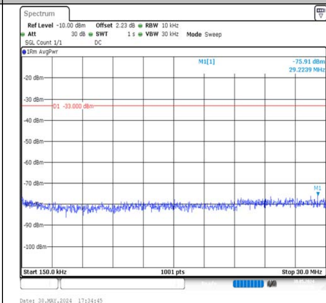
Band4-5MHz-16QAM-19975-25RB#0-0.15~30-PASS
