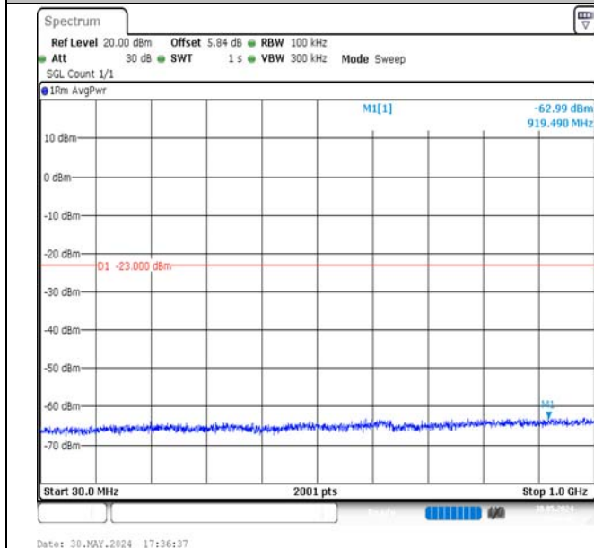
Band4-5MHz-QPSK-20175-25RB#0-30~1000-PASS
