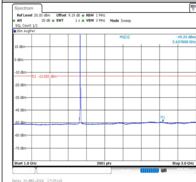
Band4-5MHz-QPSK-20175-1RB#0-1000~3000-PASS
