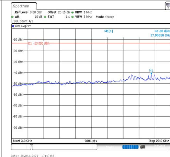
Band4-3MHz-QPSK-19965-15RB#0-3000~20000-PASS
