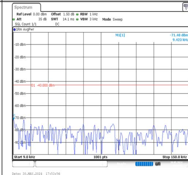
Band4-1.4MHz-16QAM-19957-1RB#5-0.009~0.15-PASS
