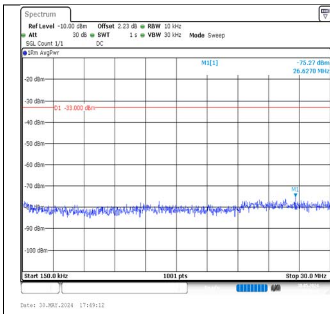
Band4-3MHz-QPSK-20175-1RB#14-0.15~30-PASS
