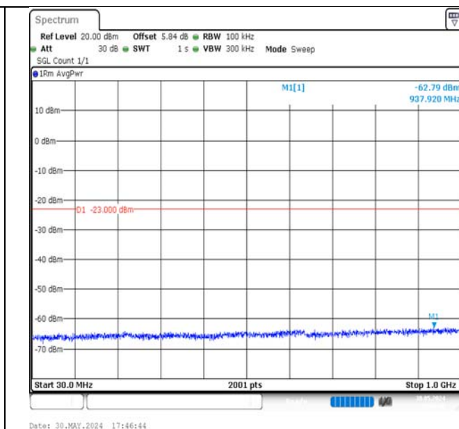
Band4-3MHz-16QAM-19965-1RB#0-30~1000-PASS
