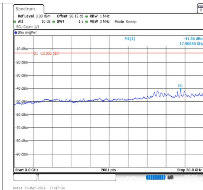
Band4-3MHz-16QAM-19965-1RB#14-3000~20000-PASS
