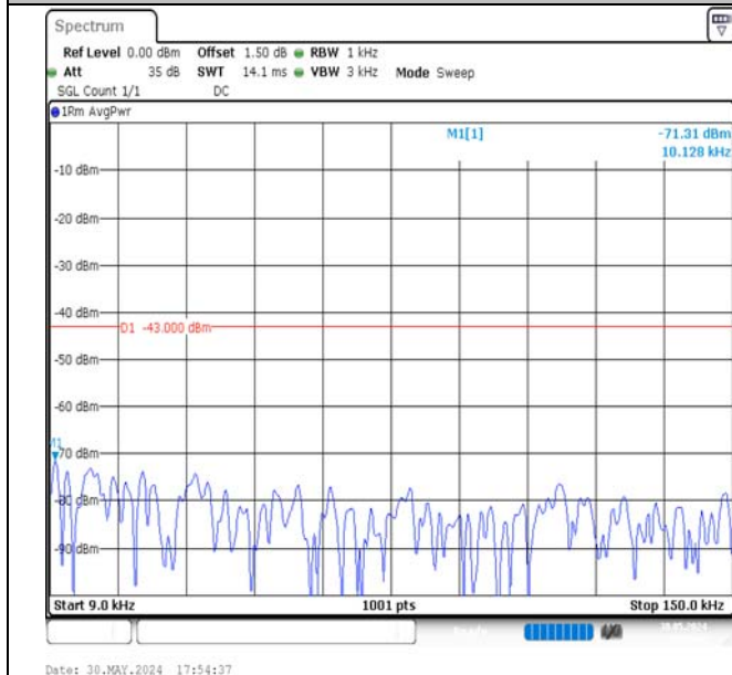
Band4-1.4MHz-16QAM-19957-6RB#0-0.009~0.15-PASS
