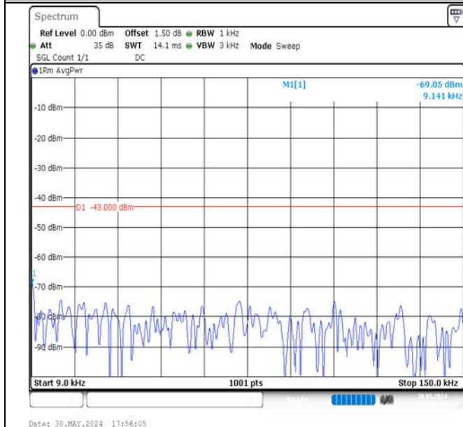
Band4-1.4MHz-16QAM-20175-1RB#5-0.009~0.15-PASS
