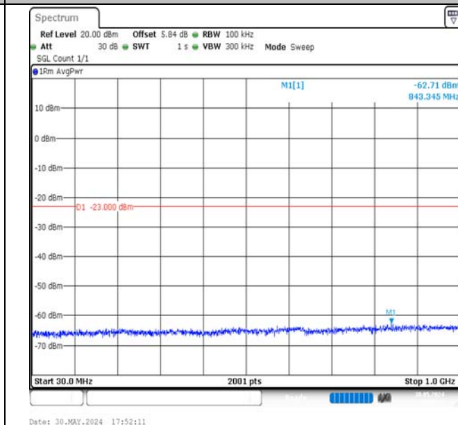
Band4-3MHz-QPSK-20385-15RB#0-30~1000-PASS
