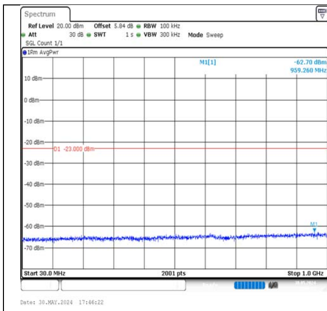
Band4-3MHz-QPSK-19965-1RB#0-30~1000-PASS
