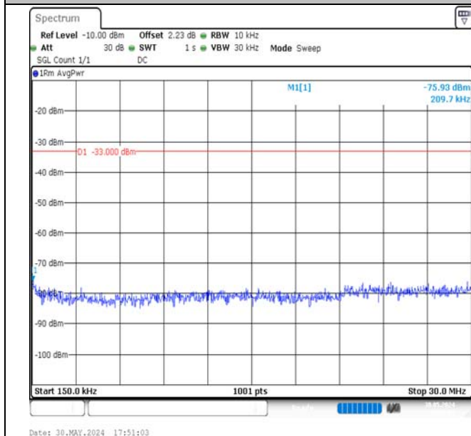
Band4-3MHz-16QAM-20385-1RB#0-0.15~30-PASS
