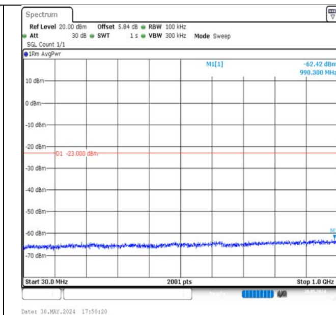
Band4-3MHz-16QAM-20175-15RB#0-30~1000-PASS
