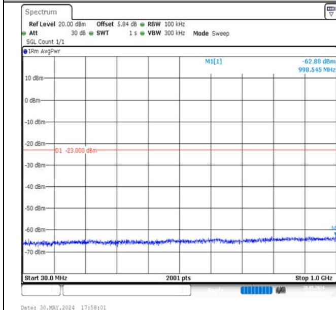
Band4-1.4MHz-QPSK-20393-1RB#5-30~1000-PASS
