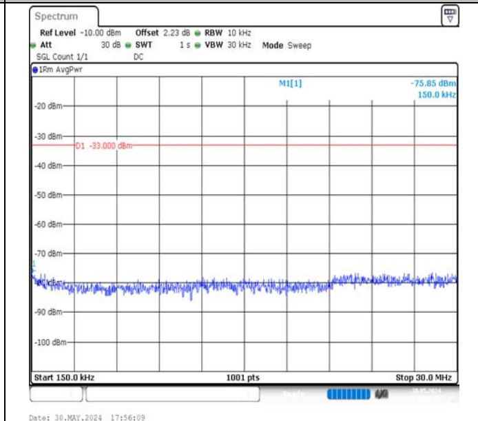
Band4-1.4MHz-16QAM-20175-1RB#5-0.15~30-PASS
