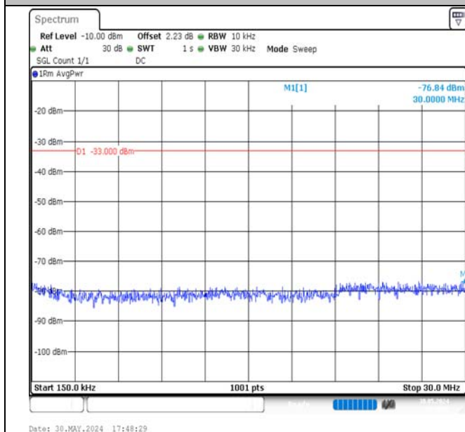
Band4-3MHz-QPSK-20175-1RB#0-0.15~30-PASS
