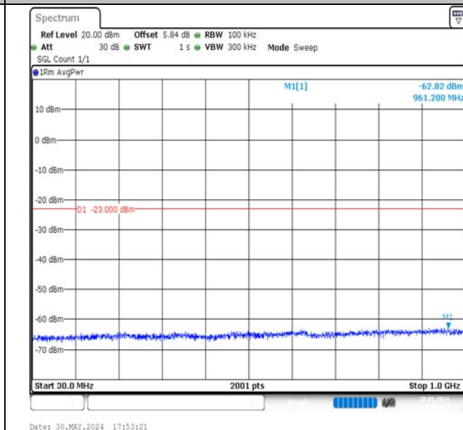
Band4-1.4MHz-16QAM-19957-1RB#0-30~1000-PASS
