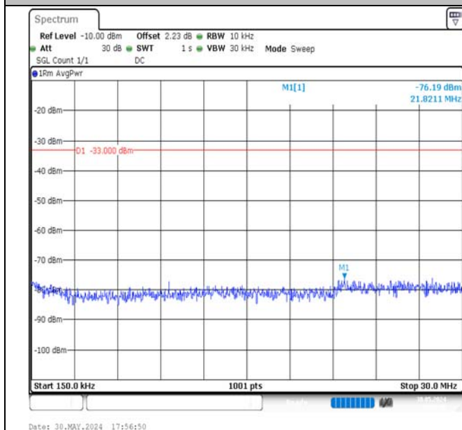
Band4-1.4MHz-16QAM-20175-6RB#0-0.15~30-PASS
