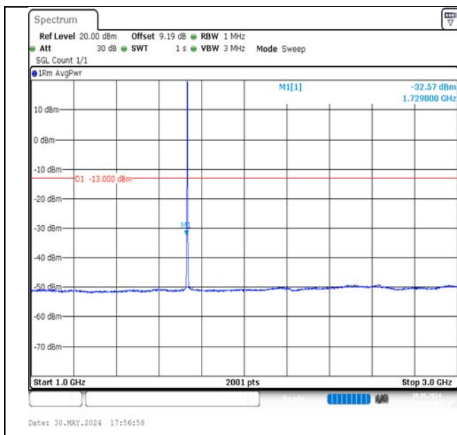
Band4-1.4MHz-16QAM-20175-6RB#0-1000~3000-PASS
