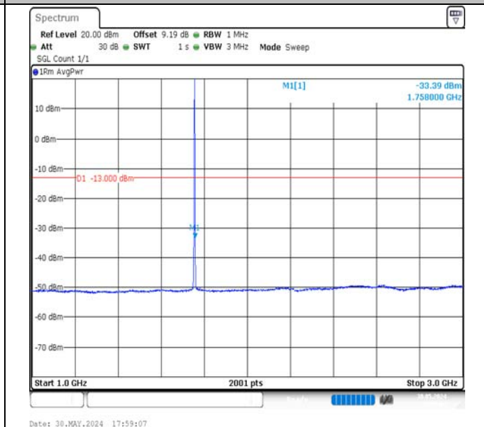
Band4-1.4MHz-16QAM-20393-6RB#0-1000~3000-PASS
