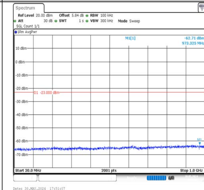
Band4-3MHz-16QAM-20385-1RB#0-30~1000-PASS
