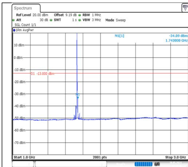
Band4-3MHz-QPSK-20175-1RB#0-1000~3000-PASS
