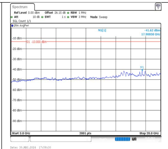
Band4-1.4MHz-16QAM-20393-1RB#5-3000~20000-PASS
