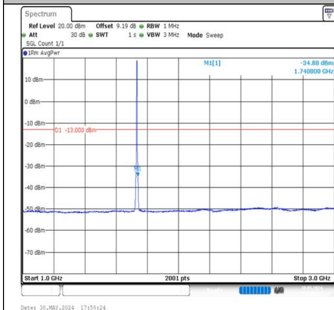
Band4-3MHz-16QAM-20175-15RB#0-1000~3000-PASS
