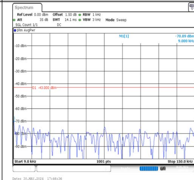
Band4-3MHz-16QAM-19965-1RB#0-0.009~0.15-PASS
