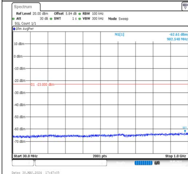
Band4-3MHz-QPSK-19965-1RB#14-30~1000-PASS
