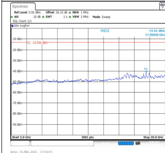
Band4-1.4MHz-16QAM-19957-6RB#0-3000~20000-PASS
