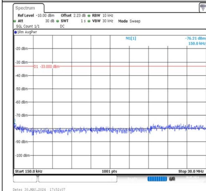
Band4-3MHz-QPSK-20385-15RB#0-0.15~30-PASS
