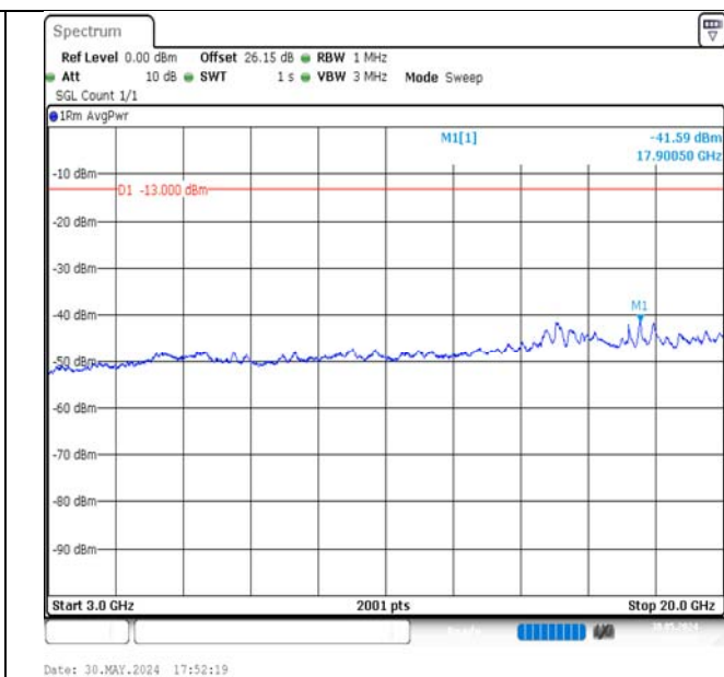
Band4-3MHz-QPSK-20385-15RB#0-3000~20000-PASS
