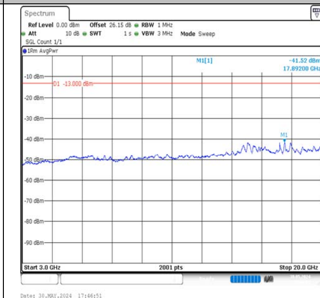
Band4-3MHz-16QAM-19965-1RB#0-3000~20000-PASS
