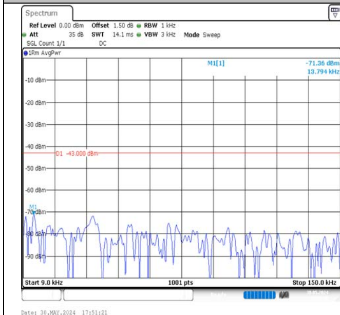
Band4-3MHz-QPSK-20385-1RB#14-0.009~0.15-PASS
