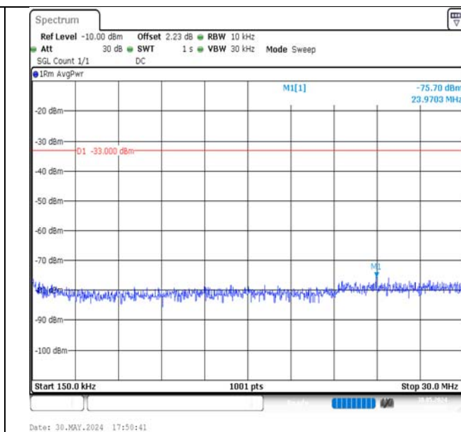
Band4-3MHz-QPSK-20385-1RB#0-0.15~30-PASS
