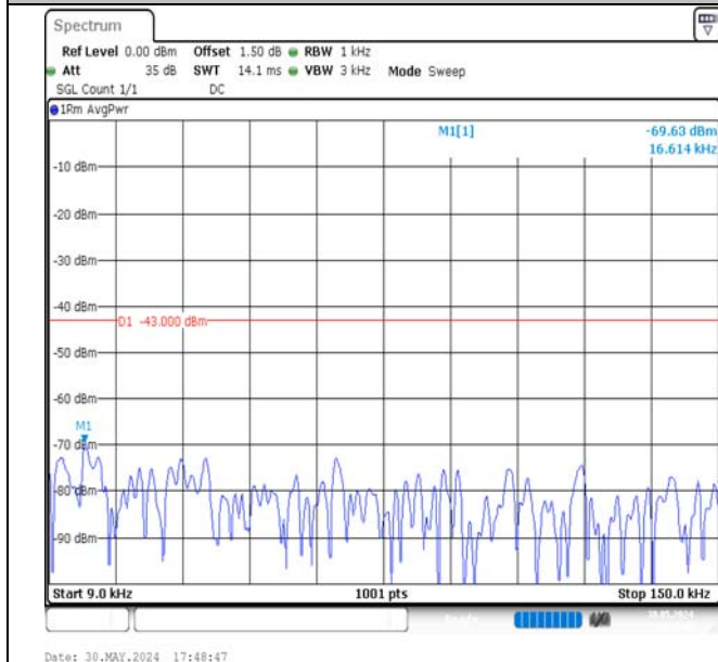
Band4-3MHz-16QAM-20175-1RB#0-0.009~0.15-PASS
