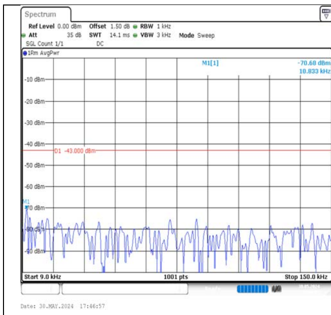
Band4-3MHz-QPSK-19965-1RB#14-0.009~0.15-PASS
