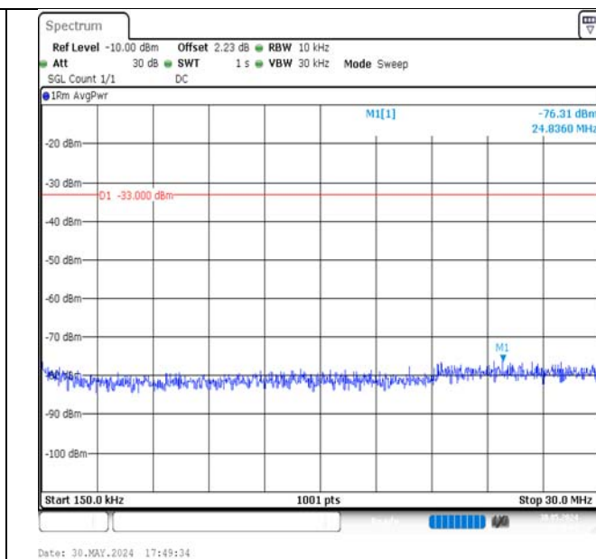
Band4-3MHz-16QAM-20175-1RB#14-0.15~30-PASS
