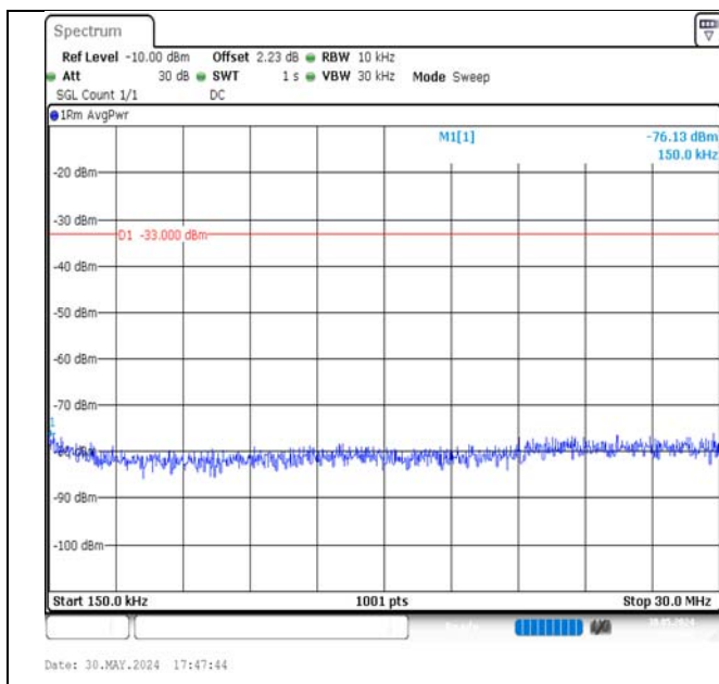
Band4-3MHz-QPSK-19965-15RB#0-0.15~30-PASS
