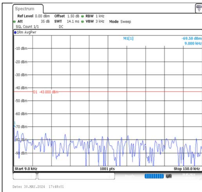
Band4-3MHz-16QAM-19965-15RB#0-0.009~0.15-PASS
