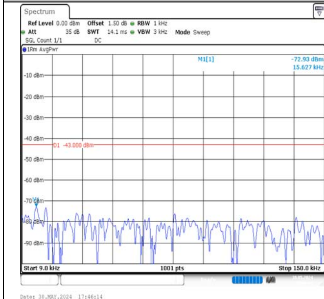
Band4-3MHz-QPSK-19965-1RB#0-0.009~0.15-PASS
