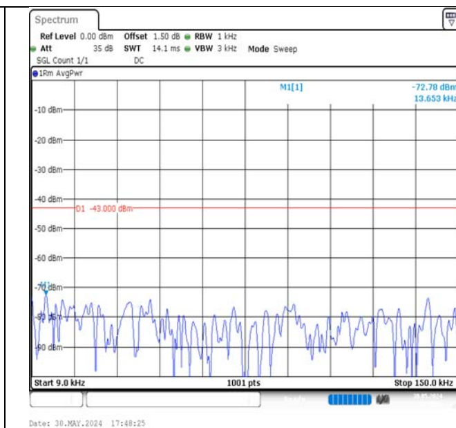
Band4-3MHz-QPSK-20175-1RB#0-0.009~0.15-PASS
