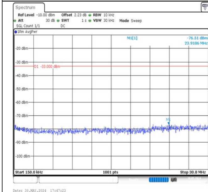
Band4-3MHz-16QAM-19965-1RB#14-0.15~30-PASS
