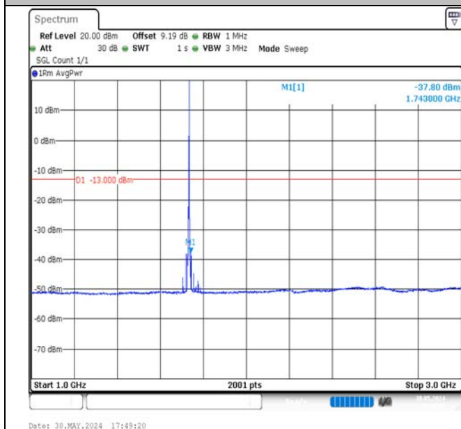
Band4-3MHz-QPSK-20175-1RB#14-1000~3000-PASS
