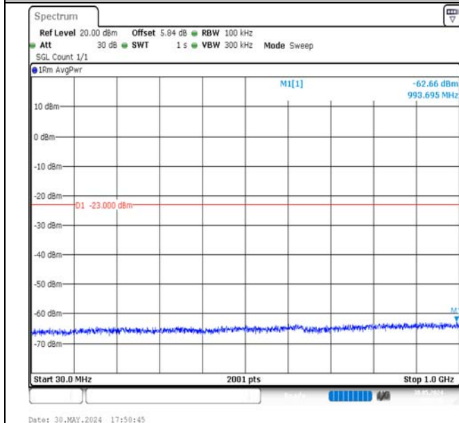
Band4-3MHz-QPSK-20385-1RB#0-30~1000-PASS
