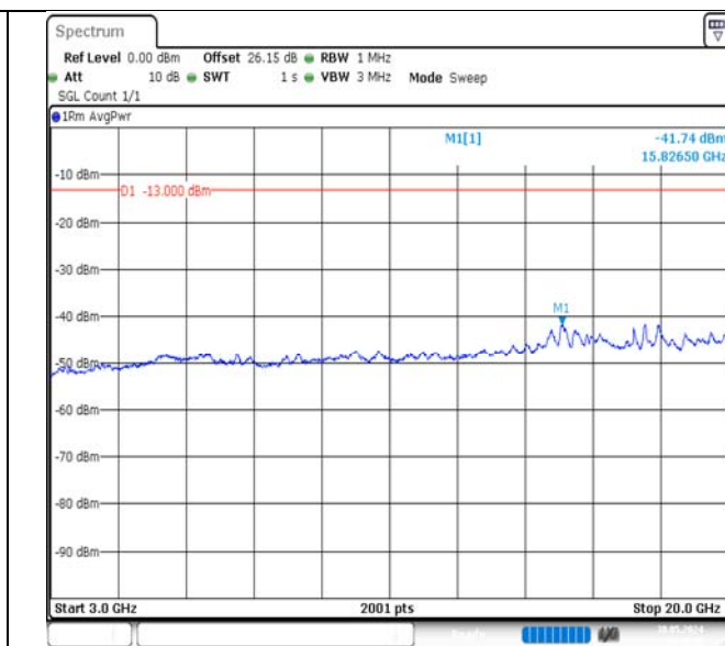
Band4-3MHz-QPSK-20175-1RB#0-3000~20000-PASS
