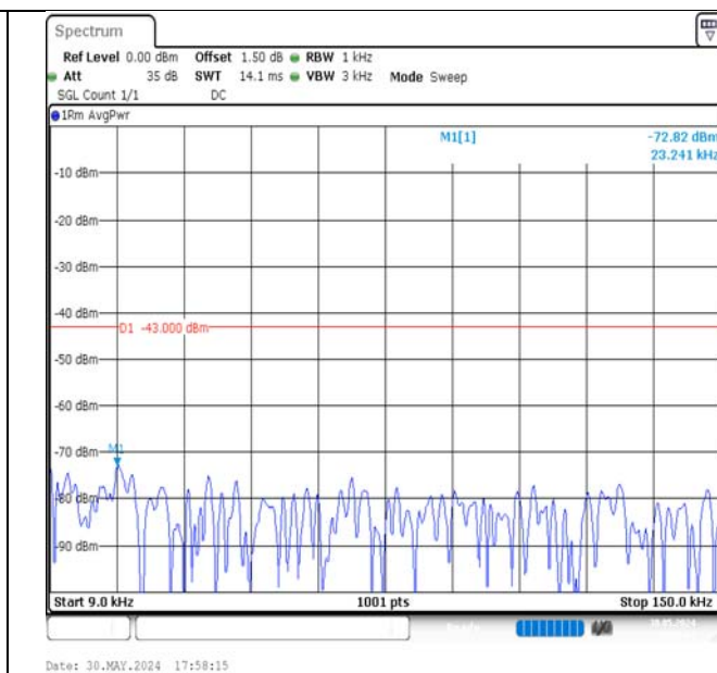
Band4-1.4MHz-16QAM-20393-1RB#5-0.009~0.15-PASS
