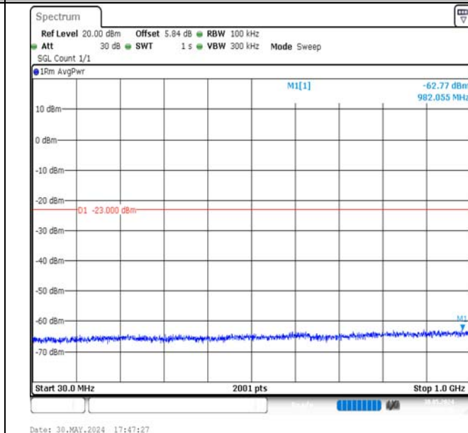
Band4-3MHz-16QAM-19965-1RB#14-30~1000-PASS
