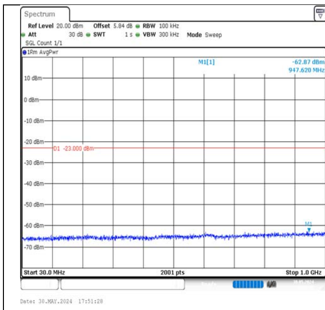
Band4-3MHz-QPSK-20385-1RB#14-30~1000-PASS
