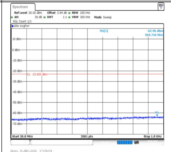
Band4-1.4MHz-16QAM-20175-6RB#0-30~1000-PASS
