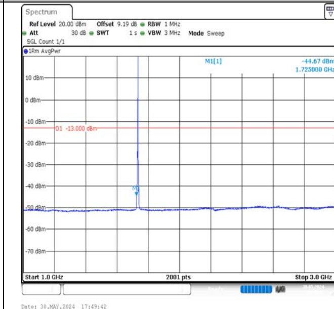
Band4-3MHz-16QAM-20175-1RB#14-1000~3000-PASS
