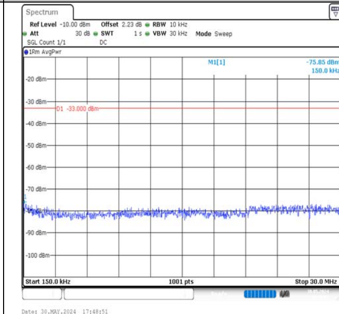
Band4-3MHz-16QAM-20175-1RB#0-0.15~30-PASS
