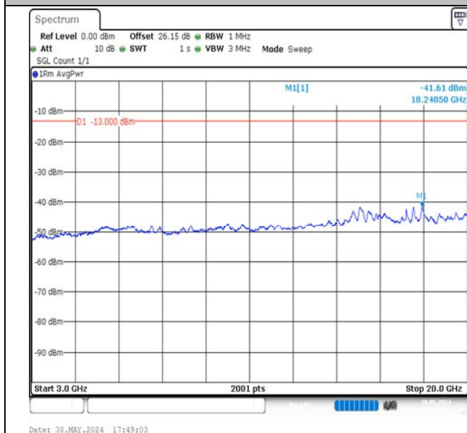
Band4-3MHz-16QAM-20175-1RB#0-3000~20000-PASS
