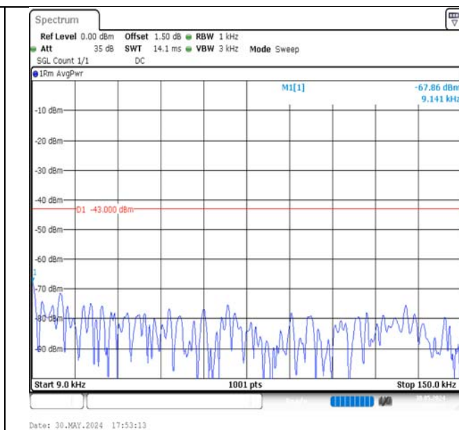
Band4-1.4MHz-16QAM-19957-1RB#0-0.009~0.15-PASS
