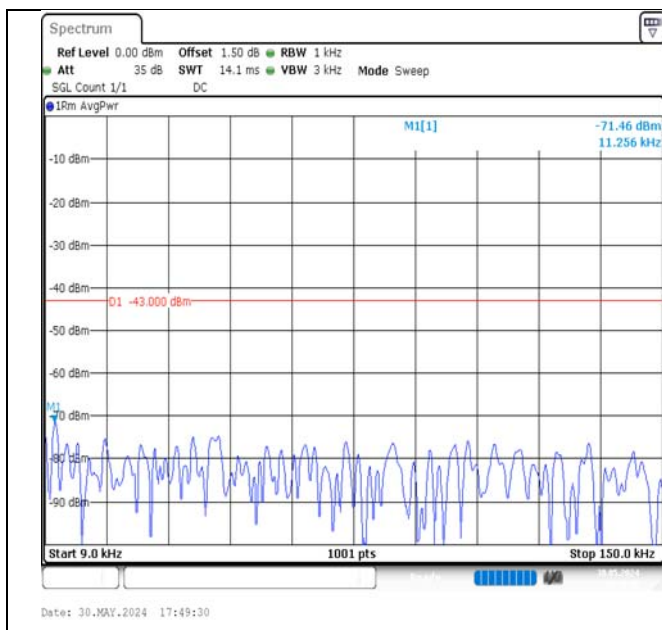
Band4-3MHz-16QAM-20175-1RB#14-0.009~0.15-PASS
