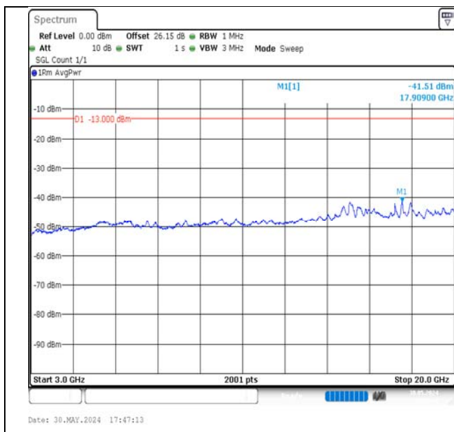
Band4-3MHz-QPSK-19965-1RB#14-3000~20000-PASS
