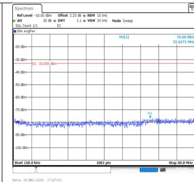
Band4-3MHz-QPSK-19965-1RB#14-0.15~30-PASS
