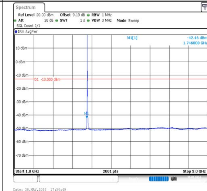
Band4-3MHz-QPSK-20385-1RB#0-1000~3000-PASS
