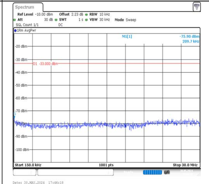
Band4-3MHz-QPSK-19965-1RB#0-0.15~30-PASS
