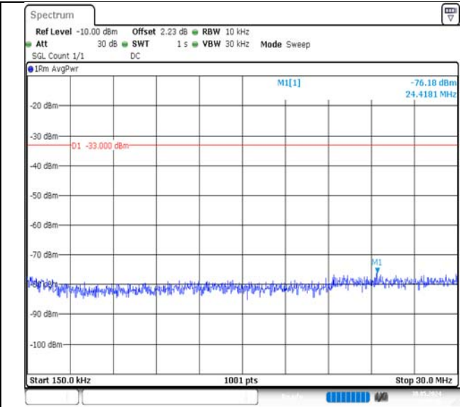
Band4-1.4MHz-16QAM-20393-1RB#0-0.15~30-PASS
