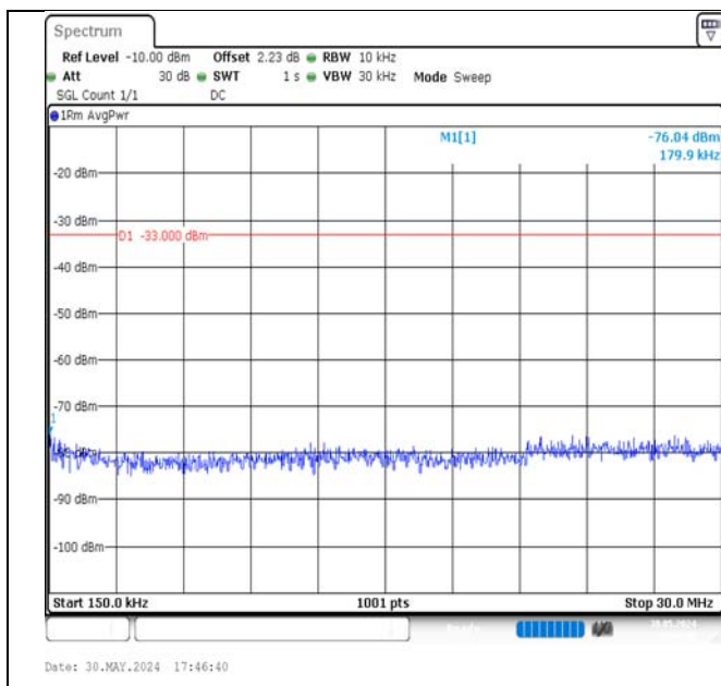
Band4-3MHz-16QAM-19965-1RB#0-0.15~30-PASS
