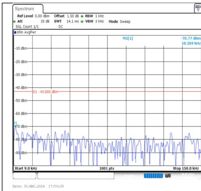
Band4-3MHz-QPSK-20385-1RB#0-0.009~0.15-PASS
