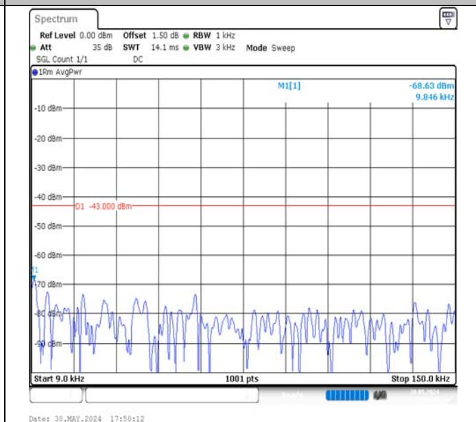
Band4-3MHz-16QAM-20175-15RB#0-0.009~0.15-PASS
