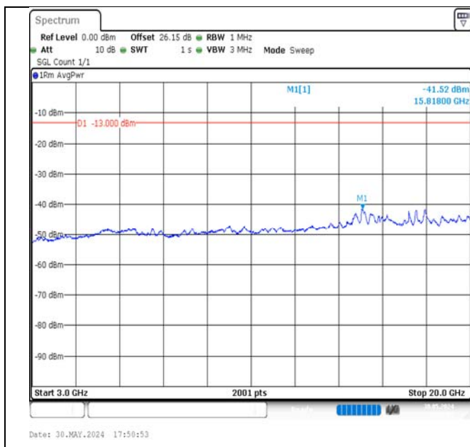
Band4-3MHz-QPSK-20385-1RB#0-3000~20000-PASS
