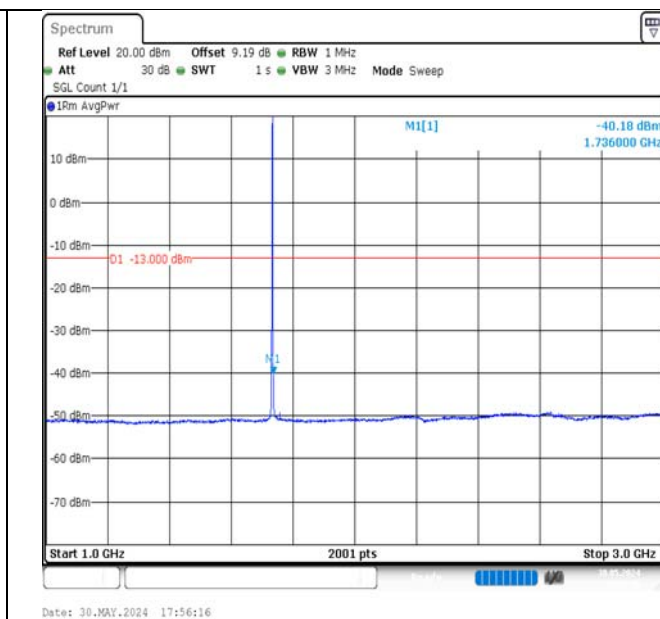
Band4-1.4MHz-16QAM-20175-1RB#5-1000~3000-PASS
