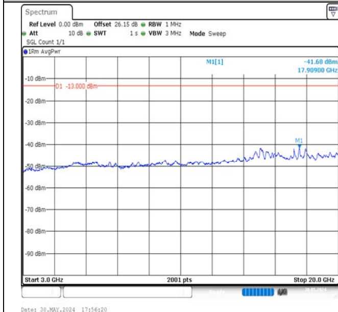
Band4-1.4MHz-16QAM-20175-1RB#5-3000~20000-PASS
