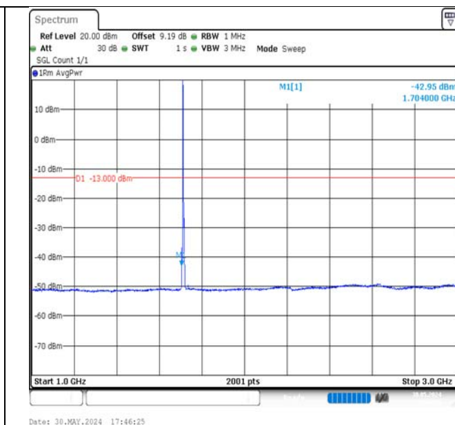
Band4-3MHz-QPSK-19965-1RB#0-1000~3000-PASS
