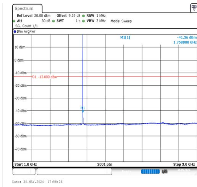
Band4-1.4MHz-16QAM-20393-1RB#5-1000~3000-PASS
