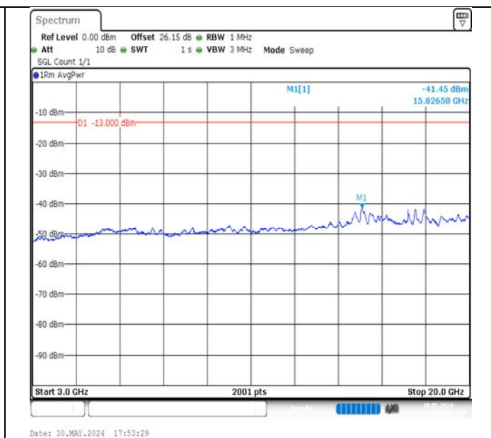
Band4-1.4MHz-16QAM-19957-1RB#0-3000~20000-PASS
