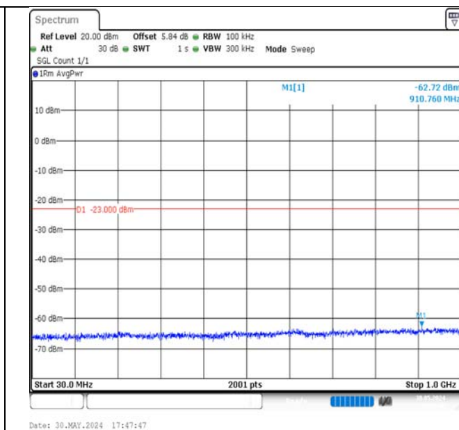
Band4-3MHz-QPSK-19965-15RB#0-30~1000-PASS
