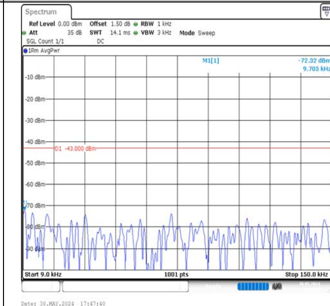
Band4-3MHz-QPSK-19965-15RB#0-0.009~0.15-PASS
