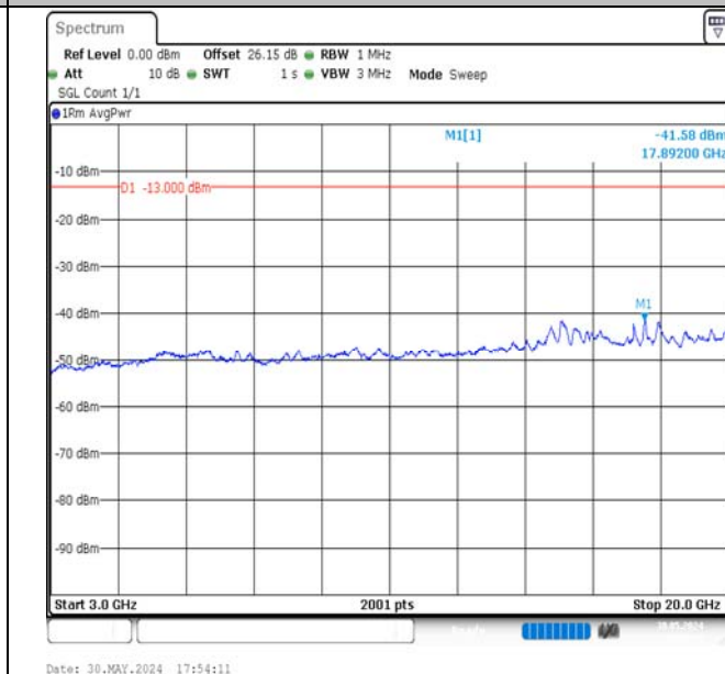
Band4-1.4MHz-16QAM-19957-1RB#5-3000~20000-PASS
