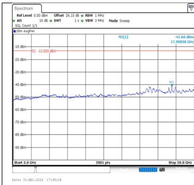
Band4-3MHz-16QAM-19965-15RB#0-3000~20000-PASS
