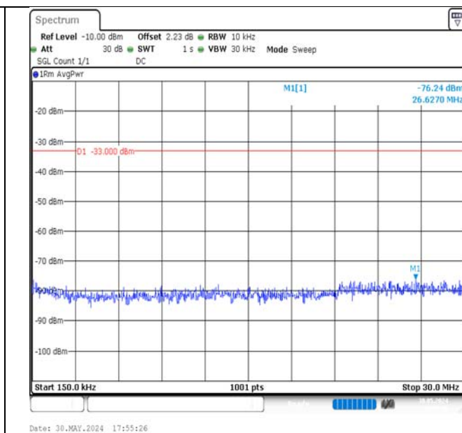
Band4-1.4MHz-16QAM-20175-1RB#0-0.15~30-PASS
