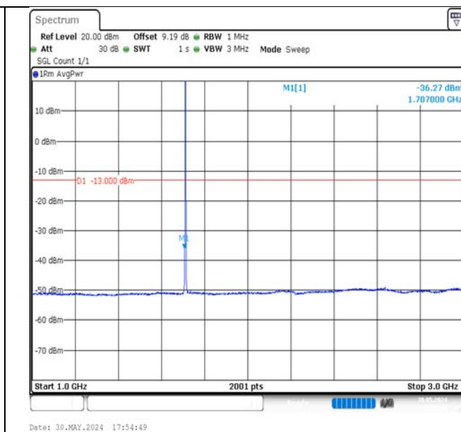
Band4-1.4MHz-16QAM-19957-6RB#0-1000~3000-PASS
