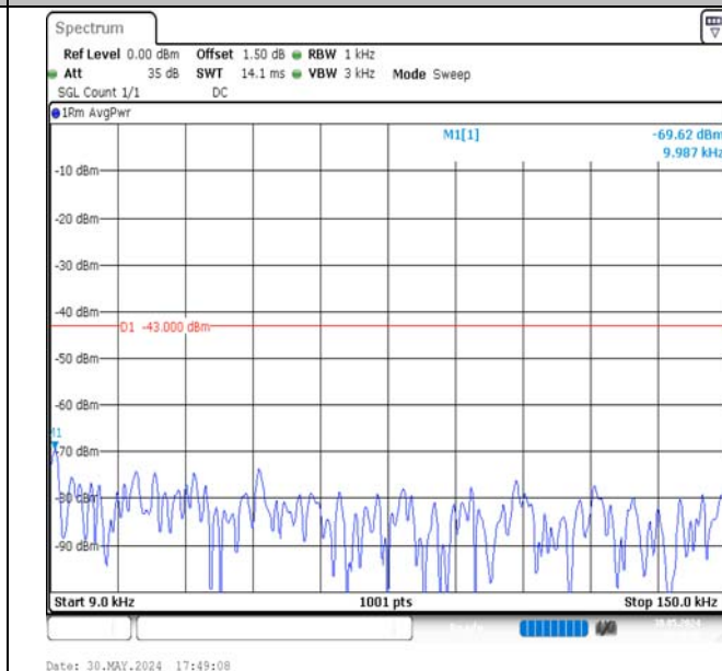
Band4-3MHz-QPSK-20175-1RB#14-0.009~0.15-PASS
