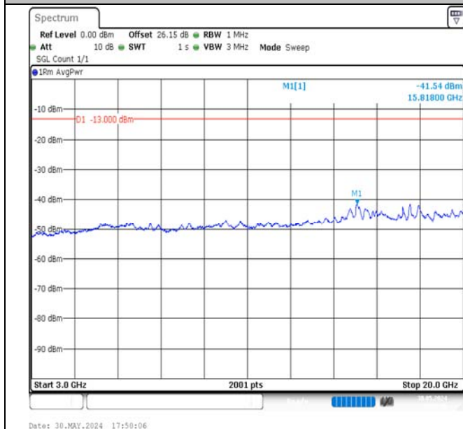
Band4-3MHz-QPSK-20175-15RB#0-3000~20000-PASS
