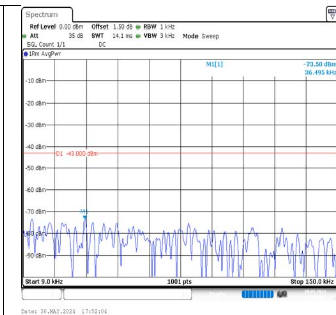
Band4-3MHz-QPSK-20385-15RB#0-0.009~0.15-PASS
