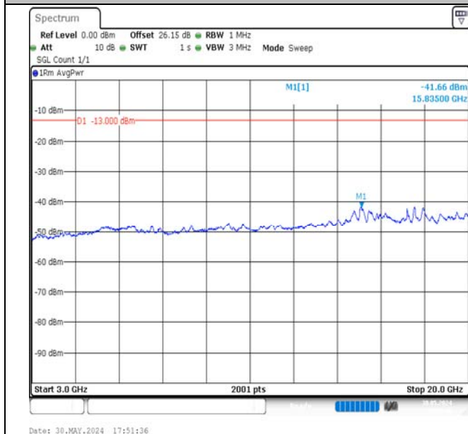
Band4-3MHz-QPSK-20385-1RB#14-3000~20000-PASS
