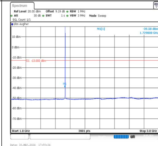
Band4-1.4MHz-16QAM-20175-1RB#0-1000~3000-PASS
