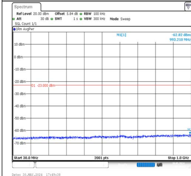
Band4-3MHz-16QAM-20175-1RB#14-30~1000-PASS
