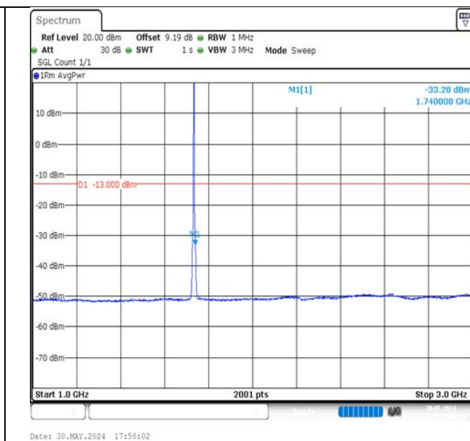
Band4-3MHz-QPSK-20175-15RB#0-1000~3000-PASS
