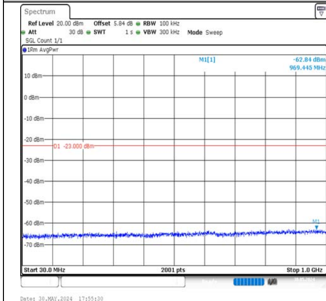
Band4-1.4MHz-16QAM-20175-1RB#0-30~1000-PASS
