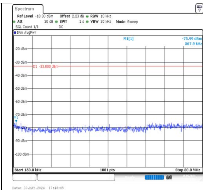
Band4-3MHz-16QAM-19965-15RB#0-0.15~30-PASS
