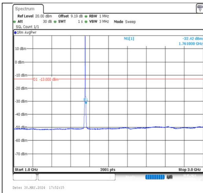
Band4-3MHz-QPSK-20385-15RB#0-1000~3000-PASS
