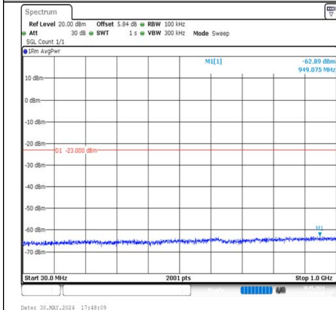
Band4-3MHz-16QAM-19965-15RB#0-30~1000-PASS
