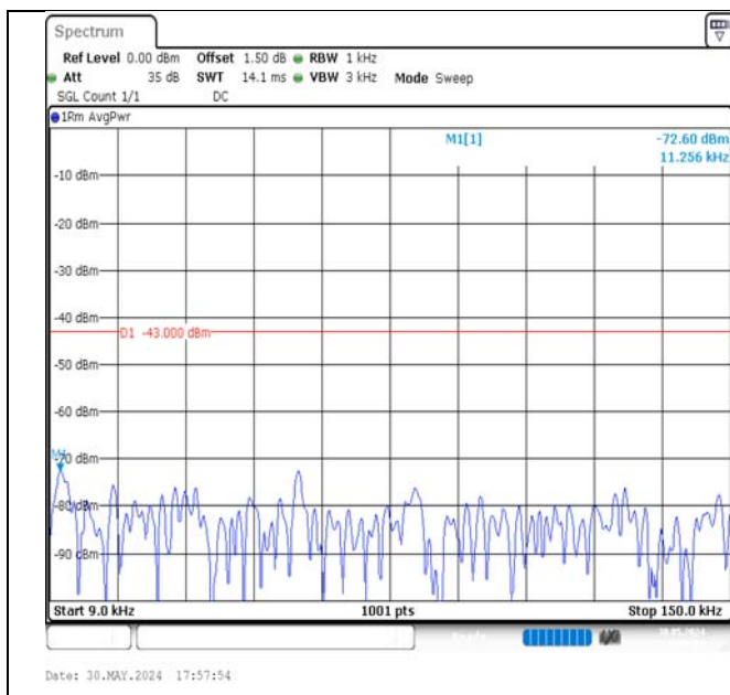
Band4-1.4MHz-QPSK-20393-1RB#5-0.009~0.15-PASS
