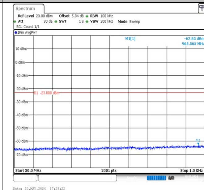
Band4-1.4MHz-16QAM-20393-1RB#5-30~1000-PASS
