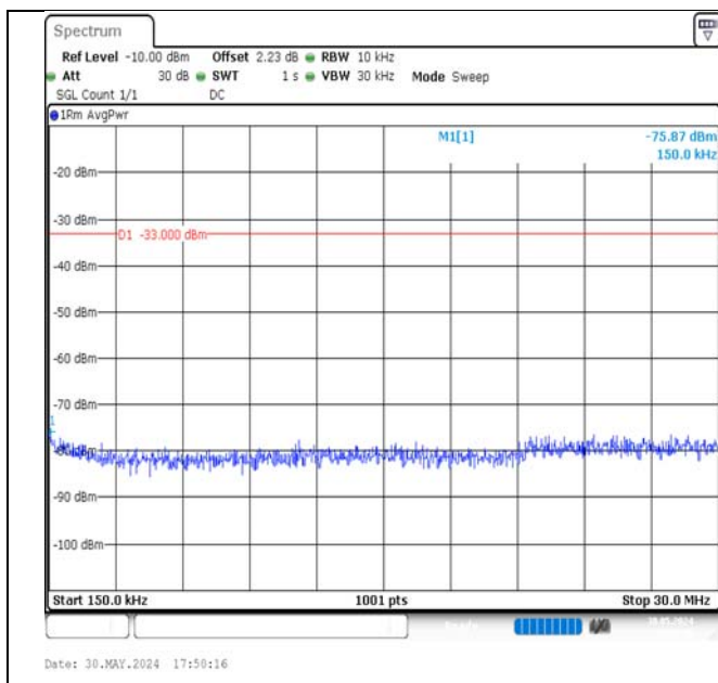
Band4-3MHz-16QAM-20175-15RB#0-0.15~30-PASS
