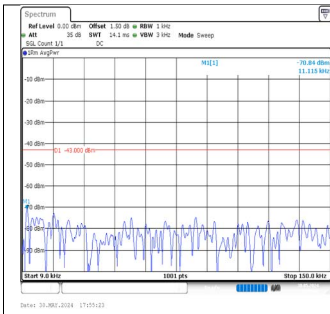
Band4-1.4MHz-16QAM-20175-1RB#0-0.009~0.15-PASS
