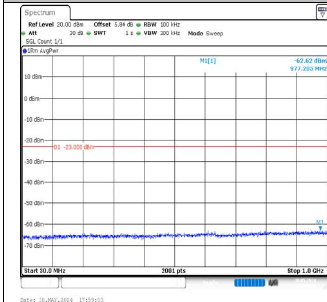
Band4-1.4MHz-16QAM-20393-6RB#0-30~1000-PASS
