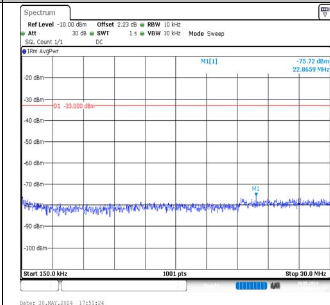
Band4-3MHz-QPSK-20385-1RB#14-0.15~30-PASS
