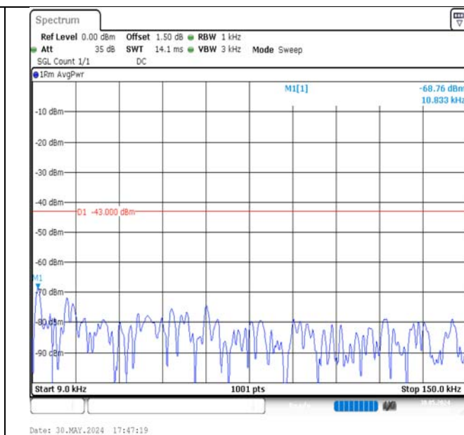
Band4-3MHz-16QAM-19965-1RB#14-0.009~0.15-PASS
