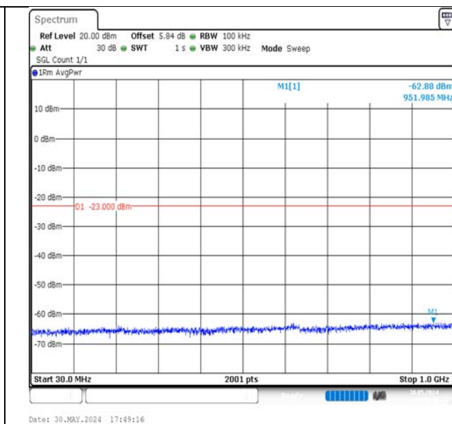
Band4-3MHz-QPSK-20175-1RB#14-30~1000-PASS
