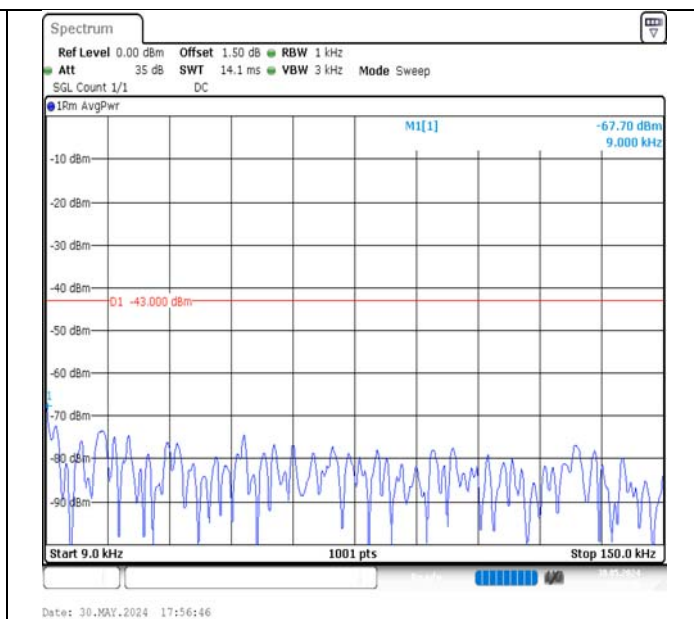
Band4-1.4MHz-16QAM-20175-6RB#0-0.009~0.15-PASS
