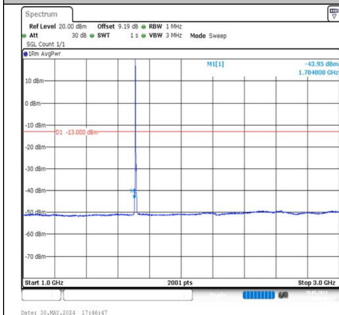
Band4-3MHz-16QAM-19965-1RB#0-1000~3000-PASS
