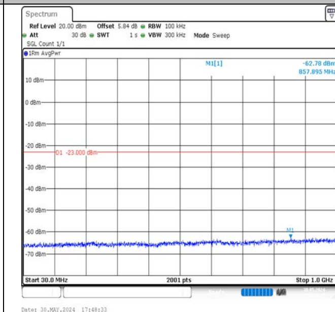
Band4-3MHz-QPSK-20175-1RB#0-30~1000-PASS
