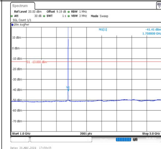
Band4-1.4MHz-QPSK-20393-1RB#5-1000~3000-PASS
