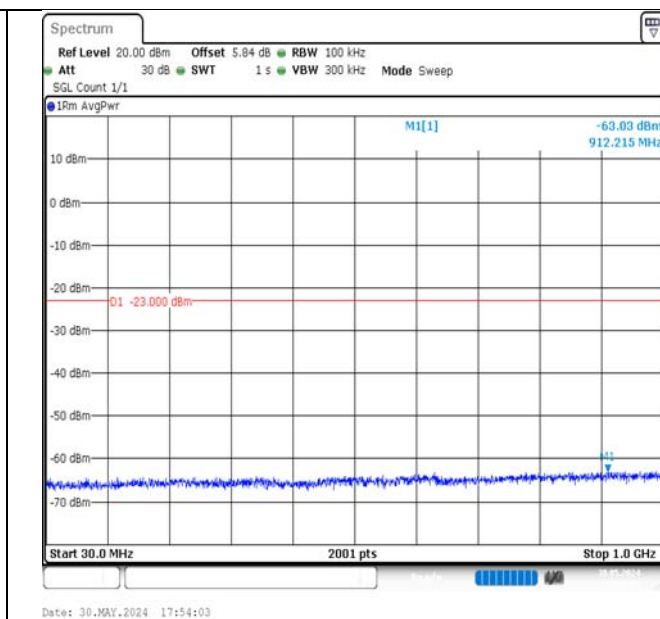
Band4-1.4MHz-16QAM-19957-1RB#5-30~1000-PASS
