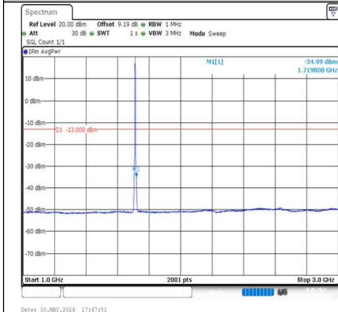
Band4-3MHz-QPSK-19965-15RB#0-1000~3000-PASS
