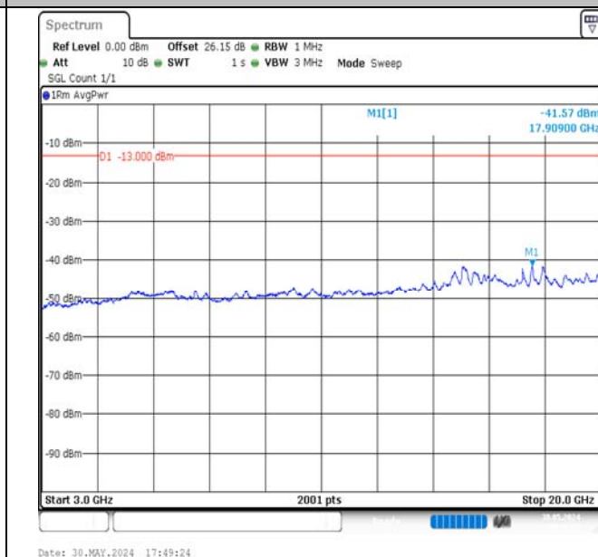
Band4-3MHz-QPSK-20175-1RB#14-3000~20000-PASS
