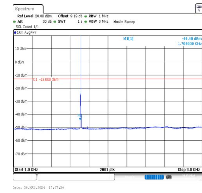
Band4-3MHz-16QAM-19965-1RB#14-1000~3000-PASS
