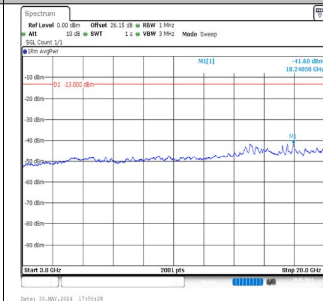
Band4-3MHz-16QAM-20175-15RB#0-3000~20000-PASS
