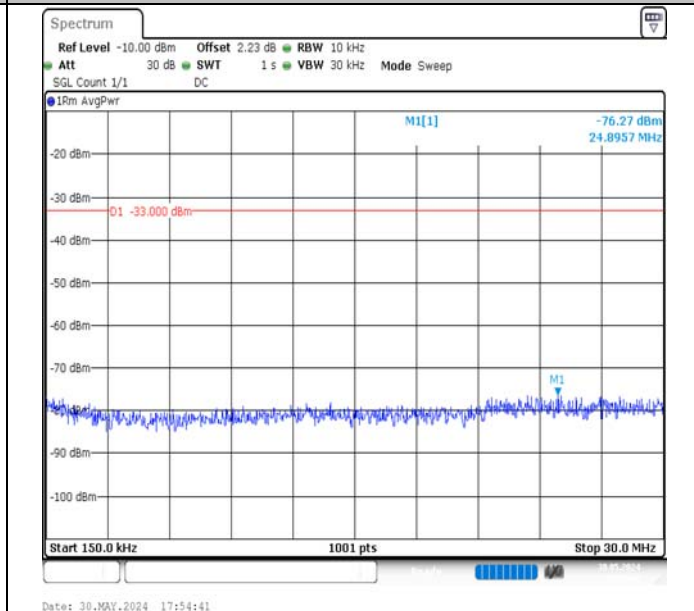
Band4-1.4MHz-16QAM-19957-6RB#0-0.15~30-PASS
