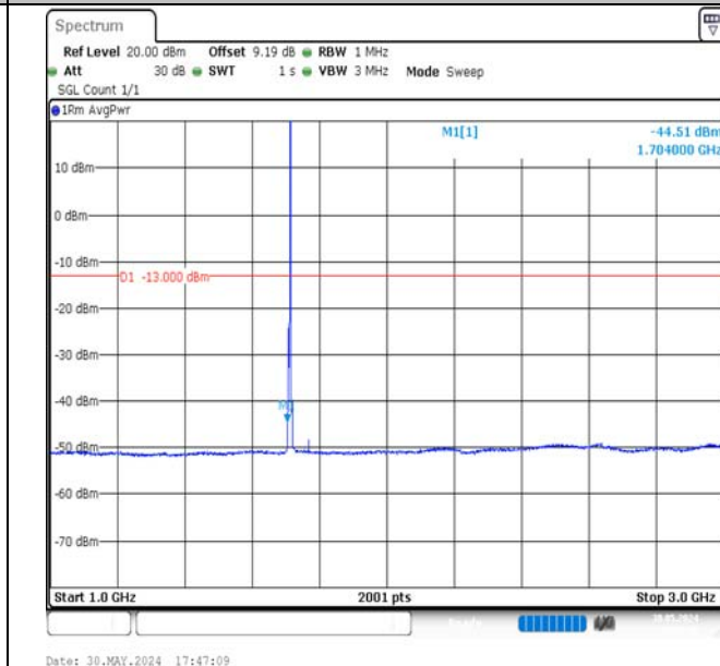
Band4-3MHz-QPSK-19965-1RB#14-1000~3000-PASS
