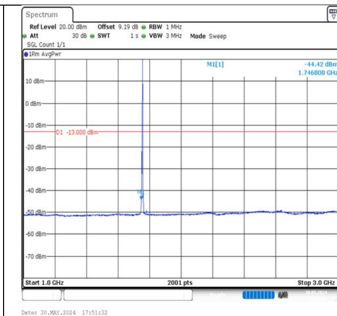
Band4-3MHz-QPSK-20385-1RB#14-1000~3000-PASS
