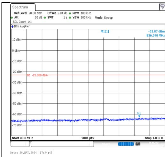
Band4-1.4MHz-16QAM-19957-6RB#0-30~1000-PASS
