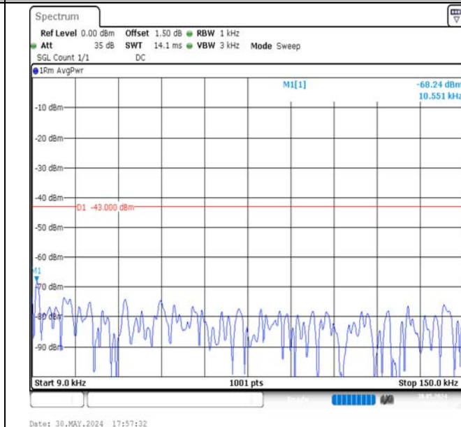
Band4-1.4MHz-16QAM-20393-1RB#0-0.009~0.15-PASS
