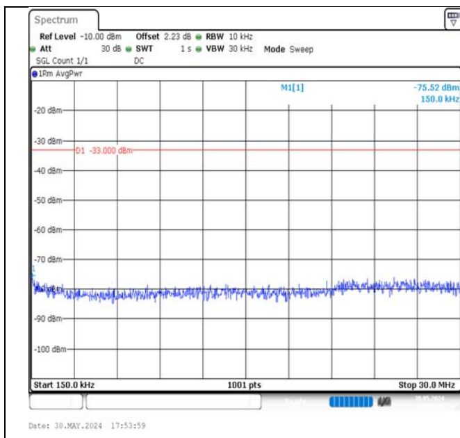
Band4-1.4MHz-16QAM-19957-1RB#5-0.15~30-PASS
