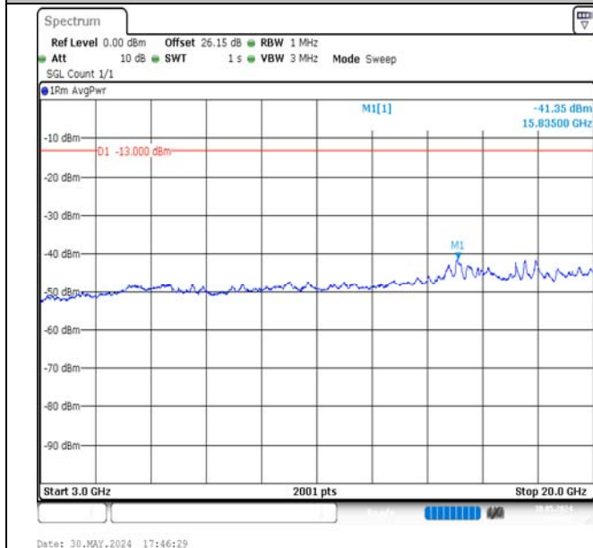
Band4-3MHz-QPSK-19965-1RB#0-3000~20000-PASS
