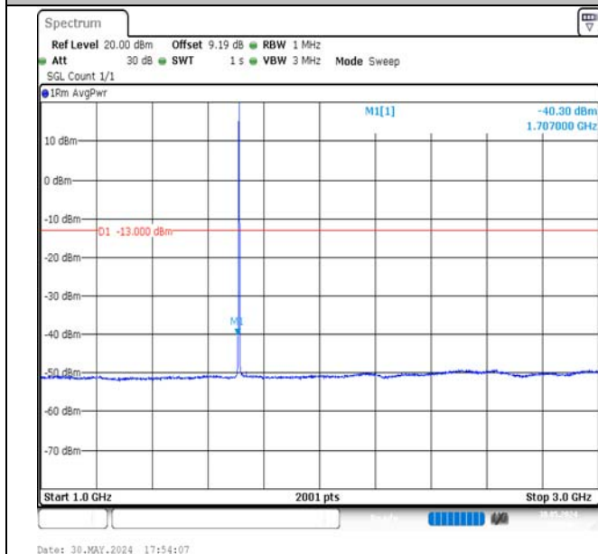
Band4-1.4MHz-16QAM-19957-1RB#5-1000~3000-PASS
