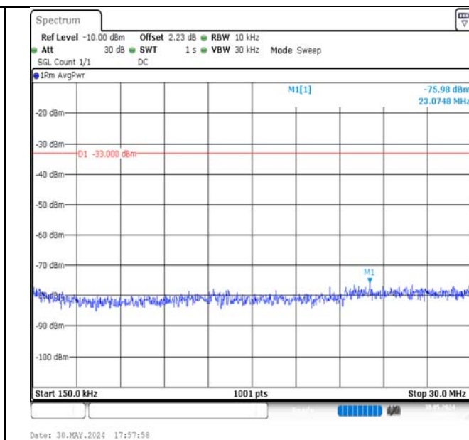
Band4-1.4MHz-QPSK-20393-1RB#5-0.15~30-PASS
