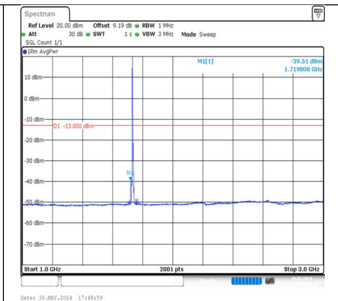
Band4-3MHz-16QAM-20175-1RB#0-1000~3000-PASS
