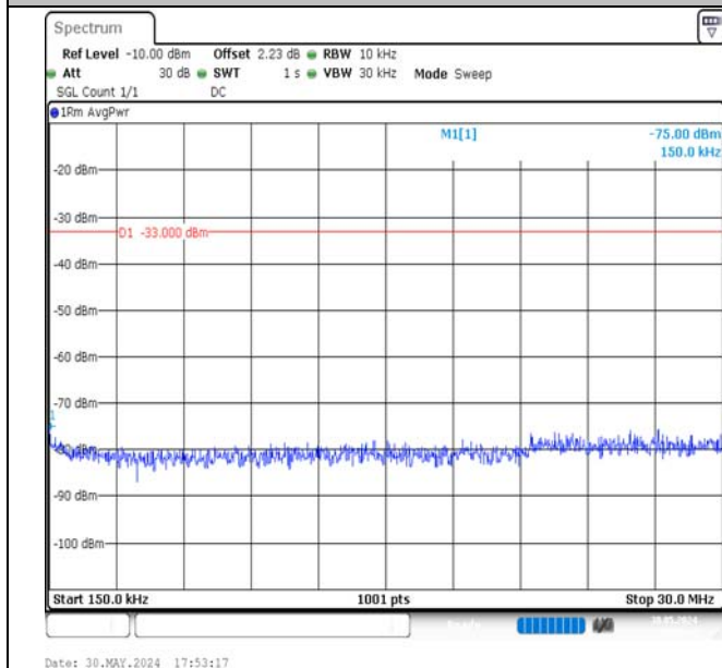
Band4-1.4MHz-16QAM-19957-1RB#0-0.15~30-PASS
