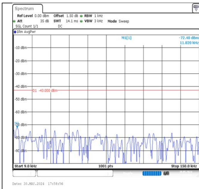
Band4-1.4MHz-16QAM-20393-6RB#0-0.009~0.15-PASS
