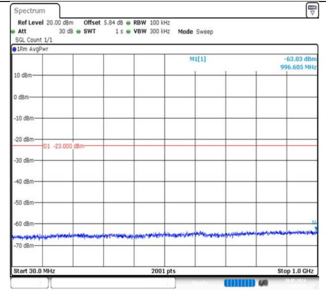
Band4-1.4MHz-16QAM-20393-1RB#0-30~1000-PASS
