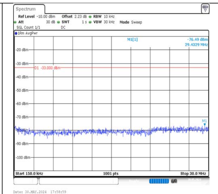
Band4-1.4MHz-16QAM-20393-6RB#0-0.15~30-PASS
