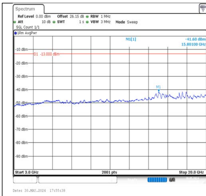
Band4-1.4MHz-16QAM-20175-1RB#0-3000~20000-PASS
