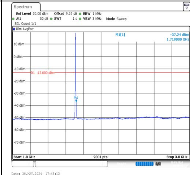
Band4-3MHz-16QAM-19965-15RB#0-1000~3000-PASS
