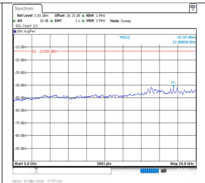
Band4-1.4MHz-16QAM-20175-6RB#0-3000~20000-PASS
