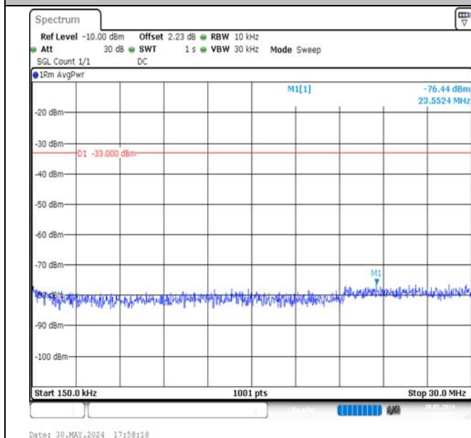
Band4-1.4MHz-16QAM-20393-1RB#5-0.15~30-PASS
