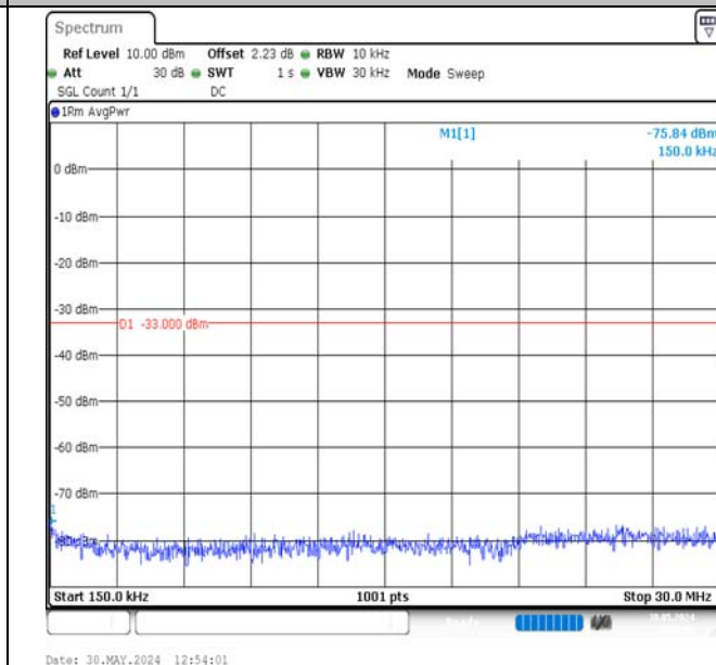
Band2-15MHz-QPSK-18675-1RB#74-0.15~30-PASS
