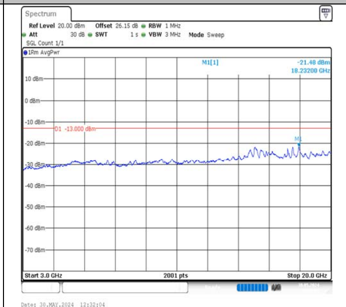
Band2-10MHz-16QAM-19150-1RB#49-3000~20000-PASS
