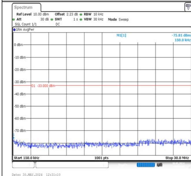
Band2-10MHz-16QAM-19150-1RB#0-0.15~30-PASS
