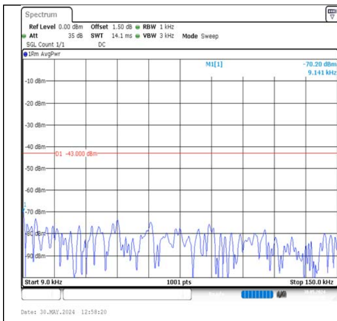
Band2-15MHz-QPSK-19125-1RB#74-0.009~0.15-PASS
