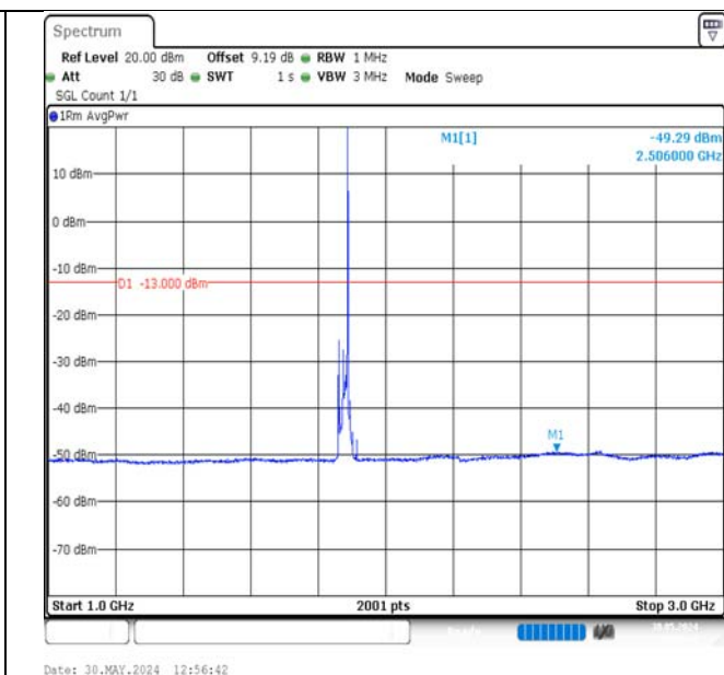
Band2-15MHz-16QAM-18900-1RB#74-1000~3000-PASS
