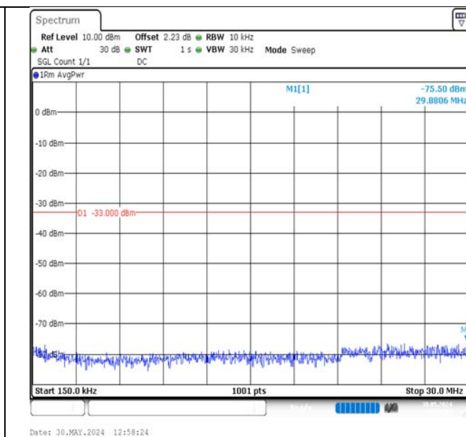
Band2-15MHz-QPSK-19125-1RB#74-0.15~30-PASS
