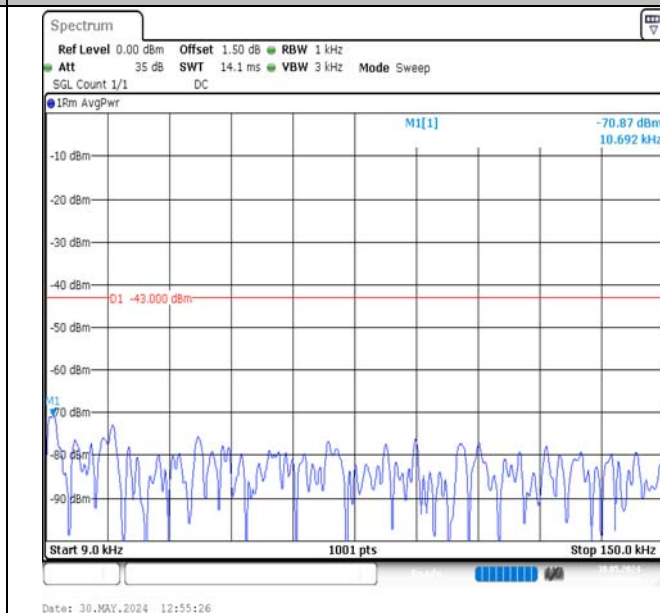
Band2-15MHz-QPSK-18900-1RB#0-0.009~0.15-PASS
