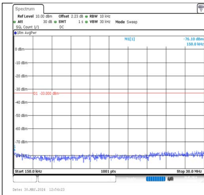
Band2-15MHz-16QAM-18675-1RB#74-0.15~30-PASS
