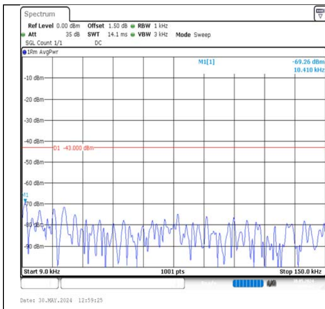
Band2-15MHz-16QAM-19125-75RB#0-0.009~0.15-PASS
