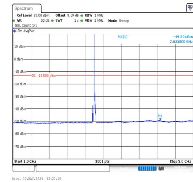
Band2-10MHz-16QAM-19150-1RB#0-1000~3000-PASS
