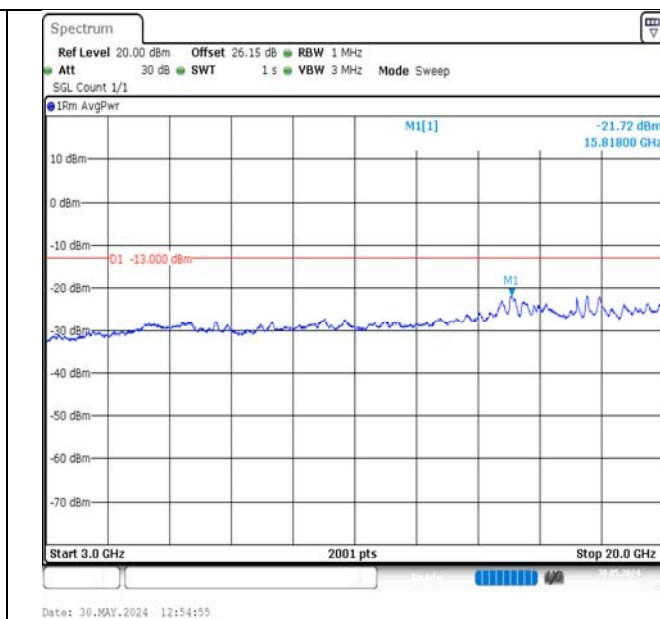
Band2-15MHz-QPSK-18675-75RB#0-3000~20000-PASS
