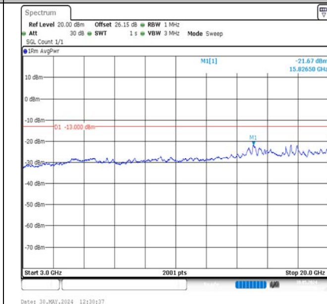
Band2-10MHz-16QAM-18900-50RB#0-3000~20000-PASS
