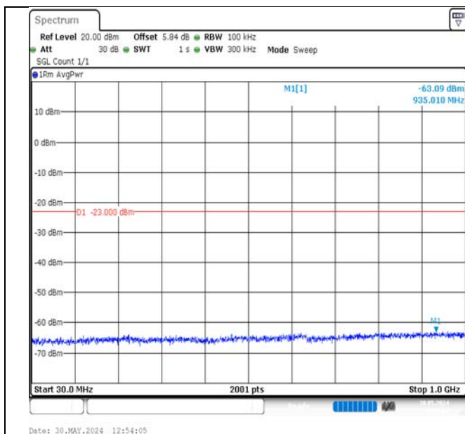
Band2-15MHz-QPSK-18675-1RB#74-30~1000-PASS
