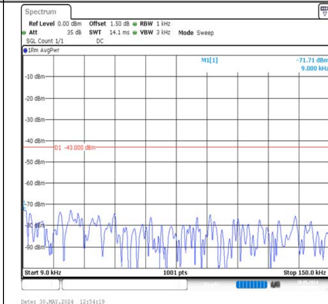
Band2-15MHz-16QAM-18675-1RB#74-0.009~0.15-PASS
