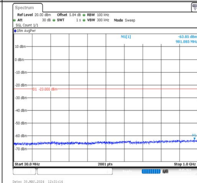
Band2-10MHz-16QAM-19150-1RB#0-30~1000-PASS
