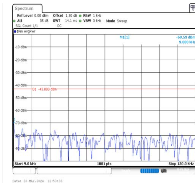
Band2-15MHz-16QAM-18675-1RB#0-0.009~0.15-PASS
