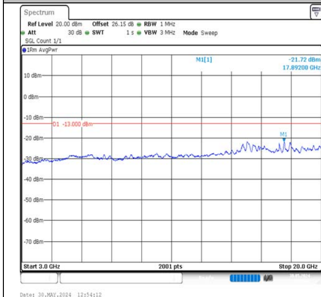
Band2-15MHz-QPSK-18675-1RB#74-3000~20000-PASS
