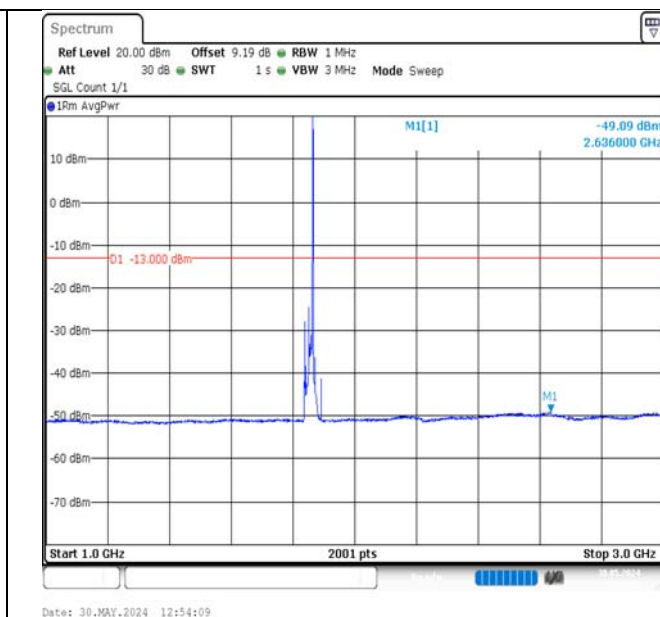
Band2-15MHz-QPSK-18675-1RB#74-1000~3000-PASS
