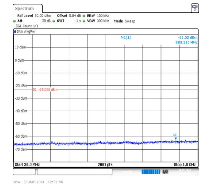
Band2-10MHz-16QAM-19150-1RB#49-30~1000-PASS
