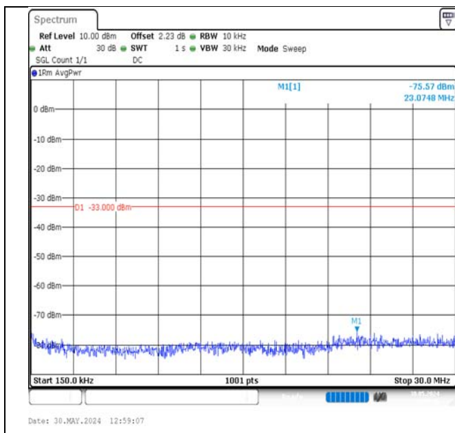
Band2-15MHz-QPSK-19125-75RB#0-0.15~30-PASS
