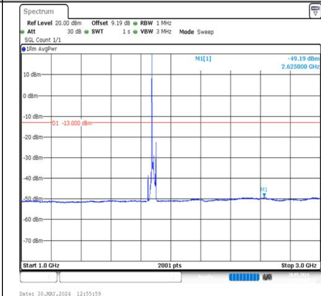
Band2-15MHz-16QAM-18900-1RB#0-1000~3000-PASS
