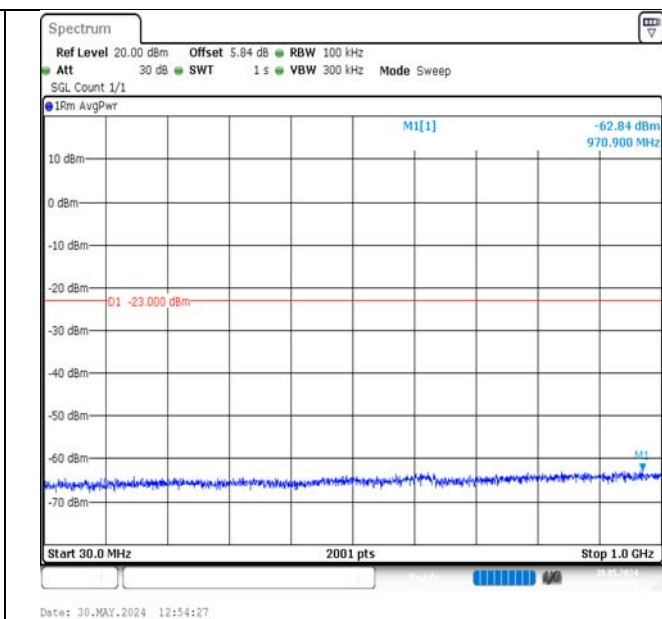
Band2-15MHz-16QAM-18675-1RB#74-30~1000-PASS
