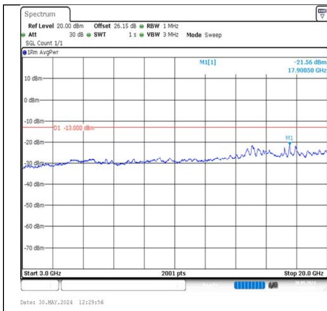
Band2-10MHz-16QAM-18900-1RB#49-3000~20000-PASS
