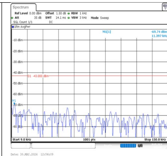
Band2-15MHz-QPSK-18900-1RB#74-0.009~0.15-PASS
