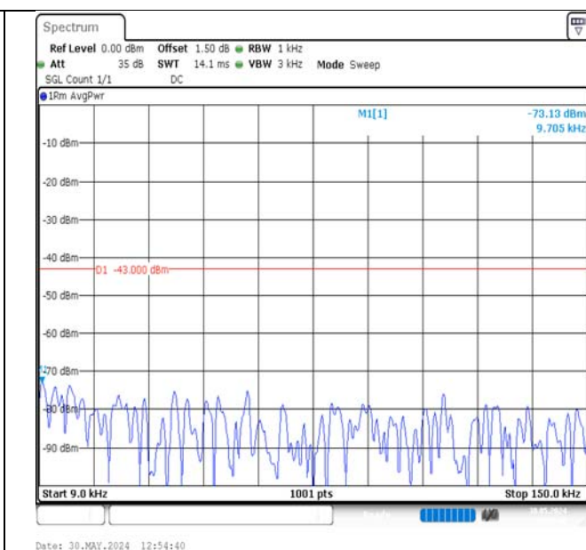
Band2-15MHz-QPSK-18675-75RB#0-0.009~0.15-PASS
