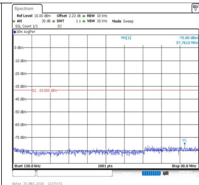
Band2-15MHz-16QAM-18900-1RB#0-0.15~30-PASS
