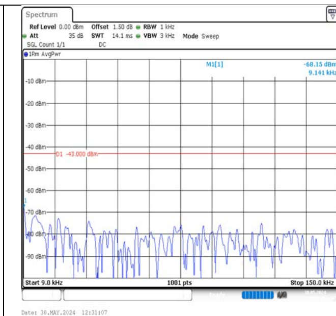
Band2-10MHz-16QAM-19150-1RB#0-0.009~0.15-PASS
