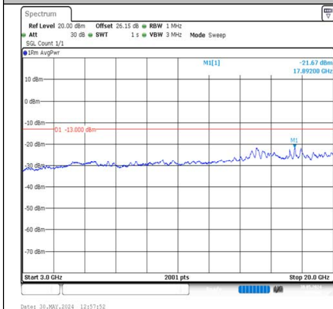
Band2-15MHz-QPSK-19125-1RB#0-3000~20000-PASS
