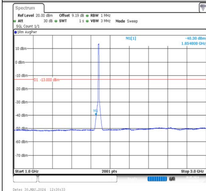
Band2-10MHz-16QAM-18900-50RB#0-1000~3000-PASS
