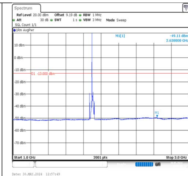
Band2-15MHz-QPSK-19125-1RB#0-1000~3000-PASS
