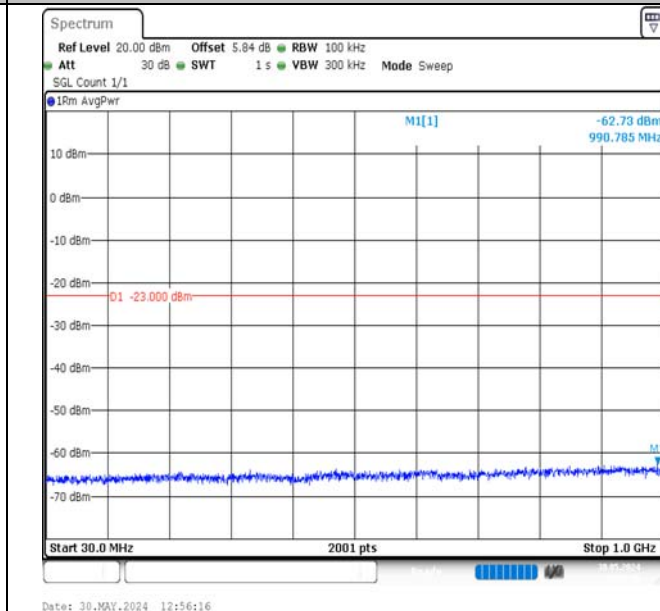
Band2-15MHz-QPSK-18900-1RB#74-30~1000-PASS
