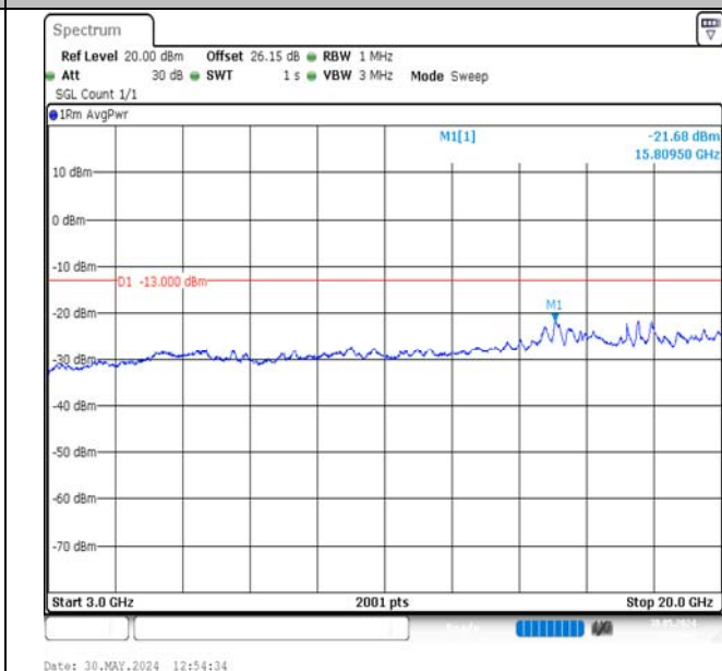
Band2-15MHz-16QAM-18675-1RB#74-3000~20000-PASS
