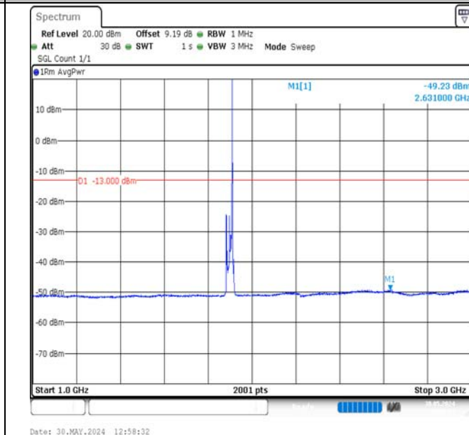
Band2-15MHz-QPSK-19125-1RB#74-1000~3000-PASS
