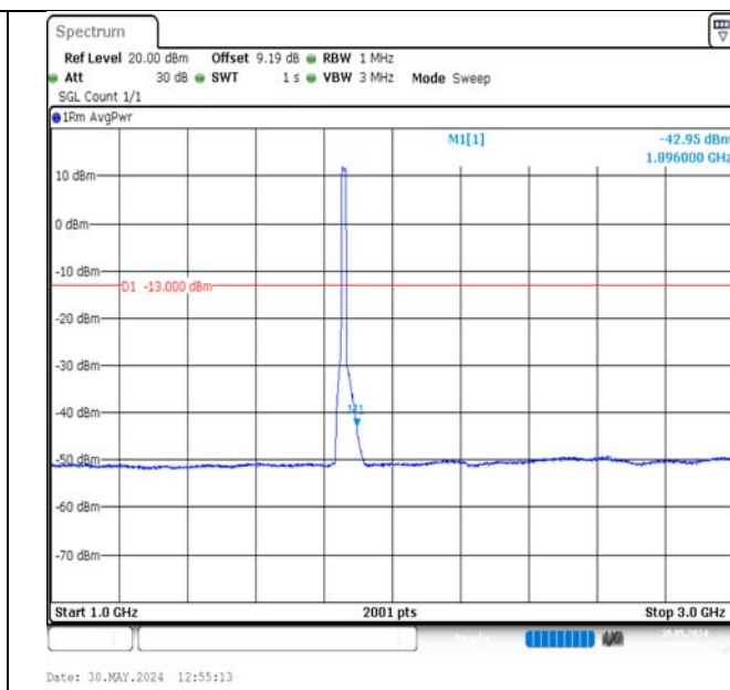
Band2-15MHz-16QAM-18675-75RB#0-1000~3000-PASS
