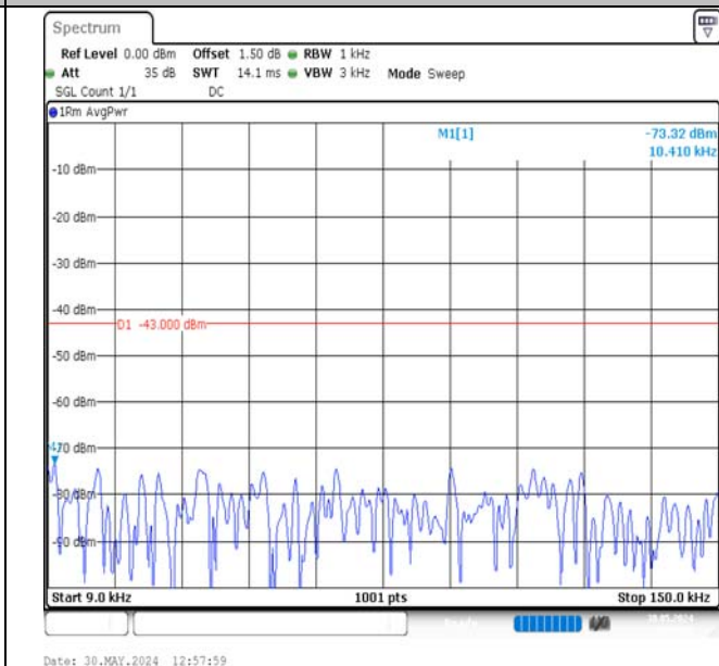
Band2-15MHz-16QAM-19125-1RB#0-0.009~0.15-PASS
