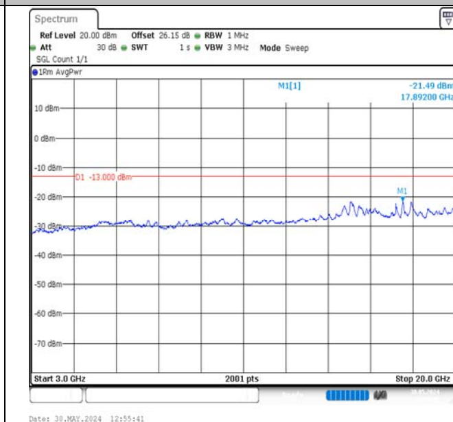
Band2-15MHz-QPSK-18900-1RB#0-3000~20000-PASS
