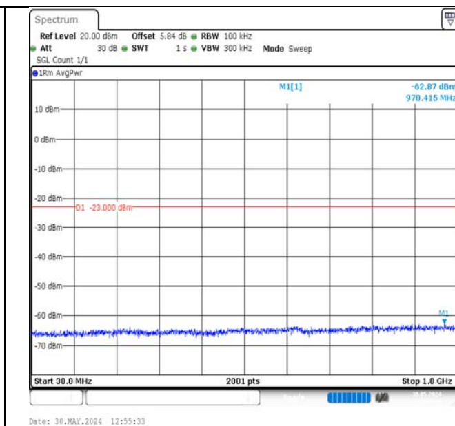
Band2-15MHz-QPSK-18900-1RB#0-30~1000-PASS
