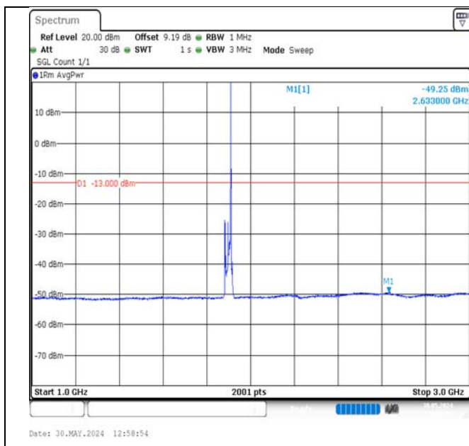
Band2-15MHz-16QAM-19125-1RB#74-1000~3000-PASS
