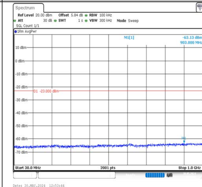
Band2-15MHz-16QAM-18675-1RB#0-30~1000-PASS
