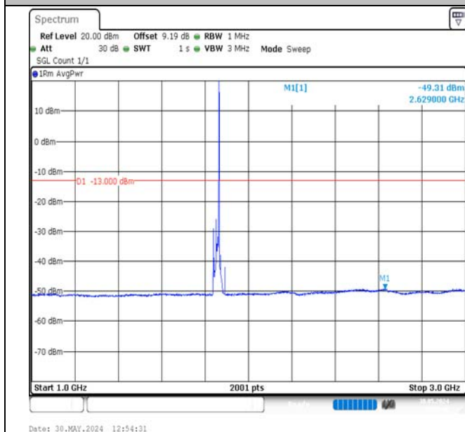
Band2-15MHz-16QAM-18675-1RB#74-1000~3000-PASS
