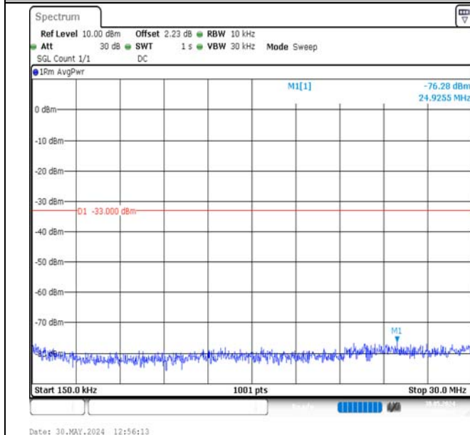
Band2-15MHz-QPSK-18900-1RB#74-0.15~30-PASS
