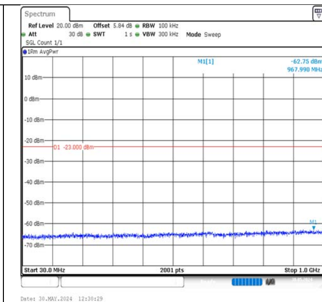
Band2-10MHz-16QAM-18900-50RB#0-30~1000-PASS
