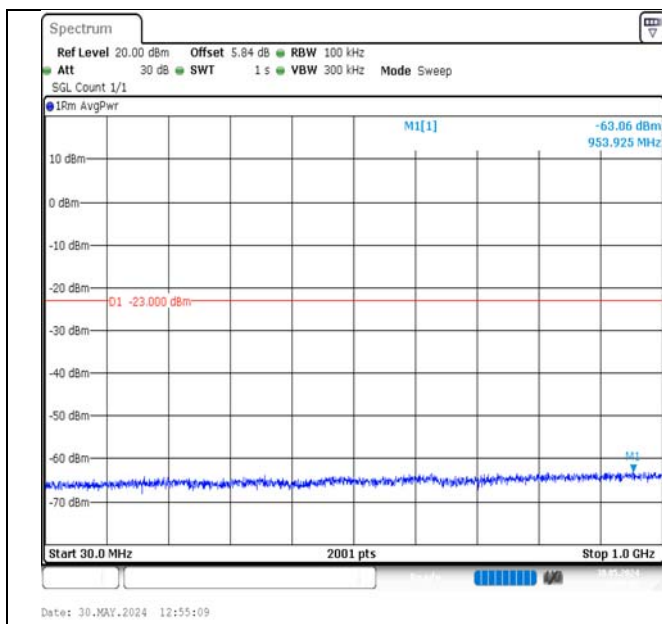
Band2-15MHz-16QAM-18675-75RB#0-30~1000-PASS
