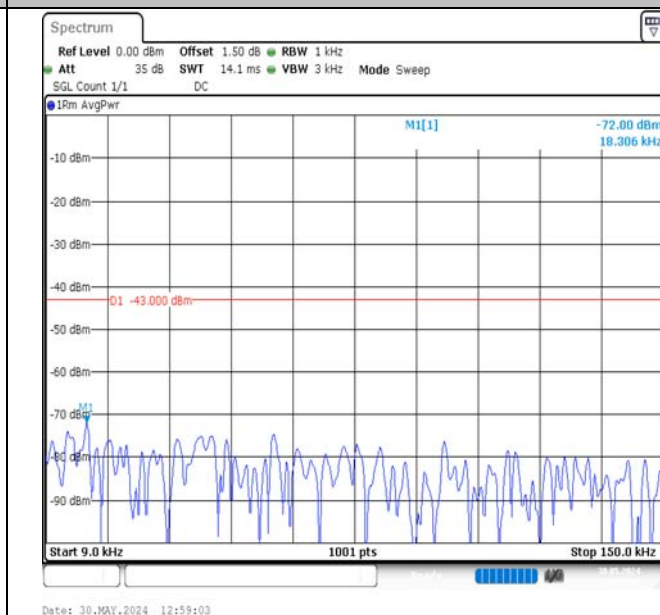
Band2-15MHz-QPSK-19125-75RB#0-0.009~0.15-PASS
