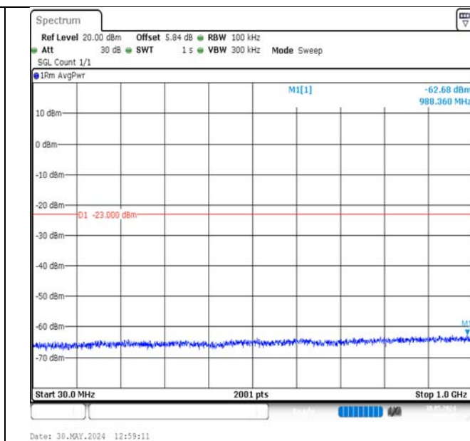
Band2-15MHz-QPSK-19125-75RB#0-30~1000-PASS
