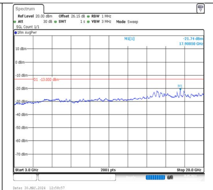
Band2-15MHz-16QAM-19125-1RB#74-3000~20000-PASS
