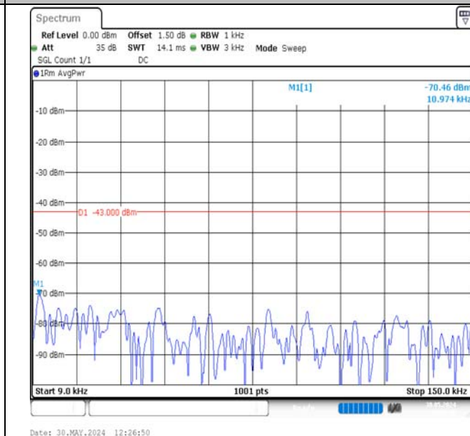
Band2-10MHz-16QAM-18650-1RB#0-0.009~0.15-PASS
