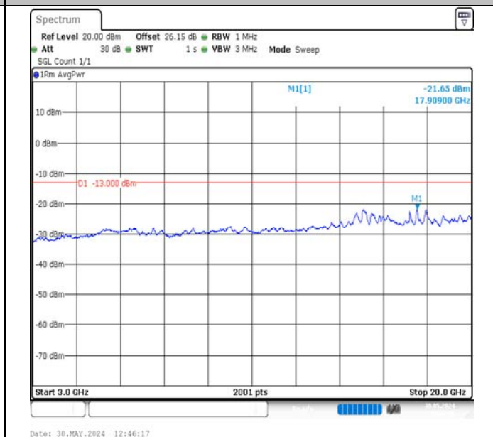
Band2-5MHz-QPSK-19175-25RB#0-3000~20000-PASS
