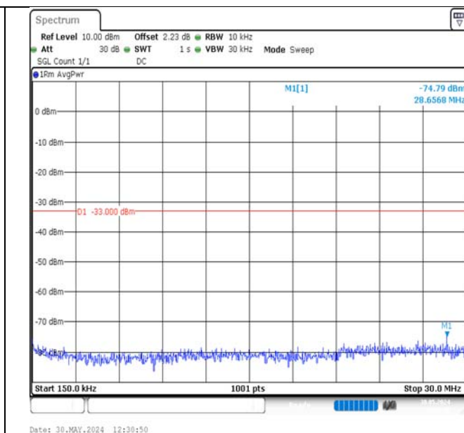
Band2-10MHz-QPSK-19150-1RB#0-0.15~30-PASS
