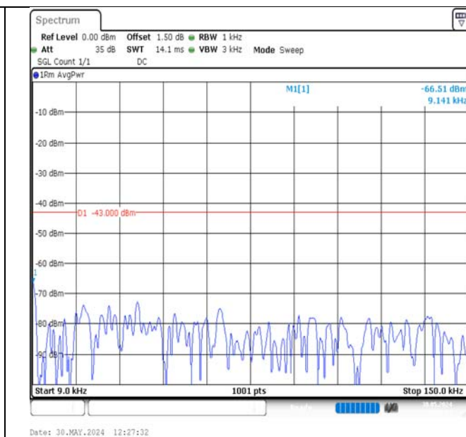
Band2-10MHz-16QAM-18650-1RB#49-0.009~0.15-PASS
