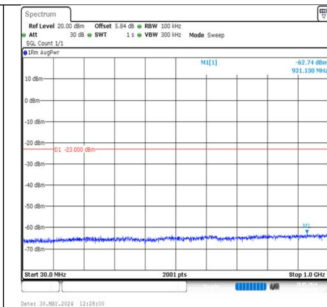
Band2-10MHz-QPSK-18650-50RB#0-30~1000-PASS
