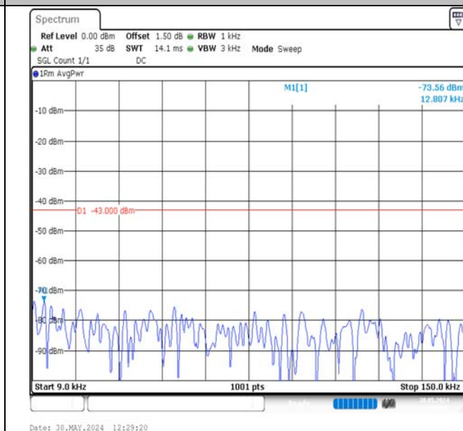
Band2-10MHz-QPSK-18900-1RB#49-0.009~0.15-PASS
