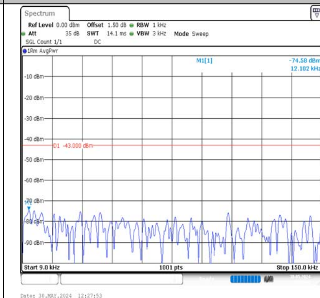
Band2-10MHz-QPSK-18650-50RB#0-0.009~0.15-PASS
