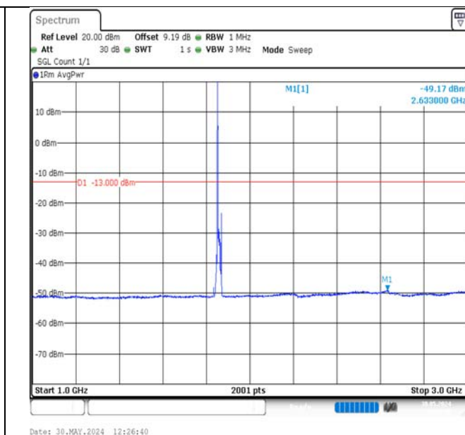
Band2-10MHz-QPSK-18650-1RB#0-1000~3000-PASS
