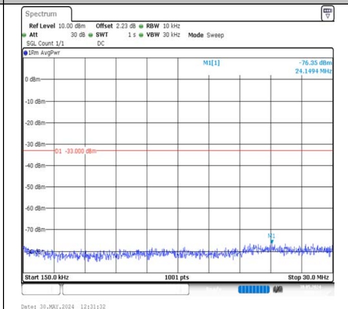
Band2-10MHz-QPSK-19150-1RB#49-0.15~30-PASS
