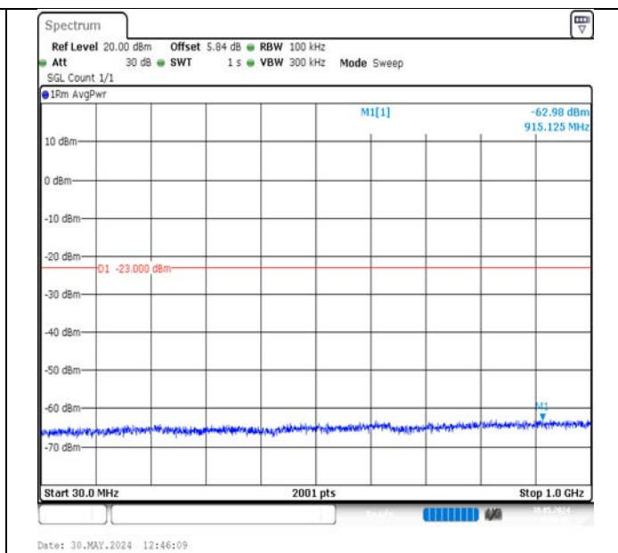
Band2-5MHz-QPSK-19175-25RB#0-30~1000-PASS
