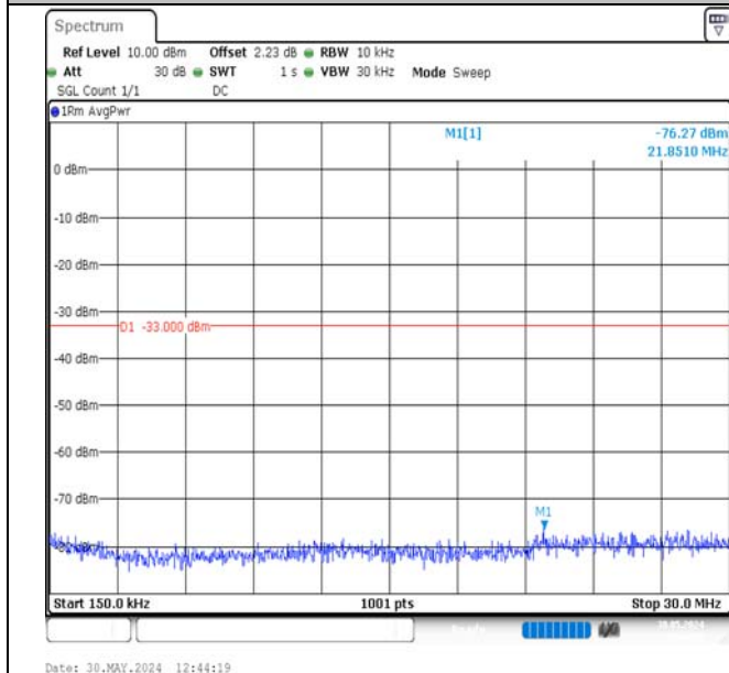
Band2-5MHz-16QAM-18900-25RB#0-0.15~30-PASS
