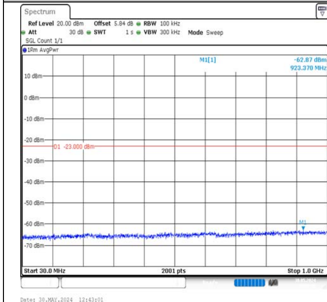
Band2-5MHz-16QAM-18900-1RB#0-30~1000-PASS
