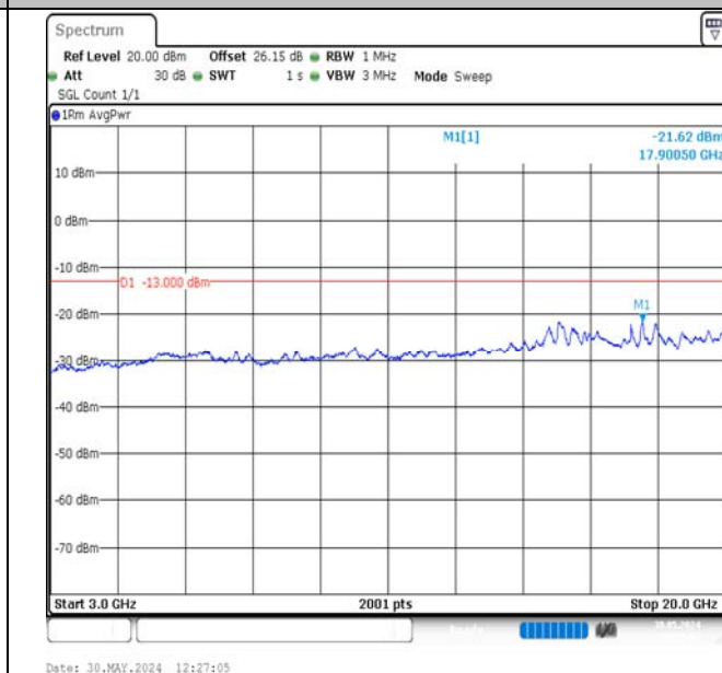
Band2-10MHz-16QAM-18650-1RB#0-3000~20000-PASS
