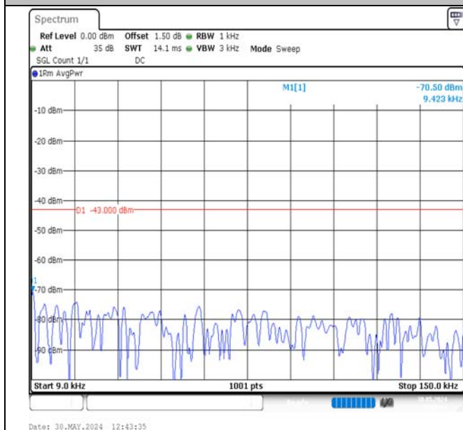
Band2-5MHz-16QAM-18900-1RB#24-0.009~0.15-PASS
