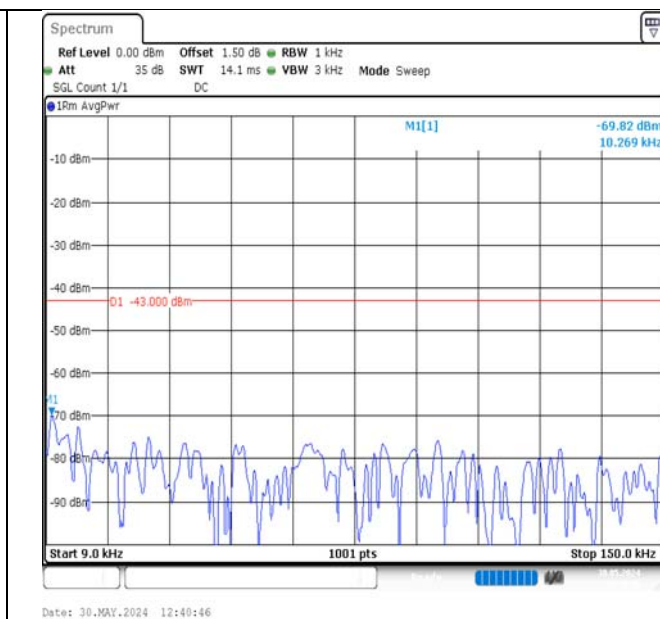
Band2-5MHz-16QAM-18625-1RB#0-0.009~0.15-PASS
