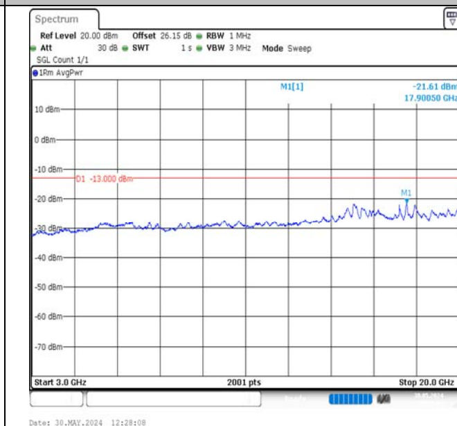
Band2-10MHz-QPSK-18650-50RB#0-3000~20000-PASS
