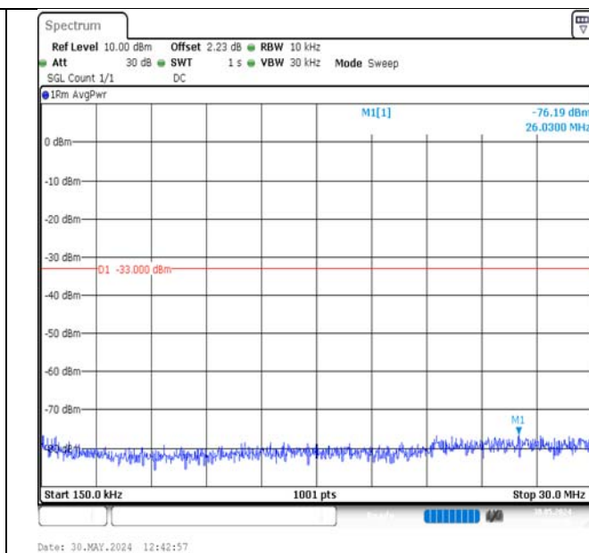
Band2-5MHz-16QAM-18900-1RB#0-0.15~30-PASS
