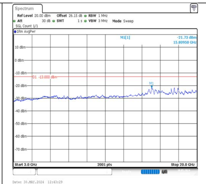
Band2-5MHz-QPSK-18900-1RB#24-3000~20000-PASS
