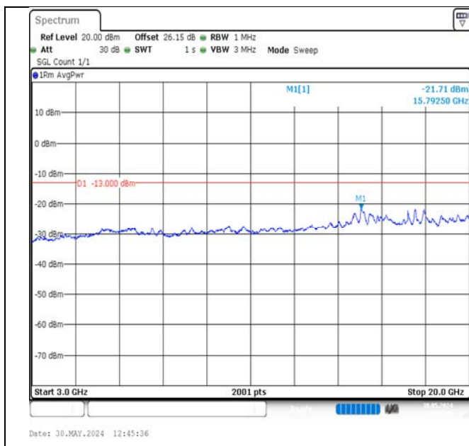
Band2-5MHz-QPSK-19175-1RB#24-3000~20000-PASS
