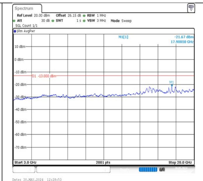
Band2-10MHz-QPSK-18900-1RB#0-3000~20000-PASS
