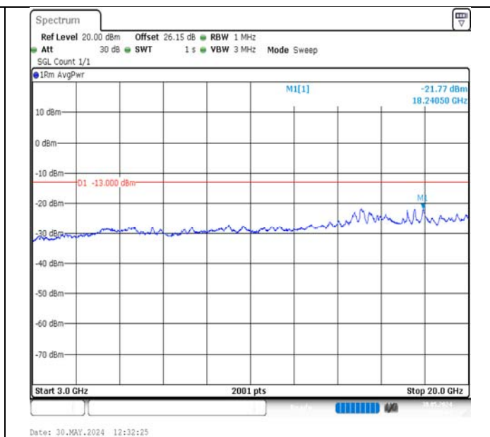
Band2-10MHz-QPSK-19150-50RB#0-3000~20000-PASS
