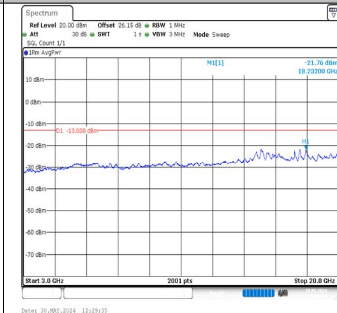
Band2-10MHz-QPSK-18900-1RB#49-3000~20000-PASS
