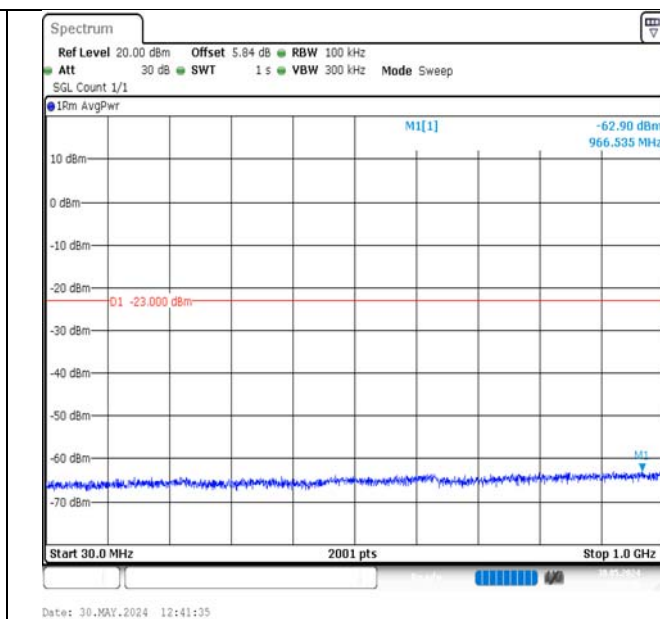
Band2-5MHz-16QAM-18625-1RB#24-30~1000-PASS
