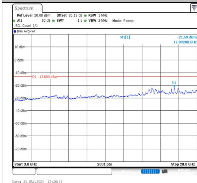
Band2-10MHz-QPSK-18650-1RB#0-3000~20000-PASS
