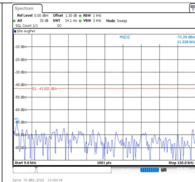
Band2-5MHz-16QAM-18900-25RB#0-0.009~0.15-PASS
