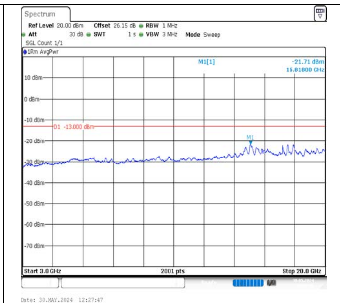
Band2-10MHz-16QAM-18650-1RB#49-3000~20000-PASS
