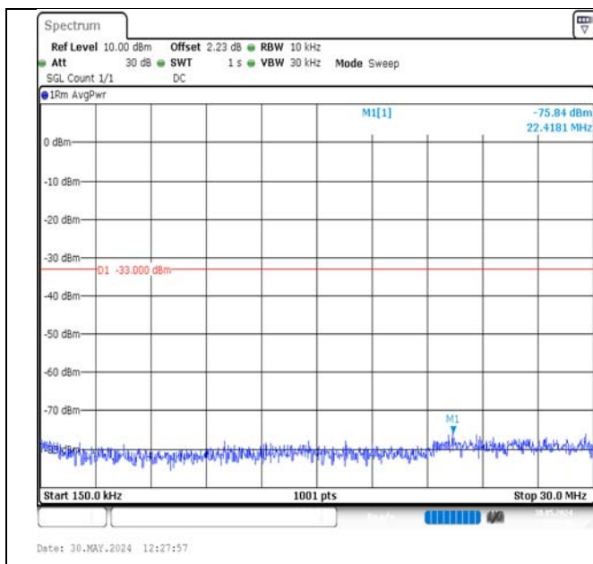
Band2-10MHz-QPSK-18650-50RB#0-0.15~30-PASS
