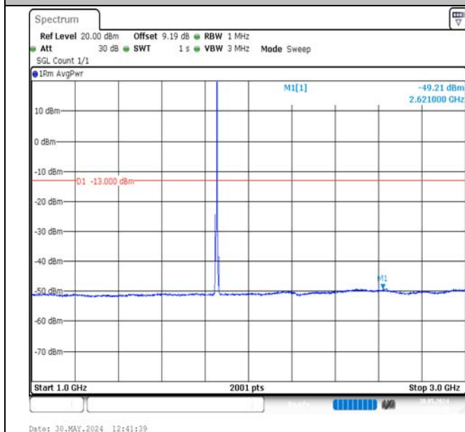
Band2-5MHz-16QAM-18625-1RB#24-1000~3000-PASS
