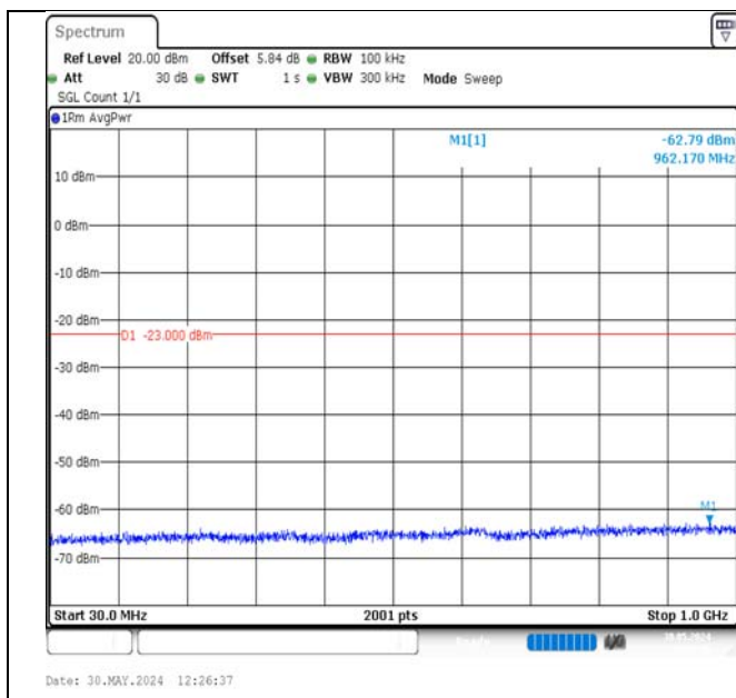
Band2-10MHz-QPSK-18650-1RB#0-30~1000-PASS
