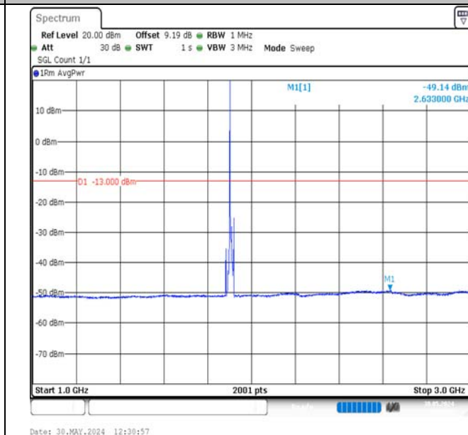
Band2-10MHz-QPSK-19150-1RB#0-1000~3000-PASS
