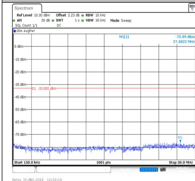
Band2-10MHz-QPSK-19150-50RB#0-0.15~30-PASS
