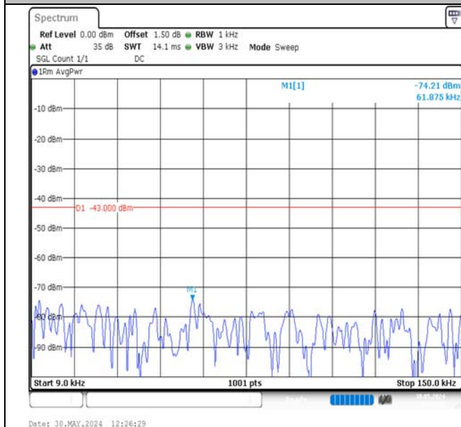
Band2-10MHz-QPSK-18650-1RB#0-0.009~0.15-PASS
