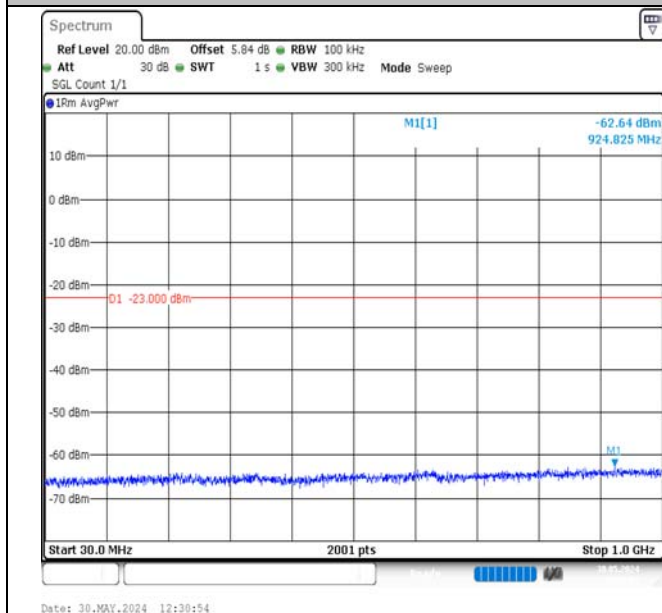
Band2-10MHz-QPSK-19150-1RB#0-30~1000-PASS
