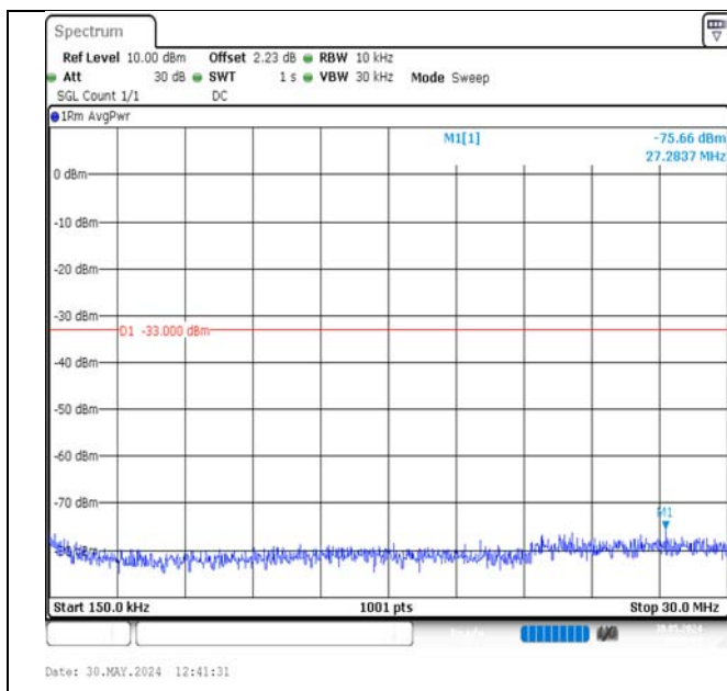
Band2-5MHz-16QAM-18625-1RB#24-0.15~30-PASS
