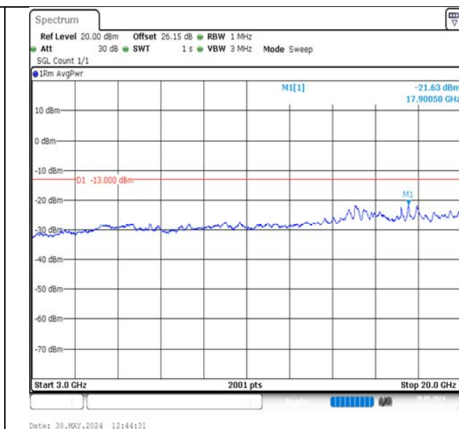
Band2-5MHz-16QAM-18900-25RB#0-3000~20000-PASS
