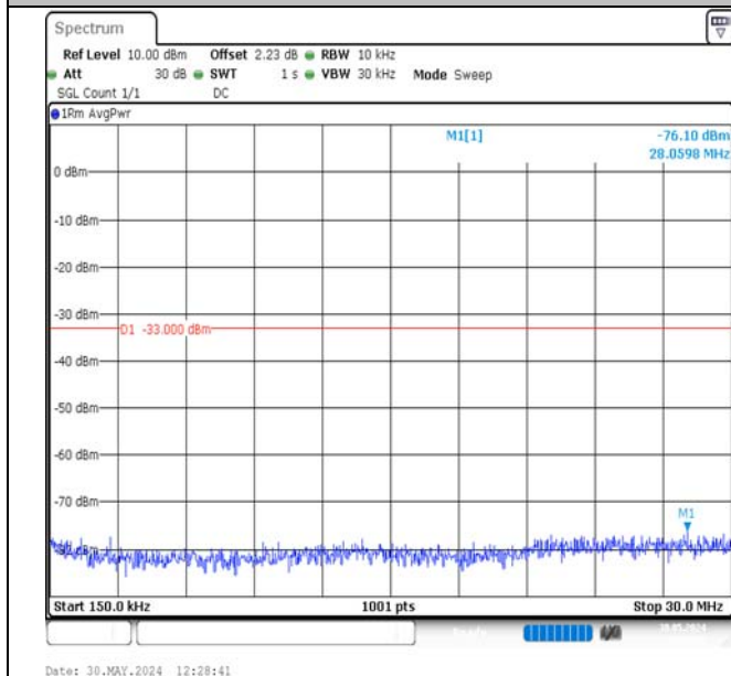
Band2-10MHz-QPSK-18900-1RB#0-0.15~30-PASS
