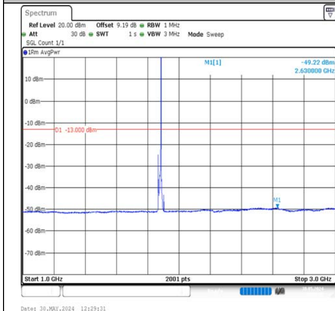
Band2-10MHz-QPSK-18900-1RB#49-1000~3000-PASS
