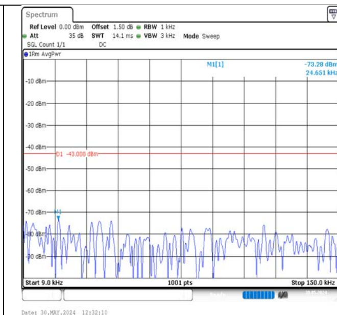
Band2-10MHz-QPSK-19150-50RB#0-0.009~0.15-PASS
