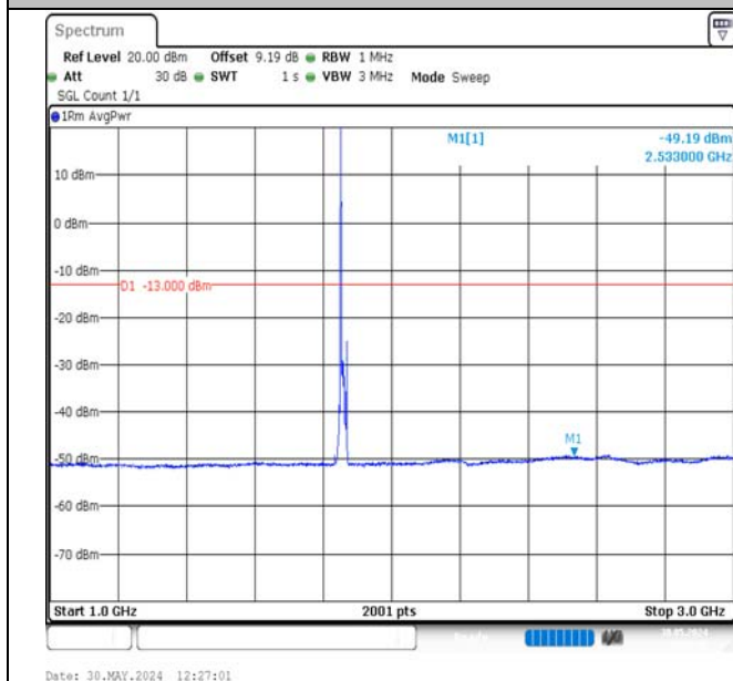
Band2-10MHz-16QAM-18650-1RB#0-1000~3000-PASS
