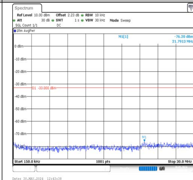
Band2-5MHz-16QAM-18900-1RB#24-0.15~30-PASS
