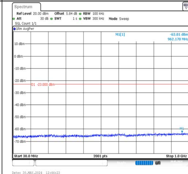
Band2-5MHz-16QAM-18900-25RB#0-30~1000-PASS
