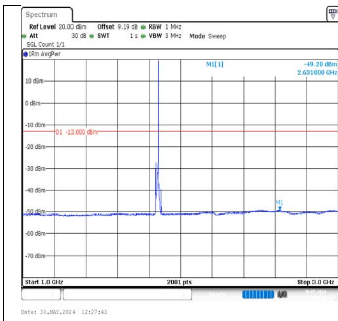
Band2-10MHz-16QAM-18650-1RB#49-1000~3000-PASS
