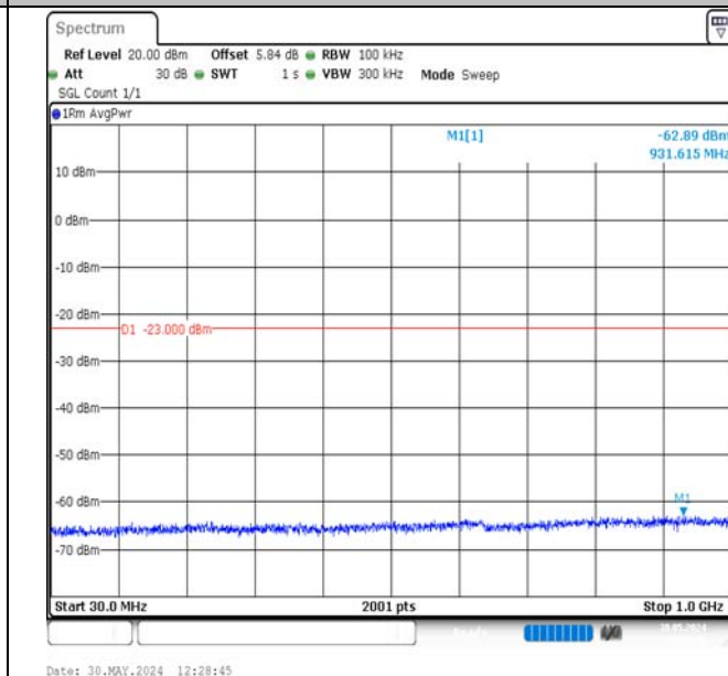
Band2-10MHz-QPSK-18900-1RB#0-30~1000-PASS
