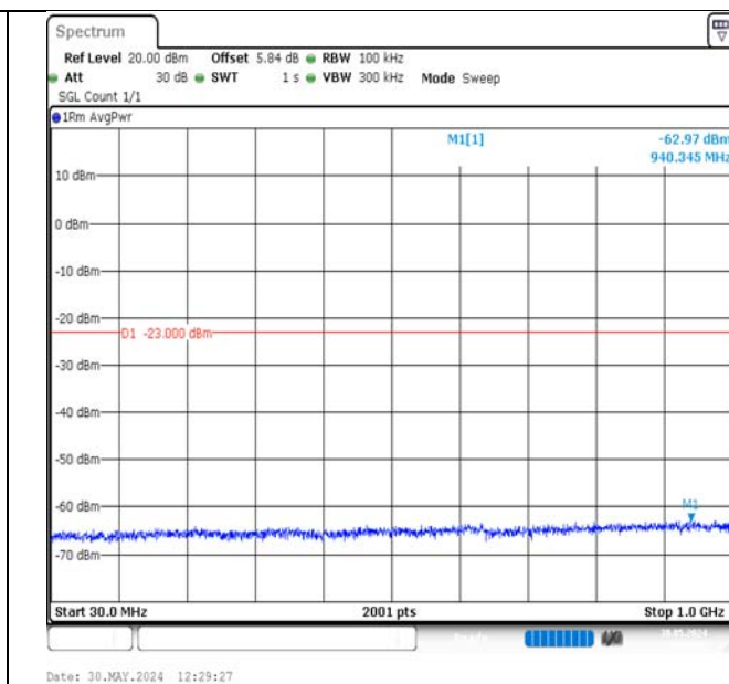
Band2-10MHz-QPSK-18900-1RB#49-30~1000-PASS
