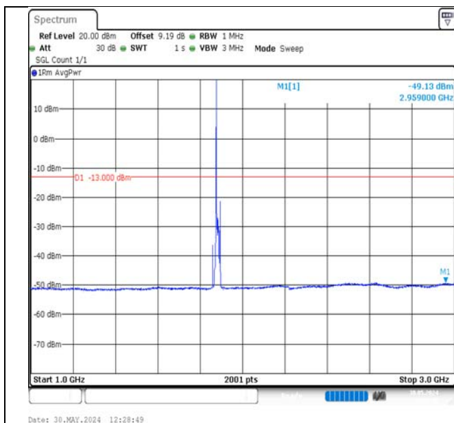
Band2-10MHz-QPSK-18900-1RB#0-1000~3000-PASS
