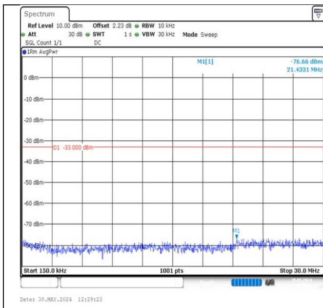
Band2-10MHz-QPSK-18900-1RB#49-0.15~30-PASS
