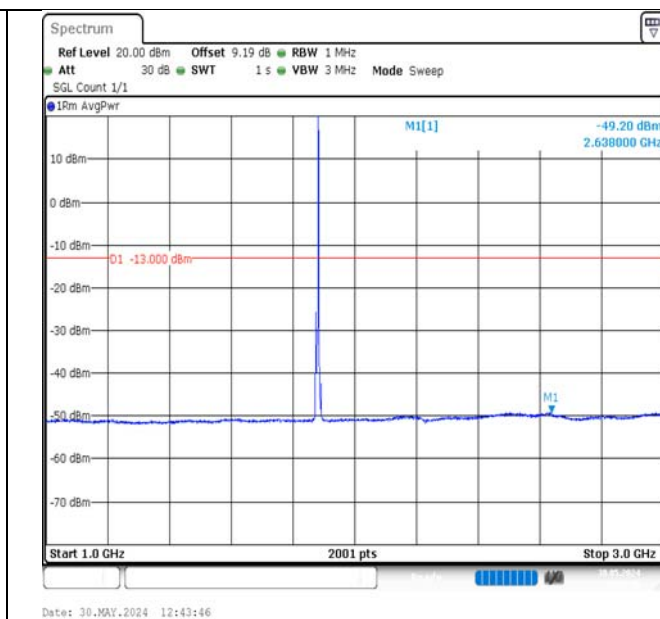
Band2-5MHz-16QAM-18900-1RB#24-1000~3000-PASS
