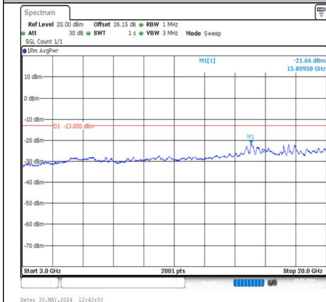
Band2-5MHz-16QAM-18900-1RB#24-3000~20000-PASS
