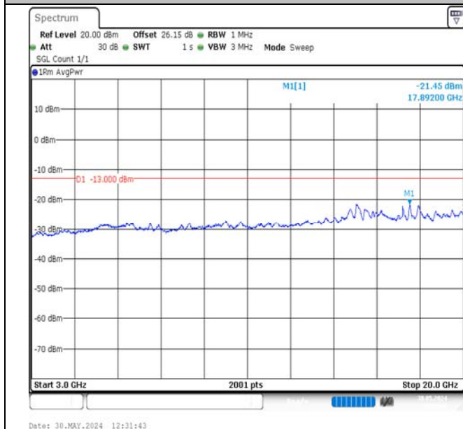
Band2-10MHz-QPSK-19150-1RB#49-3000~20000-PASS
