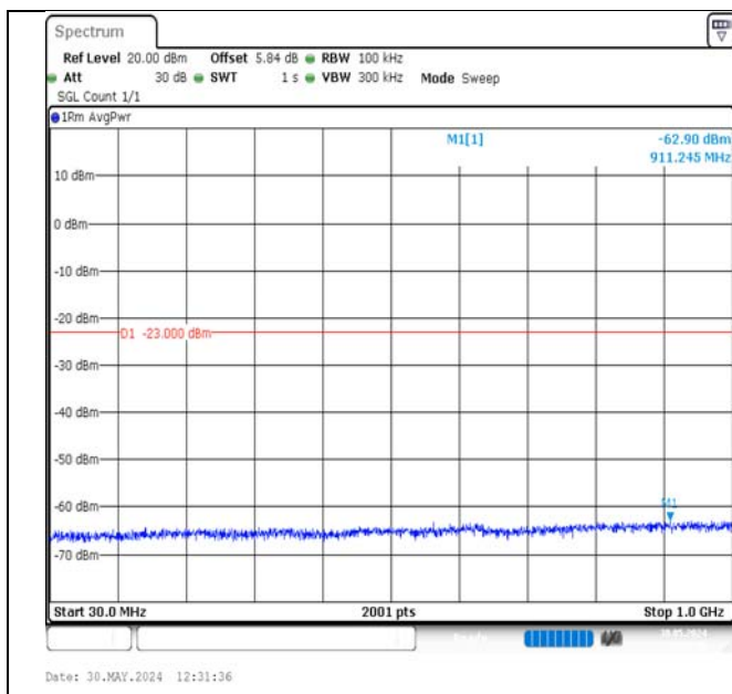
Band2-10MHz-QPSK-19150-1RB#49-30~1000-PASS
