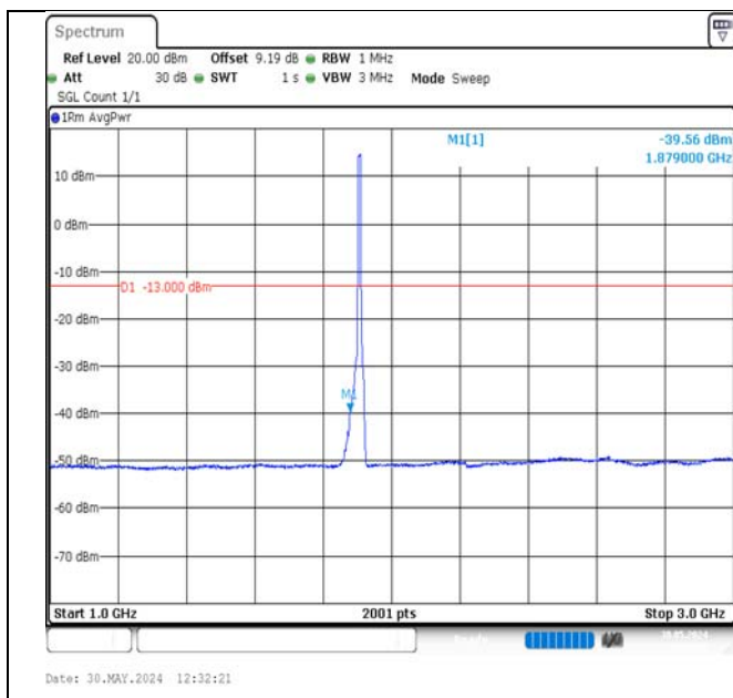
Band2-10MHz-QPSK-19150-50RB#0-1000~3000-PASS
