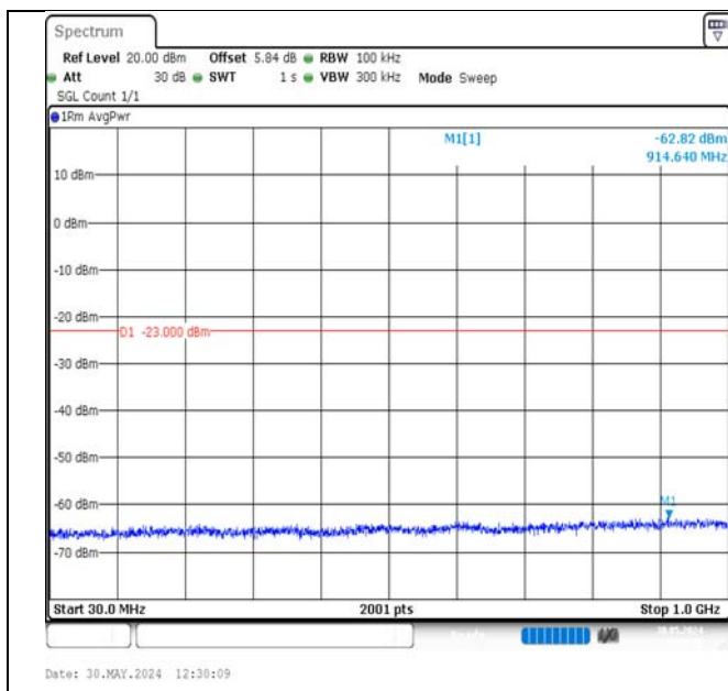
Band2-10MHz-QPSK-18900-50RB#0-30~1000-PASS
