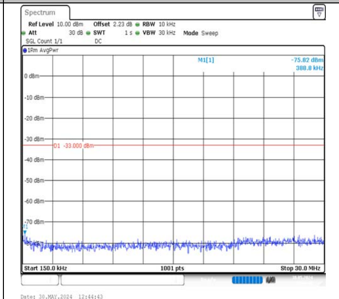
Band2-5MHz-QPSK-19175-1RB#0-0.15~30-PASS
