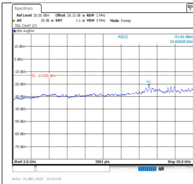
Band2-5MHz-16QAM-18900-1RB#0-3000~20000-PASS
