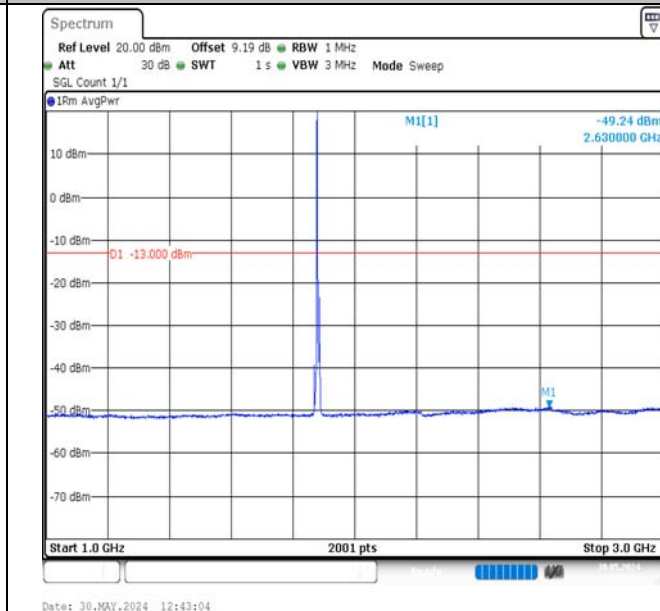
Band2-5MHz-16QAM-18900-1RB#0-1000~3000-PASS
