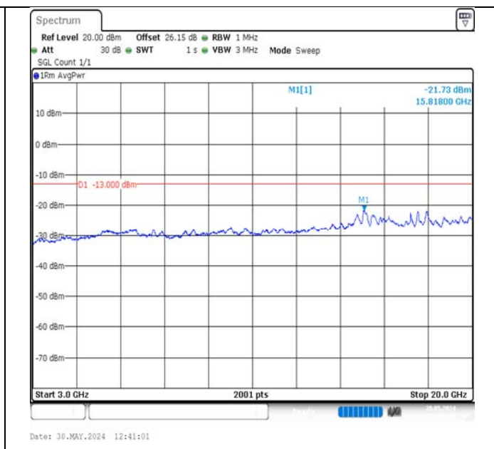
Band2-5MHz-16QAM-18625-1RB#0-3000~20000-PASS
