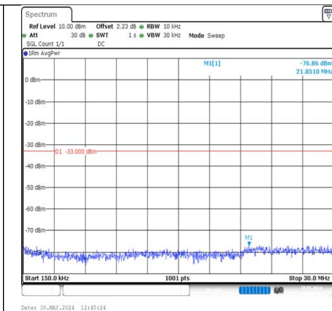
Band2-5MHz-QPSK-19175-1RB#24-0.15~30-PASS
