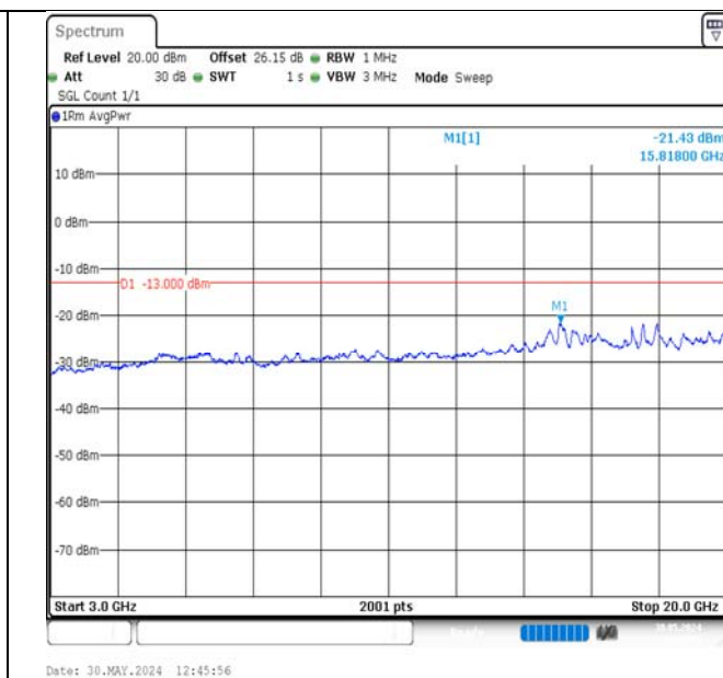
Band2-5MHz-16QAM-19175-1RB#24-3000~20000-PASS
