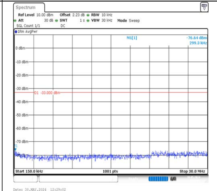
Band2-10MHz-16QAM-18900-1RB#0-0.15~30-PASS
