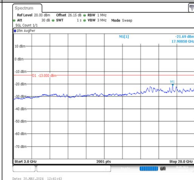
Band2-5MHz-16QAM-18625-1RB#24-3000~20000-PASS
