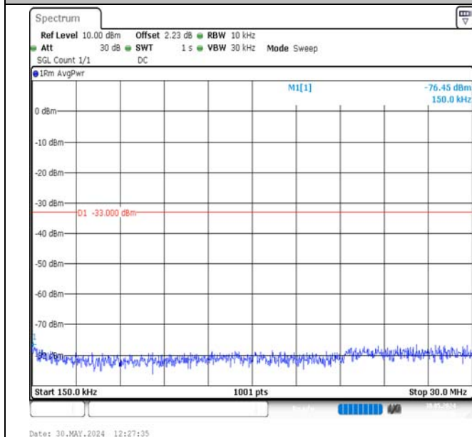
Band2-10MHz-16QAM-18650-1RB#49-0.15~30-PASS
