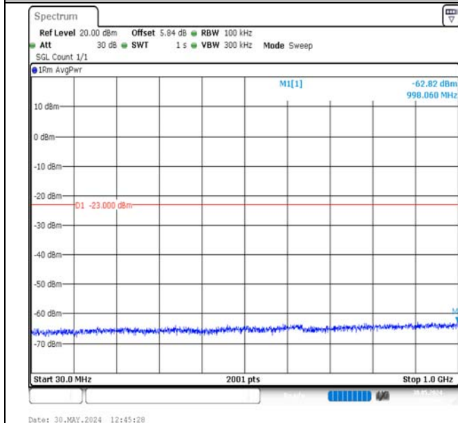
Band2-5MHz-QPSK-19175-1RB#24-30~1000-PASS
