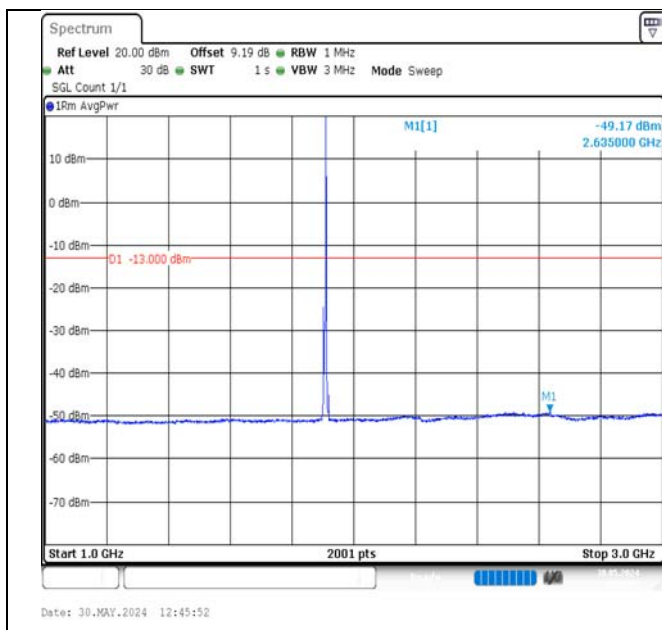
Band2-5MHz-16QAM-19175-1RB#24-1000~3000-PASS
