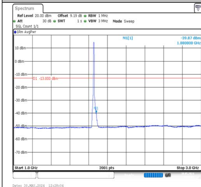
Band2-10MHz-QPSK-18650-50RB#0-1000~3000-PASS
