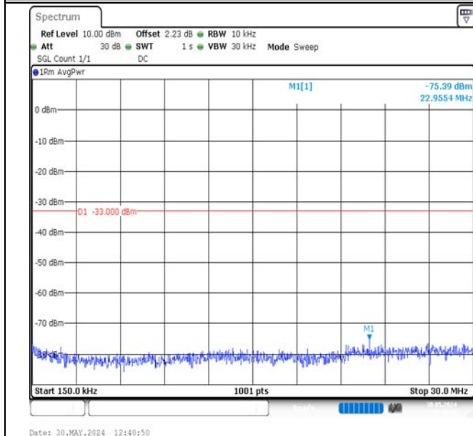
Band2-5MHz-16QAM-18625-1RB#0-0.15~30-PASS
