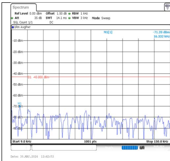
Band2-5MHz-16QAM-18900-1RB#0-0.009~0.15-PASS
