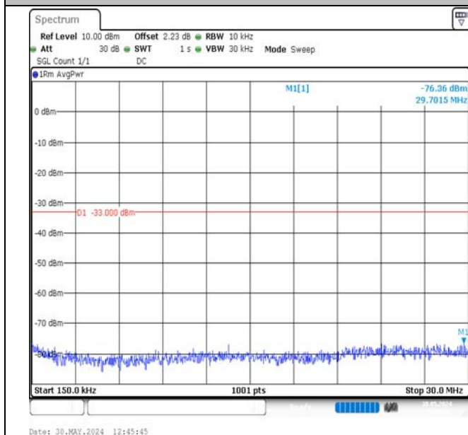
Band2-5MHz-16QAM-19175-1RB#24-0.15~30-PASS
