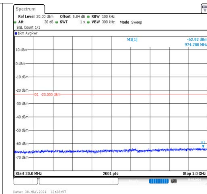
Band2-10MHz-16QAM-18650-1RB#0-30~1000-PASS
