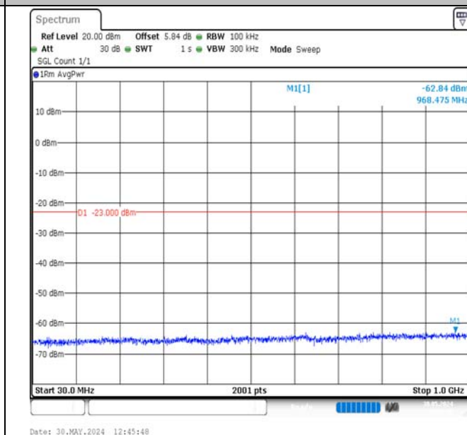
Band2-5MHz-16QAM-19175-1RB#24-30~1000-PASS
