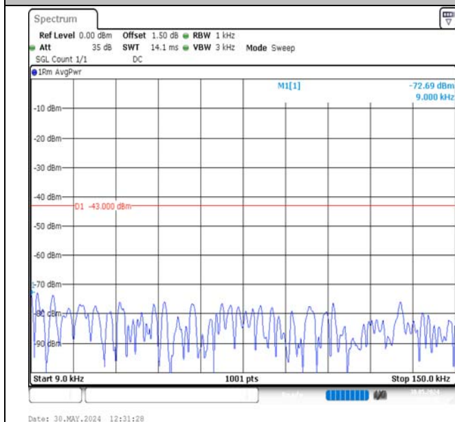
Band2-10MHz-QPSK-19150-1RB#49-0.009~0.15-PASS
