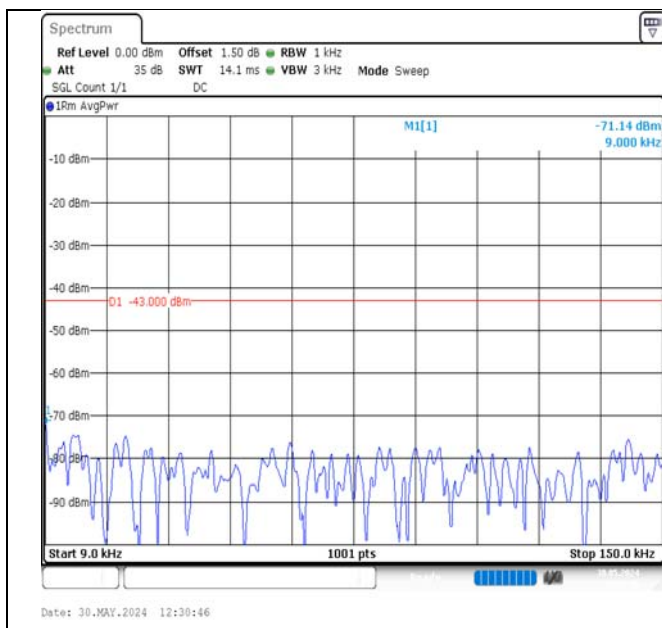
Band2-10MHz-QPSK-19150-1RB#0-0.009~0.15-PASS
