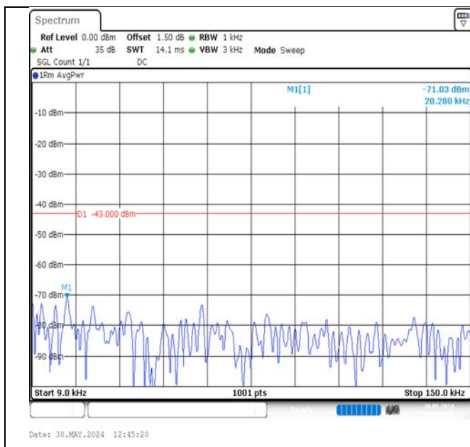
Band2-5MHz-QPSK-19175-1RB#24-0.009~0.15-PASS
