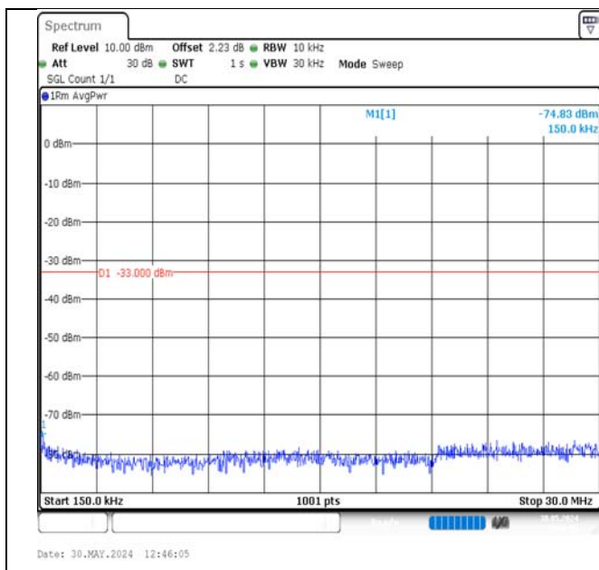
Band2-5MHz-QPSK-19175-25RB#0-0.15~30-PASS
