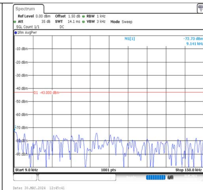
Band2-5MHz-16QAM-19175-1RB#24-0.009~0.15-PASS
