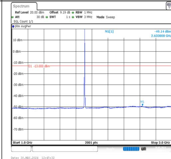
Band2-5MHz-QPSK-19175-1RB#24-1000~3000-PASS
