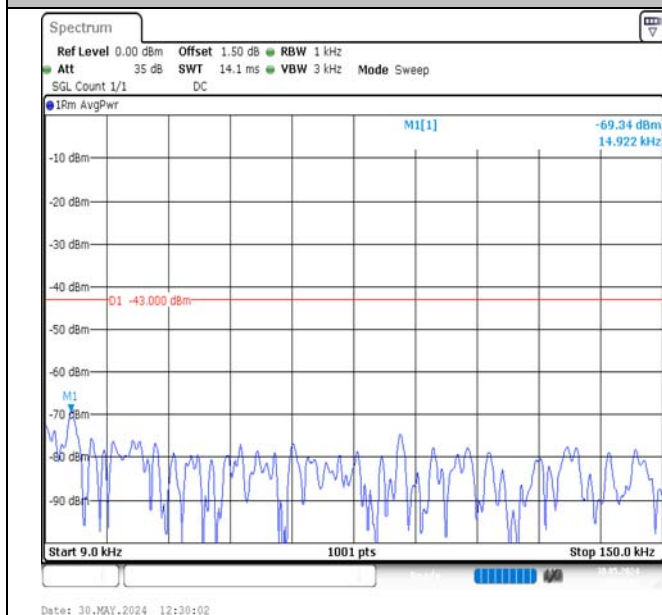
Band2-10MHz-QPSK-18900-50RB#0-0.009~0.15-PASS
