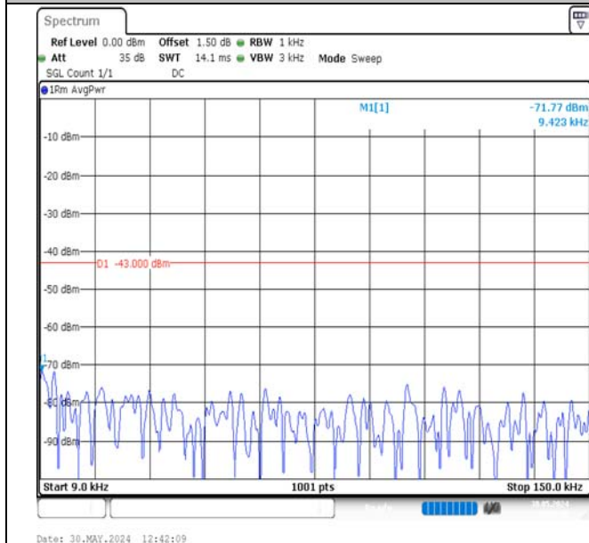
Band2-5MHz-16QAM-18625-25RB#0-0.009~0.15-PASS
