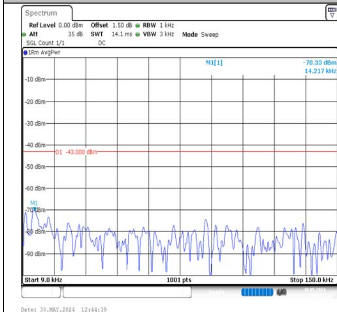
Band2-5MHz-QPSK-19175-1RB#0-0.009~0.15-PASS
