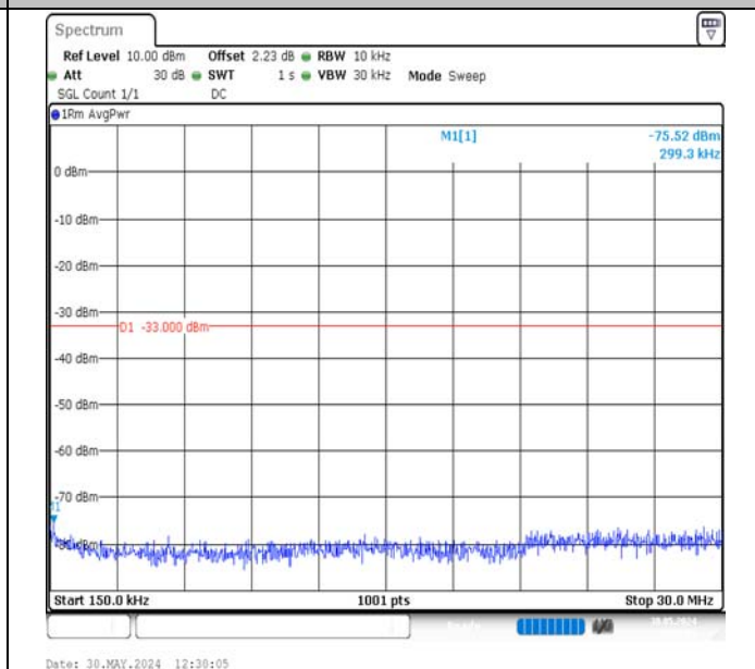
Band2-10MHz-QPSK-18900-50RB#0-0.15~30-PASS
