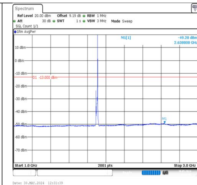
Band2-10MHz-QPSK-19150-1RB#49-1000~3000-PASS
