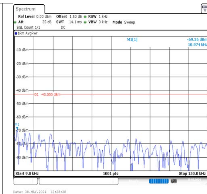
Band2-10MHz-QPSK-18900-1RB#0-0.009~0.15-PASS
