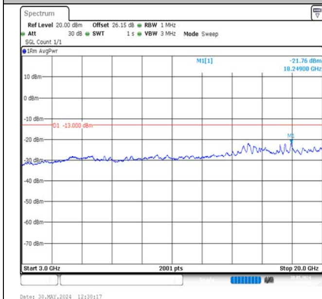
Band2-10MHz-QPSK-18900-50RB#0-3000~20000-PASS
