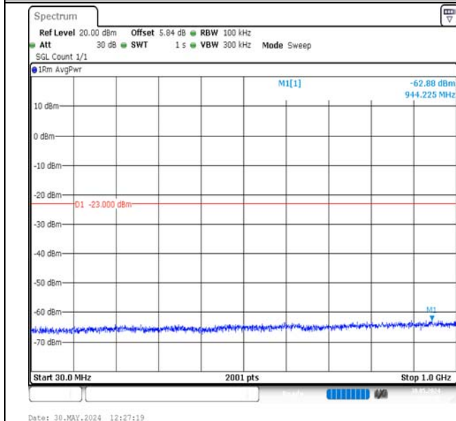
Band2-10MHz-QPSK-18650-1RB#49-30~1000-PASS
