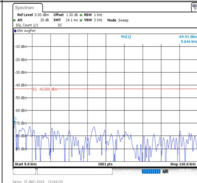
Band2-5MHz-16QAM-19175-1RB#0-0.009~0.15-PASS
