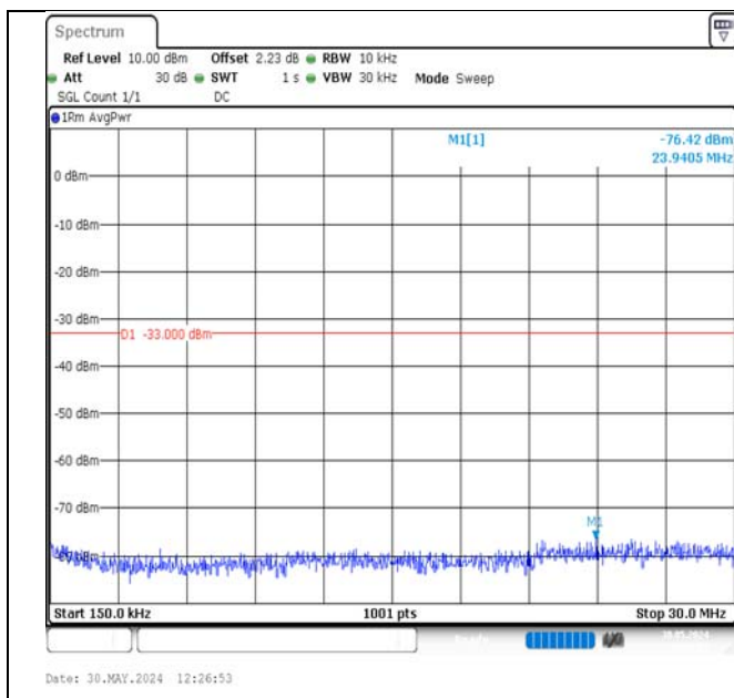
Band2-10MHz-16QAM-18650-1RB#0-0.15~30-PASS
