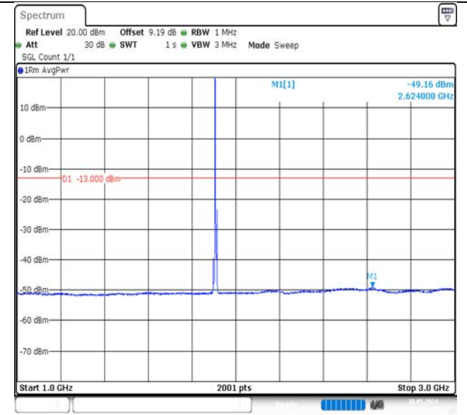
Band2-5MHz-QPSK-19175-1RB#0-1000~3000-PASS
