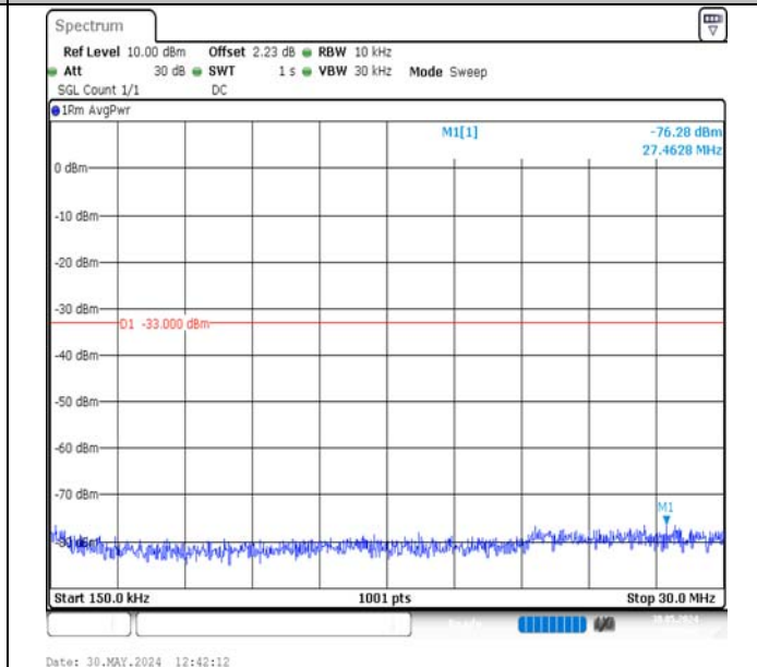
Band2-5MHz-16QAM-18625-25RB#0-0.15~30-PASS
