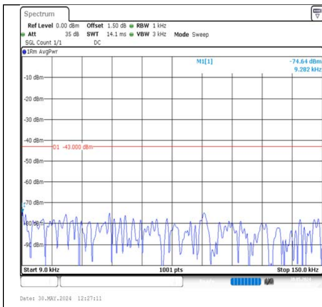
Band2-10MHz-QPSK-18650-1RB#49-0.009~0.15-PASS
