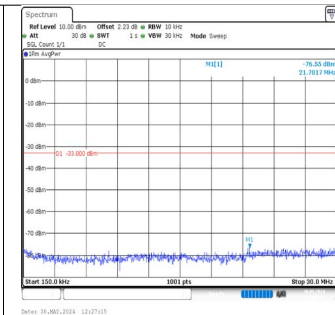
Band2-10MHz-QPSK-18650-1RB#49-0.15~30-PASS
