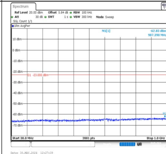
Band2-10MHz-16QAM-18650-1RB#49-30~1000-PASS
