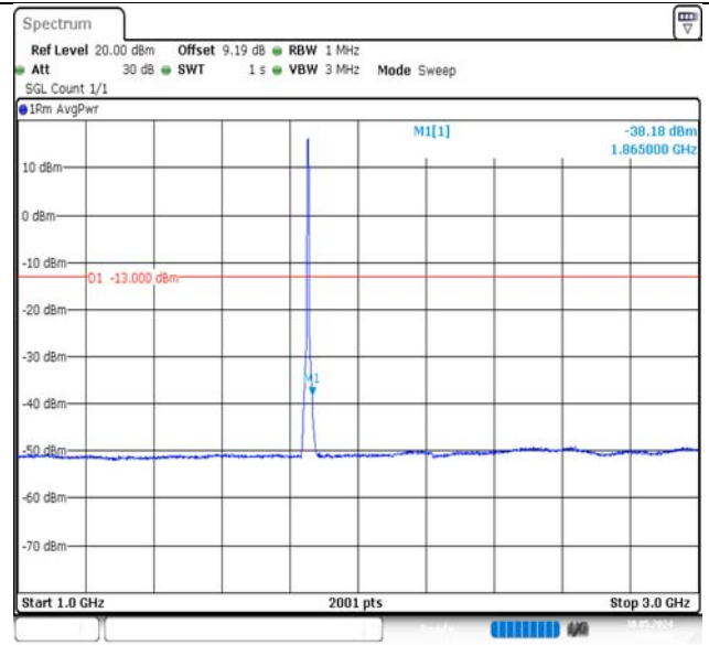
Band2-5MHz-16QAM-18625-25RB#0-1000~3000-PASS
