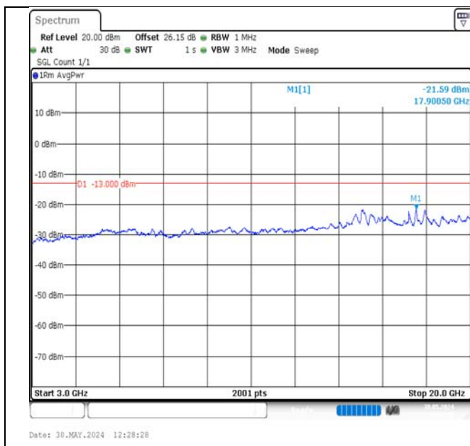
Band2-10MHz-16QAM-18650-50RB#0-3000~20000-PASS
