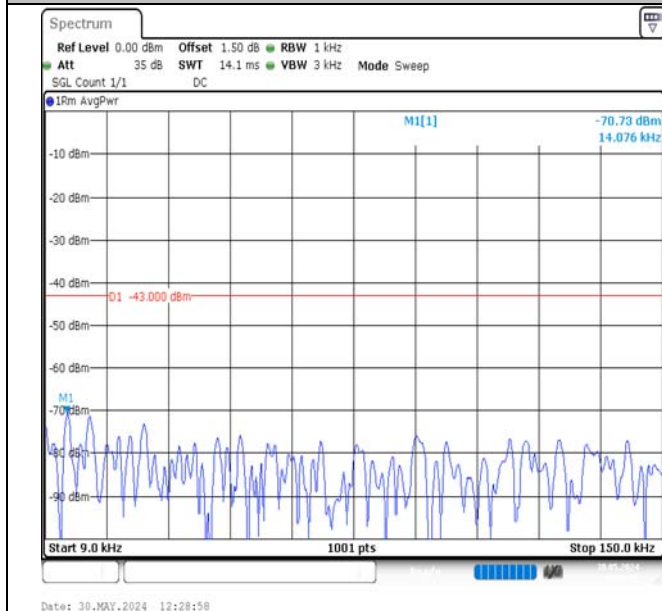
Band2-10MHz-16QAM-18900-1RB#0-0.009~0.15-PASS
