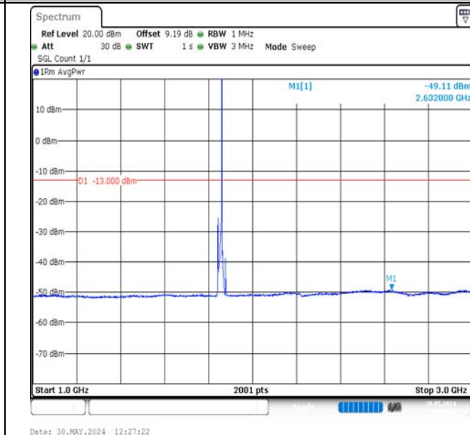
Band2-10MHz-QPSK-18650-1RB#49-1000~3000-PASS
