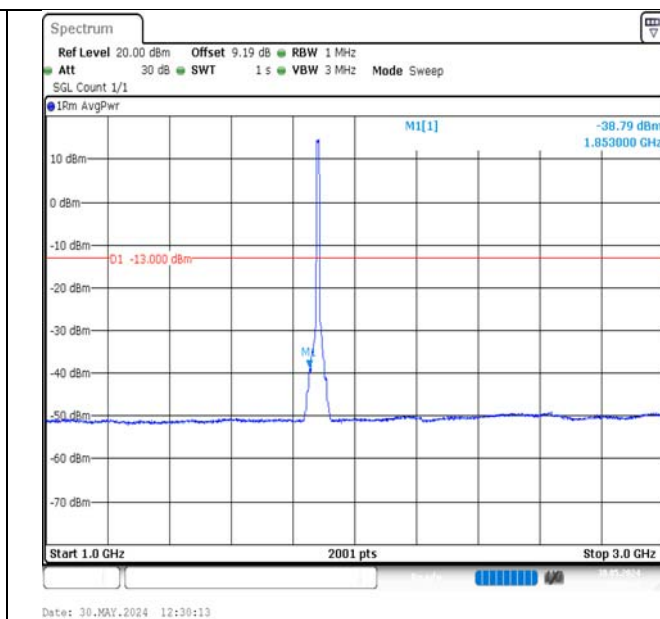
Band2-10MHz-QPSK-18900-50RB#0-1000~3000-PASS
