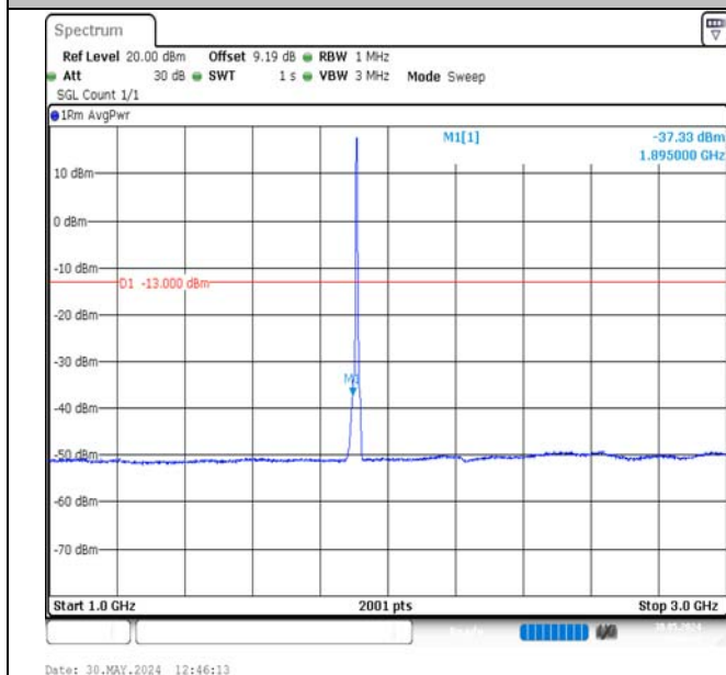
Band2-5MHz-QPSK-19175-25RB#0-1000~3000-PASS
