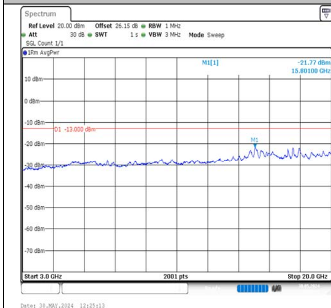
Band2-3MHz-QPSK-19185-1RB#14-3000~20000-PASS
