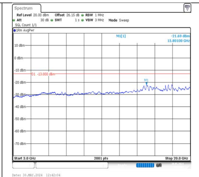
Band2-5MHz-QPSK-18625-25RB#0-3000~20000-PASS
