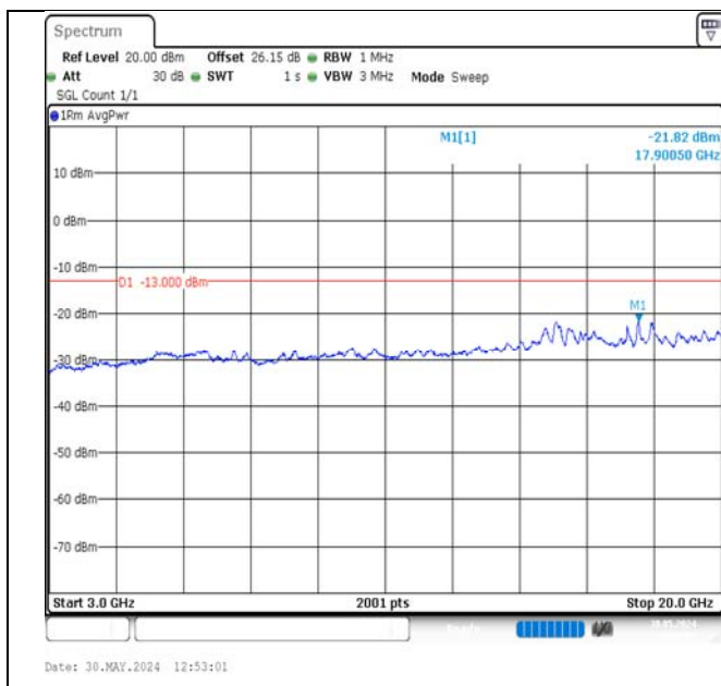
Band2-1.4MHz-16QAM-19193-6RB#0-3000~20000-PASS
