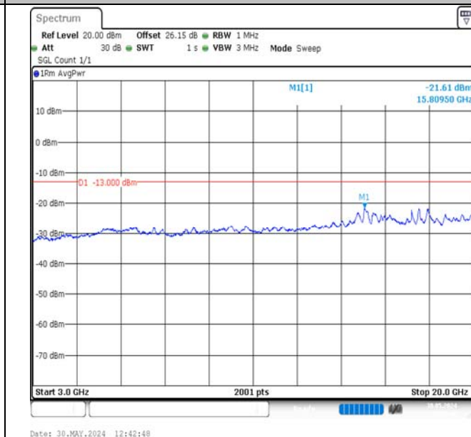
Band2-5MHz-QPSK-18900-1RB#0-3000~20000-PASS
