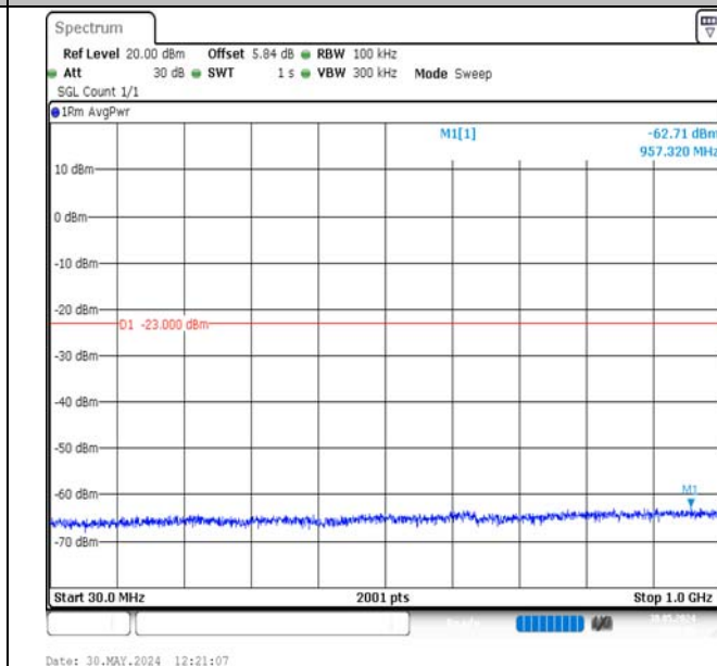
Band2-3MHz-16QAM-18615-1RB#14-30~1000-PASS
