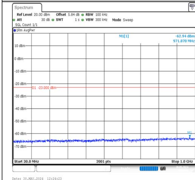
Band2-3MHz-QPSK-19185-1RB#0-30~1000-PASS
