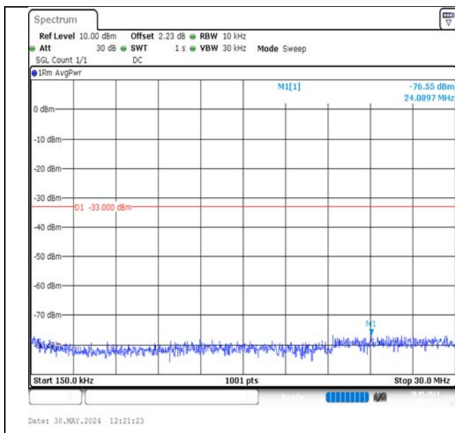
Band2-3MHz-QPSK-18615-15RB#0-0.15~30-PASS
