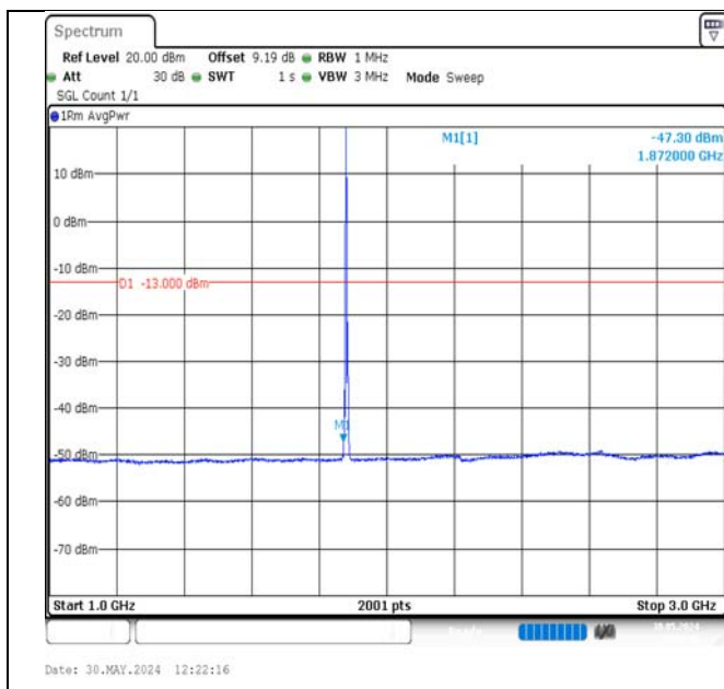
Band2-3MHz-QPSK-18900-1RB#0-1000~3000-PASS
