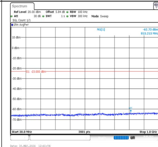
Band2-5MHz-QPSK-18625-25RB#0-30~1000-PASS
