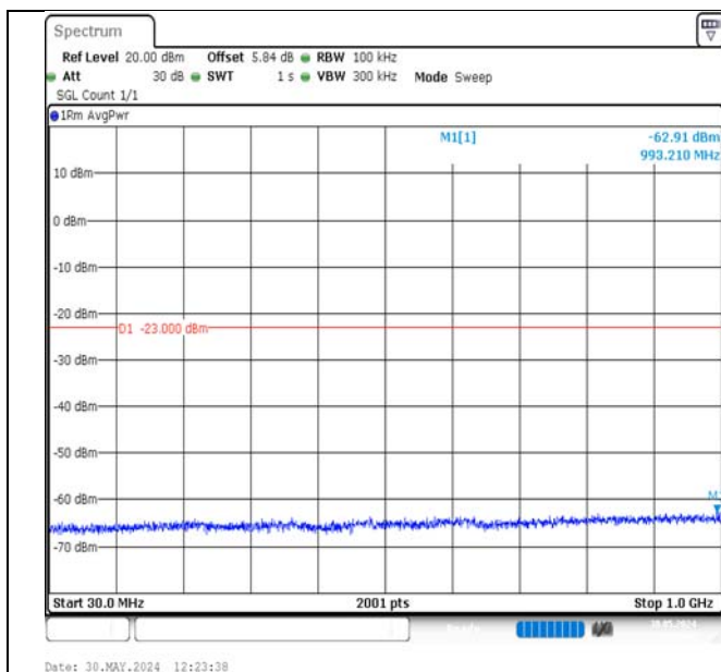
Band2-3MHz-QPSK-18900-15RB#0-30~1000-PASS
