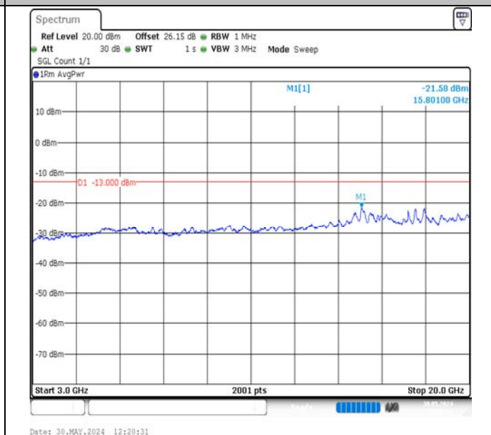
Band2-3MHz-16QAM-18615-1RB#0-3000~20000-PASS
