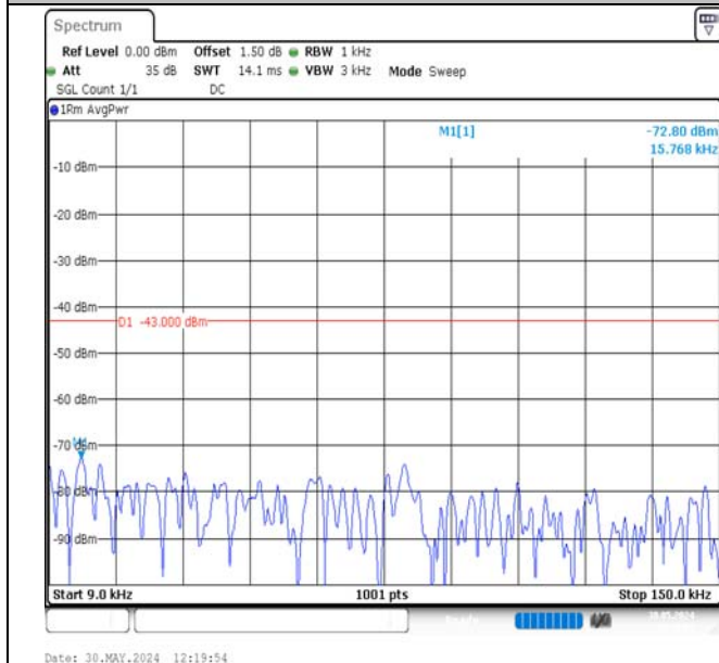
Band2-3MHz-QPSK-18615-1RB#0-0.009~0.15-PASS
