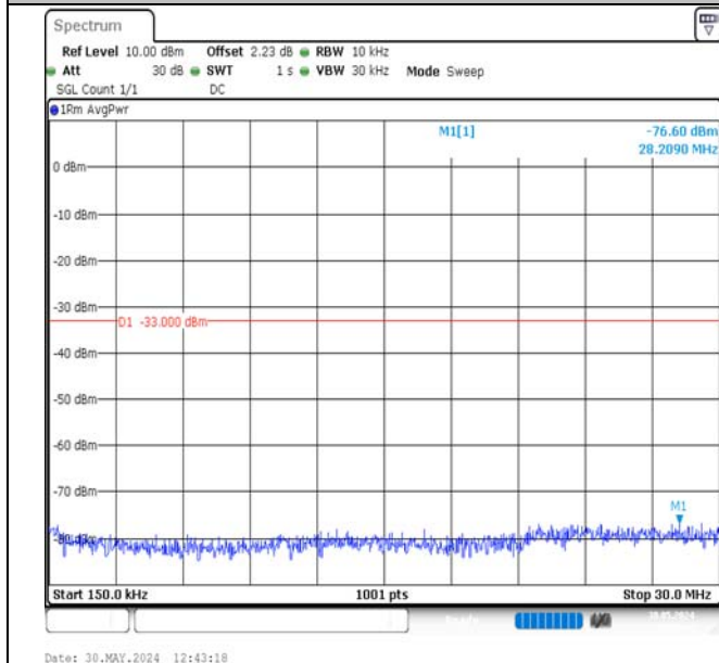
Band2-5MHz-QPSK-18900-1RB#24-0.15~30-PASS
