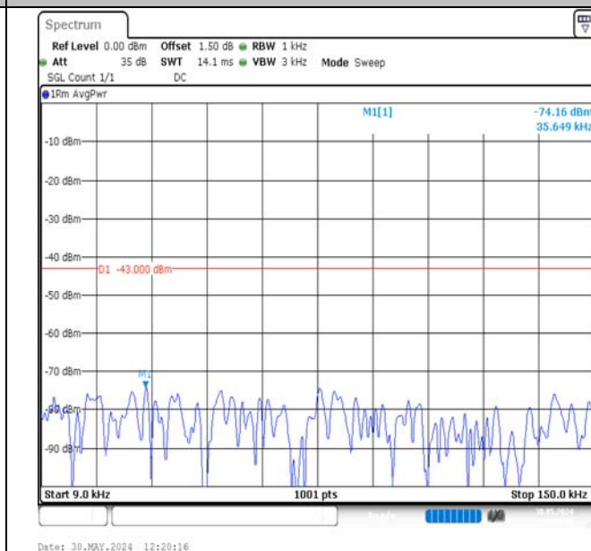
Band2-3MHz-16QAM-18615-1RB#0-0.009~0.15-PASS
