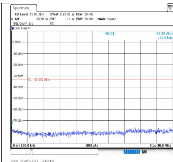
Band2-3MHz-QPSK-18615-1RB#14-0.15~30-PASS
