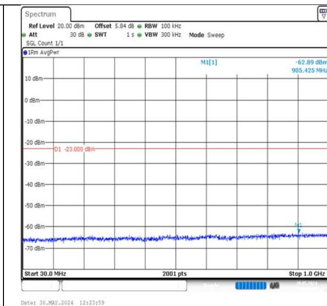
Band2-3MHz-16QAM-18900-15RB#0-30~1000-PASS
