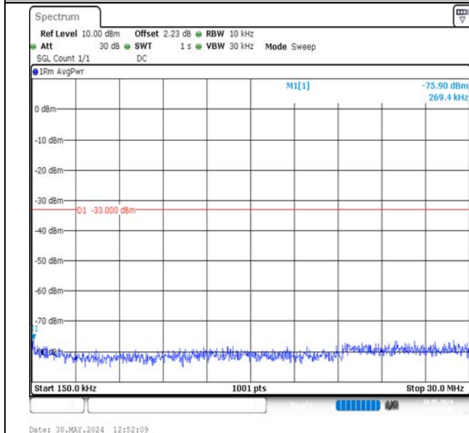
Band2-1.4MHz-16QAM-19193-1RB#5-0.15~30-PASS
