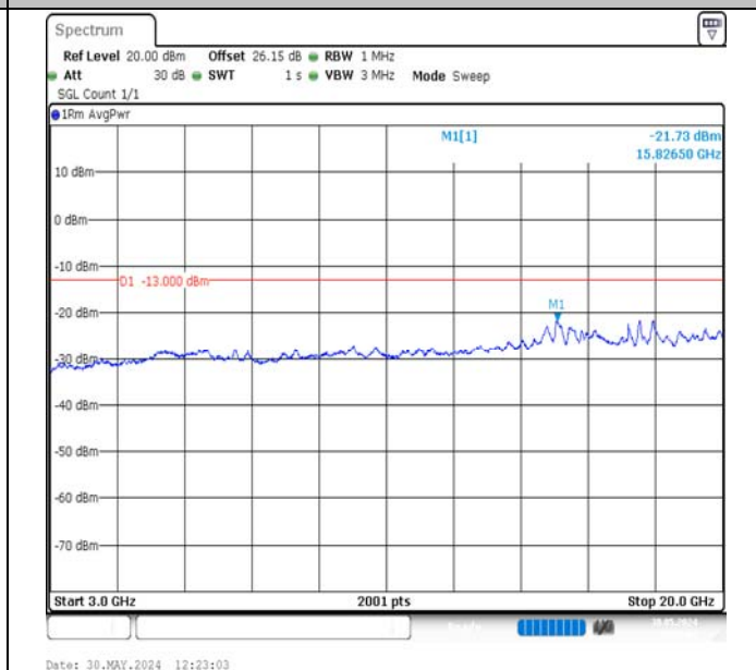
Band2-3MHz-QPSK-18900-1RB#14-3000~20000-PASS
