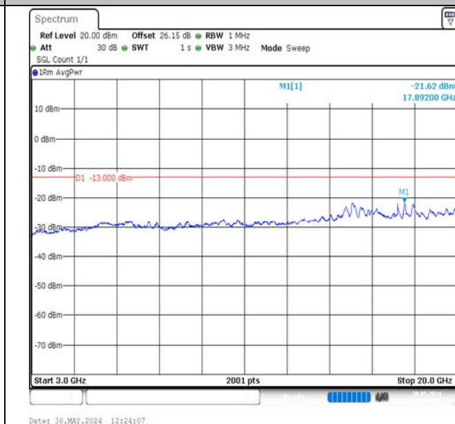
Band2-3MHz-16QAM-18900-15RB#0-3000~20000-PASS
