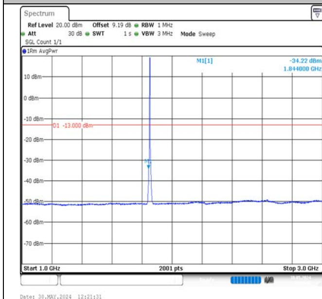
Band2-3MHz-QPSK-18615-15RB#0-1000~3000-PASS
