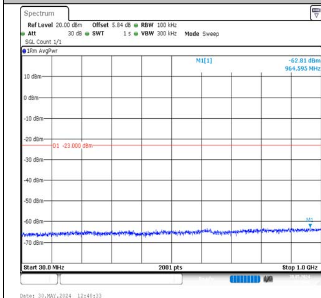
Band2-5MHz-QPSK-18625-1RB#0-30~1000-PASS
