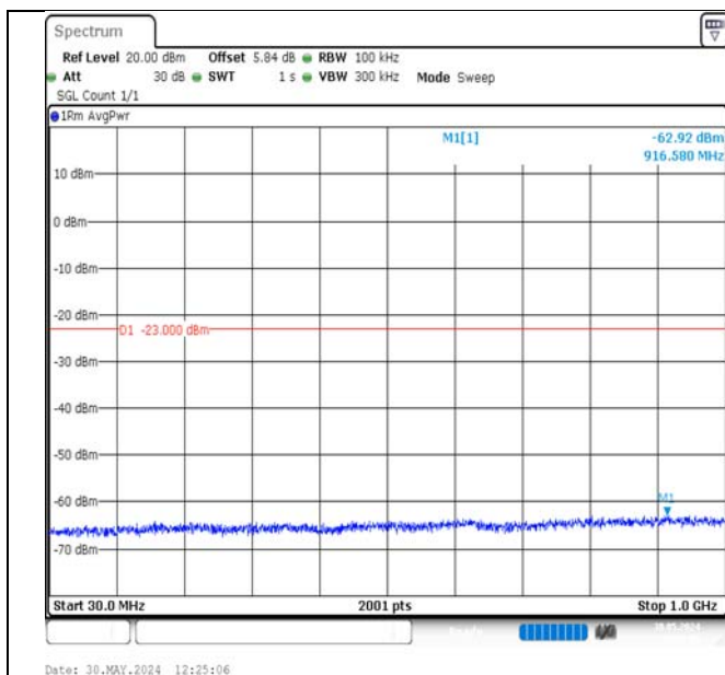
Band2-3MHz-QPSK-19185-1RB#14-30~1000-PASS
