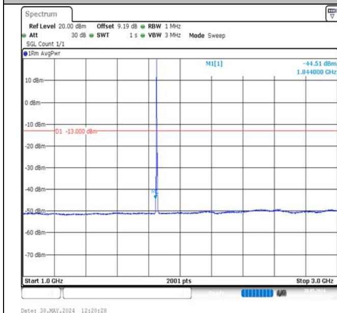
Band2-3MHz-16QAM-18615-1RB#0-1000~3000-PASS
