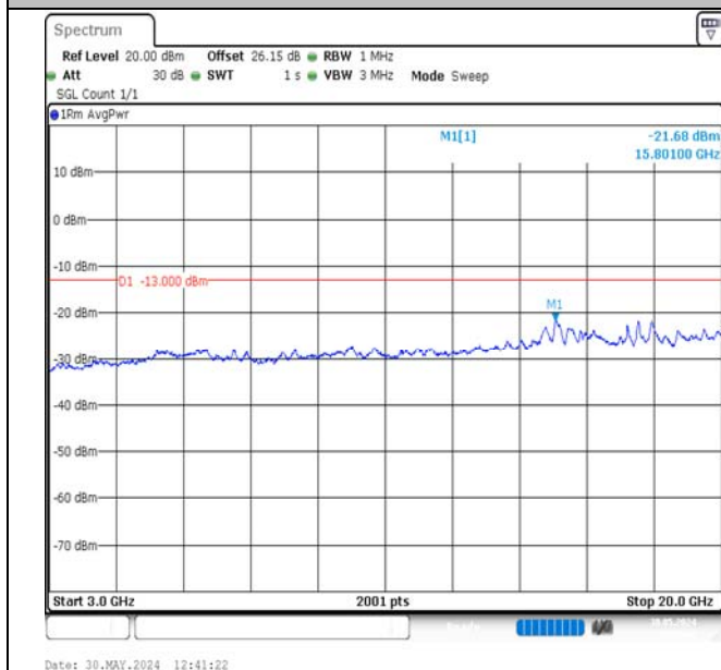
Band2-5MHz-QPSK-18625-1RB#24-3000~20000-PASS
