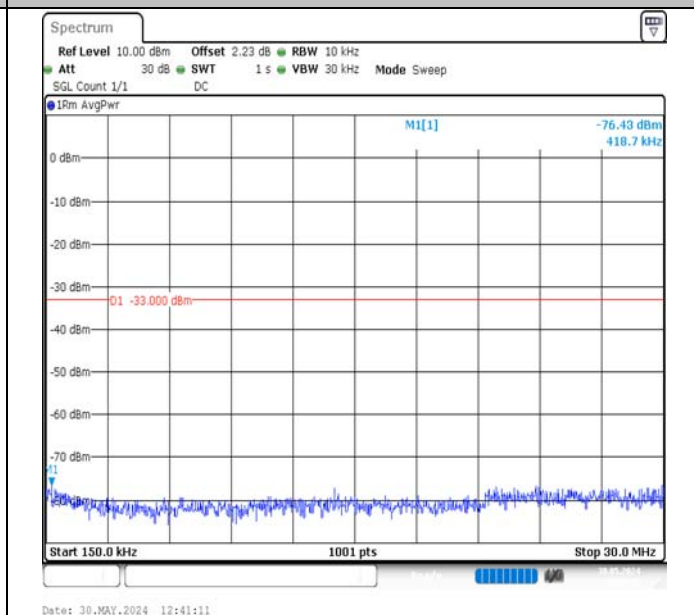
Band2-5MHz-QPSK-18625-1RB#24-0.15~30-PASS
