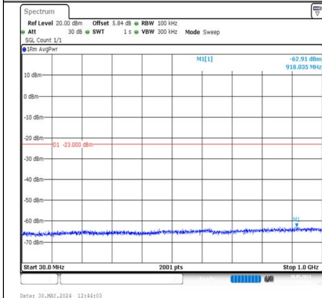
Band2-5MHz-QPSK-18900-25RB#0-30~1000-PASS
