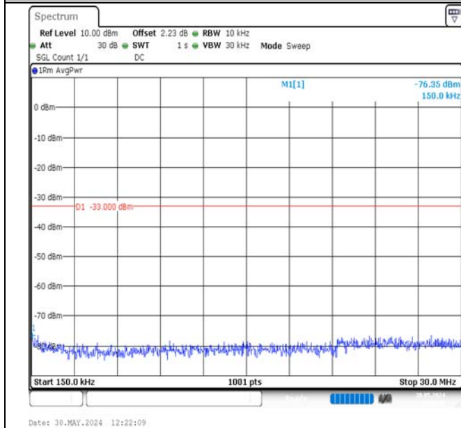
Band2-3MHz-QPSK-18900-1RB#0-0.15~30-PASS
