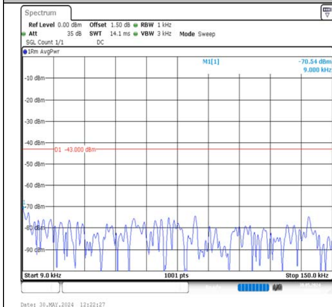
Band2-3MHz-16QAM-18900-1RB#0-0.009~0.15-PASS
