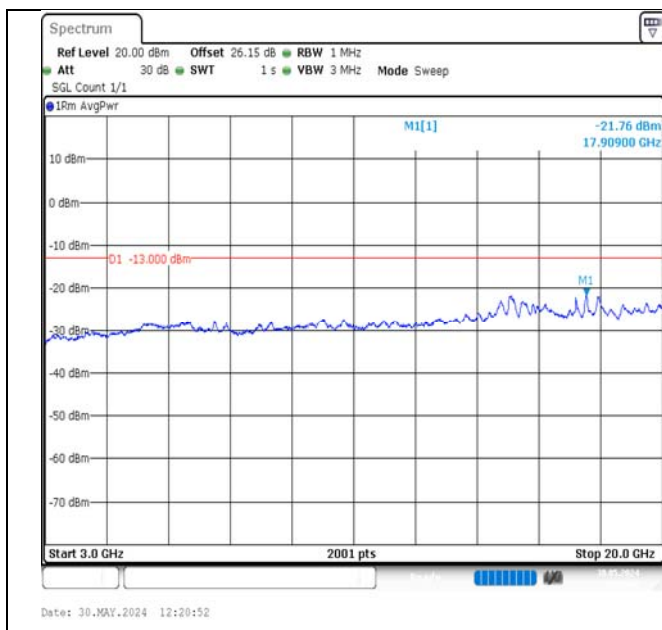
Band2-3MHz-QPSK-18615-1RB#14-3000~20000-PASS
