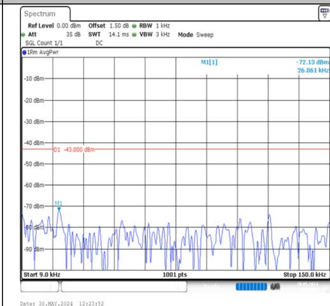
Band2-3MHz-16QAM-18900-15RB#0-0.009~0.15-PASS
