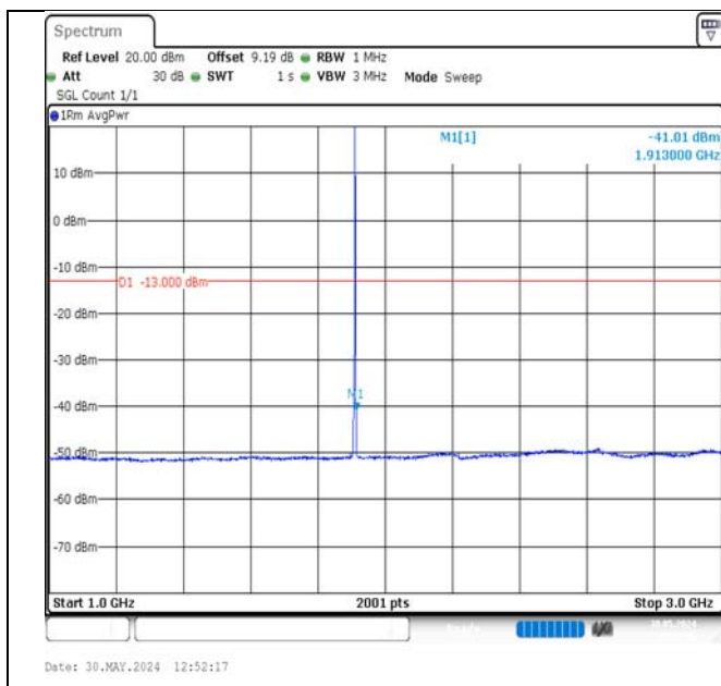
Band2-1.4MHz-16QAM-19193-1RB#5-1000~3000-PASS
