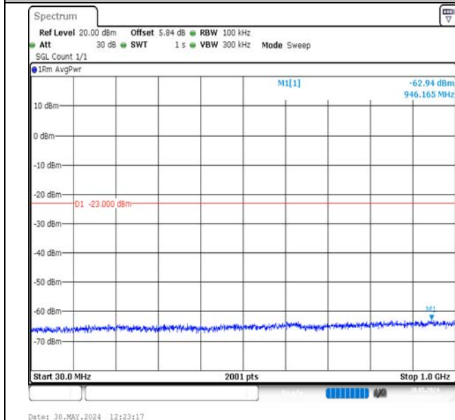
Band2-3MHz-16QAM-18900-1RB#14-30~1000-PASS
