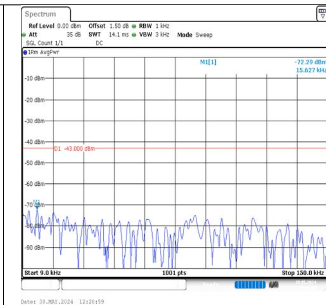
Band2-3MHz-16QAM-18615-1RB#14-0.009~0.15-PASS
