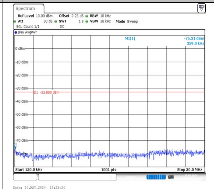
Band2-3MHz-QPSK-18900-15RB#0-0.15~30-PASS
