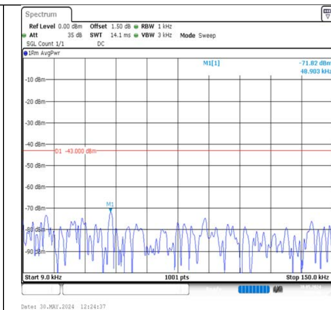
Band2-3MHz-16QAM-19185-1RB#0-0.009~0.15-PASS
