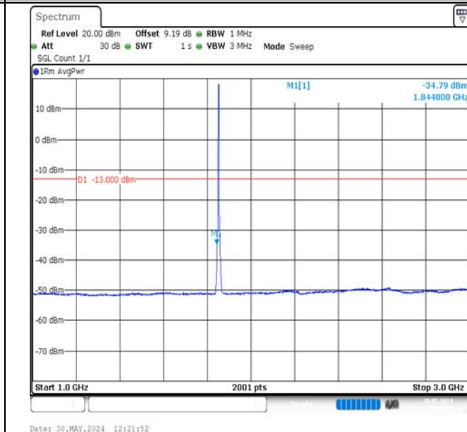
Band2-3MHz-16QAM-18615-15RB#0-1000~3000-PASS
