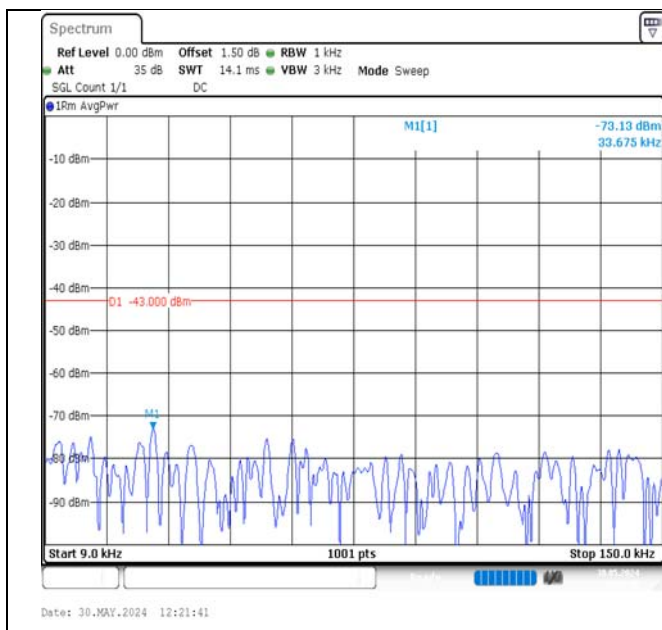
Band2-3MHz-16QAM-18615-15RB#0-0.009~0.15-PASS
