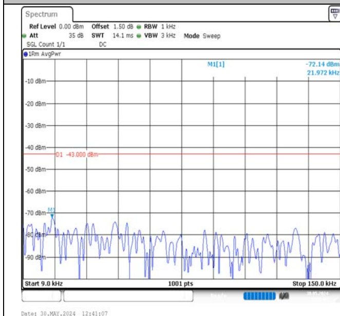
Band2-5MHz-QPSK-18625-1RB#24-0.009~0.15-PASS
