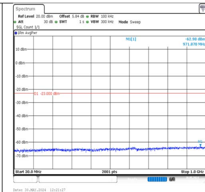
Band2-3MHz-QPSK-18615-15RB#0-30~1000-PASS
