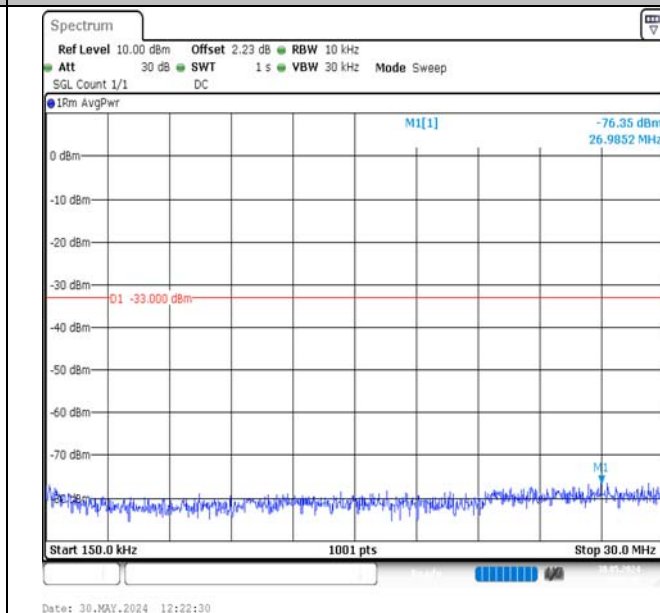
Band2-3MHz-16QAM-18900-1RB#0-0.15~30-PASS
