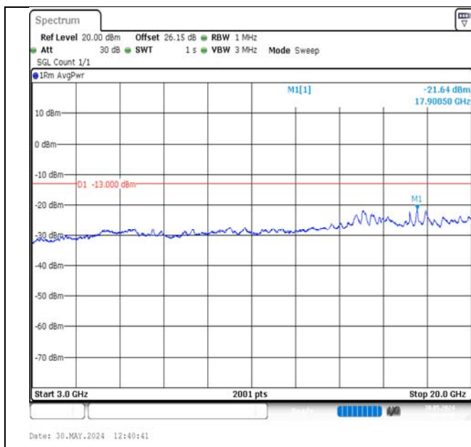
Band2-5MHz-QPSK-18625-1RB#0-3000~20000-PASS
