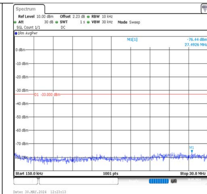
Band2-3MHz-16QAM-18900-1RB#14-0.15~30-PASS
