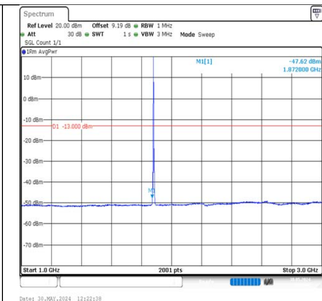
Band2-3MHz-16QAM-18900-1RB#0-1000~3000-PASS
