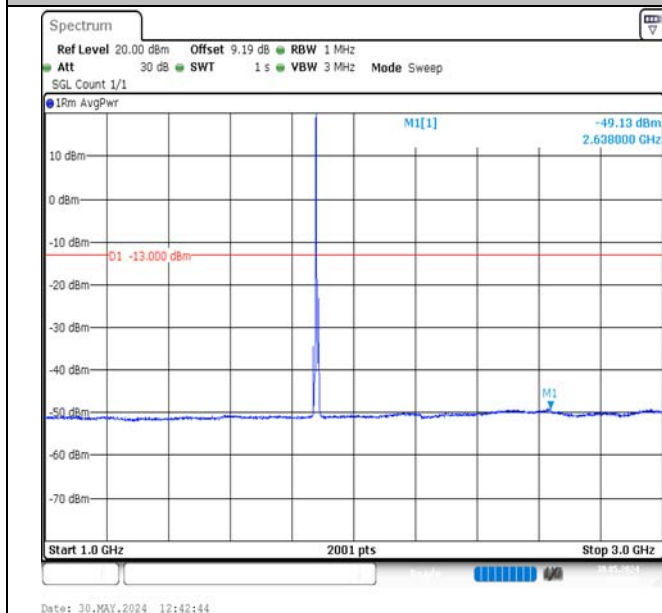
Band2-5MHz-QPSK-18900-1RB#0-1000~3000-PASS
