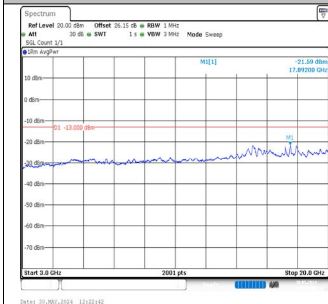
Band2-3MHz-16QAM-18900-1RB#0-3000~20000-PASS
