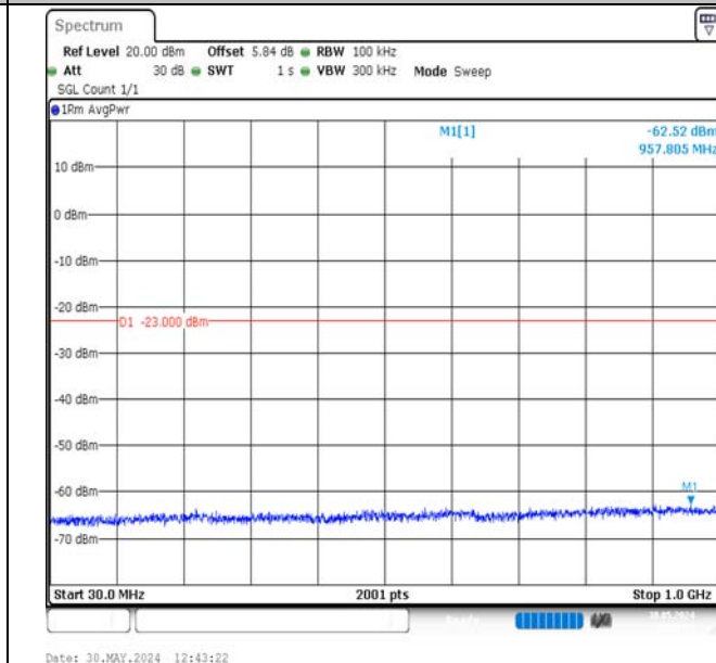
Band2-5MHz-QPSK-18900-1RB#24-30~1000-PASS
