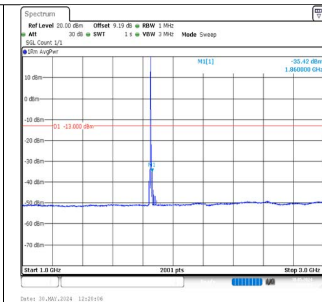
Band2-3MHz-QPSK-18615-1RB#0-1000~3000-PASS
