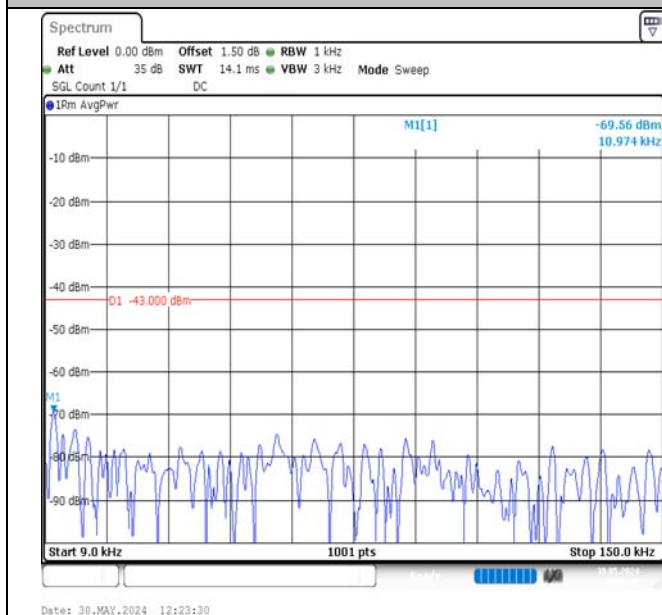
Band2-3MHz-QPSK-18900-15RB#0-0.009~0.15-PASS
