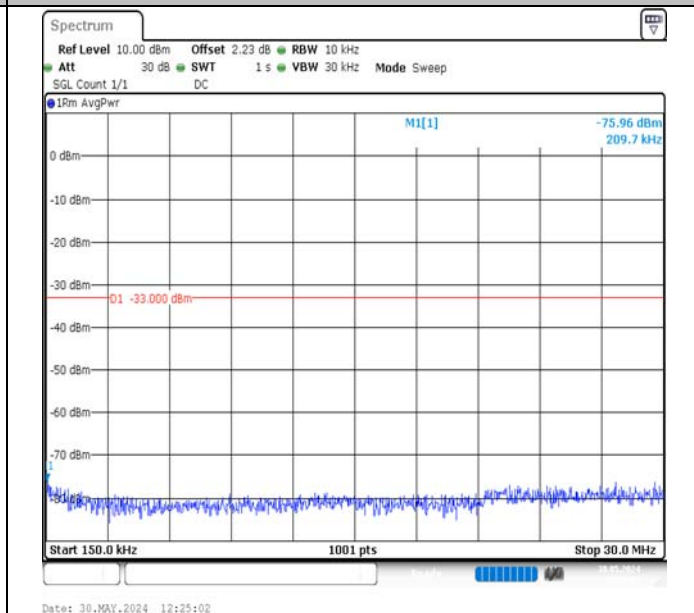
Band2-3MHz-QPSK-19185-1RB#14-0.15~30-PASS
