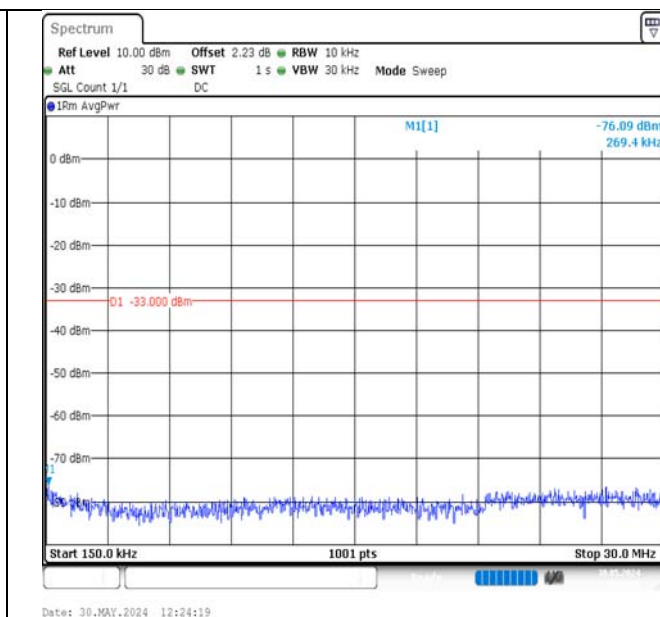
Band2-3MHz-QPSK-19185-1RB#0-0.15~30-PASS
