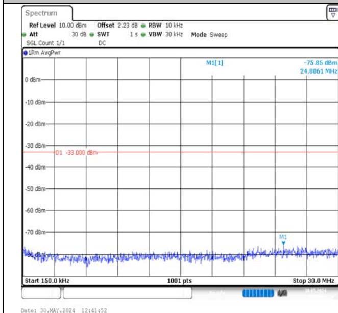
Band2-5MHz-QPSK-18625-25RB#0-0.15~30-PASS
