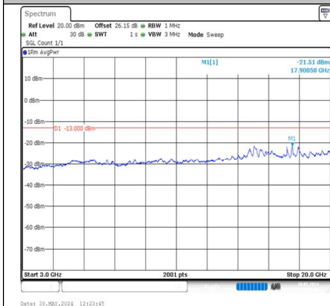
Band2-3MHz-QPSK-18900-15RB#0-3000~20000-PASS
