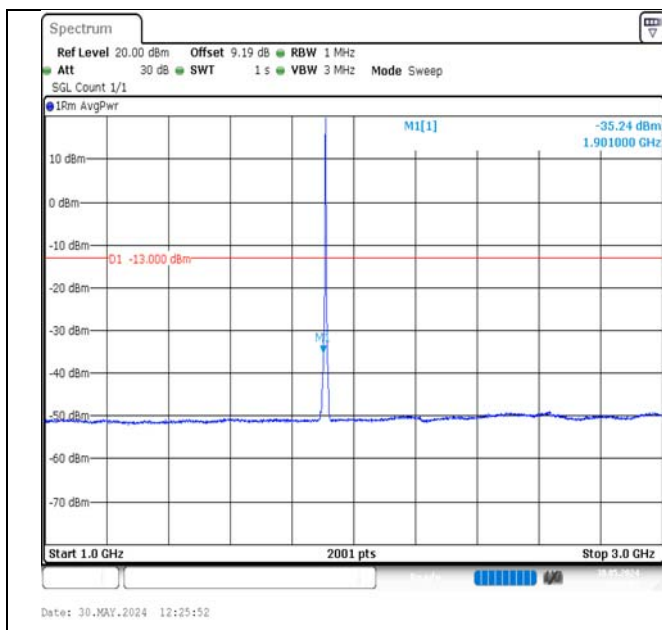
Band2-3MHz-QPSK-19185-15RB#0-1000~3000-PASS
