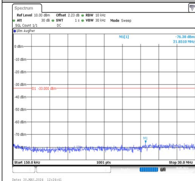
Band2-3MHz-16QAM-19185-1RB#0-0.15~30-PASS
