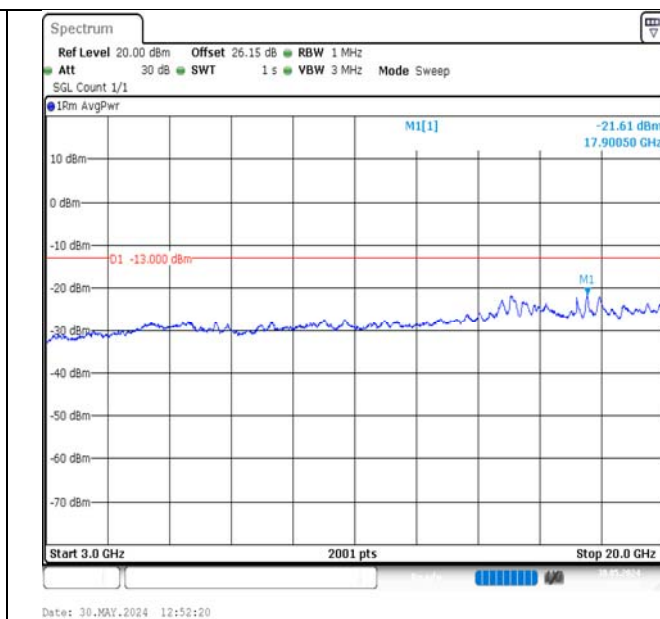
Band2-1.4MHz-16QAM-19193-1RB#5-3000~20000-PASS
