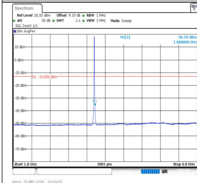
Band2-3MHz-16QAM-18900-15RB#0-1000~3000-PASS
