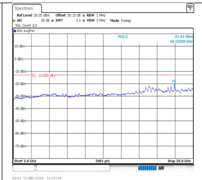
Band2-3MHz-QPSK-19185-15RB#0-3000~20000-PASS
