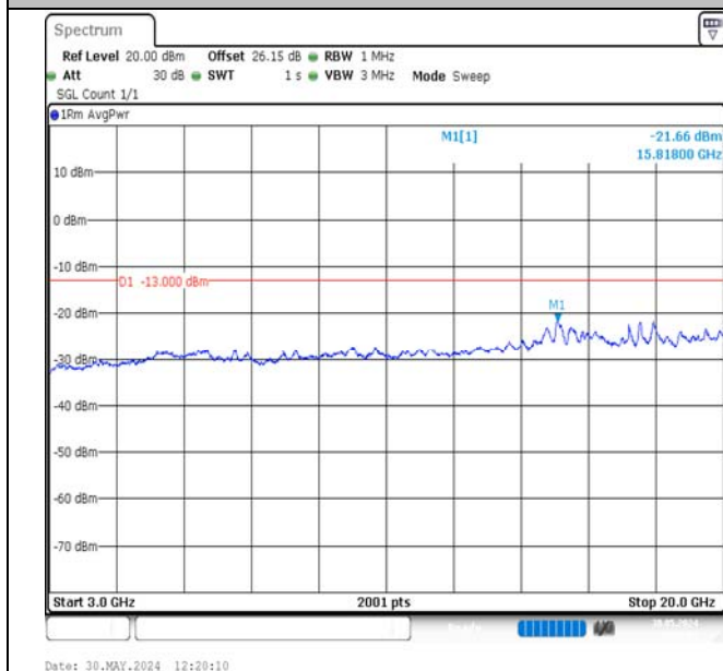
Band2-3MHz-QPSK-18615-1RB#0-3000~20000-PASS
