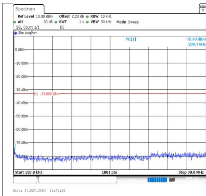
Band2-5MHz-QPSK-18900-1RB#0-0.15~30-PASS
