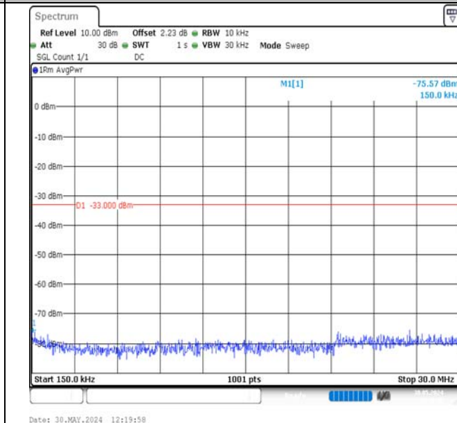
Band2-3MHz-QPSK-18615-1RB#0-0.15~30-PASS
