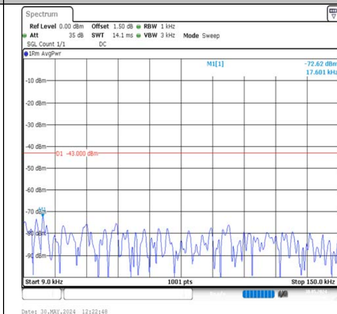
Band2-3MHz-QPSK-18900-1RB#14-0.009~0.15-PASS
