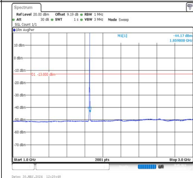
Band2-3MHz-QPSK-18615-1RB#14-1000~3000-PASS
