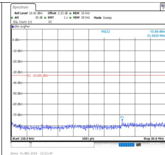
Band2-3MHz-16QAM-18615-15RB#0-0.15~30-PASS
