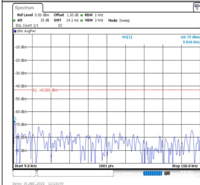
Band2-3MHz-QPSK-19185-1RB#14-0.009~0.15-PASS
