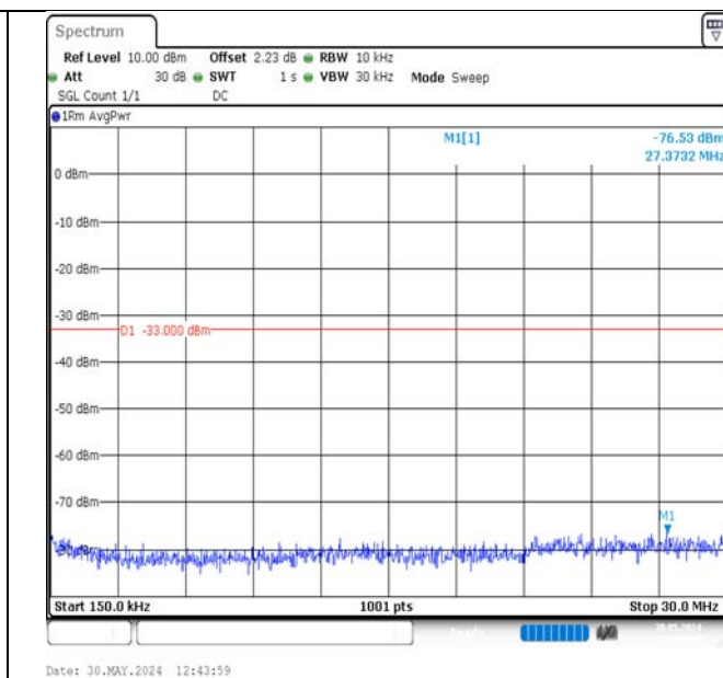
Band2-5MHz-QPSK-18900-25RB#0-0.15~30-PASS
