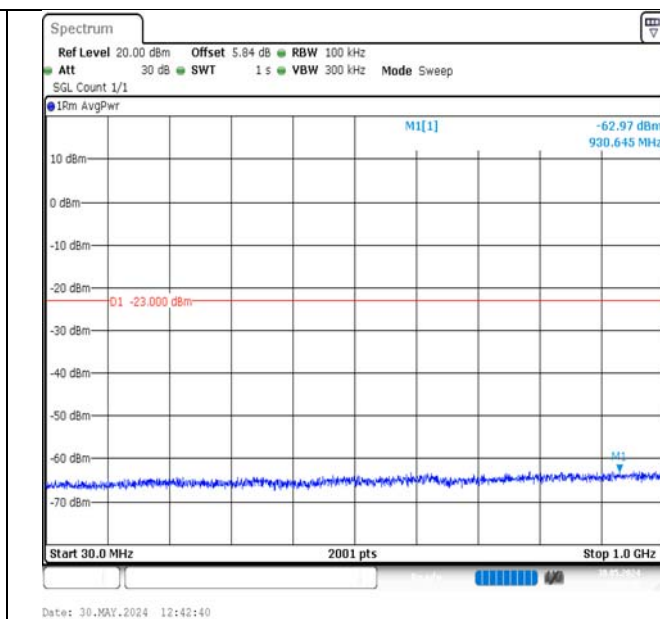
Band2-5MHz-QPSK-18900-1RB#0-30~1000-PASS
