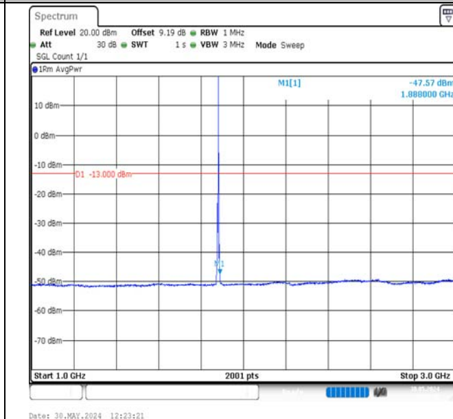
Band2-3MHz-16QAM-18900-1RB#14-1000~3000-PASS
