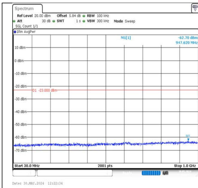
Band2-3MHz-16QAM-18900-1RB#0-30~1000-PASS
