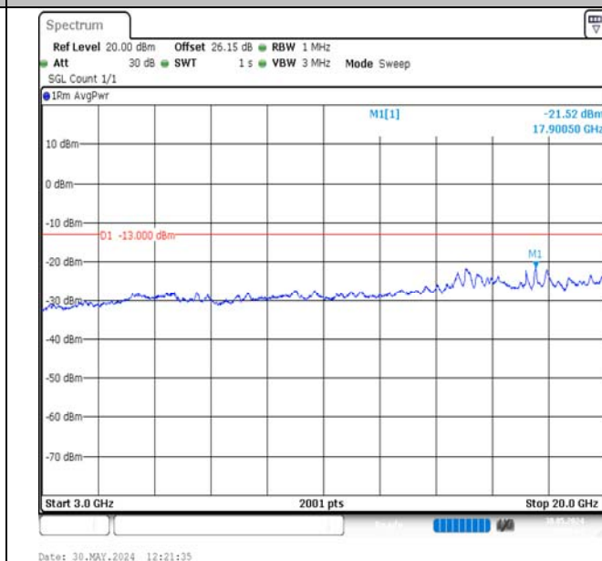
Band2-3MHz-QPSK-18615-15RB#0-3000~20000-PASS
