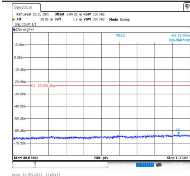
Band2-3MHz-QPSK-18615-1RB#14-30~1000-PASS
