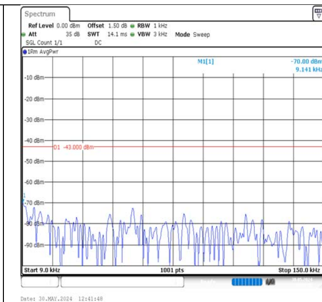
Band2-5MHz-QPSK-18625-25RB#0-0.009~0.15-PASS
