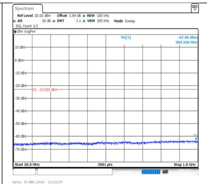
Band2-3MHz-QPSK-18900-1RB#14-30~1000-PASS
