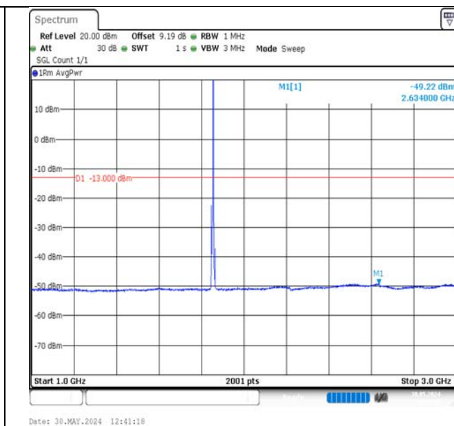
Band2-5MHz-QPSK-18625-1RB#24-1000~3000-PASS
