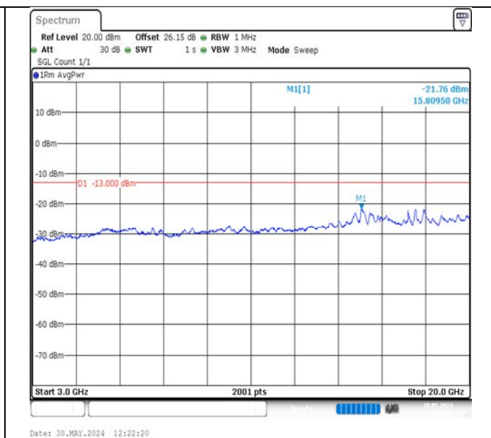
Band2-3MHz-QPSK-18900-1RB#0-3000~20000-PASS
