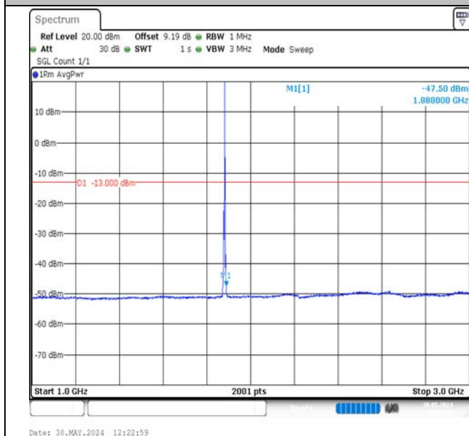
Band2-3MHz-QPSK-18900-1RB#14-1000~3000-PASS
