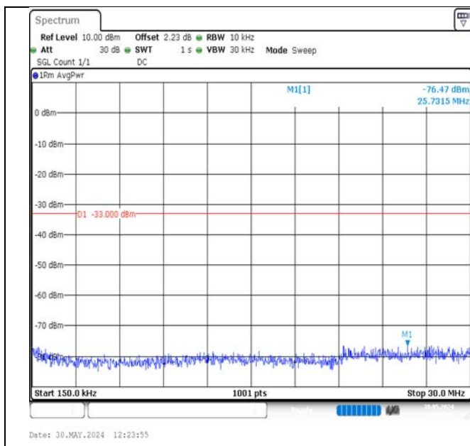
Band2-3MHz-16QAM-18900-15RB#0-0.15~30-PASS
