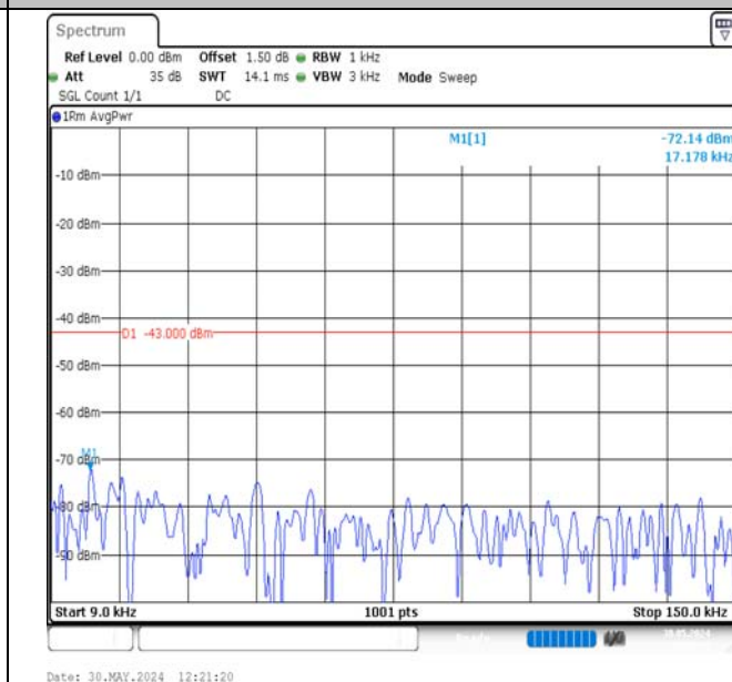
Band2-3MHz-QPSK-18615-15RB#0-0.009~0.15-PASS
