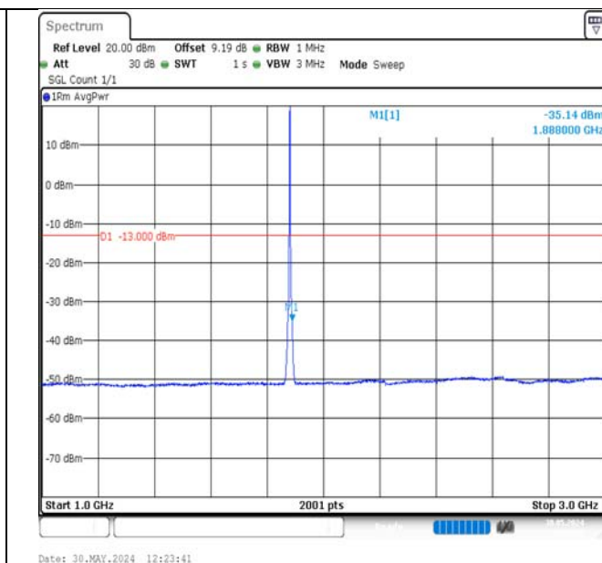
Band2-3MHz-QPSK-18900-15RB#0-1000~3000-PASS
