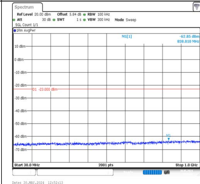
Band2-1.4MHz-16QAM-19193-1RB#5-30~1000-PASS
