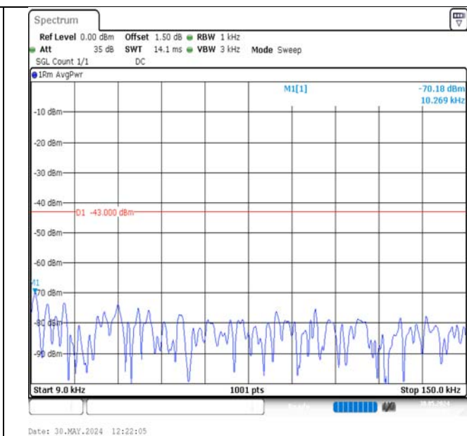
Band2-3MHz-QPSK-18900-1RB#0-0.009~0.15-PASS
