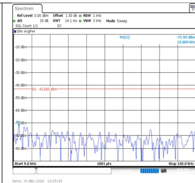
Band2-3MHz-QPSK-19185-15RB#0-0.009~0.15-PASS
