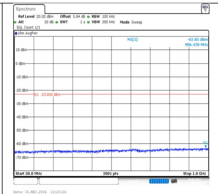
Band2-3MHz-16QAM-18615-1RB#0-30~1000-PASS
