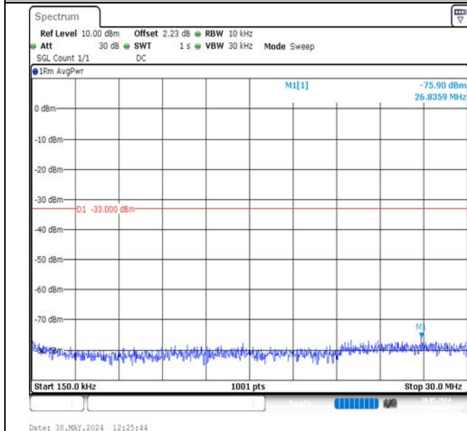
Band2-3MHz-QPSK-19185-15RB#0-0.15~30-PASS
