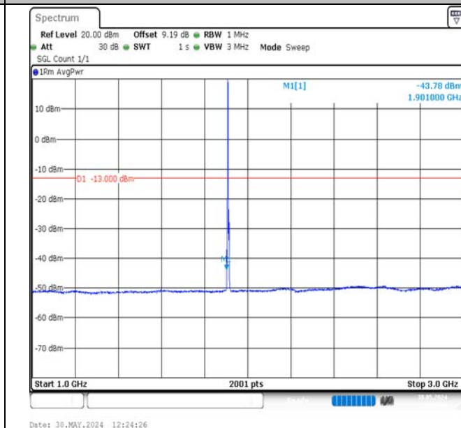
Band2-3MHz-QPSK-19185-1RB#0-1000~3000-PASS
