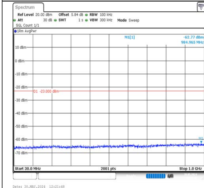
Band2-3MHz-16QAM-18615-15RB#0-30~1000-PASS
