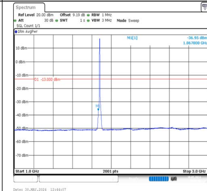
Band2-5MHz-QPSK-18900-25RB#0-1000~3000-PASS
