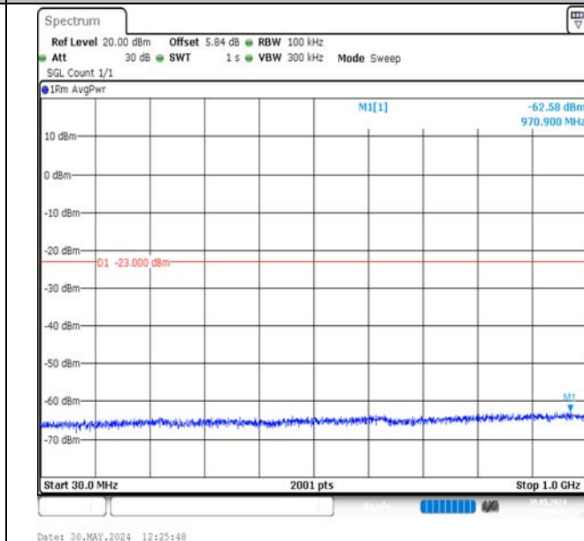
Band2-3MHz-QPSK-19185-15RB#0-30~1000-PASS
