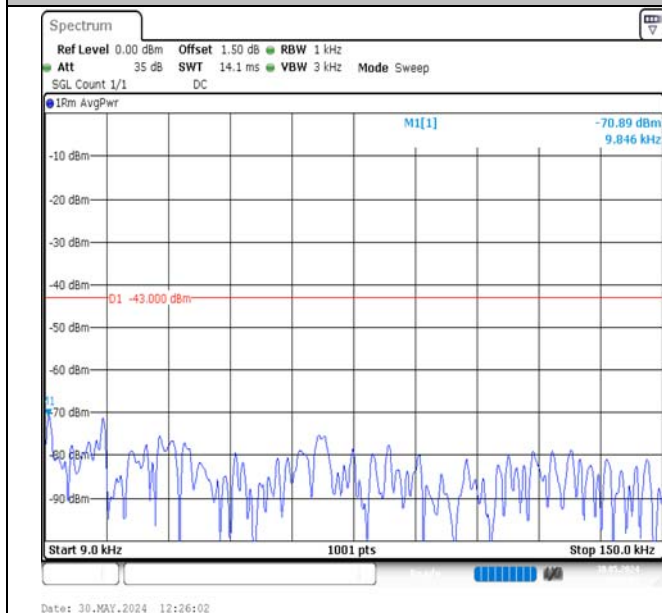
Band2-3MHz-16QAM-19185-15RB#0-0.009~0.15-PASS
