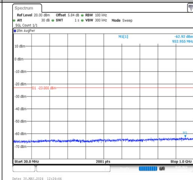
Band2-3MHz-16QAM-19185-1RB#0-30~1000-PASS
