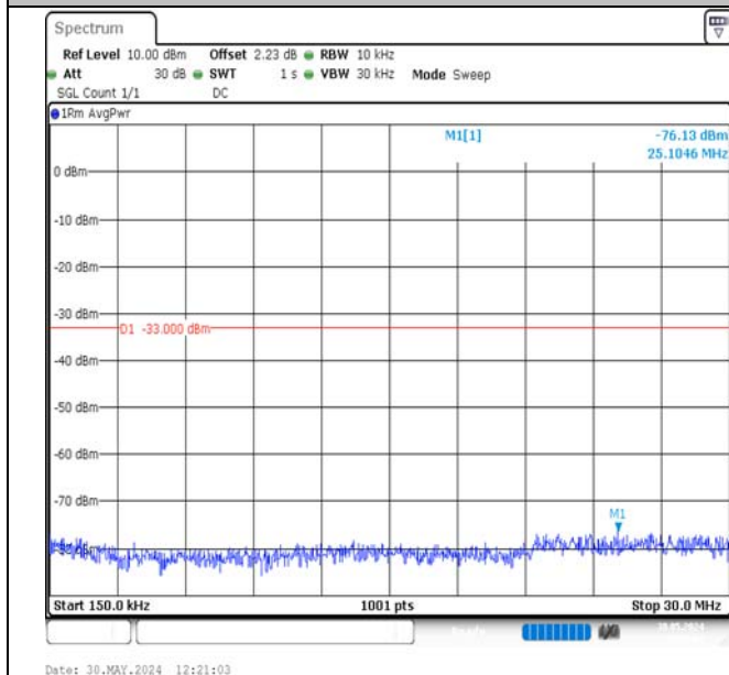
Band2-3MHz-16QAM-18615-1RB#14-0.15~30-PASS
