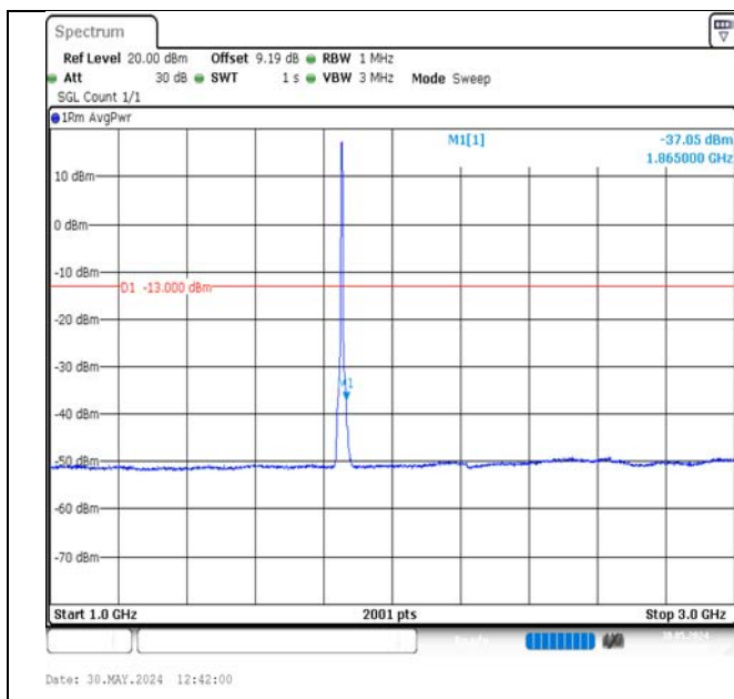
Band2-5MHz-QPSK-18625-25RB#0-1000~3000-PASS
