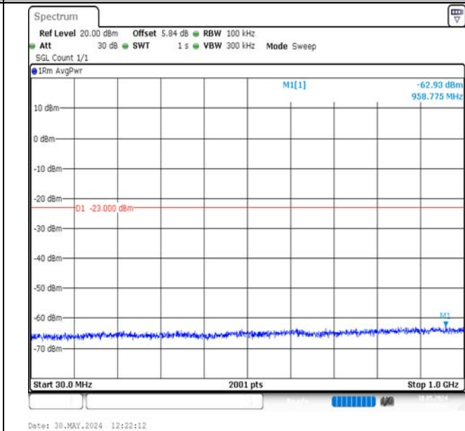
Band2-3MHz-QPSK-18900-1RB#0-30~1000-PASS
