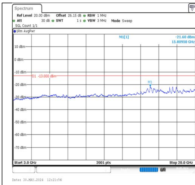
Band2-3MHz-16QAM-18615-15RB#0-3000~20000-PASS
