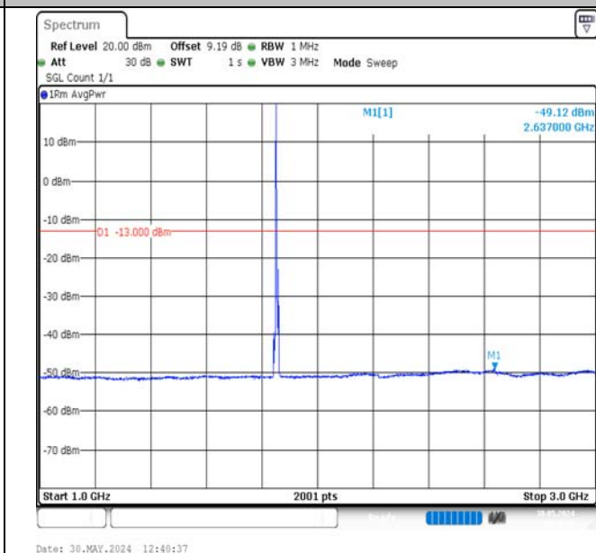
Band2-5MHz-QPSK-18625-1RB#0-1000~3000-PASS
