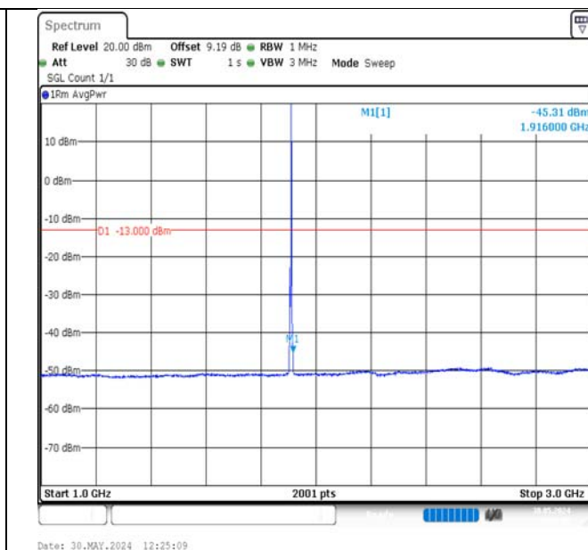
Band2-3MHz-QPSK-19185-1RB#14-1000~3000-PASS
