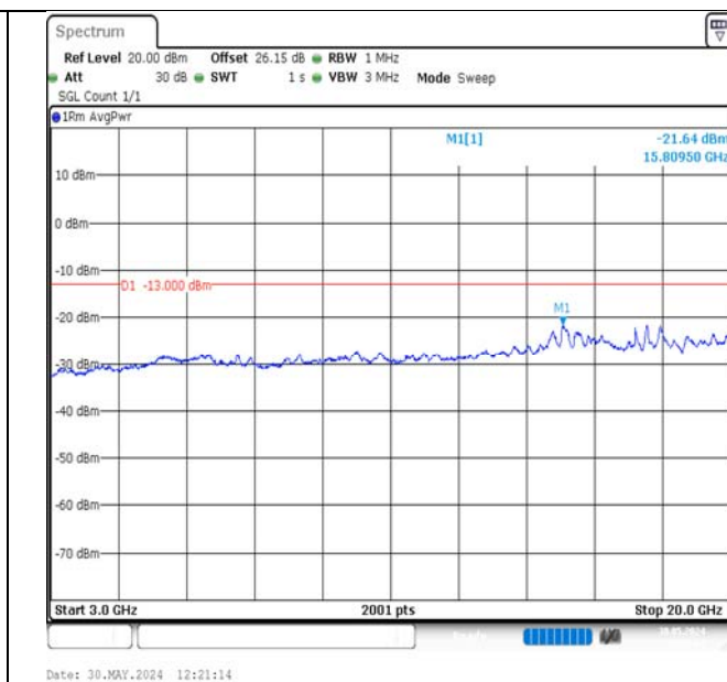
Band2-3MHz-16QAM-18615-1RB#14-3000~20000-PASS
