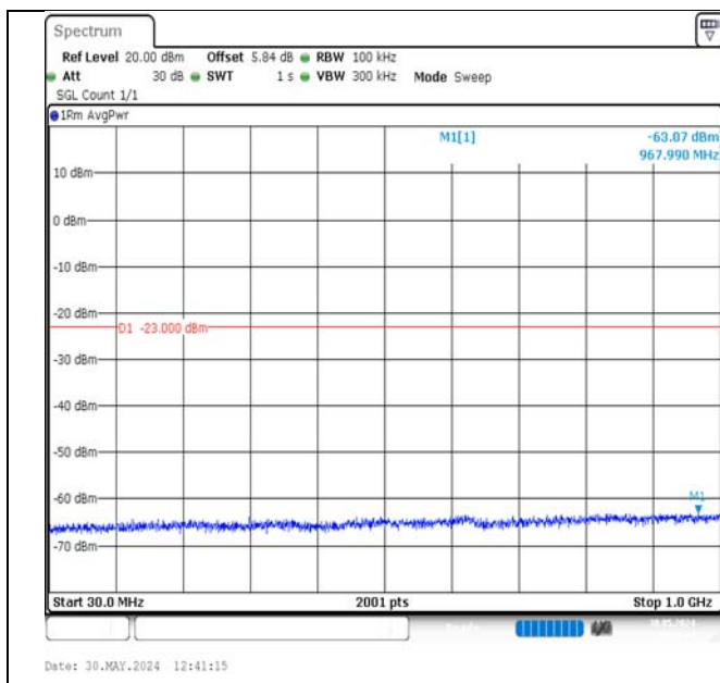
Band2-5MHz-QPSK-18625-1RB#24-30~1000-PASS
