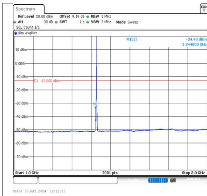
Band2-3MHz-16QAM-18615-1RB#14-1000~3000-PASS
