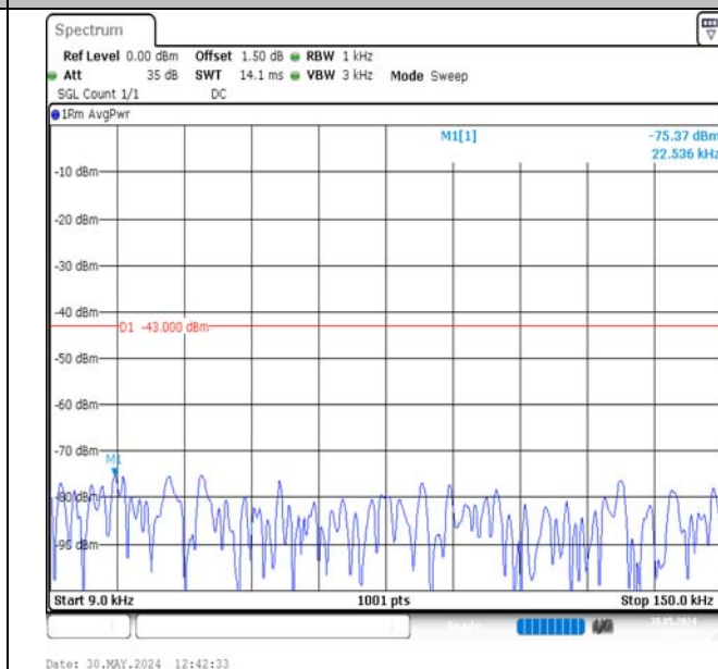
Band2-5MHz-QPSK-18900-1RB#0-0.009~0.15-PASS
