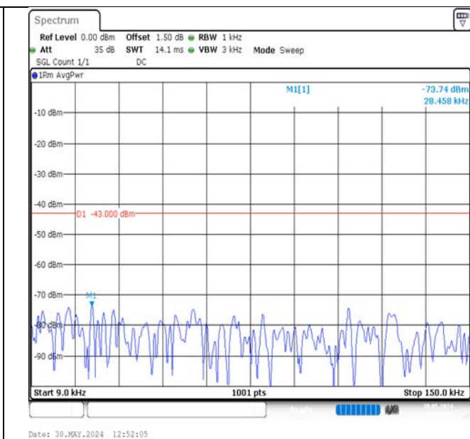
Band2-1.4MHz-16QAM-19193-1RB#5-0.009~0.15-PASS
