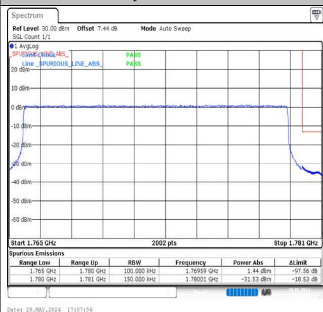
Band66-15MHz-QPSK-132597-75RB#0-PASS
