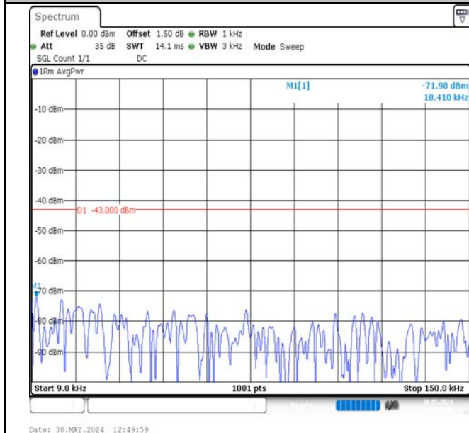
Band2-1.4MHz-16QAM-18900-1RB#5-0.009~0.15-PASS
