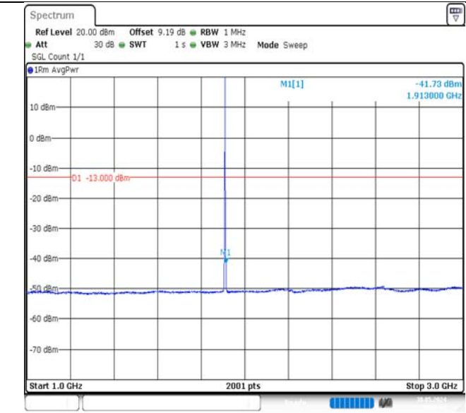
Band2-1.4MHz-QPSK-19193-1RB#0-1000~3000-PASS
