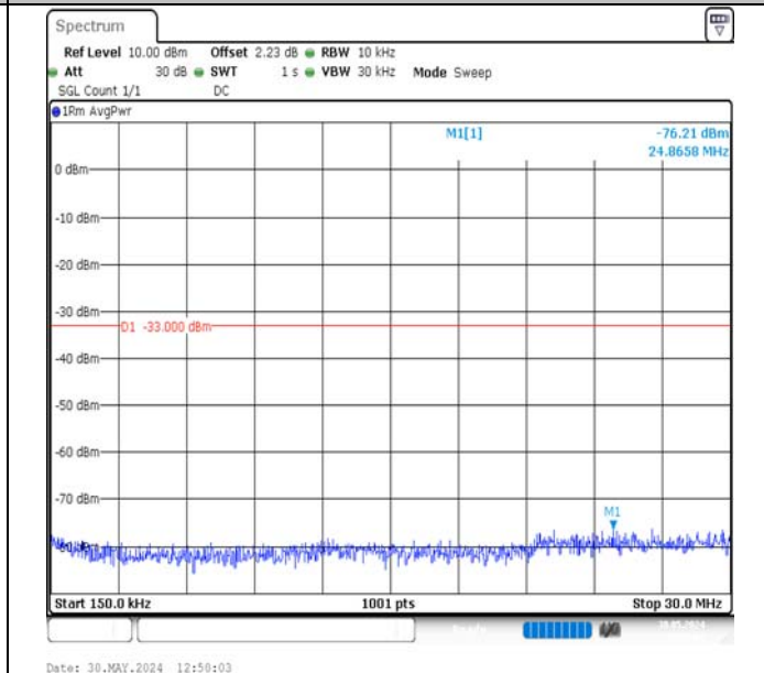
Band2-1.4MHz-16QAM-18900-1RB#5-0.15~30-PASS
