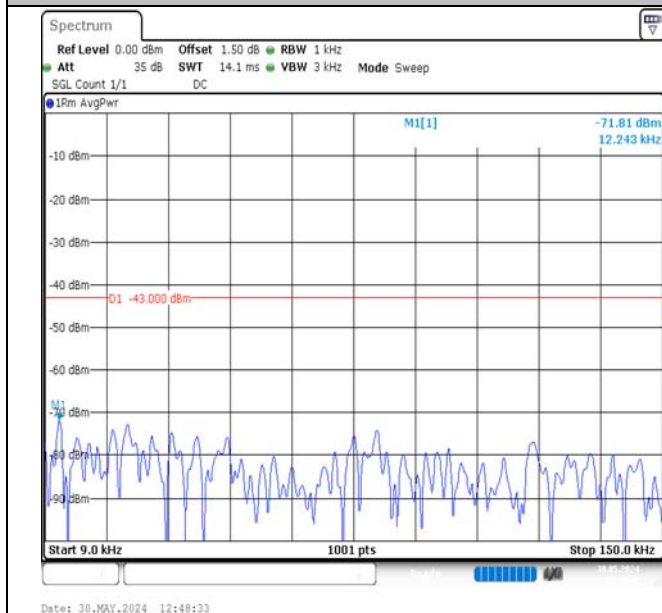
Band2-1.4MHz-16QAM-18607-6RB#0-0.009~0.15-PASS
