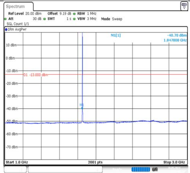
Band2-1.4MHz-QPSK-18607-1RB#5-1000~3000-PASS
