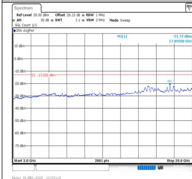
Band2-1.4MHz-16QAM-18900-1RB#5-3000~20000-PASS
