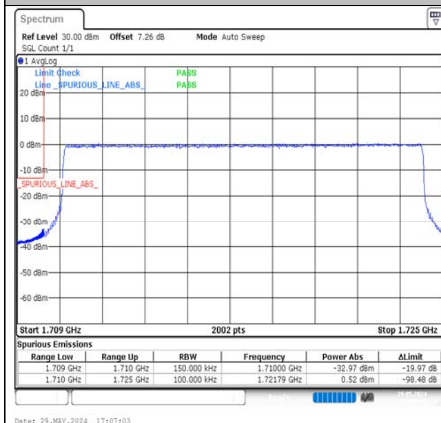
Band66-15MHz-16QAM-132047-75RB#0-PASS
