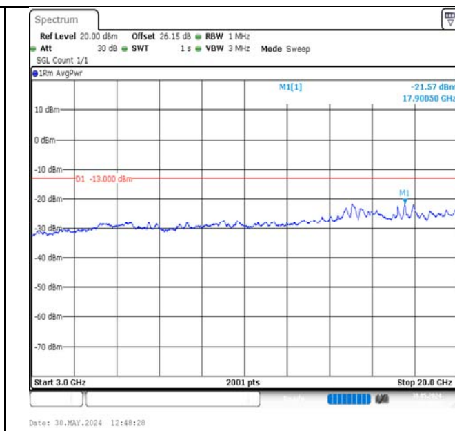
Band2-1.4MHz-QPSK-18607-6RB#0-3000~20000-PASS
