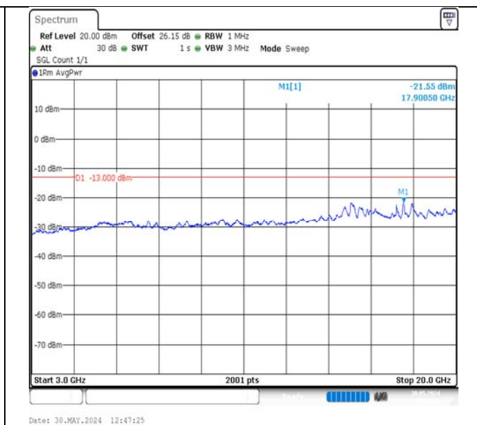
Band2-1.4MHz-16QAM-18607-1RB#0-3000~20000-PASS
