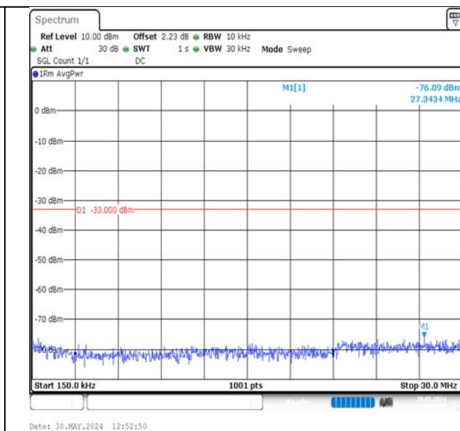
Band2-1.4MHz-16QAM-19193-6RB#0-0.15~30-PASS
