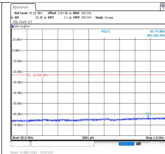
Band2-1.4MHz-16QAM-18607-1RB#5-30~1000-PASS
