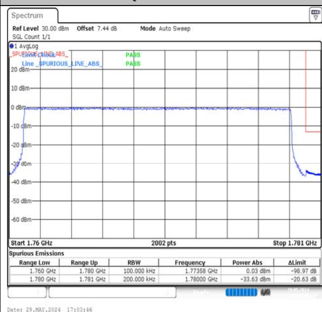
Band66-20MHz-QPSK-132572-100RB#0-PASS
