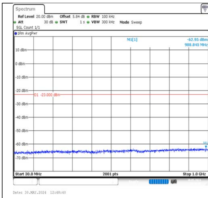
Band2-1.4MHz-16QAM-18607-6RB#0-30~1000-PASS
