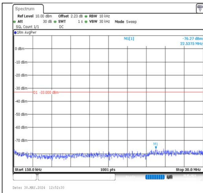
Band2-1.4MHz-QPSK-19193-6RB#0-0.15~30-PASS
