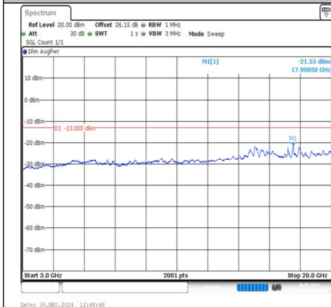
Band2-1.4MHz-16QAM-18607-6RB#0-3000~20000-PASS
