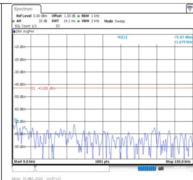
Band2-1.4MHz-16QAM-18607-1RB#0-0.009~0.15-PASS
