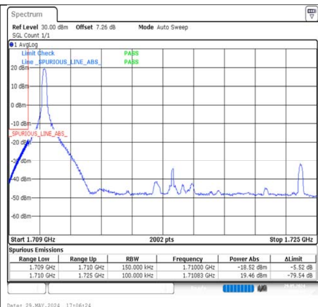
Band66-15MHz-16QAM-132047-1RB#0-PASS
