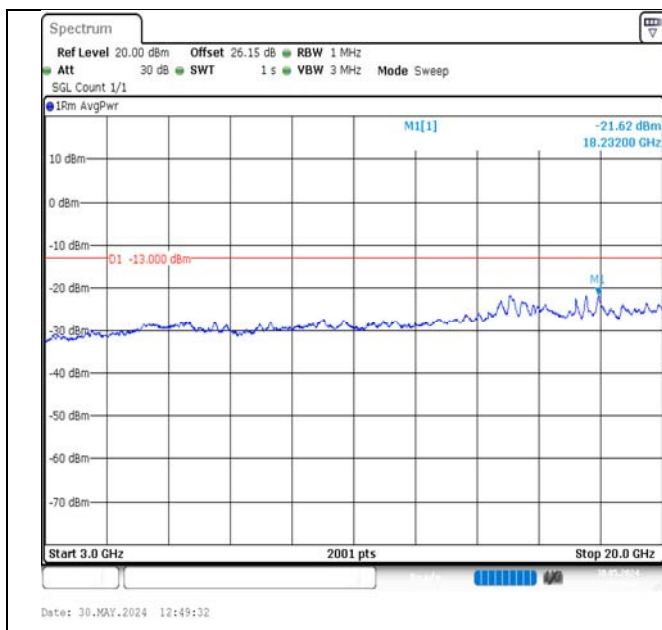
Band2-1.4MHz-16QAM-18900-1RB#0-3000~20000-PASS
