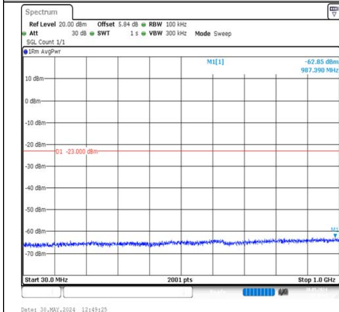
Band2-1.4MHz-16QAM-18900-1RB#0-30~1000-PASS
