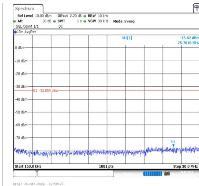
Band2-1.4MHz-QPSK-18900-6RB#0-0.15~30-PASS
