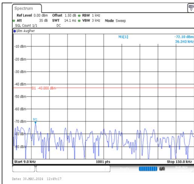
Band2-1.4MHz-16QAM-18900-1RB#0-0.009~0.15-PASS
