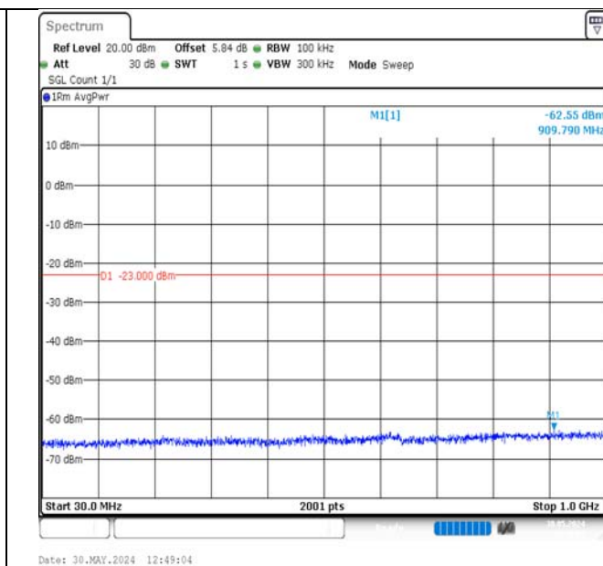
Band2-1.4MHz-QPSK-18900-1RB#0-30~1000-PASS
