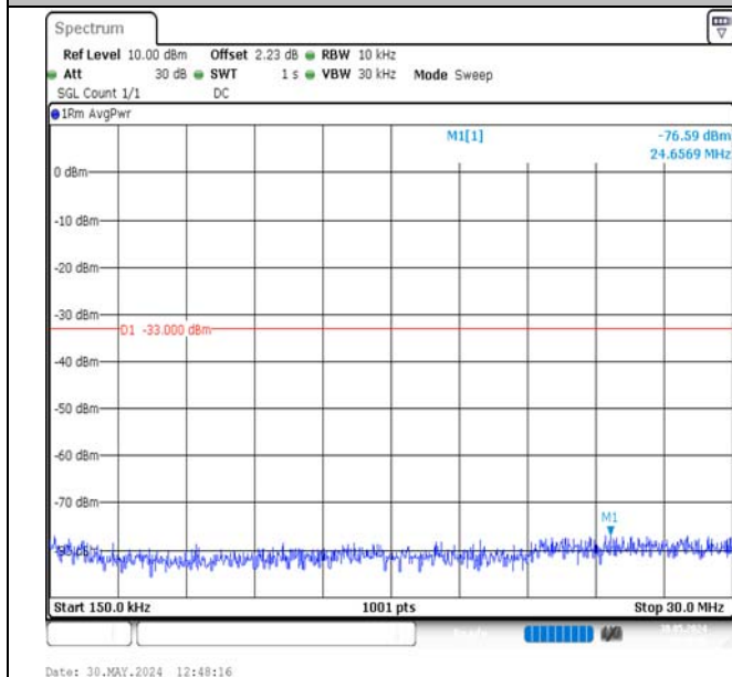
Band2-1.4MHz-QPSK-18607-6RB#0-0.15~30-PASS
