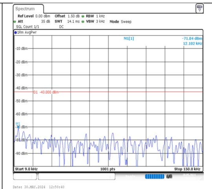
Band2-1.4MHz-16QAM-18900-6RB#0-0.009~0.15-PASS
