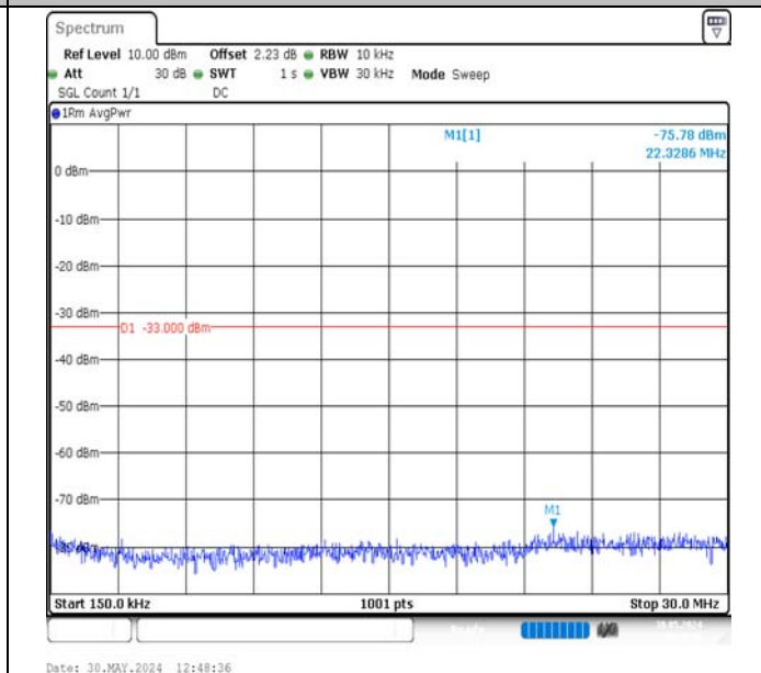
Band2-1.4MHz-16QAM-18607-6RB#0-0.15~30-PASS
