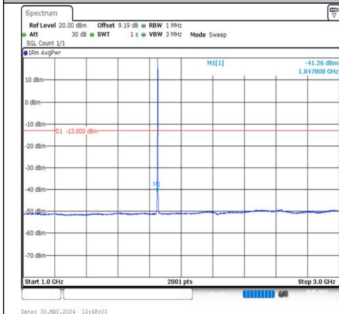
Band2-1.4MHz-16QAM-18607-1RB#5-1000~3000-PASS
