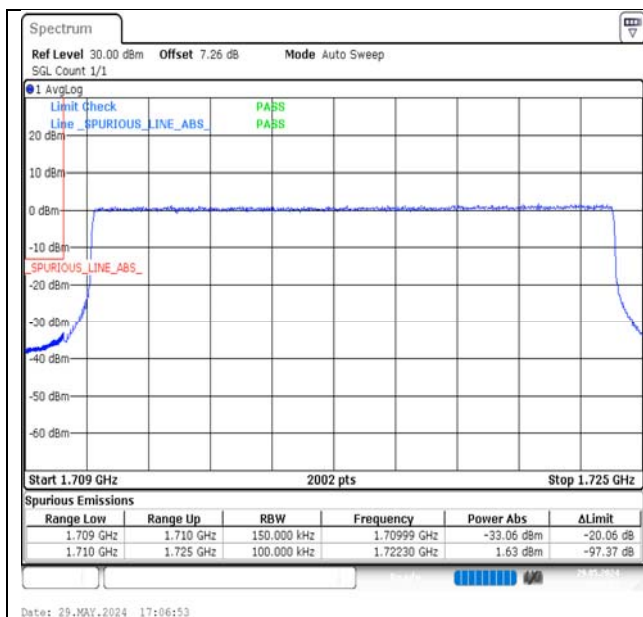
Band66-15MHz-QPSK-132047-75RB#0-PASS
