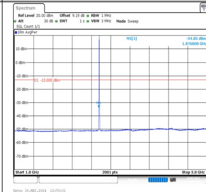
Band2-1.4MHz-QPSK-18900-6RB#0-1000~3000-PASS
