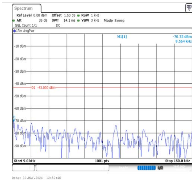
Band2-1.4MHz-16QAM-19193-6RB#0-0.009~0.15-PASS
