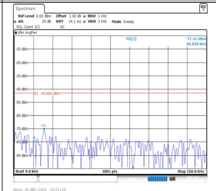
Band2-1.4MHz-16QAM-19193-1RB#0-0.009~0.15-PASS
