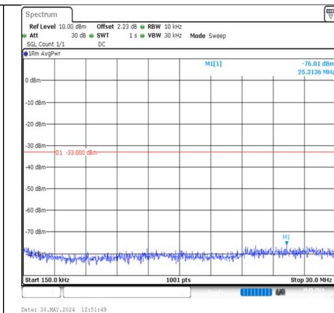
Band2-1.4MHz-QPSK-19193-1RB#5-0.15~30-PASS
