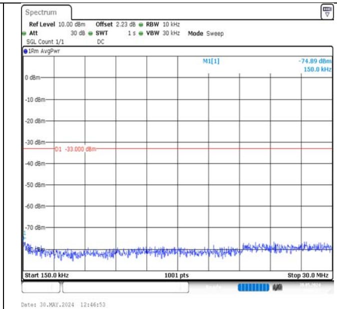
Band2-1.4MHz-QPSK-18607-1RB#0-0.15~30-PASS
