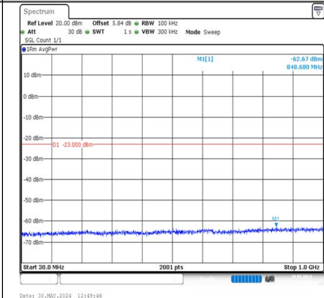
Band2-1.4MHz-QPSK-18900-1RB#5-30~1000-PASS
