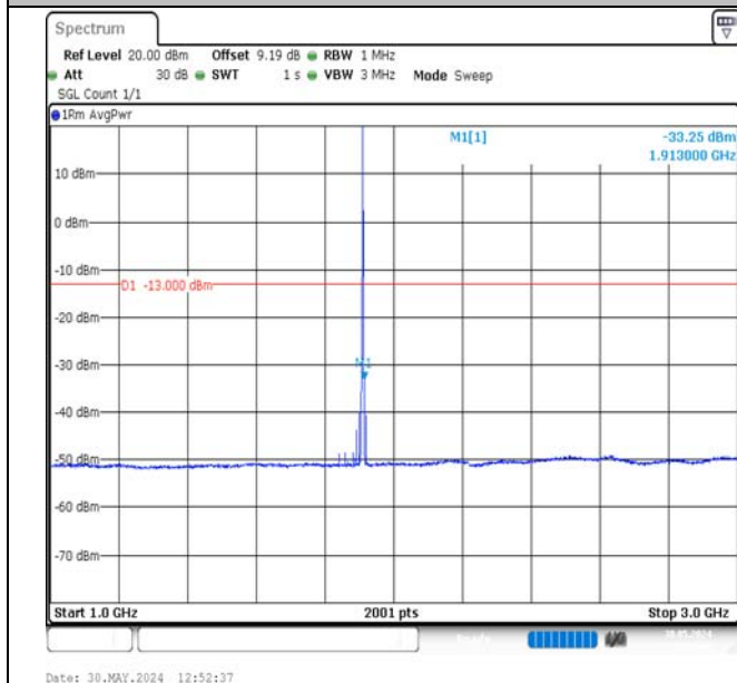
Band2-1.4MHz-QPSK-19193-6RB#0-1000~3000-PASS
