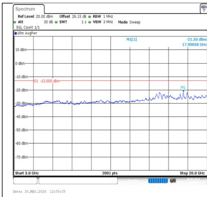
Band2-1.4MHz-QPSK-18900-6RB#0-3000~20000-PASS
