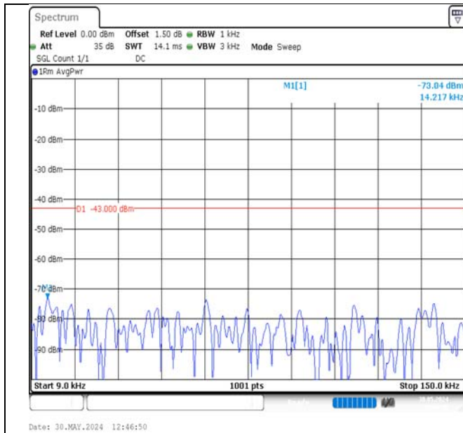
Band2-1.4MHz-QPSK-18607-1RB#0-0.009~0.15-PASS
