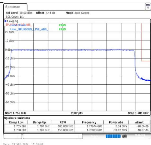
Band66-15MHz-16QAM-132597-75RB#0-PASS
