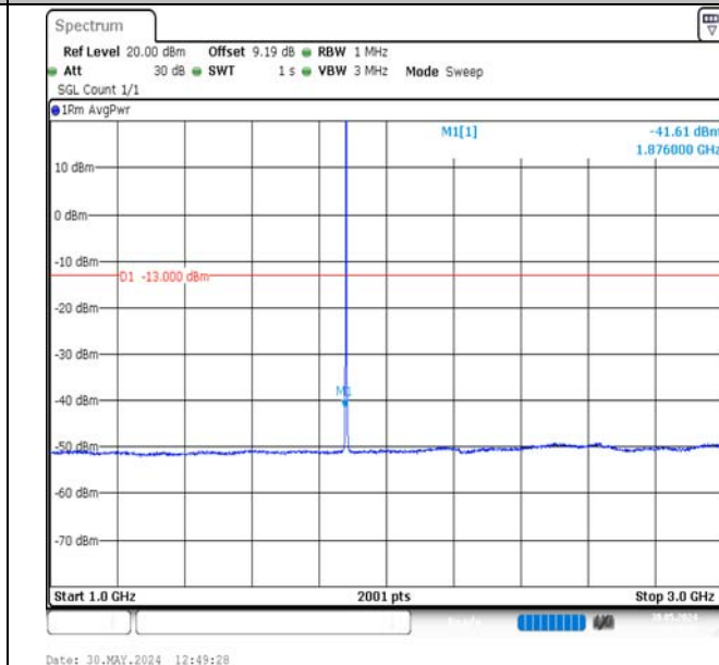
Band2-1.4MHz-16QAM-18900-1RB#0-1000~3000-PASS
