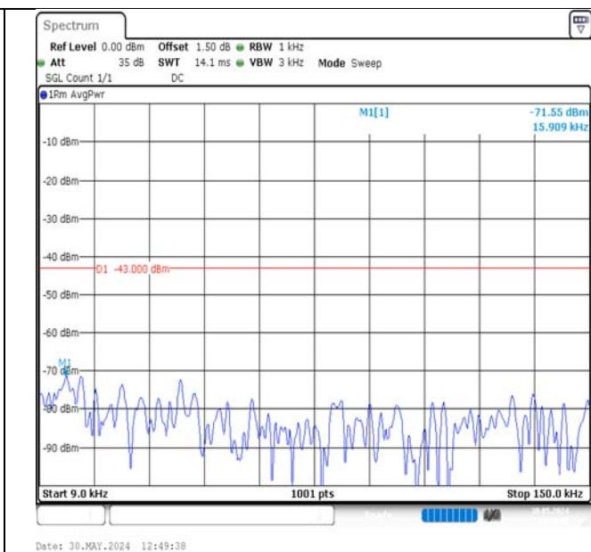
Band2-1.4MHz-QPSK-18900-1RB#5-0.009~0.15-PASS
