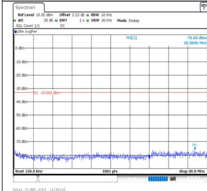
Band2-1.4MHz-QPSK-18900-1RB#5-0.15~30-PASS
