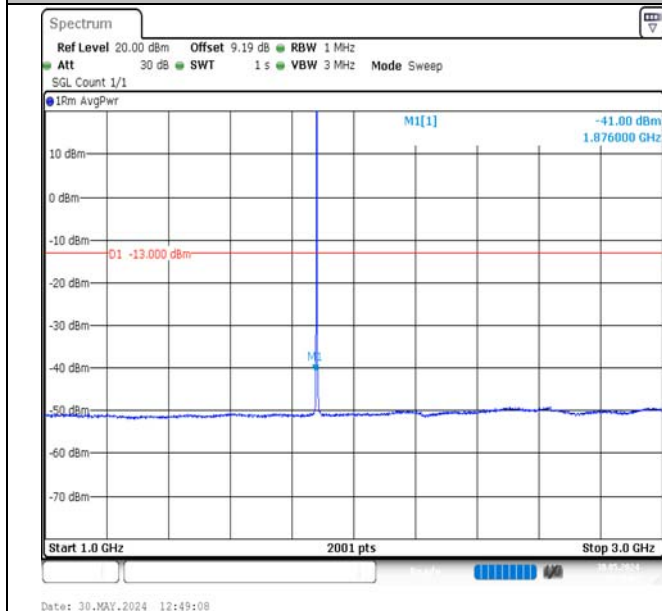
Band2-1.4MHz-QPSK-18900-1RB#0-1000~3000-PASS
