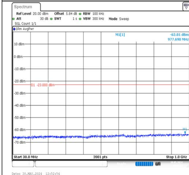
Band2-1.4MHz-16QAM-19193-6RB#0-30~1000-PASS
