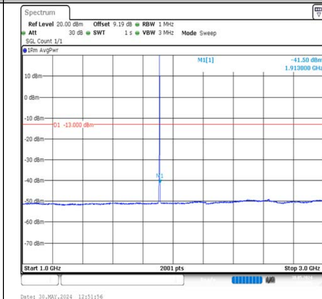
Band2-1.4MHz-QPSK-19193-1RB#5-1000~3000-PASS
