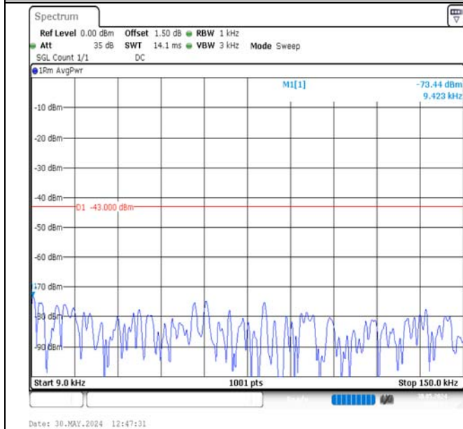
Band2-1.4MHz-QPSK-18607-1RB#5-0.009~0.15-PASS
