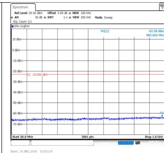
Band2-1.4MHz-QPSK-19193-6RB#0-30~1000-PASS
