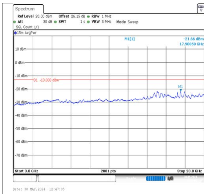
Band2-1.4MHz-QPSK-18607-1RB#0-3000~20000-PASS
