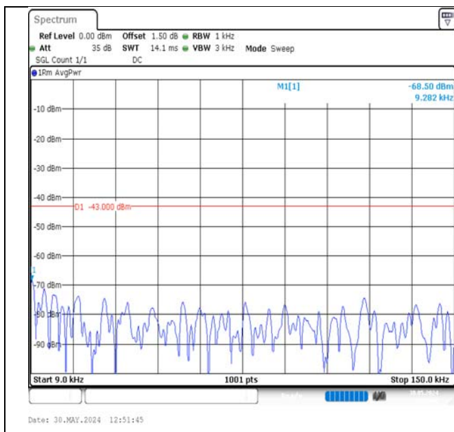
Band2-1.4MHz-QPSK-19193-1RB#5-0.009~0.15-PASS
