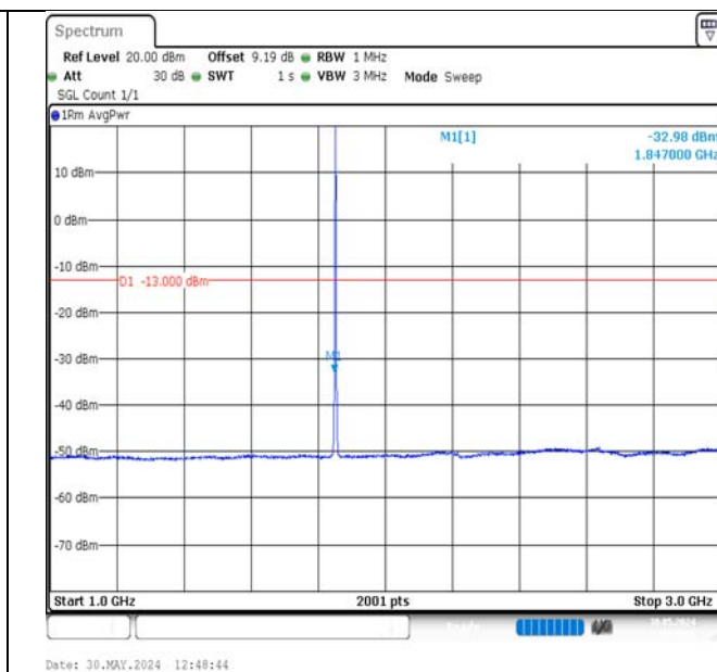
Band2-1.4MHz-16QAM-18607-6RB#0-1000~3000-PASS
