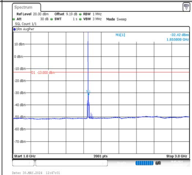
Band2-1.4MHz-QPSK-18607-1RB#0-1000~3000-PASS
