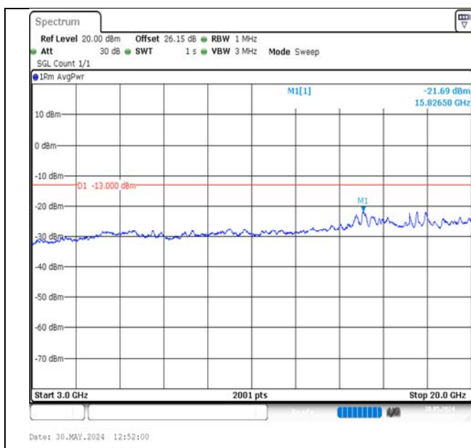
Band2-1.4MHz-QPSK-19193-1RB#5-3000~20000-PASS
