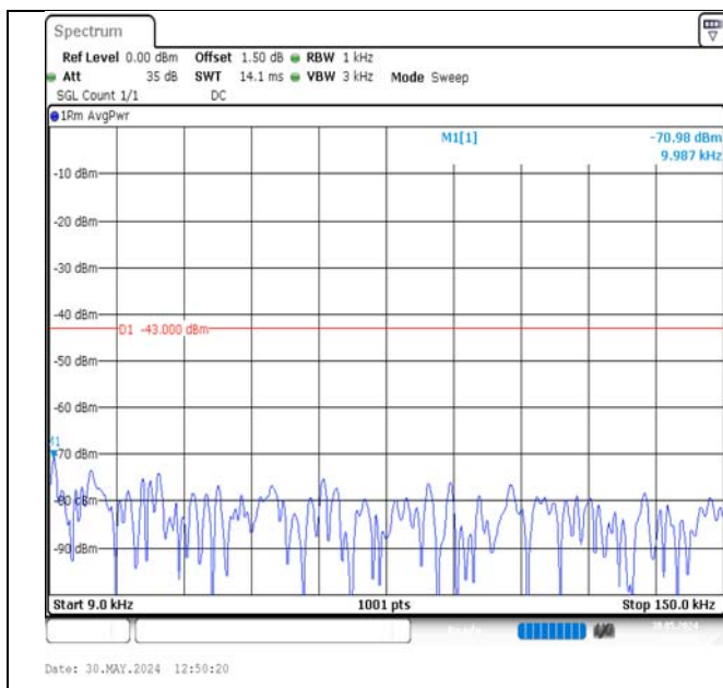
Band2-1.4MHz-QPSK-18900-6RB#0-0.009~0.15-PASS
