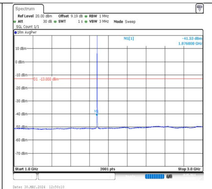
Band2-1.4MHz-16QAM-18900-1RB#5-1000~3000-PASS
