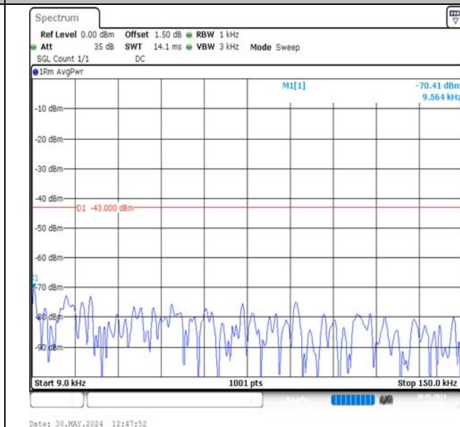
Band2-1.4MHz-16QAM-18607-1RB#5-0.009~0.15-PASS
