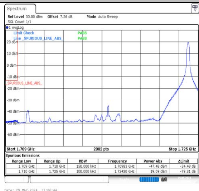
Band66-15MHz-16QAM-132047-1RB#74-PASS
