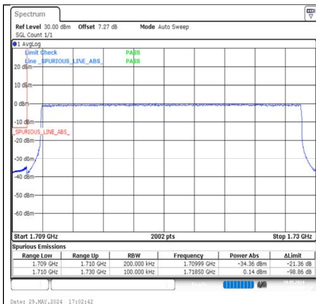
Band66-20MHz-QPSK-132072-100RB#0-PASS
