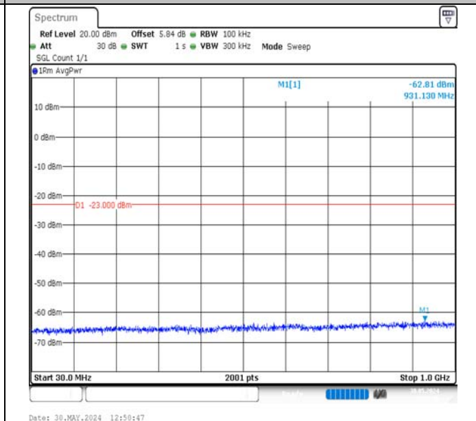
Band2-1.4MHz-16QAM-18900-6RB#0-30~1000-PASS
