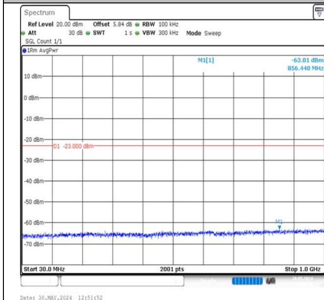
Band2-1.4MHz-QPSK-19193-1RB#5-30~1000-PASS
