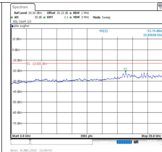
Band2-1.4MHz-QPSK-18900-1RB#5-3000~20000-PASS
