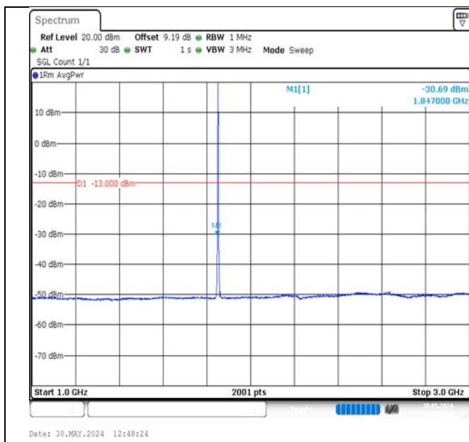
Band2-1.4MHz-QPSK-18607-6RB#0-1000~3000-PASS
