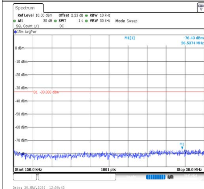
Band2-1.4MHz-16QAM-18900-6RB#0-0.15~30-PASS
