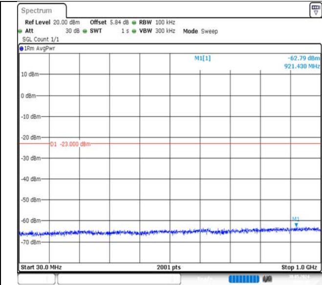
Band2-1.4MHz-QPSK-18607-1RB#5-30~1000-PASS
