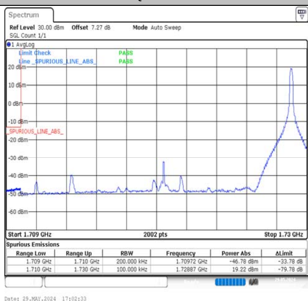
Band66-20MHz-16QAM-132072-1RB#99-PASS
