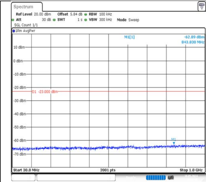
Band2-1.4MHz-QPSK-19193-1RB#0-30~1000-PASS
