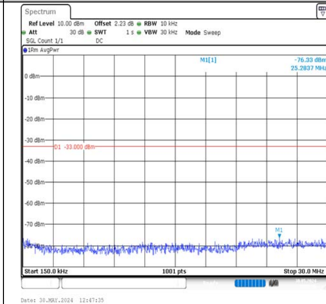
Band2-1.4MHz-QPSK-18607-1RB#5-0.15~30-PASS
