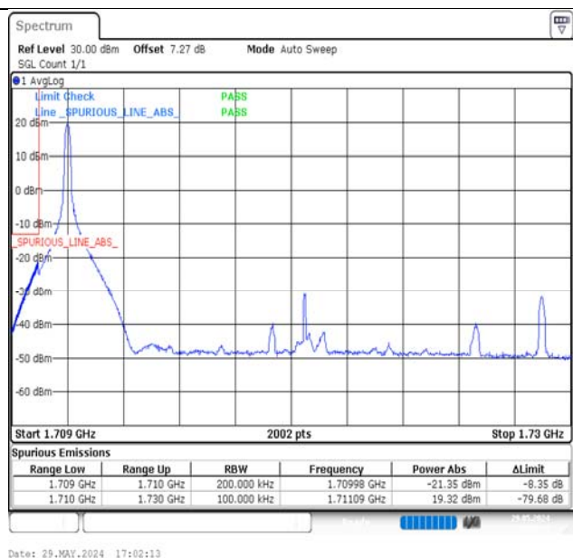
Band66-20MHz-16QAM-132072-1RB#0-PASS
