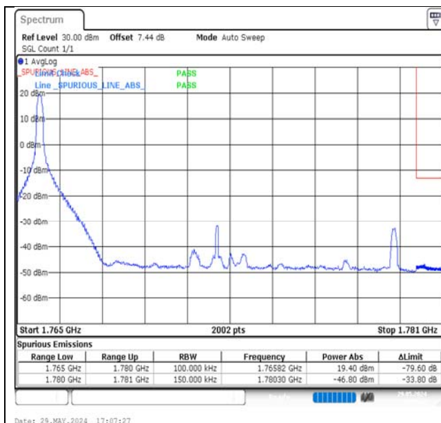
Band66-15MHz-16QAM-132597-1RB#0-PASS
