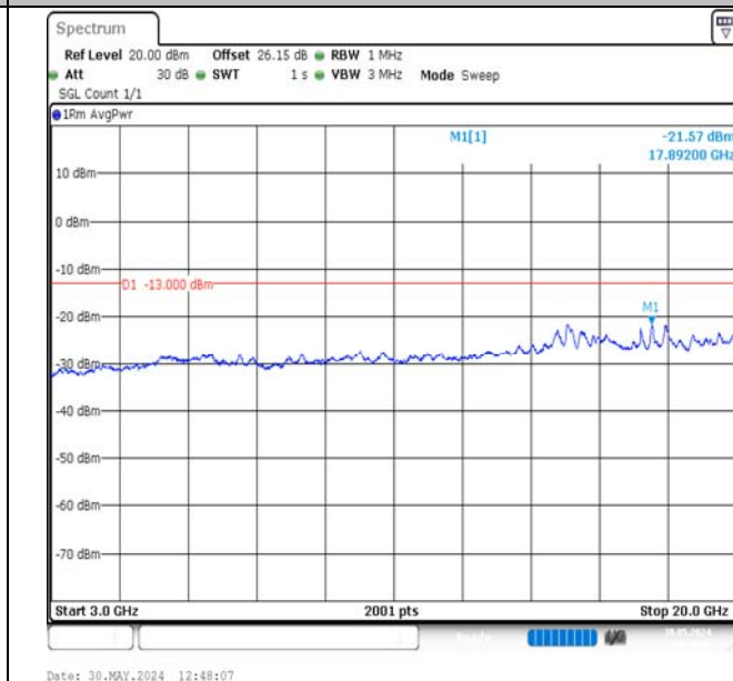
Band2-1.4MHz-16QAM-18607-1RB#5-3000~20000-PASS
