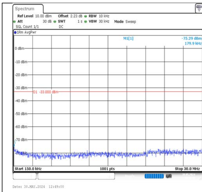
Band2-1.4MHz-QPSK-18900-1RB#0-0.15~30-PASS
