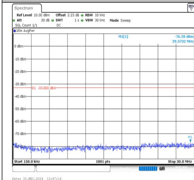
Band2-1.4MHz-16QAM-18607-1RB#0-0.15~30-PASS
