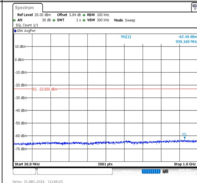
Band2-1.4MHz-QPSK-18607-6RB#0-30~1000-PASS
