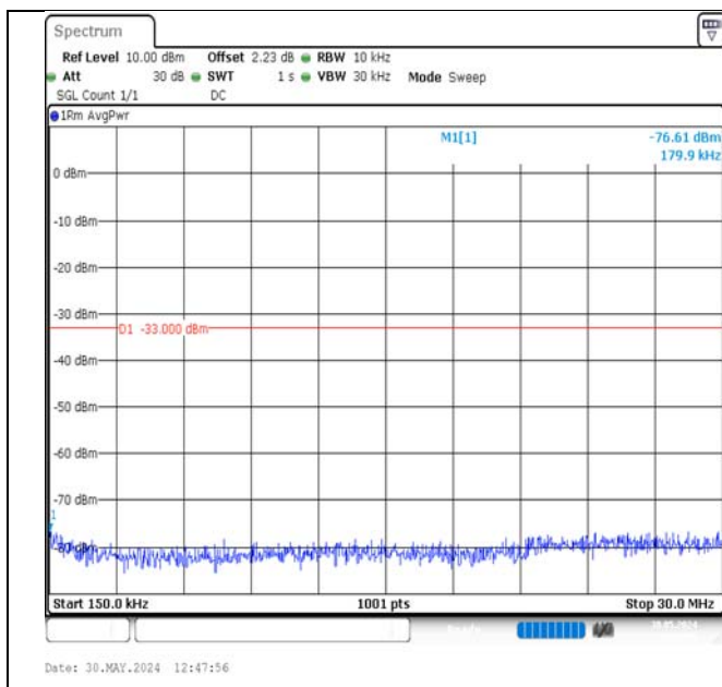
Band2-1.4MHz-16QAM-18607-1RB#5-0.15~30-PASS
