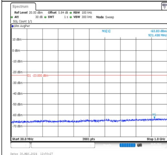
Band2-1.4MHz-QPSK-18900-6RB#0-30~1000-PASS
