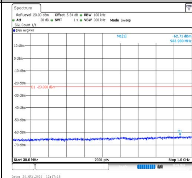
Band2-1.4MHz-16QAM-18607-1RB#0-30~1000-PASS
