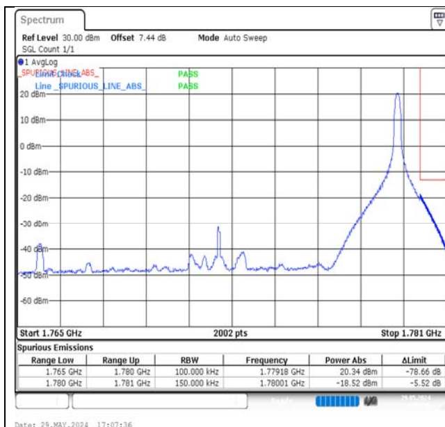
Band66-15MHz-QPSK-132597-1RB#74-PASS
