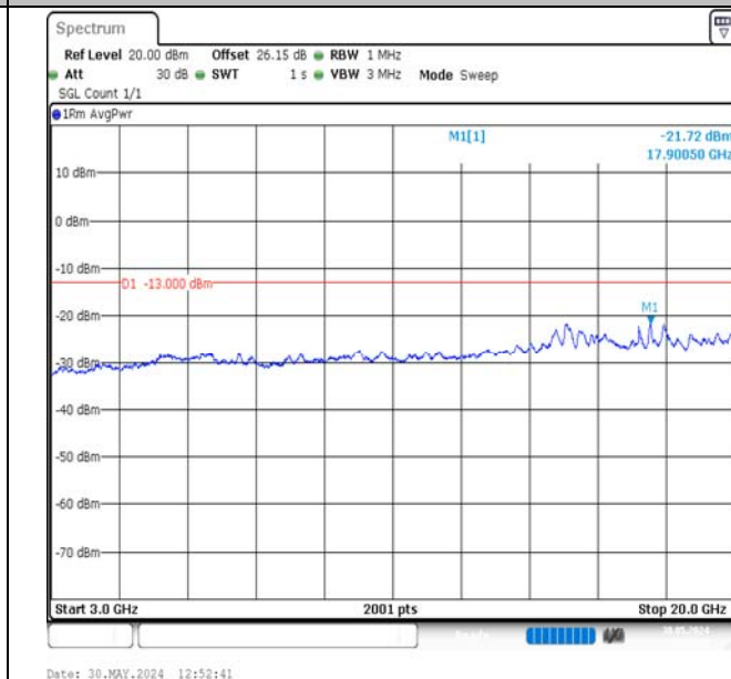
Band2-1.4MHz-QPSK-19193-6RB#0-3000~20000-PASS
