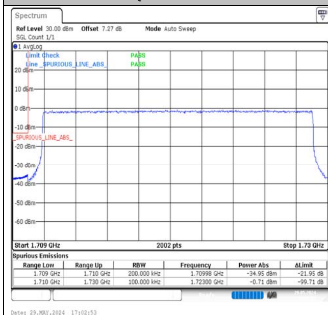
Band66-20MHz-16QAM-132072-100RB#0-PASS
