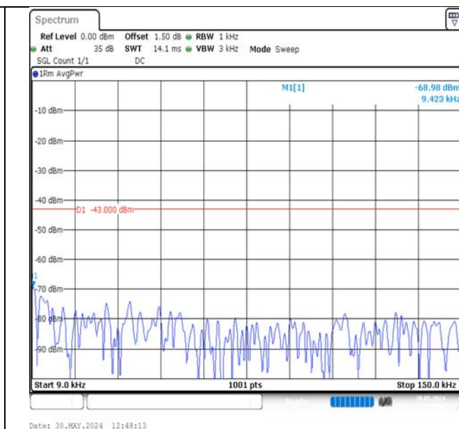
Band2-1.4MHz-QPSK-18607-6RB#0-0.009~0.15-PASS
