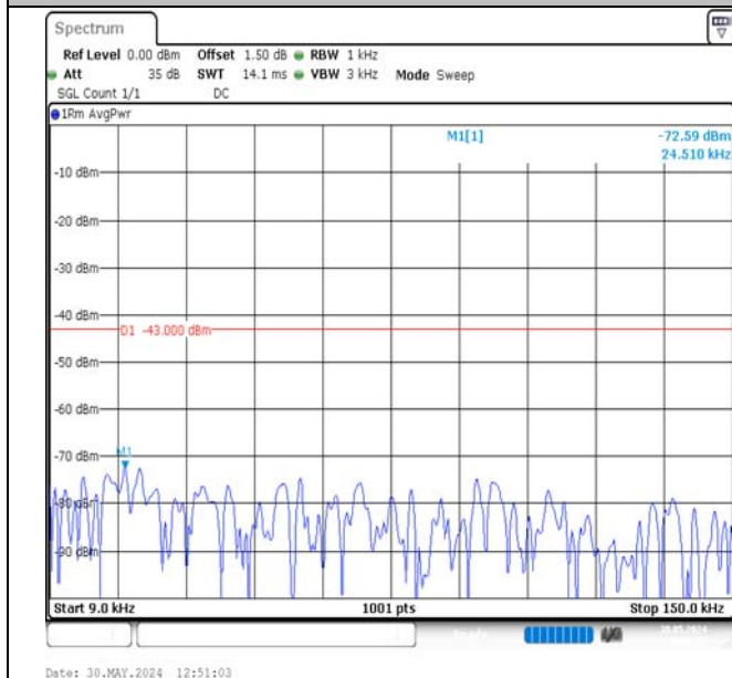
Band2-1.4MHz-QPSK-19193-1RB#0-0.009~0.15-PASS
