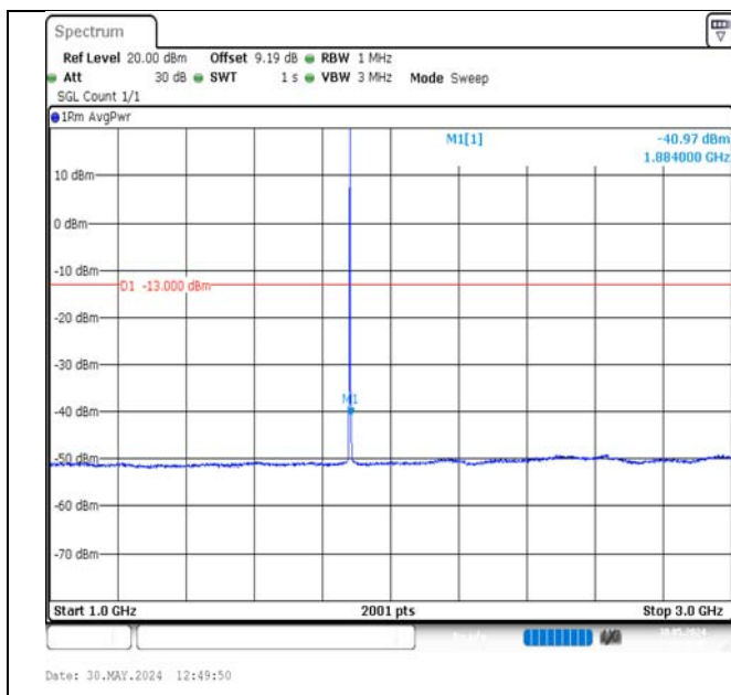
Band2-1.4MHz-QPSK-18900-1RB#5-1000~3000-PASS
