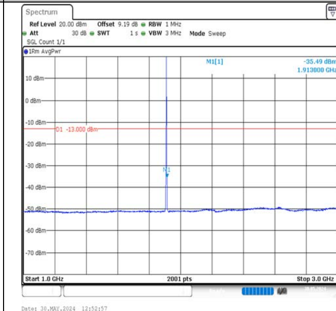
Band2-1.4MHz-16QAM-19193-6RB#0-1000~3000-PASS
