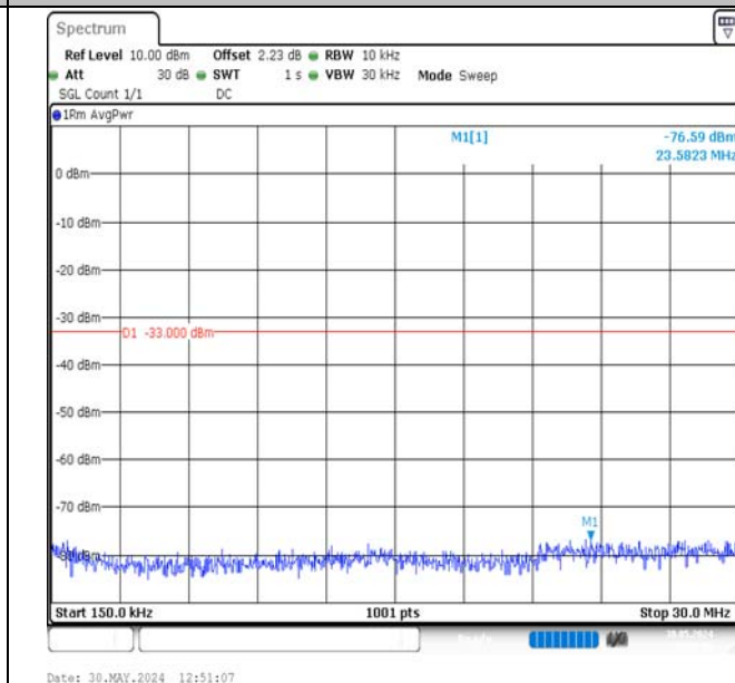
Band2-1.4MHz-QPSK-19193-1RB#0-0.15~30-PASS
