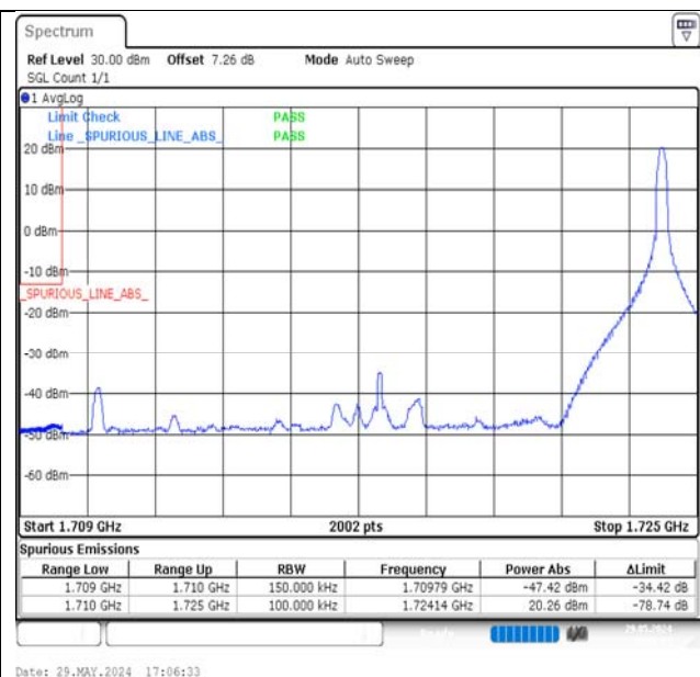
Band66-15MHz-QPSK-132047-1RB#74-PASS
