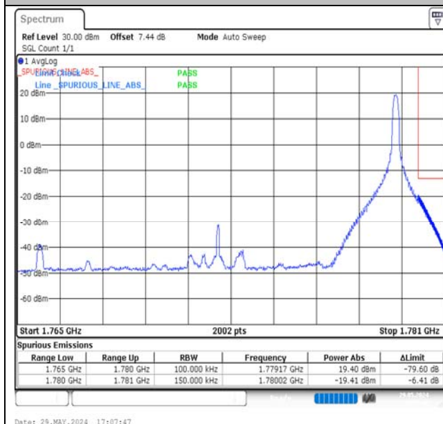
Band66-15MHz-16QAM-132597-1RB#74-PASS
