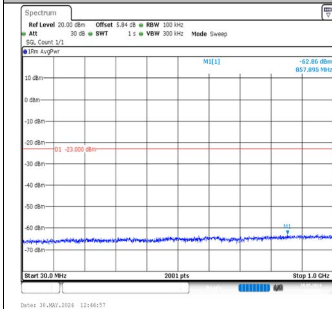
Band2-1.4MHz-QPSK-18607-1RB#0-30~1000-PASS
