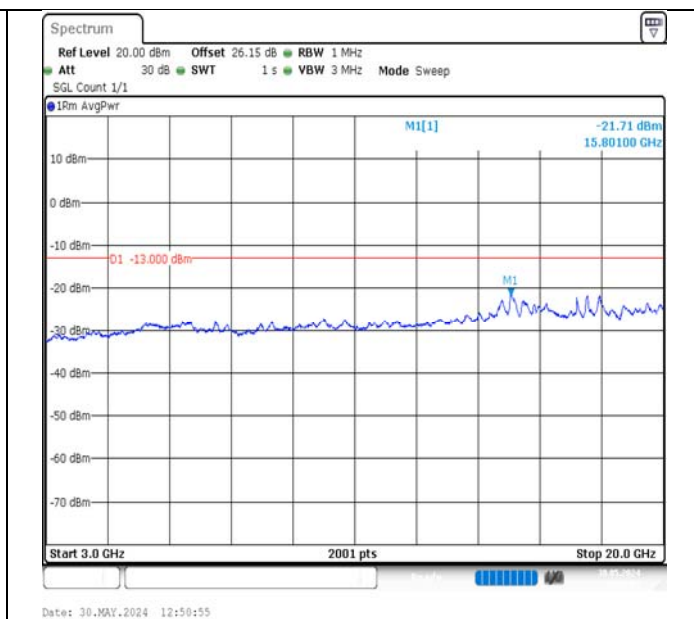
Band2-1.4MHz-16QAM-18900-6RB#0-3000~20000-PASS
