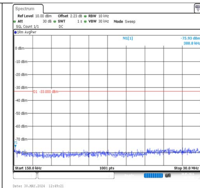
Band2-1.4MHz-16QAM-18900-1RB#0-0.15~30-PASS
