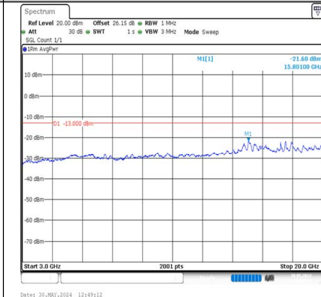
Band2-1.4MHz-QPSK-18900-1RB#0-3000~20000-PASS
