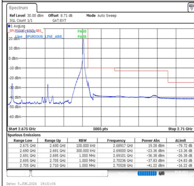
Band41-15MHz-16QAM-41515-1RB#74-PASS
