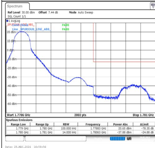
Band66-1.4MHz-QPSK-132665-1RB#0-PASS
