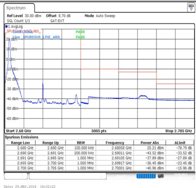
Band41-10MHz-16QAM-41540-1RB#0-PASS
