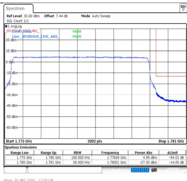
Band66-5MHz-16QAM-132647-25RB#0-PASS
