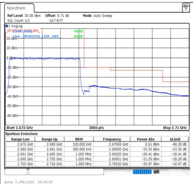
Band41-15MHz-16QAM-41515-75RB#0-PASS
