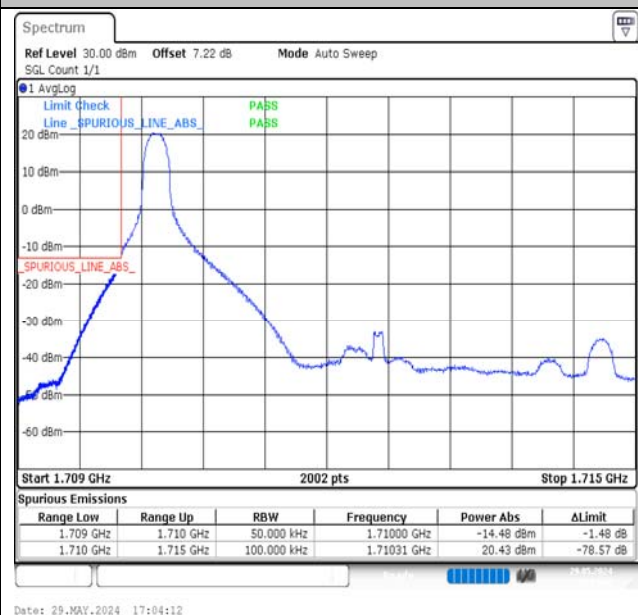
Band66-5MHz-QPSK-131997-1RB#0-PASS
