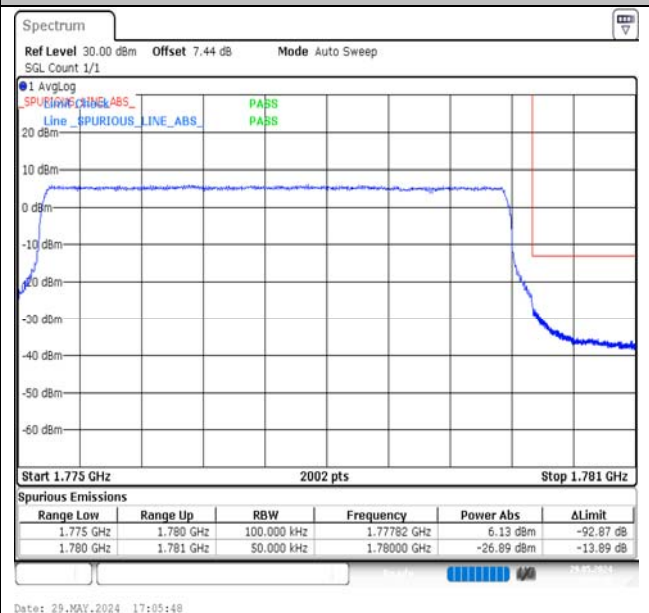
Band66-5MHz-QPSK-132647-25RB#0-PASS
