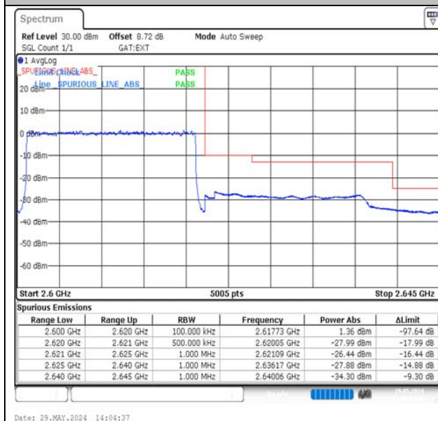
Band38-20MHz-QPSK-38150-100RB#0-PASS
