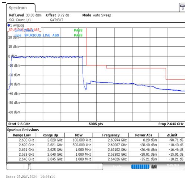
Band38-20MHz-16QAM-38150-100RB#0-PASS
