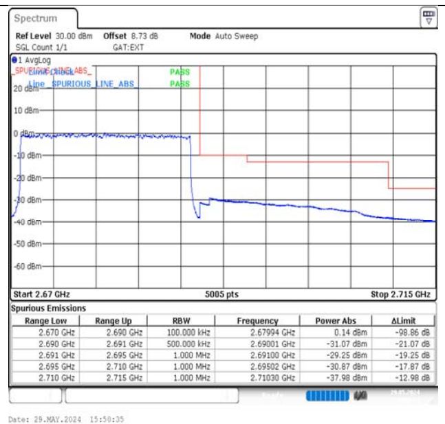
Band41-20MHz-16QAM-41490-100RB#0-PASS
