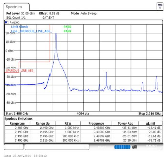
Band41-20MHz-16QAM-39750-1RB#0-PASS
