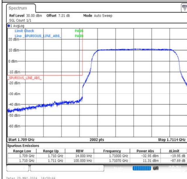
Band66-1.4MHz-16QAM-131979-6RB#0-PASS
