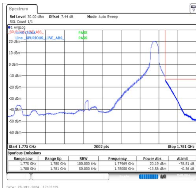
Band66-5MHz-QPSK-132647-1RB#24-PASS
