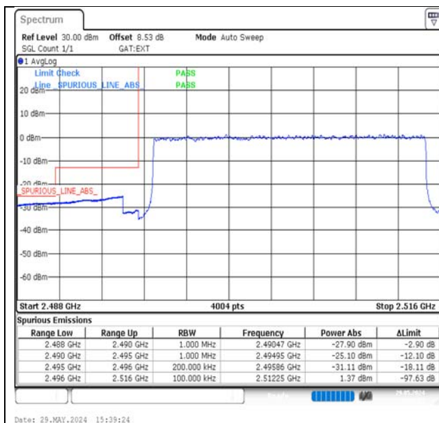
Band41-20MHz-QPSK-39750-100RB#0-PASS
