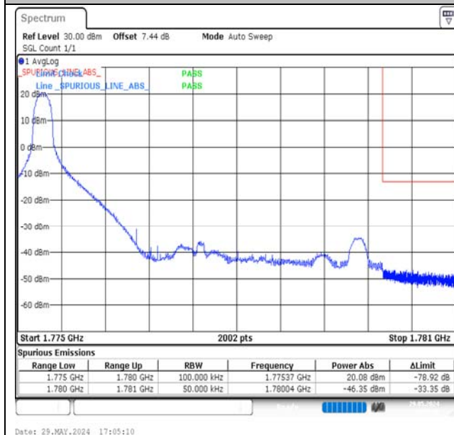
Band66-5MHz-QPSK-132647-1RB#0-PASS
