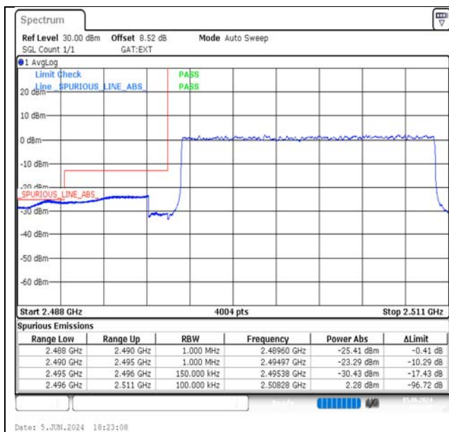
Band41-15MHz-QPSK-39725-75RB#0-PASS
