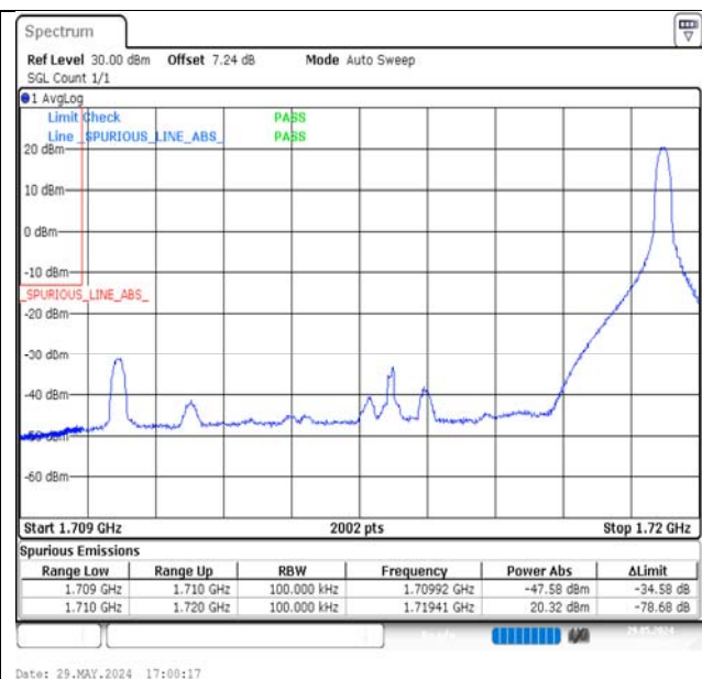
Band66-10MHz-QPSK-132022-1RB#49-PASS
