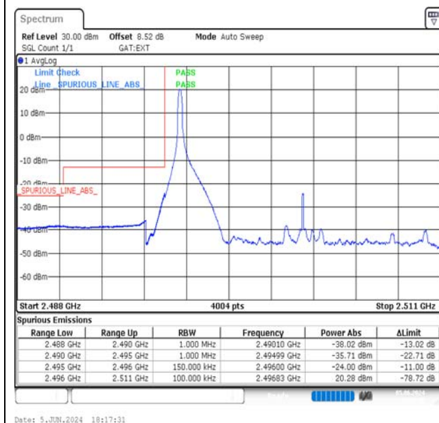
Band41-15MHz-QPSK-39725-1RB#0-PASS
