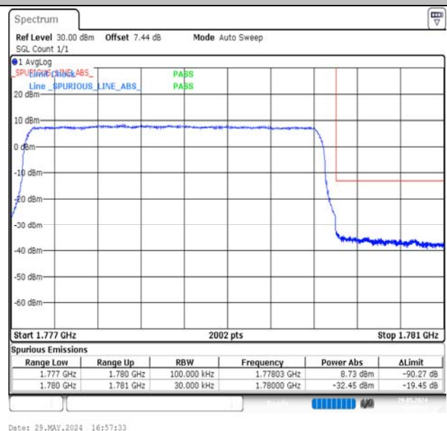
Band66-3MHz-QPSK-132657-15RB#0-PASS
