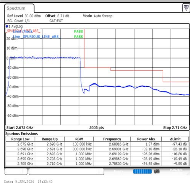
Band41-15MHz-QPSK-41515-75RB#0-PASS
