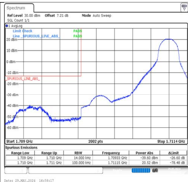
Band66-1.4MHz-QPSK-131979-1RB#5-PASS
