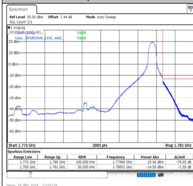
Band66-5MHz-16QAM-132647-1RB#24-PASS
