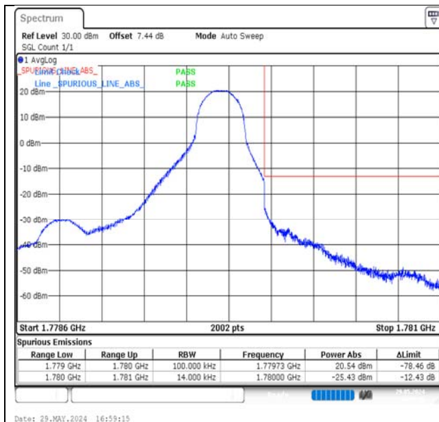
Band66-1.4MHz-QPSK-132665-1RB#5-PASS
