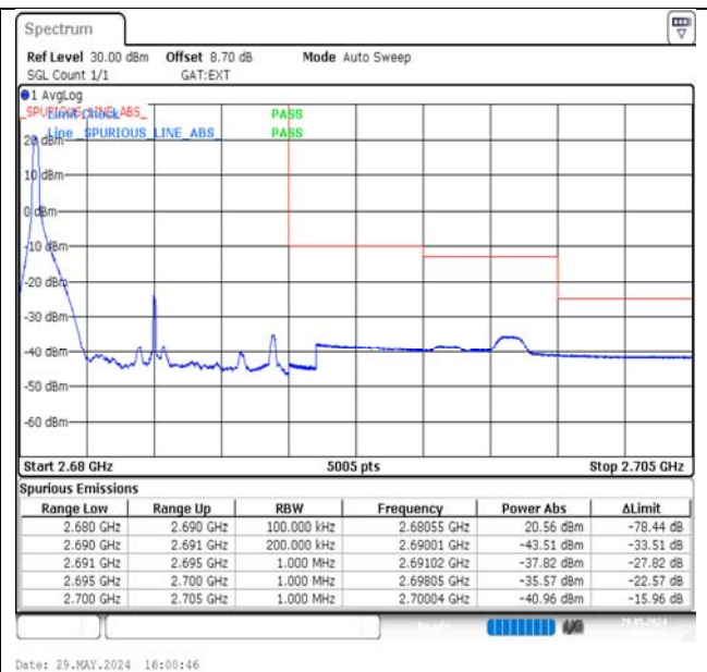
Band41-10MHz-QPSK-41540-1RB#0-PASS
