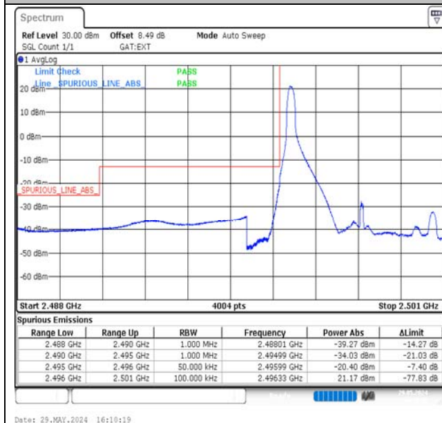
Band41-5MHz-QPSK-39675-1RB#0-PASS
