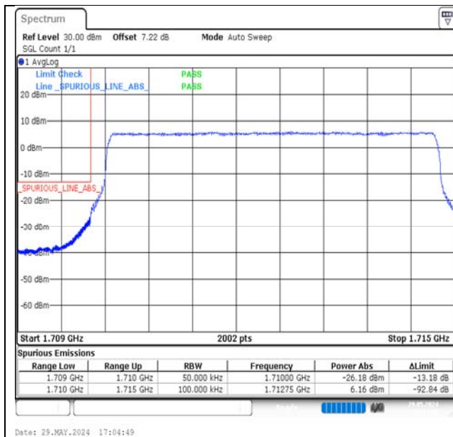
Band66-5MHz-QPSK-131997-25RB#0-PASS
