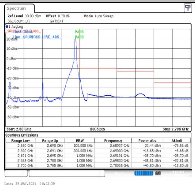
Band41-10MHz-QPSK-41540-1RB#49-PASS
