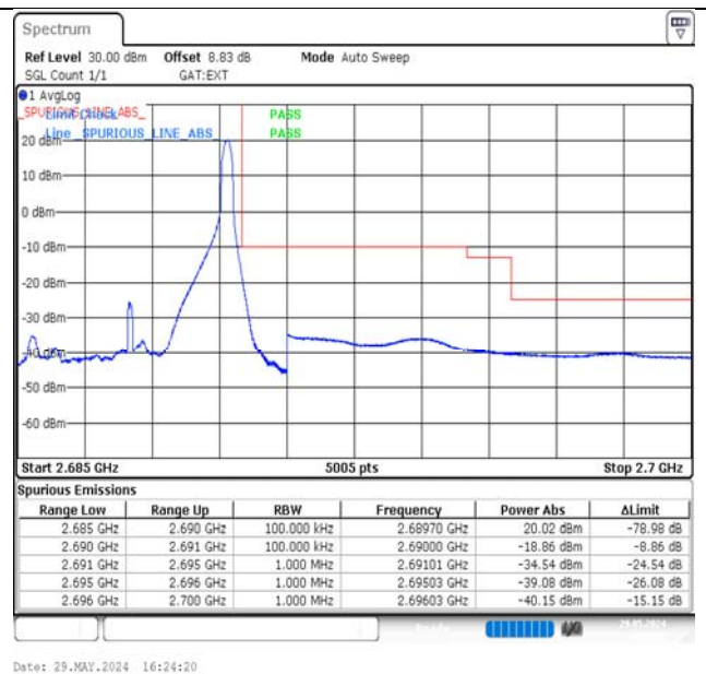
Band41-5MHz-16QAM-41565-1RB#24-PASS
