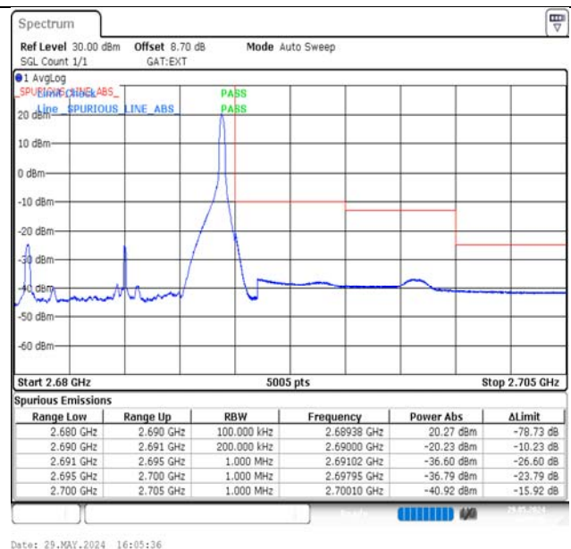
Band41-10MHz-16QAM-41540-1RB#49-PASS
