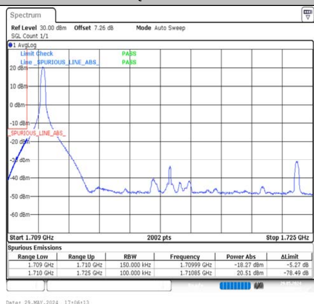
Band66-15MHz-QPSK-132047-1RB#0-PASS
