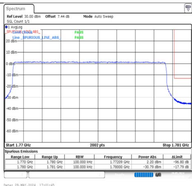
Band66-10MHz-16QAM-132622-50RB#0-PASS
