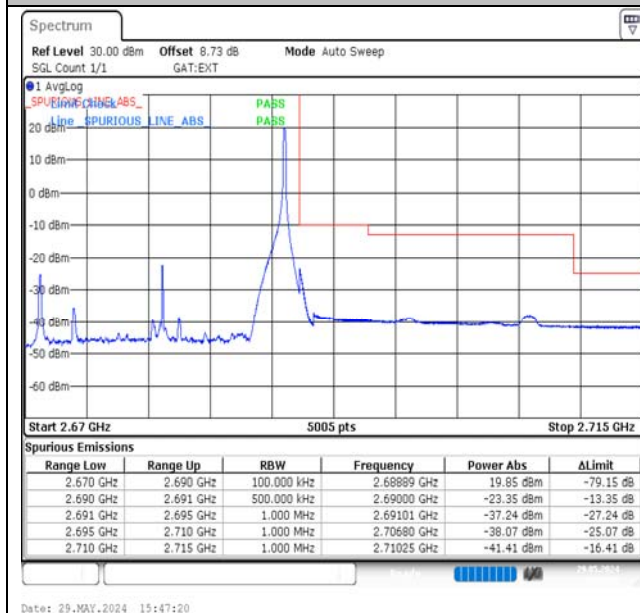
Band41-20MHz-16QAM-41490-1RB#99-PASS
