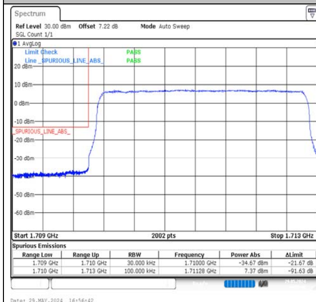
Band66-3MHz-16QAM-131987-15RB#0-PASS
