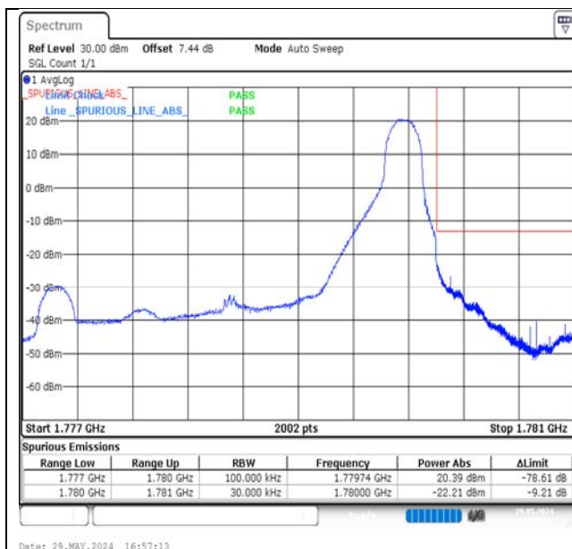
Band66-3MHz-QPSK-132657-1RB#14-PASS
