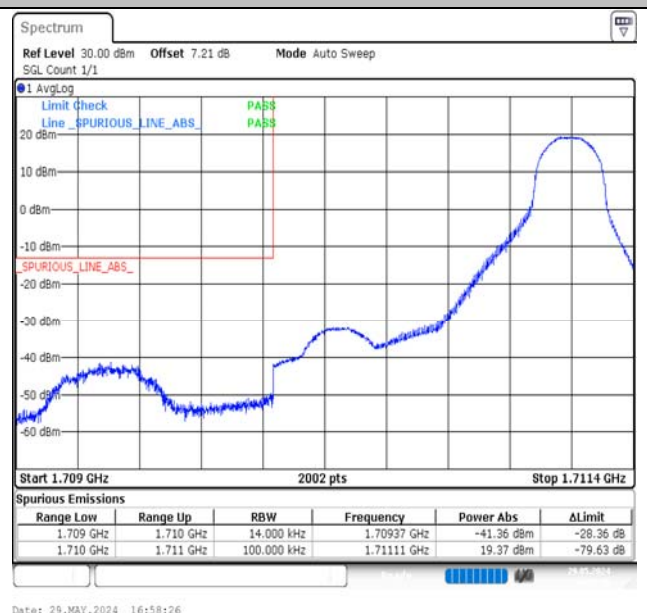
Band66-1.4MHz-16QAM-131979-1RB#5-PASS
