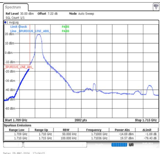
Band66-5MHz-16QAM-131997-1RB#0-PASS
