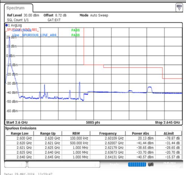
Band38-20MHz-16QAM-38150-1RB#0-PASS
