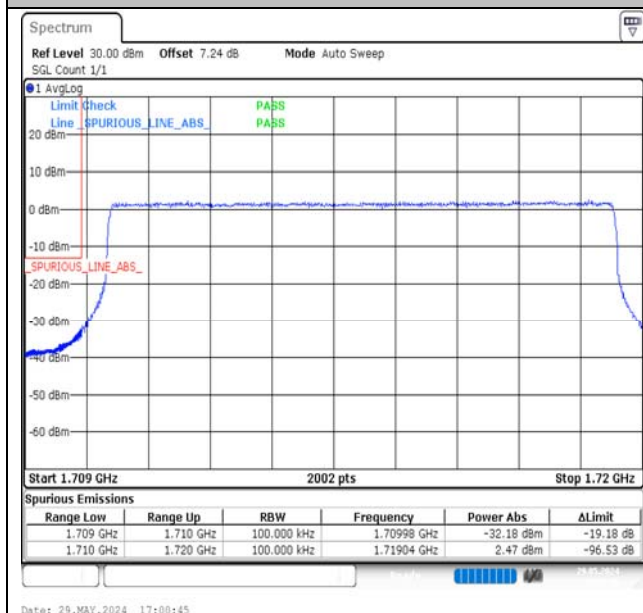
Band66-10MHz-16QAM-132022-50RB#0-PASS
