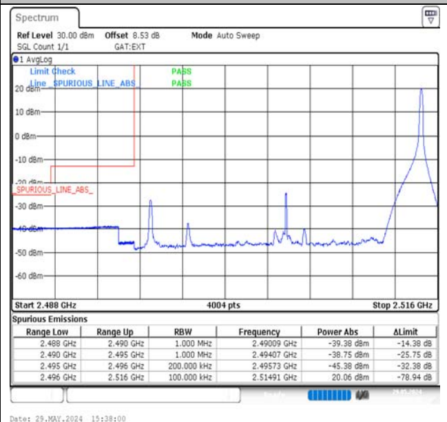
Band41-20MHz-16QAM-39750-1RB#99-PASS
