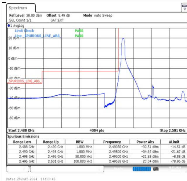
Band41-5MHz-16QAM-39675-1RB#0-PASS
