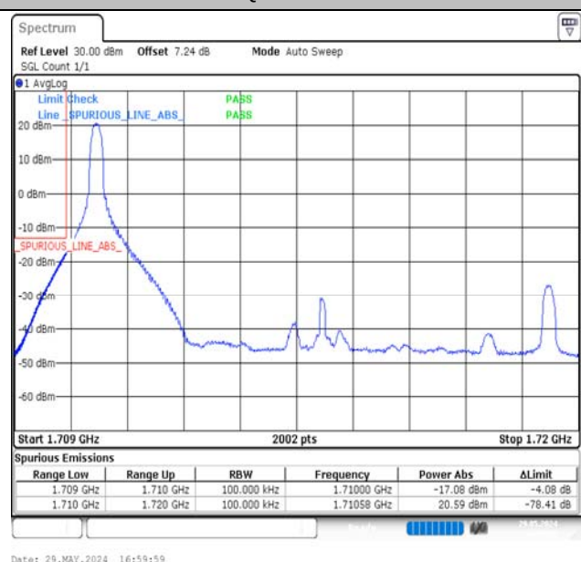
Band66-10MHz-QPSK-132022-1RB#0-PASS
