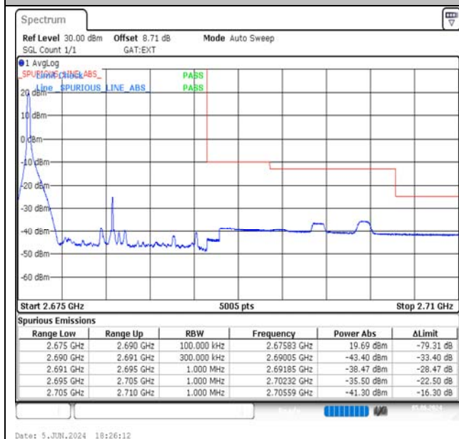
Band41-15MHz-QPSK-41515-1RB#0-PASS
