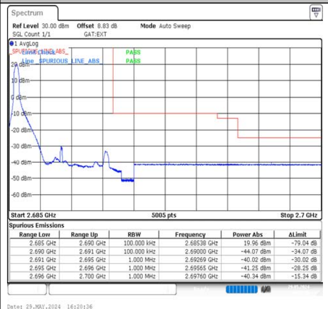
Band41-5MHz-16QAM-41565-1RB#0-PASS
