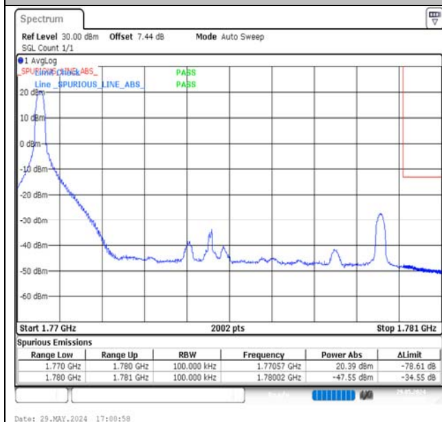
Band66-10MHz-QPSK-132622-1RB#0-PASS
