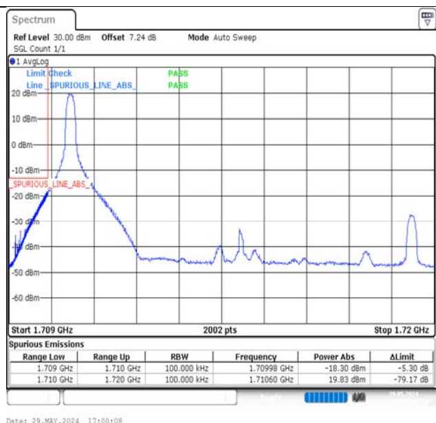
Band66-10MHz-16QAM-132022-1RB#0-PASS
