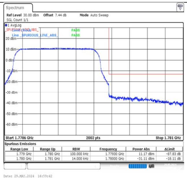
Band66-1.4MHz-16QAM-132665-6RB#0-PASS
