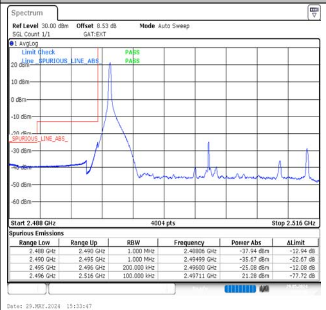
Band41-20MHz-QPSK-39750-1RB#0-PASS
