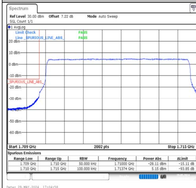
Band66-5MHz-16QAM-131997-25RB#0-PASS
