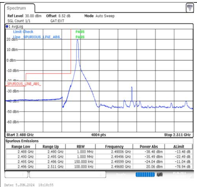
Band41-15MHz-16QAM-39725-1RB#0-PASS
