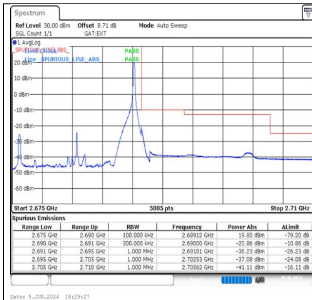
Band41-15MHz-QPSK-41515-1RB#74-PASS
