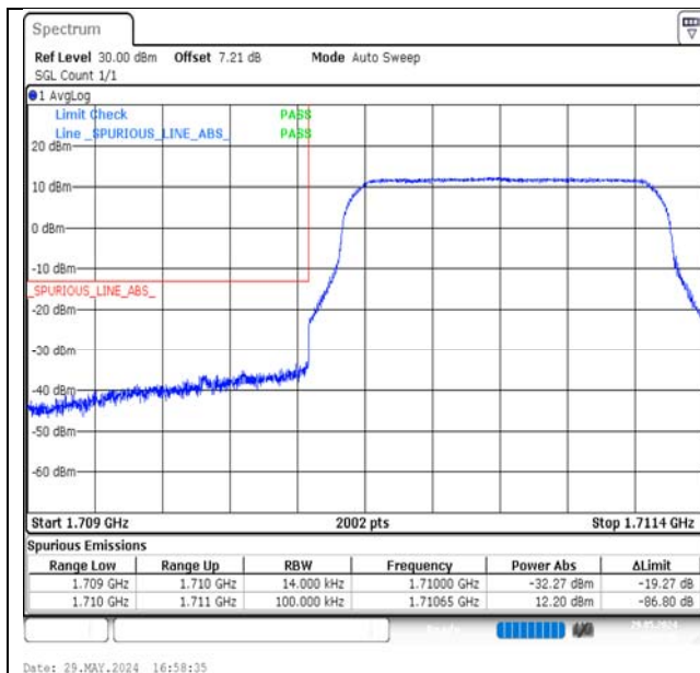
Band66-1.4MHz-QPSK-131979-6RB#0-PASS
