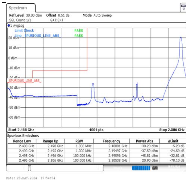
Band41-10MHz-QPSK-39700-1RB#49-PASS
