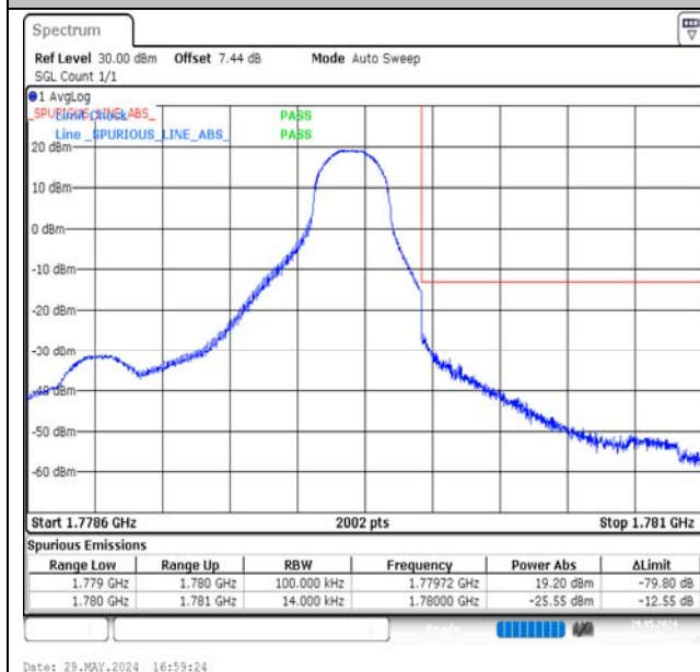
Band66-1.4MHz-16QAM-132665-1RB#5-PASS
