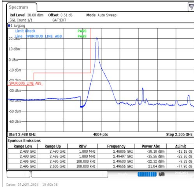
Band41-10MHz-QPSK-39700-1RB#0-PASS
