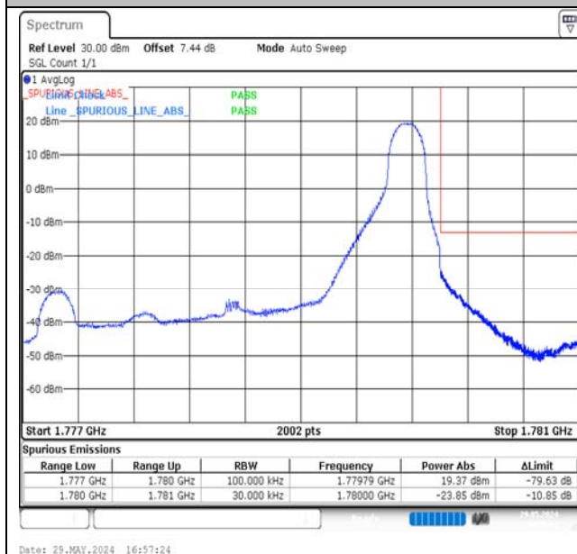
Band66-3MHz-16QAM-132657-1RB#14-PASS
