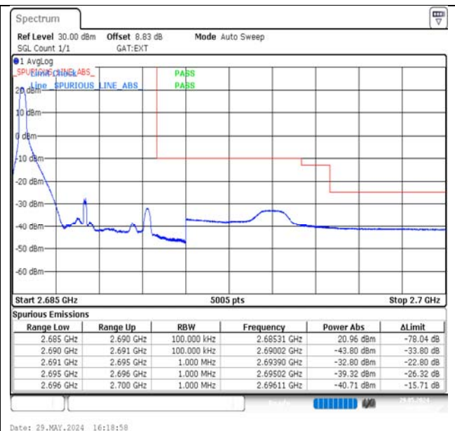
Band41-5MHz-QPSK-41565-1RB#0-PASS
