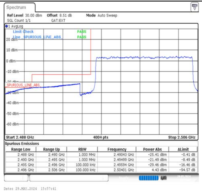
Band41-10MHz-QPSK-39700-50RB#0-PASS
