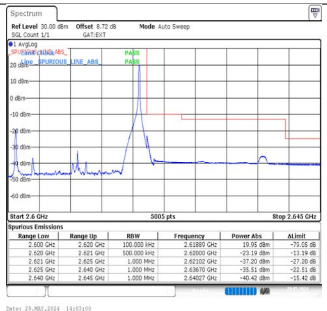
Band38-20MHz-16QAM-38150-1RB#99-PASS
