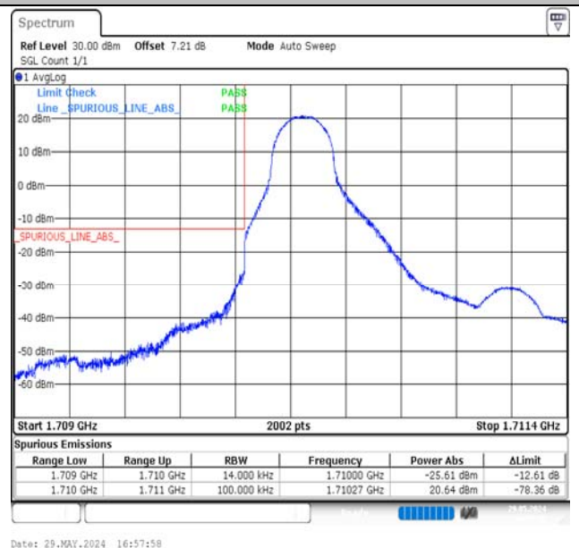
Band66-1.4MHz-QPSK-131979-1RB#0-PASS
