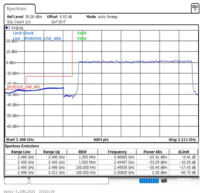
Band41-15MHz-QPSK-39725-75RB#0-PASS
