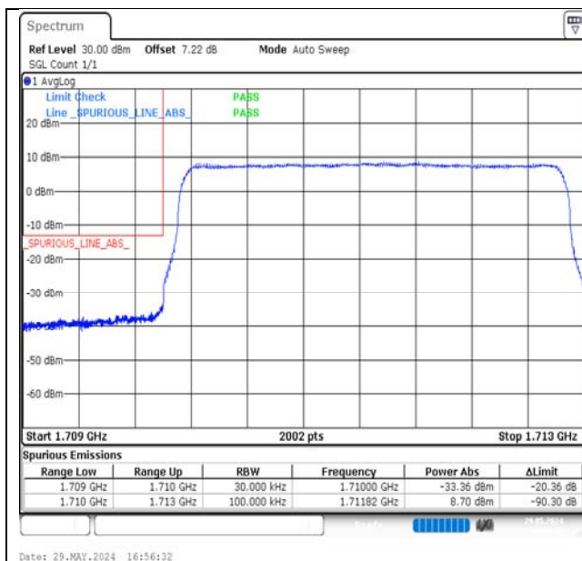
Band66-3MHz-QPSK-131987-15RB#0-PASS
