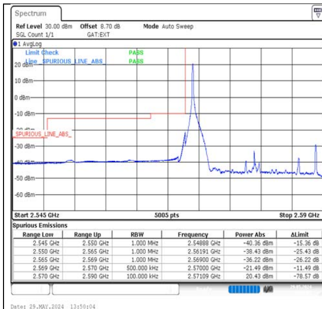
Band38-20MHz-16QAM-37850-1RB#0-PASS
