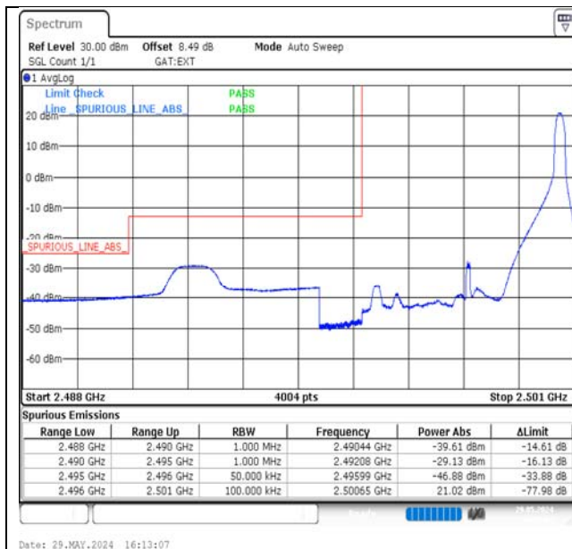
Band41-5MHz-QPSK-39675-1RB#24-PASS
