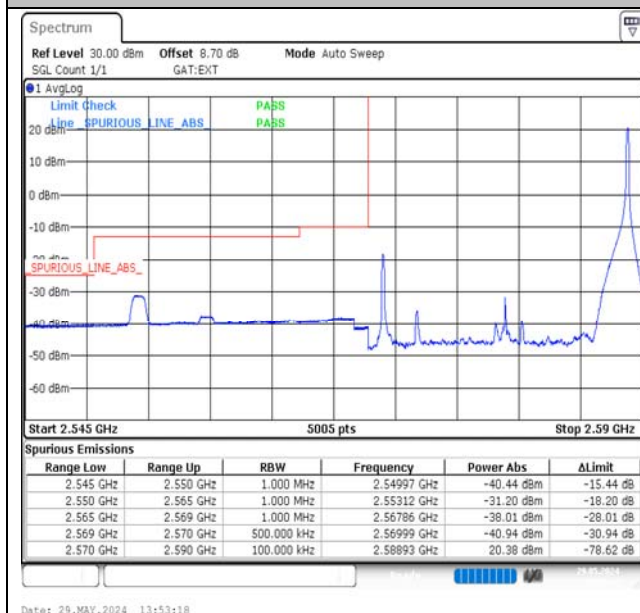
Band38-20MHz-16QAM-37850-1RB#99-PASS
