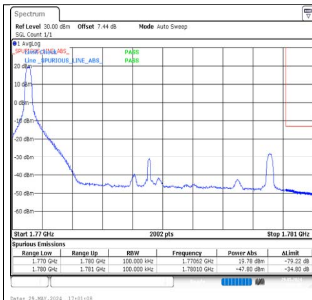
Band66-10MHz-16QAM-132622-1RB#0-PASS
