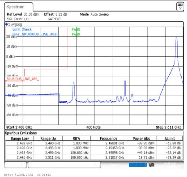
Band41-15MHz-16QAM-39725-1RB#74-PASS
