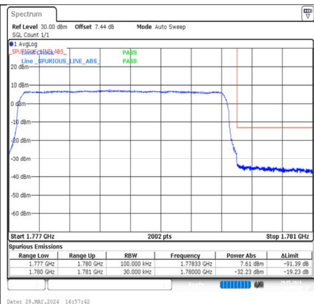
Band66-3MHz-16QAM-132657-15RB#0-PASS
