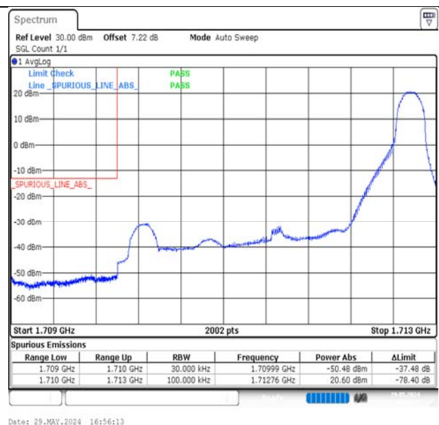
Band66-3MHz-QPSK-131987-1RB#14-PASS
