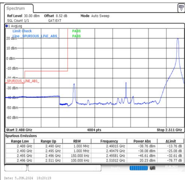
Band41-15MHz-QPSK-39725-1RB#74-PASS
