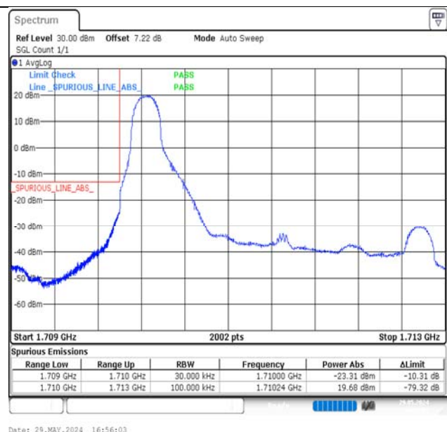
Band66-3MHz-16QAM-131987-1RB#0-PASS
