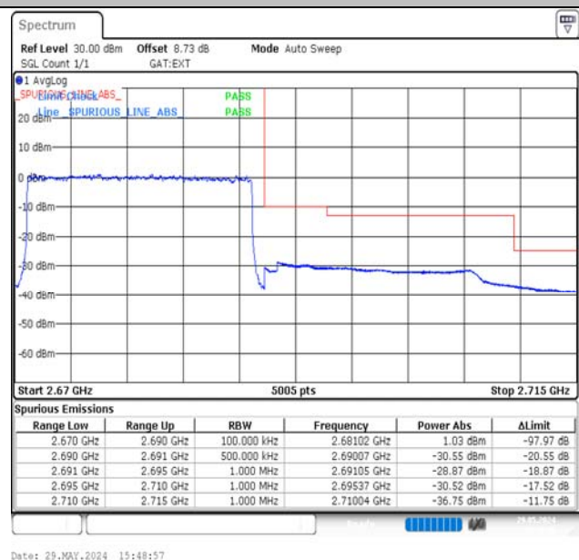
Band41-20MHz-QPSK-41490-100RB#0-PASS
