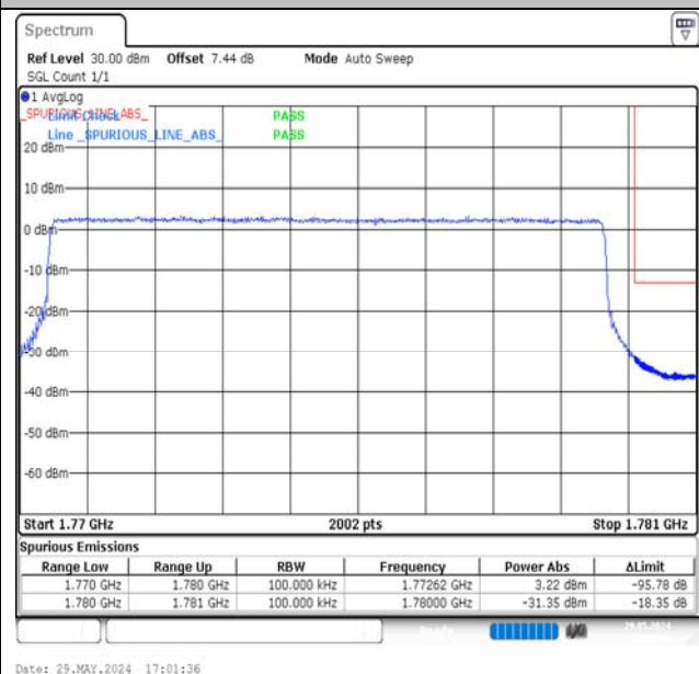
Band66-10MHz-QPSK-132622-50RB#0-PASS
