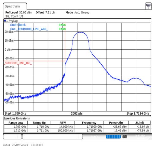
Band66-1.4MHz-16QAM-131979-1RB#0-PASS
