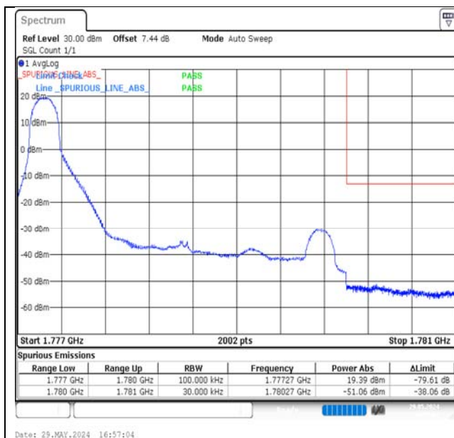
Band66-3MHz-16QAM-132657-1RB#0-PASS
