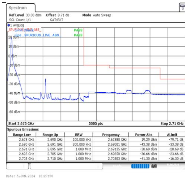
Band41-15MHz-16QAM-41515-1RB#0-PASS
