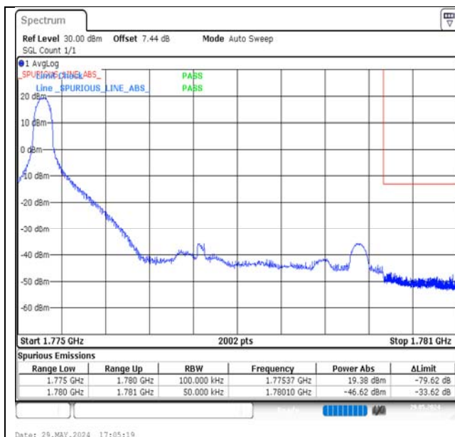
Band66-5MHz-16QAM-132647-1RB#0-PASS
