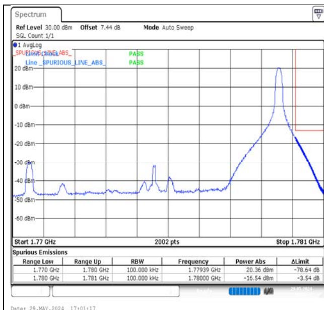
Band66-10MHz-QPSK-132622-1RB#49-PASS
