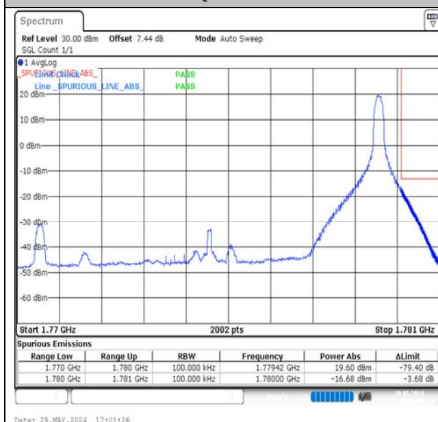
Band66-10MHz-16QAM-132622-1RB#49-PASS
