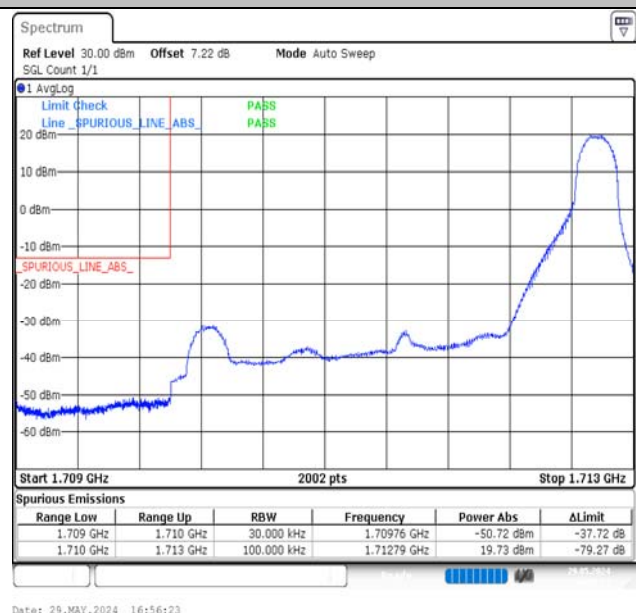
Band66-3MHz-16QAM-131987-1RB#14-PASS
