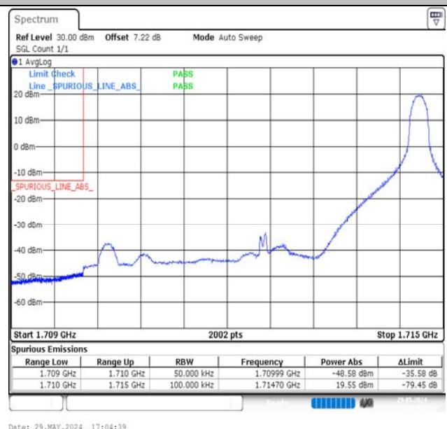
Band66-5MHz-16QAM-131997-1RB#24-PASS
