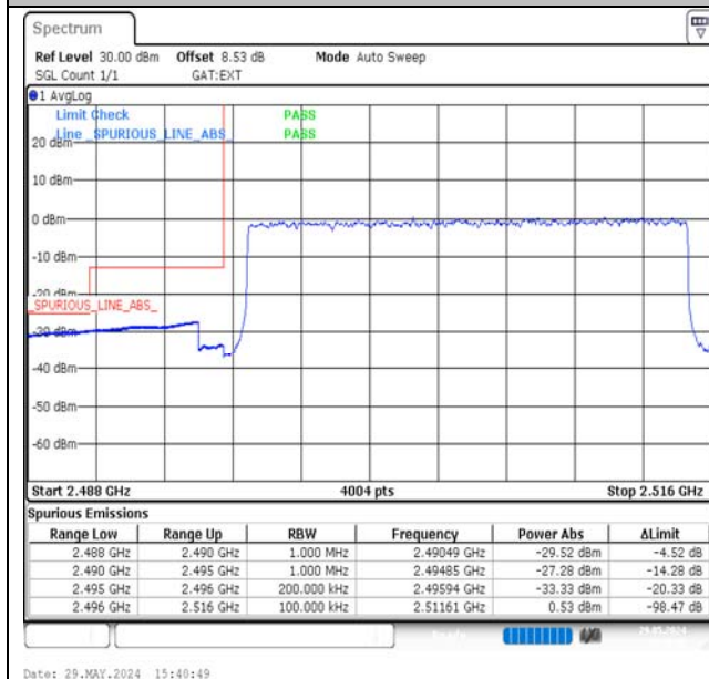
Band41-20MHz-16QAM-39750-100RB#0-PASS
