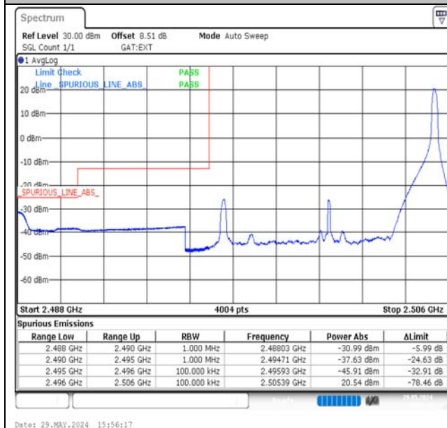
Band41-10MHz-16QAM-39700-1RB#49-PASS
