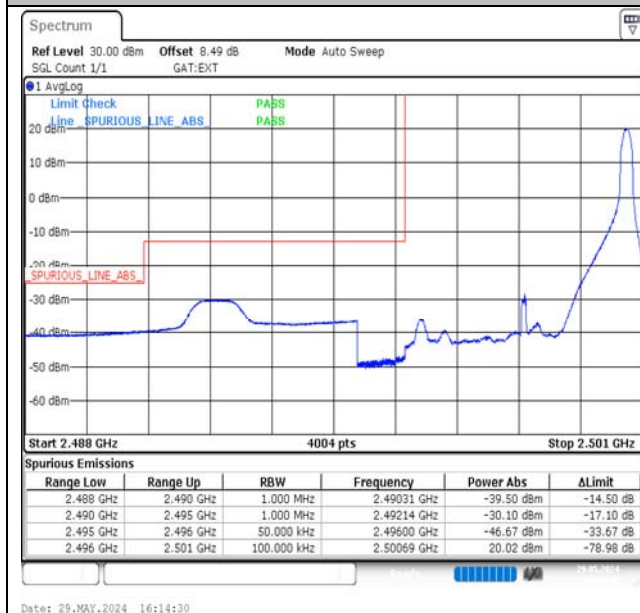
Band41-5MHz-16QAM-39675-1RB#24-PASS
