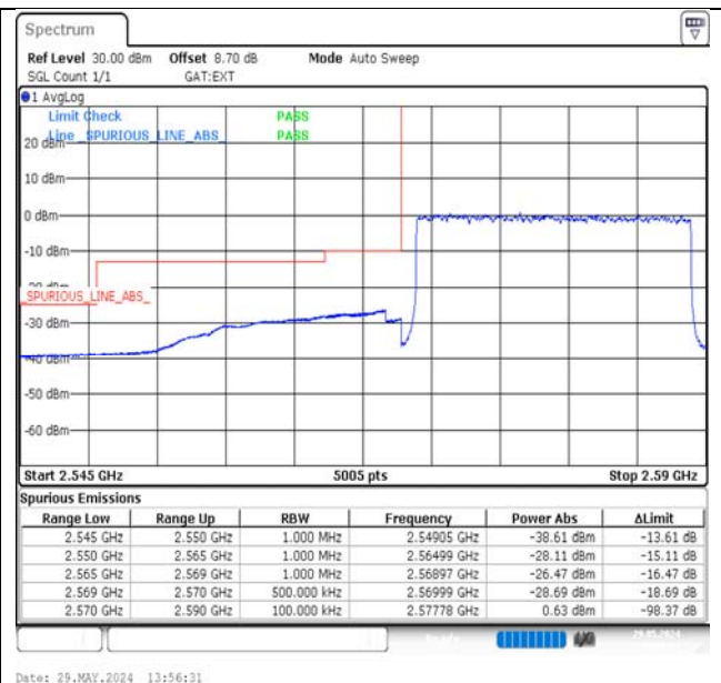
Band38-20MHz-16QAM-37850-100RB#0-PASS
