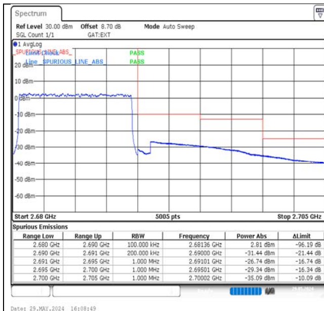
Band41-10MHz-16QAM-41540-50RB#0-PASS
