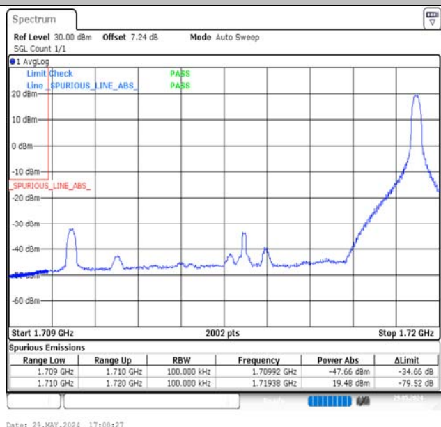
Band66-10MHz-16QAM-132022-1RB#49-PASS
