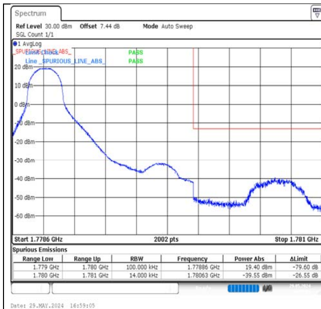
Band66-1.4MHz-16QAM-132665-1RB#0-PASS
