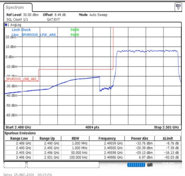
Band41-5MHz-QPSK-39675-25RB#0-PASS
