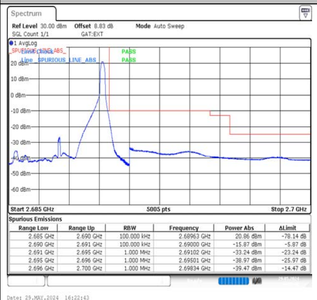
Band41-5MHz-QPSK-41565-1RB#24-PASS
