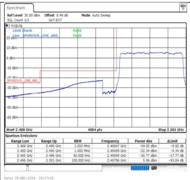
Band41-5MHz-16QAM-39675-25RB#0-PASS
