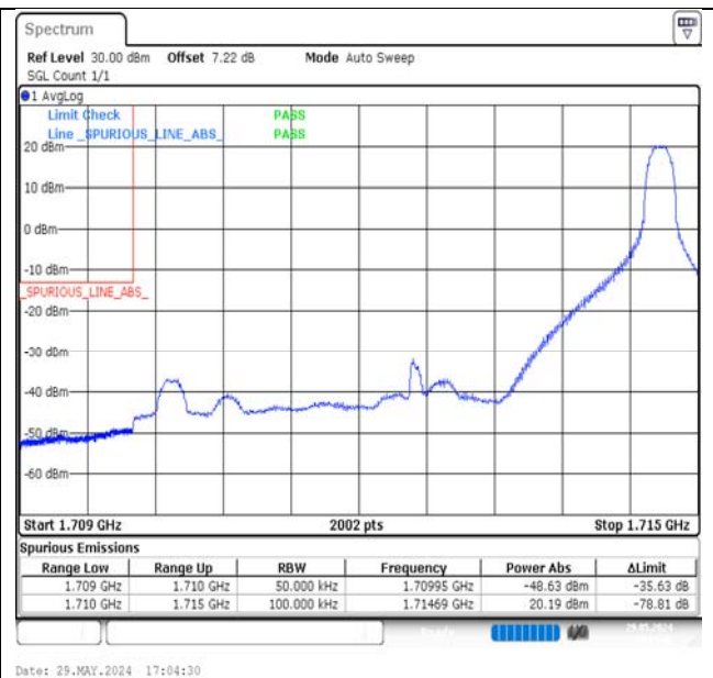
Band66-5MHz-QPSK-131997-1RB#24-PASS
