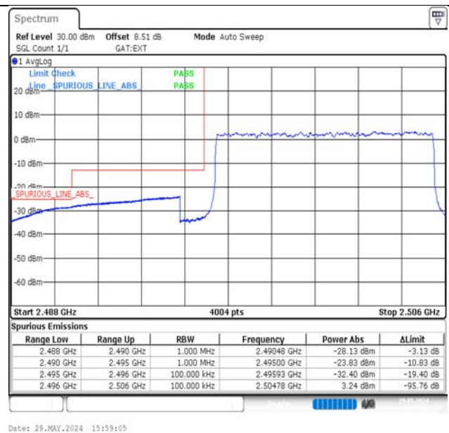
Band41-10MHz-16QAM-39700-50RB#0-PASS
