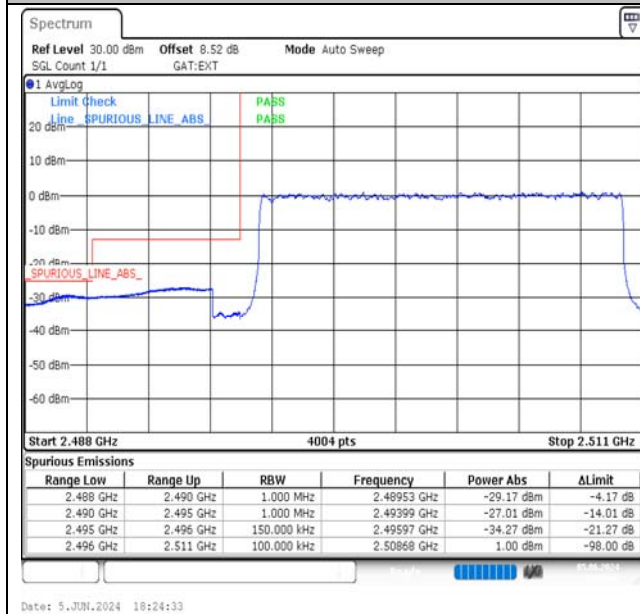
Band41-15MHz-16QAM-39725-75RB#0-PASS
