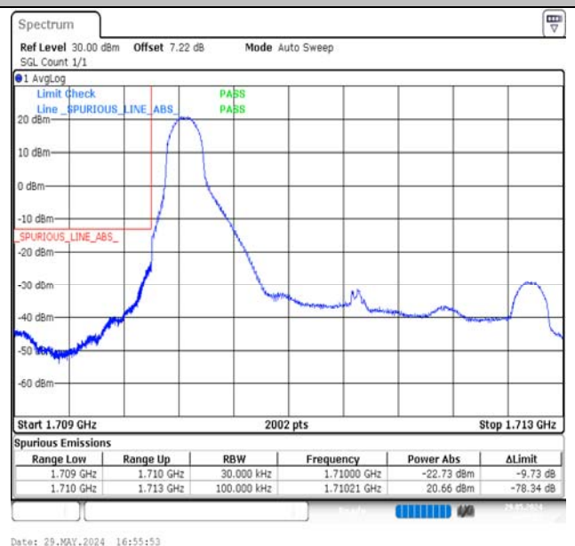
Band66-3MHz-QPSK-131987-1RB#0-PASS
