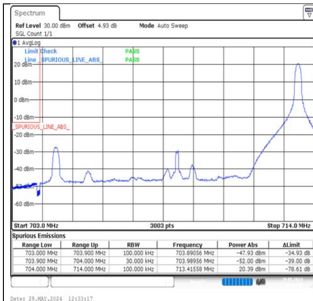
Band17-10MHz-QPSK-23780-1RB#49-PASS
