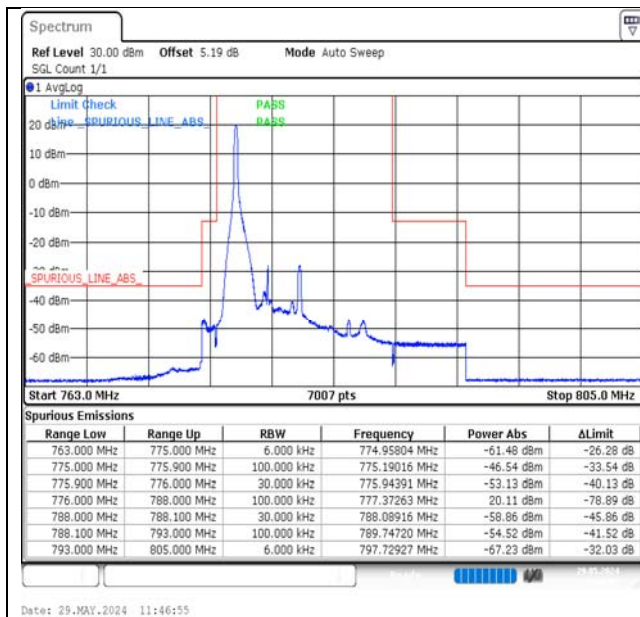
Band13-5MHz-QPSK-23205-1RB#0-PASS
