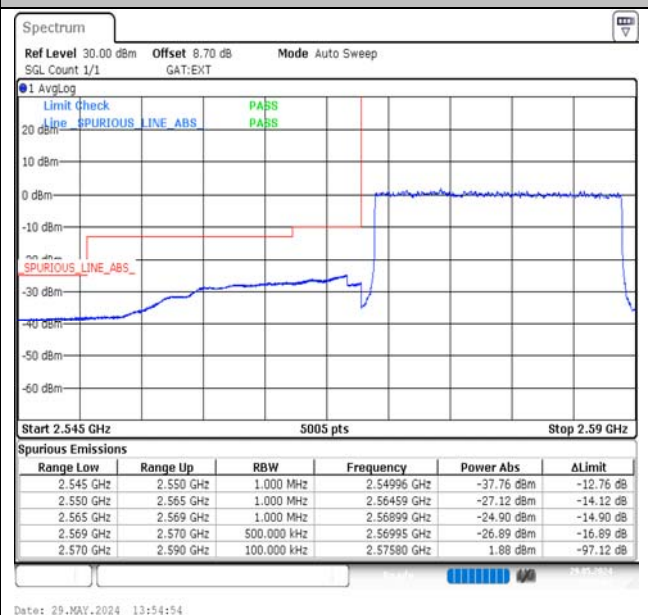
Band38-20MHz-QPSK-37850-100RB#0-PASS
