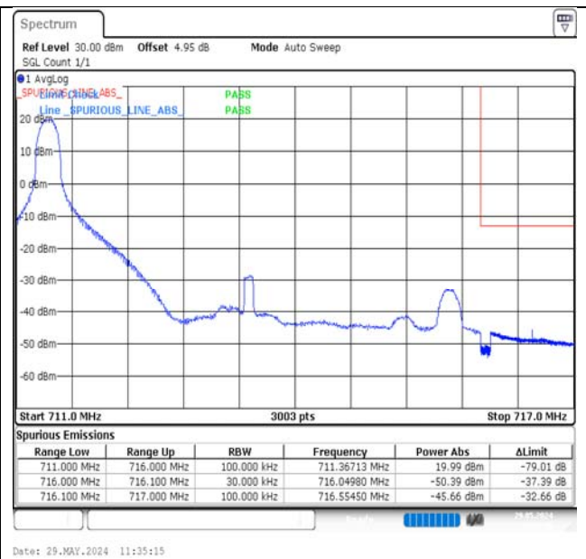
Band12-5MHz-16QAM-23155-1RB#0-PASS
