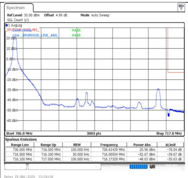
Band17-10MHz-QPSK-23800-1RB#0-PASS
