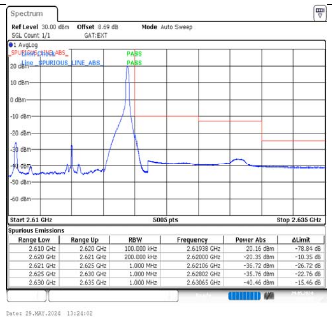
Band38-10MHz-16QAM-38200-1RB#49-PASS
