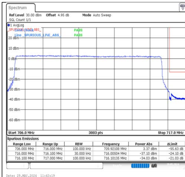
Band12-10MHz-QPSK-23130-50RB#0-PASS
