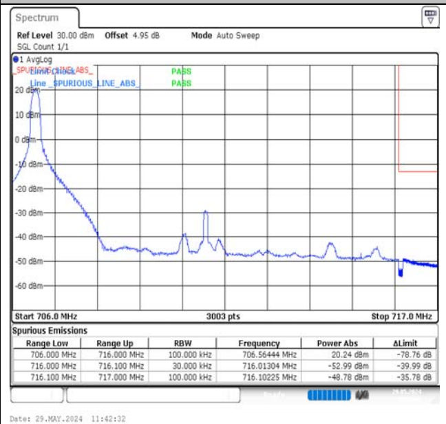
Band12-10MHz-QPSK-23130-1RB#0-PASS
