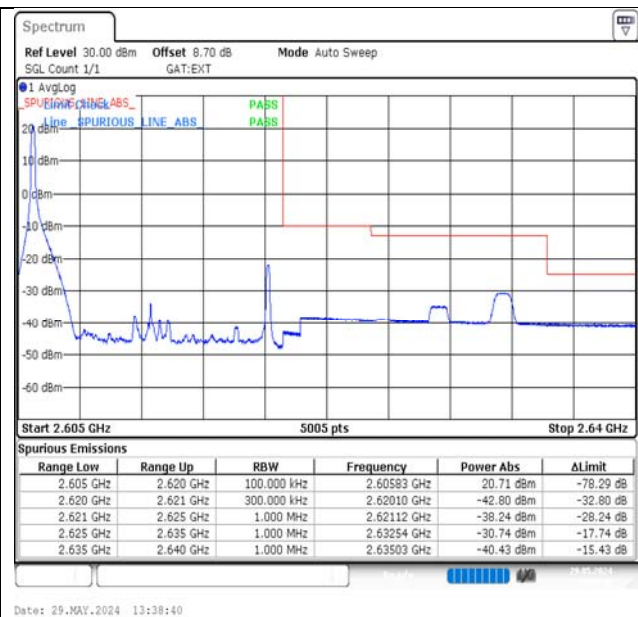
Band38-15MHz-QPSK-38175-1RB#0-PASS
