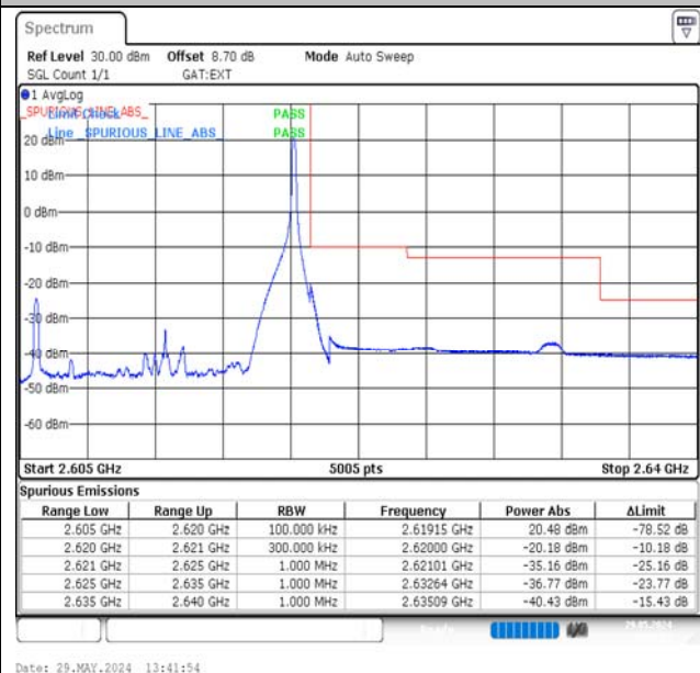
Band38-15MHz-QPSK-38175-1RB#74-PASS
