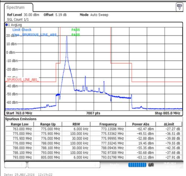
Band13-10MHz-16QAM-23230-1RB#0-PASS
