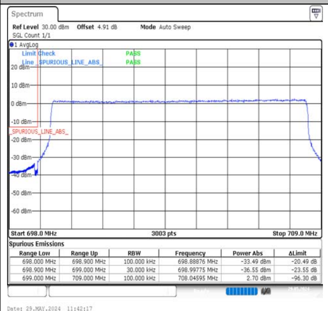
Band12-10MHz-16QAM-23060-50RB#0-PASS
