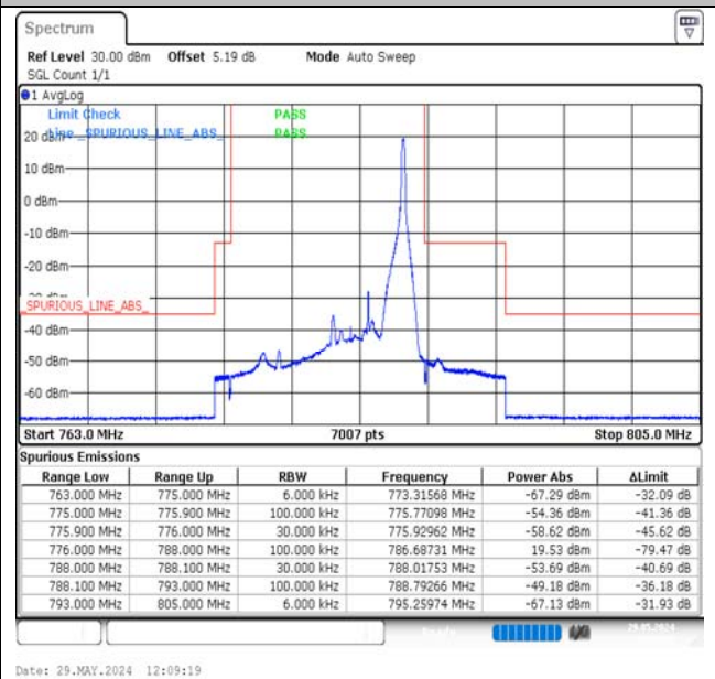
Band13-5MHz-16QAM-23255-1RB#24-PASS
