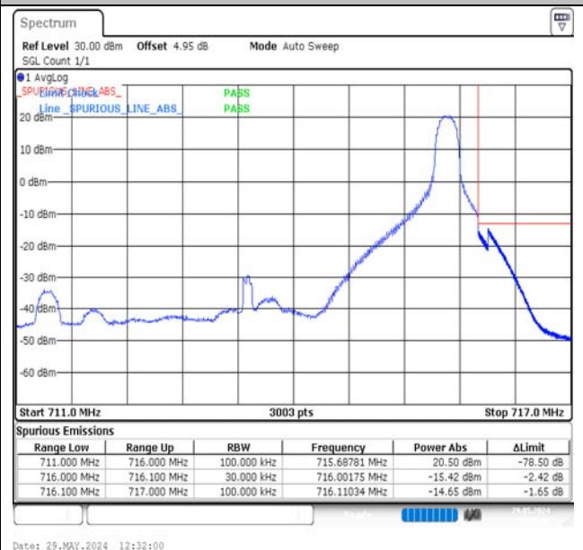
Band17-5MHz-QPSK-23825-1RB#24-PASS
