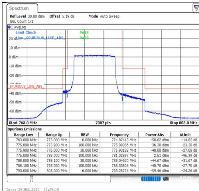
Band13-10MHz-16QAM-23230-50RB#0-PASS
