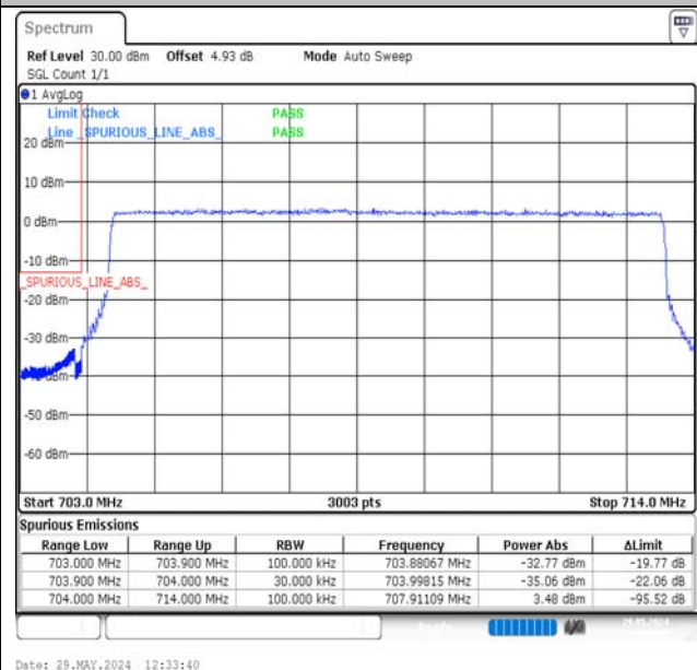
Band17-10MHz-QPSK-23780-50RB#0-PASS
