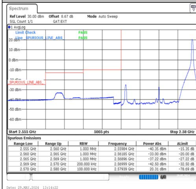
Band38-10MHz-16QAM-37800-1RB#49-PASS
