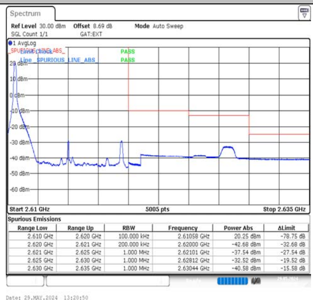
Band38-10MHz-16QAM-38200-1RB#0-PASS
