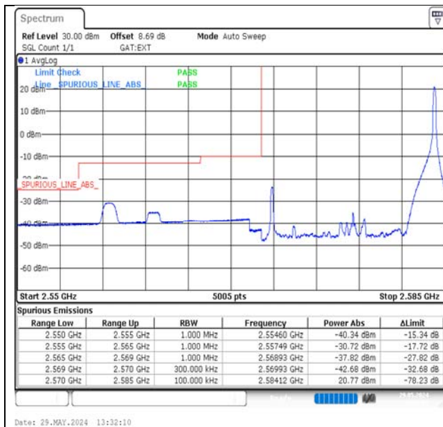
Band38-15MHz-QPSK-37825-1RB#74-PASS
