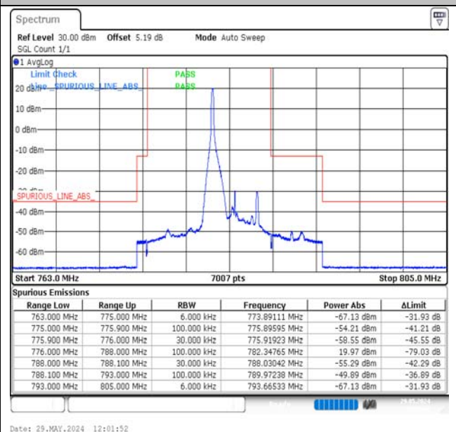
Band13-5MHz-QPSK-23255-1RB#0-PASS
