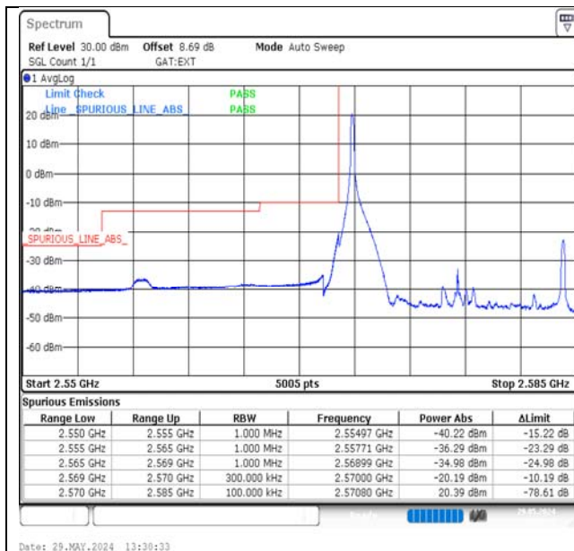
Band38-15MHz-16QAM-37825-1RB#0-PASS
