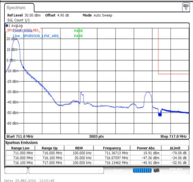
Band17-5MHz-16QAM-23825-1RB#0-PASS
