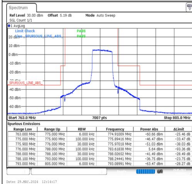
Band13-5MHz-16QAM-23255-25RB#0-PASS
