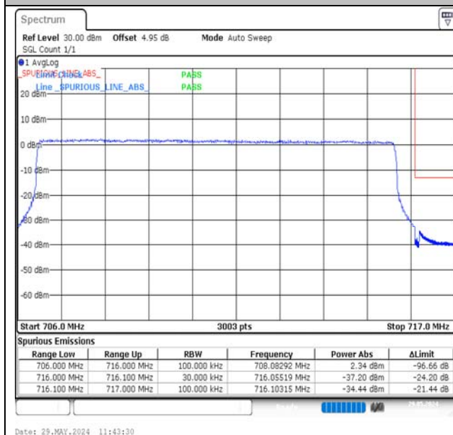
Band12-10MHz-16QAM-23130-50RB#0-PASS
