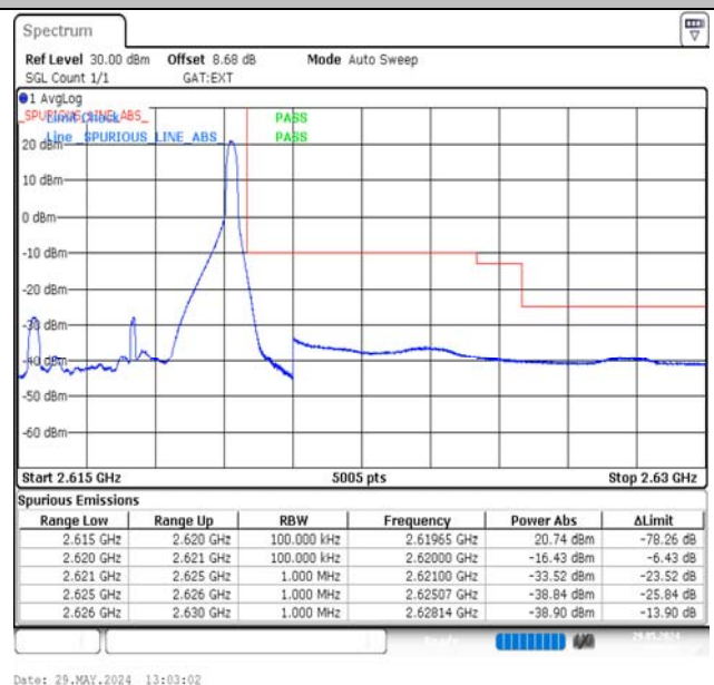
Band38-5MHz-QPSK-38225-1RB#24-PASS
