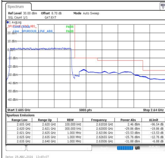
Band38-15MHz-QPSK-38175-75RB#0-PASS
