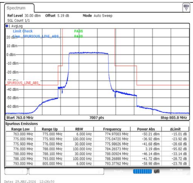
Band13-10MHz-QPSK-23230-50RB#0-PASS
