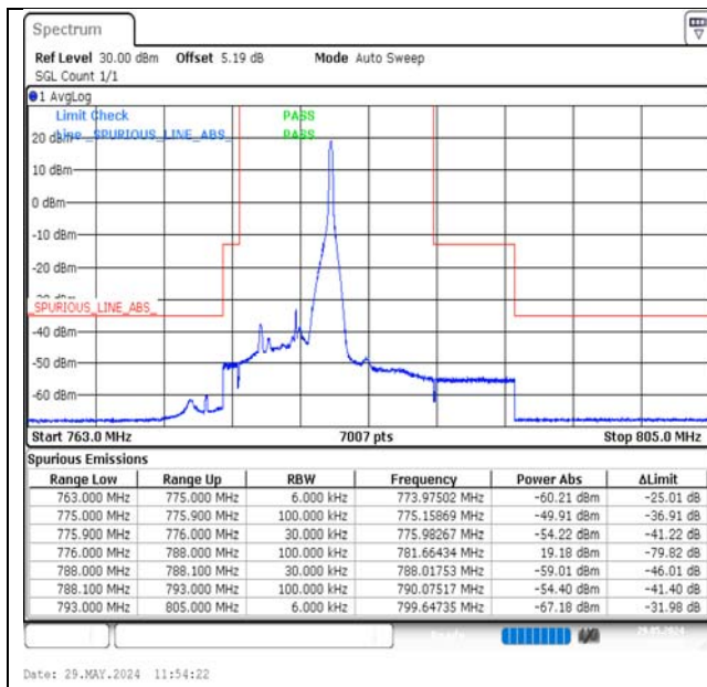
Band13-5MHz-16QAM-23205-1RB#24-PASS
