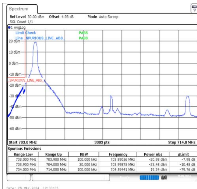
Band17-10MHz-16QAM-23780-1RB#0-PASS
