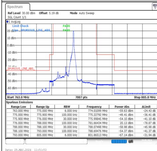
Band13-5MHz-QPSK-23205-1RB#24-PASS
