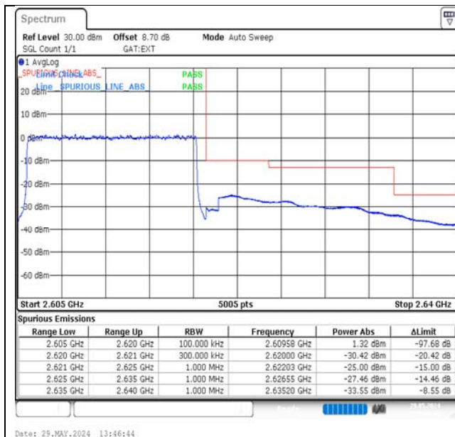
Band38-15MHz-16QAM-38175-75RB#0-PASS
