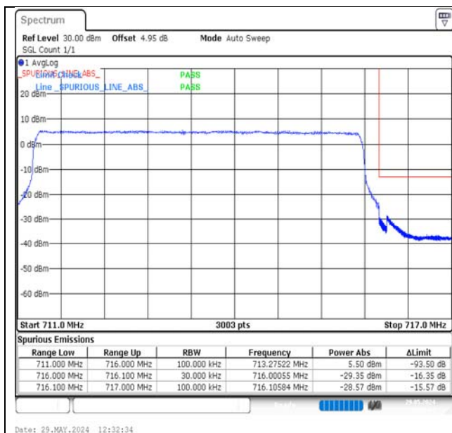
Band17-5MHz-16QAM-23825-25RB#0-PASS
