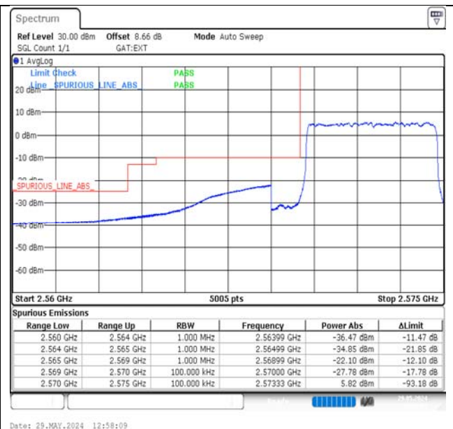
Band38-5MHz-16QAM-37775-25RB#0-PASS
