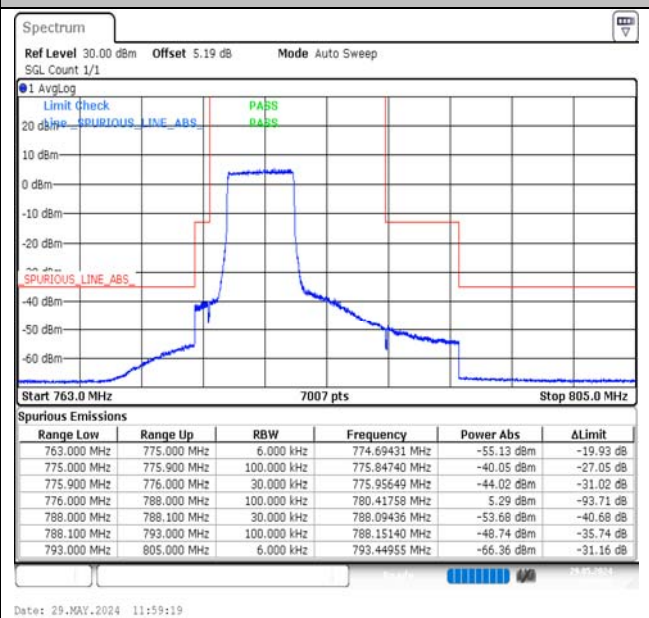
Band13-5MHz-16QAM-23205-25RB#0-PASS
