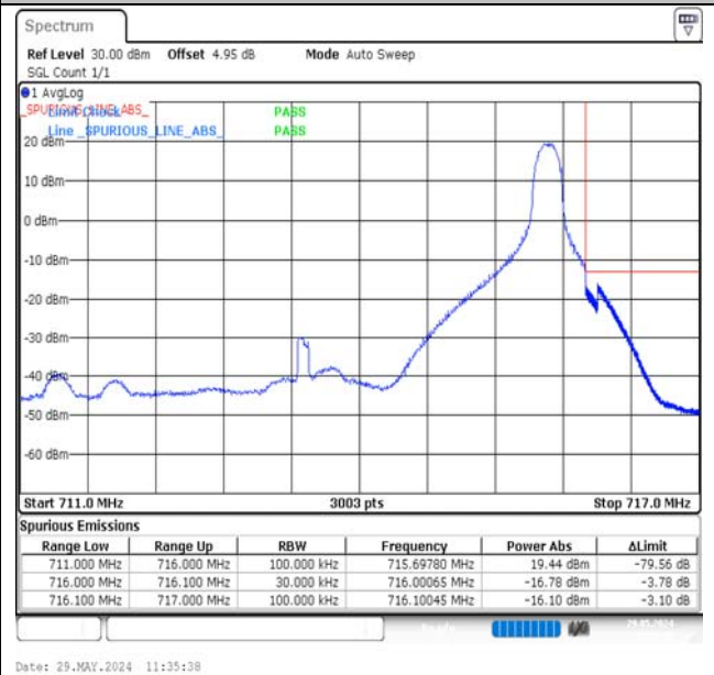
Band12-5MHz-16QAM-23155-1RB#24-PASS
