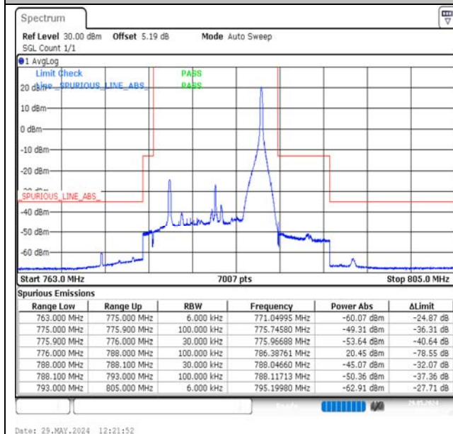
Band13-10MHz-QPSK-23230-1RB#49-PASS
