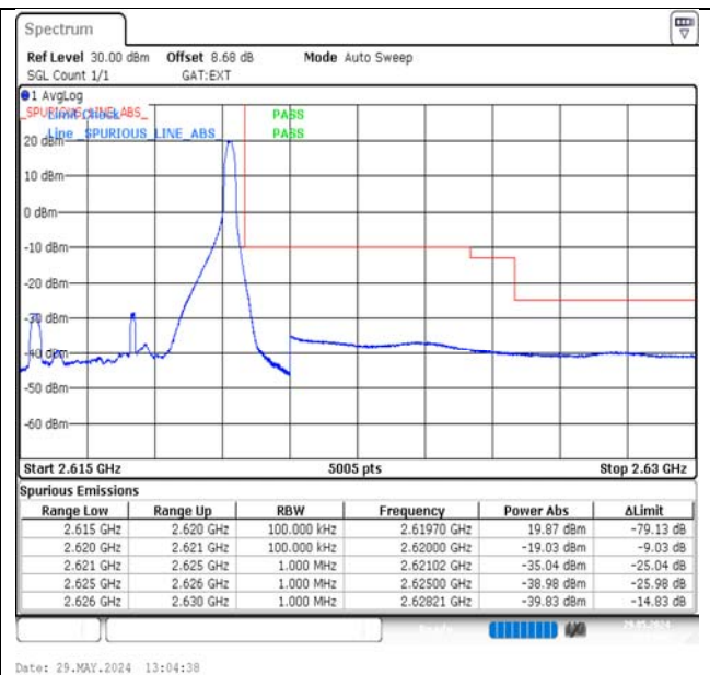
Band38-5MHz-16QAM-38225-1RB#24-PASS
