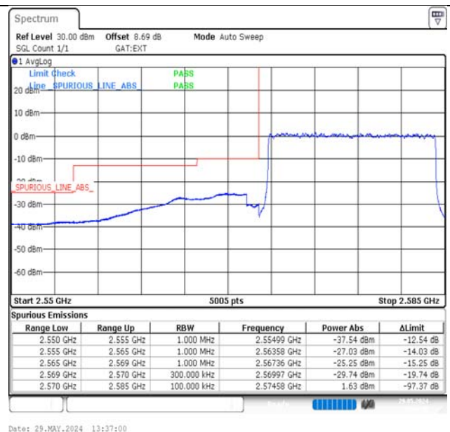
Band38-15MHz-16QAM-37825-75RB#0-PASS
