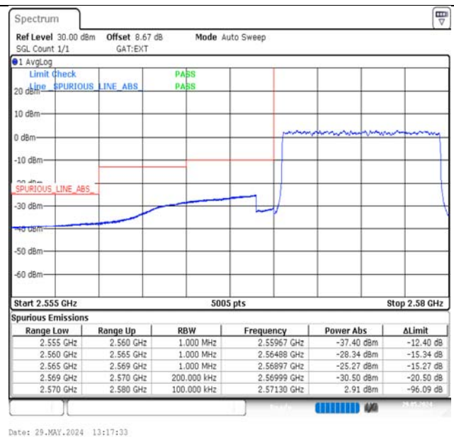
Band38-10MHz-16QAM-37800-50RB#0-PASS
