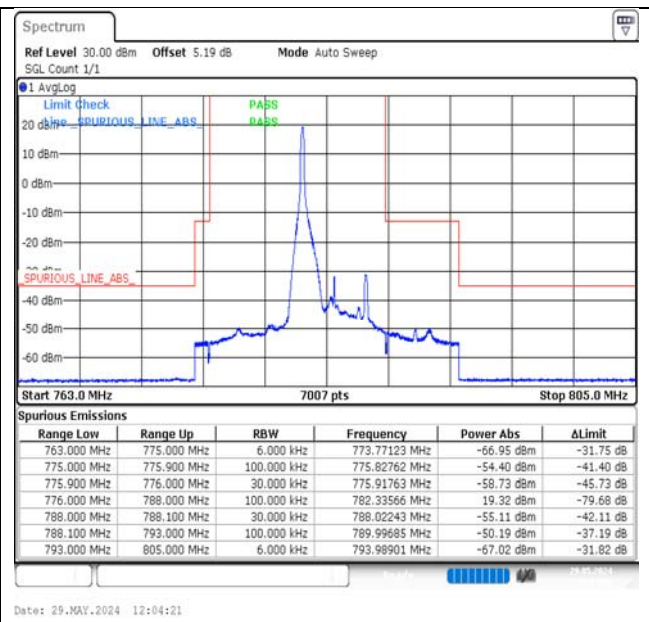
Band13-5MHz-16QAM-23255-1RB#0-PASS
