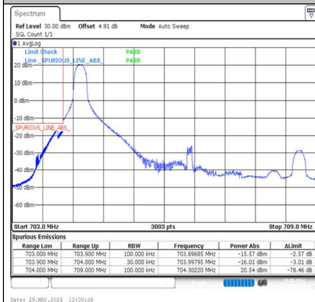
Band17-5MHz-QPSK-23755-1RB#0-PASS
