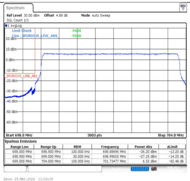
Band12-5MHz-QPSK-23035-25RB#0-PASS
