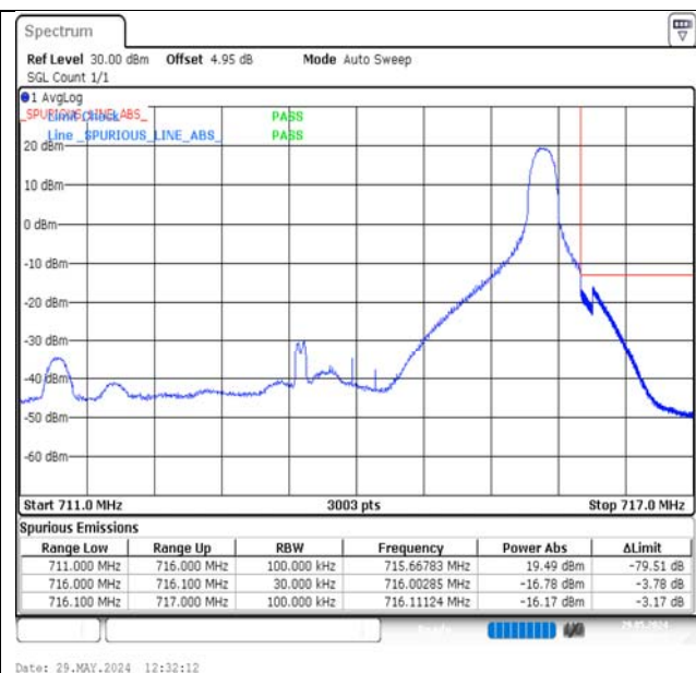
Band17-5MHz-16QAM-23825-1RB#24-PASS
