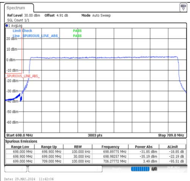
Band12-10MHz-QPSK-23060-50RB#0-PASS
