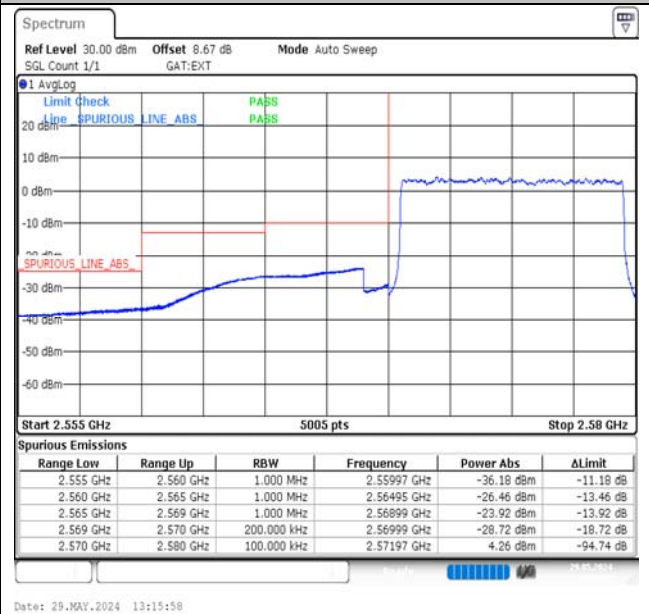
Band38-10MHz-QPSK-37800-50RB#0-PASS
