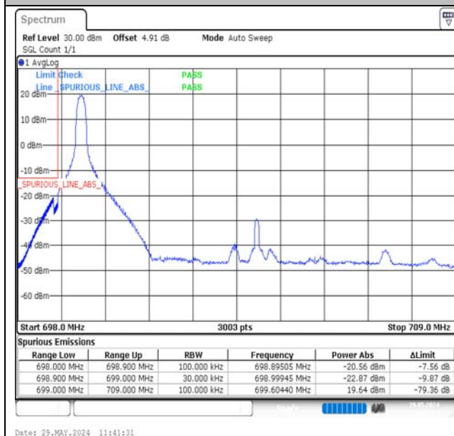
Band12-10MHz-16QAM-23060-1RB#0-PASS
