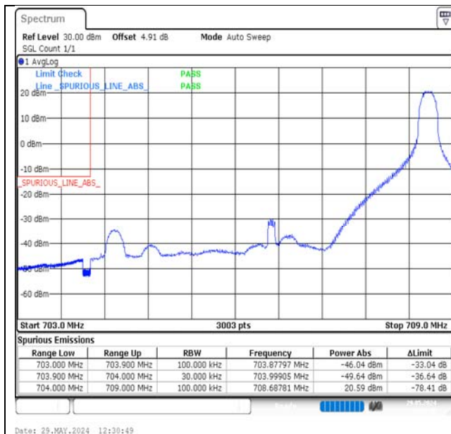
Band17-5MHz-QPSK-23755-1RB#24-PASS
