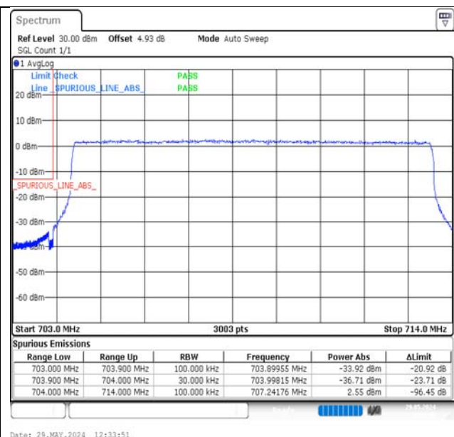
Band17-10MHz-16QAM-23780-50RB#0-PASS
