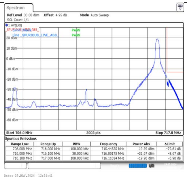
Band17-10MHz-16QAM-23800-1RB#49-PASS
