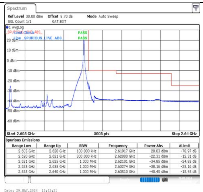
Band38-15MHz-16QAM-38175-1RB#74-PASS
