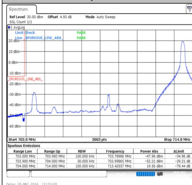
Band17-10MHz-16QAM-23780-1RB#49-PASS
