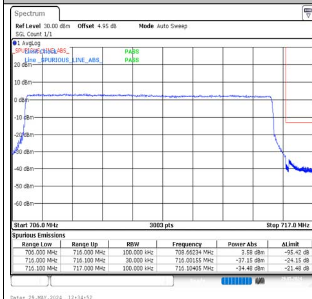
Band17-10MHz-QPSK-23800-50RB#0-PASS
