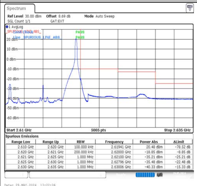
Band38-10MHz-QPSK-38200-1RB#49-PASS
