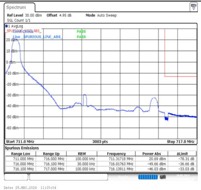
Band12-5MHz-QPSK-23155-1RB#0-PASS
