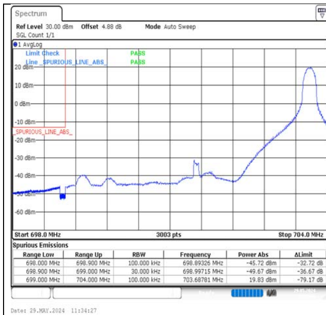
Band12-5MHz-16QAM-23035-1RB#24-PASS
