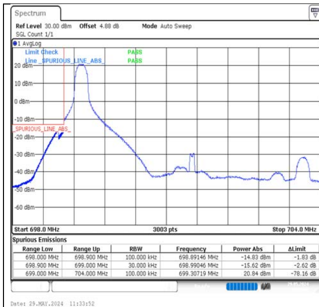
Band12-5MHz-QPSK-23035-1RB#0-PASS
