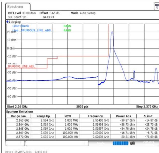
Band38-5MHz-16QAM-37775-1RB#0-PASS
