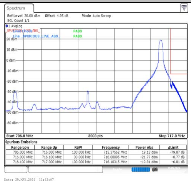
Band12-10MHz-16QAM-23130-1RB#49-PASS
