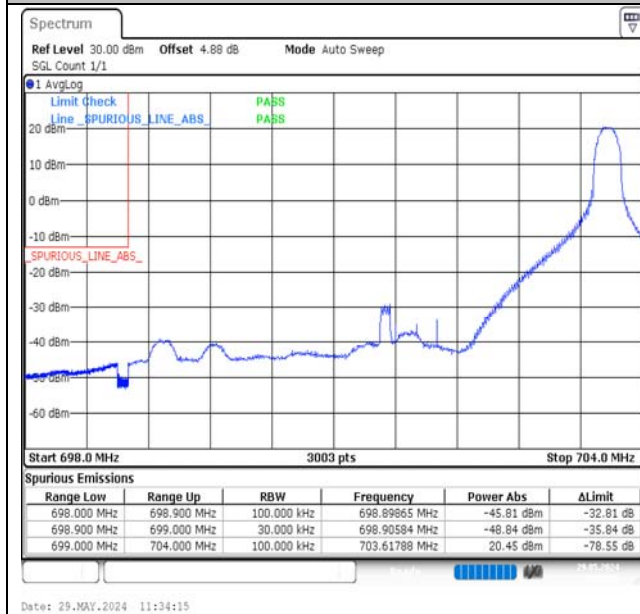
Band12-5MHz-QPSK-23035-1RB#24-PASS
