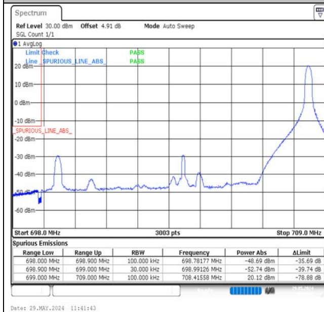
Band12-10MHz-QPSK-23060-1RB#49-PASS
