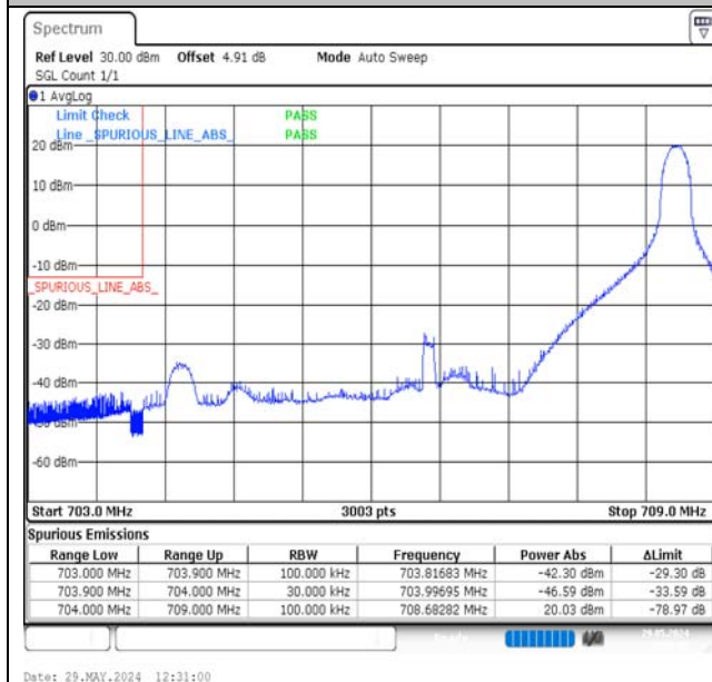
Band17-5MHz-16QAM-23755-1RB#24-PASS
