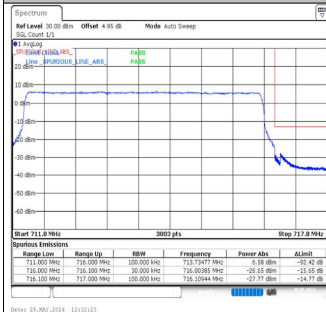
Band17-5MHz-QPSK-23825-25RB#0-PASS
