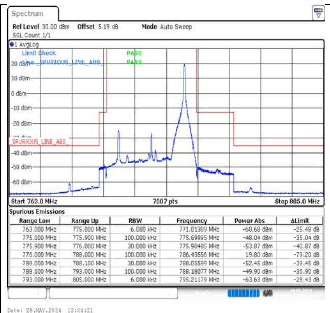
Band13-10MHz-16QAM-23230-1RB#49-PASS
