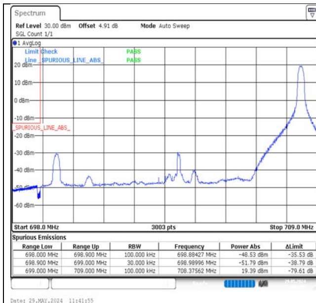
Band12-10MHz-16QAM-23060-1RB#49-PASS
