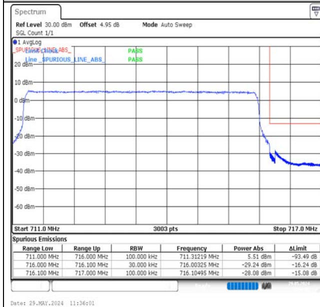
Band12-5MHz-16QAM-23155-25RB#0-PASS
