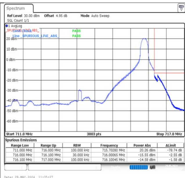
Band12-5MHz-QPSK-23155-1RB#24-PASS
