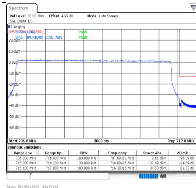
Band17-10MHz-16QAM-23800-50RB#0-PASS
