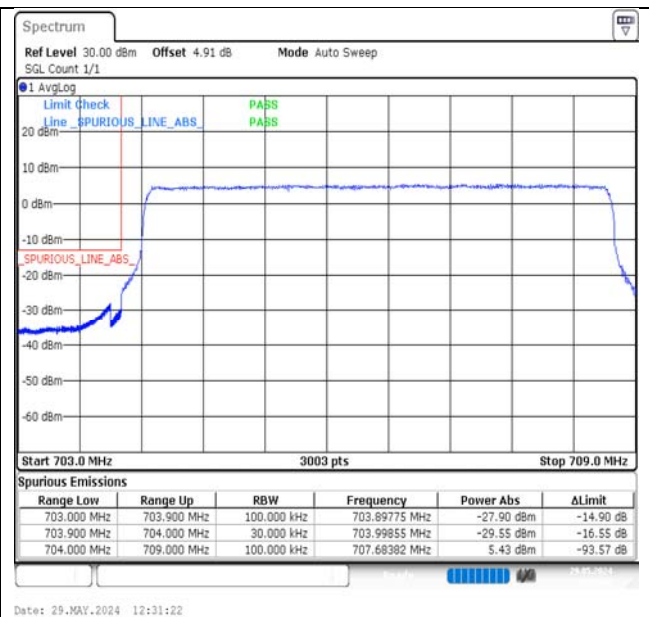
Band17-5MHz-16QAM-23755-25RB#0-PASS
