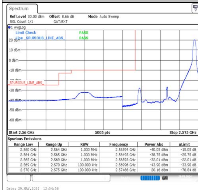
Band38-5MHz-16QAM-37775-1RB#24-PASS
