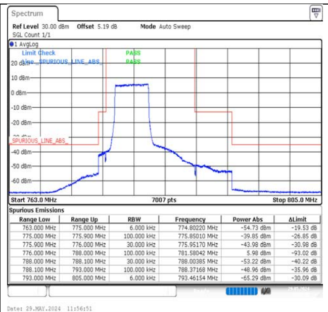
Band13-5MHz-QPSK-23205-25RB#0-PASS
