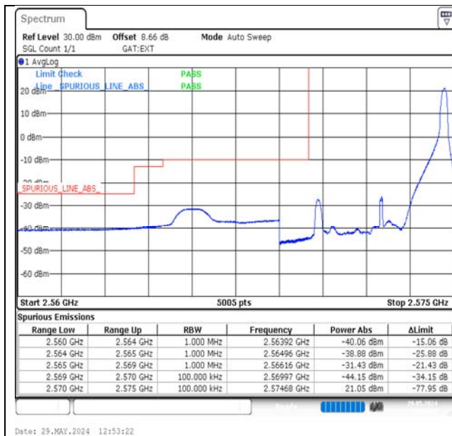
Band38-5MHz-QPSK-37775-1RB#24-PASS
