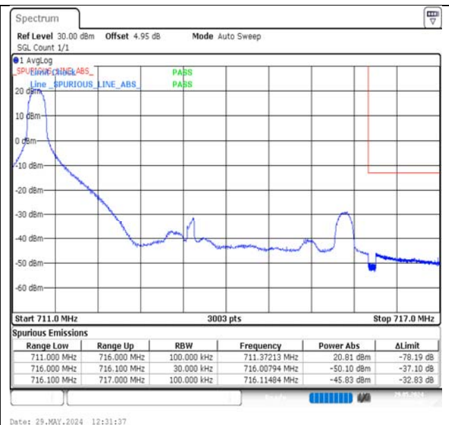
Band17-5MHz-QPSK-23825-1RB#0-PASS
