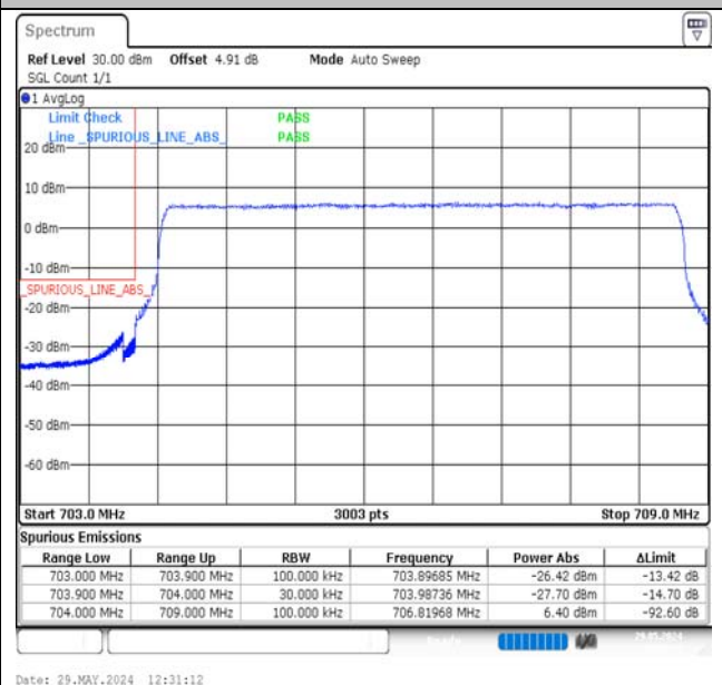
Band17-5MHz-QPSK-23755-25RB#0-PASS
