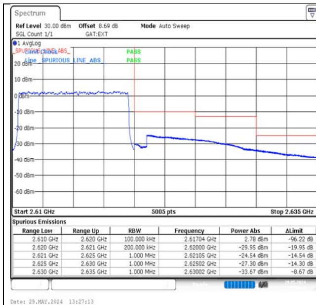
Band38-10MHz-16QAM-38200-50RB#0-PASS
