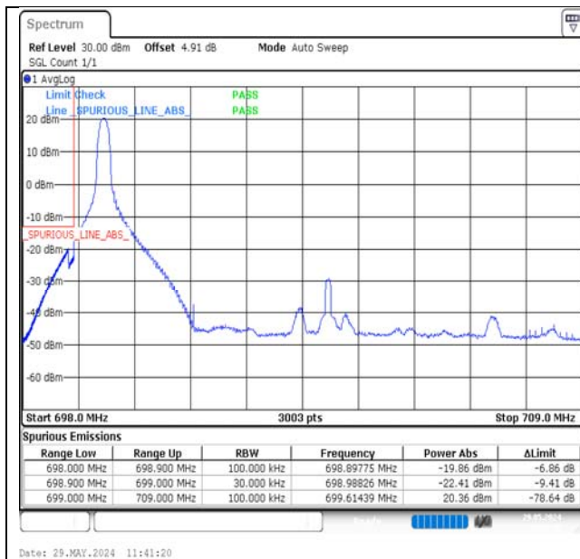
Band12-10MHz-QPSK-23060-1RB#0-PASS
