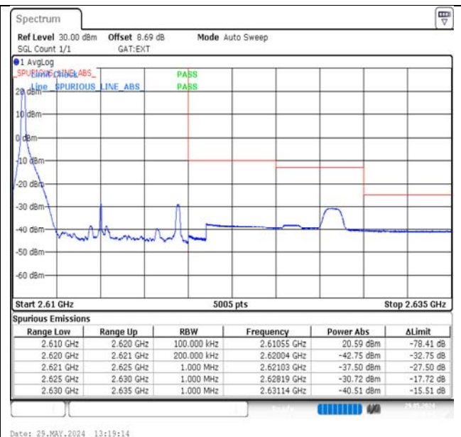
Band38-10MHz-QPSK-38200-1RB#0-PASS
