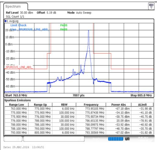
Band13-5MHz-QPSK-23255-1RB#24-PASS
