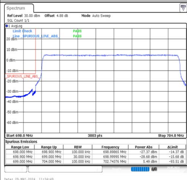
Band12-5MHz-16QAM-23035-25RB#0-PASS
