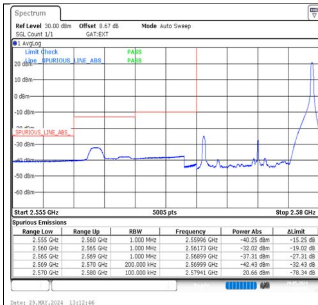
Band38-10MHz-QPSK-37800-1RB#49-PASS
