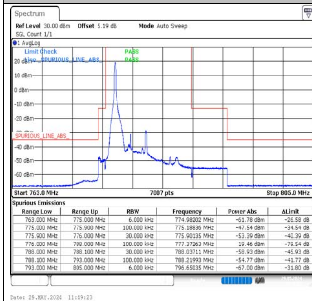
Band13-5MHz-16QAM-23205-1RB#0-PASS
