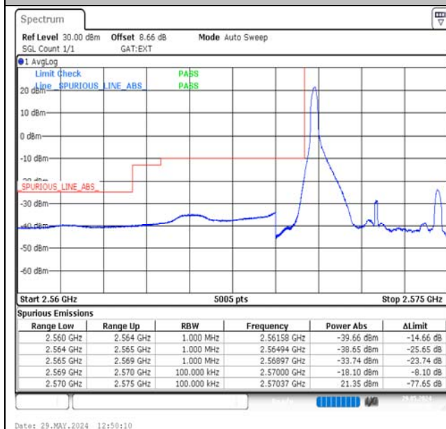
Band38-5MHz-QPSK-37775-1RB#0-PASS
