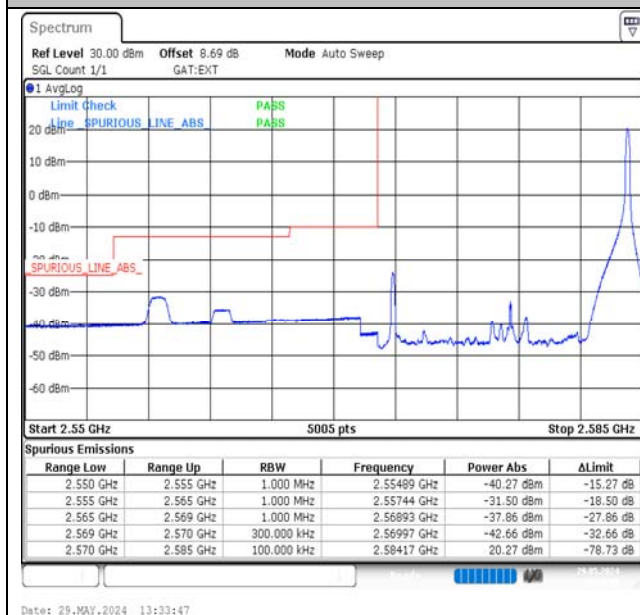
Band38-15MHz-16QAM-37825-1RB#74-PASS
