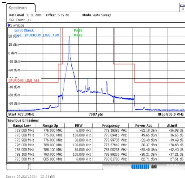
Band13-10MHz-QPSK-23230-1RB#0-PASS
