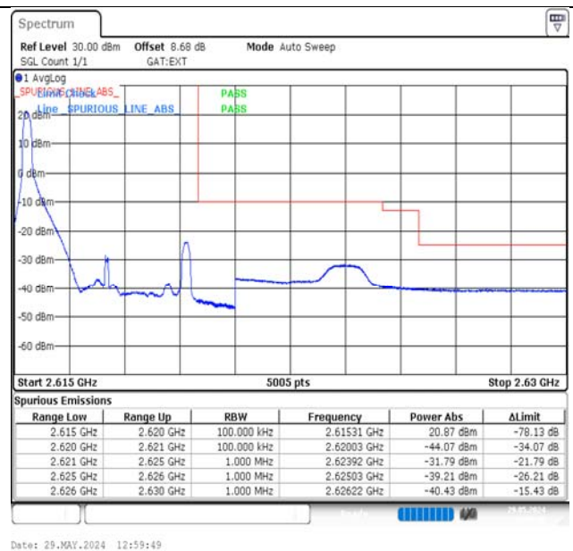
Band38-5MHz-QPSK-38225-1RB#0-PASS
