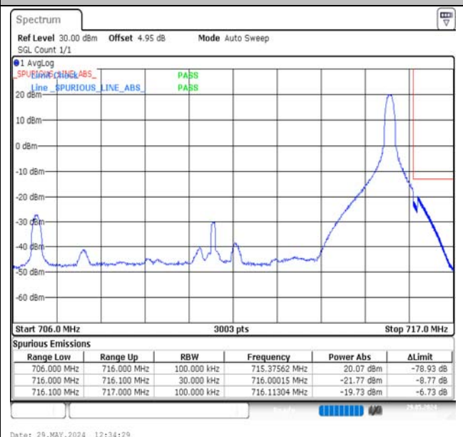
Band17-10MHz-QPSK-23800-1RB#49-PASS
