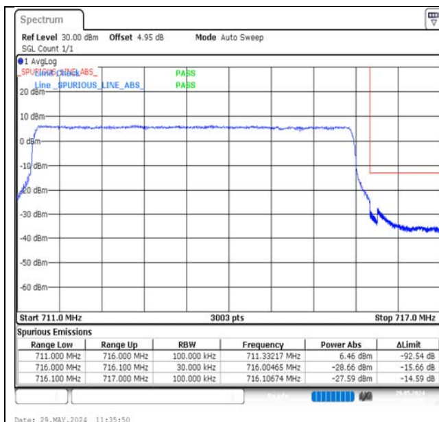
Band12-5MHz-QPSK-23155-25RB#0-PASS
