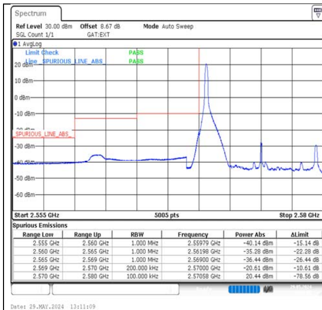
Band38-10MHz-16QAM-37800-1RB#0-PASS
