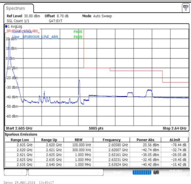
Band38-15MHz-16QAM-38175-1RB#0-PASS
