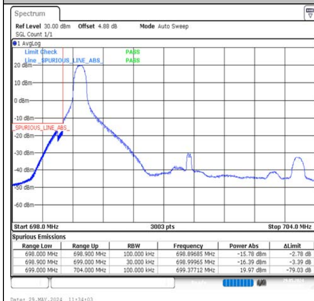
Band12-5MHz-16QAM-23035-1RB#0-PASS
