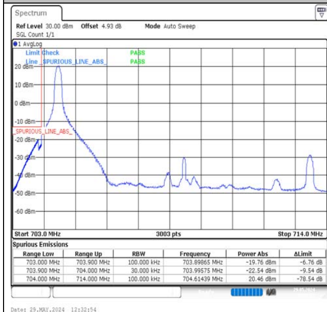
Band17-10MHz-QPSK-23780-1RB#0-PASS
