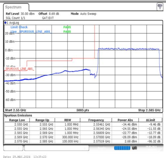
Band38-15MHz-QPSK-37825-75RB#0-PASS
