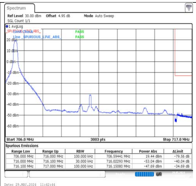
Band12-10MHz-16QAM-23130-1RB#0-PASS
