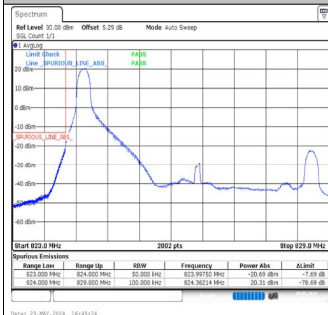
Band5-5MHz-16QAM-20425-1RB#0-PASS
