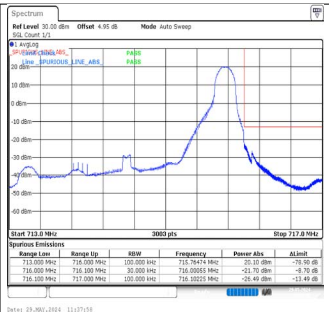
Band12-3MHz-QPSK-23165-1RB#14-PASS
