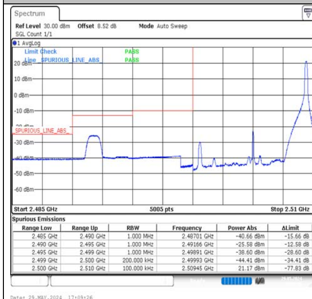
Band7-10MHz-QPSK-20800-1RB#49-PASS
