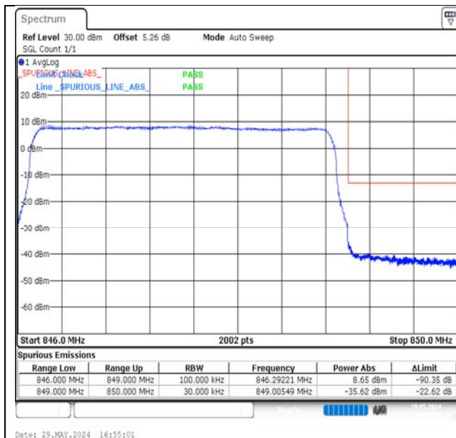
Band5-3MHz-QPSK-20635-15RB#0-PASS
