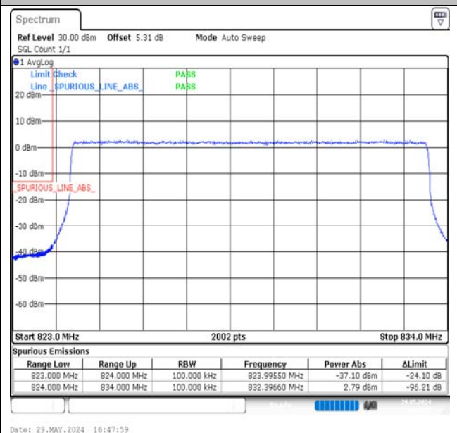
Band5-10MHz-16QAM-20450-50RB#0-PASS
