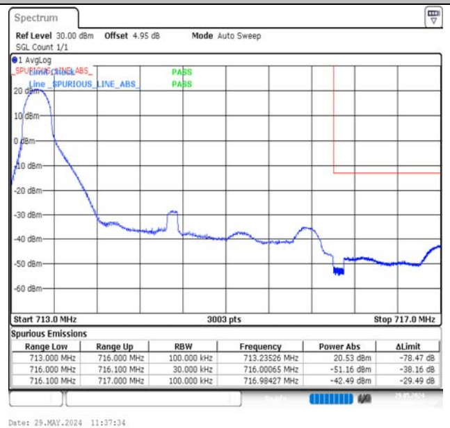
Band12-3MHz-QPSK-23165-1RB#0-PASS
