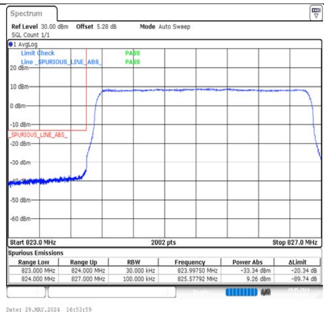
Band5-3MHz-QPSK-20415-15RB#0-PASS
