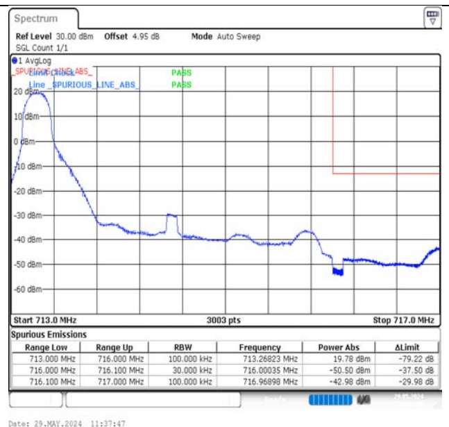
Band12-3MHz-16QAM-23165-1RB#0-PASS
