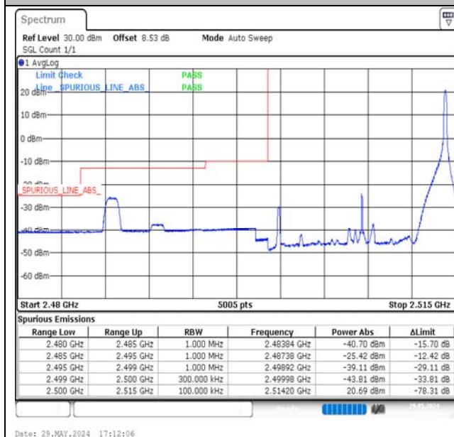
Band7-15MHz-QPSK-20825-1RB#74-PASS
