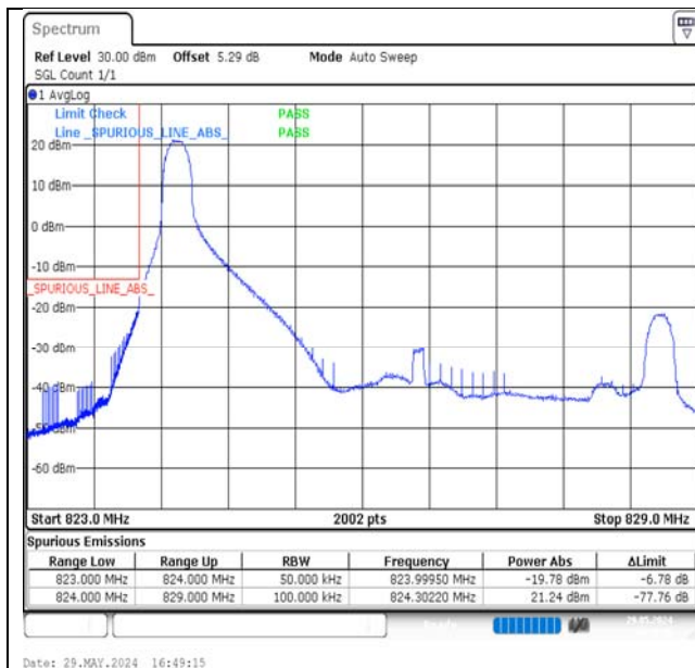
Band5-5MHz-QPSK-20425-1RB#0-PASS
