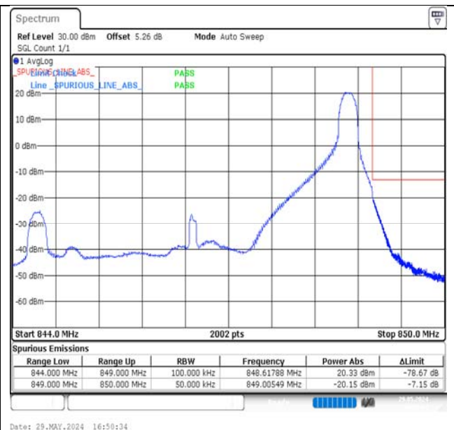
Band5-5MHz-QPSK-20625-1RB#24-PASS
