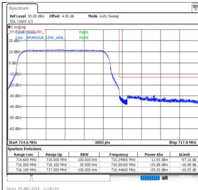
Band12-1.4MHz-QPSK-23173-6RB#0-PASS
