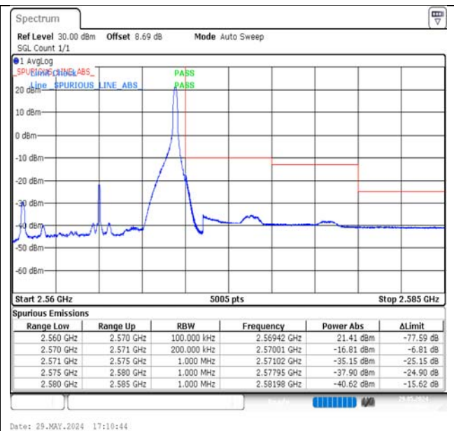
Band7-10MHz-QPSK-21400-1RB#49-PASS
