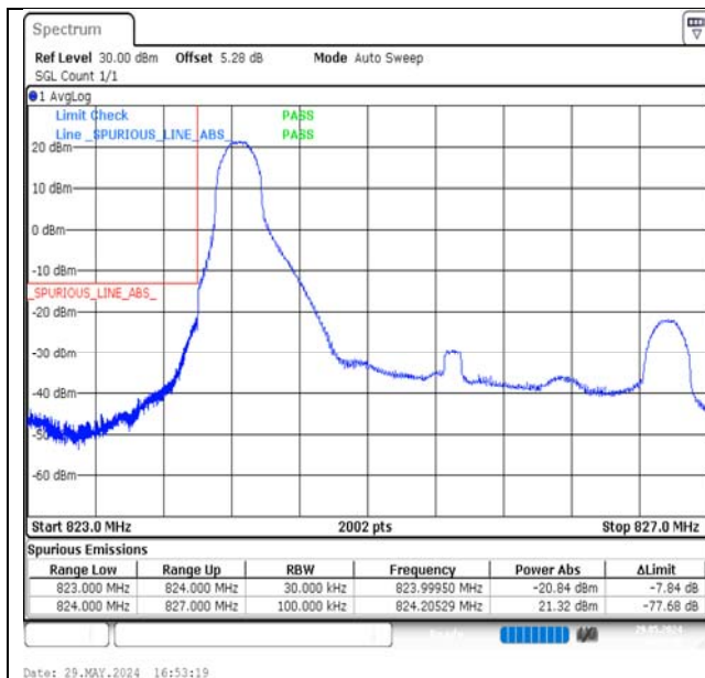
Band5-3MHz-QPSK-20415-1RB#0-PASS
