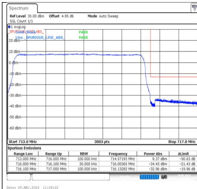
Band12-3MHz-QPSK-23165-15RB#0-PASS
