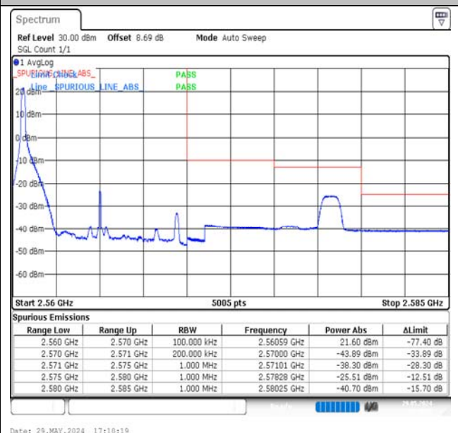
Band7-10MHz-QPSK-21400-1RB#0-PASS
