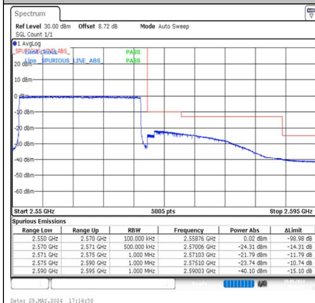
Band7-20MHz-16QAM-21350-100RB#0-PASS
