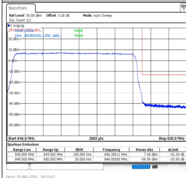
Band5-3MHz-16QAM-20635-15RB#0-PASS
