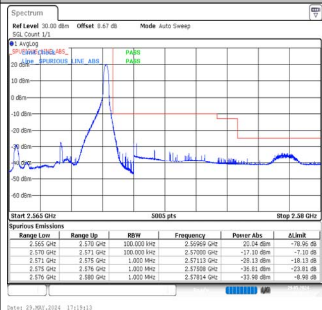
Band7-5MHz-16QAM-21425-1RB#24-PASS
