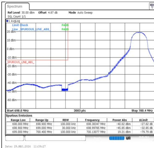
Band12-1.4MHz-16QAM-23017-1RB#5-PASS
