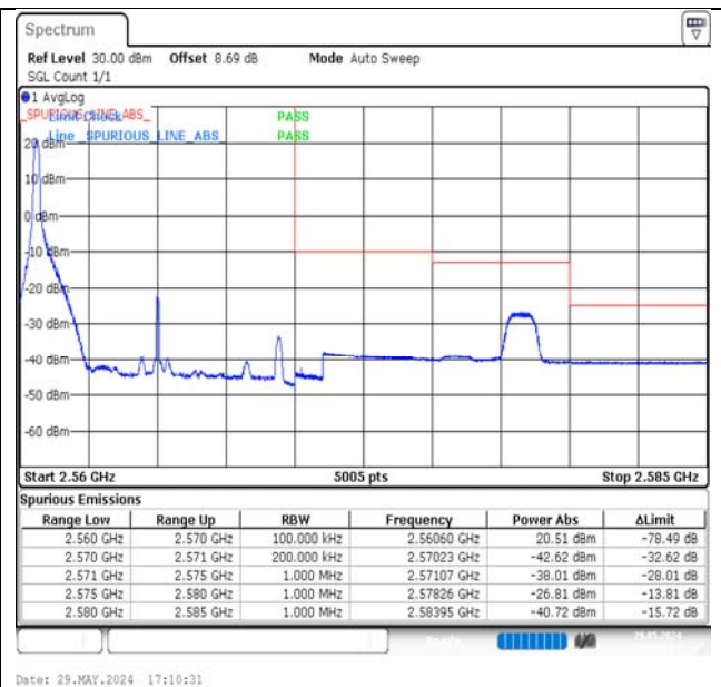
Band7-10MHz-16QAM-21400-1RB#0-PASS
