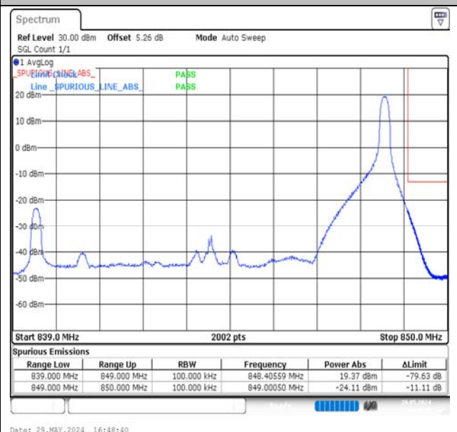
Band5-10MHz-16QAM-20600-1RB#49-PASS
