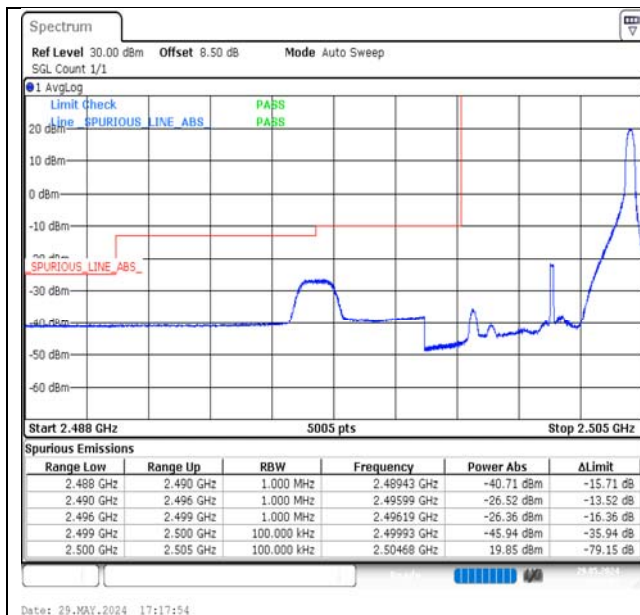
Band7-5MHz-16QAM-20775-1RB#24-PASS
