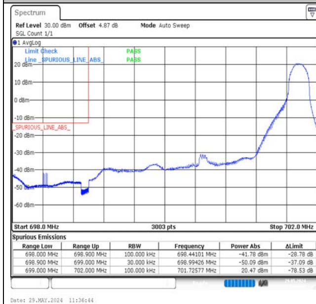
Band12-3MHz-QPSK-23025-1RB#14-PASS
