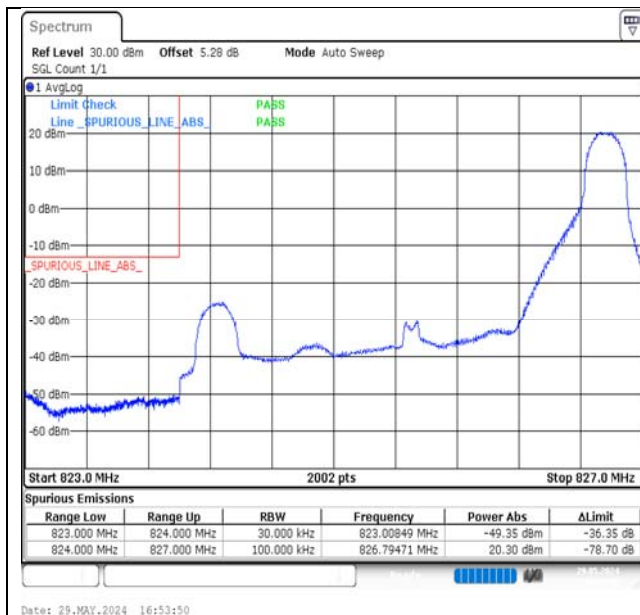
Band5-3MHz-16QAM-20415-1RB#14-PASS
