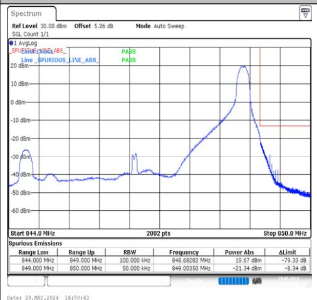
Band5-5MHz-16QAM-20625-1RB#24-PASS
