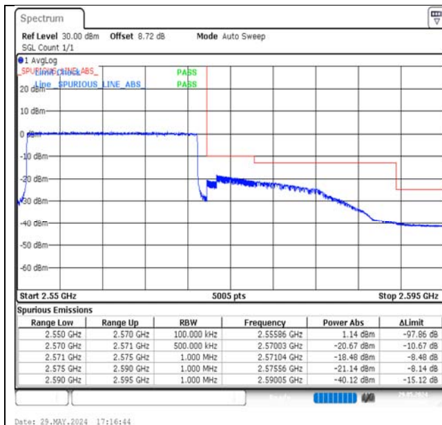
Band7-20MHz-QPSK-21350-100RB#0-PASS
