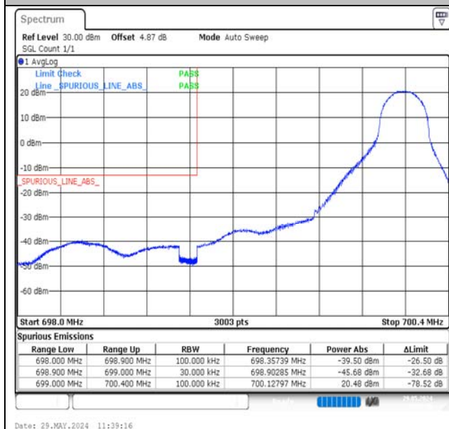
Band12-1.4MHz-QPSK-23017-1RB#5-PASS
