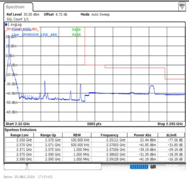
Band7-20MHz-QPSK-21350-1RB#0-PASS
