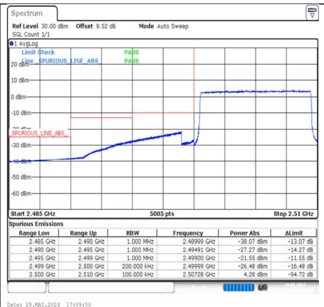
Band7-10MHz-QPSK-20800-50RB#0-PASS
