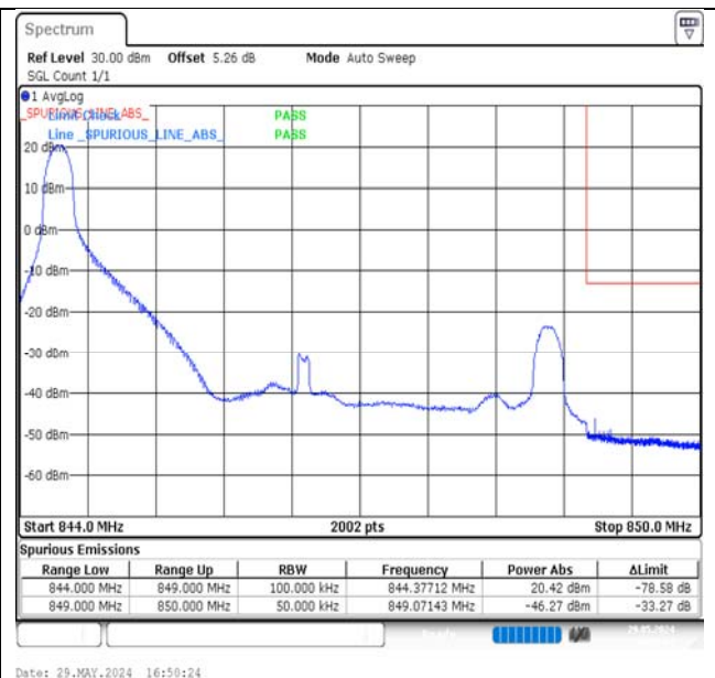
Band5-5MHz-16QAM-20625-1RB#0-PASS
