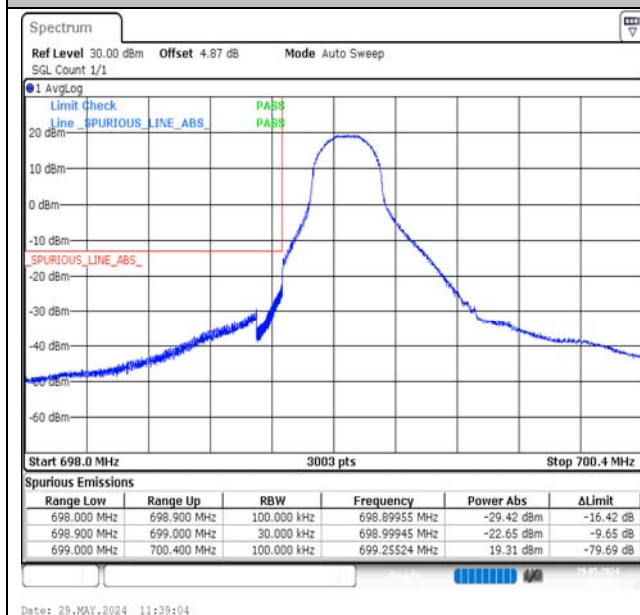
Band12-1.4MHz-16QAM-23017-1RB#0-PASS
