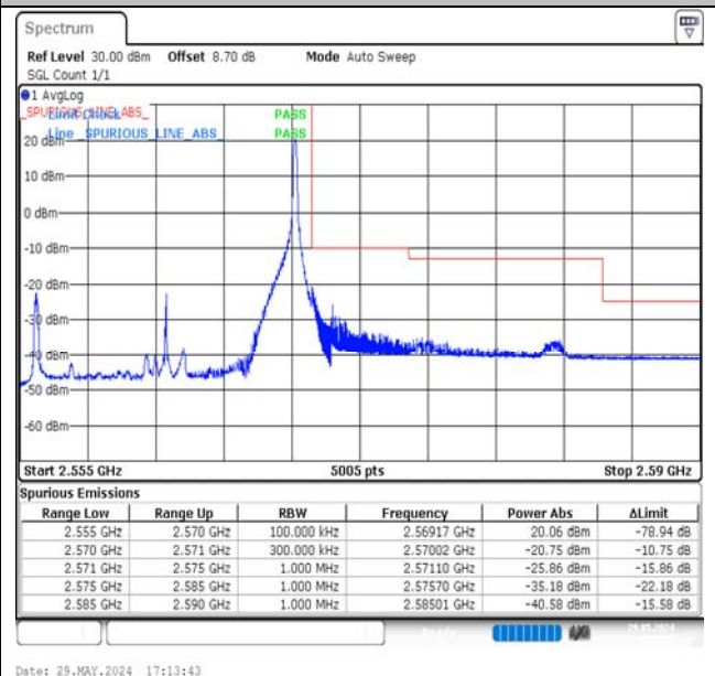
Band7-15MHz-16QAM-21375-1RB#74-PASS
