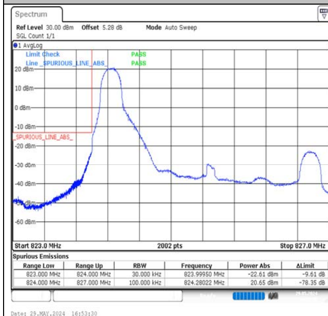
Band5-3MHz-16QAM-20415-1RB#0-PASS
