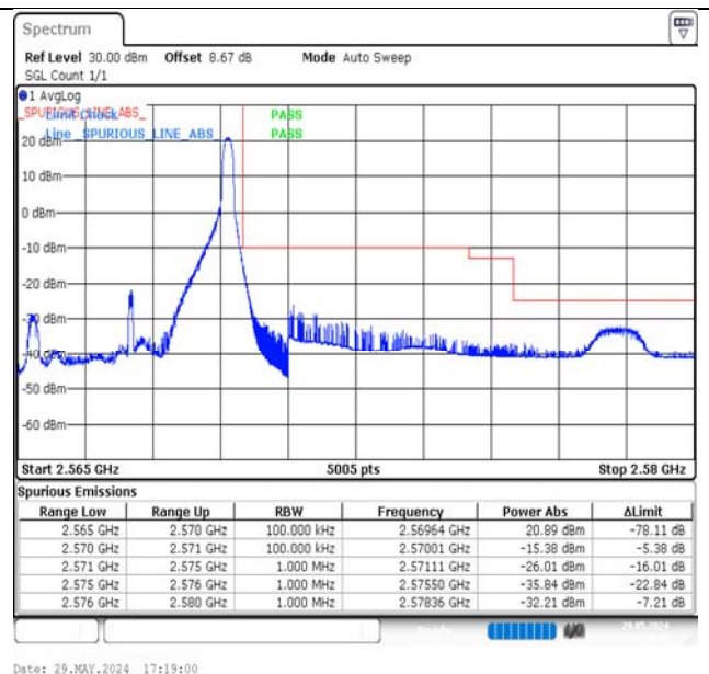
Band7-5MHz-QPSK-21425-1RB#24-PASS
