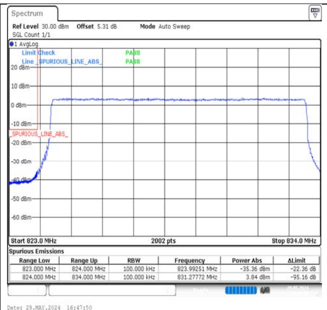
Band5-10MHz-QPSK-20450-50RB#0-PASS
