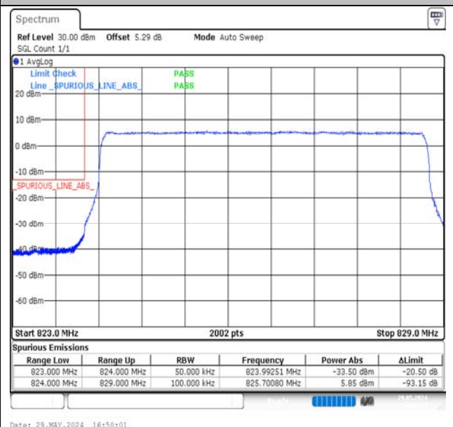
Band5-5MHz-16QAM-20425-25RB#0-PASS
