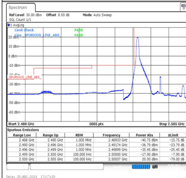
Band7-5MHz-16QAM-20775-1RB#0-PASS
