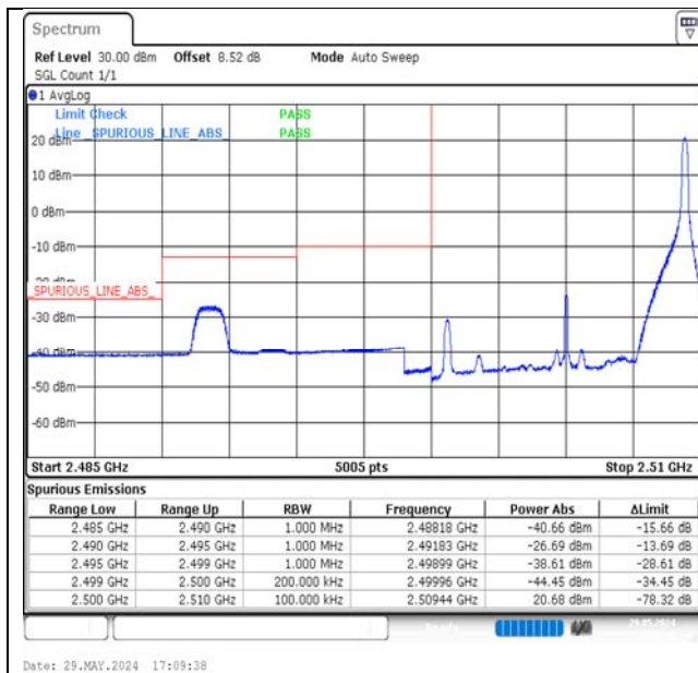
Band7-10MHz-16QAM-20800-1RB#49-PASS
