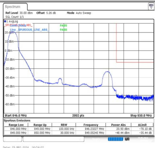
Band5-3MHz-QPSK-20635-1RB#0-PASS
