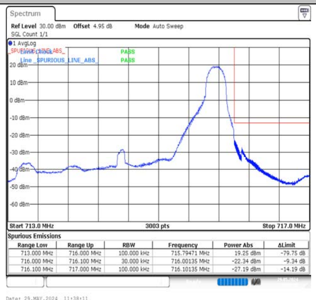
Band12-3MHz-16QAM-23165-1RB#14-PASS
