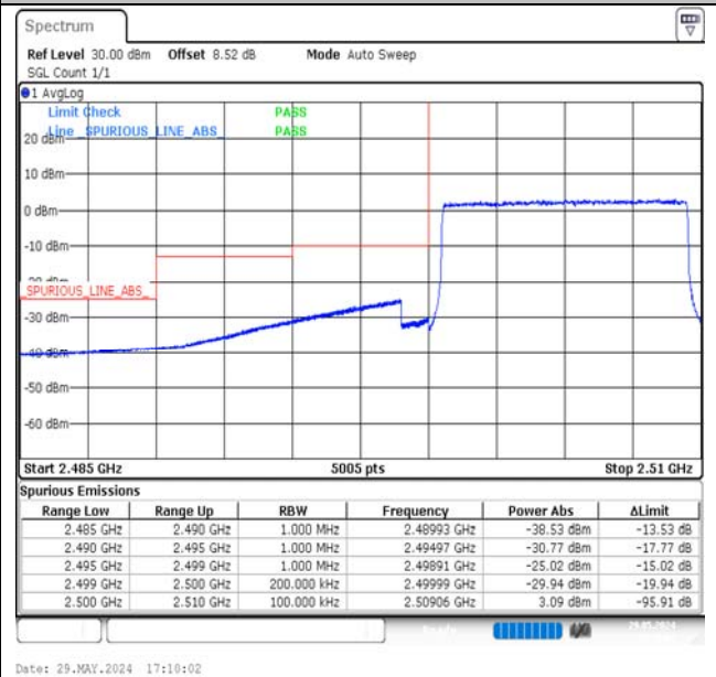
Band7-10MHz-16QAM-20800-50RB#0-PASS
