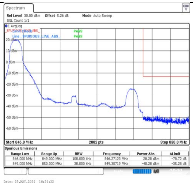
Band5-3MHz-16QAM-20635-1RB#0-PASS
