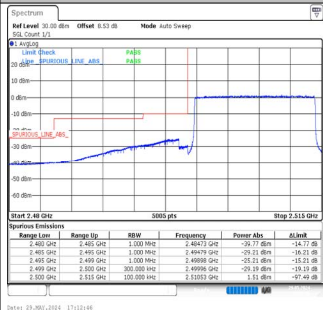
Band7-15MHz-16QAM-20825-75RB#0-PASS
