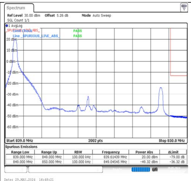
Band5-10MHz-16QAM-20600-1RB#0-PASS
