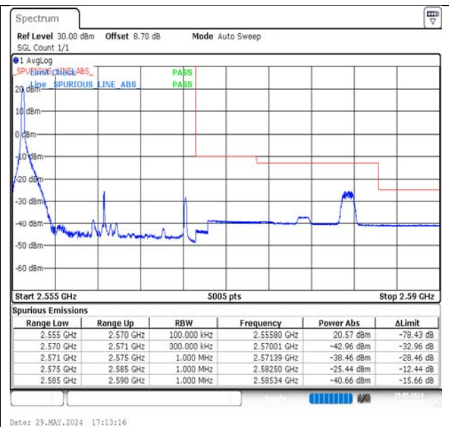
Band7-15MHz-16QAM-21375-1RB#0-PASS
