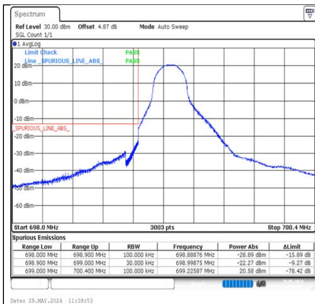
Band12-1.4MHz-QPSK-23017-1RB#0-PASS
