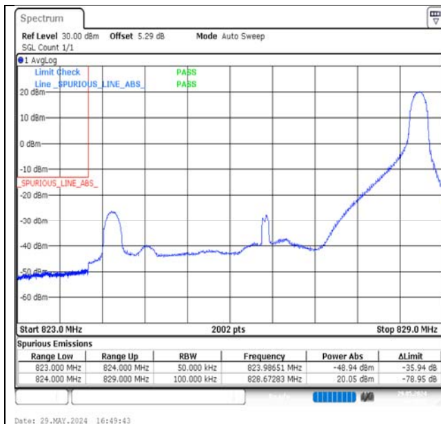
Band5-5MHz-16QAM-20425-1RB#24-PASS
