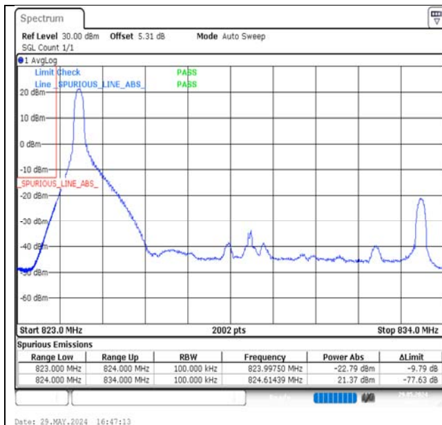
Band5-10MHz-QPSK-20450-1RB#0-PASS
