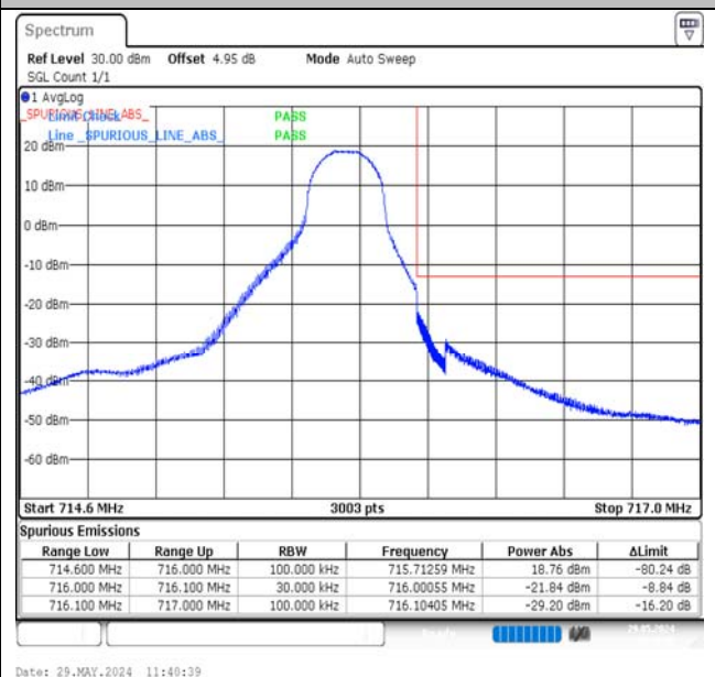
Band12-1.4MHz-16QAM-23173-1RB#5-PASS
