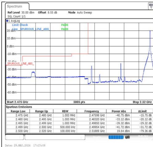
Band7-20MHz-16QAM-20850-1RB#99-PASS
