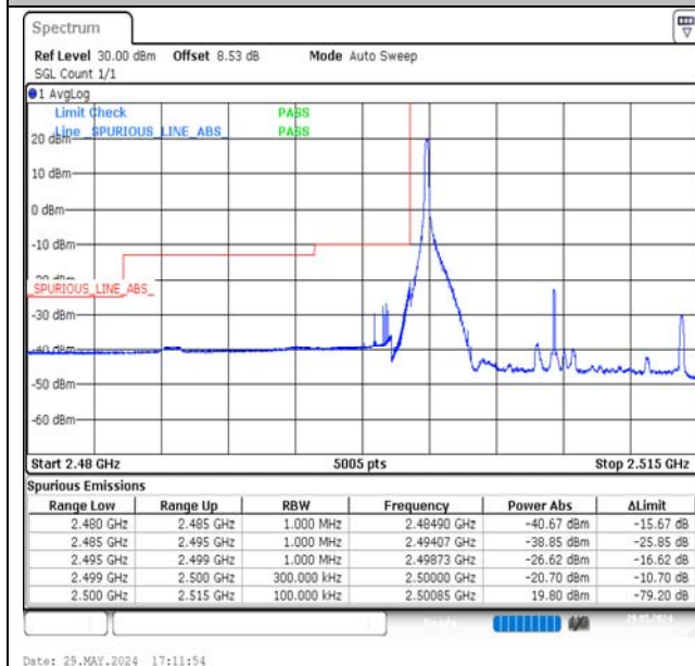
Band7-15MHz-16QAM-20825-1RB#0-PASS
