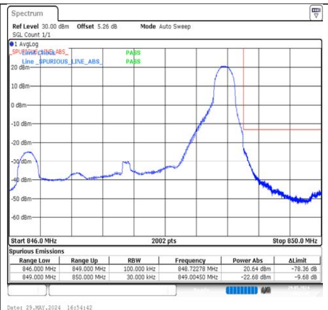
Band5-3MHz-QPSK-20635-1RB#14-PASS
