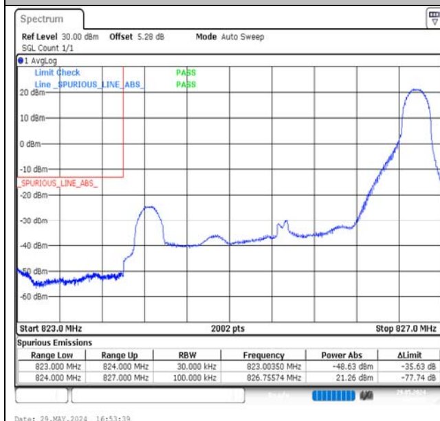
Band5-3MHz-QPSK-20415-1RB#14-PASS
