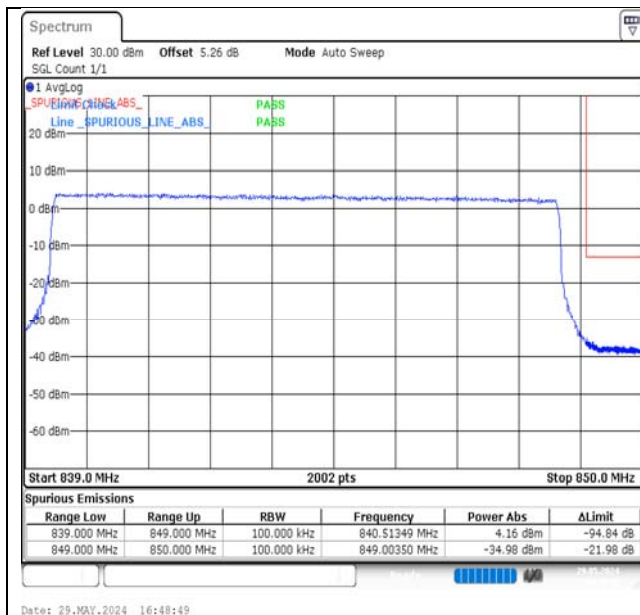
Band5-10MHz-QPSK-20600-50RB#0-PASS
