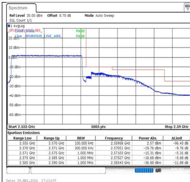
Band7-15MHz-QPSK-21375-75RB#0-PASS
