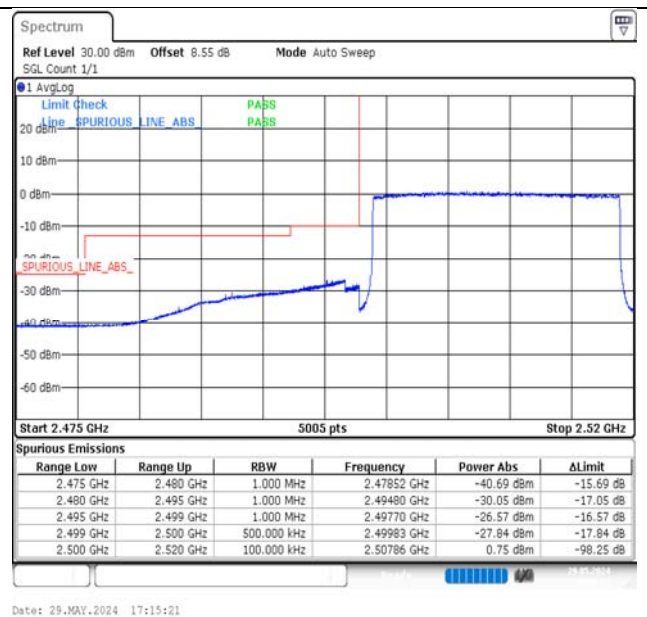
Band7-20MHz-QPSK-20850-100RB#0-PASS
