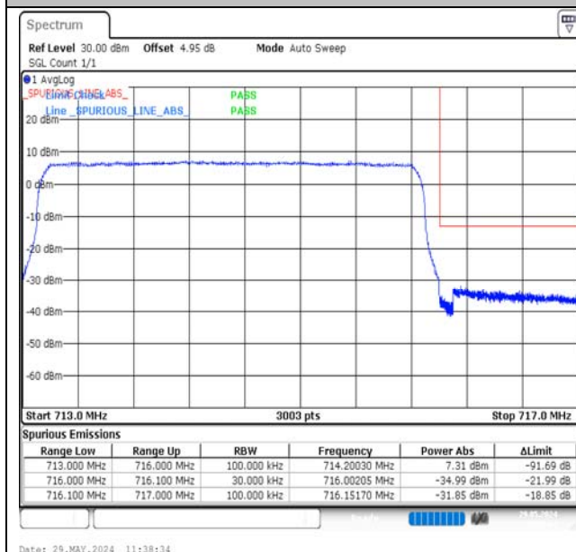
Band12-3MHz-16QAM-23165-15RB#0-PASS
