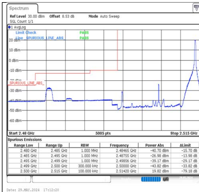
Band7-15MHz-16QAM-20825-1RB#74-PASS
