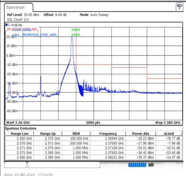
Band7-10MHz-16QAM-21400-1RB#49-PASS
