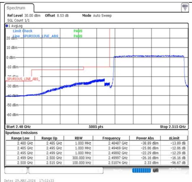
Band7-15MHz-QPSK-20825-75RB#0-PASS
