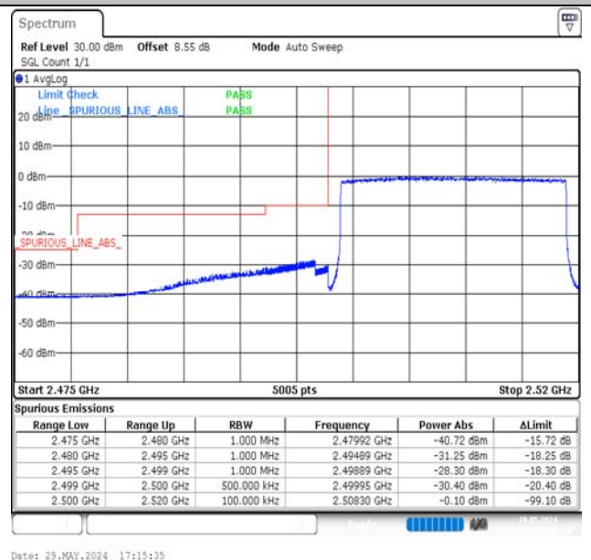
Band7-20MHz-16QAM-20850-100RB#0-PASS
