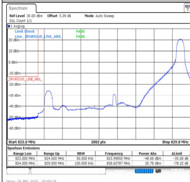
Band5-5MHz-QPSK-20425-1RB#24-PASS
