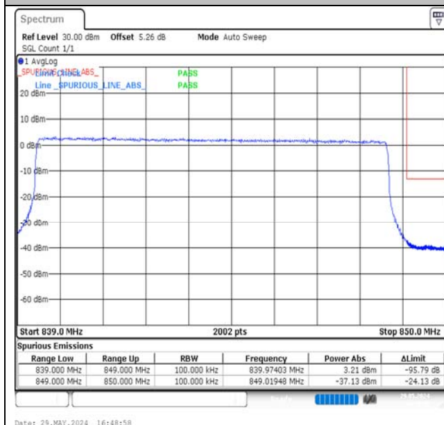
Band5-10MHz-16QAM-20600-50RB#0-PASS
