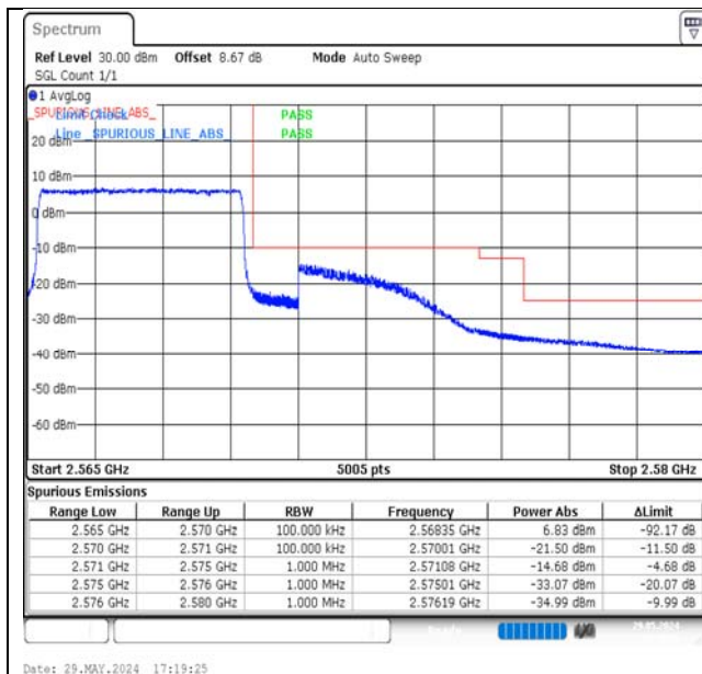
Band7-5MHz-QPSK-21425-25RB#0-PASS
