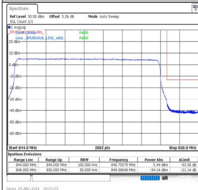
Band5-5MHz-16QAM-20625-25RB#0-PASS
