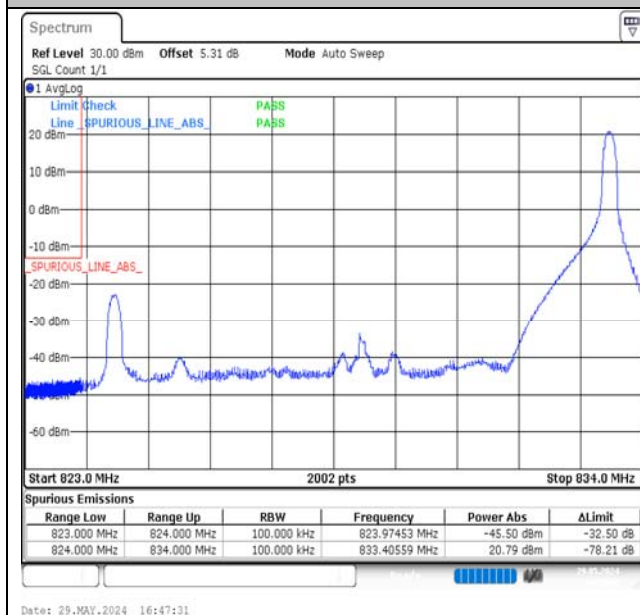
Band5-10MHz-QPSK-20450-1RB#49-PASS
