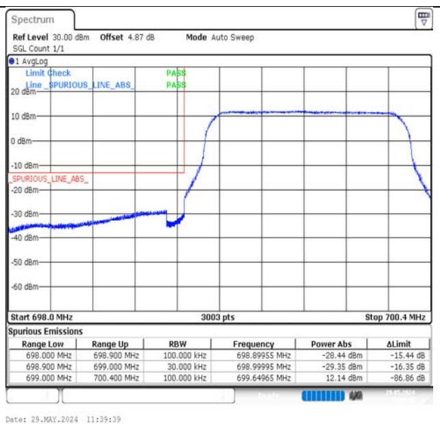
Band12-1.4MHz-QPSK-23017-6RB#0-PASS
