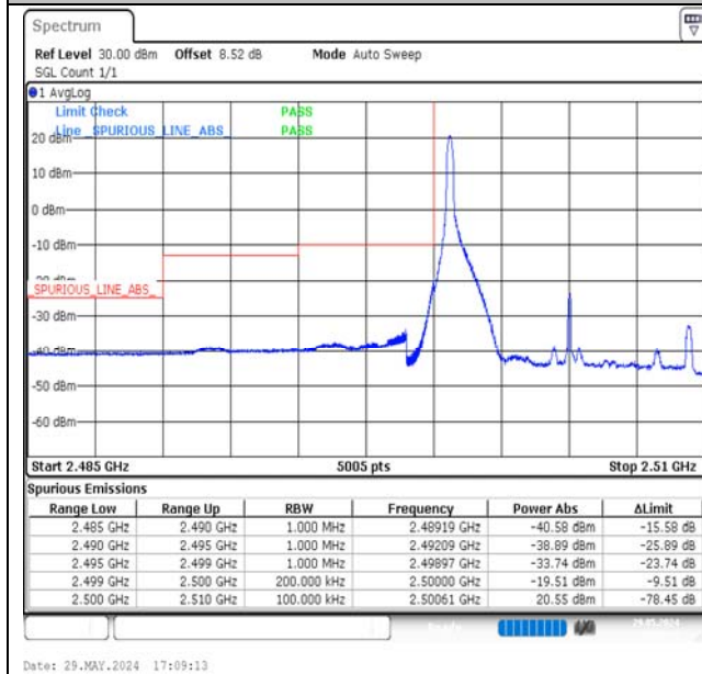
Band7-10MHz-16QAM-20800-1RB#0-PASS
