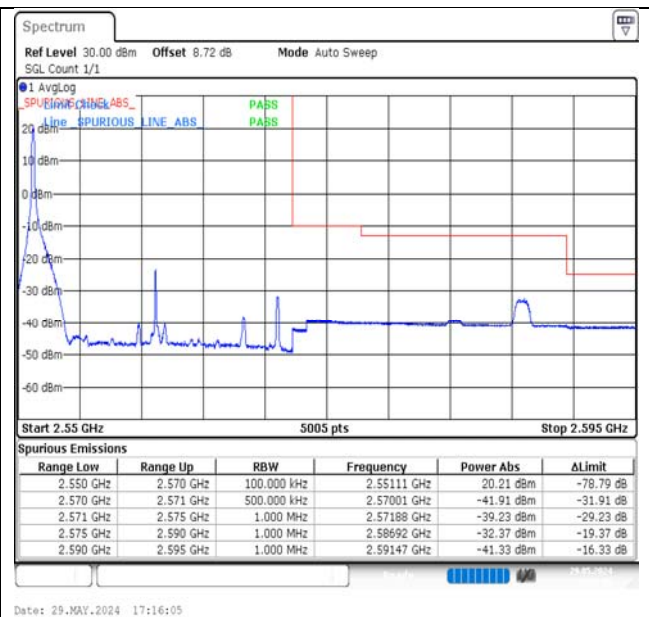
Band7-20MHz-16QAM-21350-1RB#0-PASS
