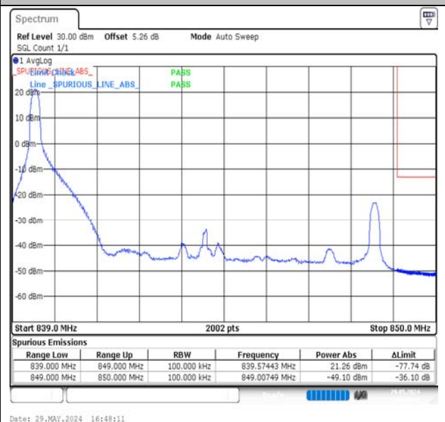
Band5-10MHz-QPSK-20600-1RB#0-PASS
