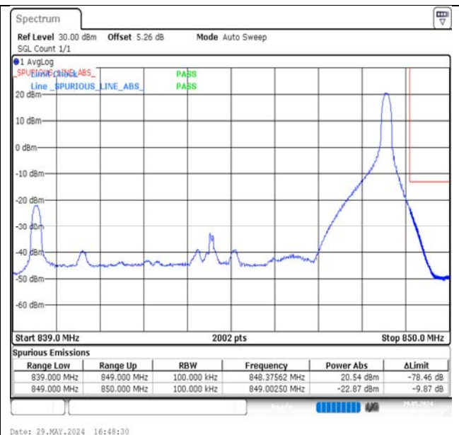
Band5-10MHz-QPSK-20600-1RB#49-PASS
