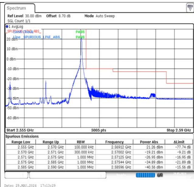
Band7-15MHz-QPSK-21375-1RB#74-PASS
