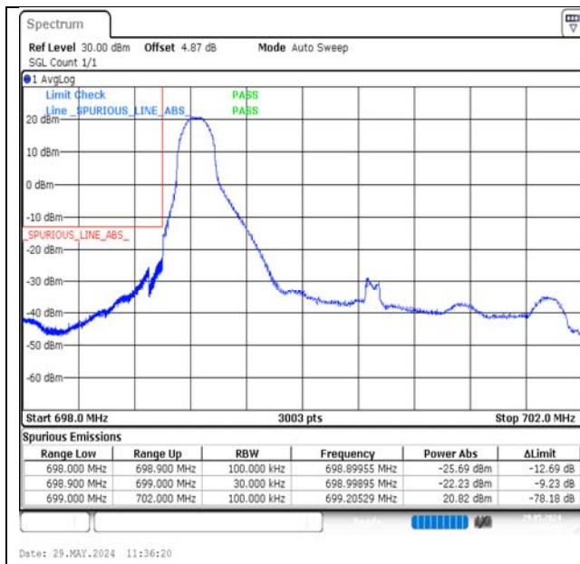
Band12-3MHz-QPSK-23025-1RB#0-PASS
