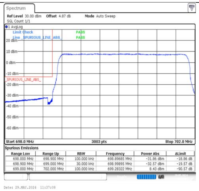
Band12-3MHz-QPSK-23025-15RB#0-PASS
