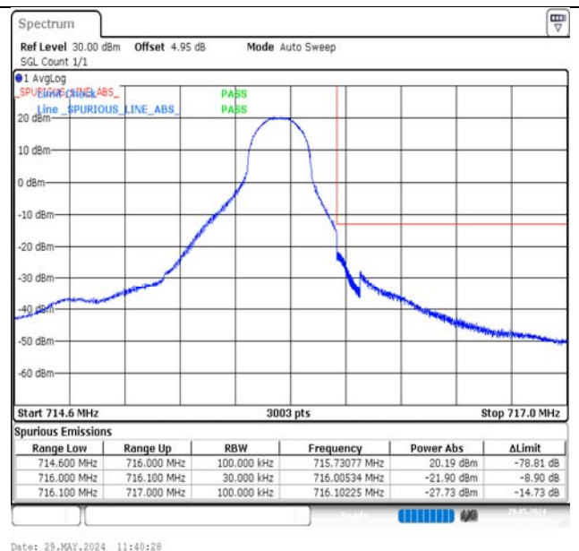
Band12-1.4MHz-QPSK-23173-1RB#5-PASS
