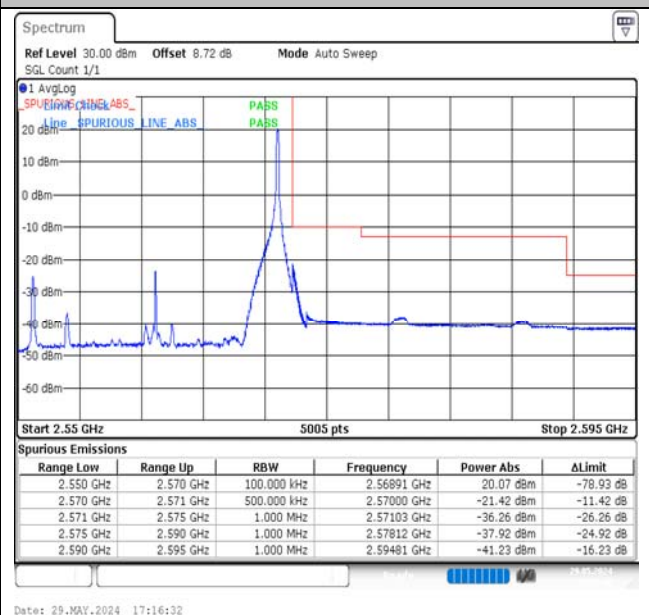
Band7-20MHz-16QAM-21350-1RB#99-PASS
