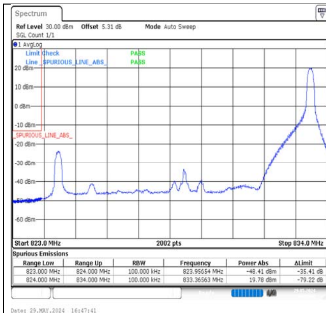
Band5-10MHz-16QAM-20450-1RB#49-PASS
