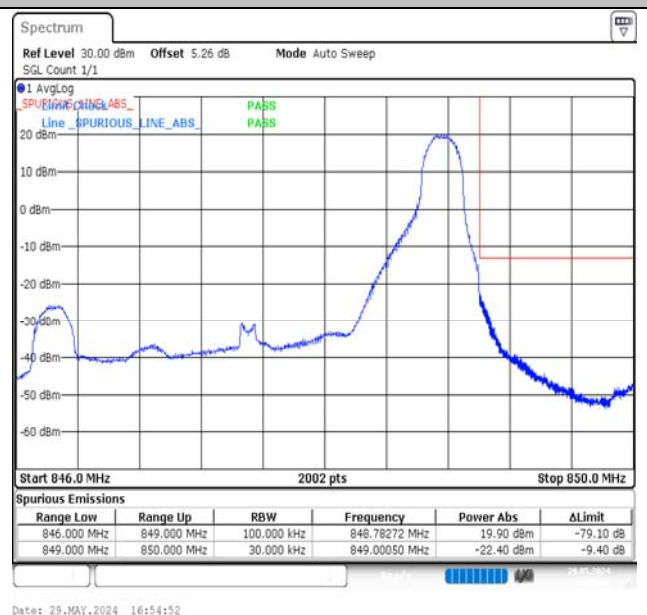
Band5-3MHz-16QAM-20635-1RB#14-PASS
