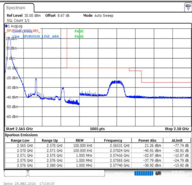
Band7-5MHz-QPSK-21425-1RB#0-PASS
