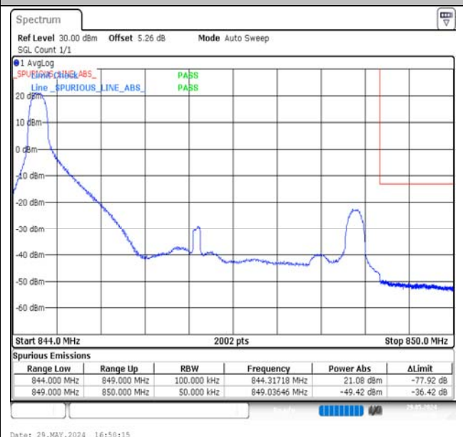
Band5-5MHz-QPSK-20625-1RB#0-PASS
