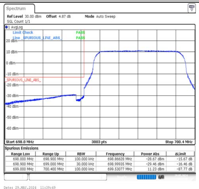
Band12-1.4MHz-16QAM-23017-6RB#0-PASS
