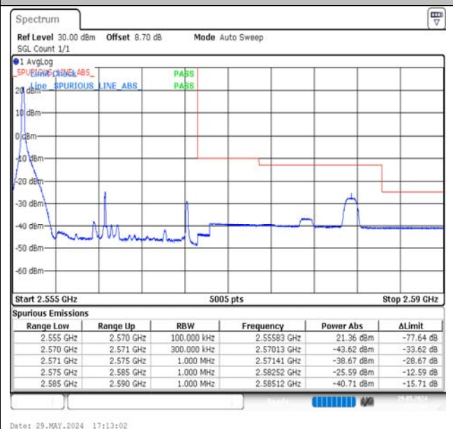
Band7-15MHz-QPSK-21375-1RB#0-PASS
