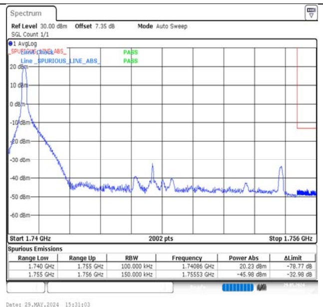
Band4-15MHz-16QAM-20325-1RB#0-PASS
