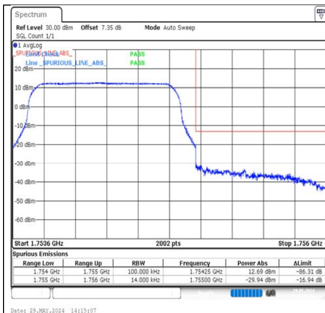
Band4-1.4MHz-QPSK-20393-6RB#0-PASS
