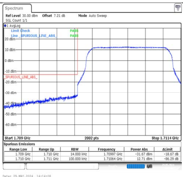
Band4-1.4MHz-QPSK-19957-6RB#0-PASS
