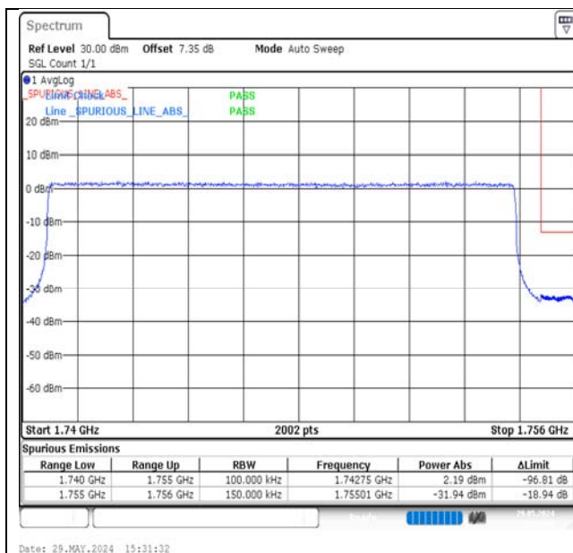
Band4-15MHz-QPSK-20325-75RB#0-PASS
