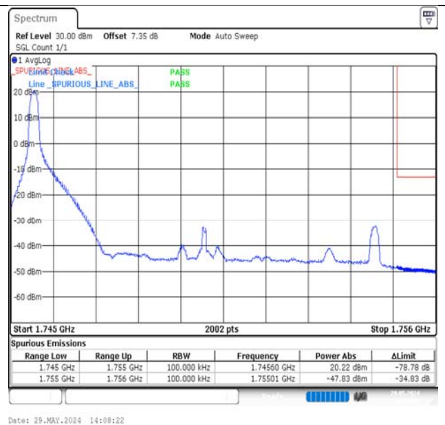
Band4-10MHz-16QAM-20350-1RB#0-PASS
