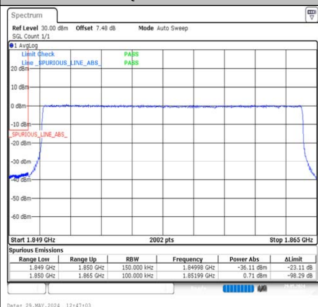
Band2-15MHz-16QAM-18675-75RB#0-PASS
