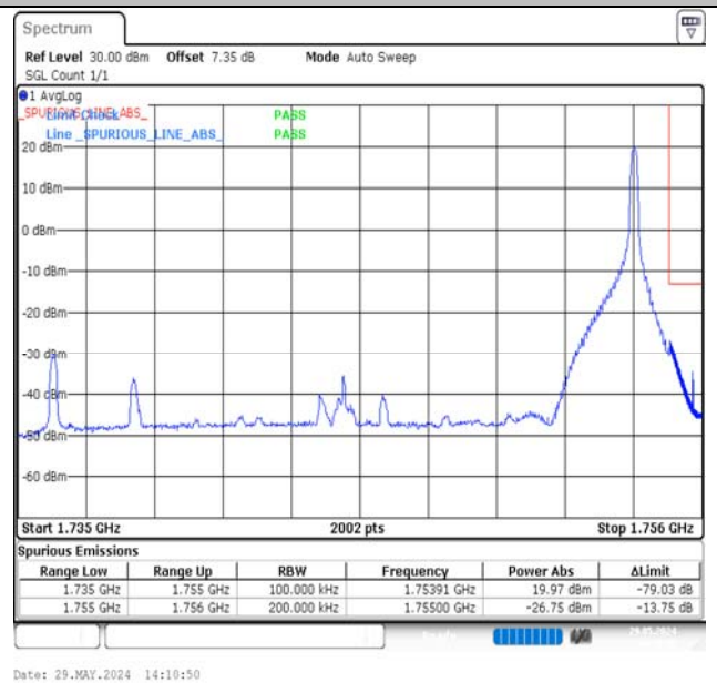
Band4-20MHz-16QAM-20300-1RB#99-PASS
