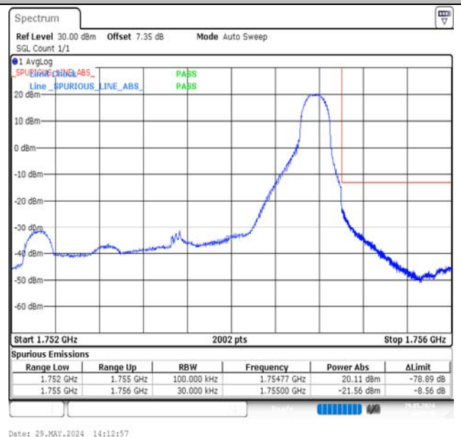
Band4-3MHz-16QAM-20385-1RB#14-PASS
