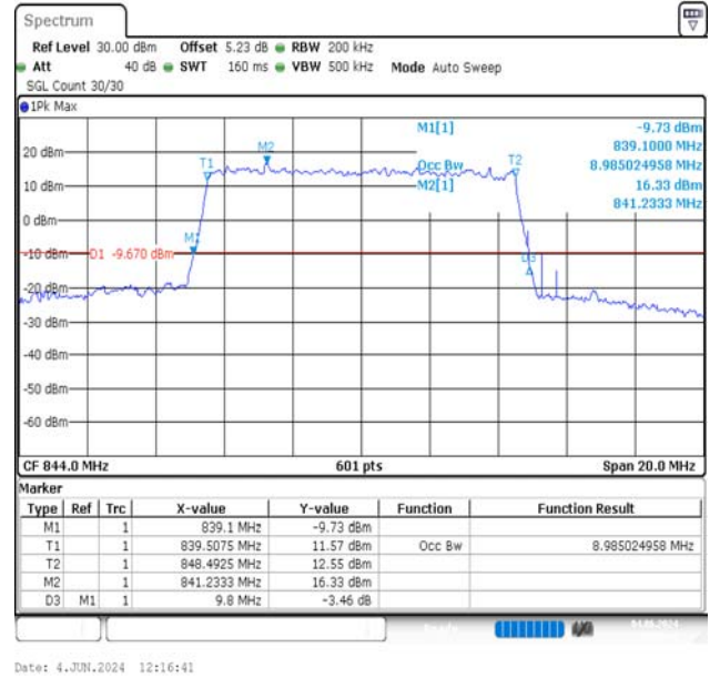
Band5-10MHz-16QAM-20600-50RB#0-PASS
