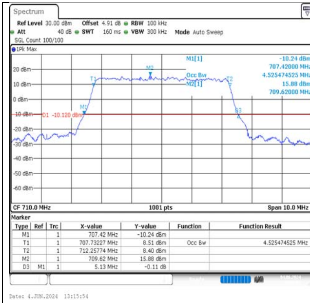
Band17-5MHz-16QAM-23790-25RB#0-PASS
