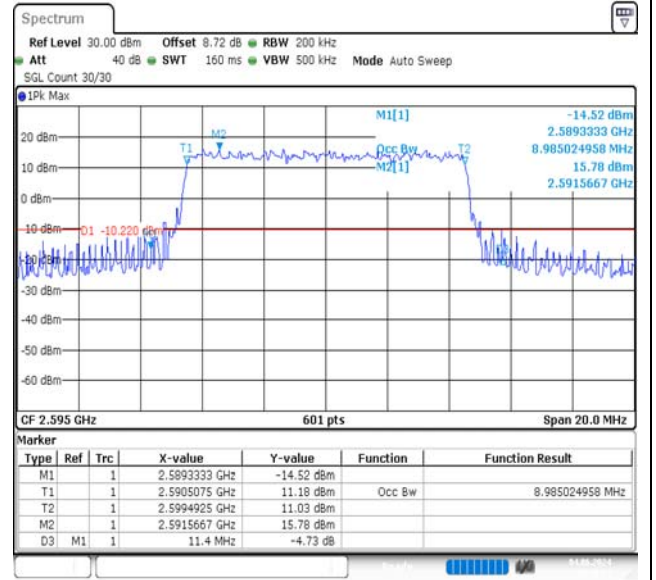
Band38-10MHz-QPSK-38000-50RB#0-PASS
