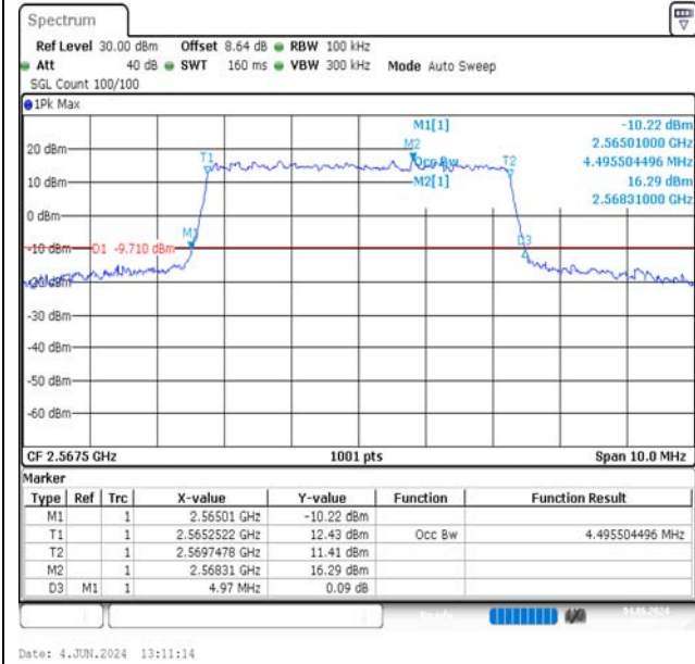
Band7-5MHz-QPSK-21425-25RB#0-PASS
