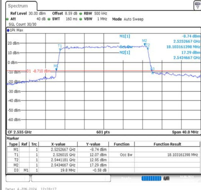
Band7-20MHz-16QAM-21100-100RB#0-PASS
