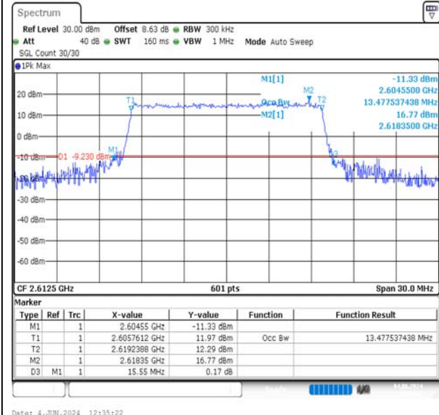
Band38-15MHz-QPSK-38175-75RB#0-PASS
