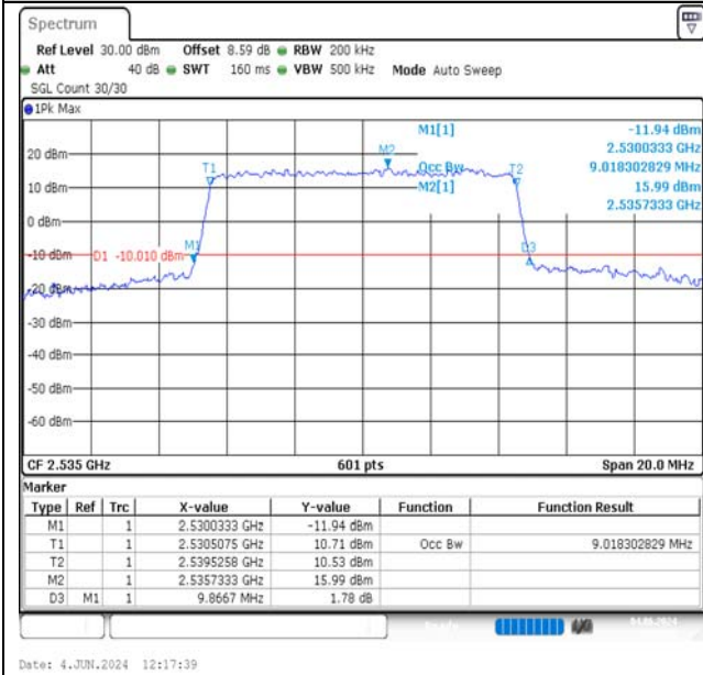
Band7-10MHz-16QAM-21100-50RB#0-PASS
