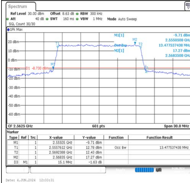
Band7-15MHz-QPSK-21375-75RB#0-PASS
