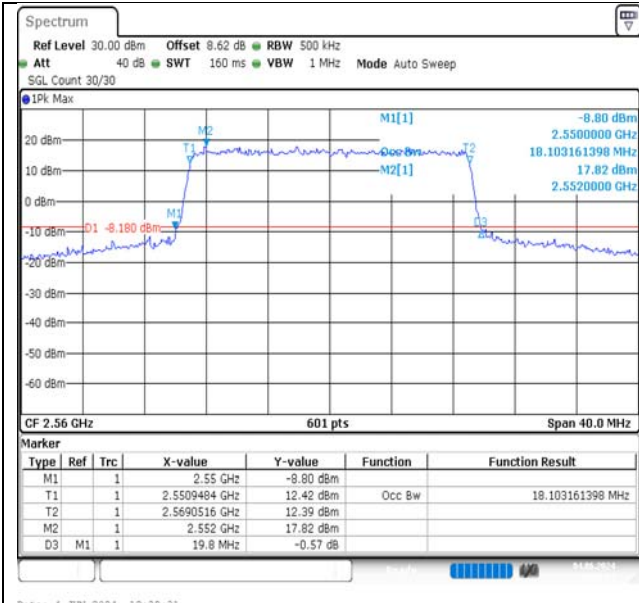
Band7-20MHz-QPSK-21350-100RB#0-PASS
