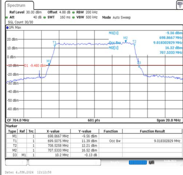
Band12-10MHz-QPSK-23060-50RB#0-PASS
