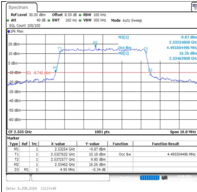
Band7-5MHz-16QAM-21100-25RB#0-PASS
