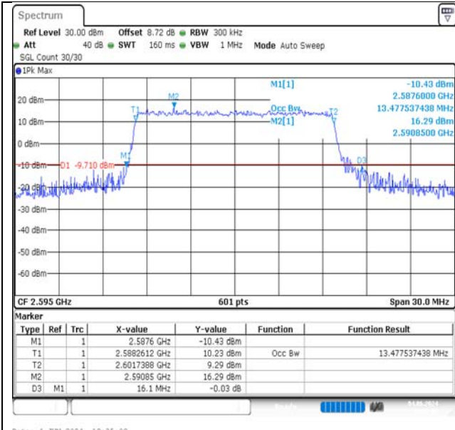
Band38-15MHz-16QAM-38000-75RB#0-PASS
