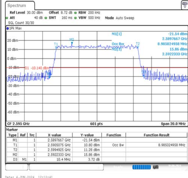
Band38-10MHz-16QAM-38000-50RB#0-PASS
