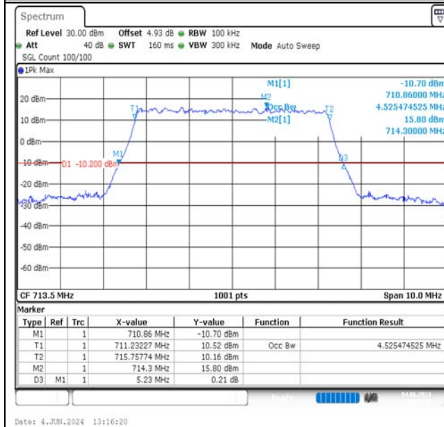
Band17-5MHz-QPSK-23825-25RB#0-PASS
