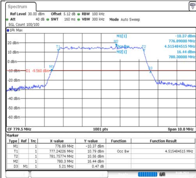
Band13-5MHz-QPSK-23205-25RB#0-PASS
