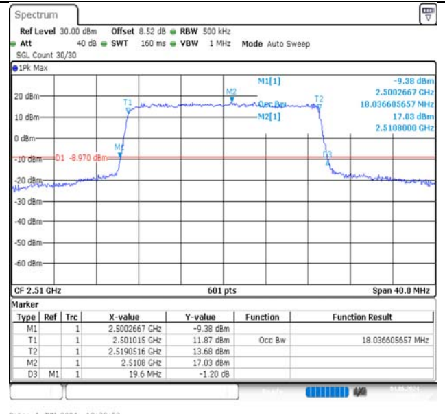
Band7-20MHz-16QAM-20850-100RB#0-PASS
