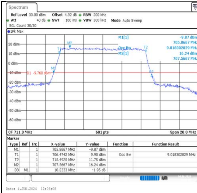
Band17-10MHz-QPSK-23800-50RB#0-PASS
