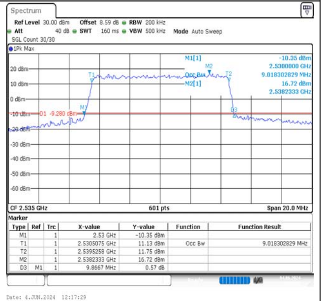
Band7-10MHz-QPSK-21100-50RB#0-PASS
