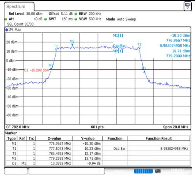
Band13-10MHz-16QAM-23230-50RB#0-PASS
