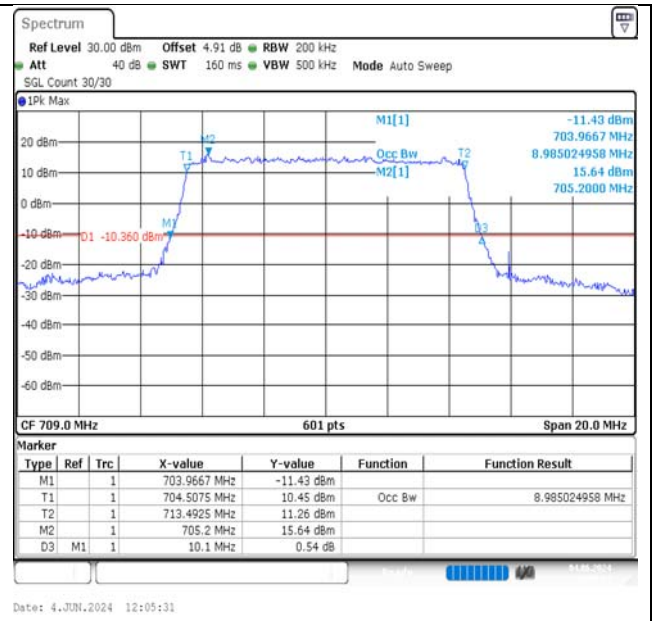
Band17-10MHz-16QAM-23780-50RB#0-PASS
