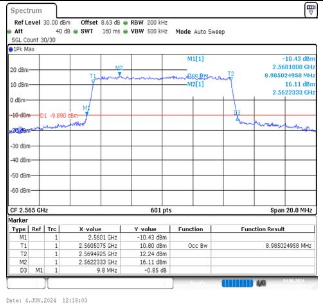
Band7-10MHz-16QAM-21400-50RB#0-PASS
