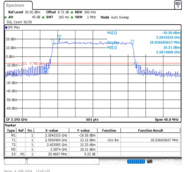
Band38-20MHz-QPSK-38000-100RB#0-PASS
