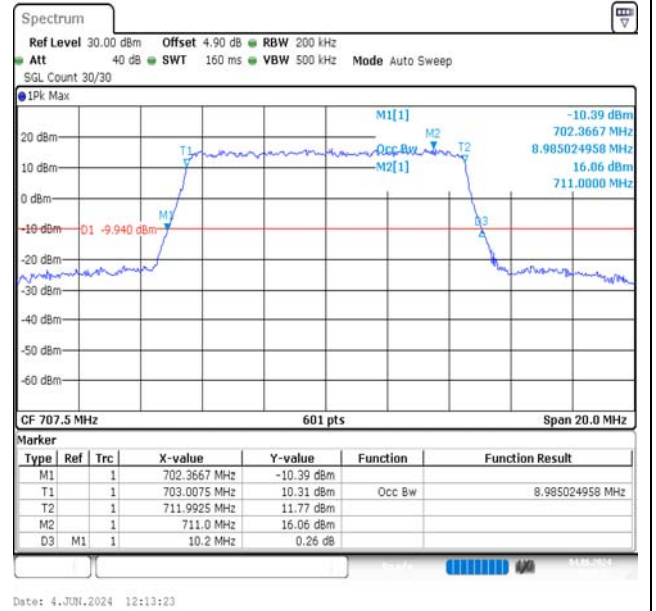
Band12-10MHz-QPSK-23095-50RB#0-PASS
