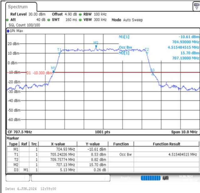
Band12-5MHz-16QAM-23095-25RB#0-PASS
