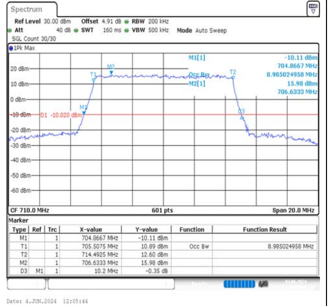
Band17-10MHz-QPSK-23790-50RB#0-PASS
