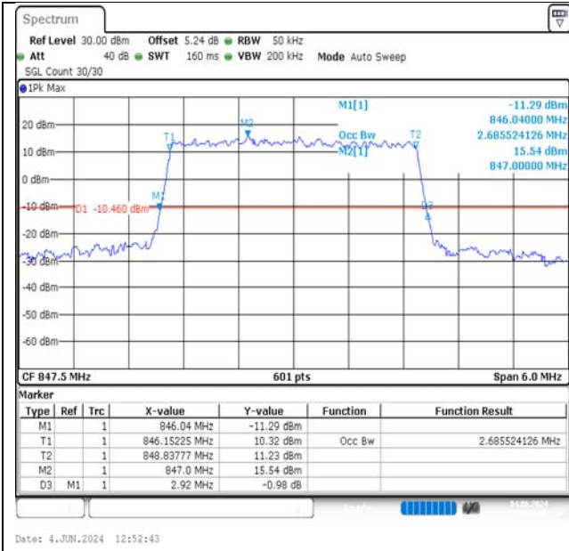
Band5-3MHz-QPSK-20635-15RB#0-PASS
