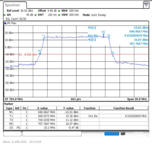
Band12-10MHz-16QAM-23060-50RB#0-PASS
