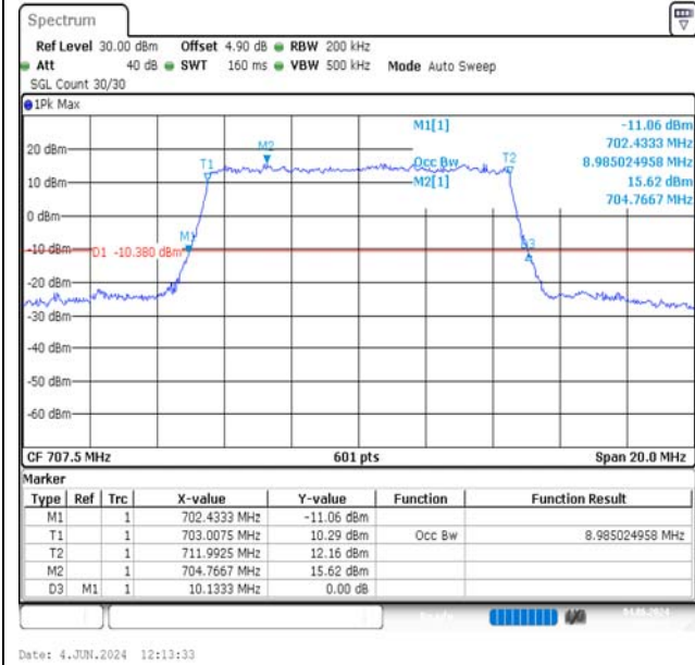
Band12-10MHz-16QAM-23095-50RB#0-PASS
