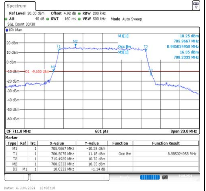
Band17-10MHz-16QAM-23800-50RB#0-PASS
