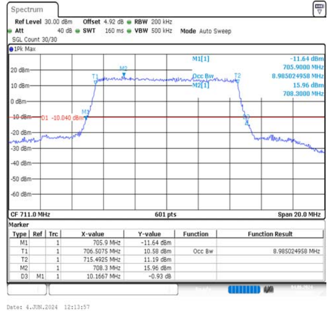
Band12-10MHz-16QAM-23130-50RB#0-PASS
