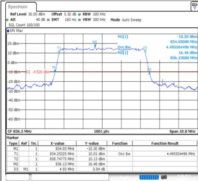
Band5-5MHz-16QAM-20525-25RB#0-PASS
