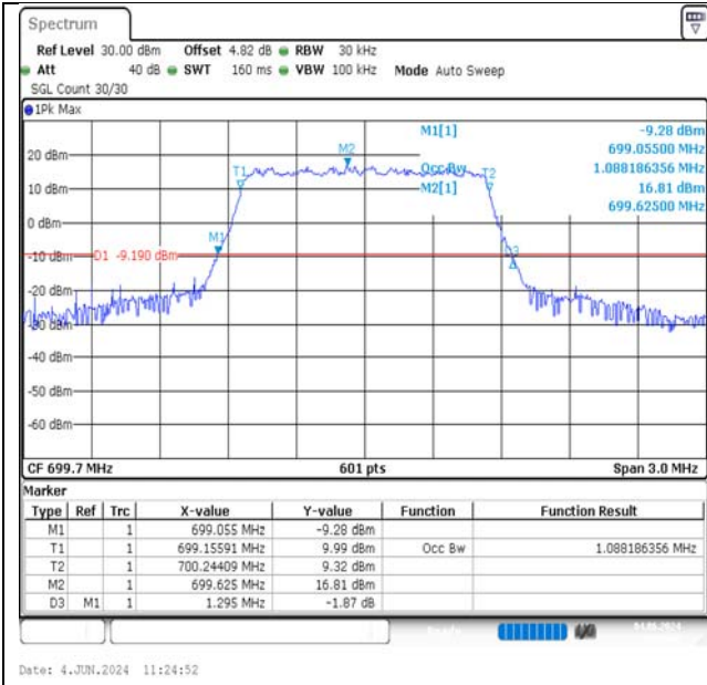
Band12-1.4MHz-QPSK-23017-6RB#0-PASS
