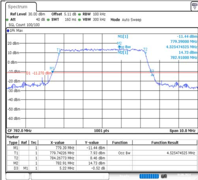
Band13-5MHz-16QAM-23230-25RB#0-PASS
