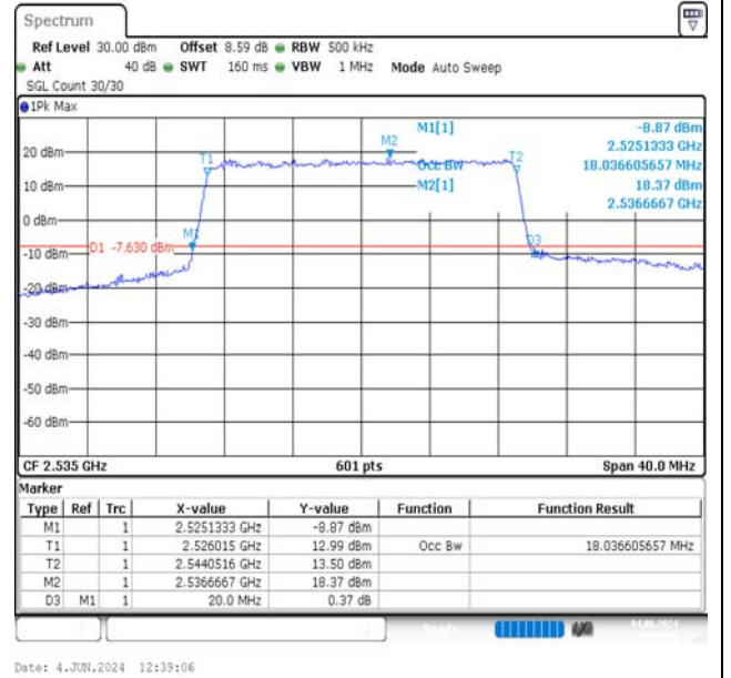
Band7-20MHz-QPSK-21100-100RB#0-PASS
