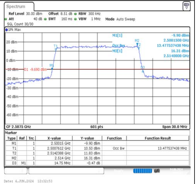
Band7-15MHz-16QAM-20825-75RB#0-PASS
