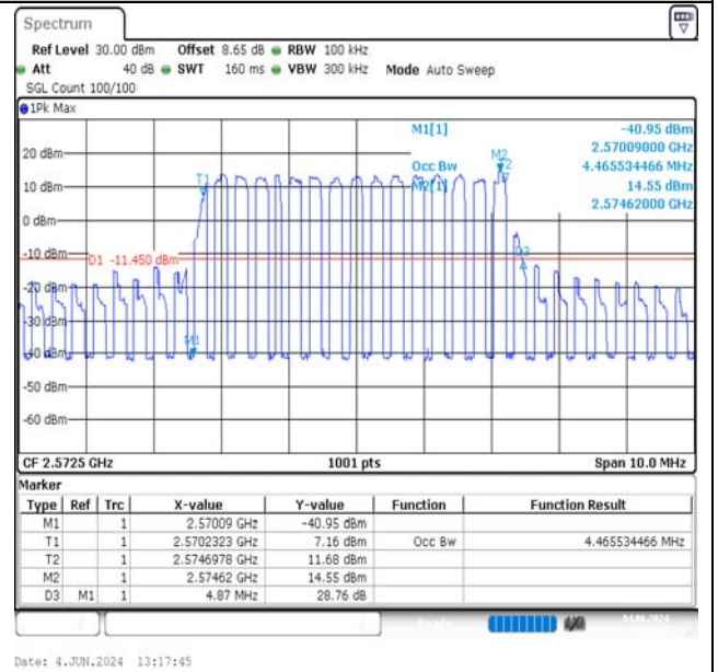
Band38-5MHz-16QAM-37775-25RB#0-PASS
