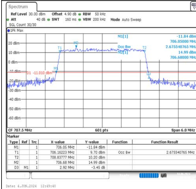
Band12-3MHz-16QAM-23095-15RB#0-PASS
