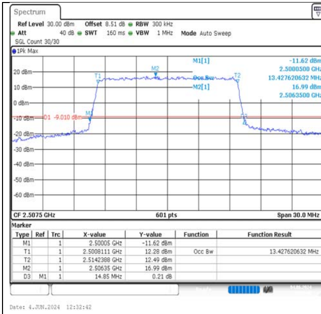
Band7-15MHz-QPSK-20825-75RB#0-PASS
