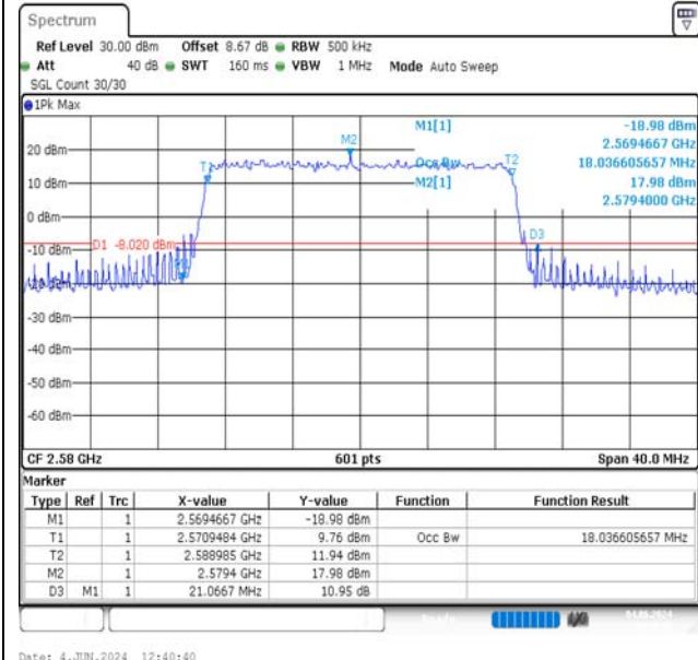
Band38-20MHz-QPSK-37850-100RB#0-PASS
