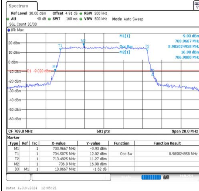
Band17-10MHz-QPSK-23780-50RB#0-PASS
