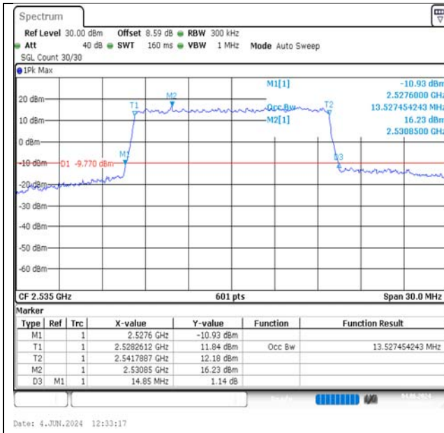
Band7-15MHz-16QAM-21100-75RB#0-PASS
