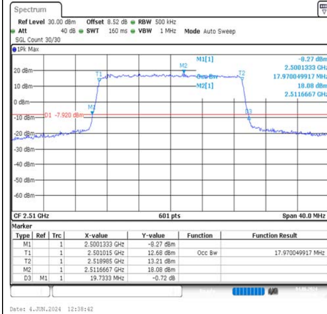
Band7-20MHz-QPSK-20850-100RB#0-PASS
