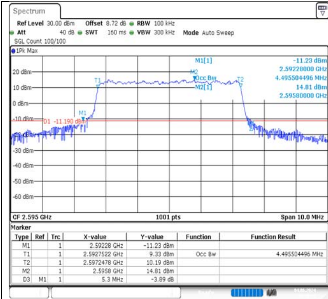
Band38-5MHz-16QAM-38000-25RB#0-PASS
