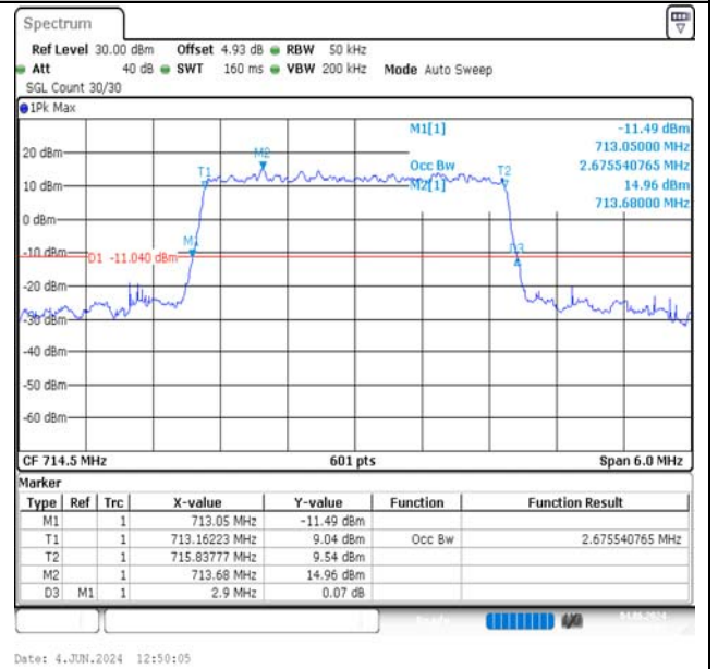
Band12-3MHz-16QAM-23165-15RB#0-PASS
