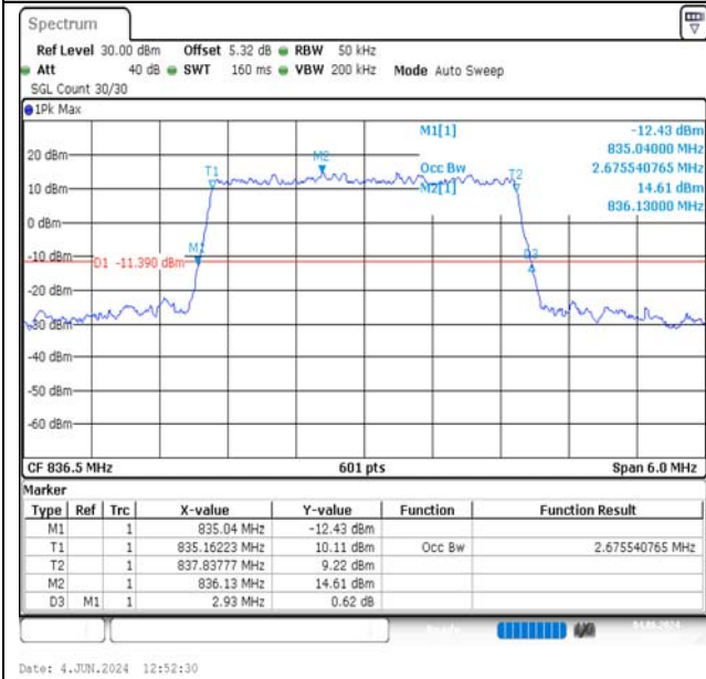
Band5-3MHz-16QAM-20525-15RB#0-PASS
