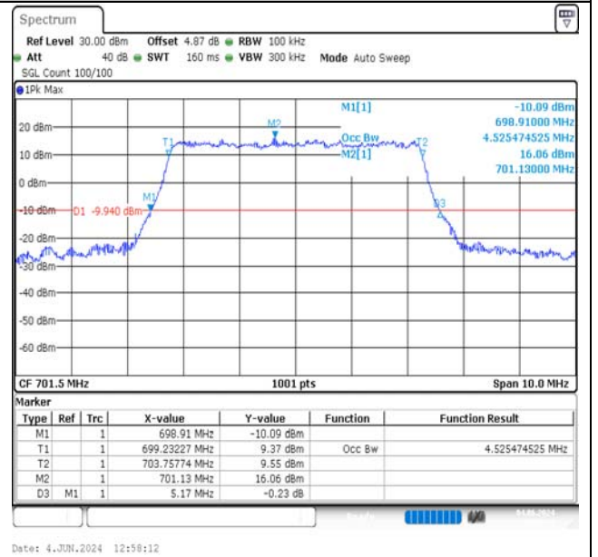
Band12-5MHz-16QAM-23035-25RB#0-PASS
