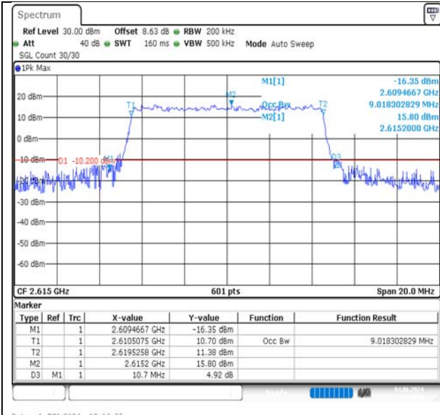
Band38-10MHz-QPSK-38200-50RB#0-PASS
