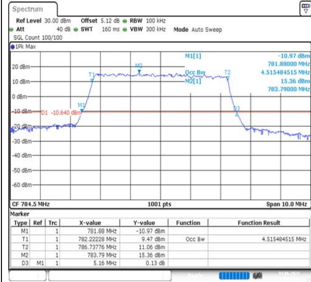
Band13-5MHz-QPSK-23205-25RB#0-PASS
