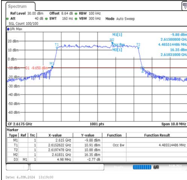
Band38-5MHz-QPSK-38225-25RB#0-PASS
