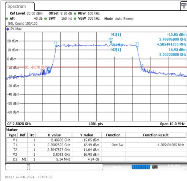
Band7-5MHz-QPSK-20775-25RB#0-PASS
