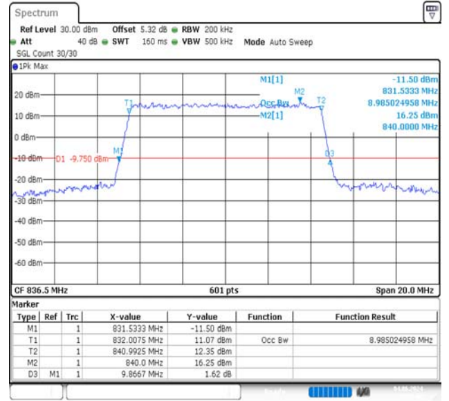
Band5-10MHz-QPSK-20525-50RB#0-PASS
