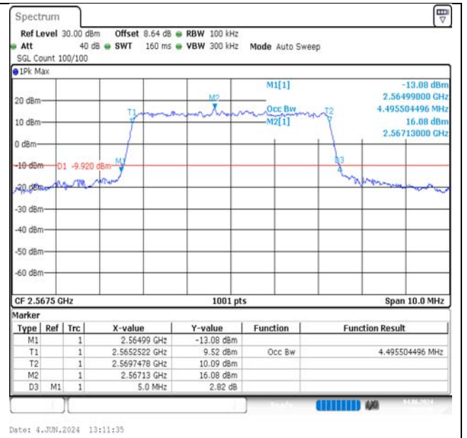
Band7-5MHz-16QAM-21425-25RB#0-PASS
