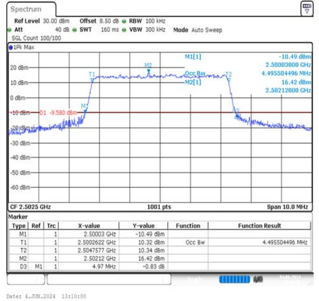
Band7-5MHz-16QAM-20775-25RB#0-PASS
