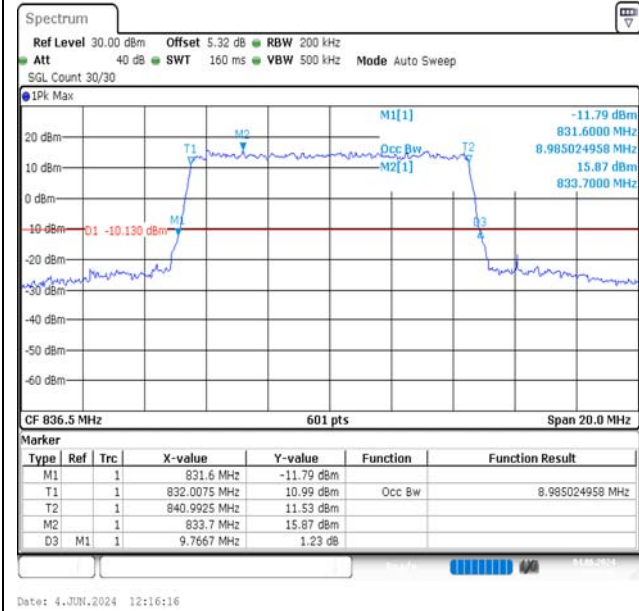
Band5-10MHz-16QAM-20525-50RB#0-PASS
