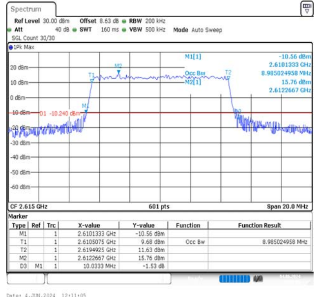
Band38-10MHz-16QAM-38200-50RB#0-PASS
