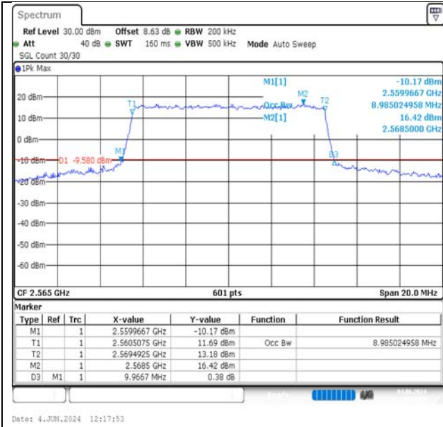
Band7-10MHz-QPSK-21400-50RB#0-PASS
