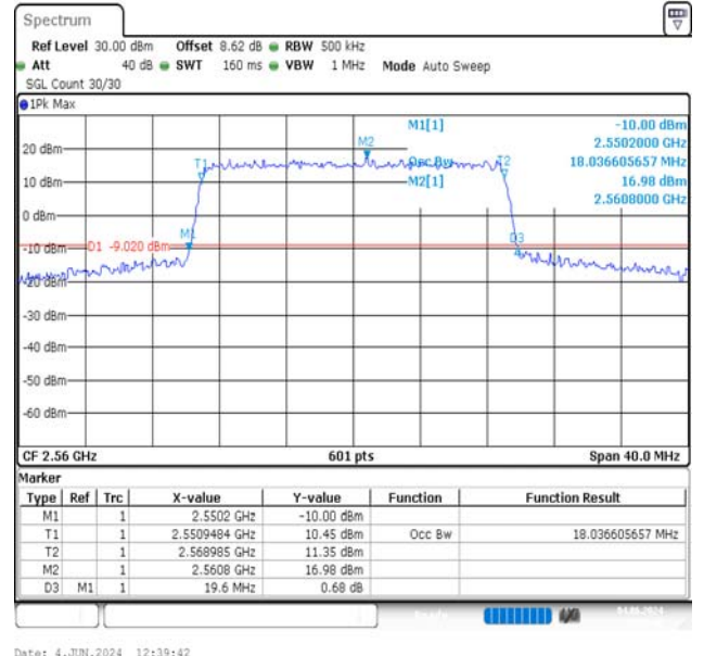
Band7-20MHz-16QAM-21350-100RB#0-PASS
