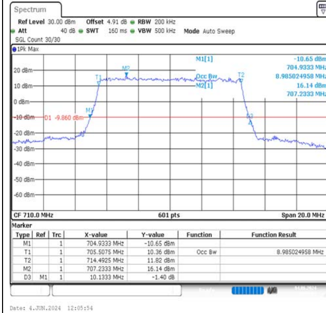
Band17-10MHz-16QAM-23790-50RB#0-PASS
