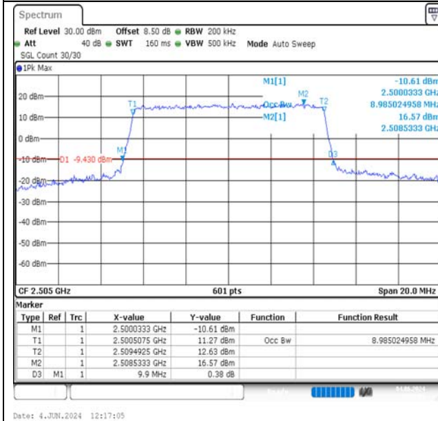
Band7-10MHz-QPSK-20800-50RB#0-PASS
