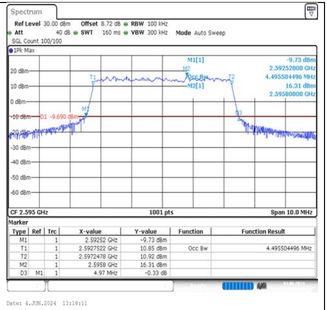
Band38-5MHz-QPSK-38000-25RB#0-PASS
