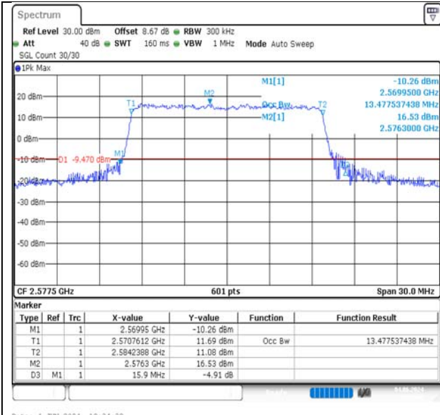
Band38-15MHz-QPSK-37825-75RB#0-PASS
