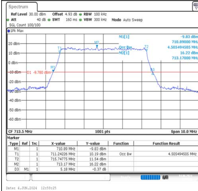
Band12-5MHz-QPSK-23155-25RB#0-PASS
