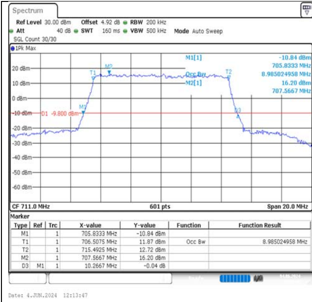
Band12-10MHz-QPSK-23130-50RB#0-PASS
