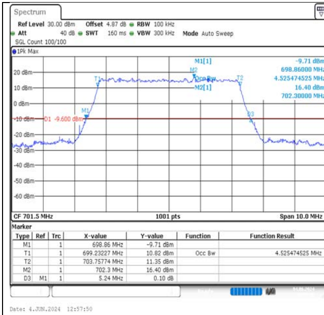
Band12-5MHz-QPSK-23035-25RB#0-PASS
