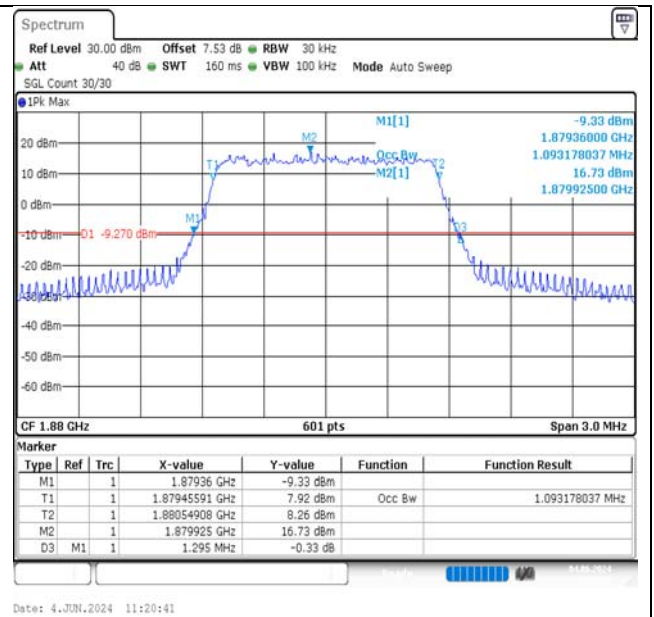
Band2-1.4MHz-QPSK-18900-6RB#0-PASS
