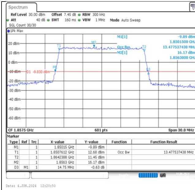
Band2-15MHz-QPSK-18675-75RB#0-PASS
