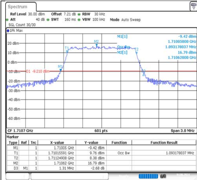
Band4-1.4MHz-QPSK-19957-6RB#0-PASS
