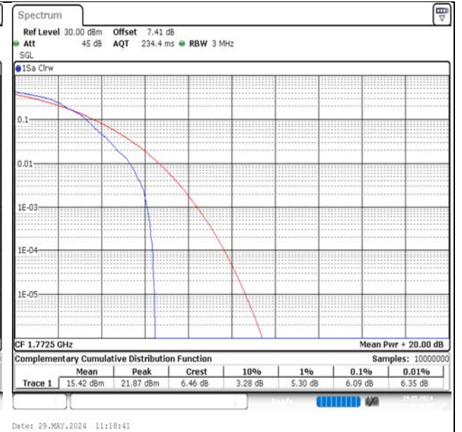
Band66-15MHz-QPSK-132597-75RB#0-PASS
