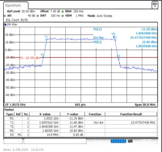
Band2-15MHz-16QAM-18675-75RB#0-PASS
