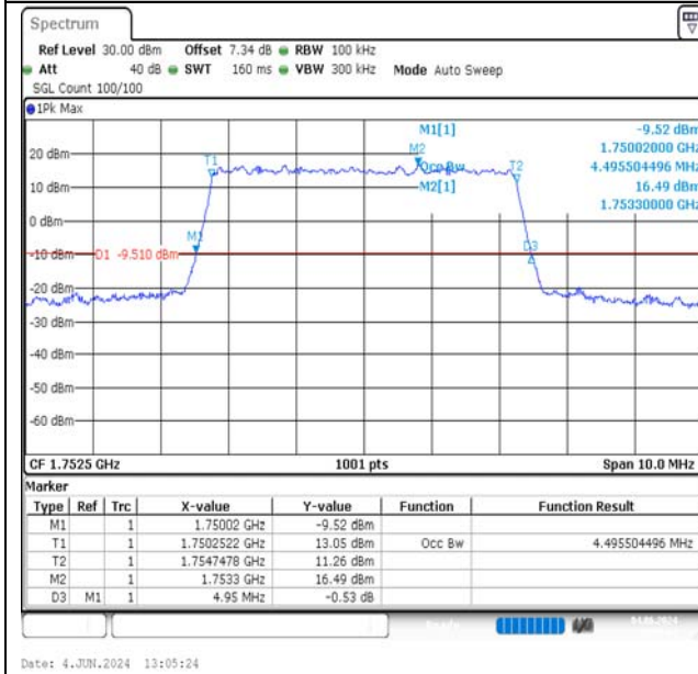
Band4-5MHz-QPSK-20375-25RB#0-PASS
