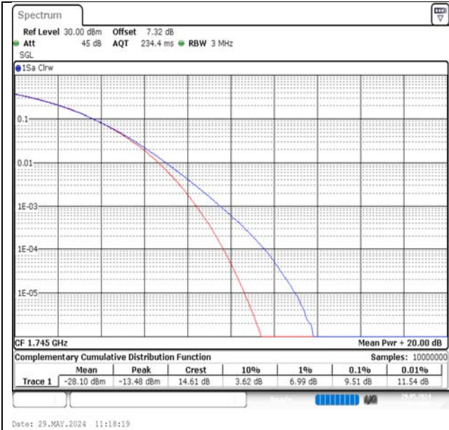
Band66-15MHz-16QAM-132322-1RB#0-PASS
