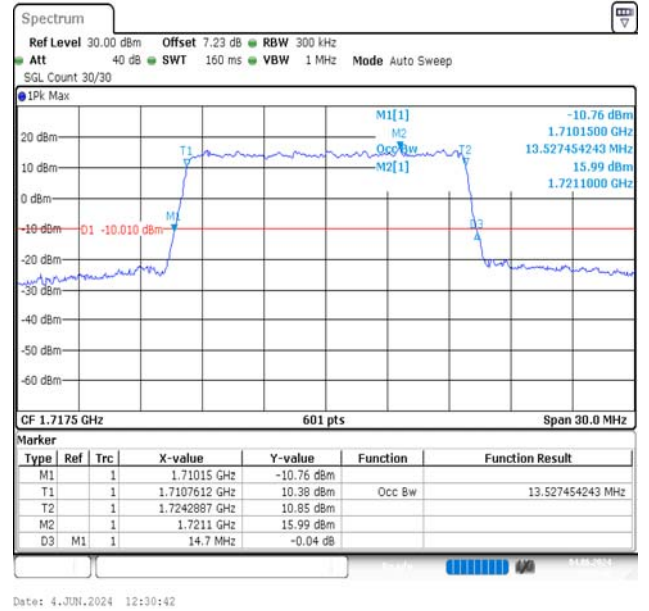
Band4-15MHz-16QAM-20025-75RB#0-PASS
