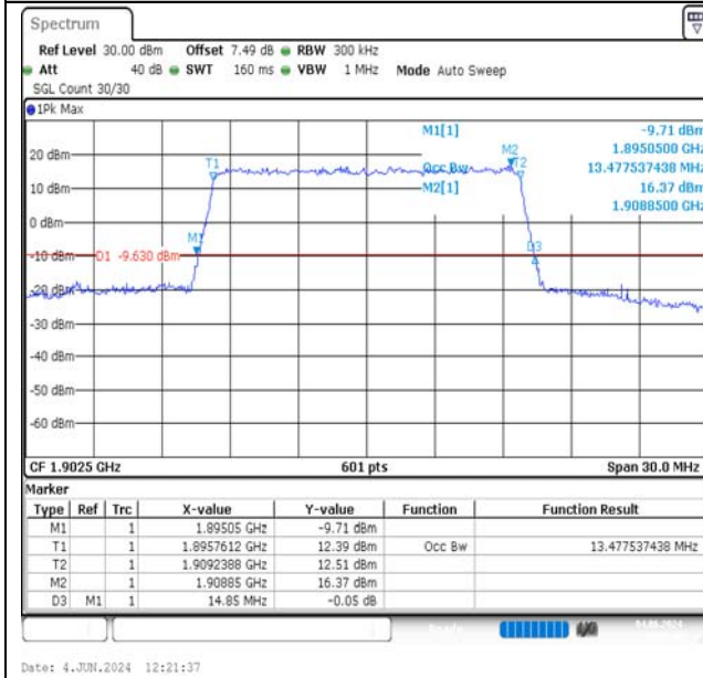
Band2-15MHz-QPSK-19125-75RB#0-PASS
