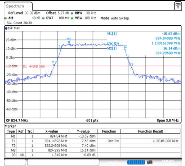
Band5-1.4MHz-16QAM-20407-6RB#0-PASS
