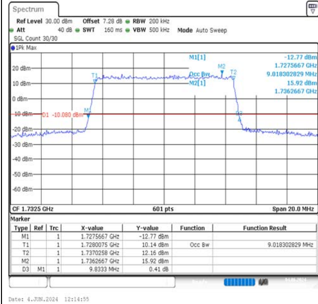
Band4-10MHz-16QAM-20175-50RB#0-PASS
