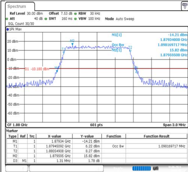
Band2-1.4MHz-16QAM-18900-6RB#0-PASS
