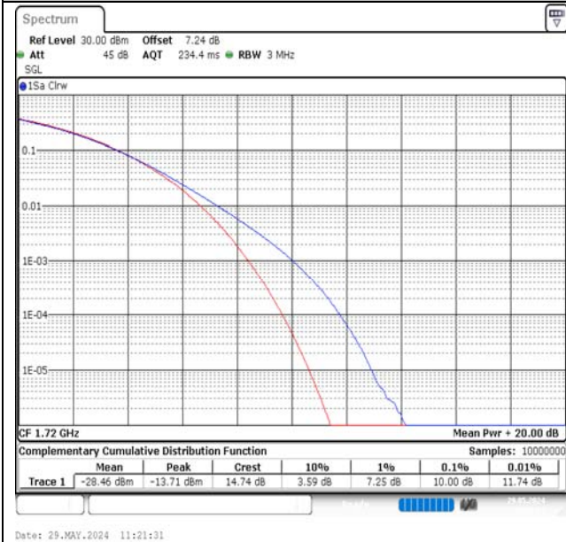
Band66-20MHz-16QAM-132072-1RB#0-PASS
