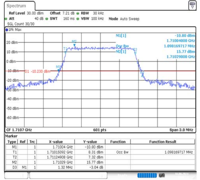
Band4-1.4MHz-16QAM-19957-6RB#0-PASS
