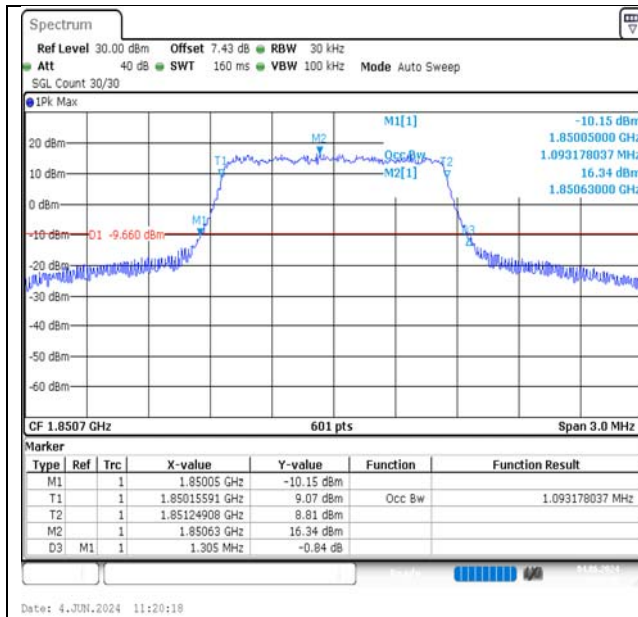
Band2-1.4MHz-QPSK-18607-6RB#0-PASS
