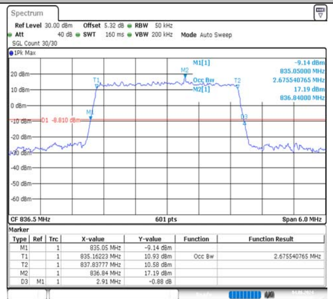
Band5-3MHz-QPSK-20525-15RB#0-PASS
