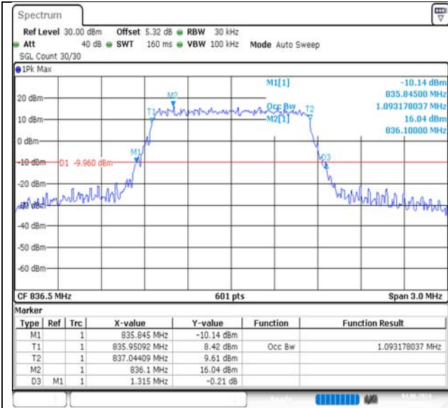
Band5-1.4MHz-16QAM-20525-6RB#0-PASS
