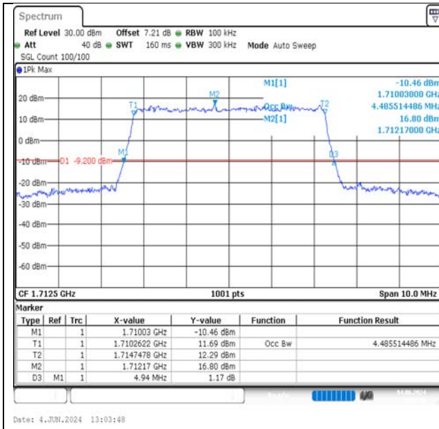
Band4-5MHz-QPSK-19975-25RB#0-PASS
