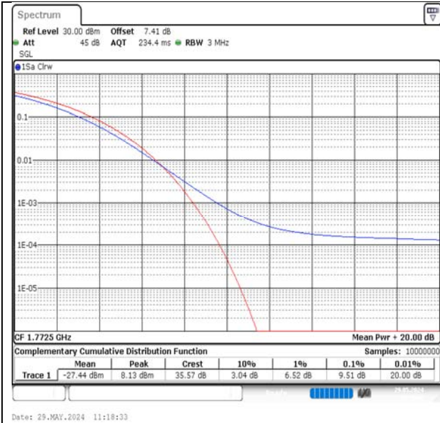
Band66-15MHz-QPSK-132597-1RB#0-PASS
