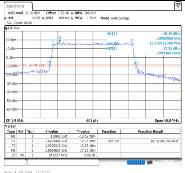
Band2-20MHz-16QAM-19100-100RB#0-PASS
