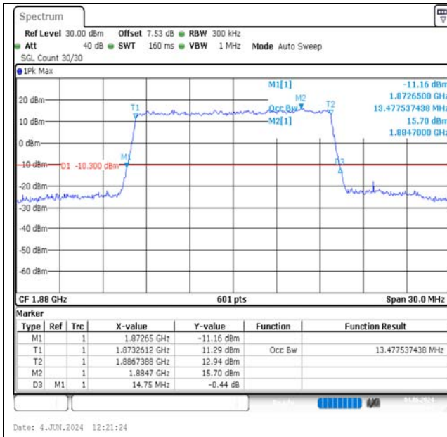
Band2-15MHz-16QAM-18900-75RB#0-PASS
