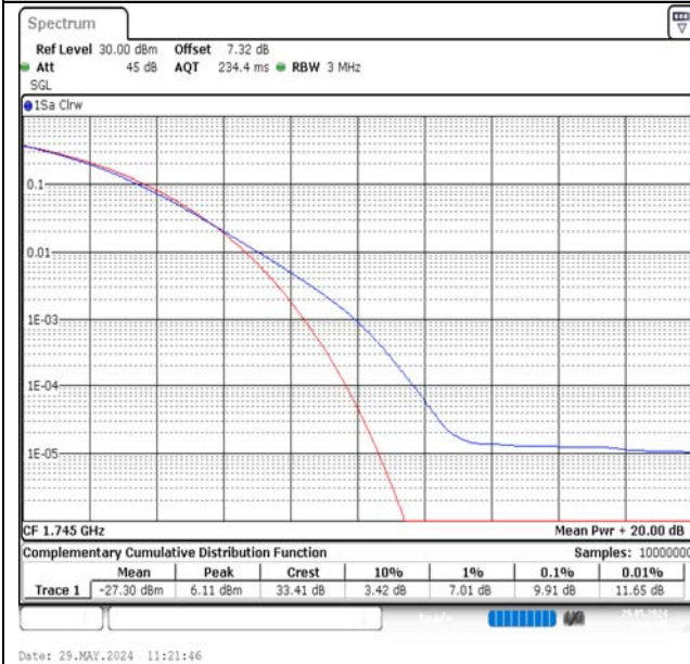
Band66-20MHz-QPSK-132322-1RB#0-PASS
