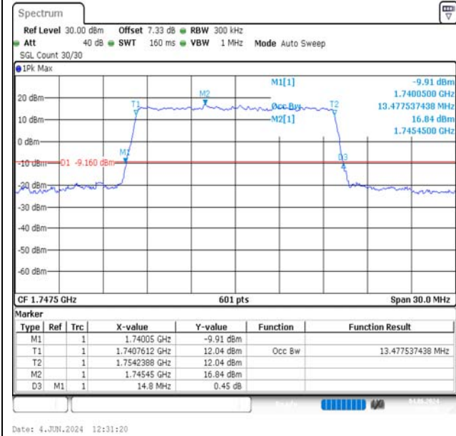
Band4-15MHz-QPSK-20325-75RB#0-PASS
