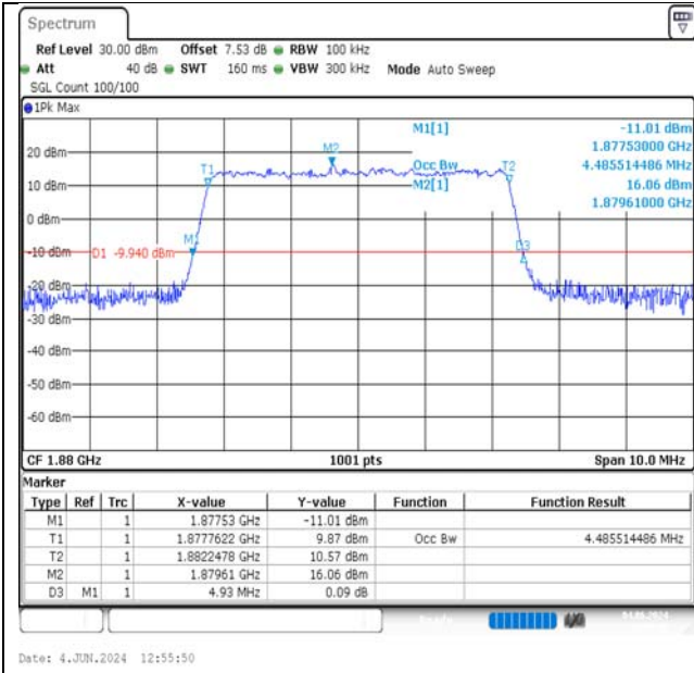
Band2-5MHz-16QAM-18900-25RB#0-PASS
