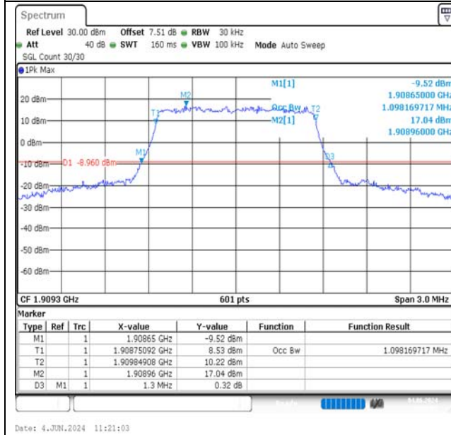
Band2-1.4MHz-QPSK-19193-6RB#0-PASS
