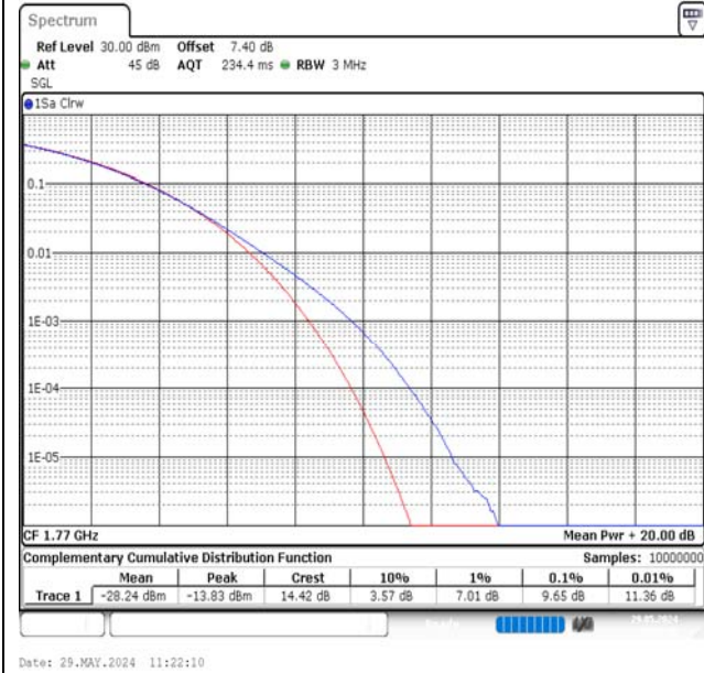
Band66-20MHz-16QAM-132572-1RB#0-PASS
