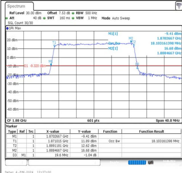
Band2-20MHz-16QAM-18900-100RB#0-PASS
