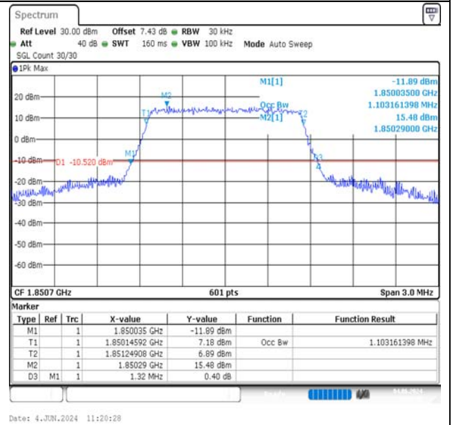
Band2-1.4MHz-16QAM-18607-6RB#0-PASS
