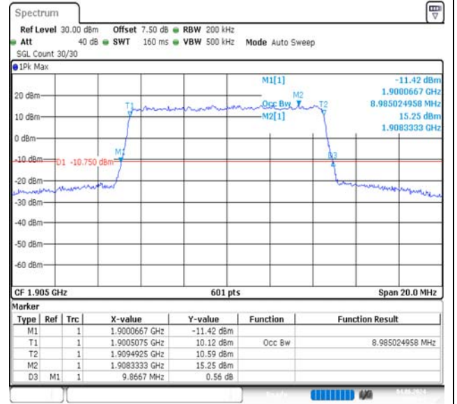
Band2-10MHz-16QAM-19150-50RB#0-PASS
