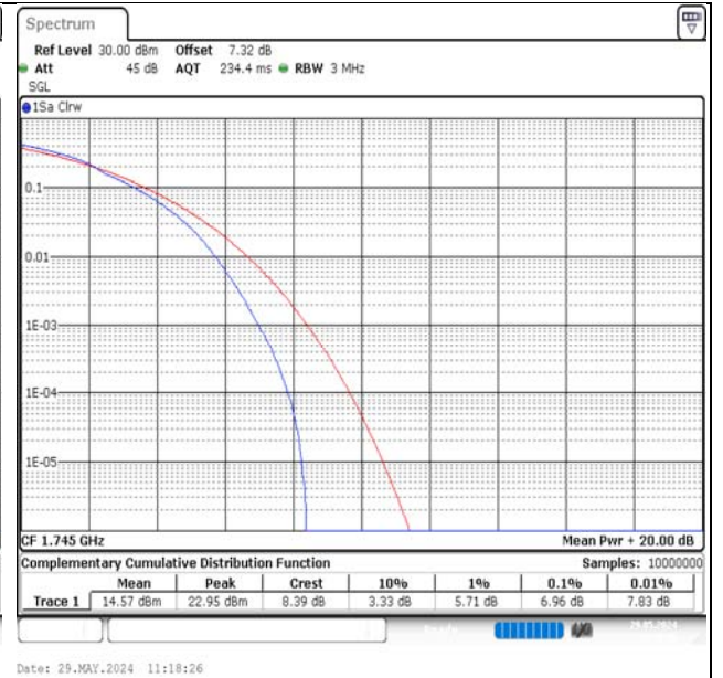
Band66-15MHz-16QAM-132322-75RB#0-PASS
