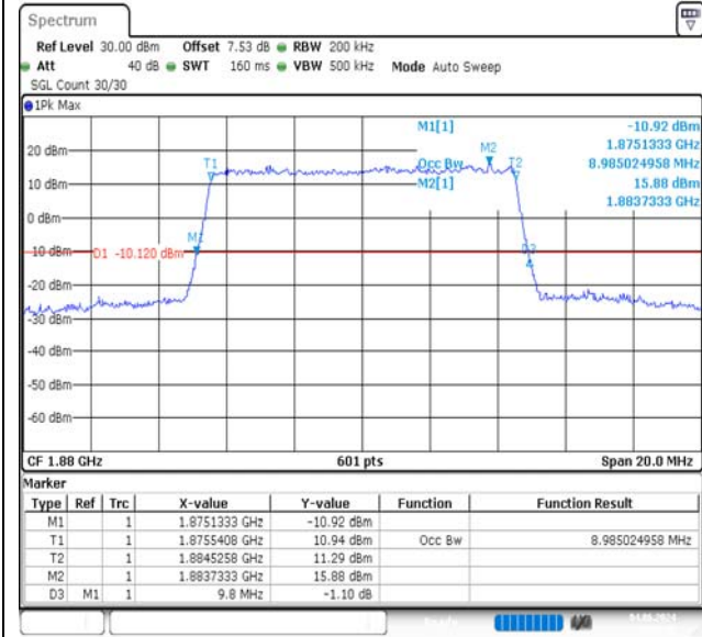
Band2-10MHz-QPSK-19150-50RB#0-PASS
