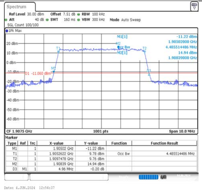
Band2-5MHz-16QAM-19175-25RB#0-PASS
