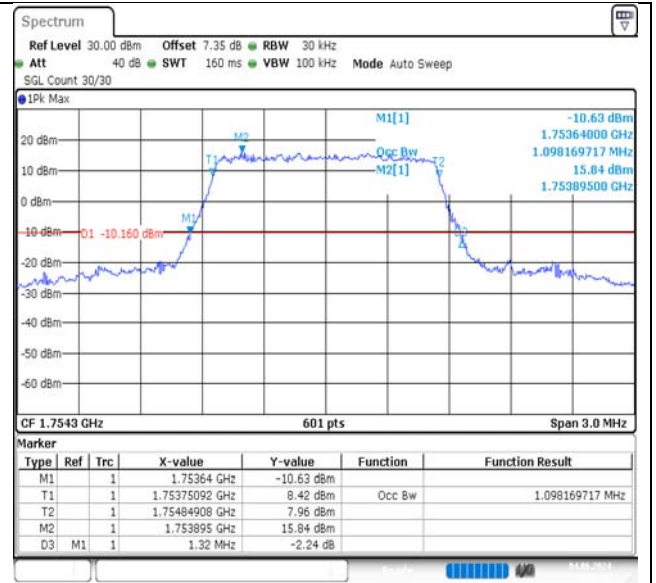
Band4-1.4MHz-16QAM-20393-6RB#0-PASS
