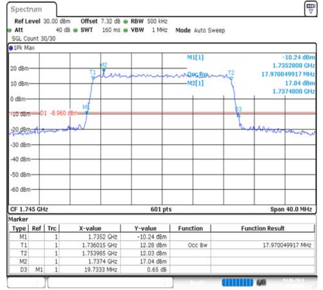
Band4-20MHz-16QAM-20300-100RB#0-PASS
