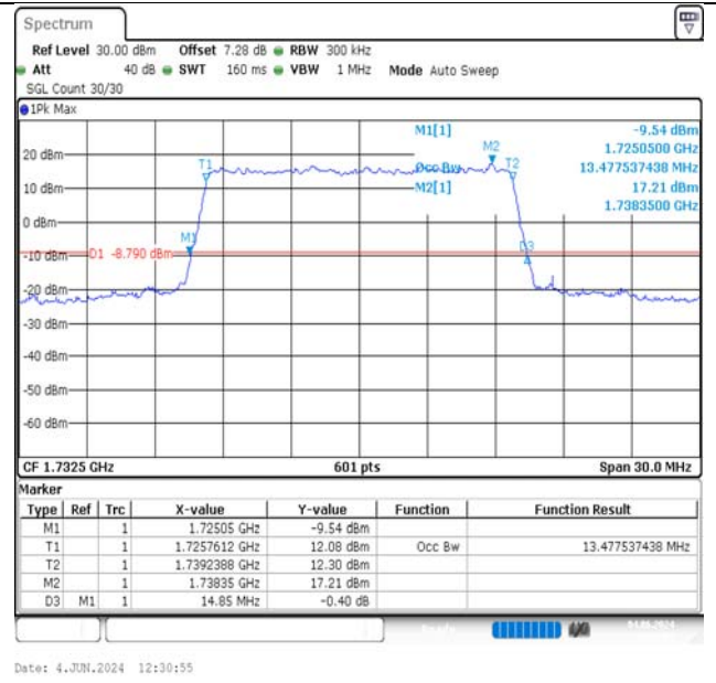
Band4-15MHz-QPSK-20175-75RB#0-PASS
