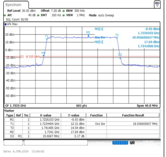
Band4-20MHz-QPSK-20325-100RB#0-PASS
