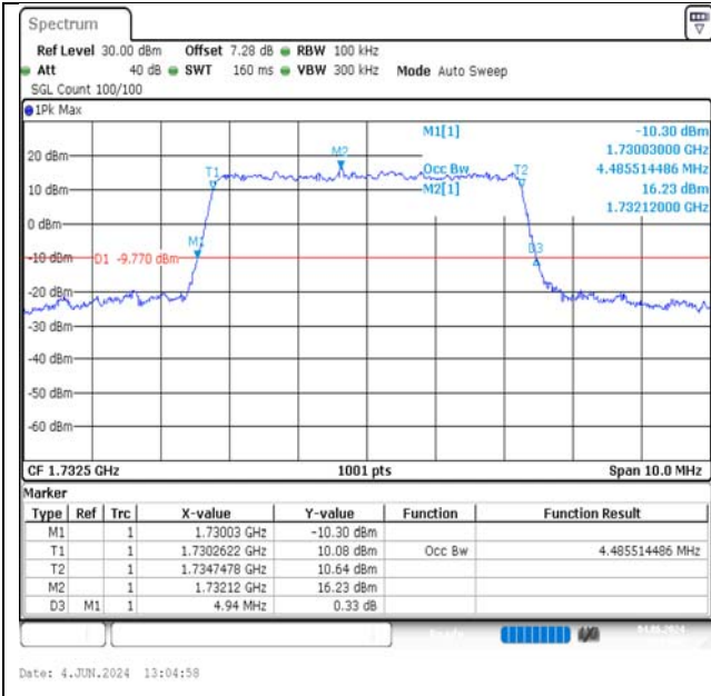
Band4-5MHz-16QAM-20175-25RB#0-PASS
