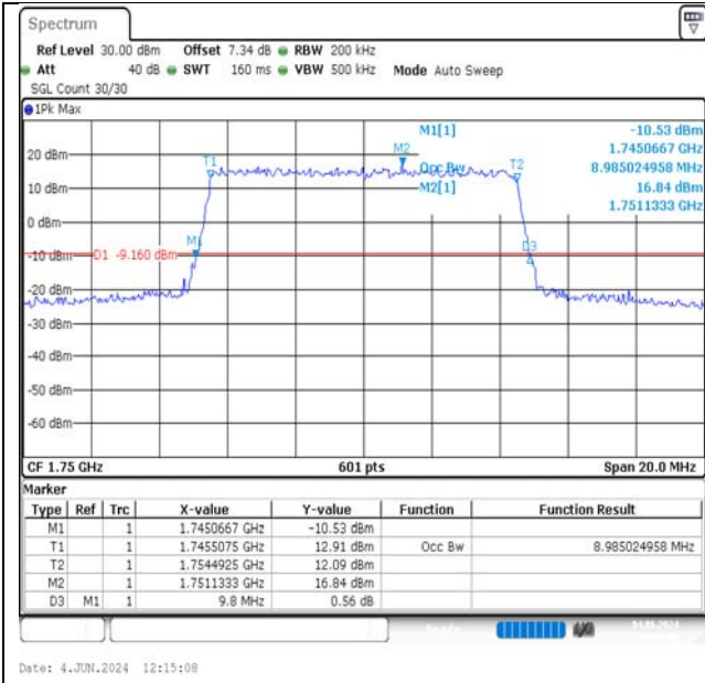
Band4-10MHz-QPSK-20350-50RB#0-PASS
