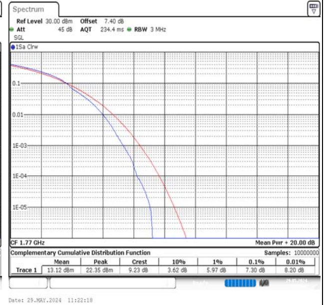
Band66-20MHz-16QAM-132572-100RB#0-PASS
