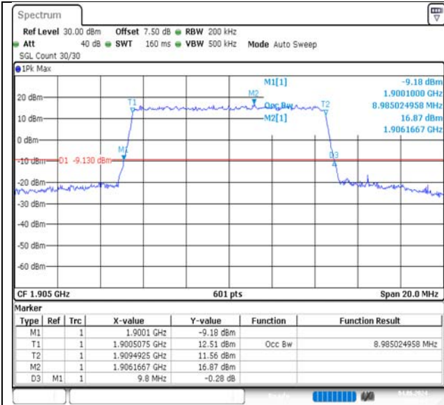
Band2-10MHz-QPSK-19150-50RB#0-PASS
