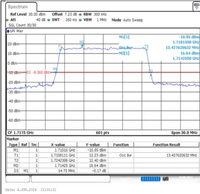
Band4-15MHz-QPSK-20025-75RB#0-PASS
