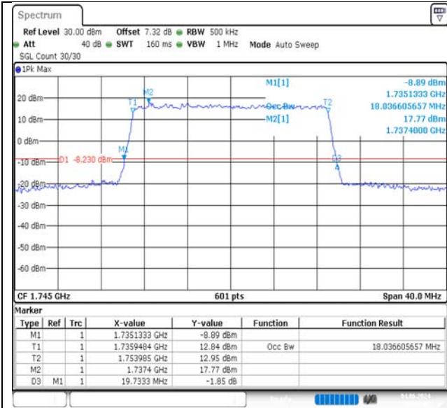
Band4-20MHz-QPSK-20300-100RB#0-PASS
