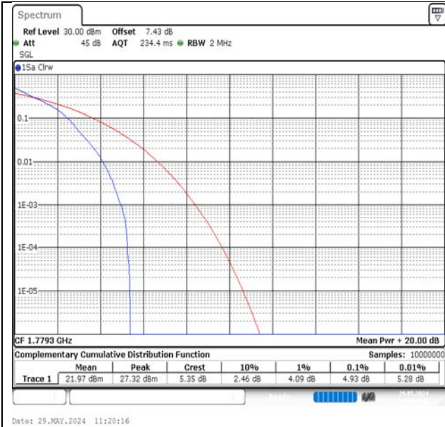
Band66-1.4MHz-QPSK-132665-1RB#0-PASS
