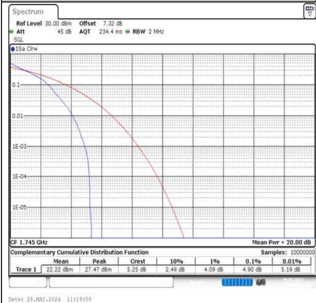
Band66-1.4MHz-QPSK-132322-1RB#0-PASS
