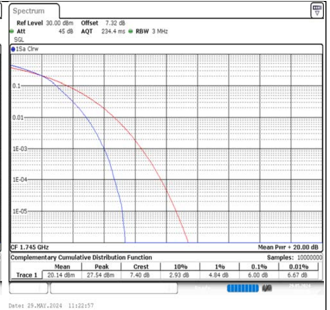
Band66-3MHz-16QAM-132322-15RB#0-PASS
