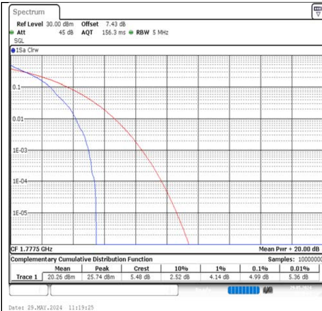
Band66-5MHz-QPSK-132647-1RB#0-PASS
