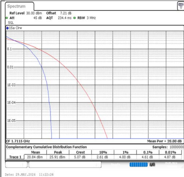
Band66-3MHz-QPSK-131987-1RB#0-PASS
