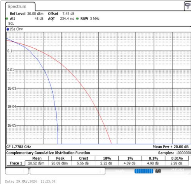
Band66-3MHz-QPSK-132657-1RB#0-PASS
