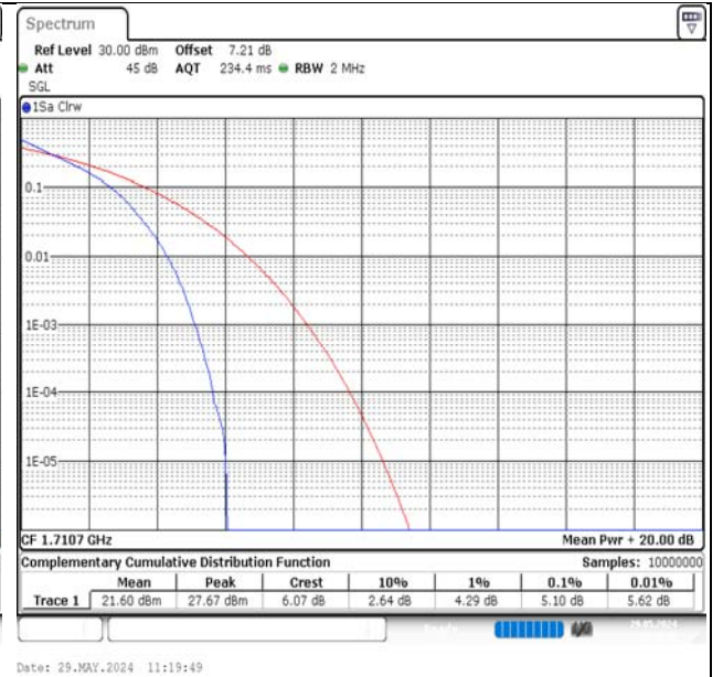
Band66-1.4MHz-QPSK-131979-6RB#0-PASS
