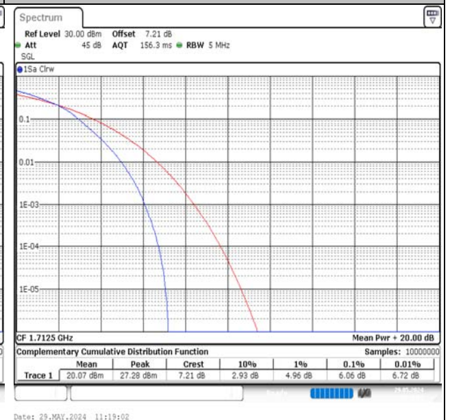
Band66-5MHz-16QAM-131997-25RB#0-PASS
