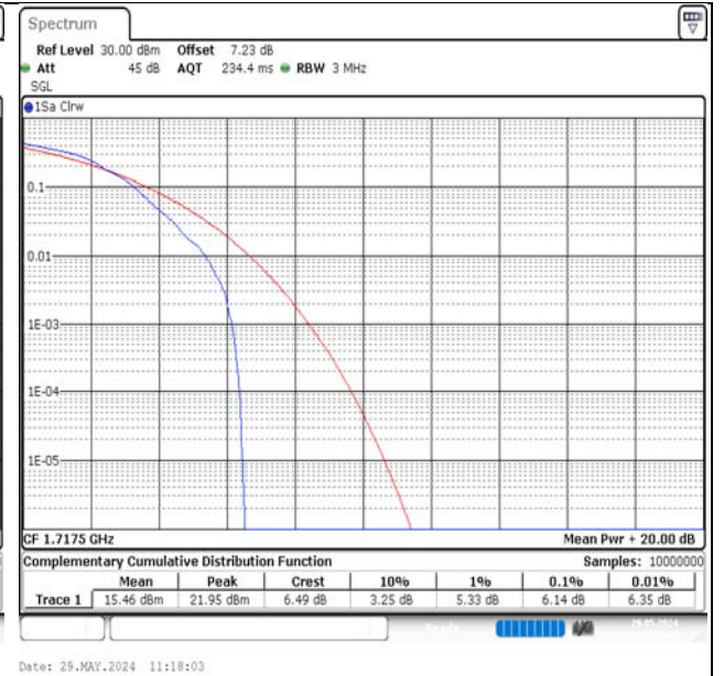
Band66-15MHz-QPSK-132047-75RB#0-PASS
