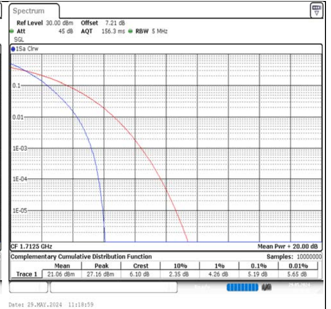
Band66-5MHz-QPSK-131997-25RB#0-PASS
