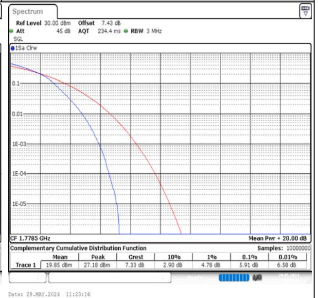
Band66-3MHz-16QAM-132657-15RB#0-PASS
