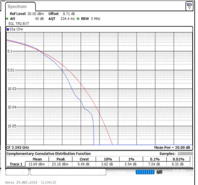
Band41-20MHz-16QAM-40620-100RB#0-PASS
