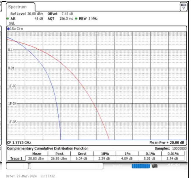
Band66-5MHz-QPSK-132647-25RB#0-PASS
