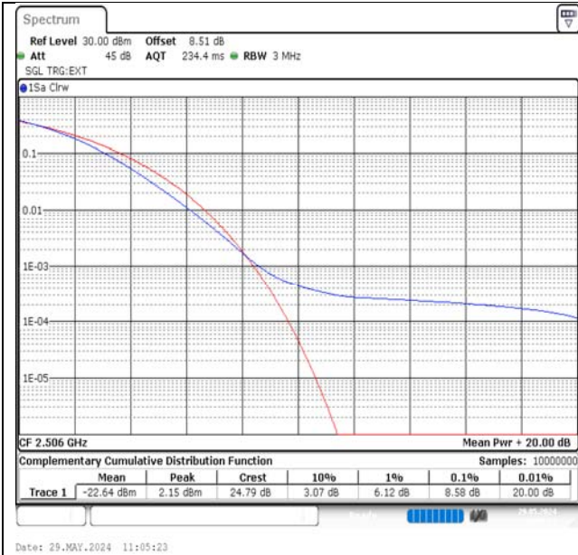
Band41-20MHz-QPSK-39750-1RB#0-PASS
