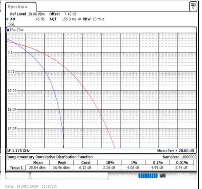
Band66-10MHz-QPSK-132622-50RB#0-PASS
