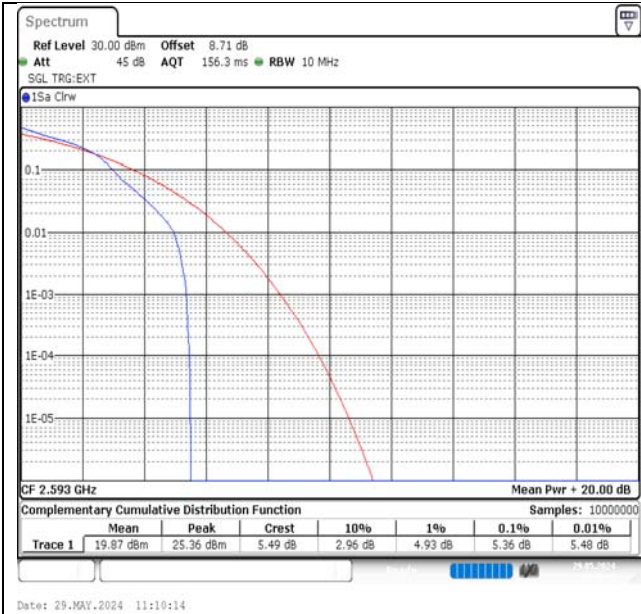
Band41-10MHz-16QAM-40620-1RB#0-PASS
