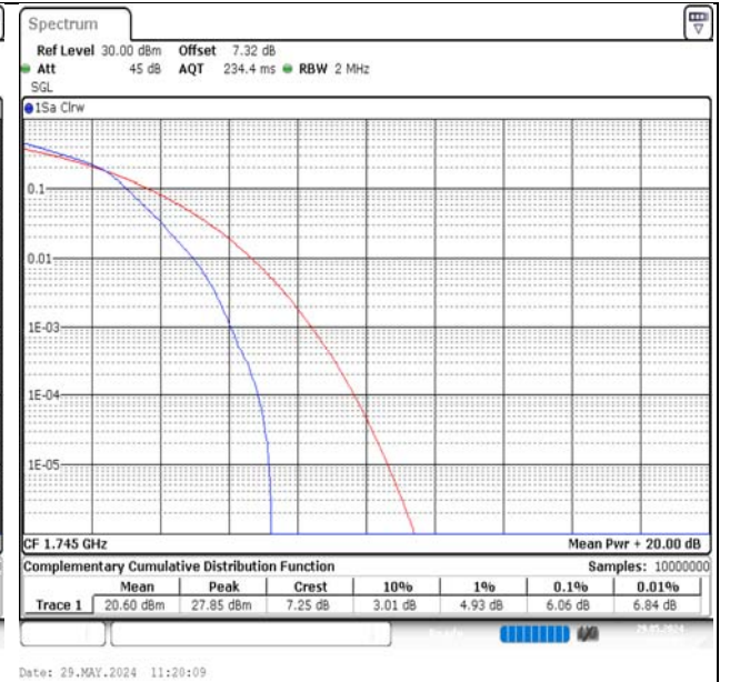
Band66-1.4MHz-16QAM-132322-6RB#0-PASS
