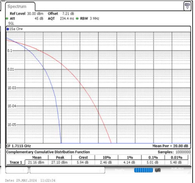
Band66-3MHz-QPSK-131987-15RB#0-PASS
