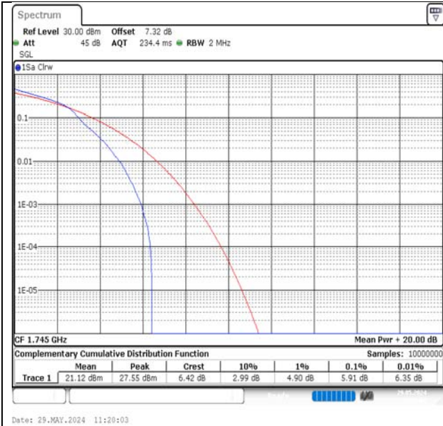
Band66-1.4MHz-16QAM-132322-1RB#0-PASS
