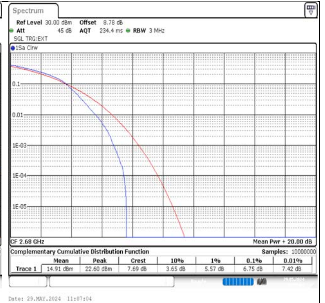
Band41-20MHz-QPSK-41490-100RB#0-PASS
