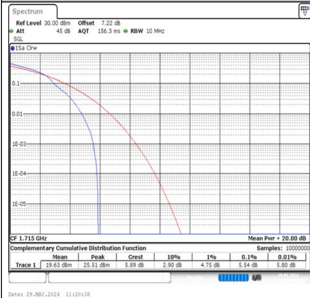
Band66-10MHz-16QAM-132022-1RB#0-PASS
