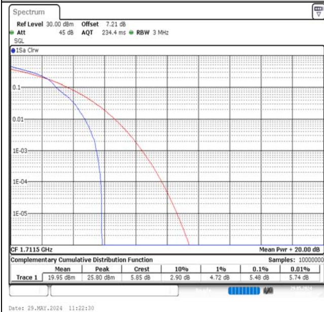
Band66-3MHz-16QAM-131987-1RB#0-PASS
