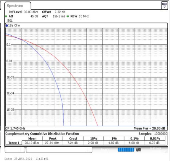
Band66-10MHz-16QAM-132322-50RB#0-PASS
