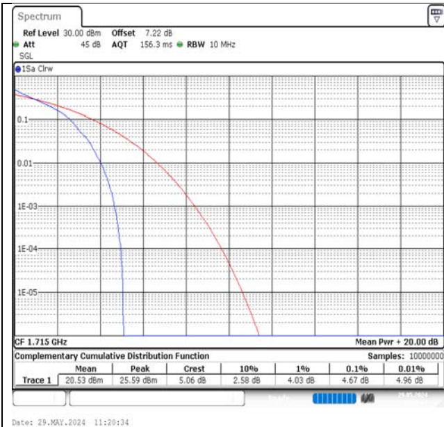
Band66-10MHz-QPSK-132022-1RB#0-PASS
