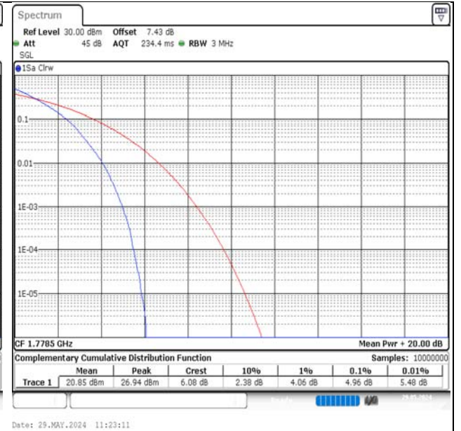
Band66-3MHz-QPSK-132657-15RB#0-PASS
