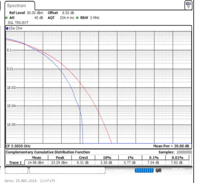
Band41-15MHz-16QAM-39725-75RB#0-PASS
