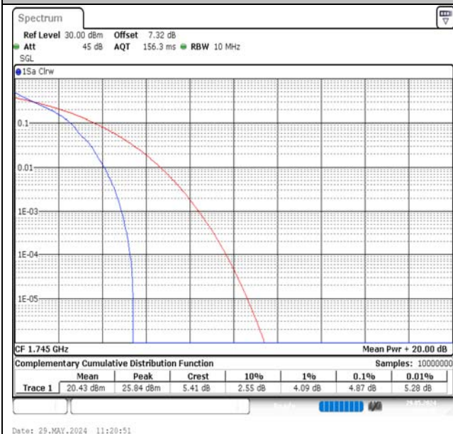
Band66-10MHz-QPSK-132322-1RB#0-PASS
