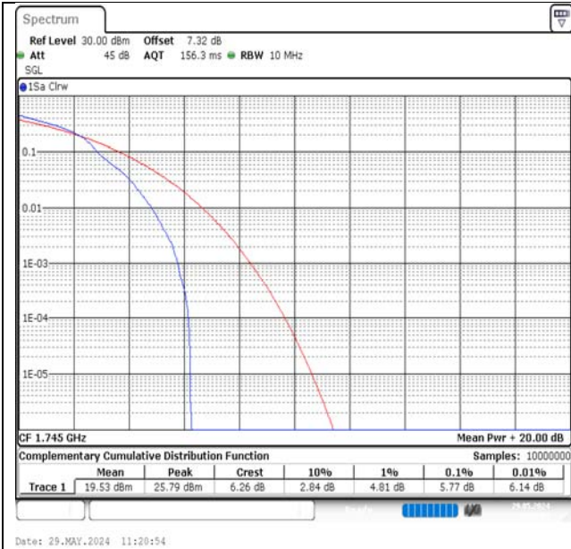
Band66-10MHz-16QAM-132322-1RB#0-PASS
