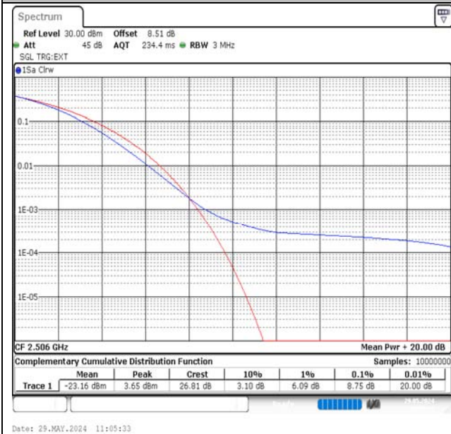
Band41-20MHz-16QAM-39750-1RB#0-PASS
