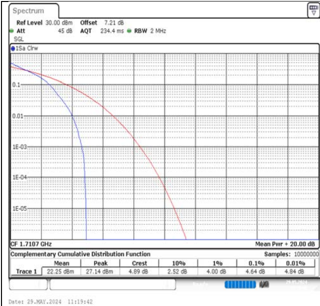
Band66-1.4MHz-QPSK-131979-1RB#0-PASS
