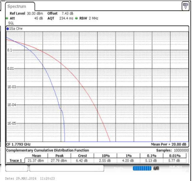
Band66-1.4MHz-QPSK-132665-6RB#0-PASS
