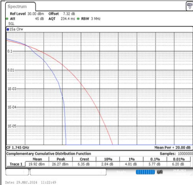
Band66-3MHz-16QAM-132322-1RB#0-PASS
