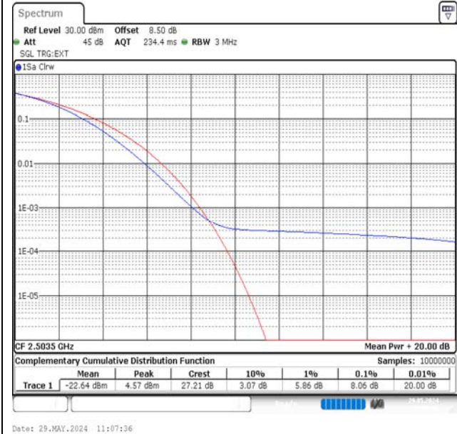
Band41-15MHz-16QAM-39725-1RB#0-PASS
