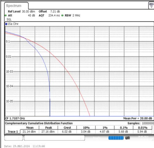
Band66-1.4MHz-16QAM-131979-1RB#0-PASS
