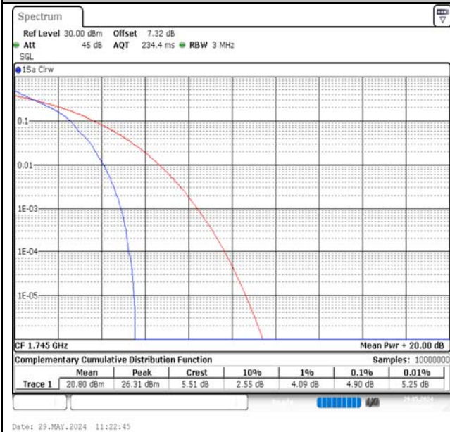
Band66-3MHz-QPSK-132322-1RB#0-PASS
