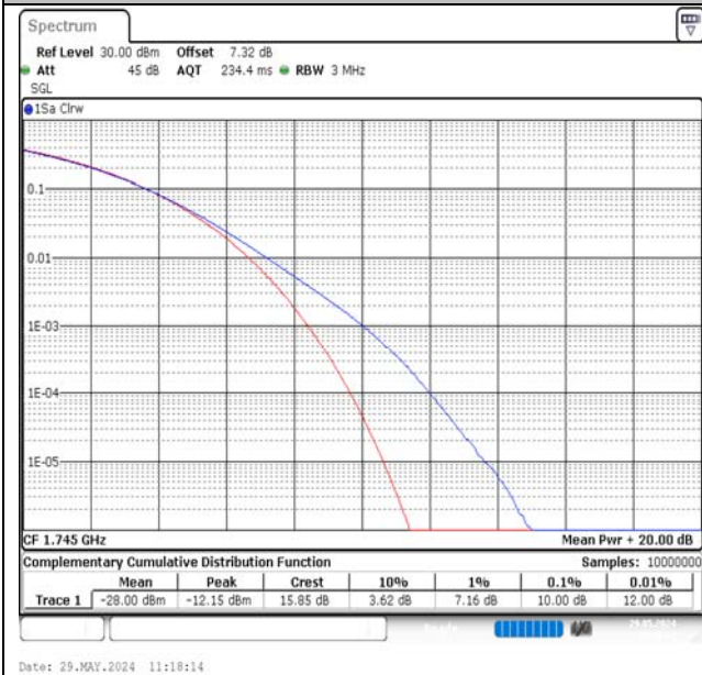
Band66-15MHz-QPSK-132322-1RB#0-PASS
