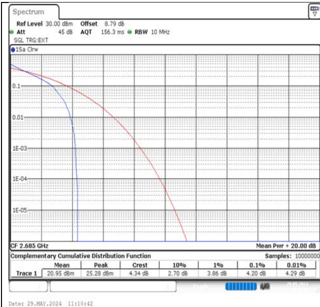
Band41-10MHz-QPSK-41540-1RB#0-PASS
