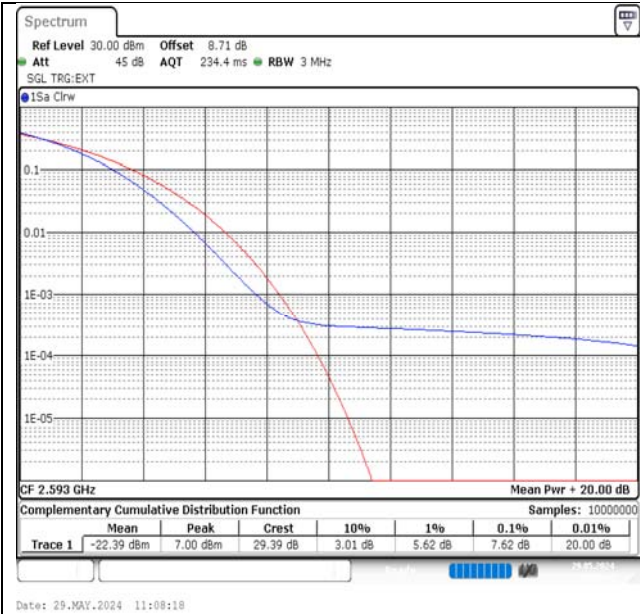
Band41-15MHz-16QAM-40620-1RB#0-PASS
