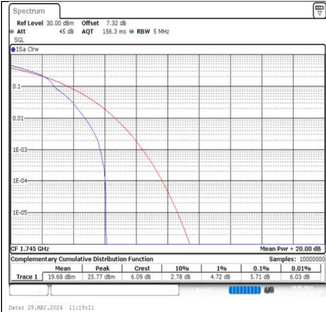
Band66-5MHz-16QAM-132322-1RB#0-PASS
