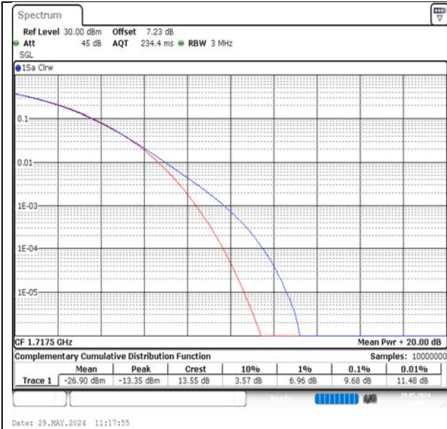
Band66-15MHz-QPSK-132047-1RB#0-PASS
