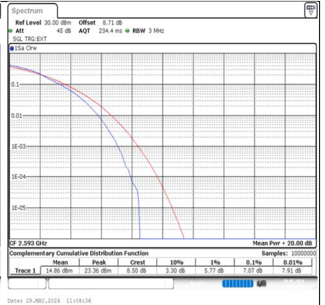
Band41-15MHz-16QAM-40620-75RB#0-PASS
