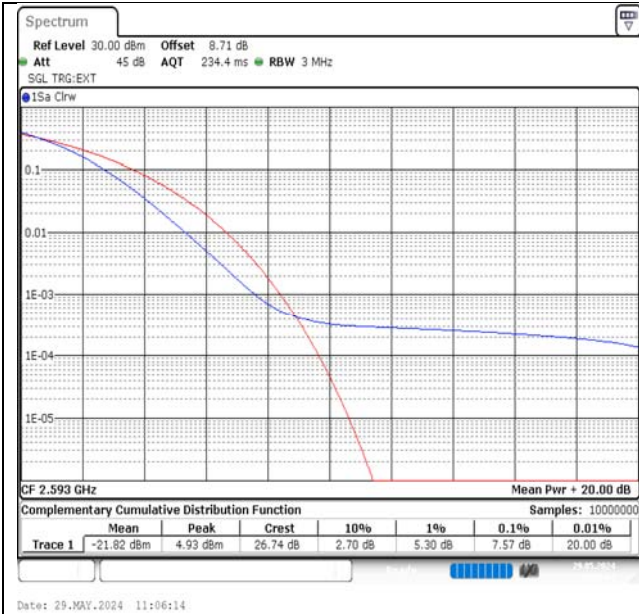
Band41-20MHz-16QAM-40620-1RB#0-PASS
