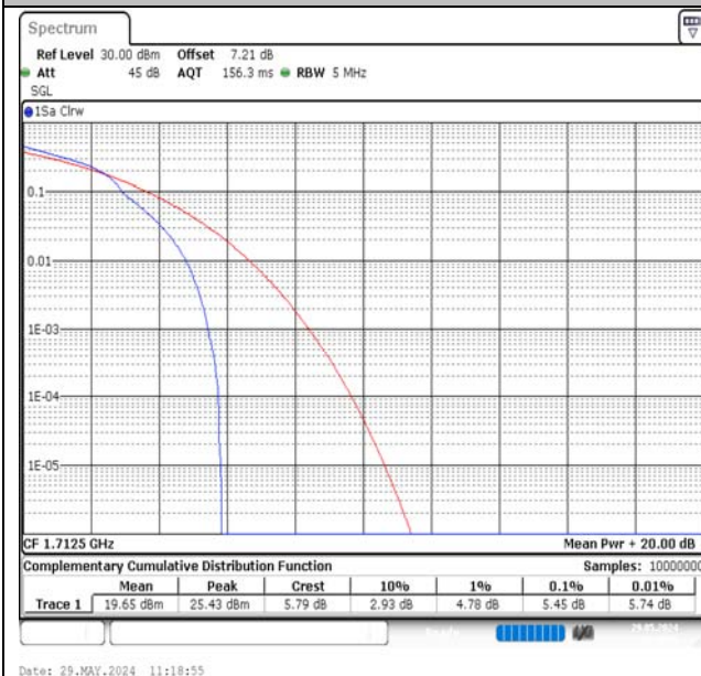
Band66-5MHz-16QAM-131997-1RB#0-PASS
