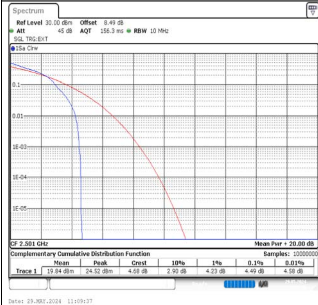
Band41-10MHz-16QAM-39700-1RB#0-PASS
