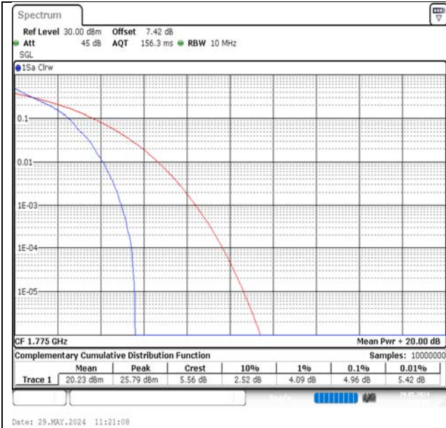
Band66-10MHz-QPSK-132622-1RB#0-PASS
