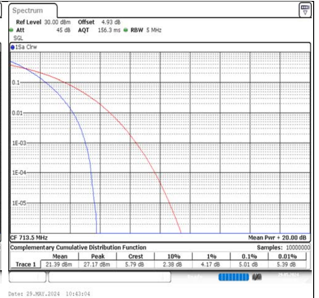
Band17-5MHz-QPSK-23825-25RB#0-PASS
