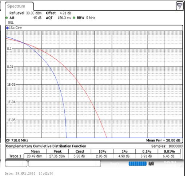
Band17-5MHz-16QAM-23790-25RB#0-PASS
