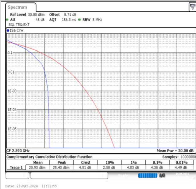
Band41-5MHz-QPSK-40620-1RB#0-PASS
