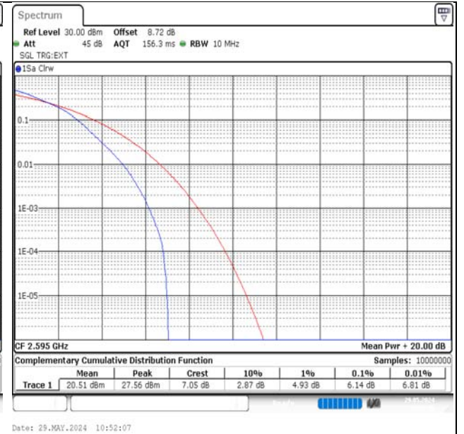
Band38-10MHz-16QAM-38000-50RB#0-PASS
