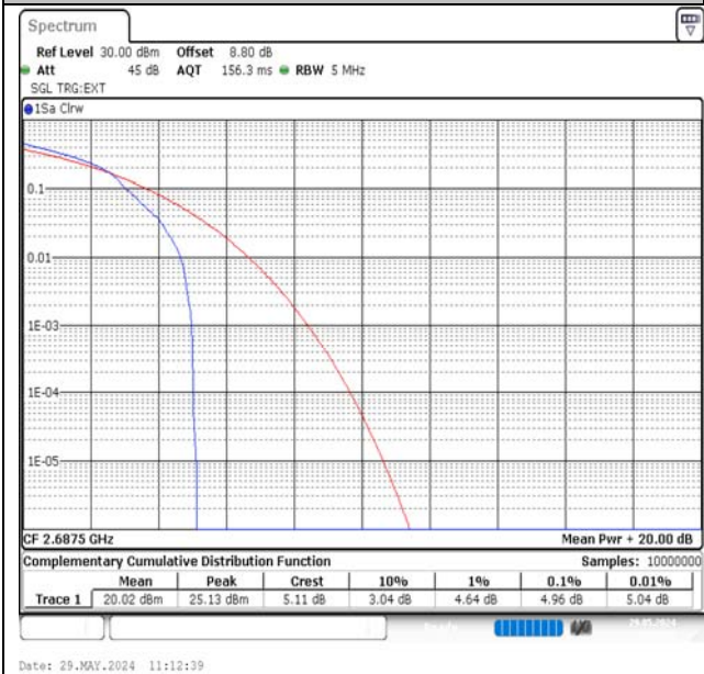
Band41-5MHz-16QAM-41565-1RB#0-PASS
