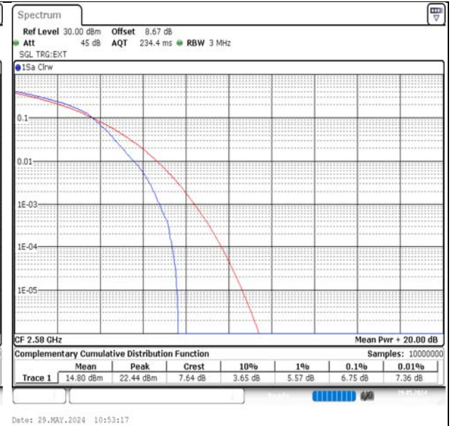
Band38-20MHz-QPSK-37850-100RB#0-PASS
