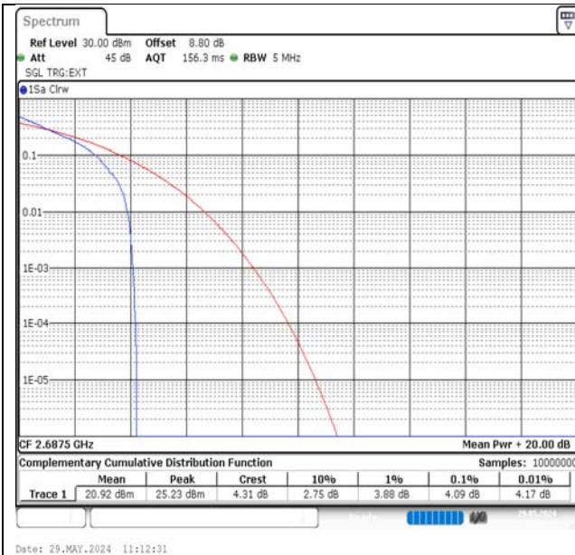
Band41-5MHz-QPSK-41565-1RB#0-PASS
