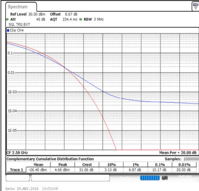
Band38-20MHz-16QAM-37850-1RB#0-PASS
