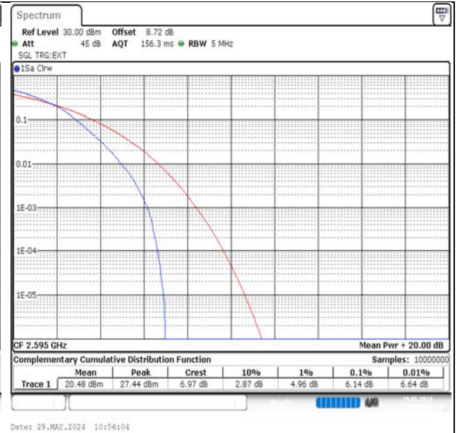
Band38-5MHz-16QAM-38000-25RB#0-PASS
