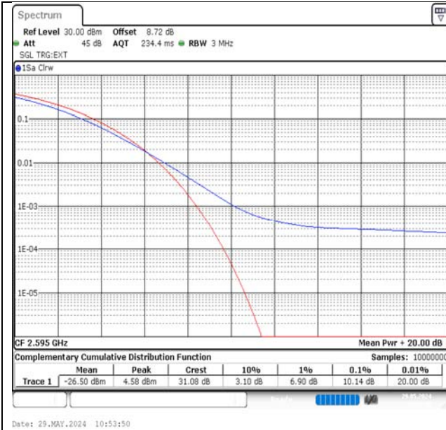
Band38-20MHz-16QAM-38000-1RB#0-PASS
