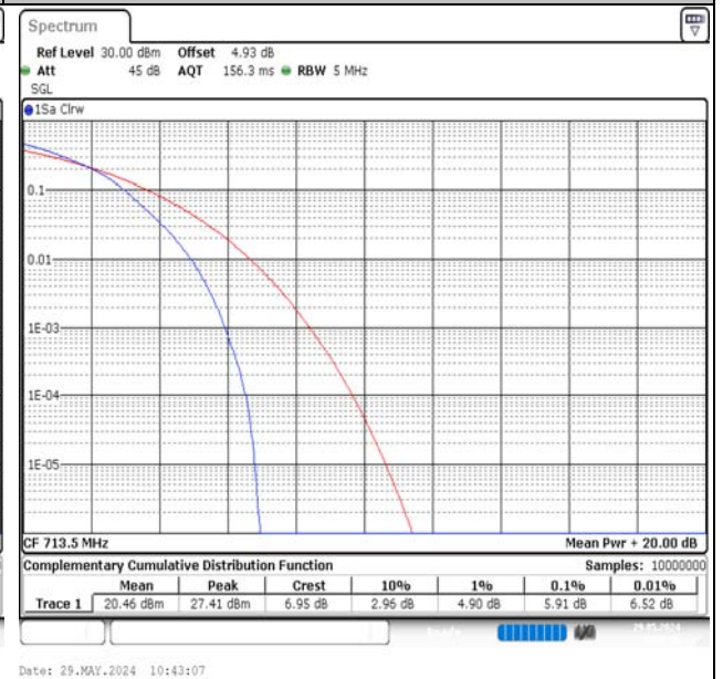
Band17-5MHz-16QAM-23825-25RB#0-PASS
