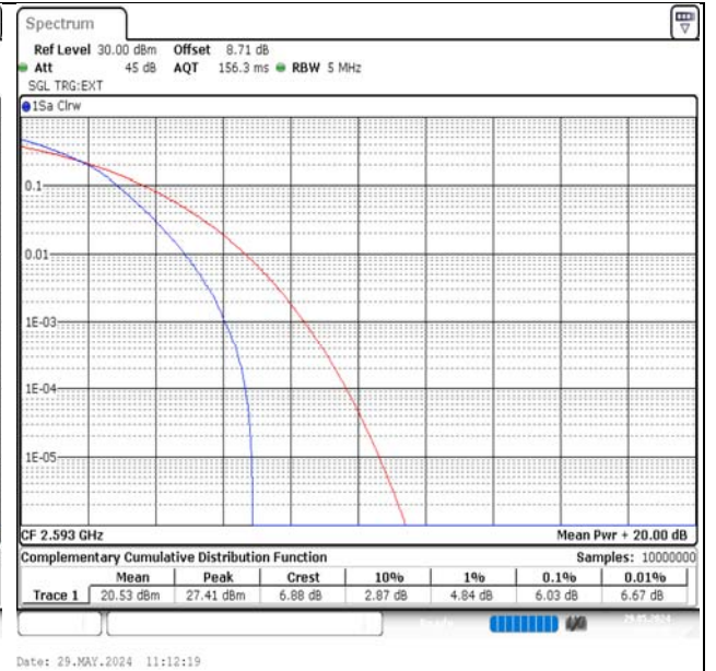
Band41-5MHz-16QAM-40620-25RB#0-PASS
