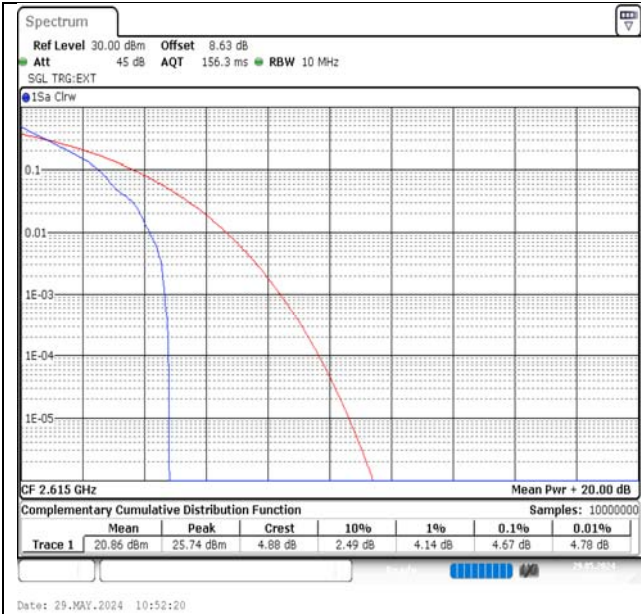
Band38-10MHz-QPSK-38200-1RB#0-PASS
