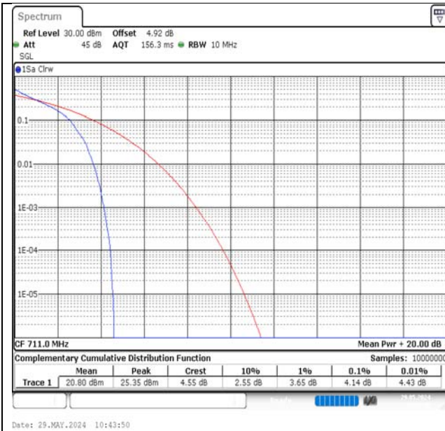
Band17-10MHz-QPSK-23800-1RB#0-PASS
