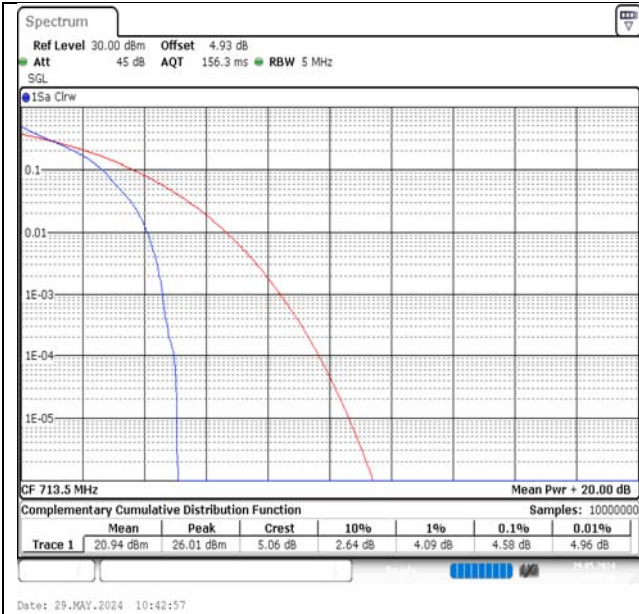
Band17-5MHz-QPSK-23825-1RB#0-PASS
