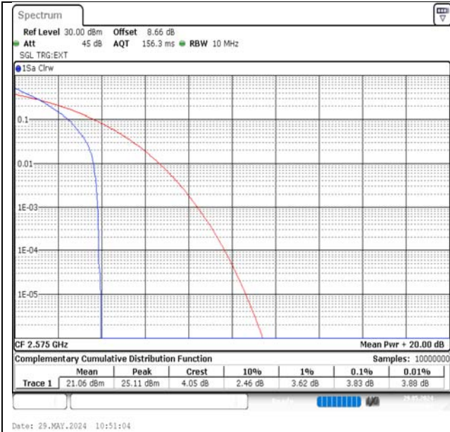
Band38-10MHz-QPSK-37800-1RB#0-PASS
