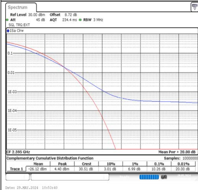
Band38-20MHz-QPSK-38000-1RB#0-PASS
