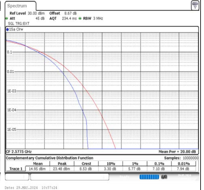
Band38-15MHz-16QAM-37825-75RB#0-PASS
