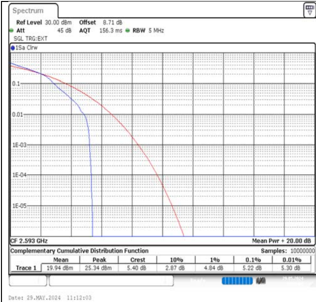
Band41-5MHz-16QAM-40620-1RB#0-PASS
