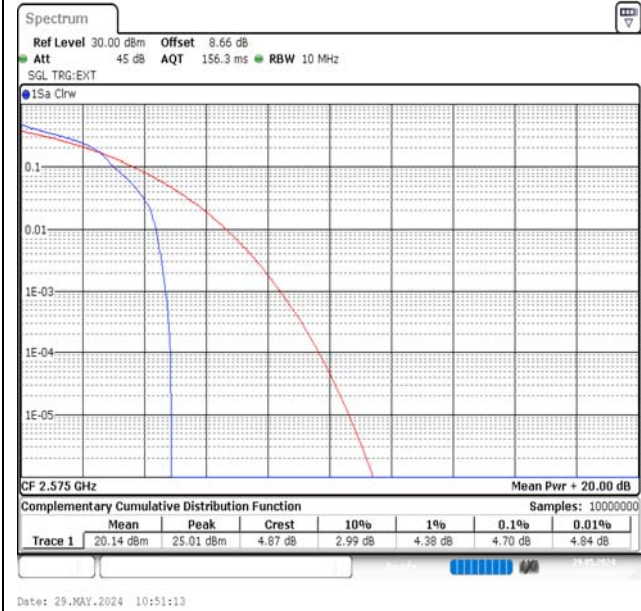
Band38-10MHz-16QAM-37800-1RB#0-PASS
