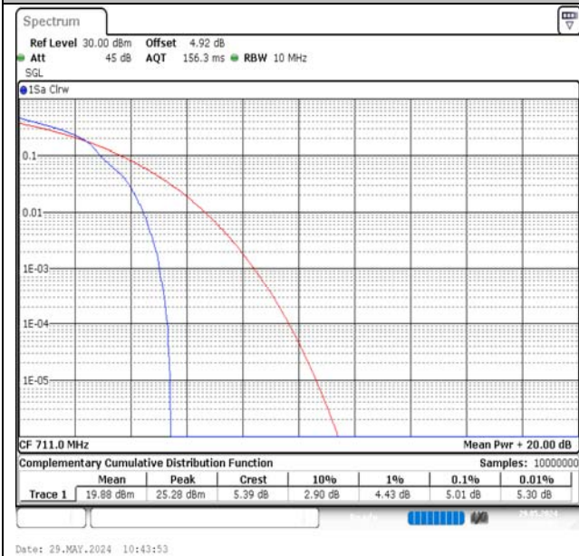
Band17-10MHz-16QAM-23800-1RB#0-PASS
