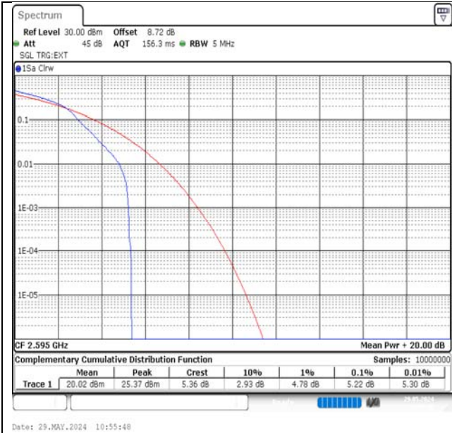
Band38-5MHz-16QAM-38000-1RB#0-PASS
