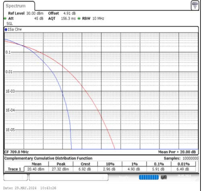
Band17-10MHz-16QAM-23780-50RB#0-PASS
