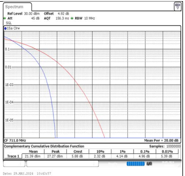
Band17-10MHz-QPSK-23800-50RB#0-PASS
