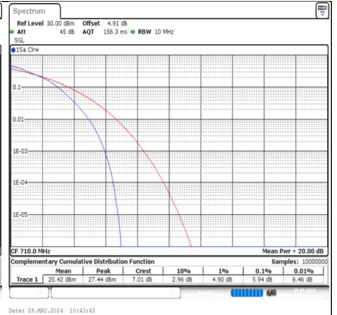
Band17-10MHz-16QAM-23790-50RB#0-PASS
