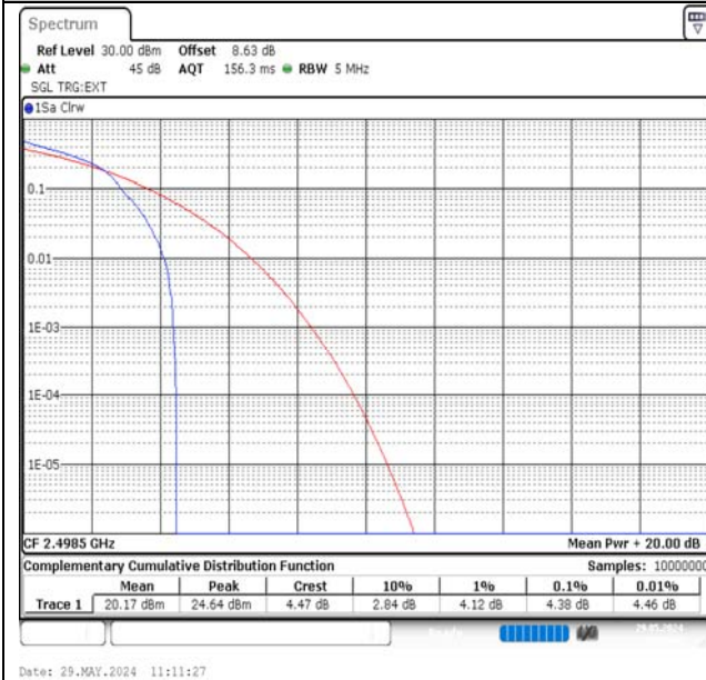
Band41-5MHz-16QAM-39675-1RB#0-PASS
