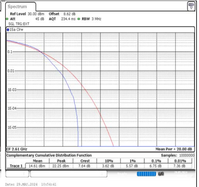
Band38-20MHz-QPSK-38150-100RB#0-PASS
