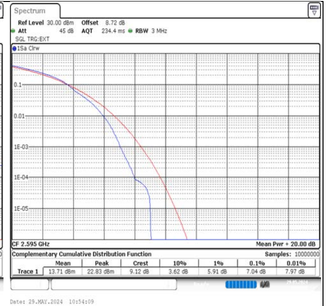
Band38-20MHz-16QAM-38000-100RB#0-PASS
