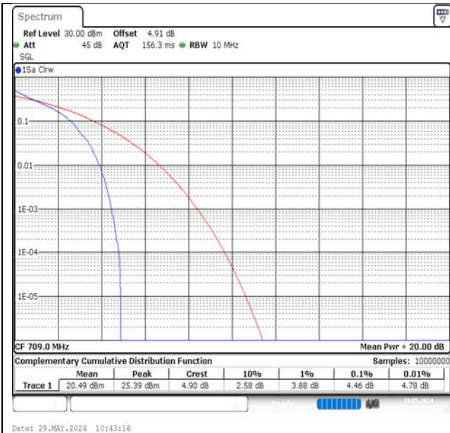
Band17-10MHz-QPSK-23780-1RB#0-PASS
