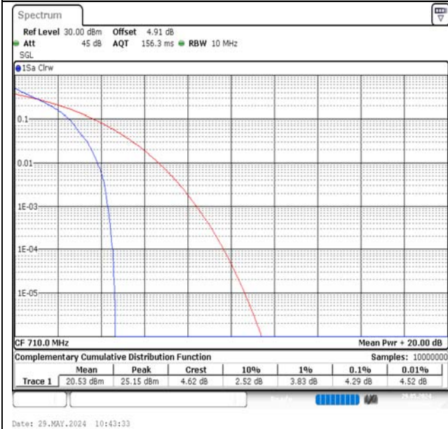
Band17-10MHz-QPSK-23790-1RB#0-PASS
