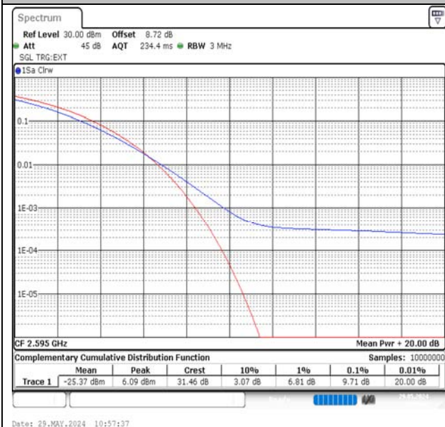
Band38-15MHz-QPSK-38000-1RB#0-PASS
