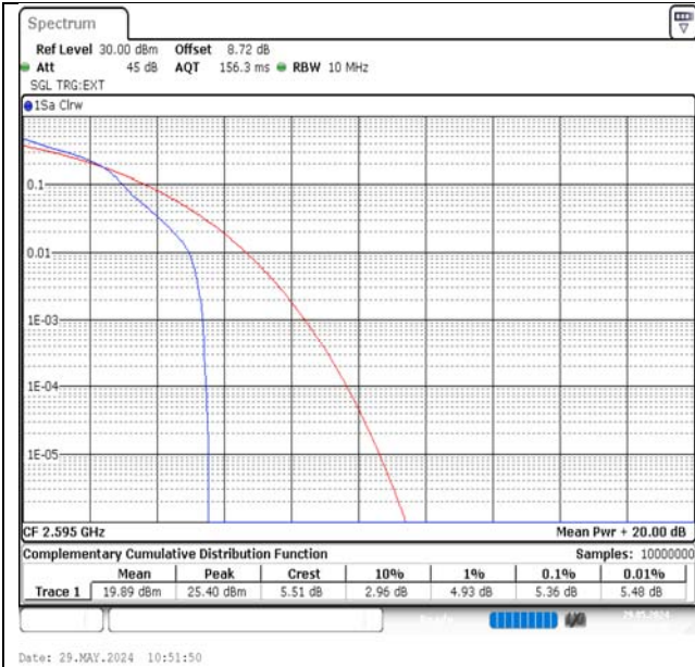
Band38-10MHz-16QAM-38000-1RB#0-PASS
