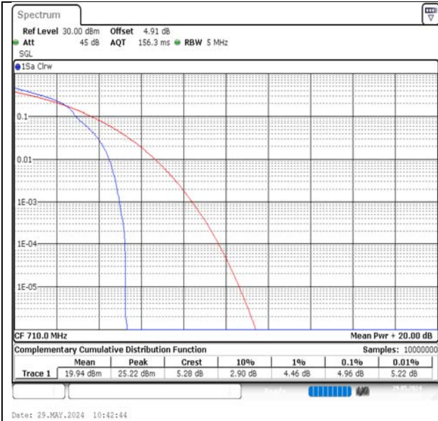
Band17-5MHz-16QAM-23790-1RB#0-PASS
