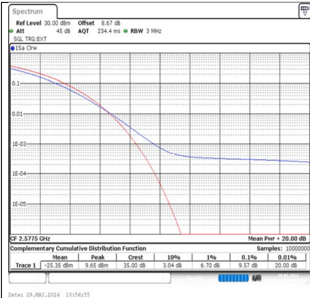
Band38-15MHz-QPSK-37825-1RB#0-PASS
