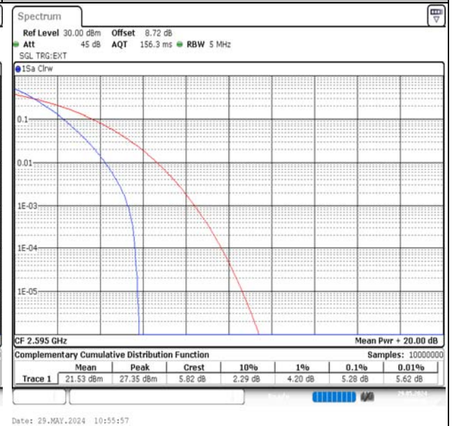
Band38-5MHz-QPSK-38000-25RB#0-PASS
