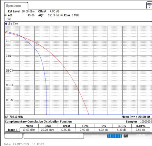
Band17-5MHz-16QAM-23755-1RB#0-PASS
