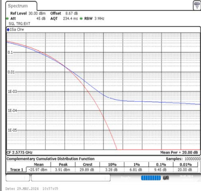
Band38-15MHz-16QAM-37825-1RB#0-PASS
