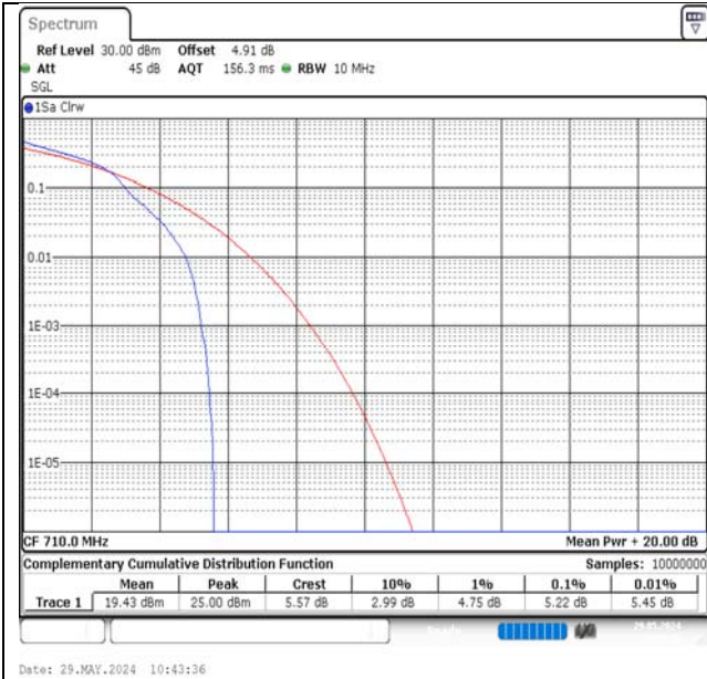
Band17-10MHz-16QAM-23790-1RB#0-PASS
