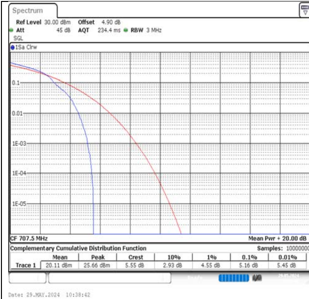
Band12-3MHz-16QAM-23095-1RB#0-PASS
