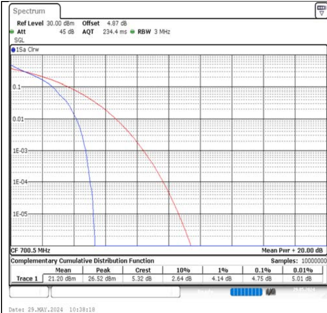
Band12-3MHz-QPSK-23025-1RB#0-PASS
