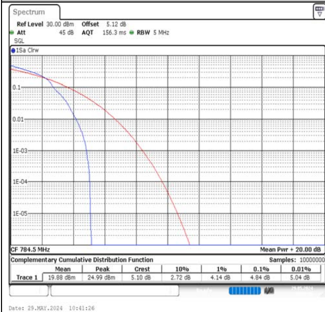
Band13-5MHz-16QAM-23255-1RB#0-PASS
