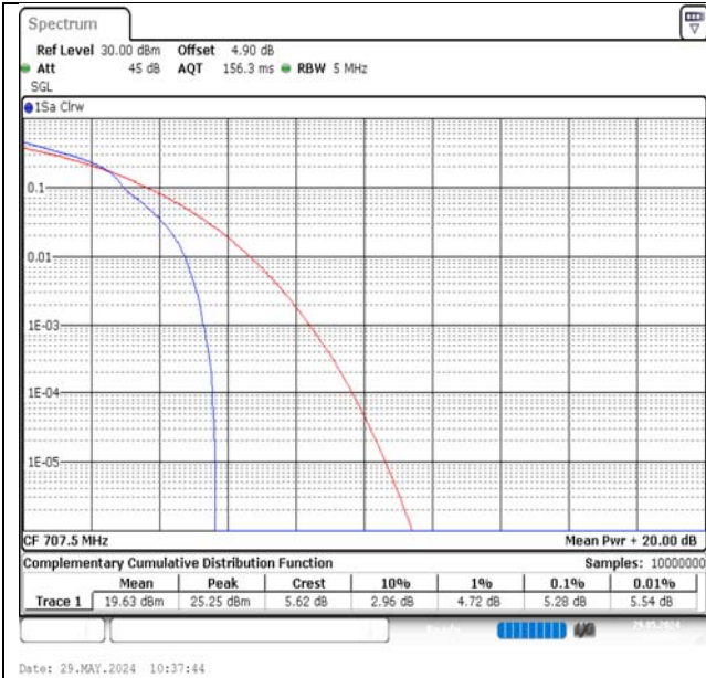
Band12-5MHz-16QAM-23095-1RB#0-PASS
