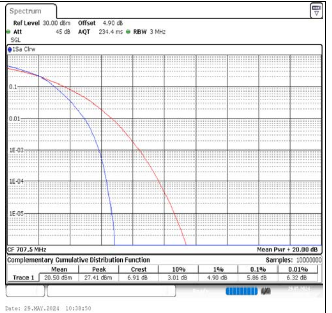
Band12-3MHz-16QAM-23095-15RB#0-PASS
