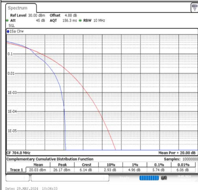
Band12-10MHz-16QAM-23060-1RB#0-PASS
