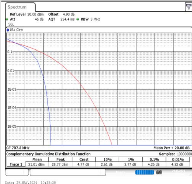
Band12-3MHz-QPSK-23095-1RB#0-PASS
