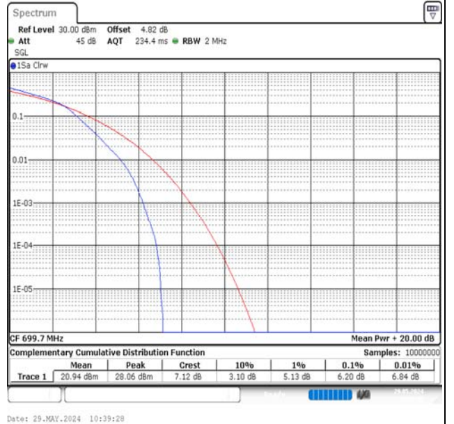
Band12-1.4MHz-16QAM-23017-6RB#0-PASS
