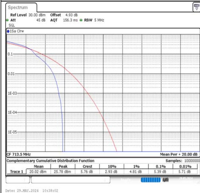
Band12-5MHz-16QAM-23155-1RB#0-PASS
