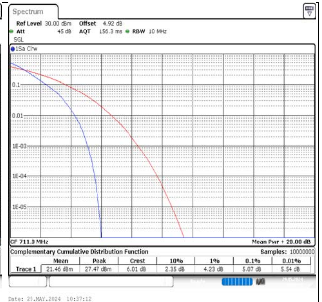
Band12-10MHz-QPSK-23130-50RB#0-PASS
