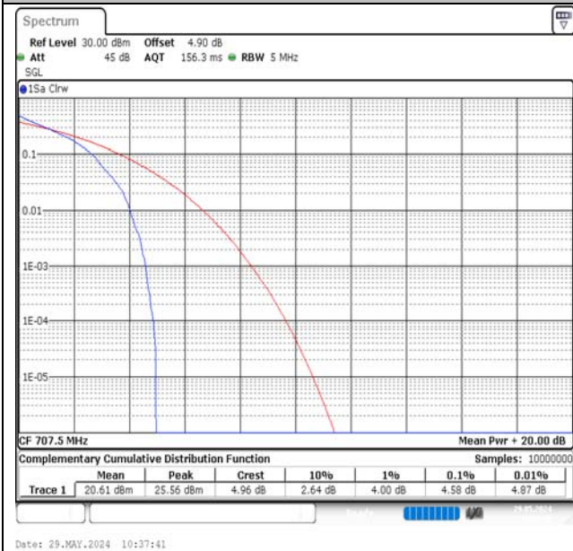
Band12-5MHz-QPSK-23095-1RB#0-PASS
