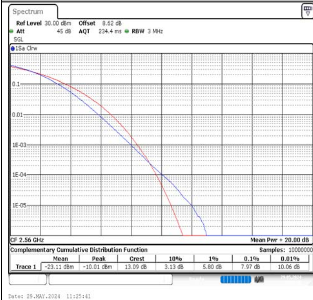
Band7-20MHz-16QAM-21350-1RB#0-PASS
