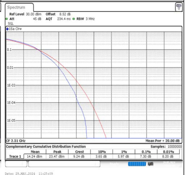
Band7-20MHz-16QAM-20850-100RB#0-PASS
