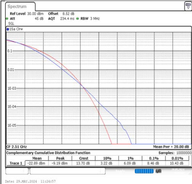
Band7-20MHz-QPSK-20850-1RB#0-PASS
