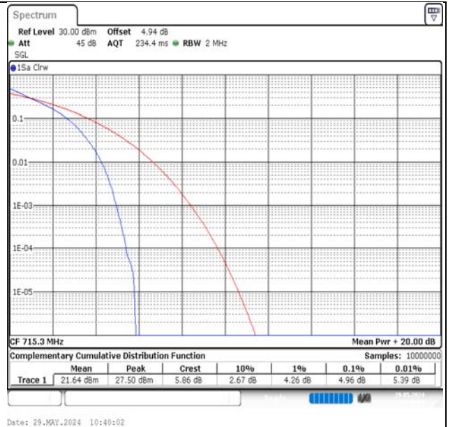
Band12-1.4MHz-QPSK-23173-6RB#0-PASS
