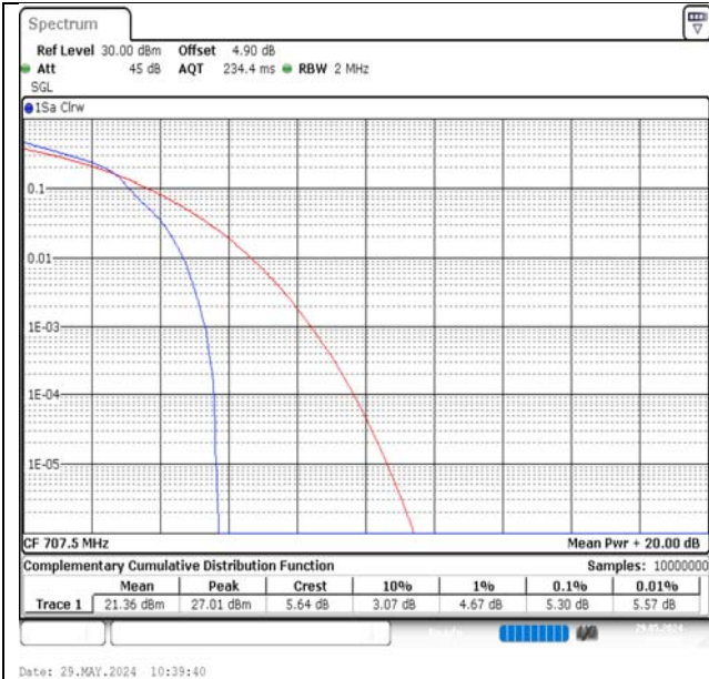
Band12-1.4MHz-16QAM-23095-1RB#0-PASS
