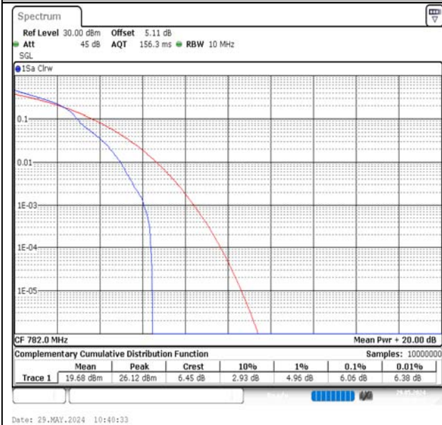
Band13-10MHz-16QAM-23230-1RB#0-PASS
