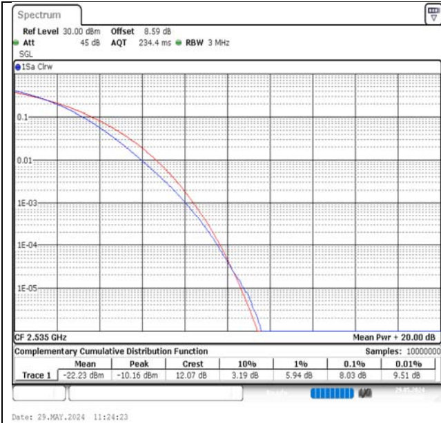
Band7-15MHz-16QAM-21100-1RB#0-PASS
