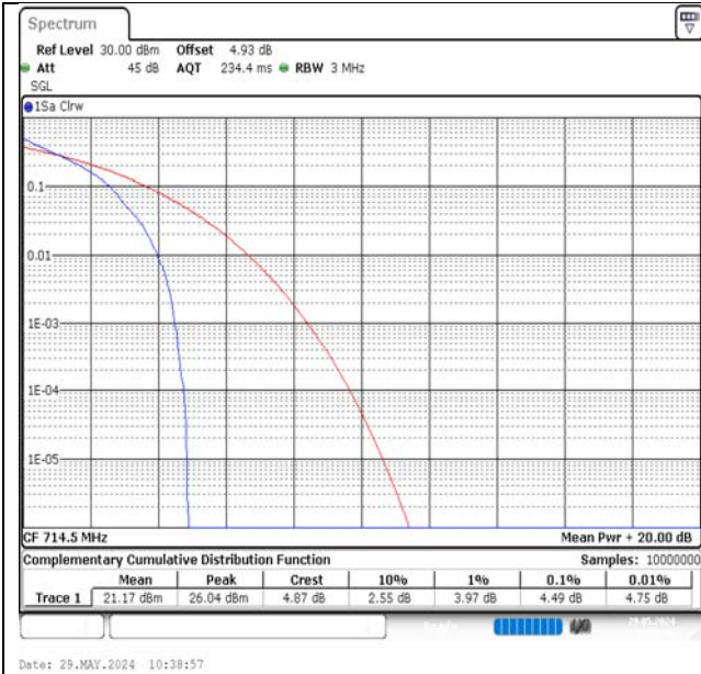
Band12-3MHz-QPSK-23165-1RB#0-PASS
