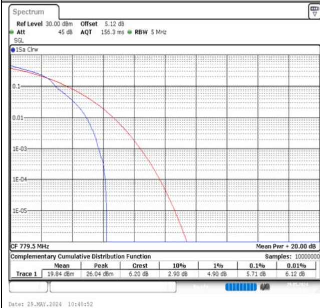
Band13-5MHz-16QAM-23205-1RB#0-PASS
