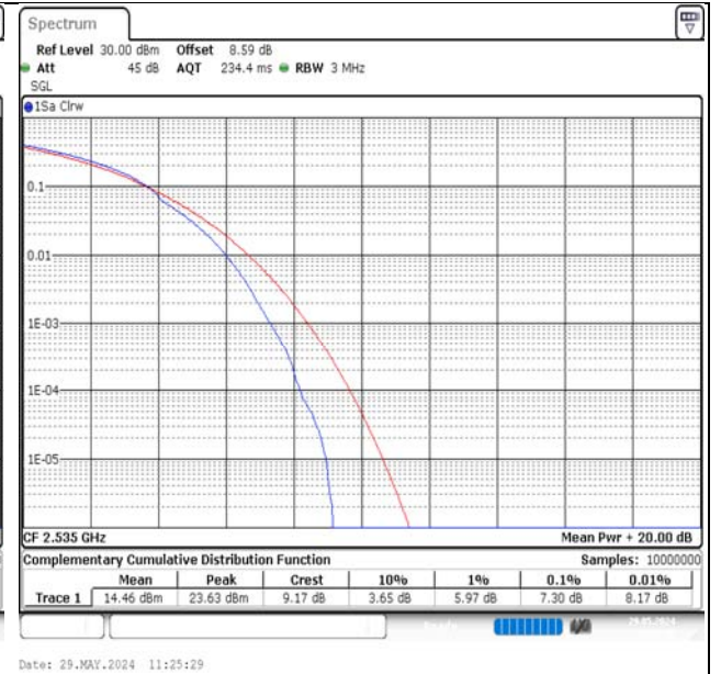
Band7-20MHz-16QAM-21100-100RB#0-PASS
