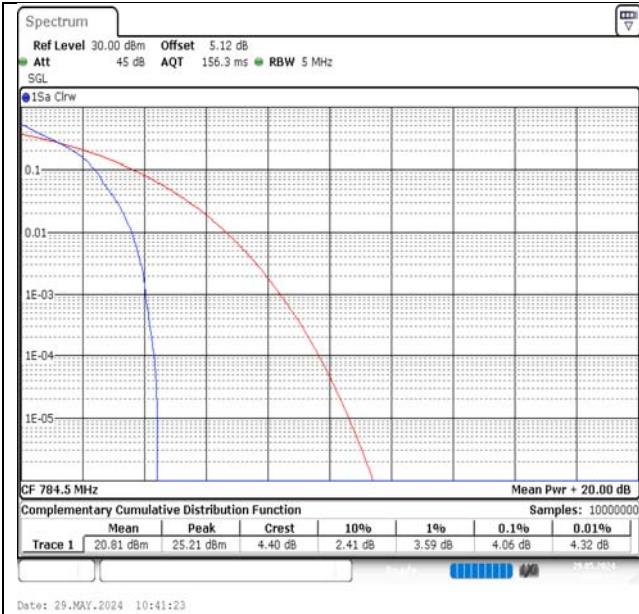
Band13-5MHz-QPSK-23255-1RB#0-PASS
