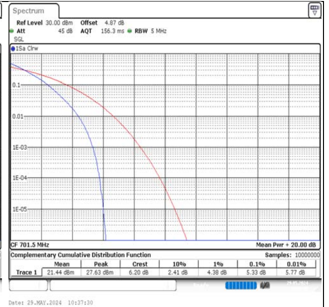
Band12-5MHz-QPSK-23035-25RB#0-PASS
