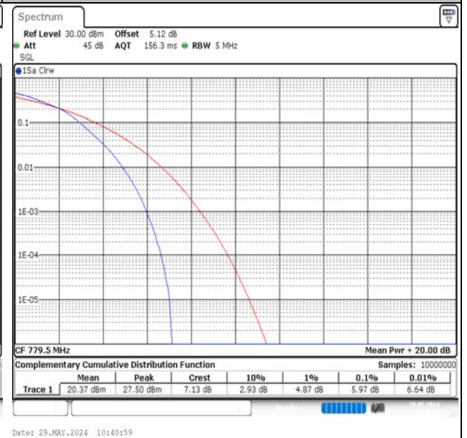
Band13-5MHz-16QAM-23205-25RB#0-PASS
