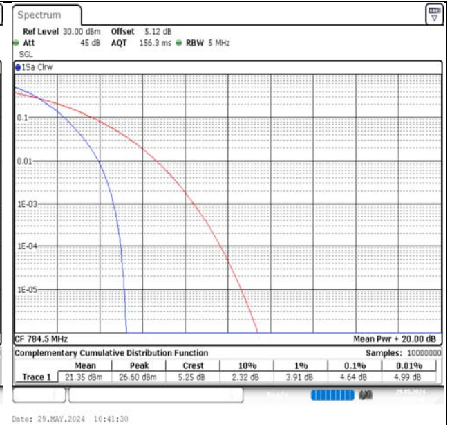
Band13-5MHz-QPSK-23255-25RB#0-PASS
