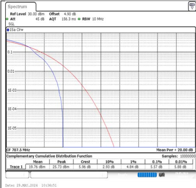
Band12-10MHz-16QAM-23095-1RB#0-PASS
