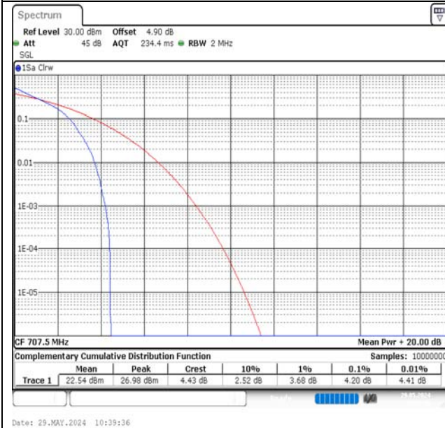
Band12-1.4MHz-QPSK-23095-1RB#0-PASS
