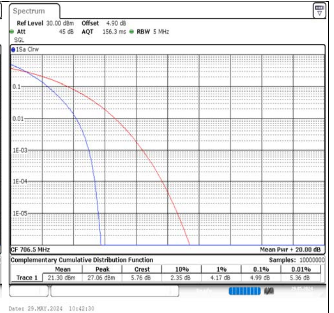
Band17-5MHz-QPSK-23755-25RB#0-PASS
