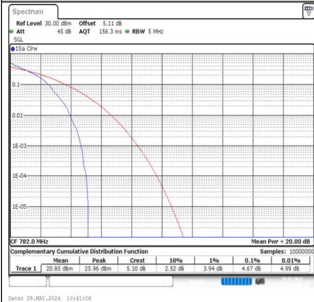
Band13-5MHz-QPSK-23230-1RB#0-PASS
