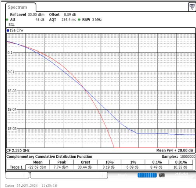
Band7-20MHz-QPSK-21100-1RB#0-PASS
