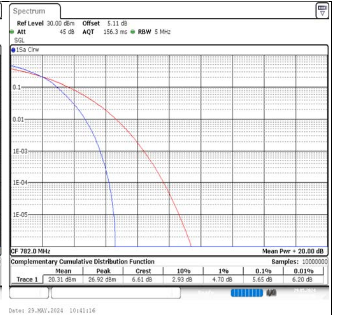
Band13-5MHz-16QAM-23230-25RB#0-PASS
