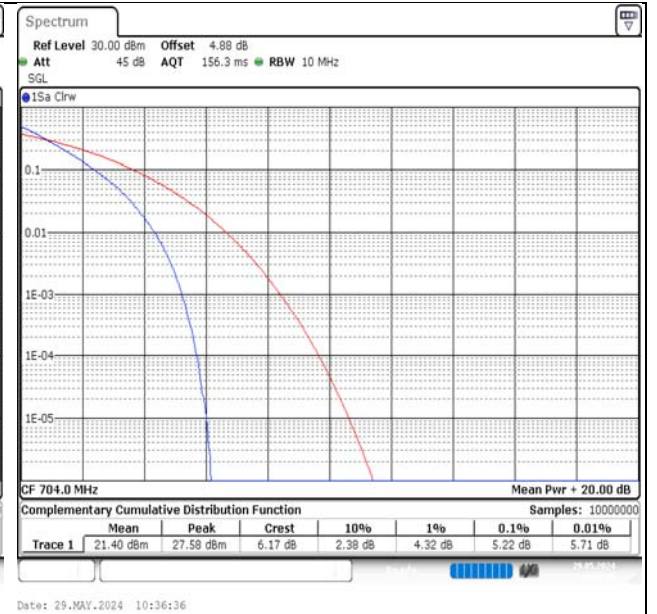
Band12-10MHz-QPSK-23060-50RB#0-PASS
