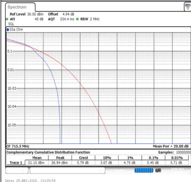
Band12-1.4MHz-16QAM-23173-1RB#0-PASS
