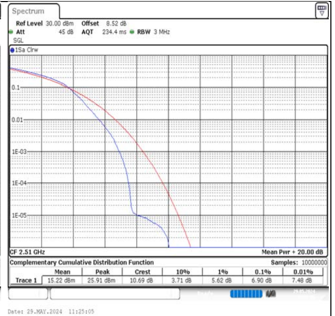
Band7-20MHz-QPSK-20850-100RB#0-PASS
