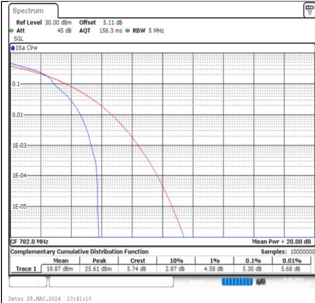
Band13-5MHz-16QAM-23230-1RB#0-PASS
