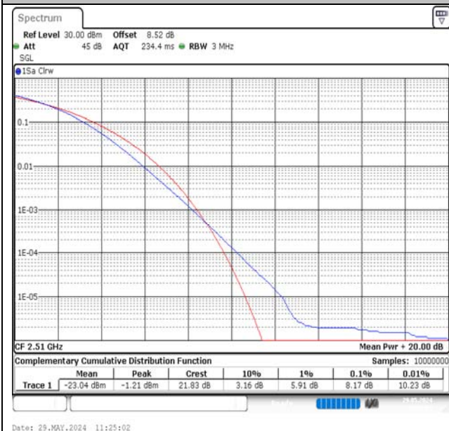
Band7-20MHz-16QAM-20850-1RB#0-PASS
