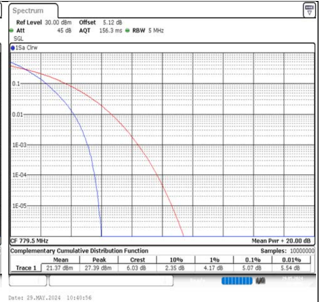
Band13-5MHz-QPSK-23205-25RB#0-PASS
