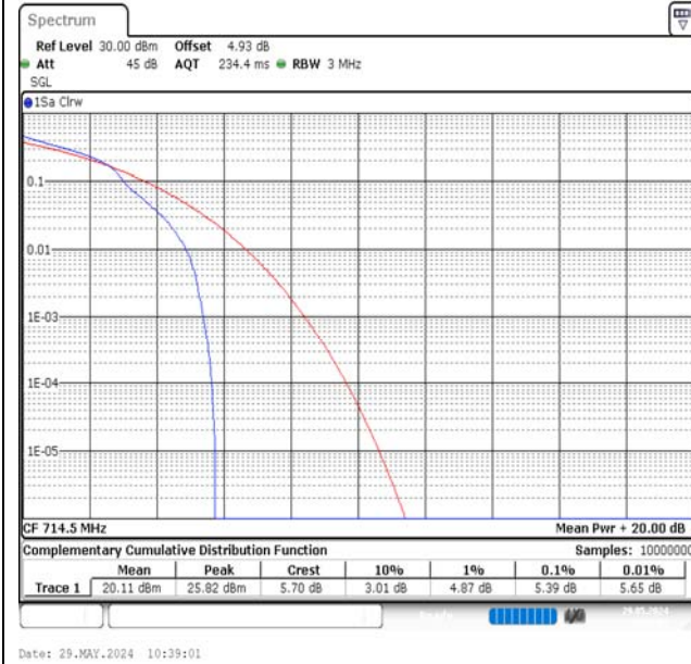
Band12-3MHz-16QAM-23165-1RB#0-PASS
