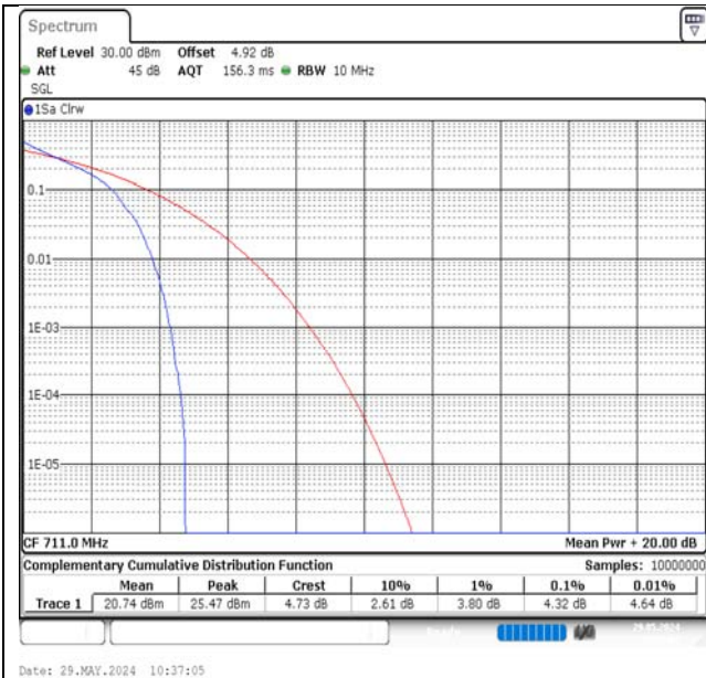
Band12-10MHz-QPSK-23130-1RB#0-PASS
