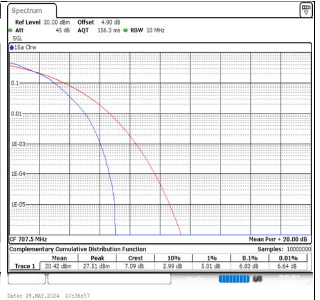
Band12-10MHz-16QAM-23095-50RB#0-PASS
