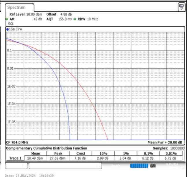
Band12-10MHz-16QAM-23060-50RB#0-PASS
