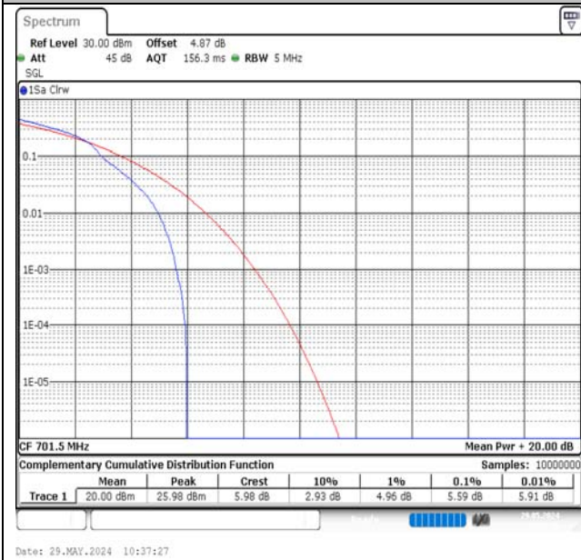
Band12-5MHz-16QAM-23035-1RB#0-PASS
