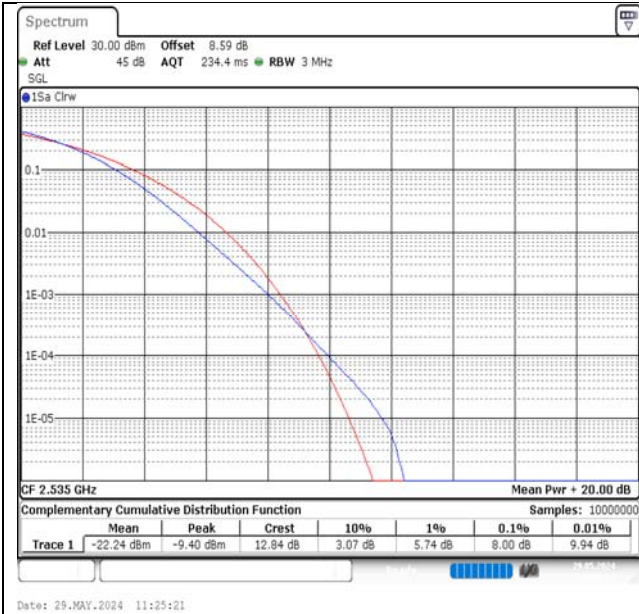
Band7-20MHz-16QAM-21100-1RB#0-PASS
