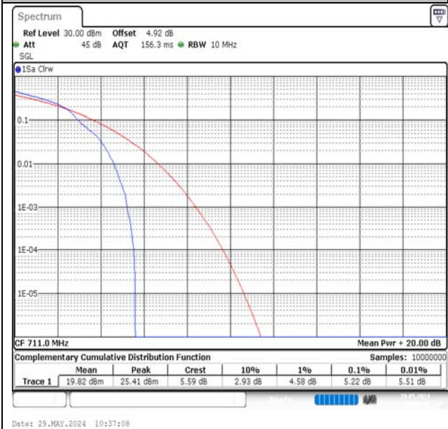
Band12-10MHz-16QAM-23130-1RB#0-PASS
