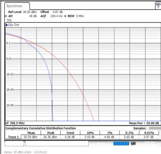
Band12-3MHz-16QAM-23025-1RB#0-PASS
