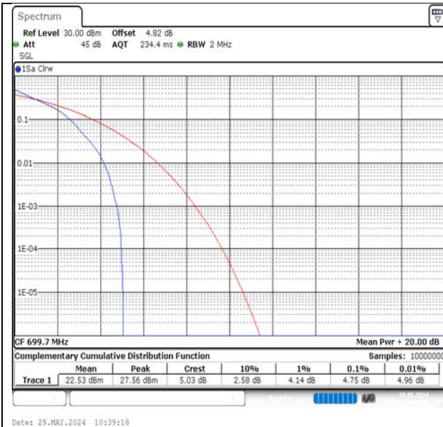
Band12-1.4MHz-QPSK-23017-1RB#0-PASS
