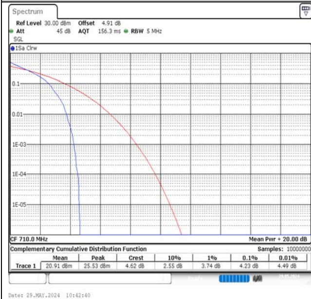
Band17-5MHz-QPSK-23790-1RB#0-PASS
