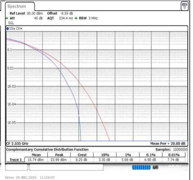
Band7-15MHz-16QAM-21100-75RB#0-PASS
