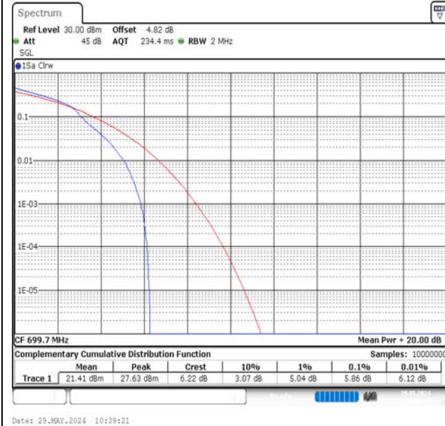
Band12-1.4MHz-16QAM-23017-1RB#0-PASS
