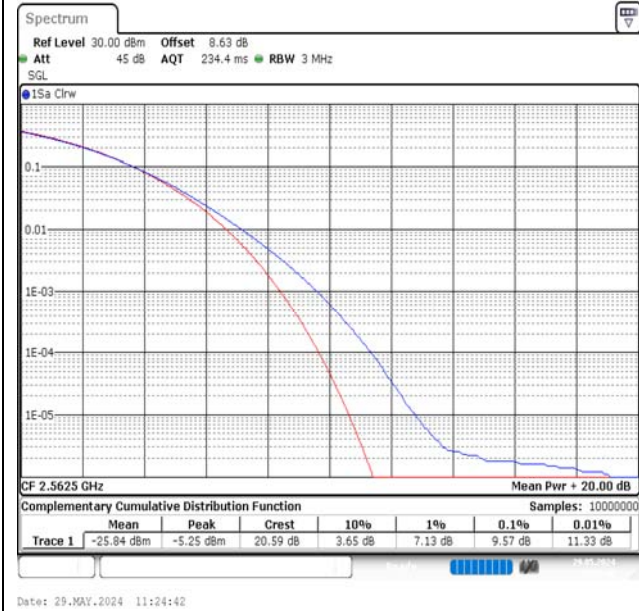
Band7-15MHz-16QAM-21375-1RB#0-PASS
