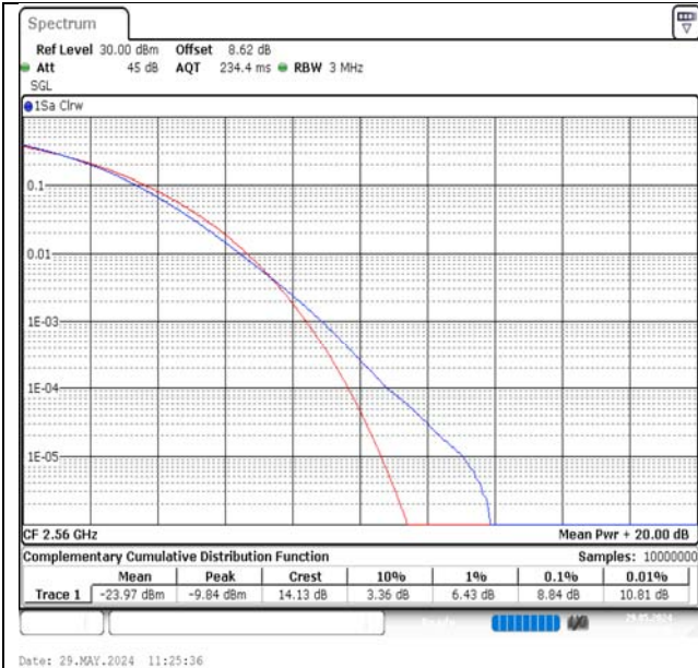
Band7-20MHz-QPSK-21350-1RB#0-PASS
