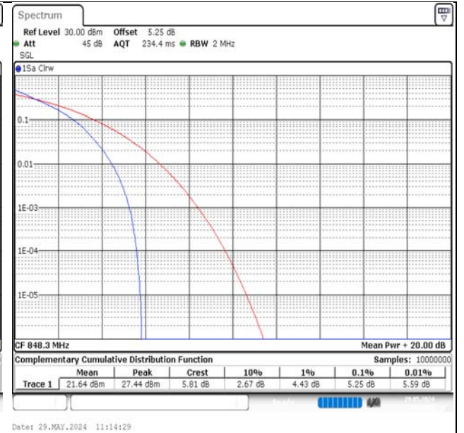
Band5-1.4MHz-QPSK-20643-6RB#0-PASS
