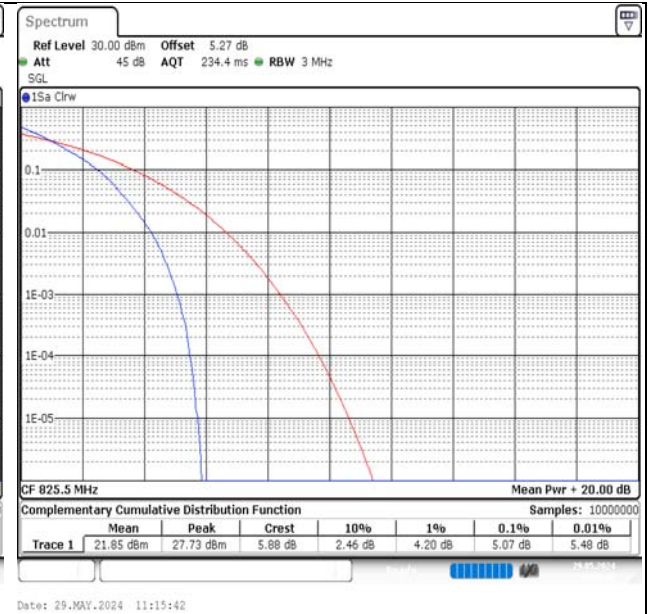
Band5-3MHz-QPSK-20415-15RB#0-PASS
