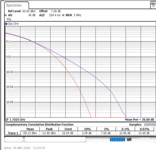
Band4-20MHz-16QAM-20175-1RB#0-PASS
