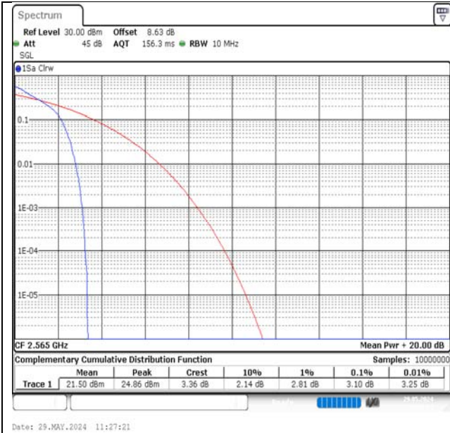
Band7-10MHz-QPSK-21400-1RB#0-PASS
