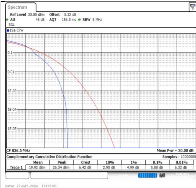
Band5-5MHz-16QAM-20525-1RB#0-PASS
