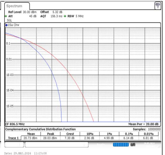
Band5-5MHz-16QAM-20525-25RB#0-PASS
