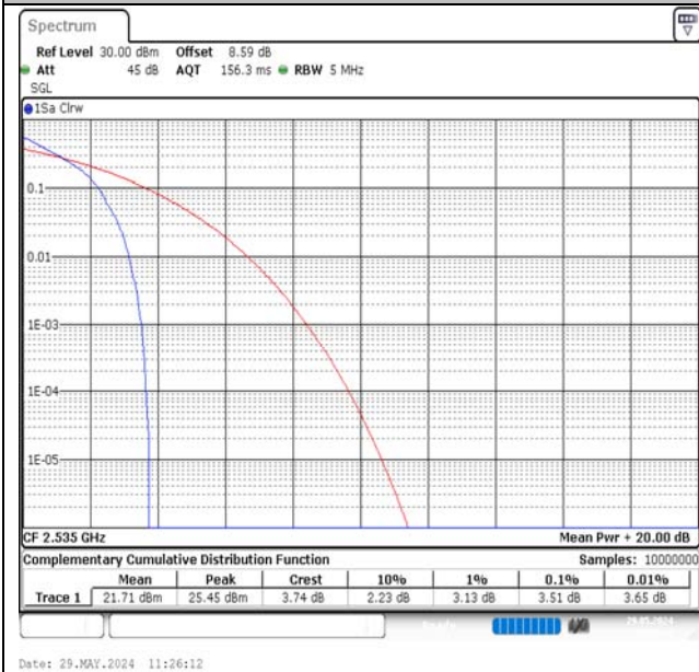
Band7-5MHz-QPSK-21100-1RB#0-PASS
