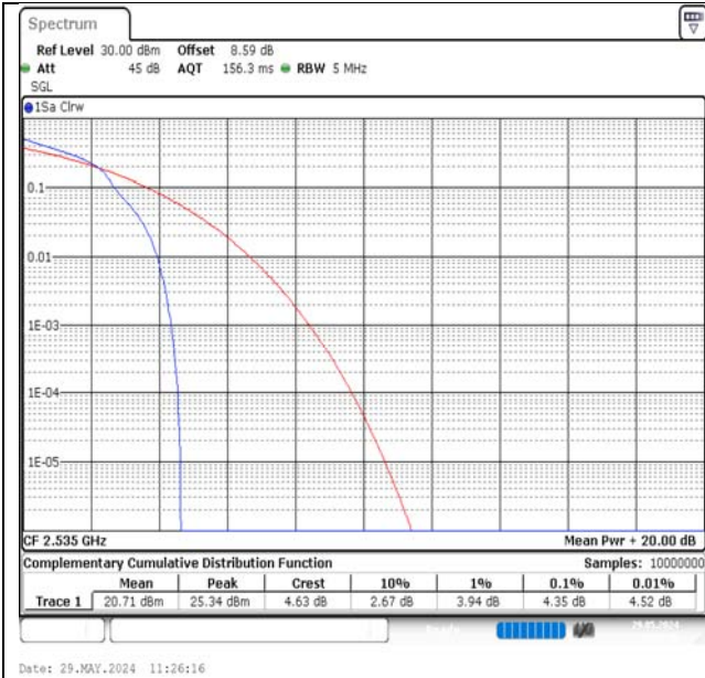
Band7-5MHz-16QAM-21100-1RB#0-PASS
