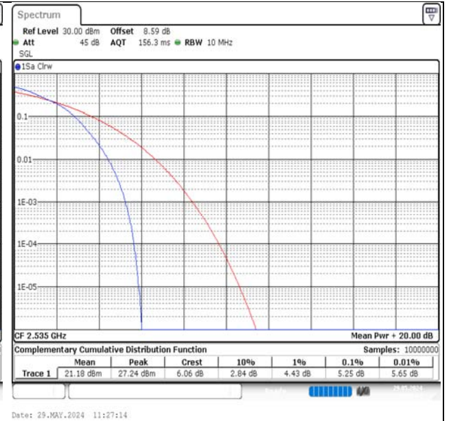
Band7-10MHz-16QAM-21100-50RB#0-PASS
