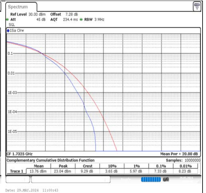
Band4-20MHz-16QAM-20175-100RB#0-PASS
