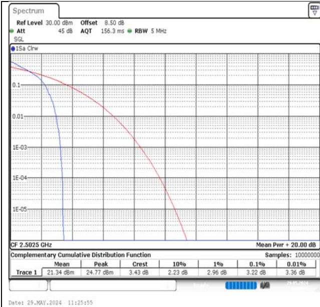
Band7-5MHz-QPSK-20775-1RB#0-PASS
