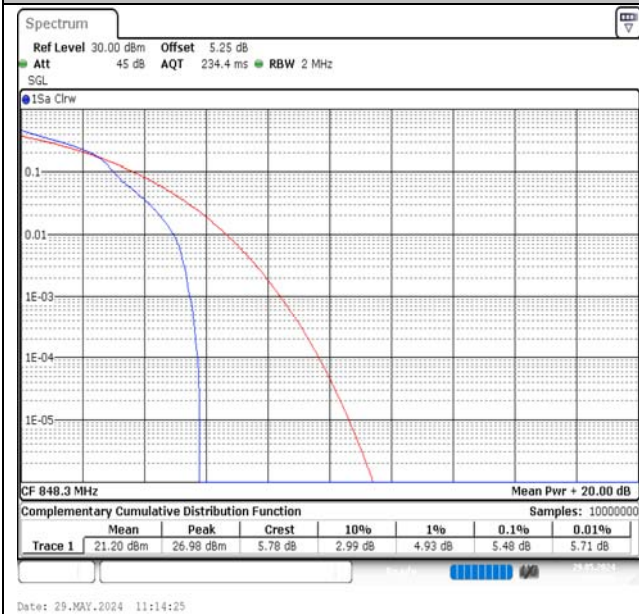
Band5-1.4MHz-16QAM-20643-1RB#0-PASS
