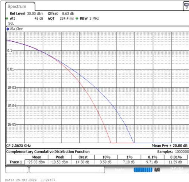
Band7-15MHz-QPSK-21375-1RB#0-PASS
