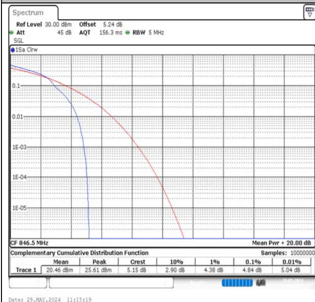
Band5-5MHz-16QAM-20625-1RB#0-PASS
