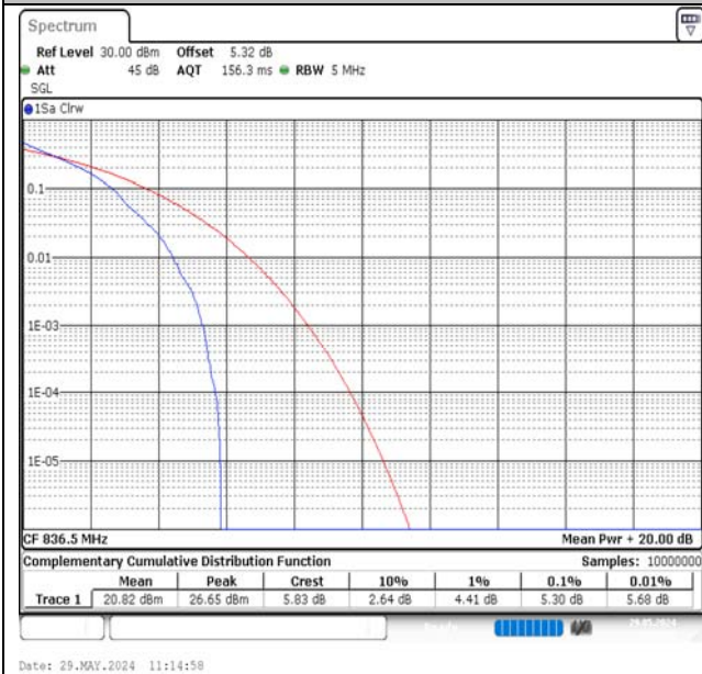
Band5-5MHz-QPSK-20525-1RB#0-PASS
