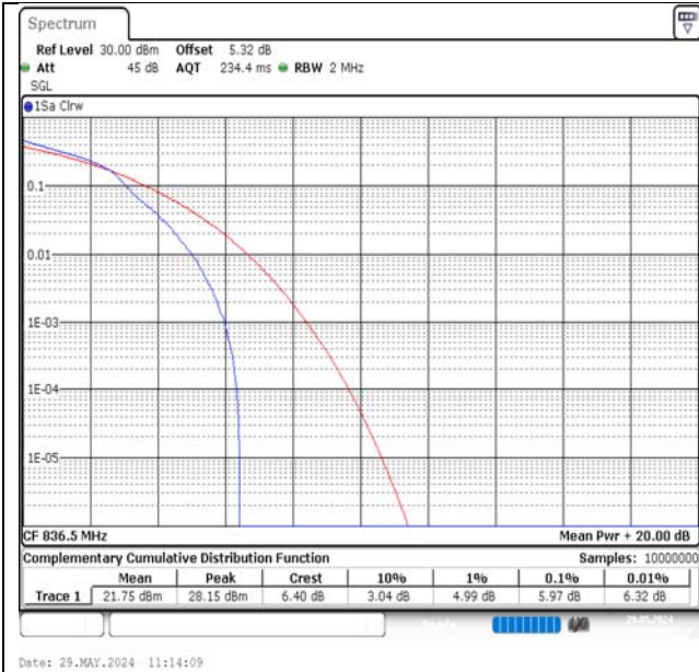
Band5-1.4MHz-16QAM-20525-1RB#0-PASS
