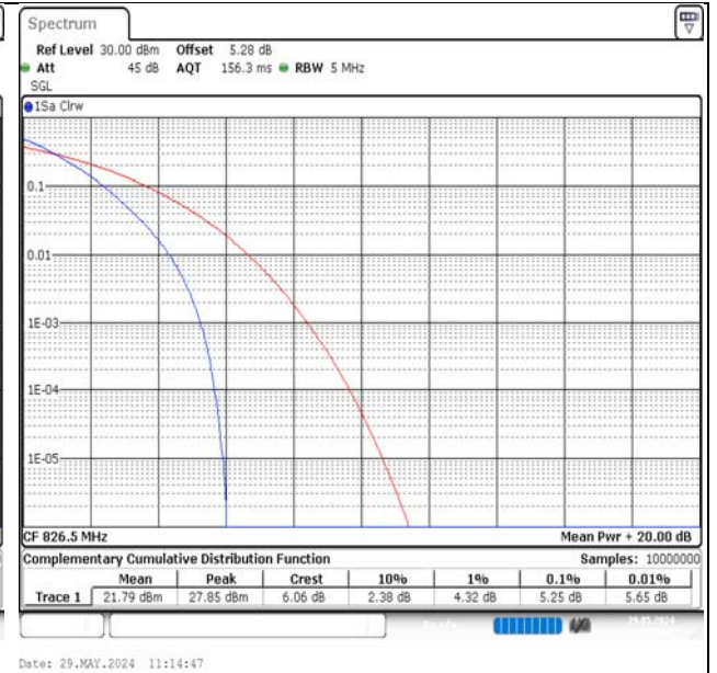
Band5-5MHz-QPSK-20425-25RB#0-PASS
