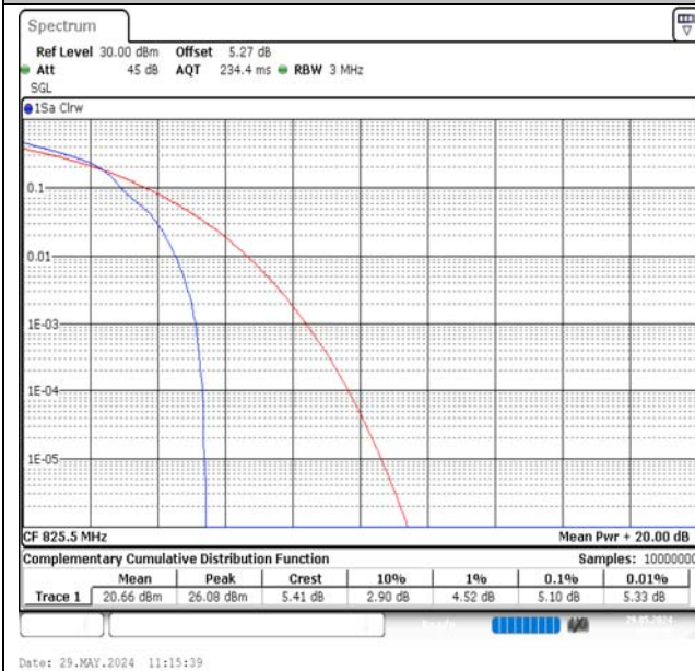
Band5-3MHz-16QAM-20415-1RB#0-PASS
