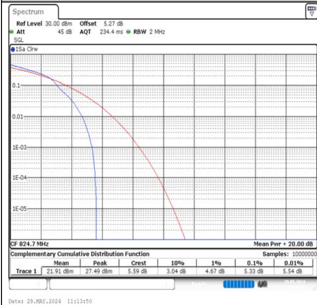
Band5-1.4MHz-16QAM-20407-1RB#0-PASS
