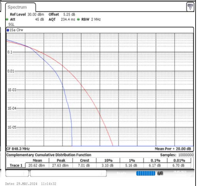
Band5-1.4MHz-16QAM-20643-6RB#0-PASS
