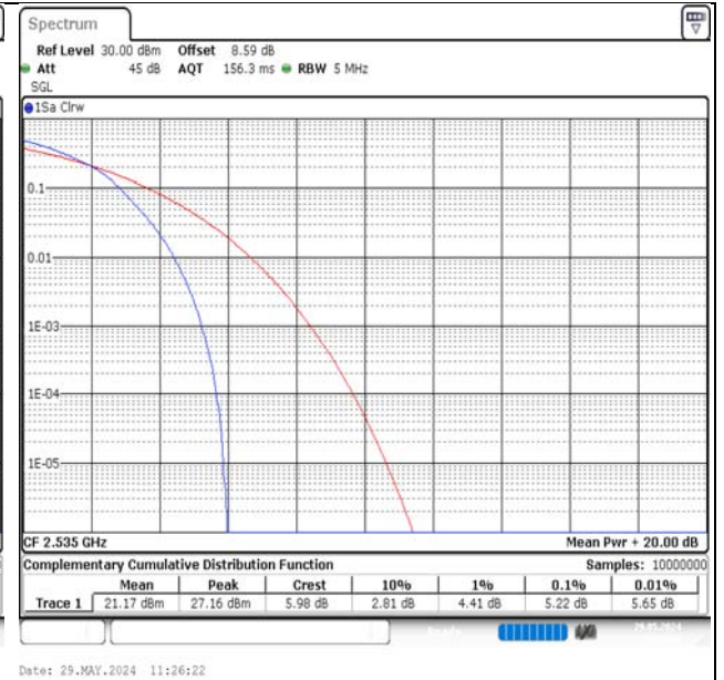
Band7-5MHz-16QAM-21100-25RB#0-PASS
