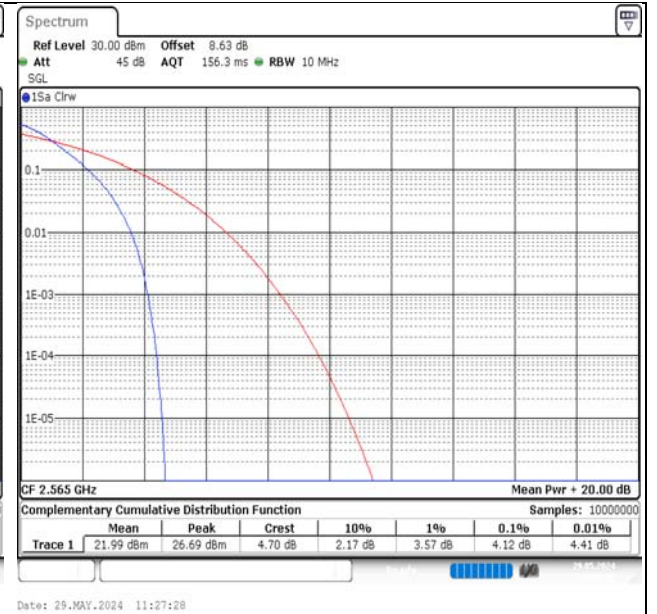
Band7-10MHz-QPSK-21400-50RB#0-PASS
