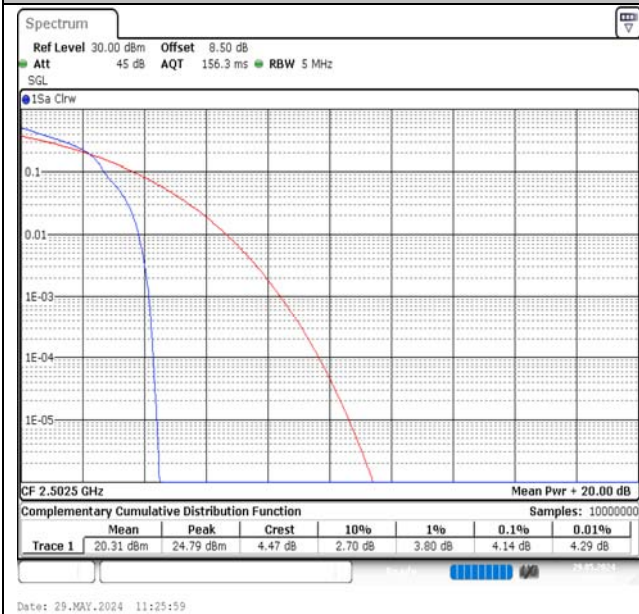
Band7-5MHz-16QAM-20775-1RB#0-PASS
