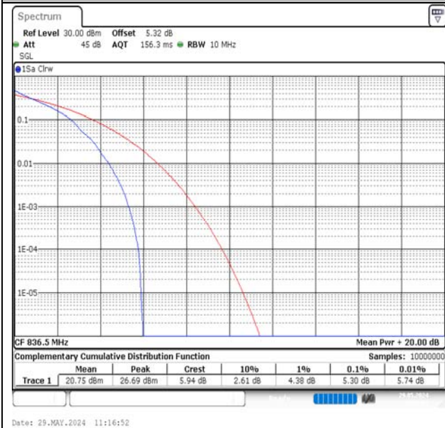
Band5-10MHz-QPSK-20525-1RB#0-PASS
