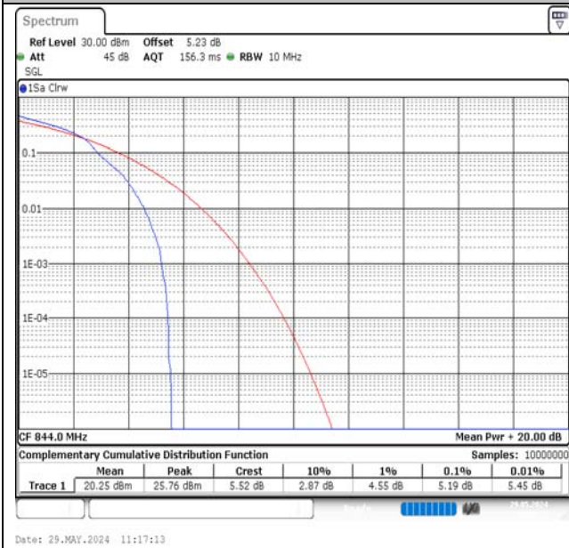
Band5-10MHz-16QAM-20600-1RB#0-PASS
