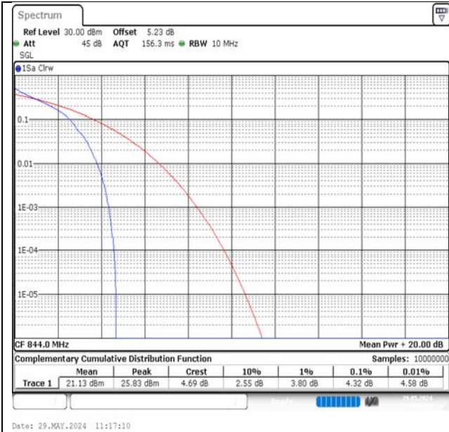
Band5-10MHz-QPSK-20600-1RB#0-PASS
