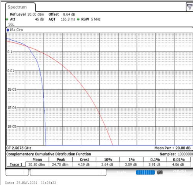
Band7-5MHz-16QAM-21425-1RB#0-PASS
