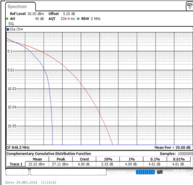
Band5-1.4MHz-QPSK-20643-1RB#0-PASS
