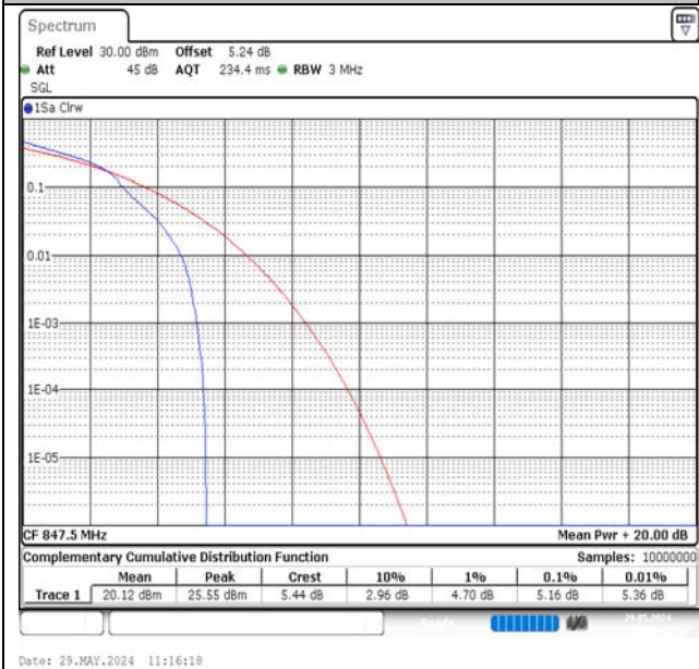
Band5-3MHz-16QAM-20635-1RB#0-PASS
