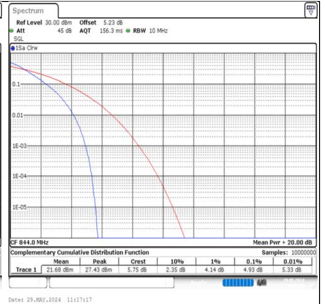
Band5-10MHz-QPSK-20600-50RB#0-PASS
