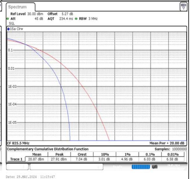
Band5-3MHz-16QAM-20415-15RB#0-PASS
