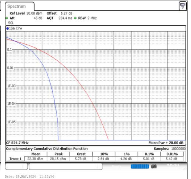
Band5-1.4MHz-QPSK-20407-6RB#0-PASS
