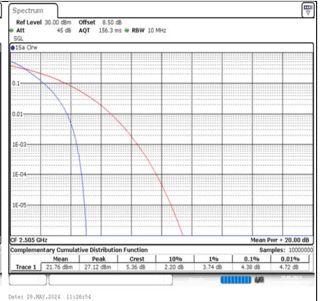
Band7-10MHz-QPSK-20800-50RB#0-PASS
