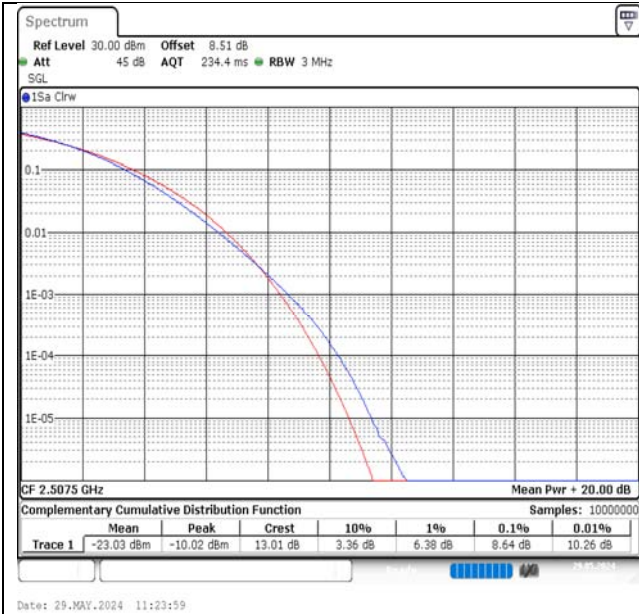
Band7-15MHz-QPSK-20825-1RB#0-PASS
