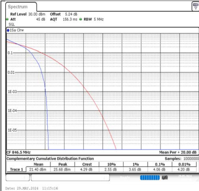
Band5-5MHz-QPSK-20625-1RB#0-PASS
