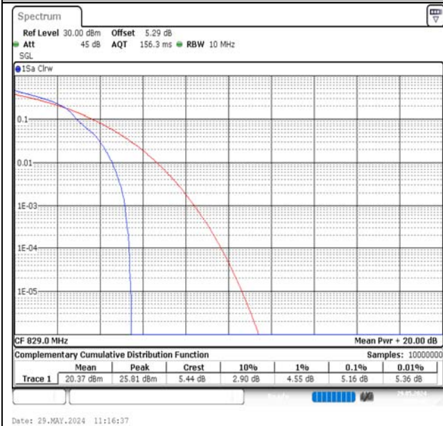
Band5-10MHz-16QAM-20450-1RB#0-PASS
