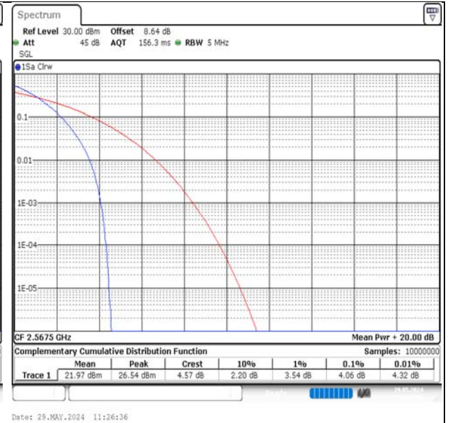
Band7-5MHz-QPSK-21425-25RB#0-PASS
