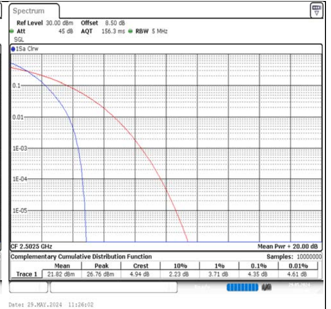
Band7-5MHz-QPSK-20775-25RB#0-PASS
