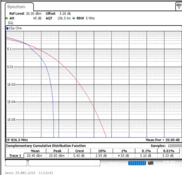
Band5-5MHz-16QAM-20425-1RB#0-PASS
