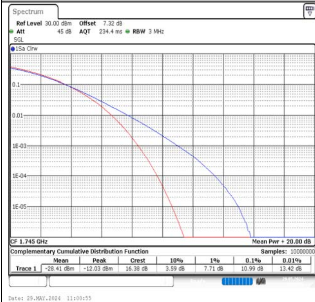
Band4-20MHz-16QAM-20300-1RB#0-PASS
