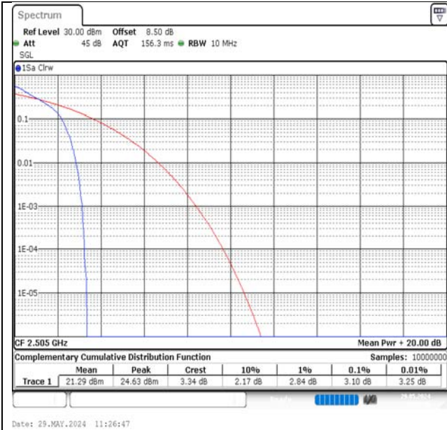
Band7-10MHz-QPSK-20800-1RB#0-PASS
