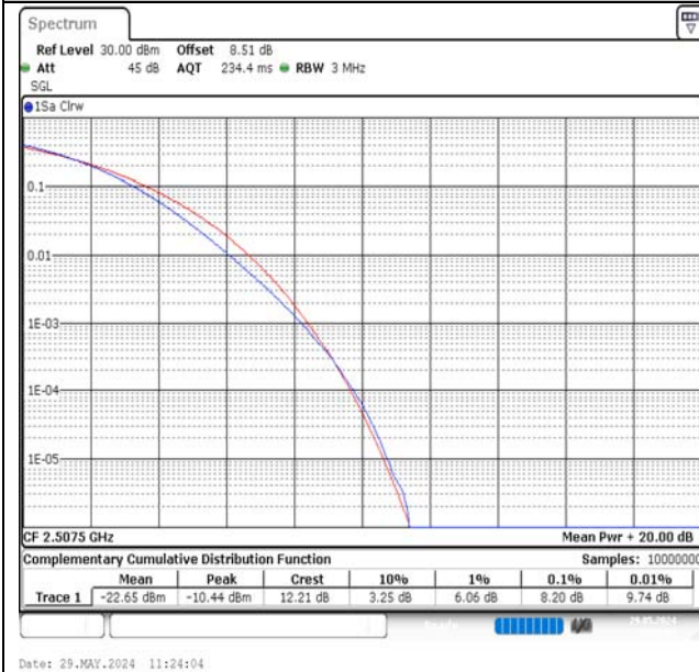
Band7-15MHz-16QAM-20825-1RB#0-PASS
