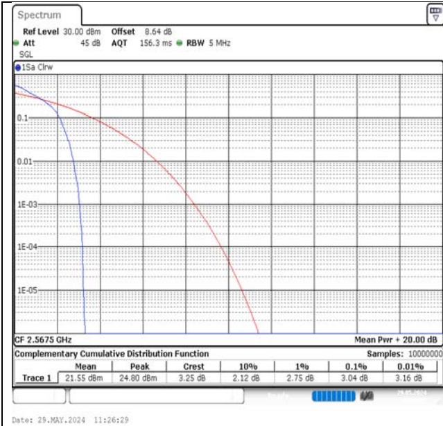
Band7-5MHz-QPSK-21425-1RB#0-PASS
