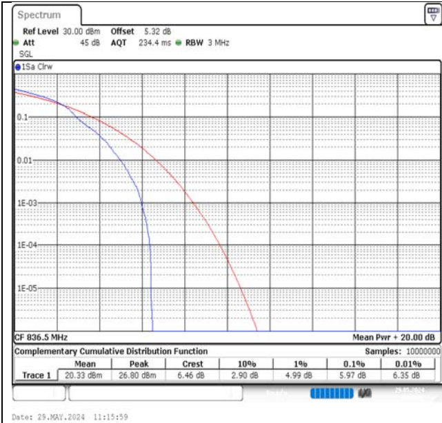
Band5-3MHz-16QAM-20525-1RB#0-PASS
