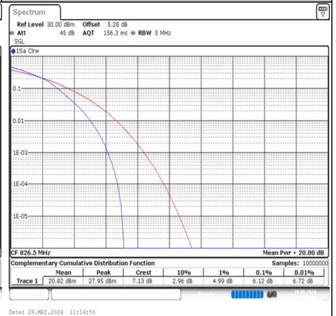
Band5-5MHz-16QAM-20425-25RB#0-PASS
