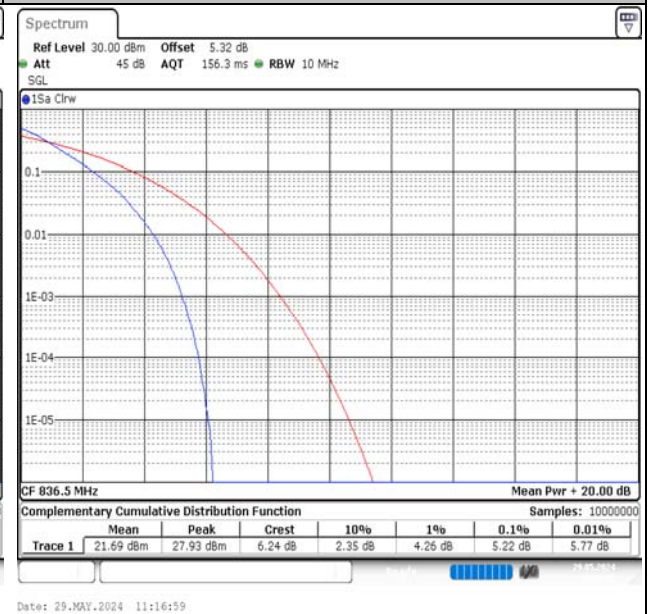
Band5-10MHz-QPSK-20525-50RB#0-PASS
