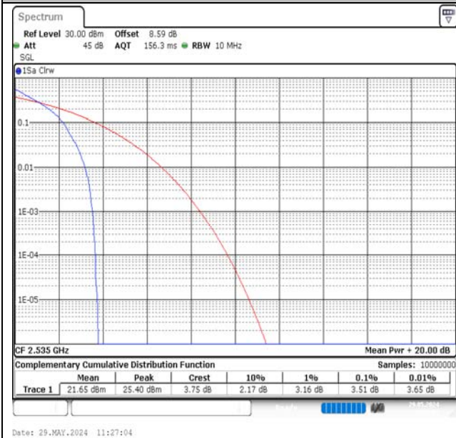
Band7-10MHz-QPSK-21100-1RB#0-PASS
