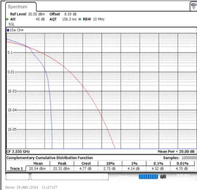
Band7-10MHz-16QAM-21100-1RB#0-PASS
