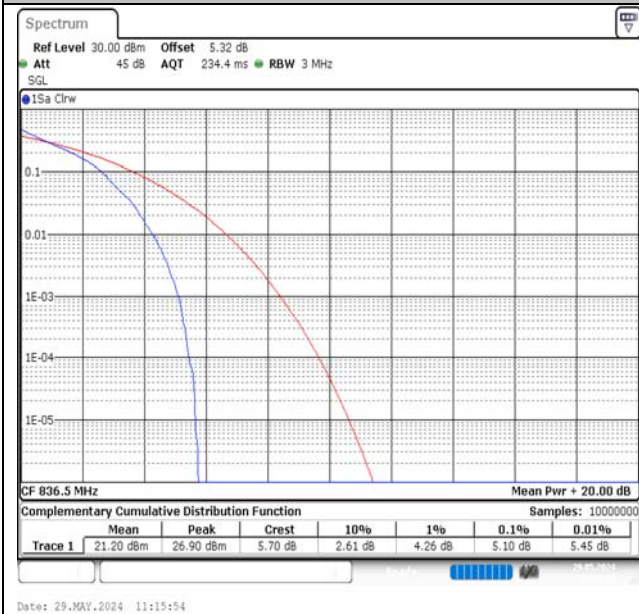
Band5-3MHz-QPSK-20525-1RB#0-PASS
