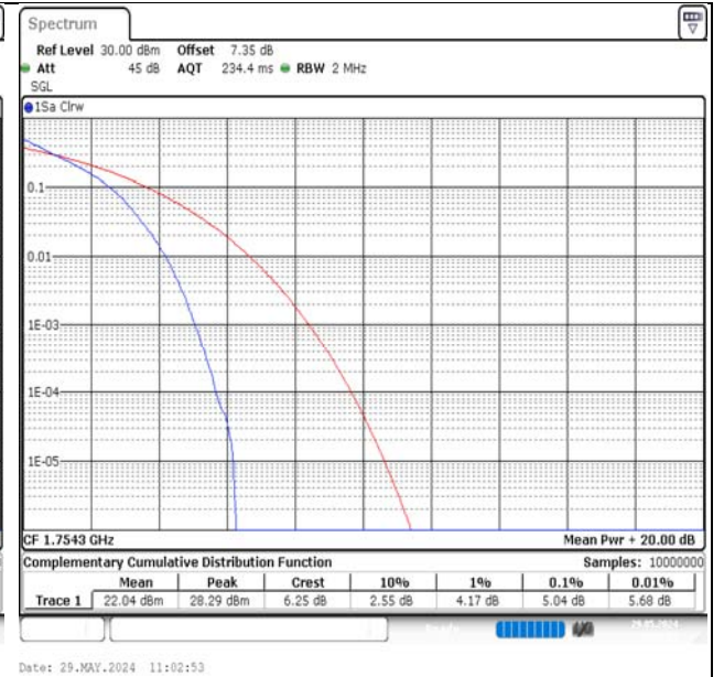
Band4-1.4MHz-QPSK-20393-6RB#0-PASS
