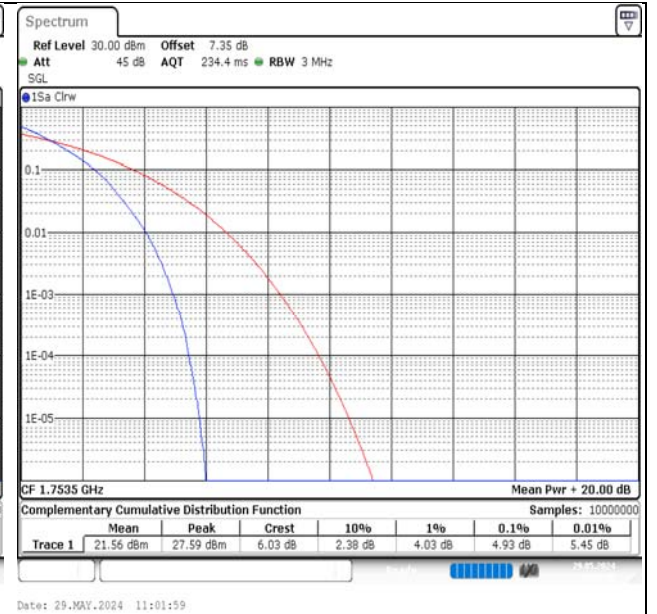
Band4-3MHz-QPSK-20385-15RB#0-PASS
