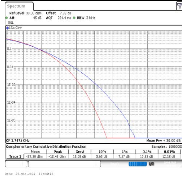
Band4-15MHz-16QAM-20325-1RB#0-PASS
