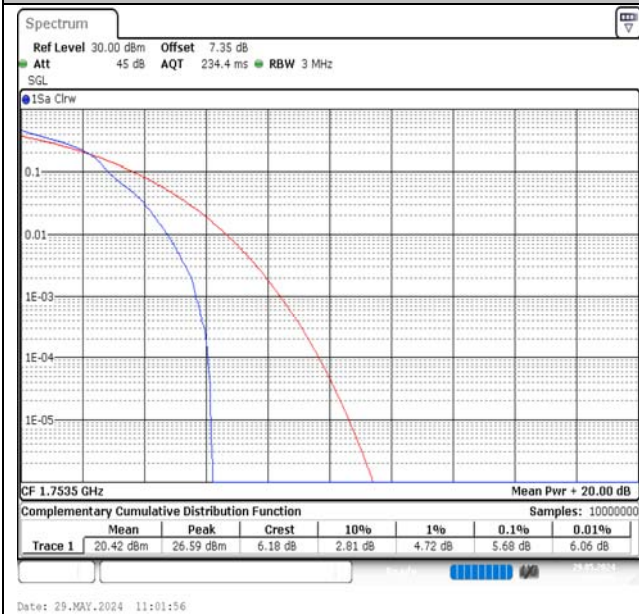
Band4-3MHz-16QAM-20385-1RB#0-PASS
