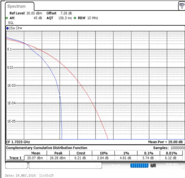
Band4-10MHz-16QAM-20175-1RB#0-PASS
