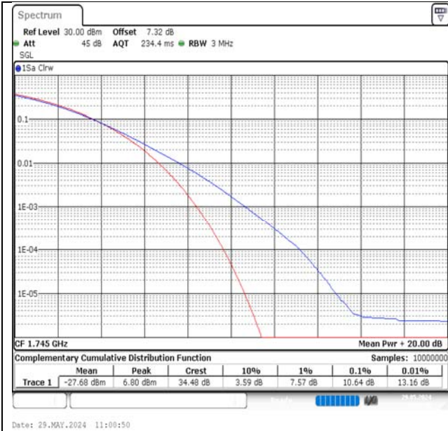
Band4-20MHz-QPSK-20300-1RB#0-PASS
