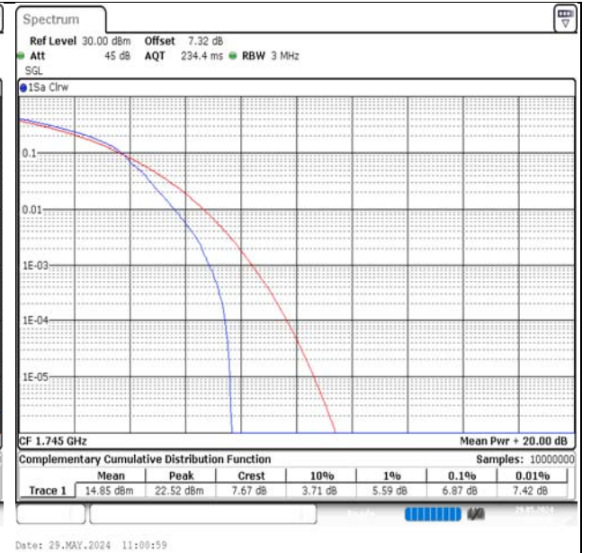
Band4-20MHz-QPSK-20300-100RB#0-PASS
