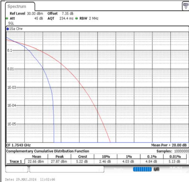
Band4-1.4MHz-QPSK-20393-1RB#0-PASS
