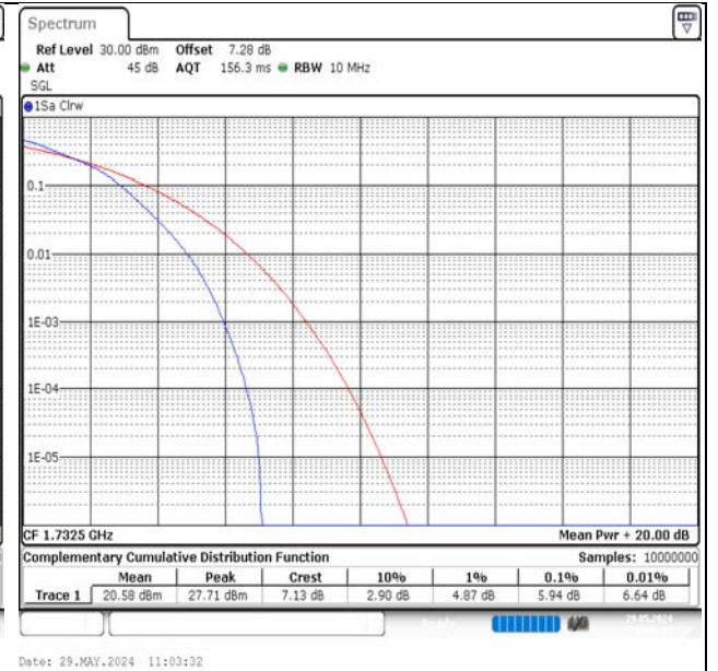
Band4-10MHz-16QAM-20175-50RB#0-PASS
