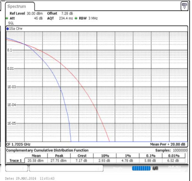
Band4-3MHz-16QAM-20175-15RB#0-PASS
