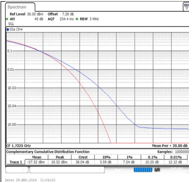
Band4-15MHz-16QAM-20175-1RB#0-PASS
