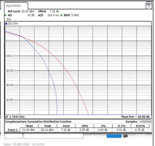
Band4-1.4MHz-16QAM-20393-6RB#0-PASS
