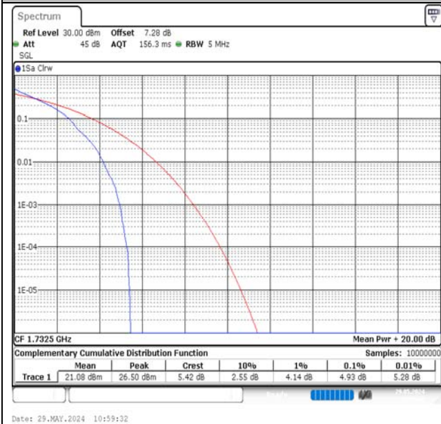
Band4-5MHz-QPSK-20175-1RB#0-PASS
