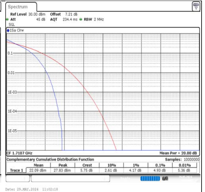
Band4-1.4MHz-QPSK-19957-6RB#0-PASS
