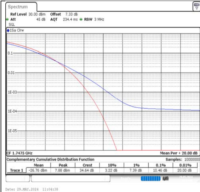
Band4-15MHz-QPSK-20325-1RB#0-PASS
