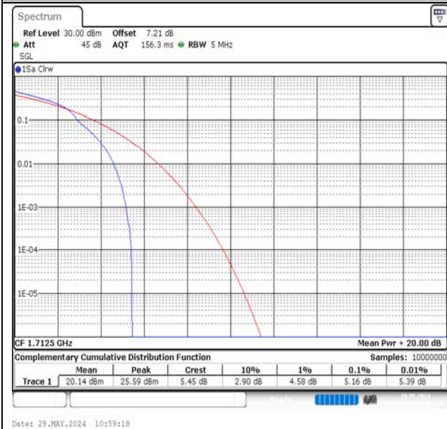
Band4-5MHz-16QAM-19975-1RB#0-PASS
