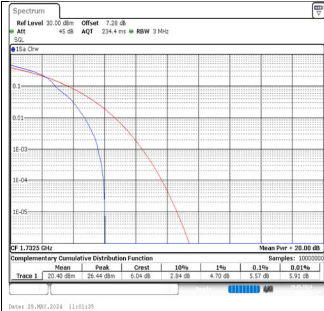
Band4-3MHz-16QAM-20175-1RB#0-PASS
