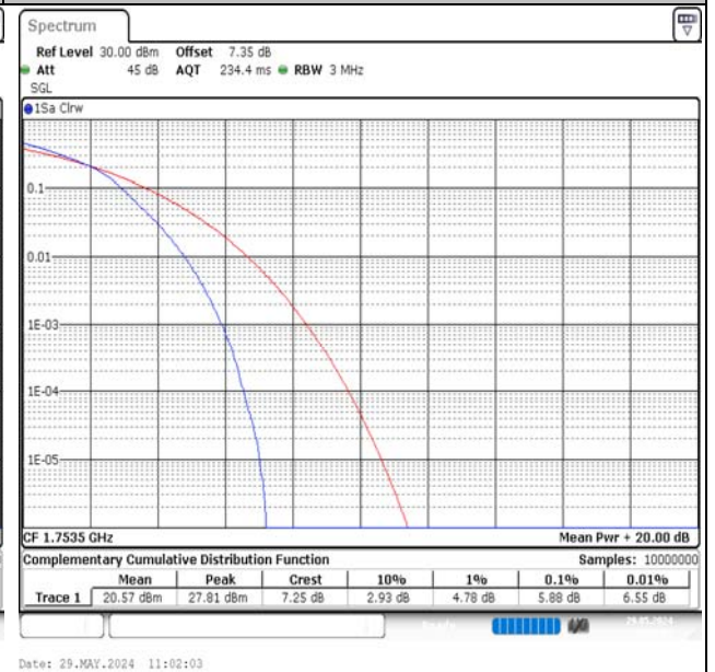
Band4-3MHz-16QAM-20385-15RB#0-PASS
