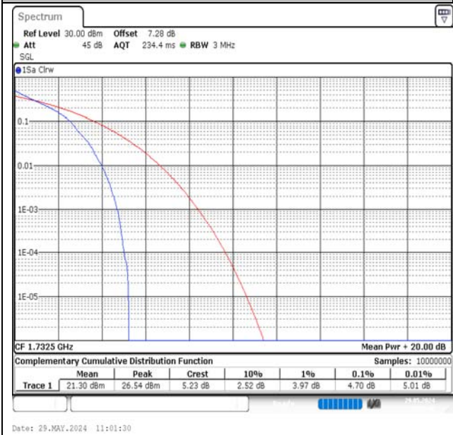
Band4-3MHz-QPSK-20175-1RB#0-PASS
