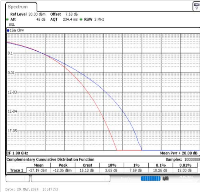
Band2-15MHz-16QAM-18900-1RB#0-PASS
