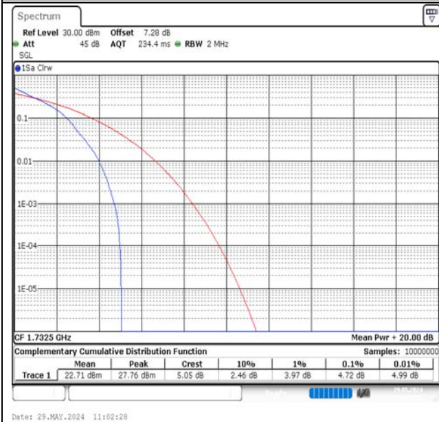
Band4-1.4MHz-QPSK-20175-1RB#0-PASS
