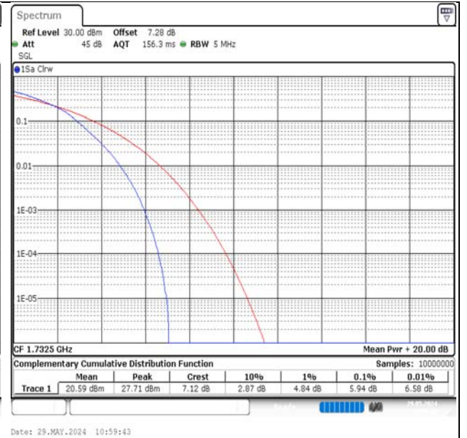
Band4-5MHz-16QAM-20175-25RB#0-PASS
