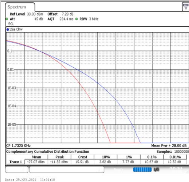
Band4-15MHz-QPSK-20175-1RB#0-PASS
