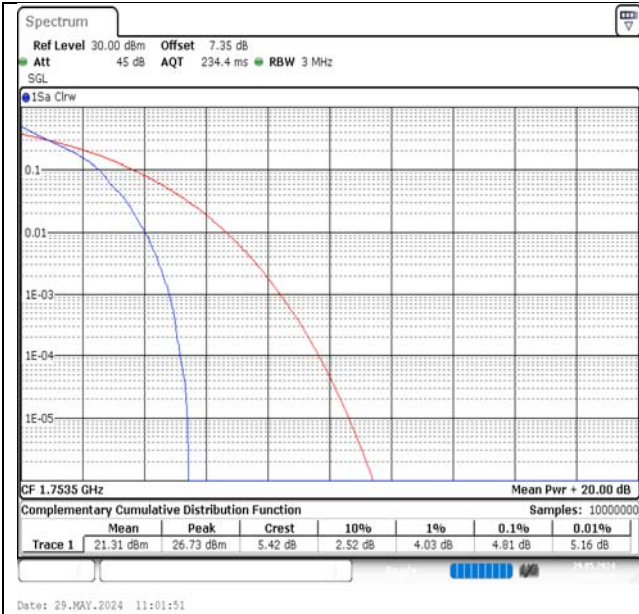
Band4-3MHz-QPSK-20385-1RB#0-PASS
