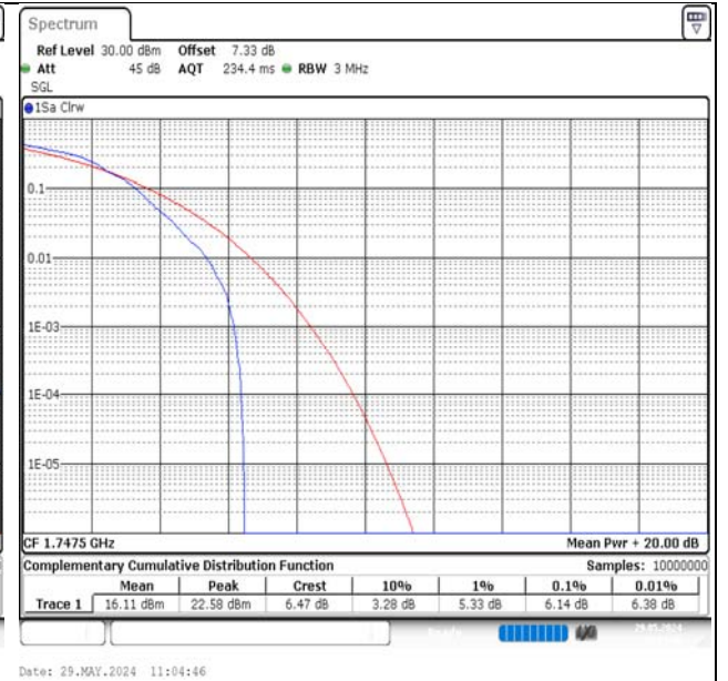
Band4-15MHz-QPSK-20325-75RB#0-PASS
