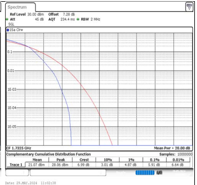
Band4-1.4MHz-16QAM-20175-6RB#0-PASS
