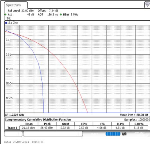
Band4-5MHz-QPSK-20375-1RB#0-PASS
