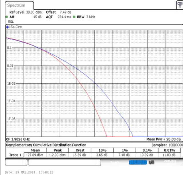
Band2-15MHz-16QAM-19125-1RB#0-PASS
