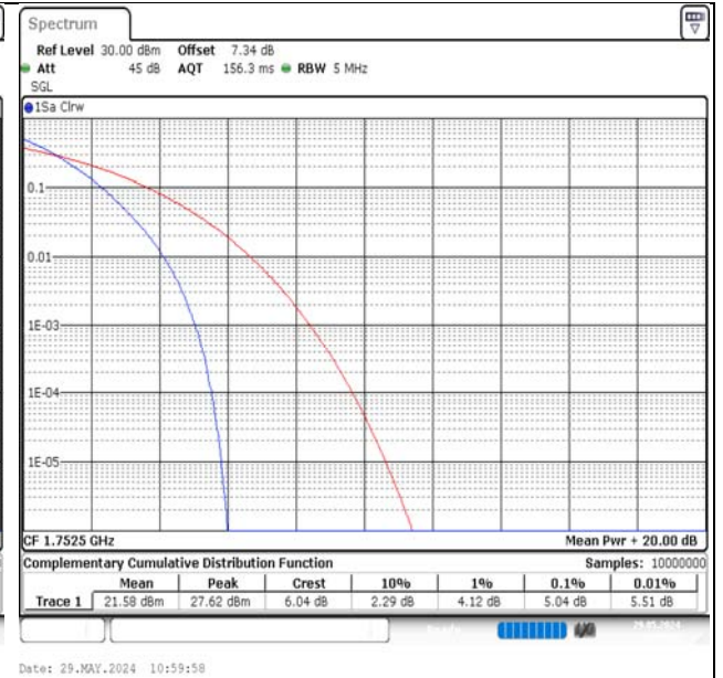
Band4-5MHz-QPSK-20375-25RB#0-PASS
