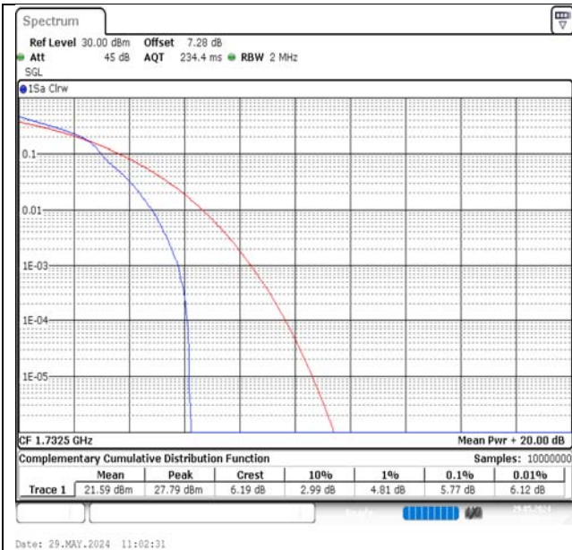
Band4-1.4MHz-16QAM-20175-1RB#0-PASS
