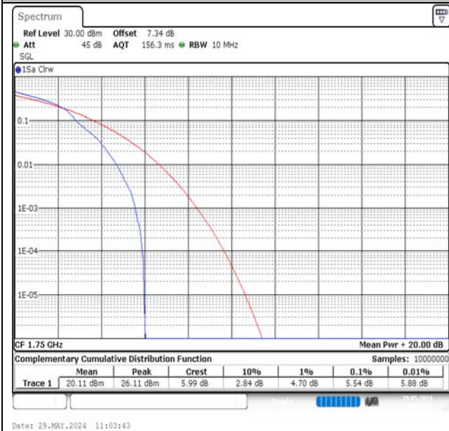
Band4-10MHz-16QAM-20350-1RB#0-PASS
