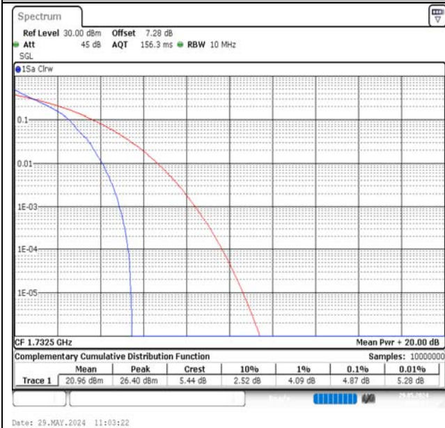
Band4-10MHz-QPSK-20175-1RB#0-PASS
