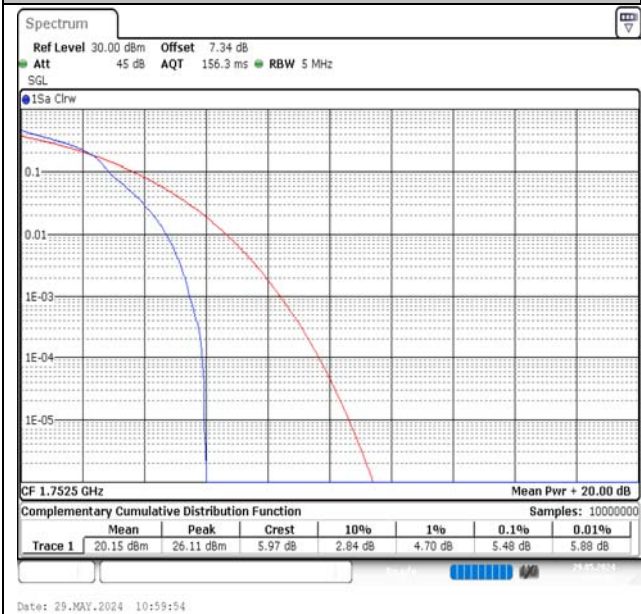
Band4-5MHz-16QAM-20375-1RB#0-PASS
