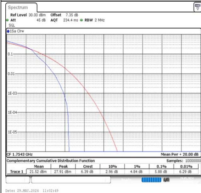
Band4-1.4MHz-16QAM-20393-1RB#0-PASS
