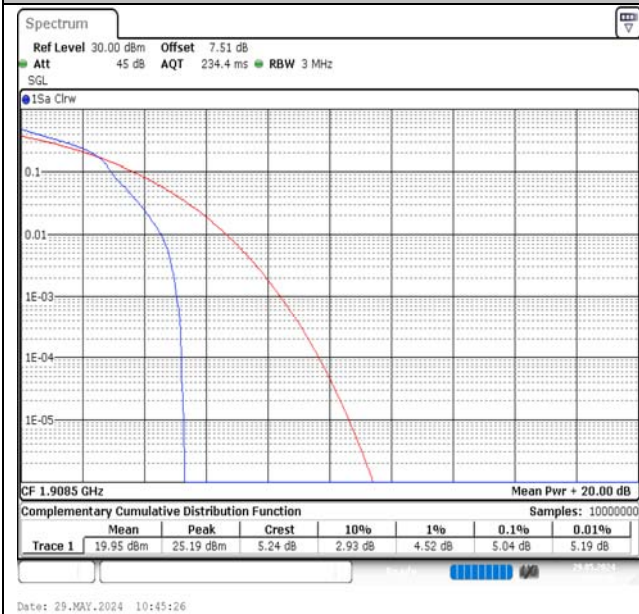
Band2-3MHz-16QAM-19185-1RB#0-PASS
