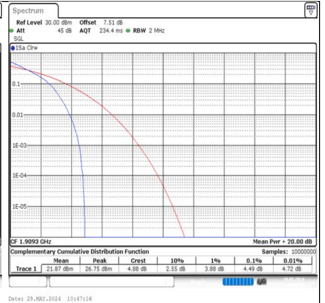
Band2-1.4MHz-QPSK-19193-6RB#0-PASS
