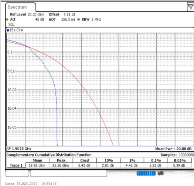
Band2-5MHz-16QAM-19175-1RB#0-PASS
