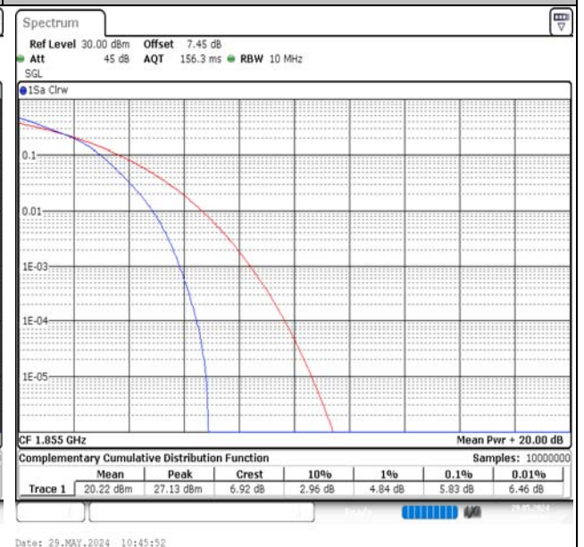
Band2-10MHz-16QAM-18650-50RB#0-PASS
