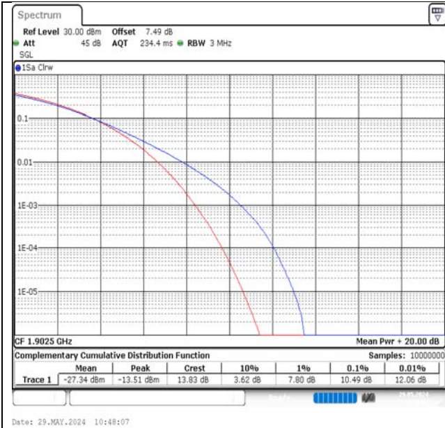
Band2-15MHz-QPSK-19125-1RB#0-PASS
