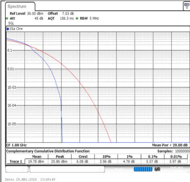
Band2-5MHz-16QAM-18900-1RB#0-PASS
