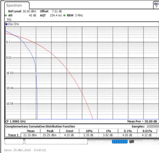
Band2-3MHz-QPSK-19185-1RB#0-PASS
