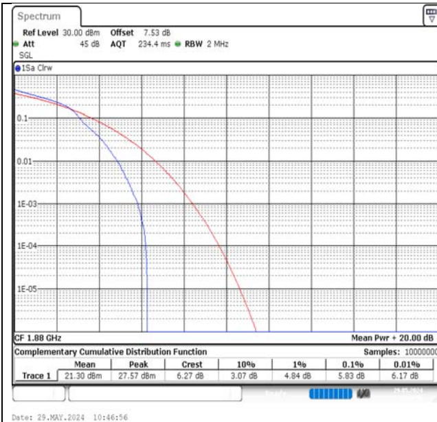
Band2-1.4MHz-16QAM-18900-1RB#0-PASS
