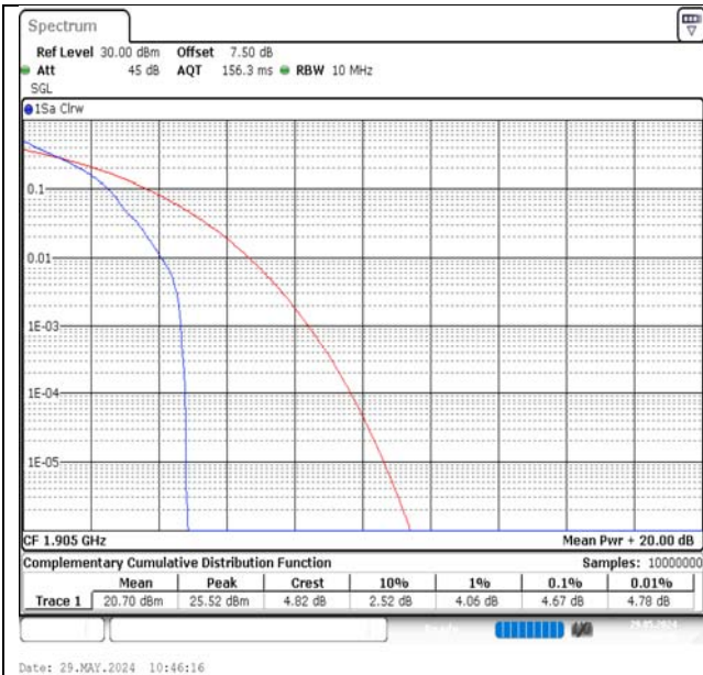
Band2-10MHz-QPSK-19150-1RB#0-PASS
