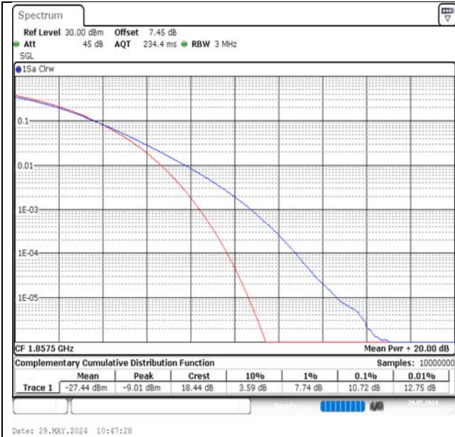
Band2-15MHz-QPSK-18675-1RB#0-PASS
