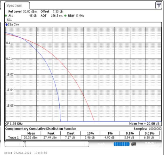
Band2-5MHz-16QAM-18900-25RB#0-PASS
