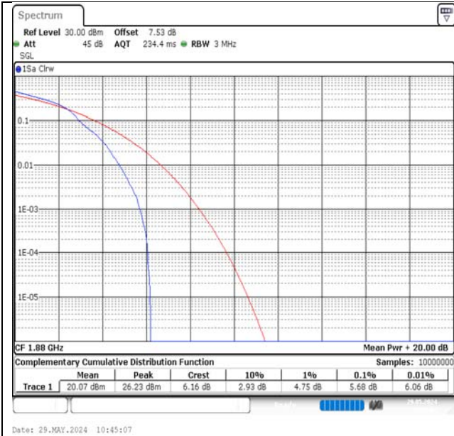
Band2-3MHz-16QAM-18900-1RB#0-PASS
