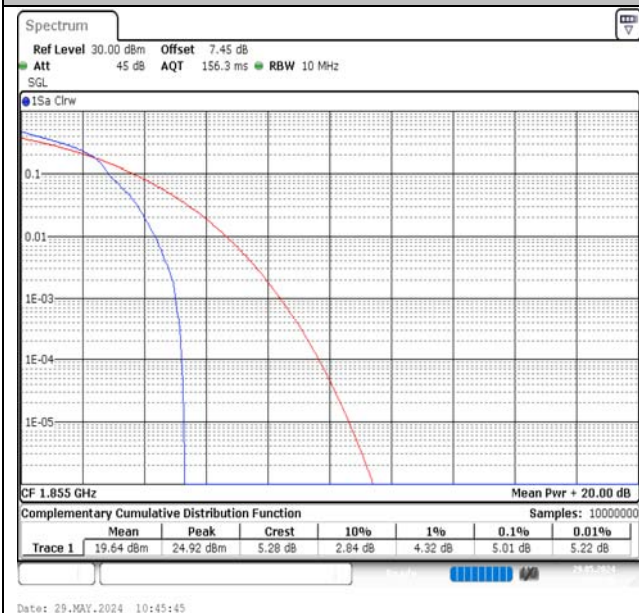
Band2-10MHz-16QAM-18650-1RB#0-PASS
