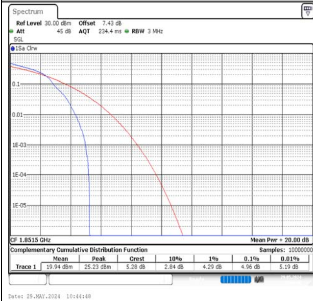
Band2-3MHz-16QAM-18615-1RB#0-PASS
