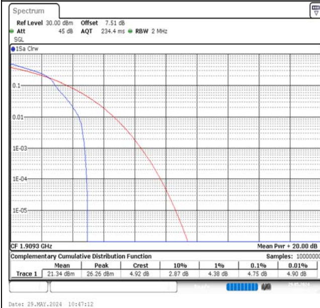
Band2-1.4MHz-16QAM-19193-1RB#0-PASS
