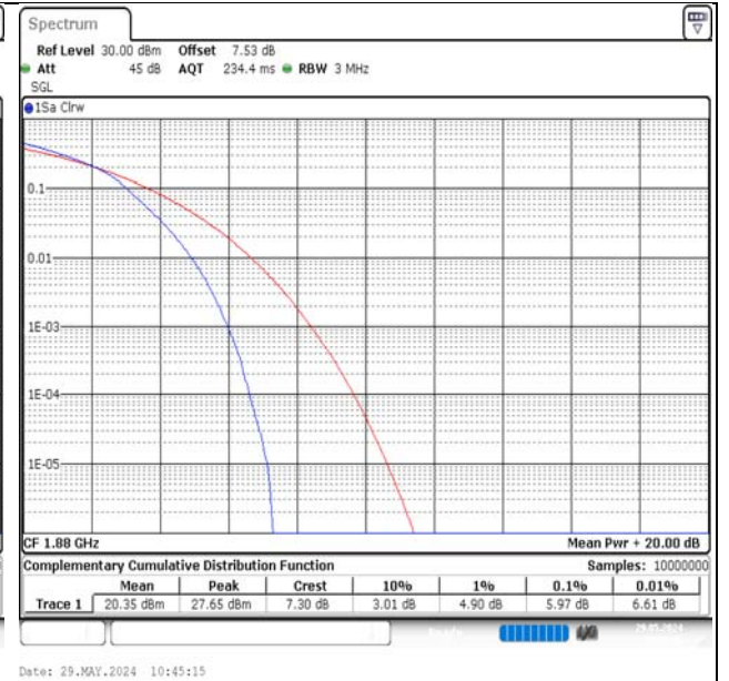
Band2-3MHz-16QAM-18900-15RB#0-PASS
