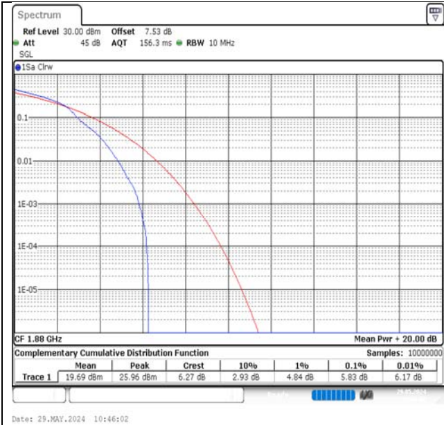
Band2-10MHz-16QAM-18900-1RB#0-PASS
