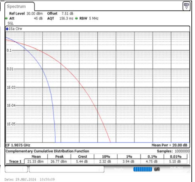
Band2-5MHz-QPSK-19175-25RB#0-PASS
